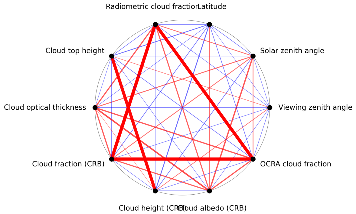
Figure 1: Map of correlation graph for 2025-03-25 to 2025-03-27.
