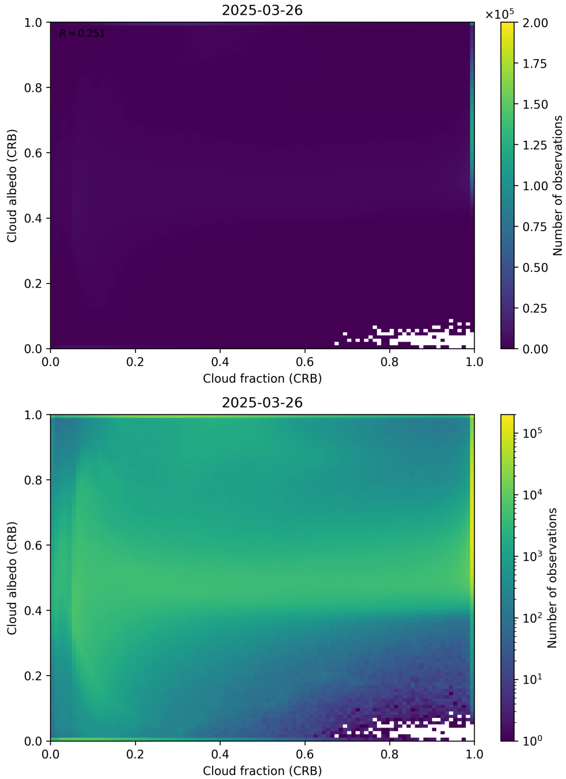
Figure 77: Scatter density plot of “Cloud fraction (CRB)” against “Cloud albedo (CRB)” for 2025-03-25 to 2025-03-27.
