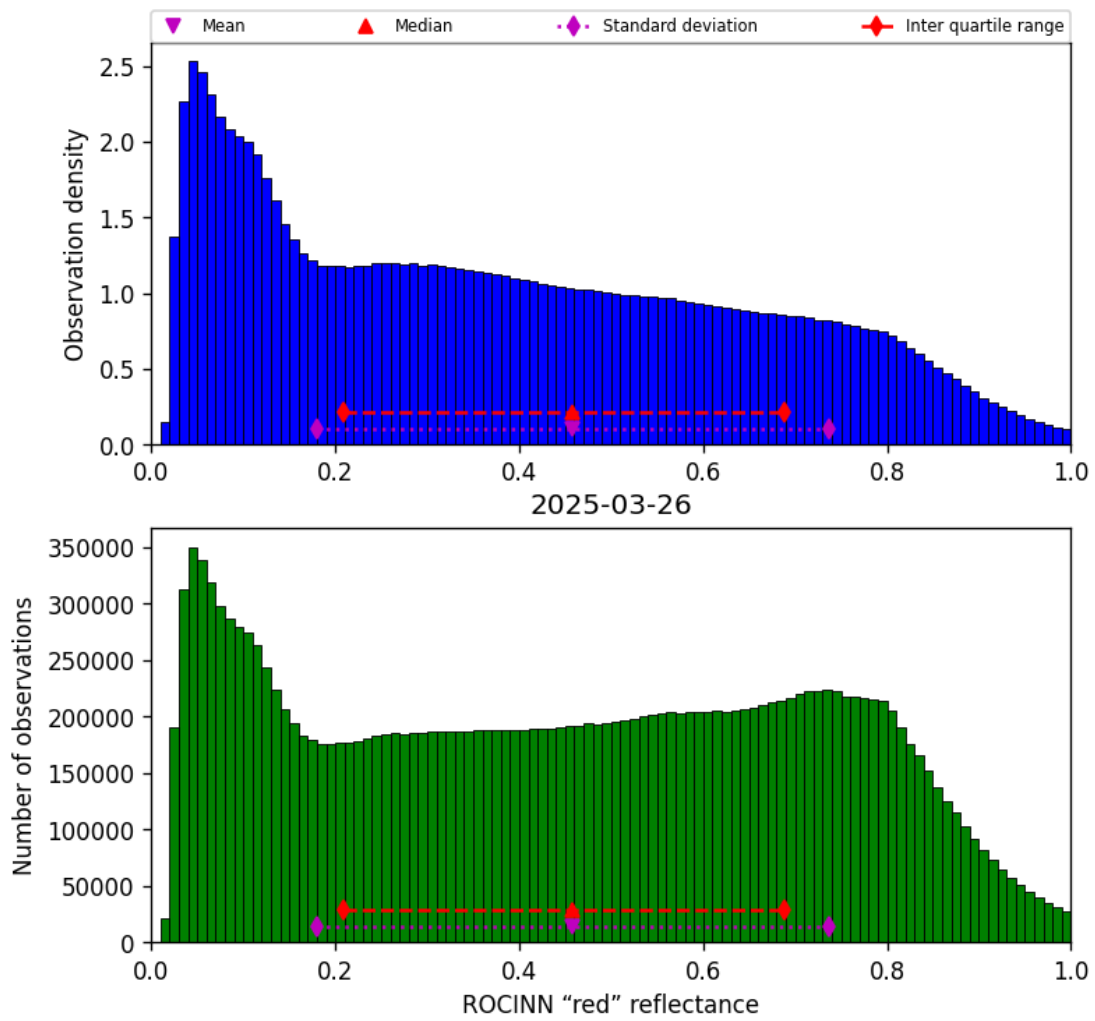
Figure 53: Histogram of “ROCINN “red” reflectance” for 2025-03-25 to 2025-03-27
