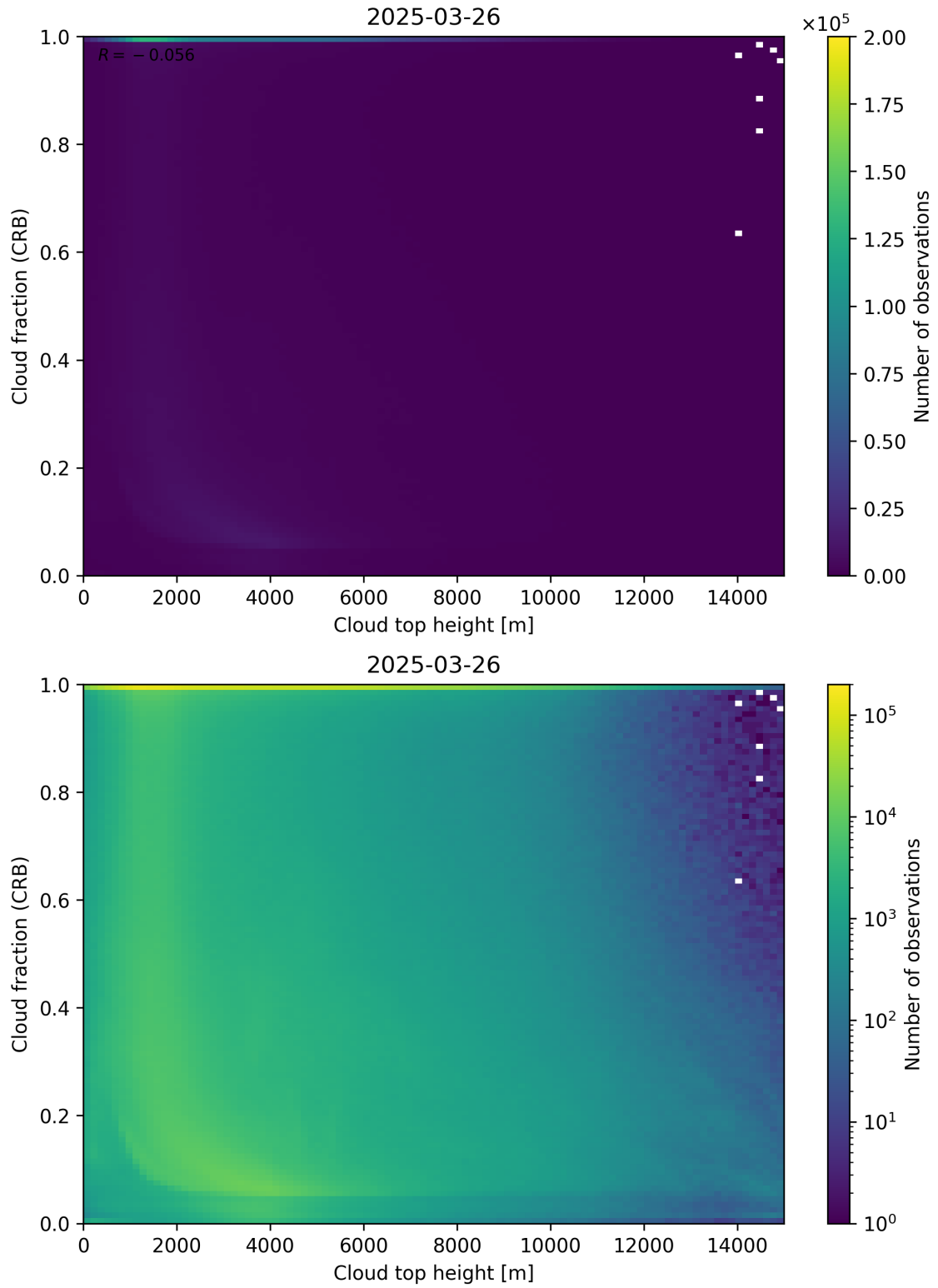
Figure 88: Scatter density plot of “Cloud top height” against “Cloud fraction (CRB)” for 2025-03-25 to 2025-03-27.
