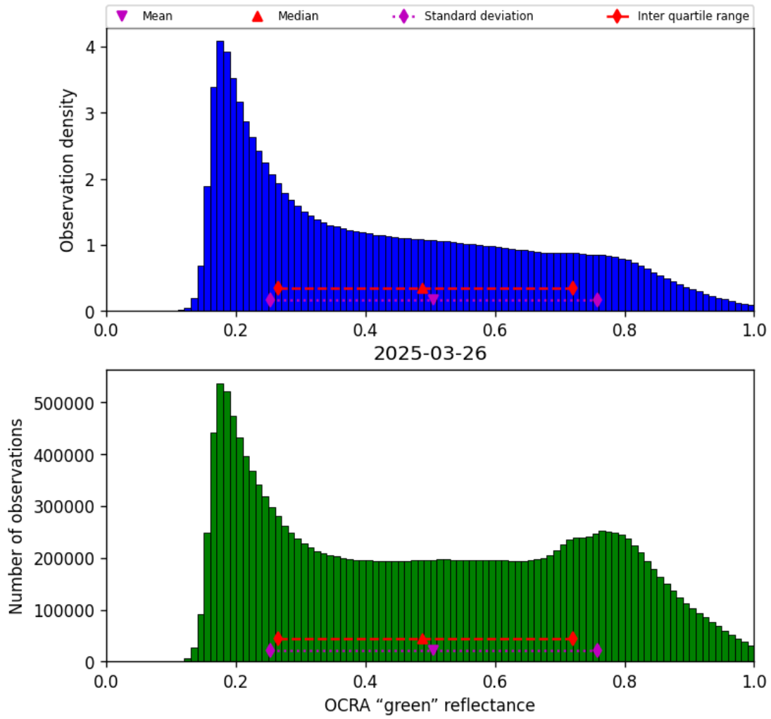
Figure 52: Histogram of “OCRA “green” reflectance” for 2025-03-25 to 2025-03-27
