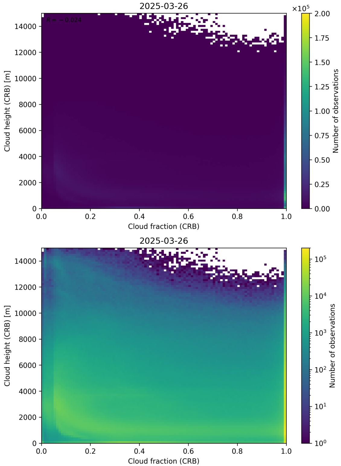
Figure 79: Scatter density plot of “Cloud fraction (CRB)” against “Cloud height (CRB)” for 2025-03-25 to 2025-03-27.
