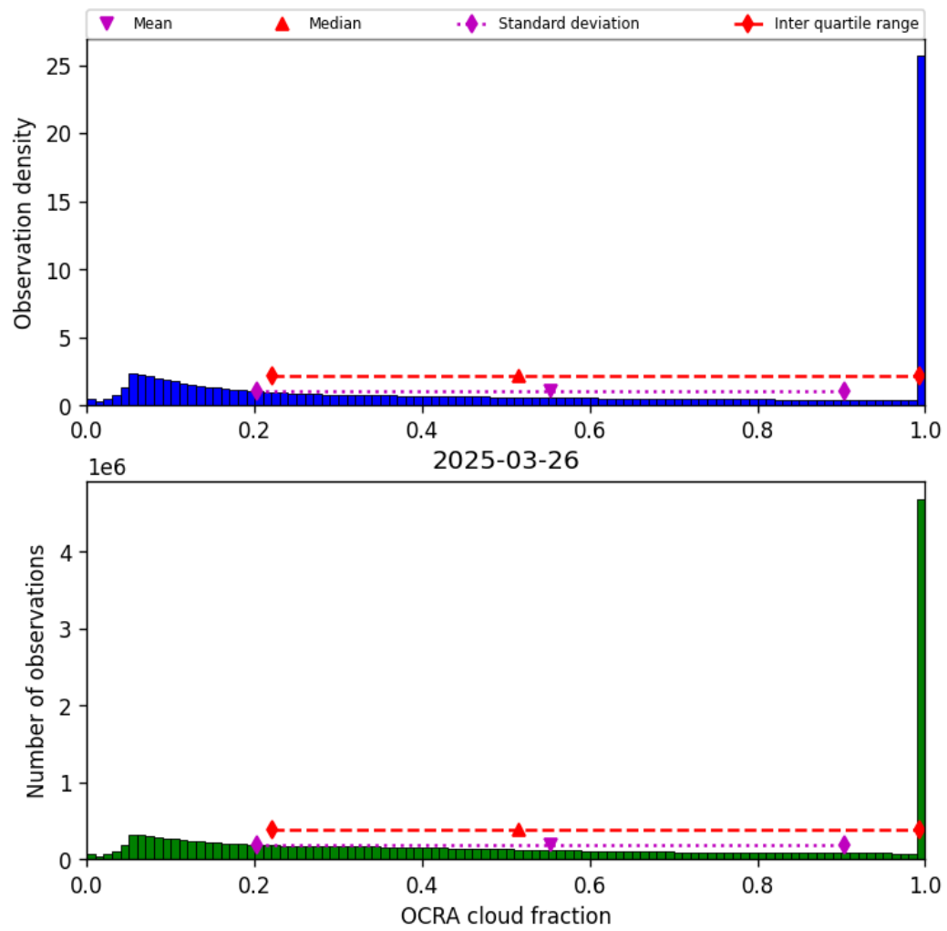
Figure 50: Histogram of “OCRA cloud fraction” for 2025-03-25 to 2025-03-27
