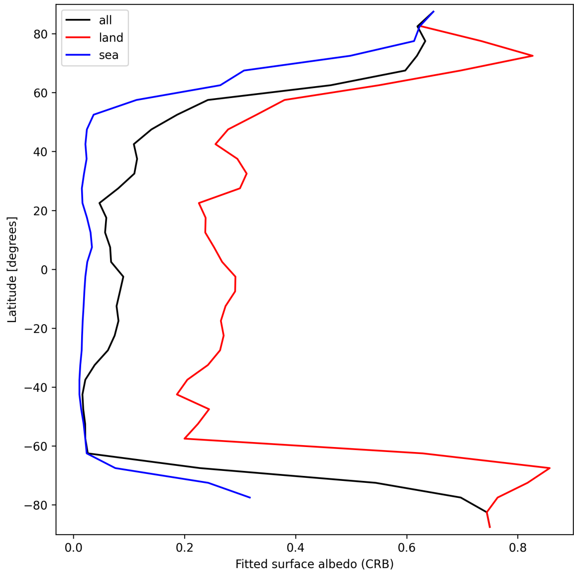
Figure 30: Zonal average of “Fitted surface albedo (CRB)” for 2025-03-25 to 2025-03-27.
