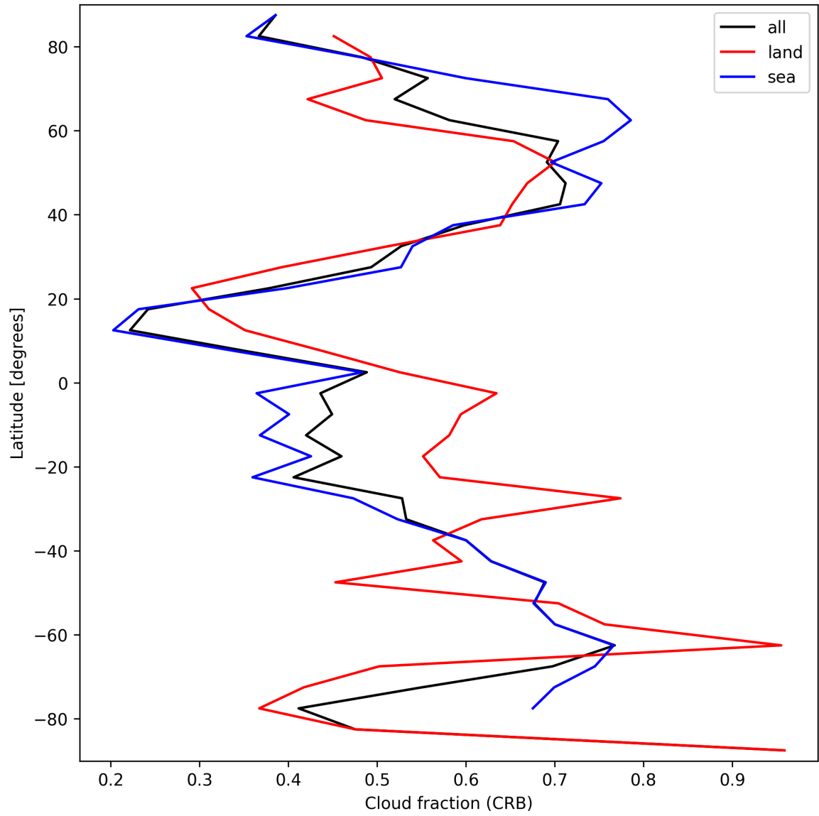
Figure 26: Zonal average of “Cloud fraction (CRB)” for 2025-03-25 to 2025-03-27.
