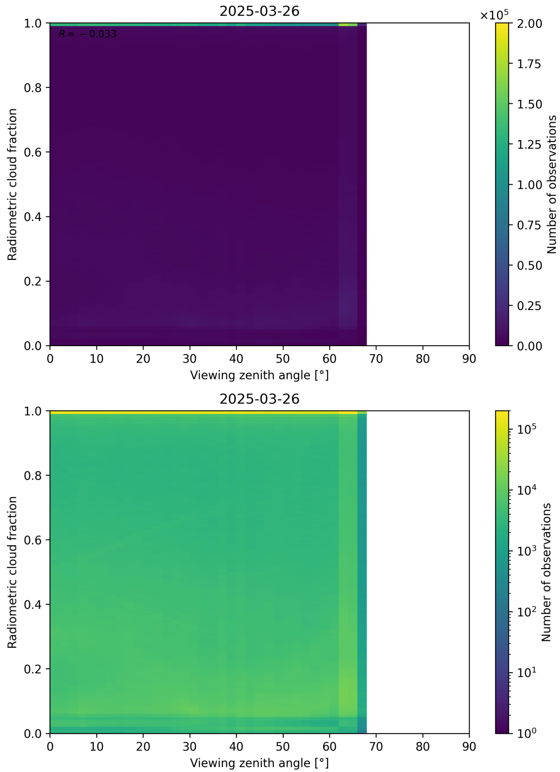
Figure 107: Scatter density plot of “Viewing zenith angle” against “Radiometric cloud fraction” for 2025-03-25 to 2025-03-27.
