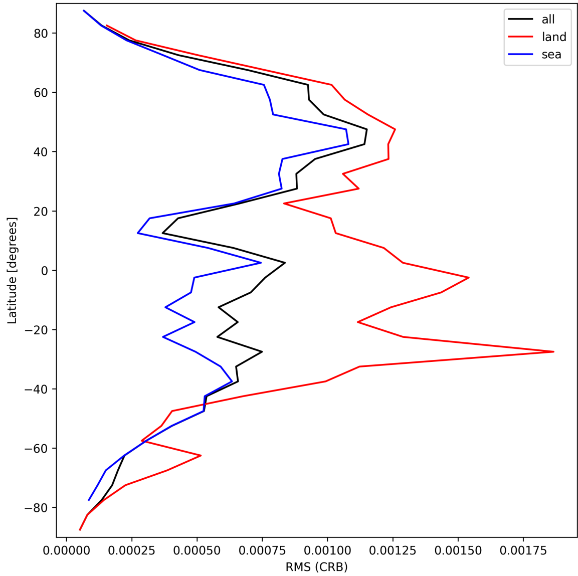
Figure 32: Zonal average of “RMS (CRB)” for 2025-03-25 to 2025-03-27.
