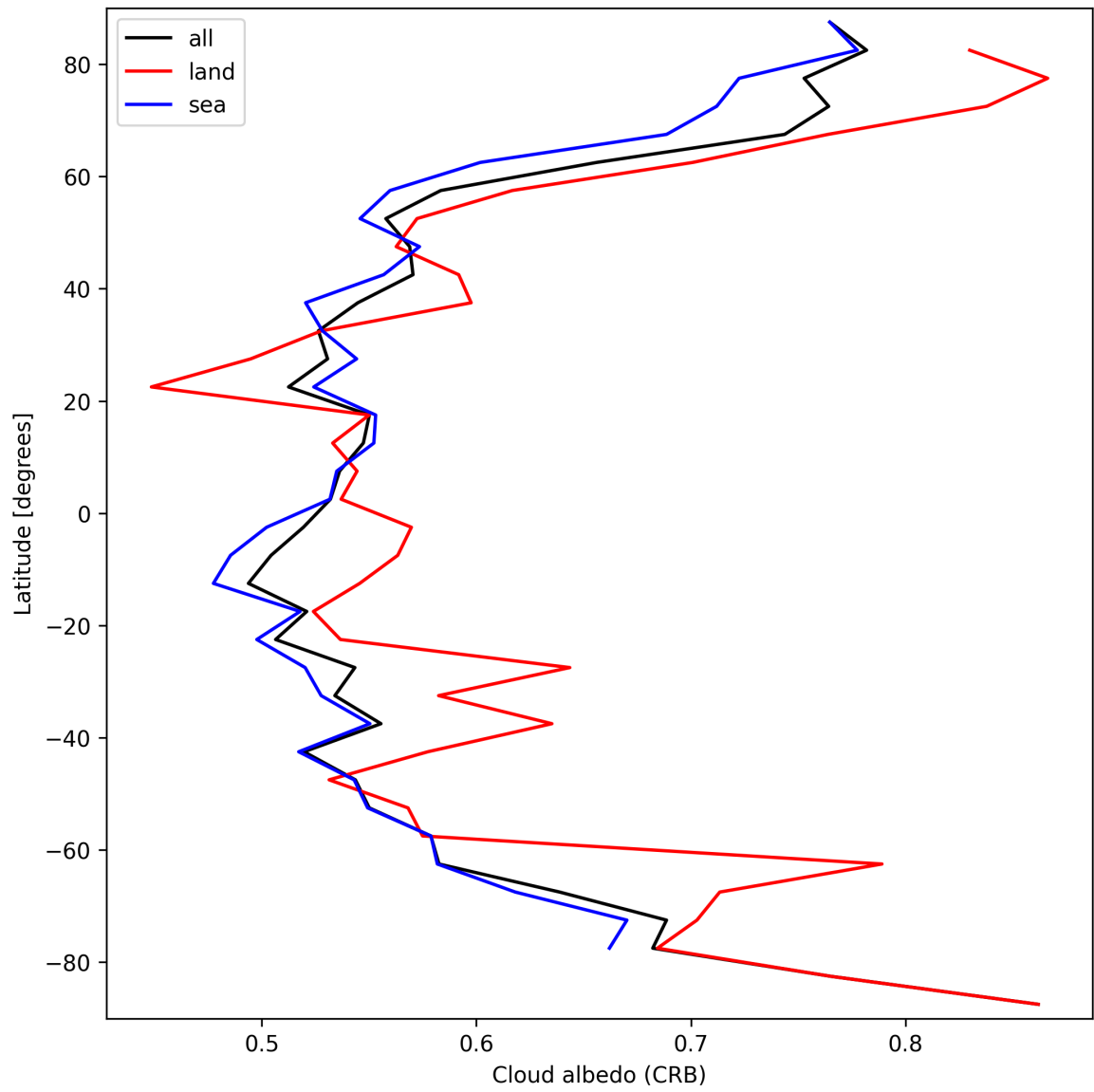
Figure 28: Zonal average of “Cloud albedo (CRB)” for 2025-03-25 to 2025-03-27.
