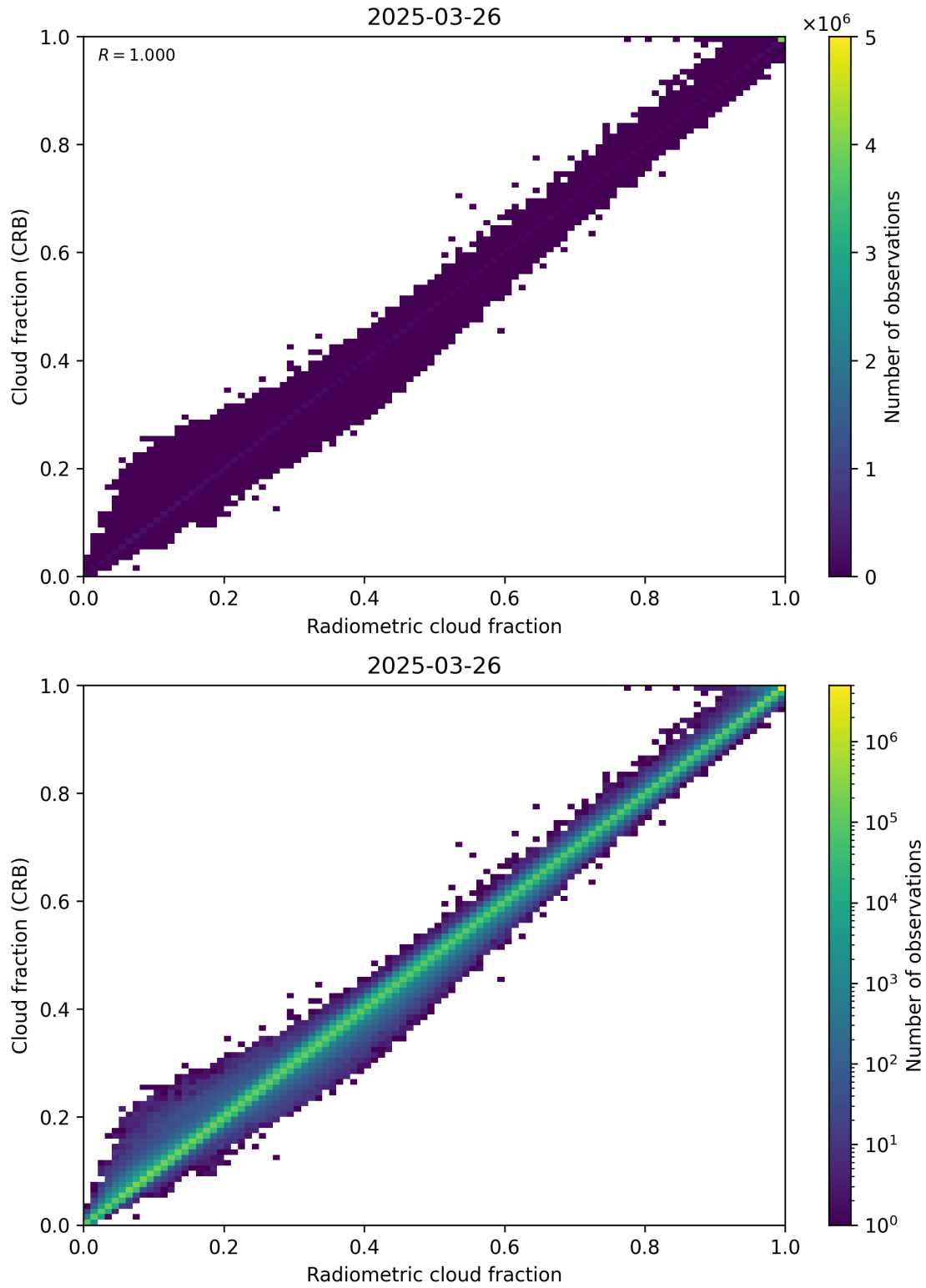
Figure 73: Scatter density plot of “Radiometric cloud fraction” against “Cloud fraction (CRB)” for 2025-03-25 to 2025-03-27.
