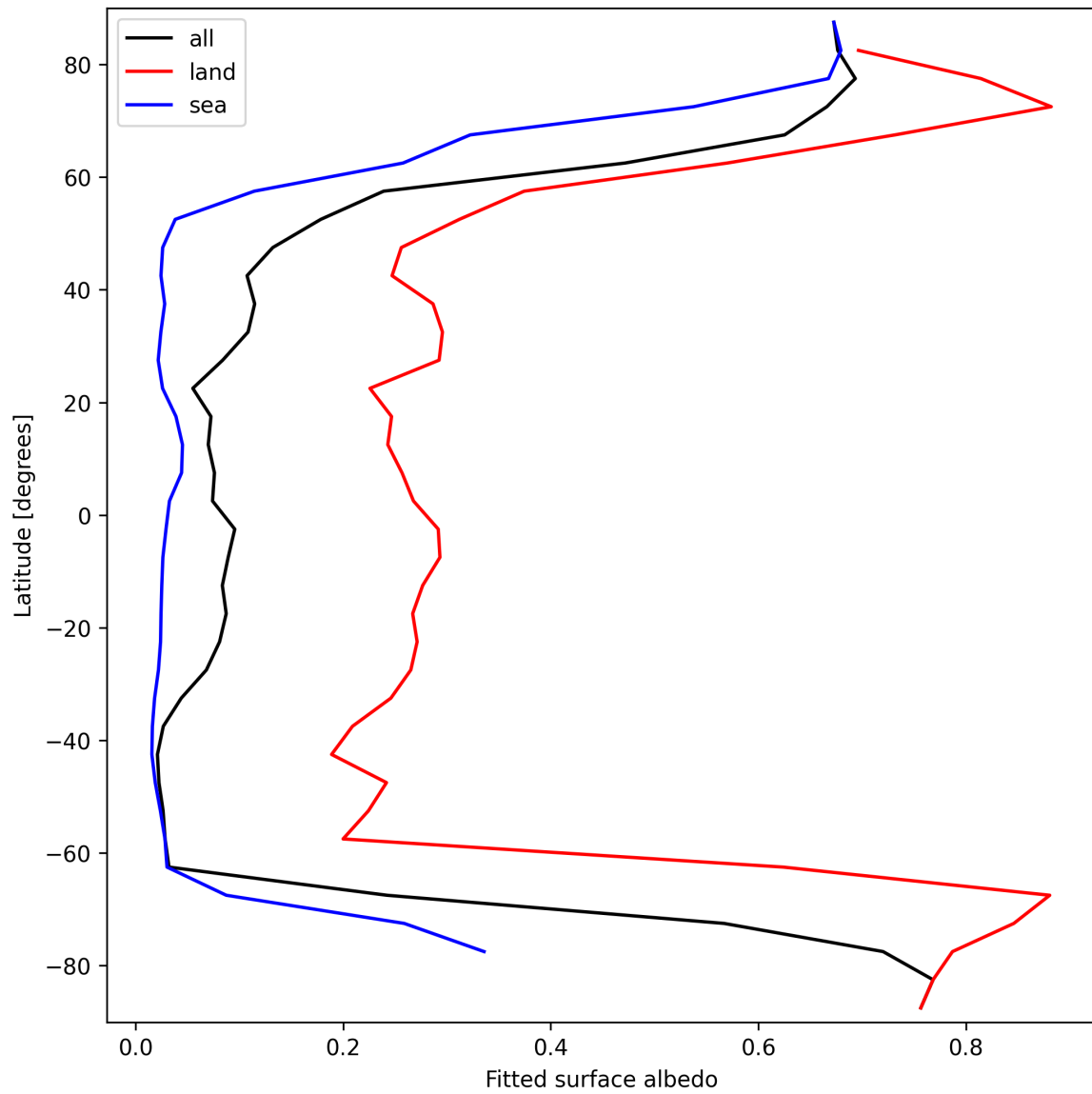
Figure 29: Zonal average of “Fitted surface albedo” for 2025-03-25 to 2025-03-27.
