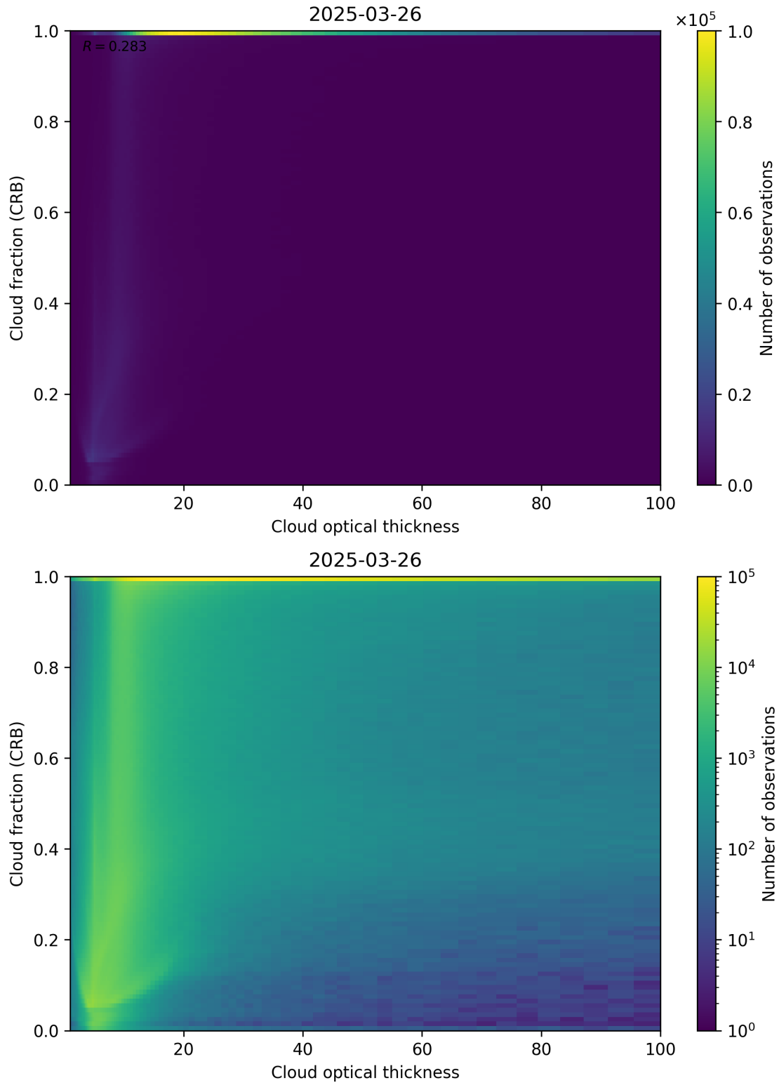
Figure 84: Scatter density plot of “Cloud optical thickness” against “Cloud fraction (CRB)” for 2025-03-25 to 2025-03-27.
