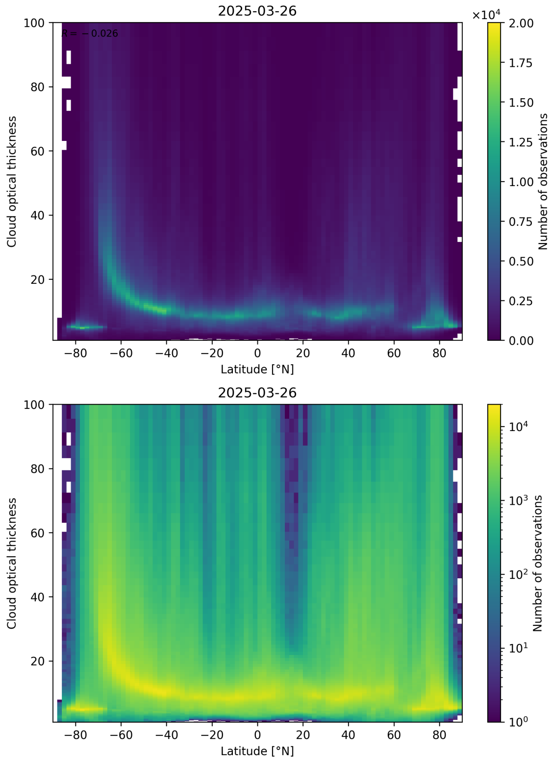
Figure 96: Scatter density plot of “Latitude” against “Cloud optical thickness” for 2025-03-25 to 2025-03-27.
