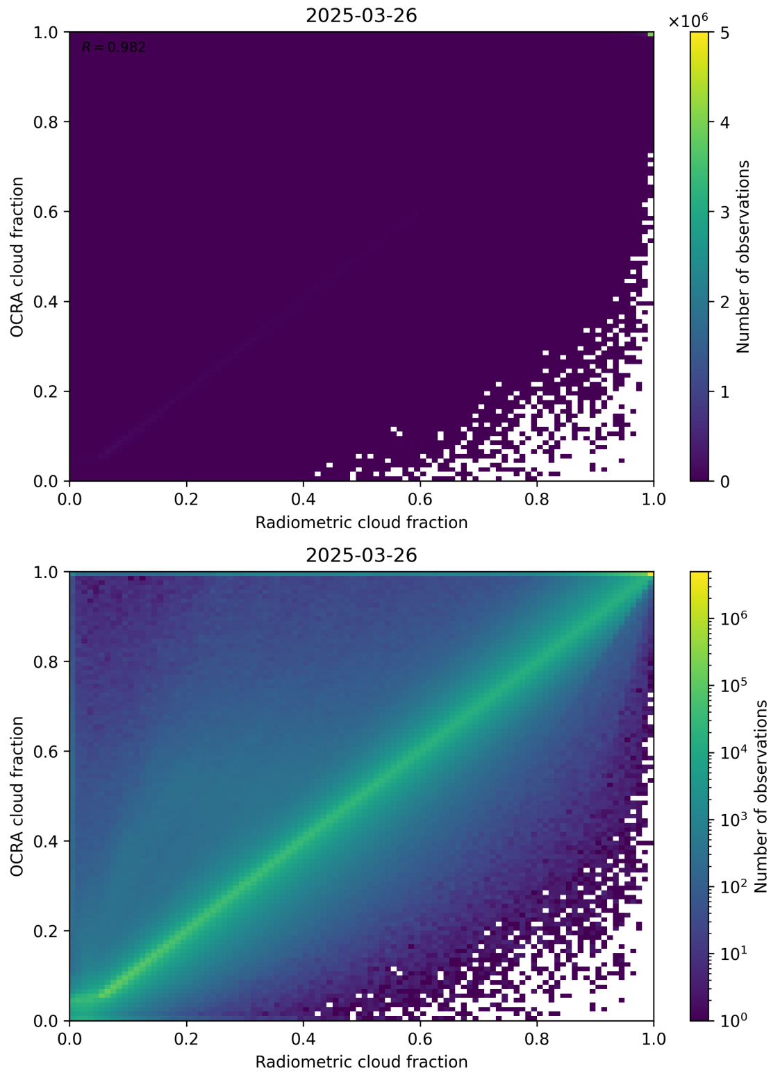
Figure 72: Scatter density plot of “Radiometric cloud fraction” against “OCRA cloud fraction” for 2025-03-25 to 2025-03-27.
