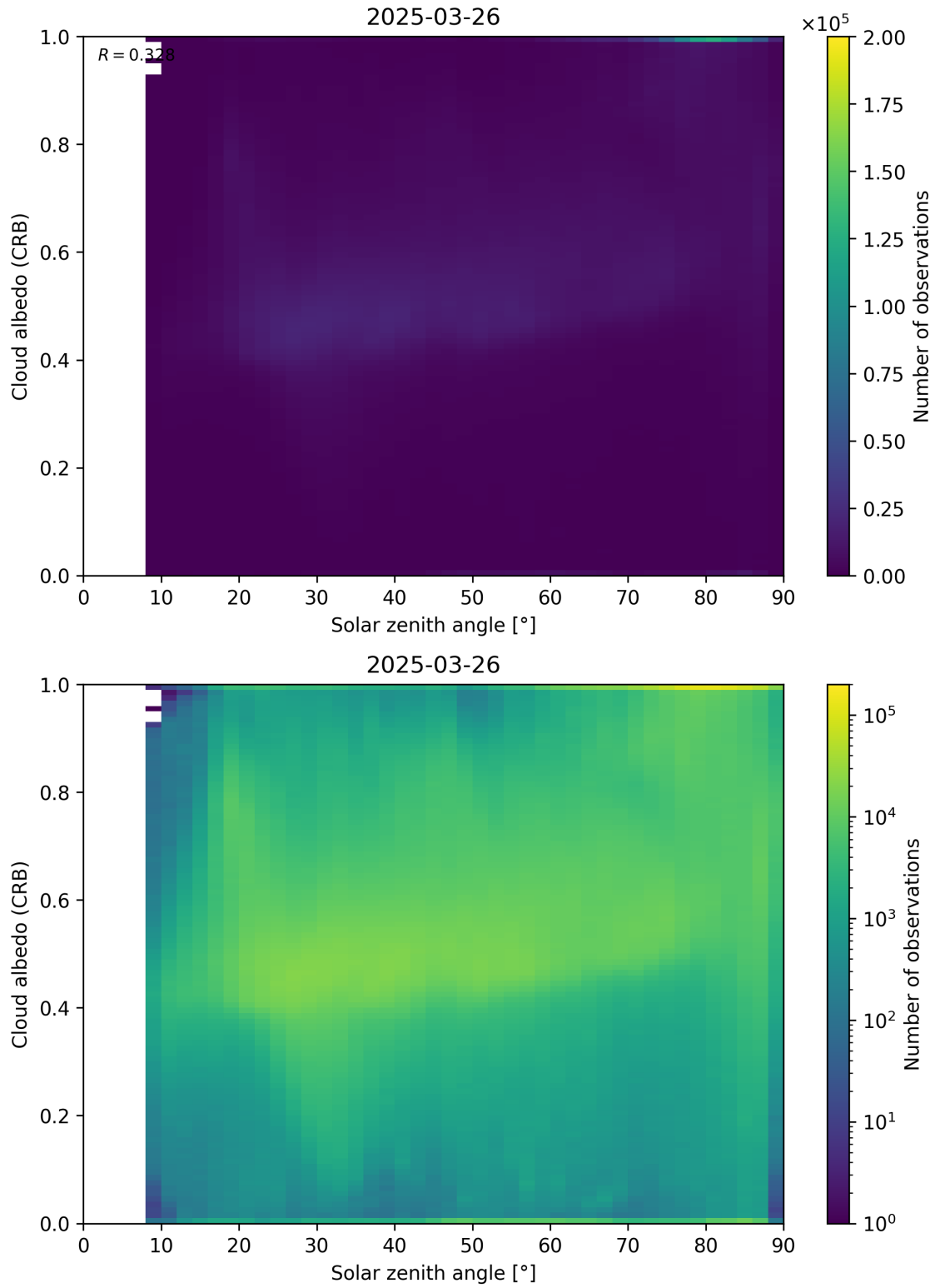
Figure 98: Scatter density plot of “Solar zenith angle” against “Cloud albedo (CRB)” for 2025-03-25 to 2025-03-27.
