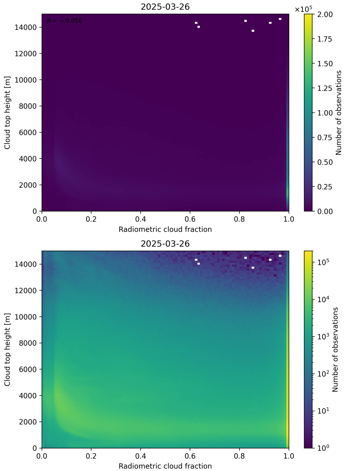
Figure 76: Scatter density plot of “Radiometric cloud fraction” against “Cloud top height” for 2025-03-25 to 2025-03-27.
