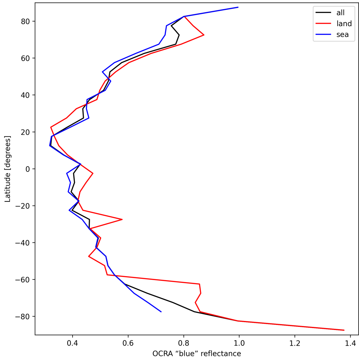
Figure 35: Zonal average of "OCRA "blue" reflectance" for 2025-03-25 to 2025-03-27.
