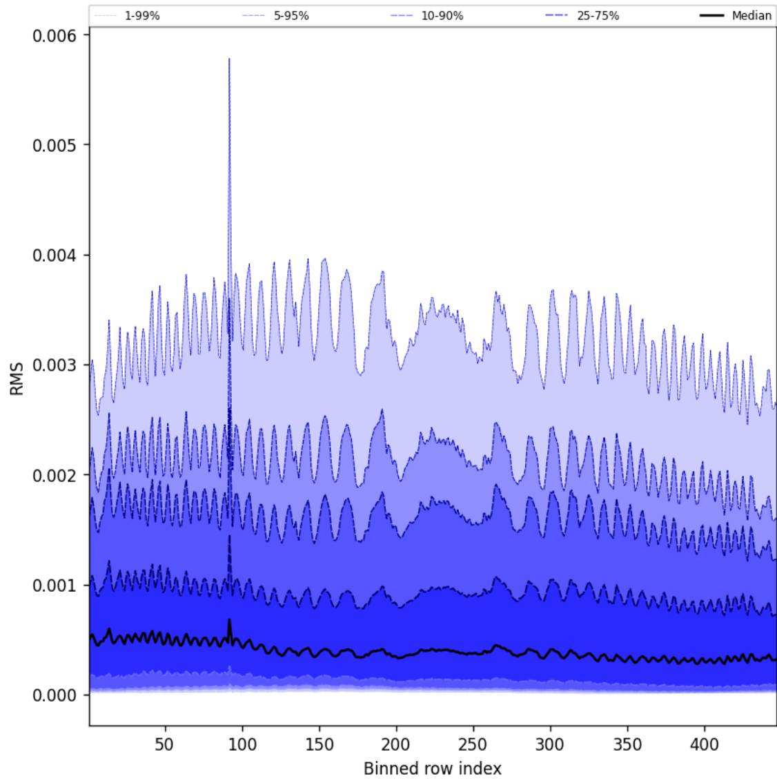
Figure 63: Along track statistics of “RMS” for 2025-03-25 to 2025-03-27
