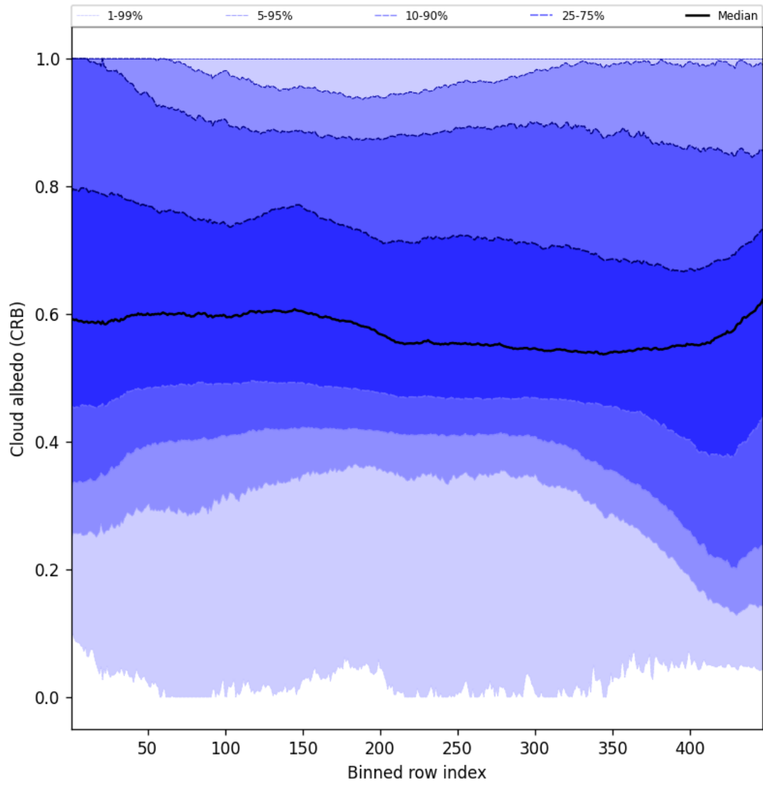
Figure 60: Along track statistics of “Cloud albedo (CRB)” for 2025-03-25 to 2025-03-27
