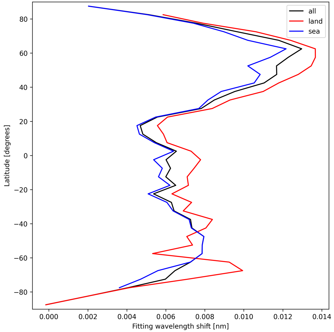
Figure 33: Zonal average of “Fitting wavelength shift” for 2025-03-25 to 2025-03-27.
