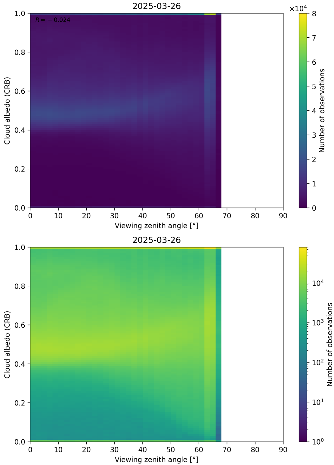
Figure 106: Scatter density plot of “Viewing zenith angle” against “Cloud albedo (CRB)” for 2025-03-25 to 2025-03-27.
