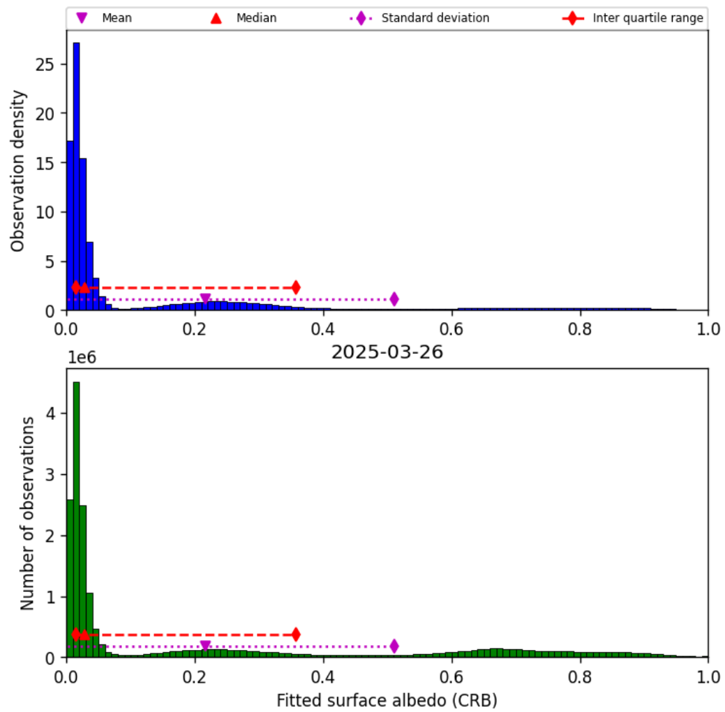
Figure 46: Histogram of “Fitted surface albedo (CRB)” for 2025-03-25 to 2025-03-27
