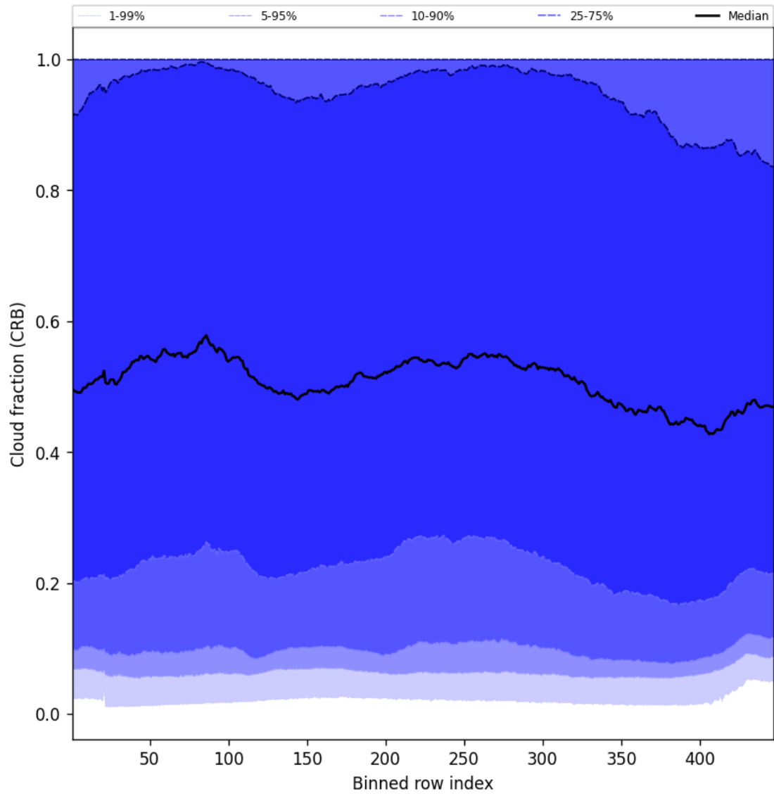
Figure 58: Along track statistics of “Cloud fraction (CRB)” for 2025-03-25 to 2025-03-27
