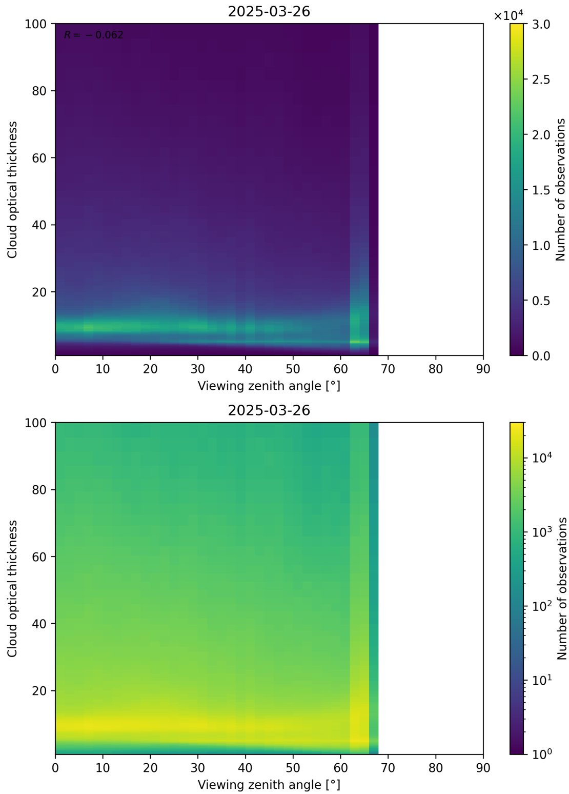
Figure 111: Scatter density plot of “Viewing zenith angle” against “Cloud optical thickness” for 2025-03-25 to 2025-03-27.
