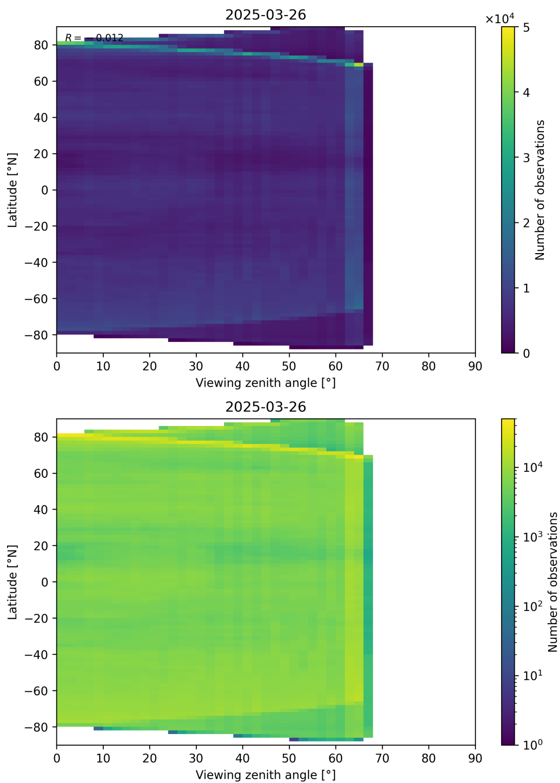
Figure 113: Scatter density plot of “Viewing zenith angle” against “Latitude” for 2025-03-25 to 2025-03-27.
