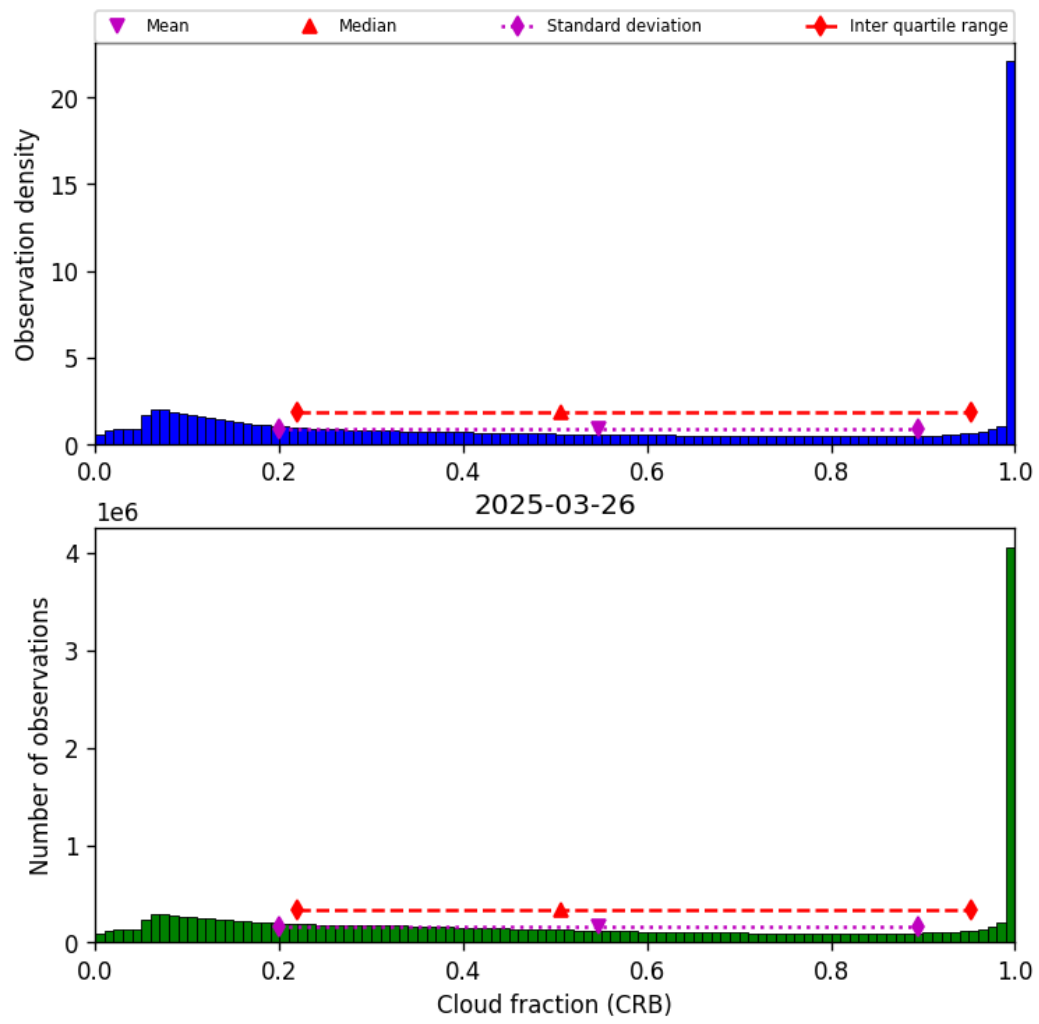
Figure 42: Histogram of “Cloud fraction (CRB)” for 2025-03-25 to 2025-03-27
