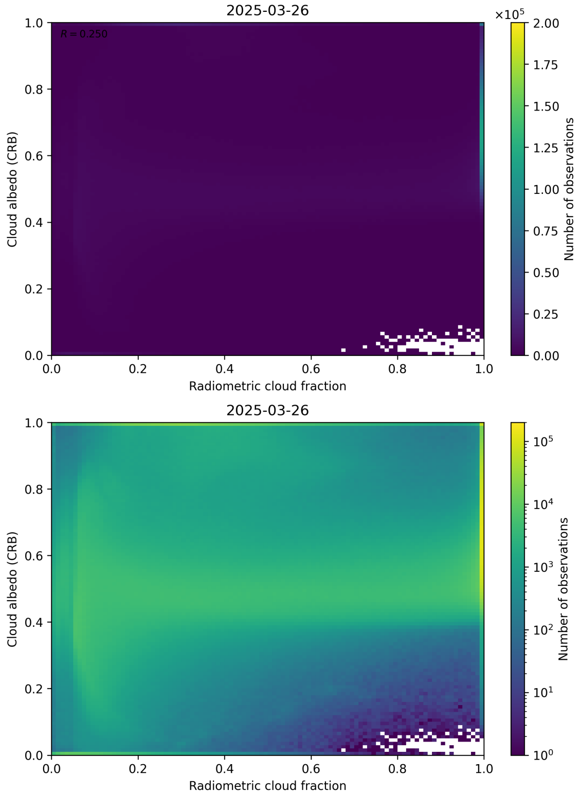
Figure 71: Scatter density plot of “Radiometric cloud fraction” against “Cloud albedo (CRB)” for 2025-03-25 to 2025-03-27.
