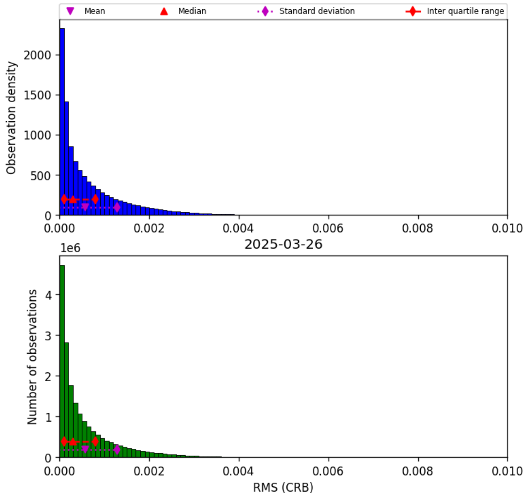
Figure 48: Histogram of “RMS (CRB)” for 2025-03-25 to 2025-03-27
