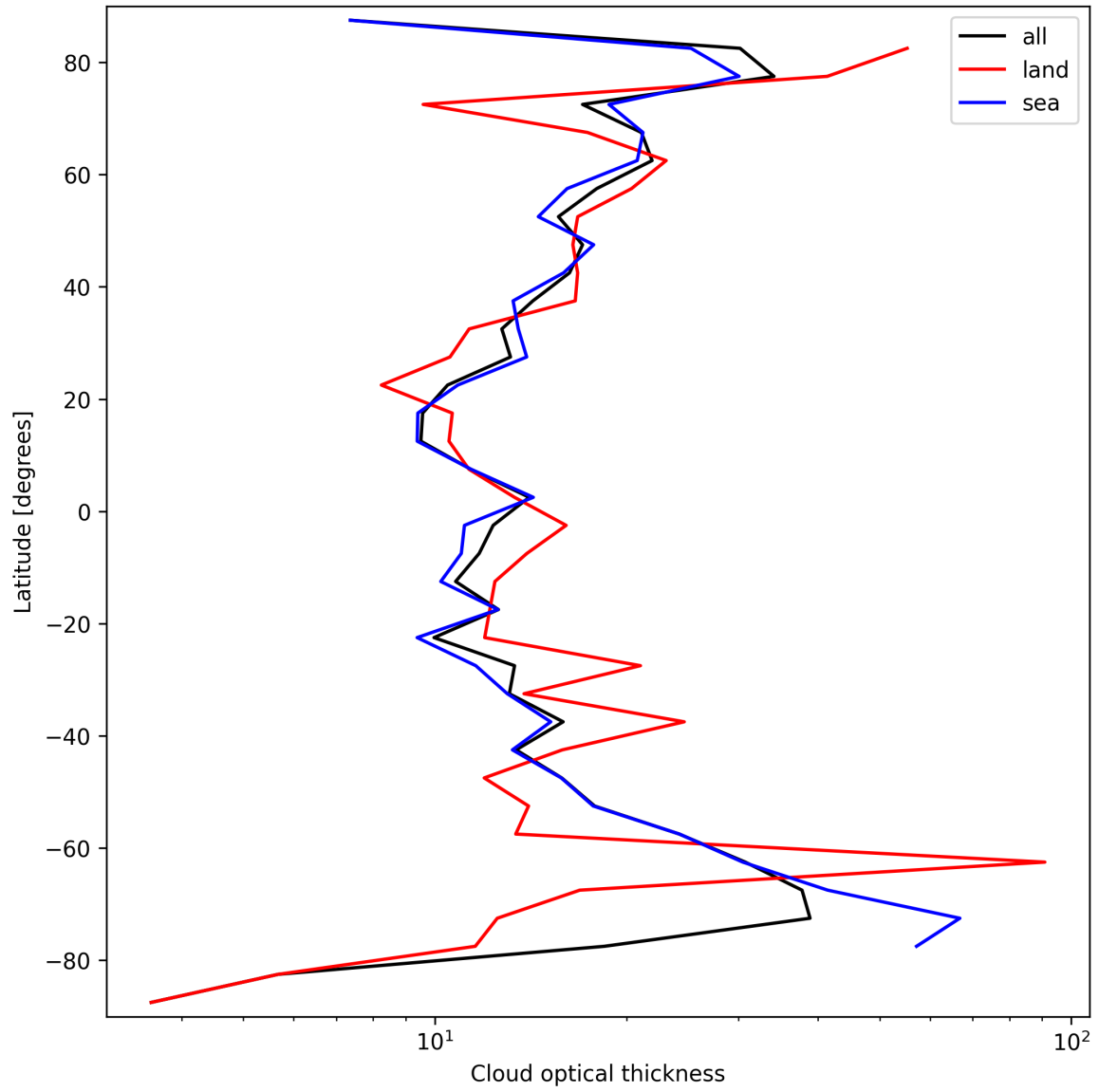
Figure 25: Zonal average of “Cloud optical thickness” for 2025-03-25 to 2025-03-27.
