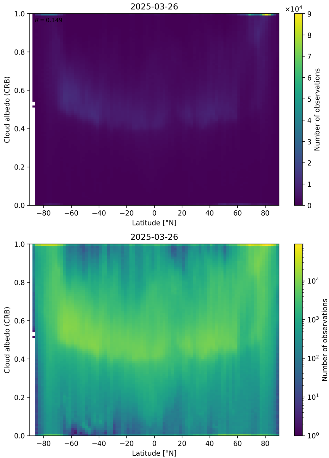
Figure 91: Scatter density plot of “Latitude” against “Cloud albedo (CRB)” for 2025-03-25 to 2025-03-27.
