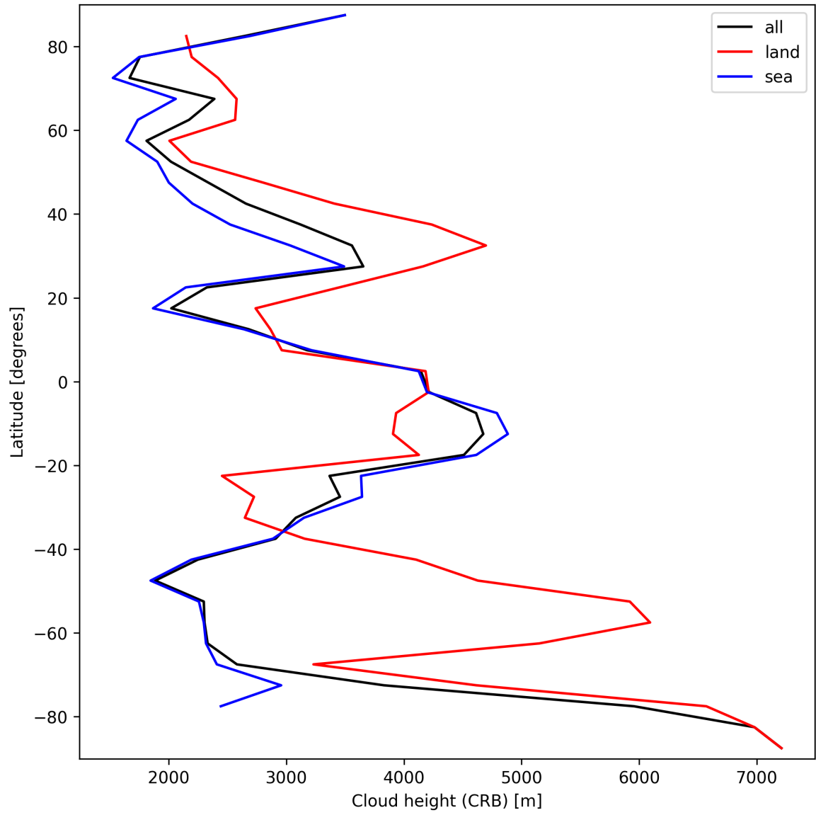
Figure 27: Zonal average of “Cloud height (CRB)” for 2025-03-25 to 2025-03-27.
