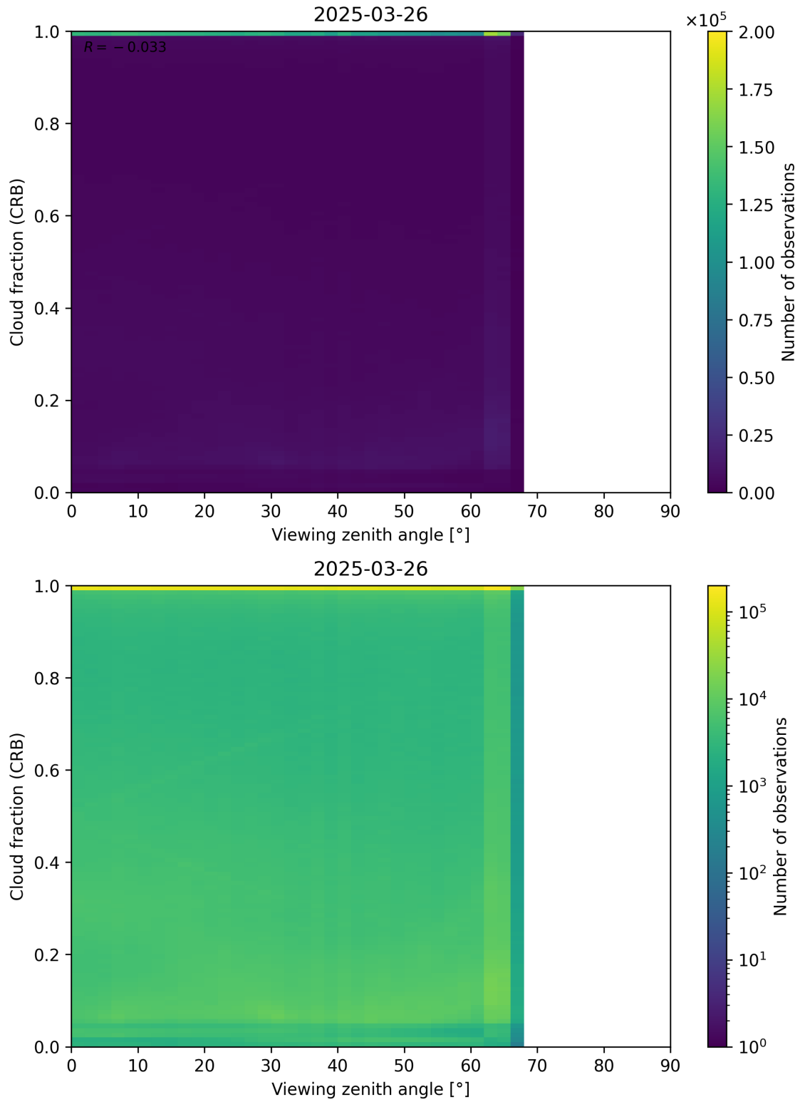
Figure 109: Scatter density plot of “Viewing zenith angle” against “Cloud fraction (CRB)” for 2025-03-25 to 2025-03-27.
