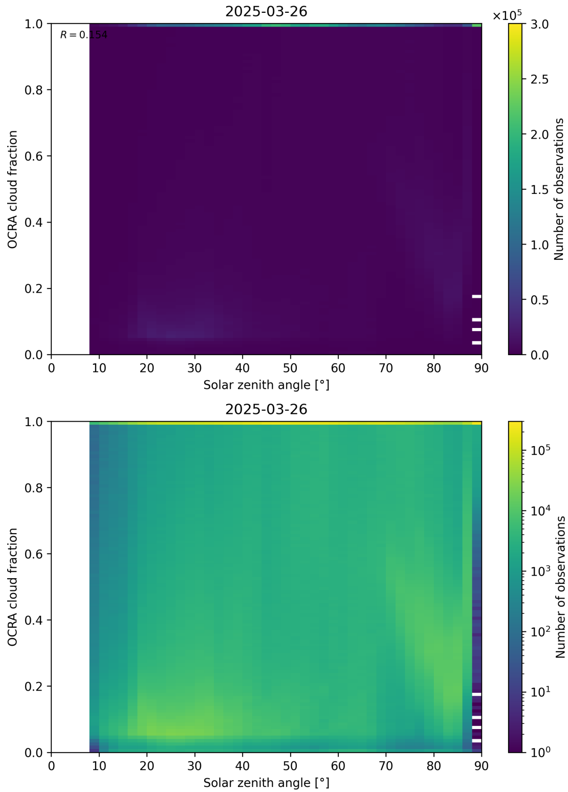
Figure 100: Scatter density plot of “Solar zenith angle” against “OCRA cloud fraction” for 2025-03-25 to 2025-03-27.
