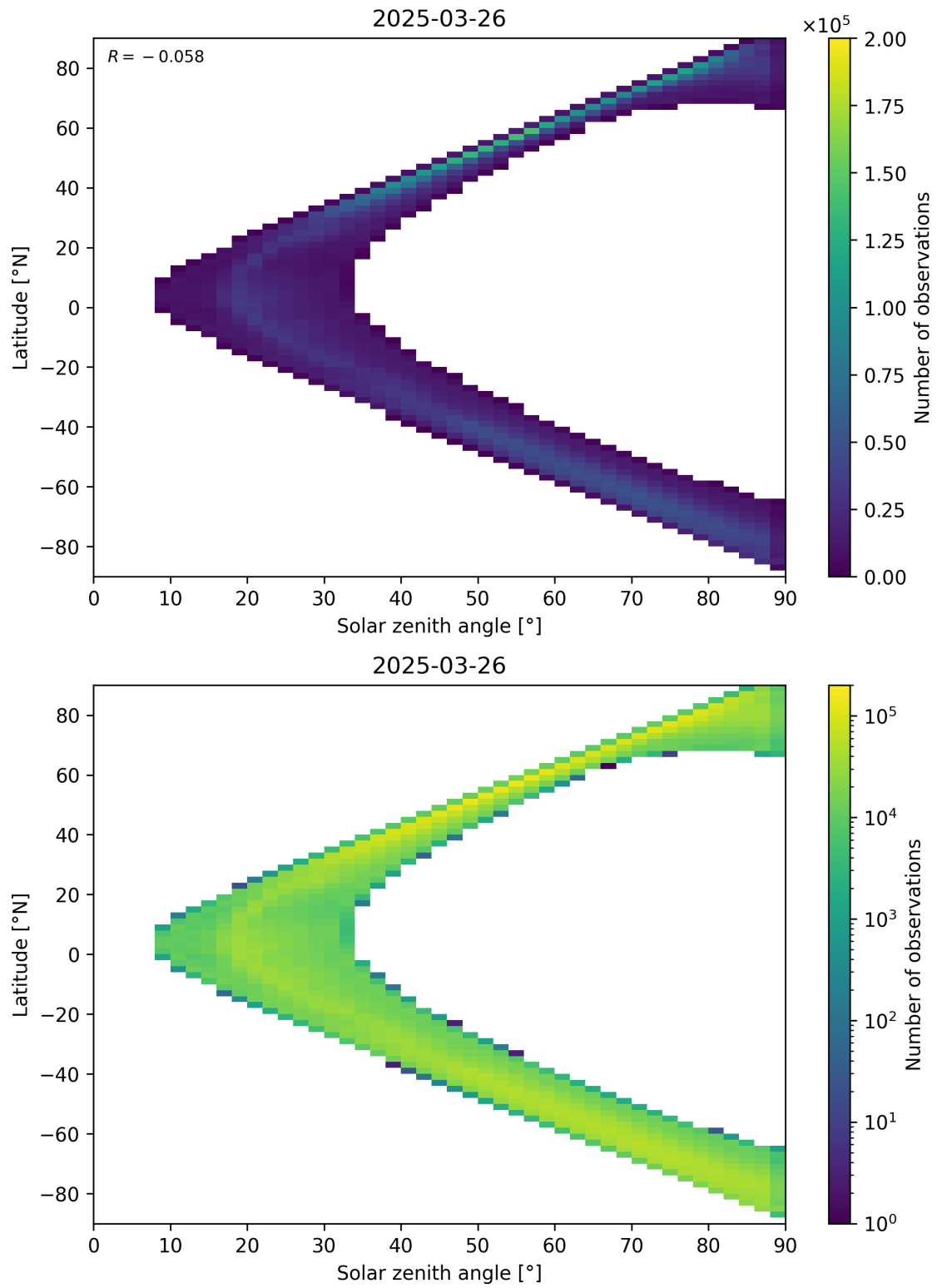
Figure 105: Scatter density plot of “Solar zenith angle” against “Latitude” for 2025-03-25 to 2025-03-27.
