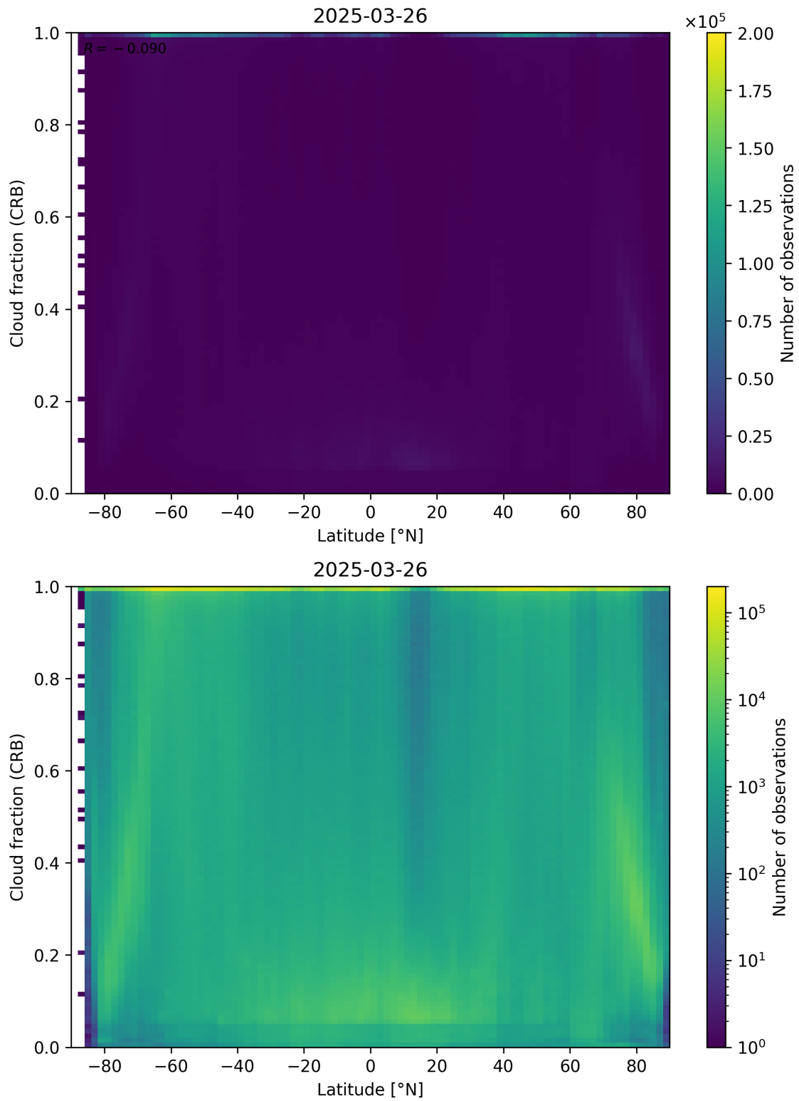
Figure 94: Scatter density plot of “Latitude” against “Cloud fraction (CRB)” for 2025-03-25 to 2025-03-27.
