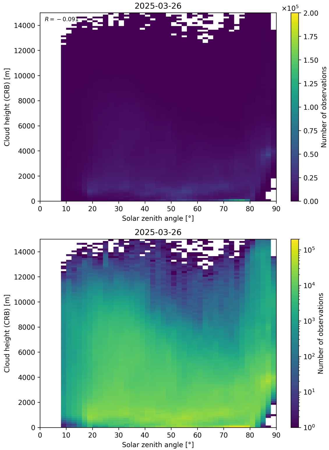
Figure 102: Scatter density plot of “Solar zenith angle” against “Cloud height (CRB)” for 2025-03-25 to 2025-03-27.
