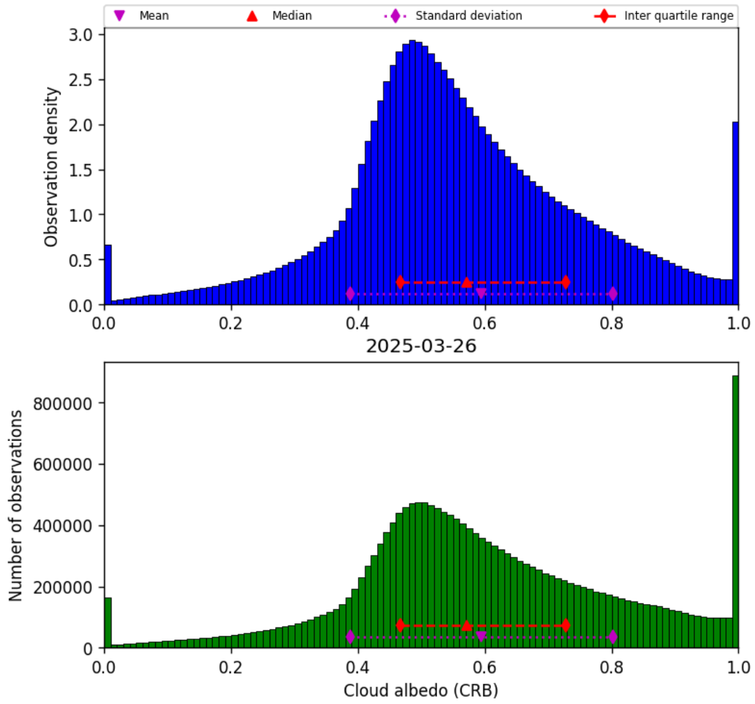
Figure 44: Histogram of “Cloud albedo (CRB)” for 2025-03-25 to 2025-03-27
