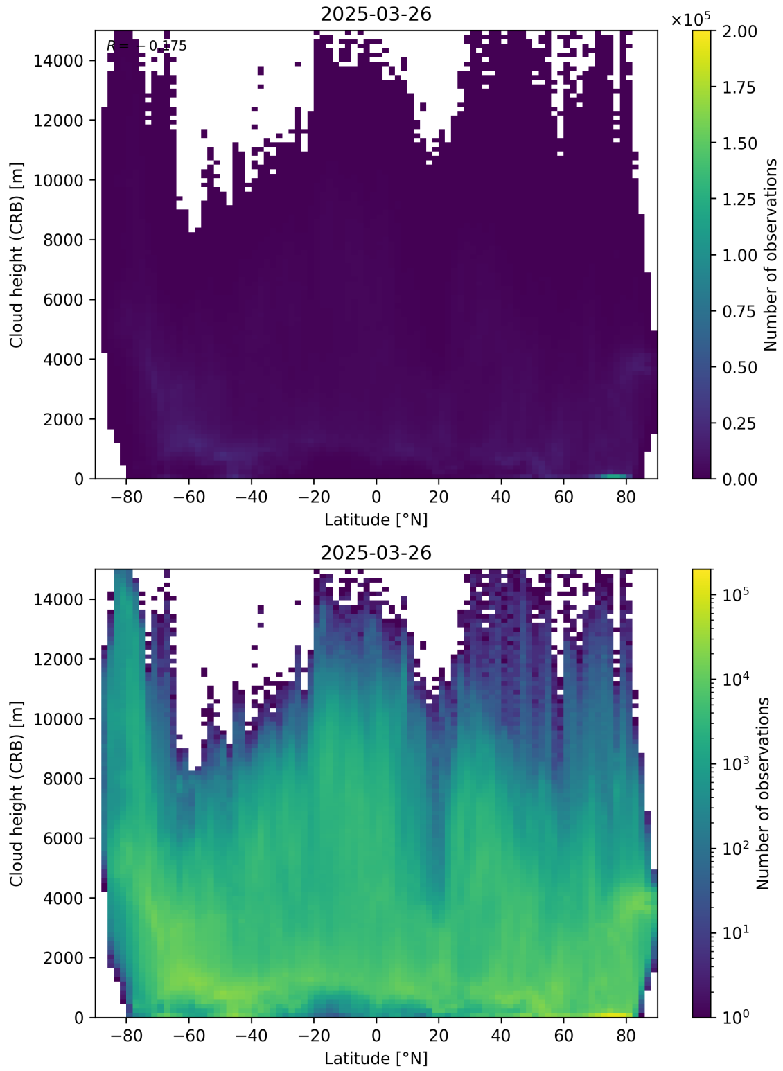
Figure 95: Scatter density plot of “Latitude” against “Cloud height (CRB)” for 2025-03-25 to 2025-03-27.
