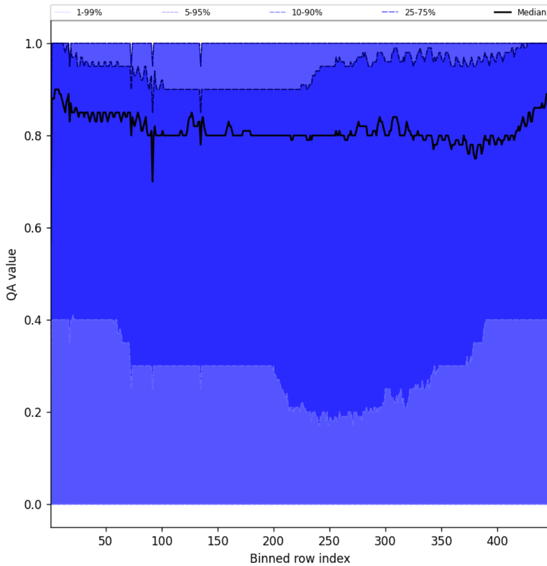
Figure 54: Along track statistics of “QA value” for 2025-03-25 to 2025-03-27
