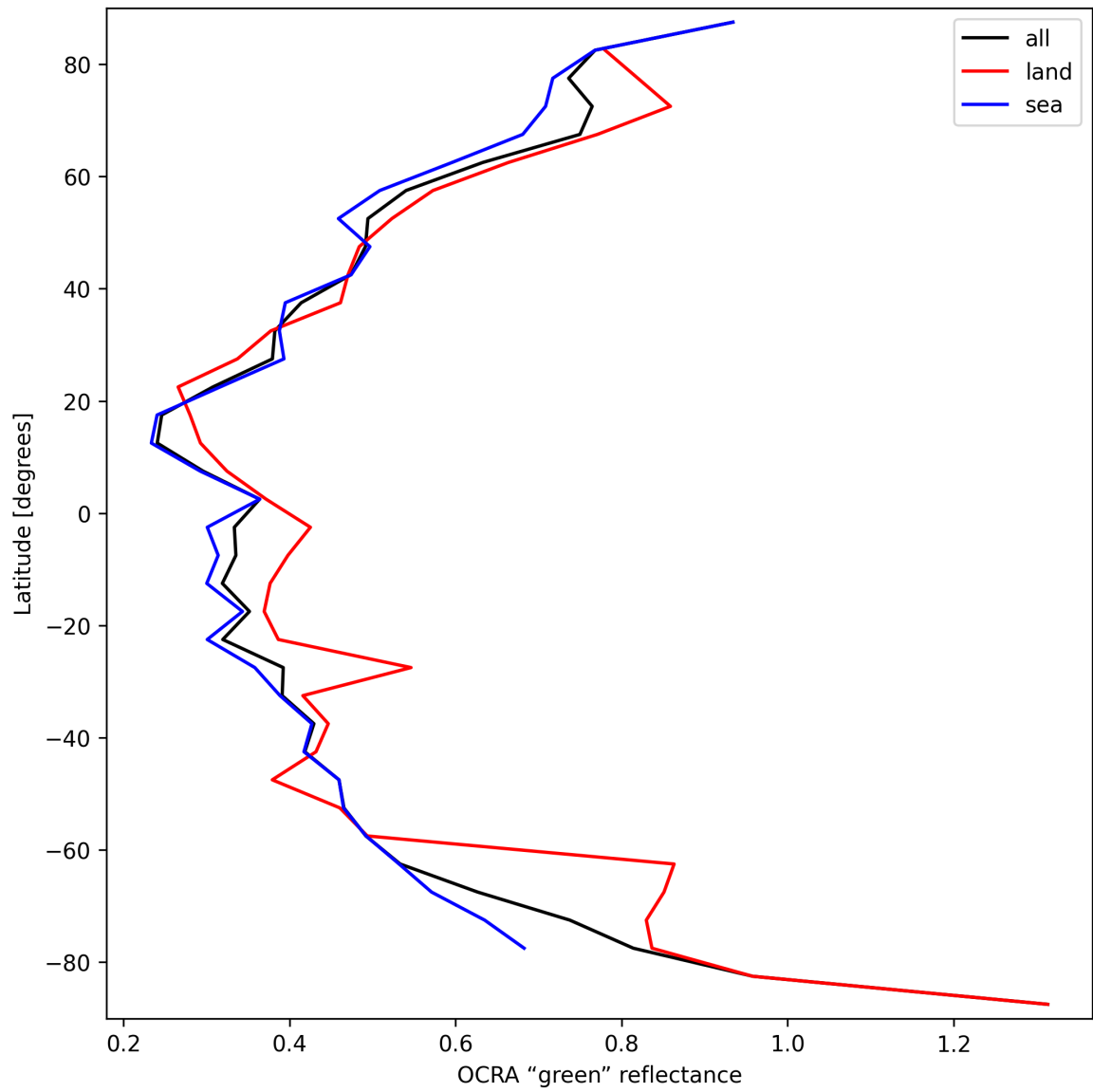
Figure 36: Zonal average of “OCRA “green” reflectance” for 2025-03-25 to 2025-03-27.
