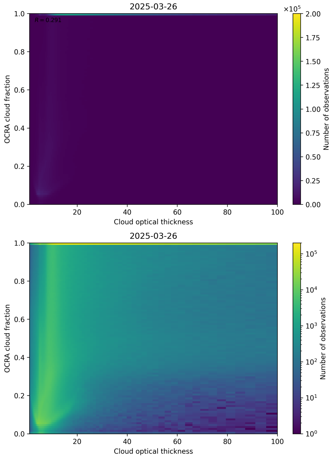
Figure 83: Scatter density plot of “Cloud optical thickness” against “OCRA cloud fraction” for 2025-03-25 to 2025-03-27.
