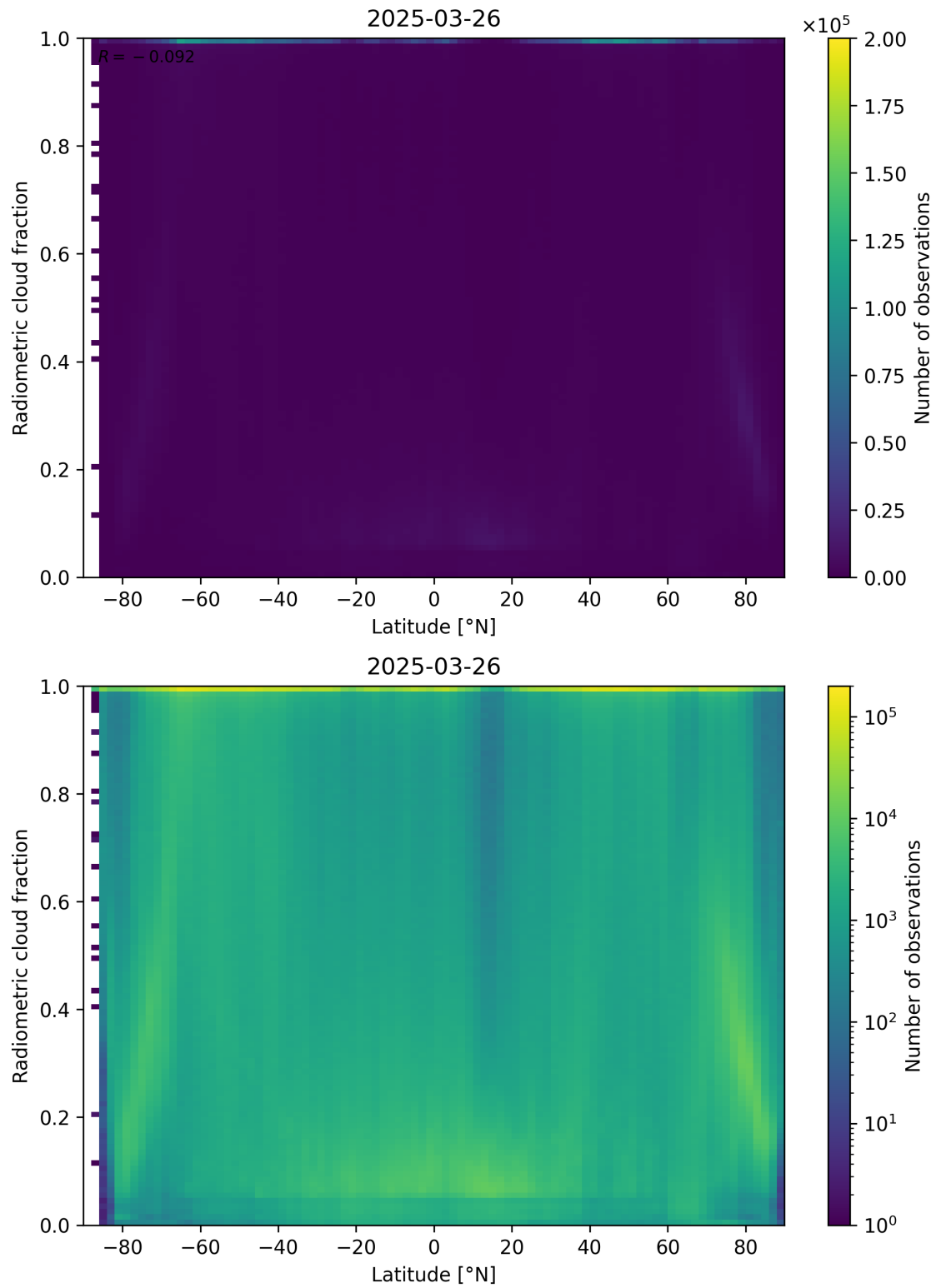
Figure 92: Scatter density plot of “Latitude” against “Radiometric cloud fraction” for 2025-03-25 to 2025-03-27.
