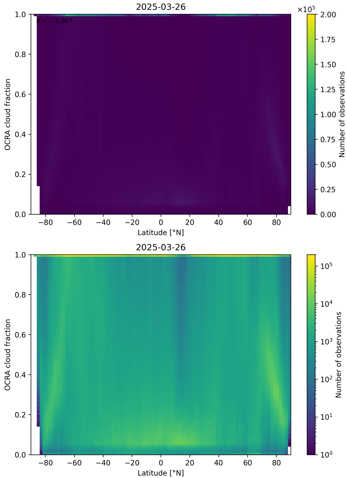
Figure 93: Scatter density plot of “Latitude” against “OCRA cloud fraction” for 2025-03-25 to 2025-03-27.
