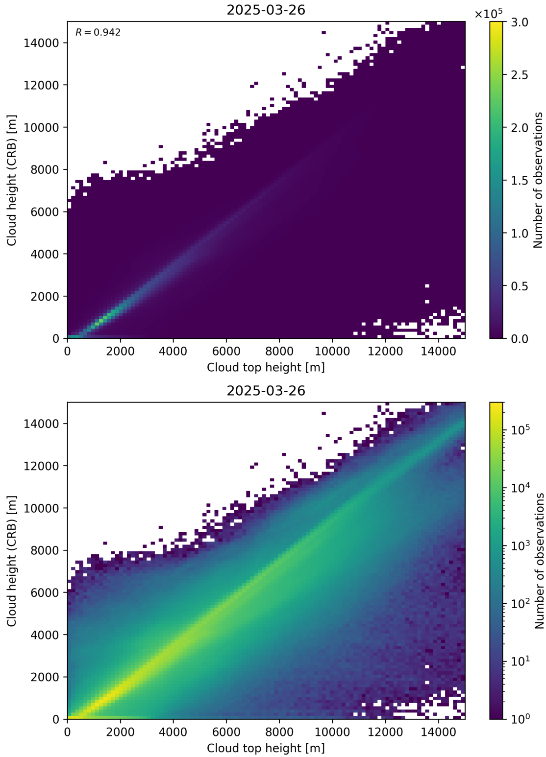
Figure 89: Scatter density plot of “Cloud top height” against “Cloud height (CRB)” for 2025-03-25 to 2025-03-27.
