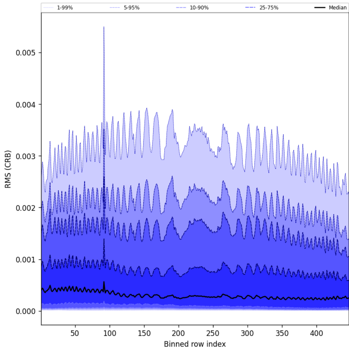
Figure 64: Along track statistics of “RMS (CRB)” for 2025-03-25 to 2025-03-27
