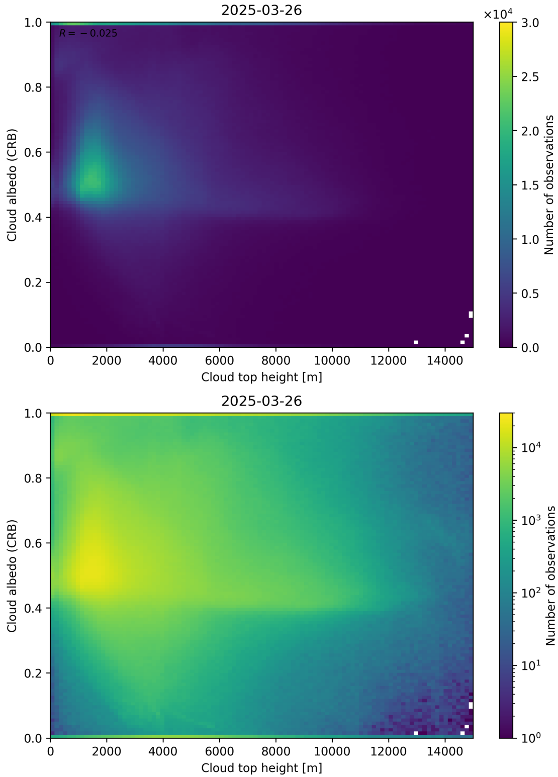
Figure 86: Scatter density plot of “Cloud top height” against “Cloud albedo (CRB)” for 2025-03-25 to 2025-03-27.
