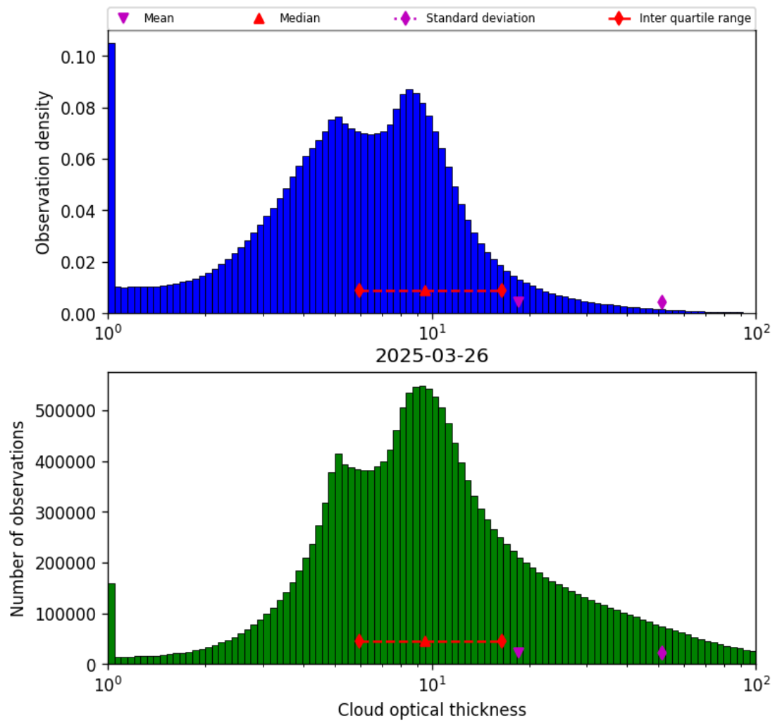
Figure 41: Histogram of “Cloud optical thickness” for 2025-03-25 to 2025-03-27
