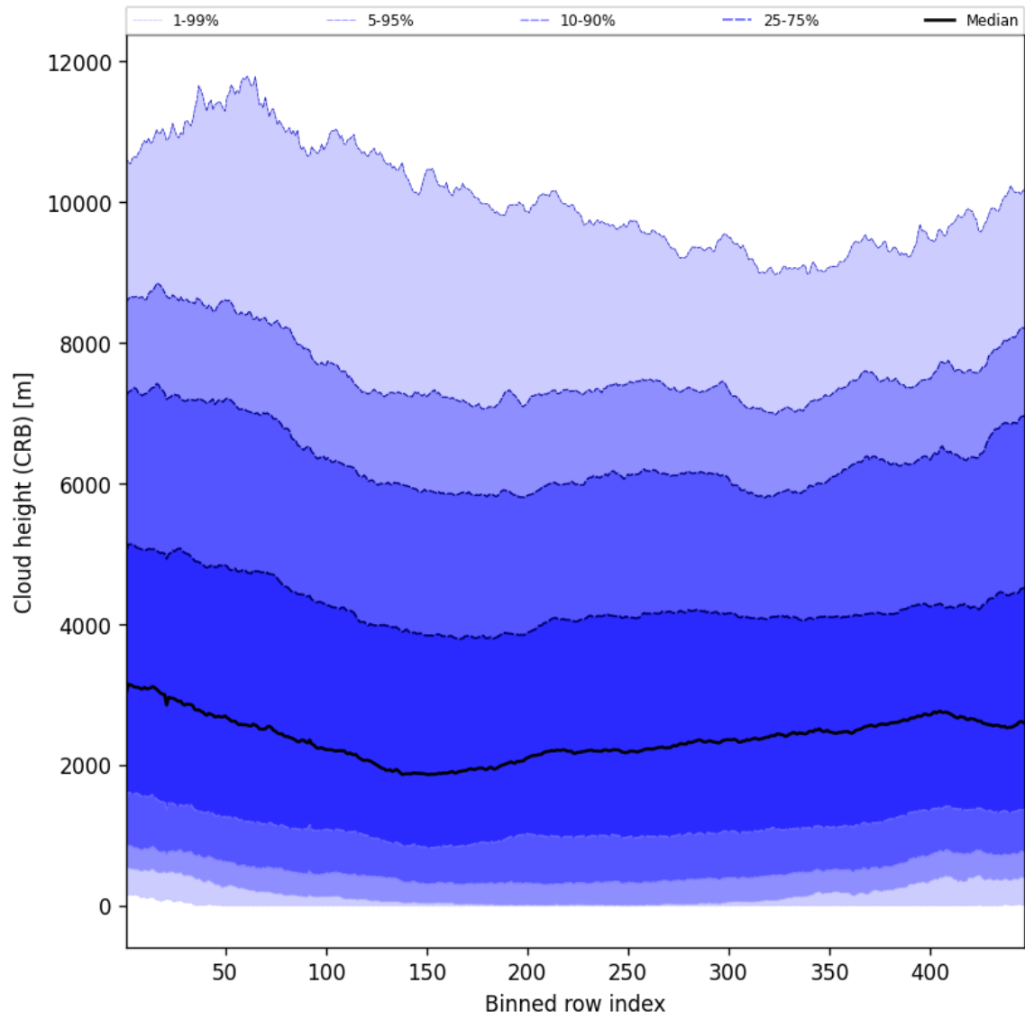
Figure 59: Along track statistics of “Cloud height (CRB)” for 2025-03-25 to 2025-03-27
