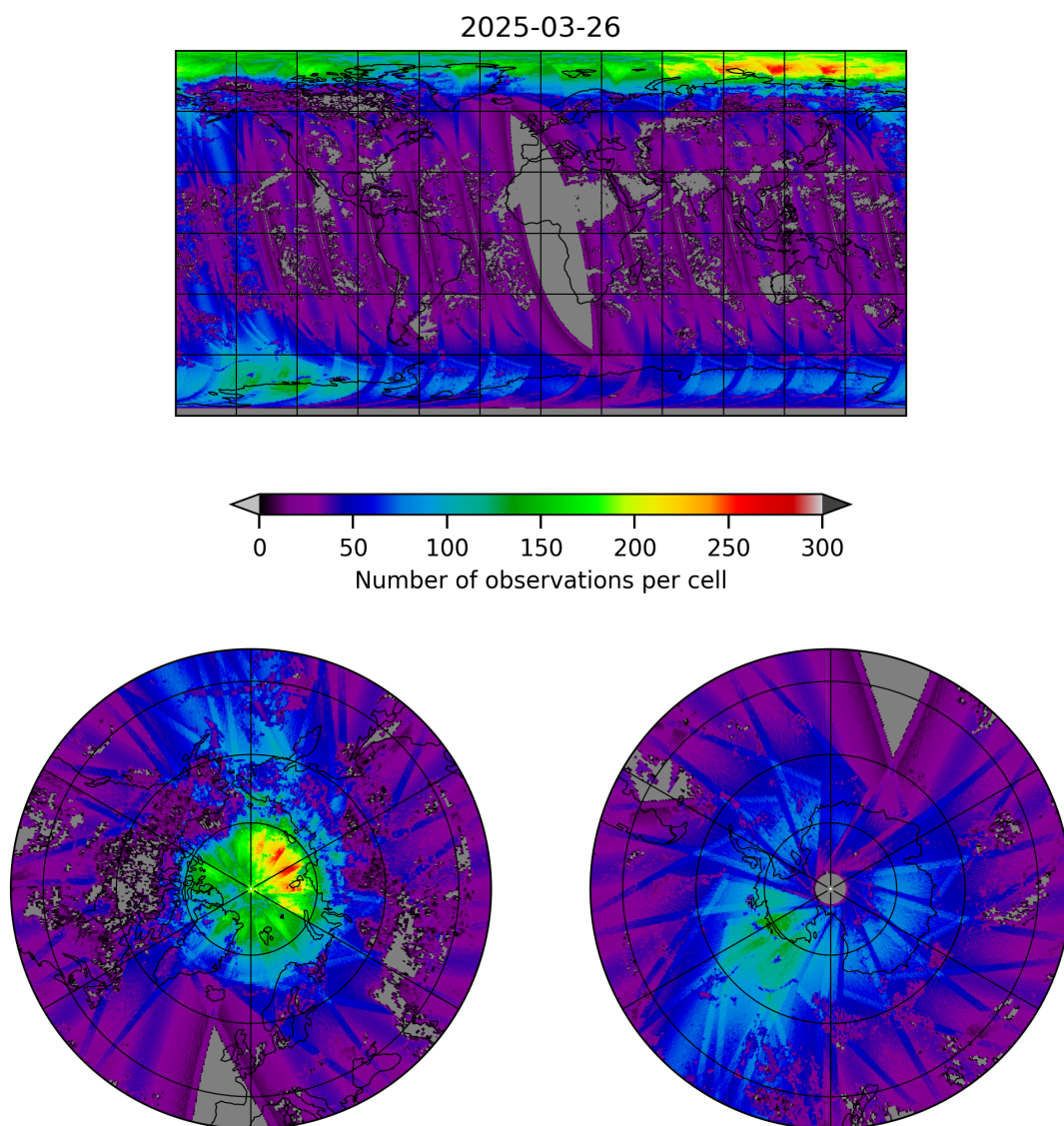
Figure 21: Map of the number of observations for 2025-03-25 to 2025-03-27
