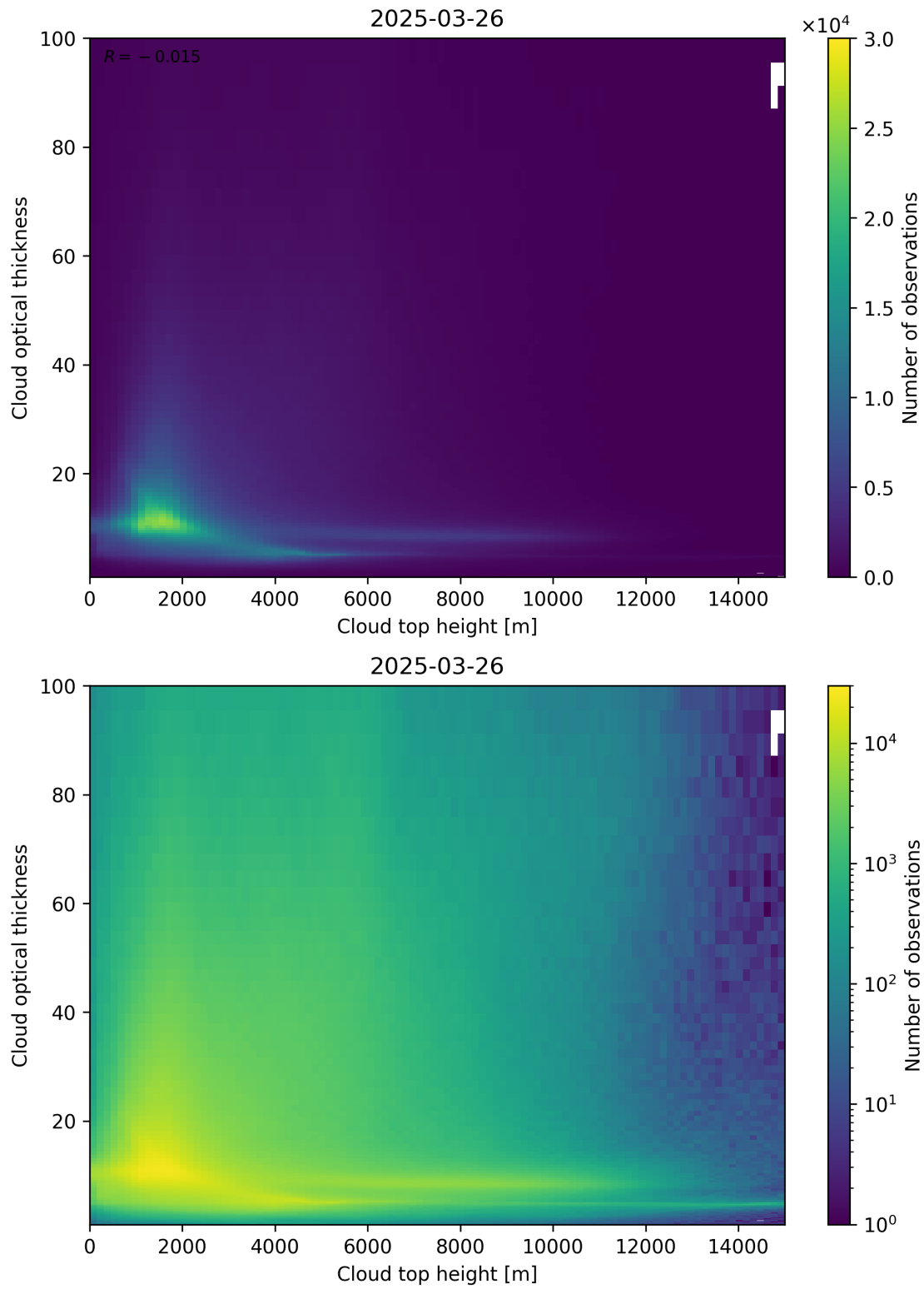
Figure 90: Scatter density plot of “Cloud top height” against “Cloud optical thickness” for 2025-03-25 to 2025-03-27.
