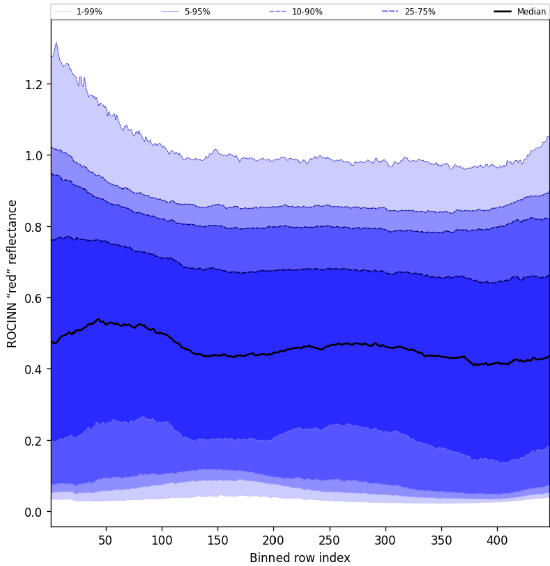
Figure 69: Along track statistics of “ROCINN “red” reflectance” for 2025-03-25 to 2025-03-27
