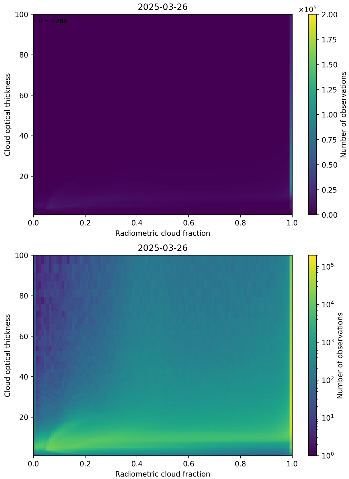
Figure 75: Scatter density plot of “Radiometric cloud fraction” against “Cloud optical thickness” for 2025-03-25 to 2025-03-27.
