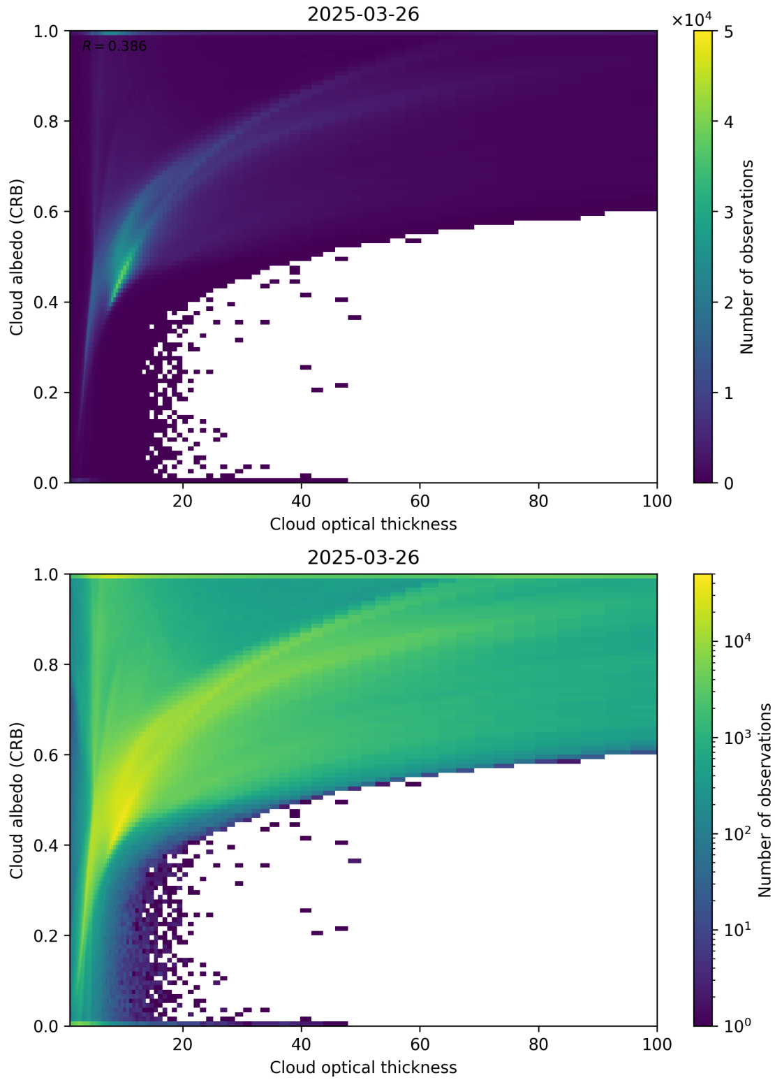
Figure 82: Scatter density plot of “Cloud optical thickness” against “Cloud albedo (CRB)” for 2025-03-25 to 2025-03-27.
