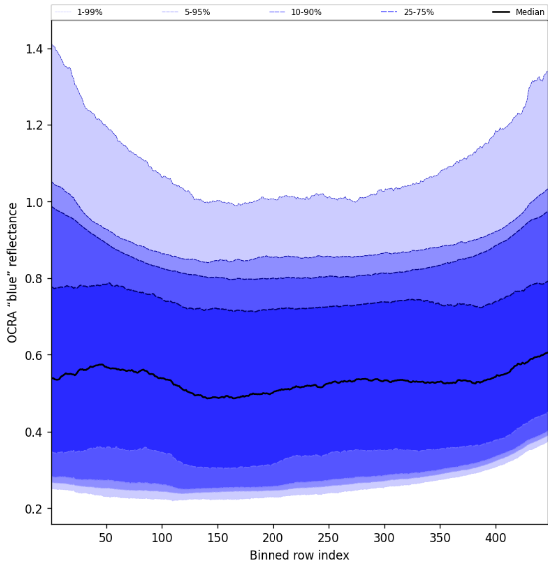
Figure 67: Along track statistics of “OCRA “blue” reflectance” for 2025-03-25 to 2025-03-27
