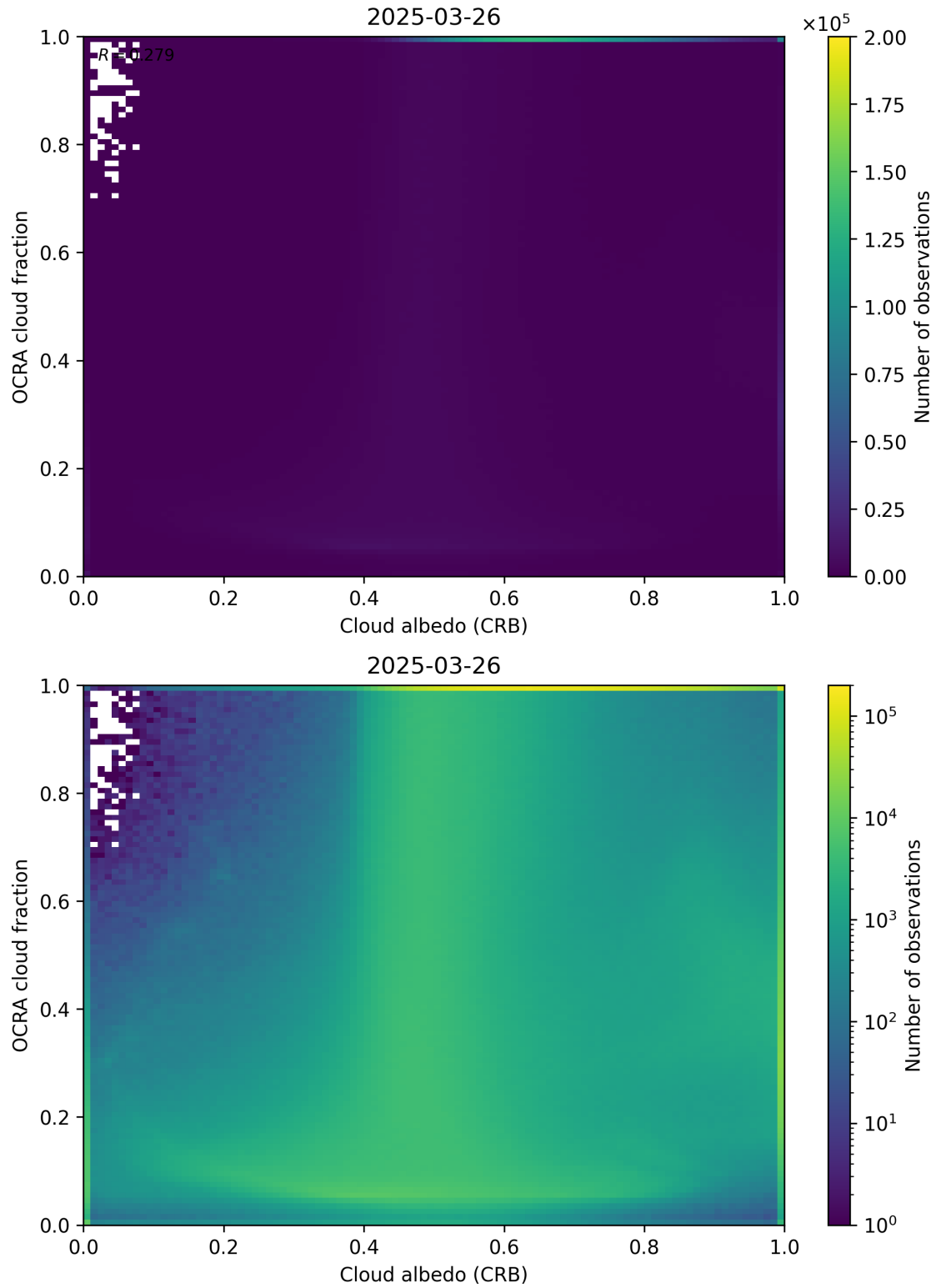
Figure 70: Scatter density plot of “Cloud albedo (CRB)” against “OCRA cloud fraction” for 2025-03-25 to 2025-03-27.
