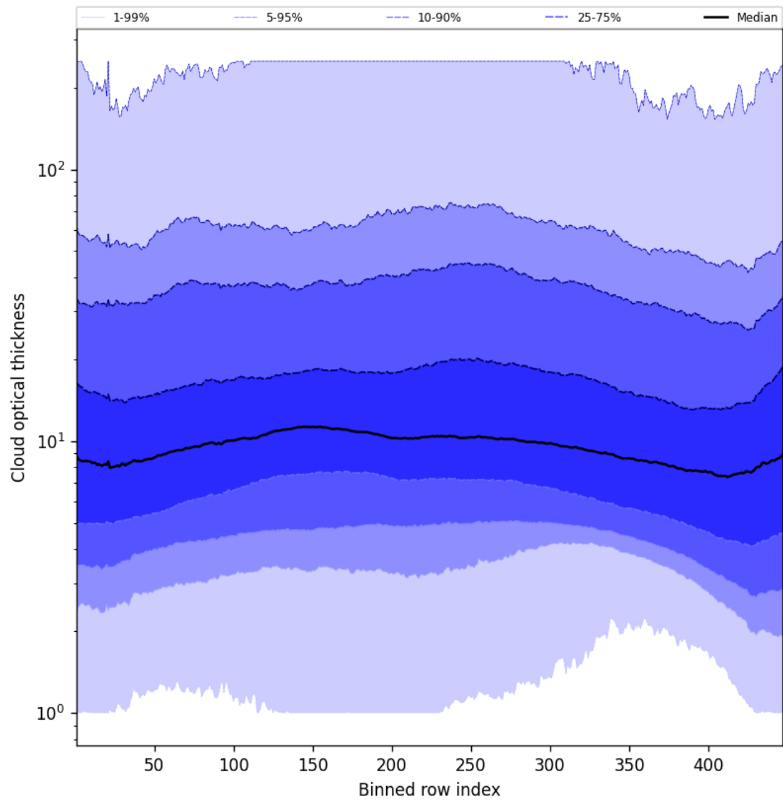
Figure 57: Along track statistics of “Cloud optical thickness” for 2025-03-25 to 2025-03-27
