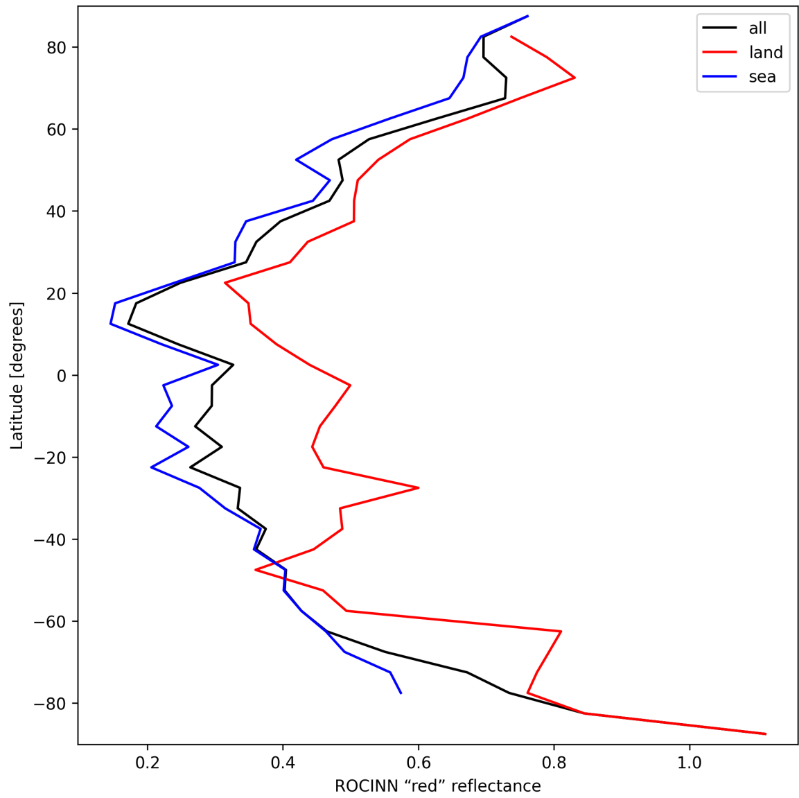
Figure 37: Zonal average of “ROCINN “red” reflectance” for 2025-03-25 to 2025-03-27.
