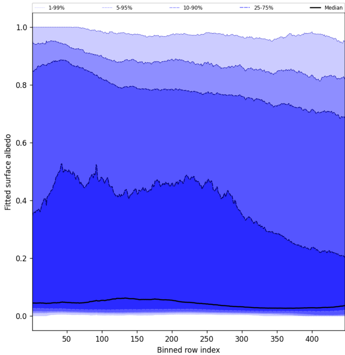
Figure 61: Along track statistics of “Fitted surface albedo” for 2025-03-25 to 2025-03-27
