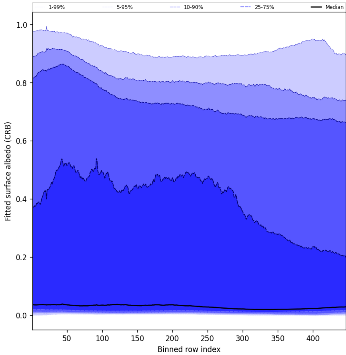
Figure 62: Along track statistics of “Fitted surface albedo (CRB)” for 2025-03-25 to 2025-03-27
