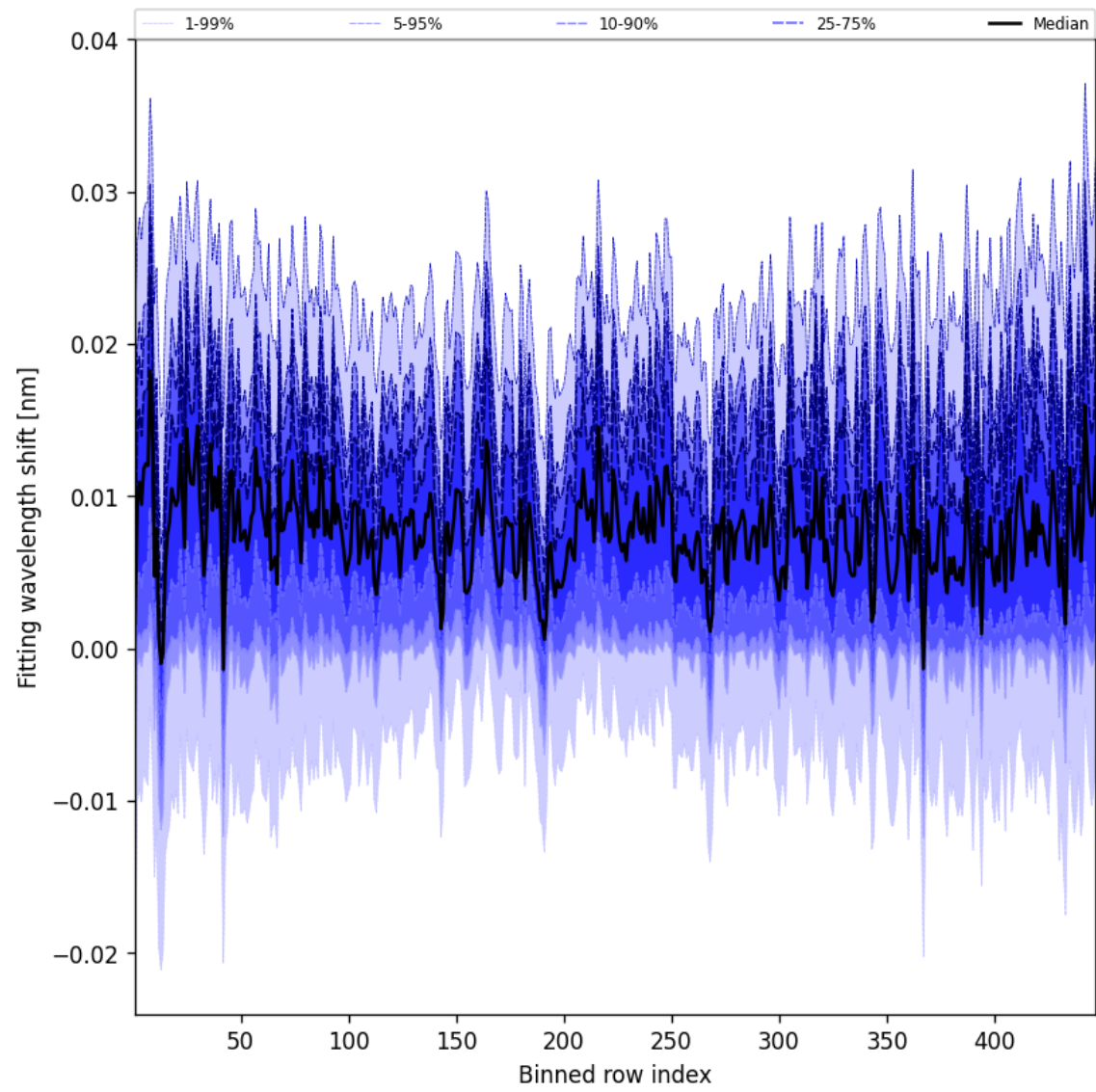
Figure 65: Along track statistics of “Fitting wavelength shift” for 2025-03-25 to 2025-03-27
