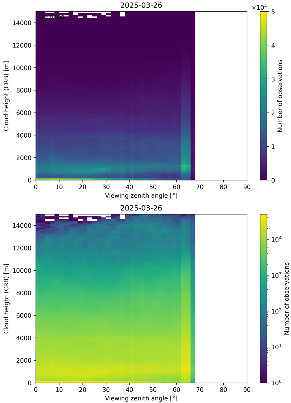
Figure 110: Scatter density plot of “Viewing zenith angle” against “Cloud height (CRB)” for 2025-03-25 to 2025-03-27.
