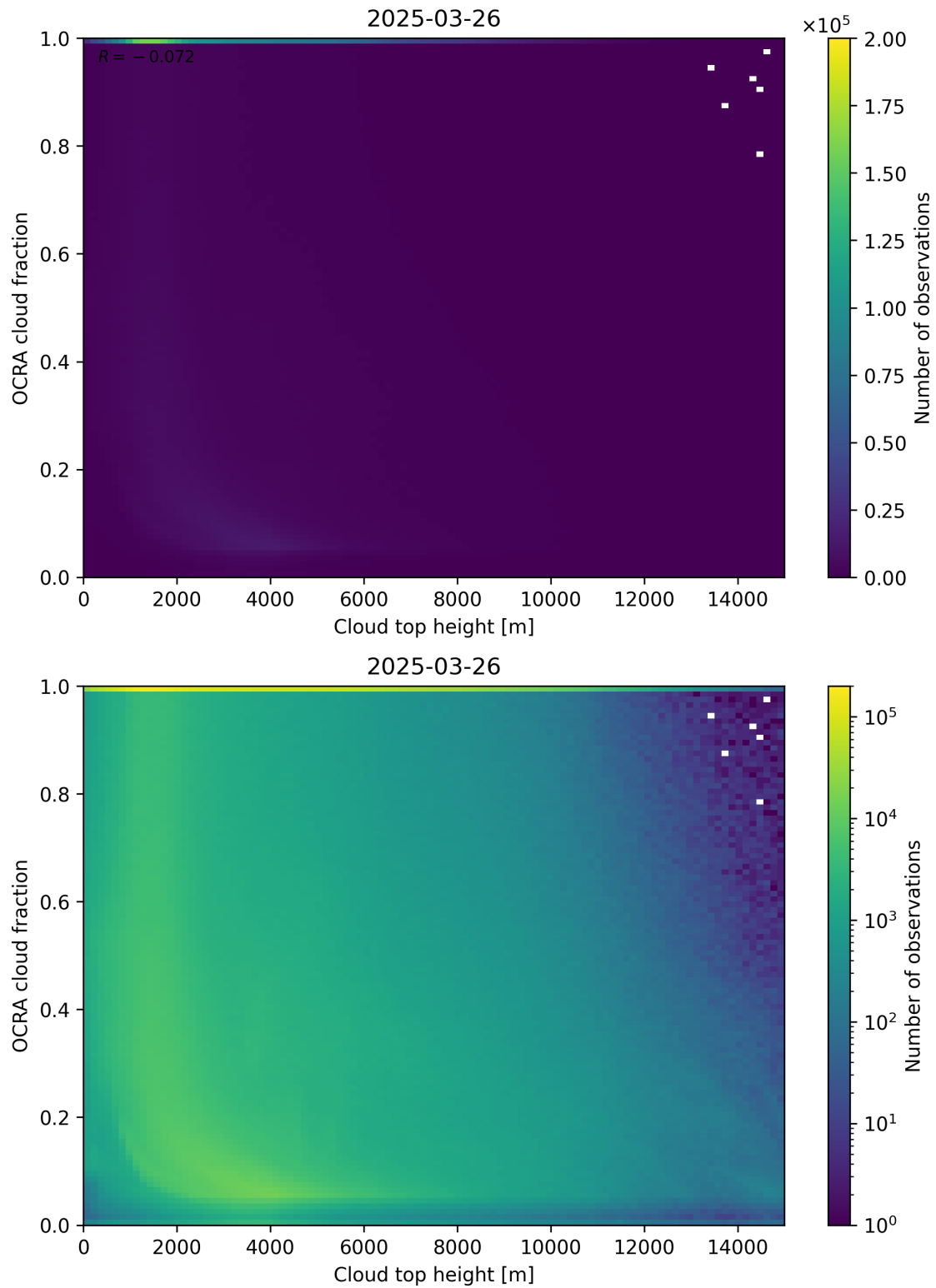
Figure 87: Scatter density plot of “Cloud top height” against “OCRA cloud fraction” for 2025-03-25 to 2025-03-27.
