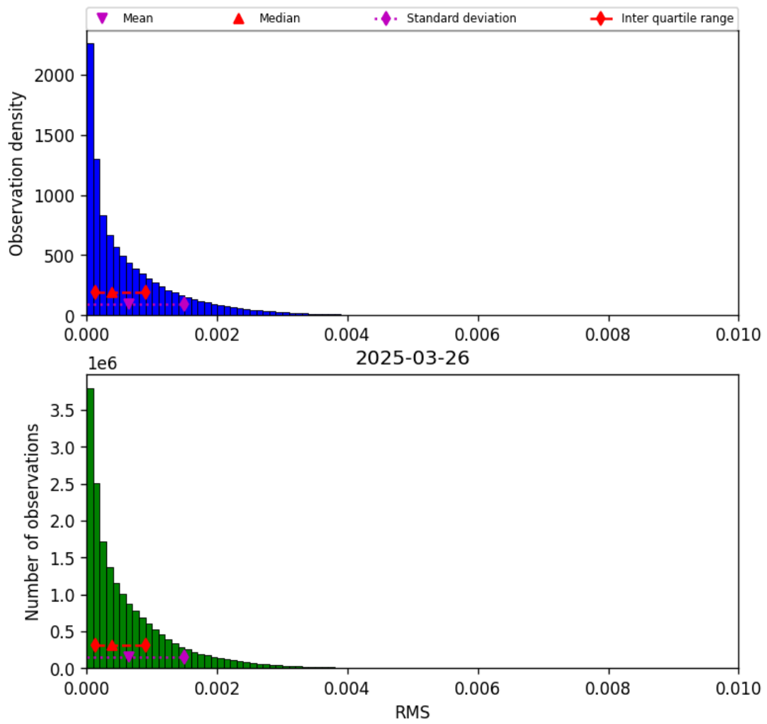
Figure 47: Histogram of “RMS” for 2025-03-25 to 2025-03-27
