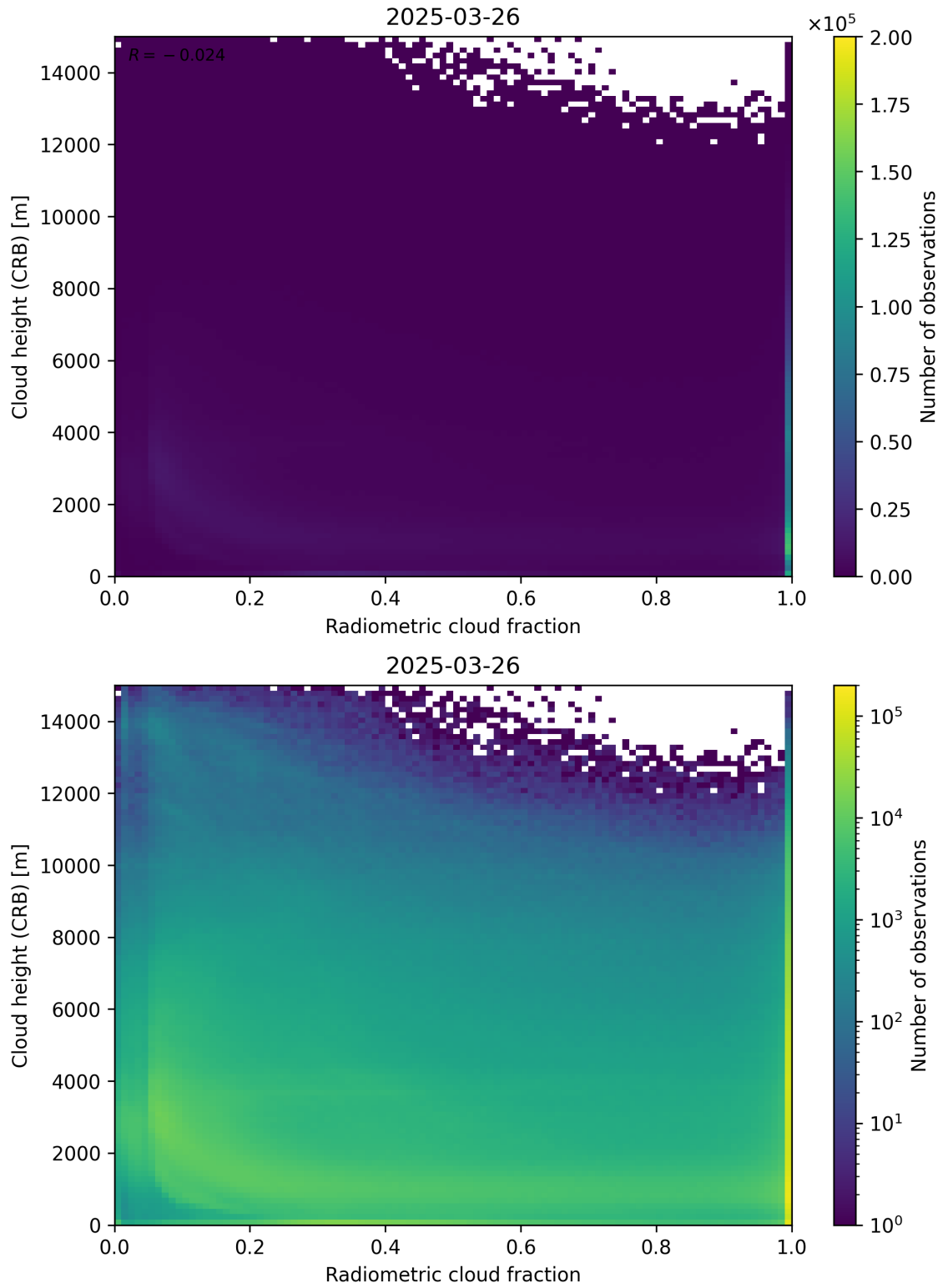
Figure 74: Scatter density plot of “Radiometric cloud fraction” against “Cloud height (CRB)” for 2025-03-25 to 2025-03-27.
