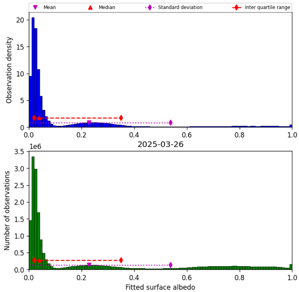
Figure 45: Histogram of “Fitted surface albedo” for 2025-03-25 to 2025-03-27
