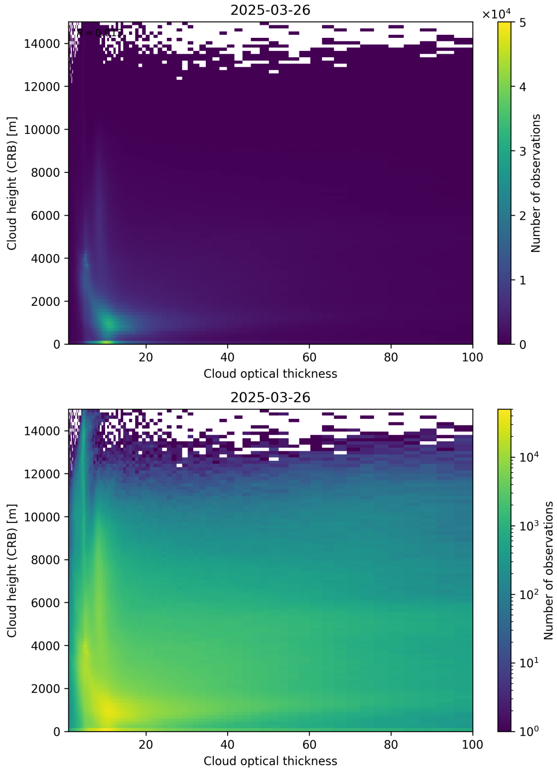
Figure 85: Scatter density plot of “Cloud optical thickness” against “Cloud height (CRB)” for 2025-03-25 to 2025-03-27.
