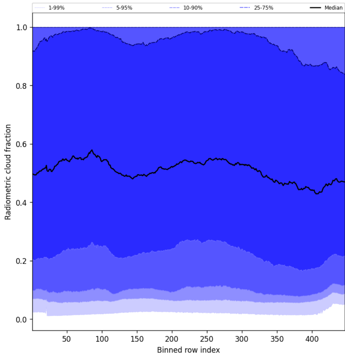
Figure 55: Along track statistics of “Radiometric cloud fraction” for 2025-03-25 to 2025-03-27
