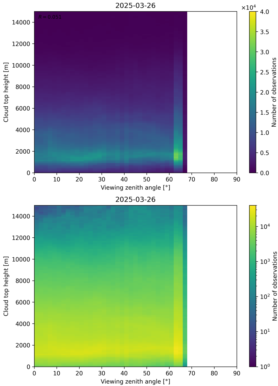
Figure 112: Scatter density plot of “Viewing zenith angle” against “Cloud top height” for 2025-03-25 to 2025-03-27.
