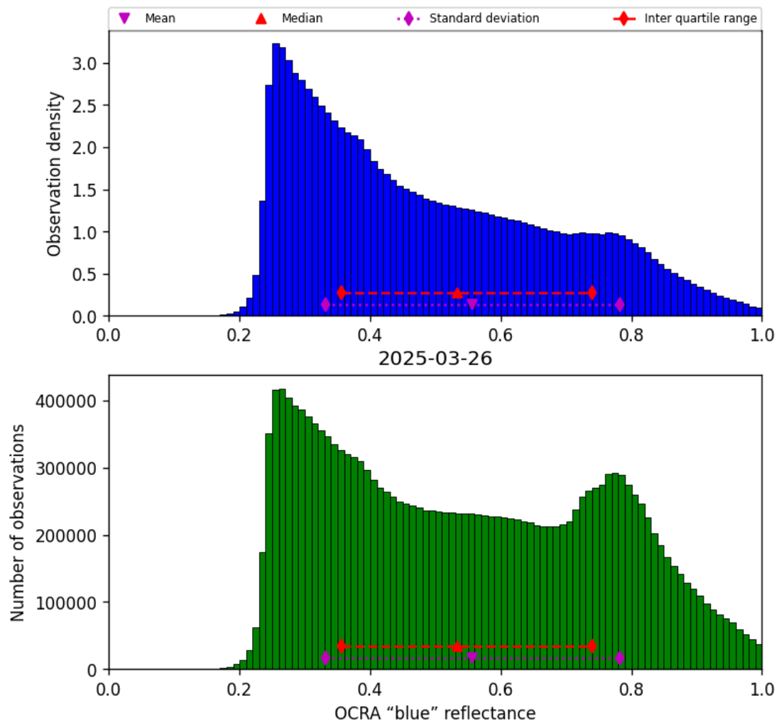
Figure 51: Histogram of “OCRA “blue” reflectance” for 2025-03-25 to 2025-03-27
