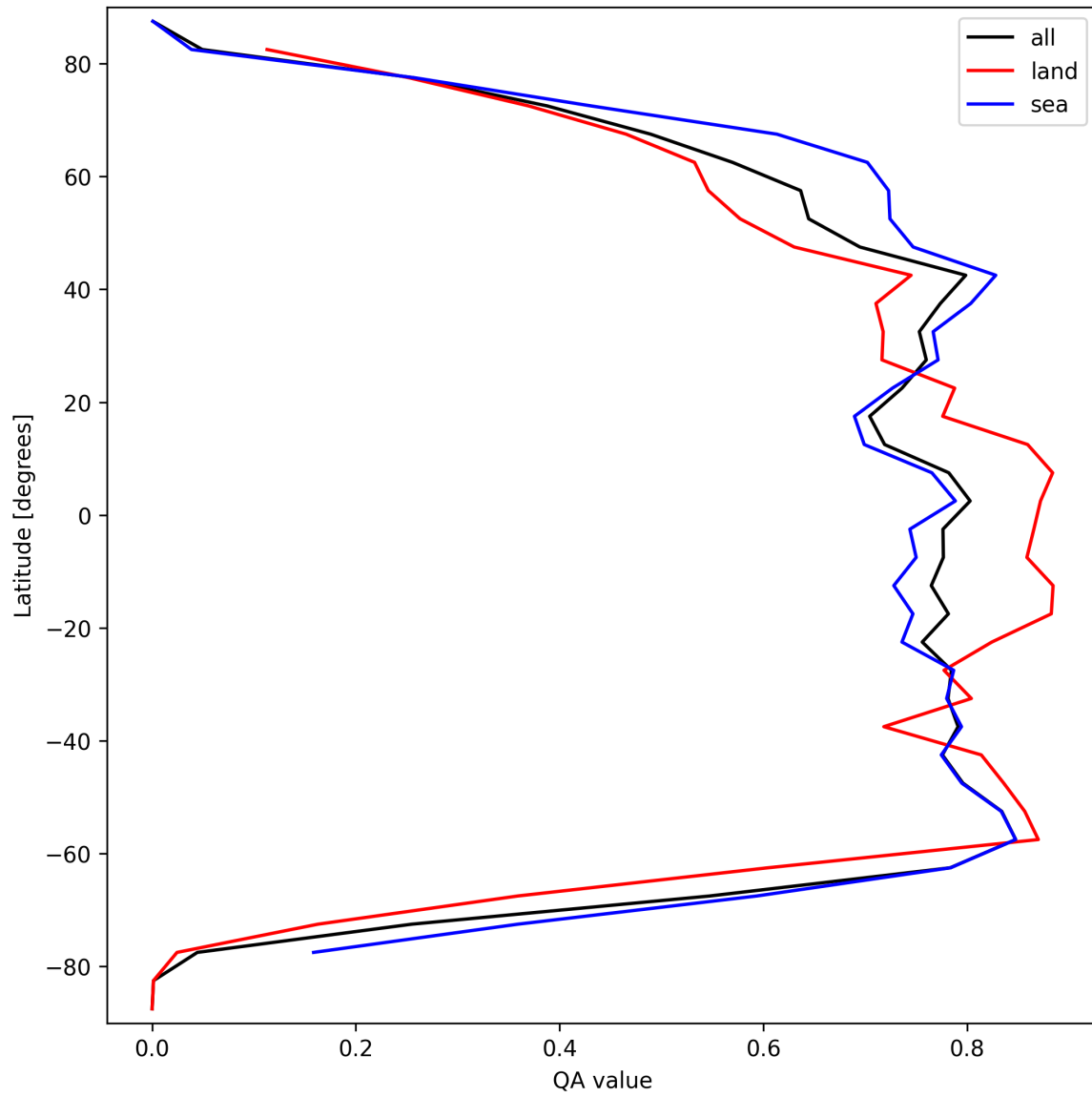
Figure 22: Zonal average of “QA value” for 2025-03-25 to 2025-03-27.
