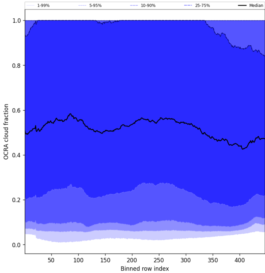
Figure 66: Along track statistics of “OCRA cloud fraction” for 2025-03-25 to 2025-03-27
