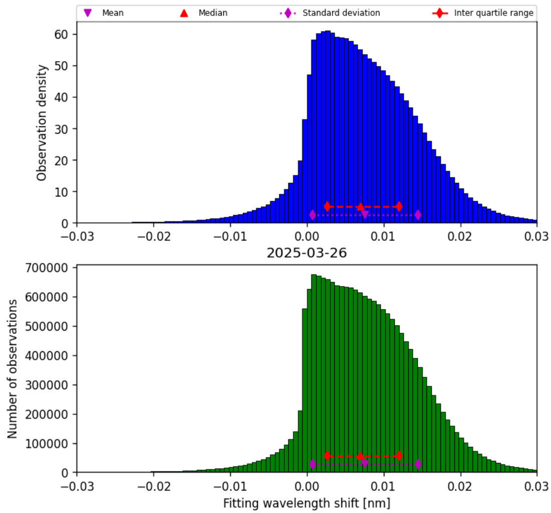
Figure 49: Histogram of “Fitting wavelength shift” for 2025-03-25 to 2025-03-27
