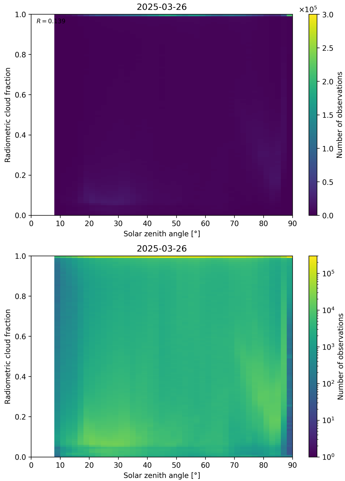
Figure 99: Scatter density plot of “Solar zenith angle” against “Radiometric cloud fraction” for 2025-03-25 to 2025-03-27.
