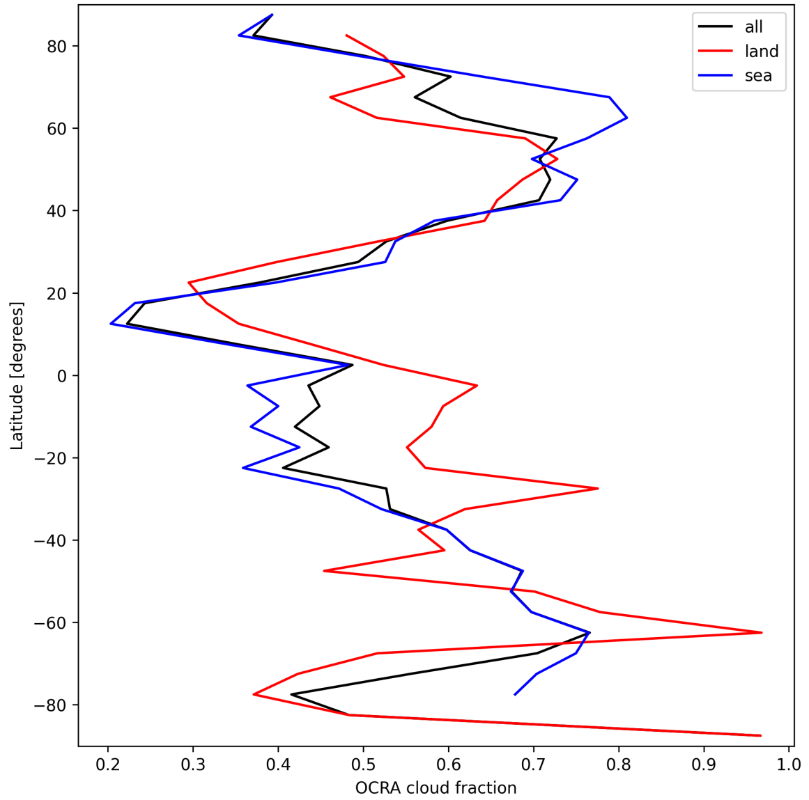
Figure 34: Zonal average of “OCRA cloud fraction” for 2025-03-25 to 2025-03-27.
