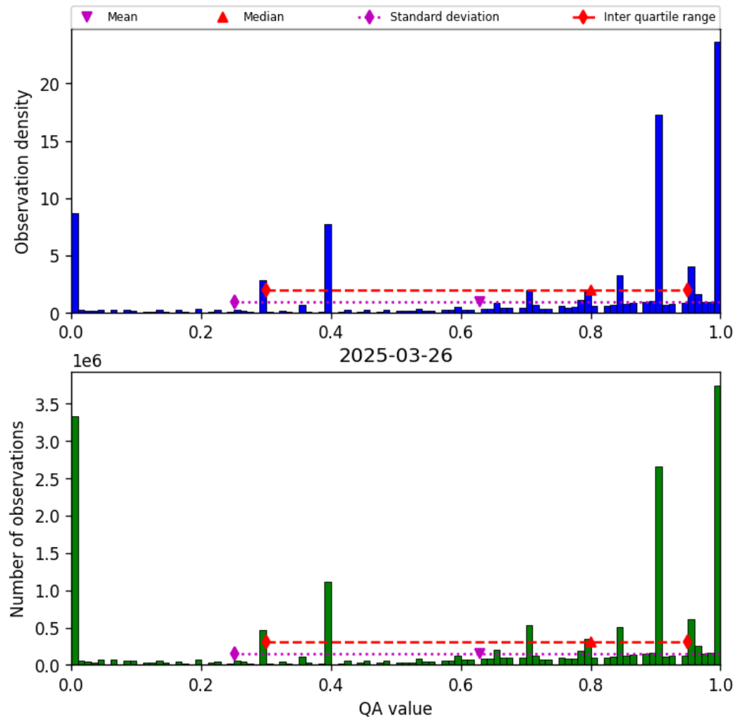
Figure 38: Histogram of “QA value” for 2025-03-25 to 2025-03-27
