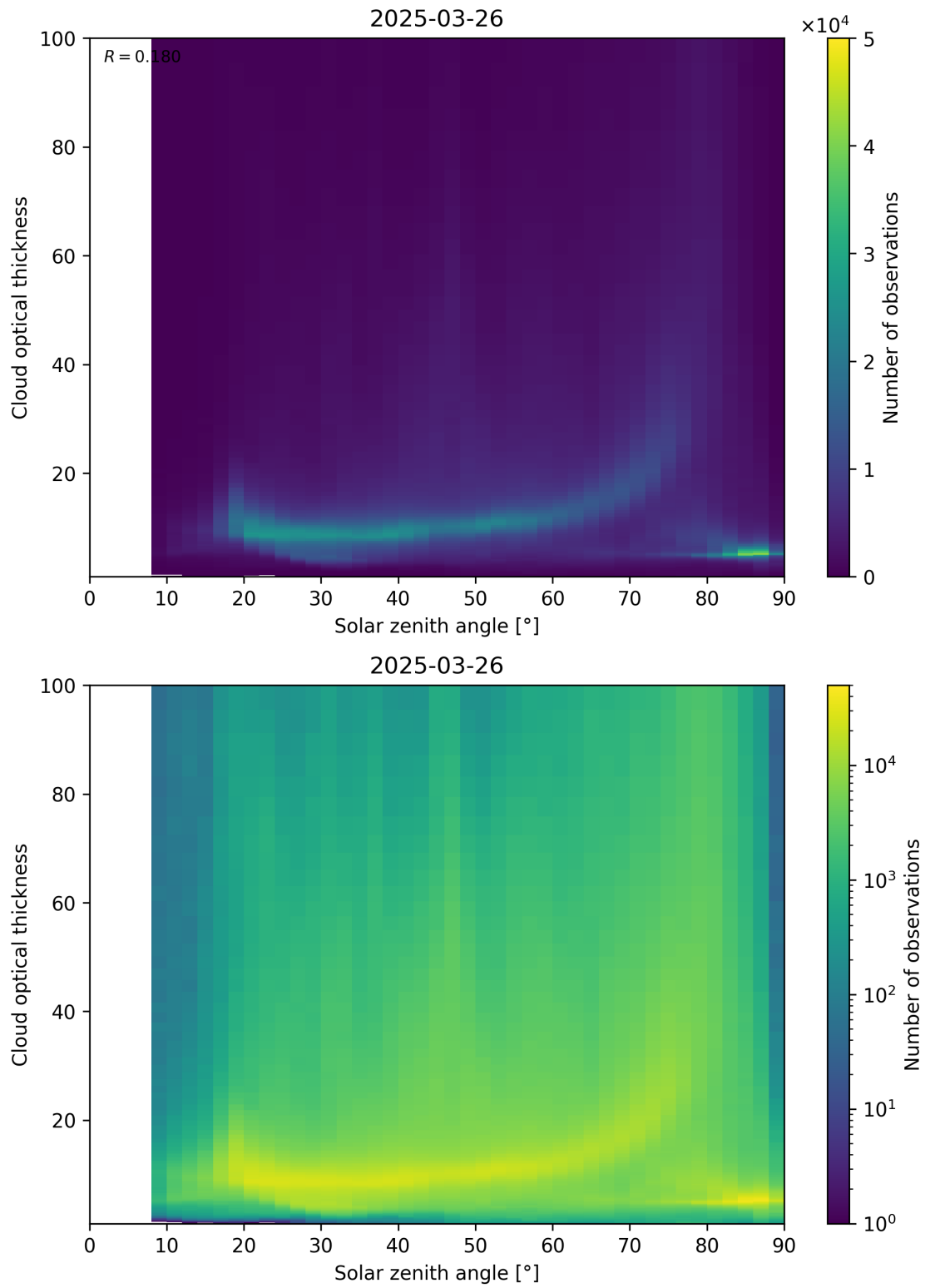
Figure 103: Scatter density plot of “Solar zenith angle” against “Cloud optical thickness” for 2025-03-25 to 2025-03-27.
