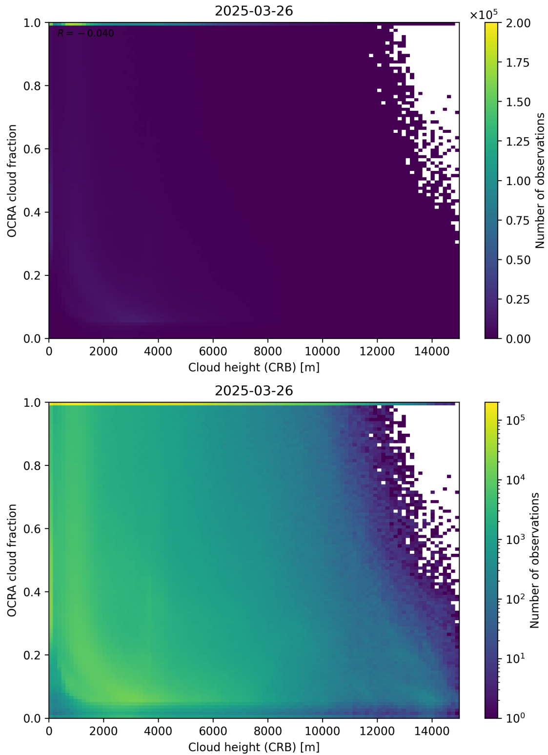
Figure 81: Scatter density plot of “Cloud height (CRB)” against “OCRA cloud fraction” for 2025-03-25 to 2025-03-27.
