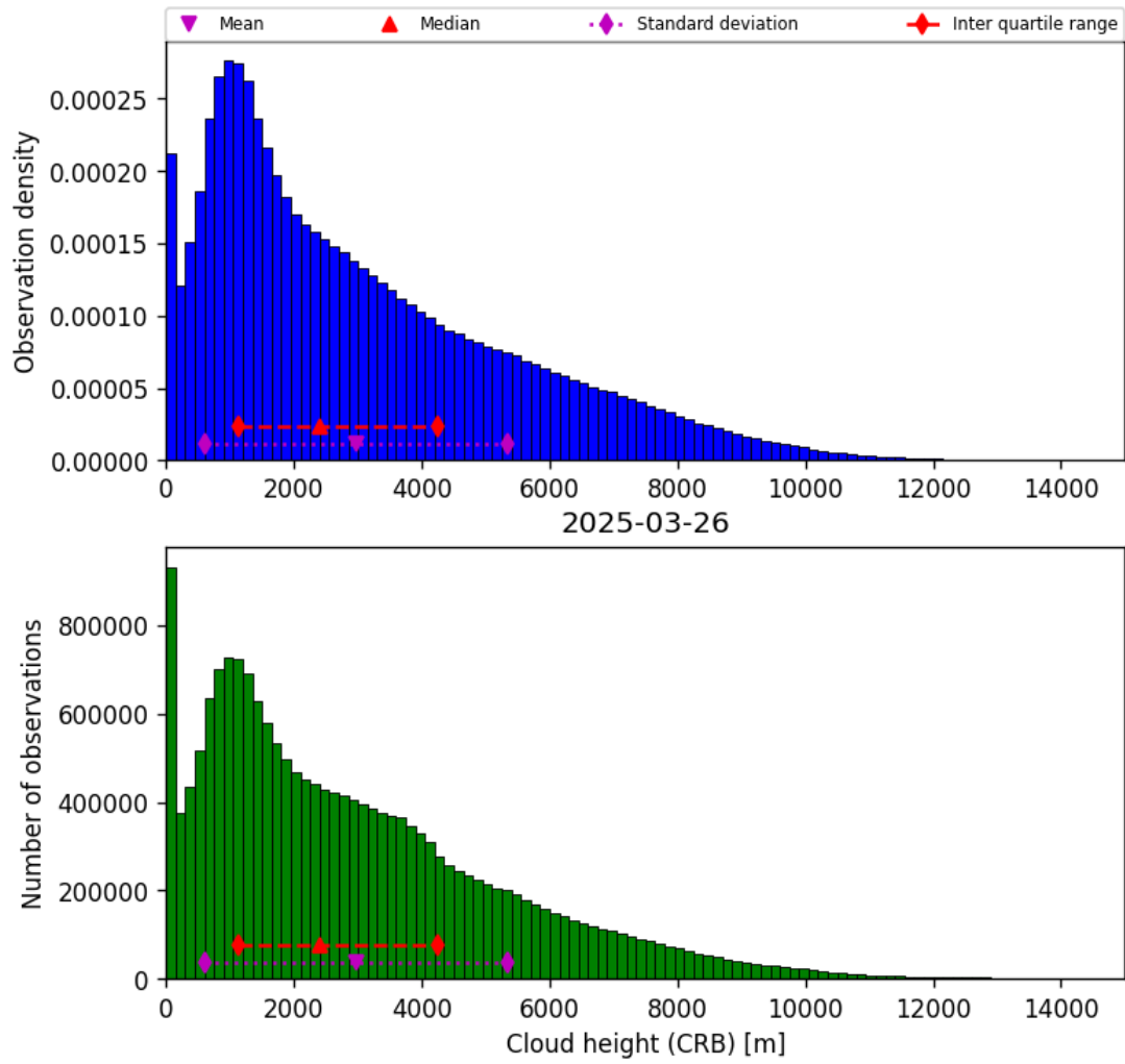
Figure 43: Histogram of “Cloud height (CRB)” for 2025-03-25 to 2025-03-27
