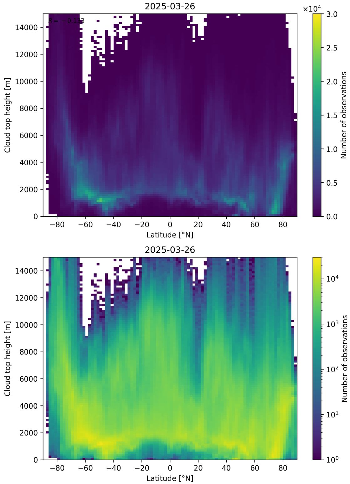
Figure 97: Scatter density plot of “Latitude” against “Cloud top height” for 2025-03-25 to 2025-03-27.
