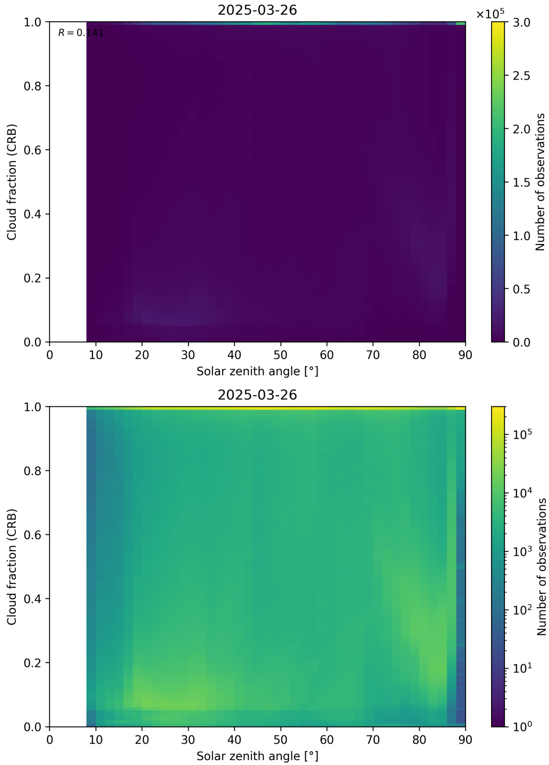
Figure 101: Scatter density plot of “Solar zenith angle” against “Cloud fraction (CRB)” for 2025-03-25 to 2025-03-27.
