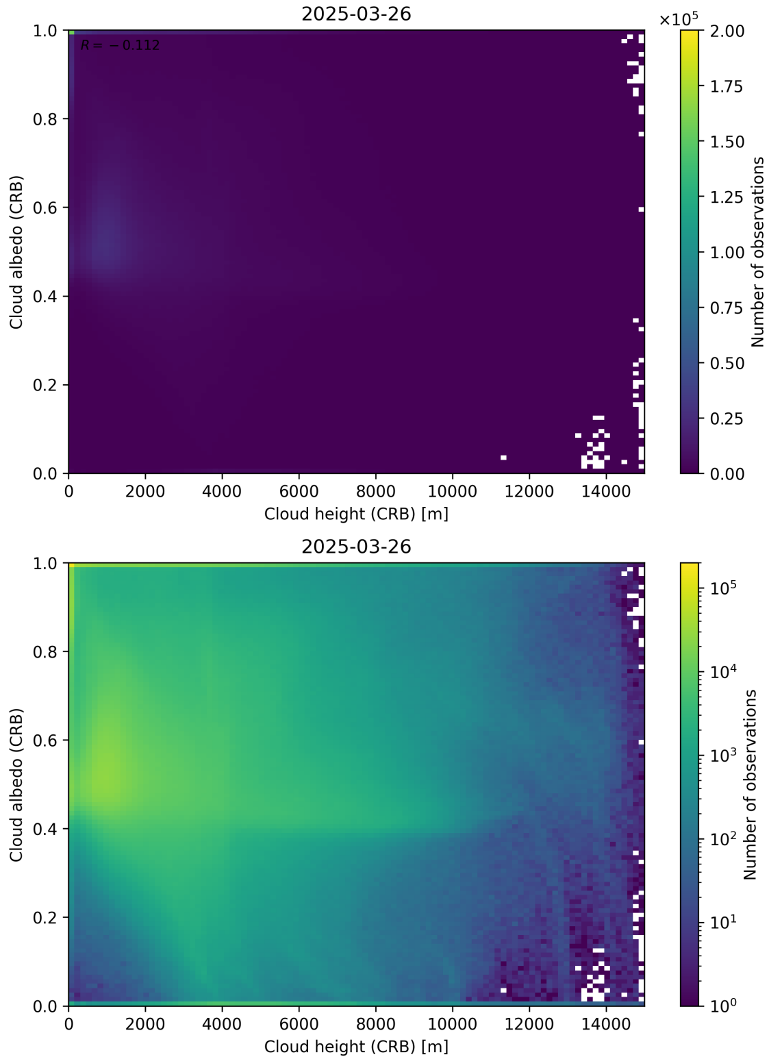
Figure 80: Scatter density plot of “Cloud height (CRB)” against “Cloud albedo (CRB)” for 2025-03-25 to 2025-03-27.
