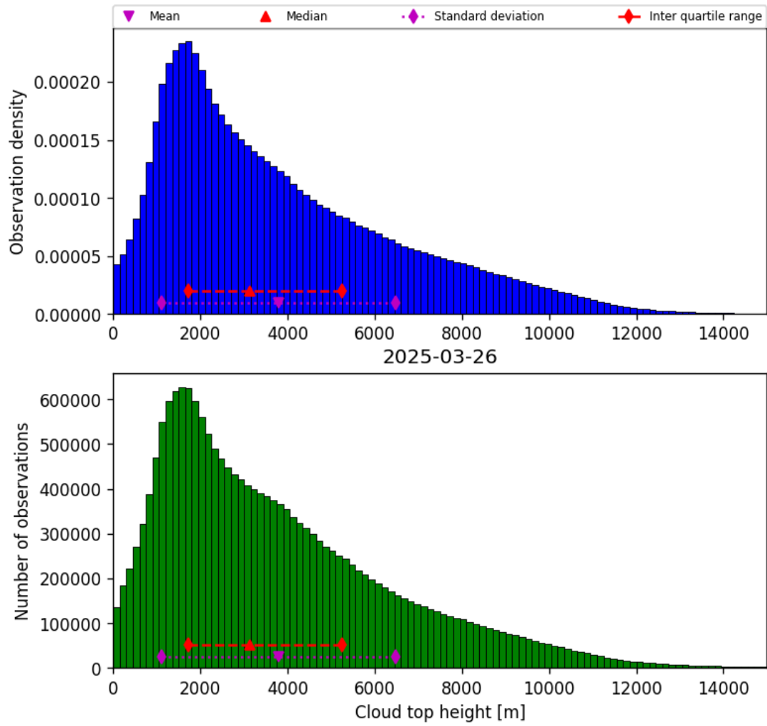
Figure 40: Histogram of “Cloud top height” for 2025-03-25 to 2025-03-27
