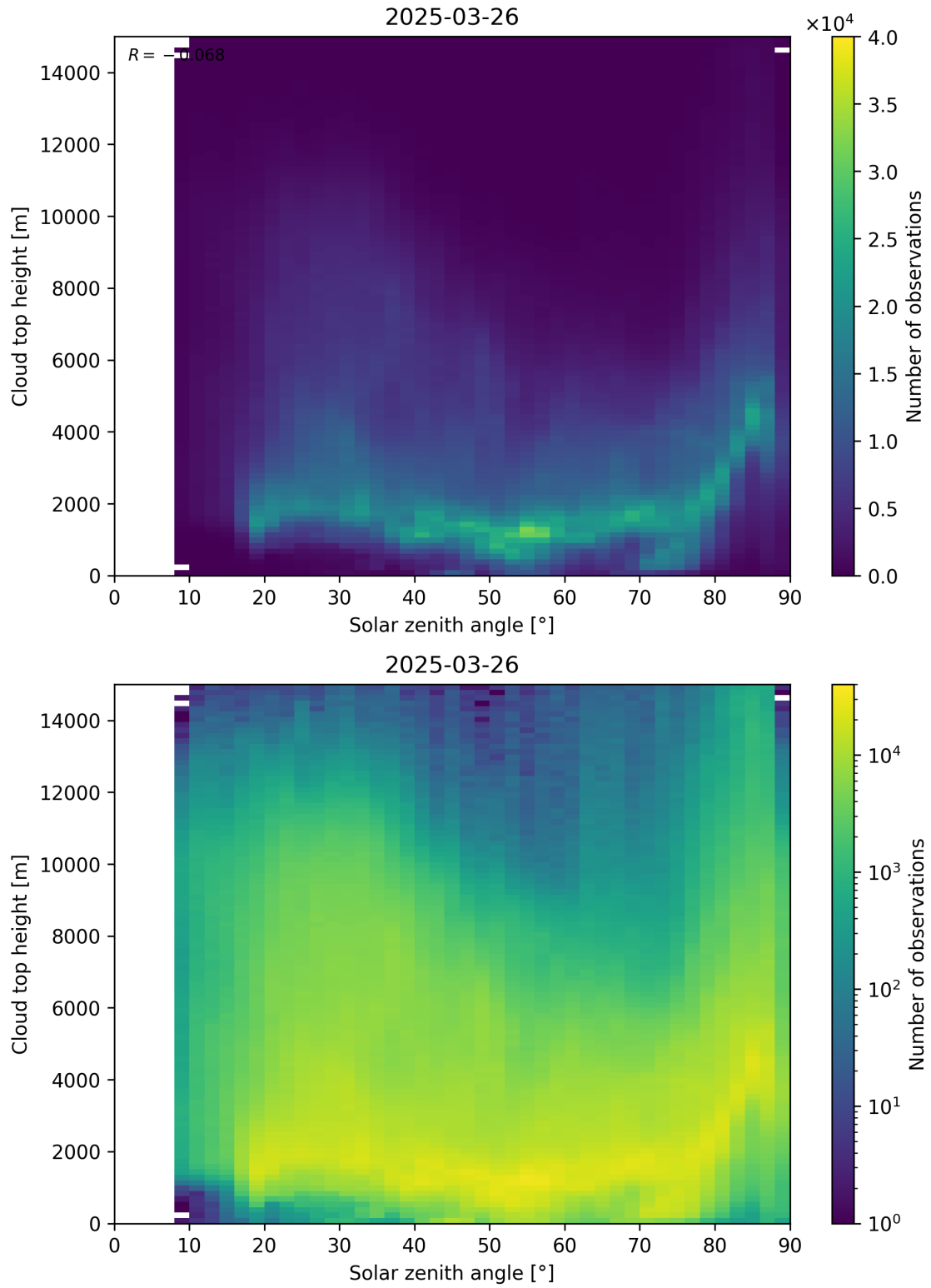
Figure 104: Scatter density plot of “Solar zenith angle” against “Cloud top height” for 2025-03-25 to 2025-03-27.
