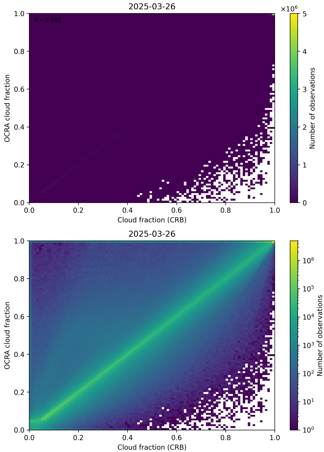
Figure 78: Scatter density plot of “Cloud fraction (CRB)” against “OCRA cloud fraction” for 2025-03-25 to 2025-03-27.
