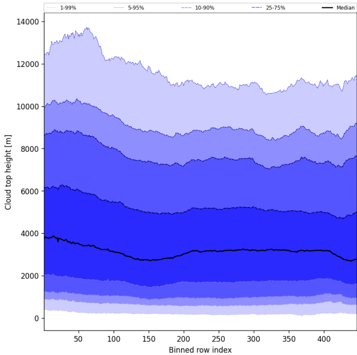
Figure 56: Along track statistics of “Cloud top height” for 2025-03-25 to 2025-03-27
