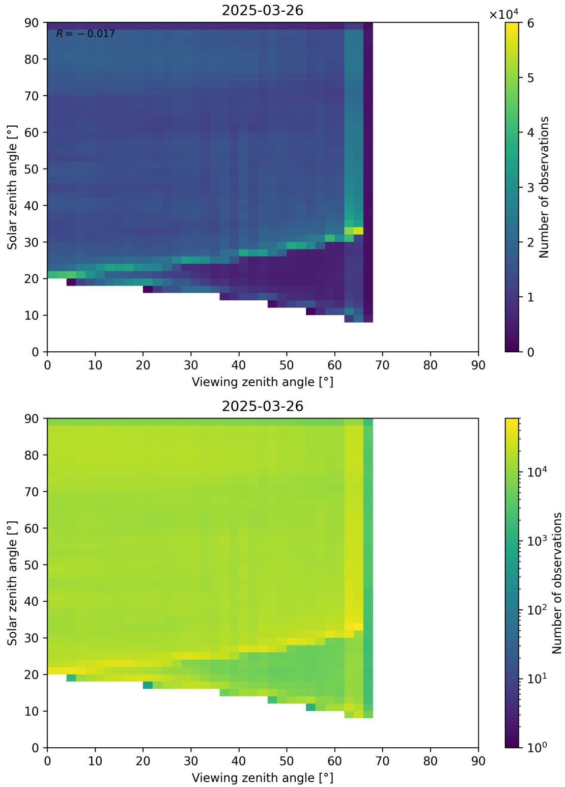
Figure 114: Scatter density plot of “Viewing zenith angle” against “Solar zenith angle” for 2025-03-25 to 2025-03-27.
