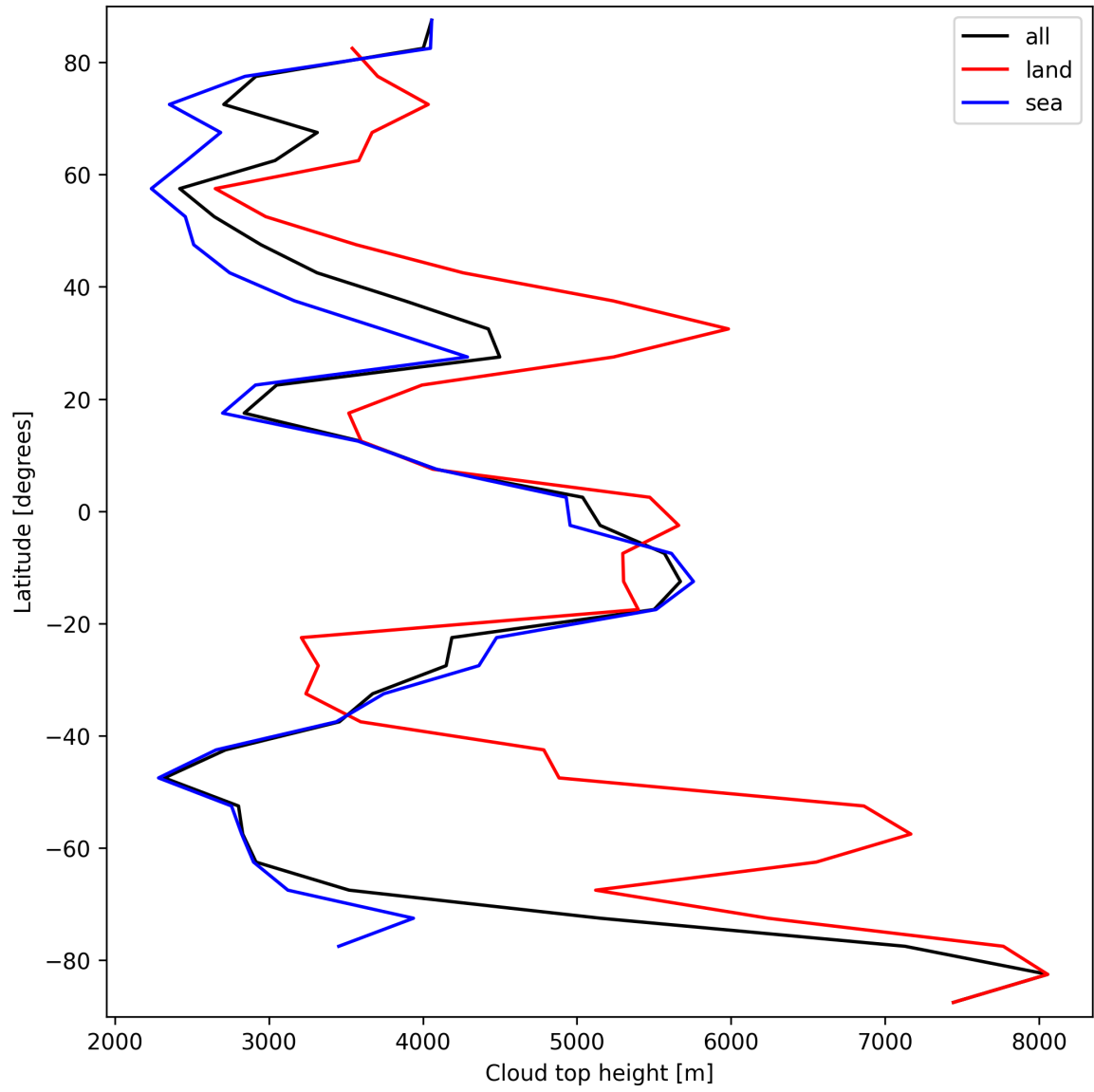
Figure 24: Zonal average of “Cloud top height” for 2025-03-25 to 2025-03-27.
