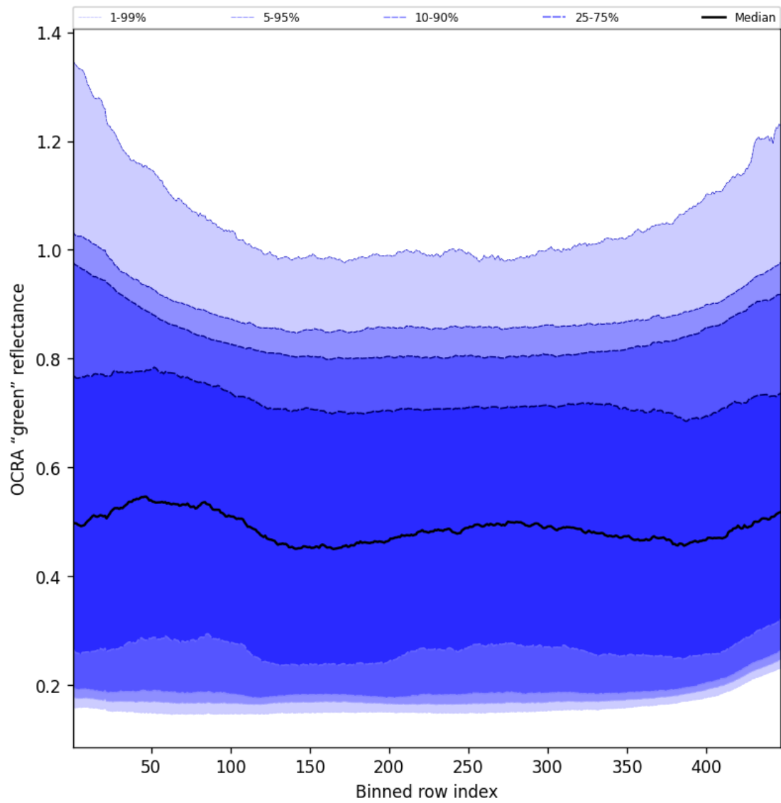
Figure 68: Along track statistics of "OCRA "green" reflectance" for 2025-03-25 to 2025-03-27
