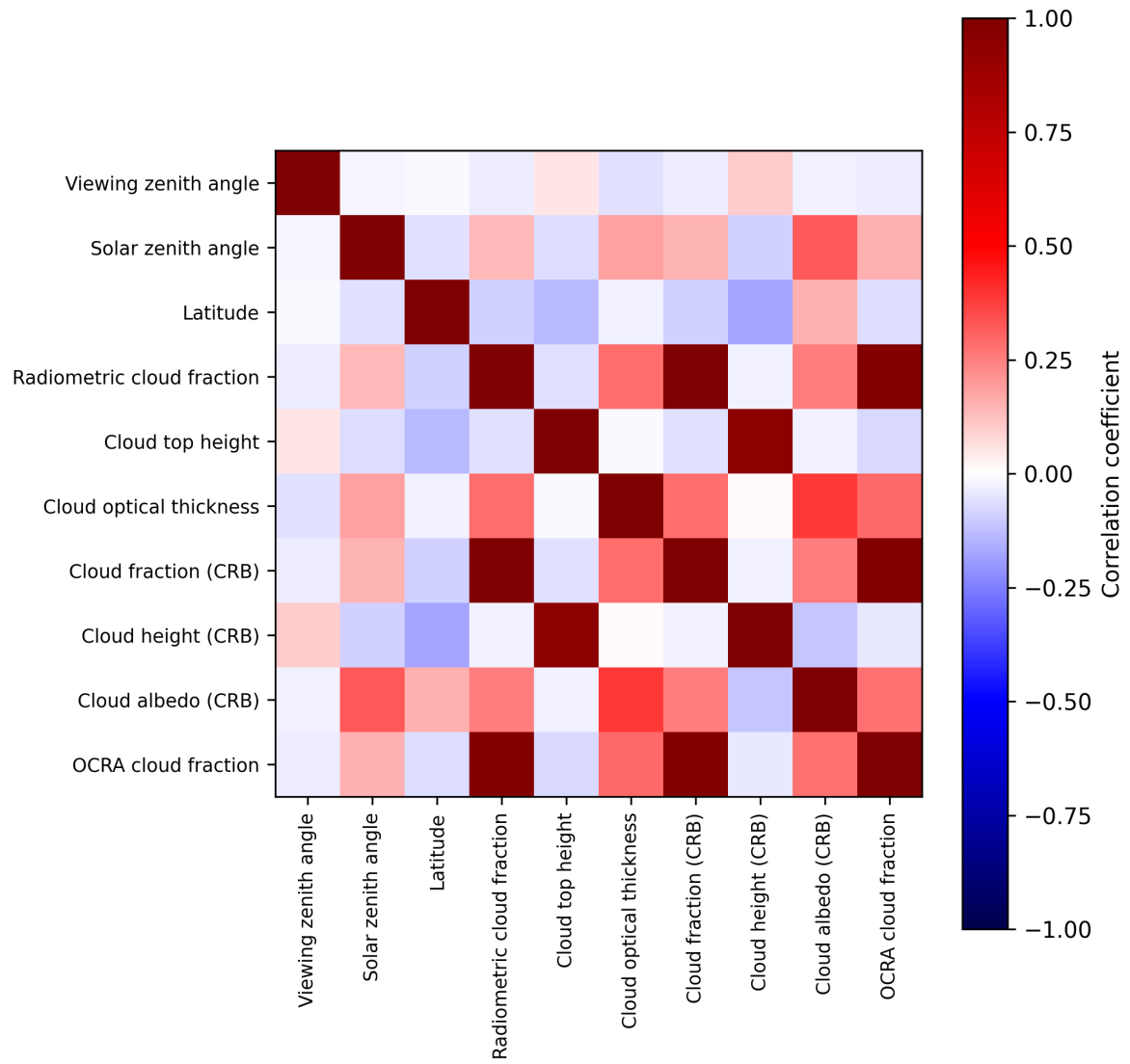
Figure 2: Map of correlation matrix for 2025-03-25 to 2025-03-27.
