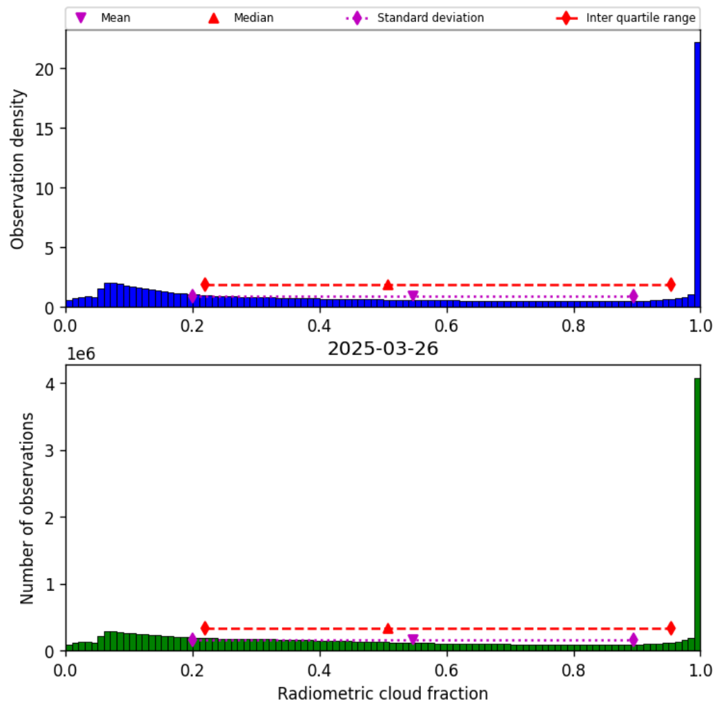
Figure 39: Histogram of "Radiometric cloud fraction" for 2025-03-25 to 2025-03-27
