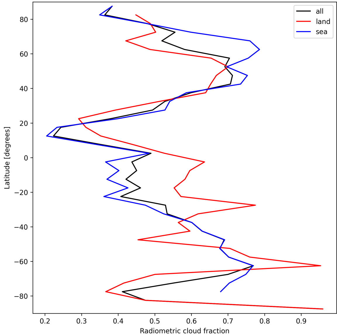
Figure 23: Zonal average of “Radiometric cloud fraction” for 2025-03-25 to 2025-03-27.
