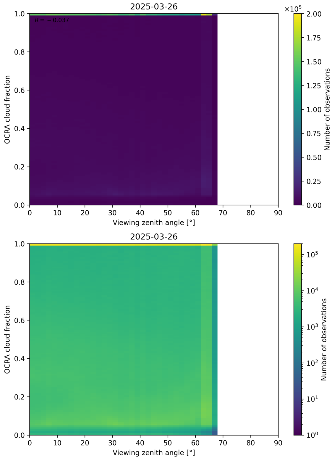
Figure 108: Scatter density plot of “Viewing zenith angle” against “OCRA cloud fraction” for 2025-03-25 to 2025-03-27.
