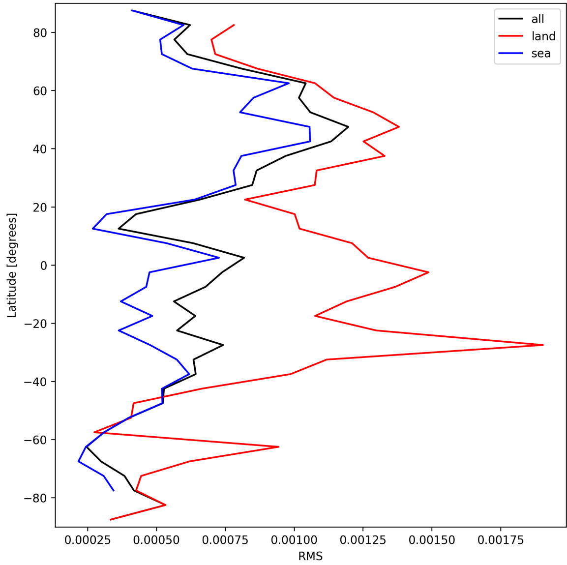
Figure 31: Zonal average of “RMS” for 2025-03-25 to 2025-03-27.
