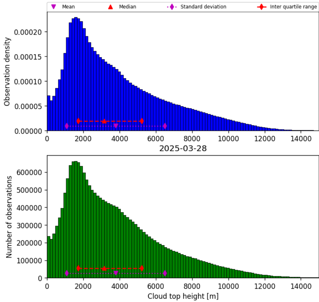
Figure 40: Histogram of “Cloud top height” for 2025-03-28 to 2025-03-29
