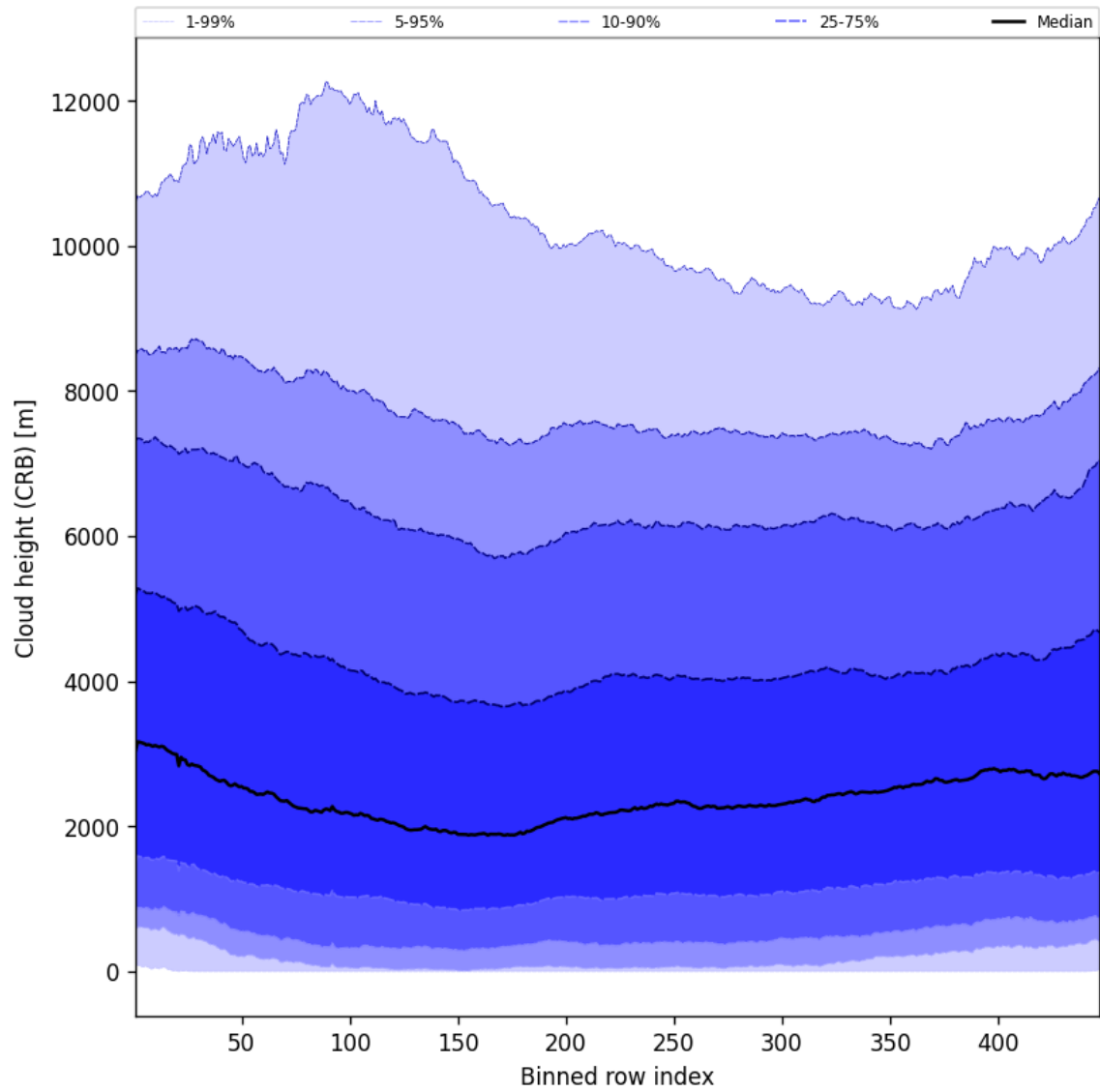
Figure 59: Along track statistics of “Cloud height (CRB)” for 2025-03-28 to 2025-03-29
