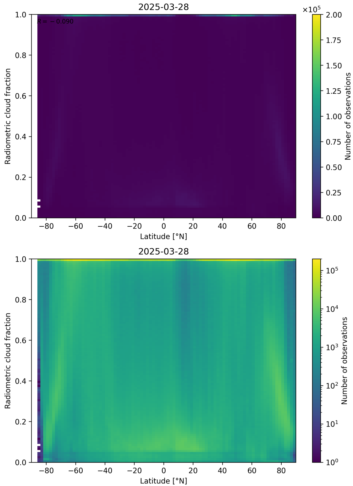
Figure 92: Scatter density plot of “Latitude” against “Radiometric cloud fraction” for 2025-03-28 to 2025-03-29.
