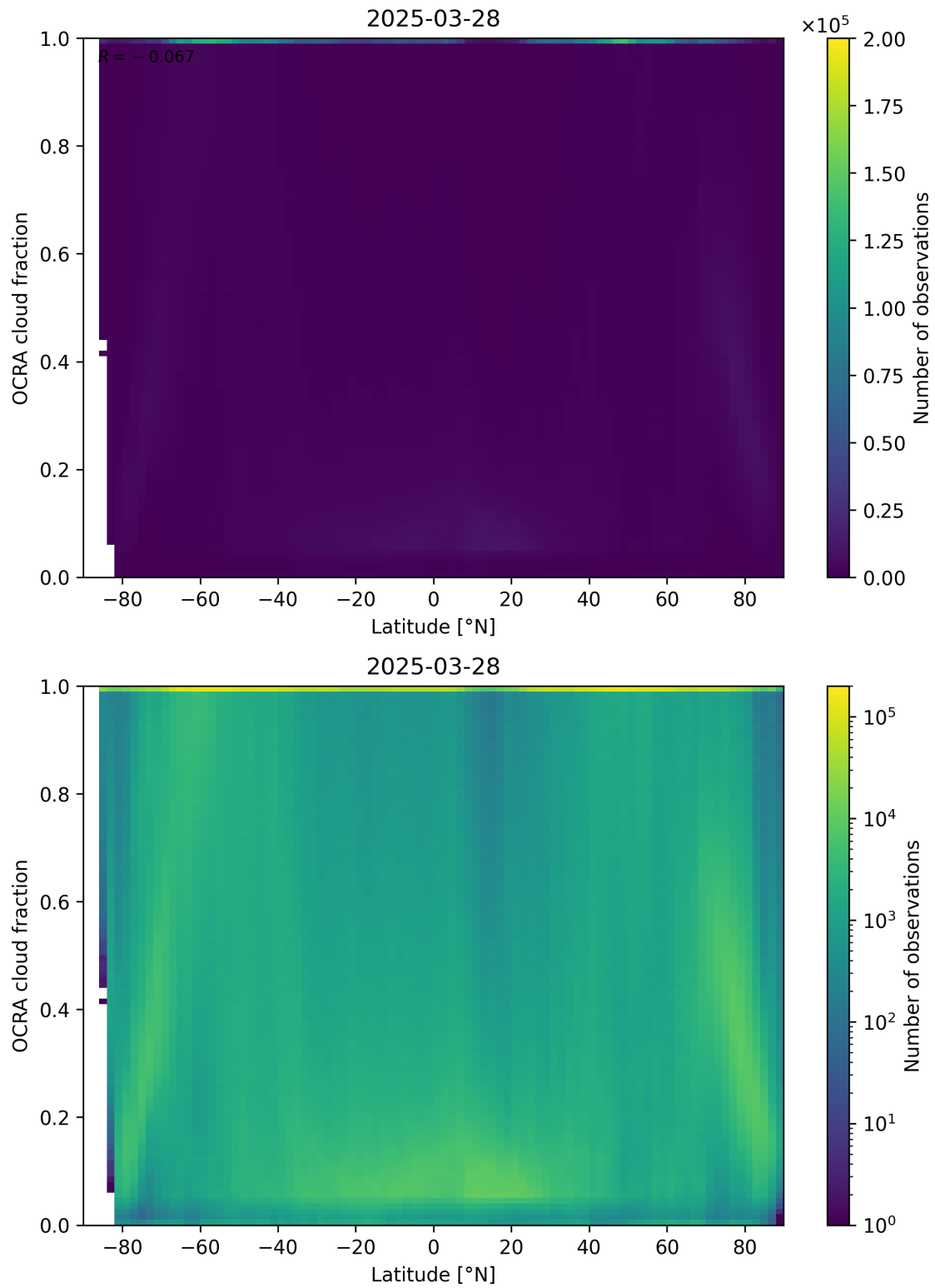
Figure 93: Scatter density plot of “Latitude” against “OCRA cloud fraction” for 2025-03-28 to 2025-03-29.
