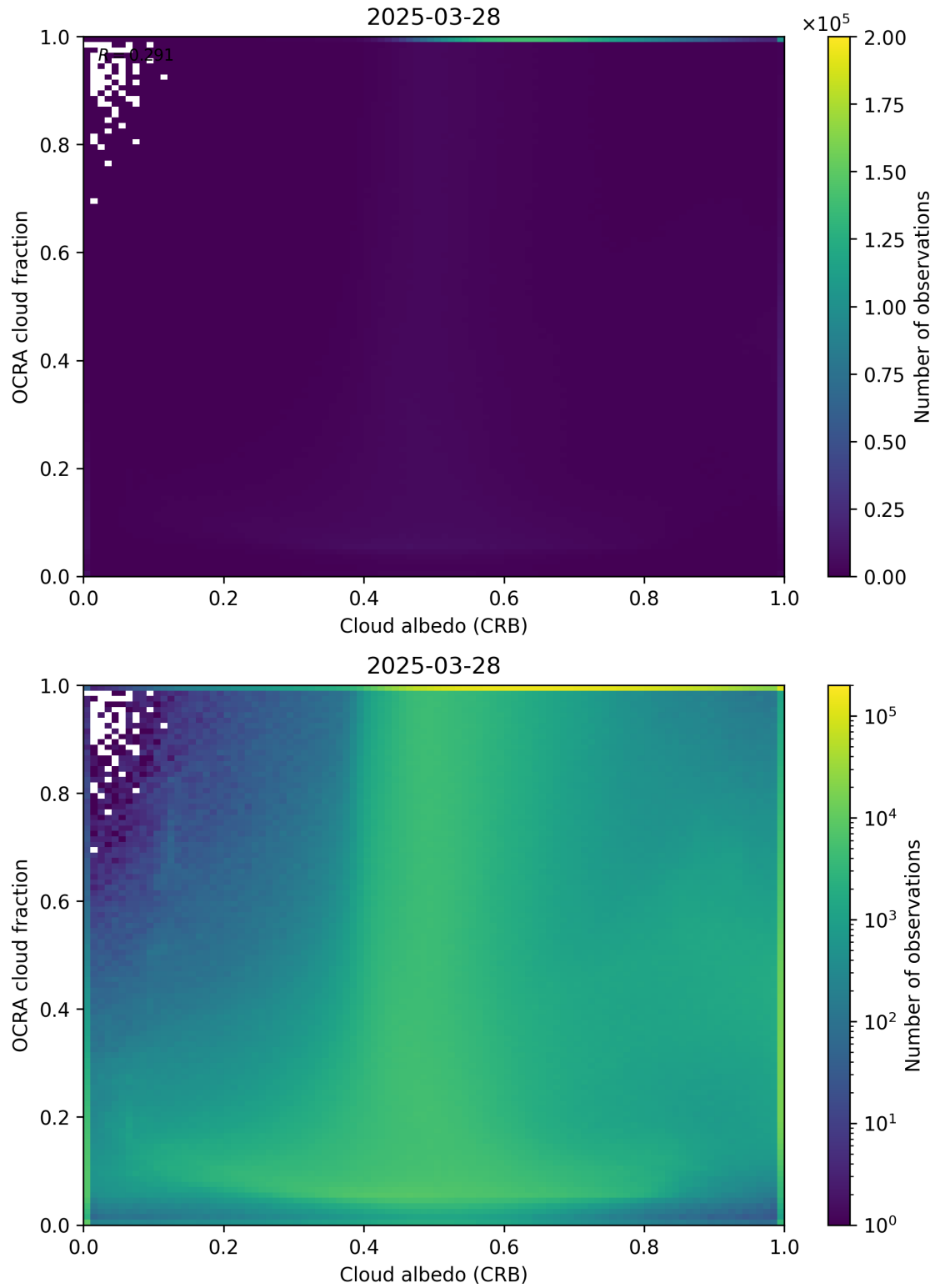
Figure 70: Scatter density plot of “Cloud albedo (CRB)” against “OCRA cloud fraction” for 2025-03-28 to 2025-03-29.
