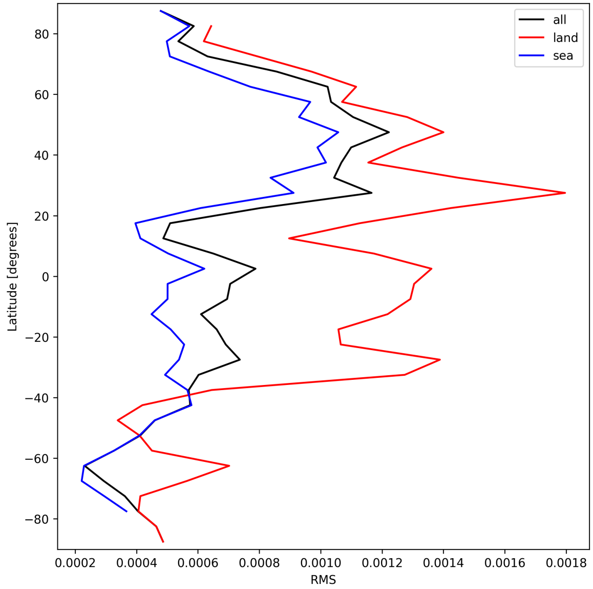
Figure 31: Zonal average of “RMS” for 2025-03-28 to 2025-03-29.
