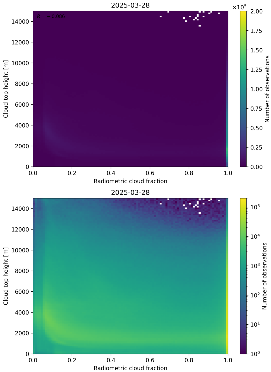
Figure 76: Scatter density plot of “Radiometric cloud fraction” against “Cloud top height” for 2025-03-28 to 2025-03-29.
