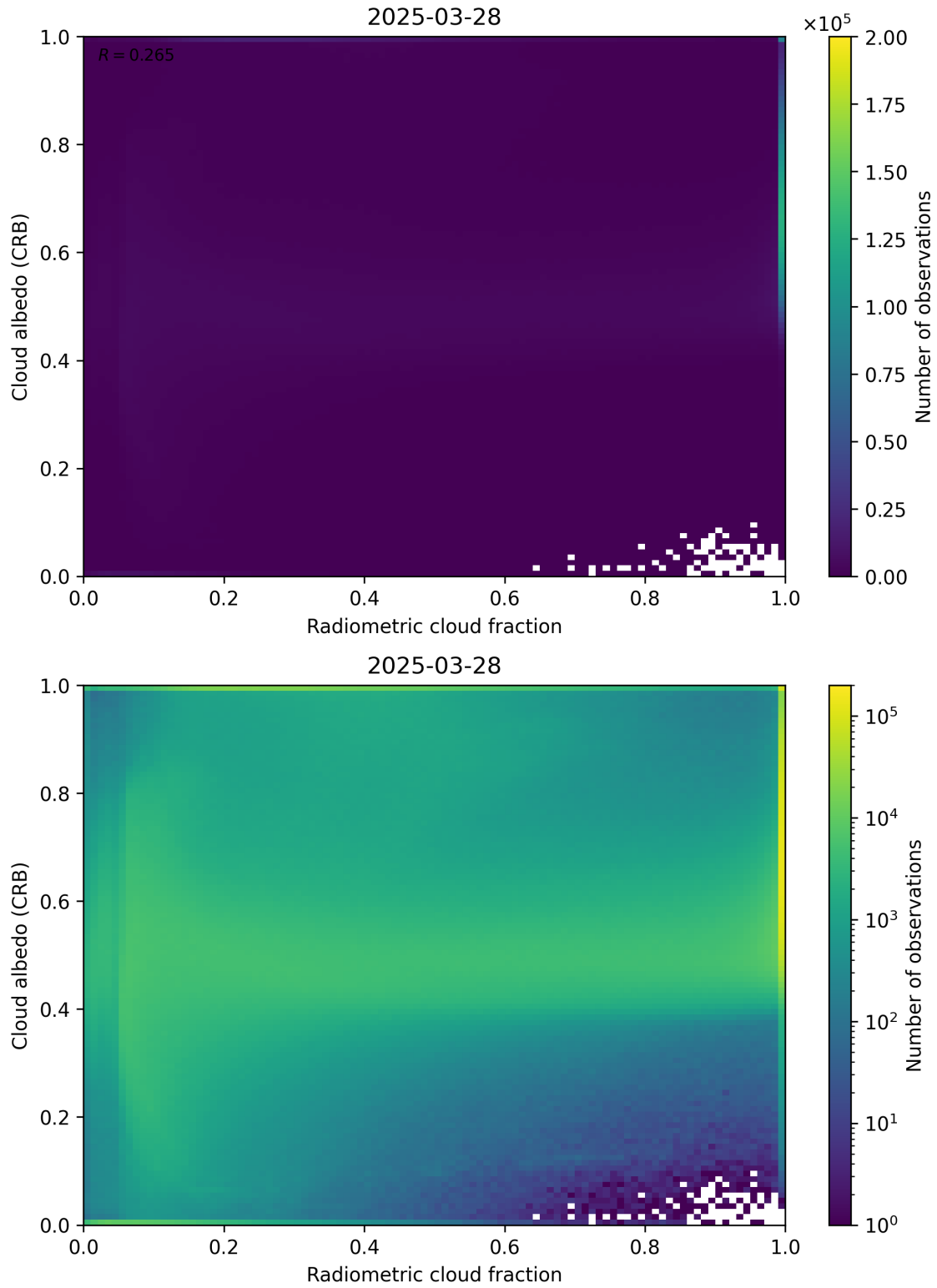
Figure 71: Scatter density plot of “Radiometric cloud fraction” against “Cloud albedo (CRB)” for 2025-03-28 to 2025-03-29.
