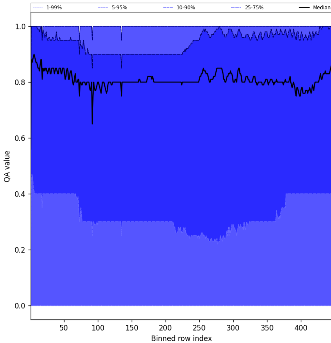
Figure 54: Along track statistics of “QA value” for 2025-03-28 to 2025-03-29
