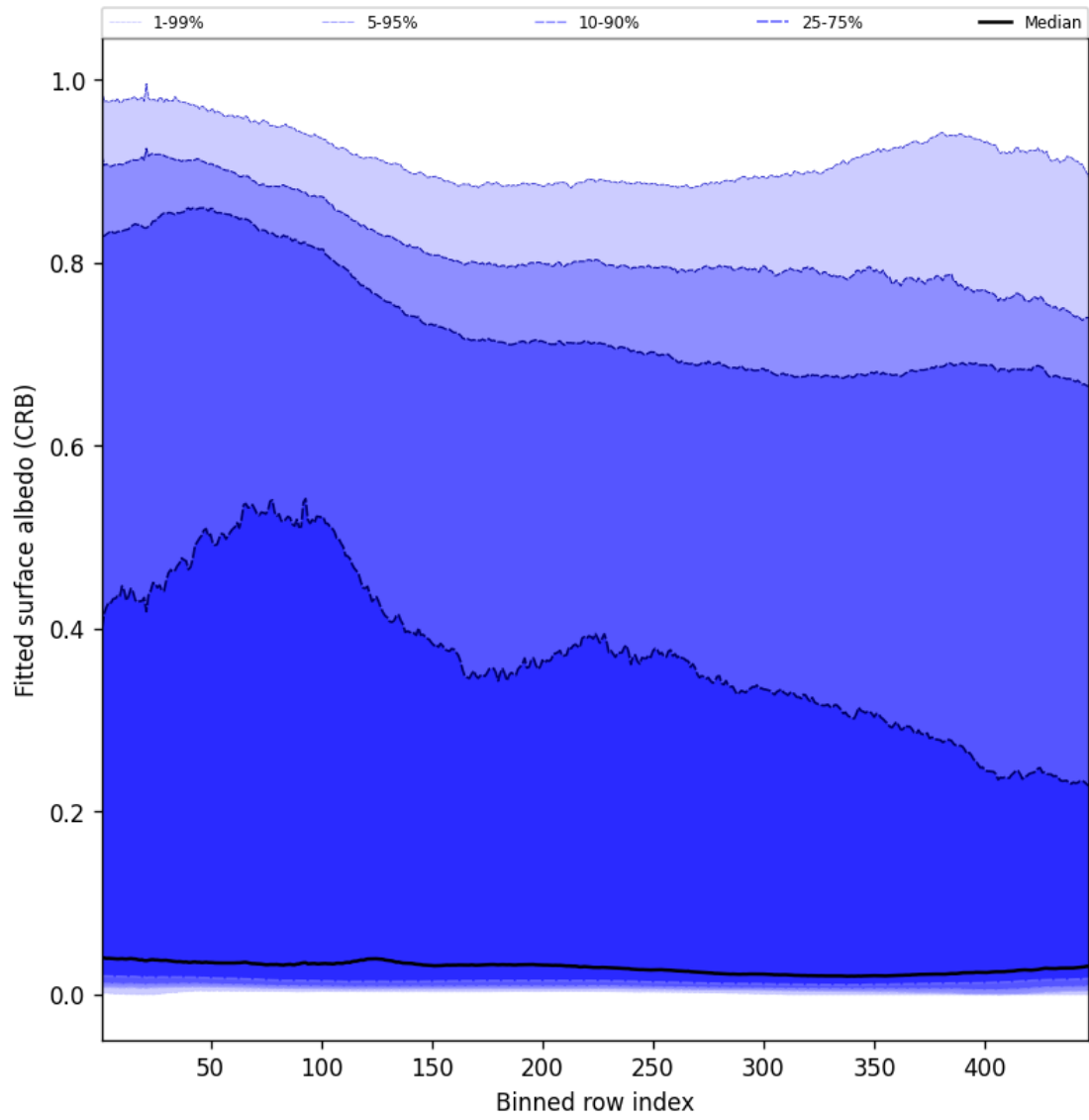
Figure 62: Along track statistics of “Fitted surface albedo (CRB)” for 2025-03-28 to 2025-03-29
