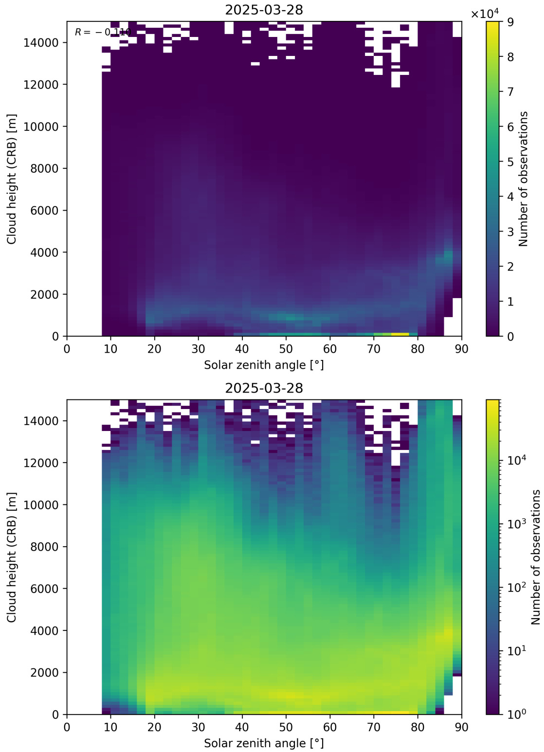
Figure 102: Scatter density plot of “Solar zenith angle” against “Cloud height (CRB)” for 2025-03-28 to 2025-03-29.
