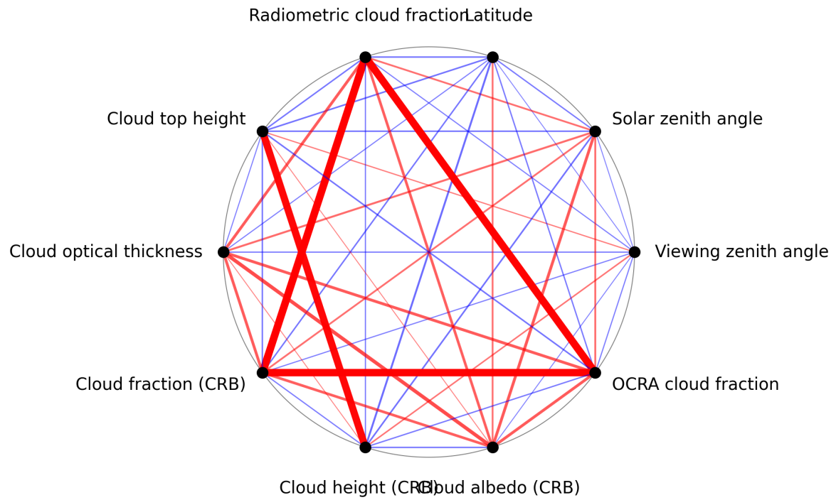
Figure 1: Map of correlation graph for 2025-03-28 to 2025-03-29.
