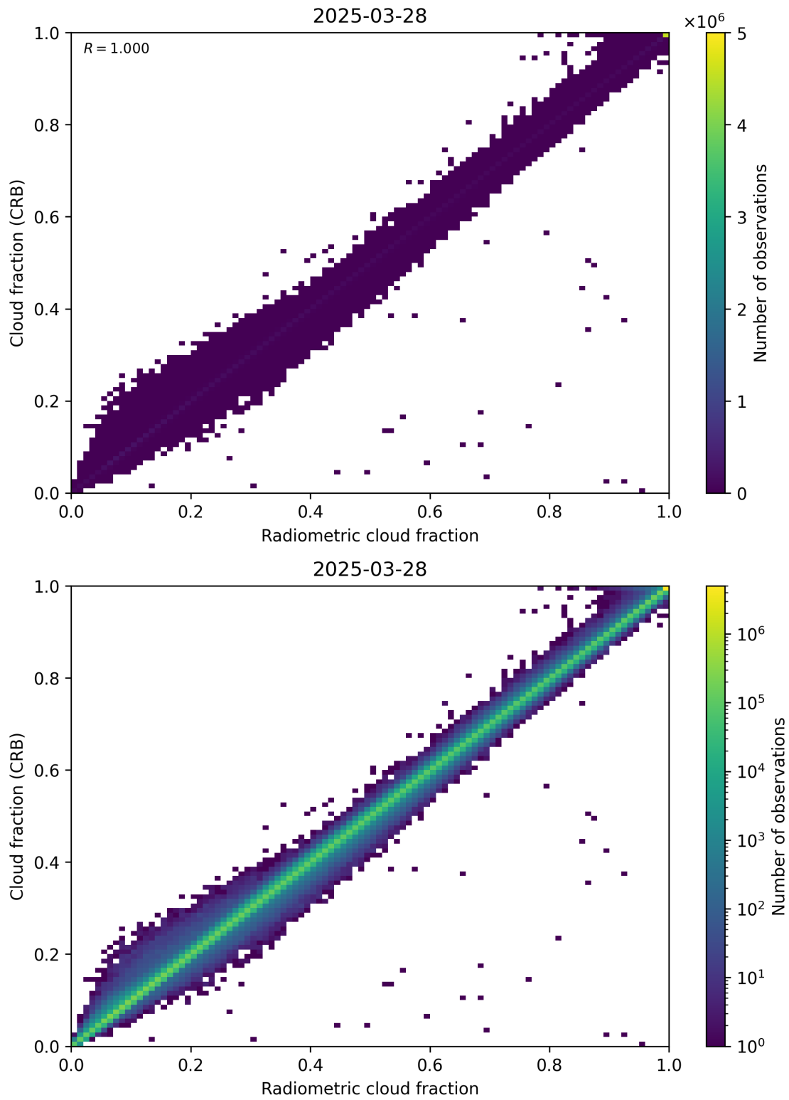
Figure 73: Scatter density plot of “Radiometric cloud fraction” against “Cloud fraction (CRB)” for 2025-03-28 to 2025-03-29.
