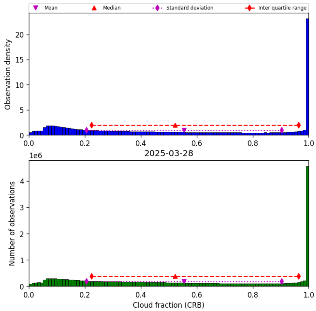
Figure 42: Histogram of “Cloud fraction (CRB)” for 2025-03-28 to 2025-03-29
