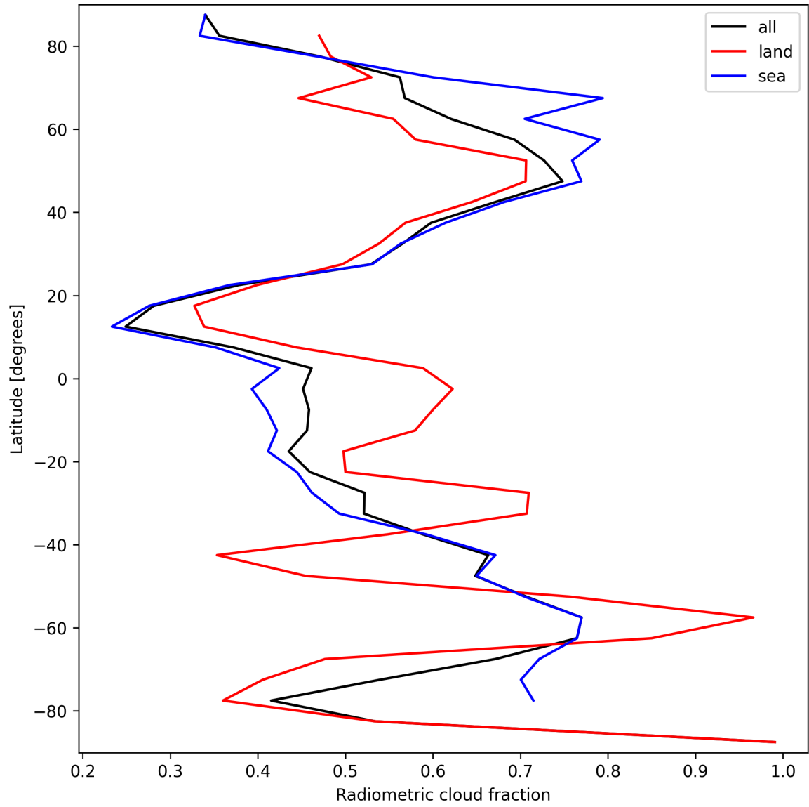
Figure 23: Zonal average of “Radiometric cloud fraction” for 2025-03-28 to 2025-03-29.
