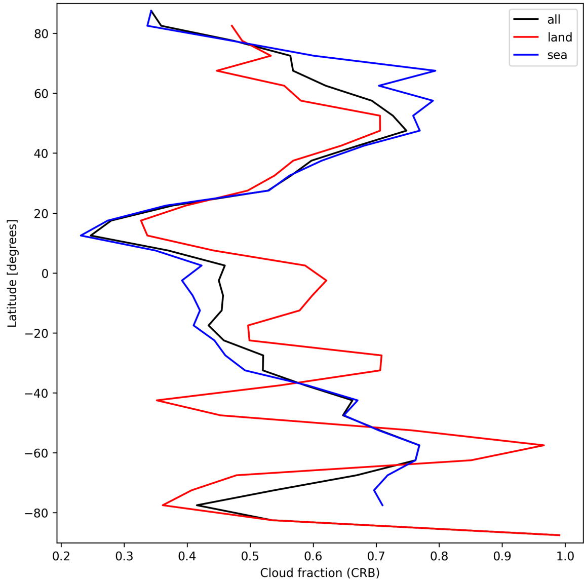
Figure 26: Zonal average of “Cloud fraction (CRB)” for 2025-03-28 to 2025-03-29.
