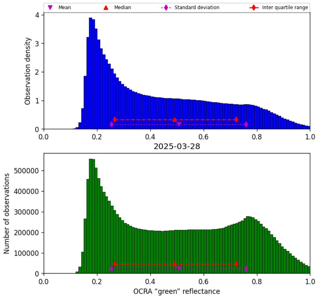
Figure 52: Histogram of “OCRA “green” reflectance” for 2025-03-28 to 2025-03-29
