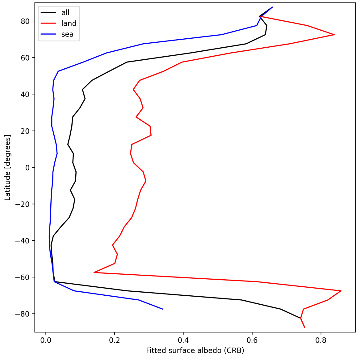
Figure 30: Zonal average of “Fitted surface albedo (CRB)” for 2025-03-28 to 2025-03-29.
