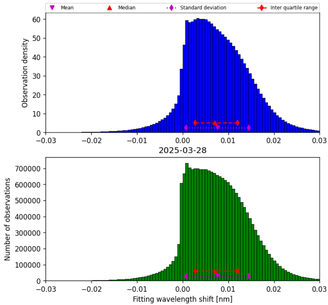
Figure 49: Histogram of “Fitting wavelength shift” for 2025-03-28 to 2025-03-29
