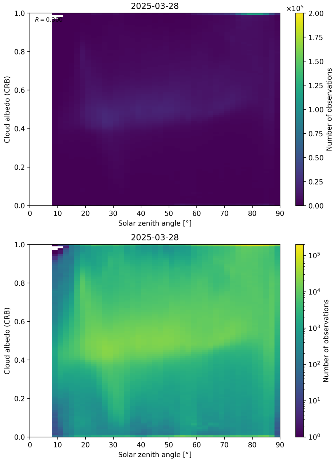
Figure 98: Scatter density plot of “Solar zenith angle” against “Cloud albedo (CRB)” for 2025-03-28 to 2025-03-29.
