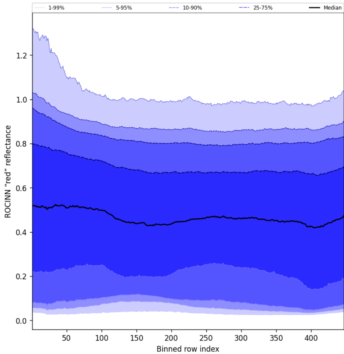
Figure 69: Along track statistics of “ROCINN “red” reflectance” for 2025-03-28 to 2025-03-29
