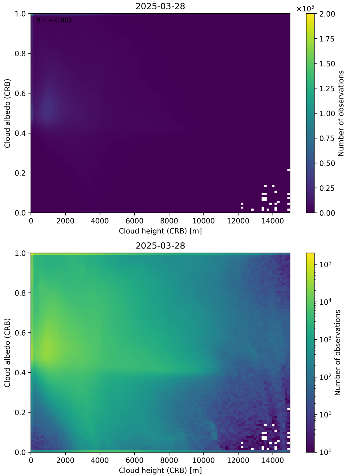
Figure 80: Scatter density plot of “Cloud height (CRB)” against “Cloud albedo (CRB)” for 2025-03-28 to 2025-03-29.
