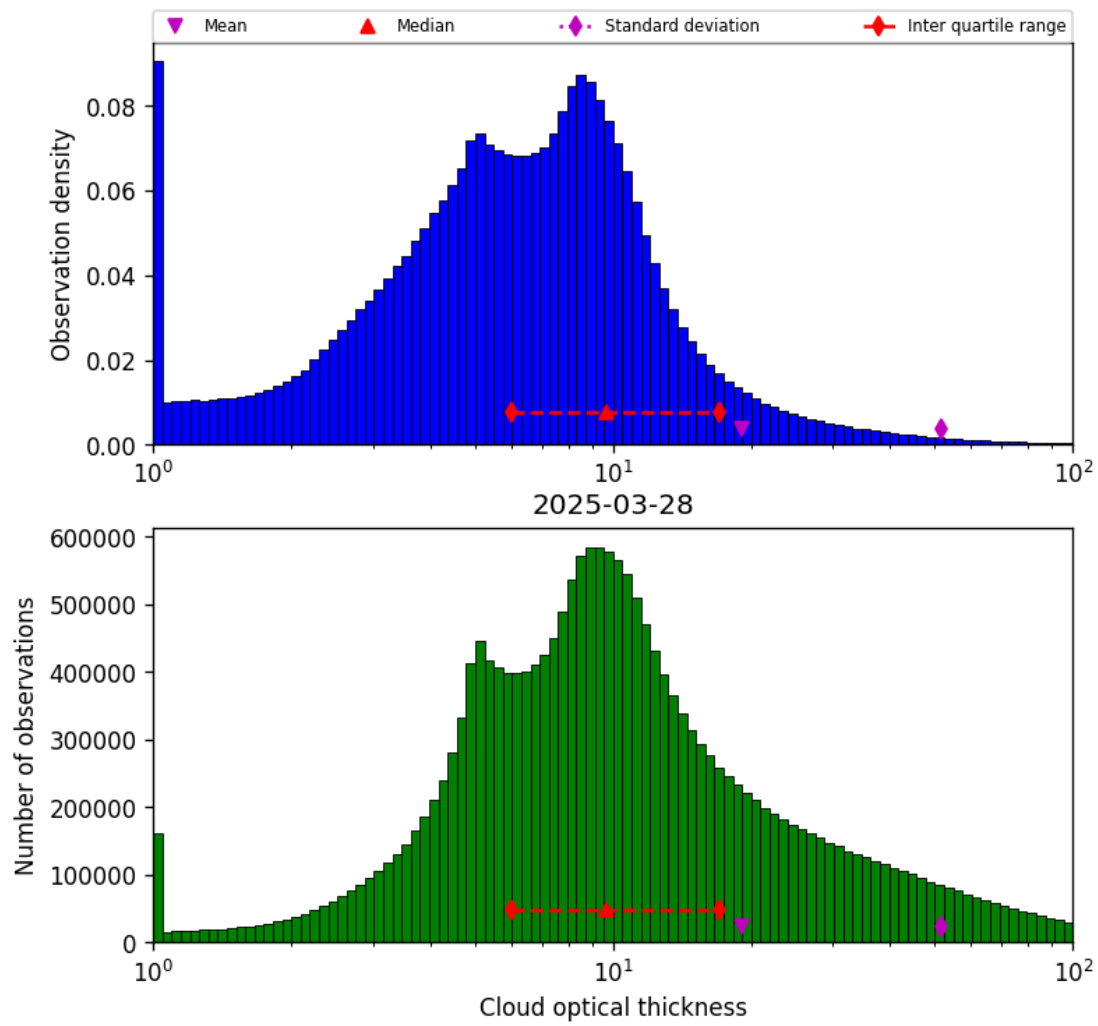
Figure 41: Histogram of “Cloud optical thickness” for 2025-03-28 to 2025-03-29
