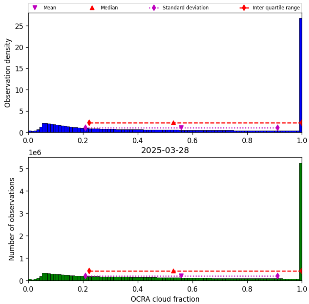
Figure 50: Histogram of “OCRA cloud fraction” for 2025-03-28 to 2025-03-29
