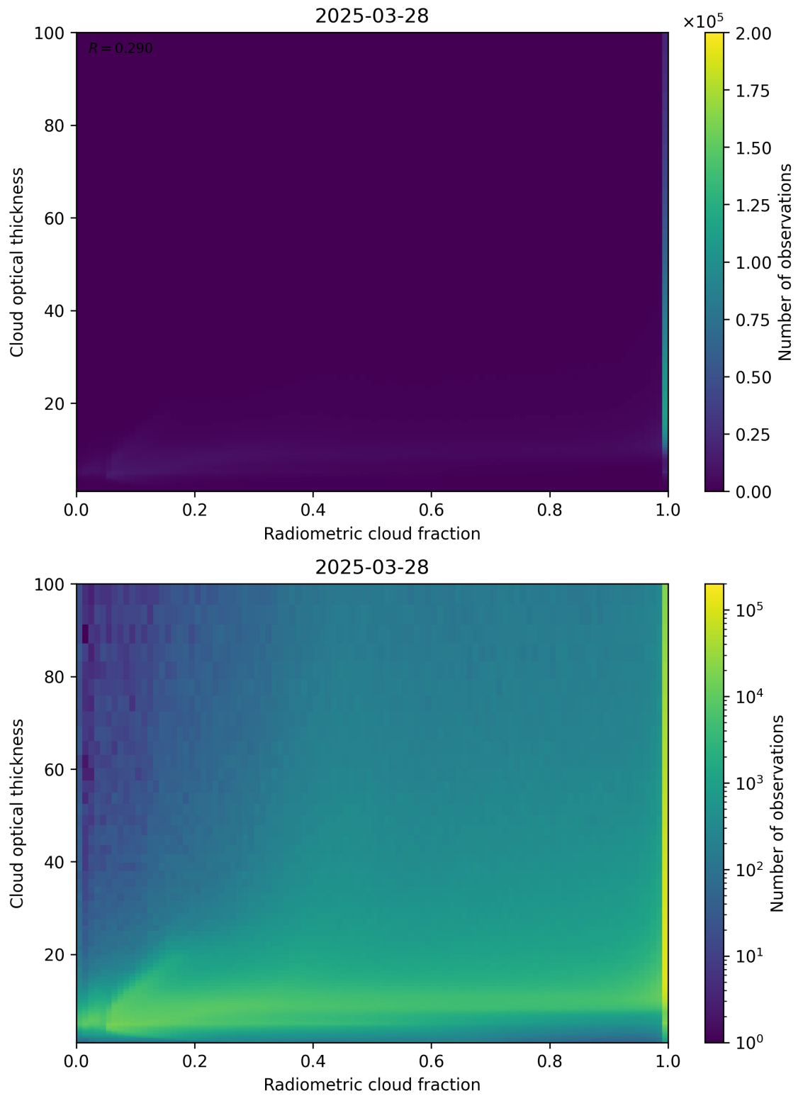
Figure 75: Scatter density plot of “Radiometric cloud fraction” against “Cloud optical thickness” for 2025-03-28 to 2025-03-29.
