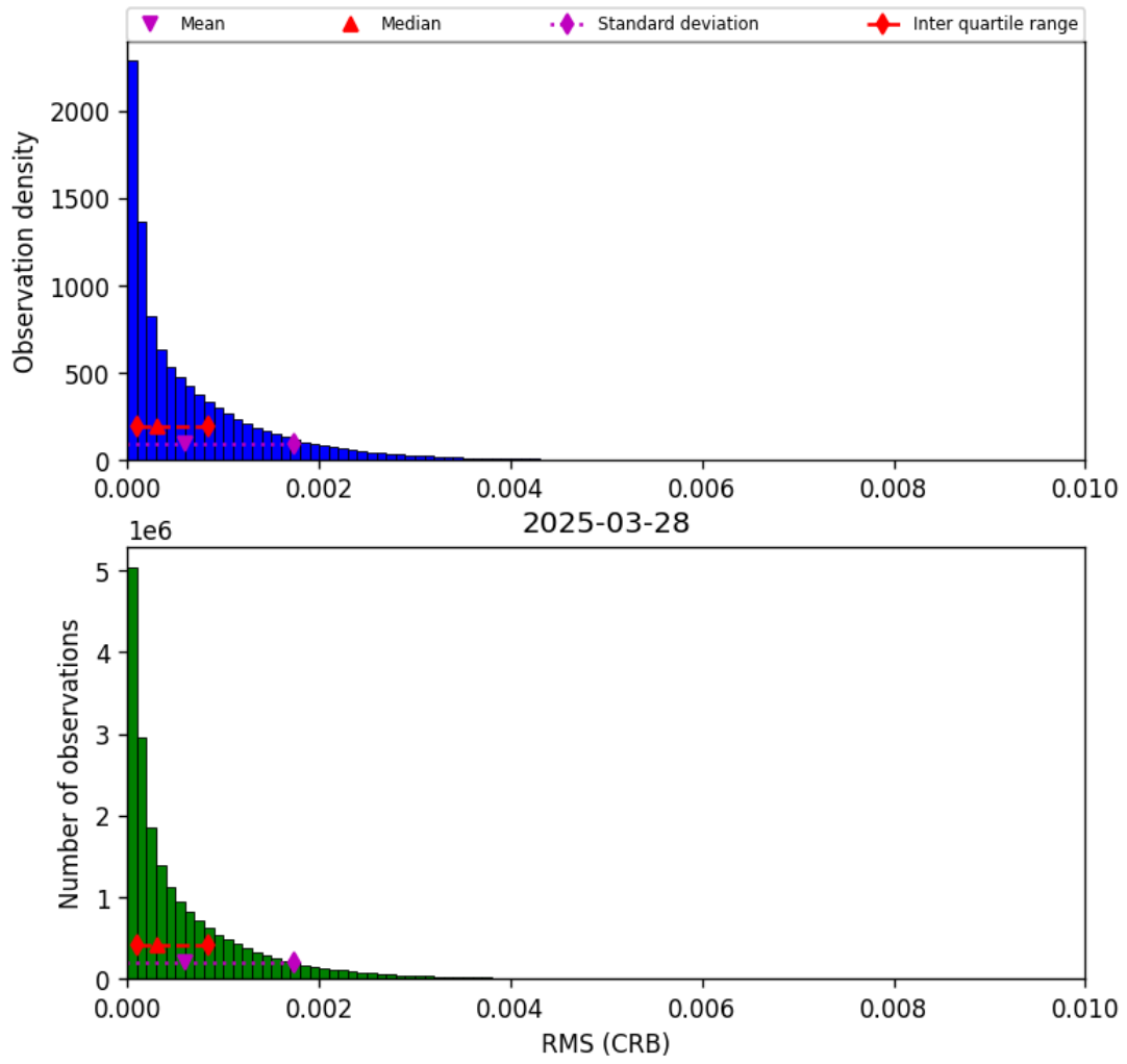
Figure 48: Histogram of "RMS (CRB)" for 2025-03-28 to 2025-03-29
