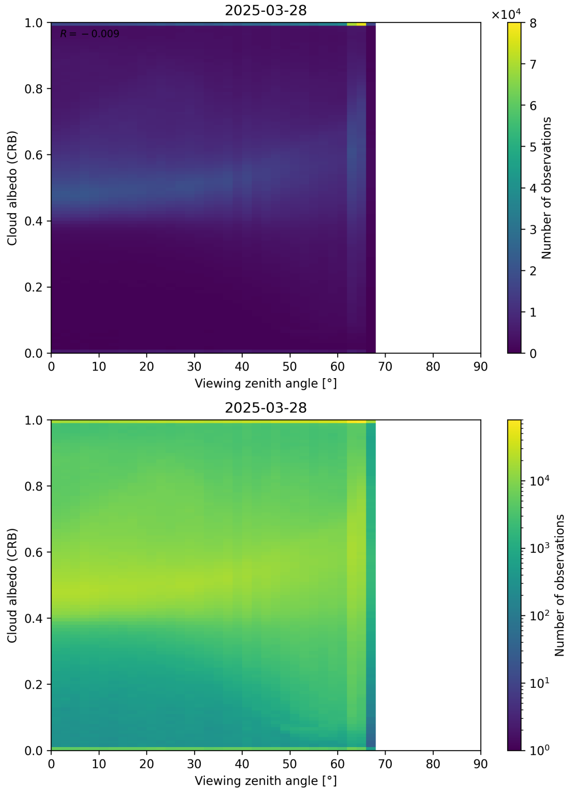
Figure 106: Scatter density plot of “Viewing zenith angle” against “Cloud albedo (CRB)” for 2025-03-28 to 2025-03-29.
