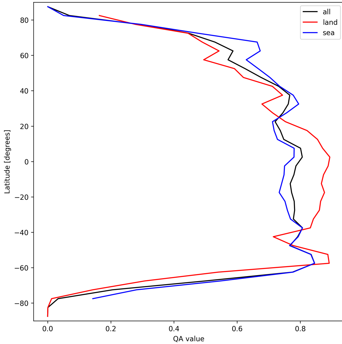
Figure 22: Zonal average of “QA value” for 2025-03-28 to 2025-03-29.
