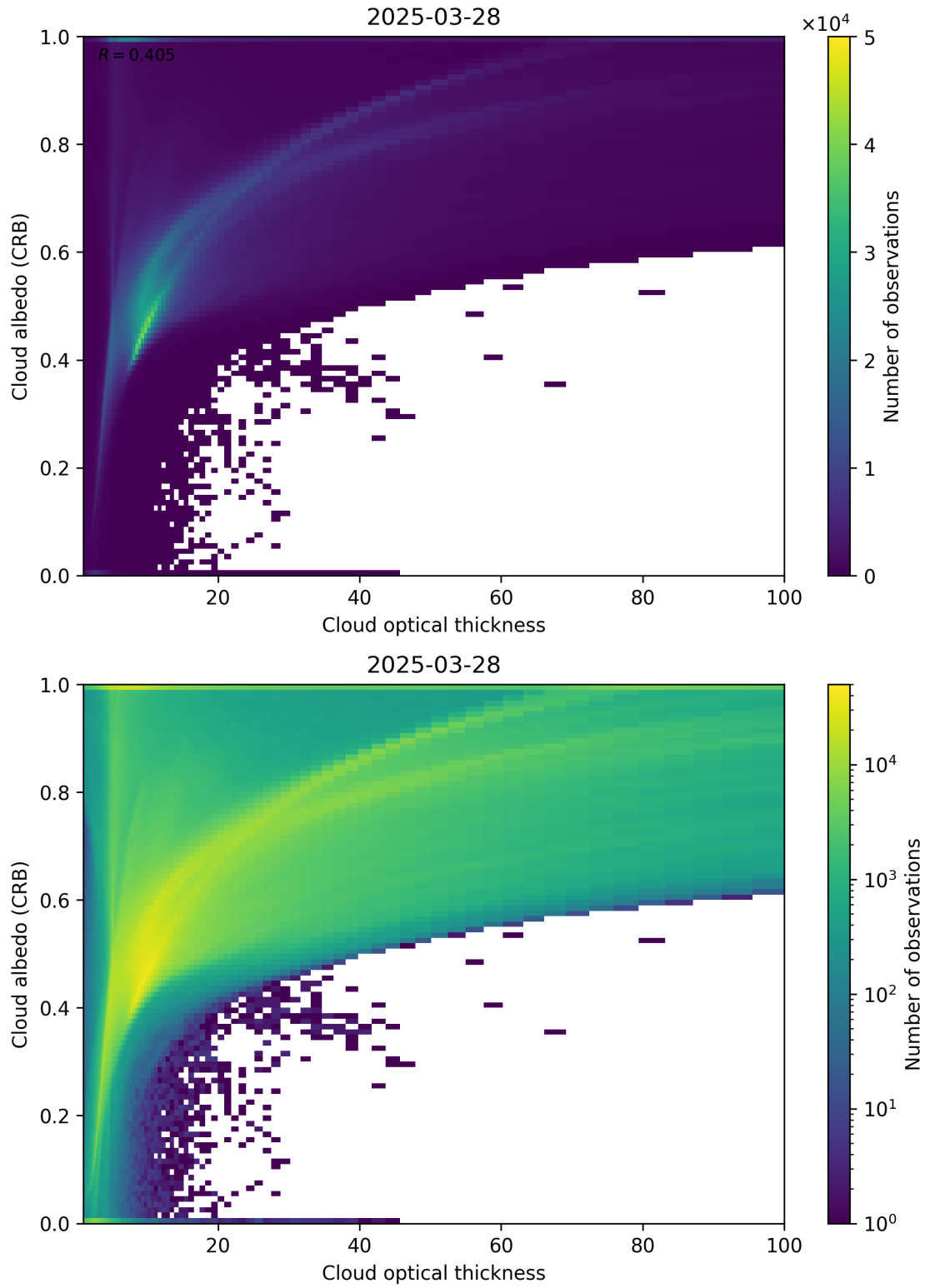
Figure 82: Scatter density plot of “Cloud optical thickness” against “Cloud albedo (CRB)” for 2025-03-28 to 2025-03-29.
