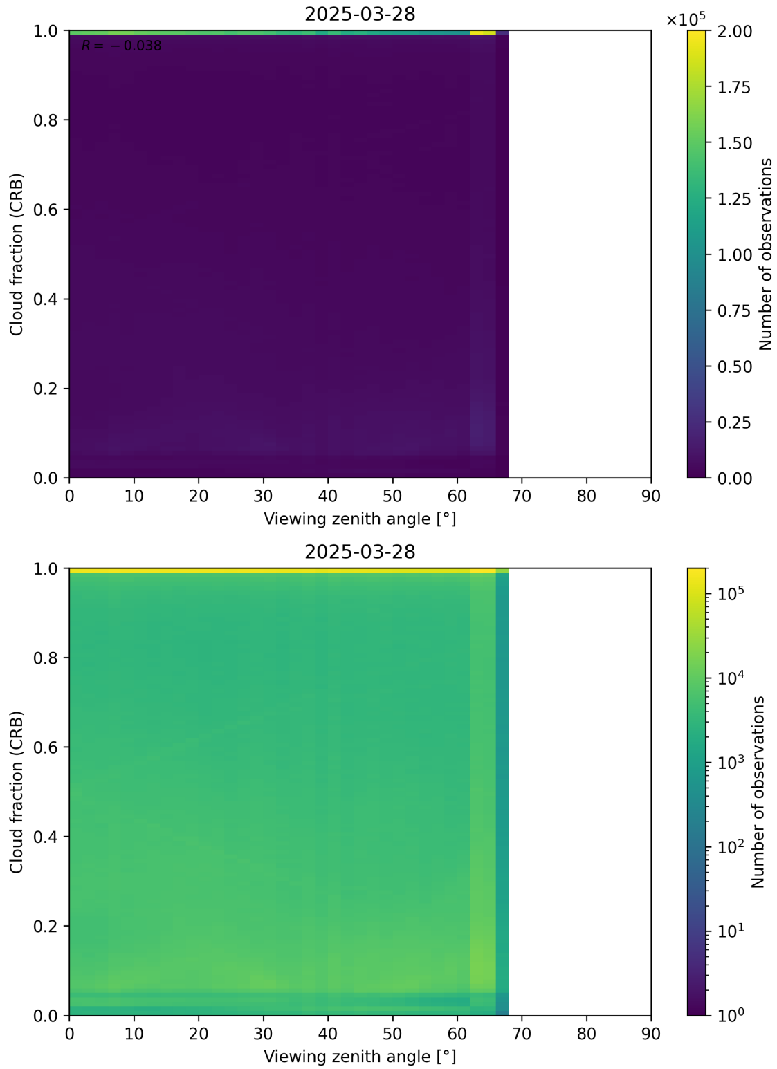
Figure 109: Scatter density plot of “Viewing zenith angle” against “Cloud fraction (CRB)” for 2025-03-28 to 2025-03-29.
