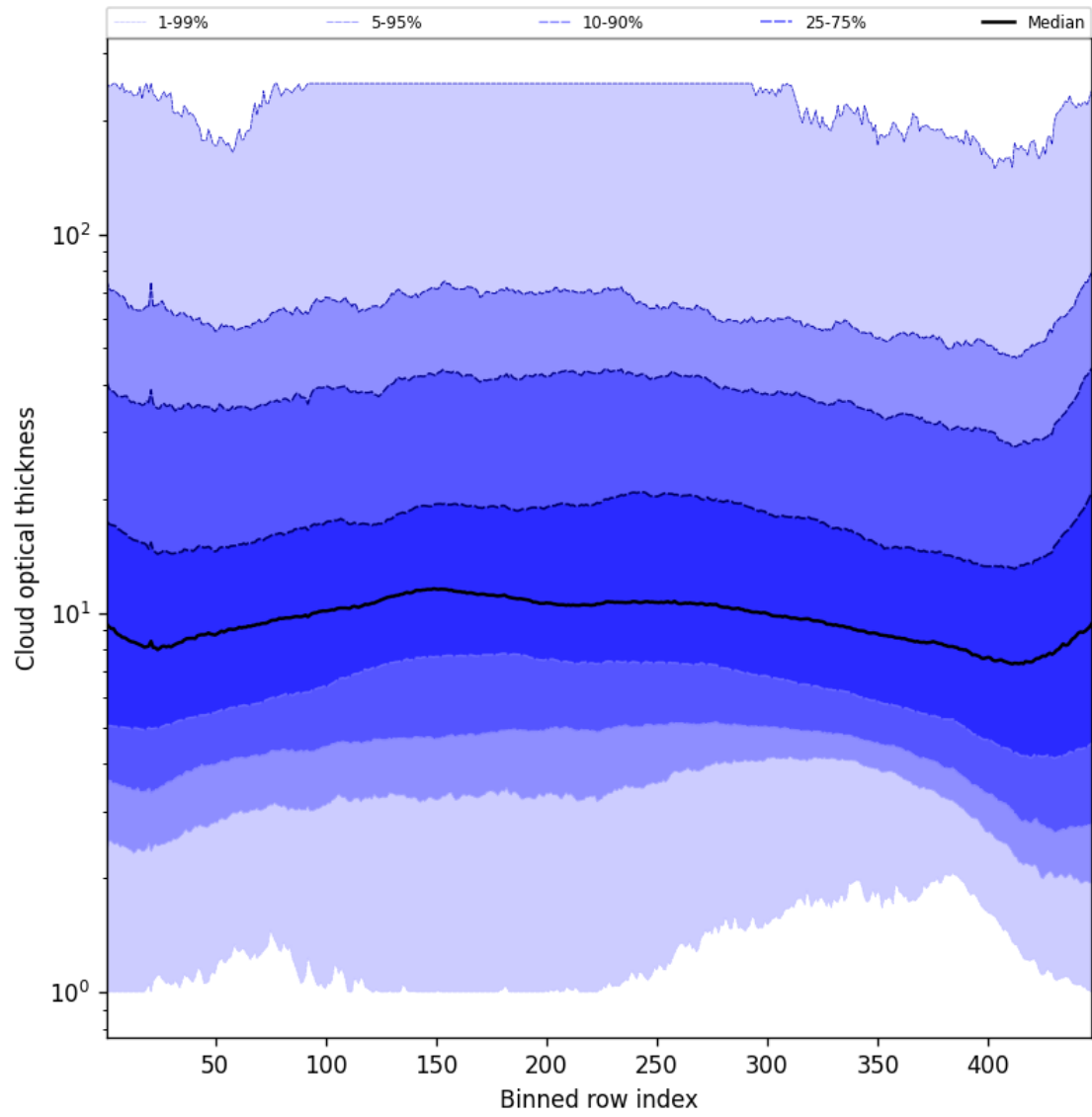
Figure 57: Along track statistics of “Cloud optical thickness” for 2025-03-28 to 2025-03-29
