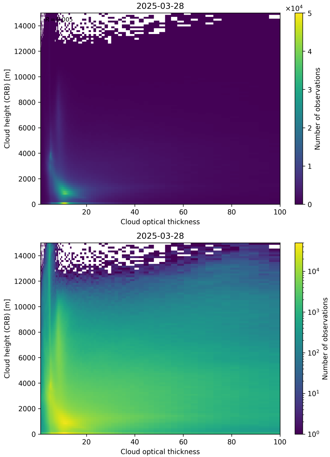
Figure 85: Scatter density plot of “Cloud optical thickness” against “Cloud height (CRB)” for 2025-03-28 to 2025-03-29.
