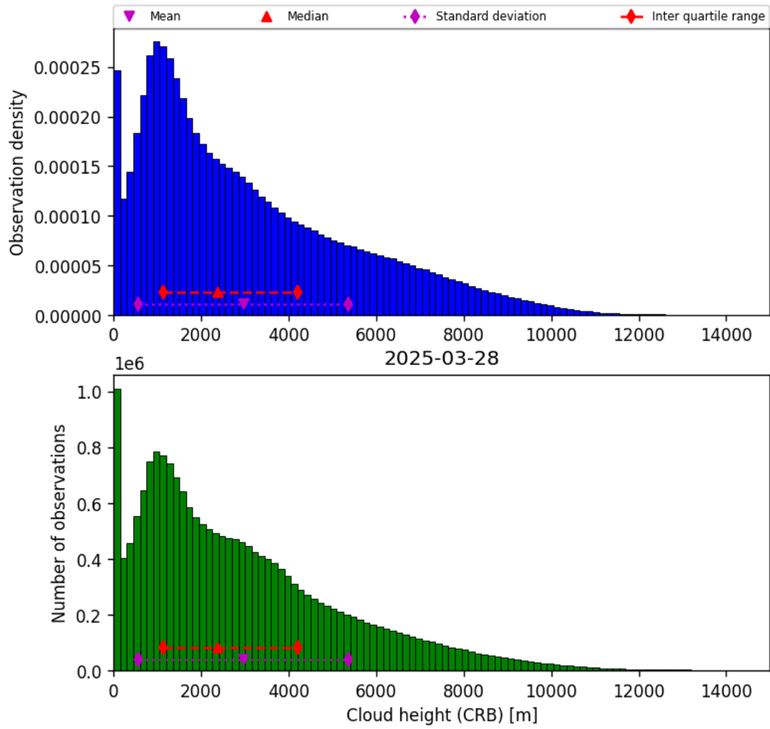
Figure 43: Histogram of “Cloud height (CRB)” for 2025-03-28 to 2025-03-29
