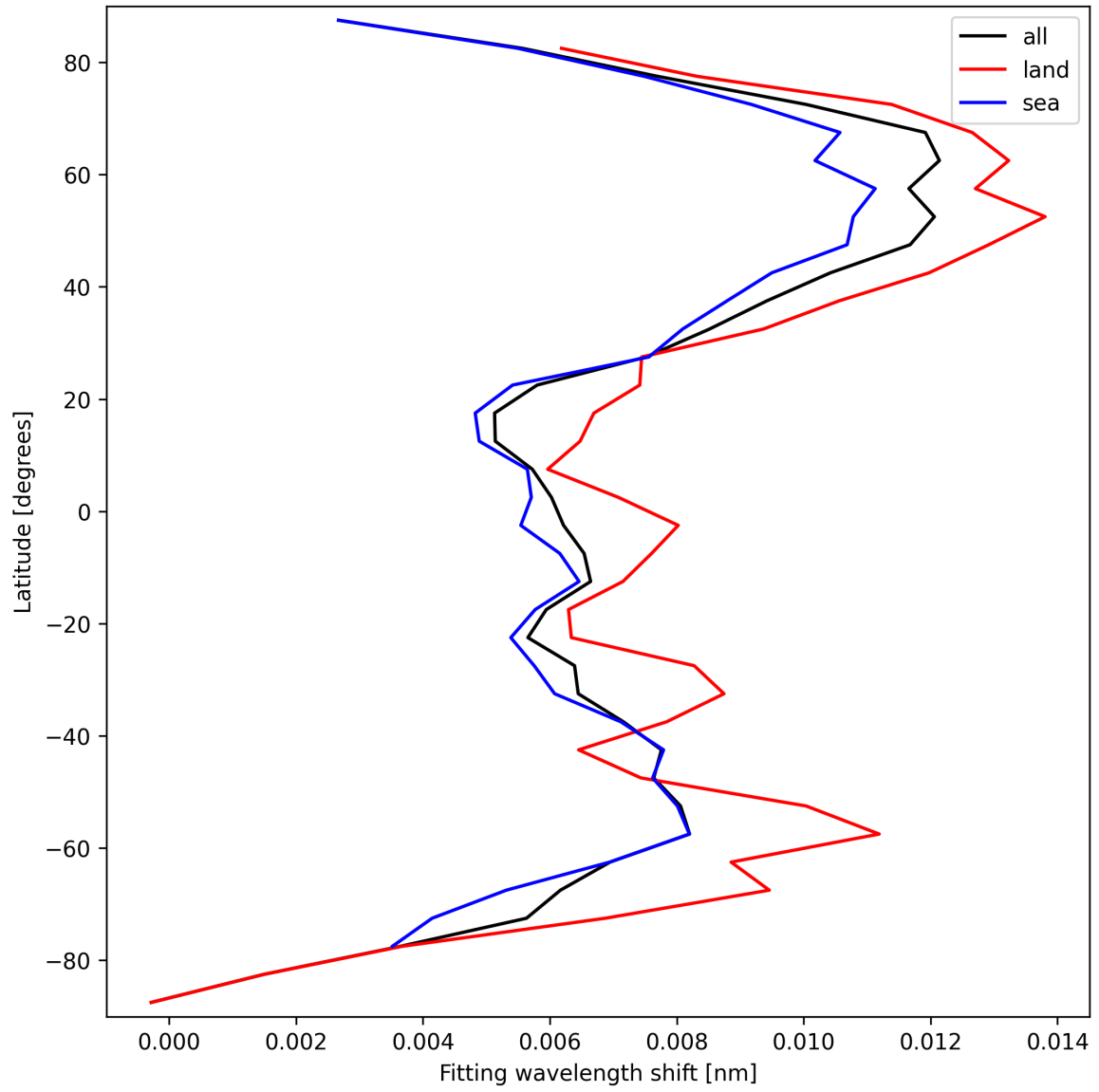
Figure 33: Zonal average of “Fitting wavelength shift” for 2025-03-28 to 2025-03-29.
