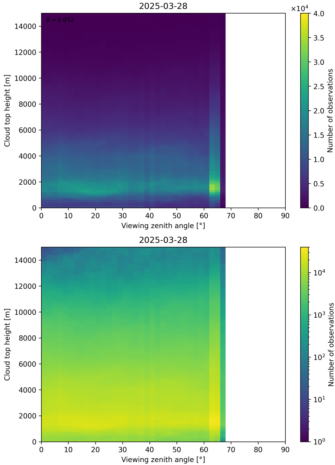
Figure 112: Scatter density plot of “Viewing zenith angle” against “Cloud top height” for 2025-03-28 to 2025-03-29.
