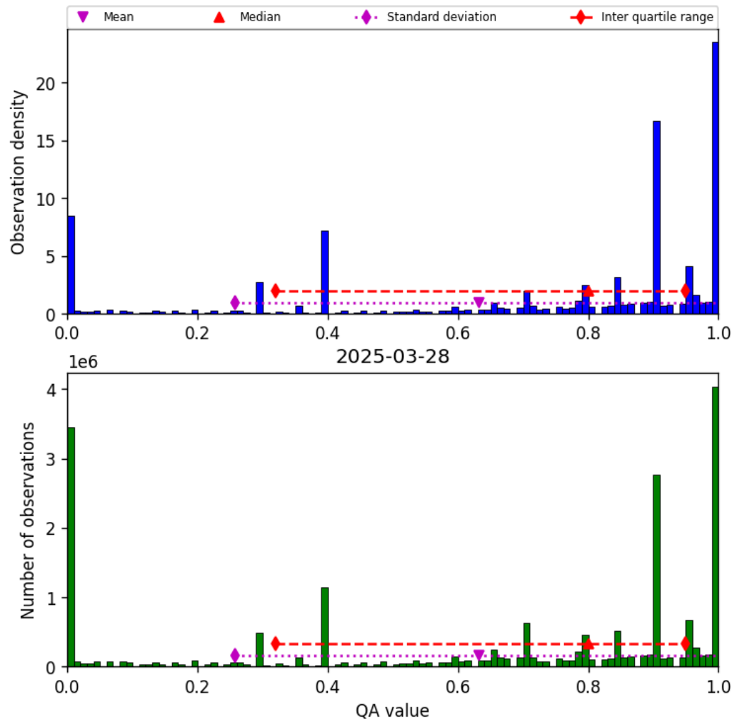
Figure 38: Histogram of “QA value” for 2025-03-28 to 2025-03-29
