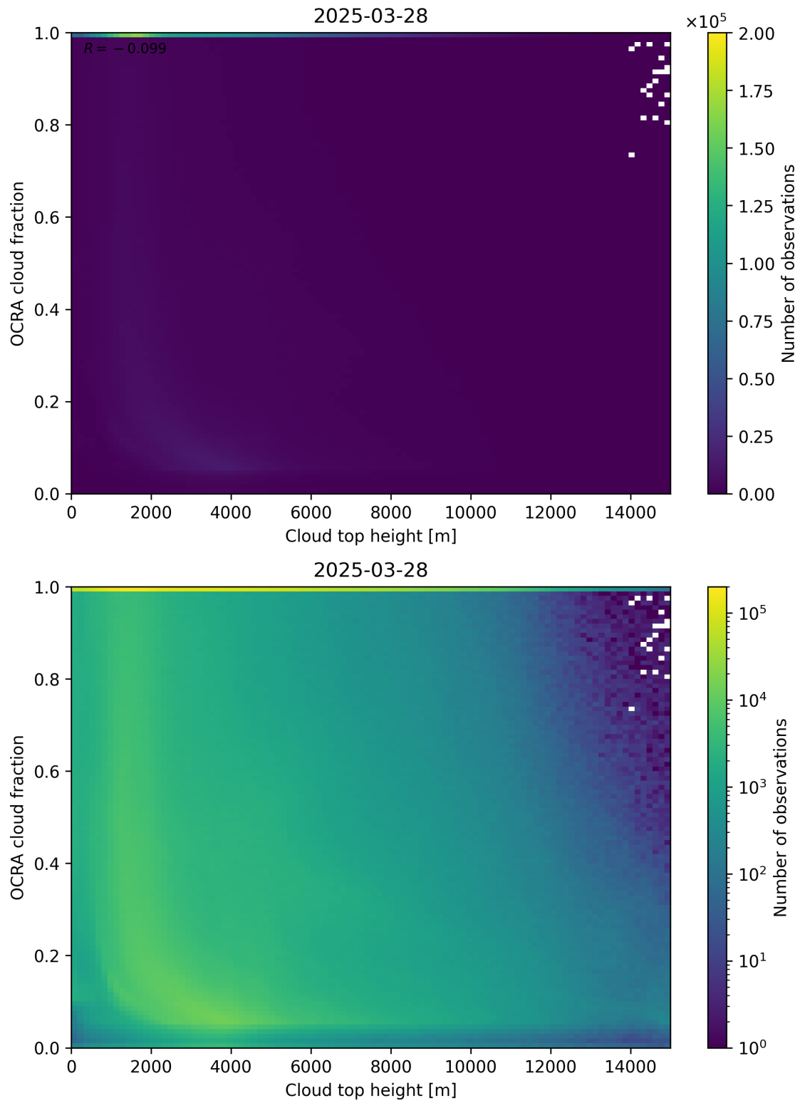
Figure 87: Scatter density plot of “Cloud top height” against “OCRA cloud fraction” for 2025-03-28 to 2025-03-29.
