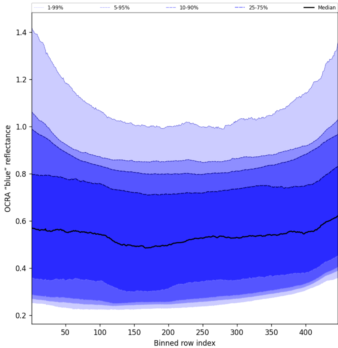
Figure 67: Along track statistics of “OCRA “blue” reflectance” for 2025-03-28 to 2025-03-29
