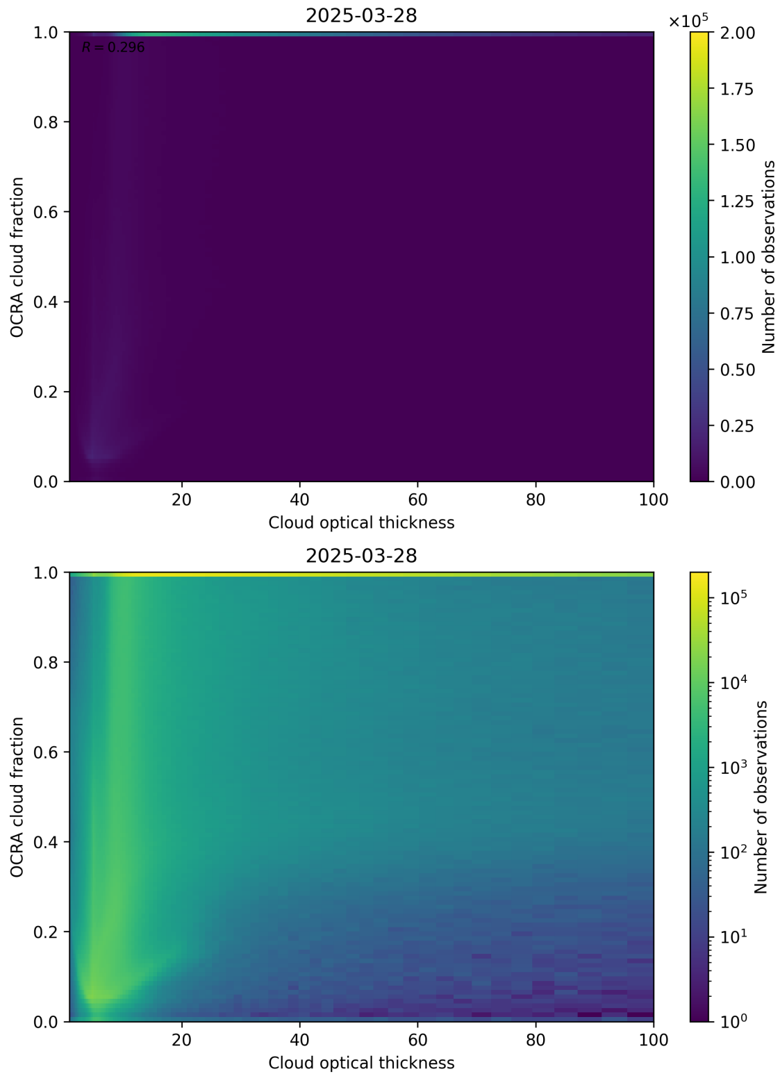
Figure 83: Scatter density plot of “Cloud optical thickness” against “OCRA cloud fraction” for 2025-03-28 to 2025-03-29.
