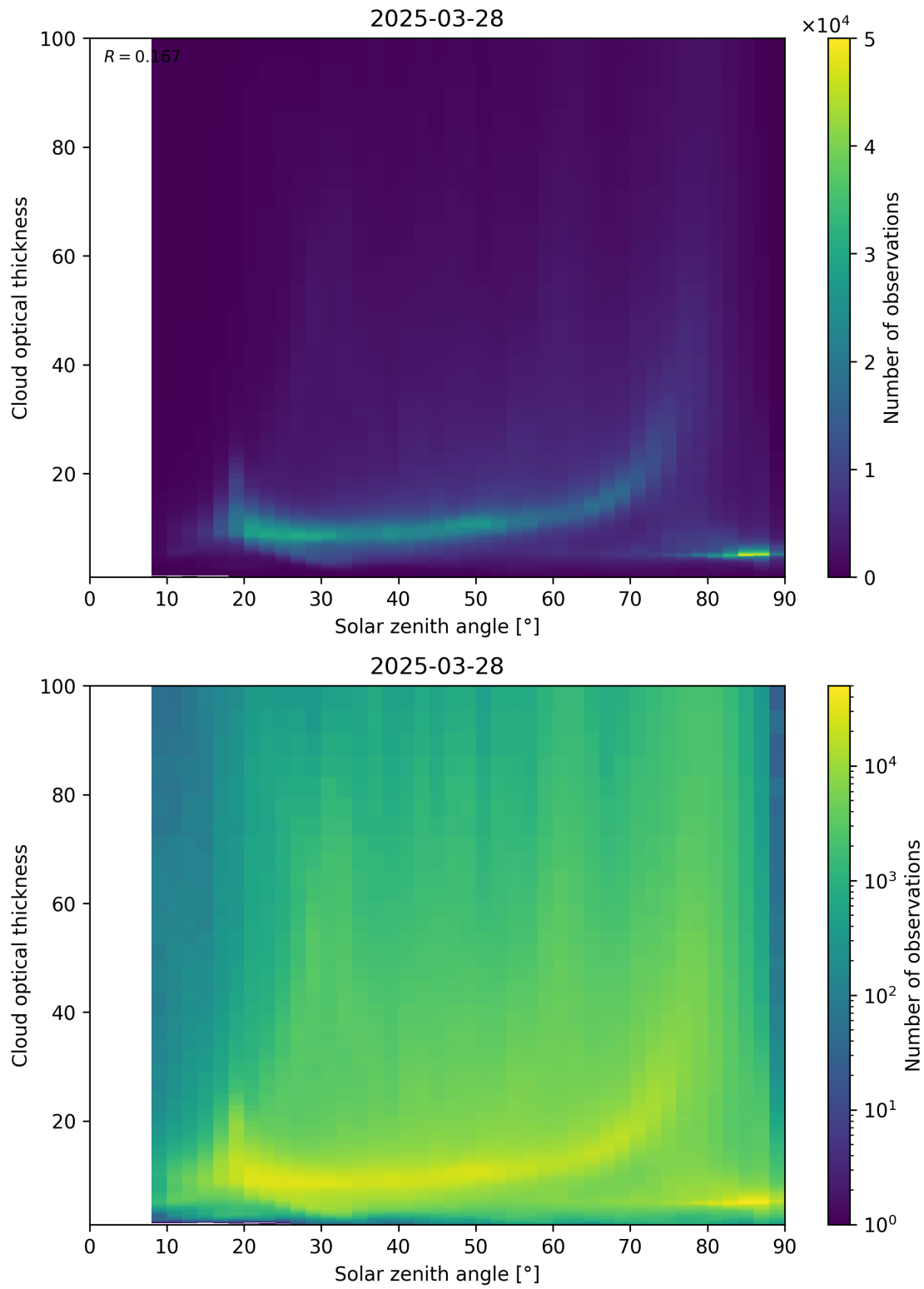
Figure 103: Scatter density plot of “Solar zenith angle” against “Cloud optical thickness” for 2025-03-28 to 2025-03-29.
