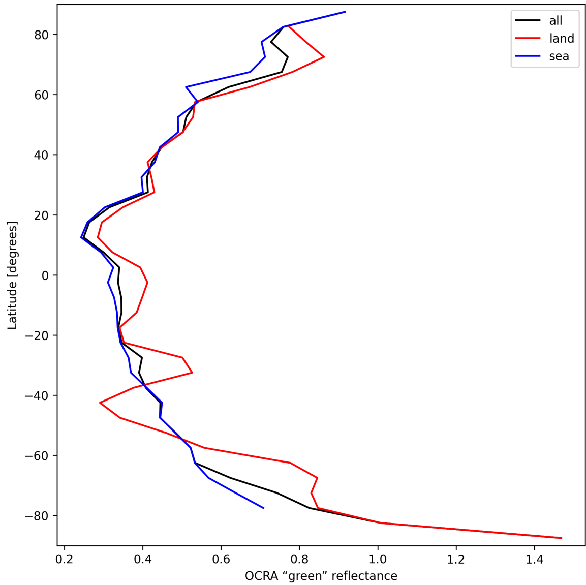
Figure 36: Zonal average of "OCRA "green" reflectance" for 2025-03-28 to 2025-03-29.
