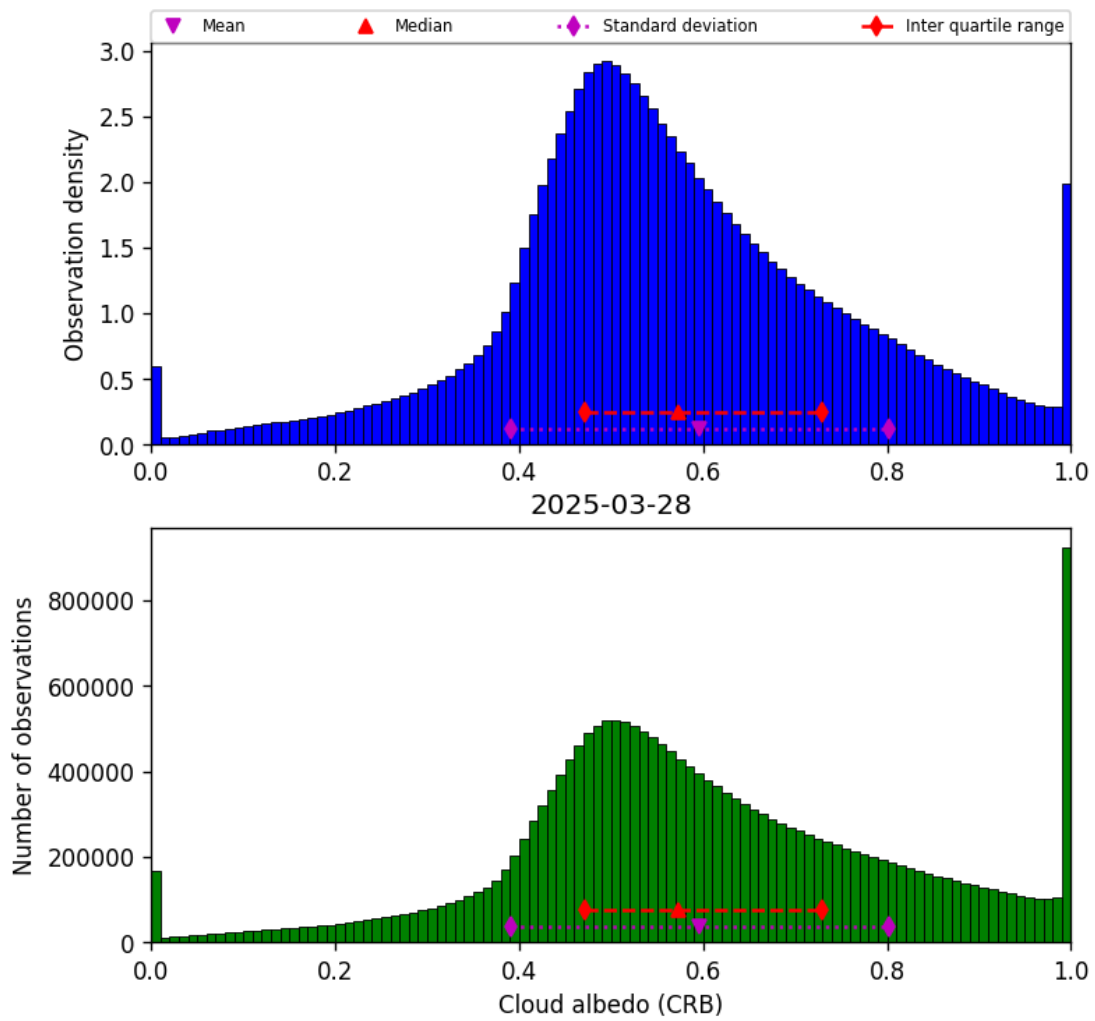
Figure 44: Histogram of “Cloud albedo (CRB)” for 2025-03-28 to 2025-03-29
