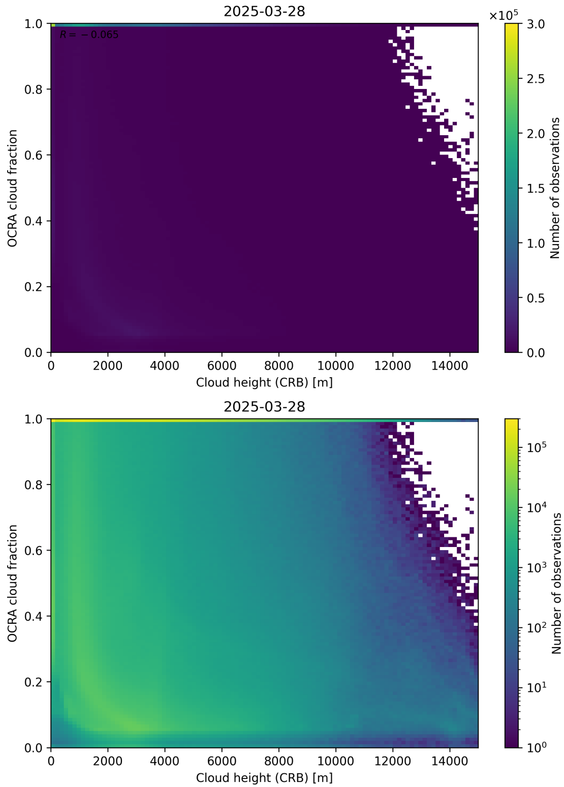
Figure 81: Scatter density plot of “Cloud height (CRB)” against “OCRA cloud fraction” for 2025-03-28 to 2025-03-29.
