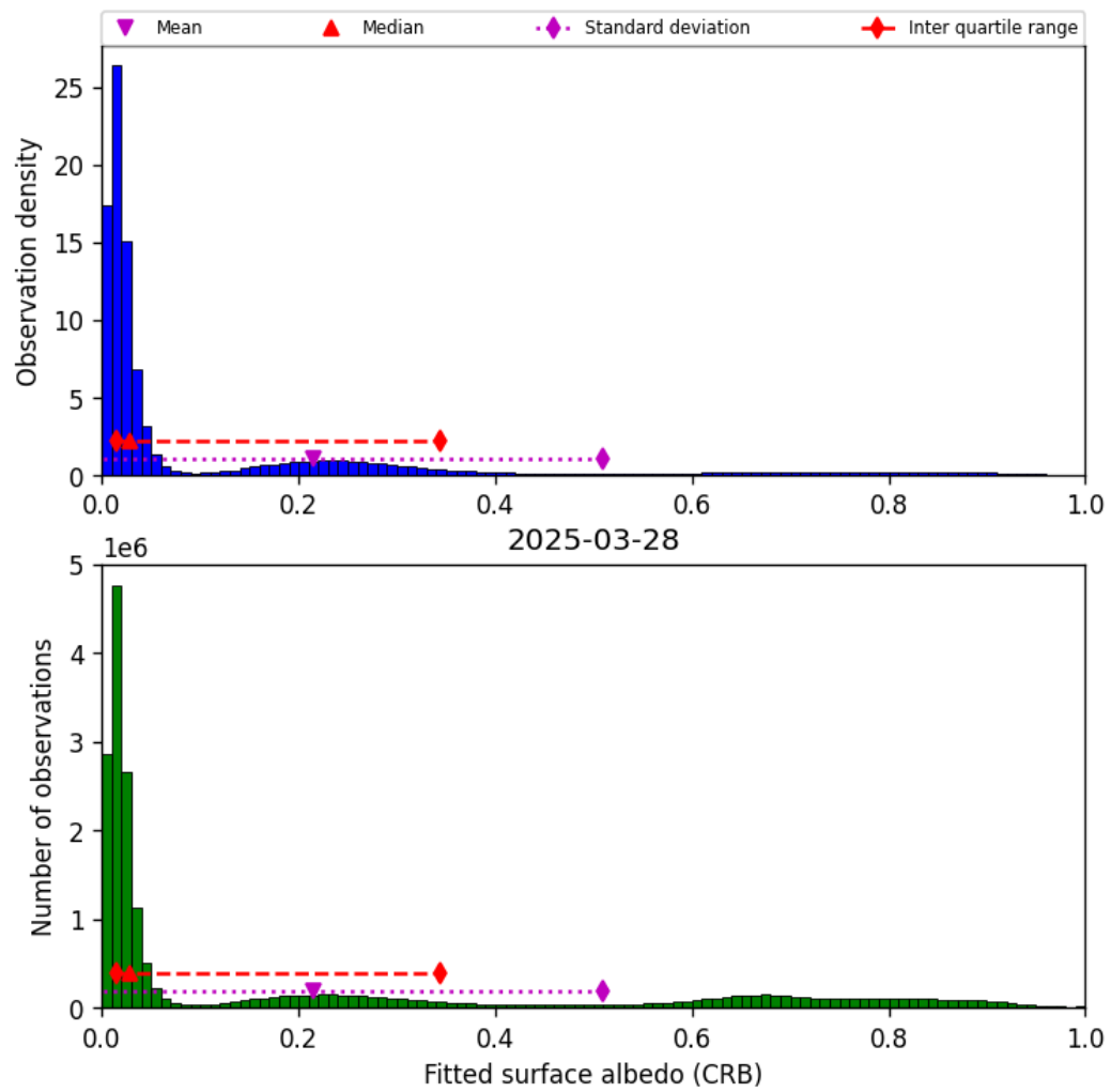
Figure 46: Histogram of “Fitted surface albedo (CRB)” for 2025-03-28 to 2025-03-29
