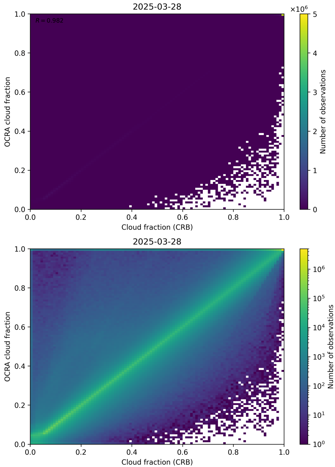
Figure 78: Scatter density plot of “Cloud fraction (CRB)” against “OCRA cloud fraction” for 2025-03-28 to 2025-03-29.
