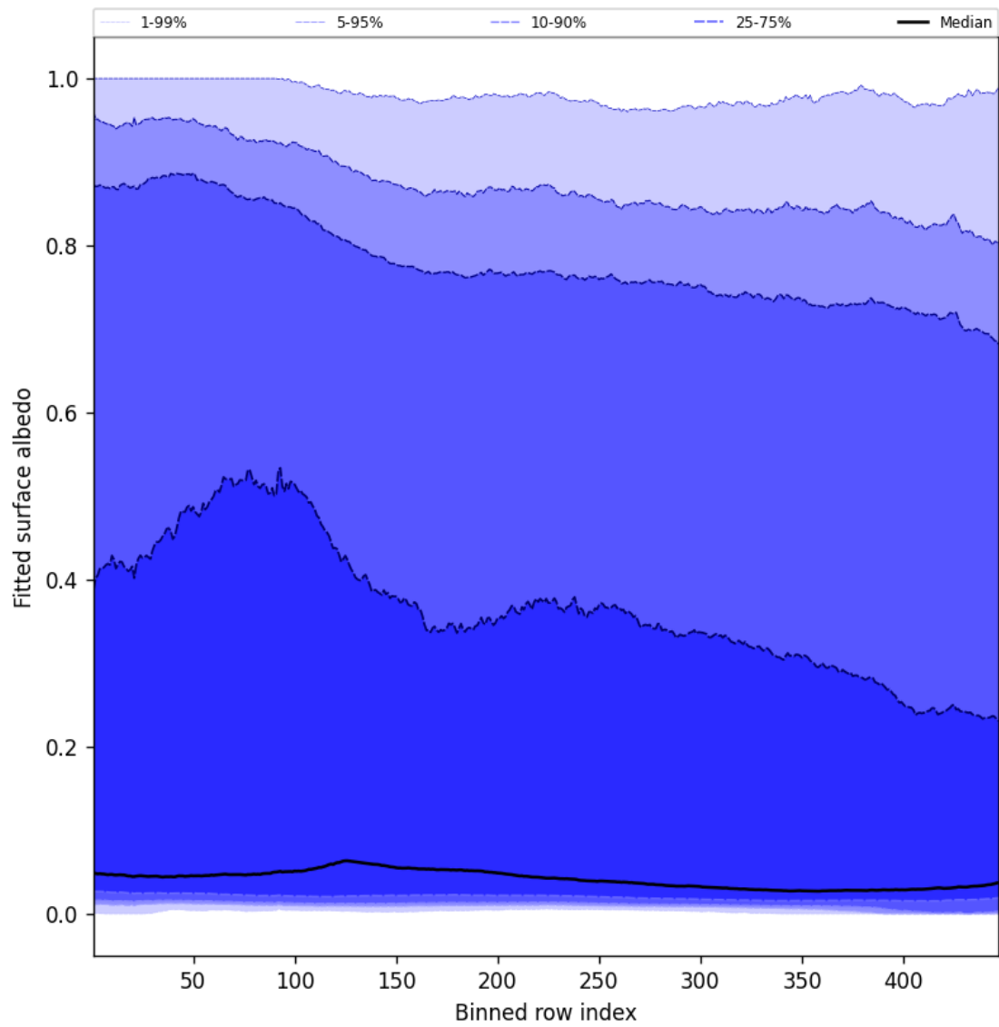
Figure 61: Along track statistics of “Fitted surface albedo” for 2025-03-28 to 2025-03-29
