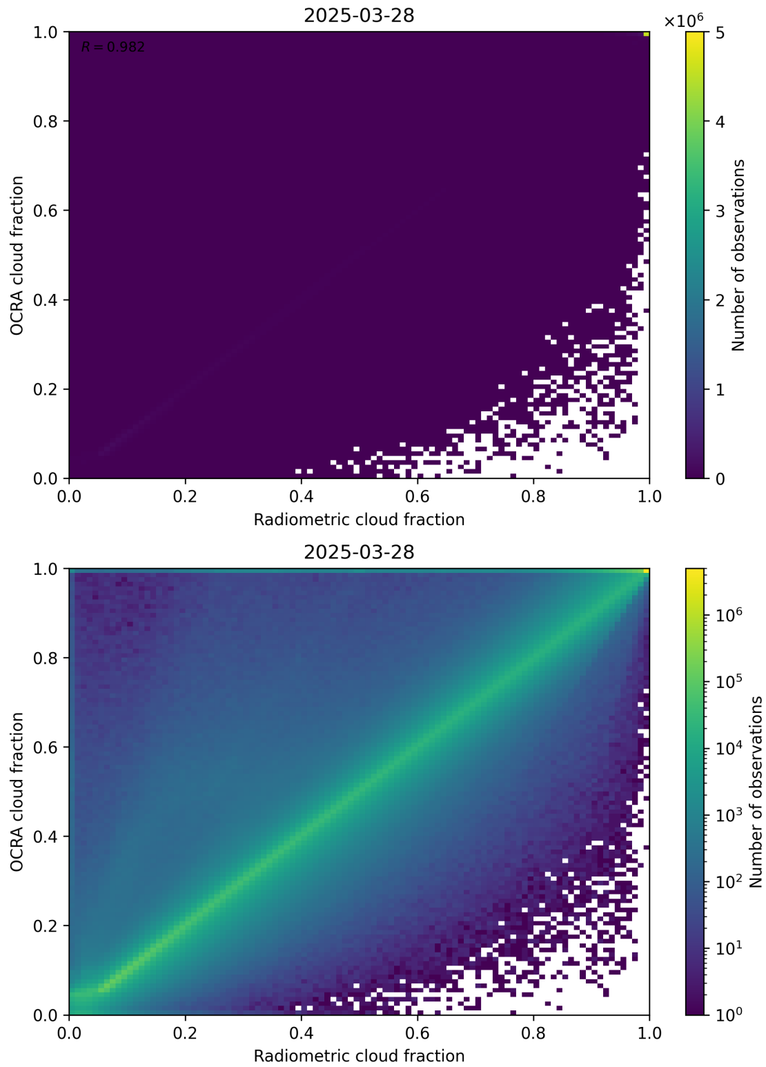
Figure 72: Scatter density plot of “Radiometric cloud fraction” against “OCRA cloud fraction” for 2025-03-28 to 2025-03-29.
