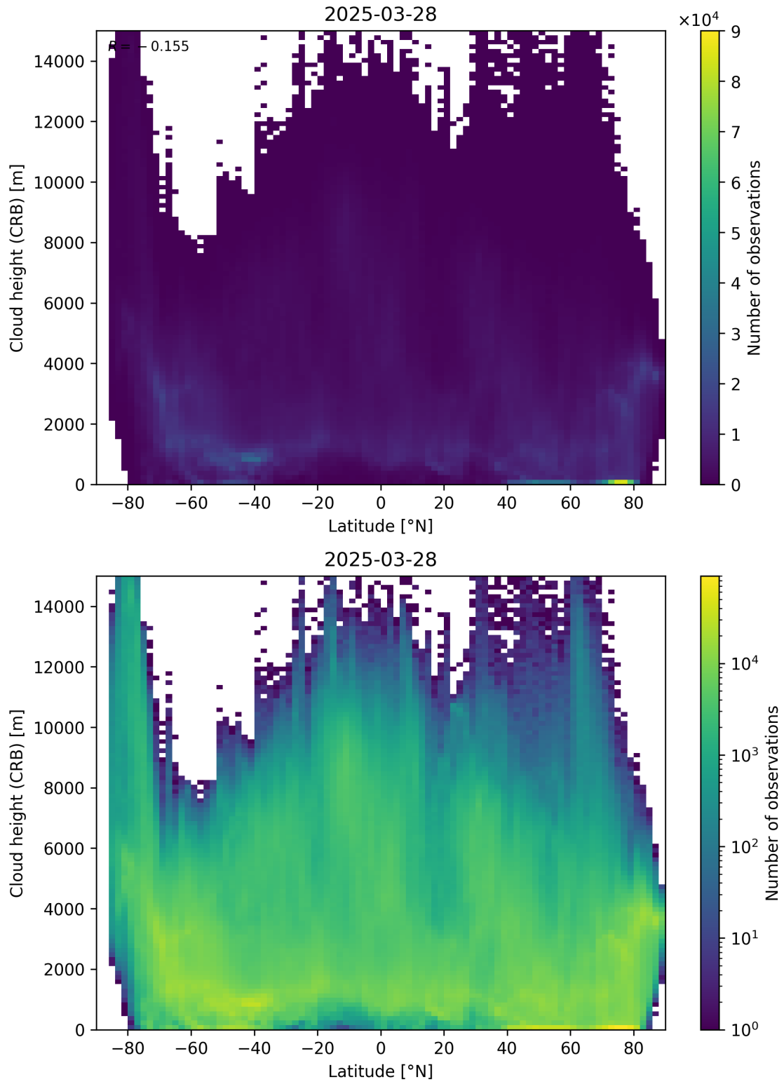
Figure 95: Scatter density plot of “Latitude” against “Cloud height (CRB)” for 2025-03-28 to 2025-03-29.
