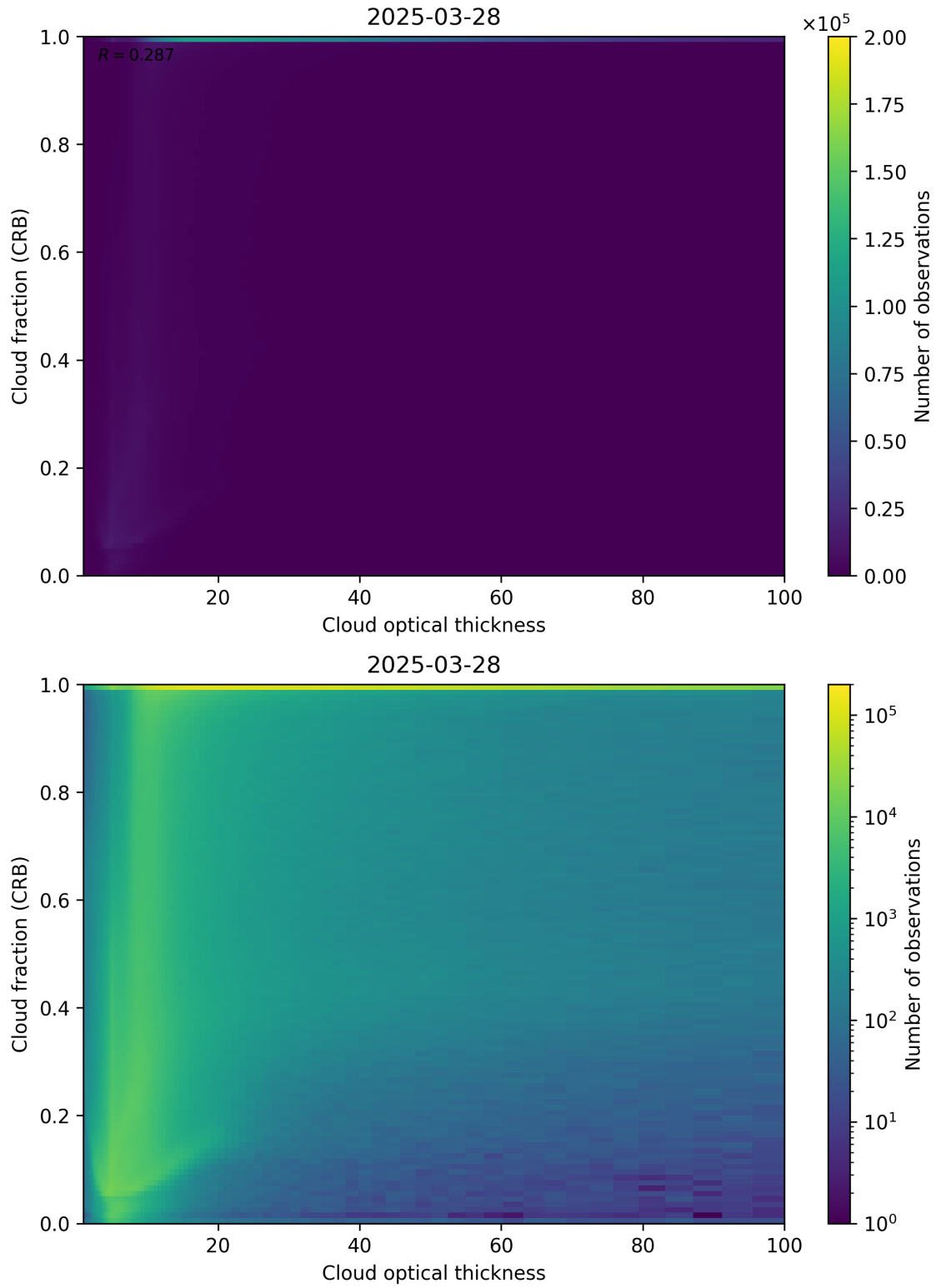
Figure 84: Scatter density plot of “Cloud optical thickness” against “Cloud fraction (CRB)” for 2025-03-28 to 2025-03-29.
