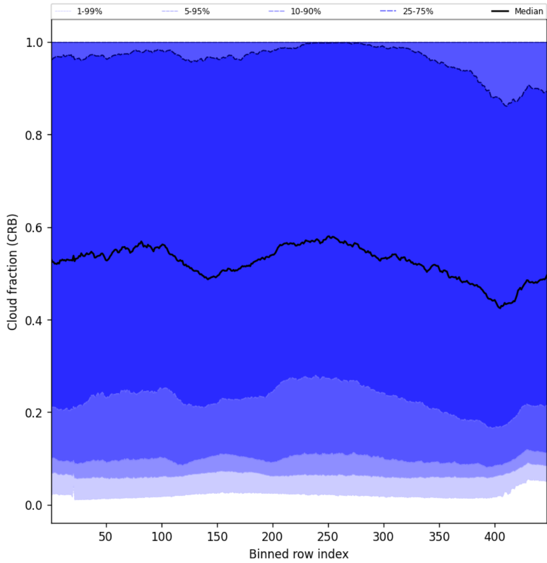
Figure 58: Along track statistics of “Cloud fraction (CRB)” for 2025-03-28 to 2025-03-29
