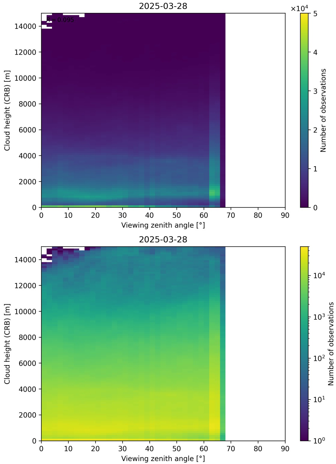
Figure 110: Scatter density plot of “Viewing zenith angle” against “Cloud height (CRB)” for 2025-03-28 to 2025-03-29.
