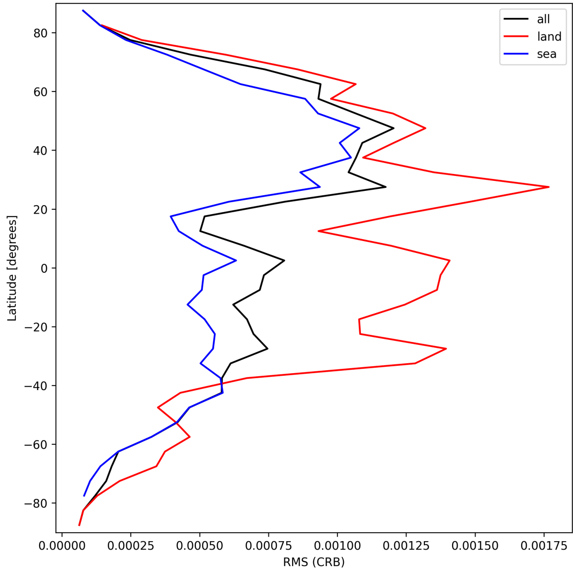
Figure 32: Zonal average of “RMS (CRB)” for 2025-03-28 to 2025-03-29.
