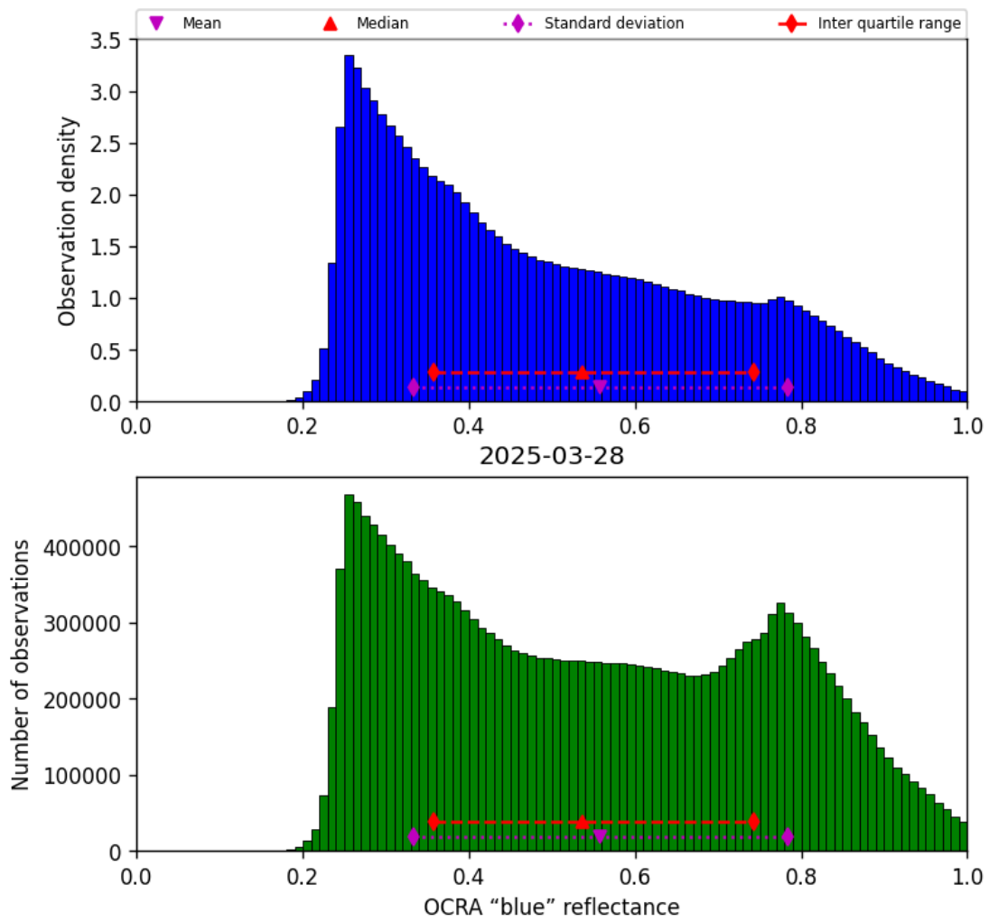
Figure 51: Histogram of “OCRA “blue” reflectance” for 2025-03-28 to 2025-03-29
