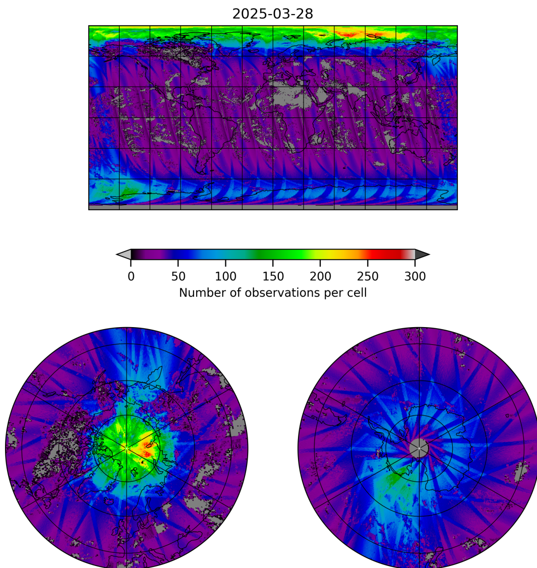
Figure 21: Map of the number of observations for 2025-03-28 to 2025-03-29
