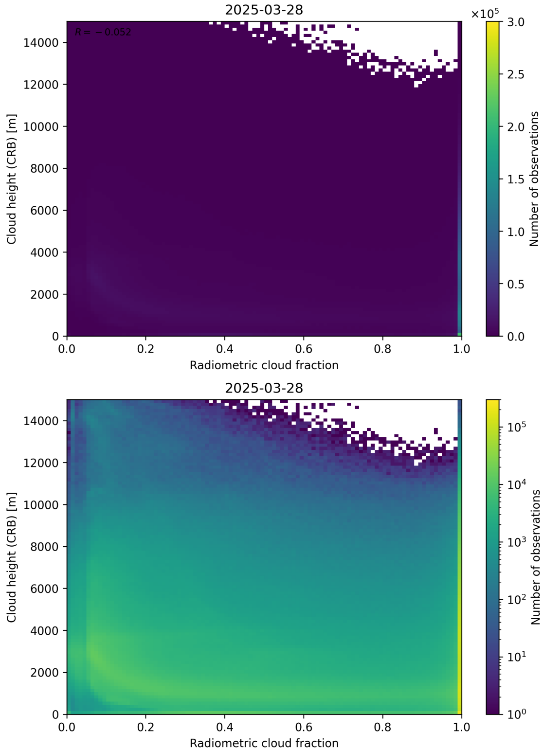
Figure 74: Scatter density plot of “Radiometric cloud fraction” against “Cloud height (CRB)” for 2025-03-28 to 2025-03-29.
