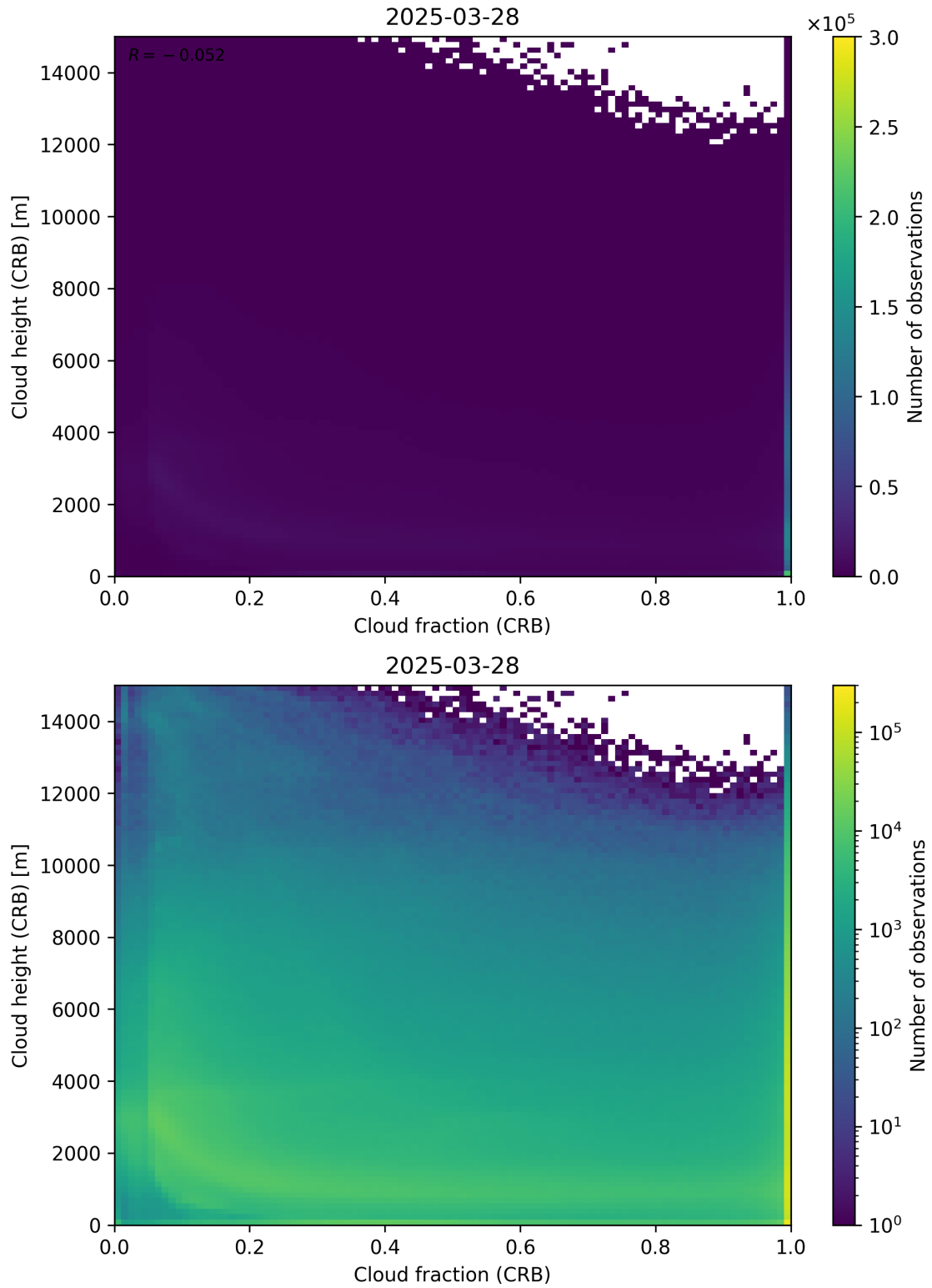
Figure 79: Scatter density plot of “Cloud fraction (CRB)” against “Cloud height (CRB)” for 2025-03-28 to 2025-03-29.
