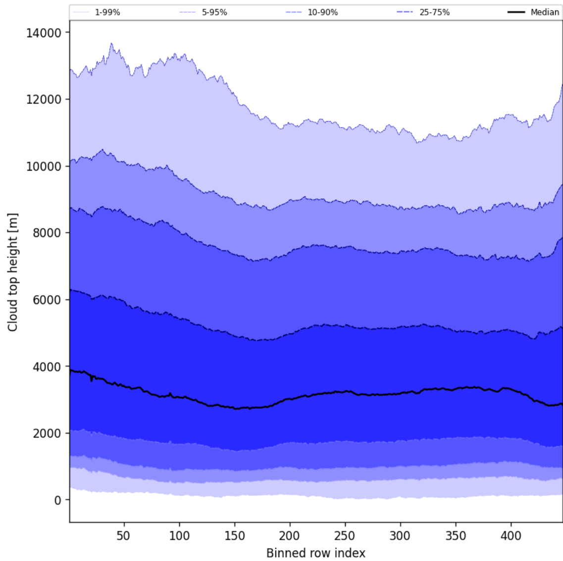
Figure 56: Along track statistics of “Cloud top height” for 2025-03-28 to 2025-03-29
