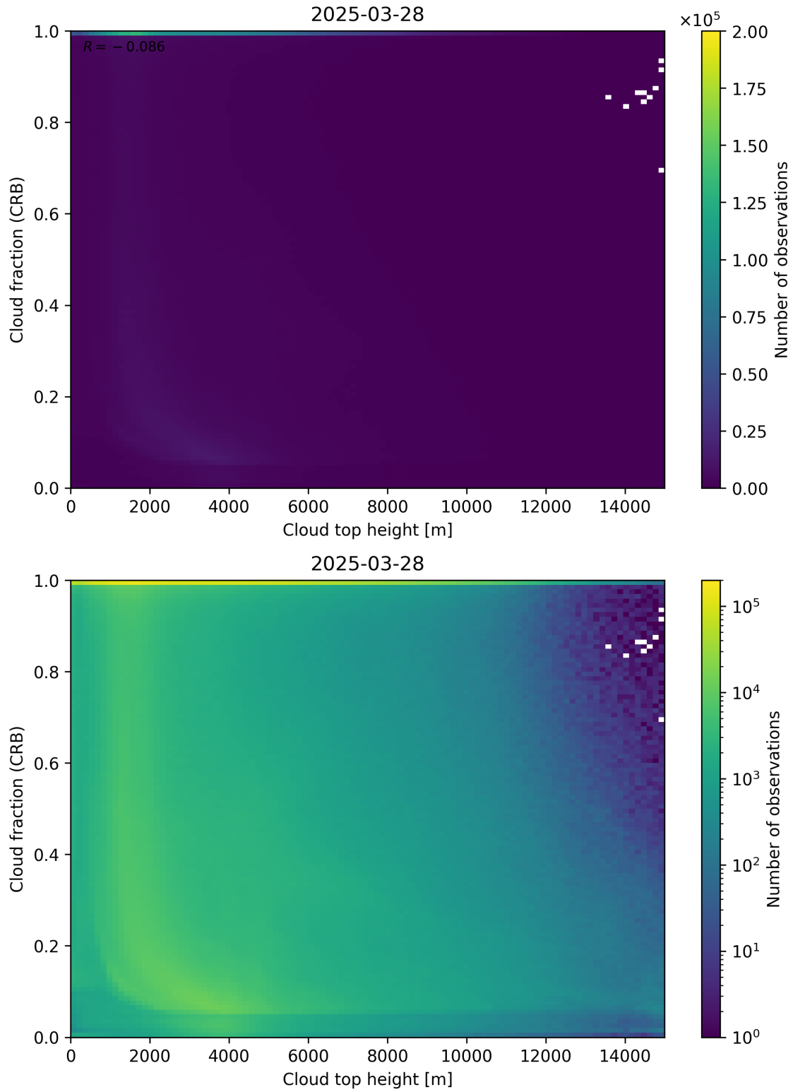
Figure 88: Scatter density plot of “Cloud top height” against “Cloud fraction (CRB)” for 2025-03-28 to 2025-03-29.
