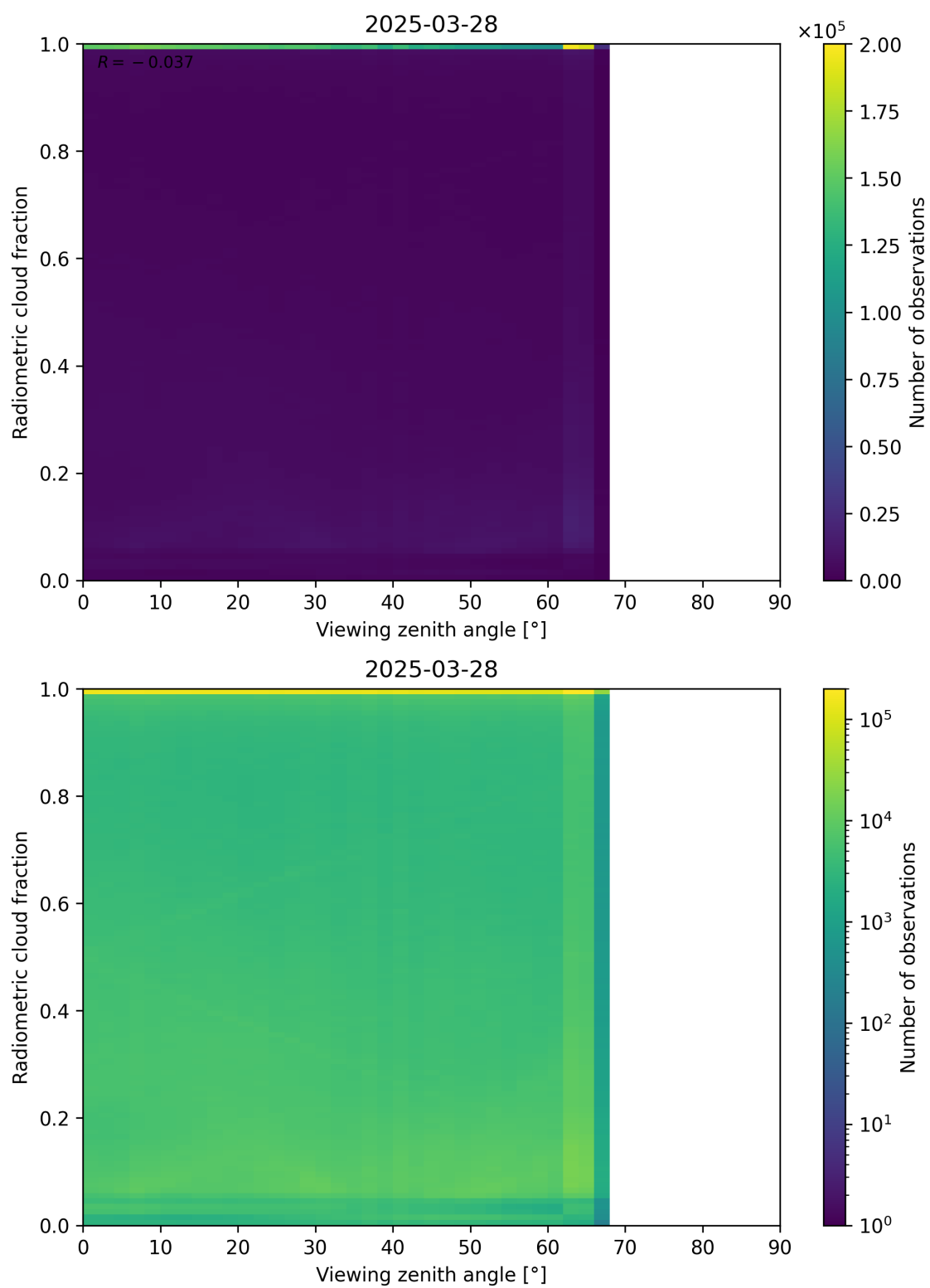
Figure 107: Scatter density plot of “Viewing zenith angle” against “Radiometric cloud fraction” for 2025-03-28 to 2025-03-29.
