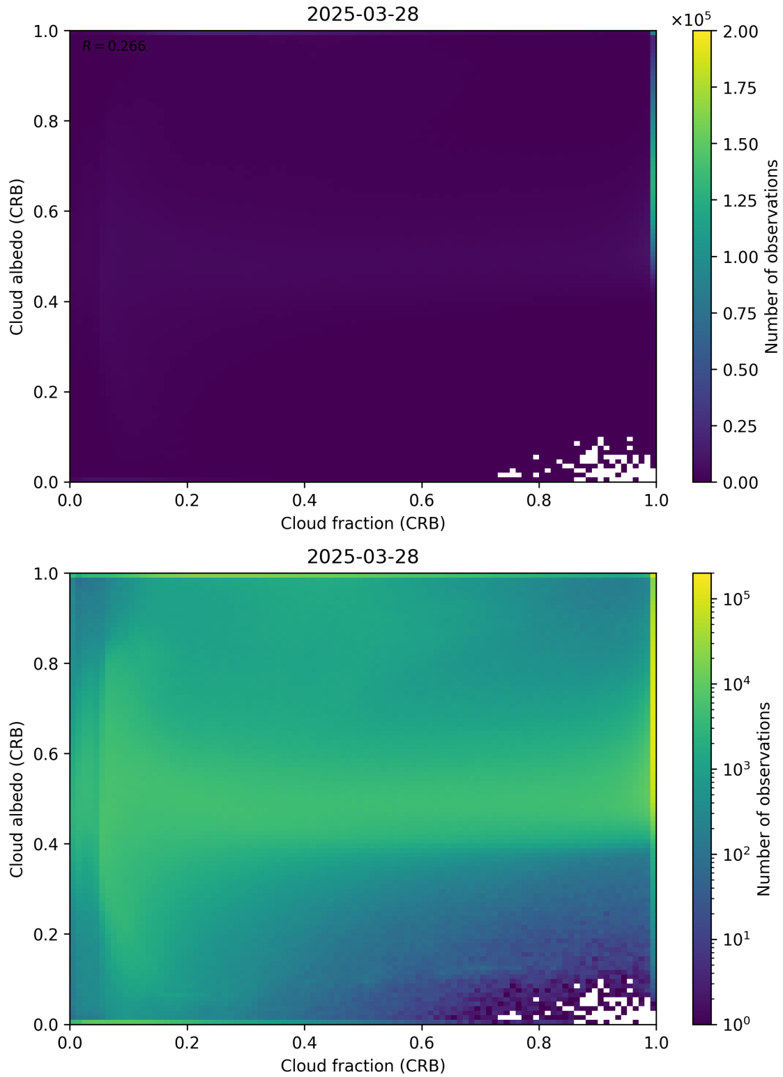
Figure 77: Scatter density plot of “Cloud fraction (CRB)” against “Cloud albedo (CRB)” for 2025-03-28 to 2025-03-29.
