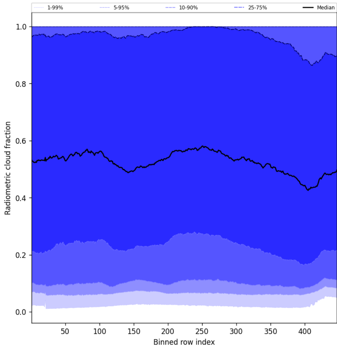
Figure 55: Along track statistics of “Radiometric cloud fraction” for 2025-03-28 to 2025-03-29
