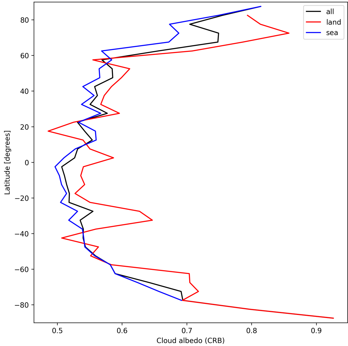
Figure 28: Zonal average of “Cloud albedo (CRB)” for 2025-03-28 to 2025-03-29.
