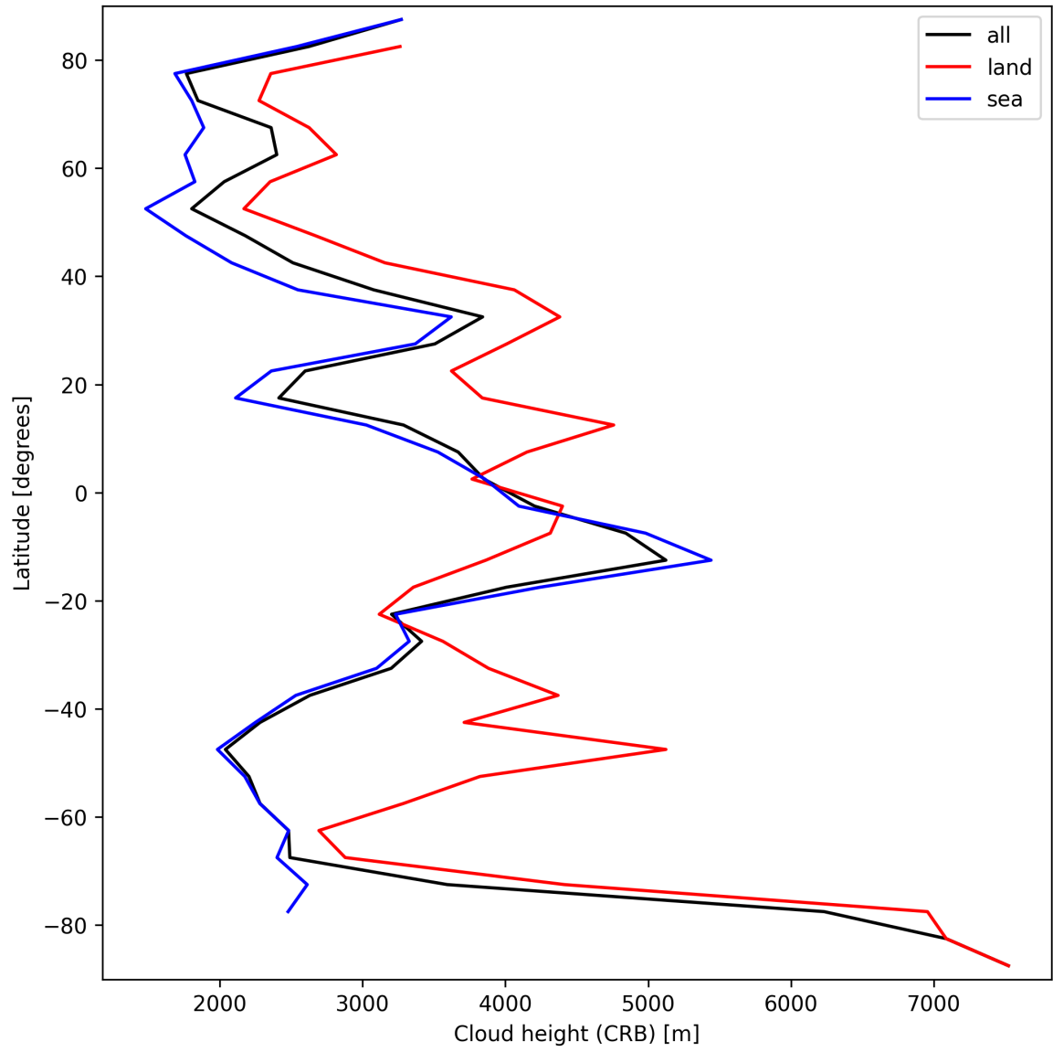
Figure 27: Zonal average of “Cloud height (CRB)” for 2025-03-28 to 2025-03-29.
