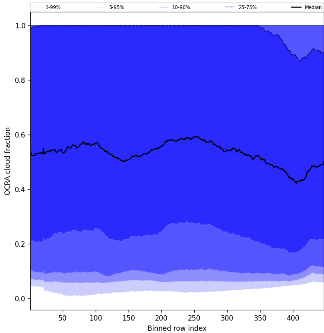
Figure 66: Along track statistics of “OCRA cloud fraction” for 2025-03-28 to 2025-03-29
