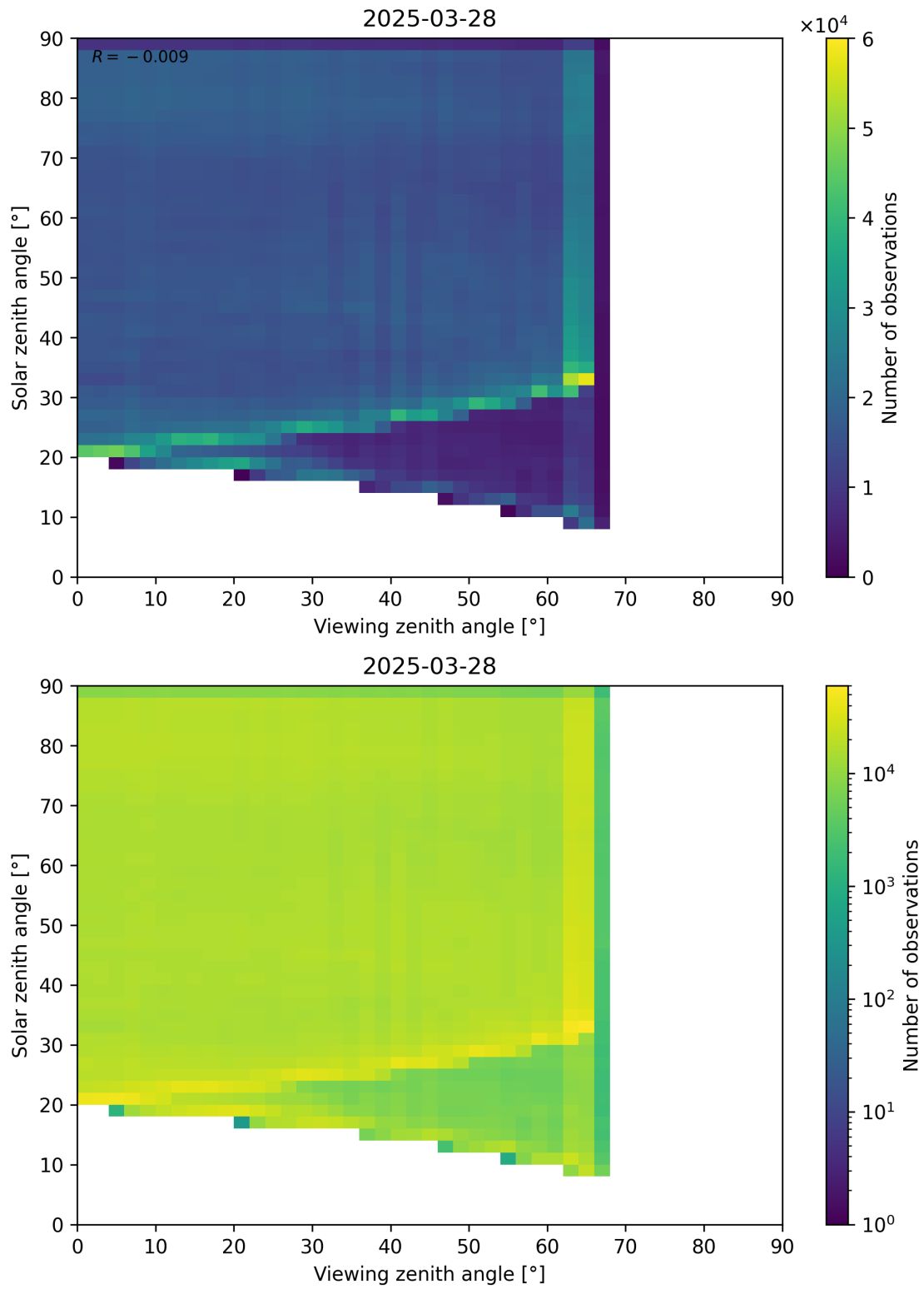
Figure 114: Scatter density plot of “Viewing zenith angle” against “Solar zenith angle” for 2025-03-28 to 2025-03-29.
