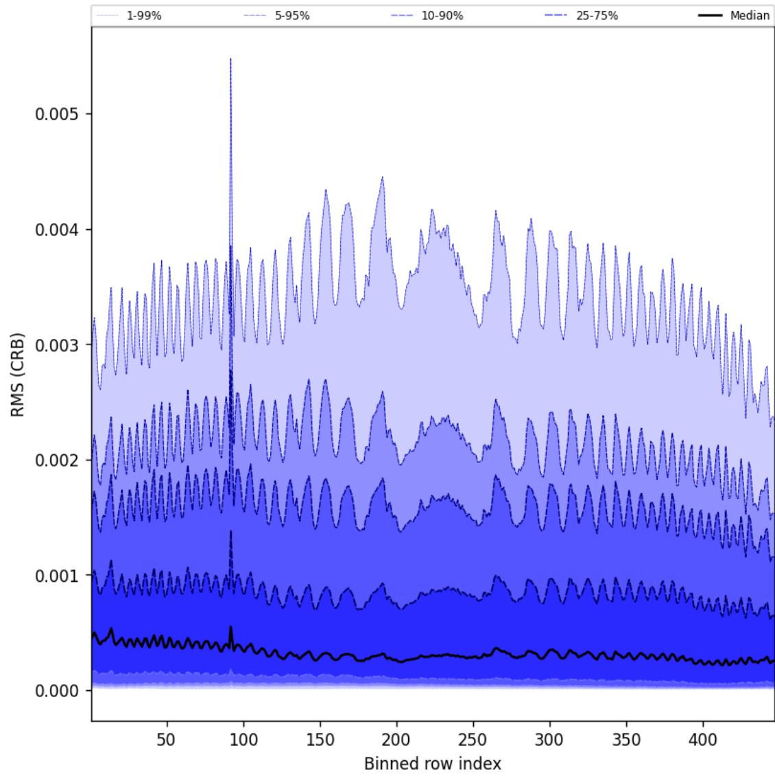
Figure 64: Along track statistics of “RMS (CRB)” for 2025-03-28 to 2025-03-29
