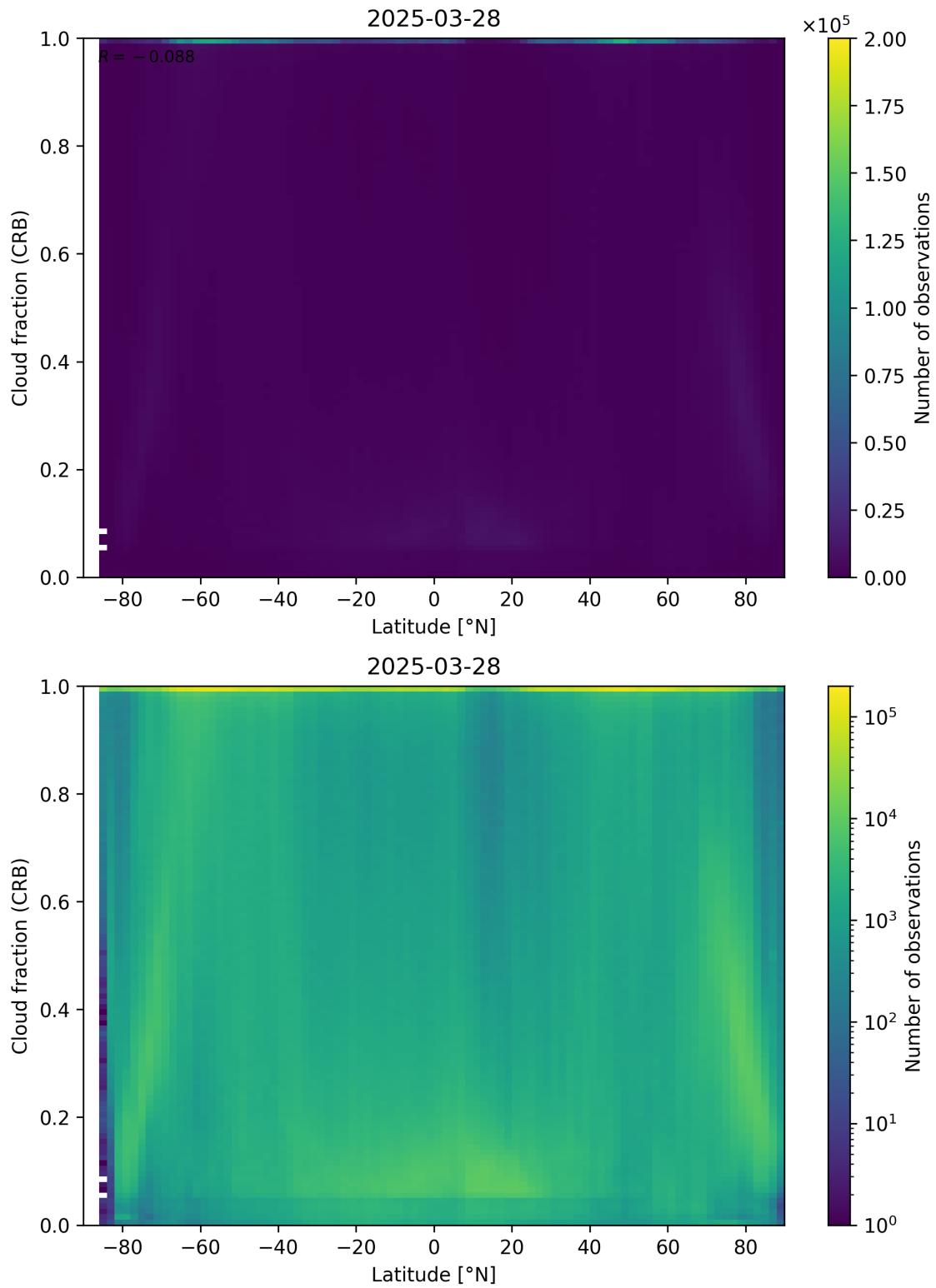
Figure 94: Scatter density plot of “Latitude” against “Cloud fraction (CRB)” for 2025-03-28 to 2025-03-29.
