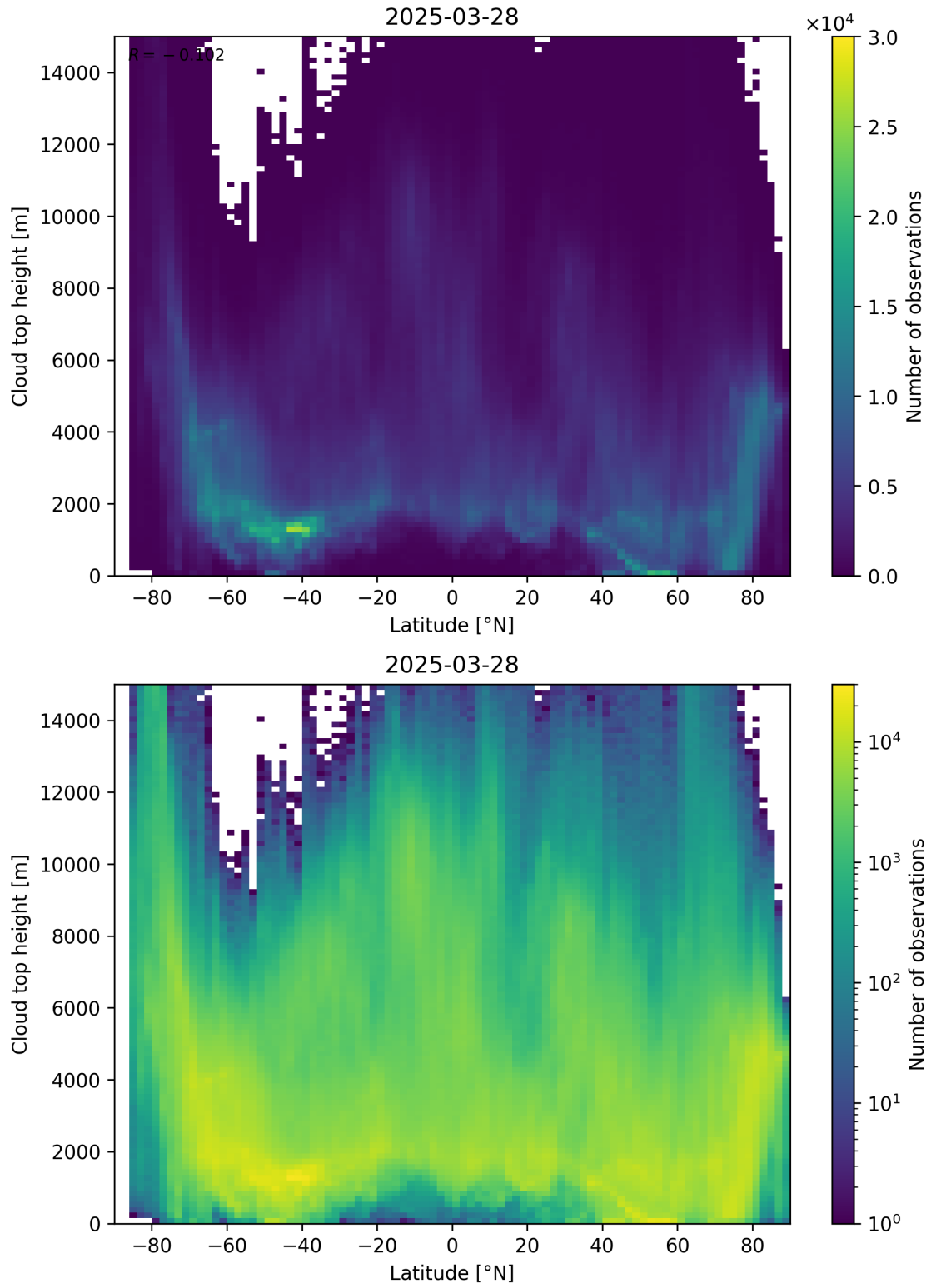
Figure 97: Scatter density plot of “Latitude” against “Cloud top height” for 2025-03-28 to 2025-03-29.
