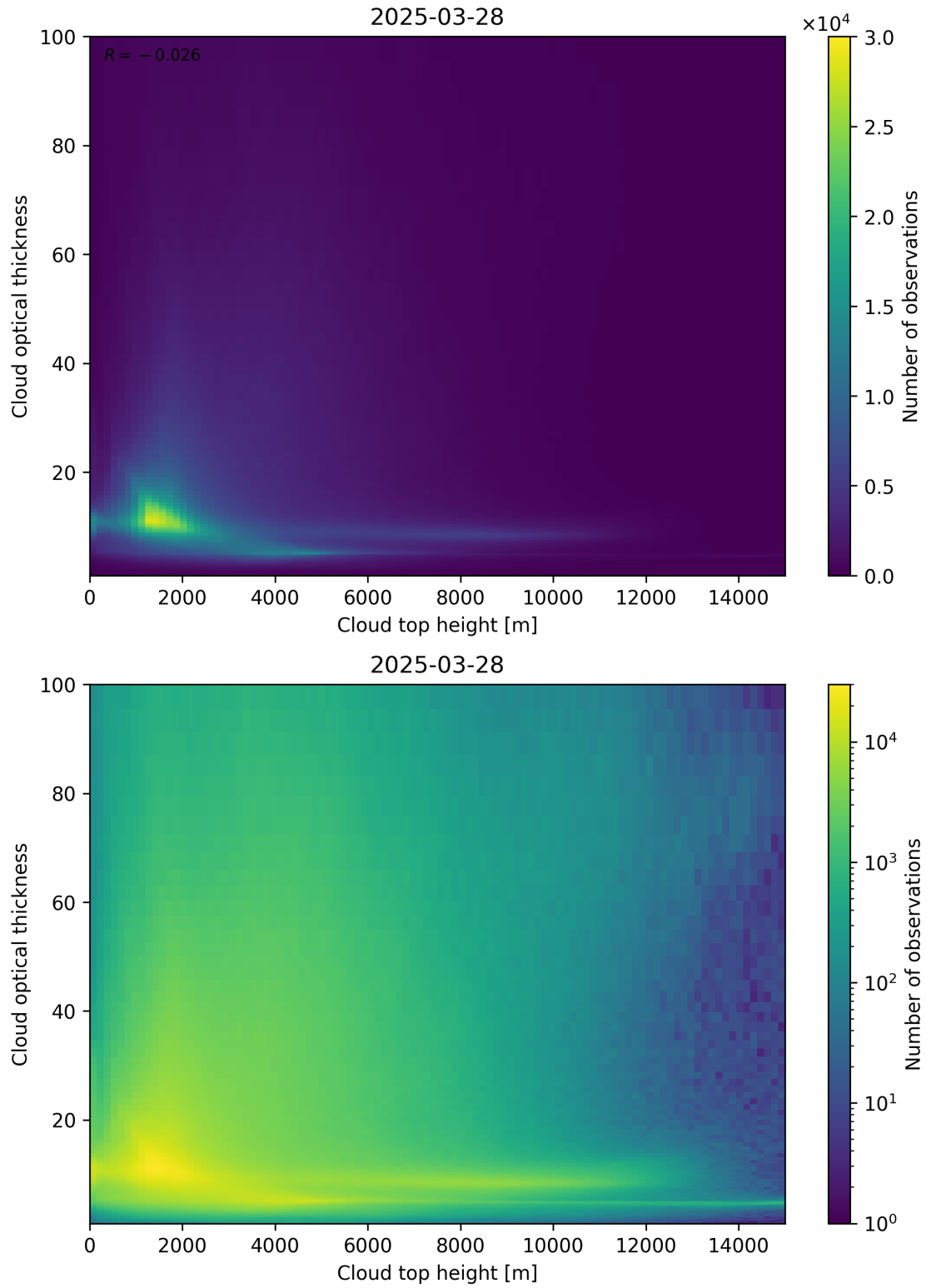
Figure 90: Scatter density plot of “Cloud top height” against “Cloud optical thickness” for 2025-03-28 to 2025-03-29.
