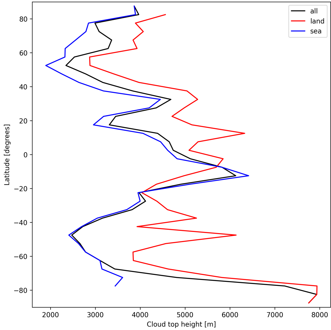
Figure 24: Zonal average of “Cloud top height” for 2025-03-28 to 2025-03-29.
