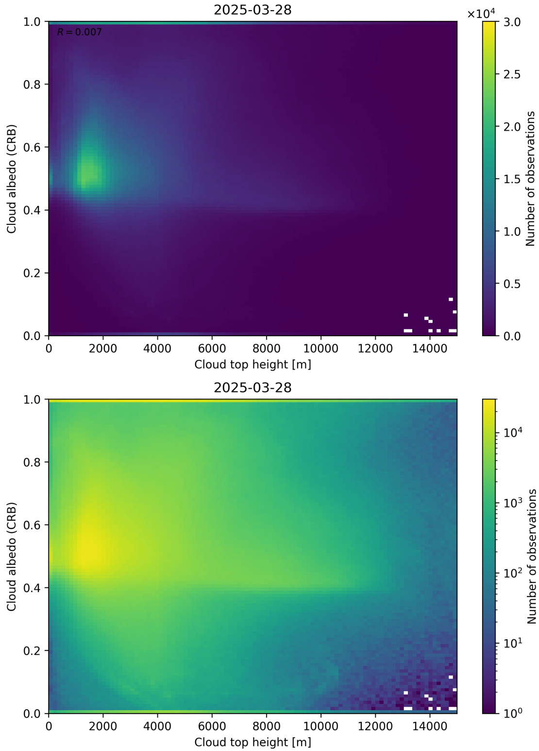
Figure 86: Scatter density plot of “Cloud top height” against “Cloud albedo (CRB)” for 2025-03-28 to 2025-03-29.
