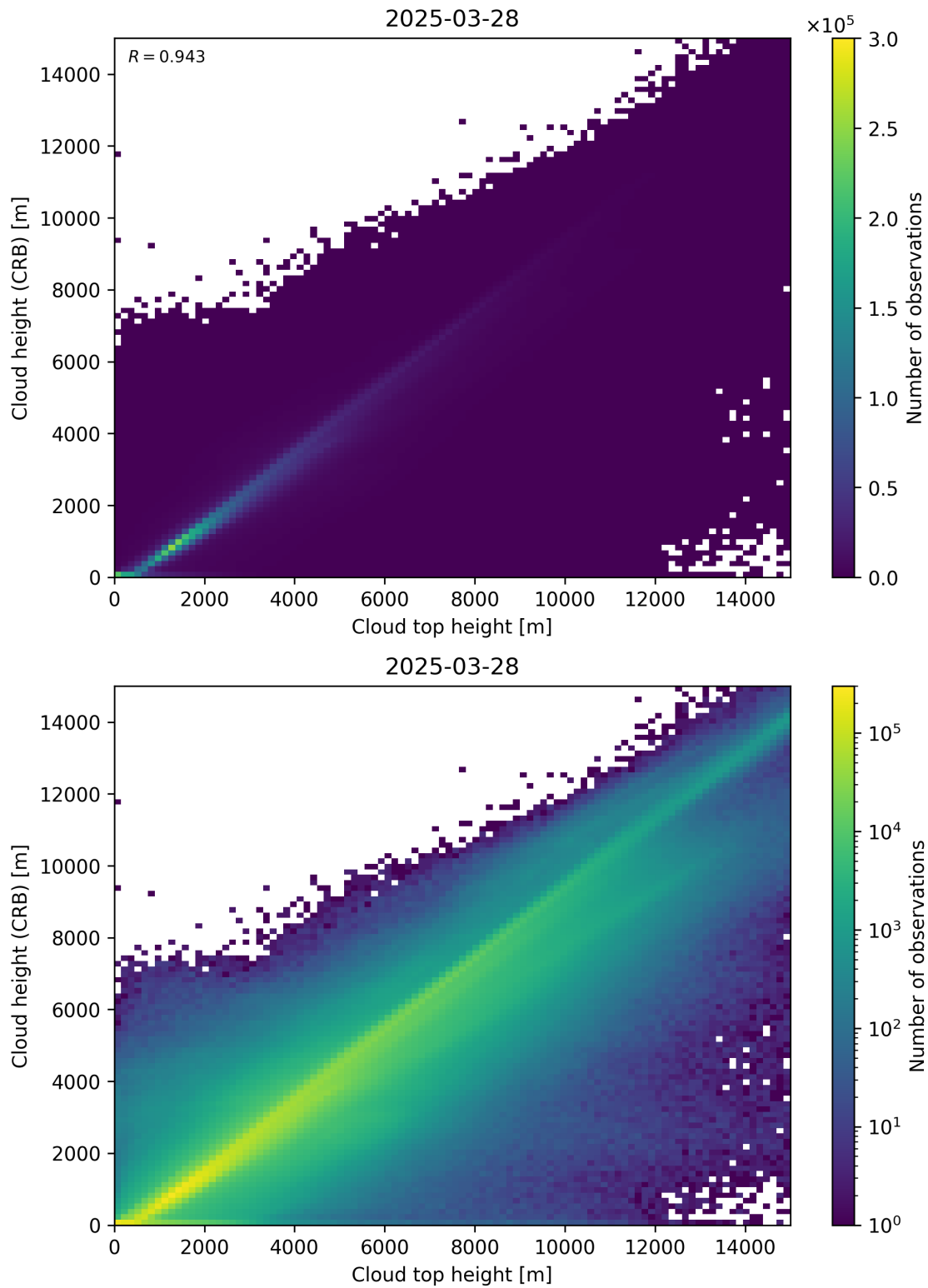
Figure 89: Scatter density plot of “Cloud top height” against “Cloud height (CRB)” for 2025-03-28 to 2025-03-29.
