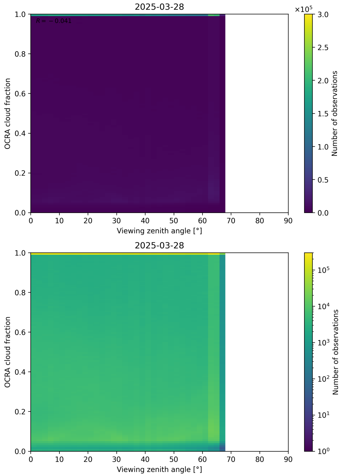
Figure 108: Scatter density plot of “Viewing zenith angle” against “OCRA cloud fraction” for 2025-03-28 to 2025-03-29.
