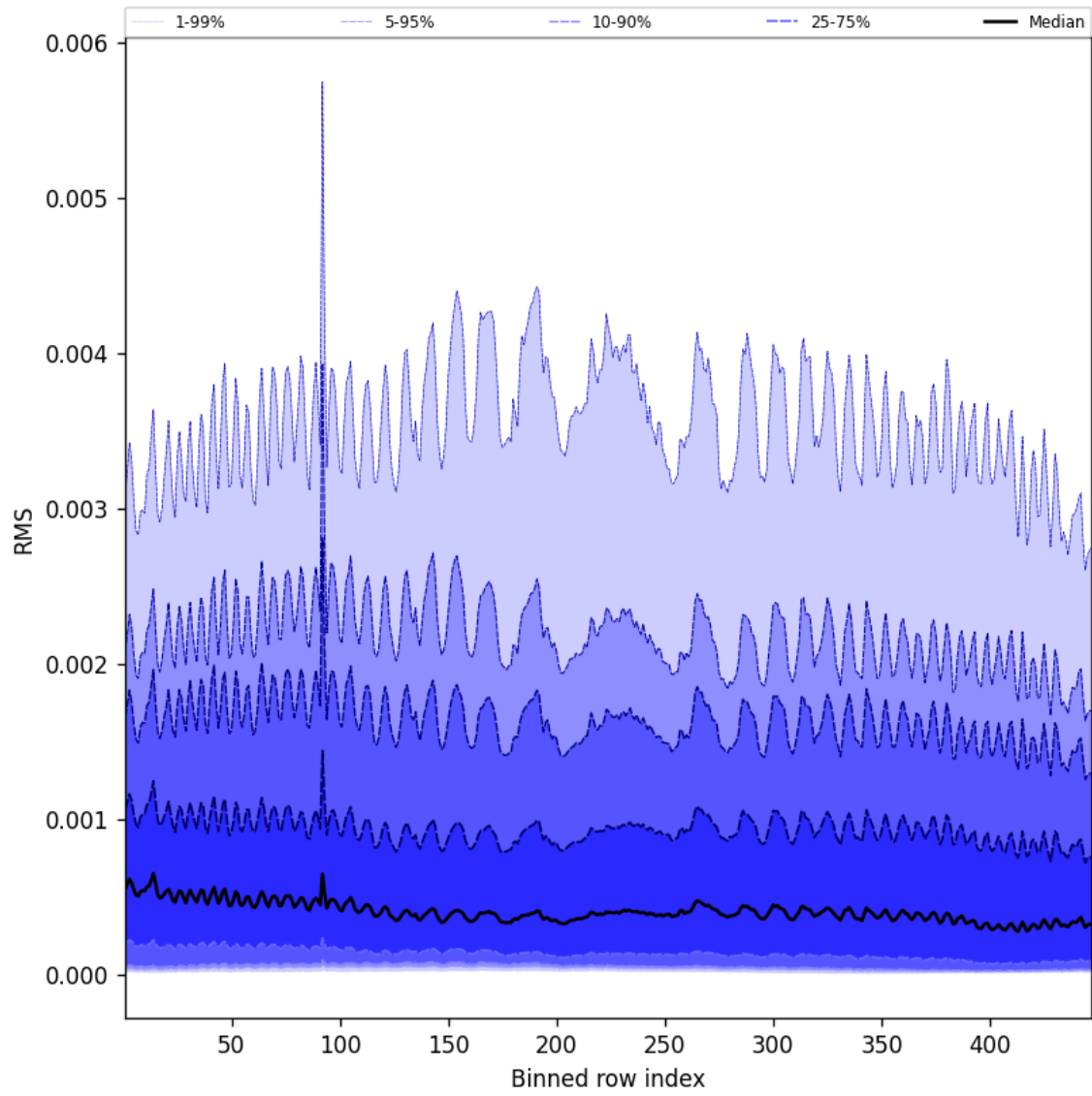
Figure 63: Along track statistics of “RMS” for 2025-03-28 to 2025-03-29
