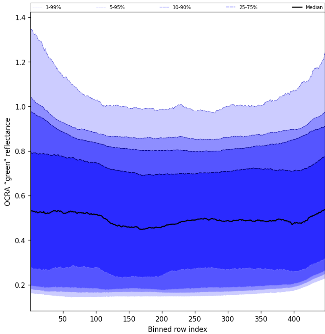
Figure 68: Along track statistics of “OCRA “green” reflectance” for 2025-03-28 to 2025-03-29
