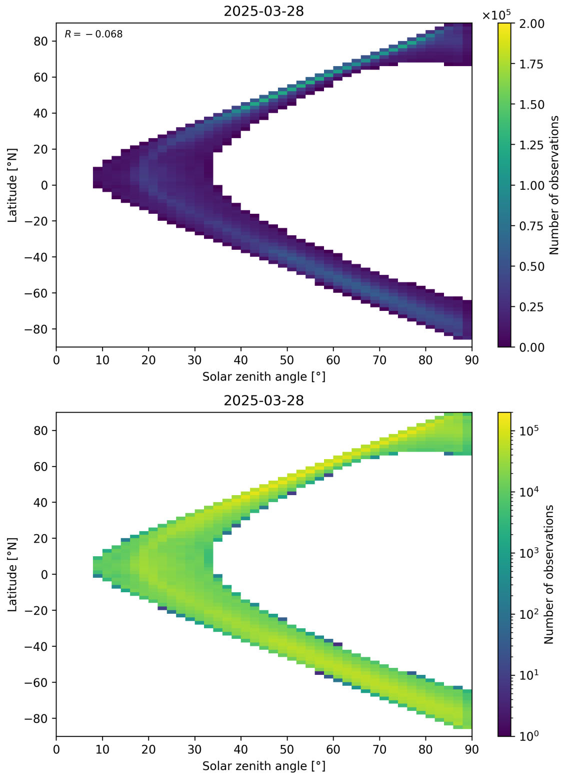
Figure 105: Scatter density plot of “Solar zenith angle” against “Latitude” for 2025-03-28 to 2025-03-29.
