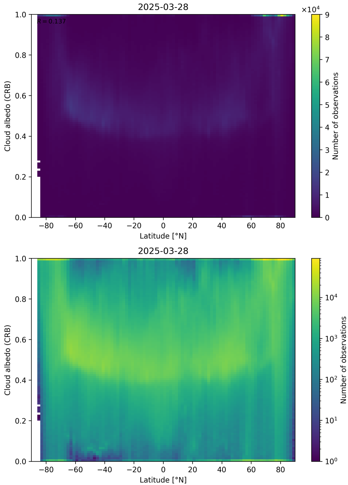
Figure 91: Scatter density plot of “Latitude” against “Cloud albedo (CRB)” for 2025-03-28 to 2025-03-29.
