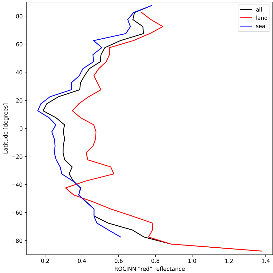
Figure 37: Zonal average of "ROCINN "red" reflectance" for 2025-03-28 to 2025-03-29.
