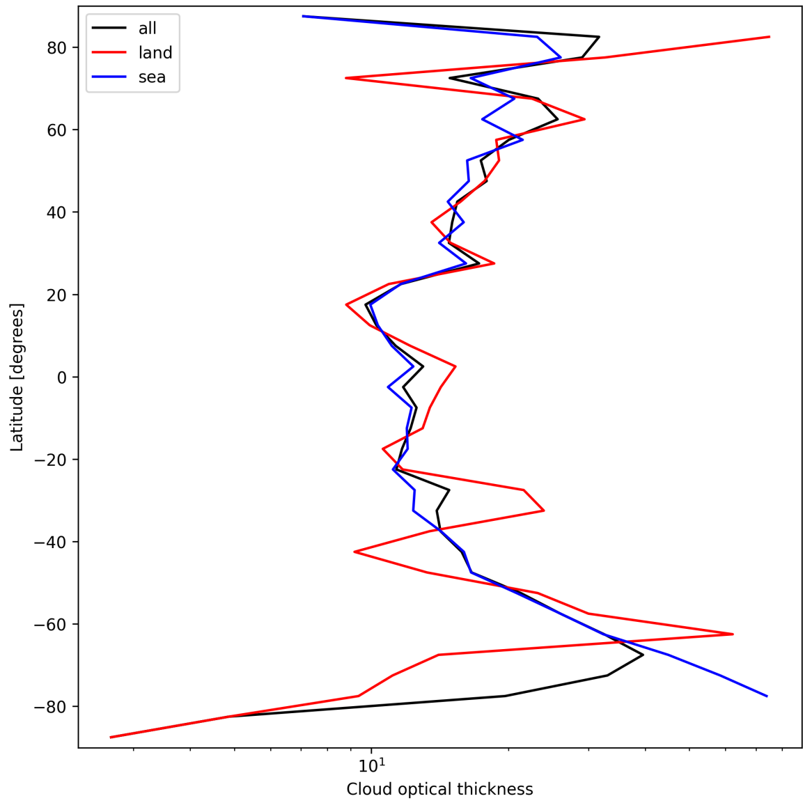
Figure 25: Zonal average of “Cloud optical thickness” for 2025-03-28 to 2025-03-29.
