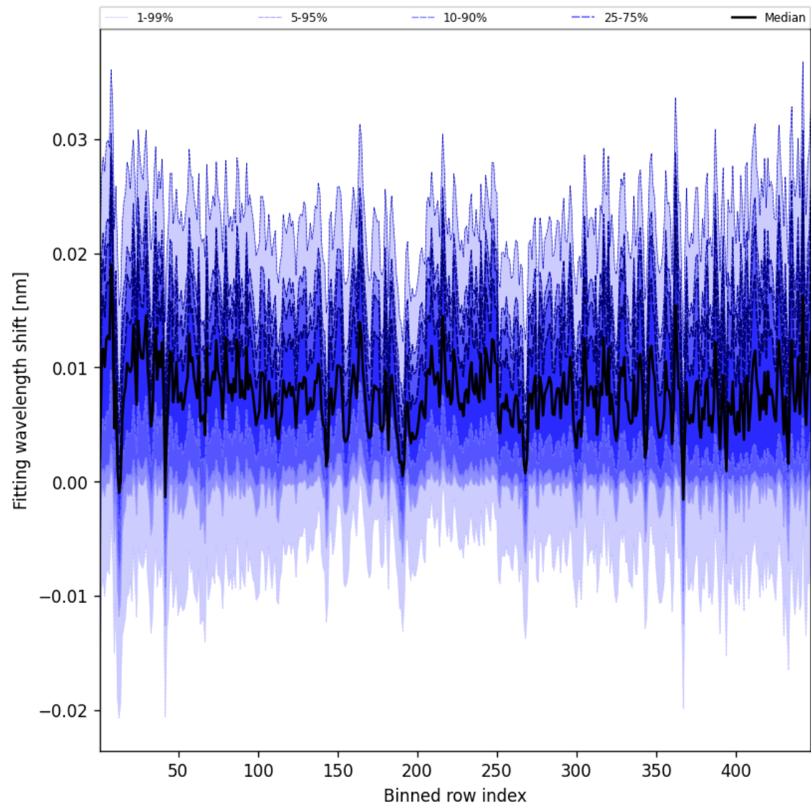
Figure 65: Along track statistics of “Fitting wavelength shift” for 2025-03-28 to 2025-03-29
