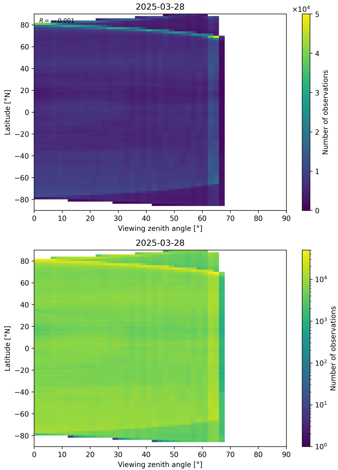
Figure 113: Scatter density plot of “Viewing zenith angle” against “Latitude” for 2025-03-28 to 2025-03-29.
