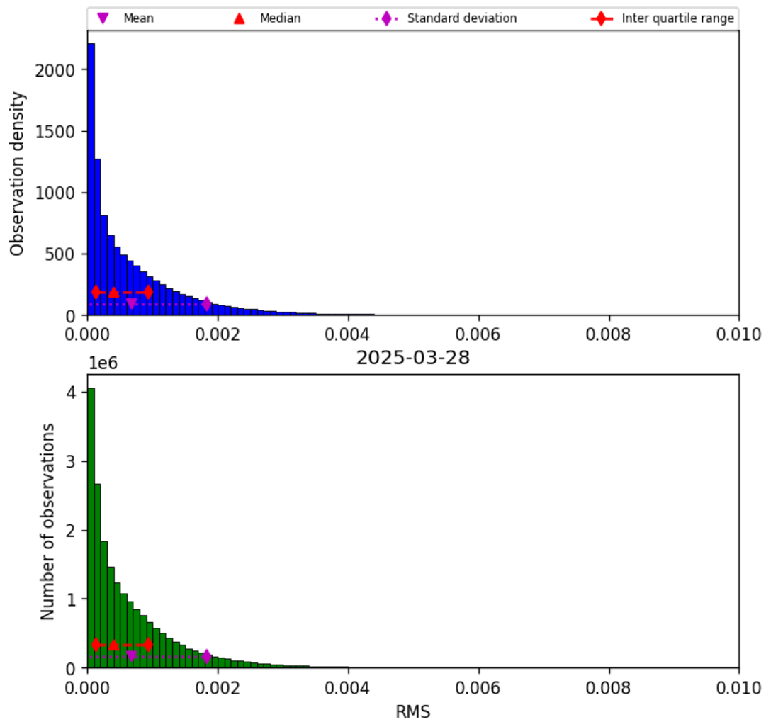
Figure 47: Histogram of “RMS” for 2025-03-28 to 2025-03-29
