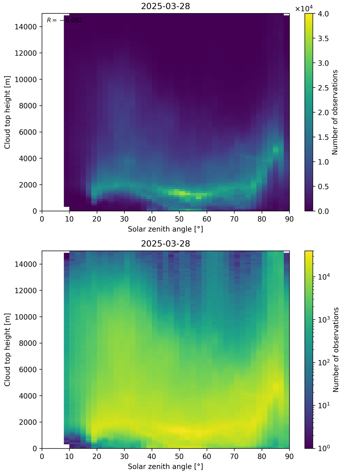
Figure 104: Scatter density plot of “Solar zenith angle” against “Cloud top height” for 2025-03-28 to 2025-03-29.
