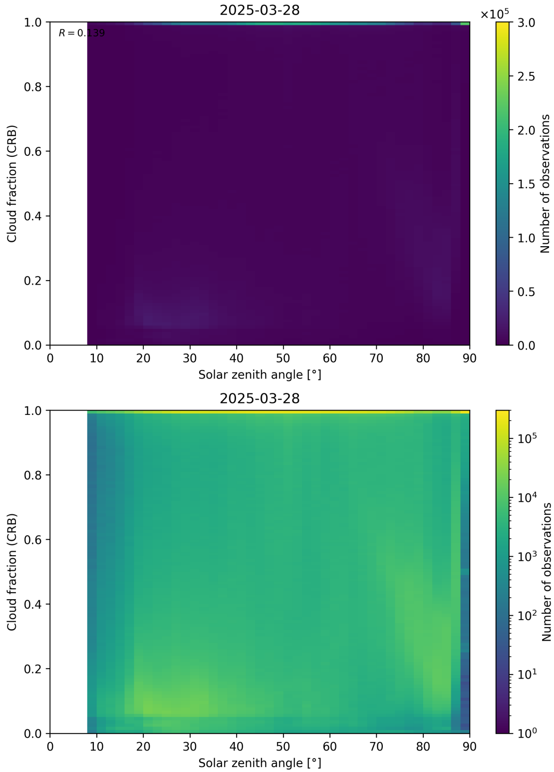
Figure 101: Scatter density plot of “Solar zenith angle” against “Cloud fraction (CRB)” for 2025-03-28 to 2025-03-29.
