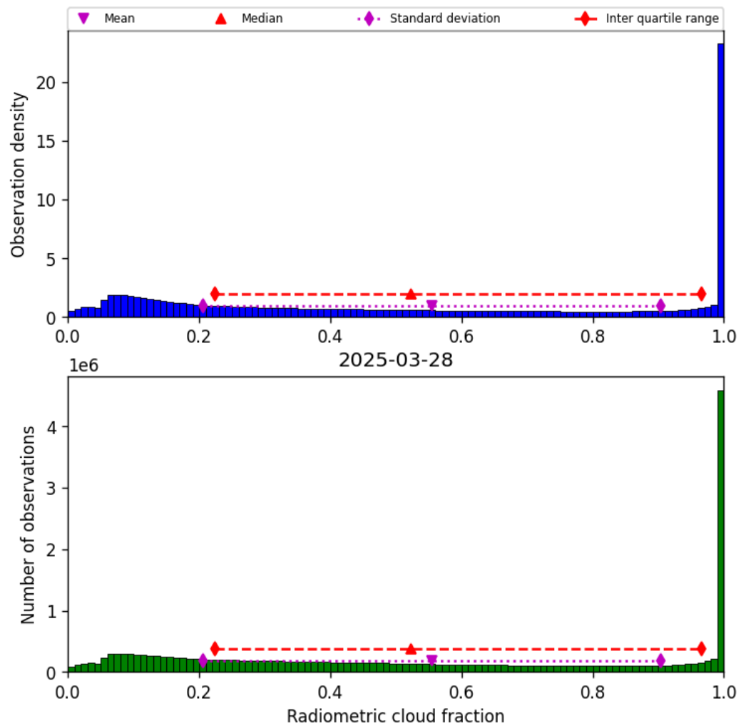
Figure 39: Histogram of “Radiometric cloud fraction” for 2025-03-28 to 2025-03-29
