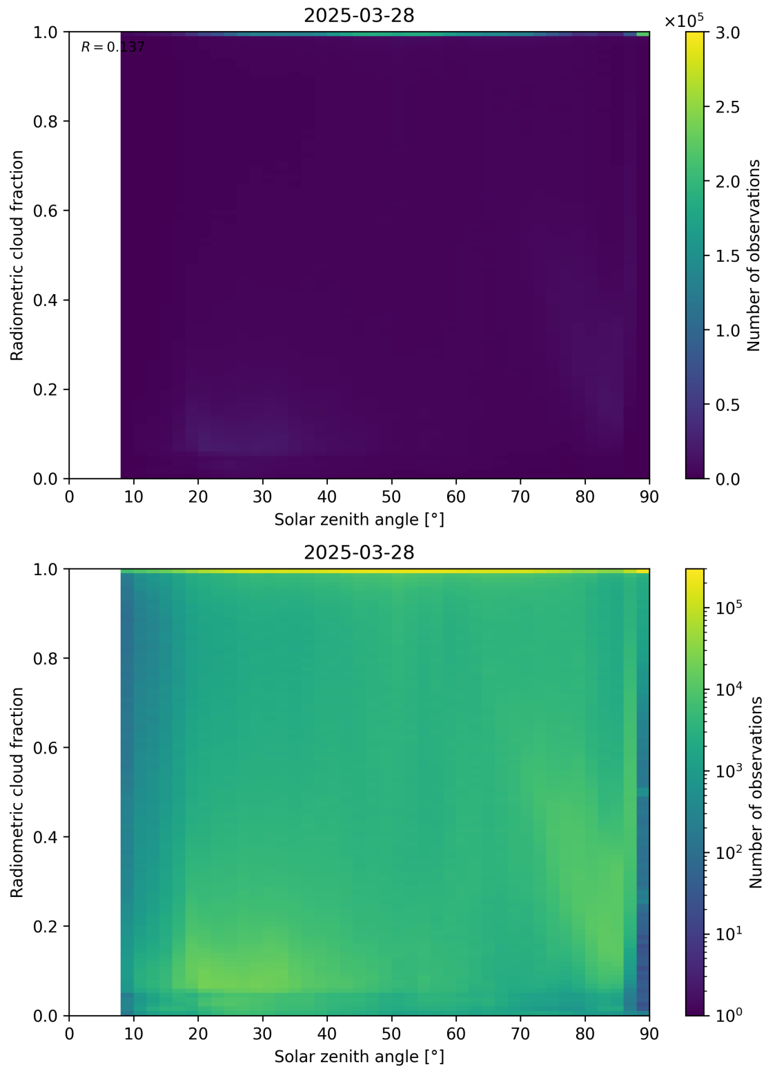
Figure 99: Scatter density plot of “Solar zenith angle” against “Radiometric cloud fraction” for 2025-03-28 to 2025-03-29.
