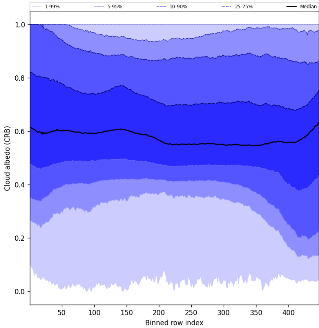
Figure 60: Along track statistics of “Cloud albedo (CRB)” for 2025-03-28 to 2025-03-29
