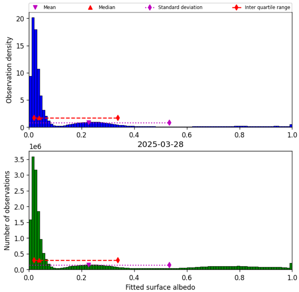
Figure 45: Histogram of “Fitted surface albedo” for 2025-03-28 to 2025-03-29
