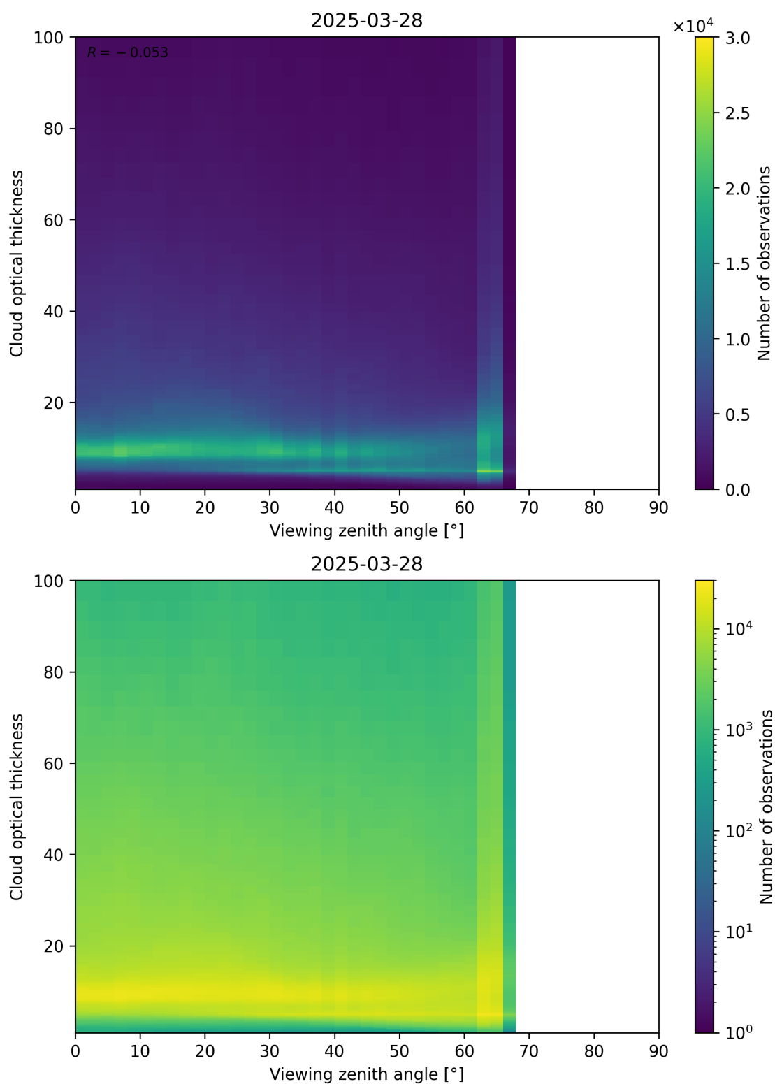
Figure 111: Scatter density plot of “Viewing zenith angle” against “Cloud optical thickness” for 2025-03-28 to 2025-03-29.
