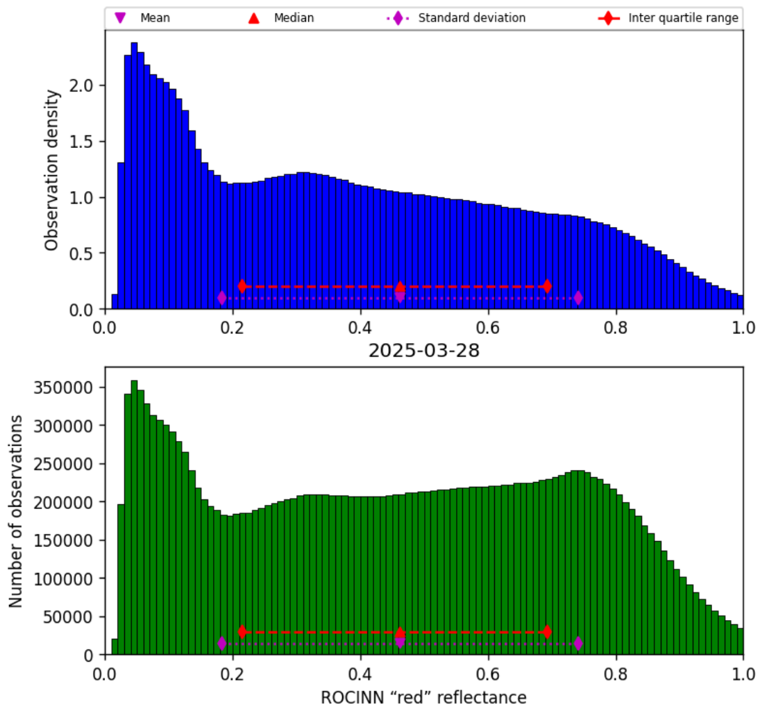
Figure 53: Histogram of “ROCINN “red” reflectance” for 2025-03-28 to 2025-03-29
