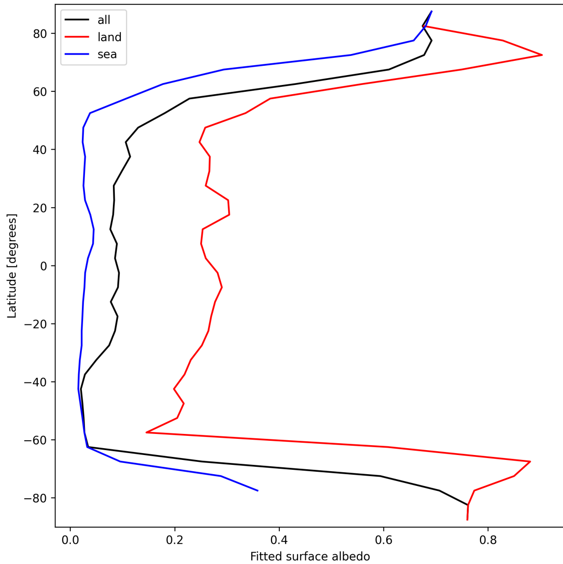
Figure 29: Zonal average of “Fitted surface albedo” for 2025-03-28 to 2025-03-29.
