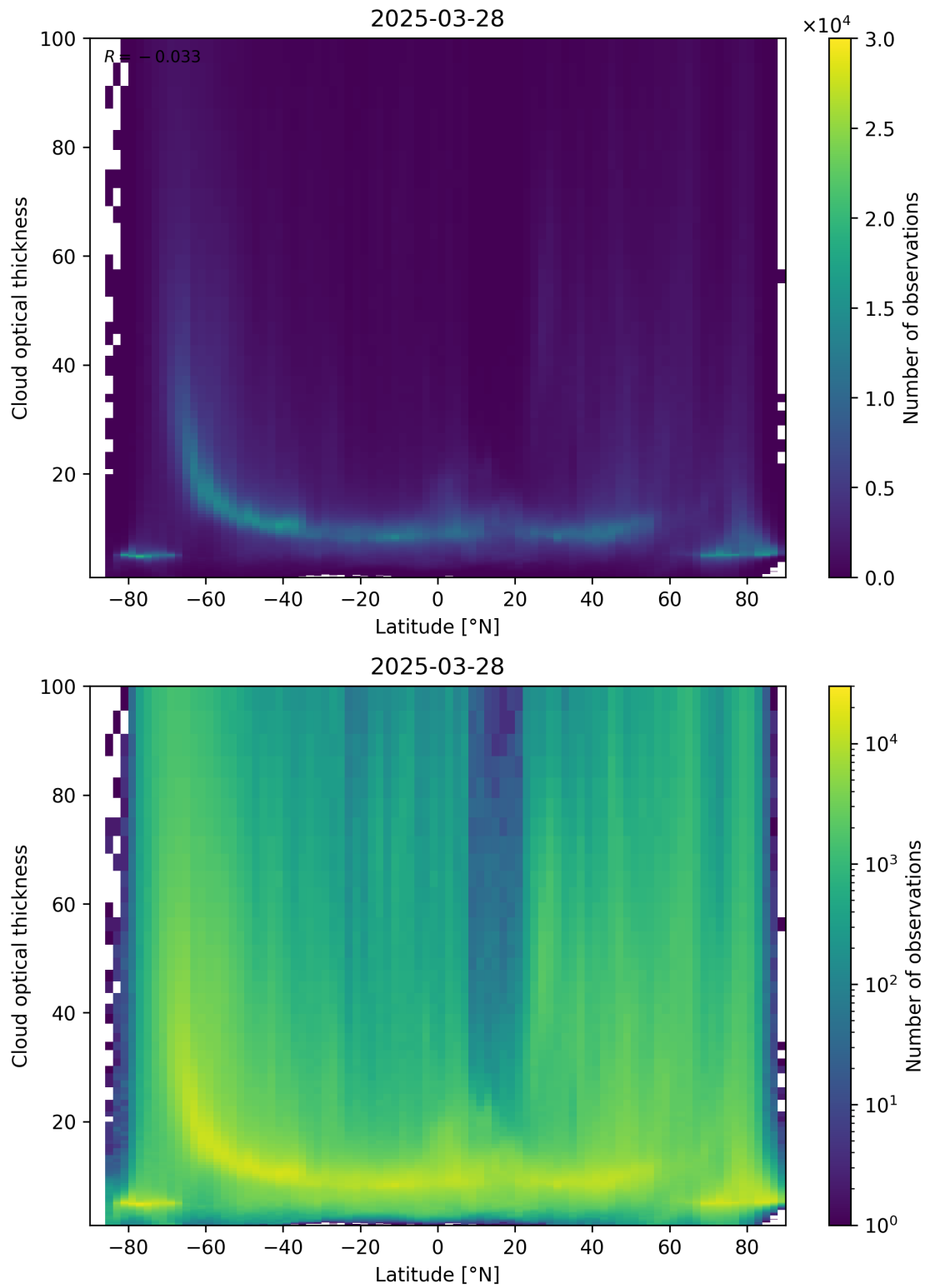
Figure 96: Scatter density plot of “Latitude” against “Cloud optical thickness” for 2025-03-28 to 2025-03-29.
