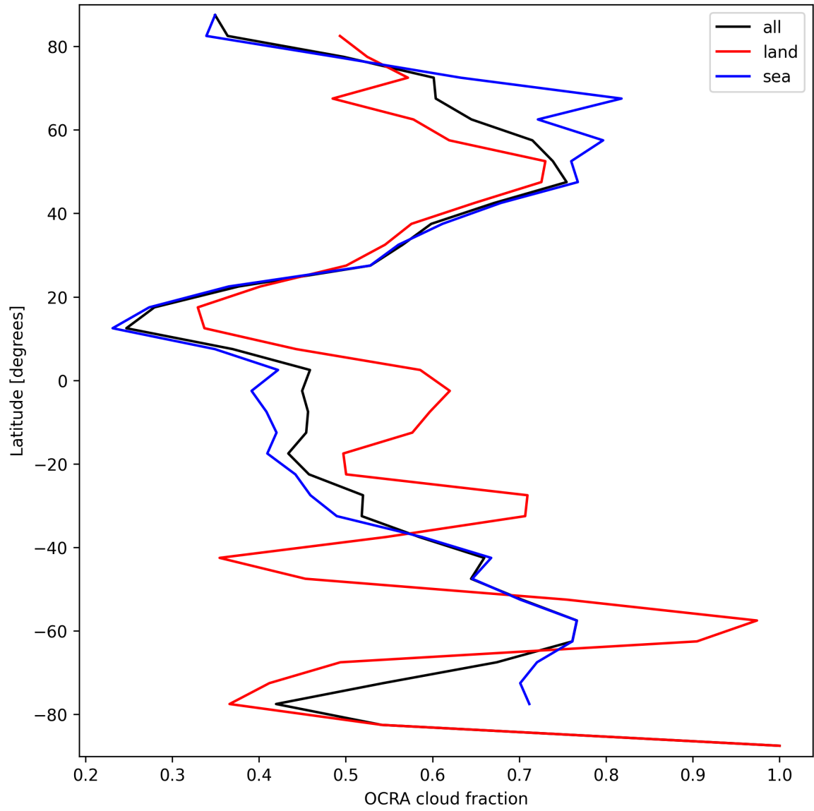
Figure 34: Zonal average of “OCRA cloud fraction” for 2025-03-28 to 2025-03-29.
