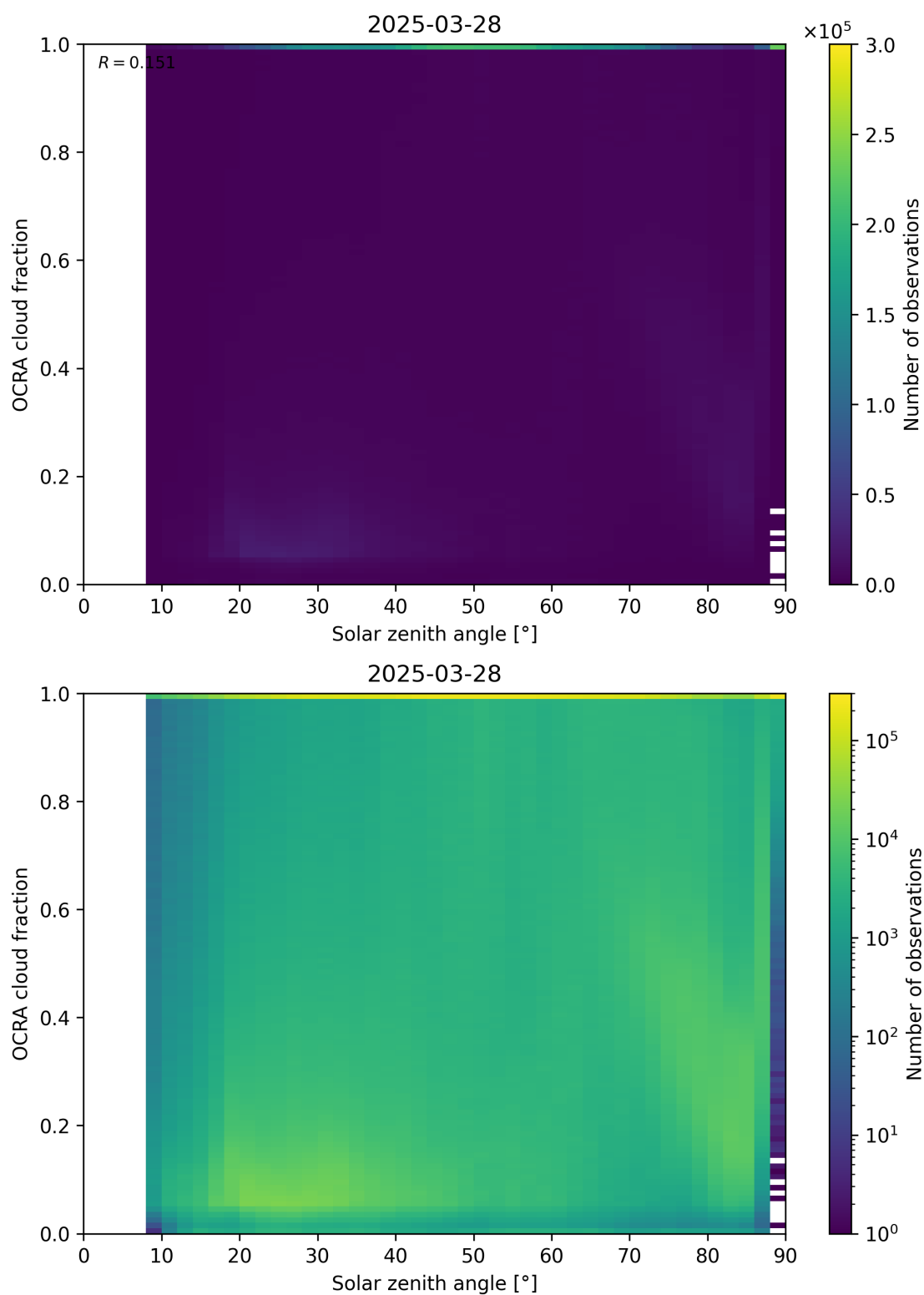
Figure 100: Scatter density plot of “Solar zenith angle” against “OCRA cloud fraction” for 2025-03-28 to 2025-03-29.
