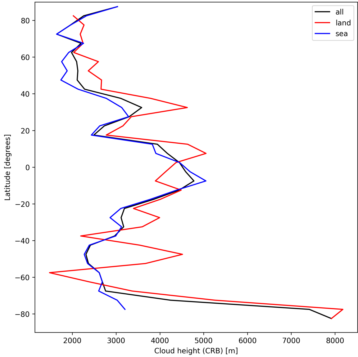
Figure 27: Zonal average of “Cloud height (CRB)” for 2025-03-30 to 2025-04-01.
