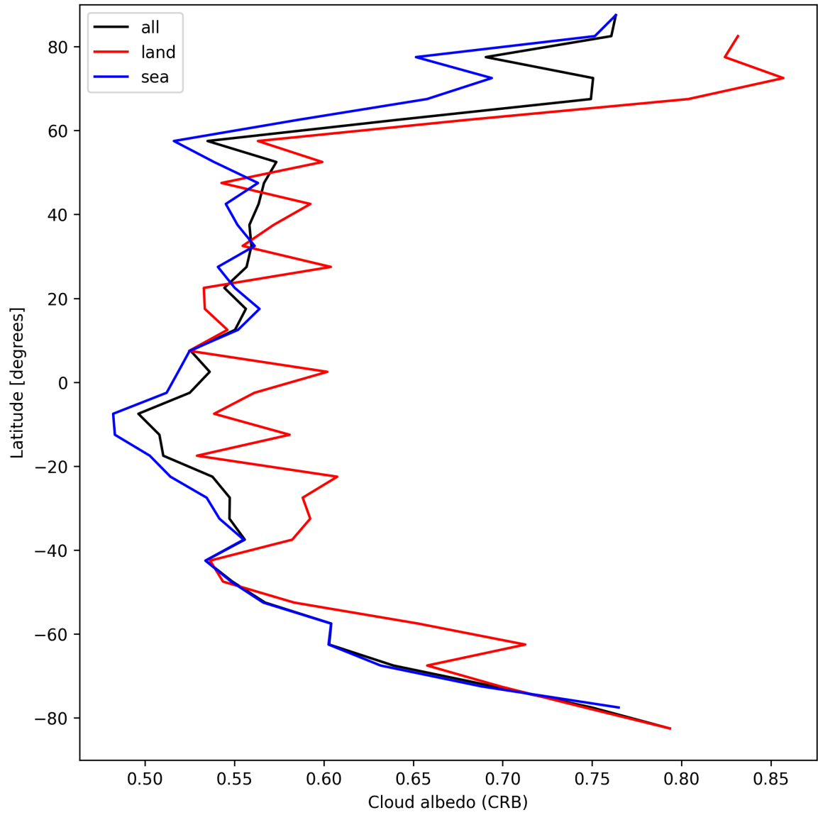
Figure 28: Zonal average of “Cloud albedo (CRB)” for 2025-03-30 to 2025-04-01.
