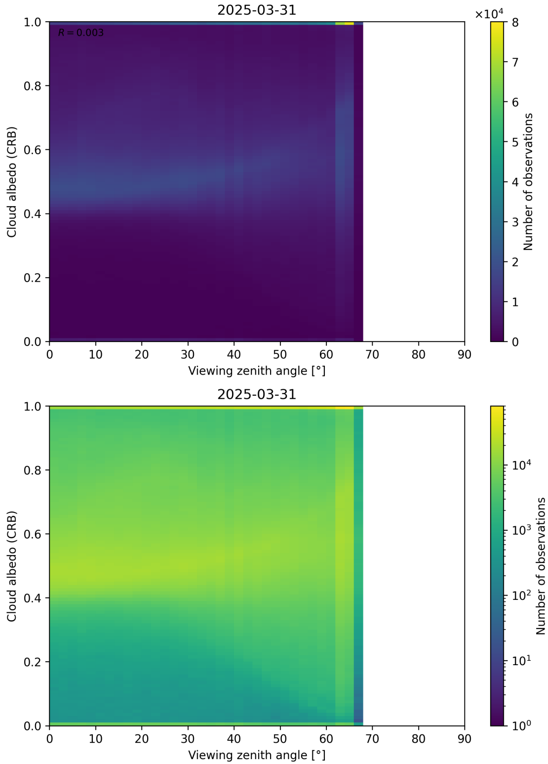
Figure 106: Scatter density plot of “Viewing zenith angle” against “Cloud albedo (CRB)” for 2025-03-30 to 2025-04-01.
