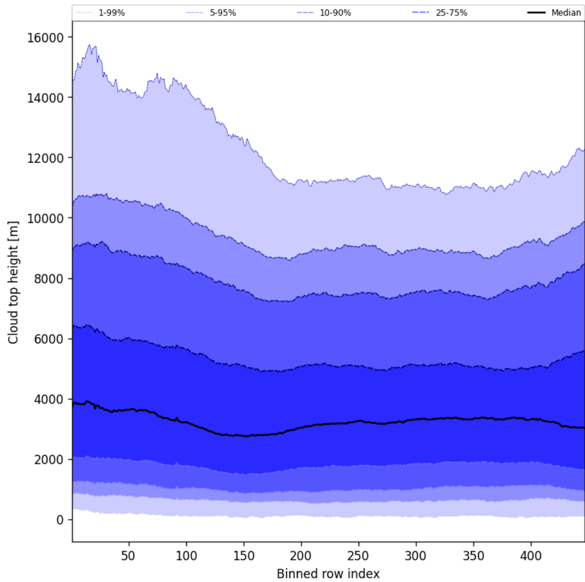
Figure 56: Along track statistics of “Cloud top height” for 2025-03-30 to 2025-04-01
