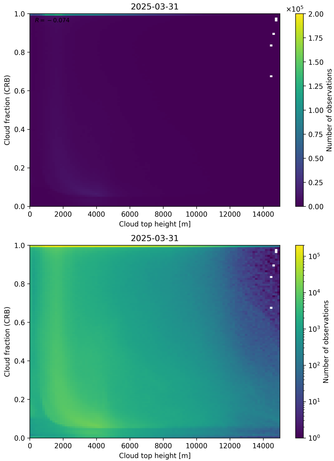
Figure 88: Scatter density plot of “Cloud top height” against “Cloud fraction (CRB)” for 2025-03-30 to 2025-04-01.
