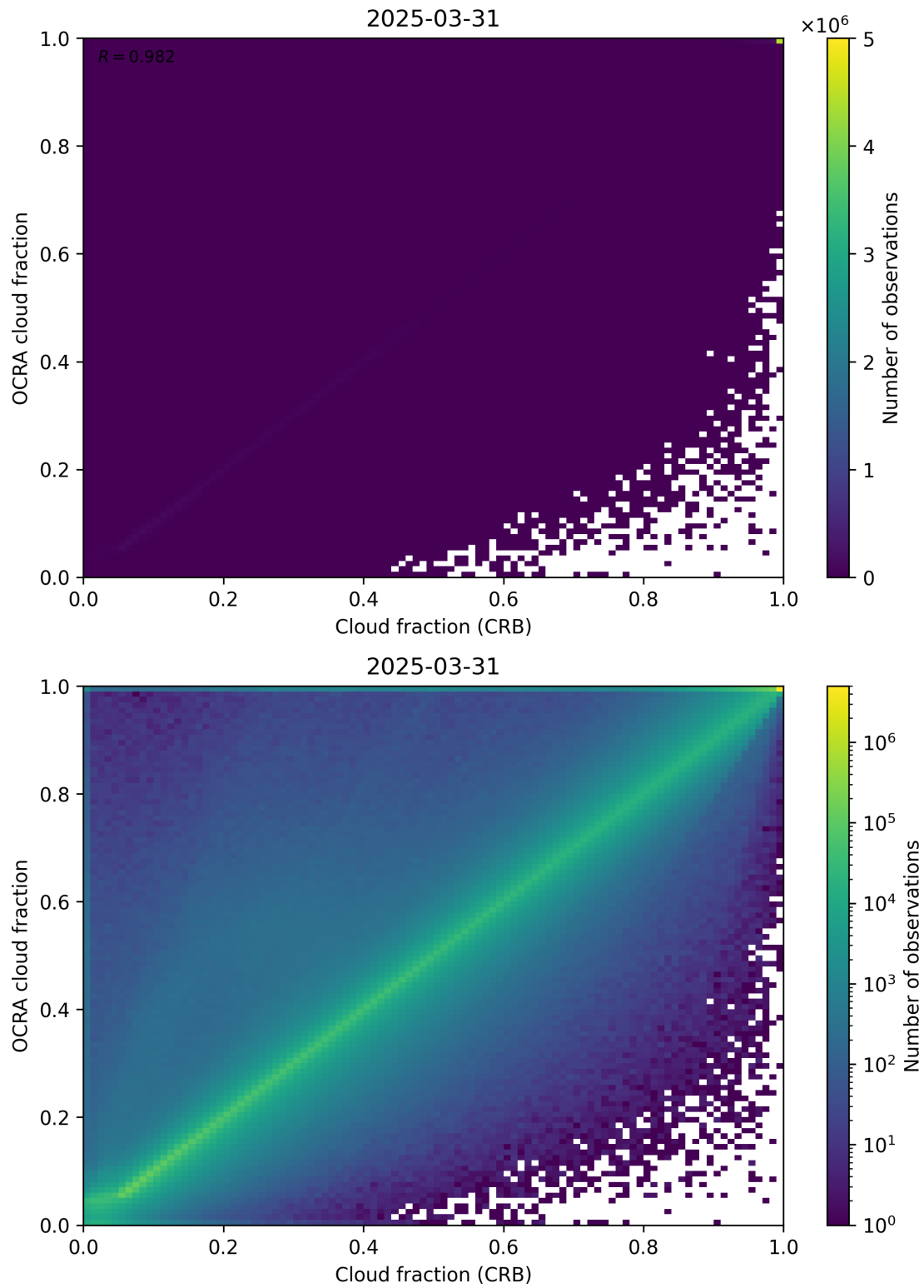
Figure 78: Scatter density plot of “Cloud fraction (CRB)” against “OCRA cloud fraction” for 2025-03-30 to 2025-04-01.
