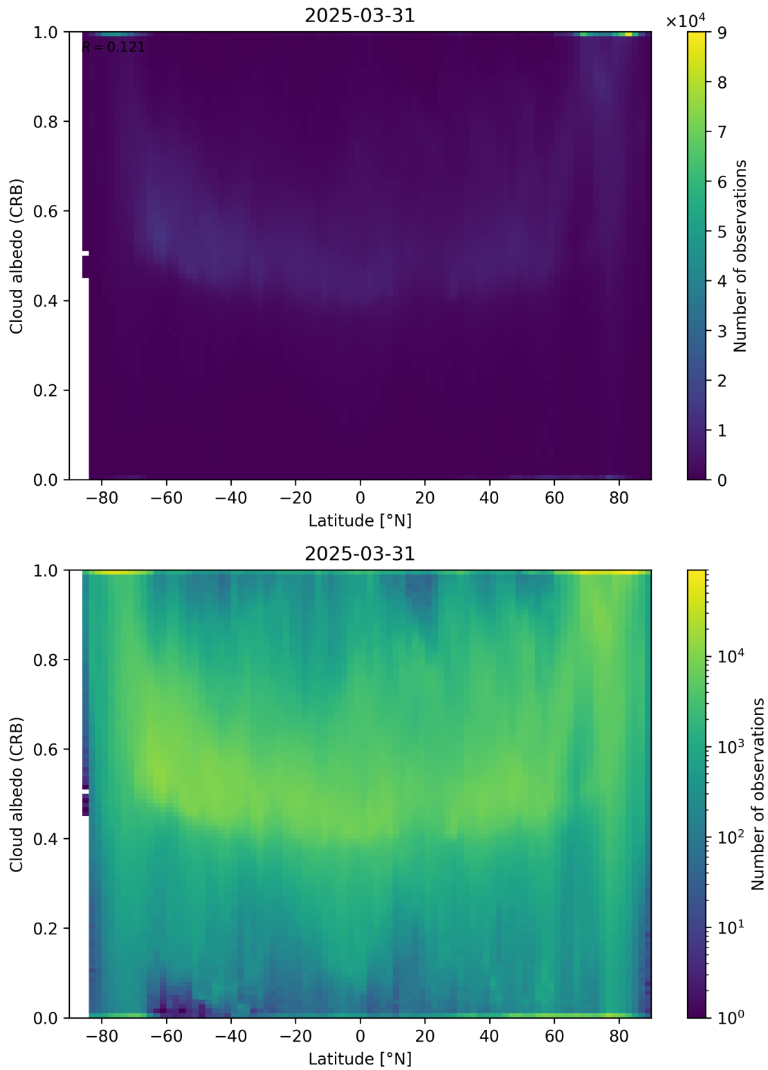
Figure 91: Scatter density plot of “Latitude” against “Cloud albedo (CRB)” for 2025-03-30 to 2025-04-01.
