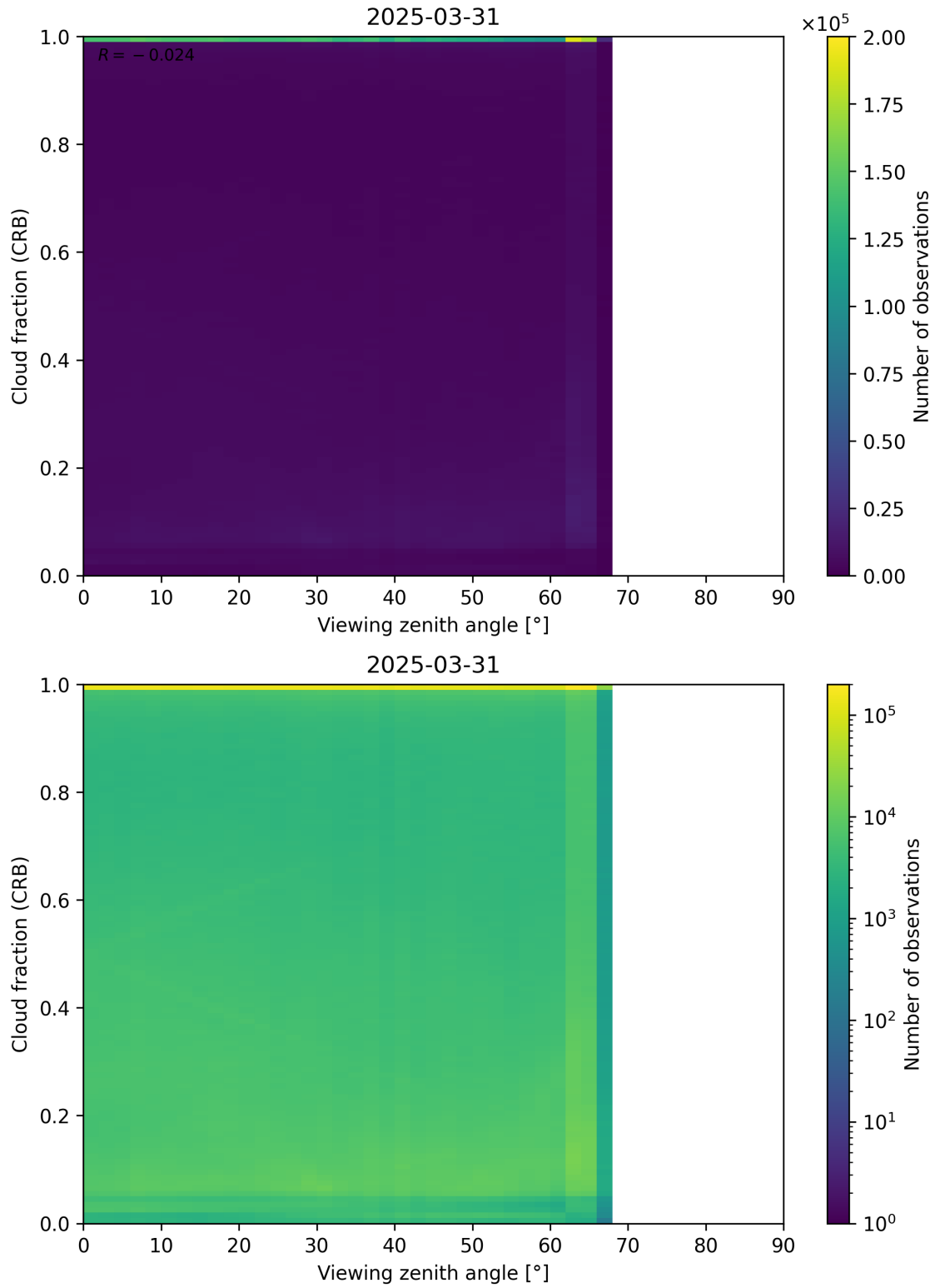
Figure 109: Scatter density plot of “Viewing zenith angle” against “Cloud fraction (CRB)” for 2025-03-30 to 2025-04-01.
