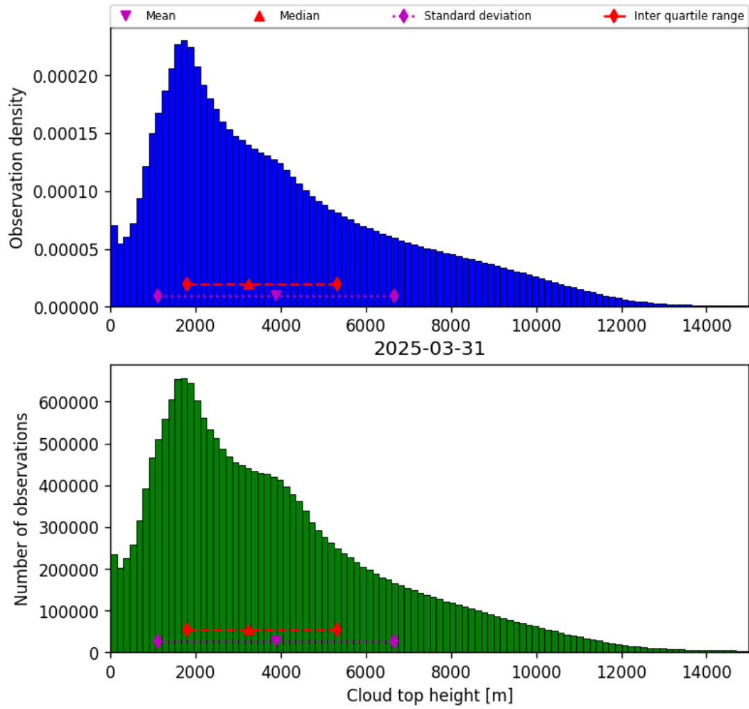
Figure 40: Histogram of “Cloud top height” for 2025-03-30 to 2025-04-01
