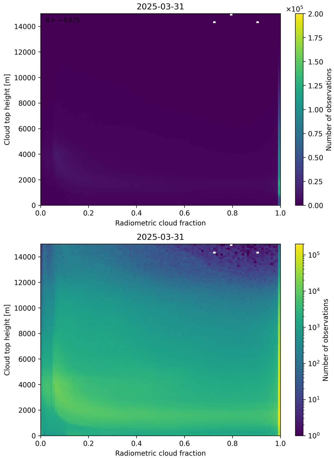
Figure 76: Scatter density plot of “Radiometric cloud fraction” against “Cloud top height” for 2025-03-30 to 2025-04-01.
