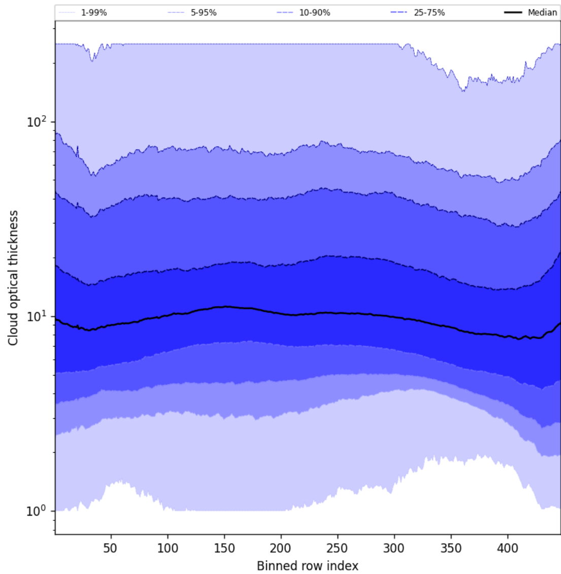
Figure 57: Along track statistics of “Cloud optical thickness” for 2025-03-30 to 2025-04-01
