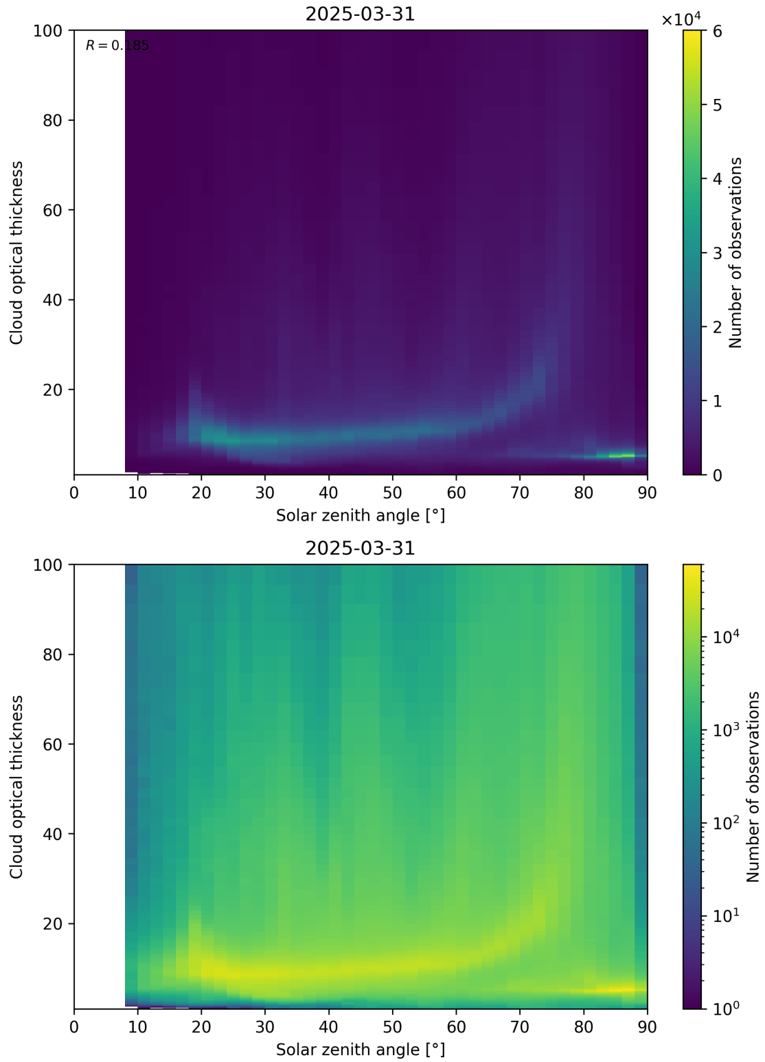
Figure 103: Scatter density plot of “Solar zenith angle” against “Cloud optical thickness” for 2025-03-30 to 2025-04-01.
