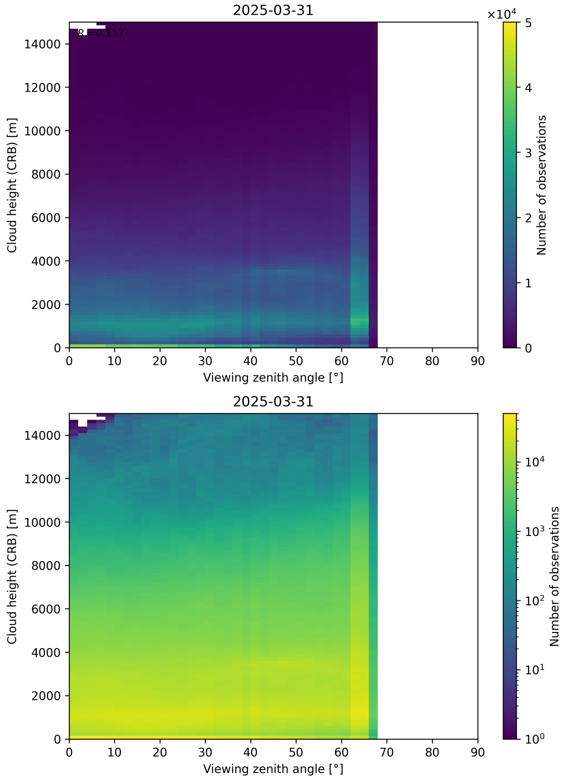
Figure 110: Scatter density plot of “Viewing zenith angle” against “Cloud height (CRB)” for 2025-03-30 to 2025-04-01.
