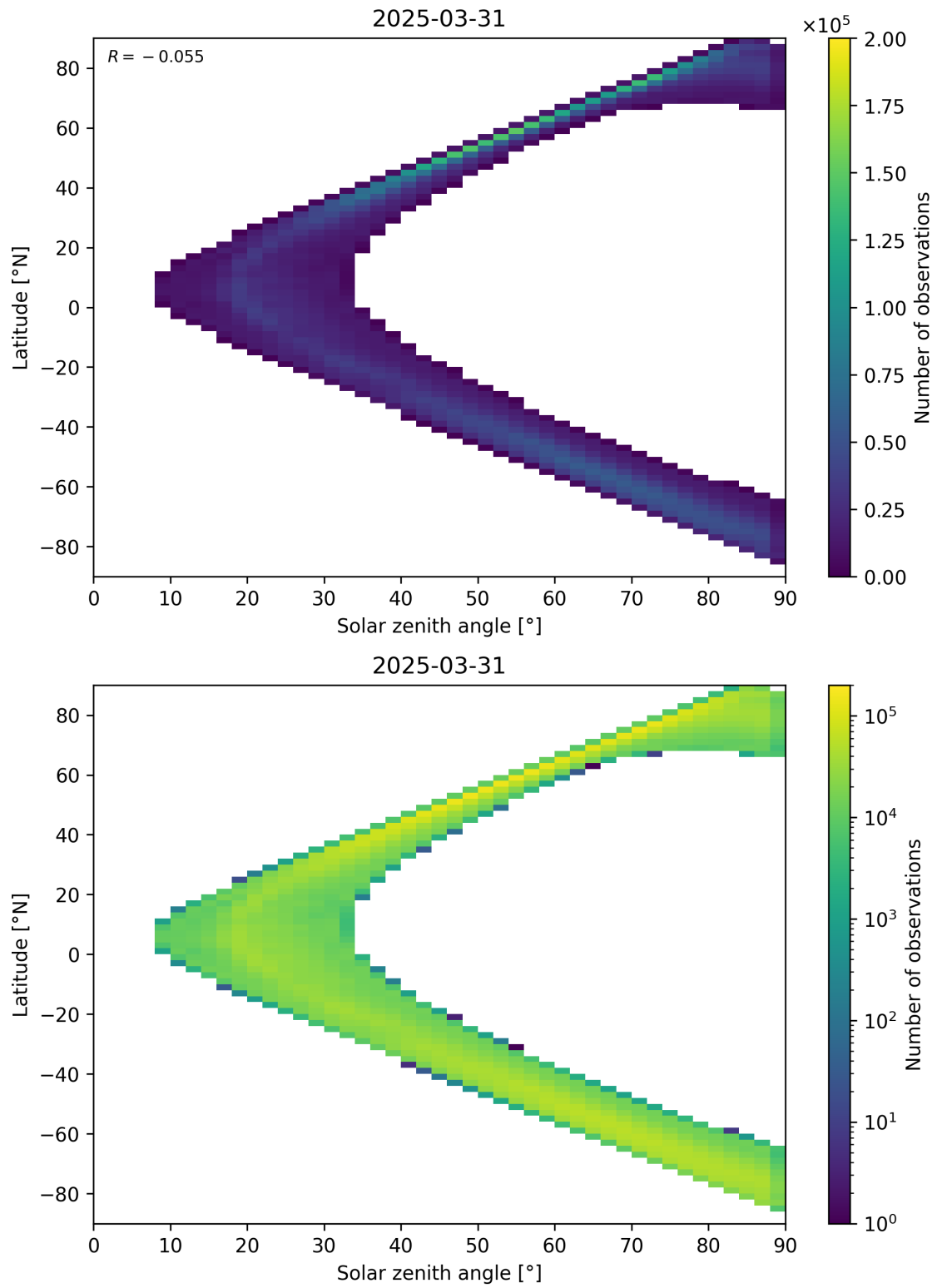
Figure 105: Scatter density plot of “Solar zenith angle” against “Latitude” for 2025-03-30 to 2025-04-01.
