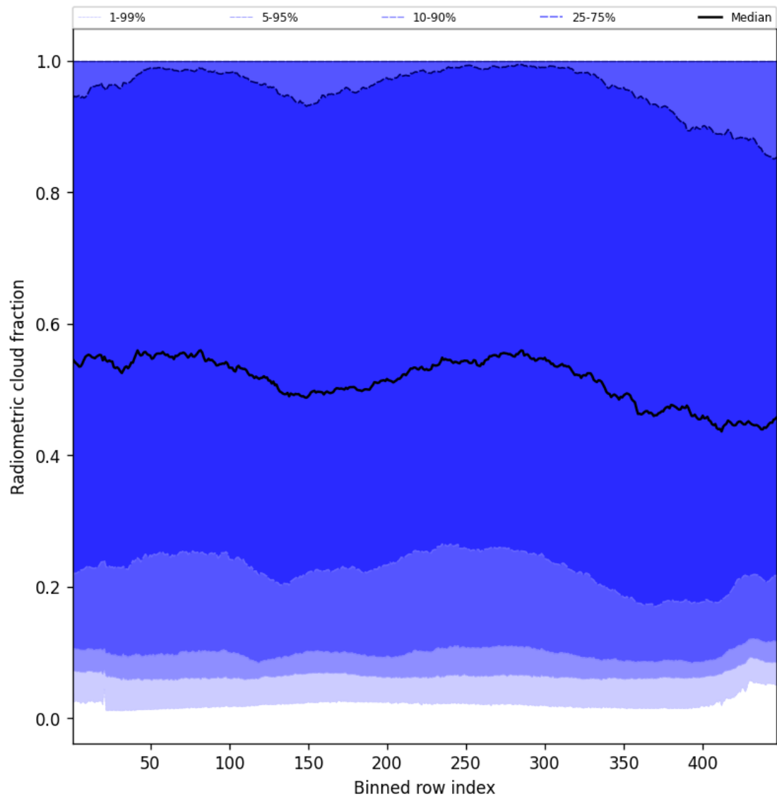
Figure 55: Along track statistics of “Radiometric cloud fraction” for 2025-03-30 to 2025-04-01
