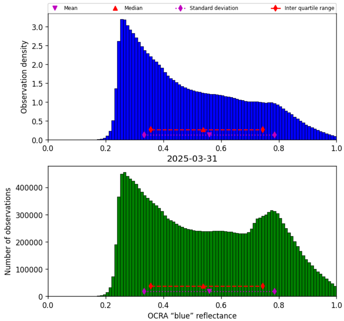
Figure 51: Histogram of “OCRA “blue” reflectance” for 2025-03-30 to 2025-04-01
