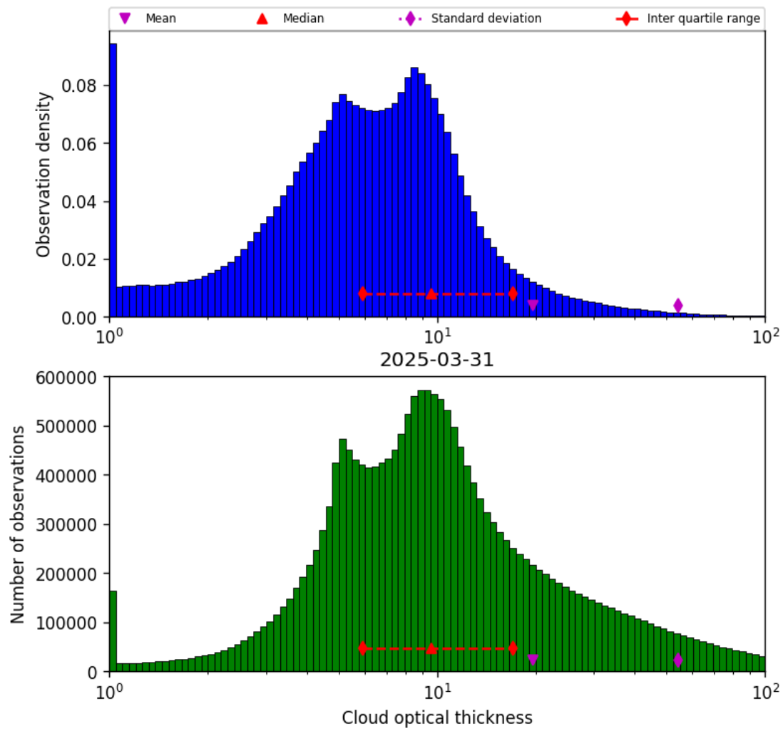
Figure 41: Histogram of “Cloud optical thickness” for 2025-03-30 to 2025-04-01
