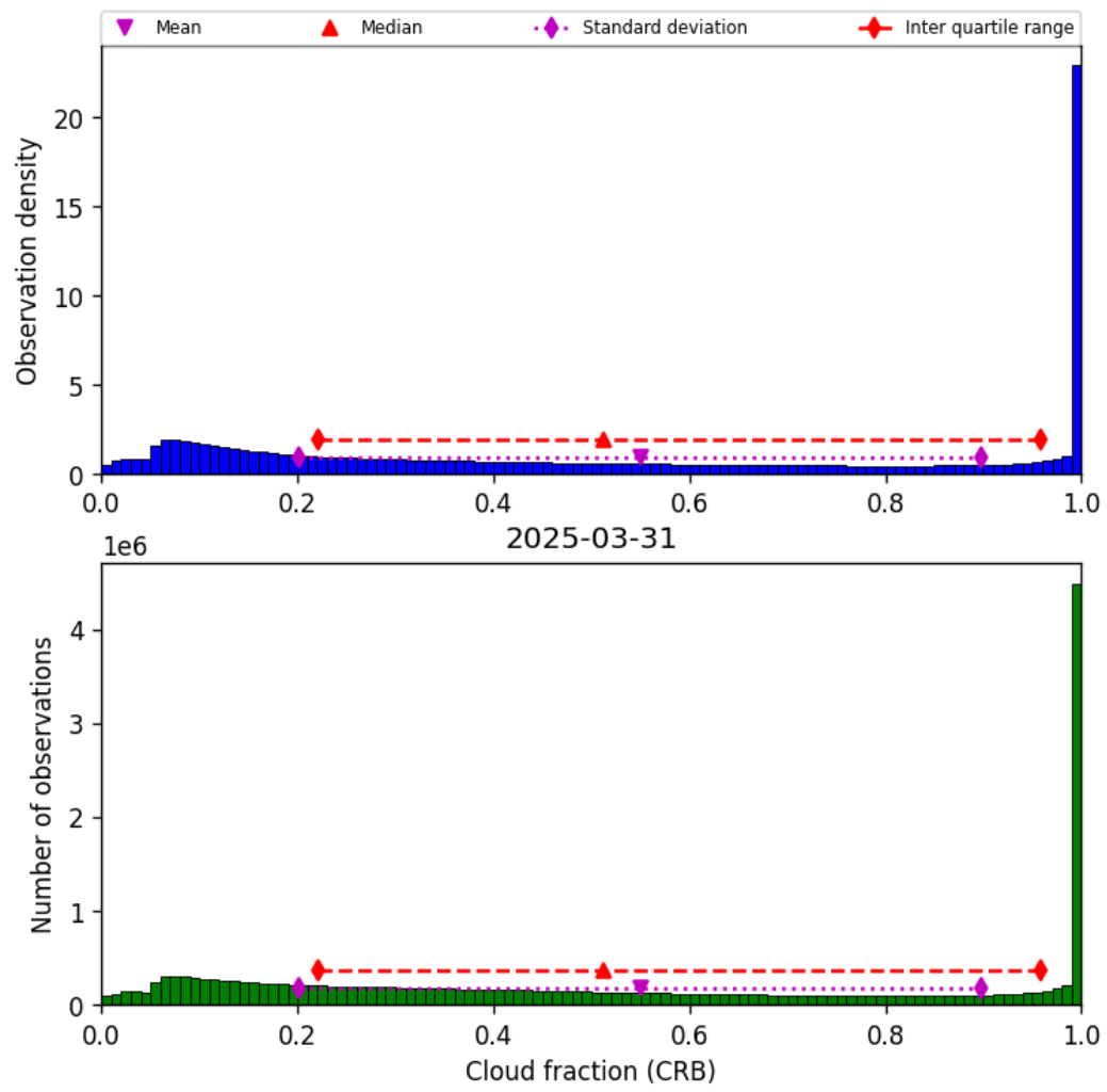
Figure 42: Histogram of “Cloud fraction (CRB)” for 2025-03-30 to 2025-04-01
