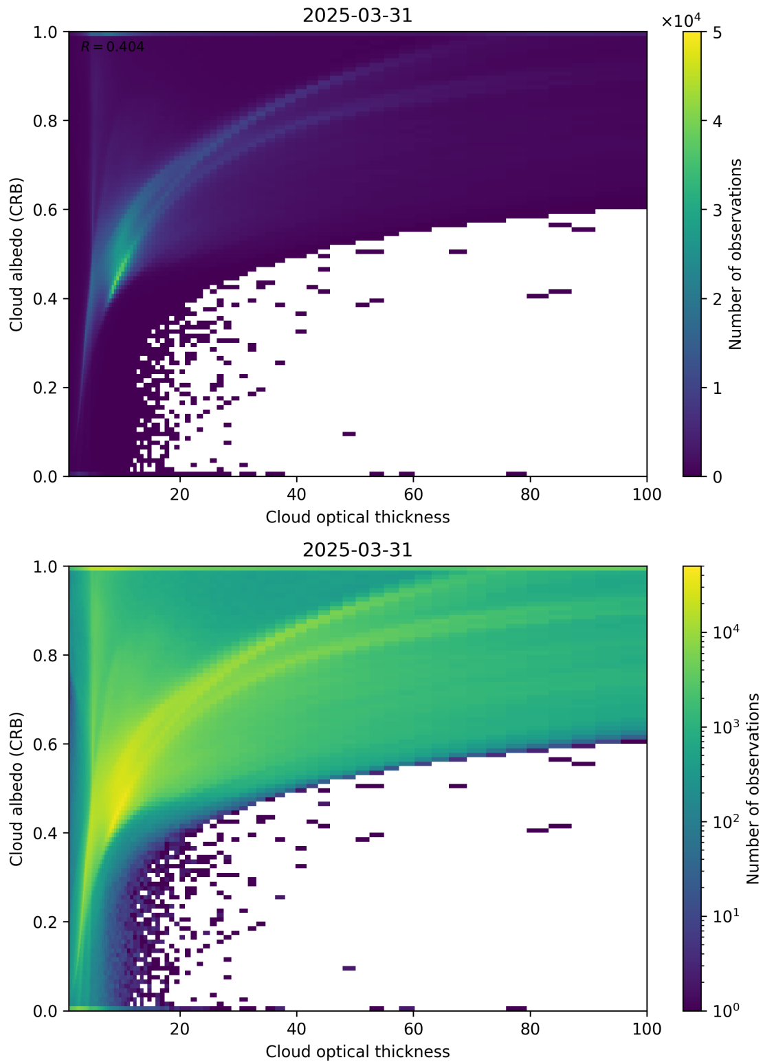
Figure 82: Scatter density plot of “Cloud optical thickness” against “Cloud albedo (CRB)” for 2025-03-30 to 2025-04-01.
