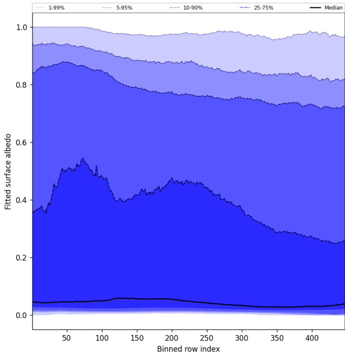
Figure 61: Along track statistics of “Fitted surface albedo” for 2025-03-30 to 2025-04-01
