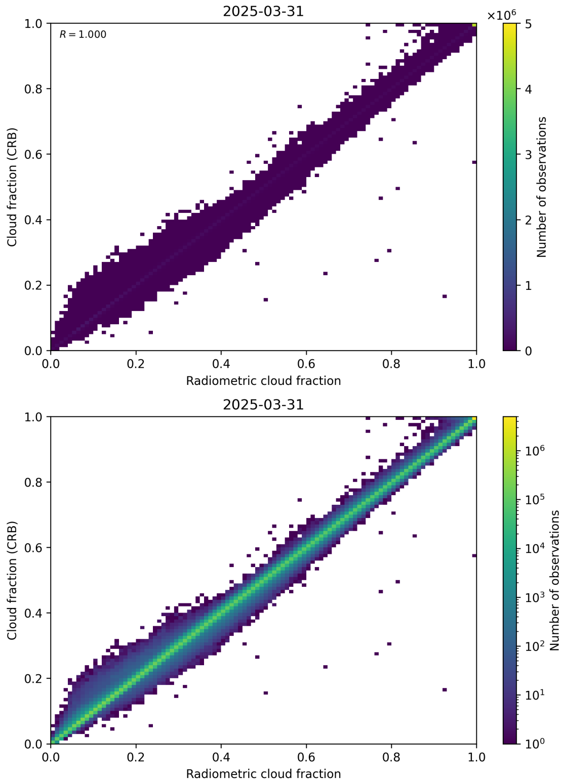
Figure 73: Scatter density plot of “Radiometric cloud fraction” against “Cloud fraction (CRB)” for 2025-03-30 to 2025-04-01.
