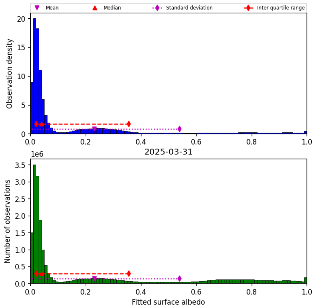
Figure 45: Histogram of “Fitted surface albedo” for 2025-03-30 to 2025-04-01
