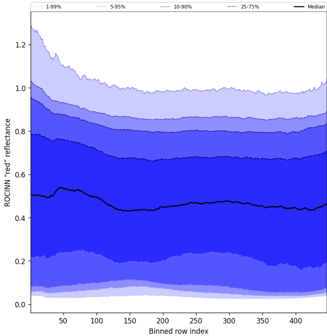
Figure 69: Along track statistics of “ROCINN “red” reflectance” for 2025-03-30 to 2025-04-01
