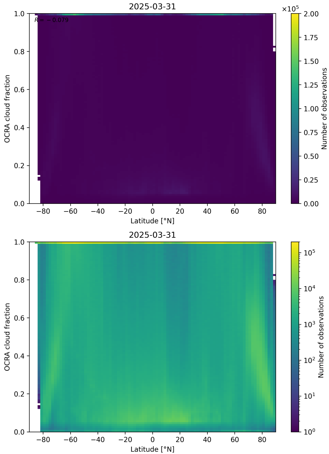
Figure 93: Scatter density plot of “Latitude” against “OCRA cloud fraction” for 2025-03-30 to 2025-04-01.
