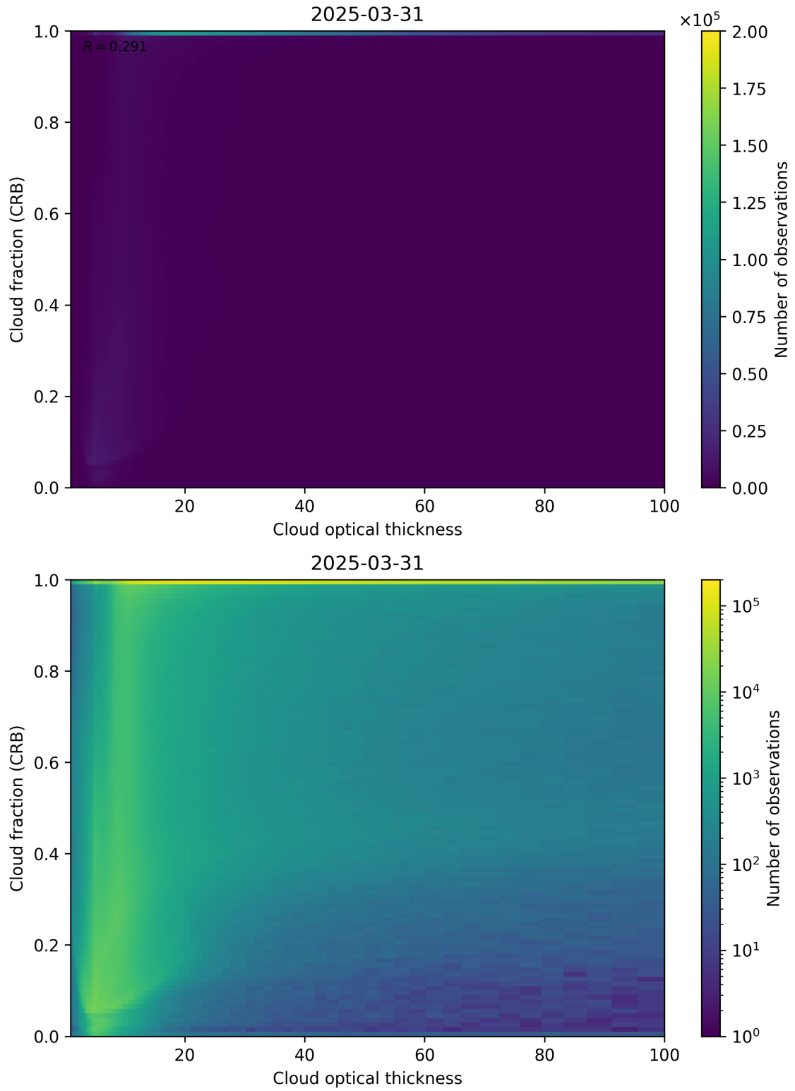
Figure 84: Scatter density plot of “Cloud optical thickness” against “Cloud fraction (CRB)” for 2025-03-30 to 2025-04-01.
