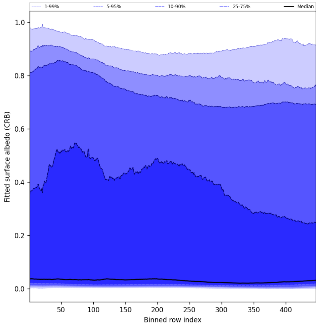
Figure 62: Along track statistics of “Fitted surface albedo (CRB)” for 2025-03-30 to 2025-04-01
