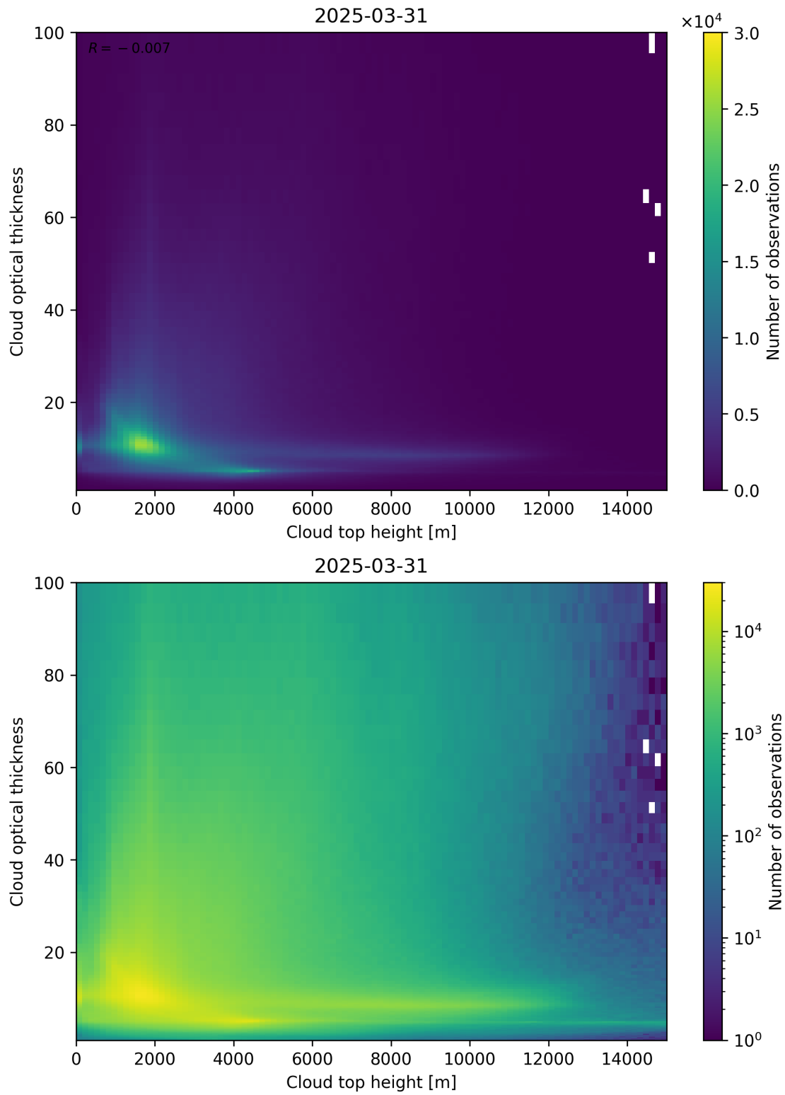
Figure 90: Scatter density plot of “Cloud top height” against “Cloud optical thickness” for 2025-03-30 to 2025-04-01.
