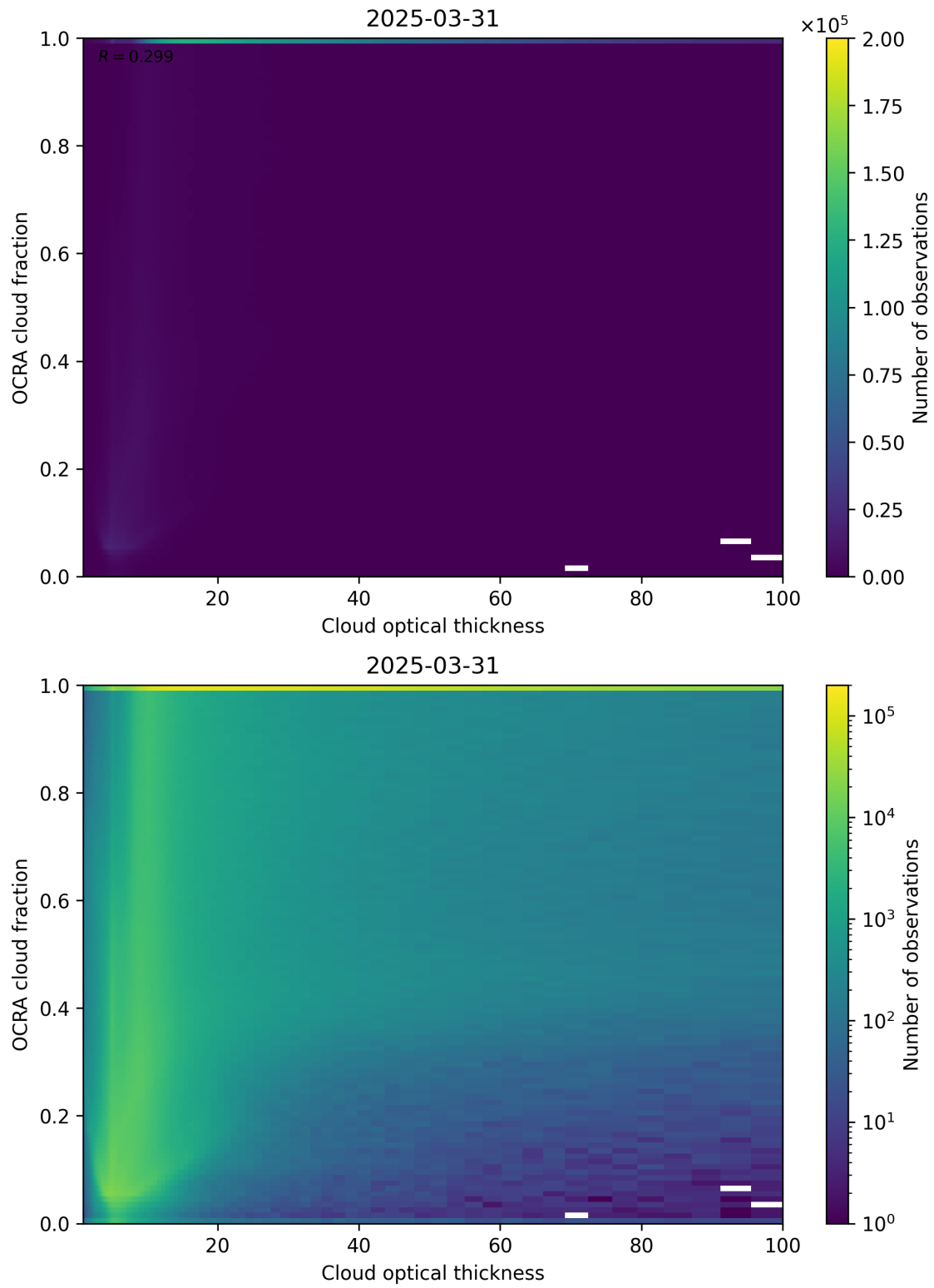
Figure 83: Scatter density plot of “Cloud optical thickness” against “OCRA cloud fraction” for 2025-03-30 to 2025-04-01.
