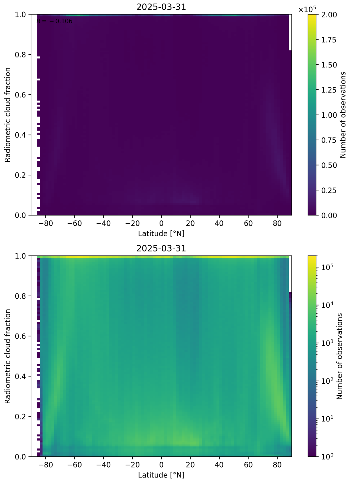
Figure 92: Scatter density plot of “Latitude” against “Radiometric cloud fraction” for 2025-03-30 to 2025-04-01.
