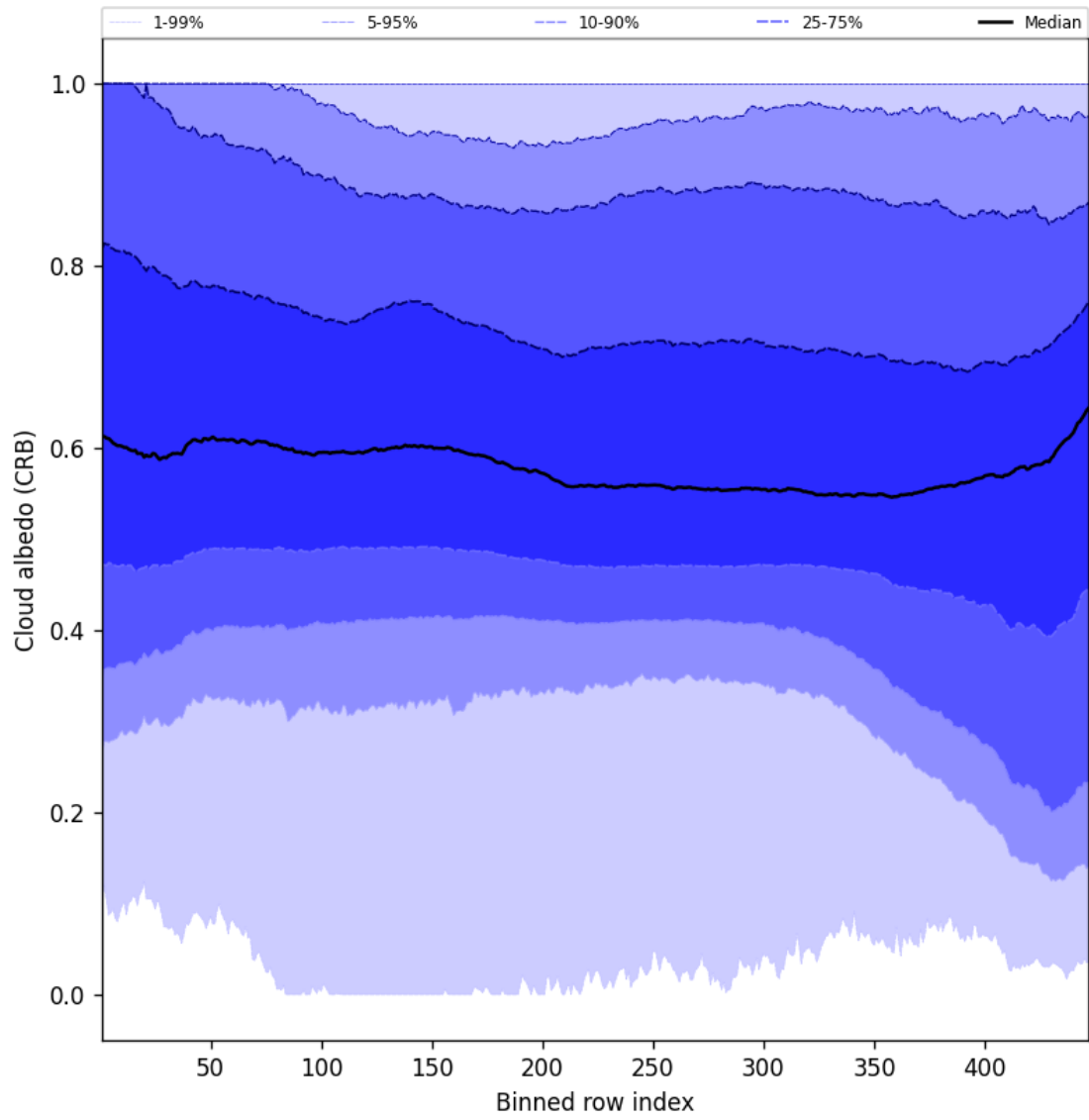
Figure 60: Along track statistics of “Cloud albedo (CRB)” for 2025-03-30 to 2025-04-01
