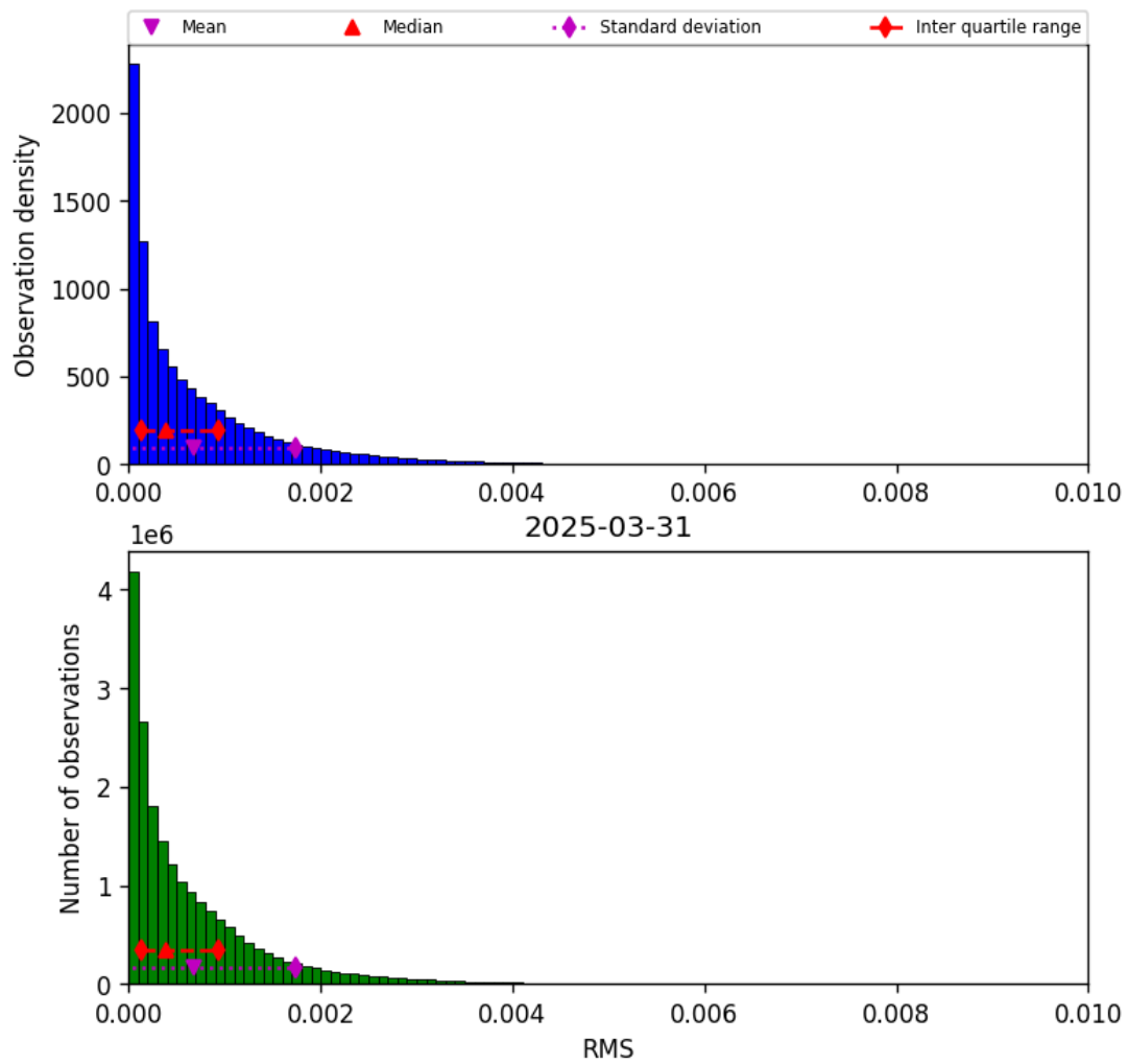
Figure 47: Histogram of “RMS” for 2025-03-30 to 2025-04-01
