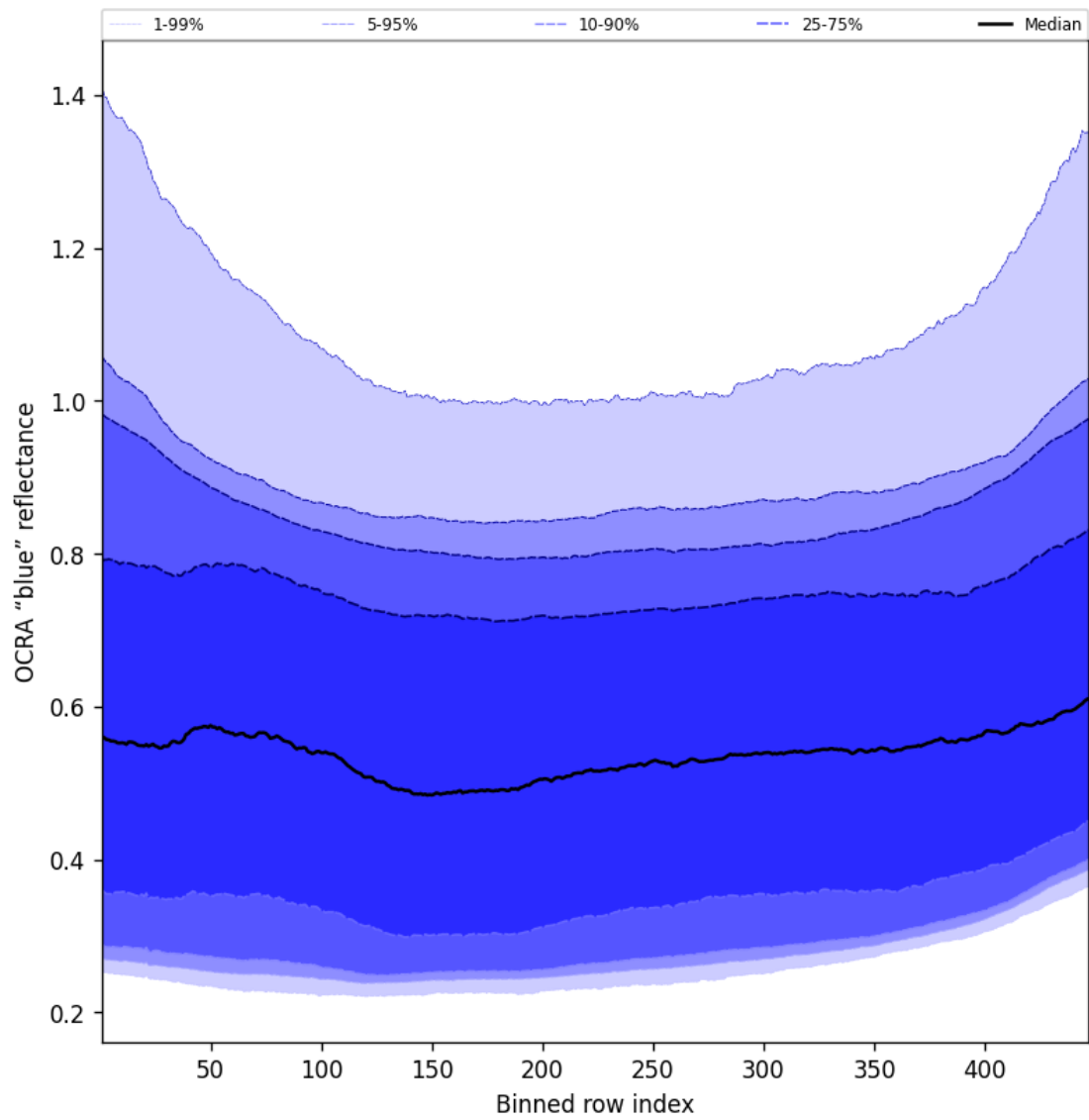
Figure 67: Along track statistics of “OCRA “blue” reflectance” for 2025-03-30 to 2025-04-01
