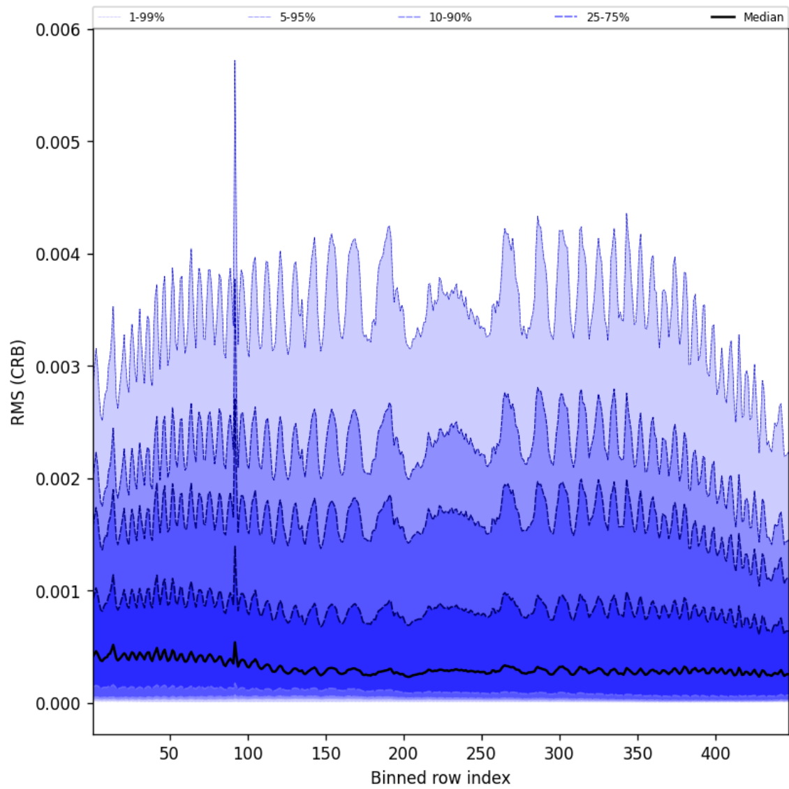
Figure 64: Along track statistics of “RMS (CRB)” for 2025-03-30 to 2025-04-01
