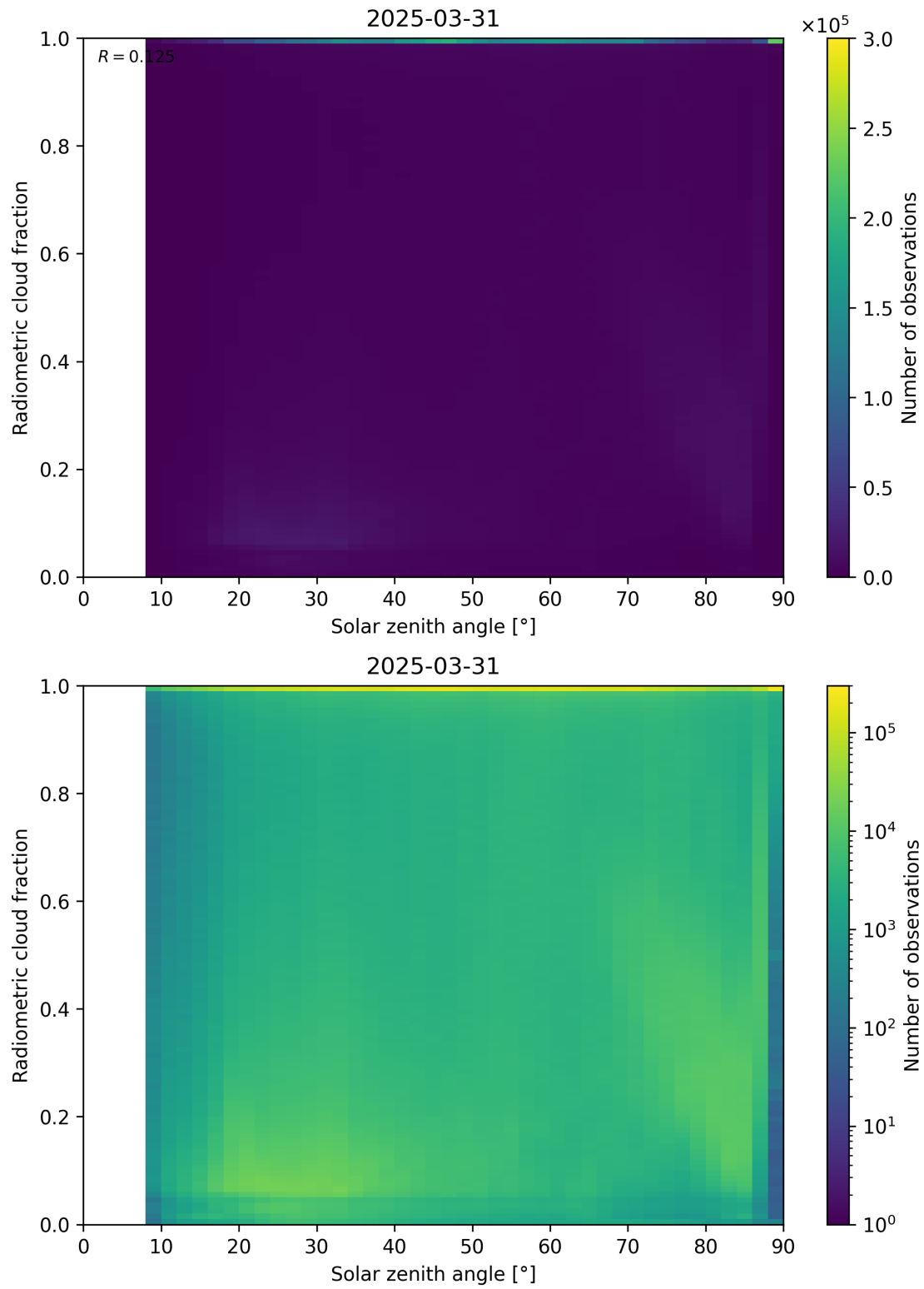
Figure 99: Scatter density plot of “Solar zenith angle” against “Radiometric cloud fraction” for 2025-03-30 to 2025-04-01.
