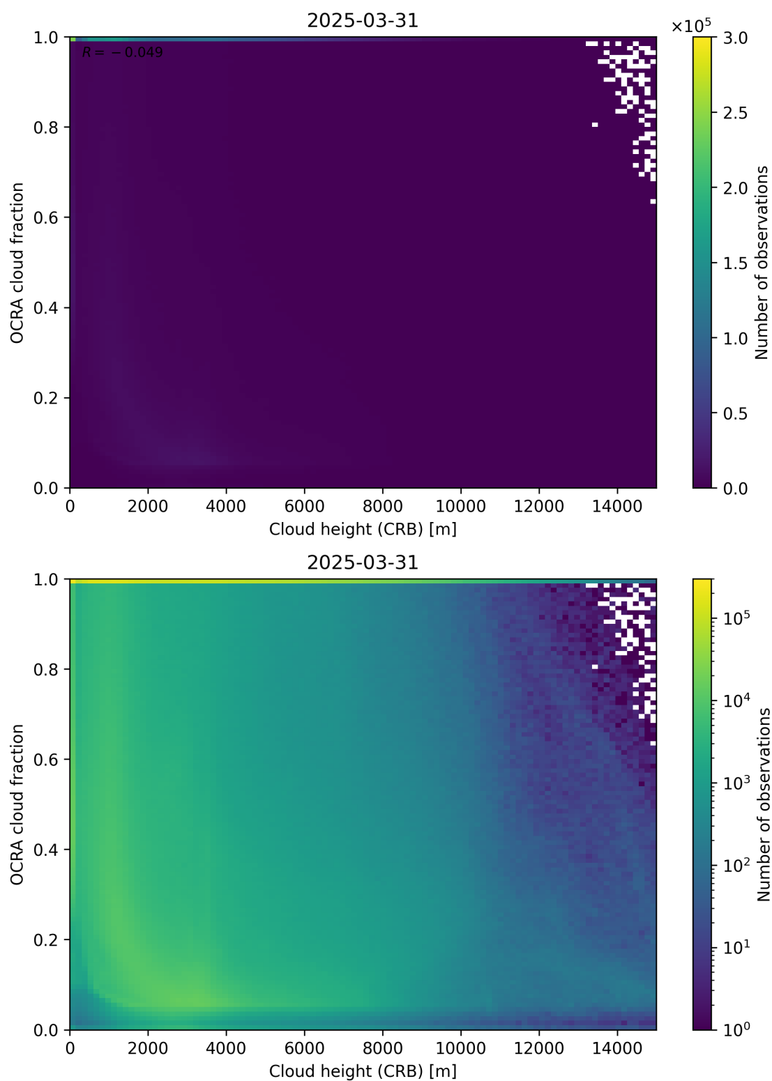
Figure 81: Scatter density plot of “Cloud height (CRB)” against “OCRA cloud fraction” for 2025-03-30 to 2025-04-01.
