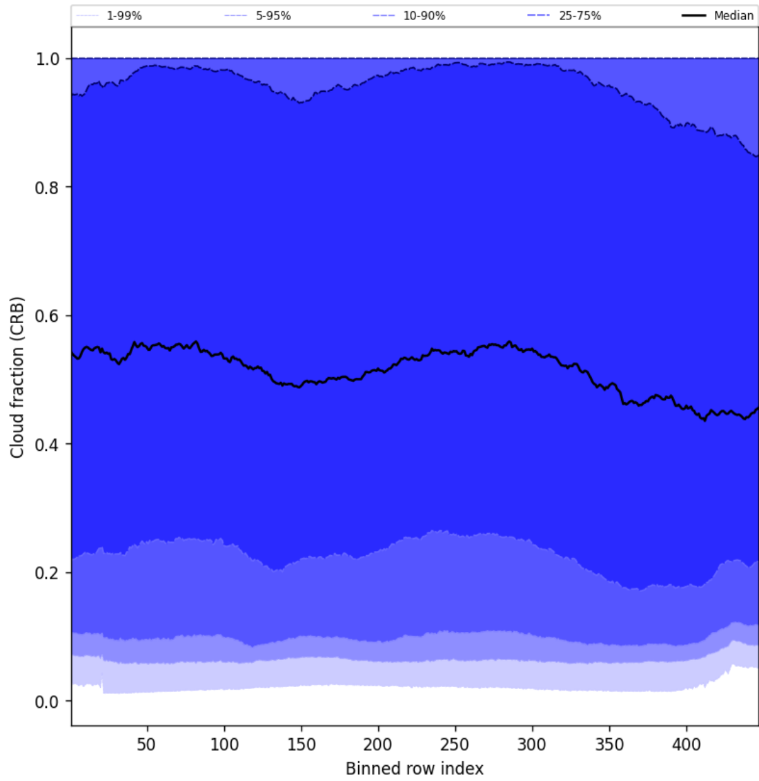
Figure 58: Along track statistics of “Cloud fraction (CRB)” for 2025-03-30 to 2025-04-01
