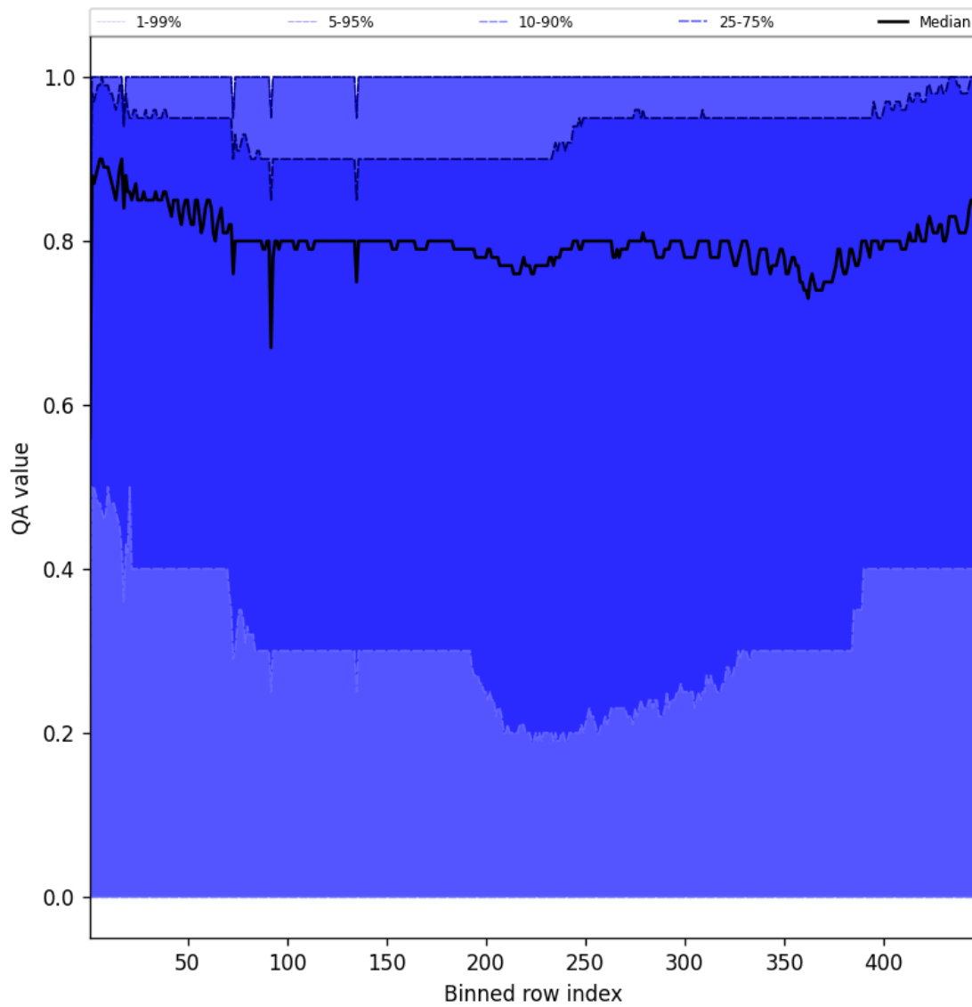
Figure 54: Along track statistics of “QA value” for 2025-03-30 to 2025-04-01
