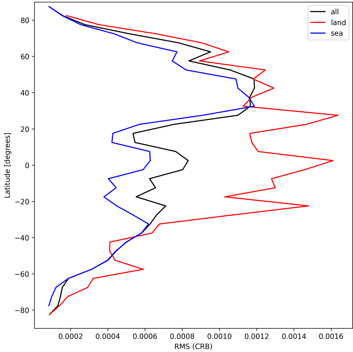
Figure 32: Zonal average of “RMS (CRB)” for 2025-03-30 to 2025-04-01.
