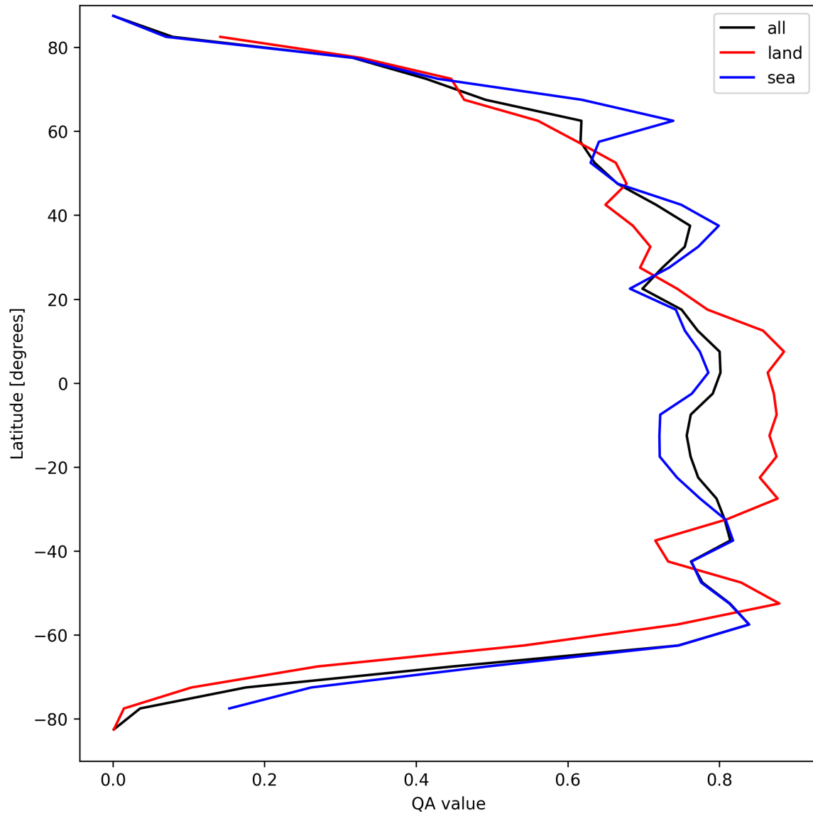
Figure 22: Zonal average of “QA value” for 2025-03-30 to 2025-04-01.
