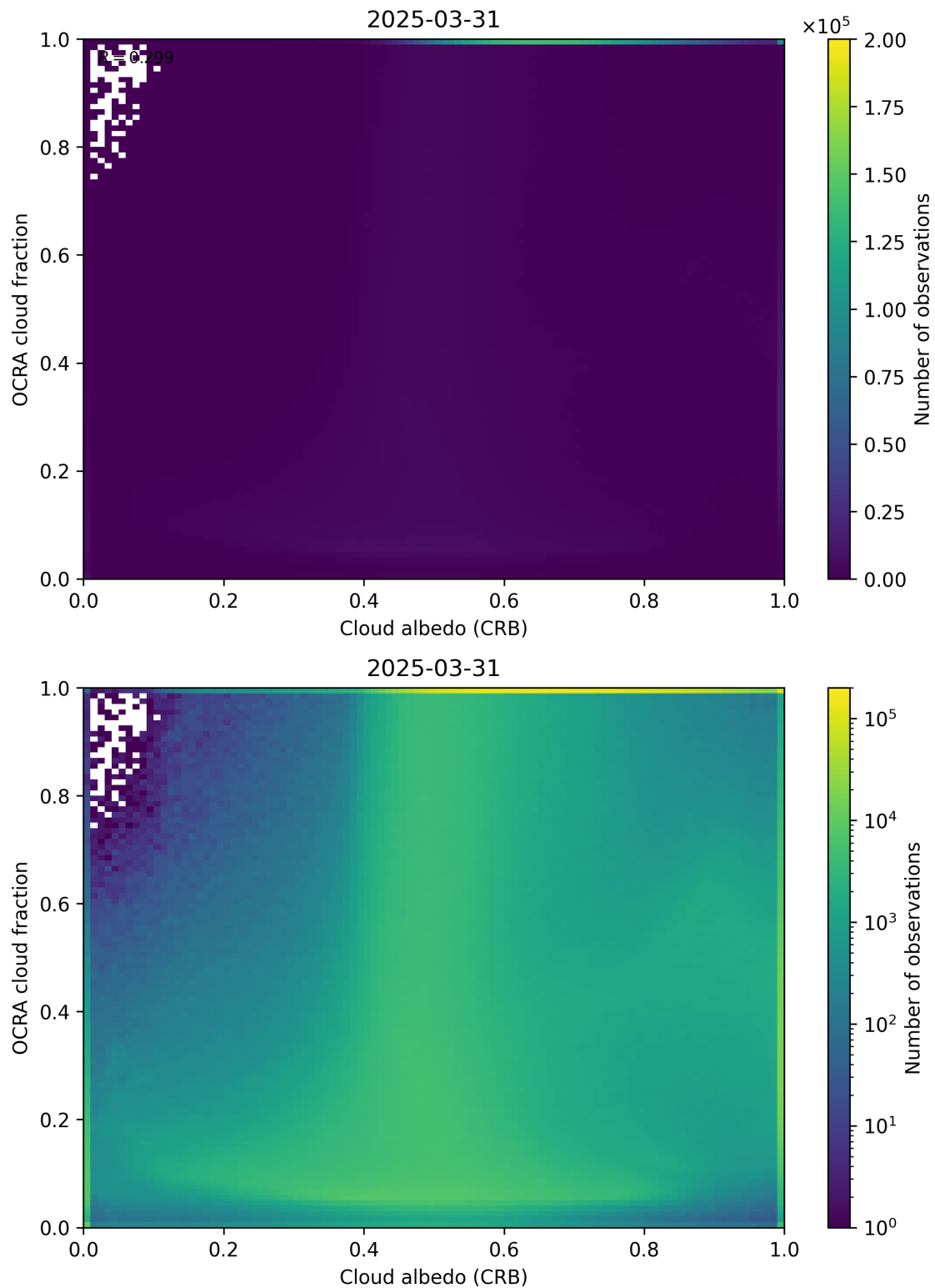
Figure 70: Scatter density plot of “Cloud albedo (CRB)” against “OCRA cloud fraction” for 2025-03-30 to 2025-04-01.
