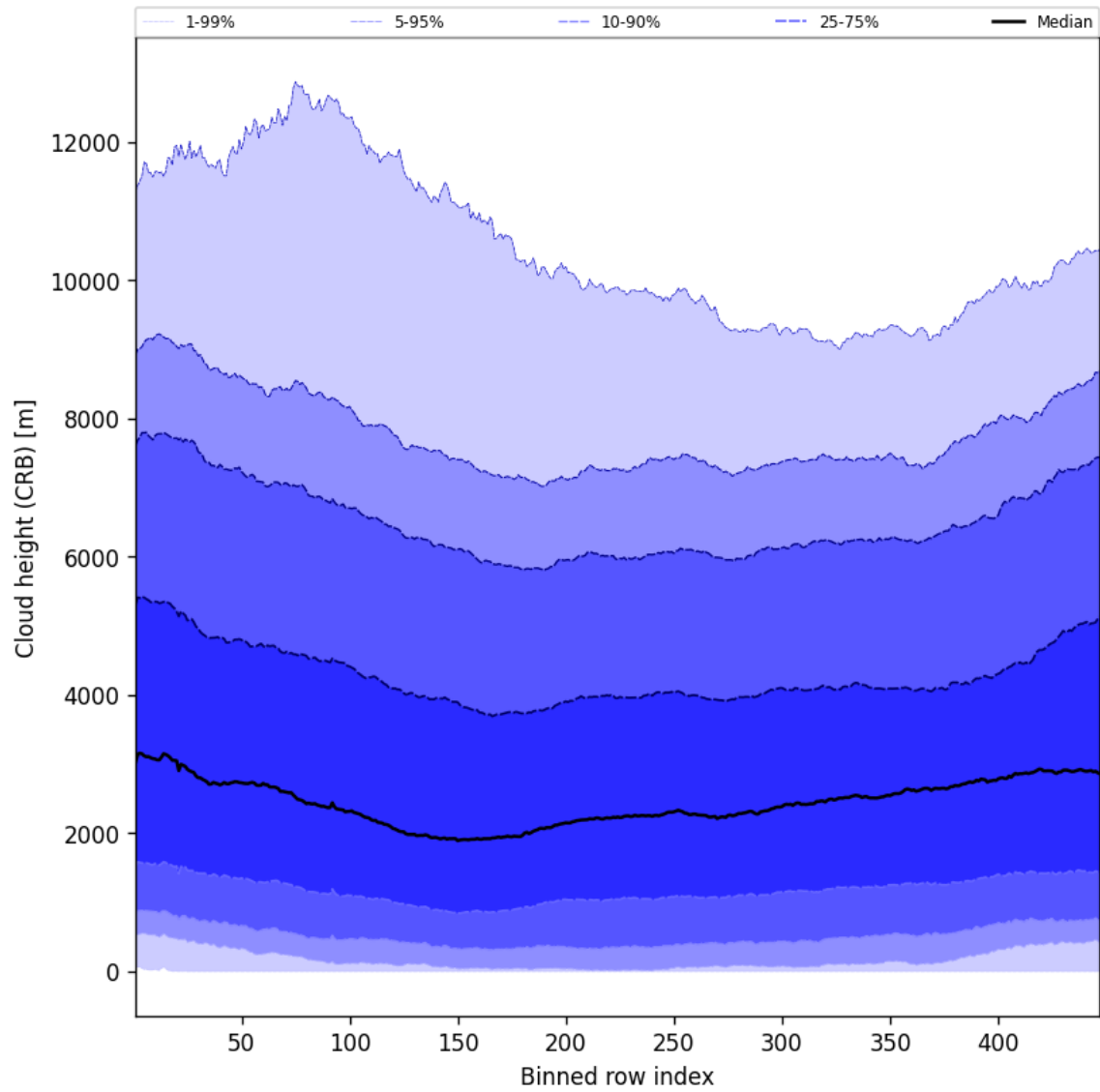
Figure 59: Along track statistics of “Cloud height (CRB)” for 2025-03-30 to 2025-04-01
