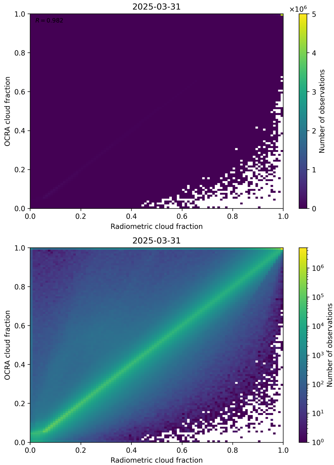
Figure 72: Scatter density plot of “Radiometric cloud fraction” against “OCRA cloud fraction” for 2025-03-30 to 2025-04-01.
