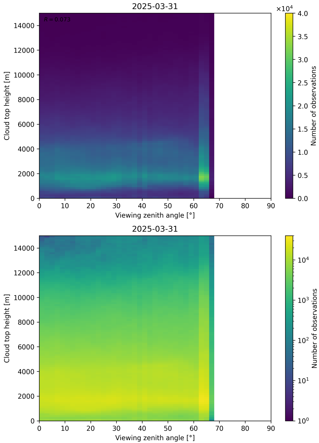
Figure 112: Scatter density plot of “Viewing zenith angle” against “Cloud top height” for 2025-03-30 to 2025-04-01.
