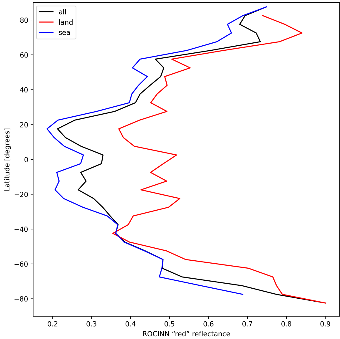
Figure 37: Zonal average of “ROCINN “red” reflectance” for 2025-03-30 to 2025-04-01.
