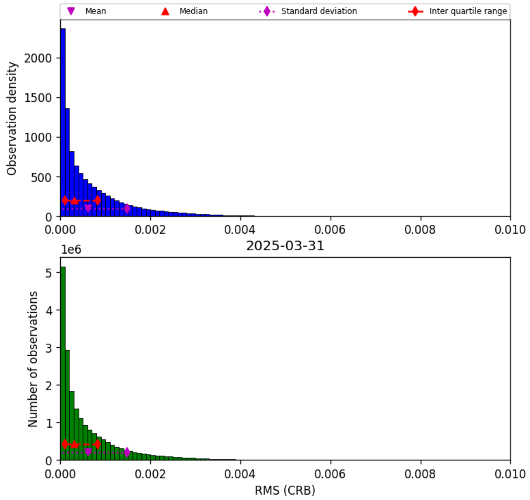
Figure 48: Histogram of “RMS (CRB)” for 2025-03-30 to 2025-04-01
