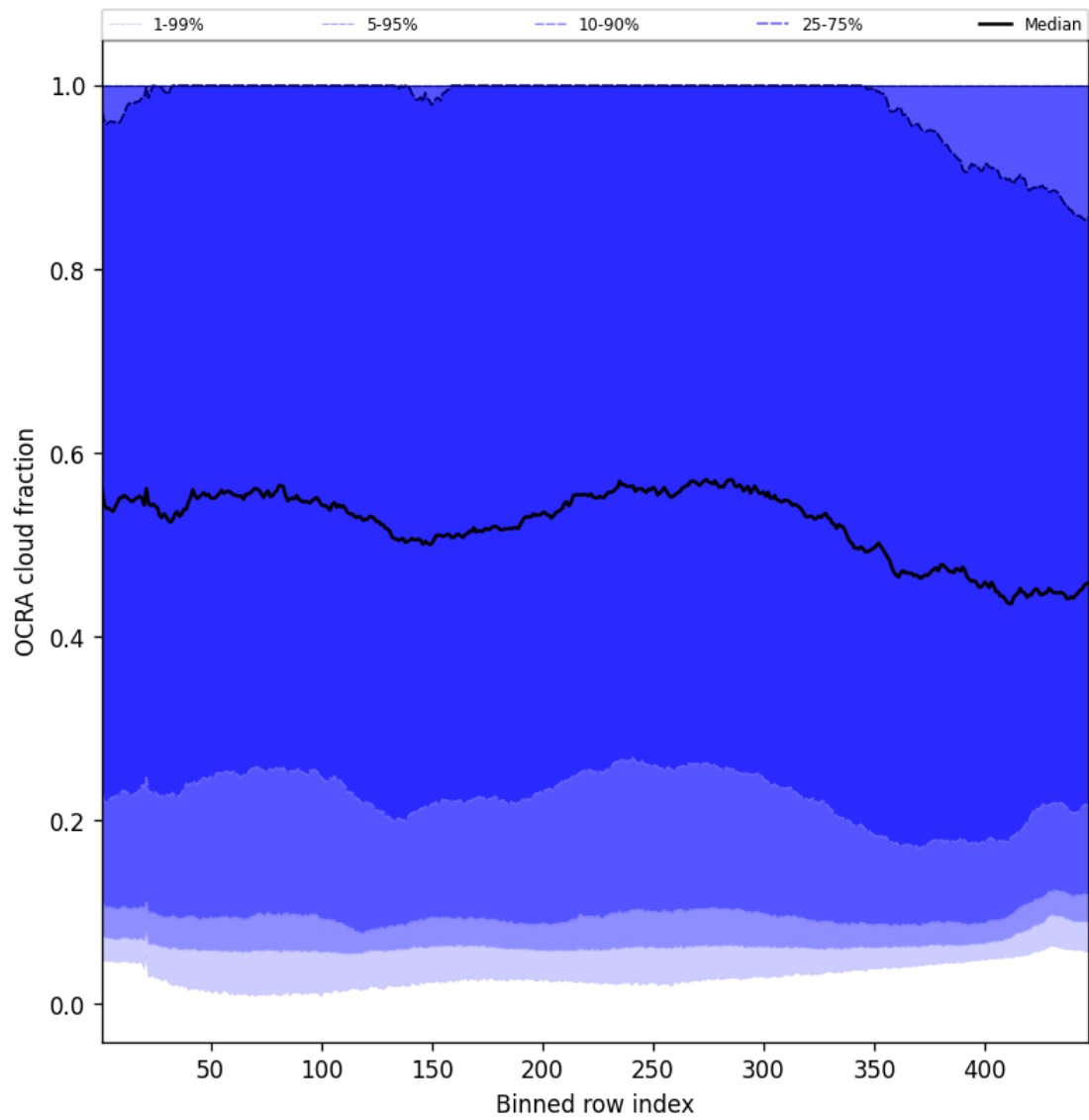
Figure 66: Along track statistics of “OCRA cloud fraction” for 2025-03-30 to 2025-04-01
