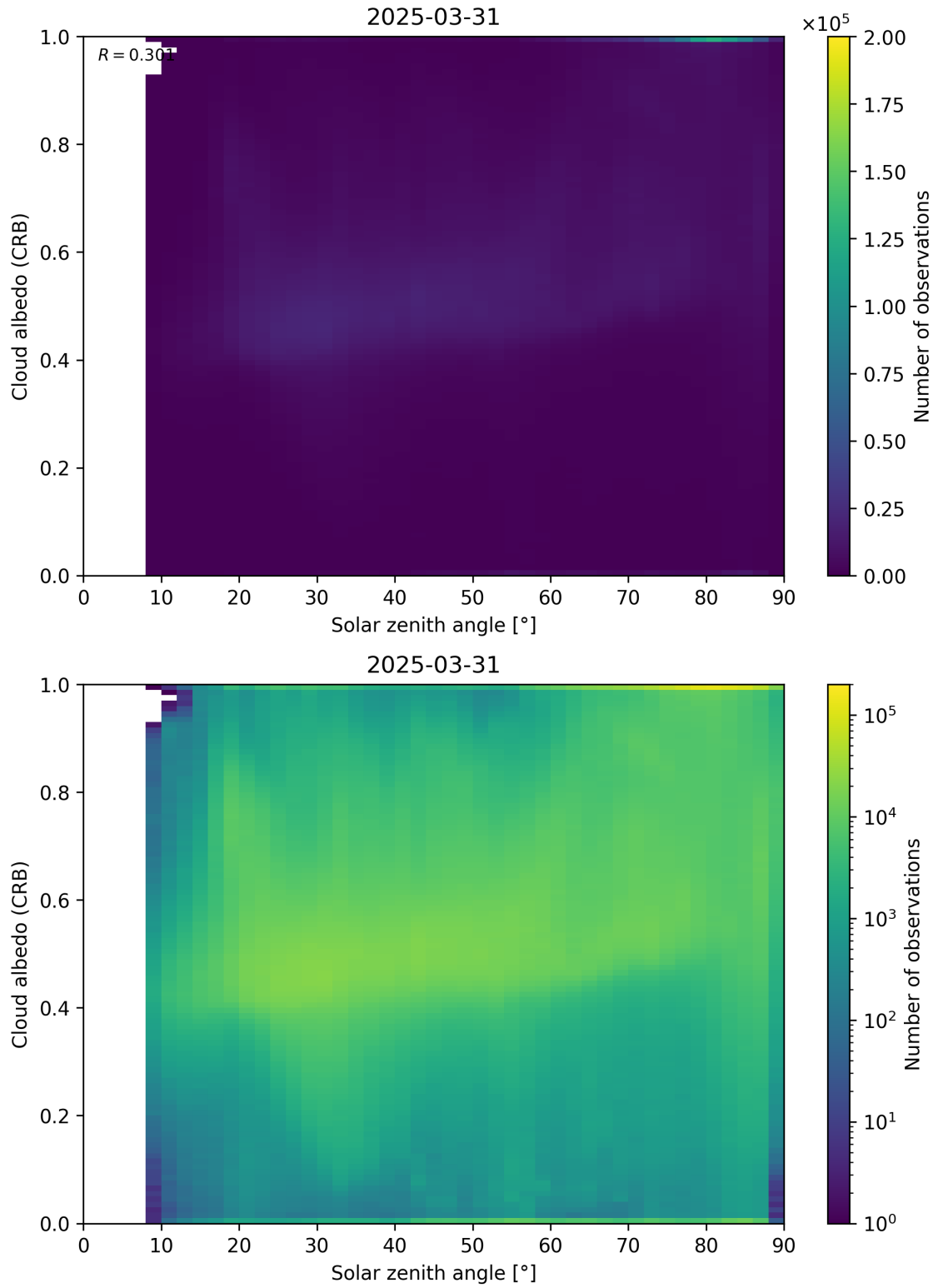
Figure 98: Scatter density plot of “Solar zenith angle” against “Cloud albedo (CRB)” for 2025-03-30 to 2025-04-01.
