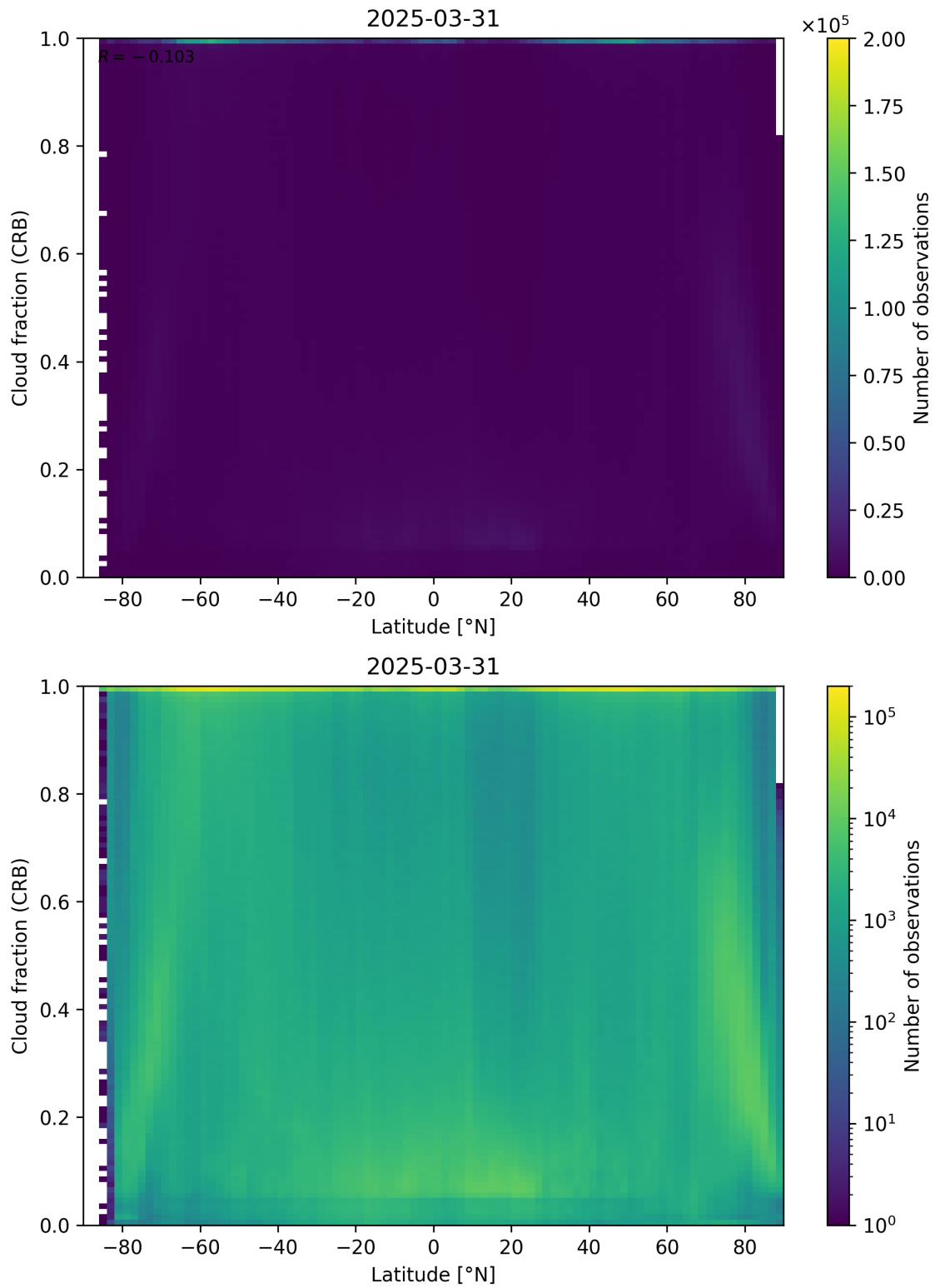
Figure 94: Scatter density plot of “Latitude” against “Cloud fraction (CRB)” for 2025-03-30 to 2025-04-01.
