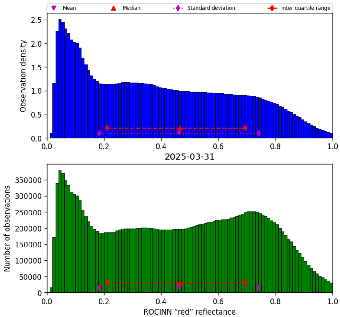
Figure 53: Histogram of “ROCINN “red” reflectance” for 2025-03-30 to 2025-04-01
