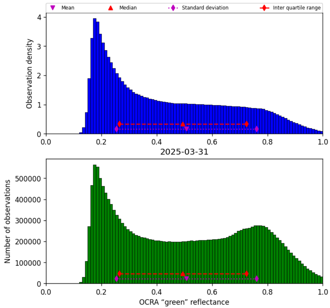
Figure 52: Histogram of “OCRA “green” reflectance” for 2025-03-30 to 2025-04-01
