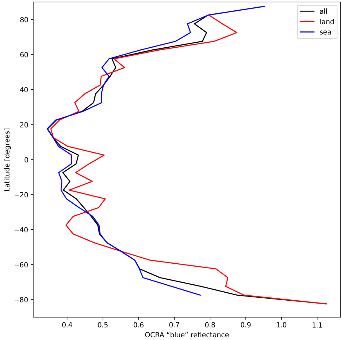
Figure 35: Zonal average of "OCRA "blue" reflectance" for 2025-03-30 to 2025-04-01.
