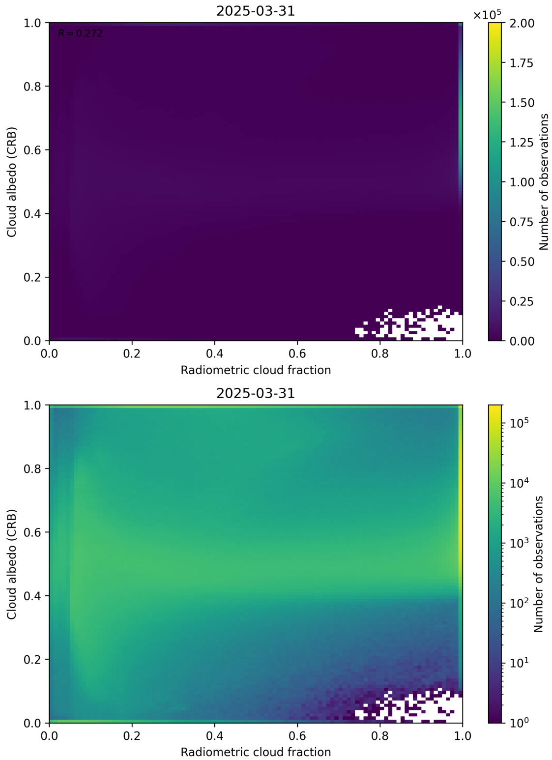
Figure 71: Scatter density plot of “Radiometric cloud fraction” against “Cloud albedo (CRB)” for 2025-03-30 to 2025-04-01.
