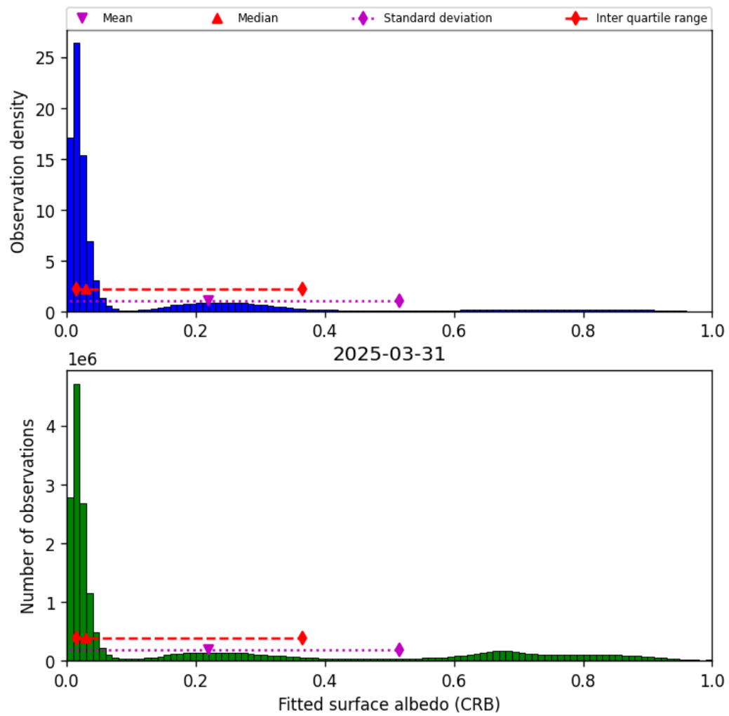
Figure 46: Histogram of “Fitted surface albedo (CRB)” for 2025-03-30 to 2025-04-01
