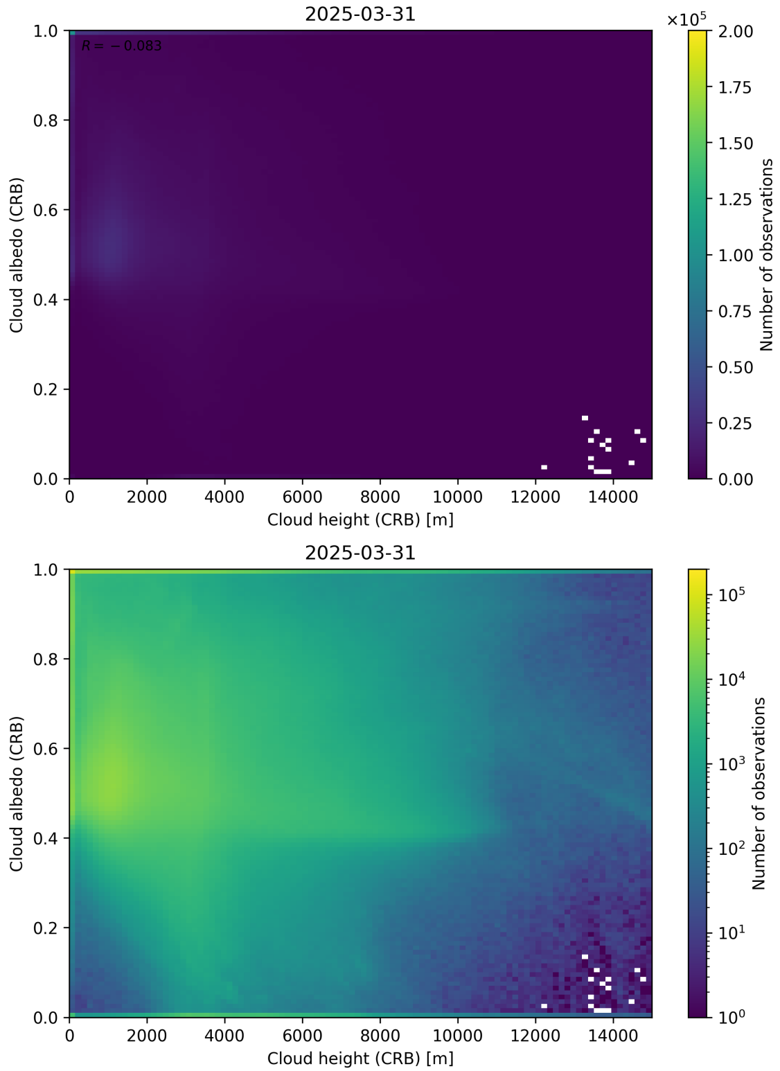
Figure 80: Scatter density plot of “Cloud height (CRB)” against “Cloud albedo (CRB)” for 2025-03-30 to 2025-04-01.
