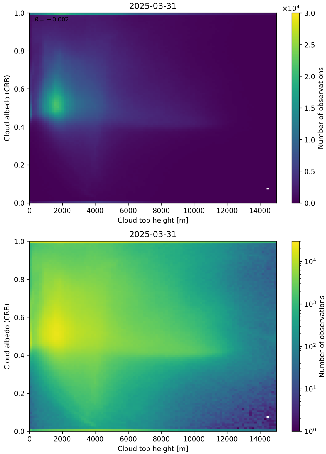
Figure 86: Scatter density plot of “Cloud top height” against “Cloud albedo (CRB)” for 2025-03-30 to 2025-04-01.
