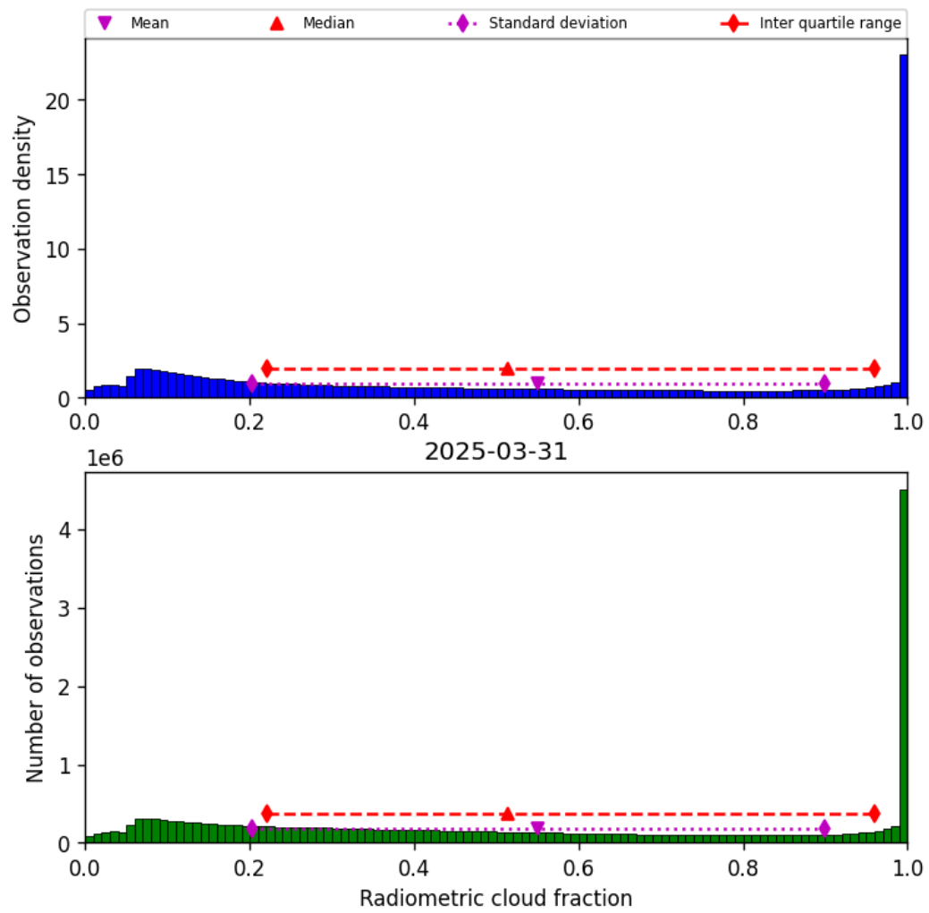
Figure 39: Histogram of “Radiometric cloud fraction” for 2025-03-30 to 2025-04-01
