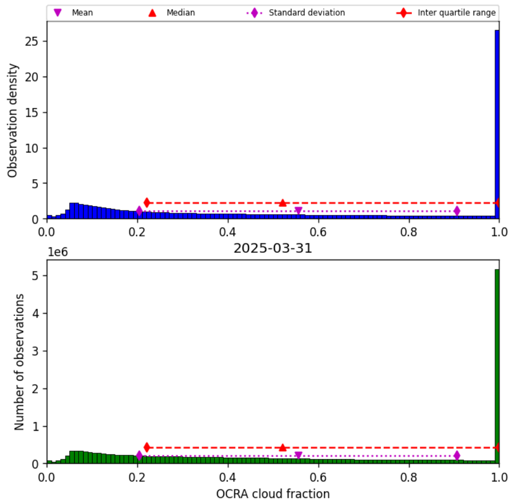
Figure 50: Histogram of “OCRA cloud fraction” for 2025-03-30 to 2025-04-01
