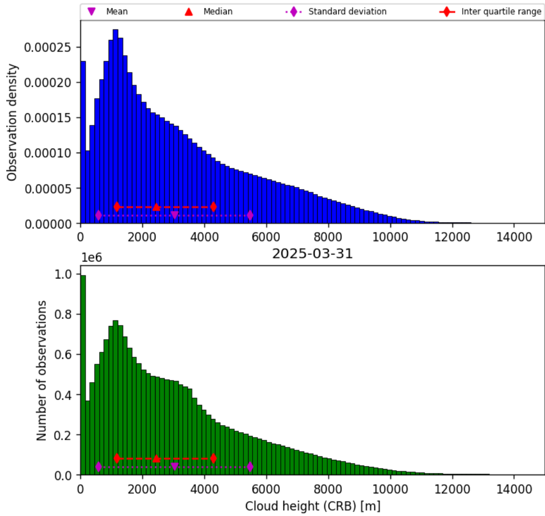
Figure 43: Histogram of “Cloud height (CRB)” for 2025-03-30 to 2025-04-01
