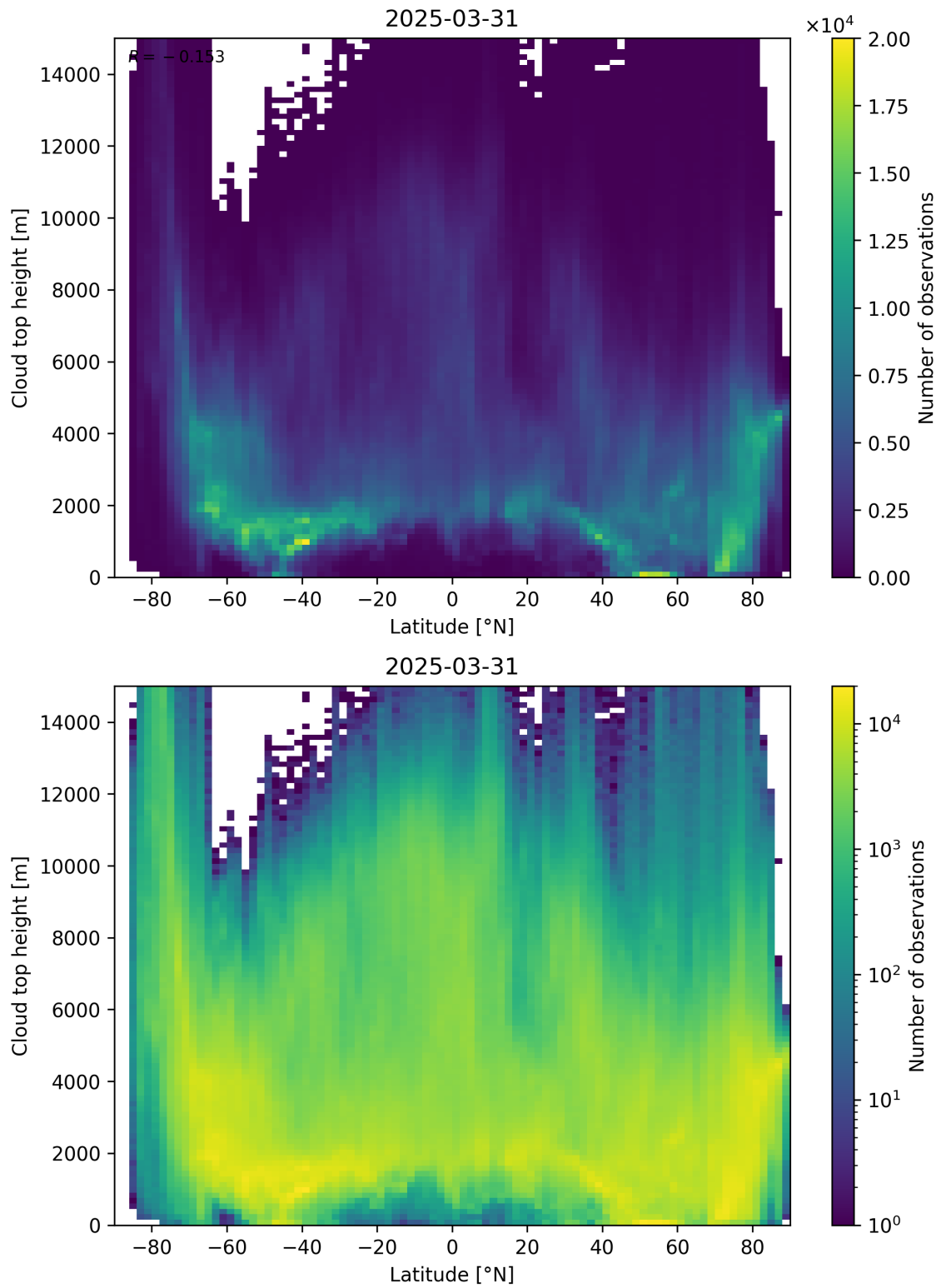
Figure 97: Scatter density plot of “Latitude” against “Cloud top height” for 2025-03-30 to 2025-04-01.
