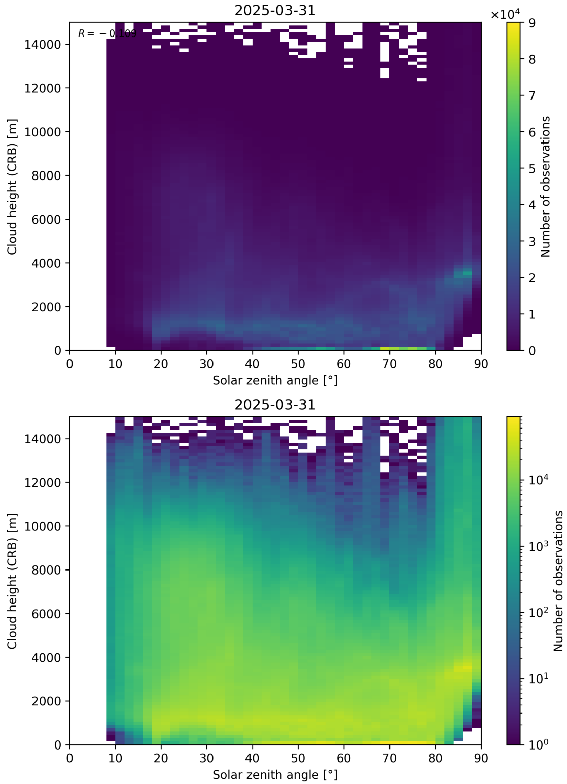
Figure 102: Scatter density plot of “Solar zenith angle” against “Cloud height (CRB)” for 2025-03-30 to 2025-04-01.
