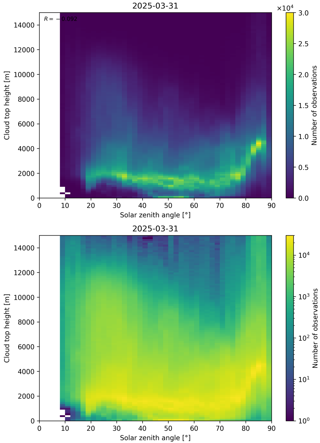
Figure 104: Scatter density plot of “Solar zenith angle” against “Cloud top height” for 2025-03-30 to 2025-04-01.
