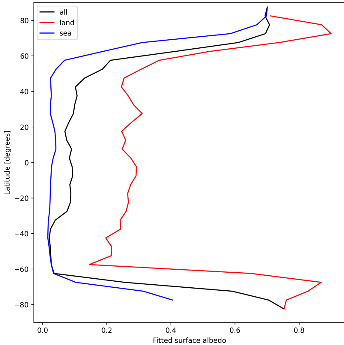
Figure 29: Zonal average of “Fitted surface albedo” for 2025-03-30 to 2025-04-01.
