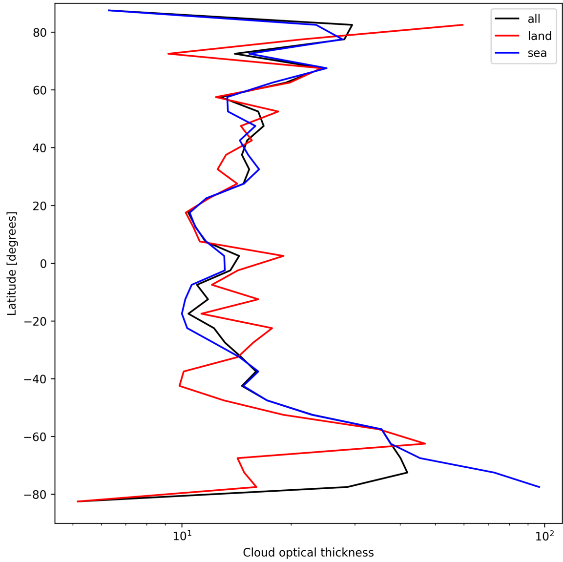
Figure 25: Zonal average of “Cloud optical thickness” for 2025-03-30 to 2025-04-01.
