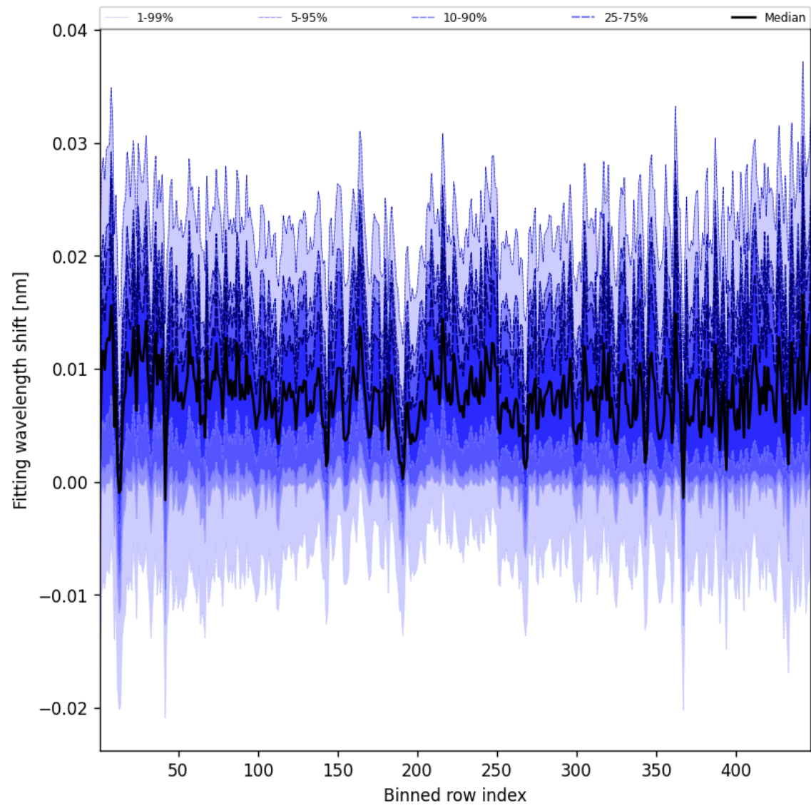
Figure 65: Along track statistics of “Fitting wavelength shift” for 2025-03-30 to 2025-04-01
