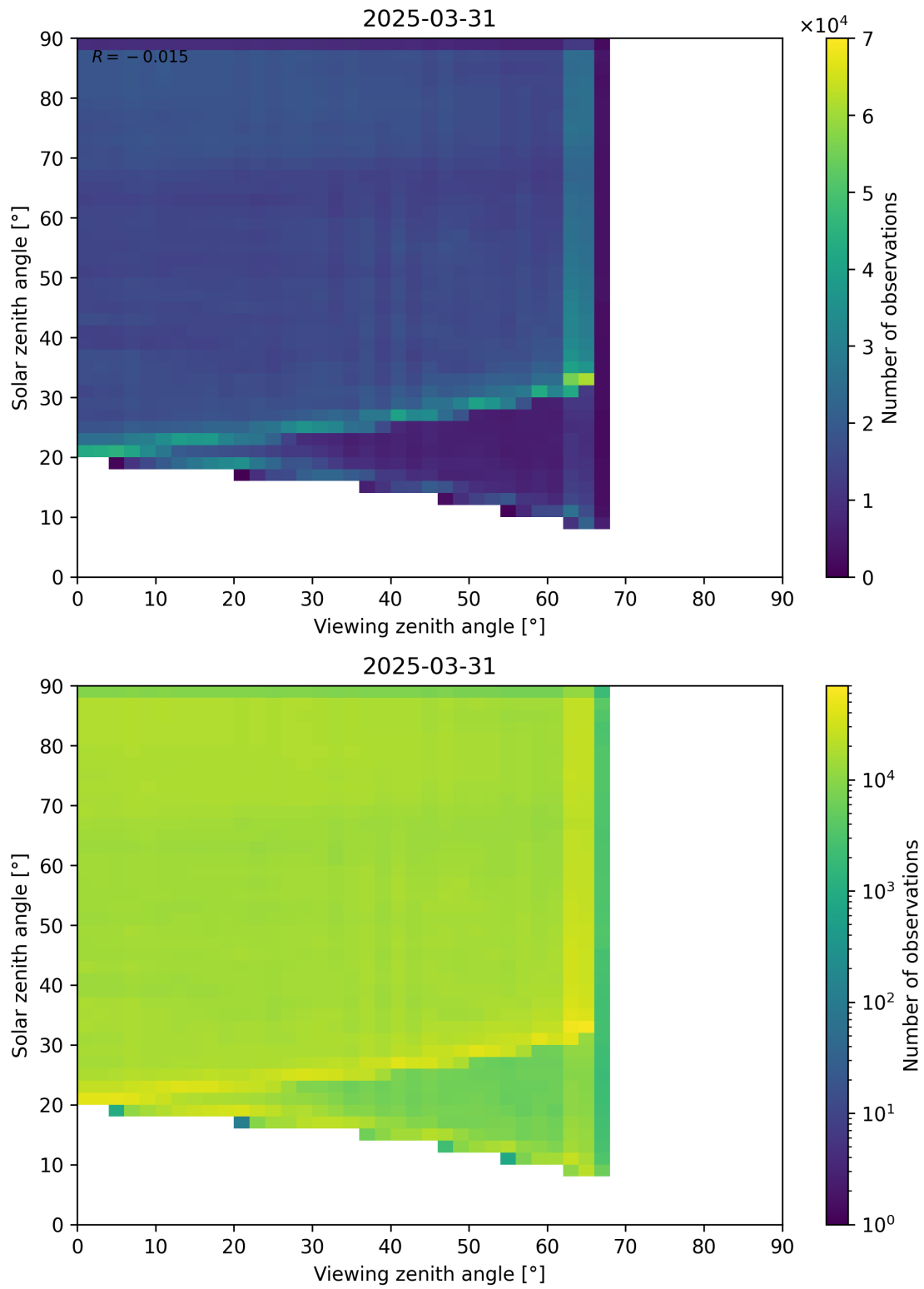
Figure 114: Scatter density plot of “Viewing zenith angle” against “Solar zenith angle” for 2025-03-30 to 2025-04-01.
