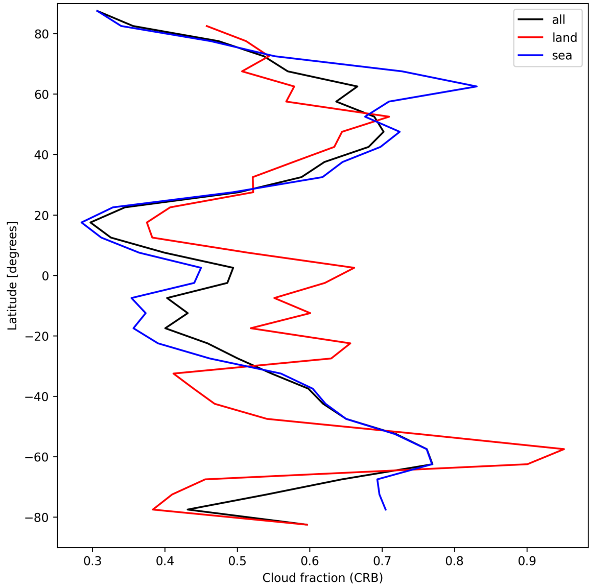
Figure 26: Zonal average of “Cloud fraction (CRB)” for 2025-03-30 to 2025-04-01.
