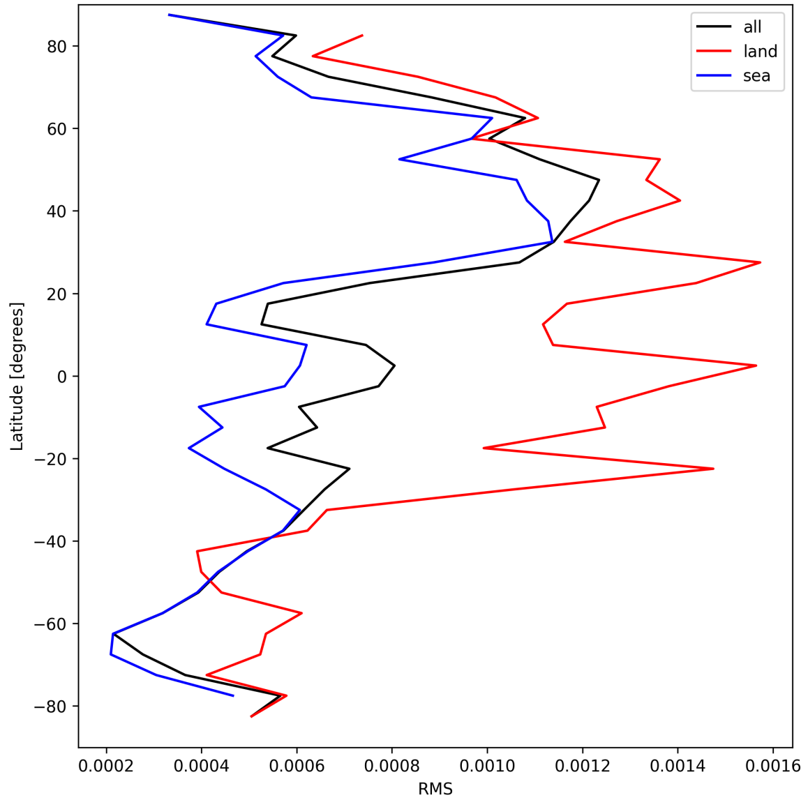
Figure 31: Zonal average of “RMS” for 2025-03-30 to 2025-04-01.
