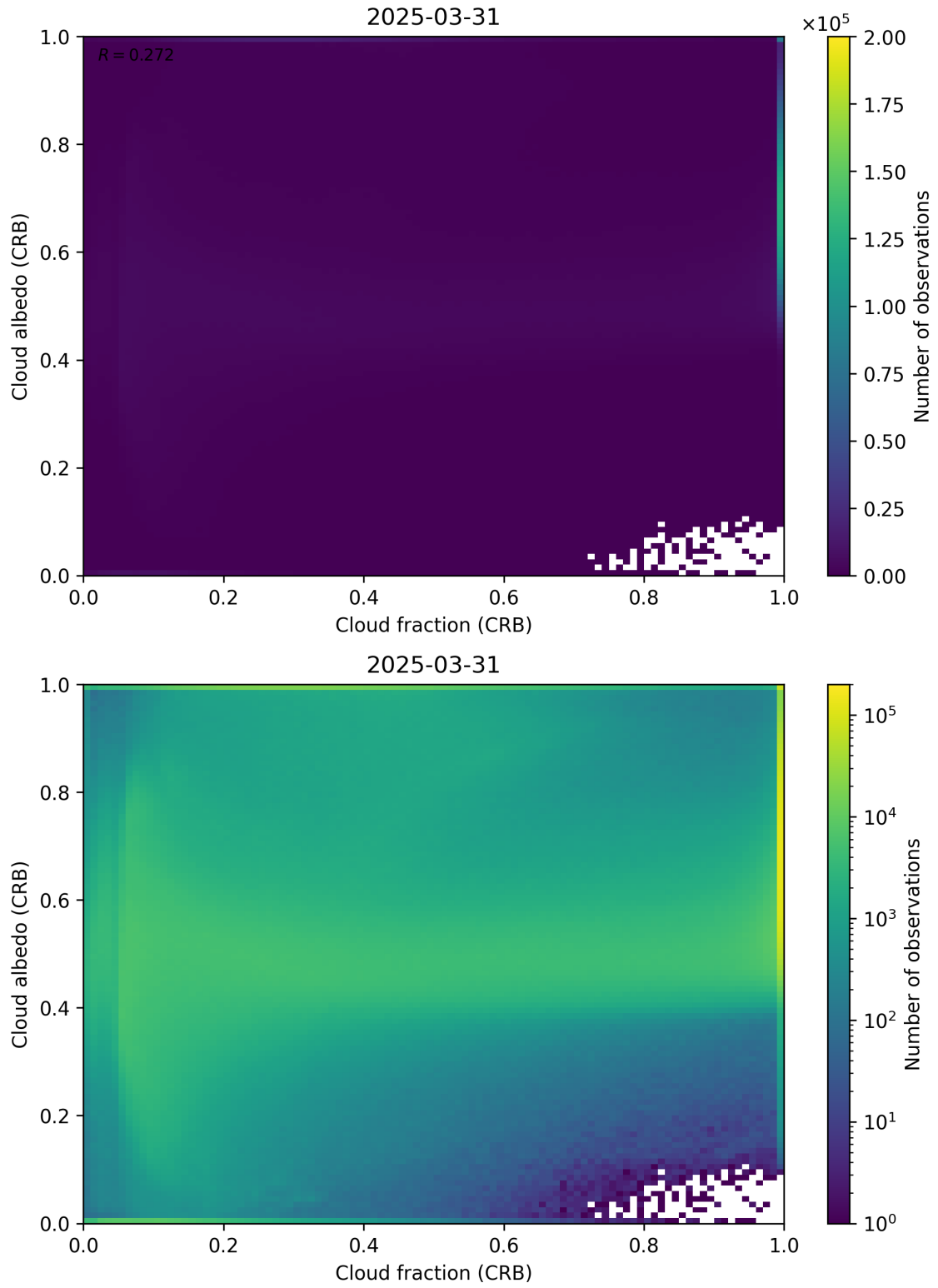
Figure 77: Scatter density plot of “Cloud fraction (CRB)” against “Cloud albedo (CRB)” for 2025-03-30 to 2025-04-01.
