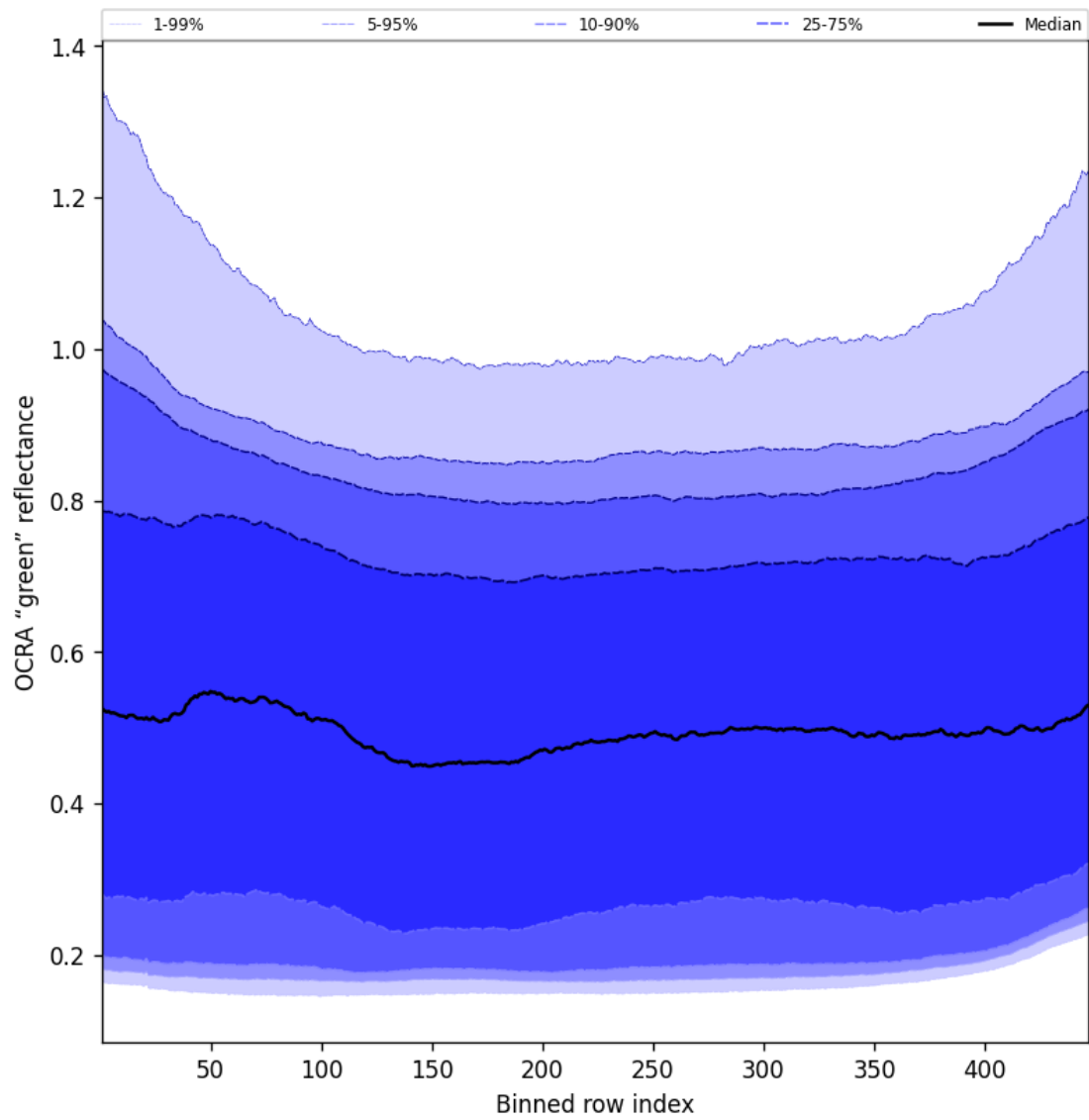
Figure 68: Along track statistics of “OCRA “green” reflectance” for 2025-03-30 to 2025-04-01
