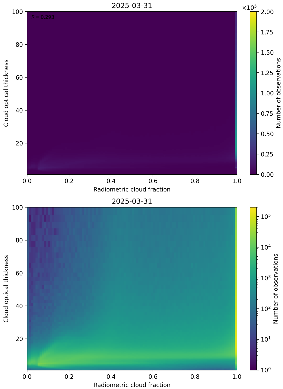
Figure 75: Scatter density plot of “Radiometric cloud fraction” against “Cloud optical thickness” for 2025-03-30 to 2025-04-01.
