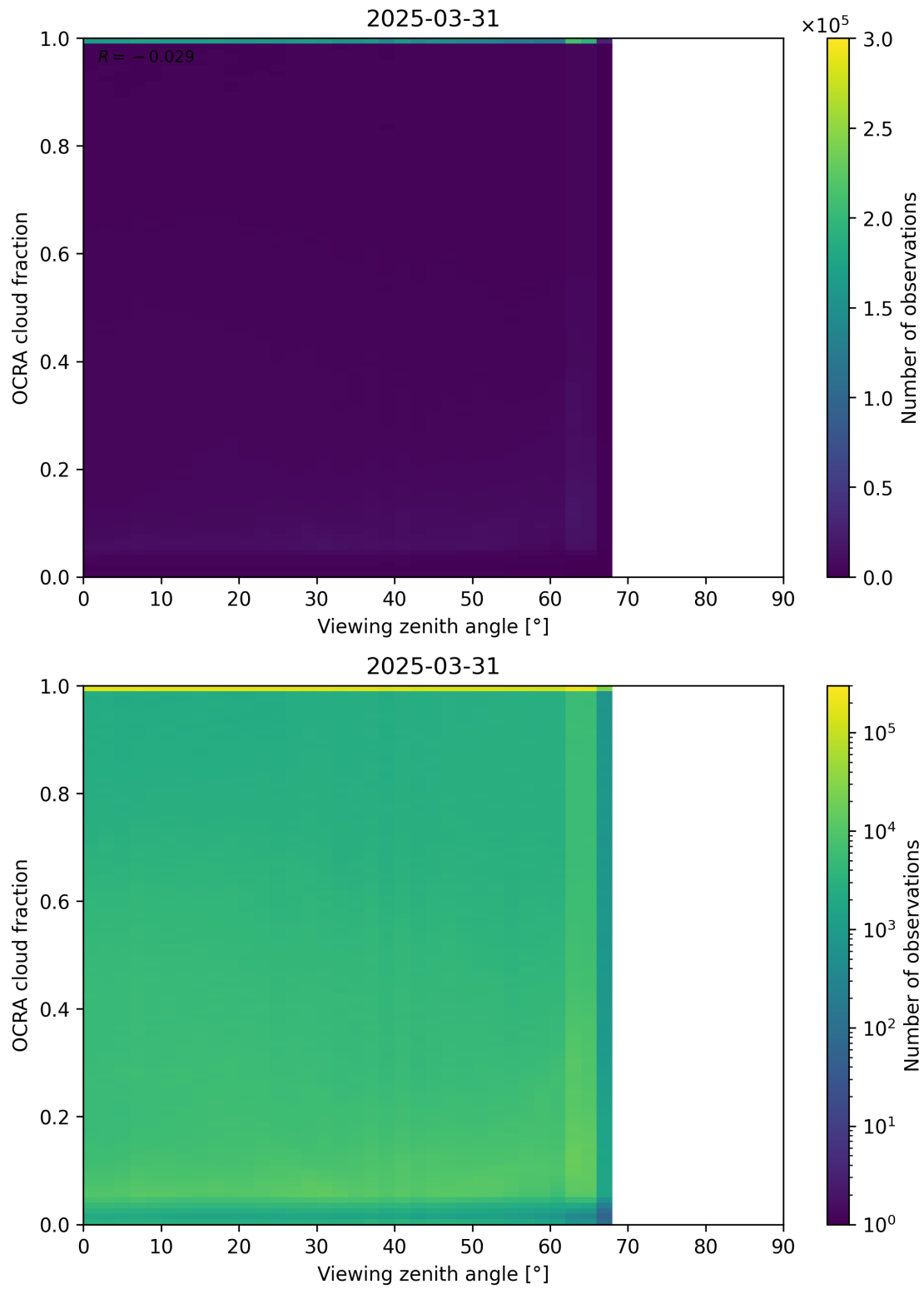
Figure 108: Scatter density plot of “Viewing zenith angle” against “OCRA cloud fraction” for 2025-03-30 to 2025-04-01.
