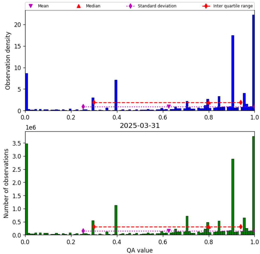
Figure 38: Histogram of “QA value” for 2025-03-30 to 2025-04-01
