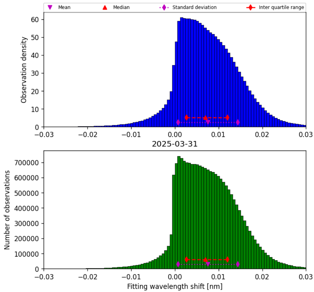
Figure 49: Histogram of “Fitting wavelength shift” for 2025-03-30 to 2025-04-01
