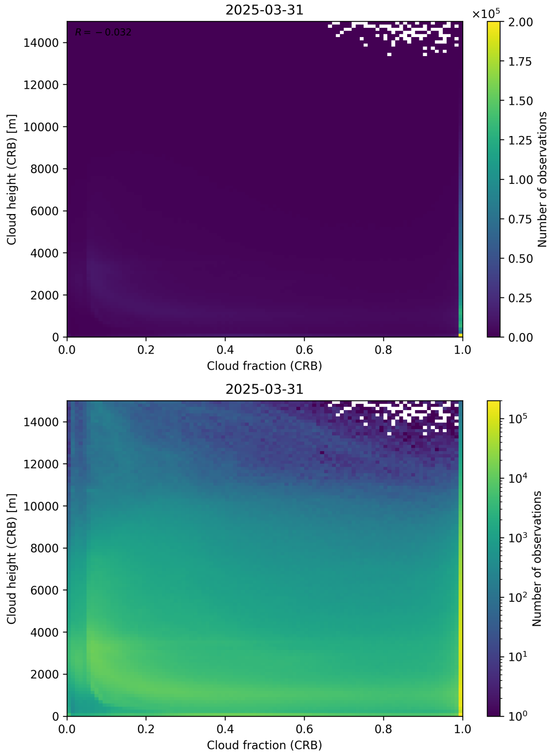
Figure 79: Scatter density plot of “Cloud fraction (CRB)” against “Cloud height (CRB)” for 2025-03-30 to 2025-04-01.
