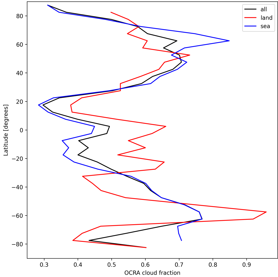
Figure 34: Zonal average of “OCRA cloud fraction” for 2025-03-30 to 2025-04-01.
