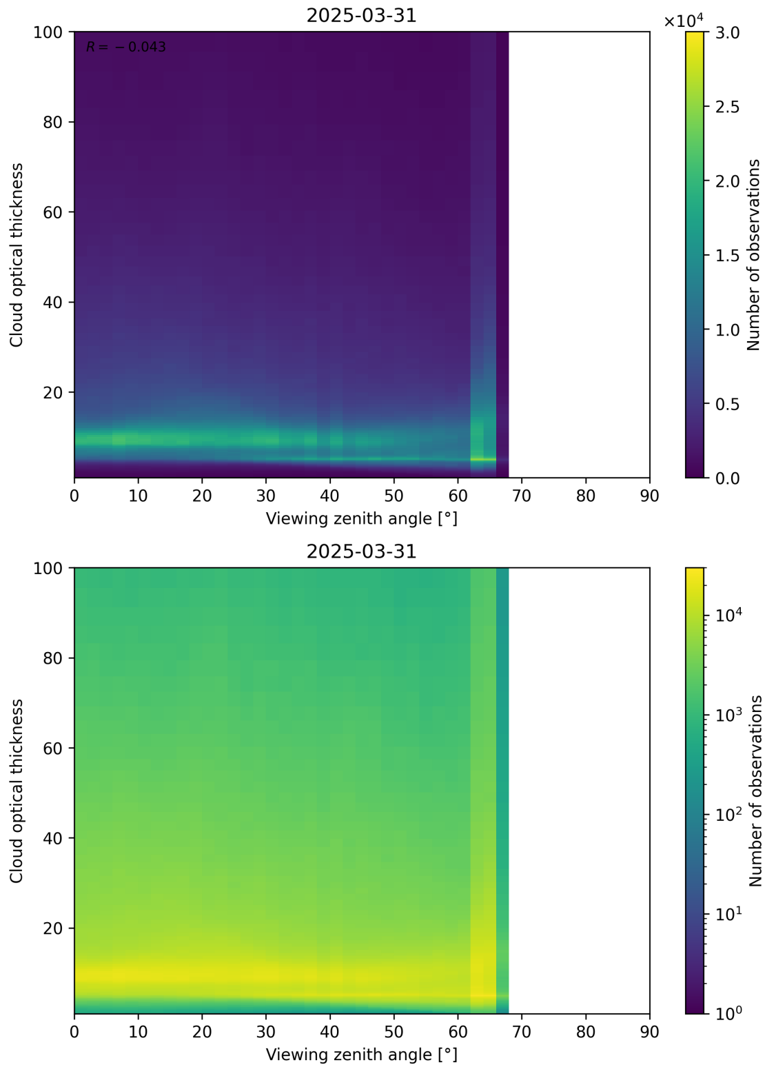
Figure 111: Scatter density plot of “Viewing zenith angle” against “Cloud optical thickness” for 2025-03-30 to 2025-04-01.
