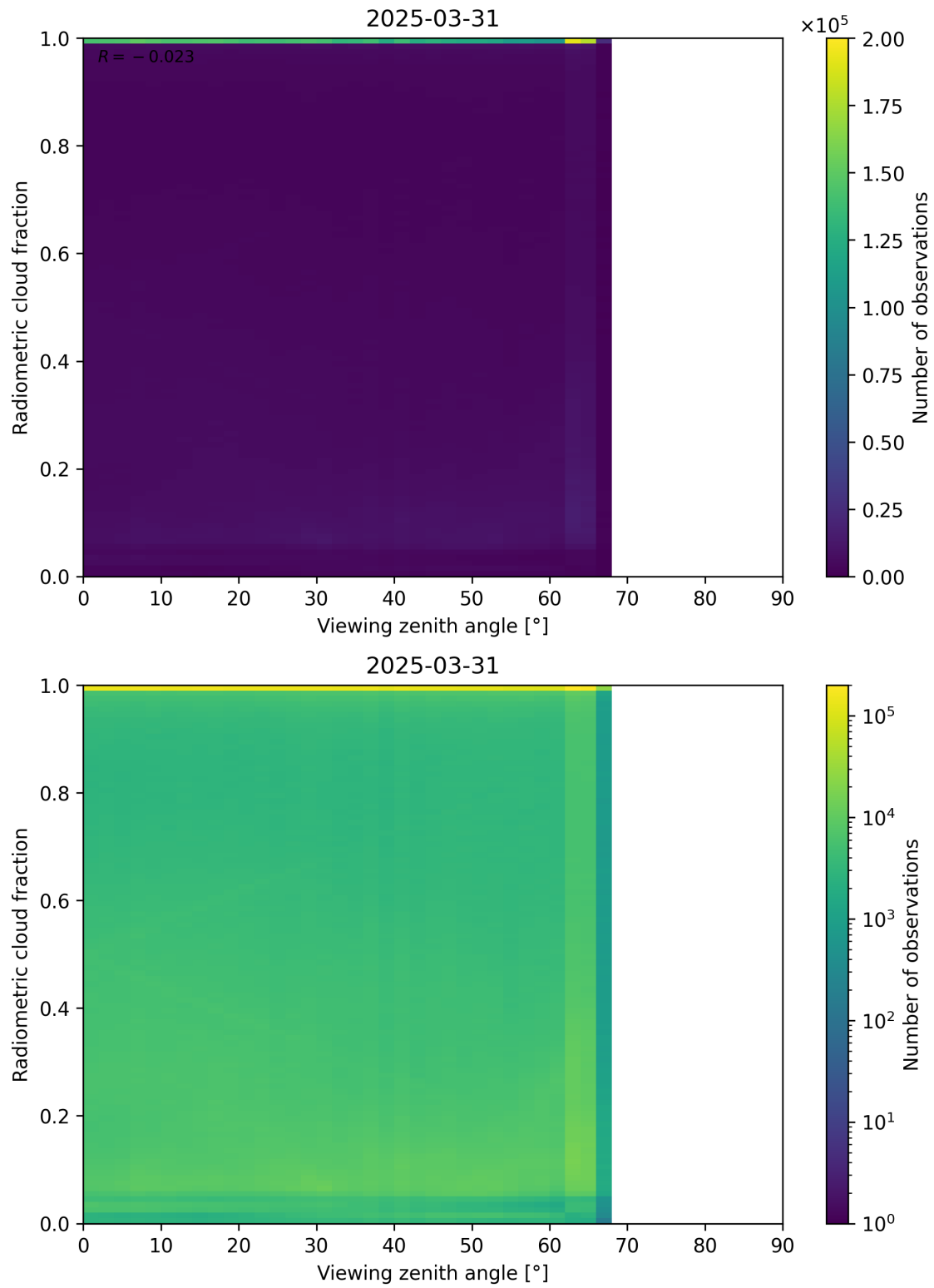
Figure 107: Scatter density plot of “Viewing zenith angle” against “Radiometric cloud fraction” for 2025-03-30 to 2025-04-01.
