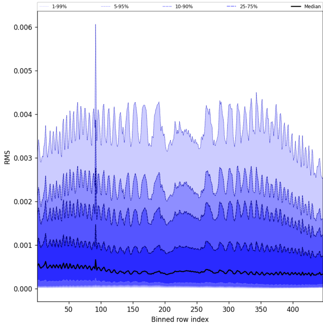
Figure 63: Along track statistics of “RMS” for 2025-03-30 to 2025-04-01
