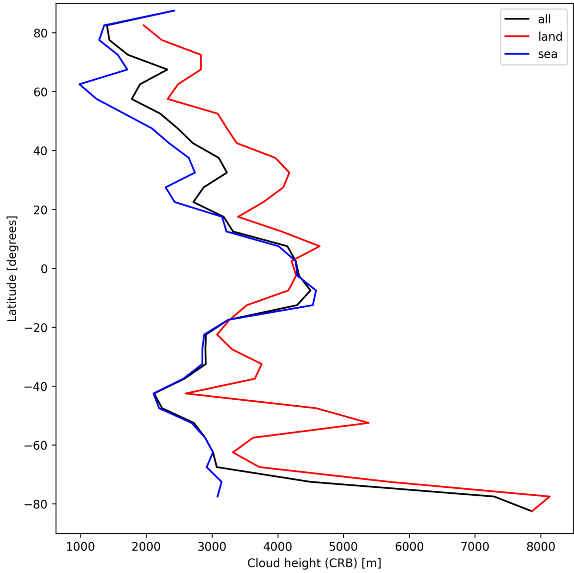
Figure 27: Zonal average of “Cloud height (CRB)” for 2025-04-04 to 2025-04-06.
