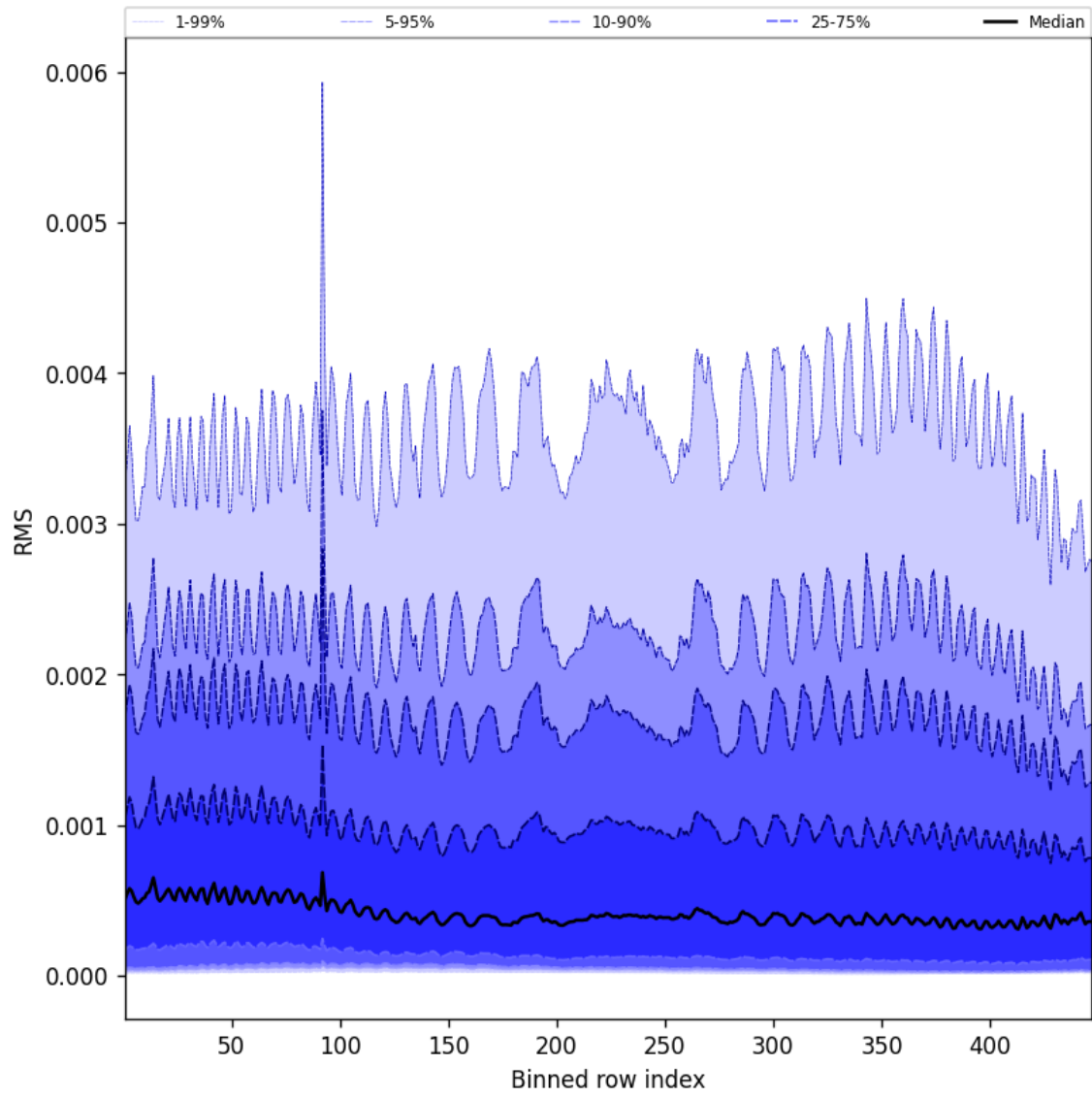
Figure 63: Along track statistics of “RMS” for 2025-04-04 to 2025-04-06
