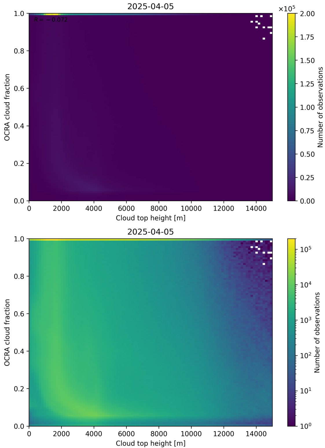
Figure 87: Scatter density plot of “Cloud top height” against “OCRA cloud fraction” for 2025-04-04 to 2025-04-06.
