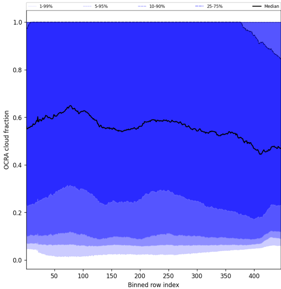
Figure 66: Along track statistics of “OCRA cloud fraction” for 2025-04-04 to 2025-04-06
