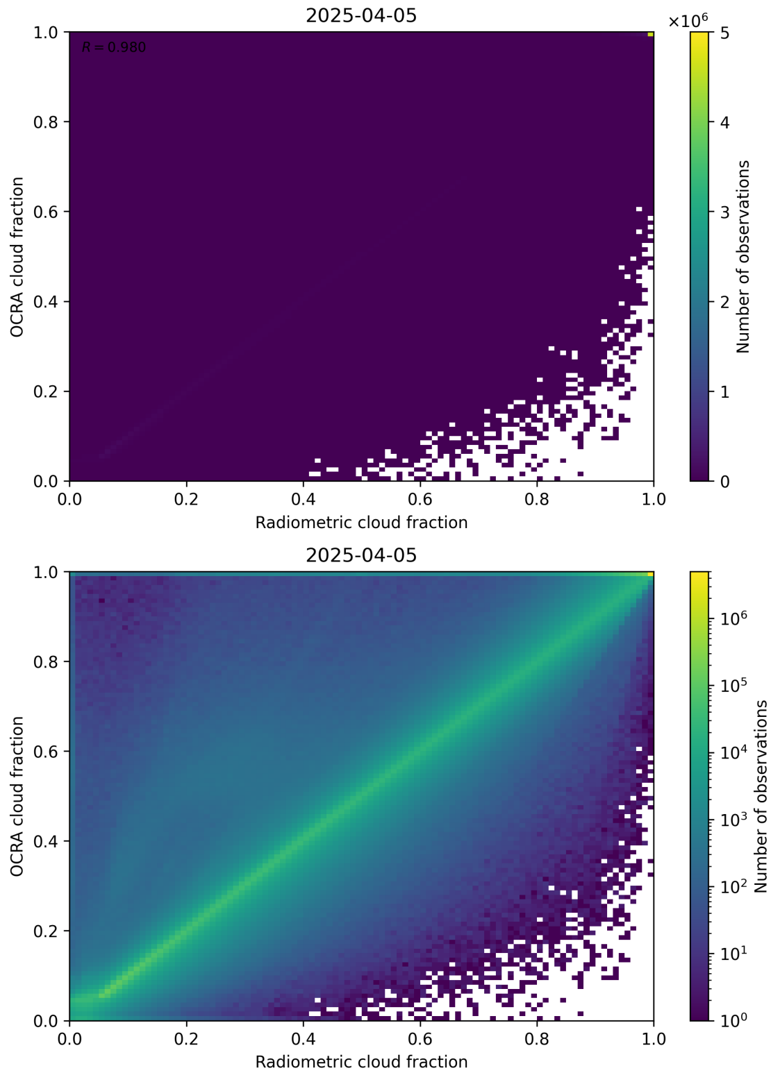
Figure 72: Scatter density plot of “Radiometric cloud fraction” against “OCRA cloud fraction” for 2025-04-04 to 2025-04-06.
