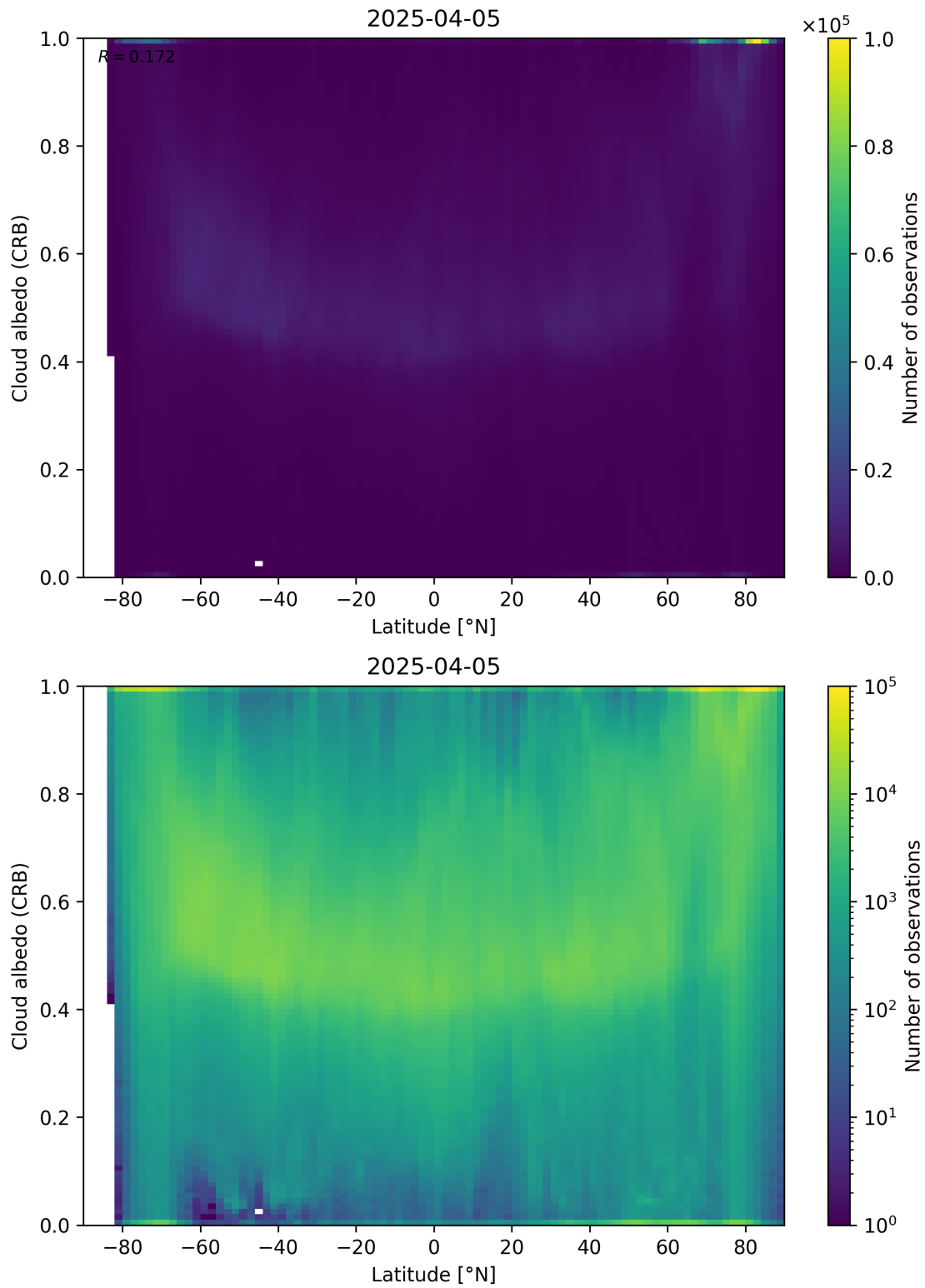
Figure 91: Scatter density plot of “Latitude” against “Cloud albedo (CRB)” for 2025-04-04 to 2025-04-06.
