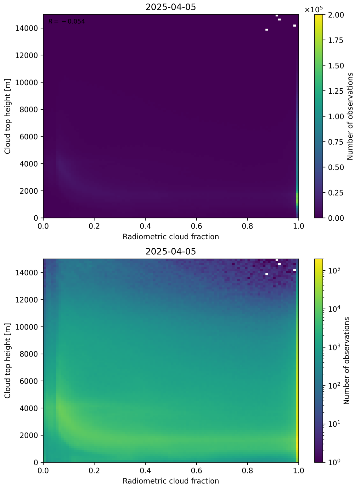
Figure 76: Scatter density plot of “Radiometric cloud fraction” against “Cloud top height” for 2025-04-04 to 2025-04-06.
