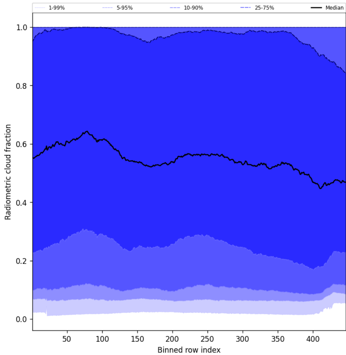
Figure 55: Along track statistics of “Radiometric cloud fraction” for 2025-04-04 to 2025-04-06
