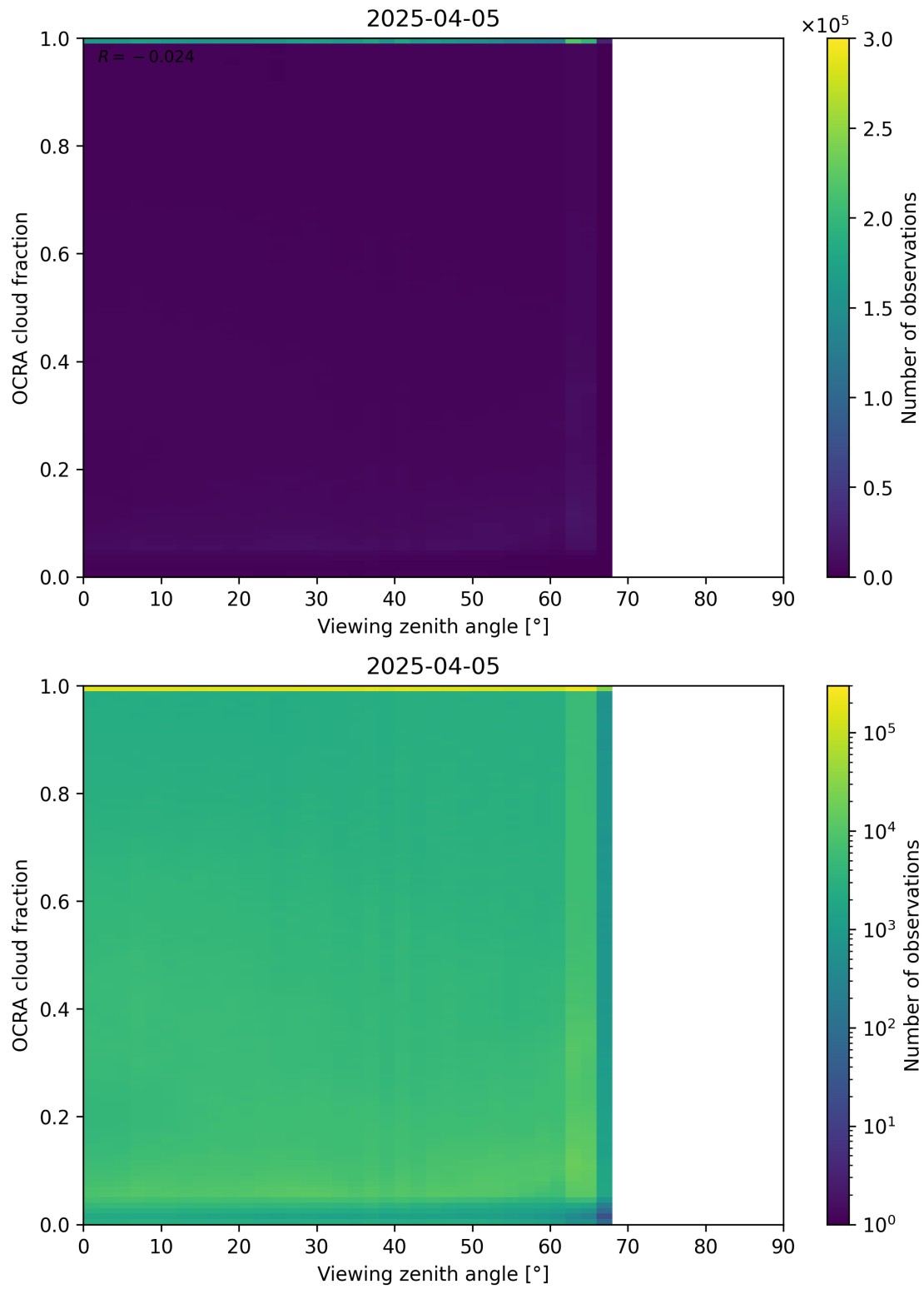
Figure 108: Scatter density plot of “Viewing zenith angle” against “OCRA cloud fraction” for 2025-04-04 to 2025-04-06.
