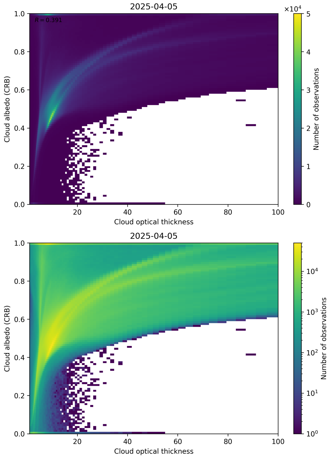
Figure 82: Scatter density plot of “Cloud optical thickness” against “Cloud albedo (CRB)” for 2025-04-04 to 2025-04-06.
