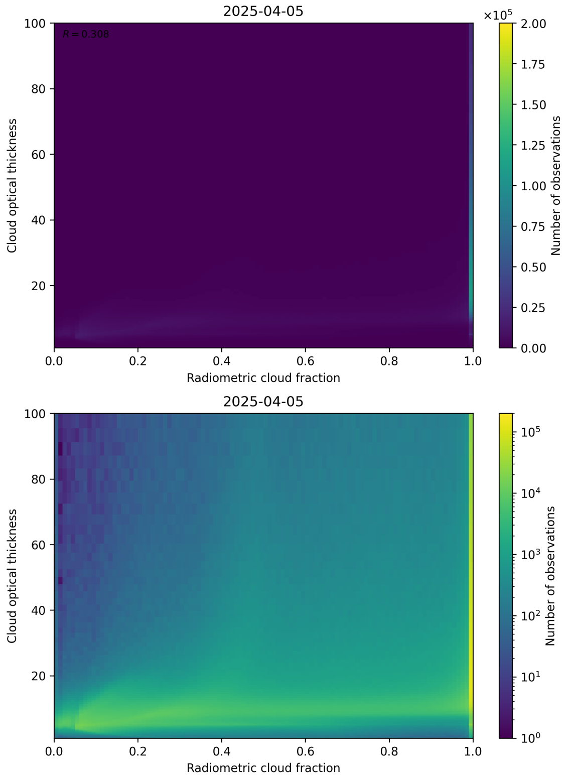
Figure 75: Scatter density plot of “Radiometric cloud fraction” against “Cloud optical thickness” for 2025-04-04 to 2025-04-06.
