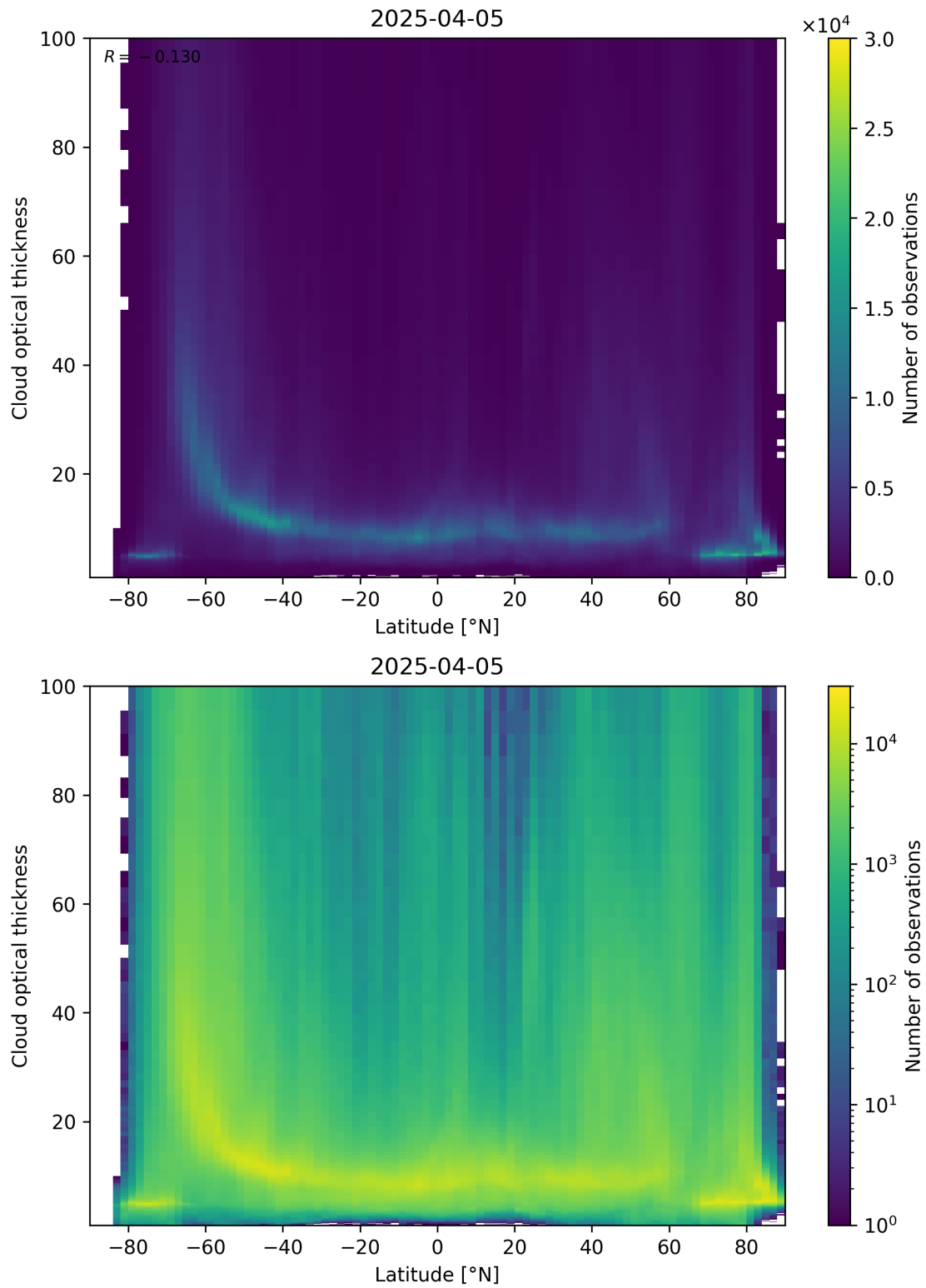
Figure 96: Scatter density plot of “Latitude” against “Cloud optical thickness” for 2025-04-04 to 2025-04-06.
