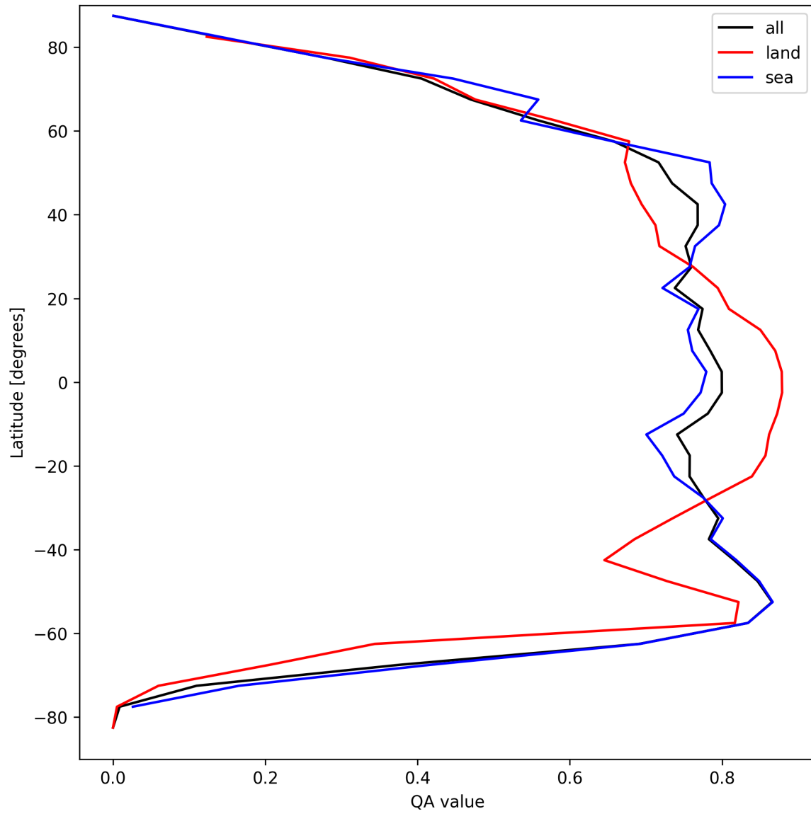
Figure 22: Zonal average of “QA value” for 2025-04-04 to 2025-04-06.
