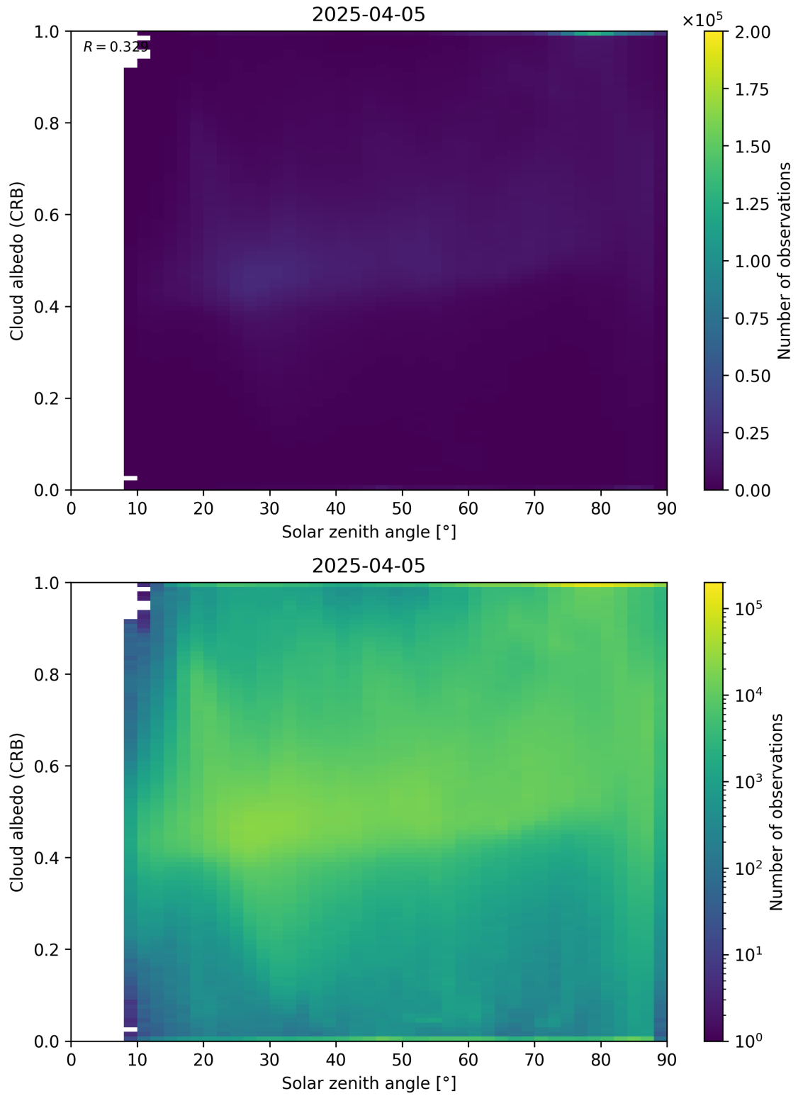
Figure 98: Scatter density plot of “Solar zenith angle” against “Cloud albedo (CRB)” for 2025-04-04 to 2025-04-06.
