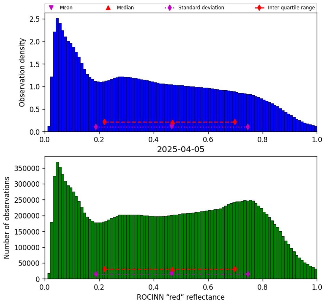
Figure 53: Histogram of “ROCINN “red” reflectance” for 2025-04-04 to 2025-04-06
