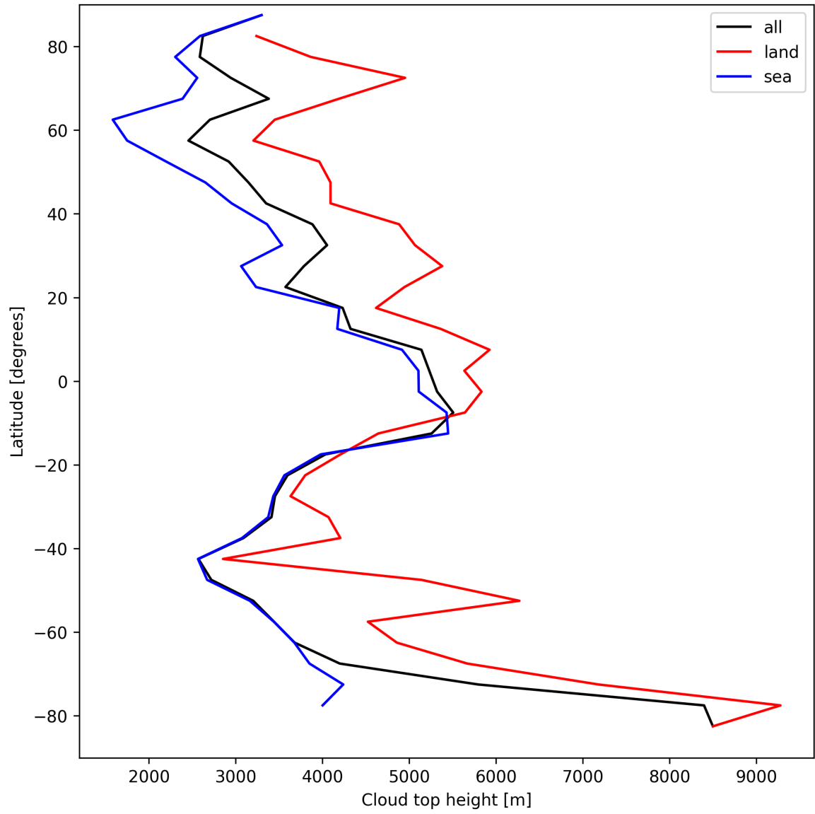
Figure 24: Zonal average of “Cloud top height” for 2025-04-04 to 2025-04-06.
