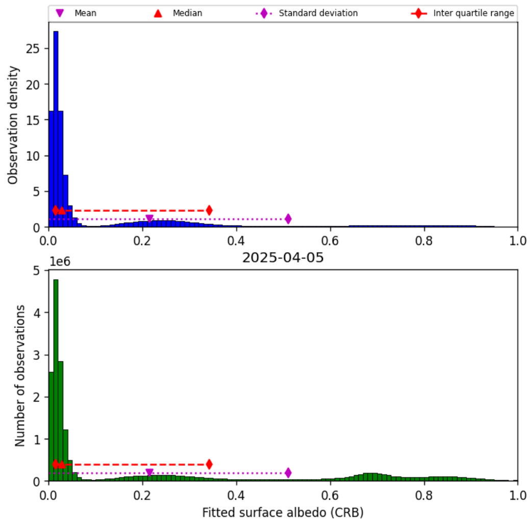
Figure 46: Histogram of “Fitted surface albedo (CRB)” for 2025-04-04 to 2025-04-06
