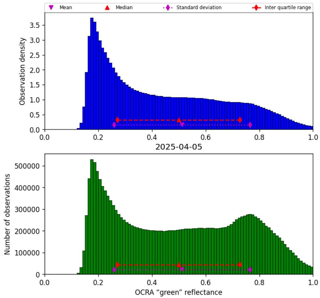
Figure 52: Histogram of “OCRA “green” reflectance” for 2025-04-04 to 2025-04-06
