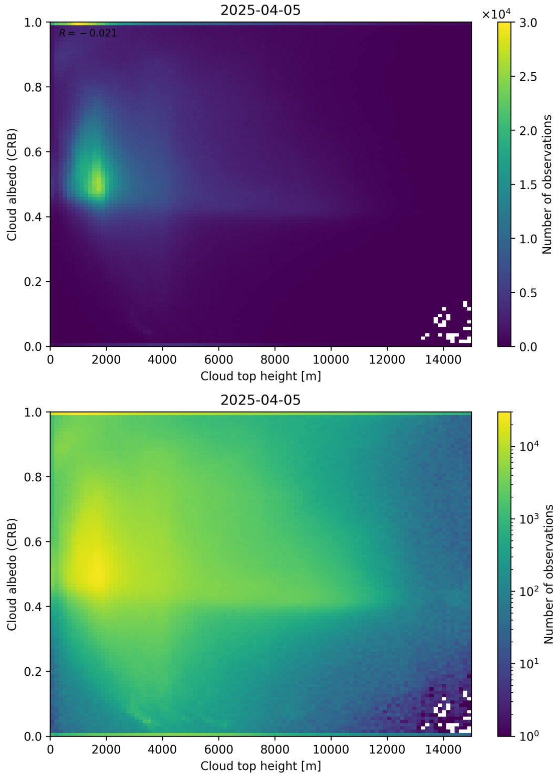
Figure 86: Scatter density plot of “Cloud top height” against “Cloud albedo (CRB)” for 2025-04-04 to 2025-04-06.
