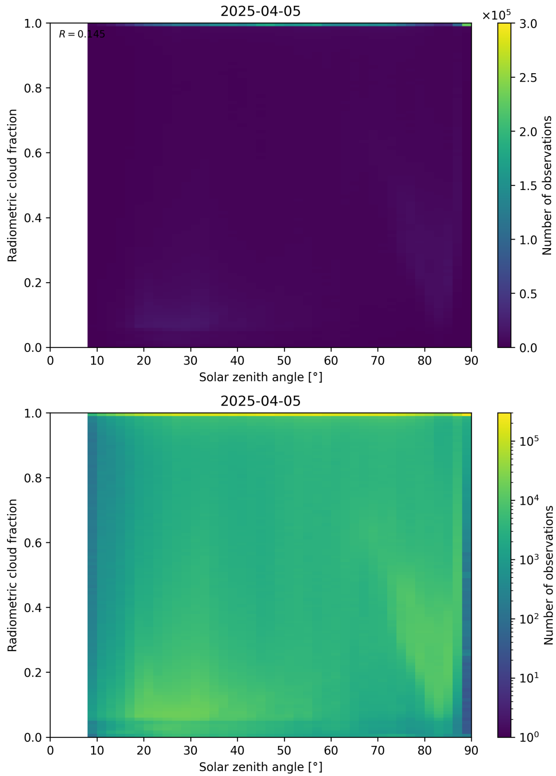
Figure 99: Scatter density plot of “Solar zenith angle” against “Radiometric cloud fraction” for 2025-04-04 to 2025-04-06.
