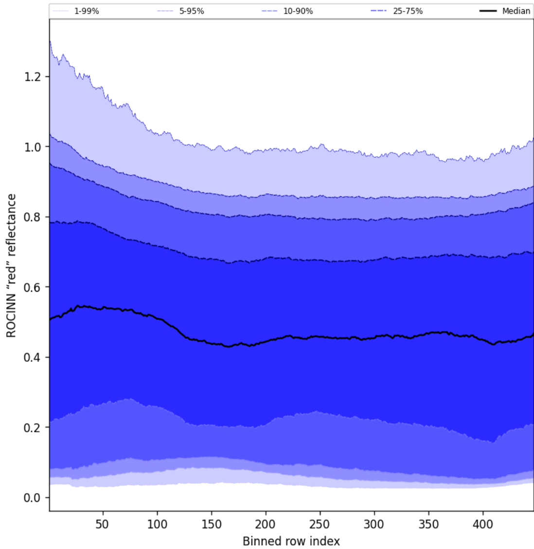
Figure 69: Along track statistics of “ROCINN “red” reflectance” for 2025-04-04 to 2025-04-06
