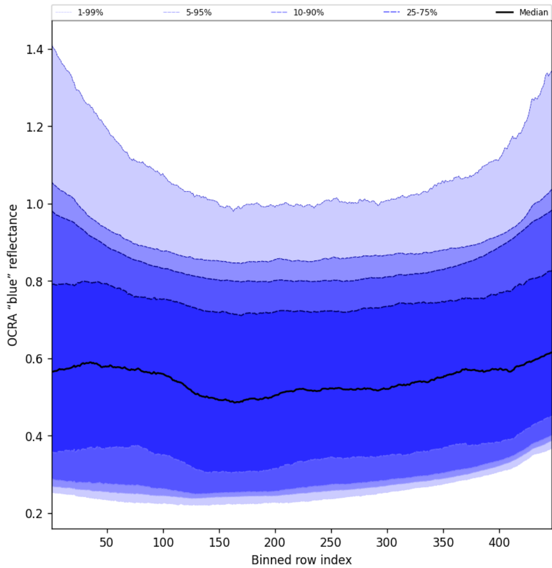
Figure 67: Along track statistics of “OCRA “blue” reflectance” for 2025-04-04 to 2025-04-06
