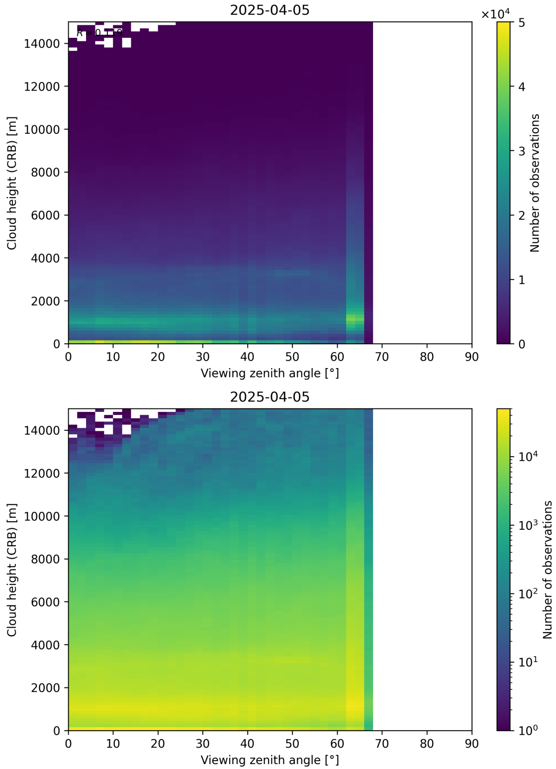
Figure 110: Scatter density plot of “Viewing zenith angle” against “Cloud height (CRB)” for 2025-04-04 to 2025-04-06.
