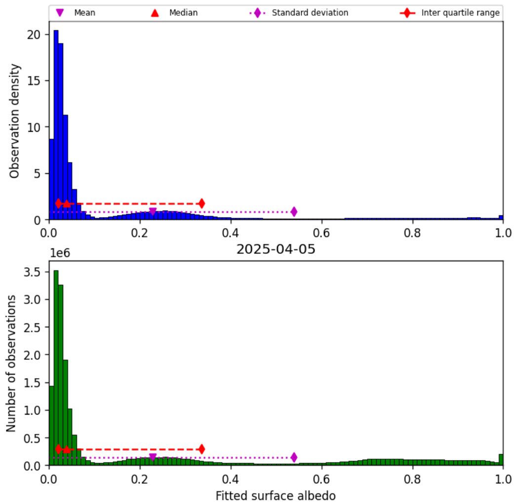
Figure 45: Histogram of “Fitted surface albedo” for 2025-04-04 to 2025-04-06
