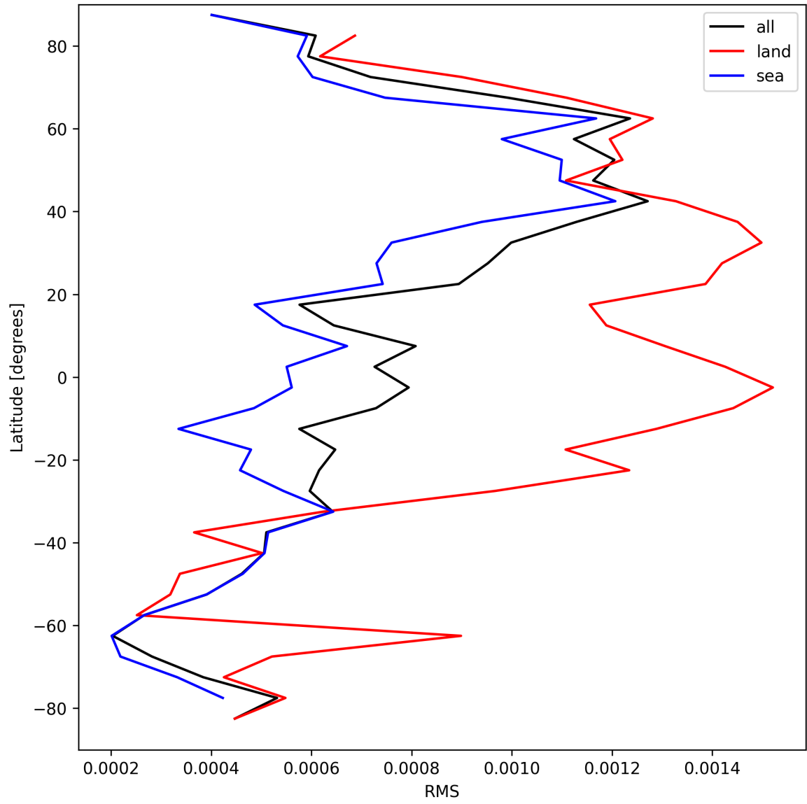
Figure 31: Zonal average of “RMS” for 2025-04-04 to 2025-04-06.
