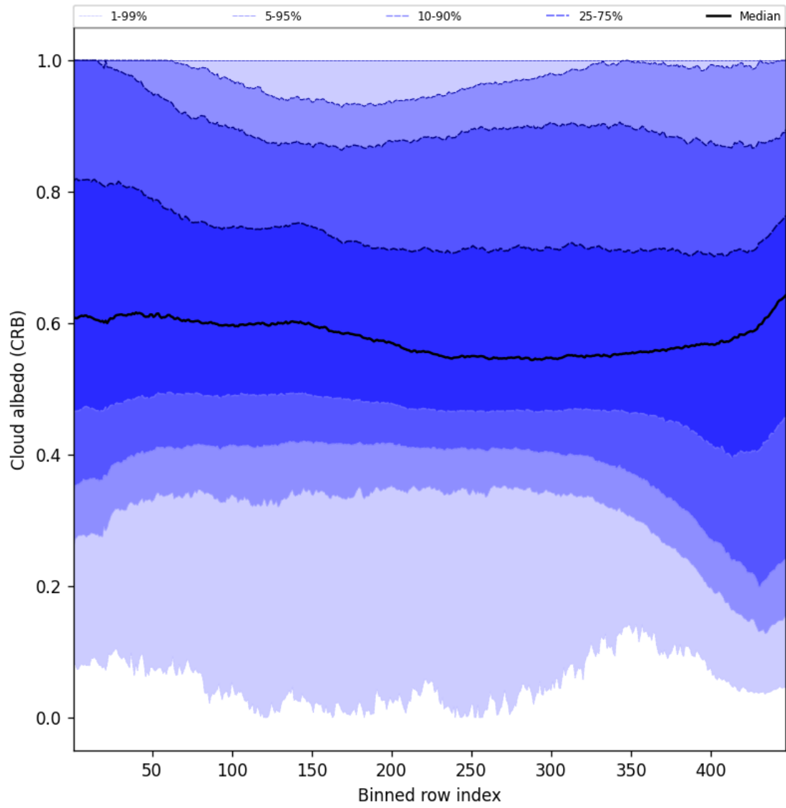
Figure 60: Along track statistics of “Cloud albedo (CRB)” for 2025-04-04 to 2025-04-06
