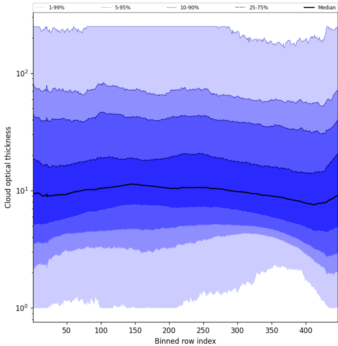
Figure 57: Along track statistics of “Cloud optical thickness” for 2025-04-04 to 2025-04-06
