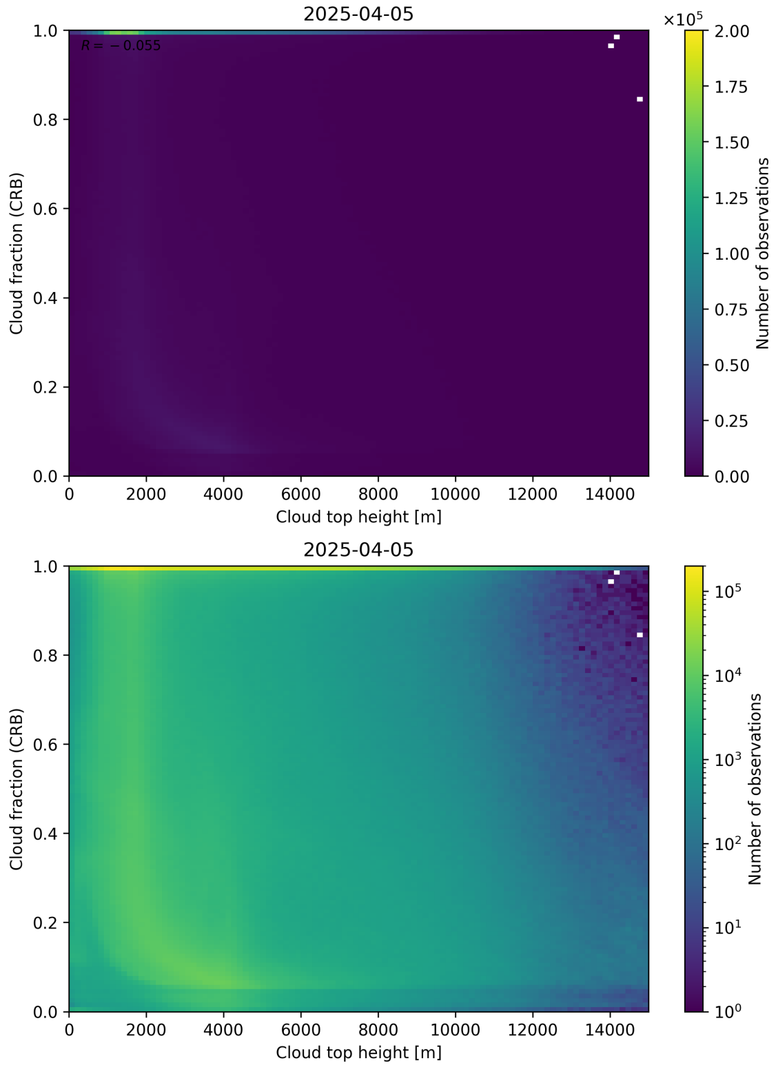
Figure 88: Scatter density plot of “Cloud top height” against “Cloud fraction (CRB)” for 2025-04-04 to 2025-04-06.
