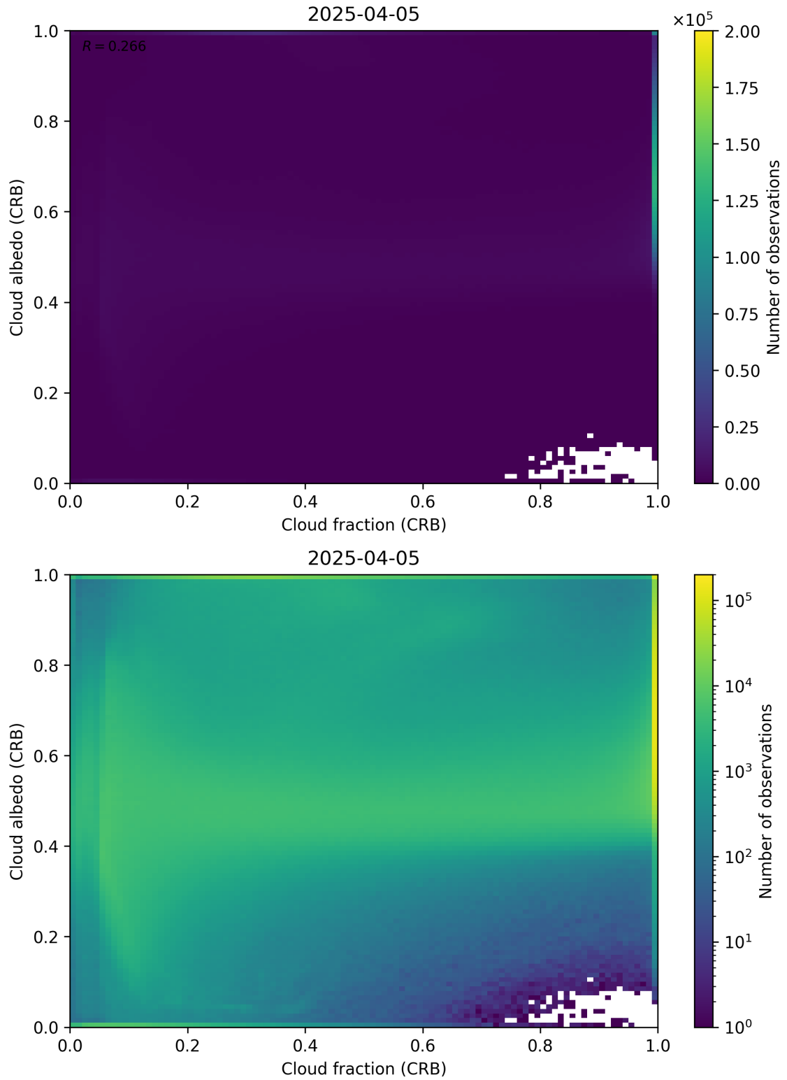
Figure 77: Scatter density plot of “Cloud fraction (CRB)” against “Cloud albedo (CRB)” for 2025-04-04 to 2025-04-06.
