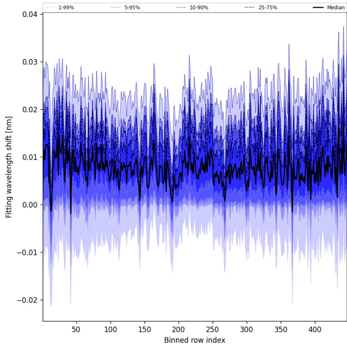
Figure 65: Along track statistics of “Fitting wavelength shift” for 2025-04-04 to 2025-04-06
