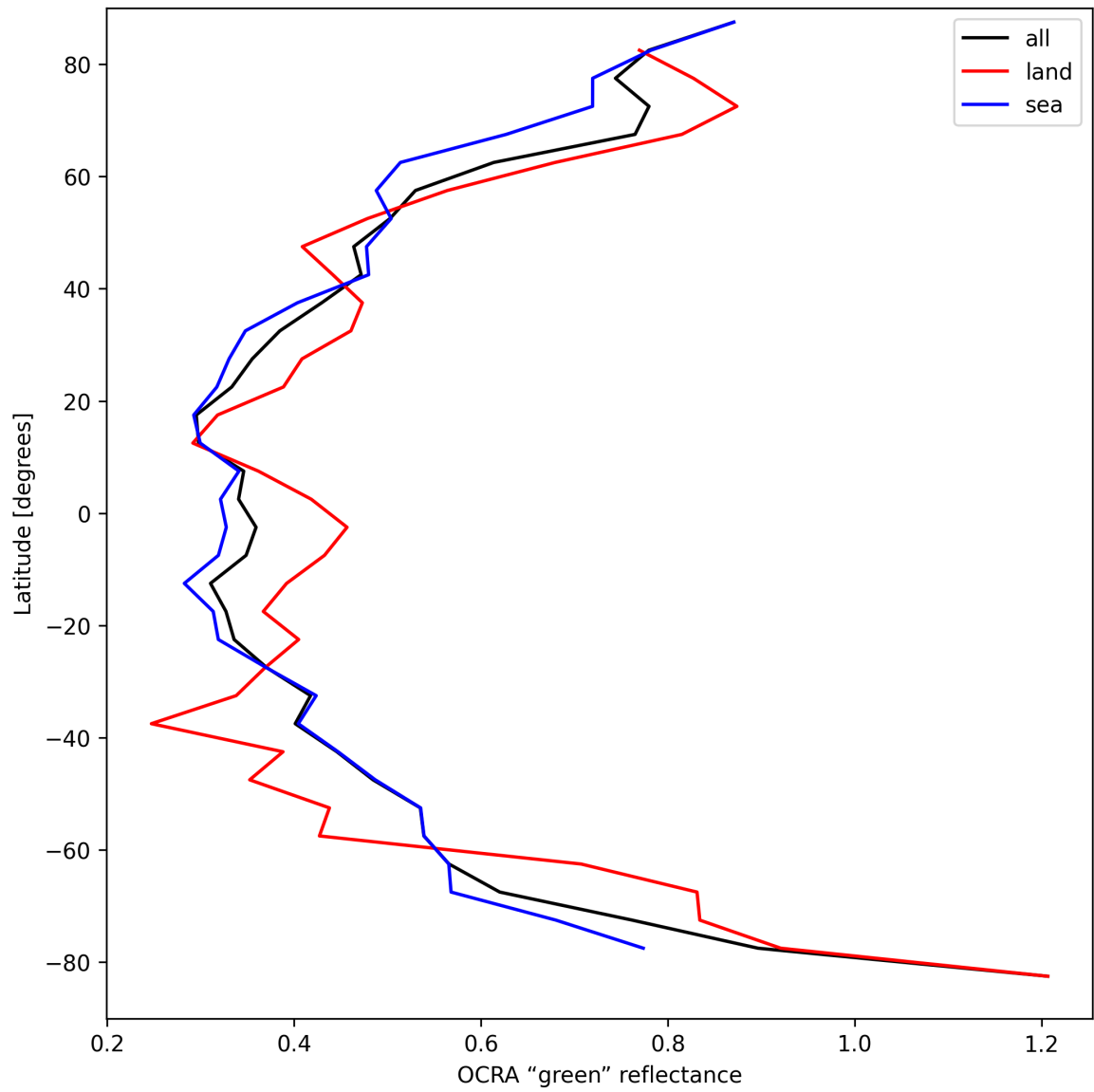
Figure 36: Zonal average of "OCRA "green" reflectance" for 2025-04-04 to 2025-04-06.
