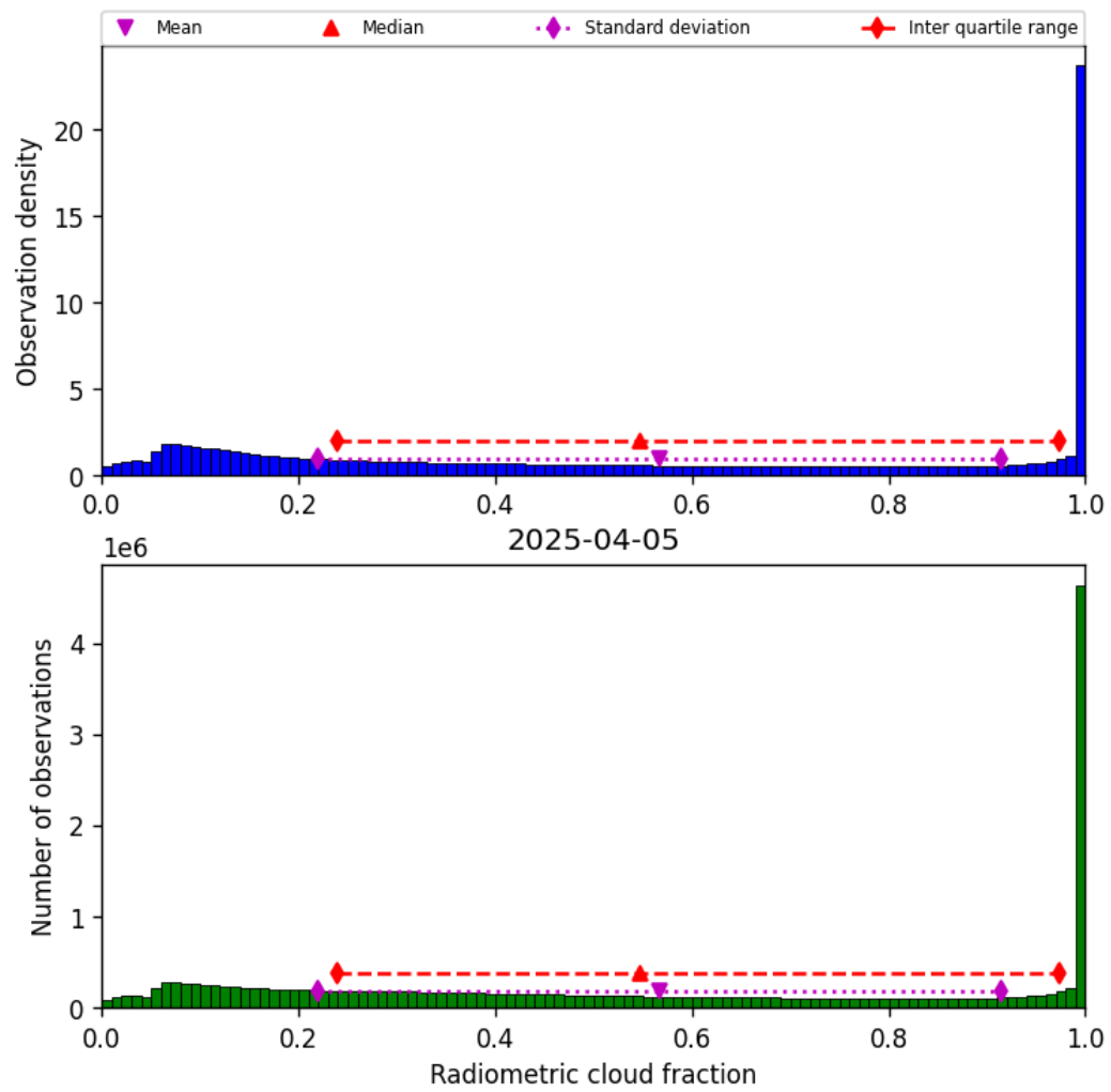
Figure 39: Histogram of “Radiometric cloud fraction” for 2025-04-04 to 2025-04-06
