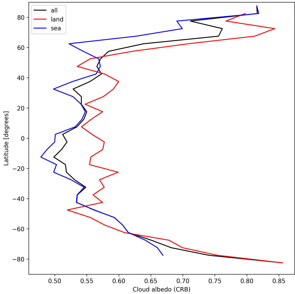
Figure 28: Zonal average of “Cloud albedo (CRB)” for 2025-04-04 to 2025-04-06.
