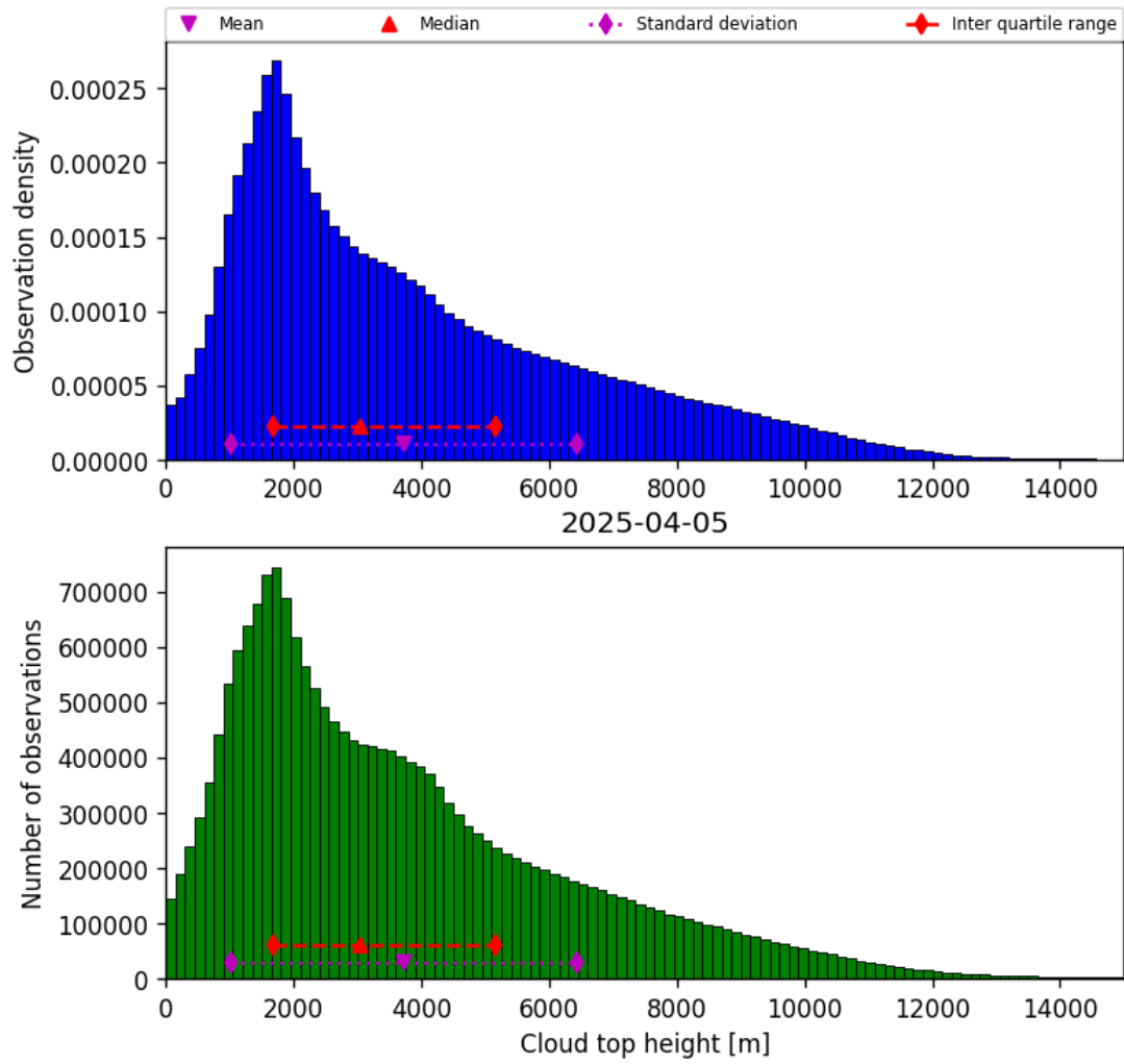
Figure 40: Histogram of “Cloud top height” for 2025-04-04 to 2025-04-06
