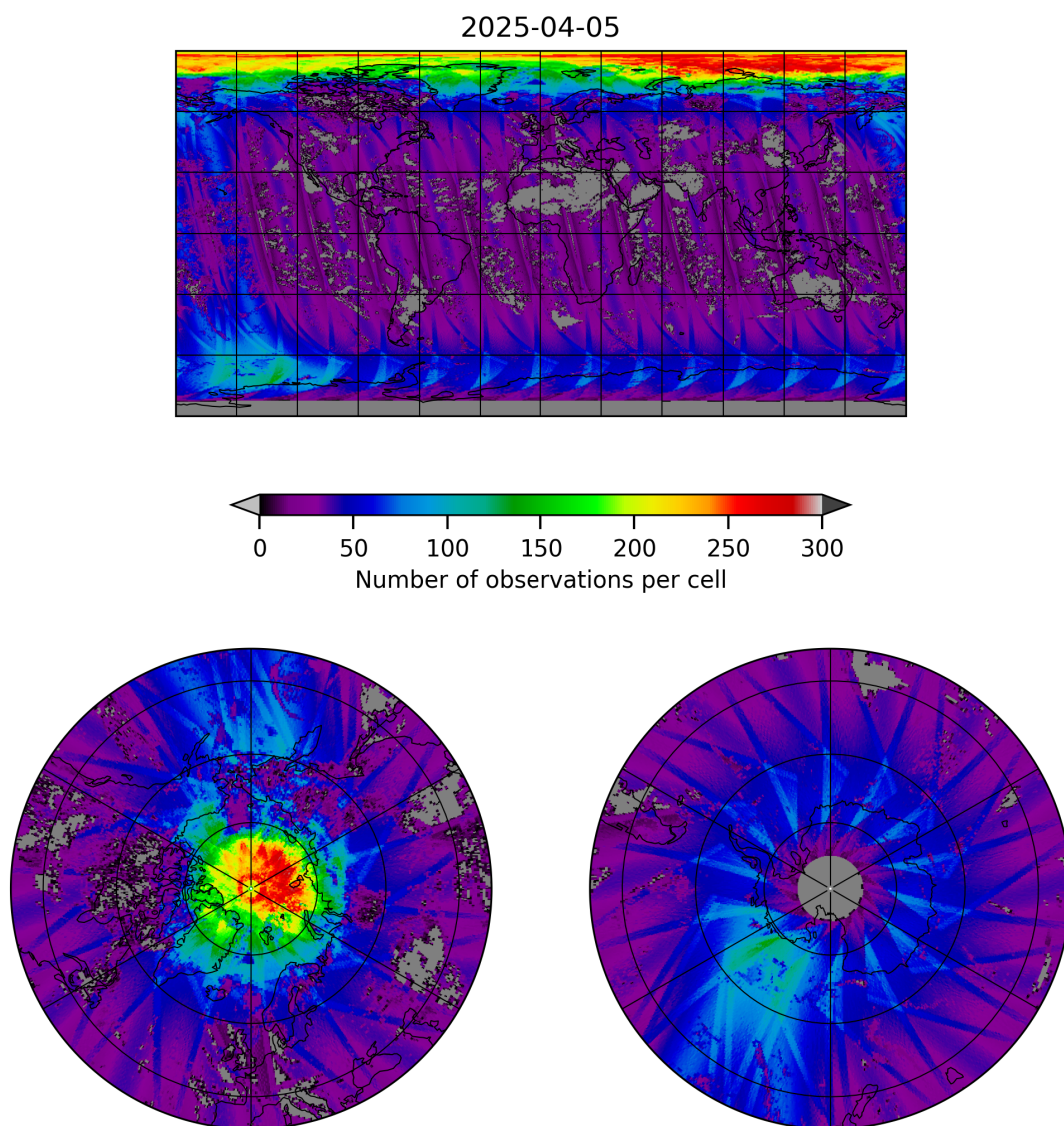
Figure 21: Map of the number of observations for 2025-04-04 to 2025-04-06
