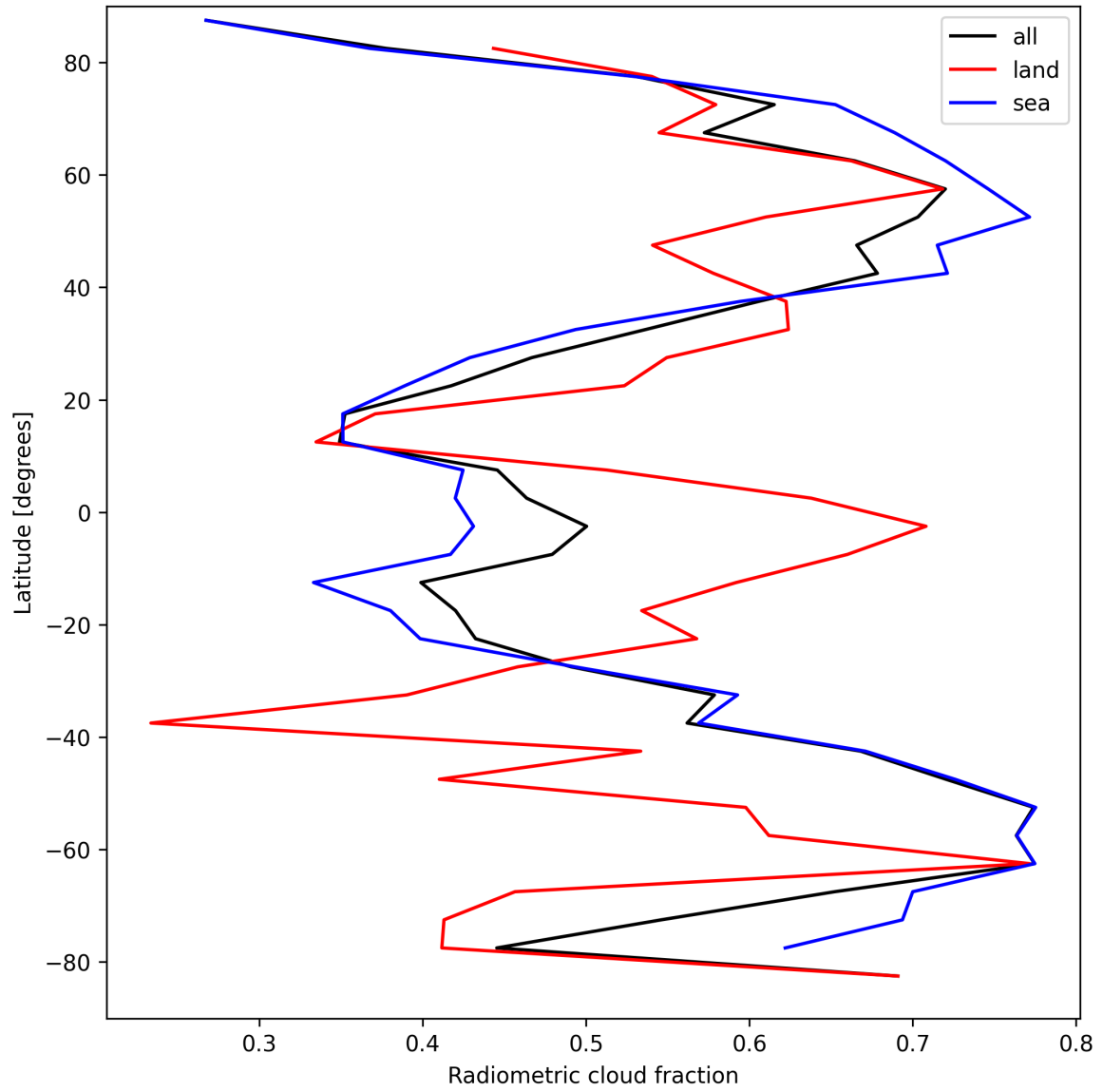
Figure 23: Zonal average of “Radiometric cloud fraction” for 2025-04-04 to 2025-04-06.
