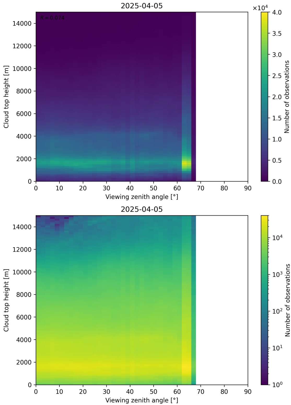
Figure 112: Scatter density plot of “Viewing zenith angle” against “Cloud top height” for 2025-04-04 to 2025-04-06.
