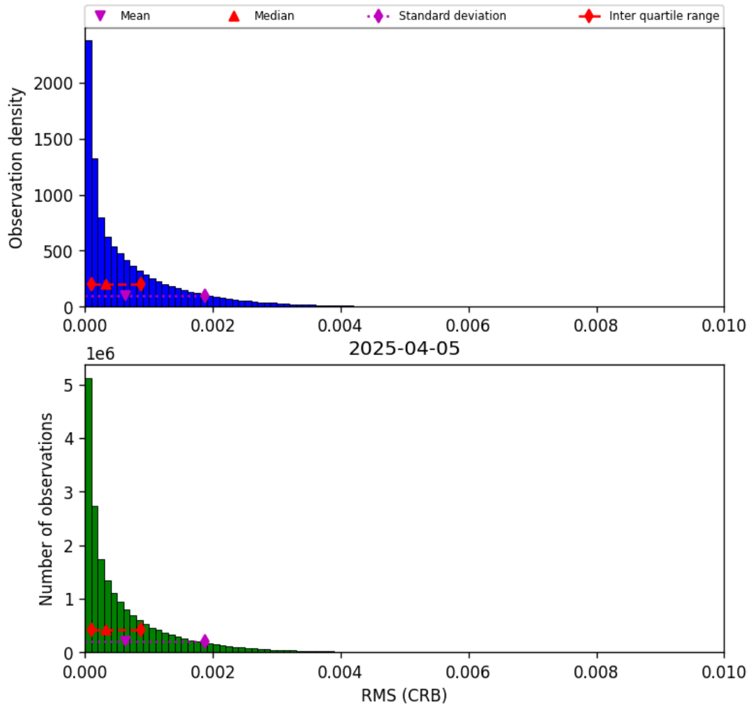
Figure 48: Histogram of “RMS (CRB)” for 2025-04-04 to 2025-04-06
