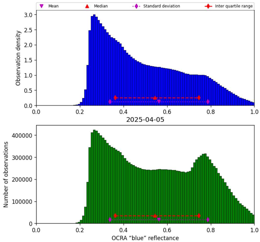
Figure 51: Histogram of “OCRA “blue” reflectance” for 2025-04-04 to 2025-04-06
