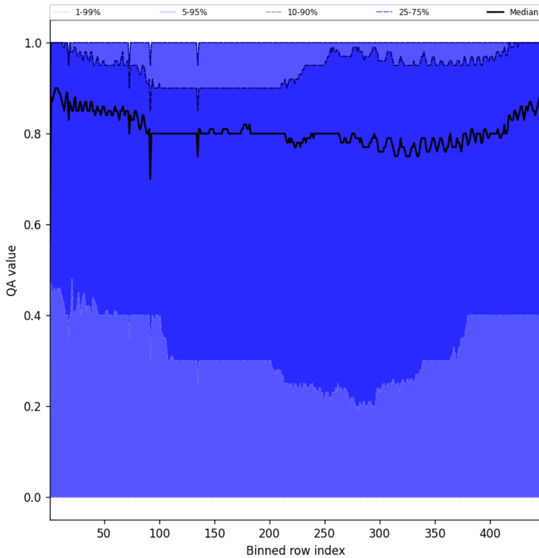
Figure 54: Along track statistics of “QA value” for 2025-04-04 to 2025-04-06
