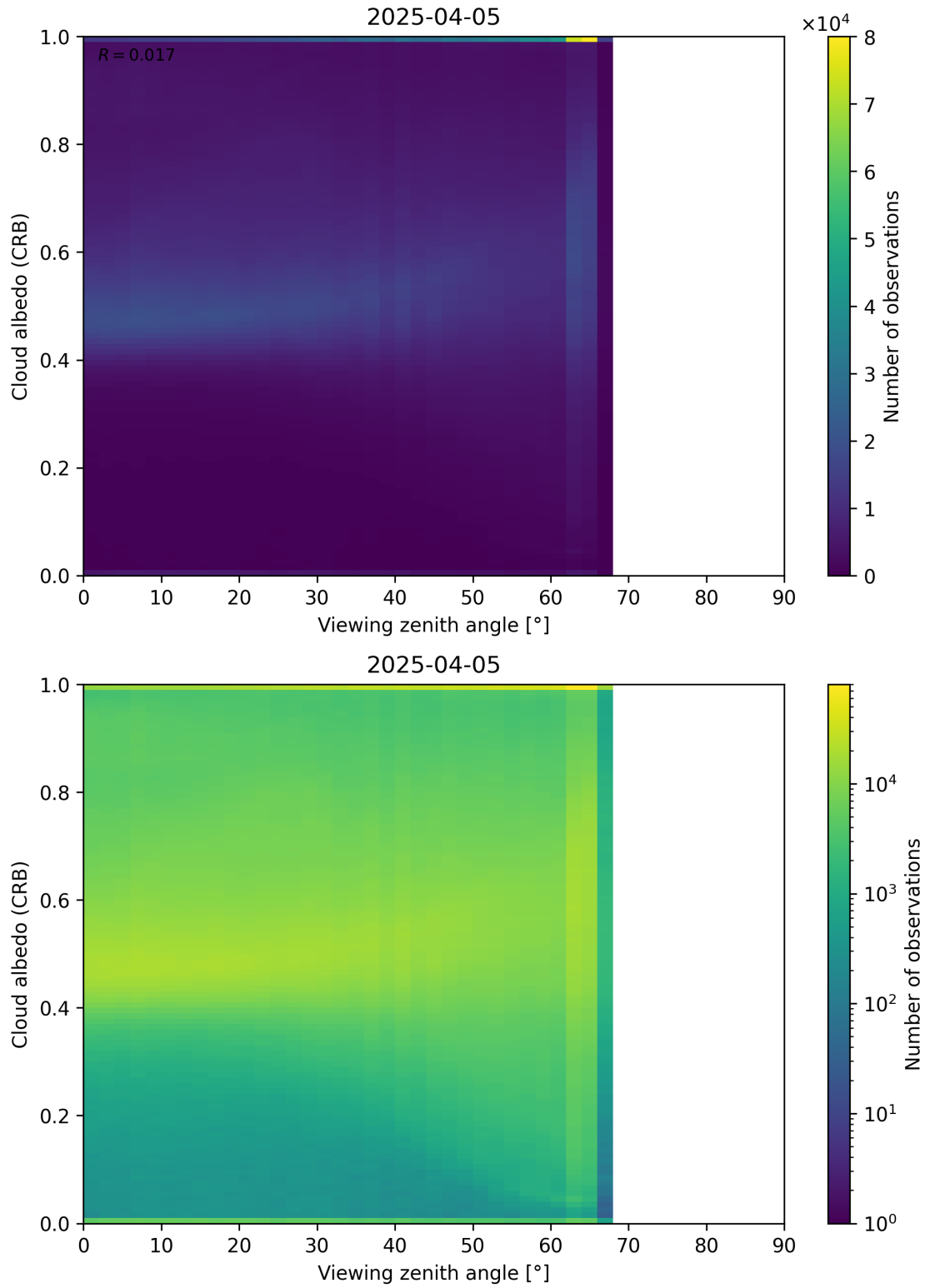
Figure 106: Scatter density plot of “Viewing zenith angle” against “Cloud albedo (CRB)” for 2025-04-04 to 2025-04-06.
