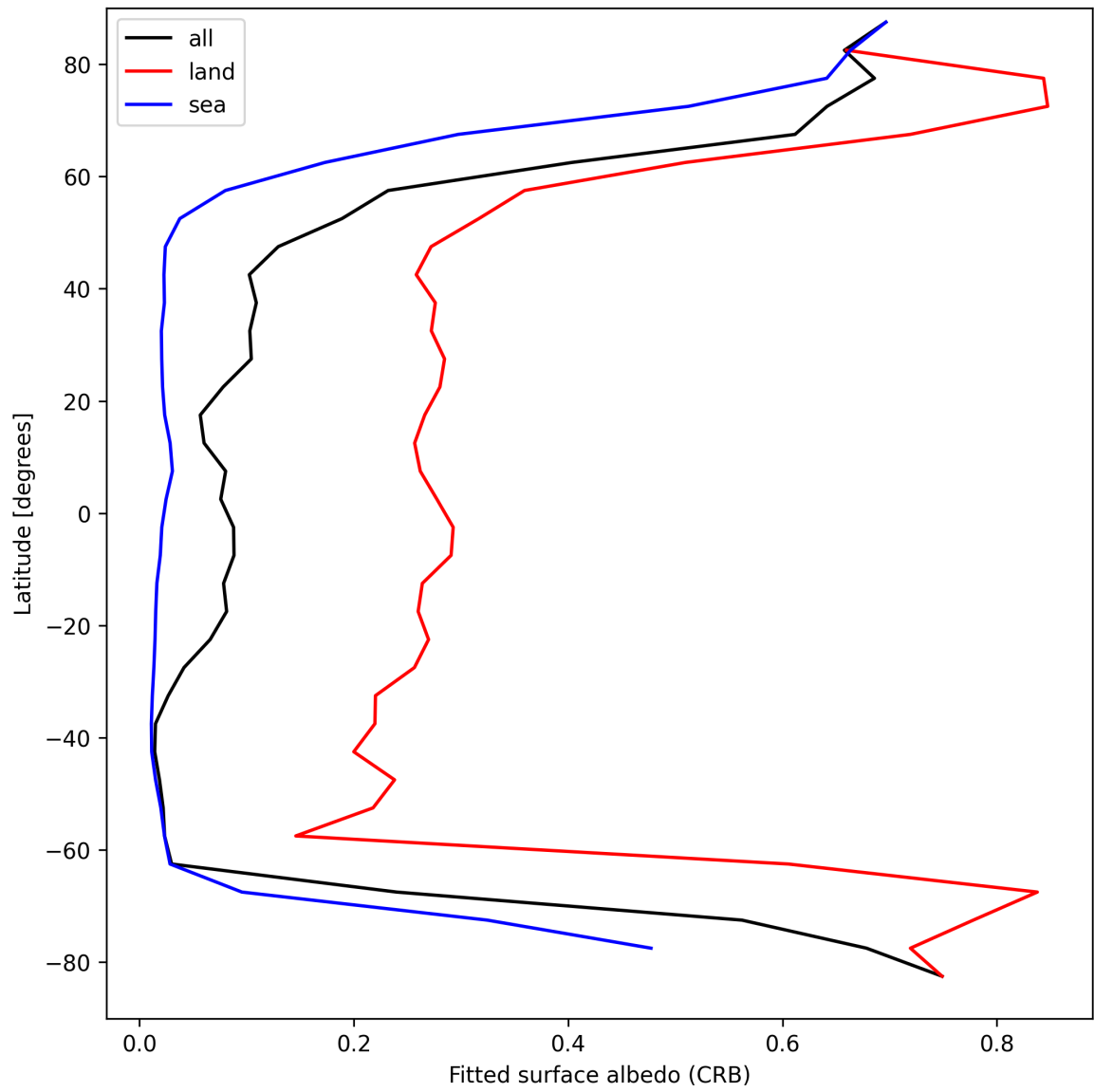
Figure 30: Zonal average of “Fitted surface albedo (CRB)” for 2025-04-04 to 2025-04-06.
