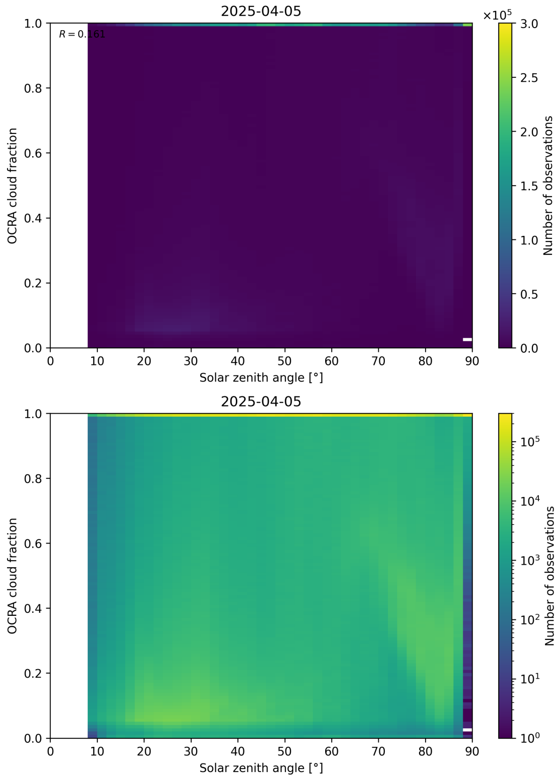
Figure 100: Scatter density plot of “Solar zenith angle” against “OCRA cloud fraction” for 2025-04-04 to 2025-04-06.
