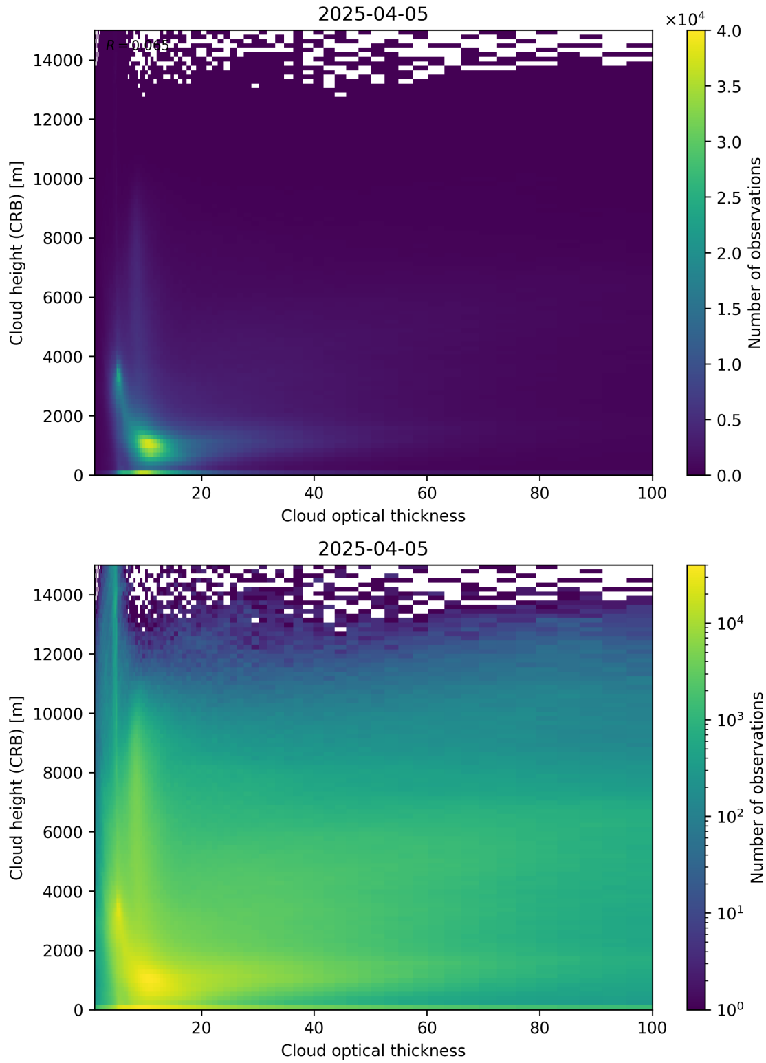
Figure 85: Scatter density plot of “Cloud optical thickness” against “Cloud height (CRB)” for 2025-04-04 to 2025-04-06.
