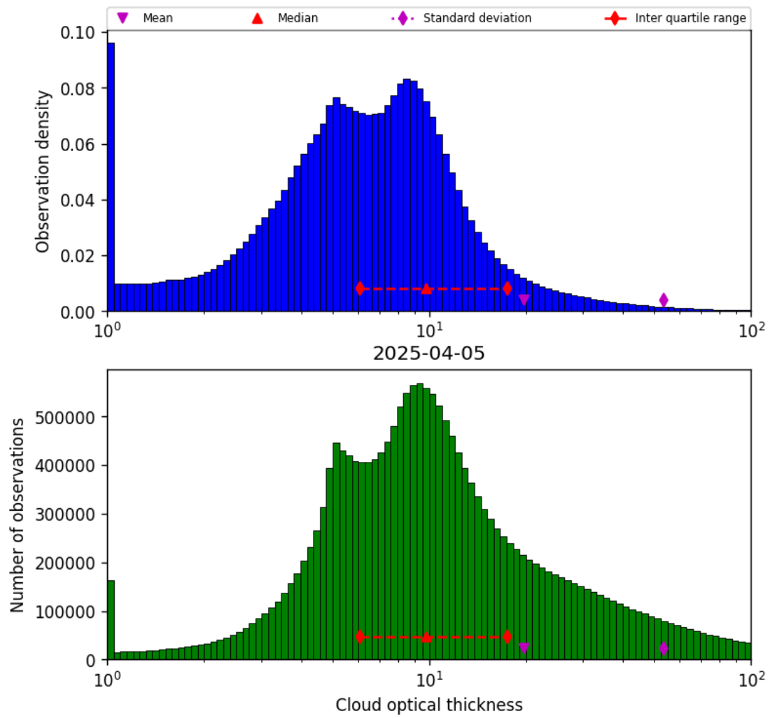
Figure 41: Histogram of “Cloud optical thickness” for 2025-04-04 to 2025-04-06
