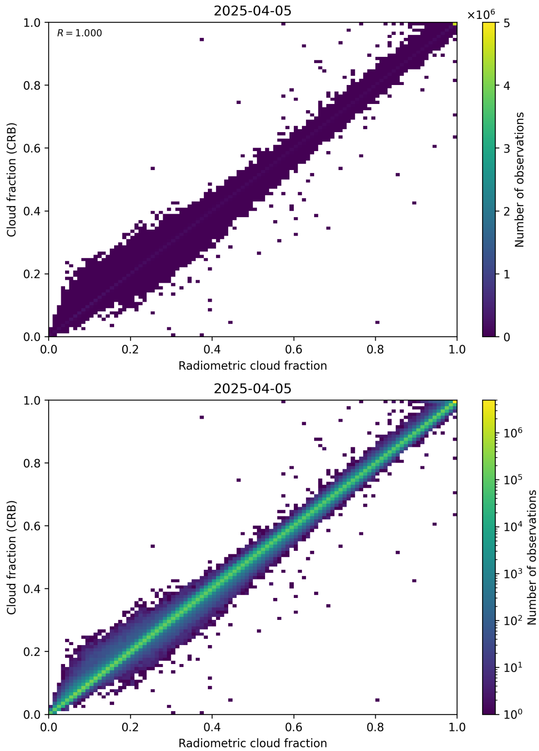
Figure 73: Scatter density plot of “Radiometric cloud fraction” against “Cloud fraction (CRB)” for 2025-04-04 to 2025-04-06.
