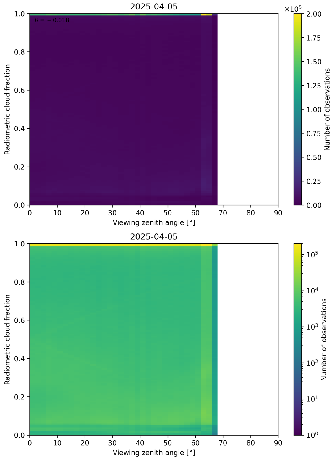
Figure 107: Scatter density plot of “Viewing zenith angle” against “Radiometric cloud fraction” for 2025-04-04 to 2025-04-06.
