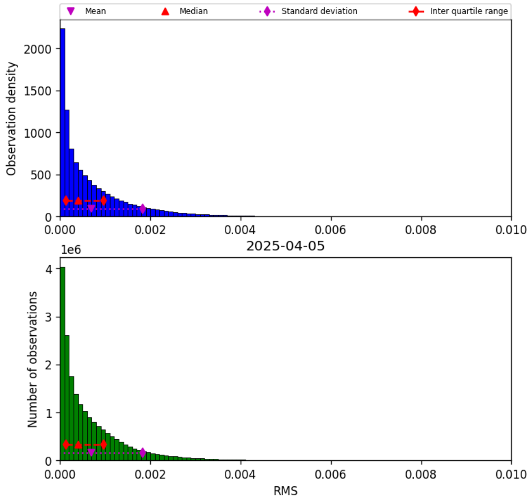
Figure 47: Histogram of “RMS” for 2025-04-04 to 2025-04-06
