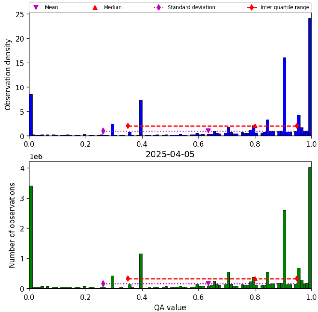
Figure 38: Histogram of “QA value” for 2025-04-04 to 2025-04-06
