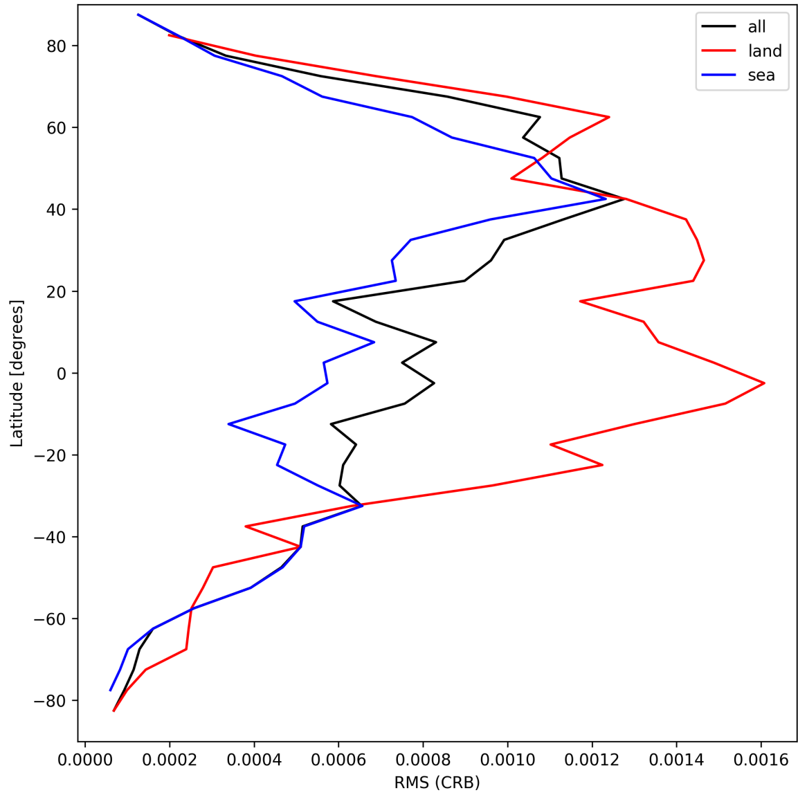
Figure 32: Zonal average of “RMS (CRB)” for 2025-04-04 to 2025-04-06.
