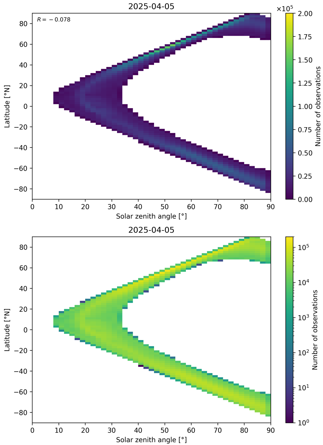
Figure 105: Scatter density plot of “Solar zenith angle” against “Latitude” for 2025-04-04 to 2025-04-06.
