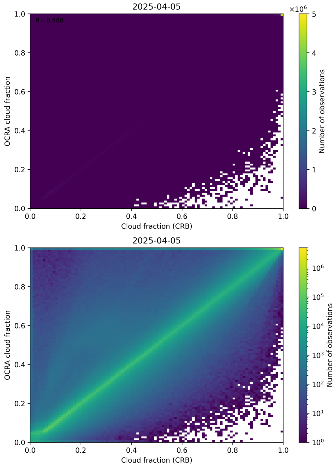
Figure 78: Scatter density plot of “Cloud fraction (CRB)” against “OCRA cloud fraction” for 2025-04-04 to 2025-04-06.
