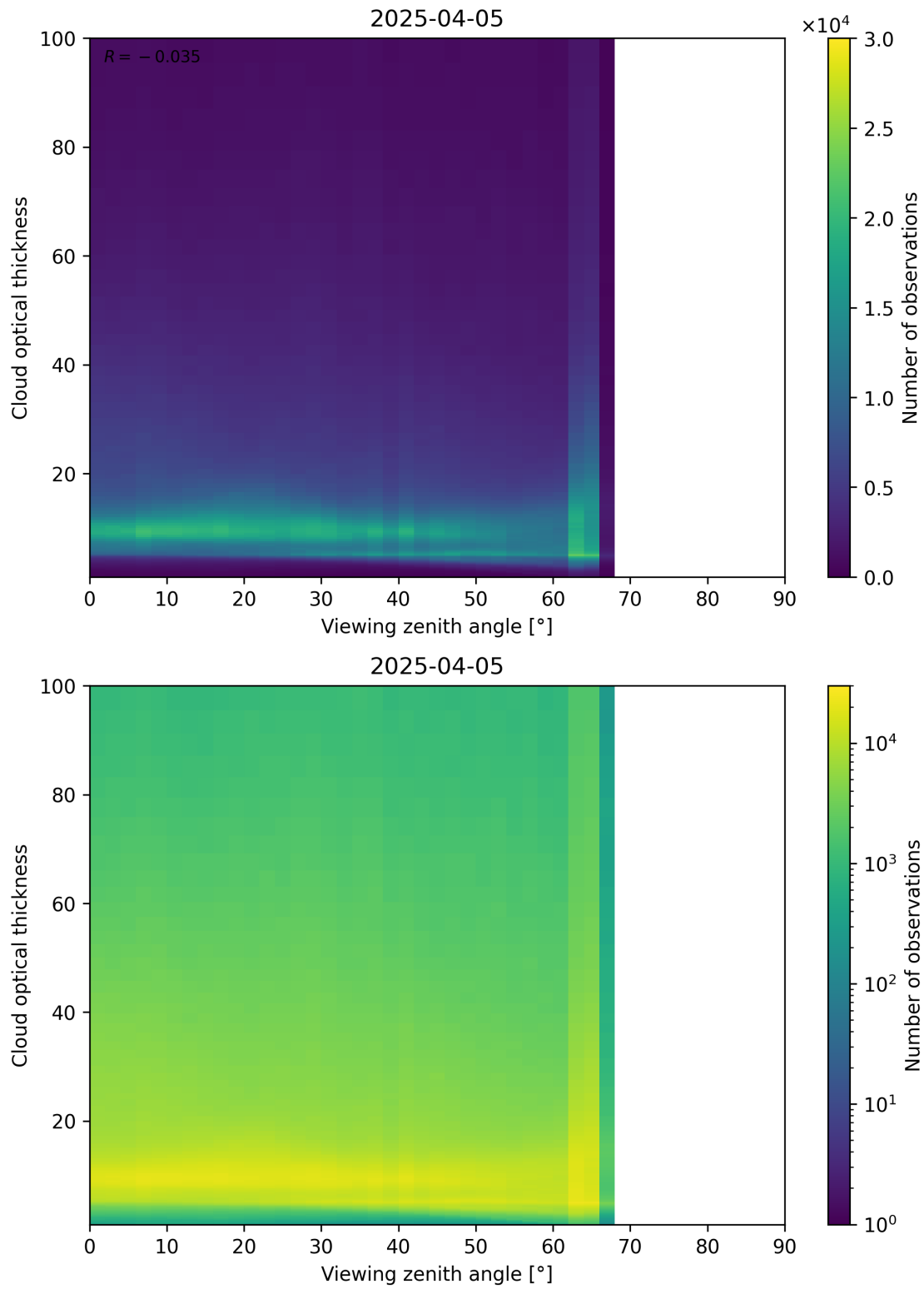
Figure 111: Scatter density plot of “Viewing zenith angle” against “Cloud optical thickness” for 2025-04-04 to 2025-04-06.
