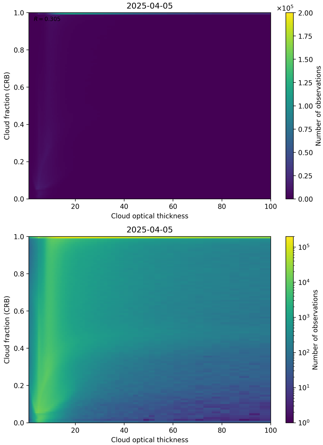
Figure 84: Scatter density plot of “Cloud optical thickness” against “Cloud fraction (CRB)” for 2025-04-04 to 2025-04-06.
