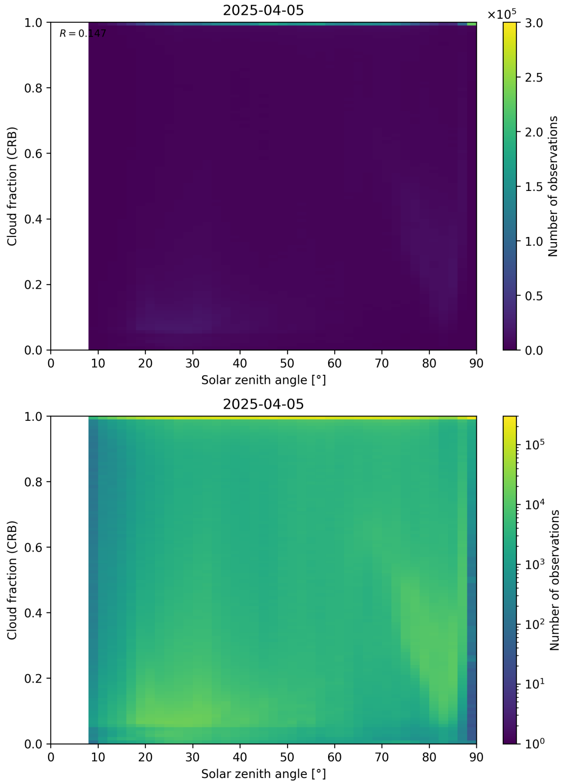
Figure 101: Scatter density plot of “Solar zenith angle” against “Cloud fraction (CRB)” for 2025-04-04 to 2025-04-06.
