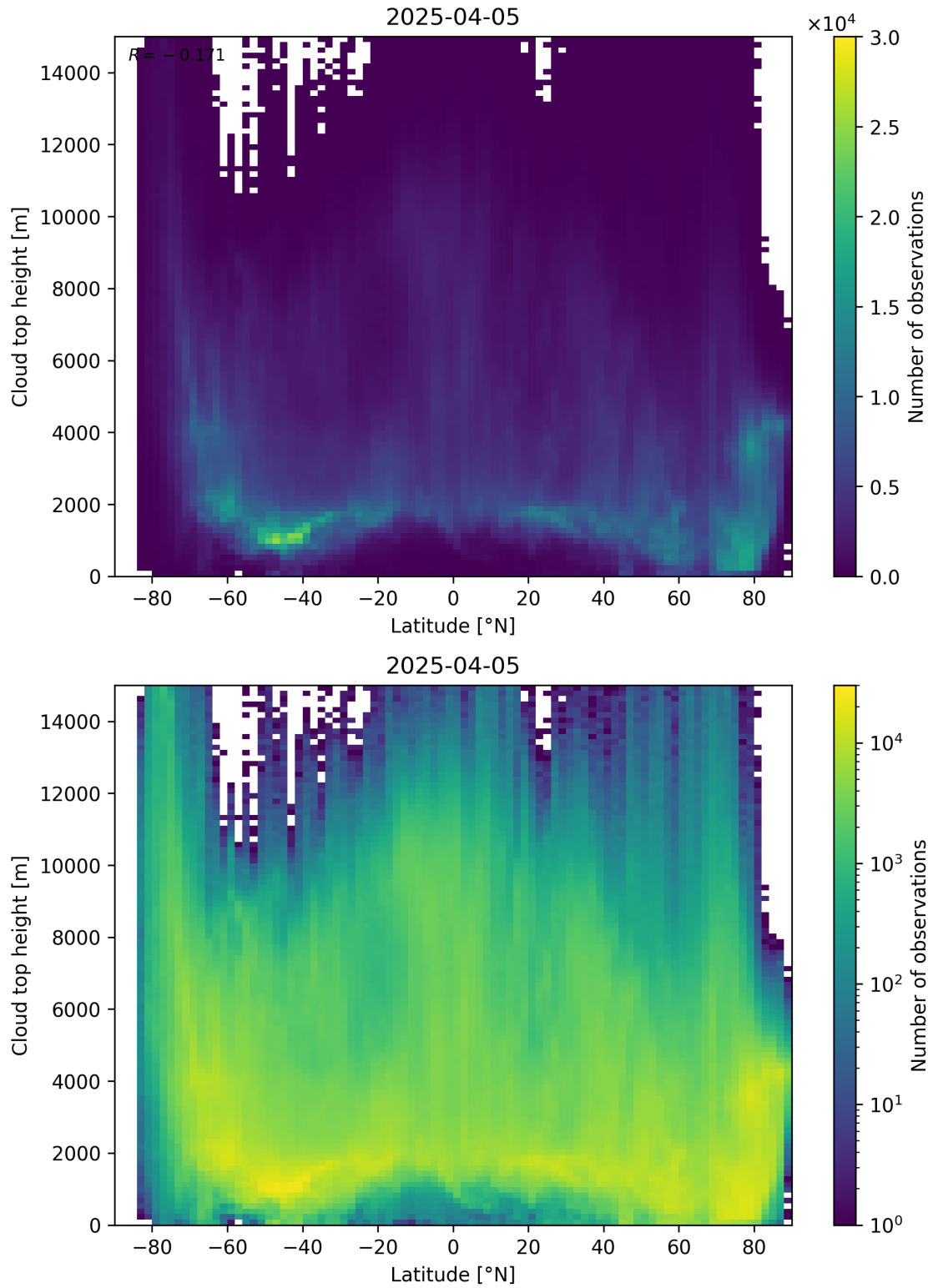
Figure 97: Scatter density plot of “Latitude” against “Cloud top height” for 2025-04-04 to 2025-04-06.
