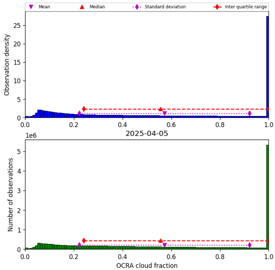
Figure 50: Histogram of “OCRA cloud fraction” for 2025-04-04 to 2025-04-06
