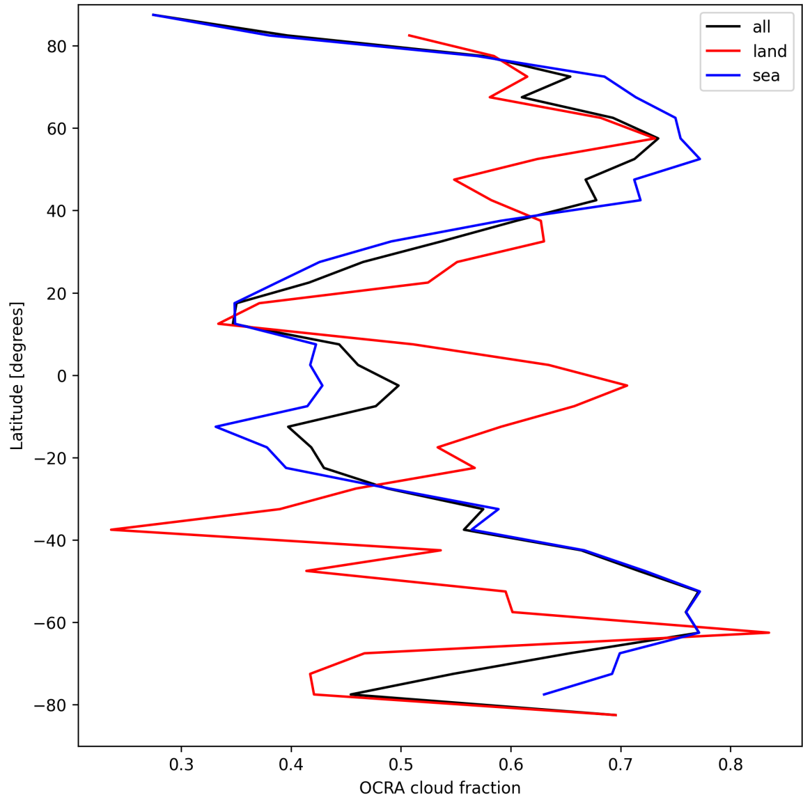
Figure 34: Zonal average of “OCRA cloud fraction” for 2025-04-04 to 2025-04-06.
