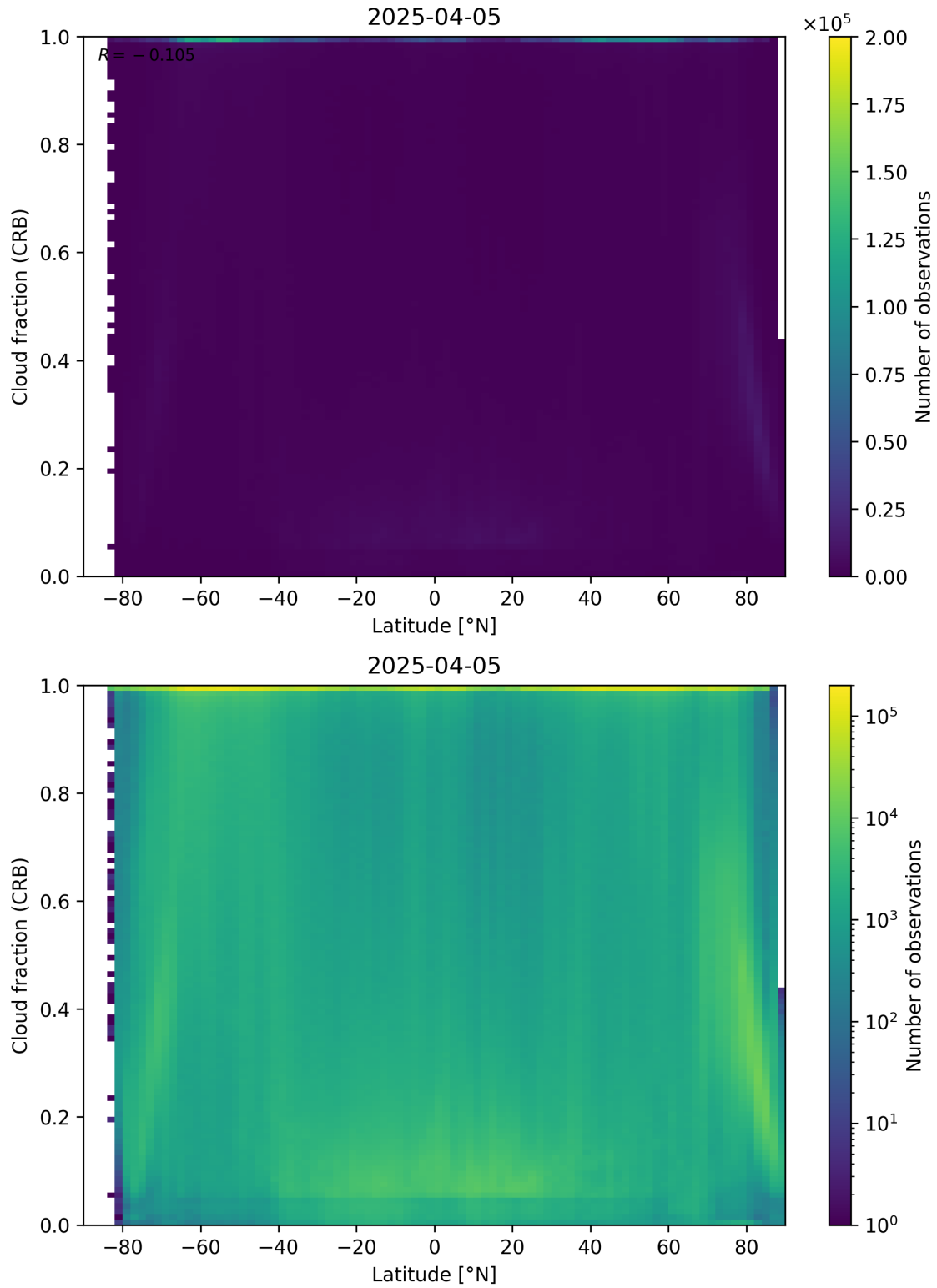
Figure 94: Scatter density plot of “Latitude” against “Cloud fraction (CRB)” for 2025-04-04 to 2025-04-06.
