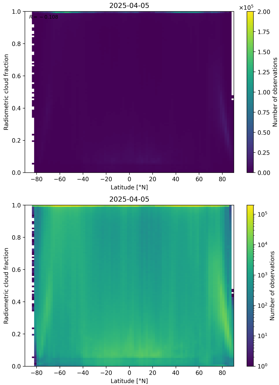
Figure 92: Scatter density plot of “Latitude” against “Radiometric cloud fraction” for 2025-04-04 to 2025-04-06.
