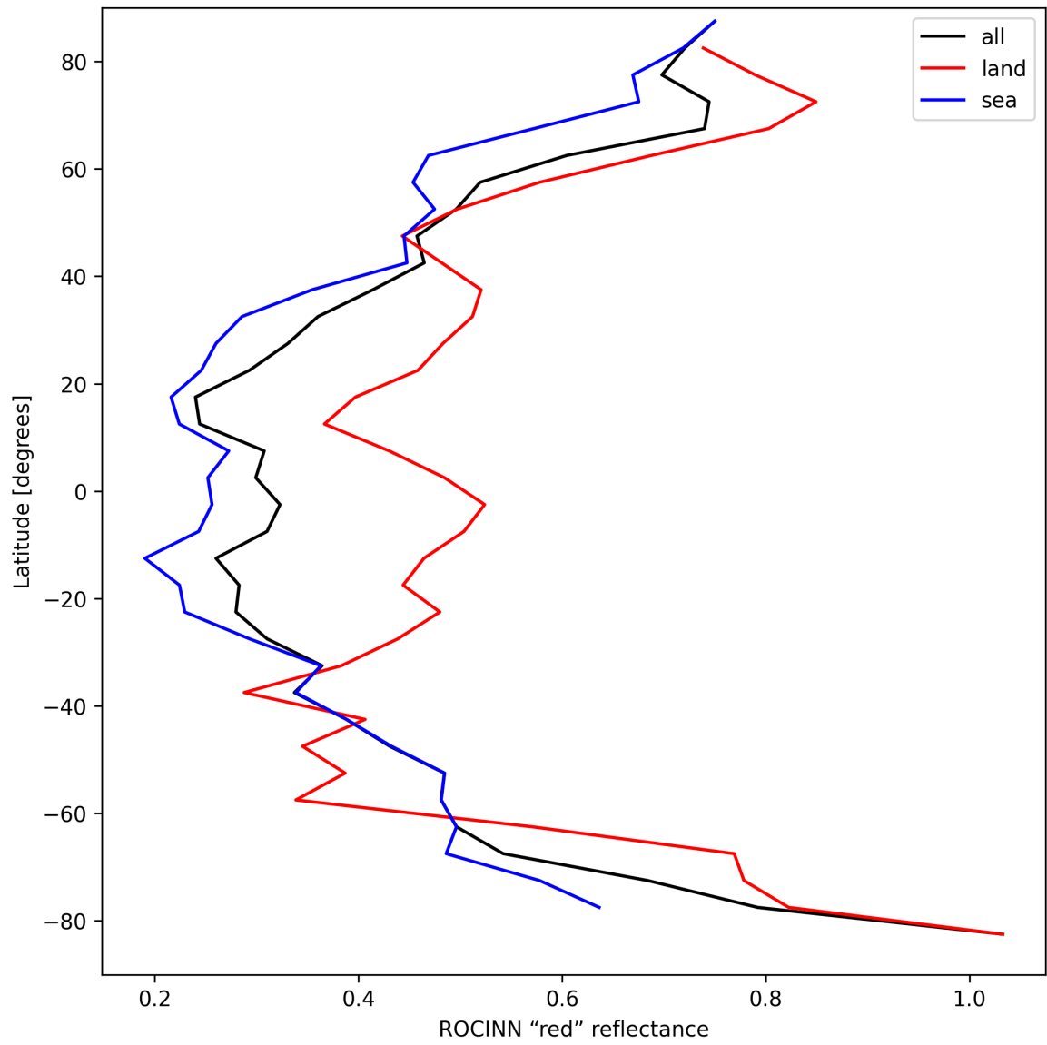
Figure 37: Zonal average of "ROCINN "red" reflectance" for 2025-04-04 to 2025-04-06.
