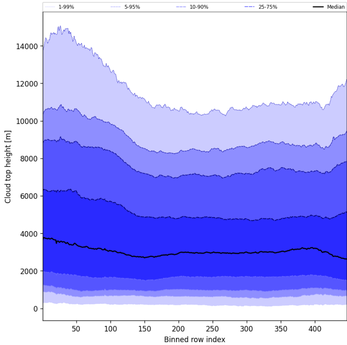
Figure 56: Along track statistics of “Cloud top height” for 2025-04-04 to 2025-04-06
