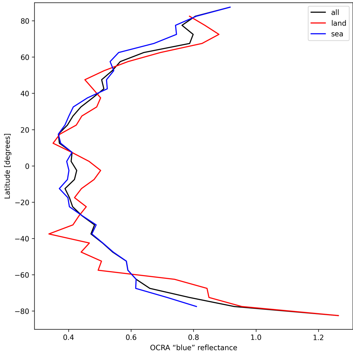
Figure 35: Zonal average of "OCRA "blue" reflectance" for 2025-04-04 to 2025-04-06.
