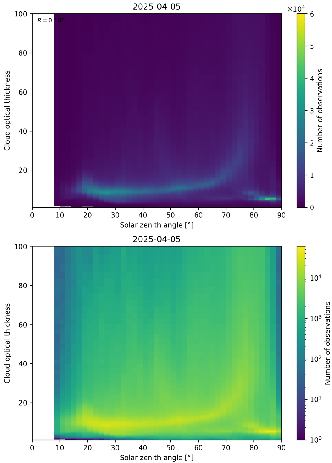
Figure 103: Scatter density plot of “Solar zenith angle” against “Cloud optical thickness” for 2025-04-04 to 2025-04-06.
