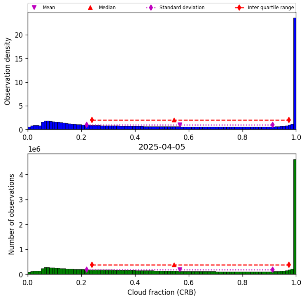
Figure 42: Histogram of “Cloud fraction (CRB)” for 2025-04-04 to 2025-04-06
