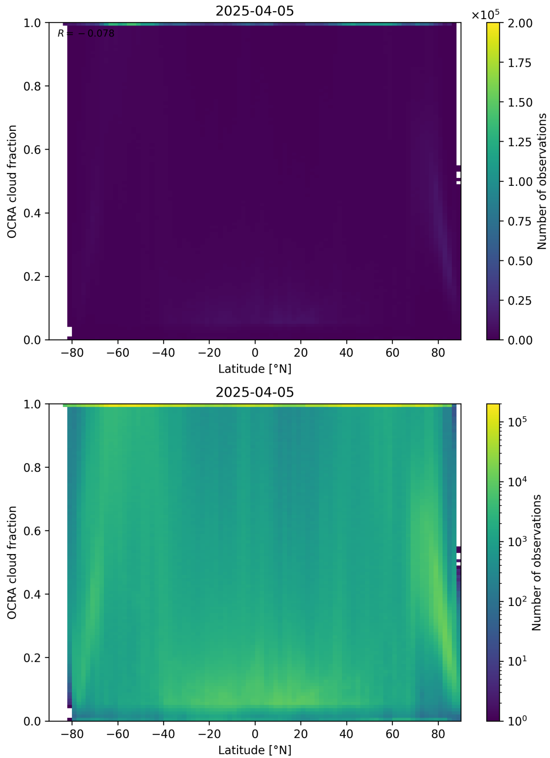
Figure 93: Scatter density plot of “Latitude” against “OCRA cloud fraction” for 2025-04-04 to 2025-04-06.
