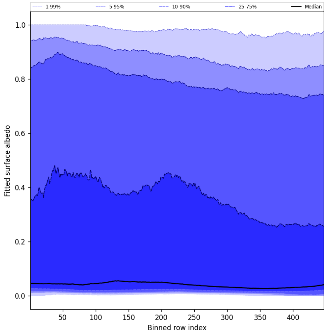
Figure 61: Along track statistics of “Fitted surface albedo” for 2025-04-04 to 2025-04-06
