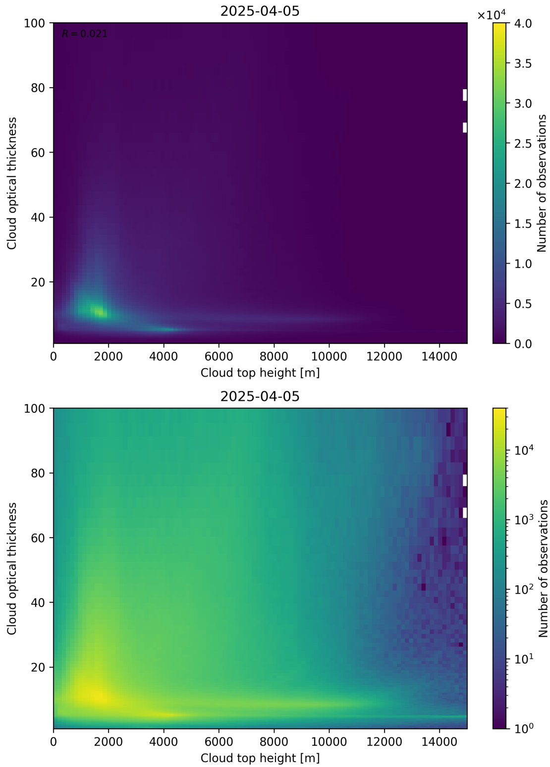
Figure 90: Scatter density plot of “Cloud top height” against “Cloud optical thickness” for 2025-04-04 to 2025-04-06.
