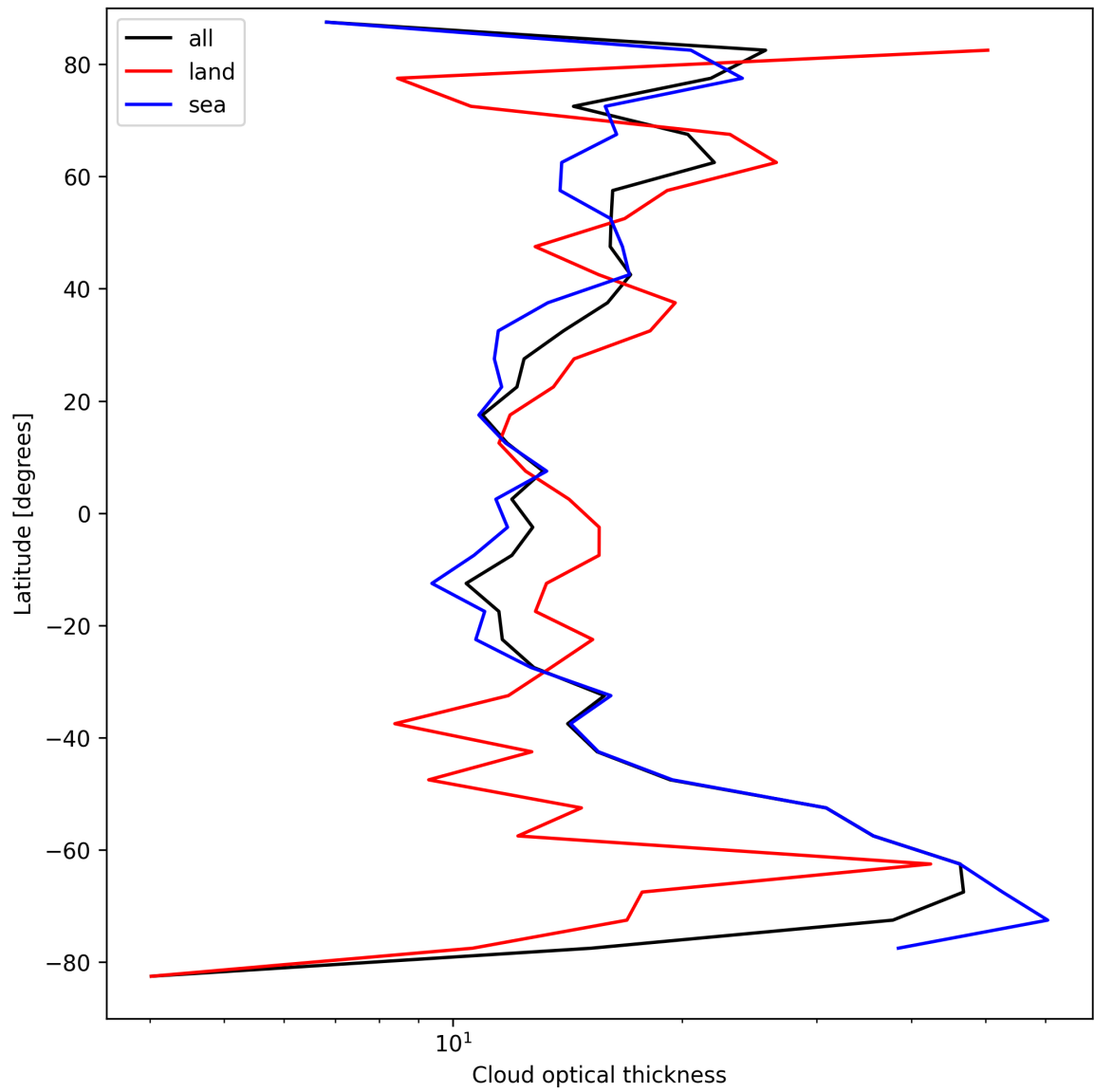
Figure 25: Zonal average of “Cloud optical thickness” for 2025-04-04 to 2025-04-06.
