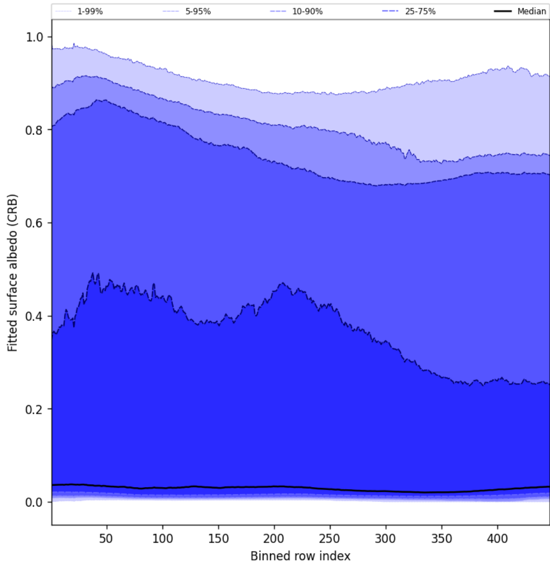
Figure 62: Along track statistics of “Fitted surface albedo (CRB)” for 2025-04-04 to 2025-04-06
