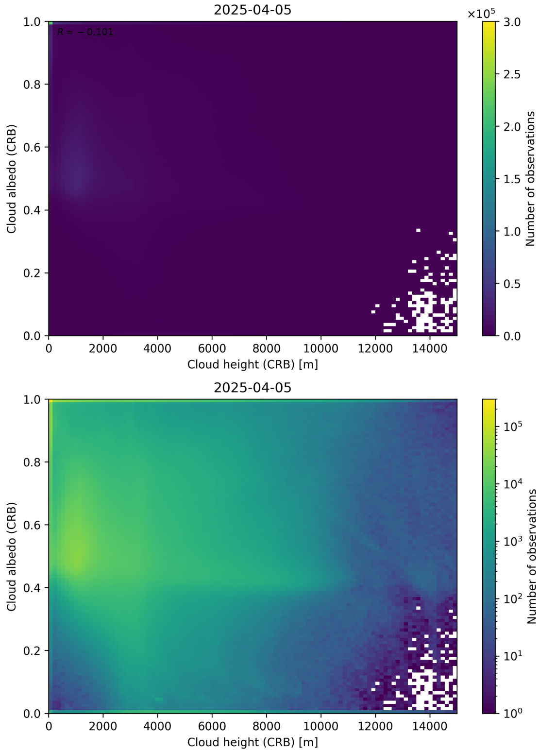
Figure 80: Scatter density plot of “Cloud height (CRB)” against “Cloud albedo (CRB)” for 2025-04-04 to 2025-04-06.
