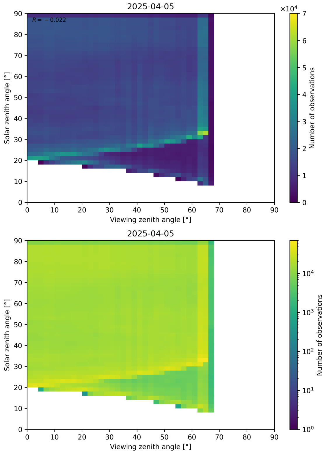
Figure 114: Scatter density plot of “Viewing zenith angle” against “Solar zenith angle” for 2025-04-04 to 2025-04-06.
