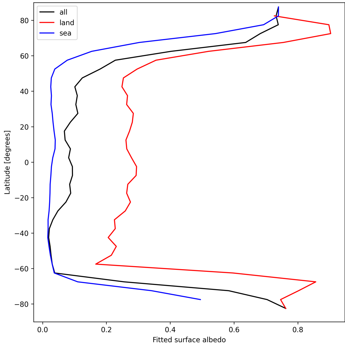
Figure 29: Zonal average of “Fitted surface albedo” for 2025-04-04 to 2025-04-06.
