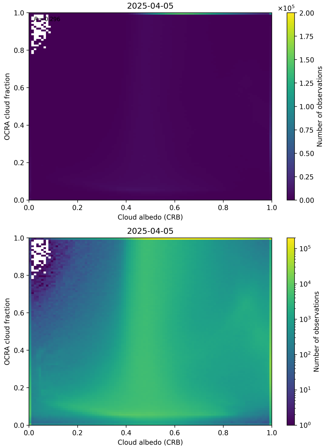
Figure 70: Scatter density plot of “Cloud albedo (CRB)” against “OCRA cloud fraction” for 2025-04-04 to 2025-04-06.
