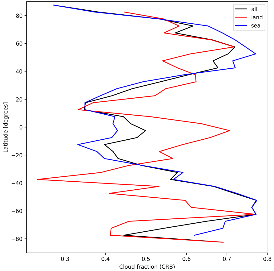
Figure 26: Zonal average of “Cloud fraction (CRB)” for 2025-04-04 to 2025-04-06.
