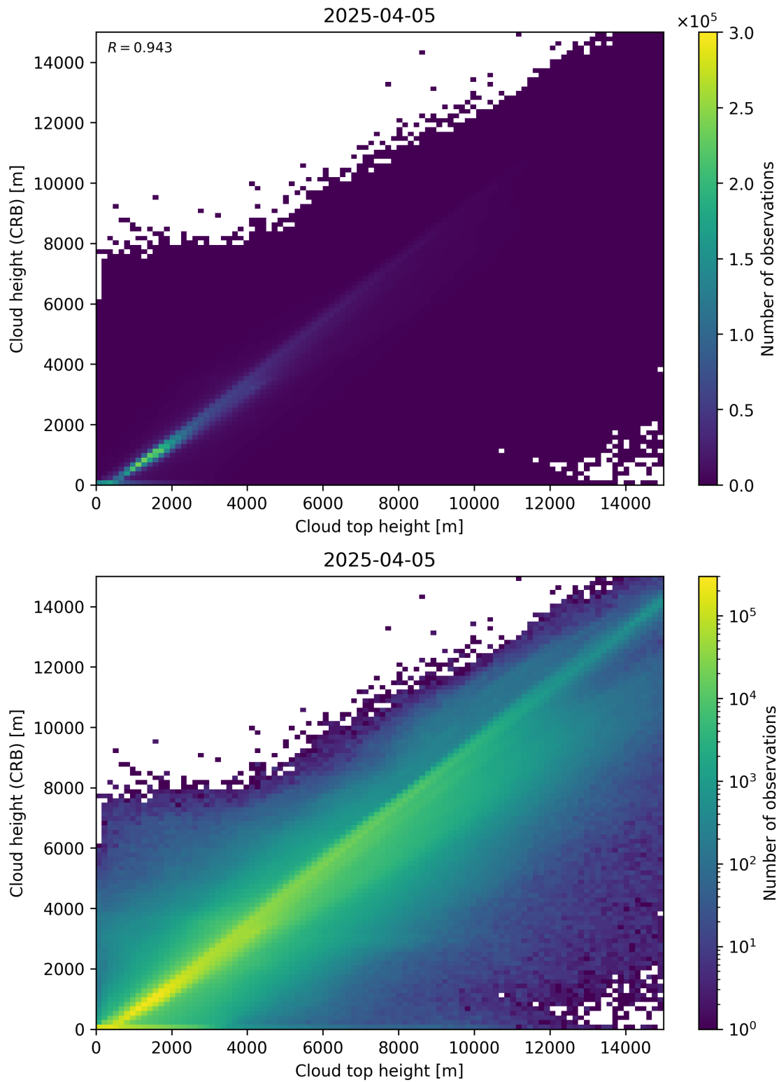
Figure 89: Scatter density plot of “Cloud top height” against “Cloud height (CRB)” for 2025-04-04 to 2025-04-06.
