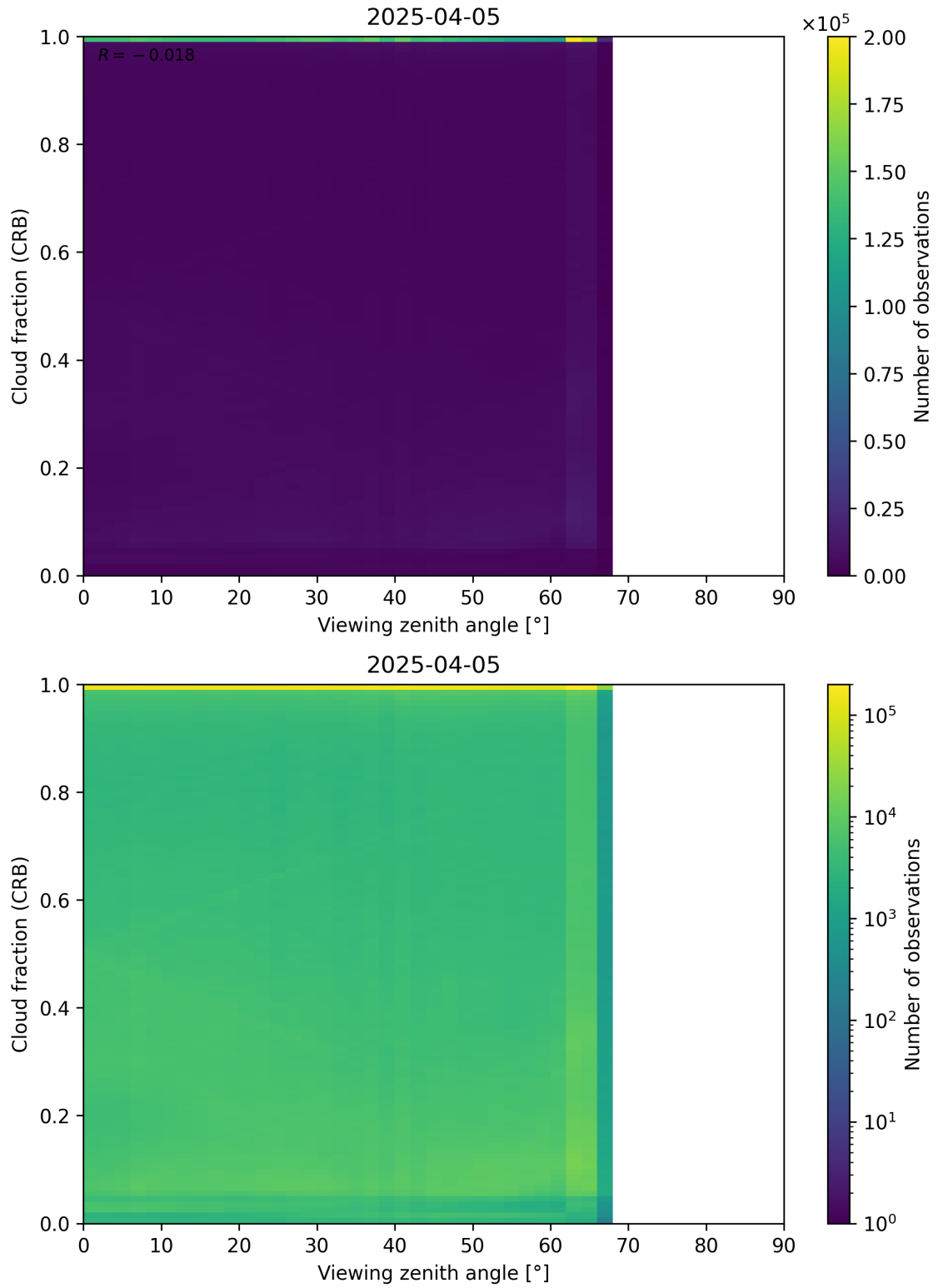
Figure 109: Scatter density plot of “Viewing zenith angle” against “Cloud fraction (CRB)” for 2025-04-04 to 2025-04-06.
