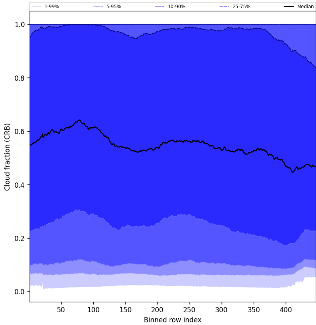
Figure 58: Along track statistics of “Cloud fraction (CRB)” for 2025-04-04 to 2025-04-06
