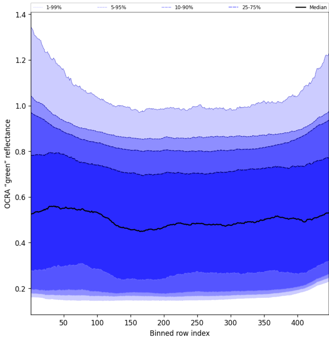
Figure 68: Along track statistics of “OCRA “green” reflectance” for 2025-04-04 to 2025-04-06
