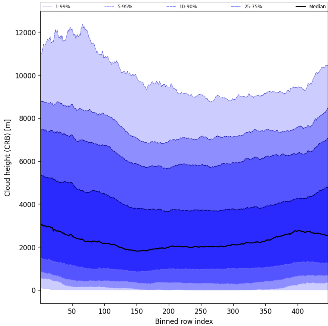
Figure 59: Along track statistics of “Cloud height (CRB)” for 2025-04-04 to 2025-04-06
