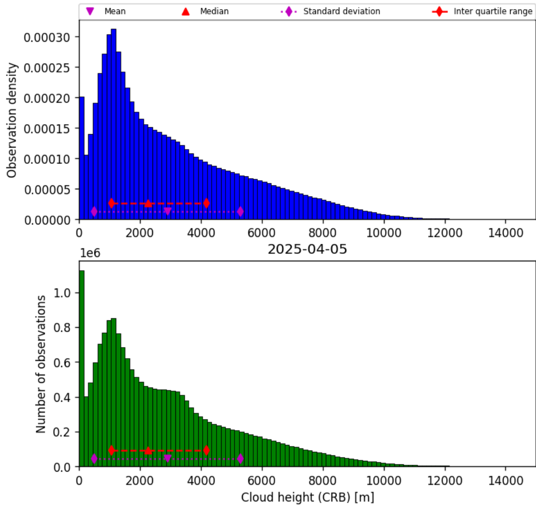
Figure 43: Histogram of “Cloud height (CRB)” for 2025-04-04 to 2025-04-06
