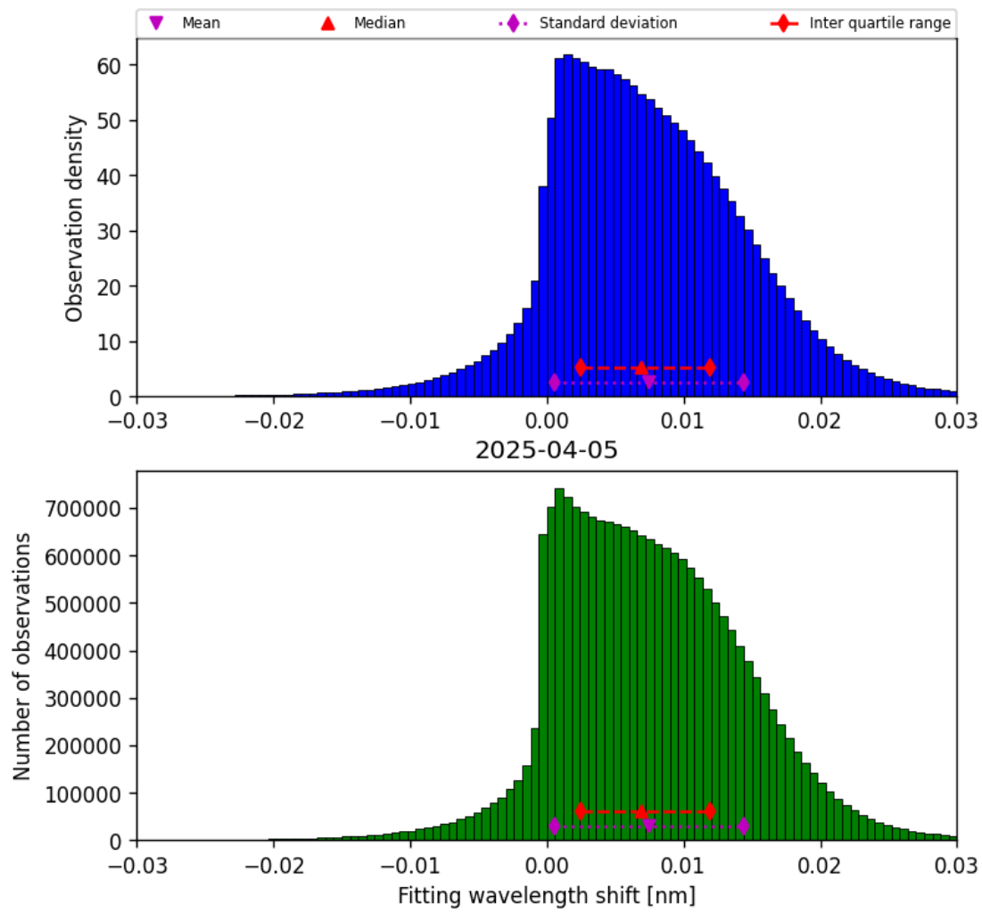
Figure 49: Histogram of “Fitting wavelength shift” for 2025-04-04 to 2025-04-06
