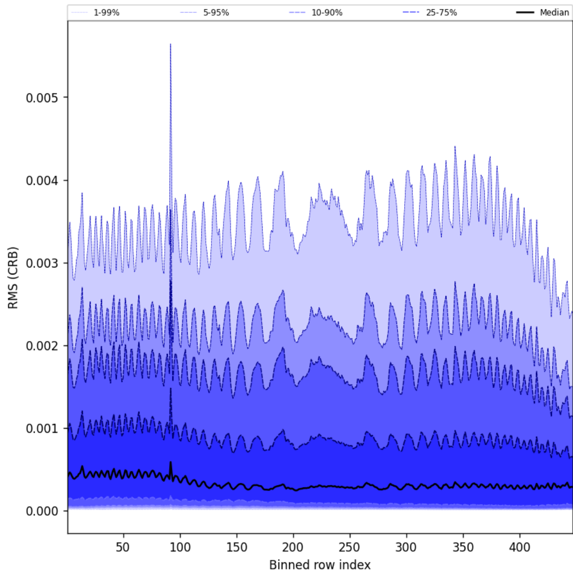
Figure 64: Along track statistics of “RMS (CRB)” for 2025-04-04 to 2025-04-06
