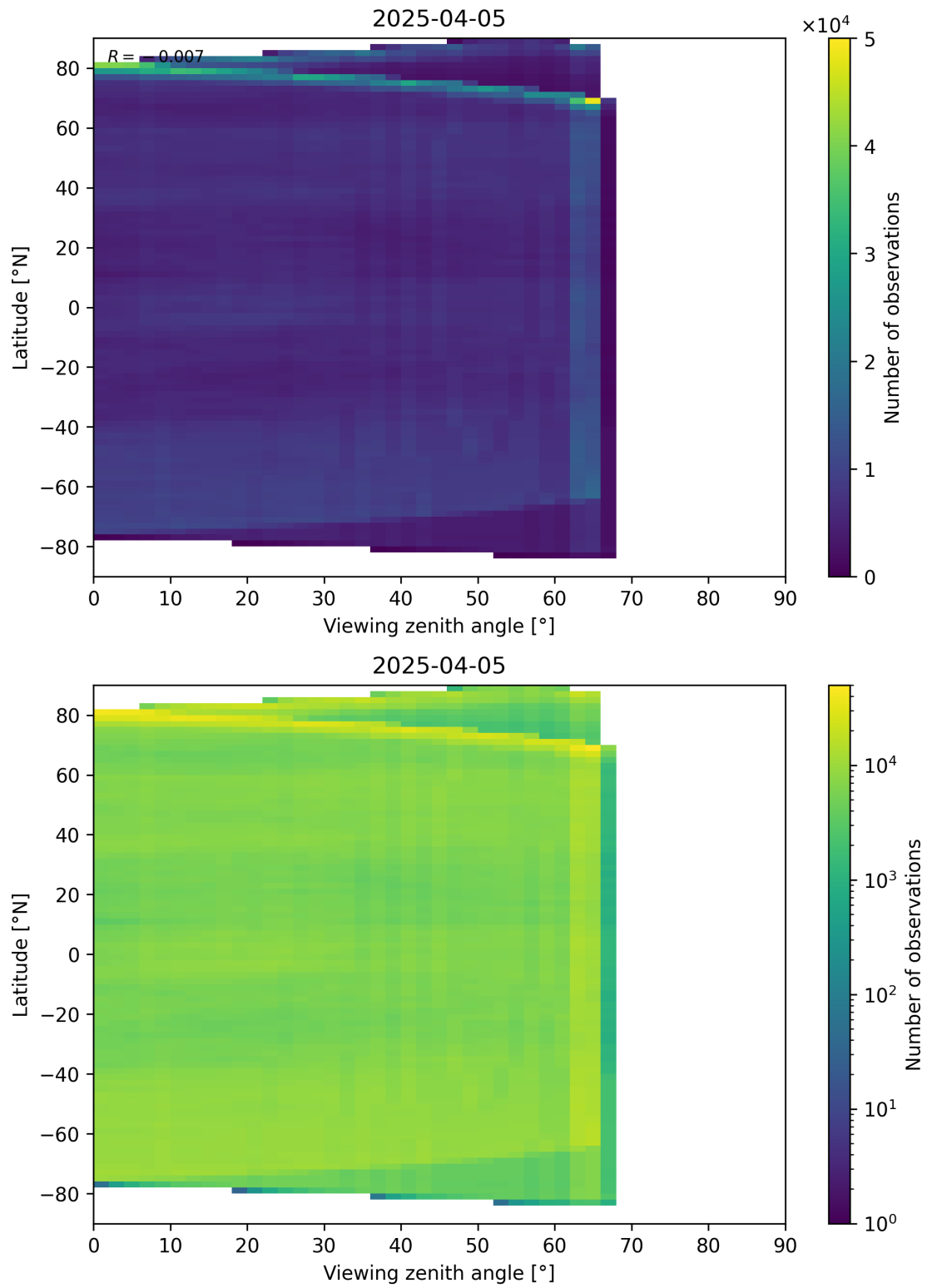
Figure 113: Scatter density plot of “Viewing zenith angle” against “Latitude” for 2025-04-04 to 2025-04-06.
