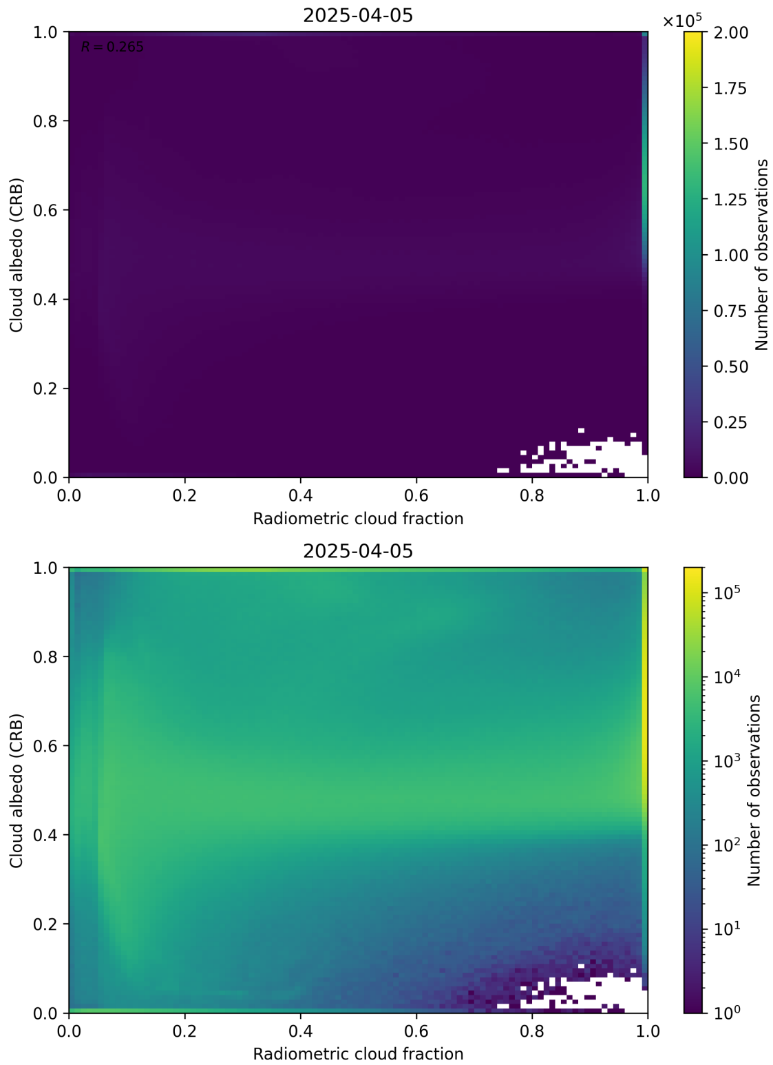
Figure 71: Scatter density plot of “Radiometric cloud fraction” against “Cloud albedo (CRB)” for 2025-04-04 to 2025-04-06.
