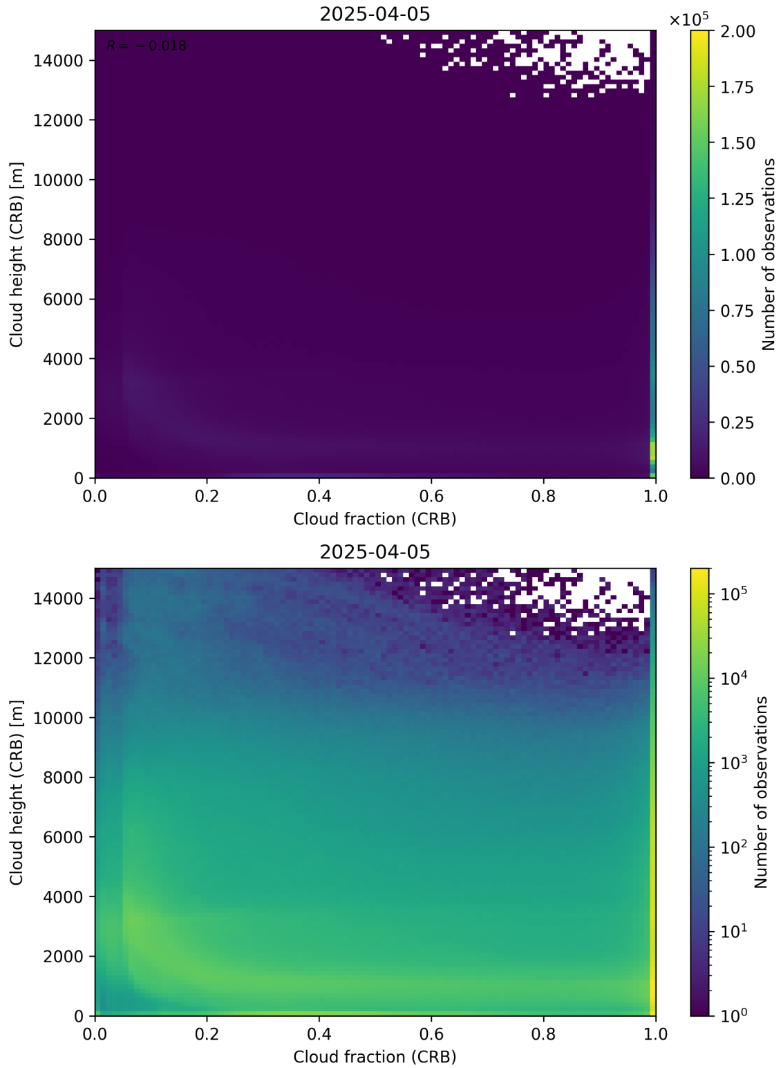
Figure 79: Scatter density plot of “Cloud fraction (CRB)” against “Cloud height (CRB)” for 2025-04-04 to 2025-04-06.
