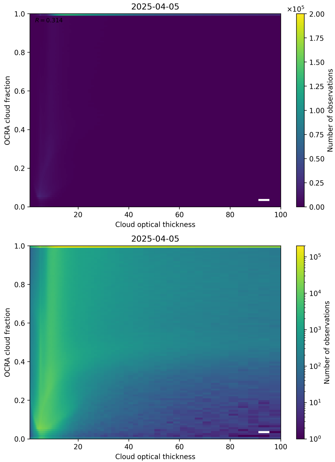
Figure 83: Scatter density plot of “Cloud optical thickness” against “OCRA cloud fraction” for 2025-04-04 to 2025-04-06.
