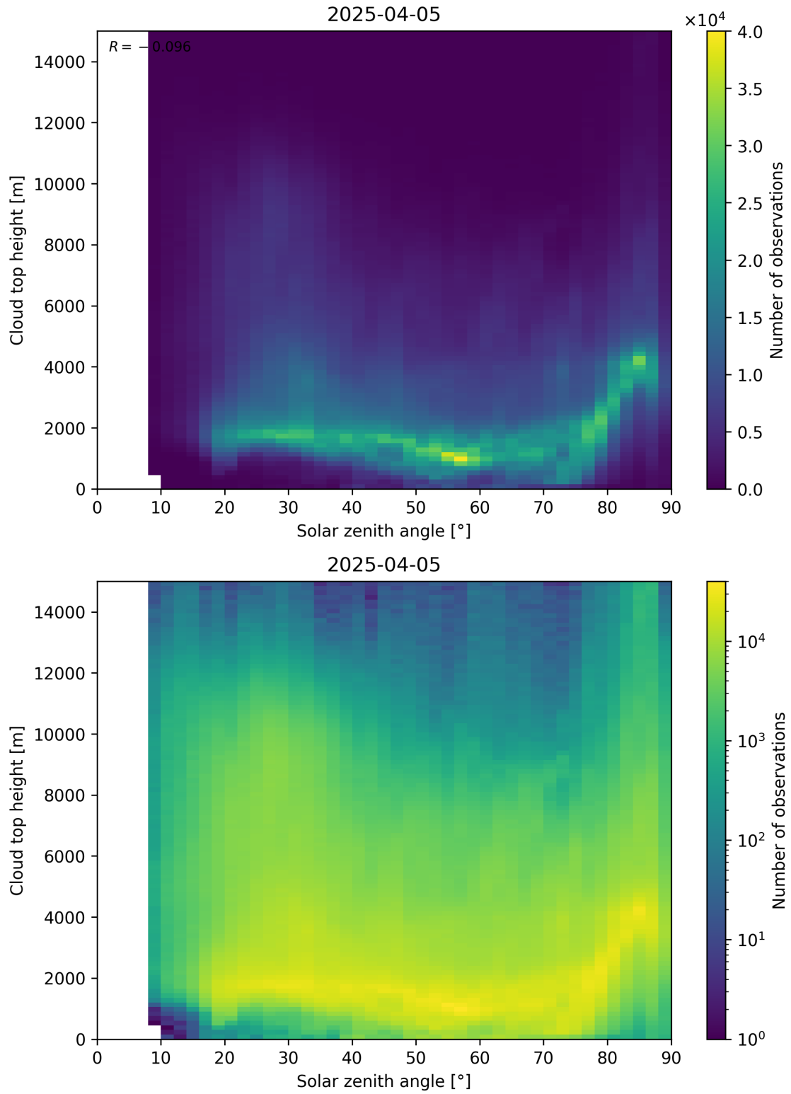
Figure 104: Scatter density plot of “Solar zenith angle” against “Cloud top height” for 2025-04-04 to 2025-04-06.
