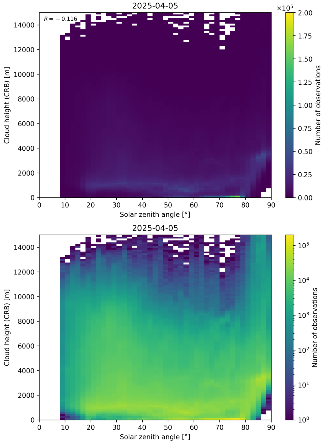
Figure 102: Scatter density plot of “Solar zenith angle” against “Cloud height (CRB)” for 2025-04-04 to 2025-04-06.
