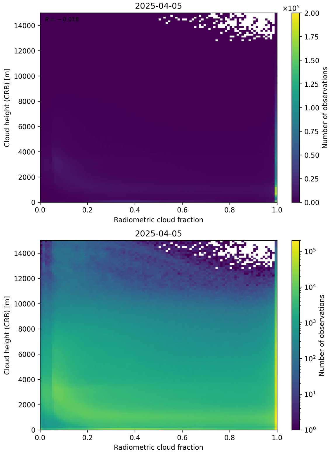
Figure 74: Scatter density plot of “Radiometric cloud fraction” against “Cloud height (CRB)” for 2025-04-04 to 2025-04-06.
