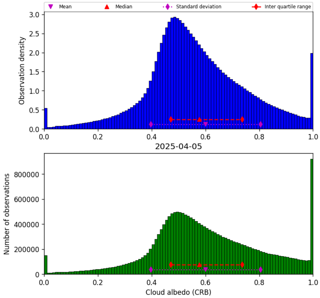
Figure 44: Histogram of “Cloud albedo (CRB)” for 2025-04-04 to 2025-04-06
