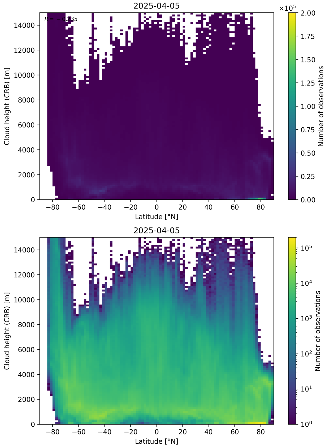
Figure 95: Scatter density plot of “Latitude” against “Cloud height (CRB)” for 2025-04-04 to 2025-04-06.
