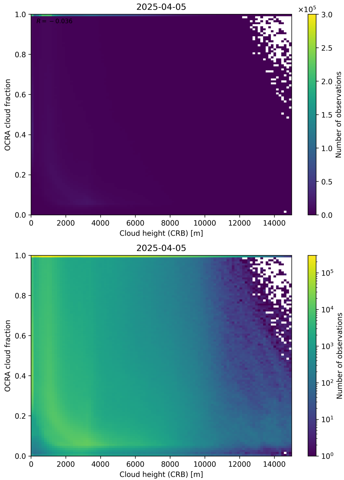
Figure 81: Scatter density plot of “Cloud height (CRB)” against “OCRA cloud fraction” for 2025-04-04 to 2025-04-06.
