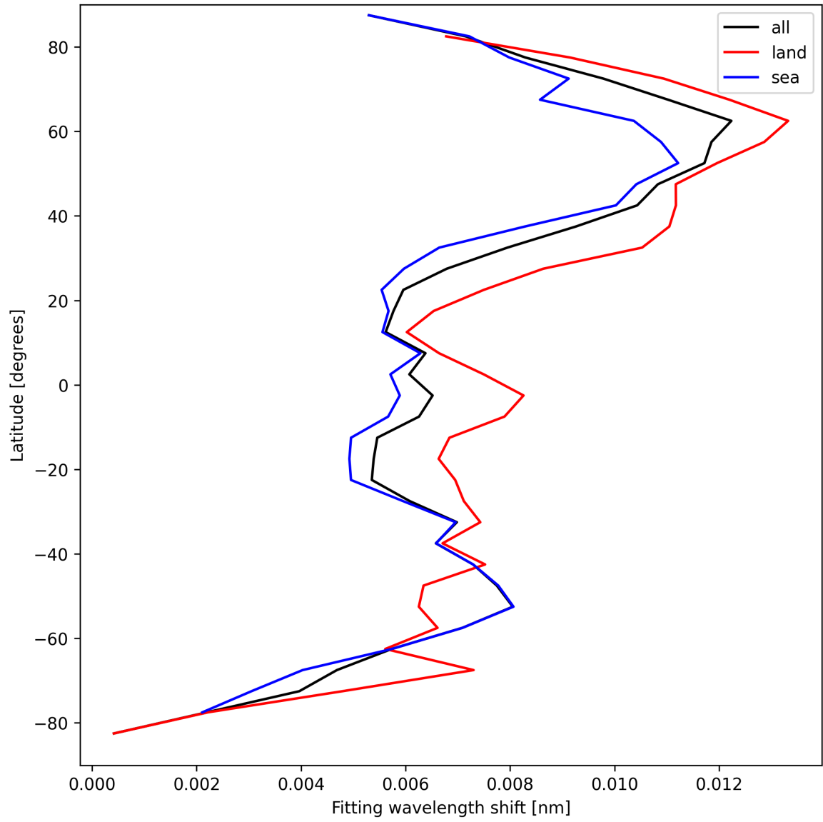
Figure 33: Zonal average of “Fitting wavelength shift” for 2025-04-04 to 2025-04-06.
