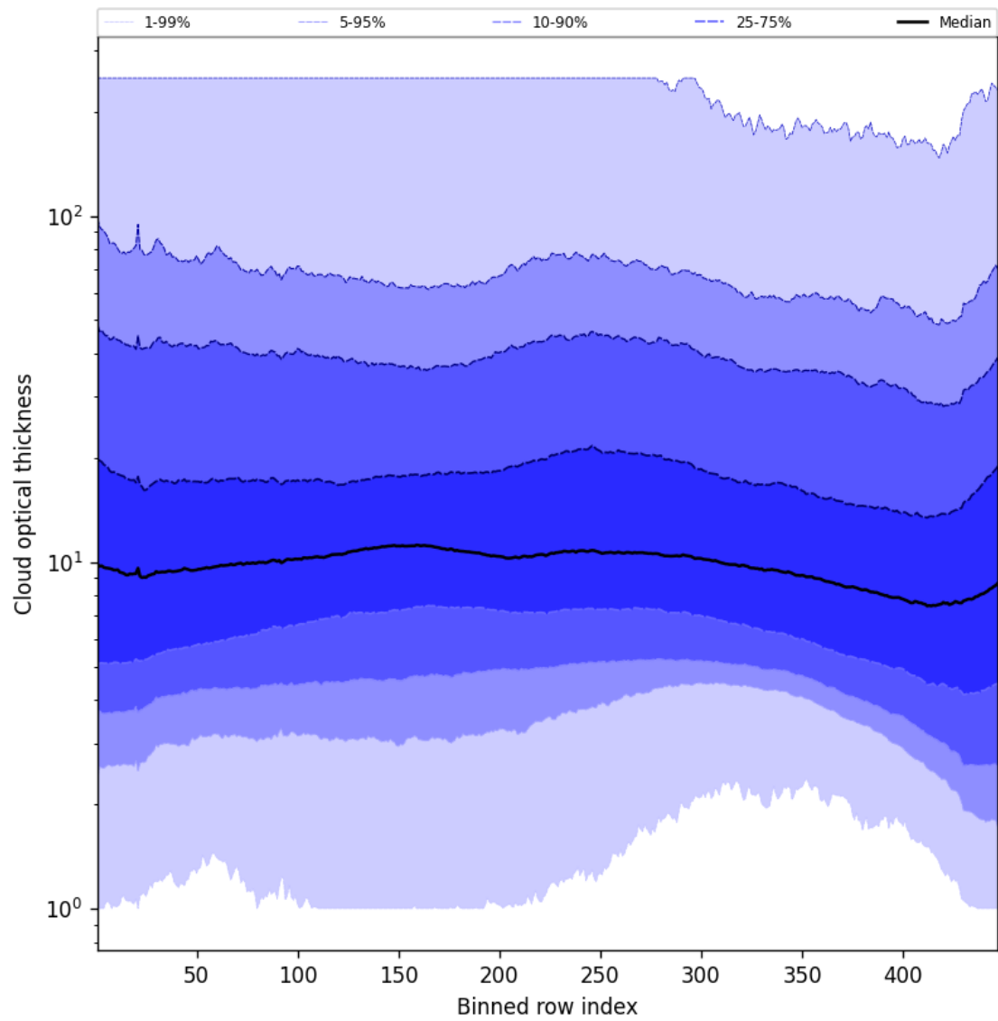
Figure 57: Along track statistics of “Cloud optical thickness” for 2025-04-05 to 2025-04-07
