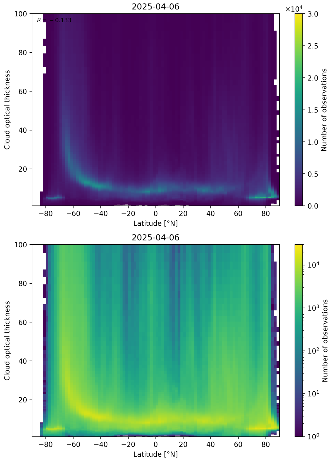
Figure 96: Scatter density plot of “Latitude” against “Cloud optical thickness” for 2025-04-05 to 2025-04-07.
