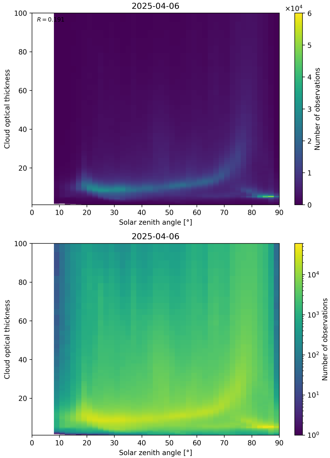
Figure 103: Scatter density plot of “Solar zenith angle” against “Cloud optical thickness” for 2025-04-05 to 2025-04-07.
