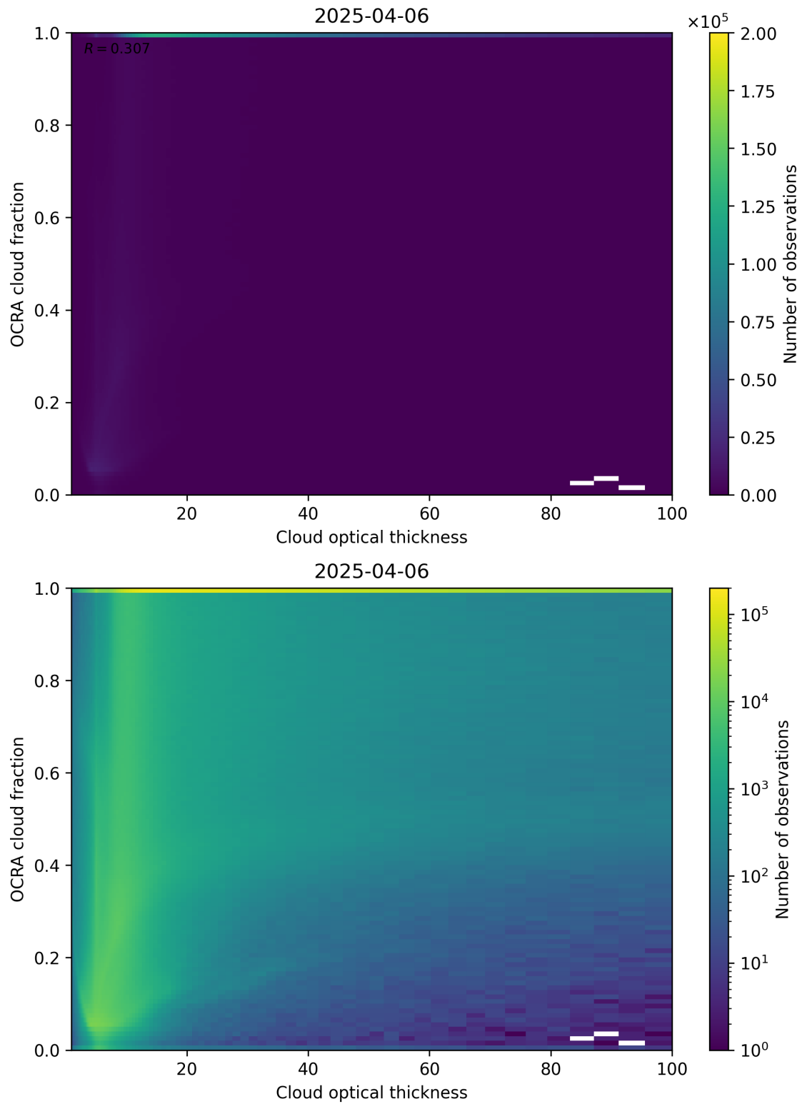
Figure 83: Scatter density plot of “Cloud optical thickness” against “OCRA cloud fraction” for 2025-04-05 to 2025-04-07.
