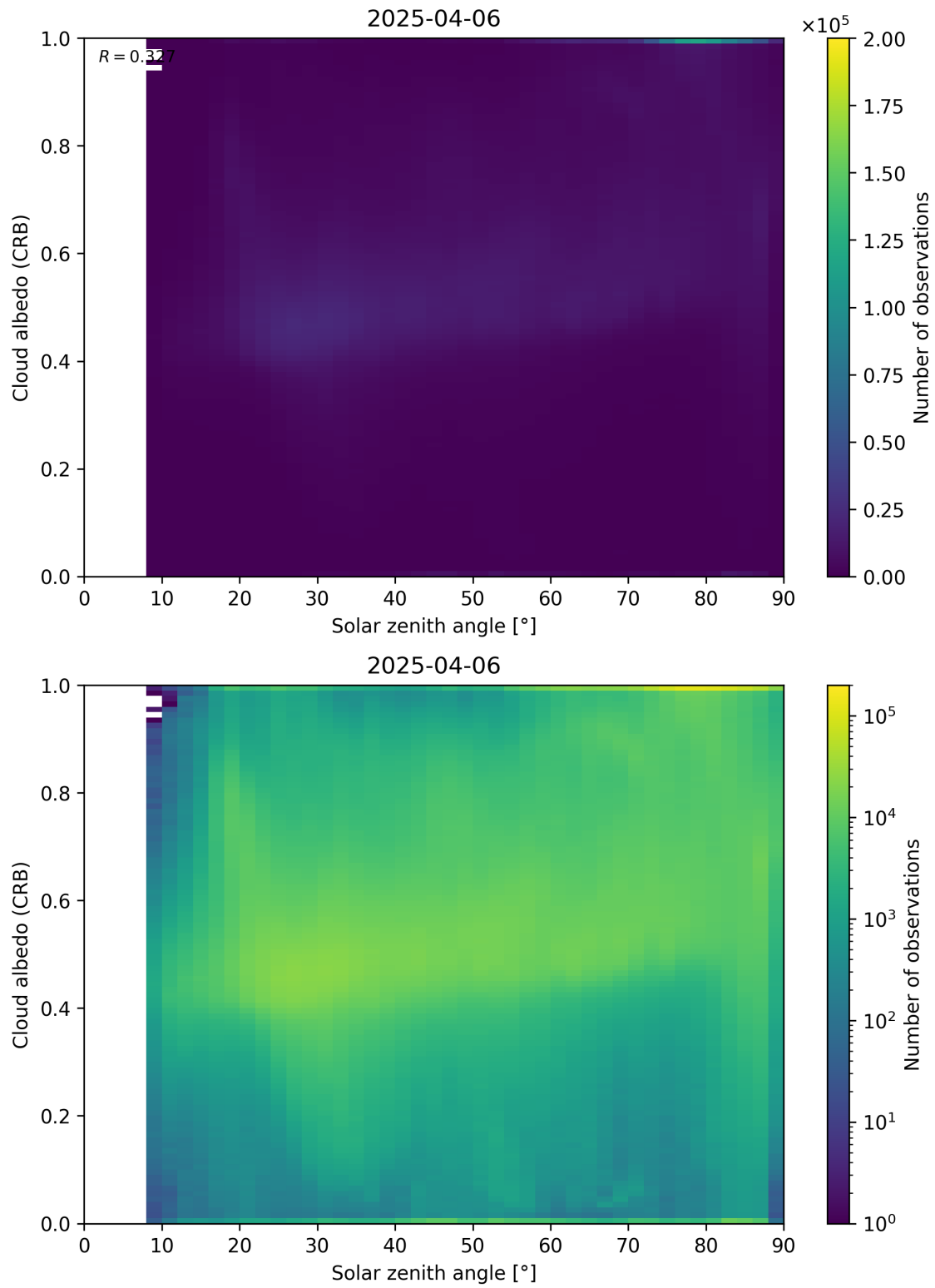
Figure 98: Scatter density plot of “Solar zenith angle” against “Cloud albedo (CRB)” for 2025-04-05 to 2025-04-07.
