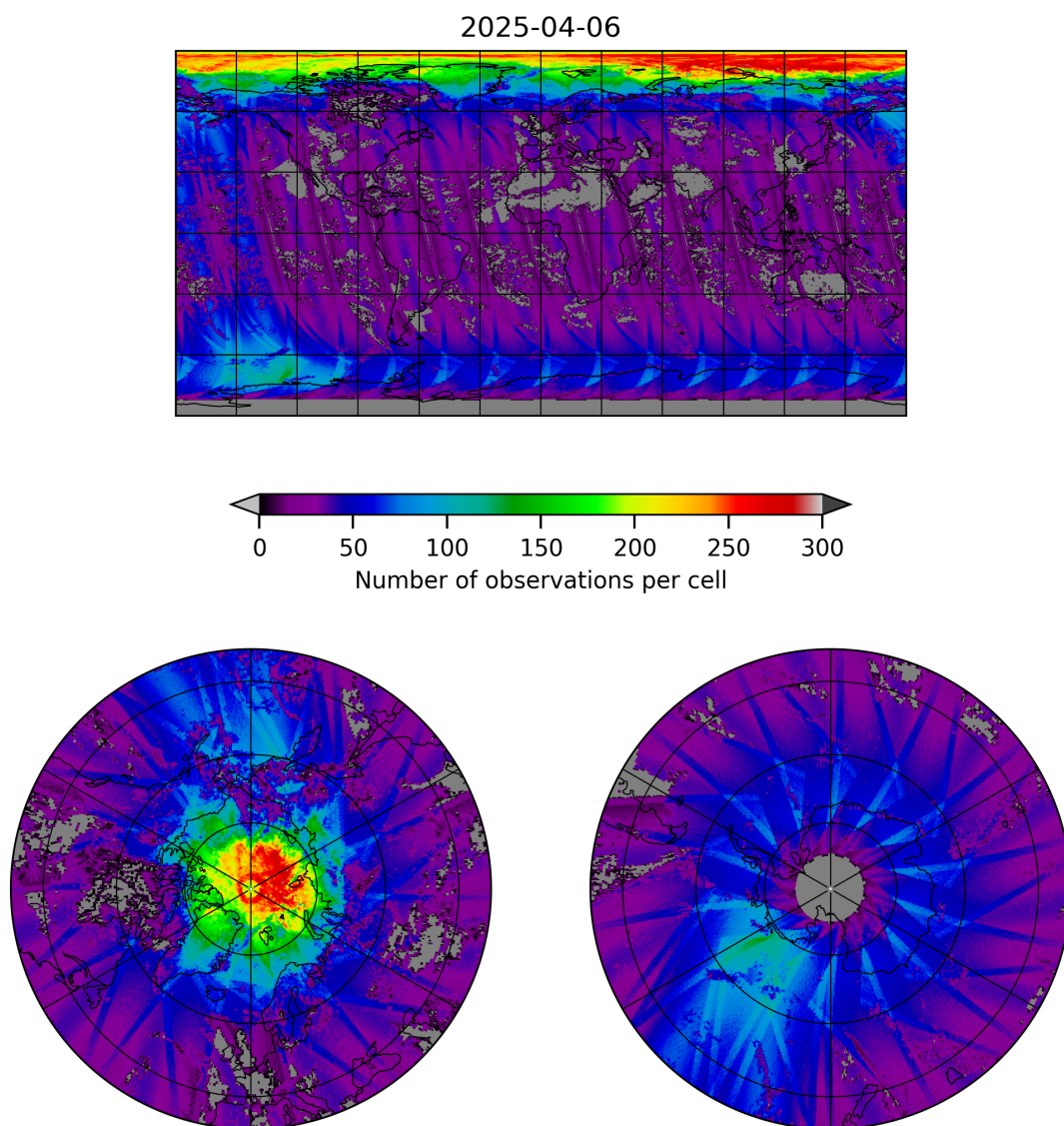
Figure 21: Map of the number of observations for 2025-04-05 to 2025-04-07
