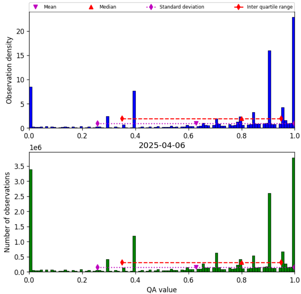
Figure 38: Histogram of “QA value” for 2025-04-05 to 2025-04-07
