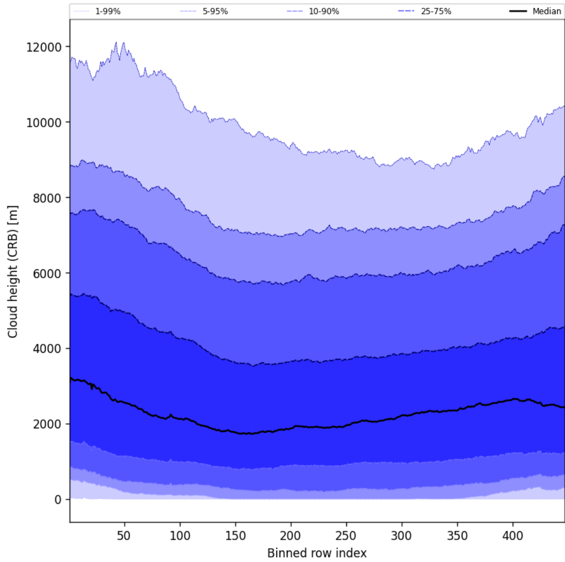
Figure 59: Along track statistics of “Cloud height (CRB)” for 2025-04-05 to 2025-04-07
