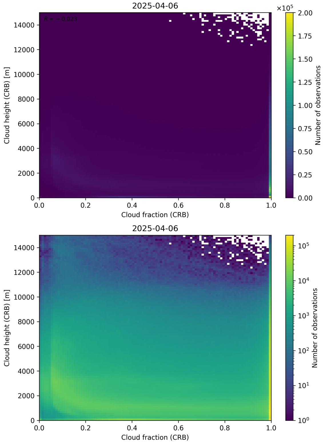
Figure 79: Scatter density plot of “Cloud fraction (CRB)” against “Cloud height (CRB)” for 2025-04-05 to 2025-04-07.
