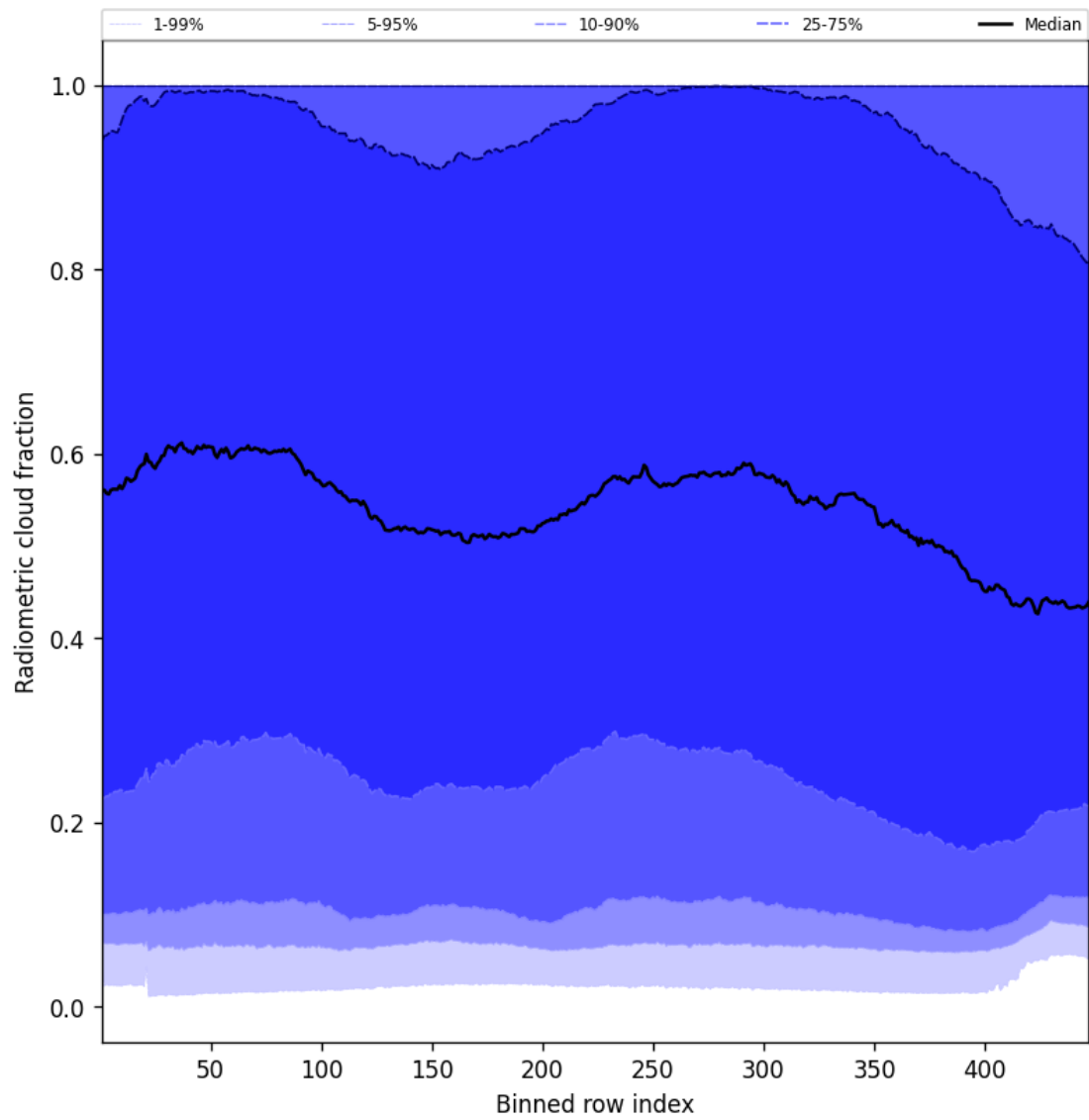
Figure 55: Along track statistics of “Radiometric cloud fraction” for 2025-04-05 to 2025-04-07
