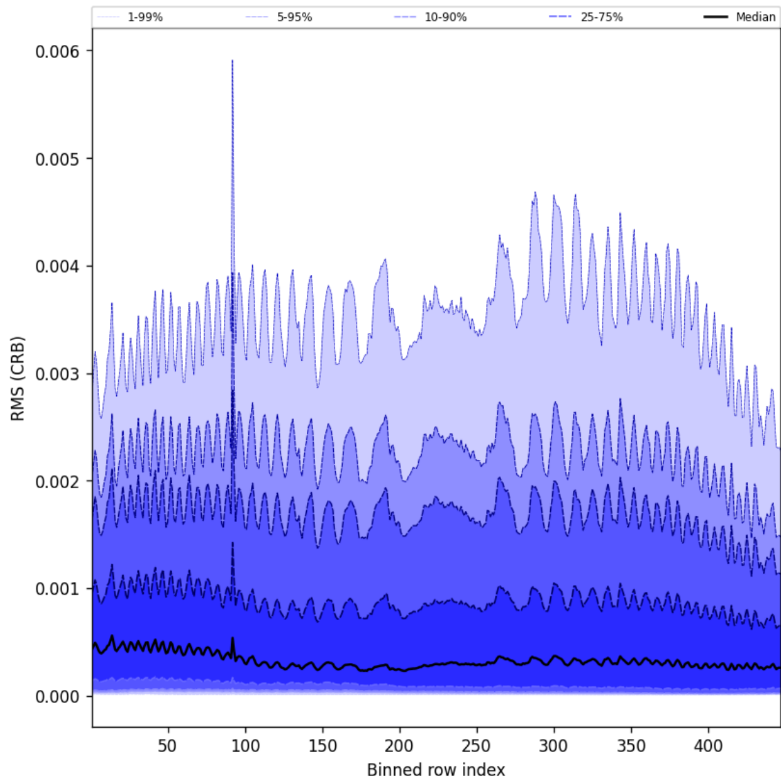
Figure 64: Along track statistics of “RMS (CRB)” for 2025-04-05 to 2025-04-07
