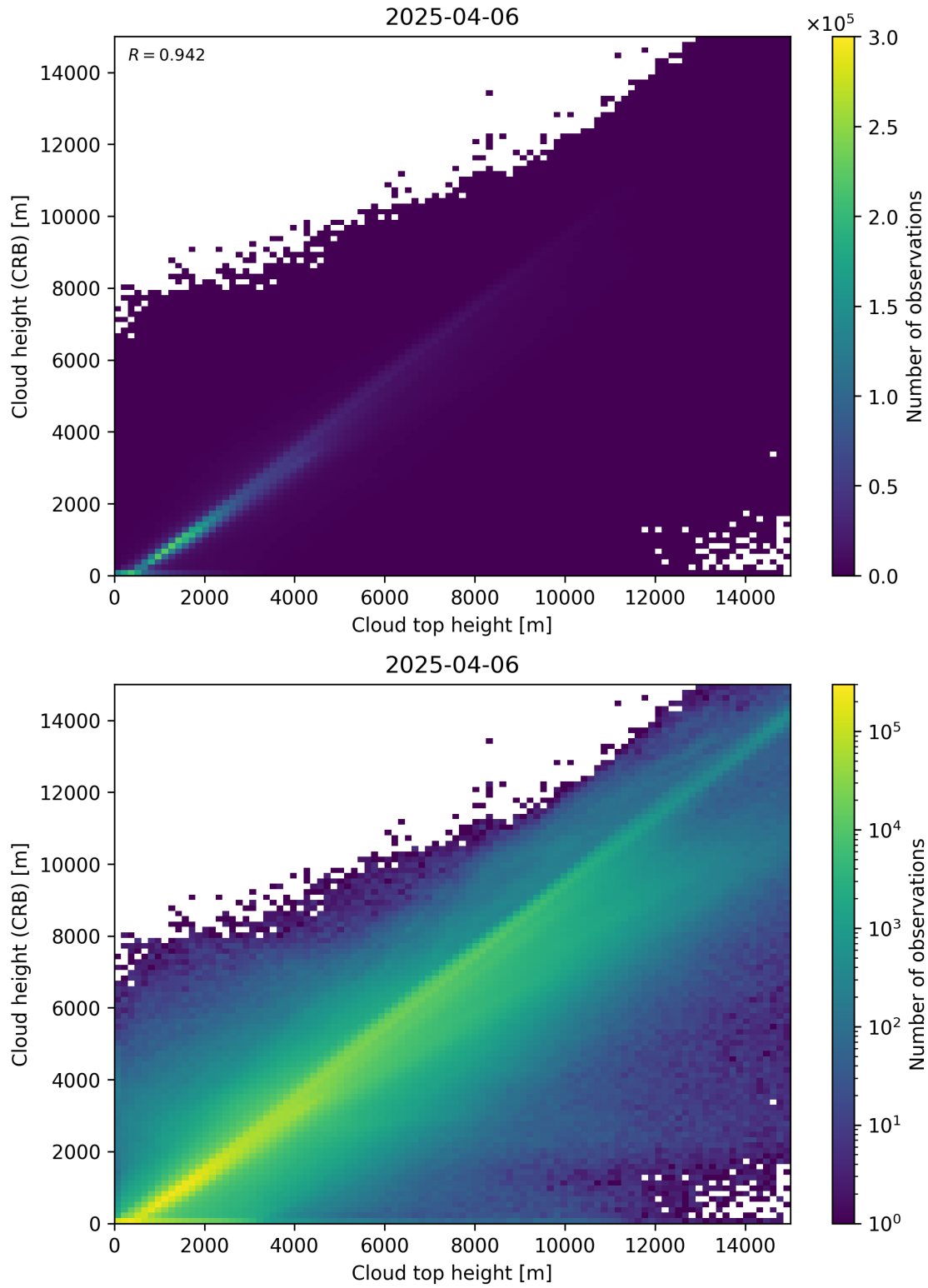
Figure 89: Scatter density plot of “Cloud top height” against “Cloud height (CRB)” for 2025-04-05 to 2025-04-07.
