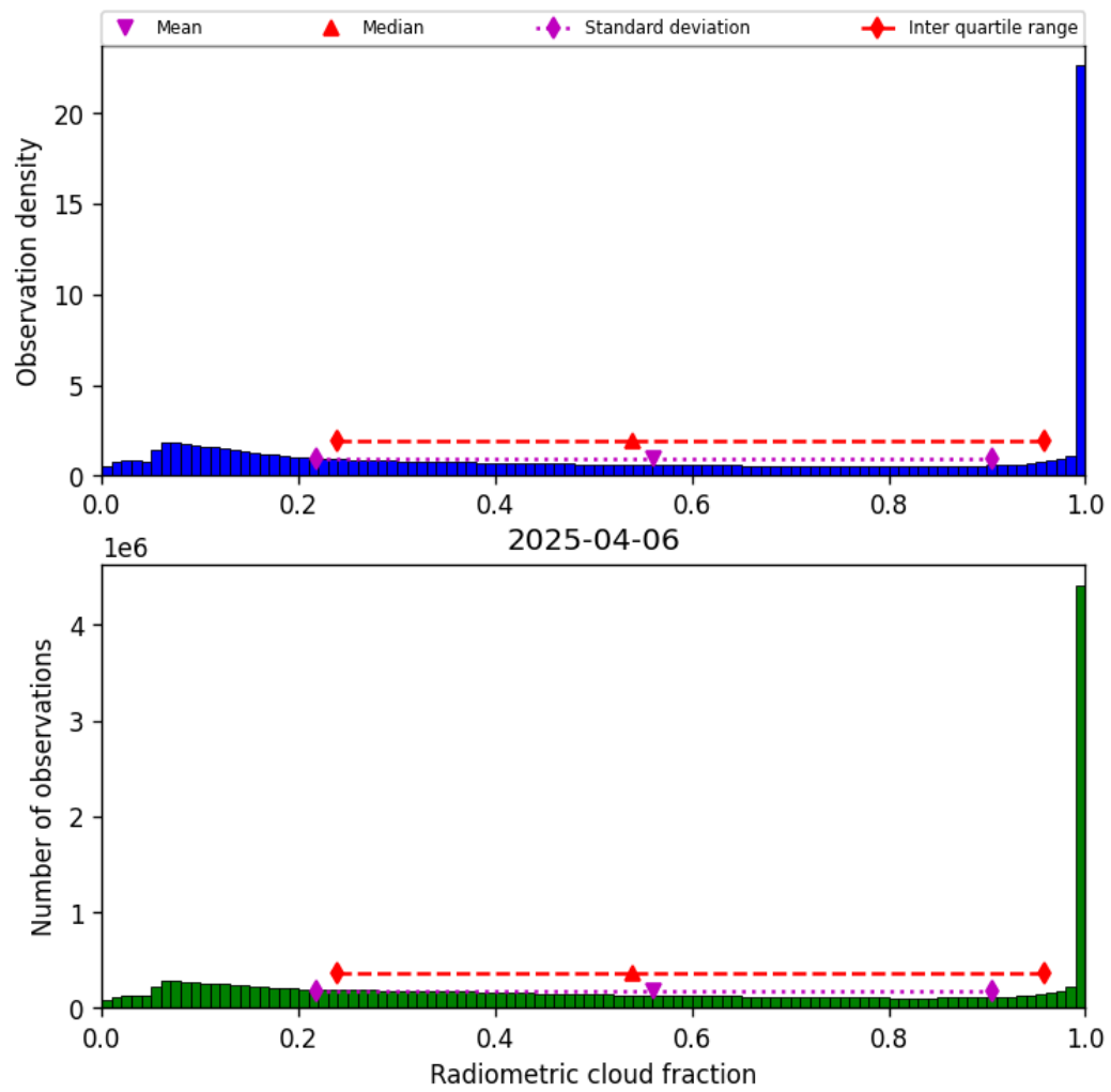
Figure 39: Histogram of “Radiometric cloud fraction” for 2025-04-05 to 2025-04-07
