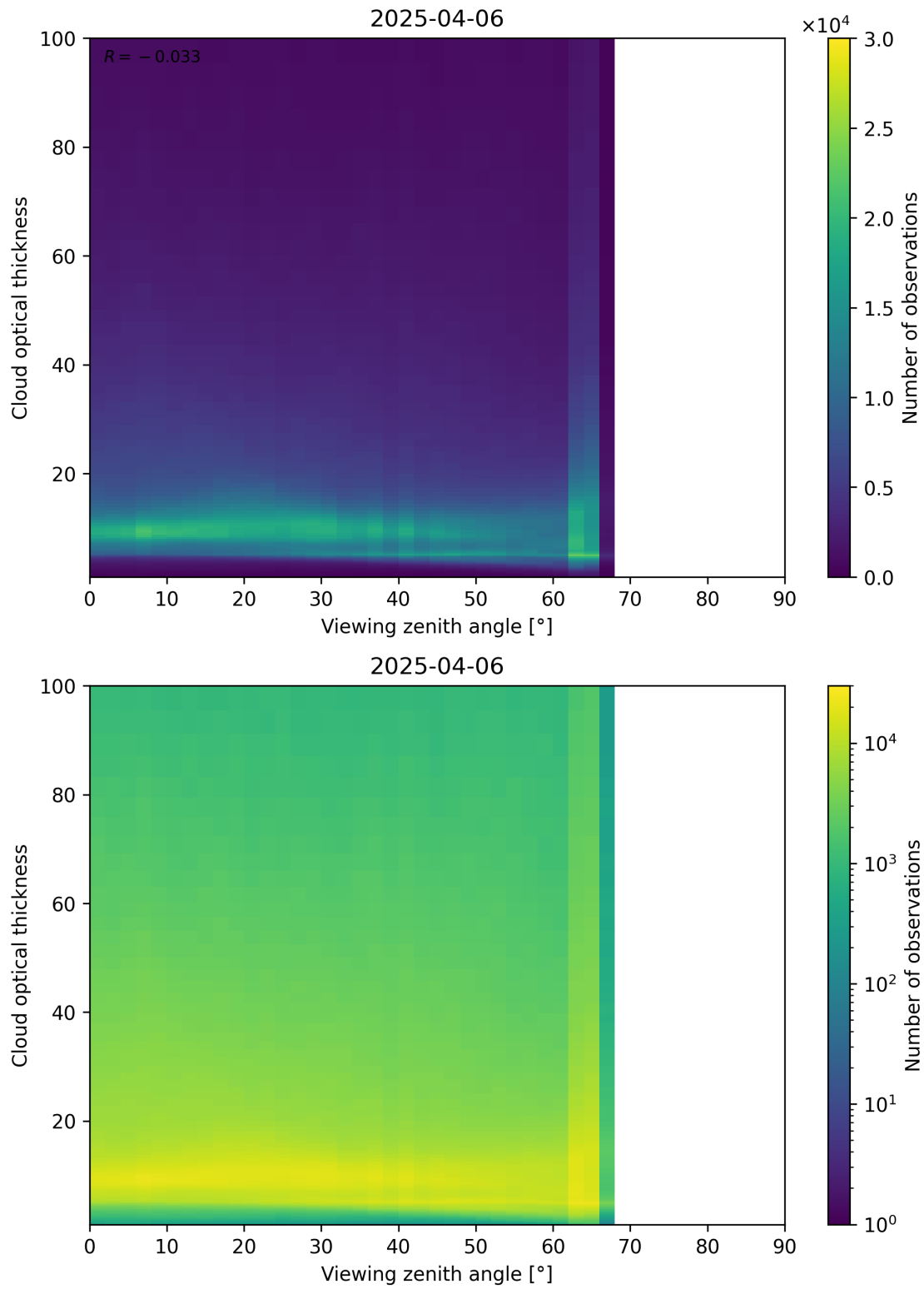
Figure 111: Scatter density plot of “Viewing zenith angle” against “Cloud optical thickness” for 2025-04-05 to 2025-04-07.
