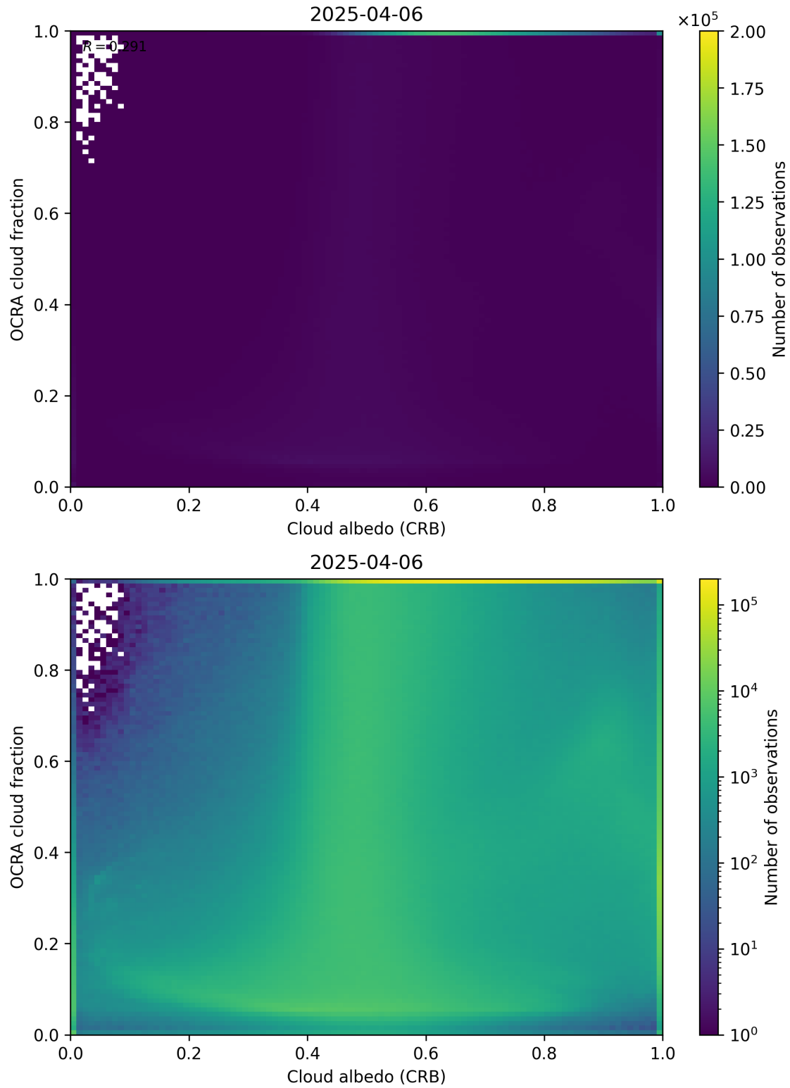
Figure 70: Scatter density plot of “Cloud albedo (CRB)” against “OCRA cloud fraction” for 2025-04-05 to 2025-04-07.
