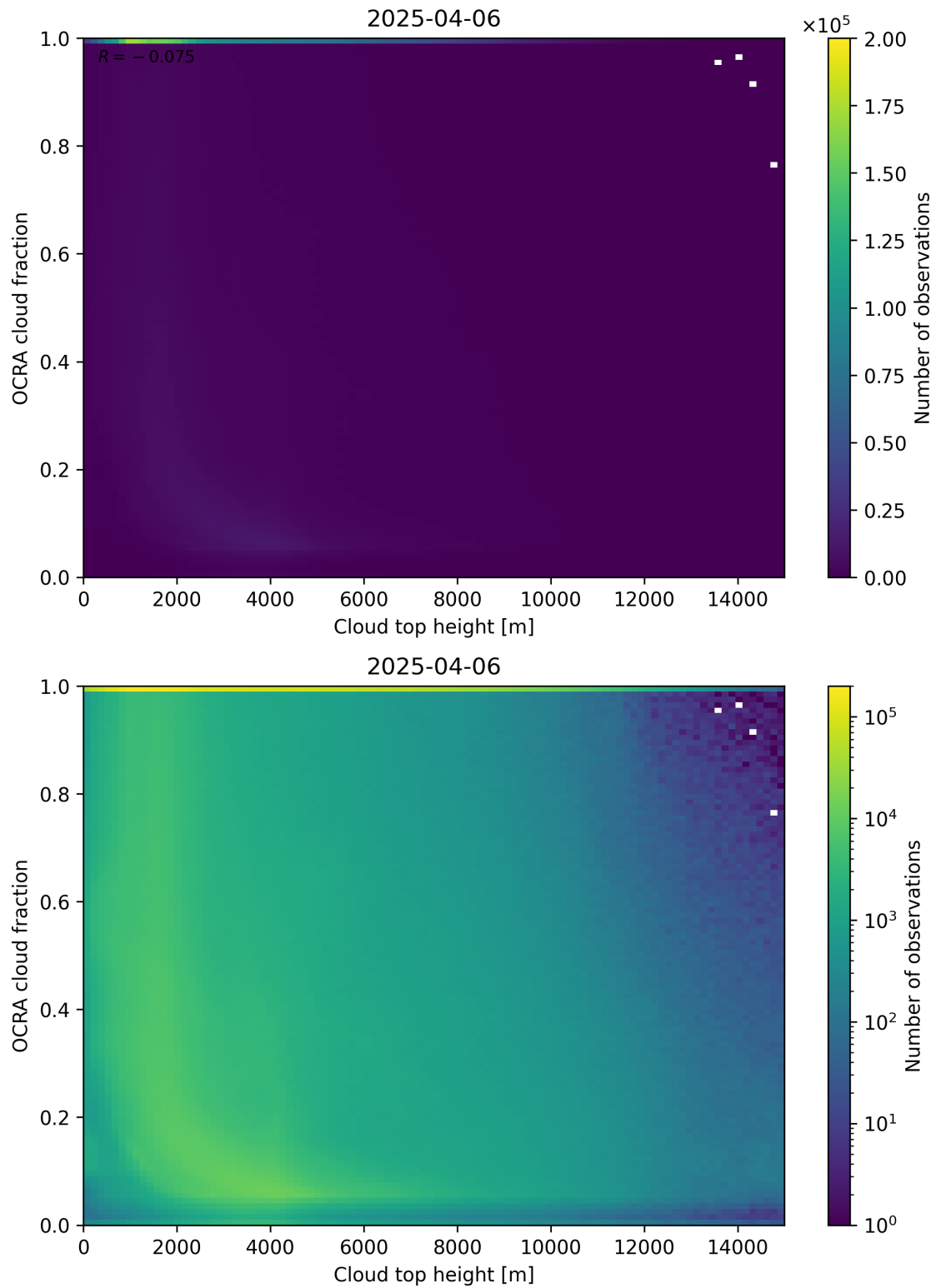
Figure 87: Scatter density plot of “Cloud top height” against “OCRA cloud fraction” for 2025-04-05 to 2025-04-07.
