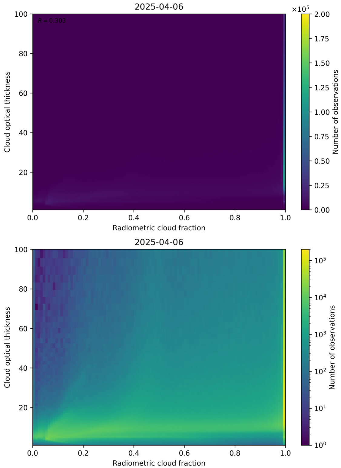
Figure 75: Scatter density plot of “Radiometric cloud fraction” against “Cloud optical thickness” for 2025-04-05 to 2025-04-07.
