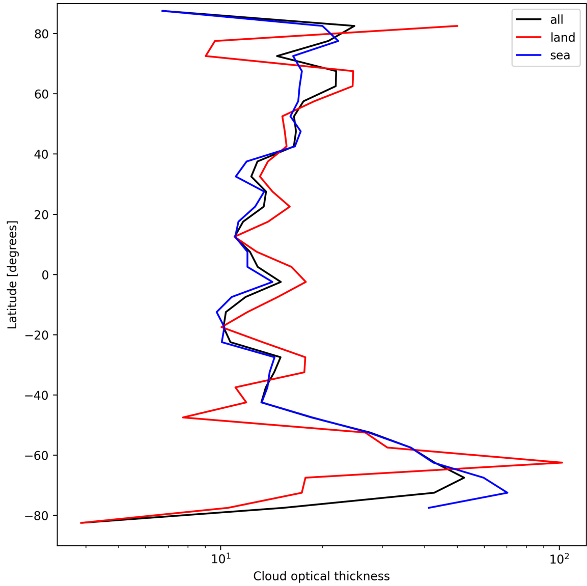
Figure 25: Zonal average of “Cloud optical thickness” for 2025-04-05 to 2025-04-07.
