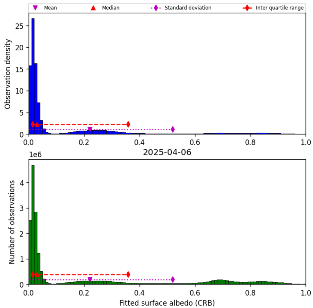
Figure 46: Histogram of “Fitted surface albedo (CRB)” for 2025-04-05 to 2025-04-07
