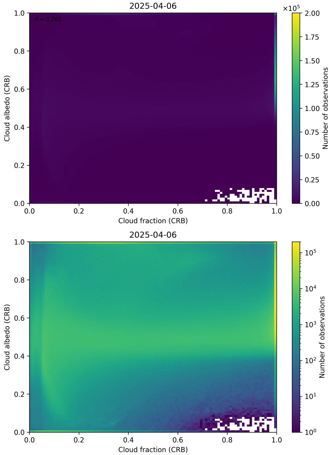
Figure 77: Scatter density plot of “Cloud fraction (CRB)” against “Cloud albedo (CRB)” for 2025-04-05 to 2025-04-07.
