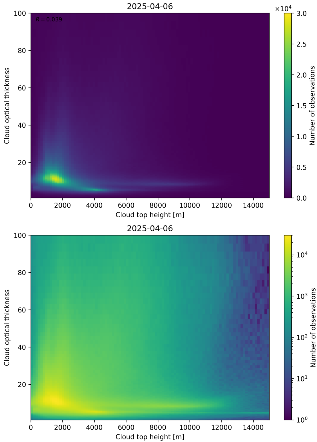
Figure 90: Scatter density plot of “Cloud top height” against “Cloud optical thickness” for 2025-04-05 to 2025-04-07.
