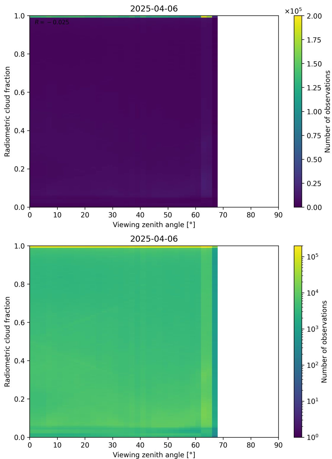
Figure 107: Scatter density plot of “Viewing zenith angle” against “Radiometric cloud fraction” for 2025-04-05 to 2025-04-07.
