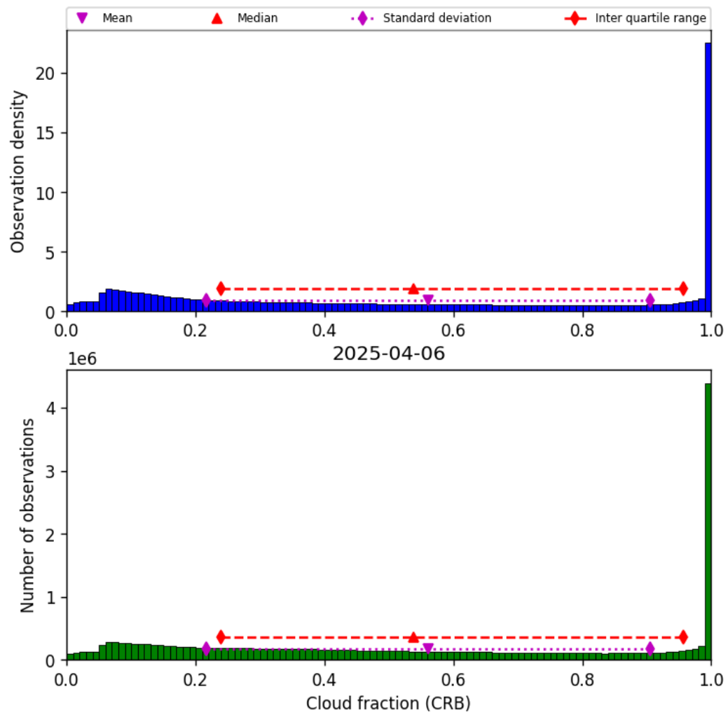
Figure 42: Histogram of “Cloud fraction (CRB)” for 2025-04-05 to 2025-04-07
