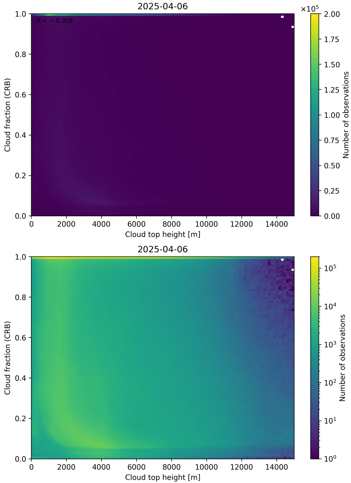
Figure 88: Scatter density plot of “Cloud top height” against “Cloud fraction (CRB)” for 2025-04-05 to 2025-04-07.
