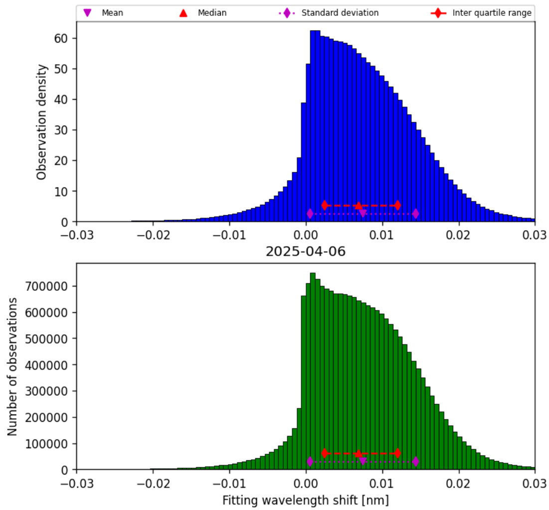
Figure 49: Histogram of “Fitting wavelength shift” for 2025-04-05 to 2025-04-07
