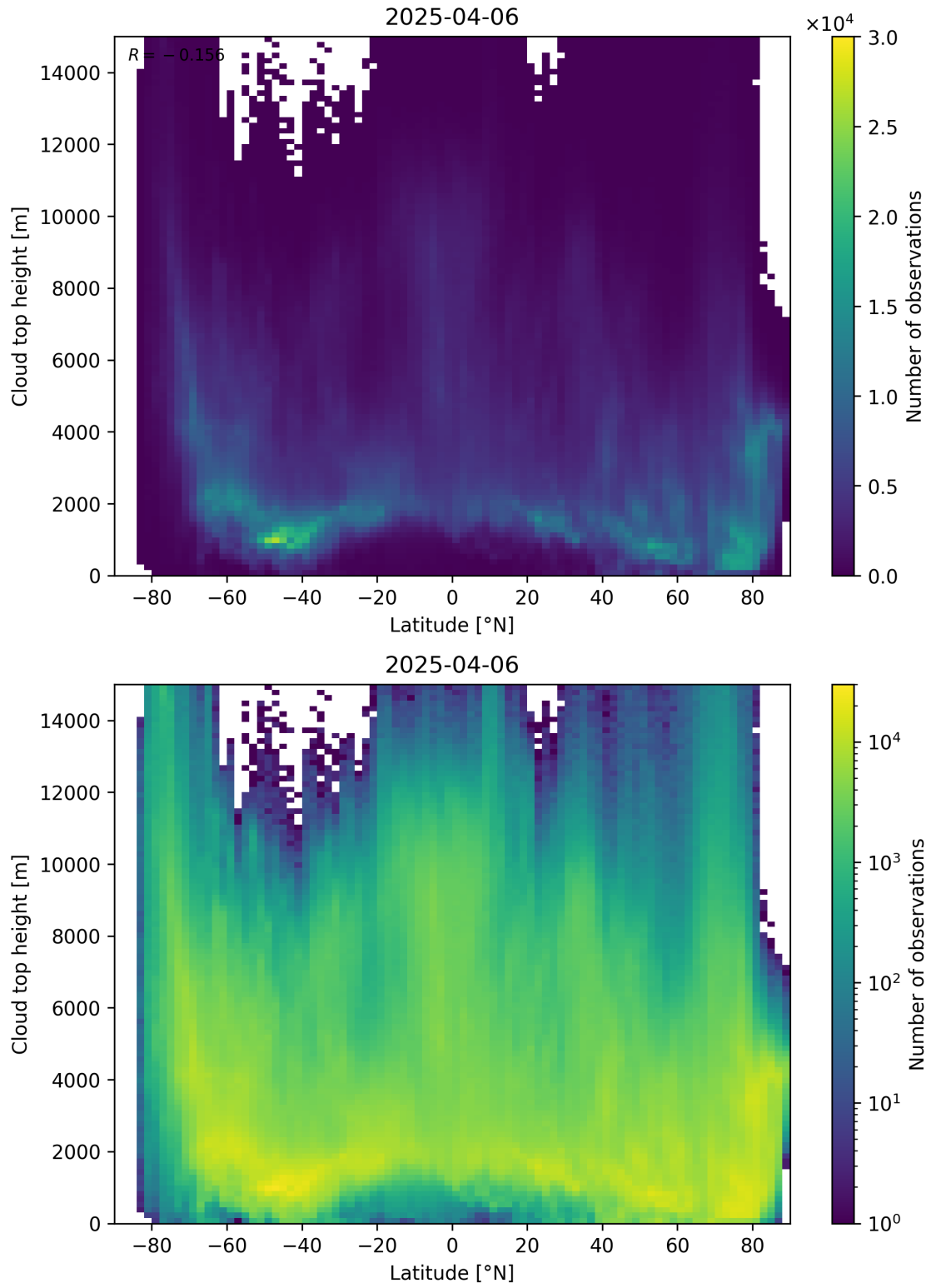
Figure 97: Scatter density plot of “Latitude” against “Cloud top height” for 2025-04-05 to 2025-04-07.
