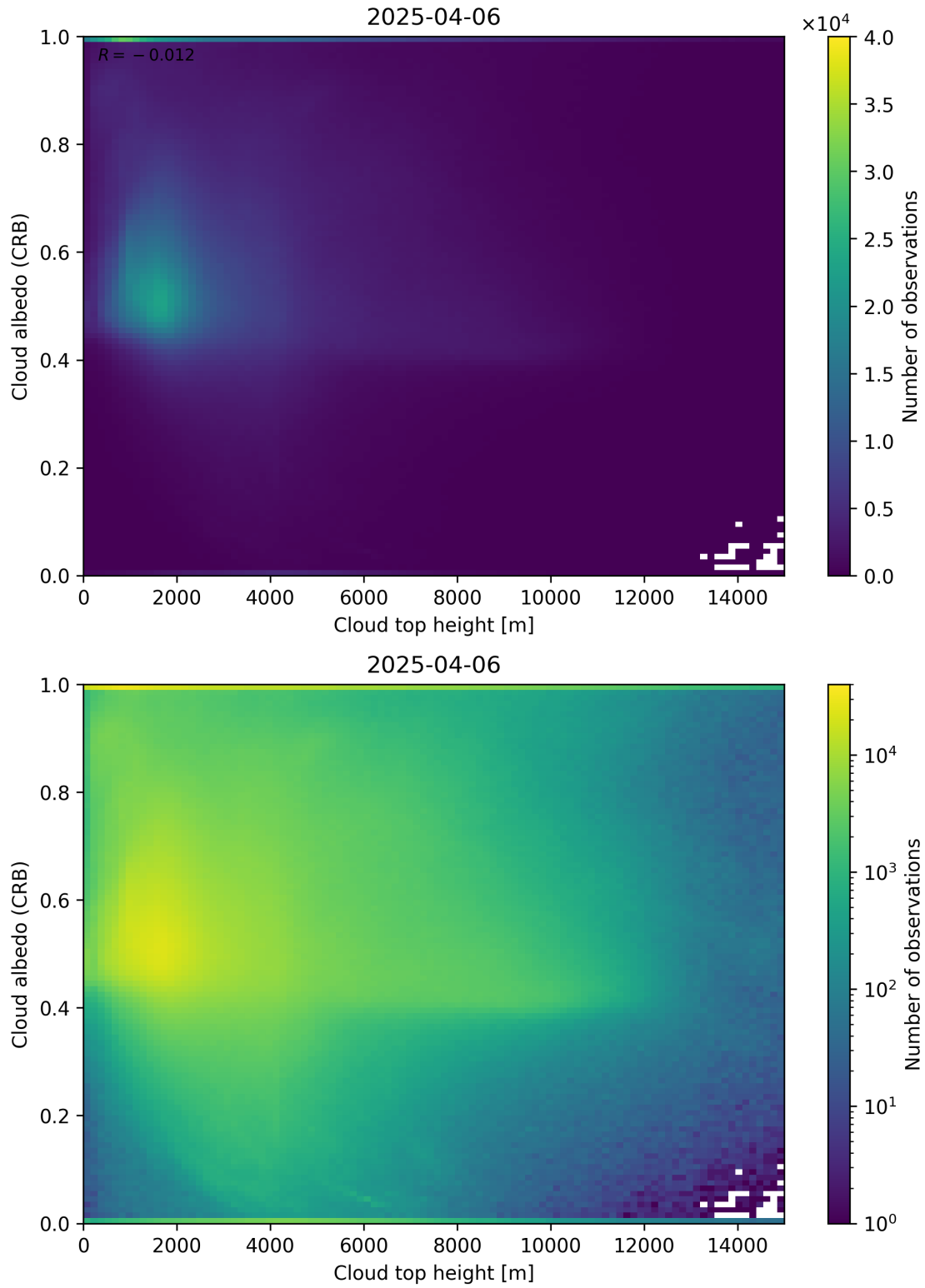
Figure 86: Scatter density plot of “Cloud top height” against “Cloud albedo (CRB)” for 2025-04-05 to 2025-04-07.
