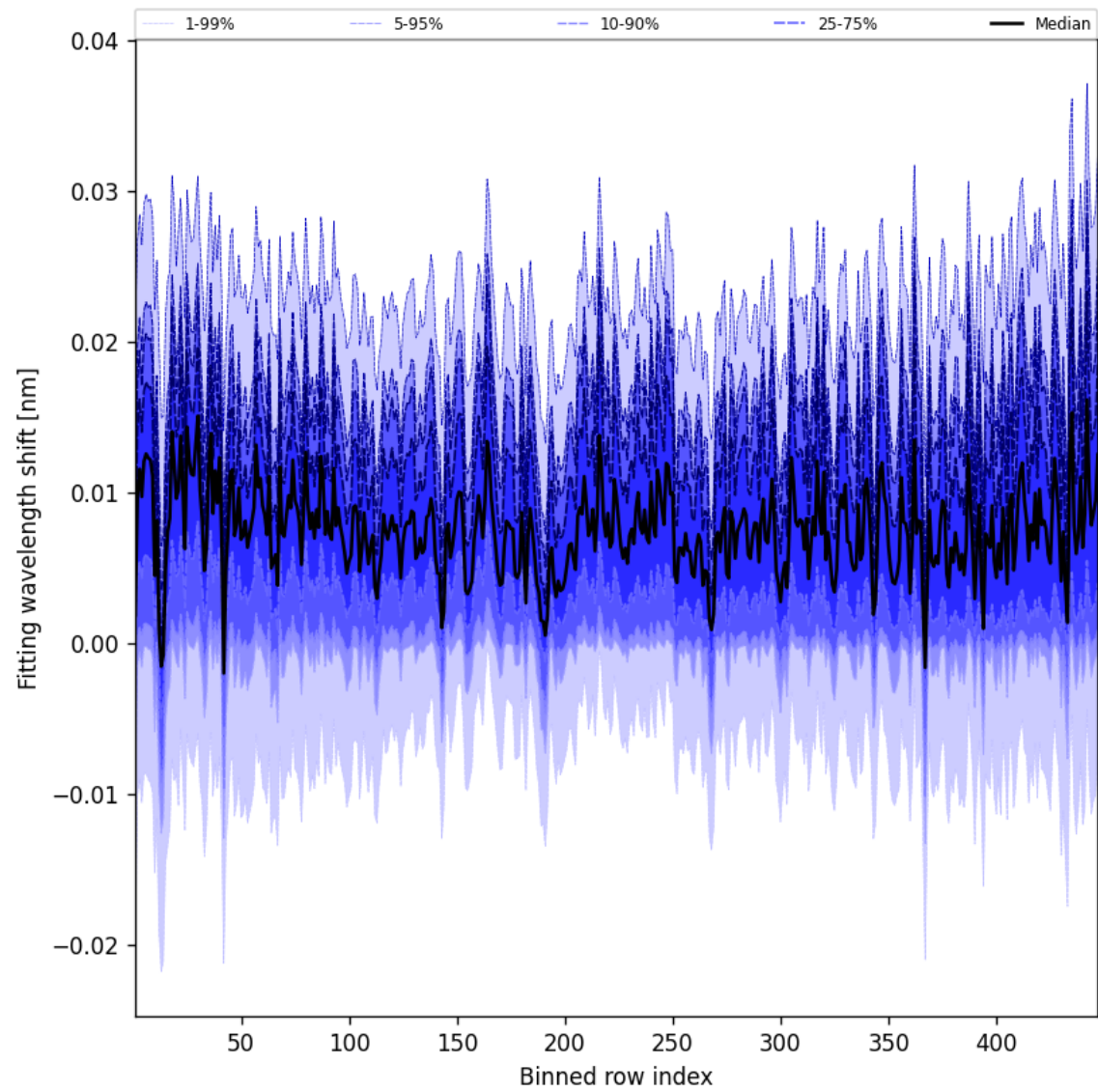
Figure 65: Along track statistics of “Fitting wavelength shift” for 2025-04-05 to 2025-04-07
