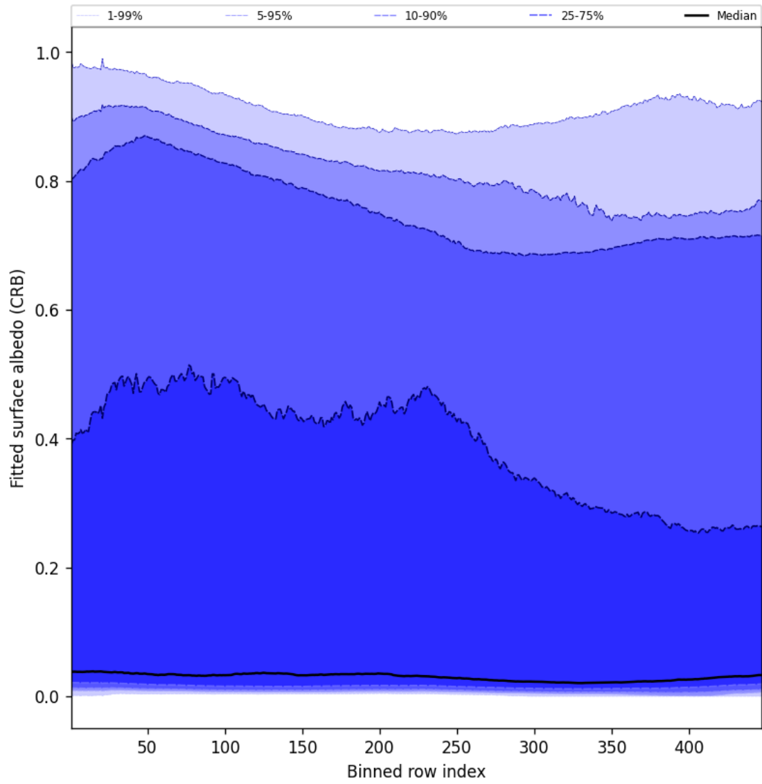
Figure 62: Along track statistics of “Fitted surface albedo (CRB)” for 2025-04-05 to 2025-04-07
