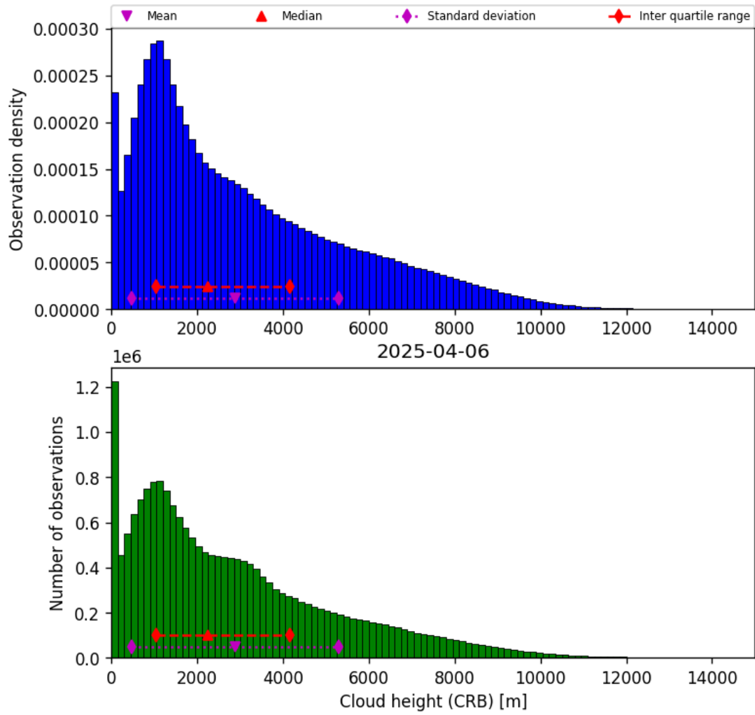
Figure 43: Histogram of “Cloud height (CRB)” for 2025-04-05 to 2025-04-07
