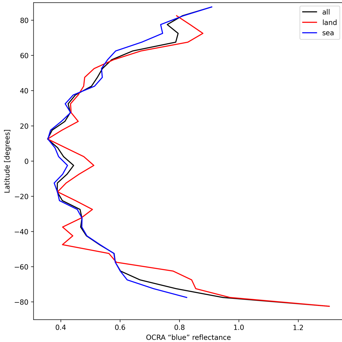
Figure 35: Zonal average of “OCRA “blue” reflectance” for 2025-04-05 to 2025-04-07.
