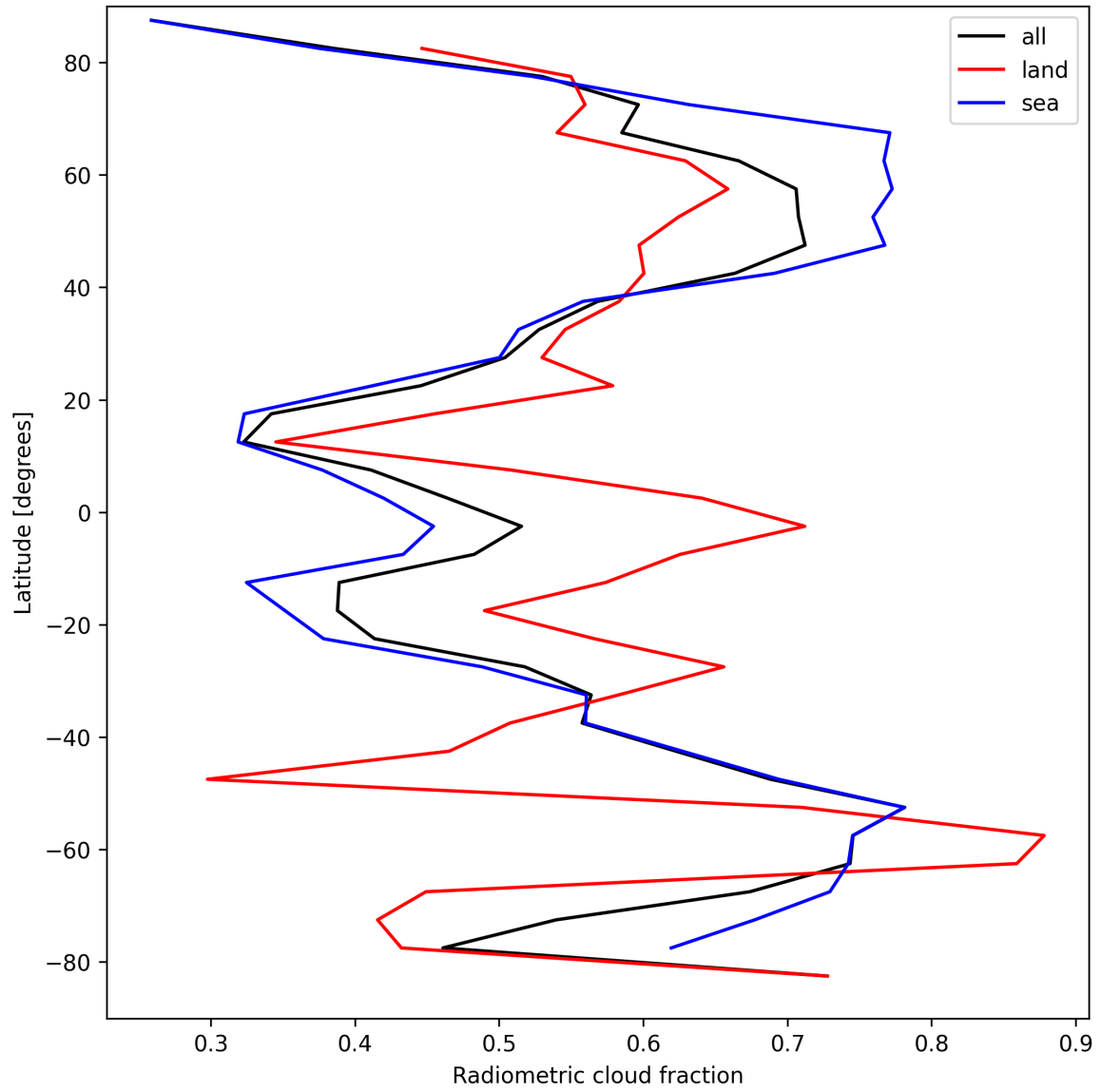
Figure 23: Zonal average of “Radiometric cloud fraction” for 2025-04-05 to 2025-04-07.
