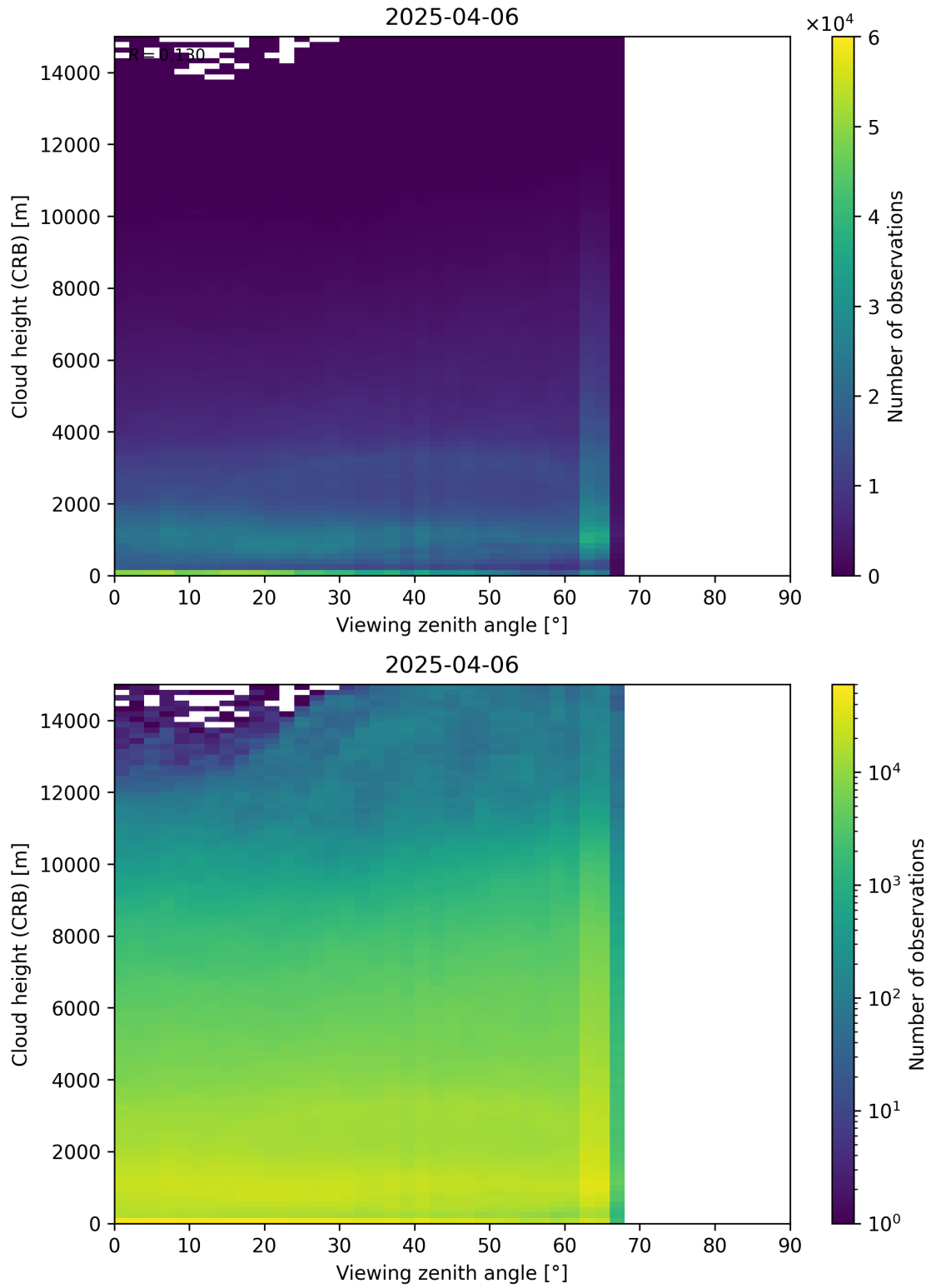
Figure 110: Scatter density plot of “Viewing zenith angle” against “Cloud height (CRB)” for 2025-04-05 to 2025-04-07.
