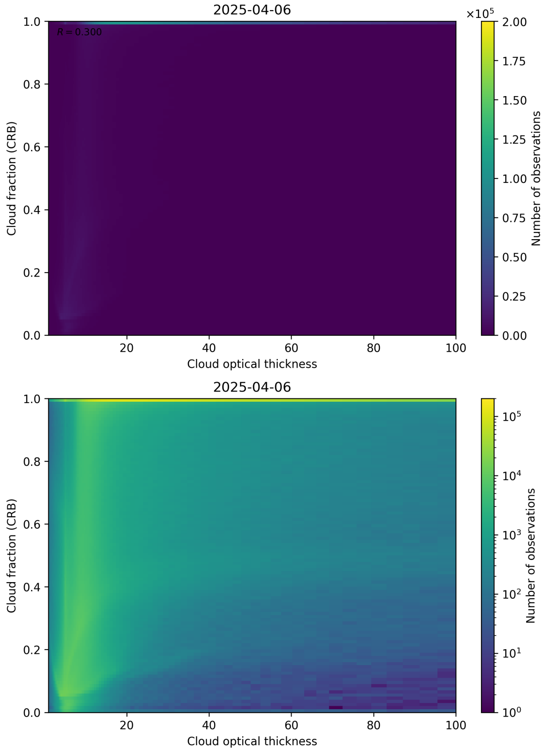
Figure 84: Scatter density plot of “Cloud optical thickness” against “Cloud fraction (CRB)” for 2025-04-05 to 2025-04-07.
