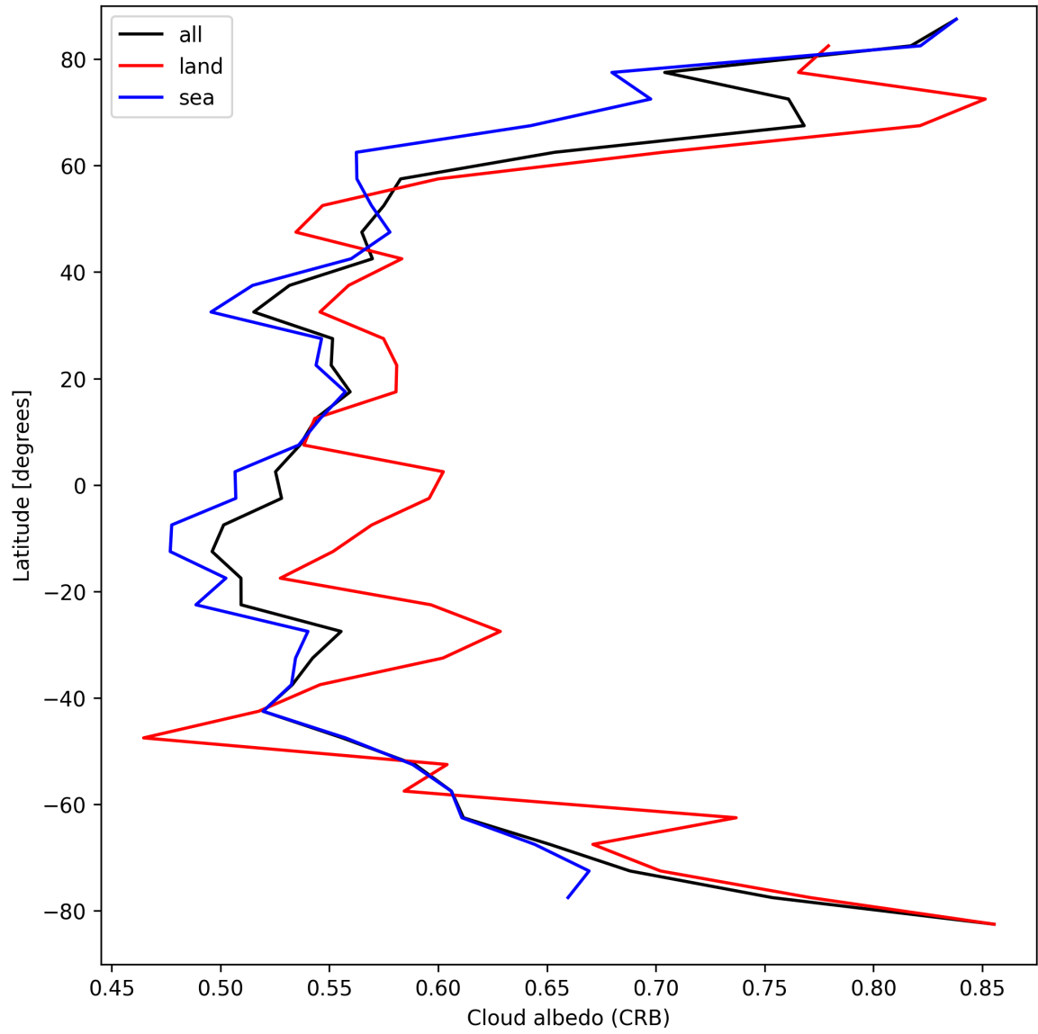
Figure 28: Zonal average of “Cloud albedo (CRB)” for 2025-04-05 to 2025-04-07.
