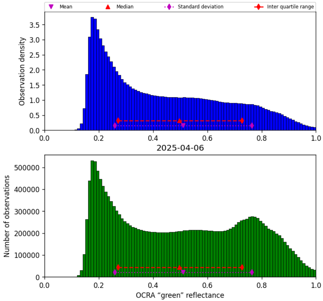
Figure 52: Histogram of “OCRA “green” reflectance” for 2025-04-05 to 2025-04-07
