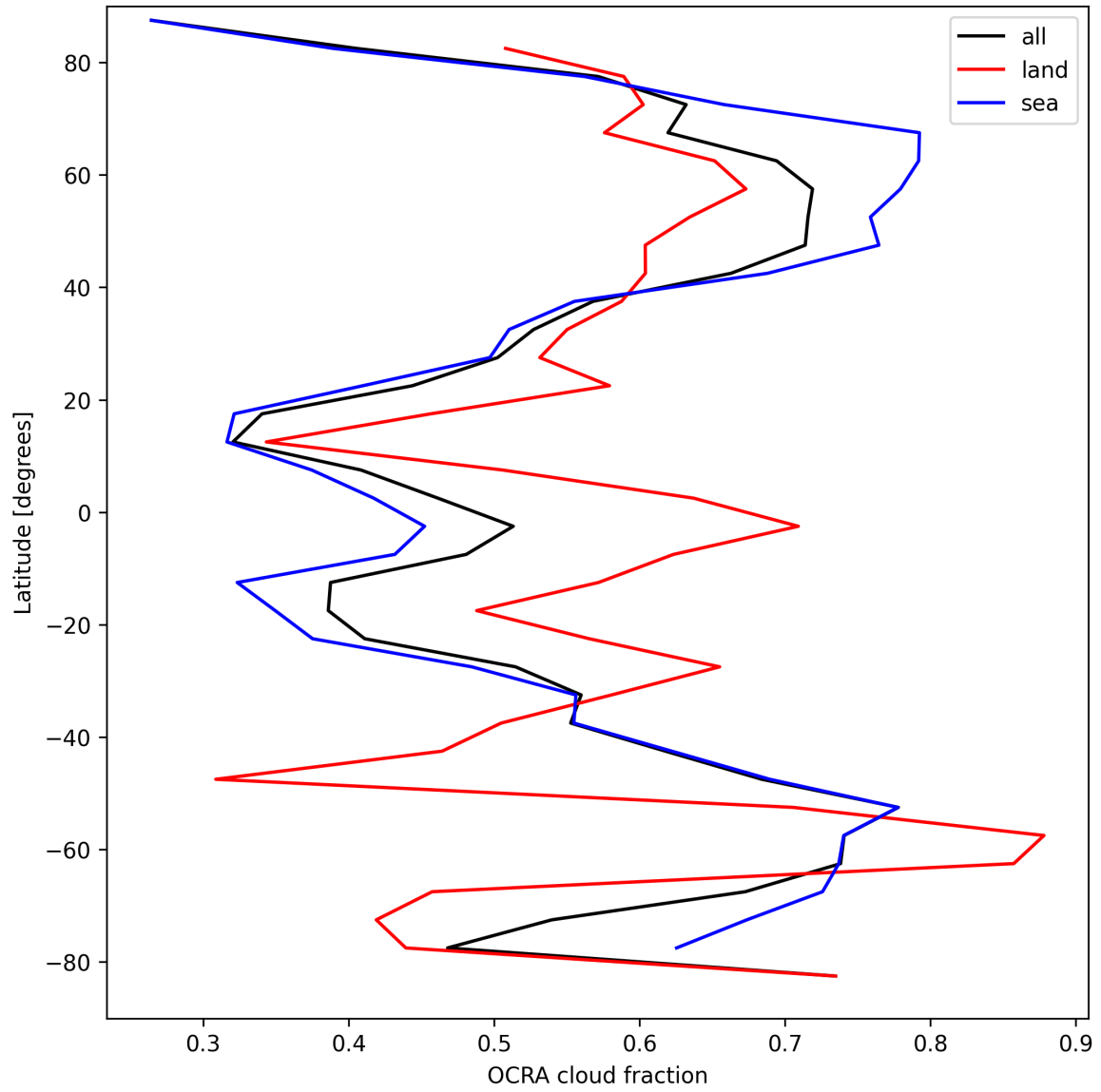
Figure 34: Zonal average of “OCRA cloud fraction” for 2025-04-05 to 2025-04-07.
