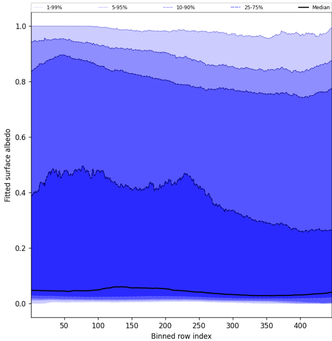
Figure 61: Along track statistics of “Fitted surface albedo” for 2025-04-05 to 2025-04-07
