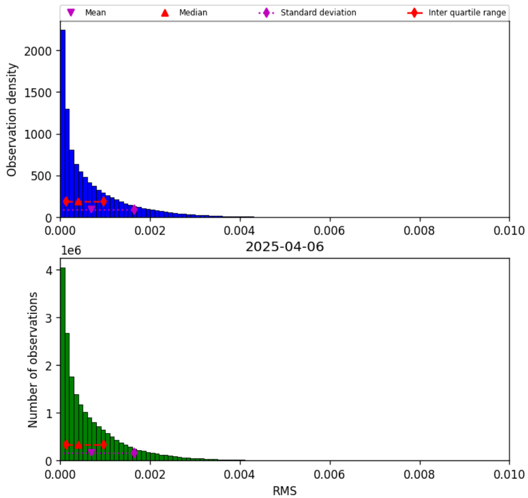
Figure 47: Histogram of “RMS” for 2025-04-05 to 2025-04-07
