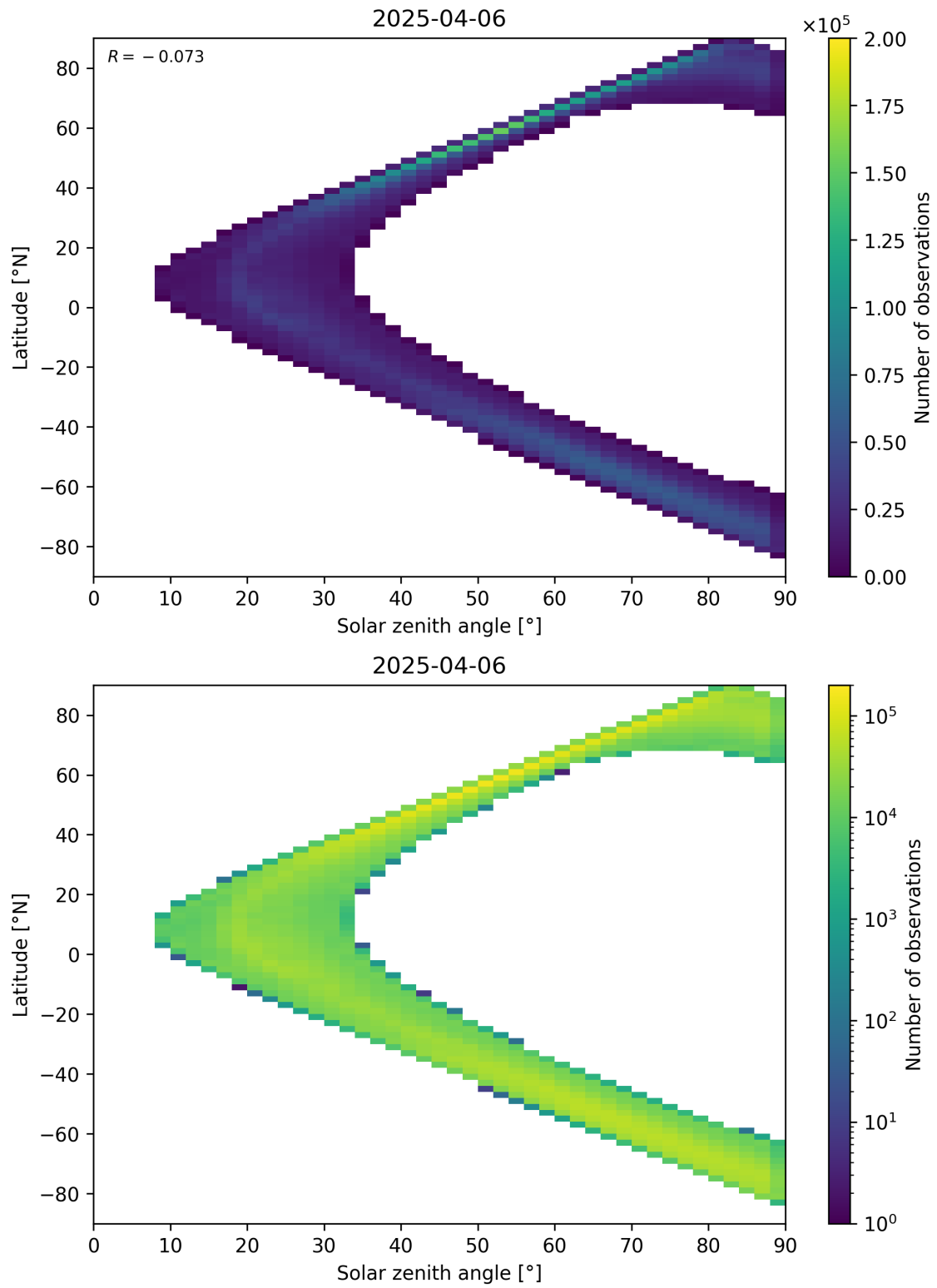
Figure 105: Scatter density plot of “Solar zenith angle” against “Latitude” for 2025-04-05 to 2025-04-07.
