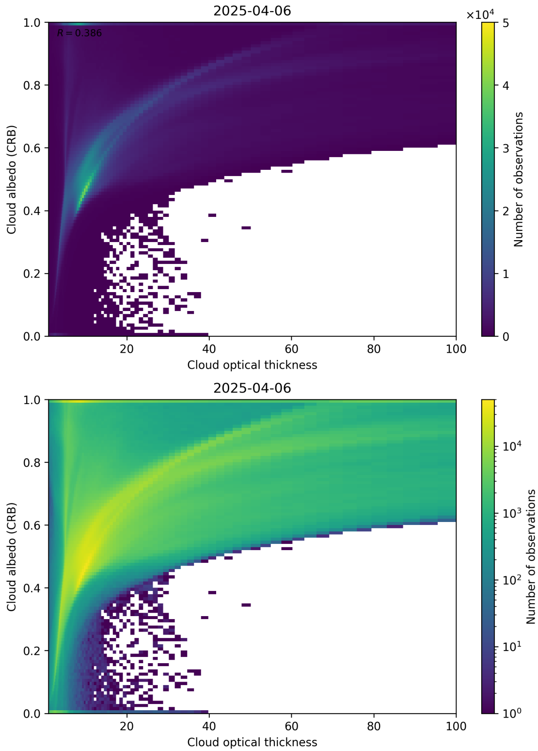
Figure 82: Scatter density plot of “Cloud optical thickness” against “Cloud albedo (CRB)” for 2025-04-05 to 2025-04-07.
