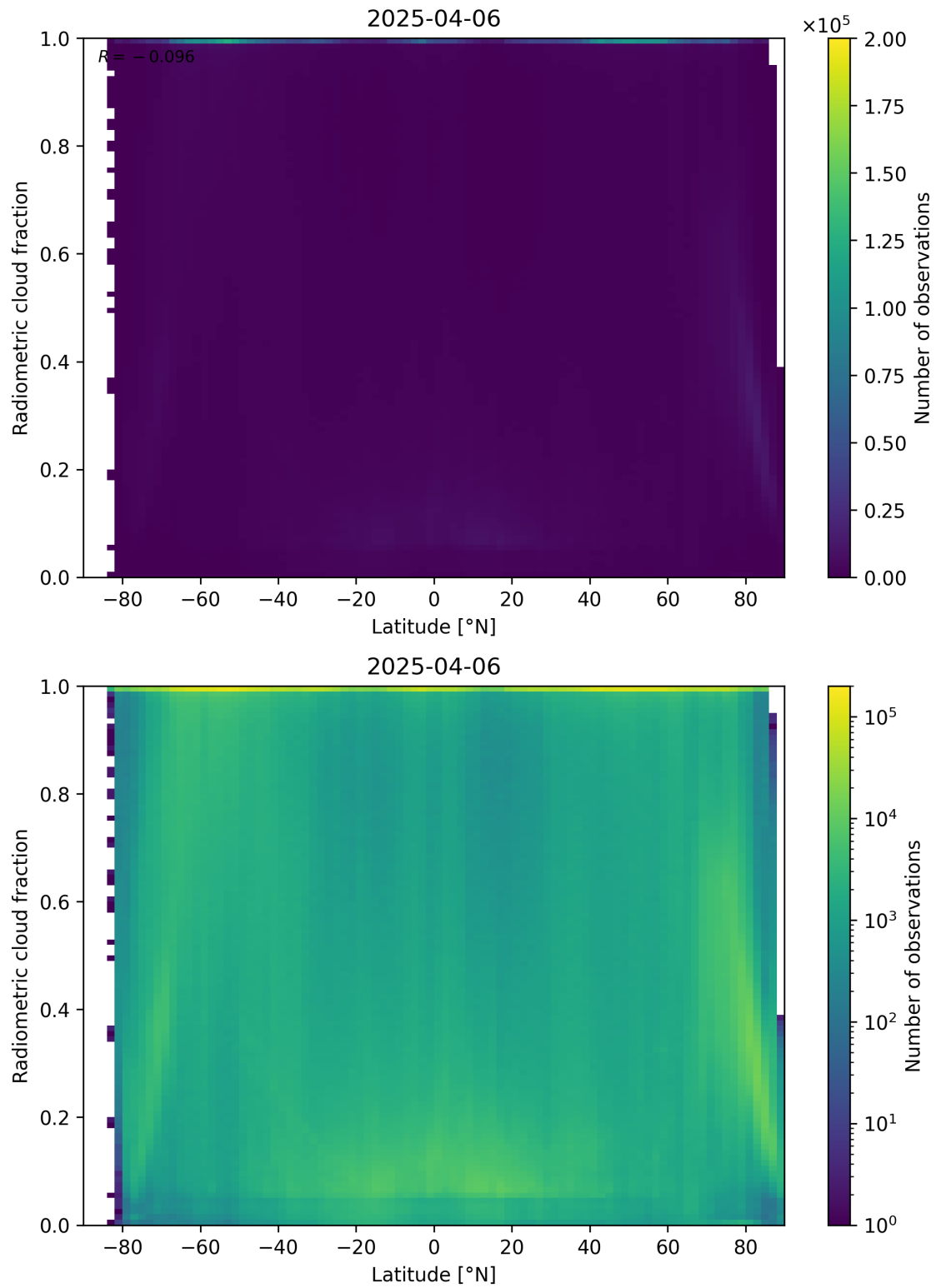
Figure 92: Scatter density plot of “Latitude” against “Radiometric cloud fraction” for 2025-04-05 to 2025-04-07.
