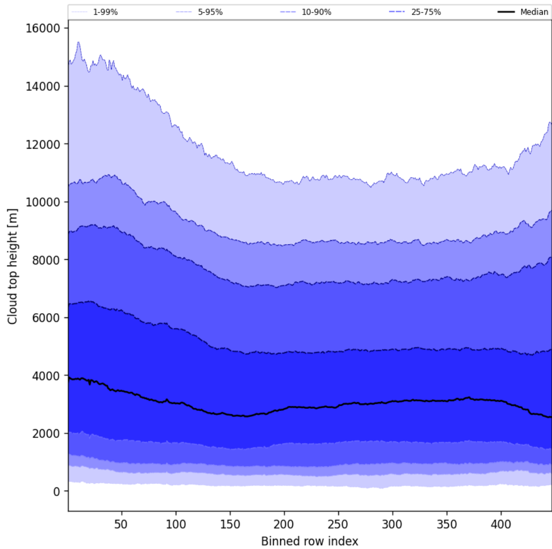
Figure 56: Along track statistics of “Cloud top height” for 2025-04-05 to 2025-04-07
