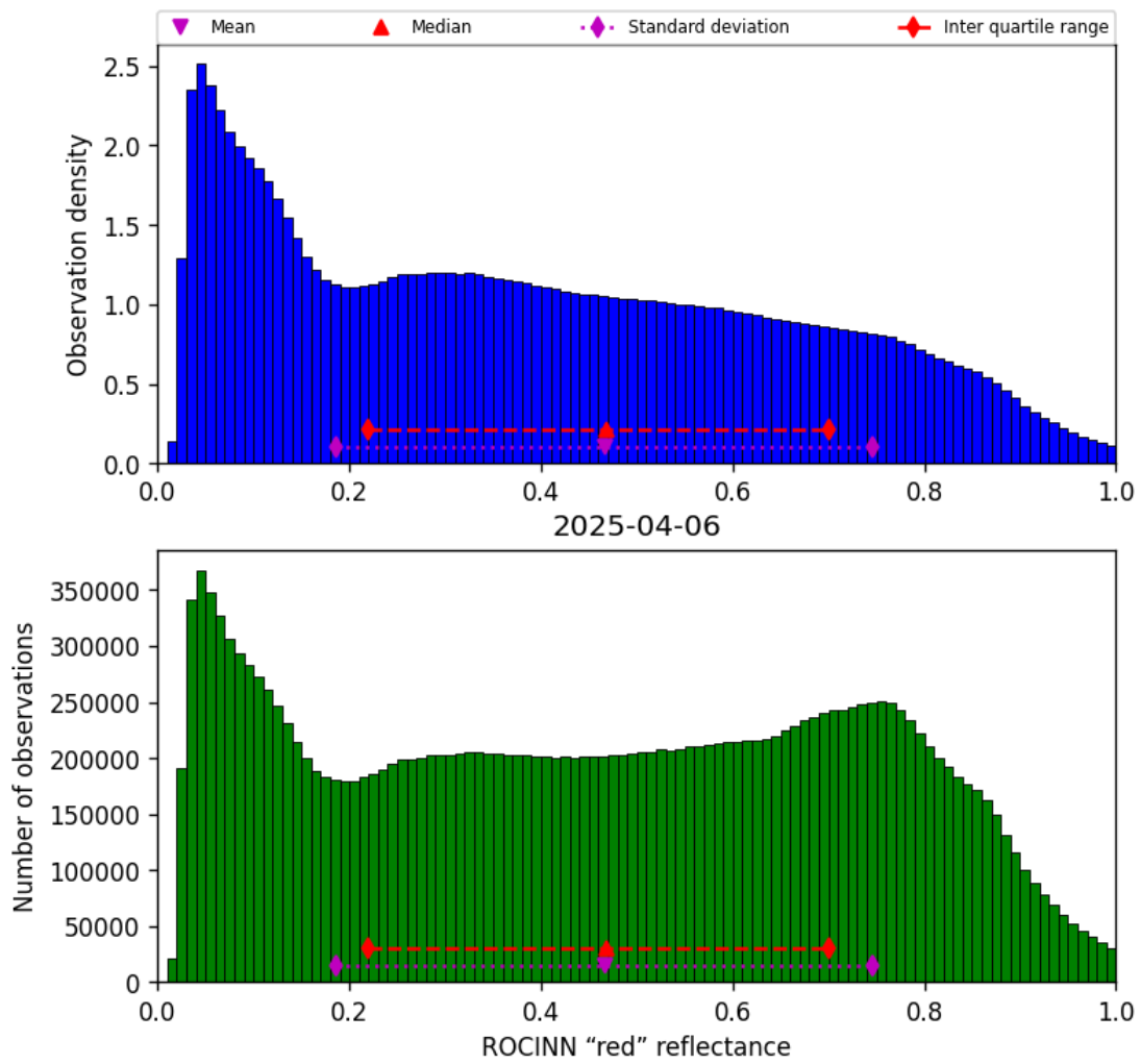
Figure 53: Histogram of “ROCINN “red” reflectance” for 2025-04-05 to 2025-04-07
