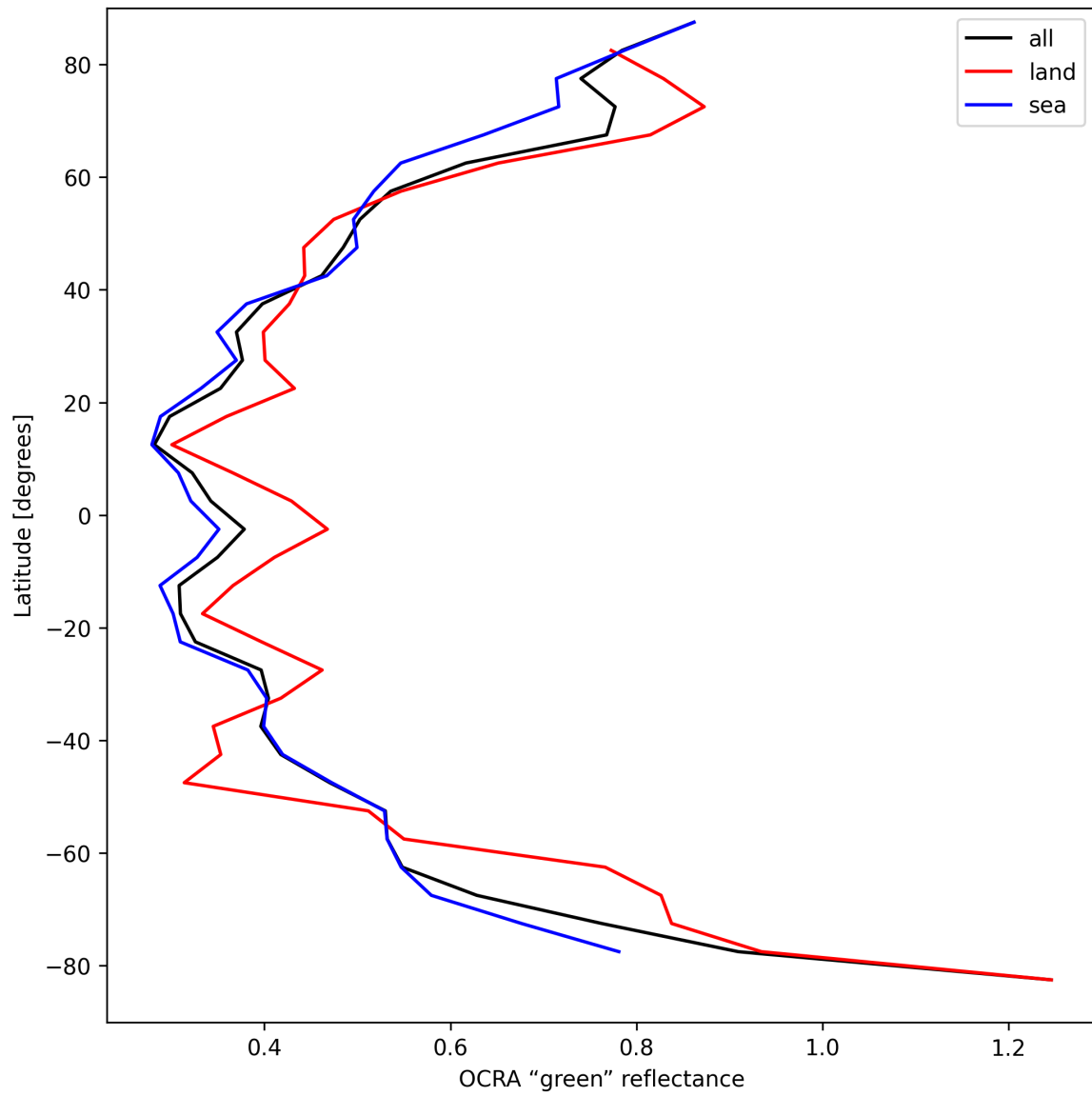
Figure 36: Zonal average of “OCRA “green” reflectance” for 2025-04-05 to 2025-04-07.
