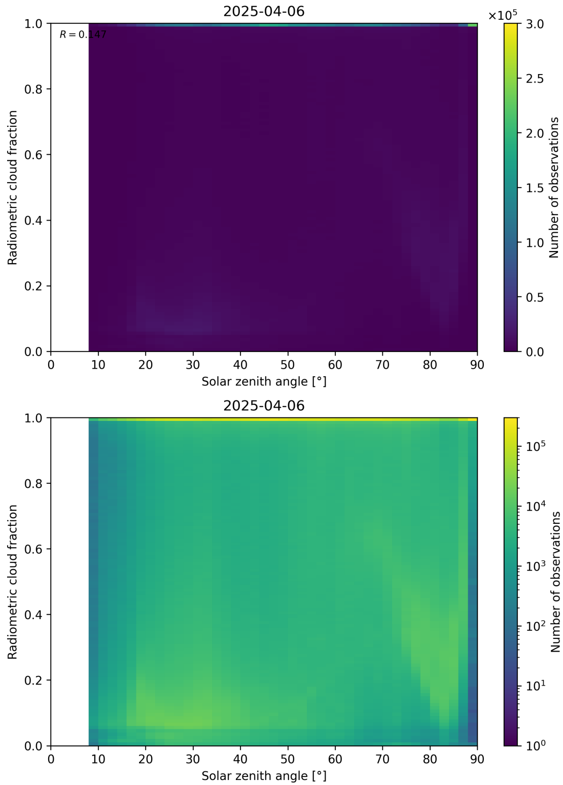
Figure 99: Scatter density plot of “Solar zenith angle” against “Radiometric cloud fraction” for 2025-04-05 to 2025-04-07.
