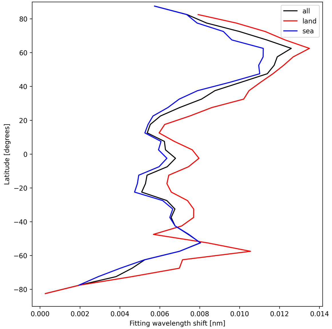
Figure 33: Zonal average of “Fitting wavelength shift” for 2025-04-05 to 2025-04-07.
