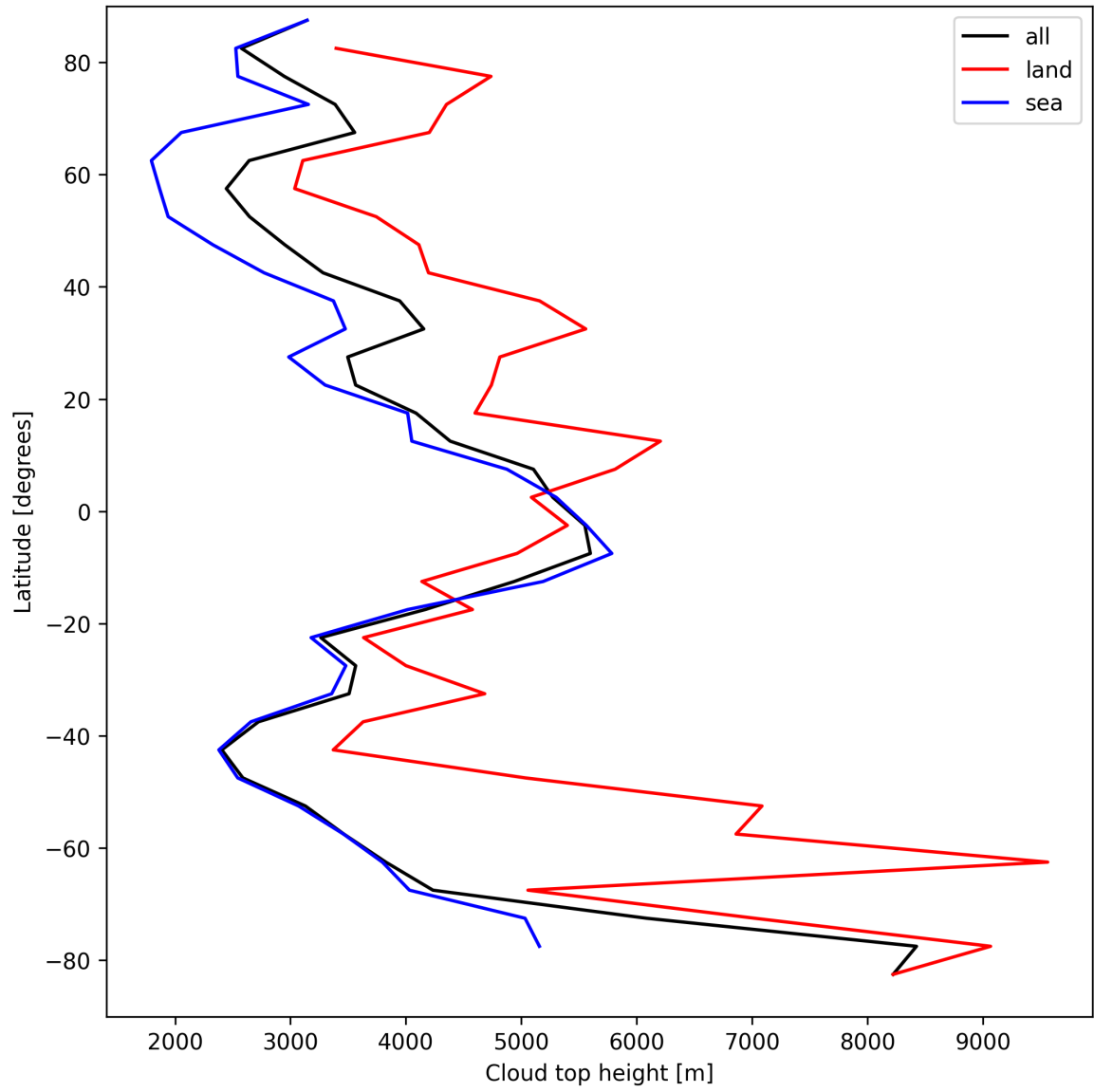
Figure 24: Zonal average of “Cloud top height” for 2025-04-05 to 2025-04-07.
