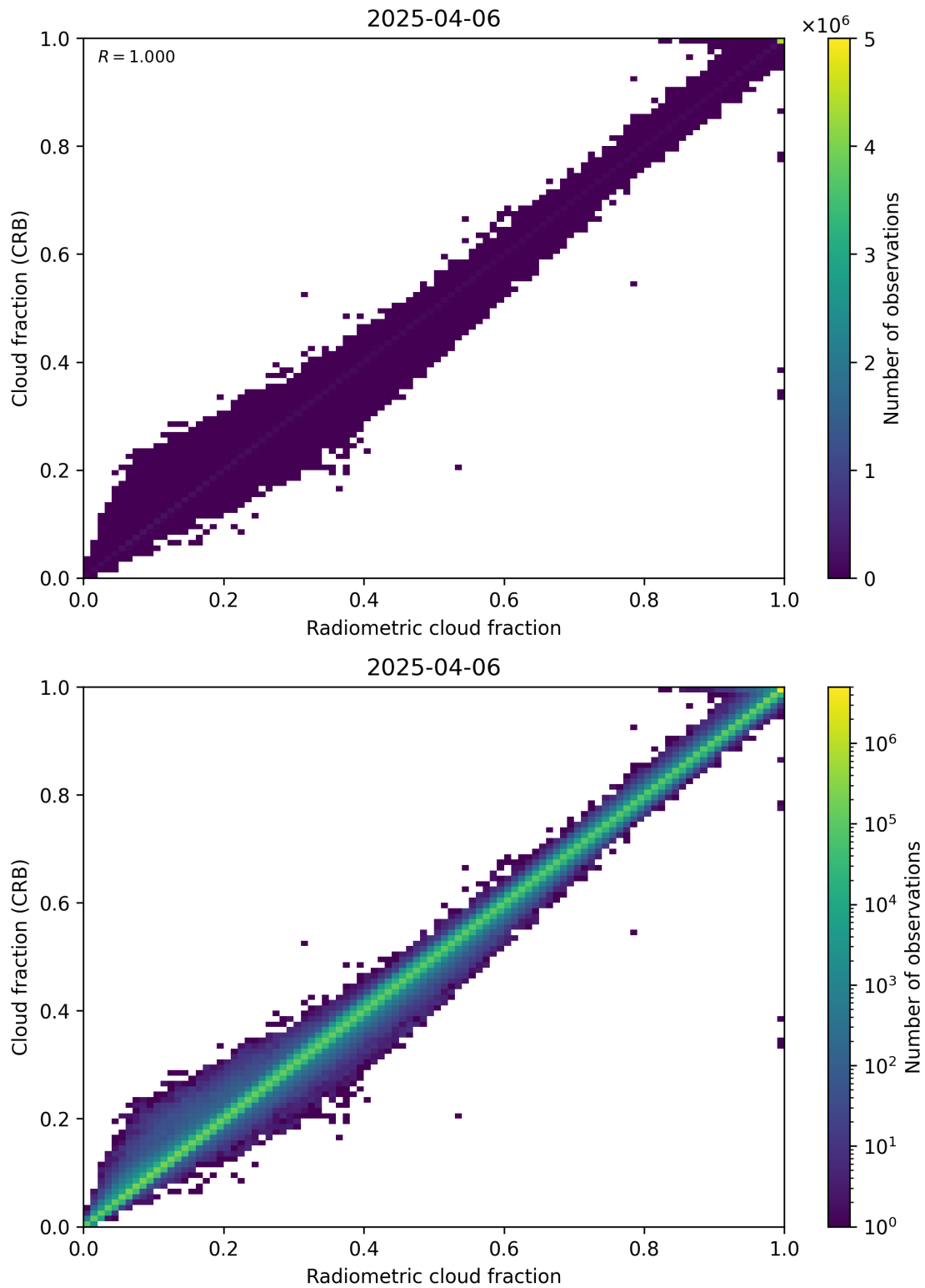
Figure 73: Scatter density plot of “Radiometric cloud fraction” against “Cloud fraction (CRB)” for 2025-04-05 to 2025-04-07.
