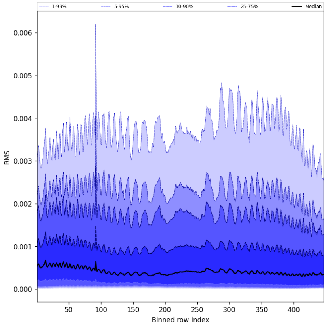
Figure 63: Along track statistics of “RMS” for 2025-04-05 to 2025-04-07
