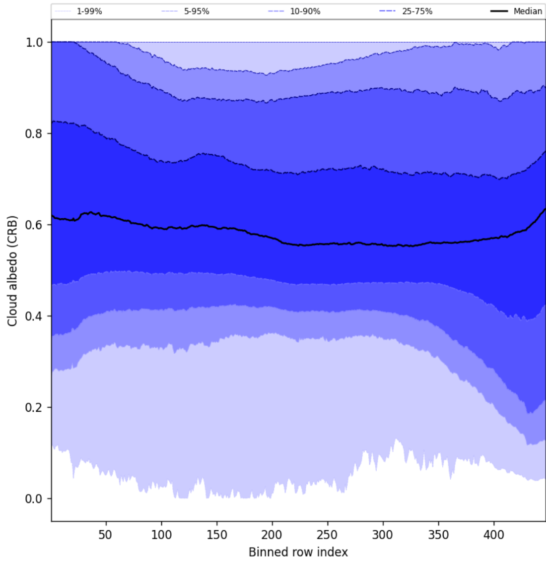
Figure 60: Along track statistics of “Cloud albedo (CRB)” for 2025-04-05 to 2025-04-07
