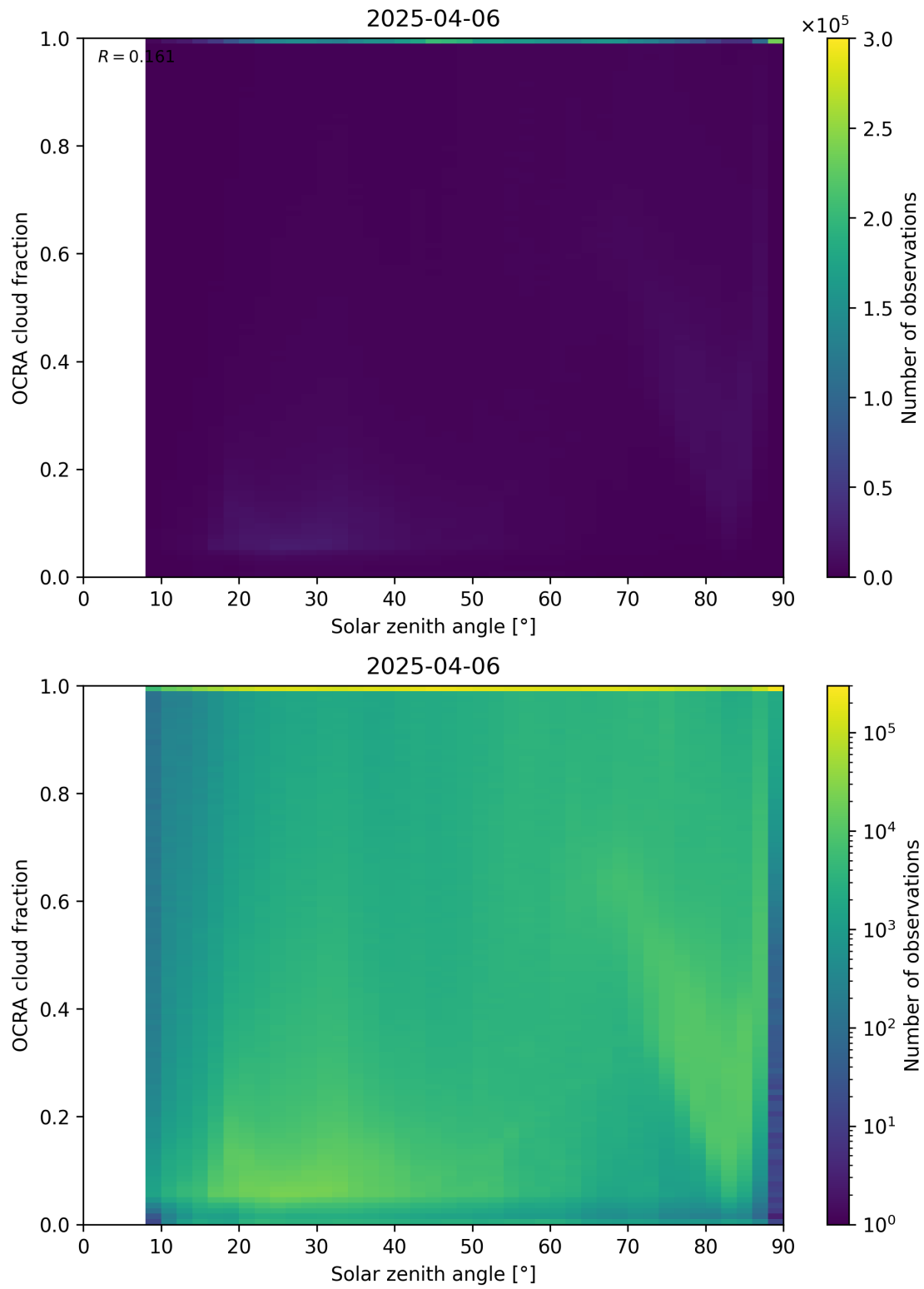
Figure 100: Scatter density plot of “Solar zenith angle” against “OCRA cloud fraction” for 2025-04-05 to 2025-04-07.
