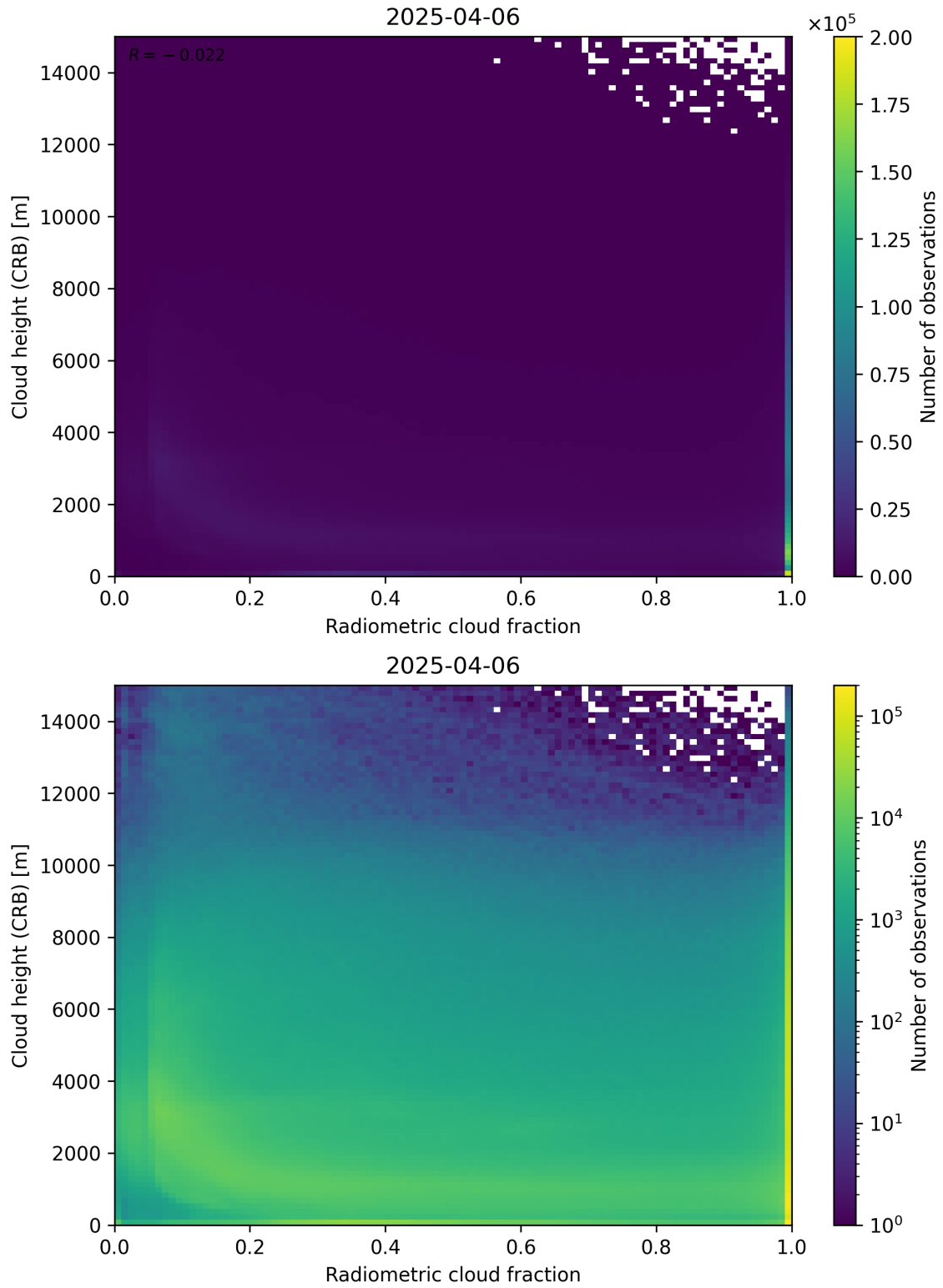
Figure 74: Scatter density plot of “Radiometric cloud fraction” against “Cloud height (CRB)” for 2025-04-05 to 2025-04-07.
