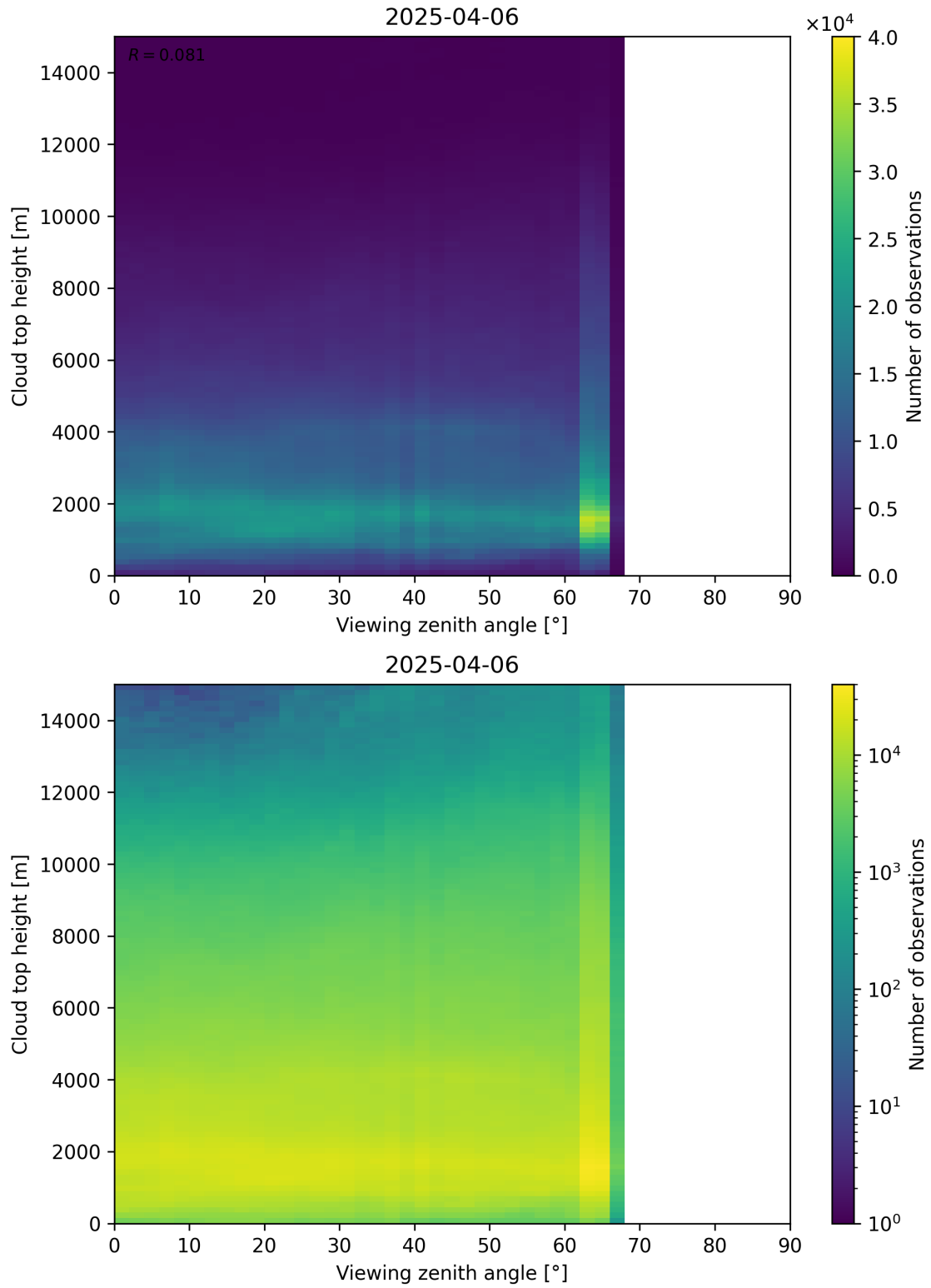
Figure 112: Scatter density plot of “Viewing zenith angle” against “Cloud top height” for 2025-04-05 to 2025-04-07.
