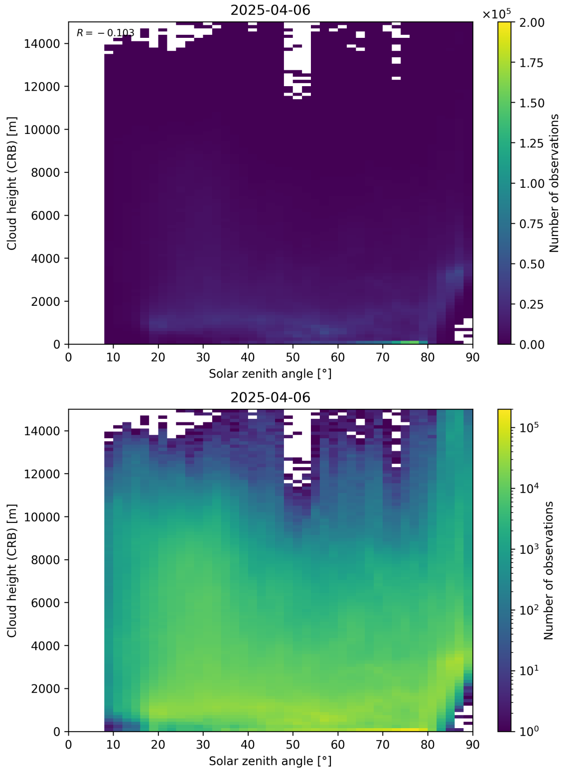
Figure 102: Scatter density plot of “Solar zenith angle” against “Cloud height (CRB)” for 2025-04-05 to 2025-04-07.
