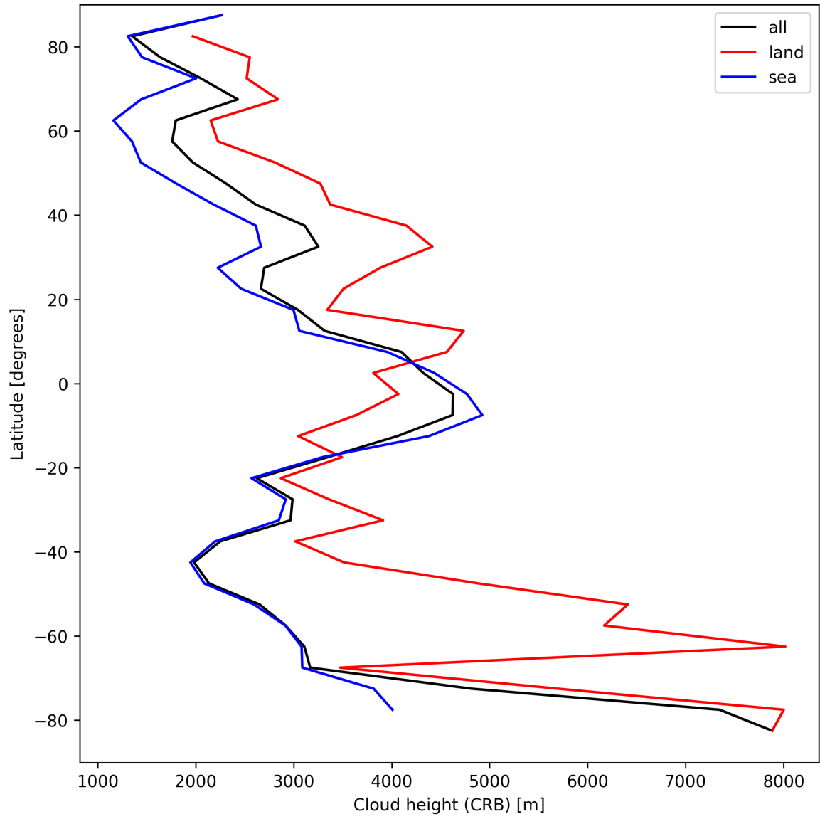
Figure 27: Zonal average of “Cloud height (CRB)” for 2025-04-05 to 2025-04-07.
