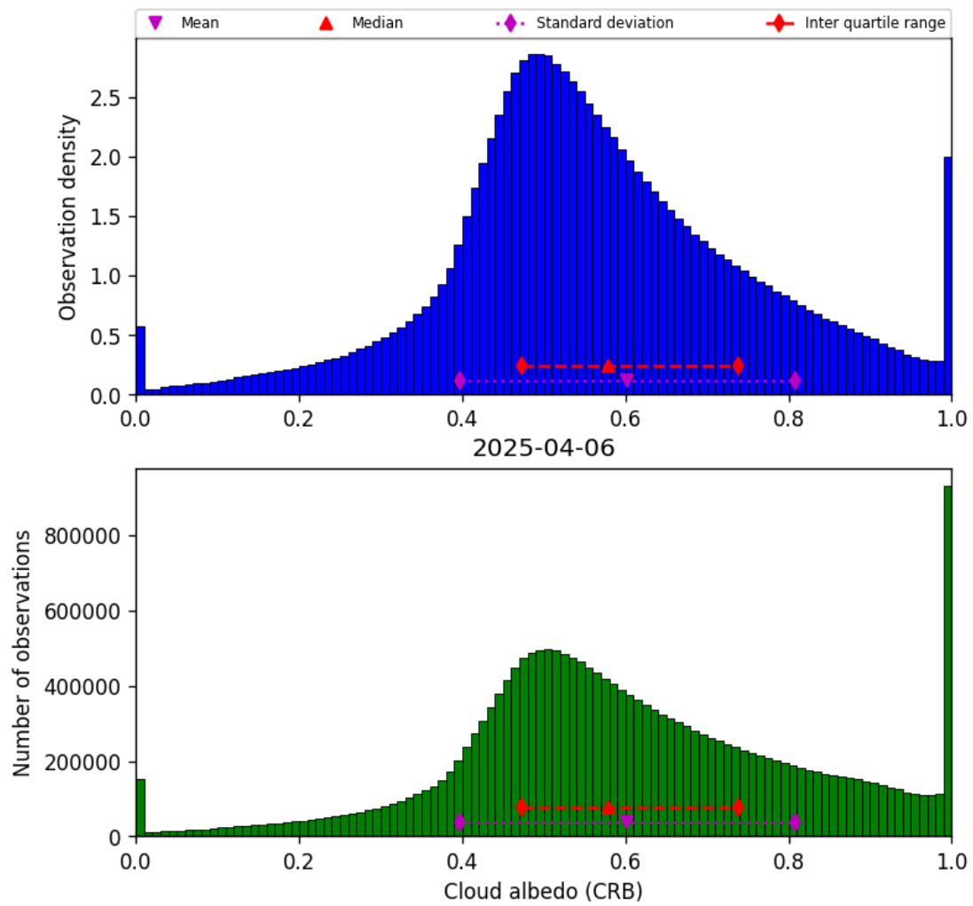
Figure 44: Histogram of “Cloud albedo (CRB)” for 2025-04-05 to 2025-04-07
