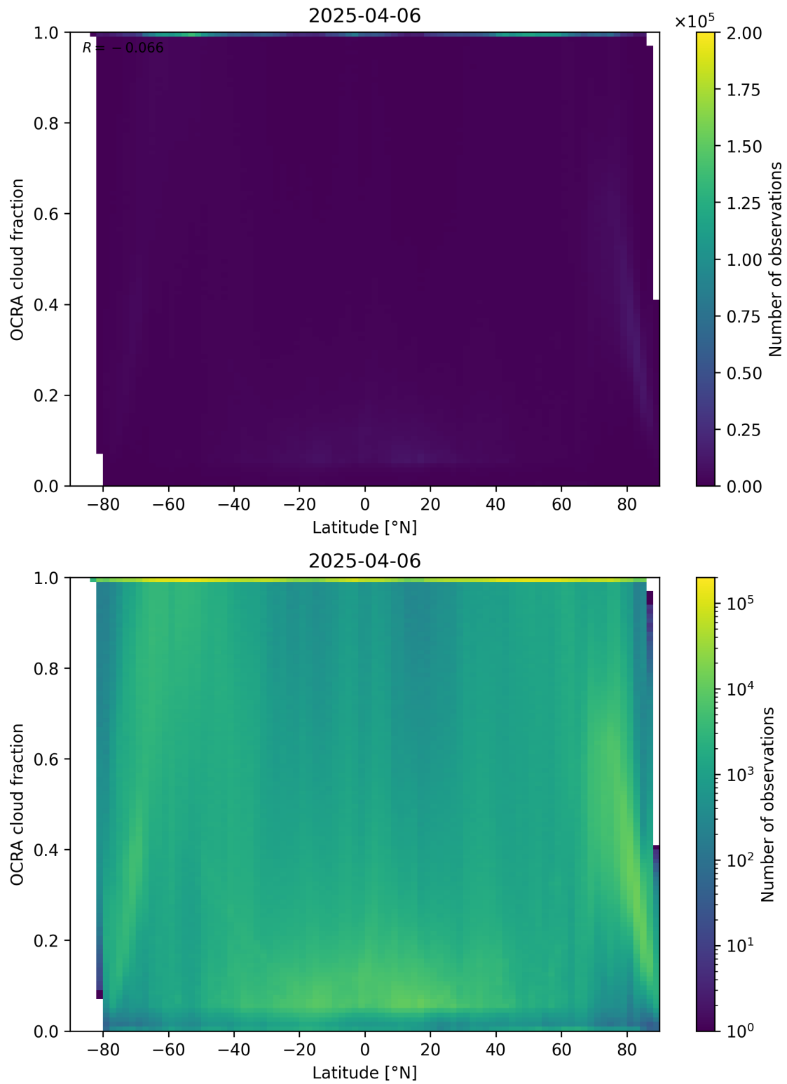
Figure 93: Scatter density plot of “Latitude” against “OCRA cloud fraction” for 2025-04-05 to 2025-04-07.
