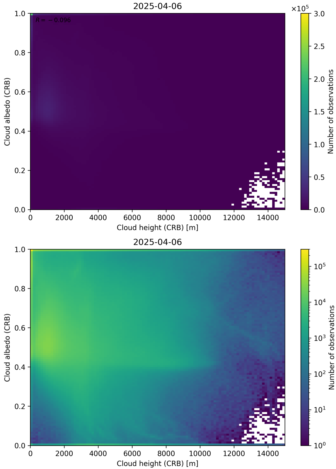
Figure 80: Scatter density plot of “Cloud height (CRB)” against “Cloud albedo (CRB)” for 2025-04-05 to 2025-04-07.
