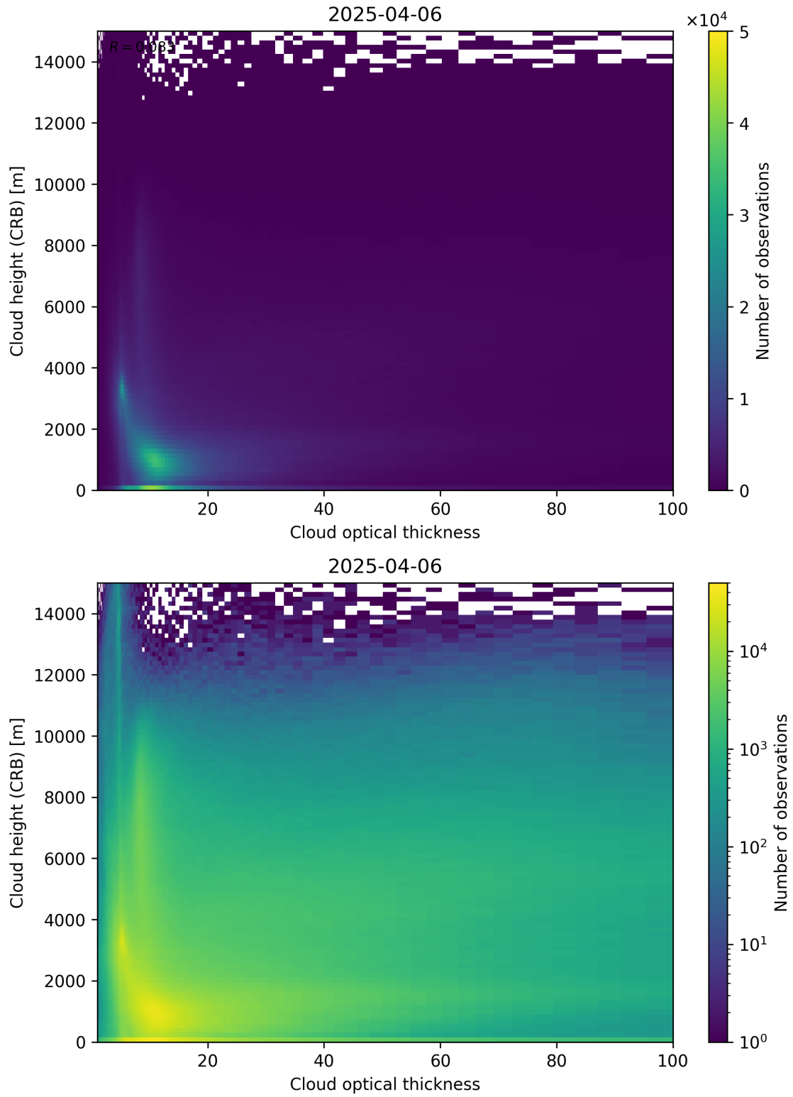
Figure 85: Scatter density plot of “Cloud optical thickness” against “Cloud height (CRB)” for 2025-04-05 to 2025-04-07.
