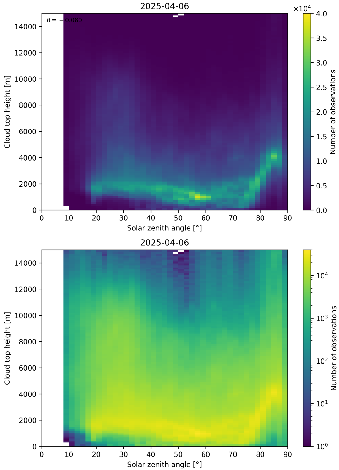
Figure 104: Scatter density plot of “Solar zenith angle” against “Cloud top height” for 2025-04-05 to 2025-04-07.
