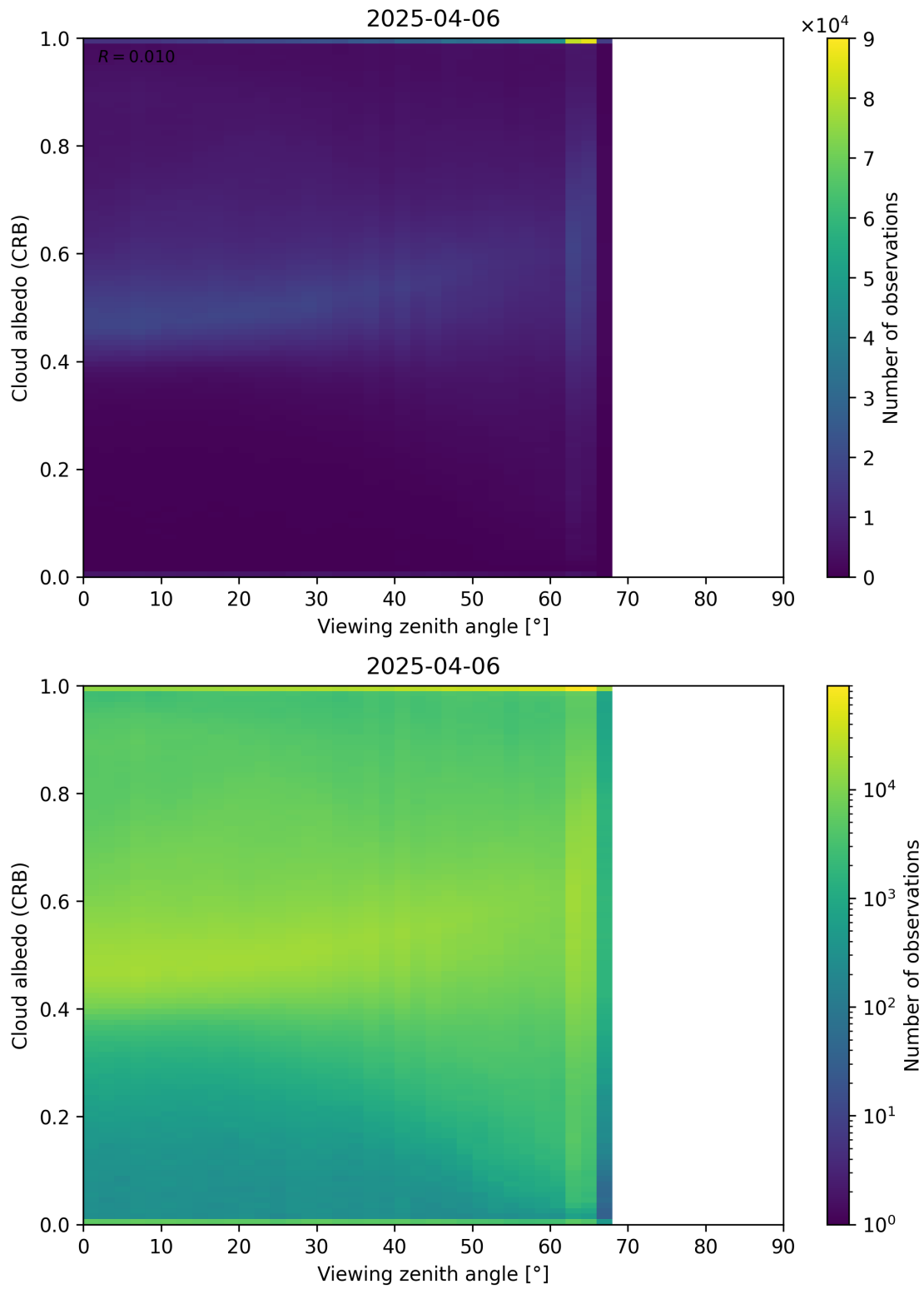
Figure 106: Scatter density plot of “Viewing zenith angle” against “Cloud albedo (CRB)” for 2025-04-05 to 2025-04-07.
