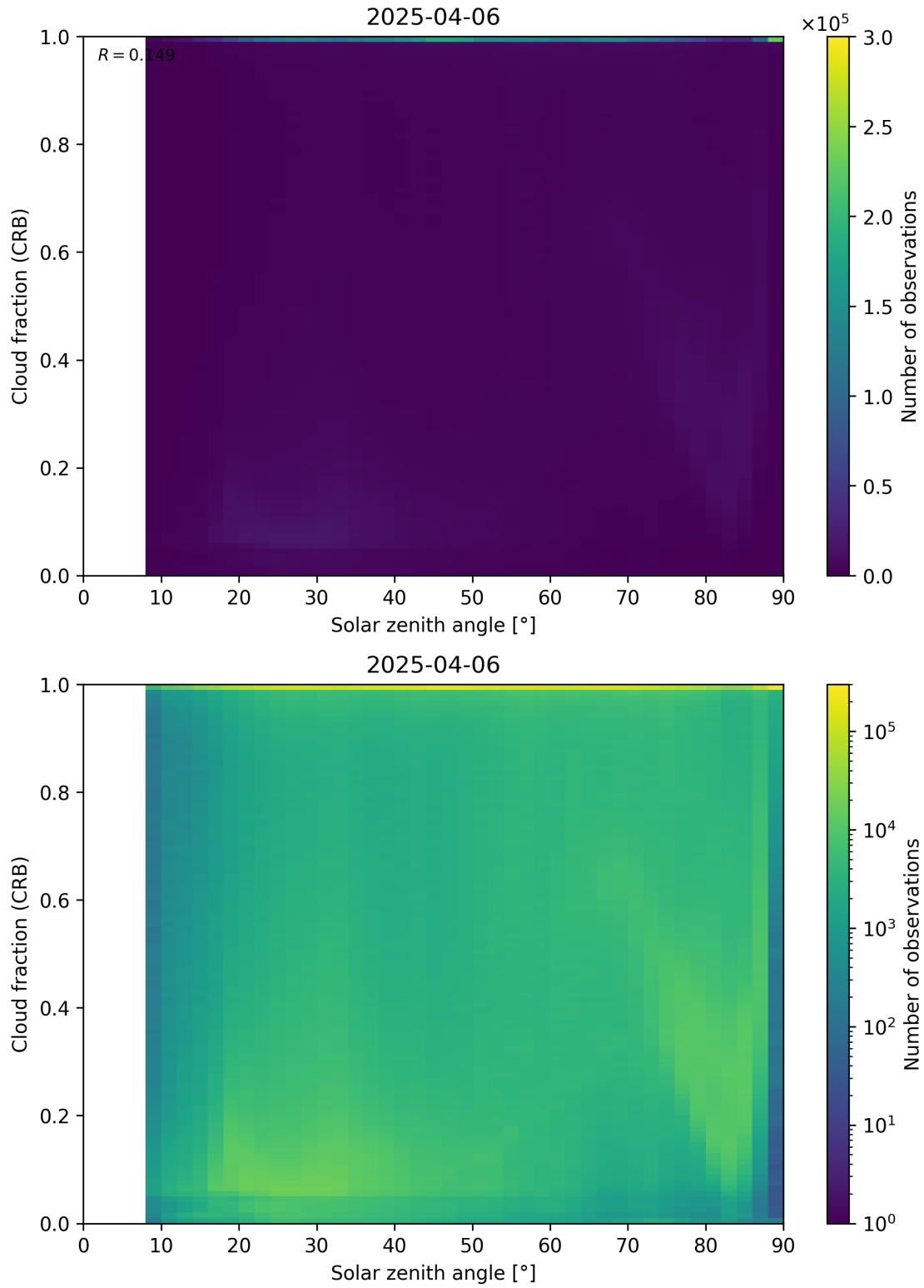
Figure 101: Scatter density plot of “Solar zenith angle” against “Cloud fraction (CRB)” for 2025-04-05 to 2025-04-07.
