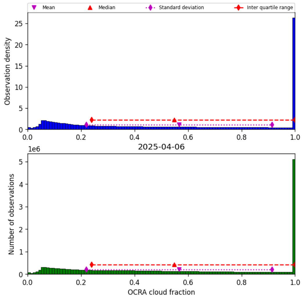
Figure 50: Histogram of “OCRA cloud fraction” for 2025-04-05 to 2025-04-07
