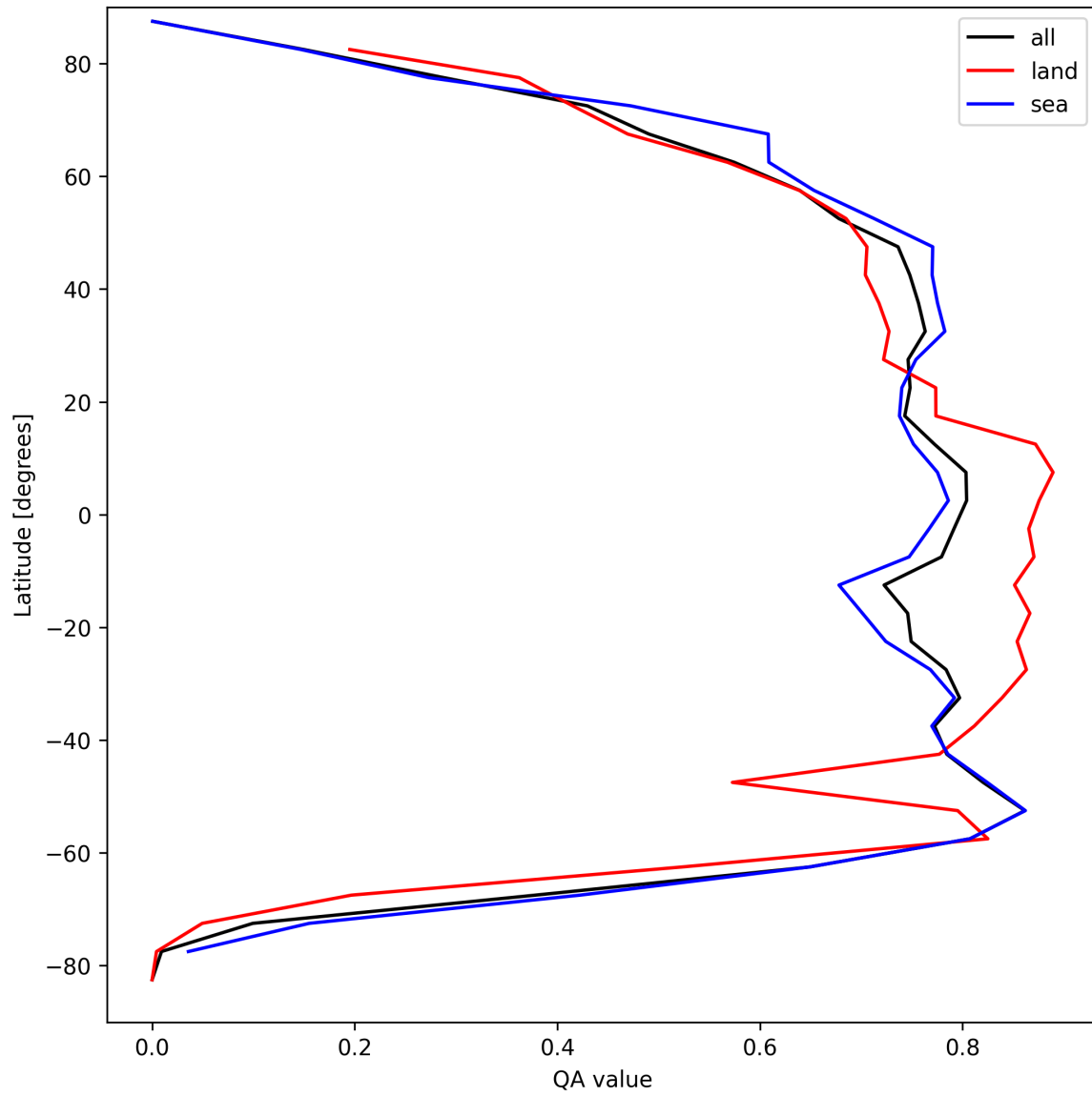
Figure 22: Zonal average of “QA value” for 2025-04-05 to 2025-04-07.
