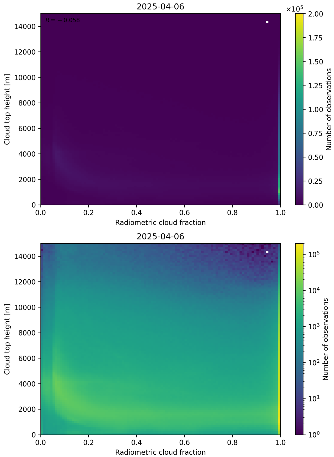
Figure 76: Scatter density plot of “Radiometric cloud fraction” against “Cloud top height” for 2025-04-05 to 2025-04-07.
