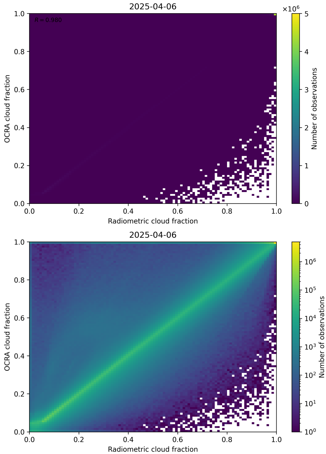
Figure 72: Scatter density plot of “Radiometric cloud fraction” against “OCRA cloud fraction” for 2025-04-05 to 2025-04-07.
