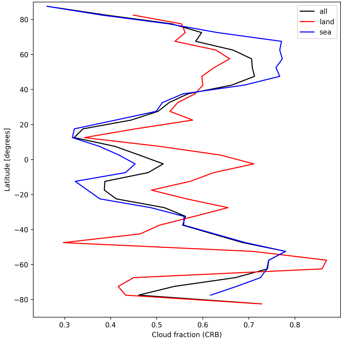
Figure 26: Zonal average of “Cloud fraction (CRB)” for 2025-04-05 to 2025-04-07.
