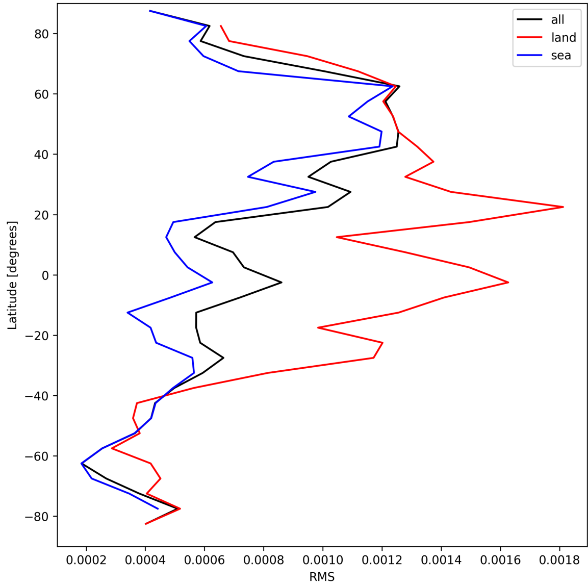
Figure 31: Zonal average of “RMS” for 2025-04-05 to 2025-04-07.
