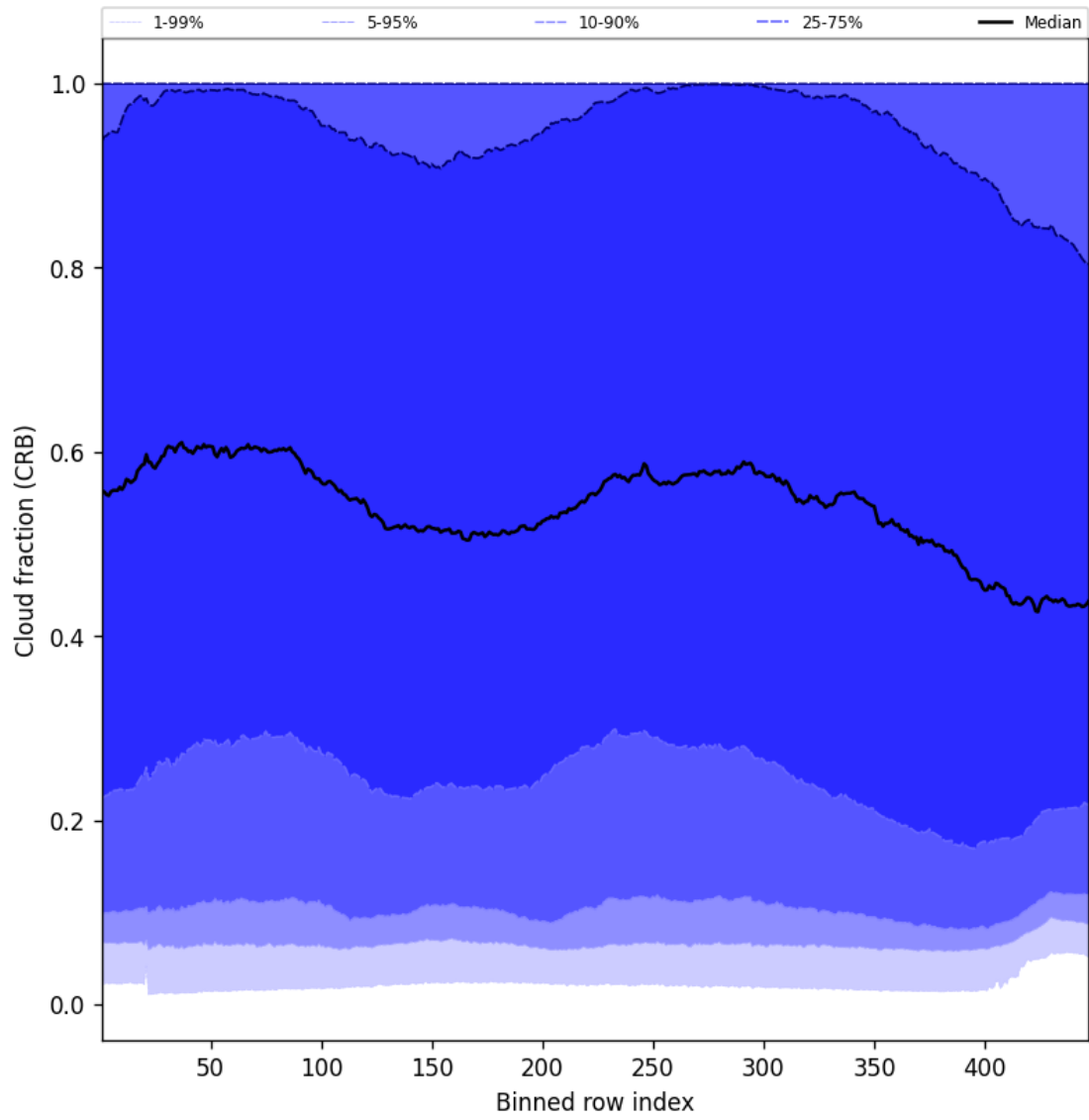
Figure 58: Along track statistics of “Cloud fraction (CRB)” for 2025-04-05 to 2025-04-07
