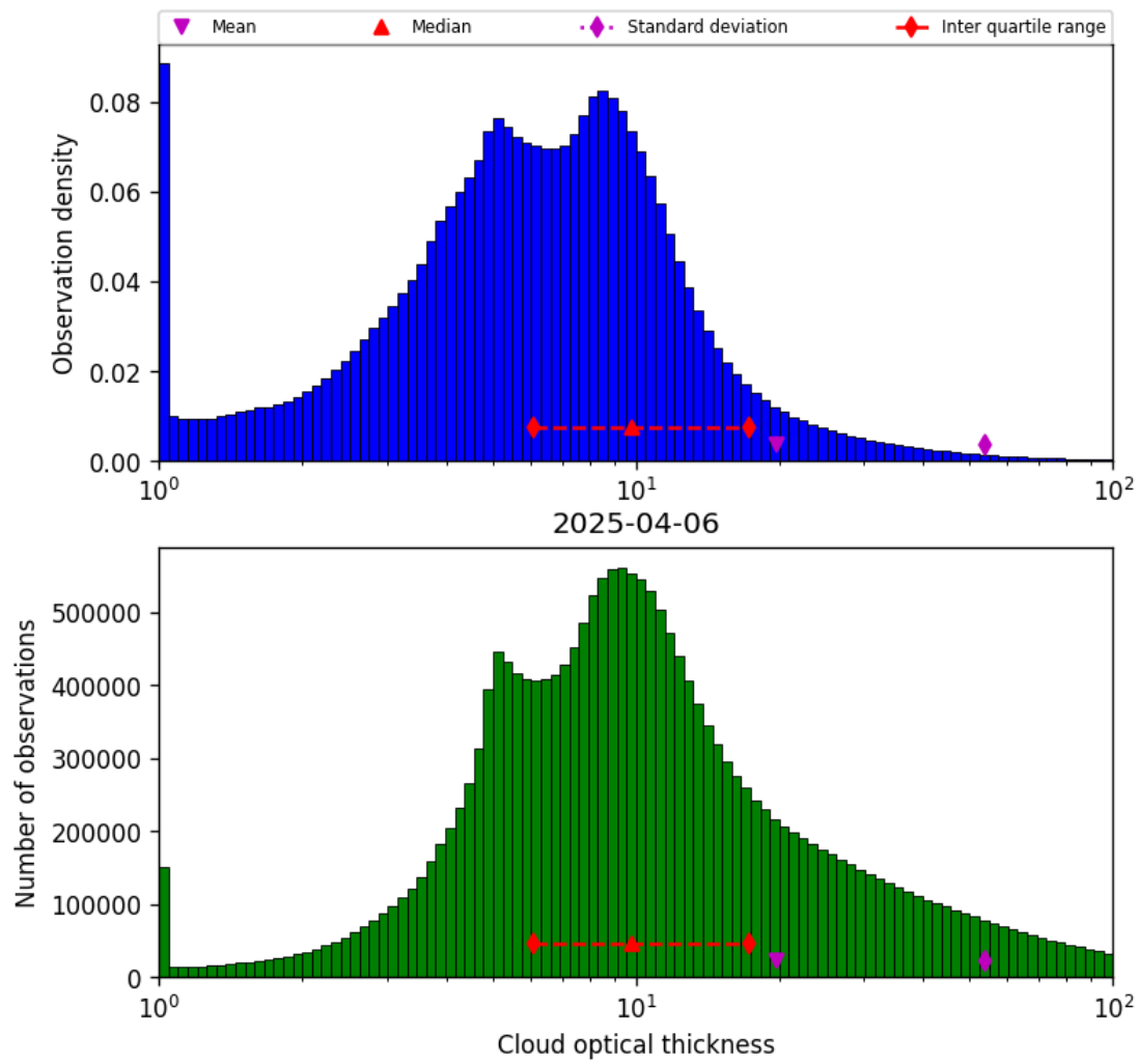
Figure 41: Histogram of “Cloud optical thickness” for 2025-04-05 to 2025-04-07
