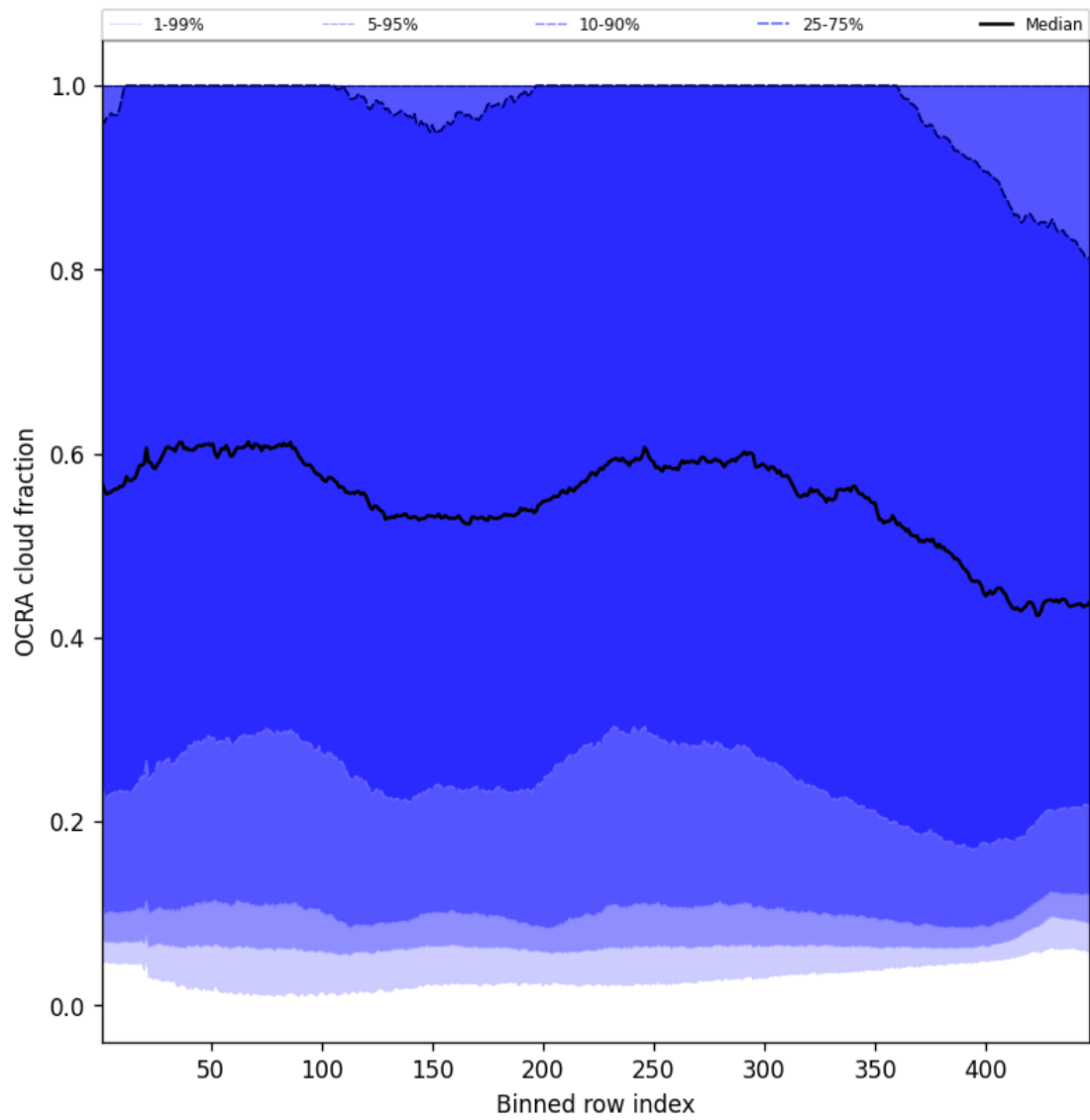
Figure 66: Along track statistics of “OCRA cloud fraction” for 2025-04-05 to 2025-04-07
