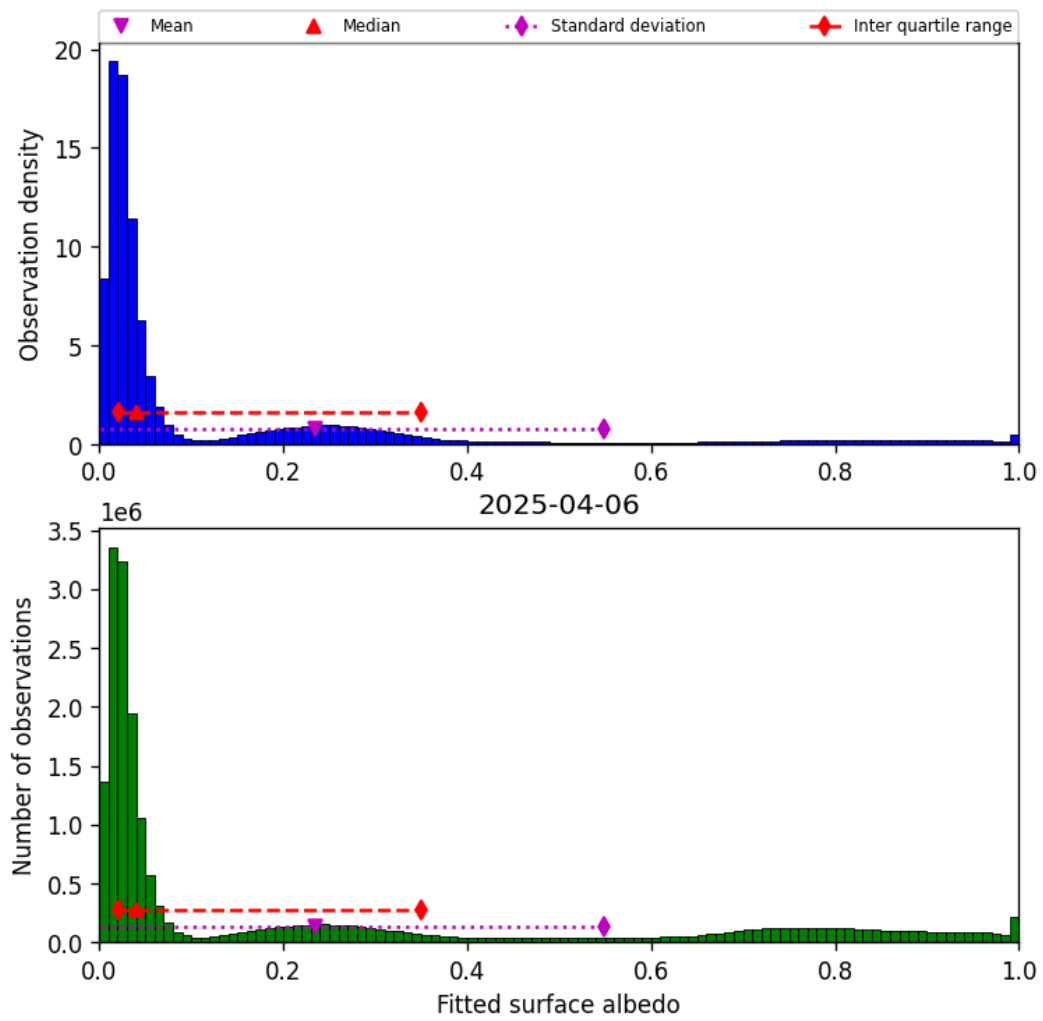
Figure 45: Histogram of “Fitted surface albedo” for 2025-04-05 to 2025-04-07
