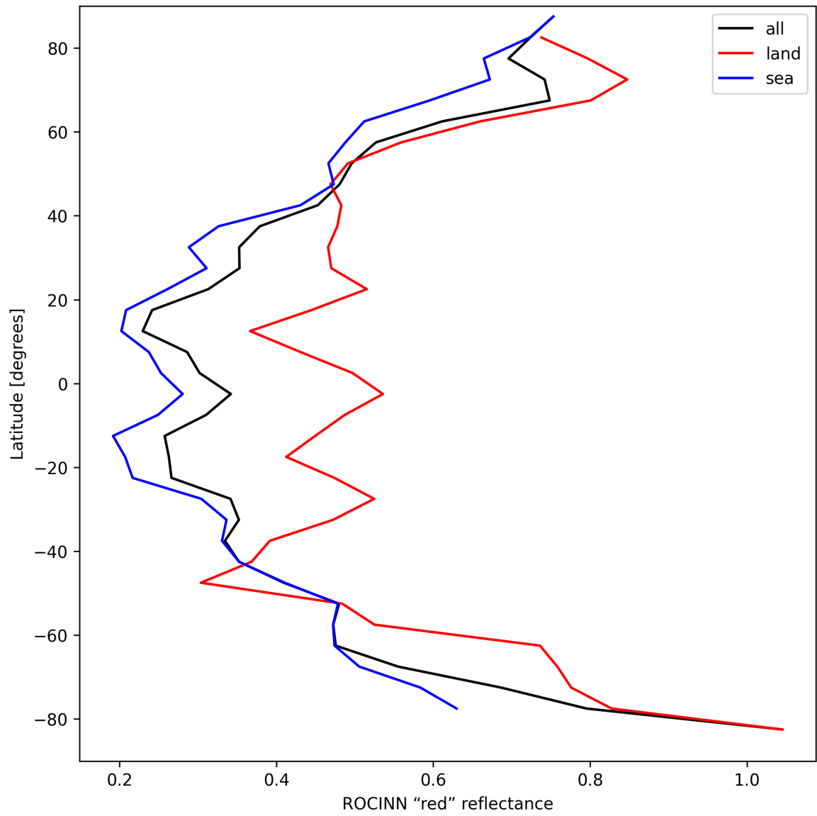
Figure 37: Zonal average of "ROCINN "red" reflectance" for 2025-04-05 to 2025-04-07.
