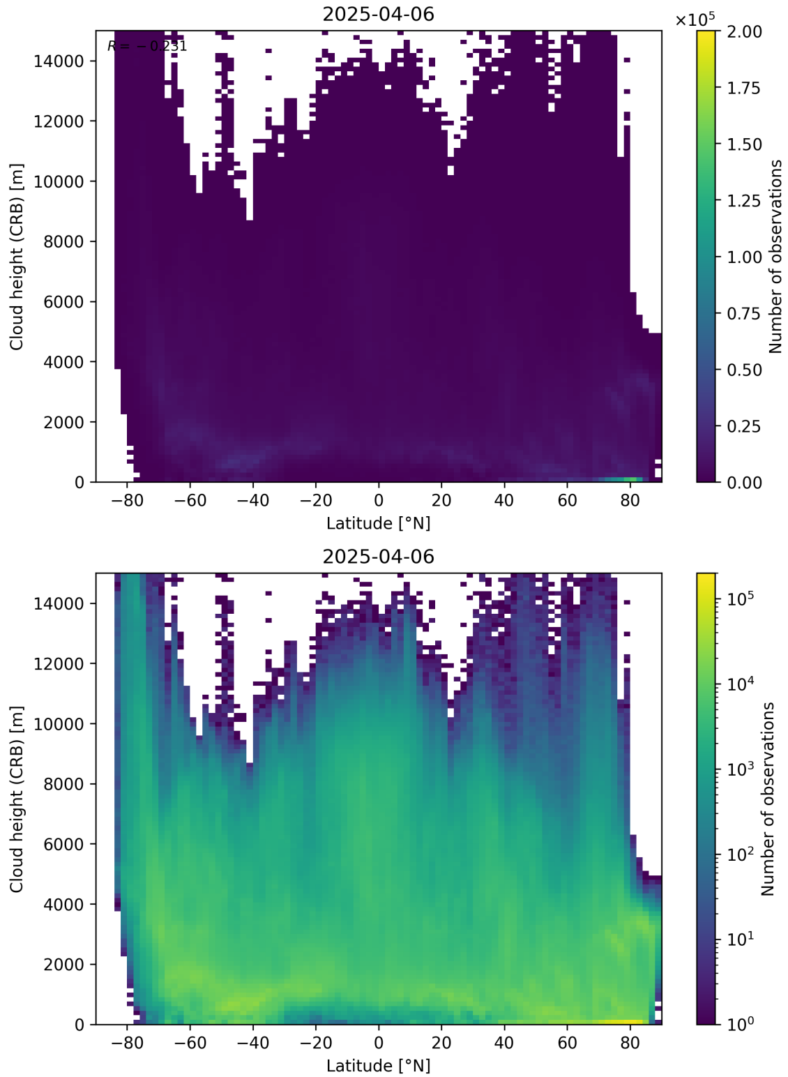
Figure 95: Scatter density plot of “Latitude” against “Cloud height (CRB)” for 2025-04-05 to 2025-04-07.
