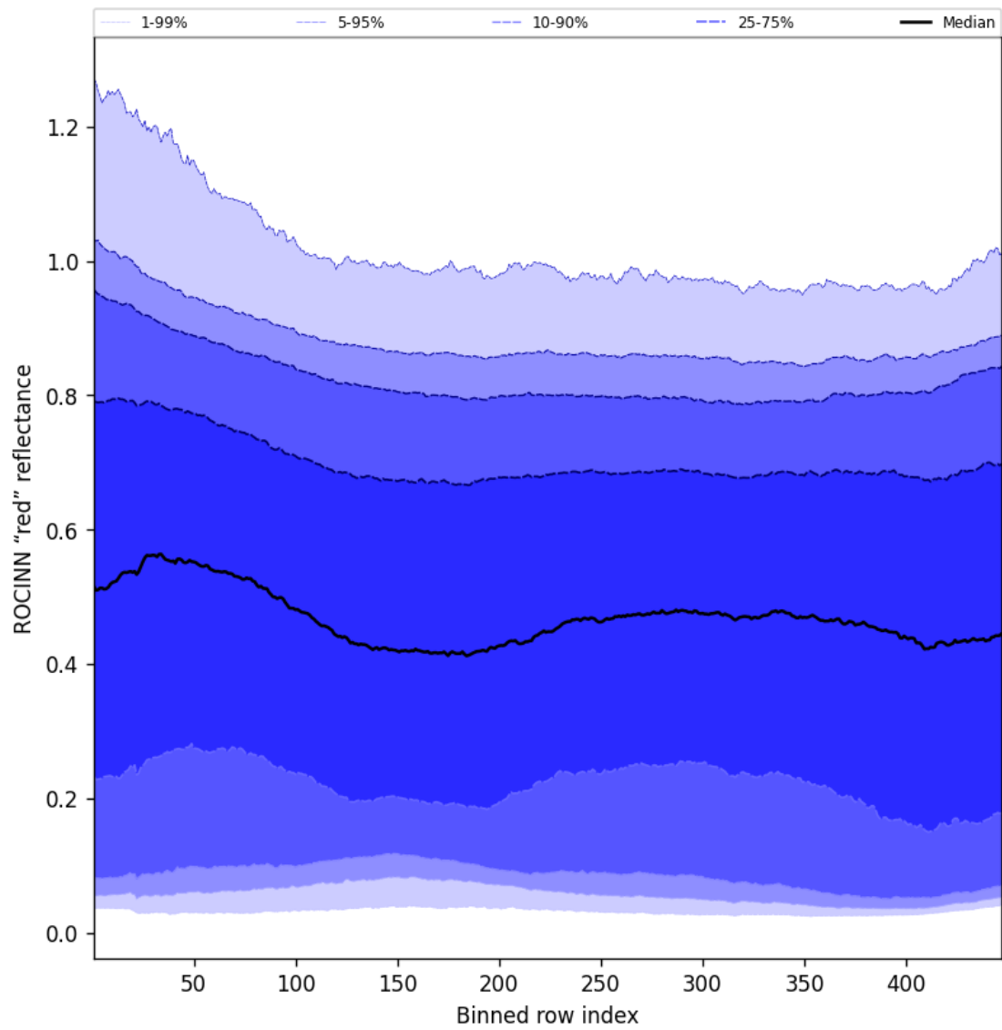
Figure 69: Along track statistics of "ROCINN "red" reflectance" for 2025-04-05 to 2025-04-07
