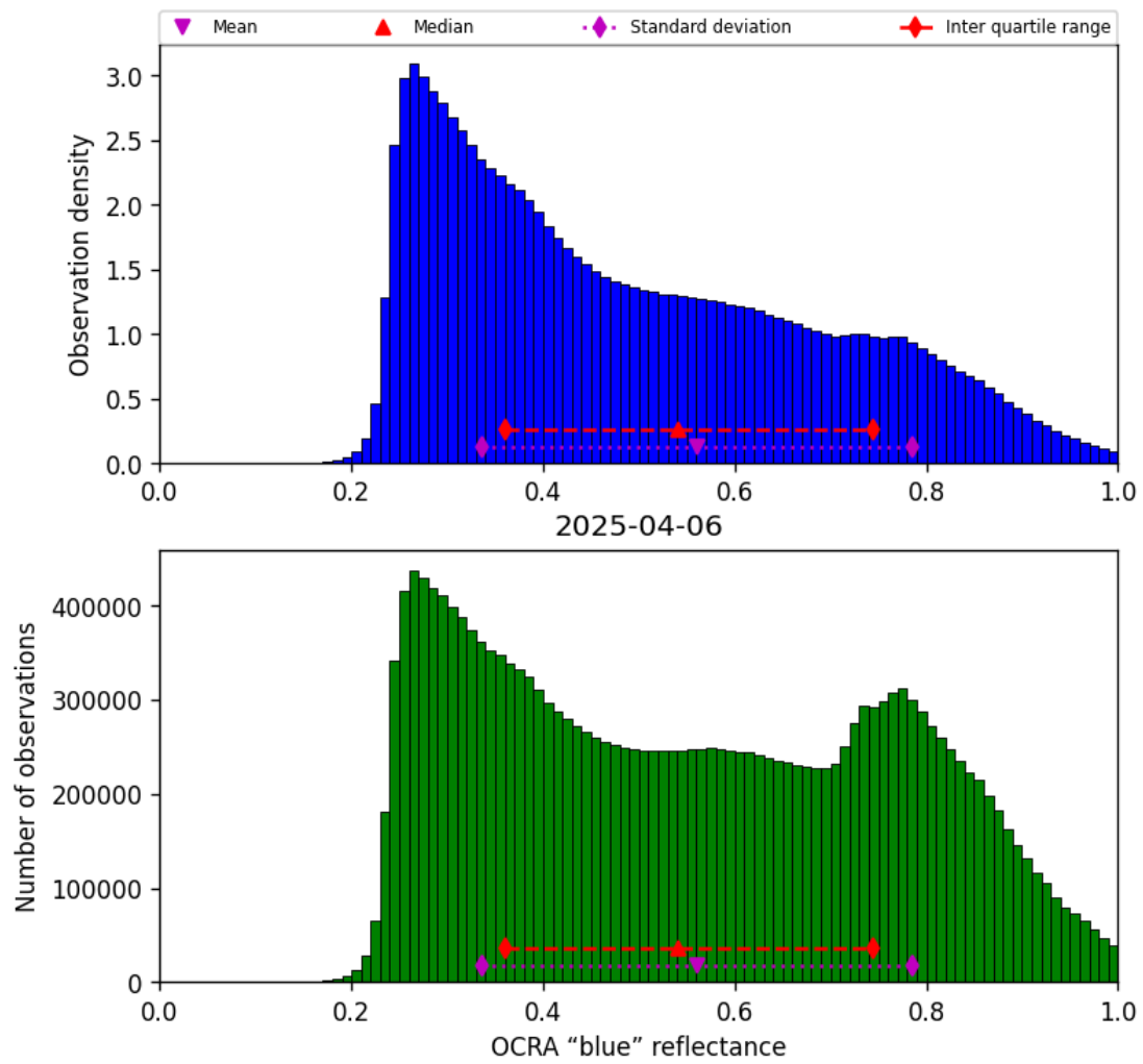
Figure 51: Histogram of “OCRA “blue” reflectance” for 2025-04-05 to 2025-04-07
