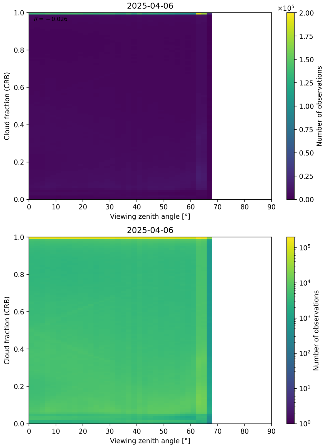
Figure 109: Scatter density plot of “Viewing zenith angle” against “Cloud fraction (CRB)” for 2025-04-05 to 2025-04-07.
