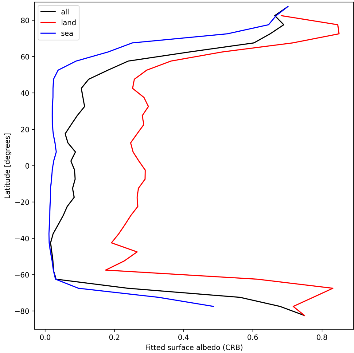
Figure 30: Zonal average of “Fitted surface albedo (CRB)” for 2025-04-05 to 2025-04-07.
