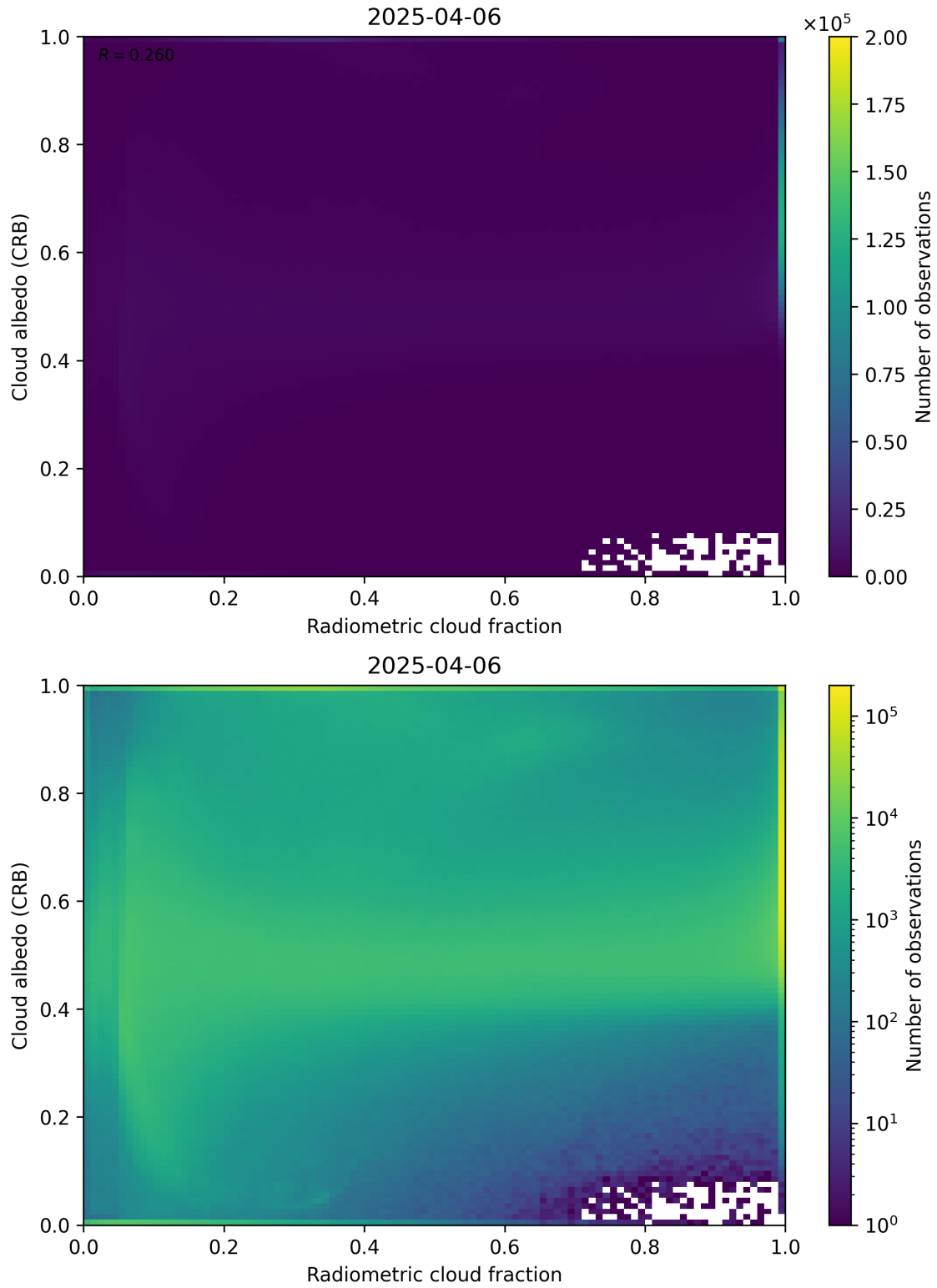
Figure 71: Scatter density plot of “Radiometric cloud fraction” against “Cloud albedo (CRB)” for 2025-04-05 to 2025-04-07.
