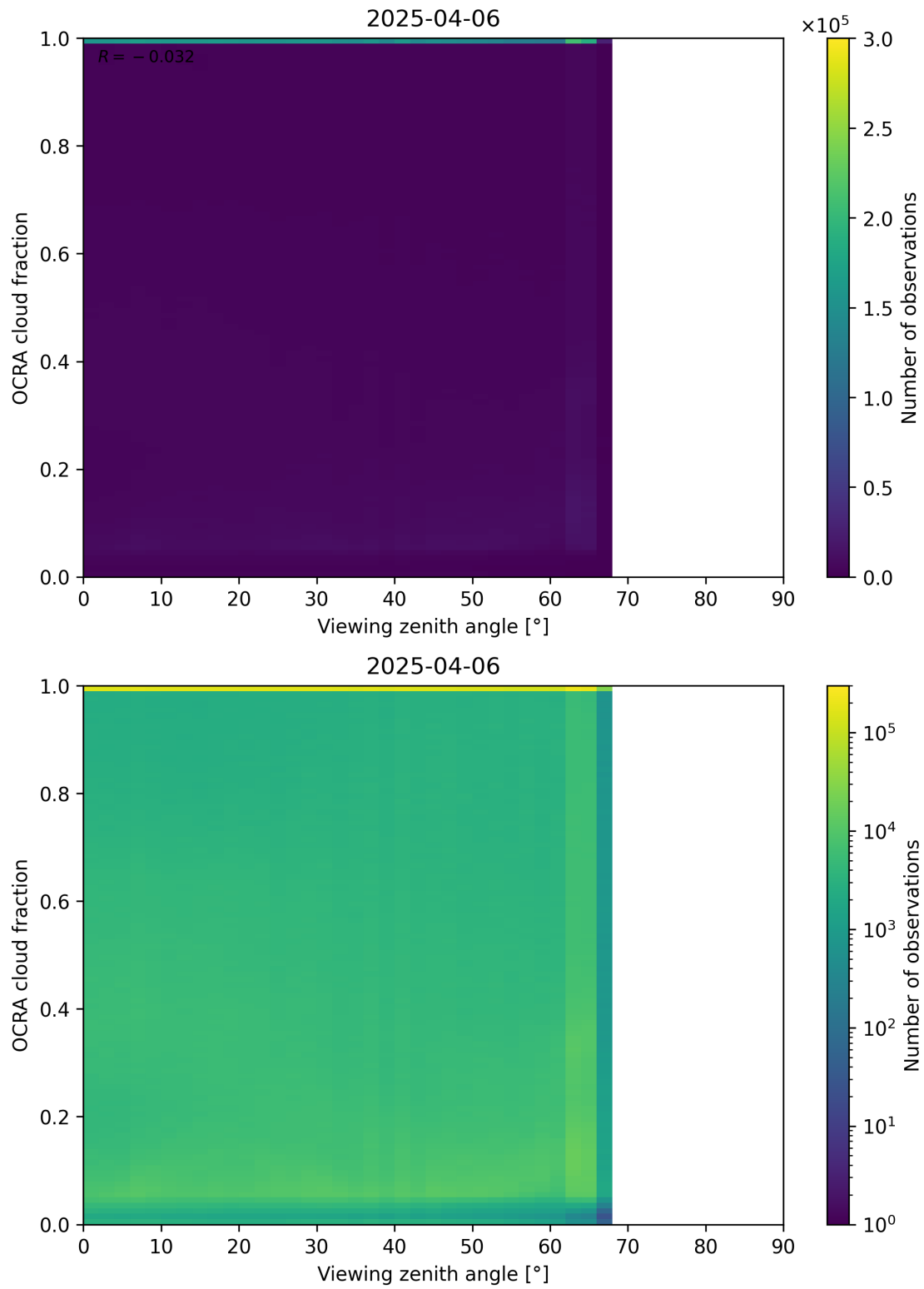
Figure 108: Scatter density plot of “Viewing zenith angle” against “OCRA cloud fraction” for 2025-04-05 to 2025-04-07.
