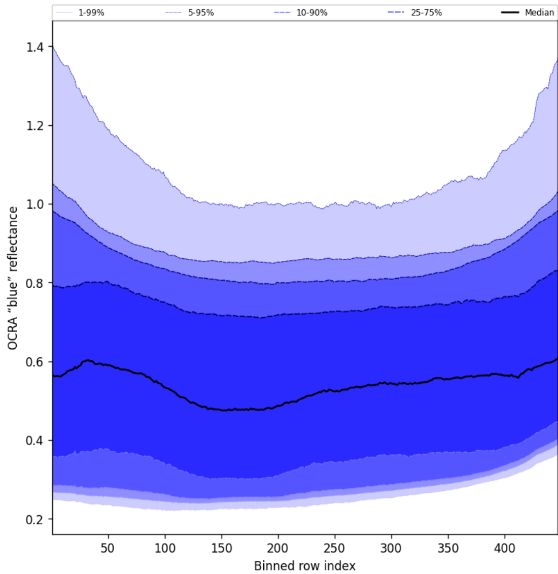
Figure 67: Along track statistics of “OCRA “blue” reflectance” for 2025-04-05 to 2025-04-07
