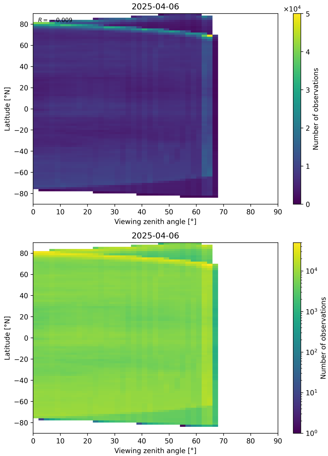
Figure 113: Scatter density plot of “Viewing zenith angle” against “Latitude” for 2025-04-05 to 2025-04-07.
