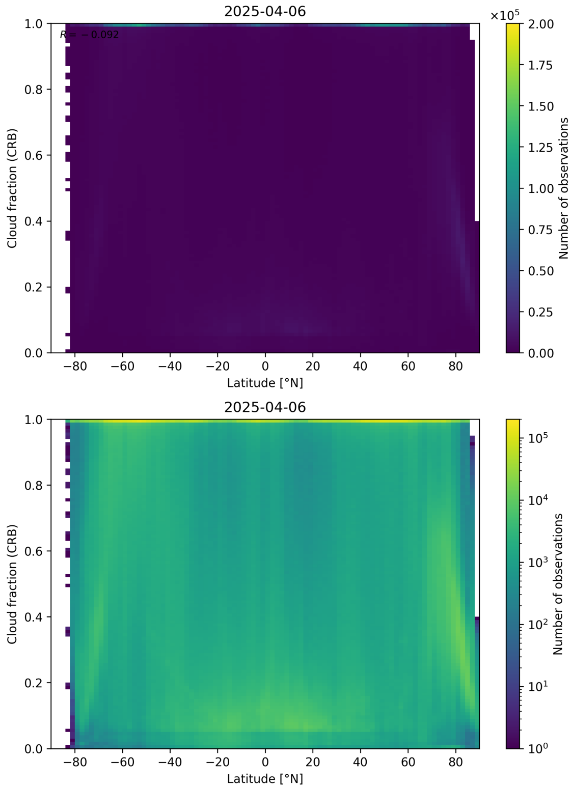
Figure 94: Scatter density plot of “Latitude” against “Cloud fraction (CRB)” for 2025-04-05 to 2025-04-07.
