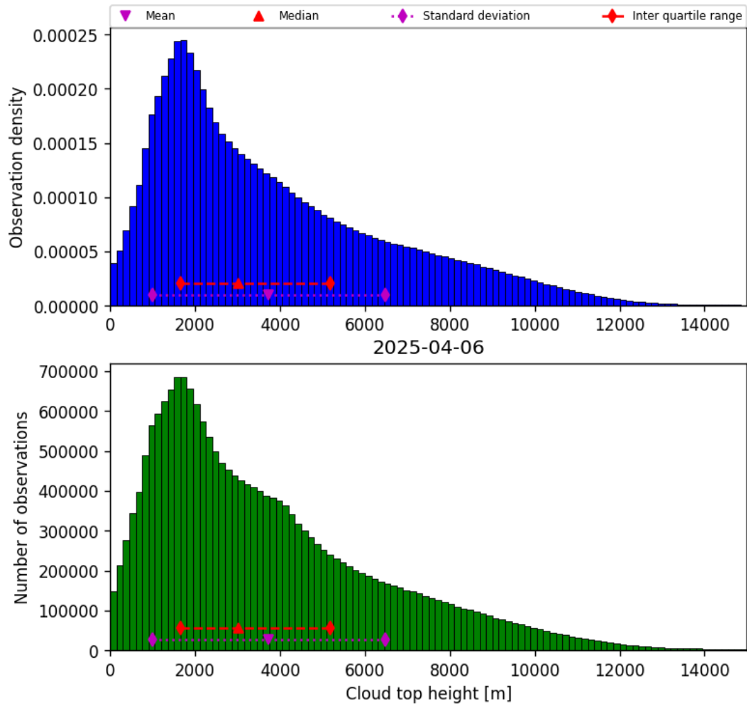
Figure 40: Histogram of “Cloud top height” for 2025-04-05 to 2025-04-07
