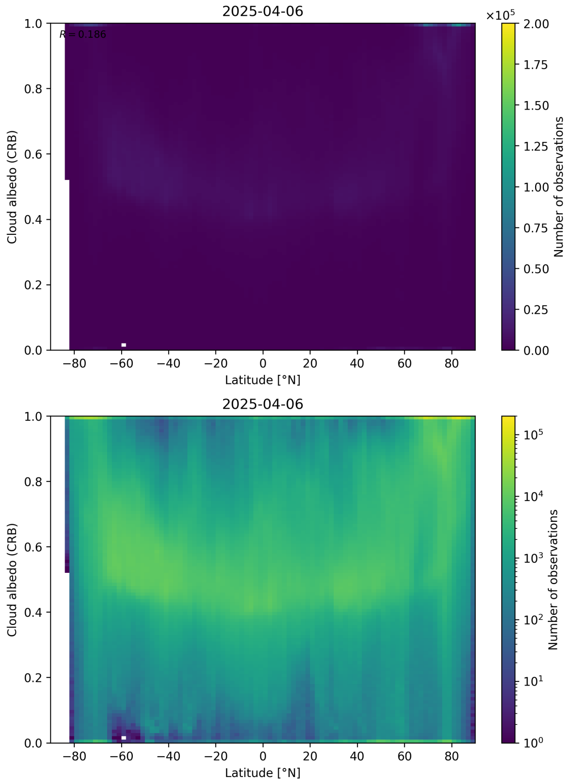
Figure 91: Scatter density plot of “Latitude” against “Cloud albedo (CRB)” for 2025-04-05 to 2025-04-07.
