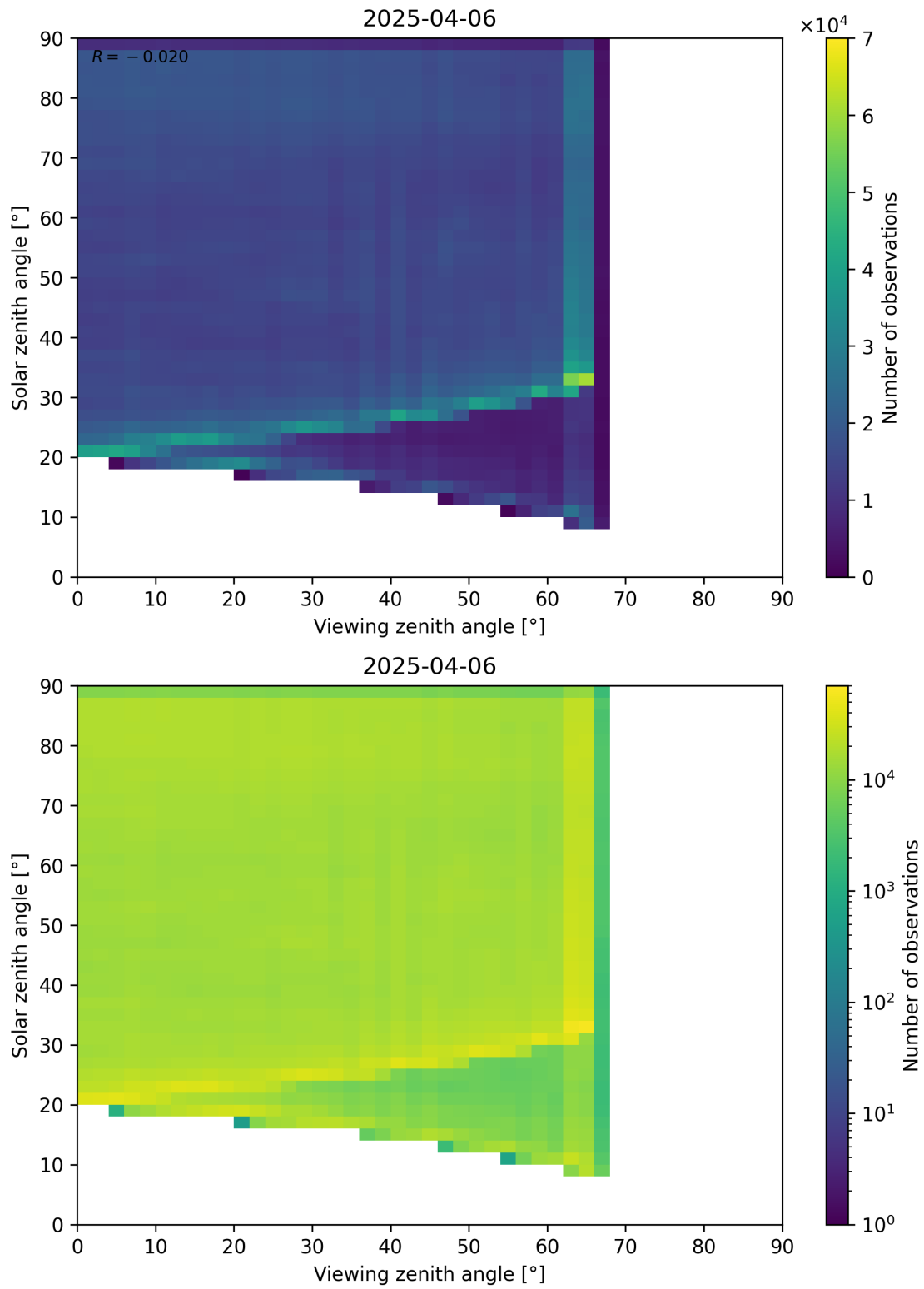
Figure 114: Scatter density plot of “Viewing zenith angle” against “Solar zenith angle” for 2025-04-05 to 2025-04-07.
