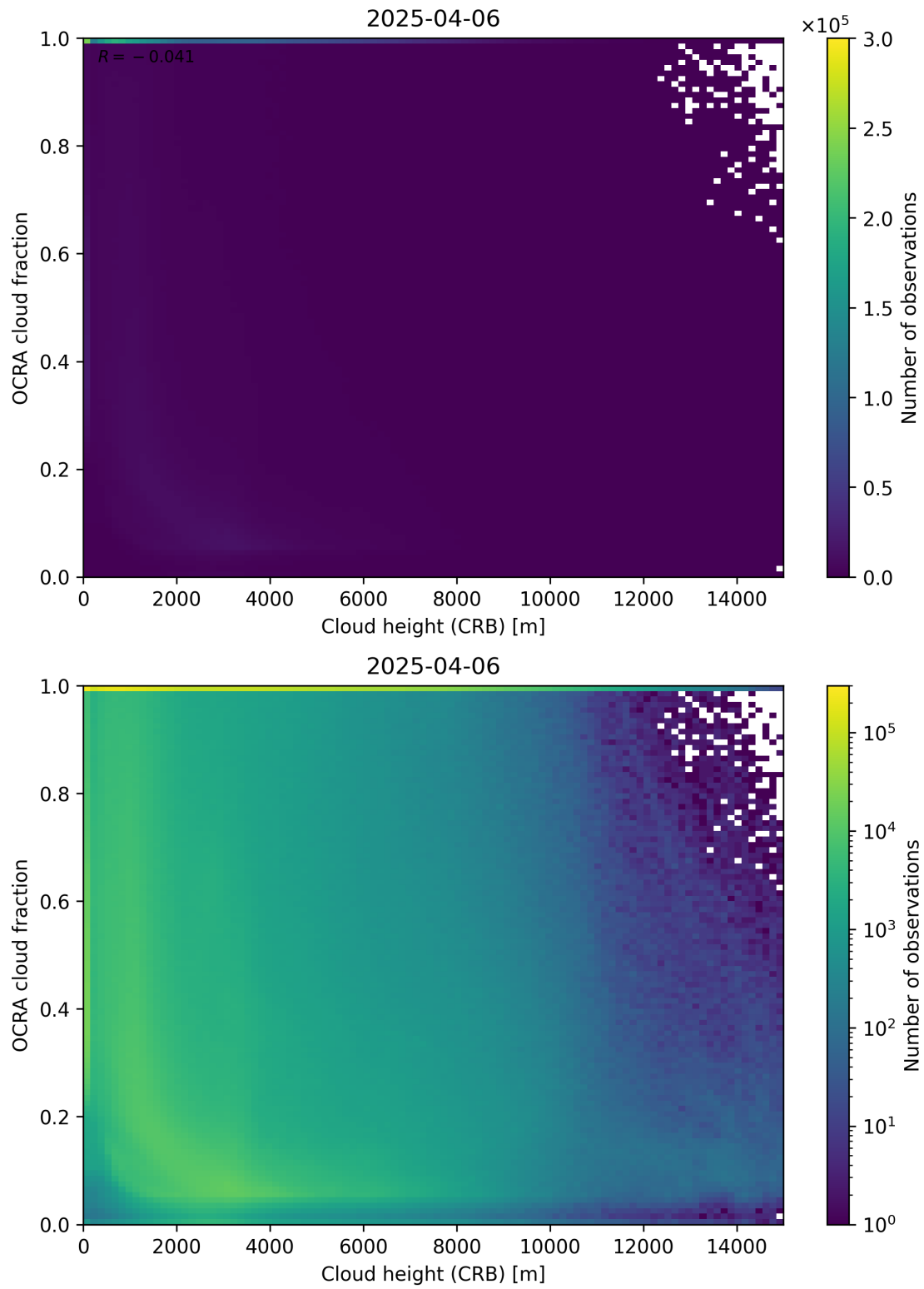
Figure 81: Scatter density plot of “Cloud height (CRB)” against “OCRA cloud fraction” for 2025-04-05 to 2025-04-07.
