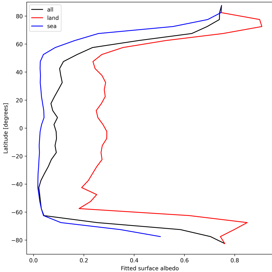
Figure 29: Zonal average of “Fitted surface albedo” for 2025-04-05 to 2025-04-07.
