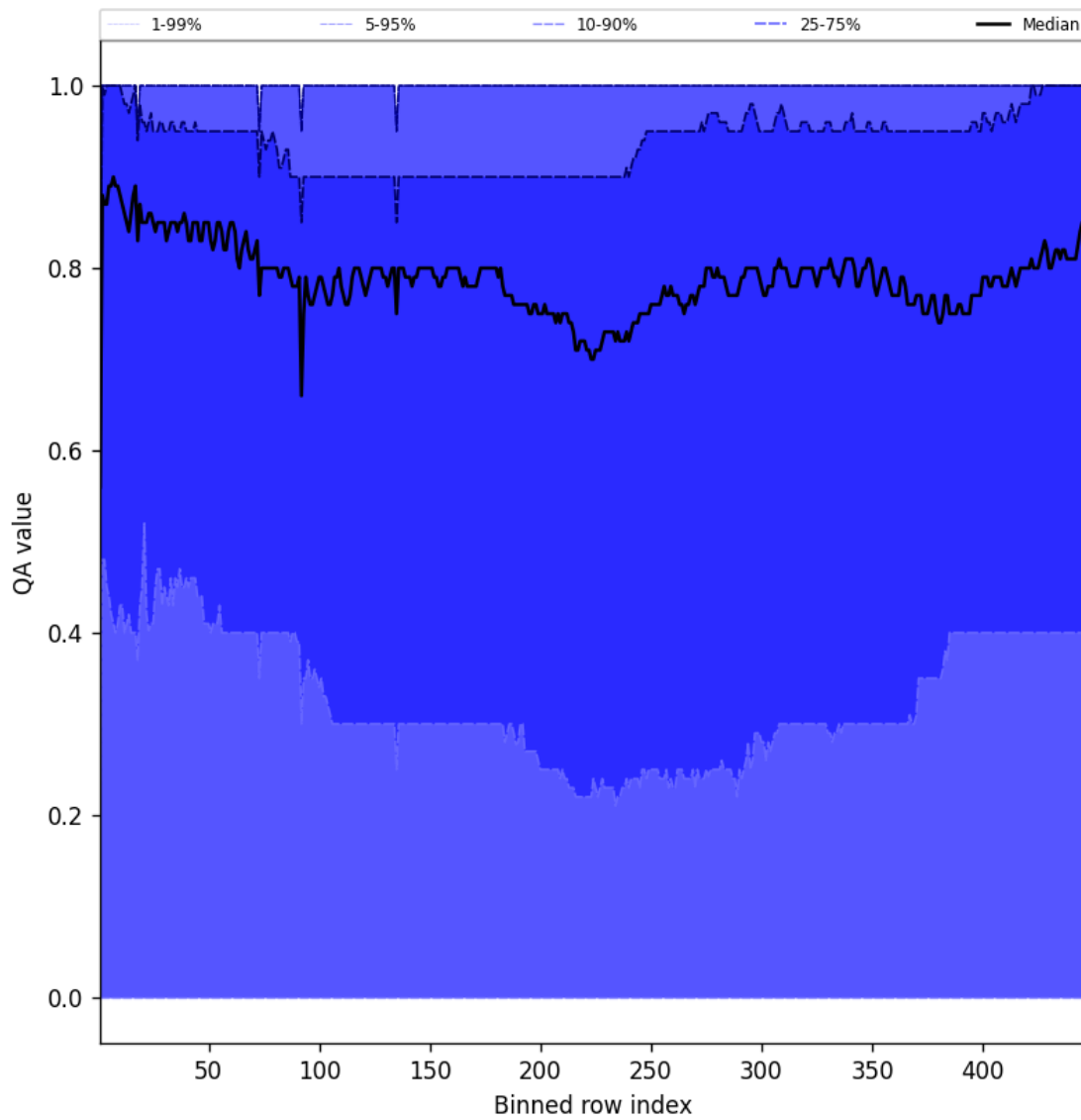
Figure 54: Along track statistics of “QA value” for 2025-04-05 to 2025-04-07
