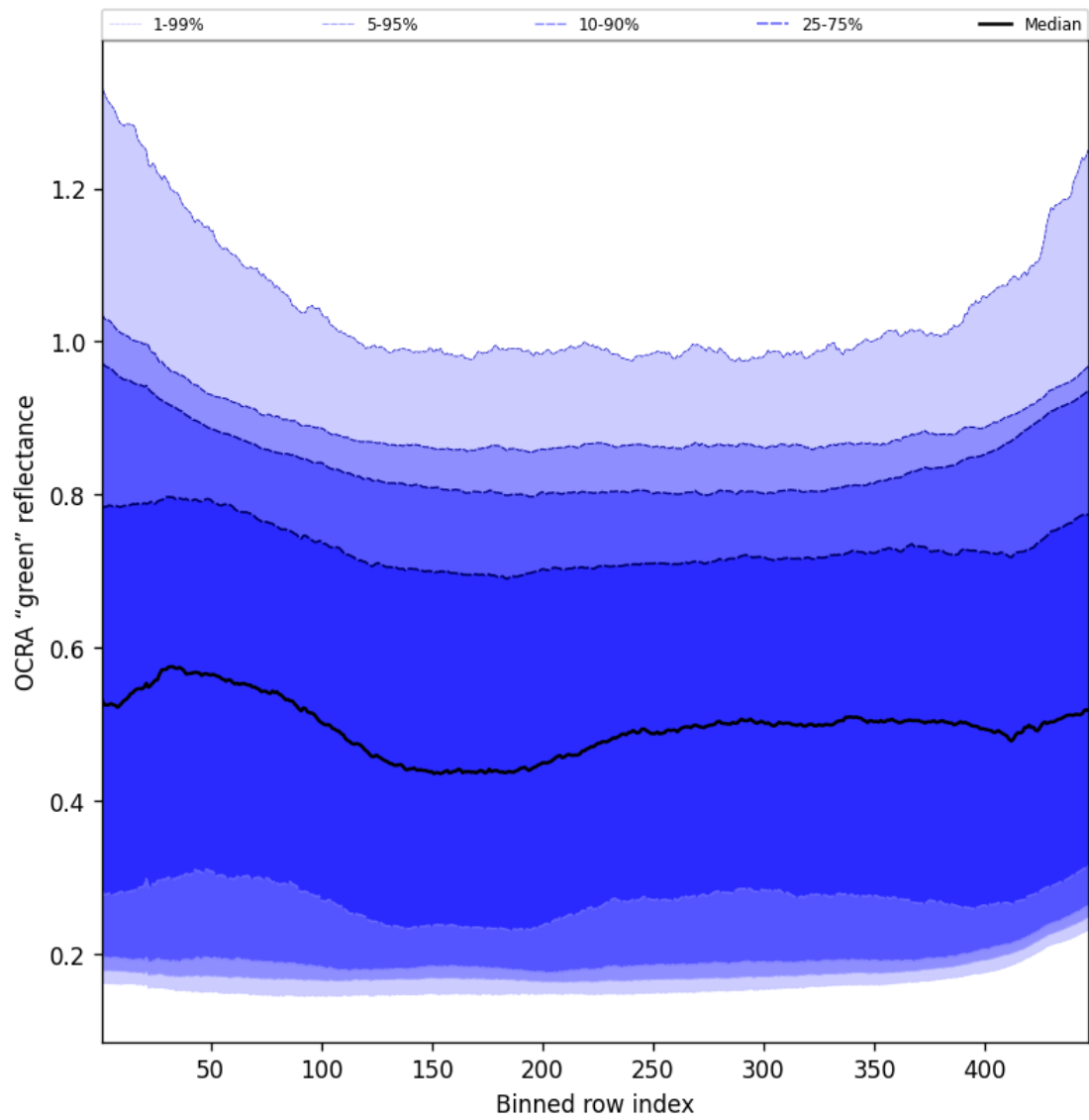
Figure 68: Along track statistics of "OCRA "green" reflectance" for 2025-04-05 to 2025-04-07
