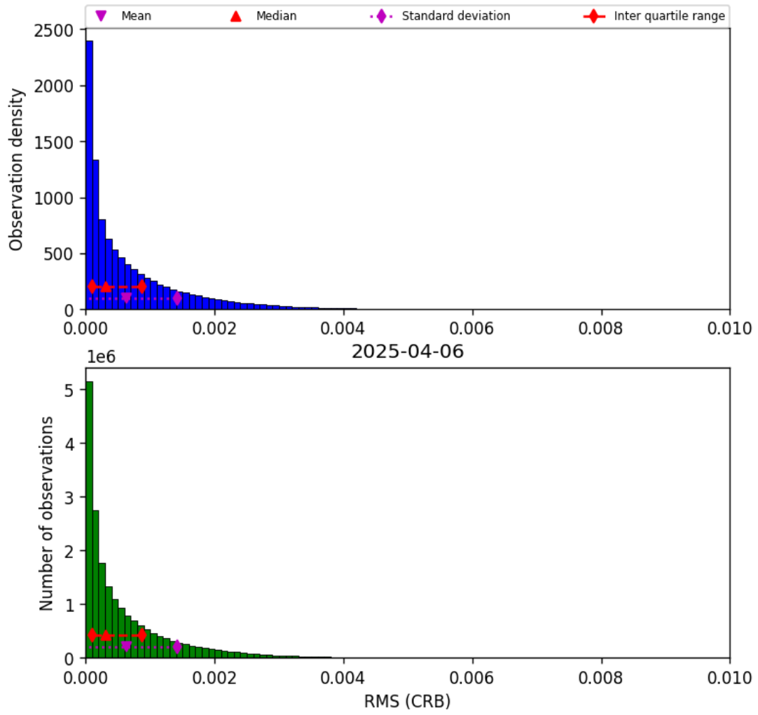
Figure 48: Histogram of “RMS (CRB)” for 2025-04-05 to 2025-04-07
