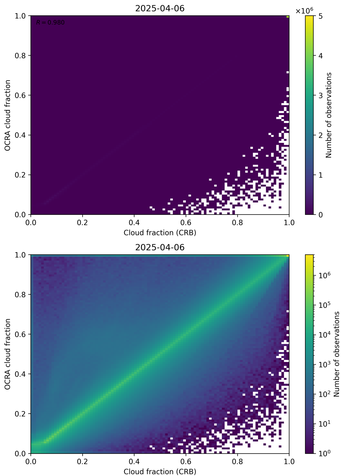
Figure 78: Scatter density plot of “Cloud fraction (CRB)” against “OCRA cloud fraction” for 2025-04-05 to 2025-04-07.
