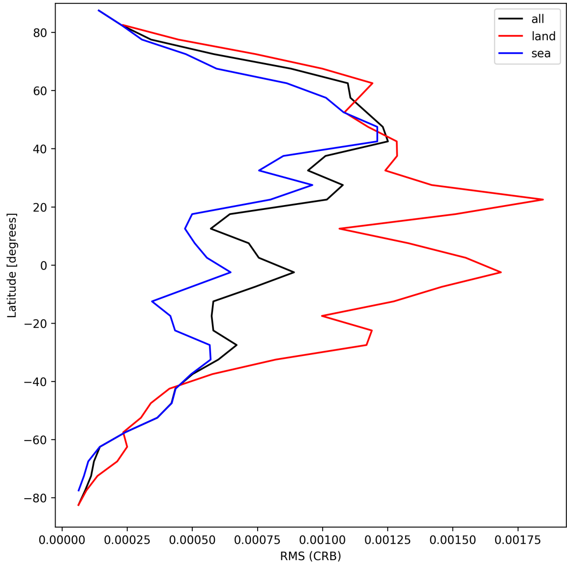
Figure 32: Zonal average of “RMS (CRB)” for 2025-04-05 to 2025-04-07.
