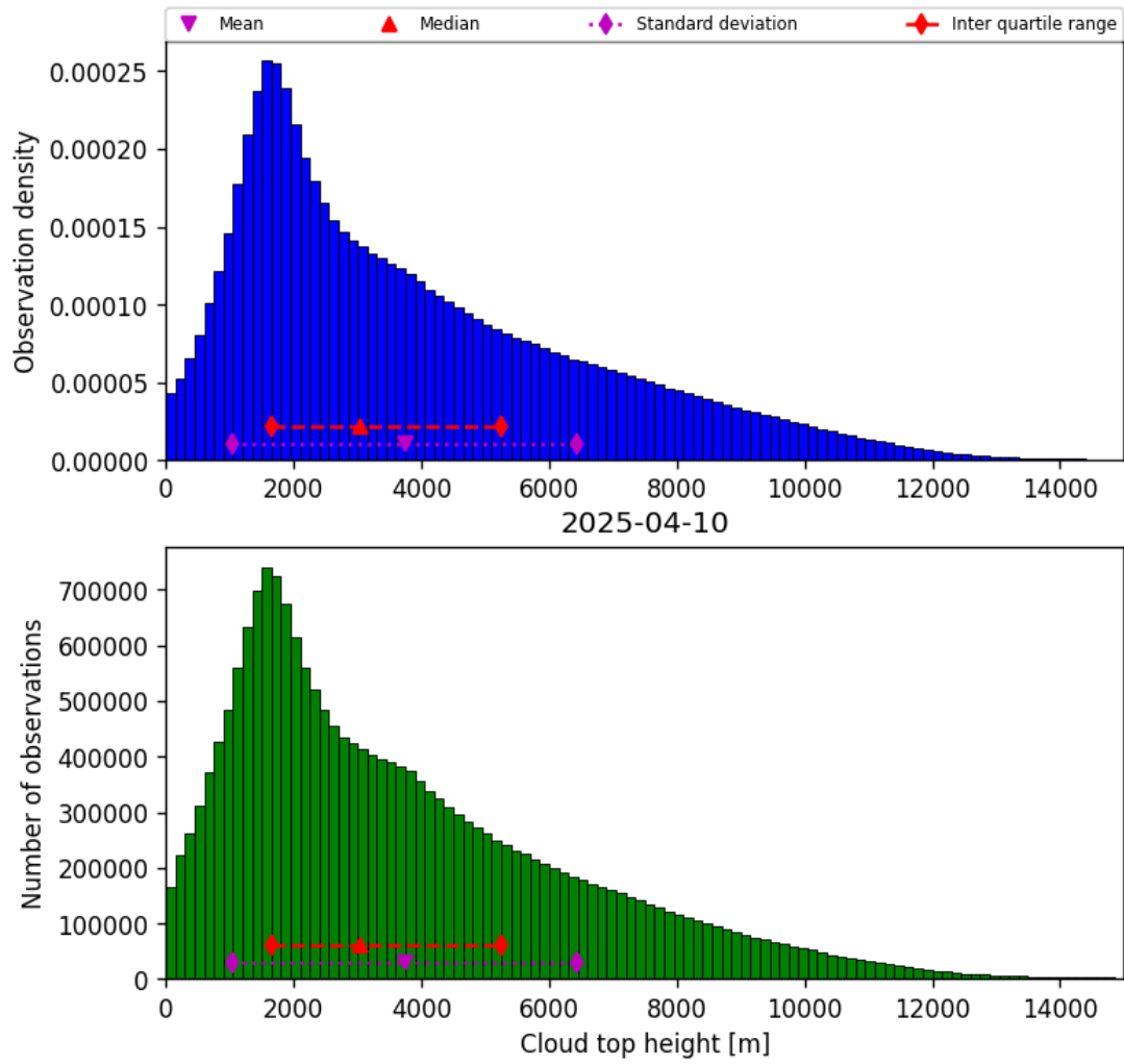
Figure 40: Histogram of “Cloud top height” for 2025-04-09 to 2025-04-11
