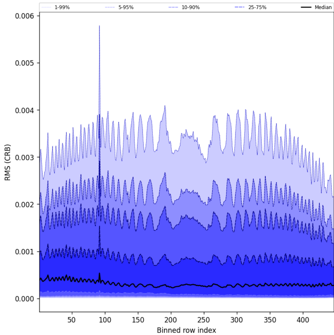
Figure 64: Along track statistics of “RMS (CRB)” for 2025-04-09 to 2025-04-11
