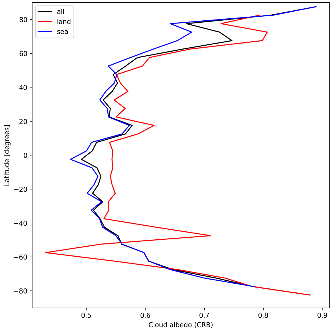
Figure 28: Zonal average of “Cloud albedo (CRB)” for 2025-04-09 to 2025-04-11.
