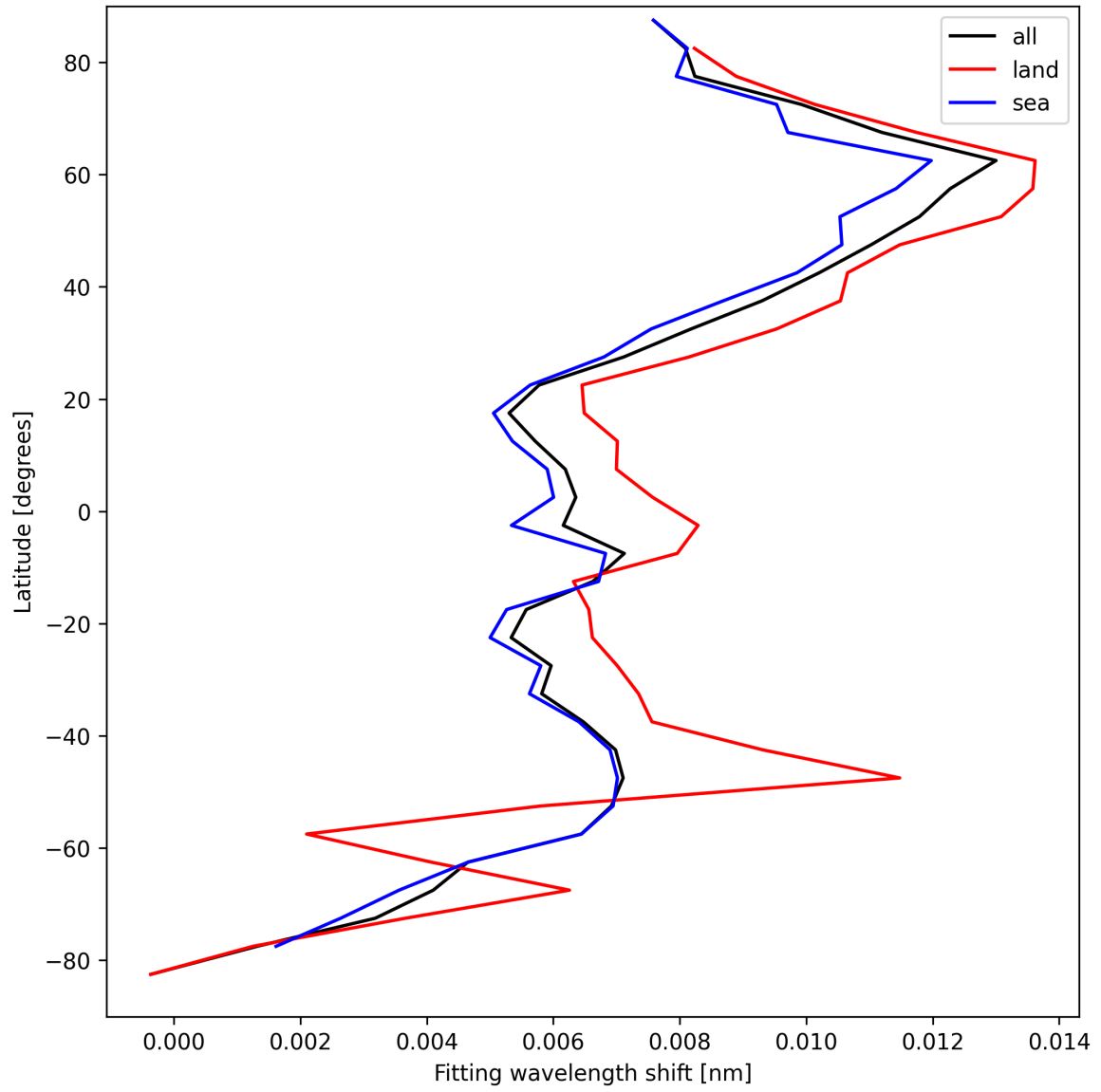
Figure 33: Zonal average of “Fitting wavelength shift” for 2025-04-09 to 2025-04-11.
