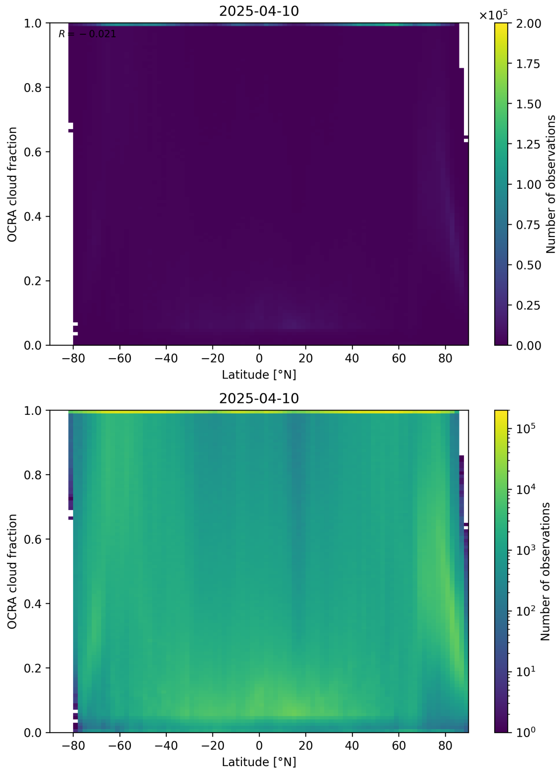
Figure 93: Scatter density plot of “Latitude” against “OCRA cloud fraction” for 2025-04-09 to 2025-04-11.
