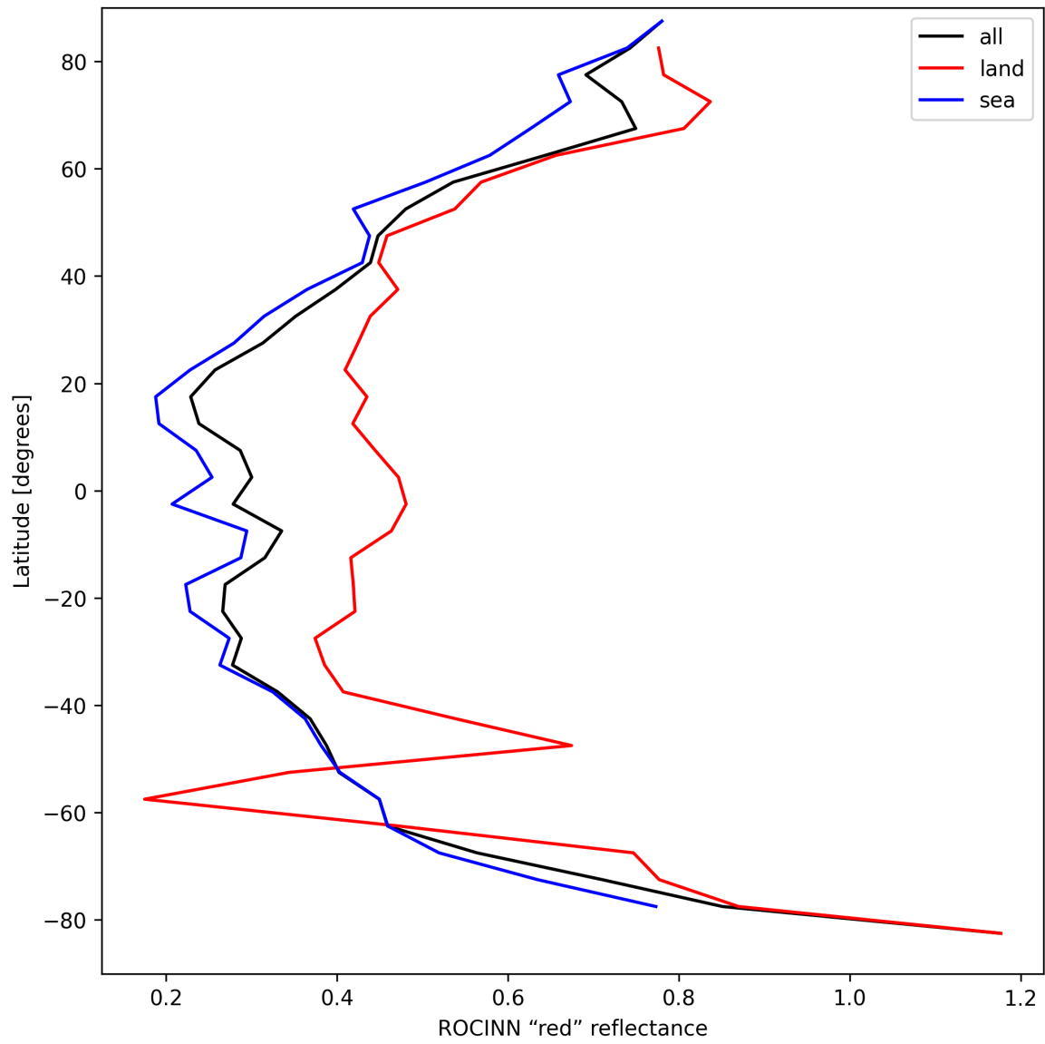
Figure 37: Zonal average of “ROCINN “red” reflectance” for 2025-04-09 to 2025-04-11.
