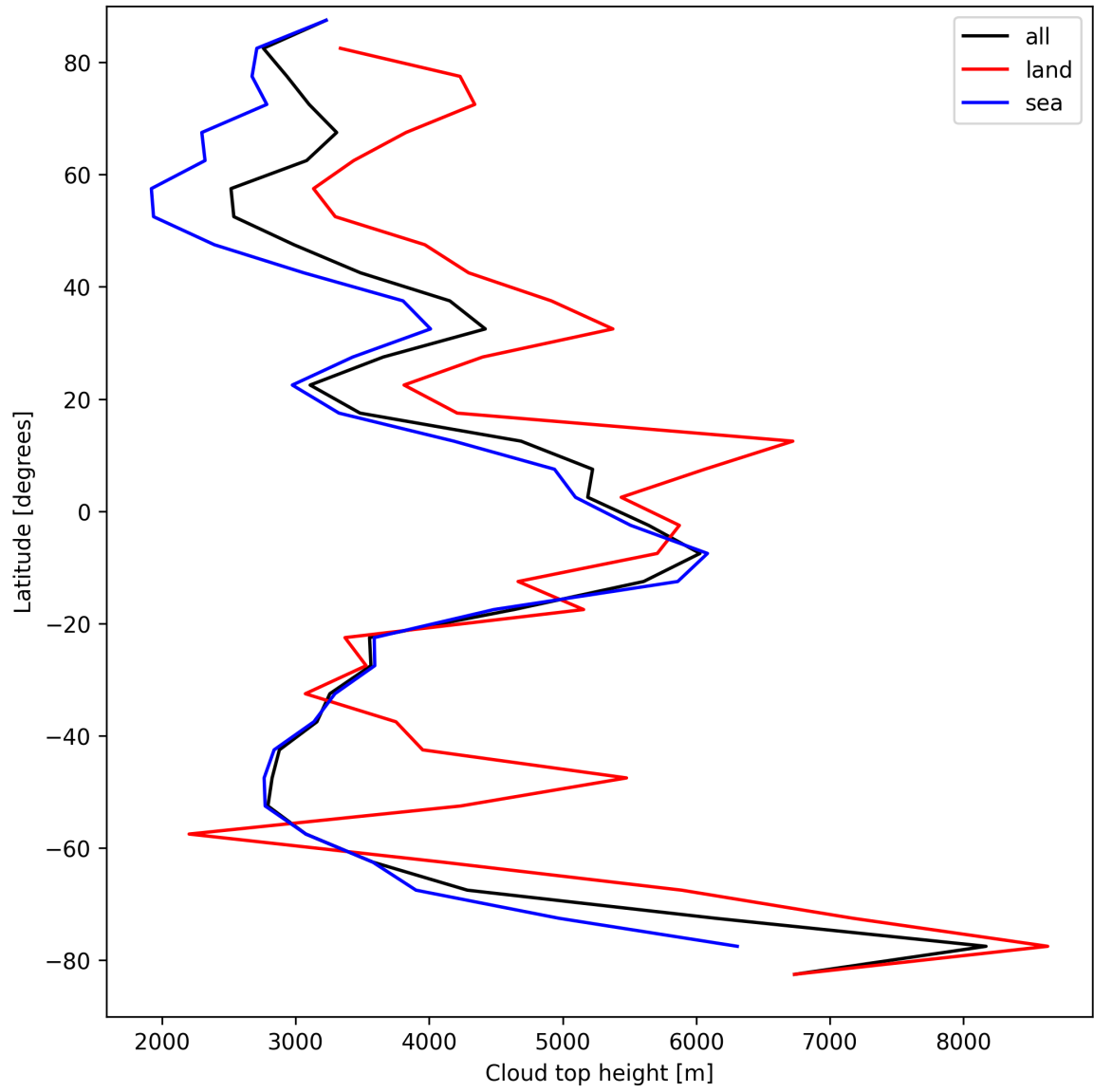
Figure 24: Zonal average of “Cloud top height” for 2025-04-09 to 2025-04-11.
