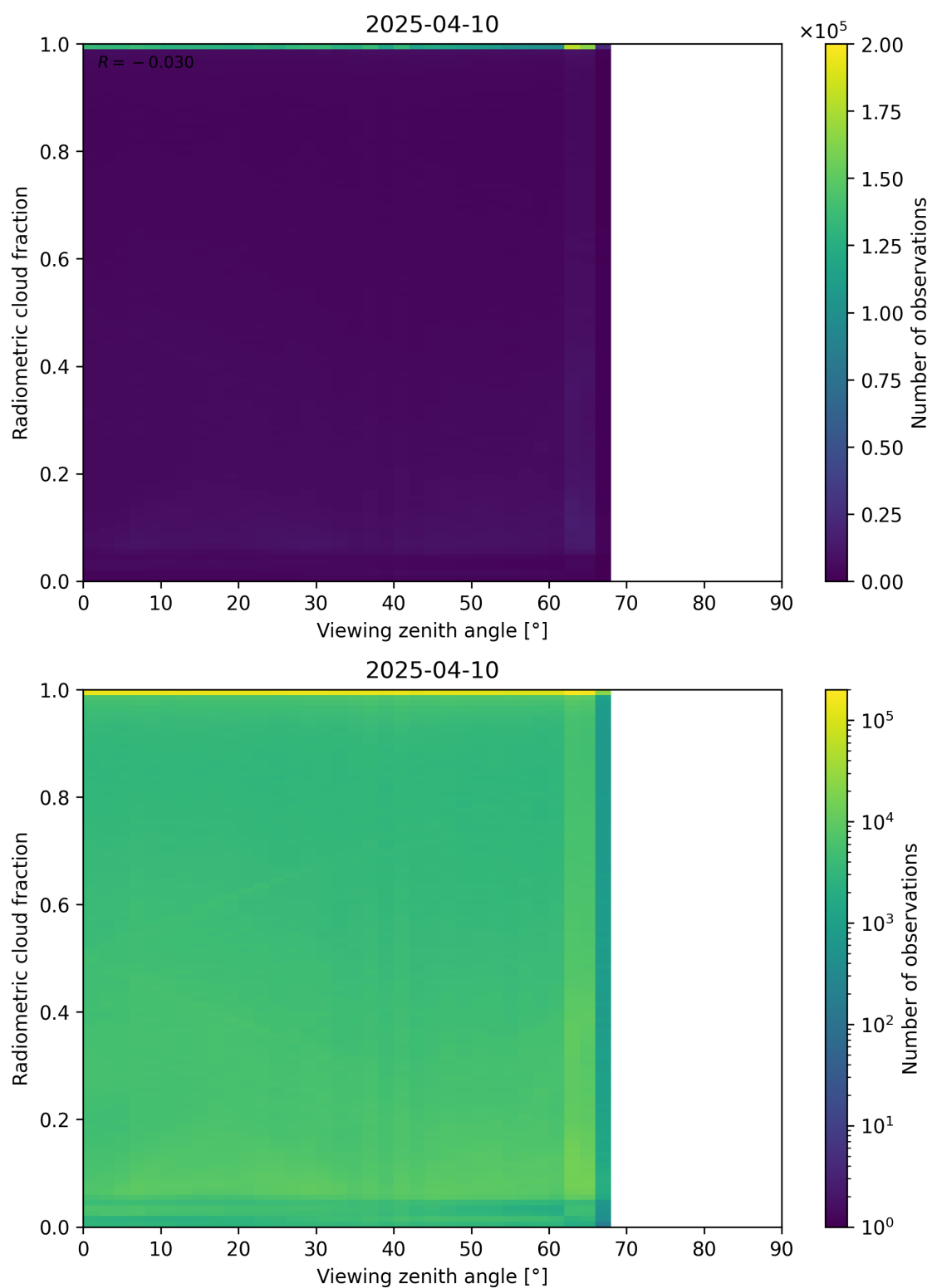
Figure 107: Scatter density plot of “Viewing zenith angle” against “Radiometric cloud fraction” for 2025-04-09 to 2025-04-11.
