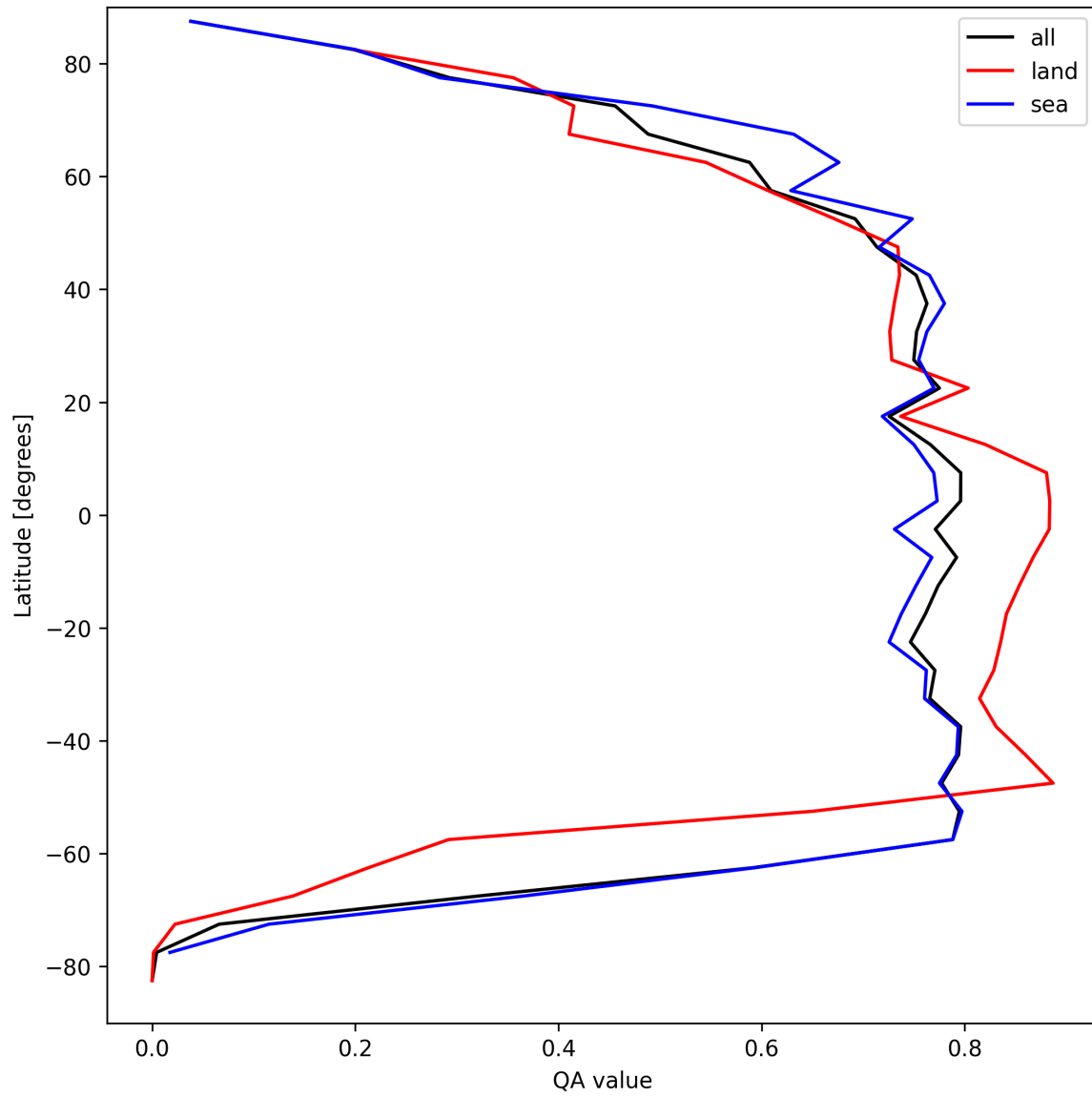
Figure 22: Zonal average of “QA value” for 2025-04-09 to 2025-04-11.
