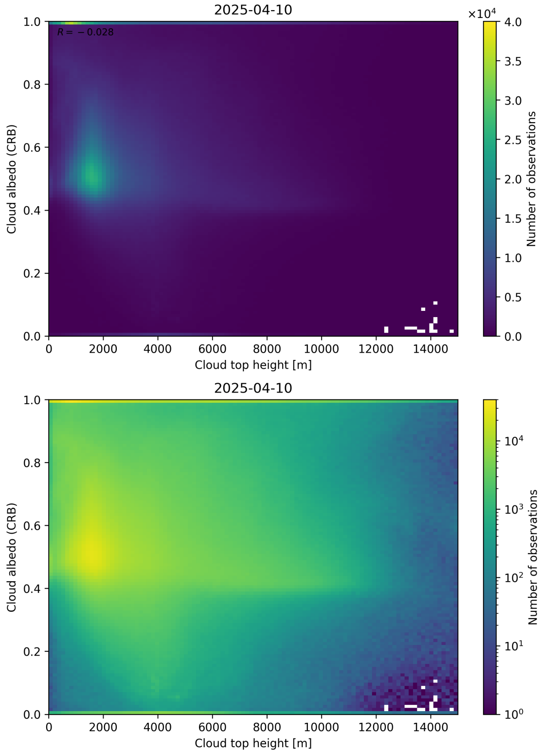
Figure 86: Scatter density plot of “Cloud top height” against “Cloud albedo (CRB)” for 2025-04-09 to 2025-04-11.
