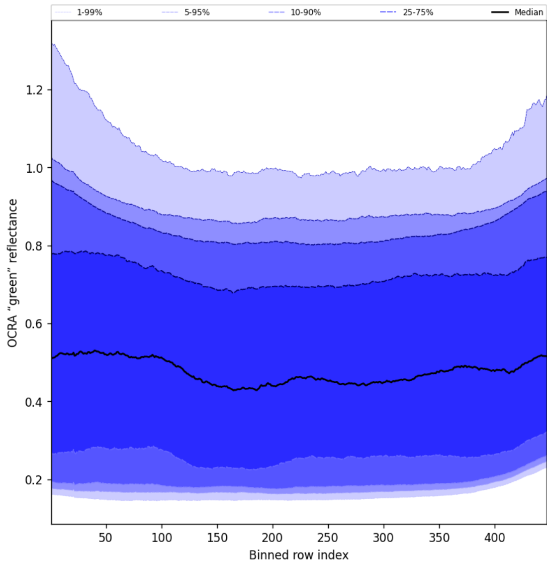
Figure 68: Along track statistics of “OCRA “green” reflectance” for 2025-04-09 to 2025-04-11
