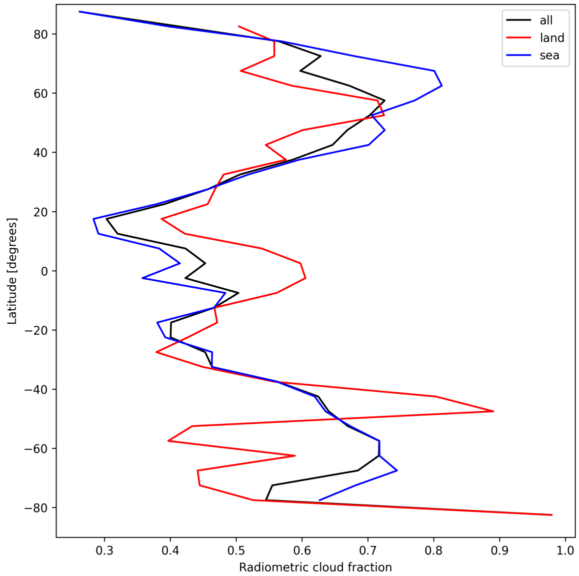
Figure 23: Zonal average of “Radiometric cloud fraction” for 2025-04-09 to 2025-04-11.
