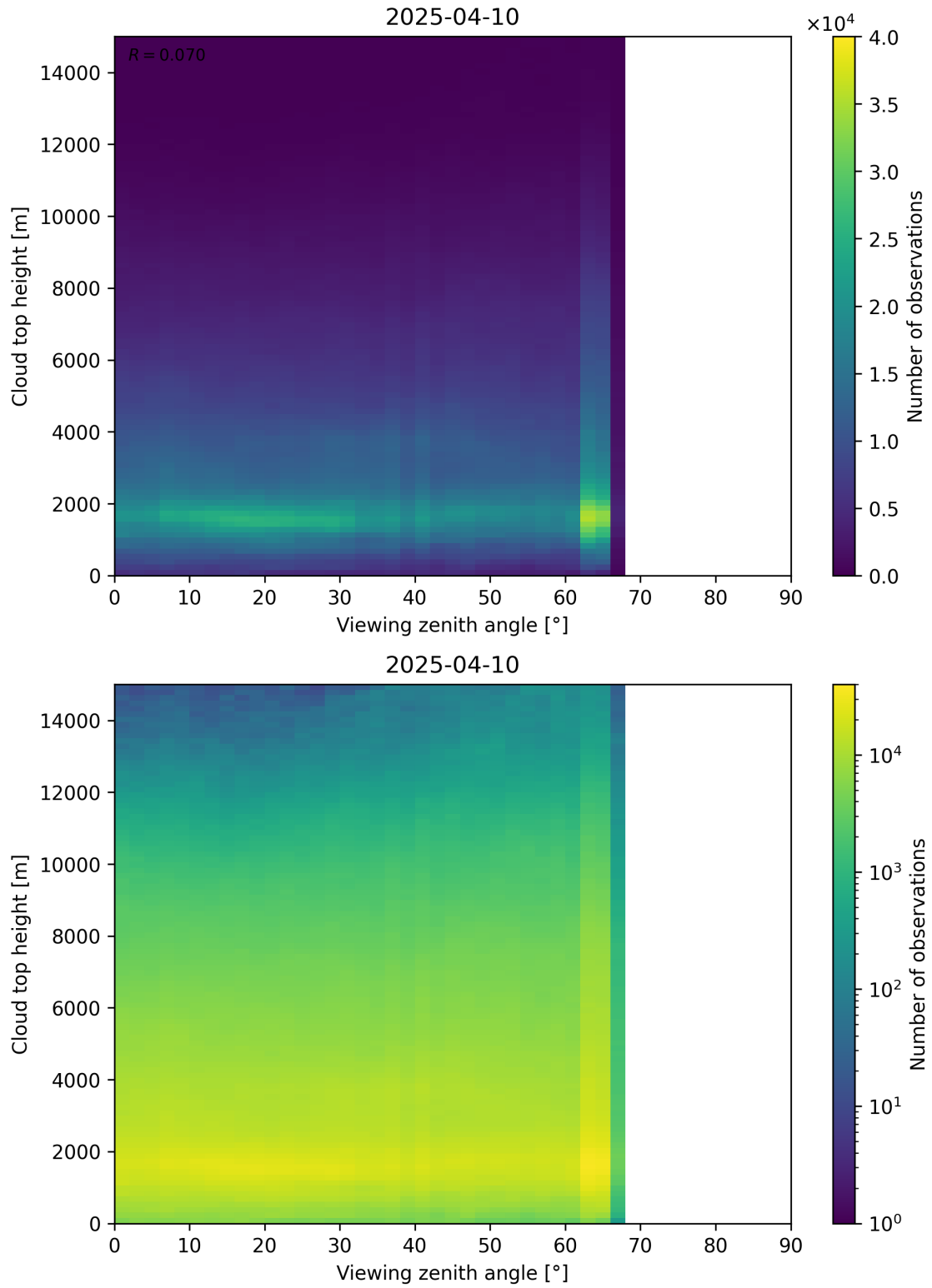
Figure 112: Scatter density plot of “Viewing zenith angle” against “Cloud top height” for 2025-04-09 to 2025-04-11.
