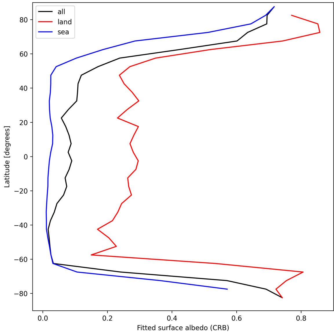
Figure 30: Zonal average of “Fitted surface albedo (CRB)” for 2025-04-09 to 2025-04-11.
