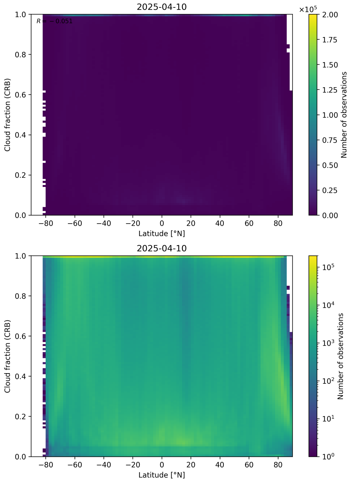
Figure 94: Scatter density plot of “Latitude” against “Cloud fraction (CRB)” for 2025-04-09 to 2025-04-11.
