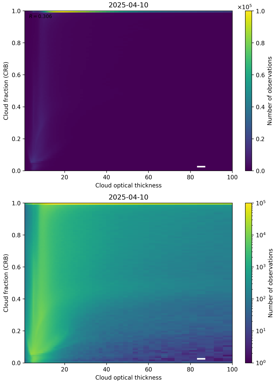
Figure 84: Scatter density plot of “Cloud optical thickness” against “Cloud fraction (CRB)” for 2025-04-09 to 2025-04-11.
