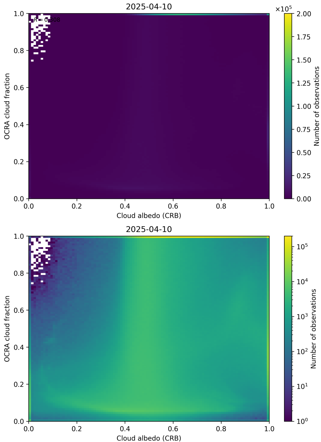
Figure 70: Scatter density plot of “Cloud albedo (CRB)” against “OCRA cloud fraction” for 2025-04-09 to 2025-04-11.
