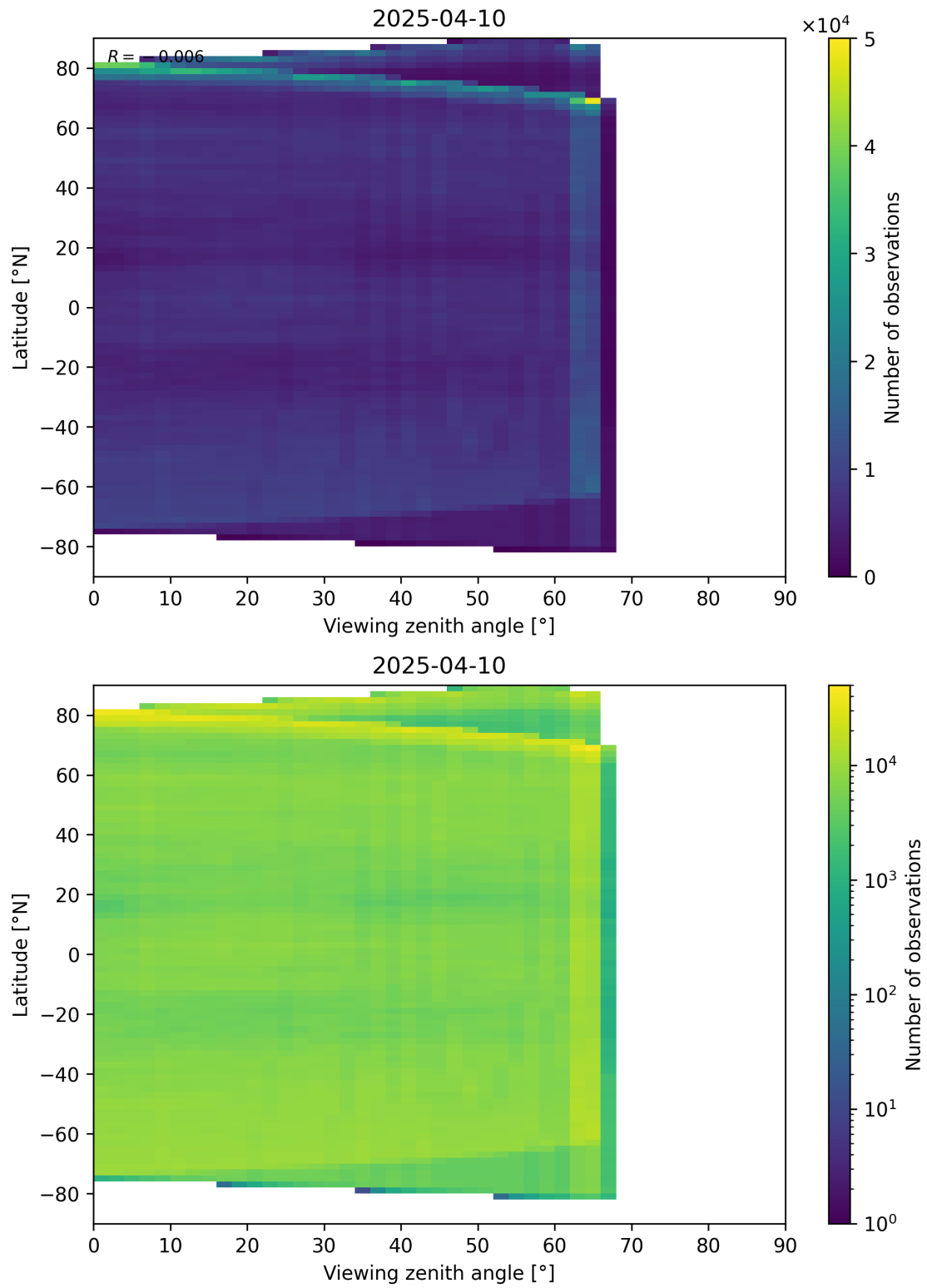
Figure 113: Scatter density plot of “Viewing zenith angle” against “Latitude” for 2025-04-09 to 2025-04-11.
