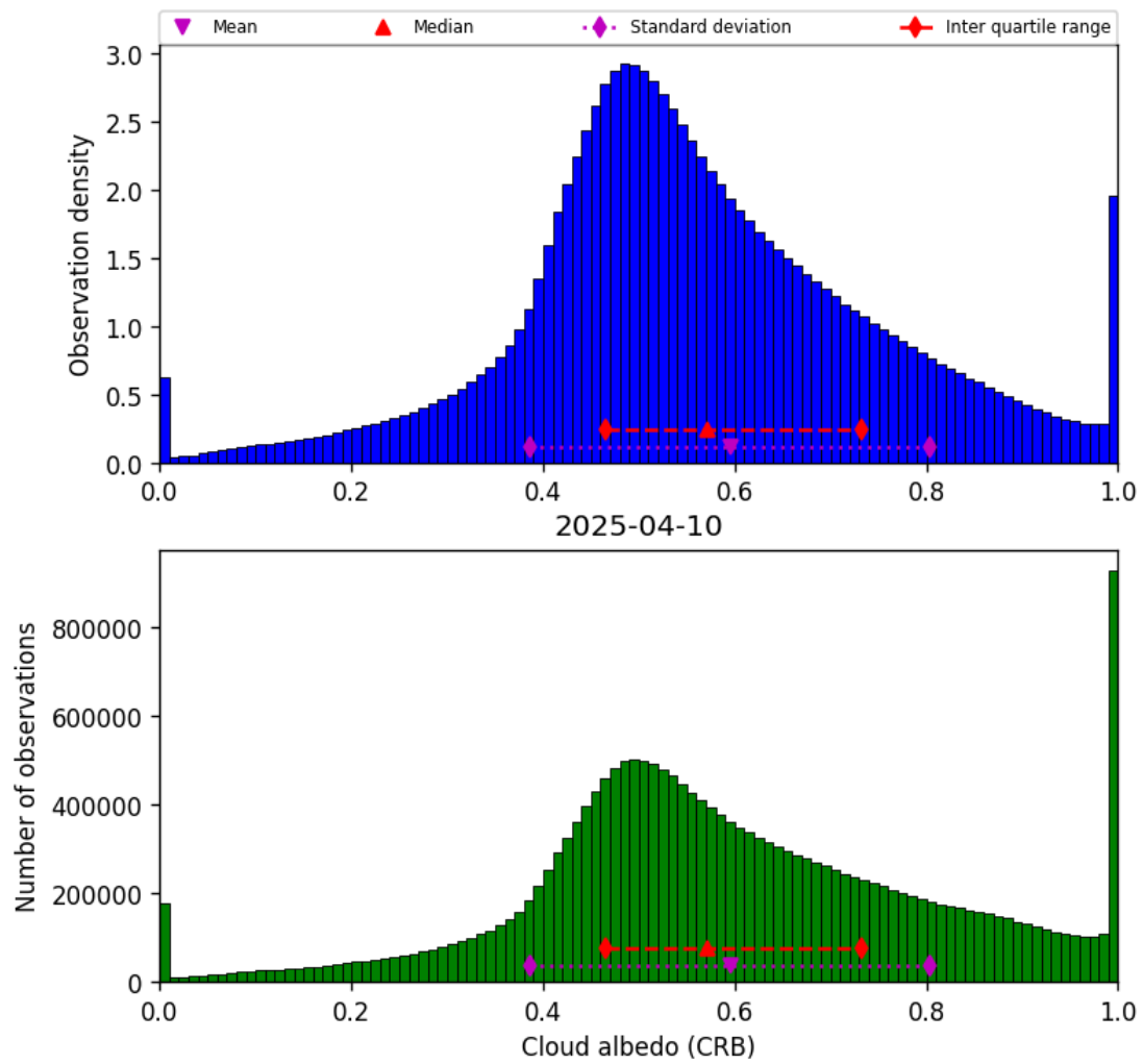
Figure 44: Histogram of “Cloud albedo (CRB)” for 2025-04-09 to 2025-04-11
