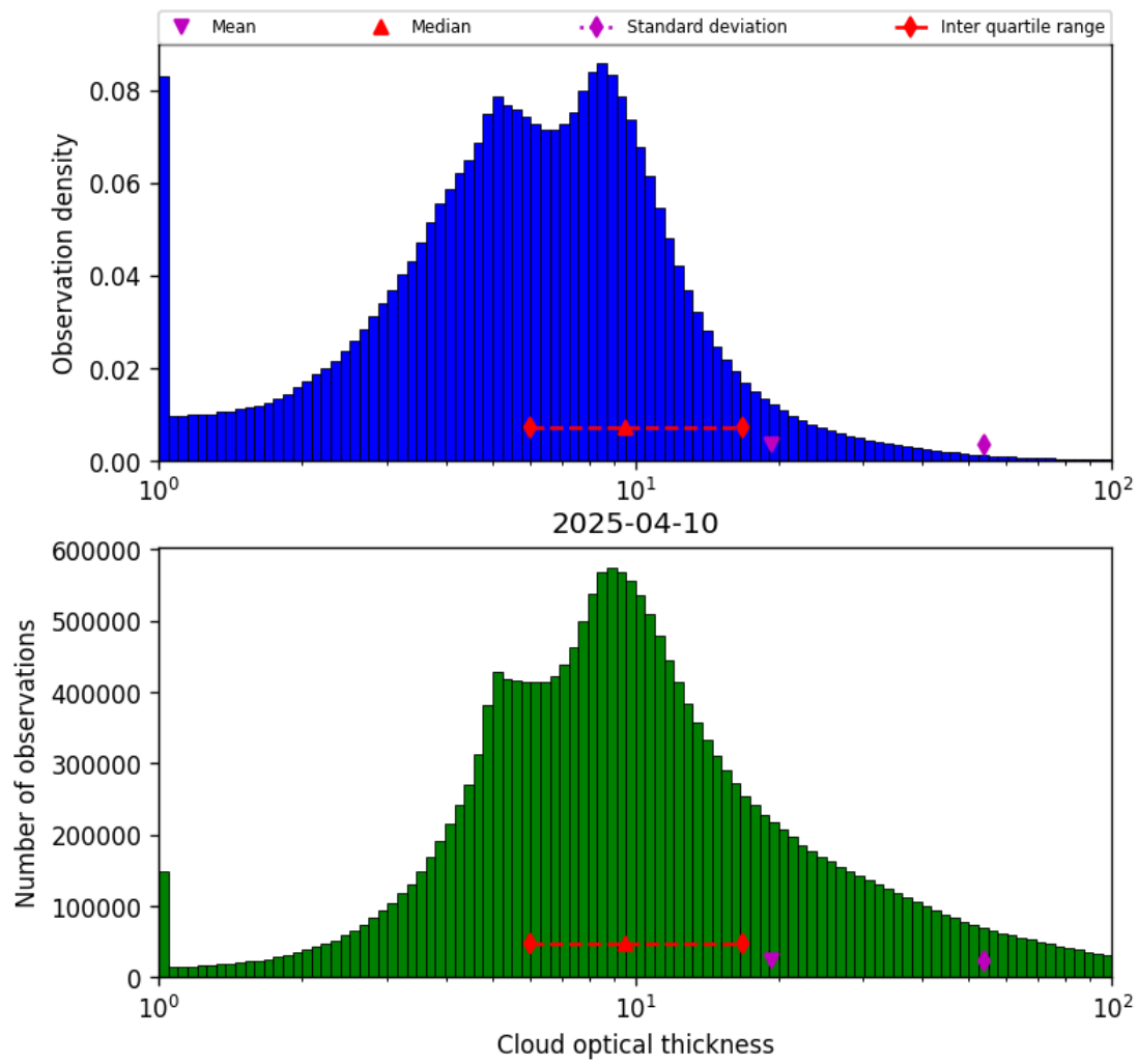
Figure 41: Histogram of “Cloud optical thickness” for 2025-04-09 to 2025-04-11
