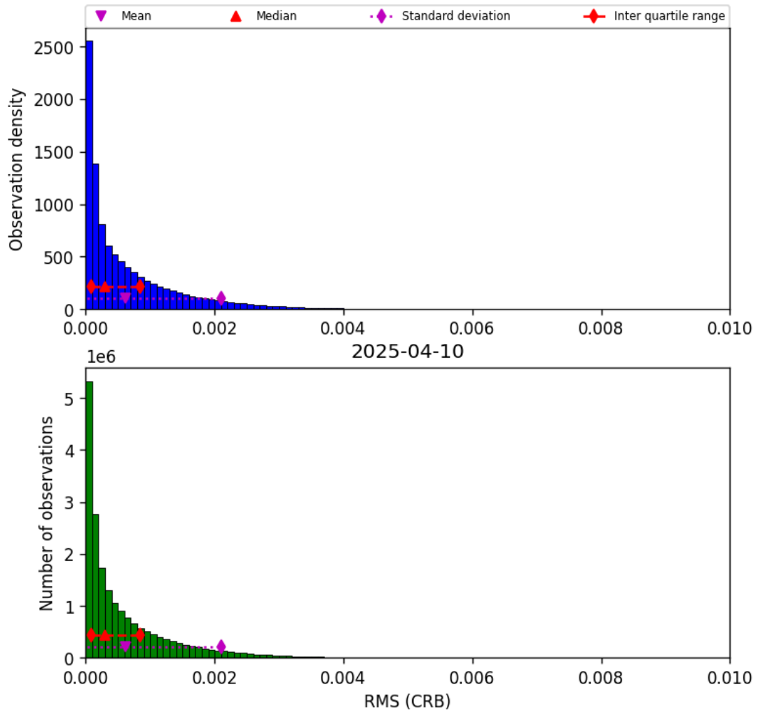
Figure 48: Histogram of “RMS (CRB)” for 2025-04-09 to 2025-04-11
