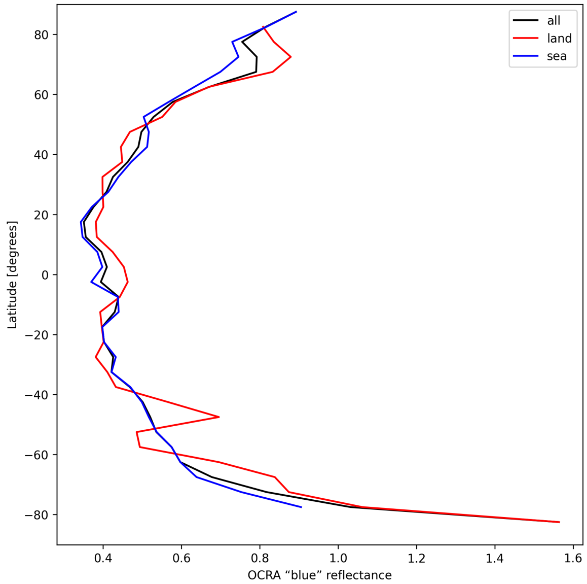
Figure 35: Zonal average of “OCRA “blue” reflectance” for 2025-04-09 to 2025-04-11.
