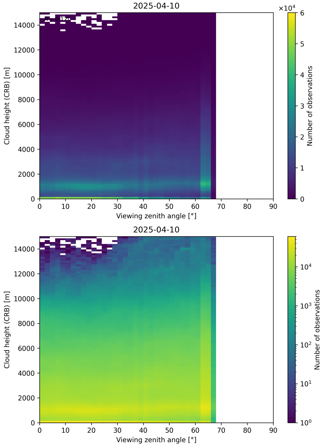
Figure 110: Scatter density plot of “Viewing zenith angle” against “Cloud height (CRB)” for 2025-04-09 to 2025-04-11.
