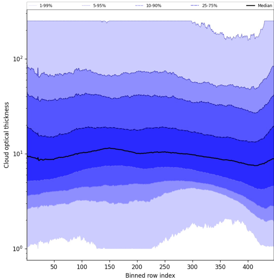
Figure 57: Along track statistics of “Cloud optical thickness” for 2025-04-09 to 2025-04-11
