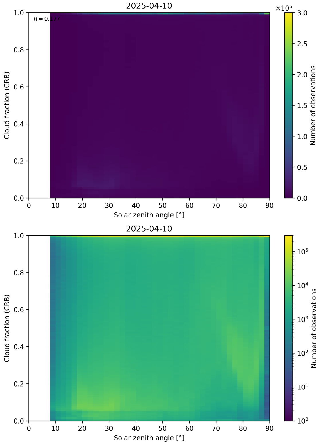
Figure 101: Scatter density plot of “Solar zenith angle” against “Cloud fraction (CRB)” for 2025-04-09 to 2025-04-11.
