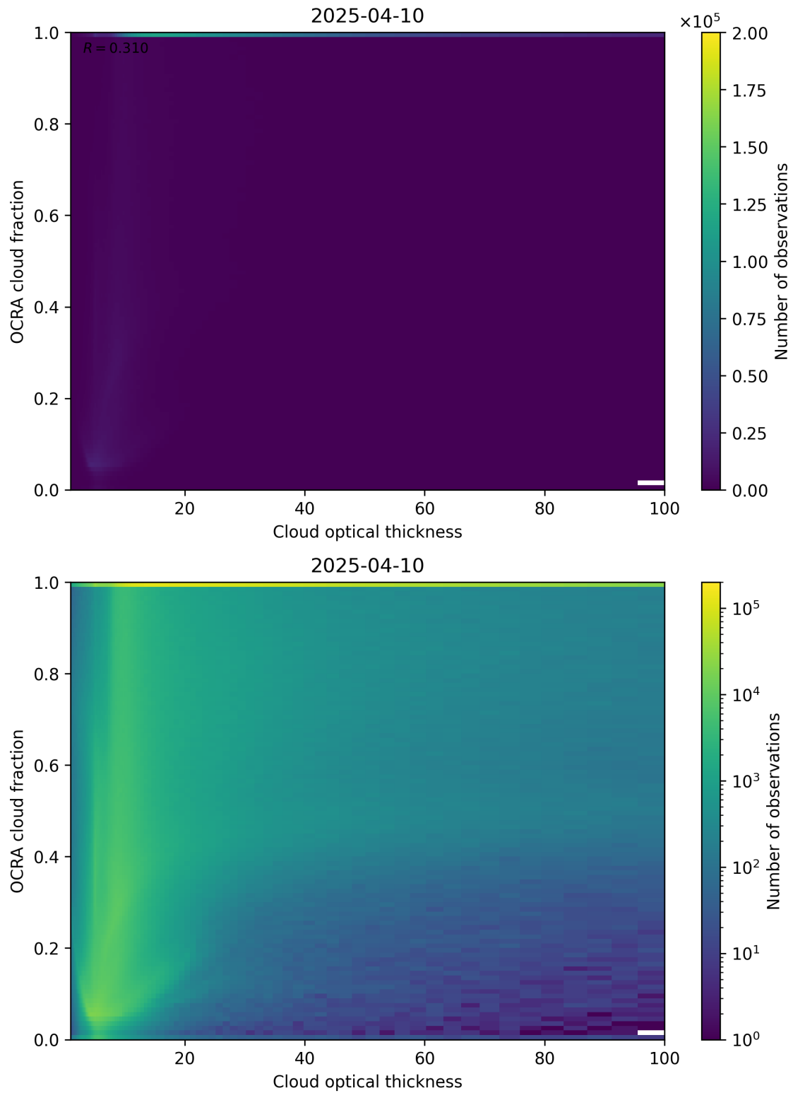
Figure 83: Scatter density plot of “Cloud optical thickness” against “OCRA cloud fraction” for 2025-04-09 to 2025-04-11.
