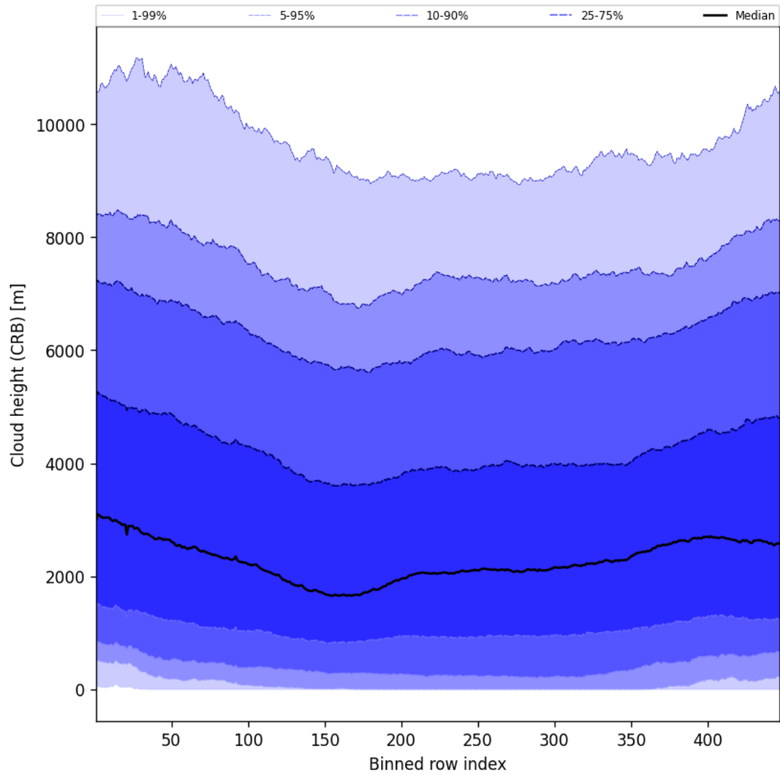
Figure 59: Along track statistics of “Cloud height (CRB)” for 2025-04-09 to 2025-04-11
