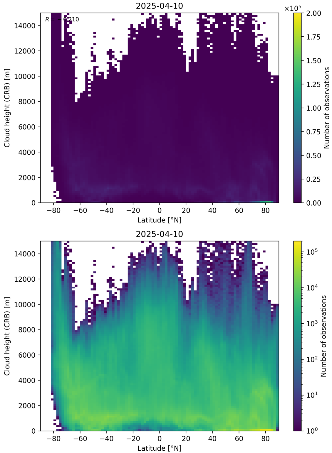
Figure 95: Scatter density plot of “Latitude” against “Cloud height (CRB)” for 2025-04-09 to 2025-04-11.
