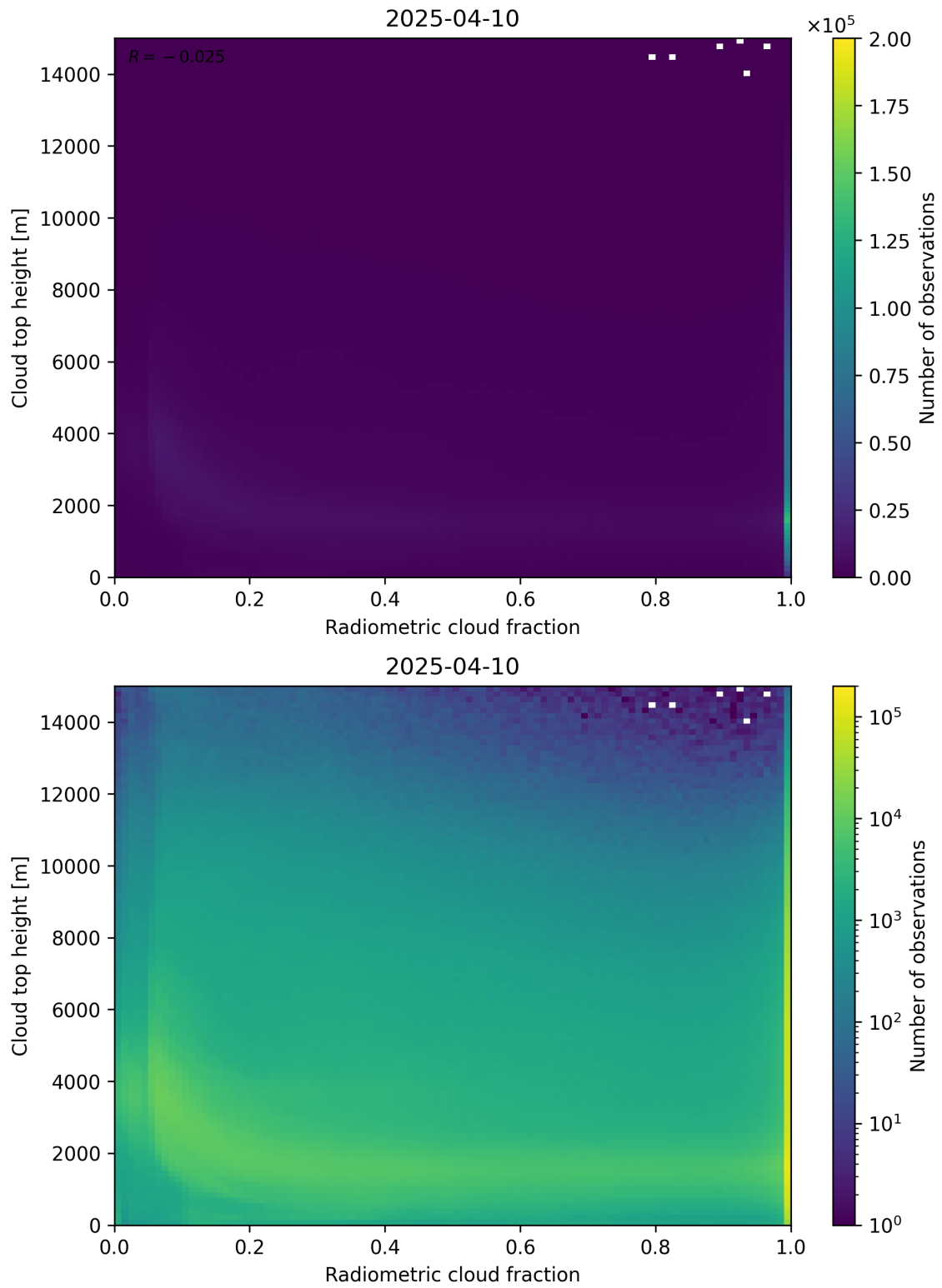
Figure 76: Scatter density plot of “Radiometric cloud fraction” against “Cloud top height” for 2025-04-09 to 2025-04-11.
