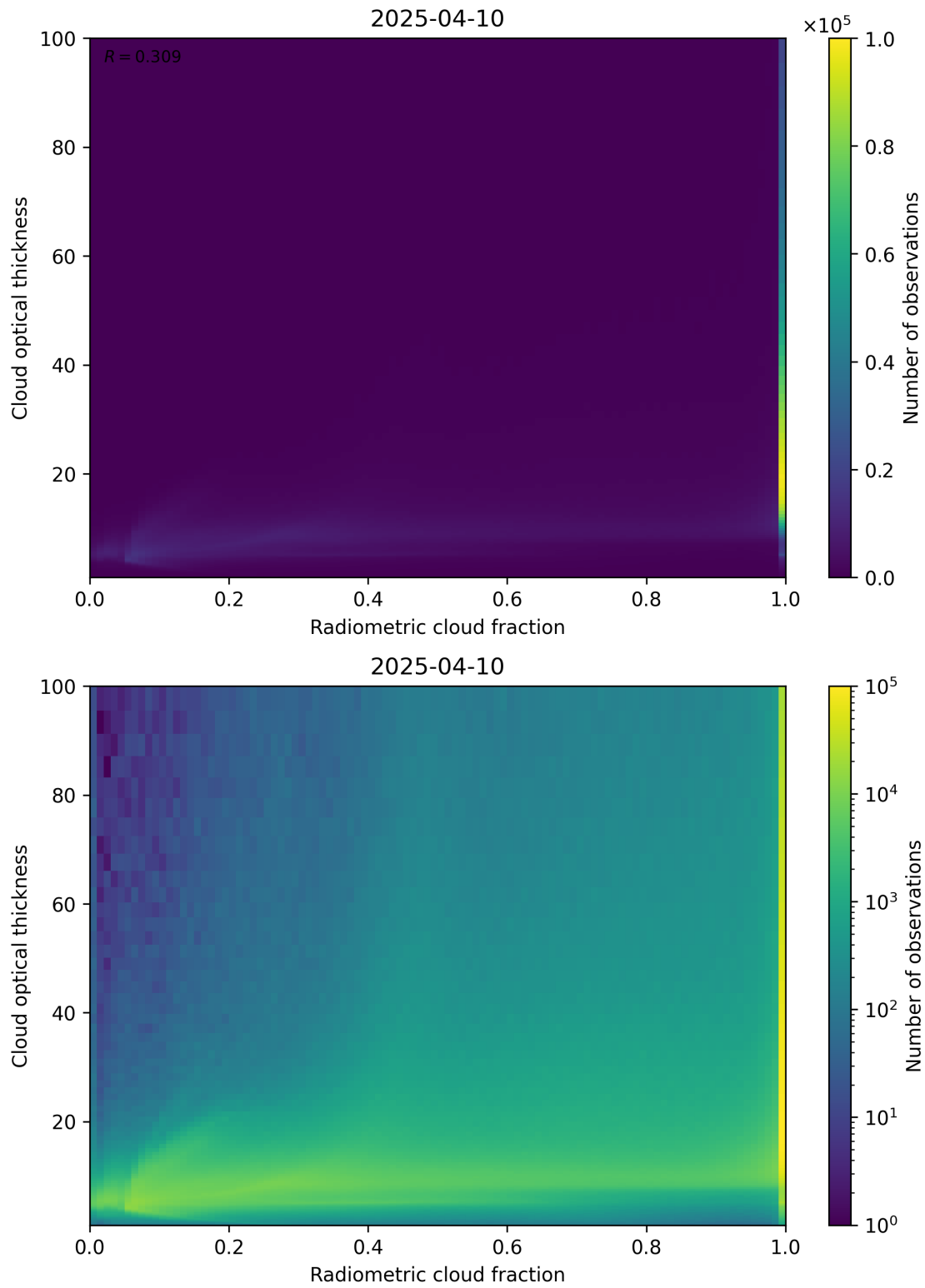
Figure 75: Scatter density plot of “Radiometric cloud fraction” against “Cloud optical thickness” for 2025-04-09 to 2025-04-11.
