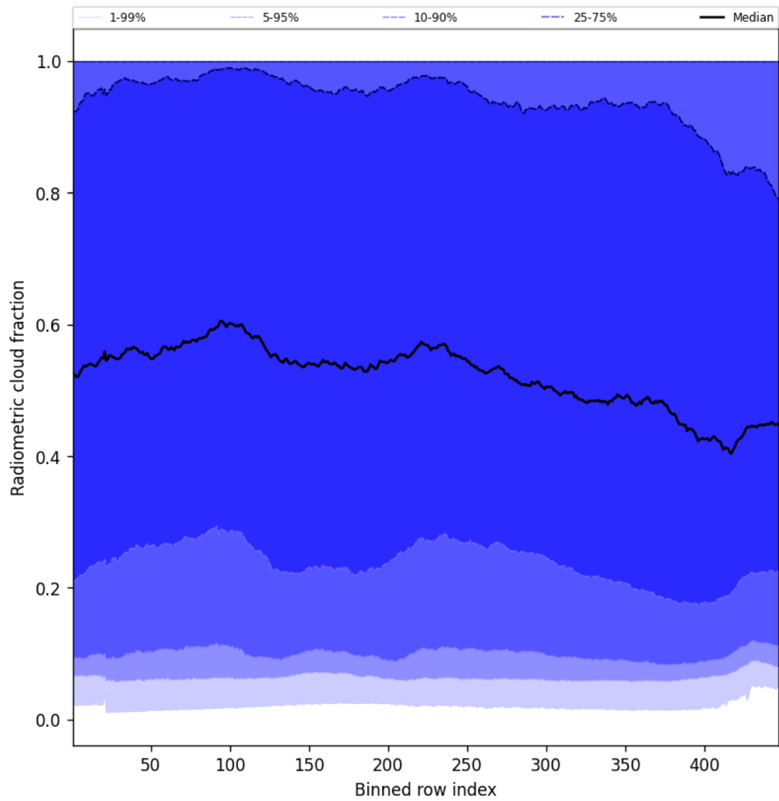
Figure 55: Along track statistics of “Radiometric cloud fraction” for 2025-04-09 to 2025-04-11
