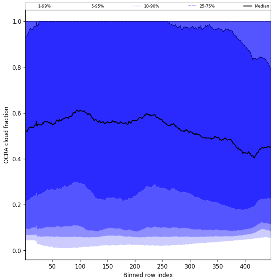
Figure 66: Along track statistics of “OCRA cloud fraction” for 2025-04-09 to 2025-04-11
