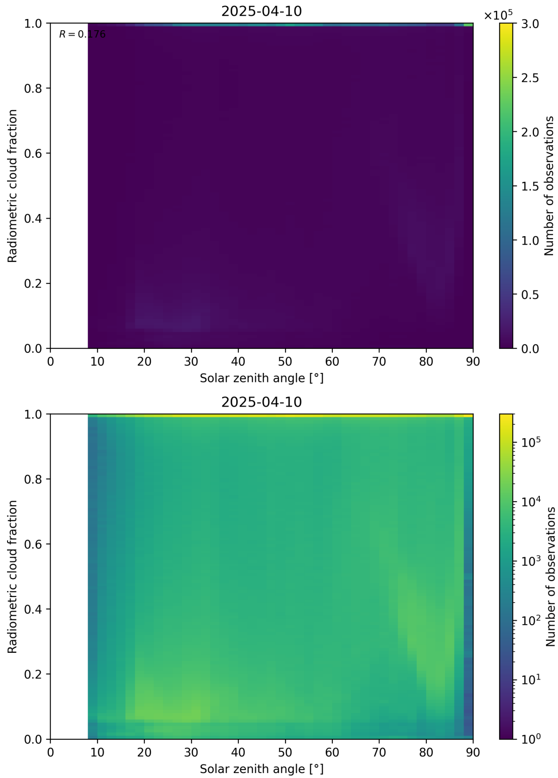
Figure 99: Scatter density plot of “Solar zenith angle” against “Radiometric cloud fraction” for 2025-04-09 to 2025-04-11.
