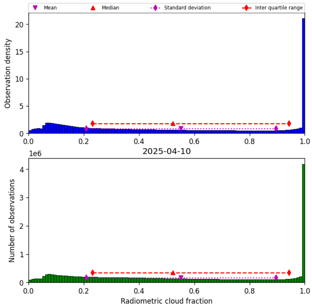
Figure 39: Histogram of “Radiometric cloud fraction” for 2025-04-09 to 2025-04-11
