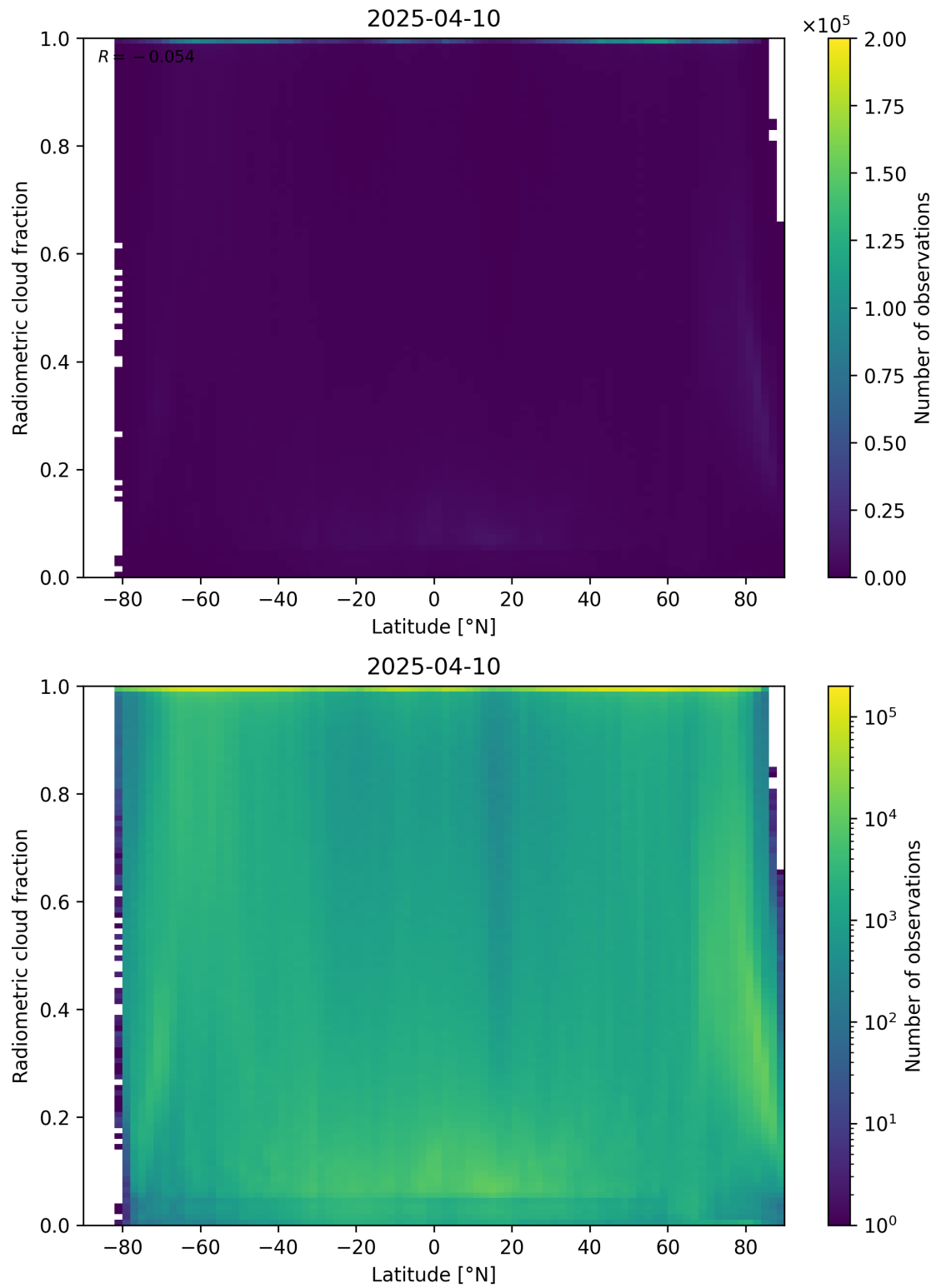
Figure 92: Scatter density plot of “Latitude” against “Radiometric cloud fraction” for 2025-04-09 to 2025-04-11.
