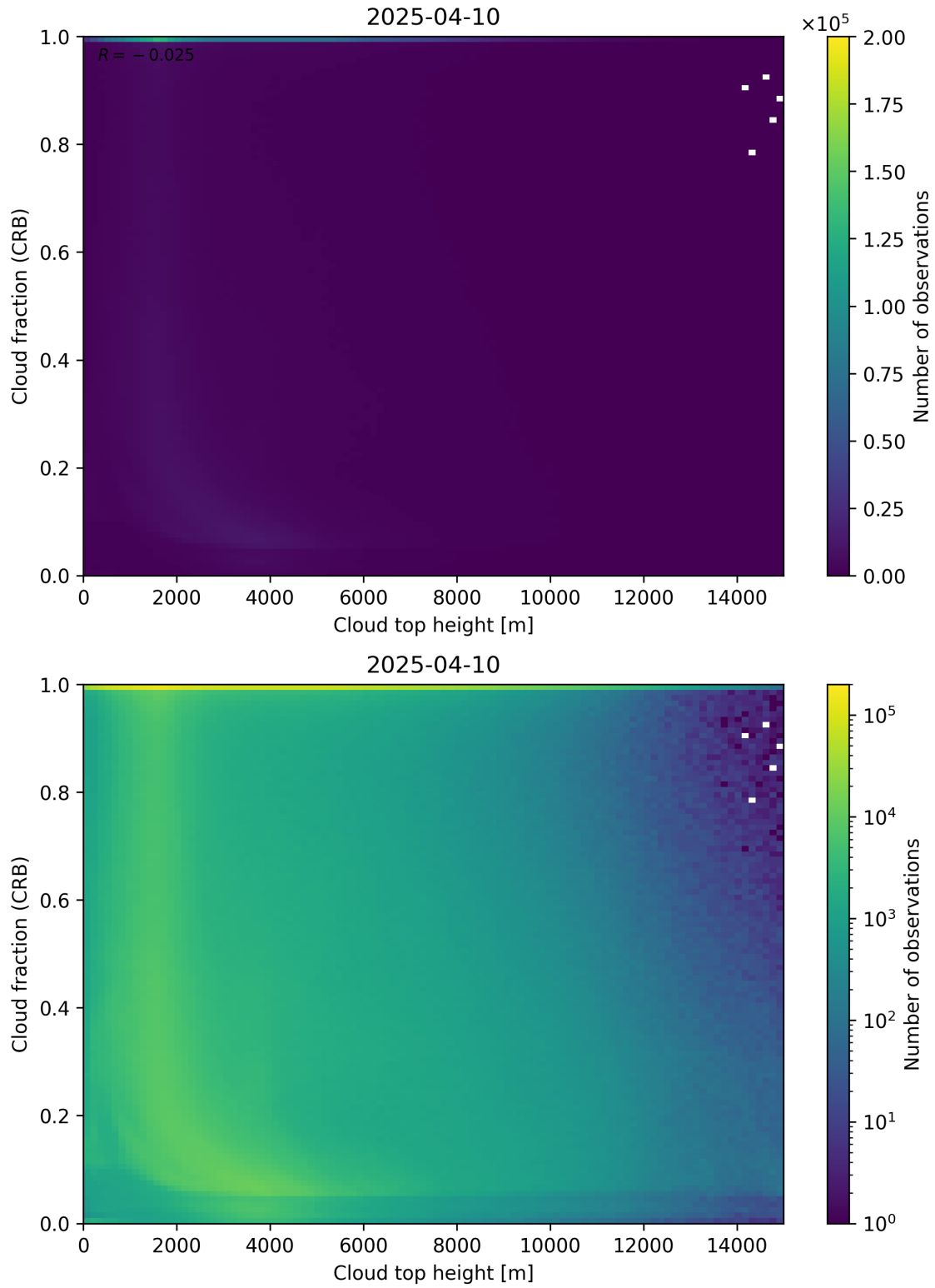
Figure 88: Scatter density plot of “Cloud top height” against “Cloud fraction (CRB)” for 2025-04-09 to 2025-04-11.
