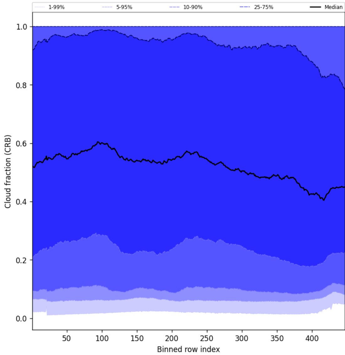
Figure 58: Along track statistics of “Cloud fraction (CRB)” for 2025-04-09 to 2025-04-11
