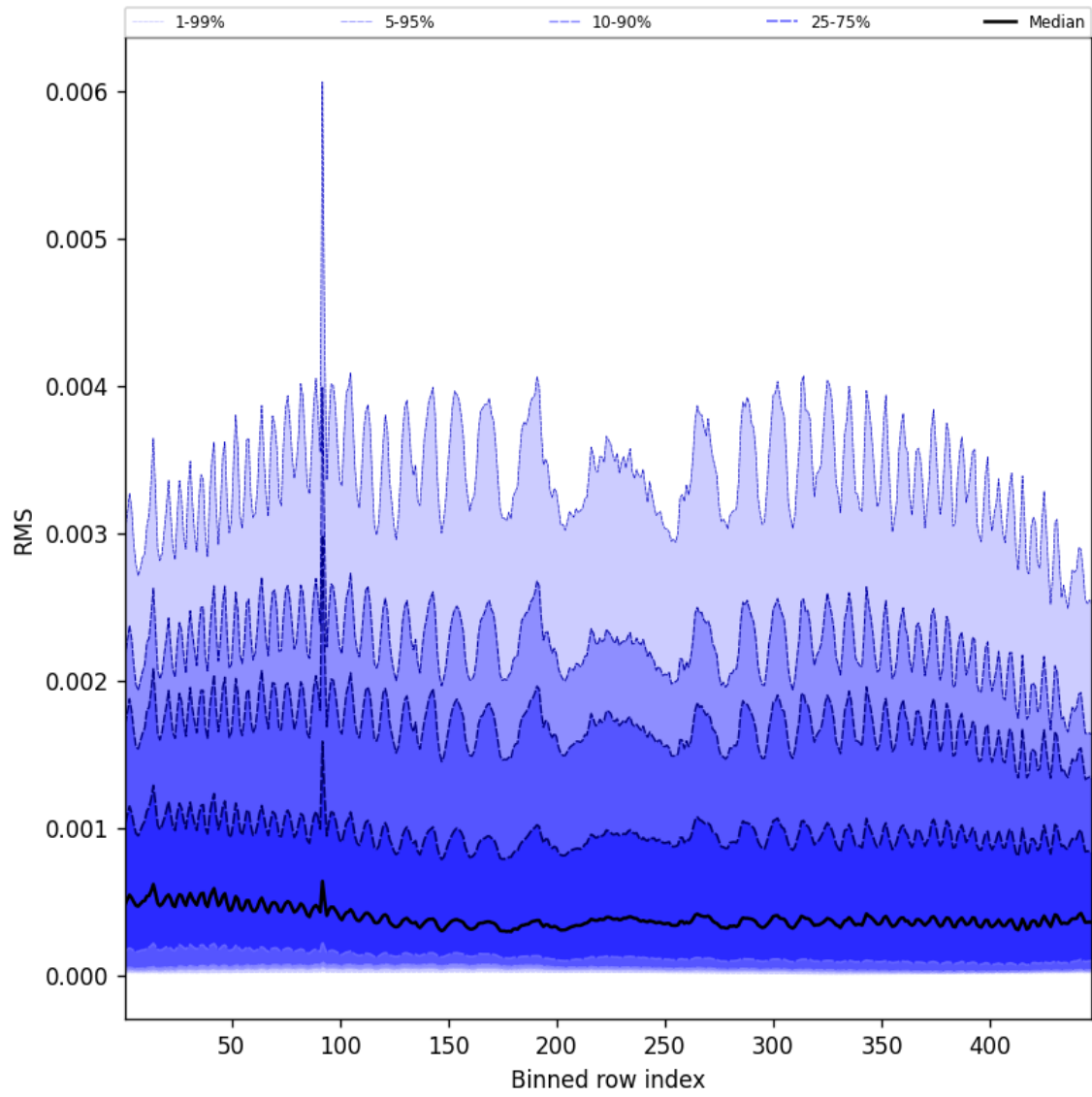
Figure 63: Along track statistics of “RMS” for 2025-04-09 to 2025-04-11
