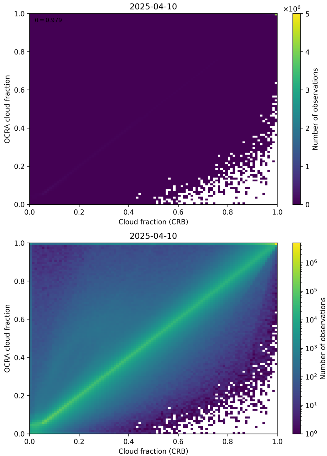
Figure 78: Scatter density plot of “Cloud fraction (CRB)” against “OCRA cloud fraction” for 2025-04-09 to 2025-04-11.
