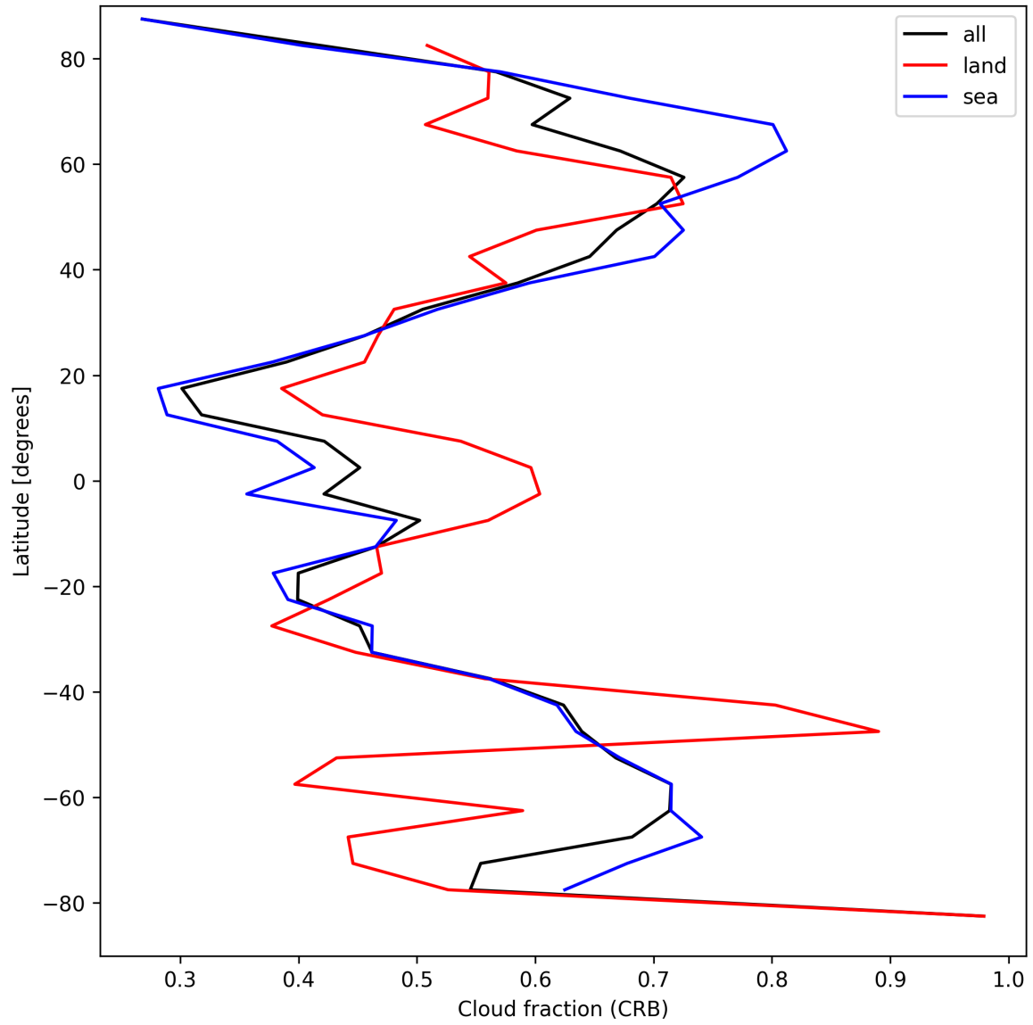
Figure 26: Zonal average of “Cloud fraction (CRB)” for 2025-04-09 to 2025-04-11.
