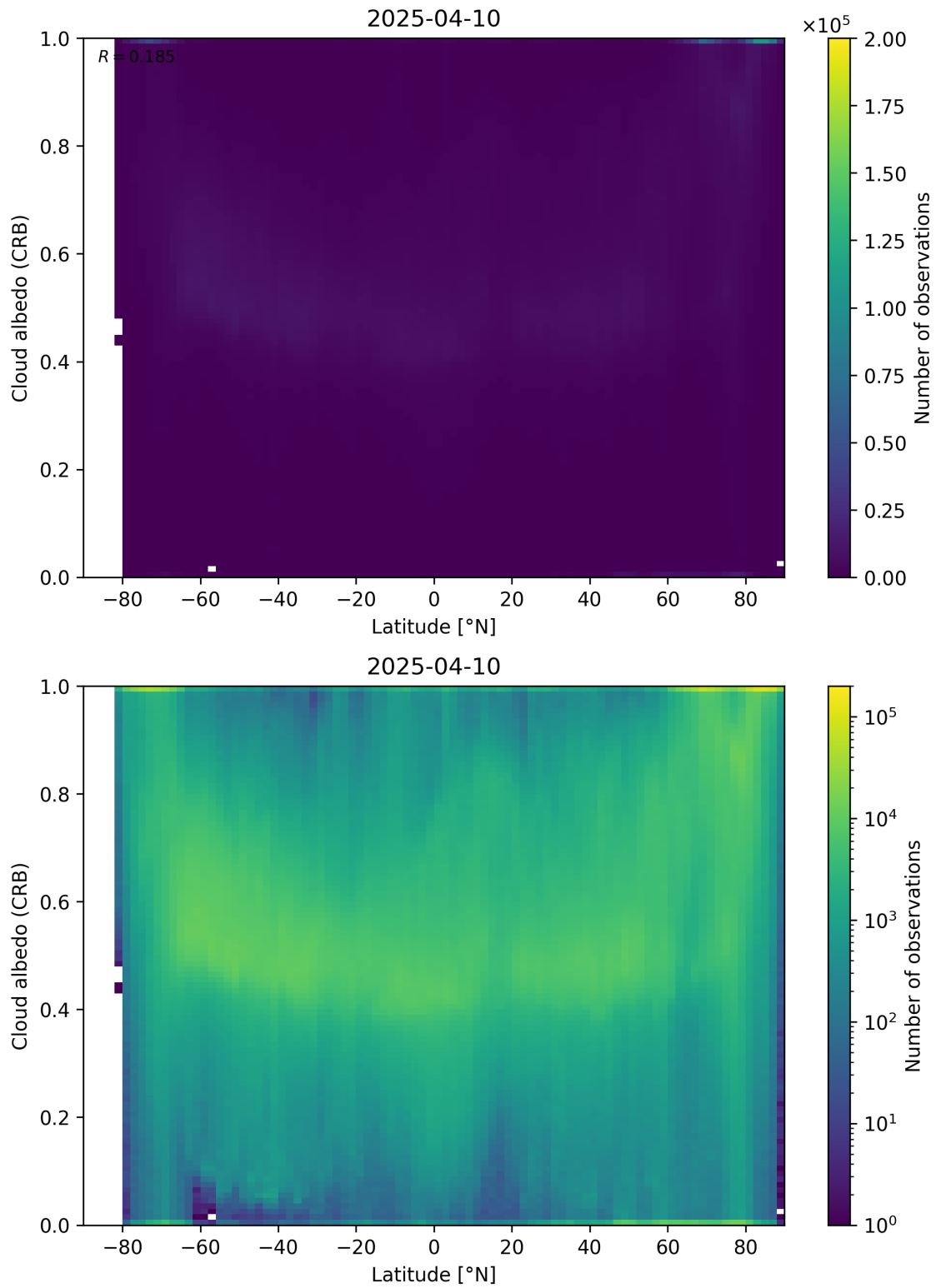
Figure 91: Scatter density plot of “Latitude” against “Cloud albedo (CRB)” for 2025-04-09 to 2025-04-11.
