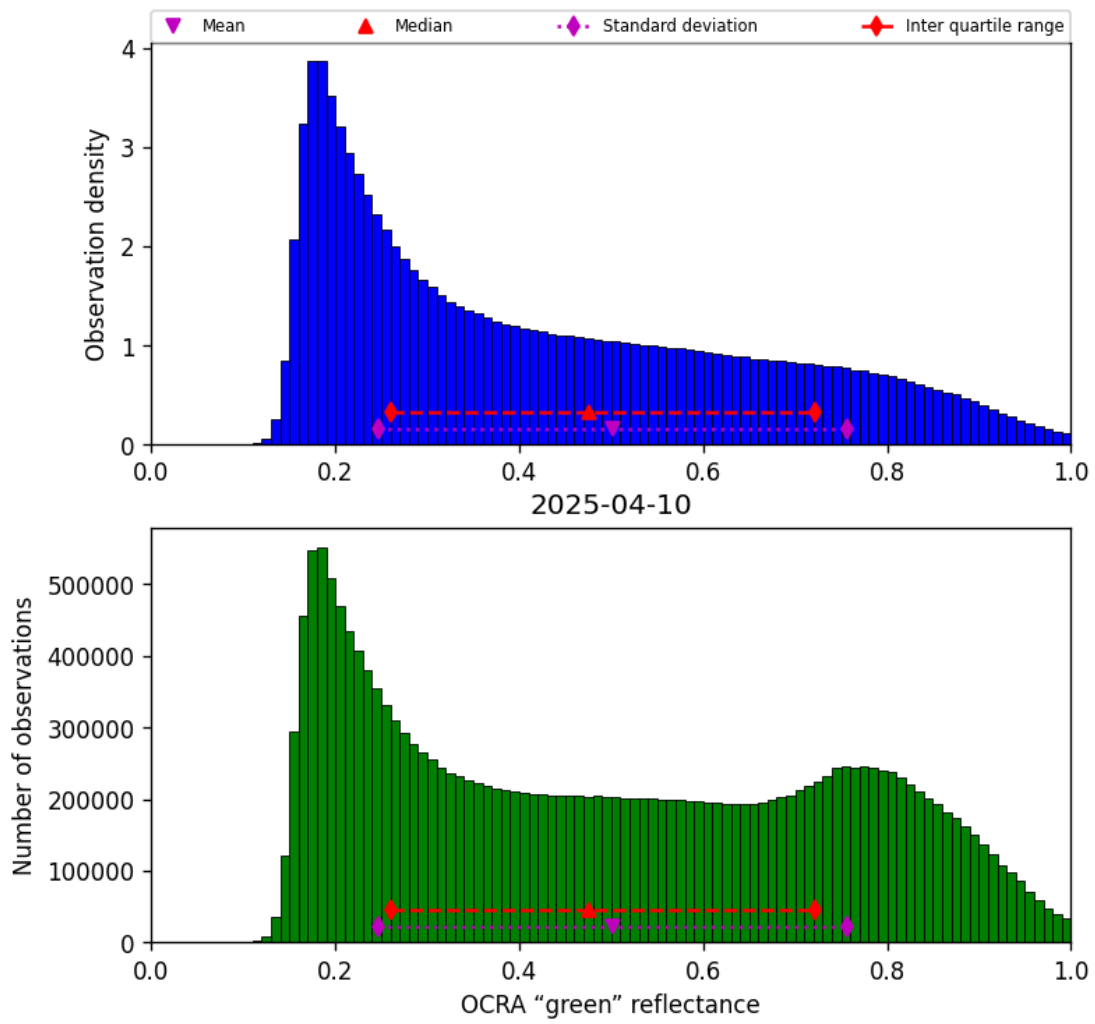
Figure 52: Histogram of “OCRA “green” reflectance” for 2025-04-09 to 2025-04-11
