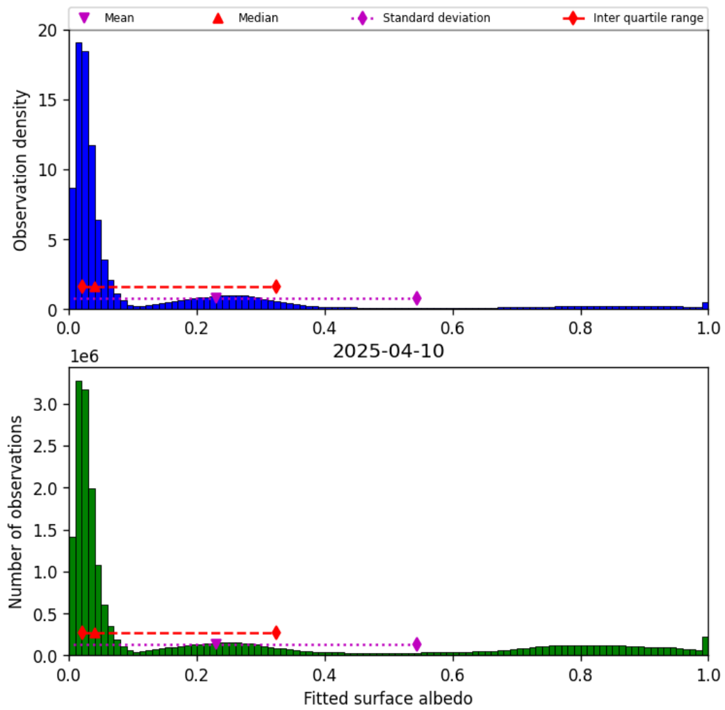
Figure 45: Histogram of “Fitted surface albedo” for 2025-04-09 to 2025-04-11
