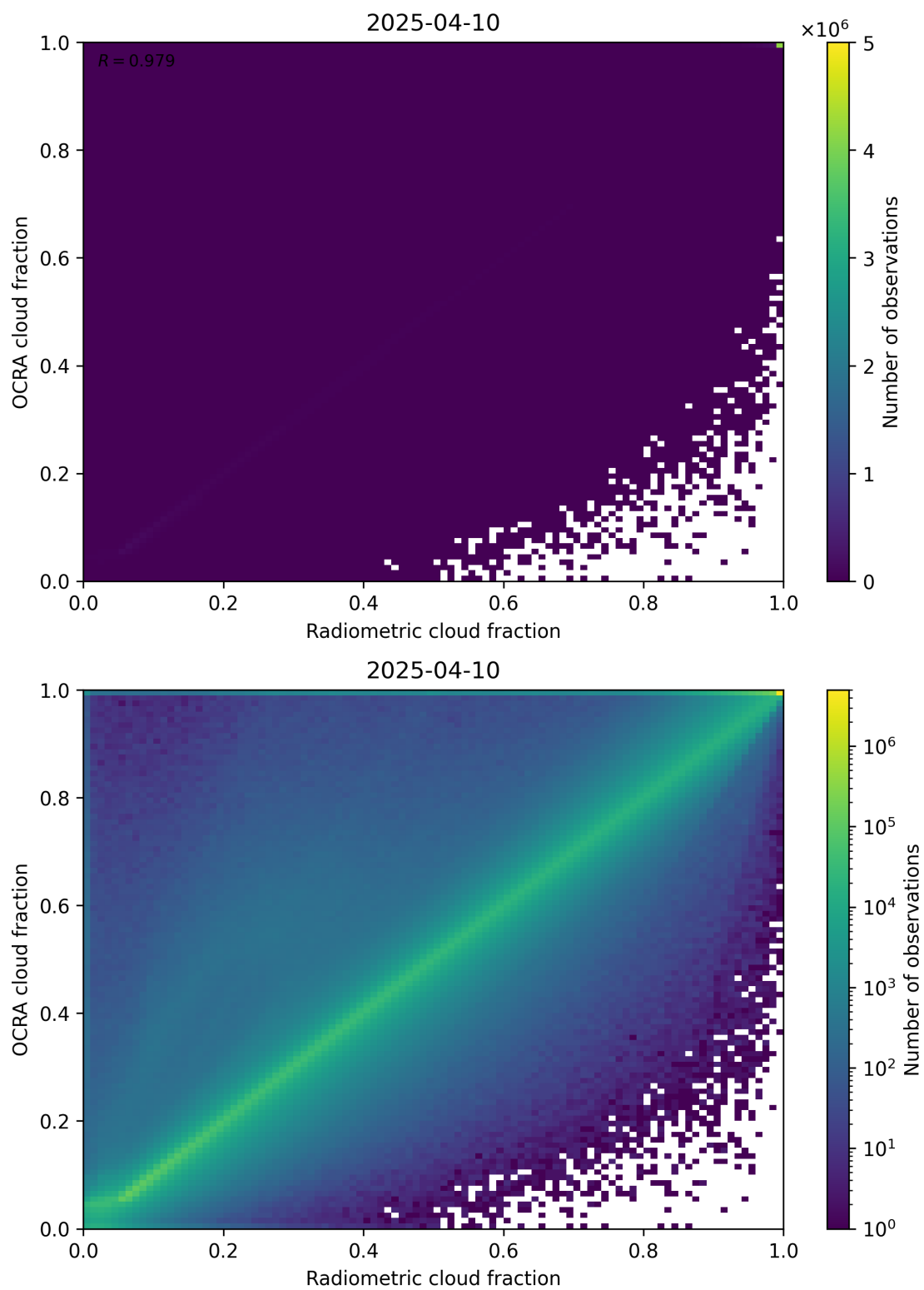
Figure 72: Scatter density plot of “Radiometric cloud fraction” against “OCRA cloud fraction” for 2025-04-09 to 2025-04-11.
