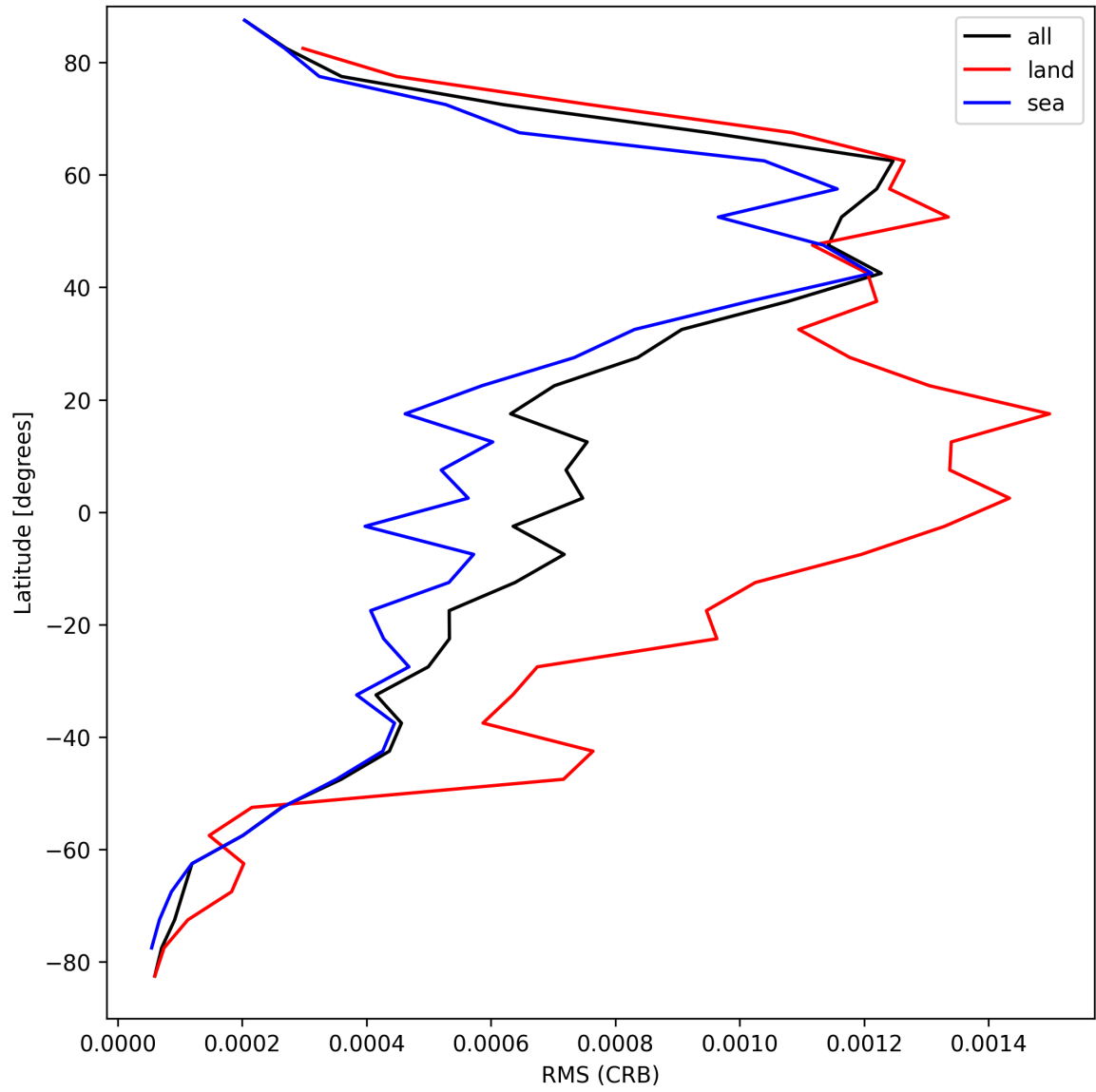
Figure 32: Zonal average of “RMS (CRB)” for 2025-04-09 to 2025-04-11.
