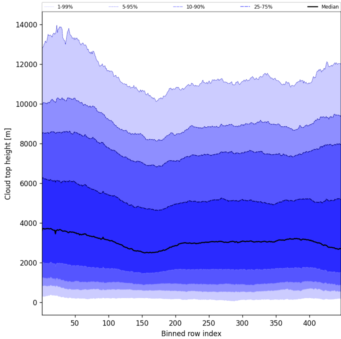
Figure 56: Along track statistics of “Cloud top height” for 2025-04-09 to 2025-04-11
