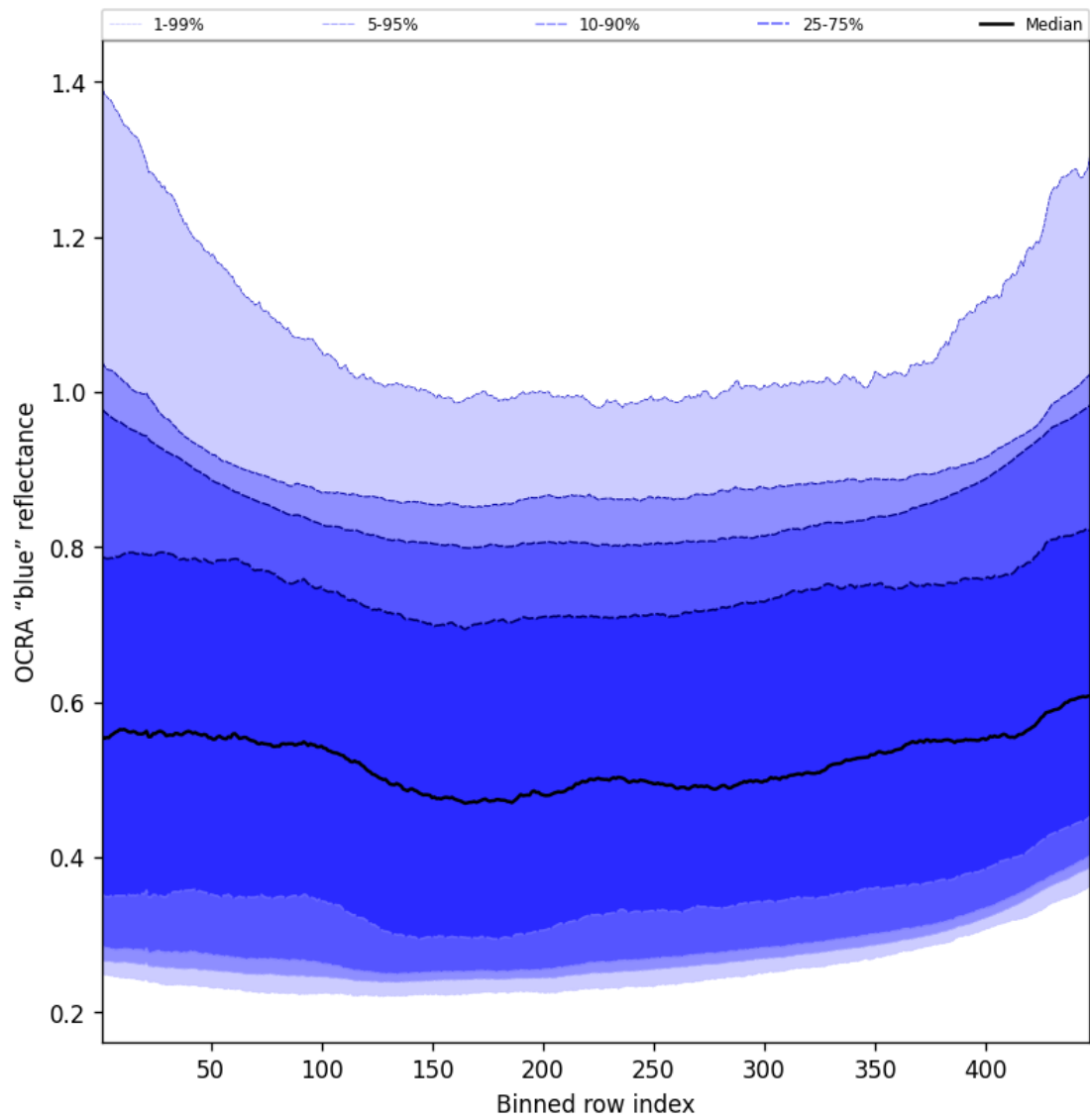
Figure 67: Along track statistics of “OCRA “blue” reflectance” for 2025-04-09 to 2025-04-11
