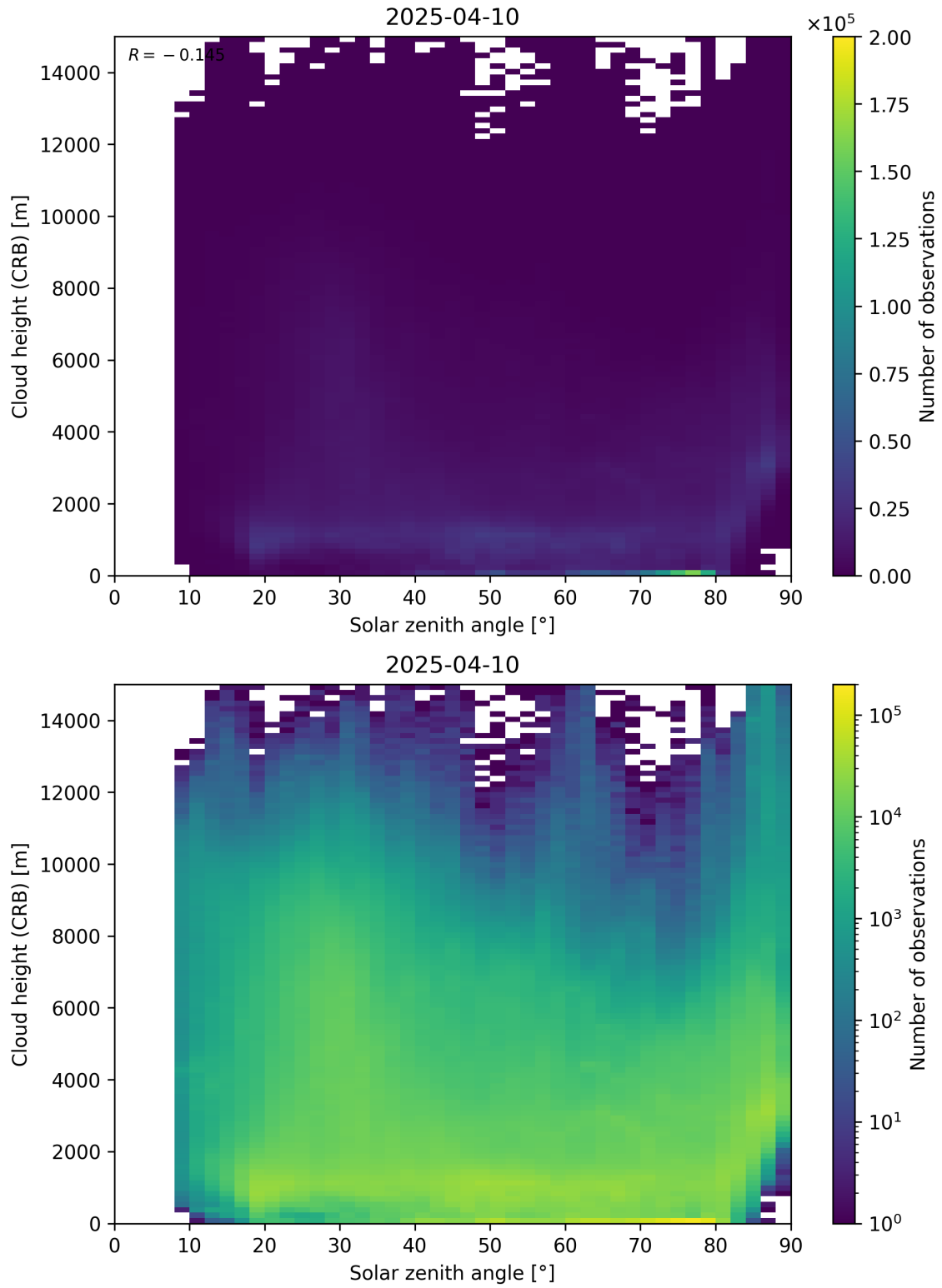
Figure 102: Scatter density plot of “Solar zenith angle” against “Cloud height (CRB)” for 2025-04-09 to 2025-04-11.
