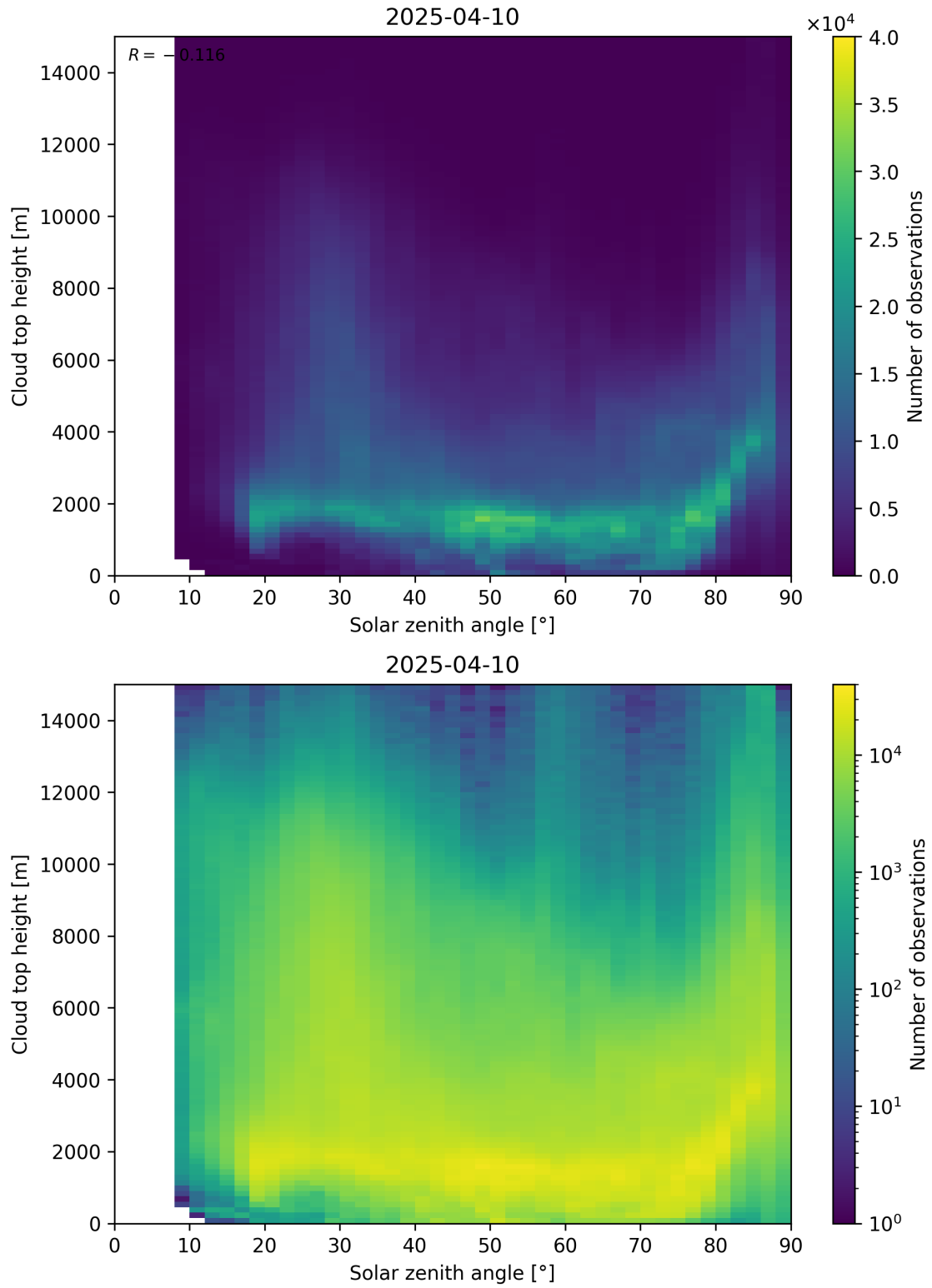
Figure 104: Scatter density plot of “Solar zenith angle” against “Cloud top height” for 2025-04-09 to 2025-04-11.
