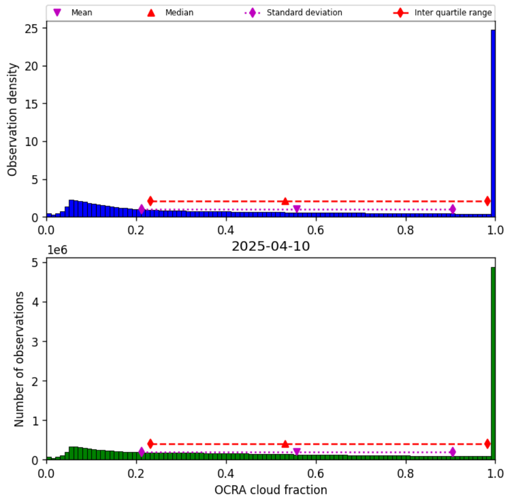
Figure 50: Histogram of “OCRA cloud fraction” for 2025-04-09 to 2025-04-11
