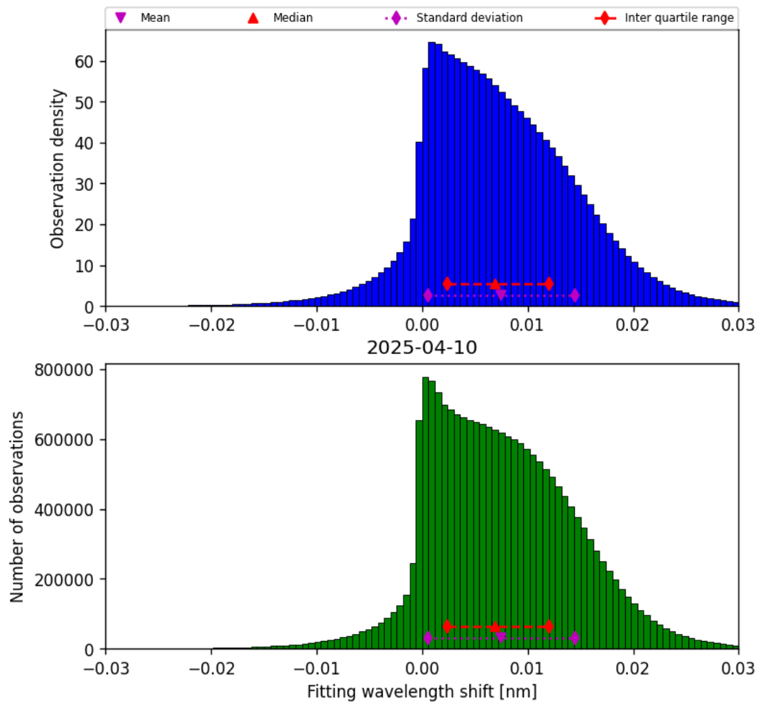
Figure 49: Histogram of “Fitting wavelength shift” for 2025-04-09 to 2025-04-11
