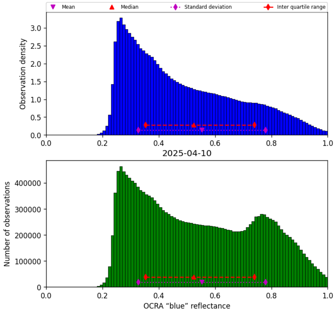
Figure 51: Histogram of “OCRA “blue” reflectance” for 2025-04-09 to 2025-04-11
