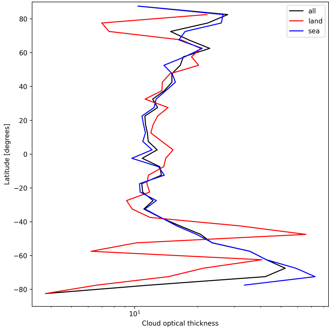
Figure 25: Zonal average of “Cloud optical thickness” for 2025-04-09 to 2025-04-11.
