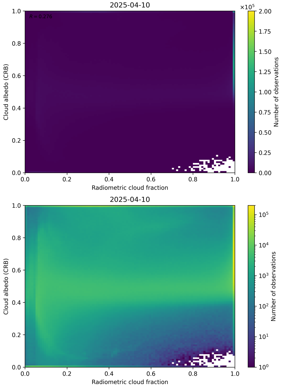
Figure 71: Scatter density plot of “Radiometric cloud fraction” against “Cloud albedo (CRB)” for 2025-04-09 to 2025-04-11.
