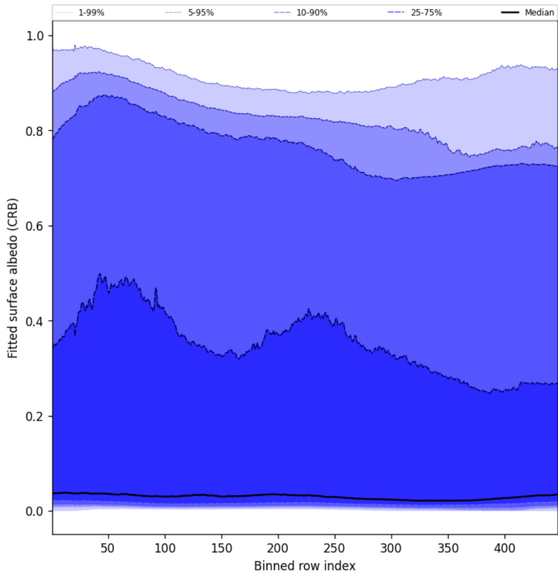
Figure 62: Along track statistics of “Fitted surface albedo (CRB)” for 2025-04-09 to 2025-04-11
