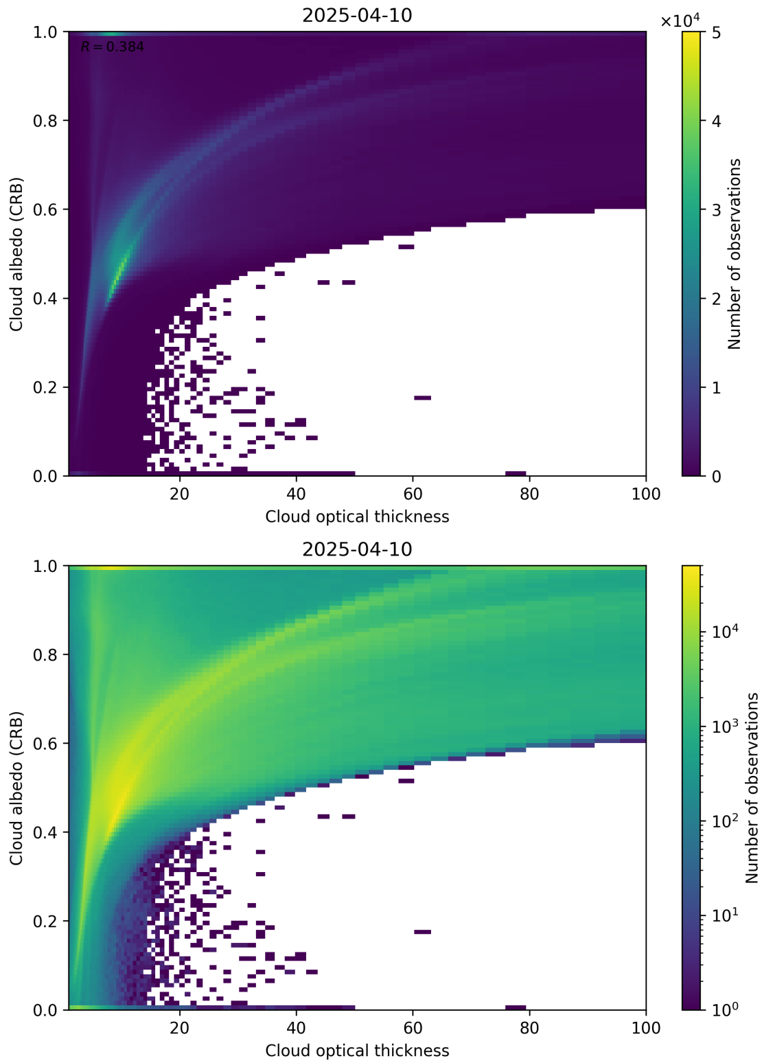
Figure 82: Scatter density plot of “Cloud optical thickness” against “Cloud albedo (CRB)” for 2025-04-09 to 2025-04-11.
