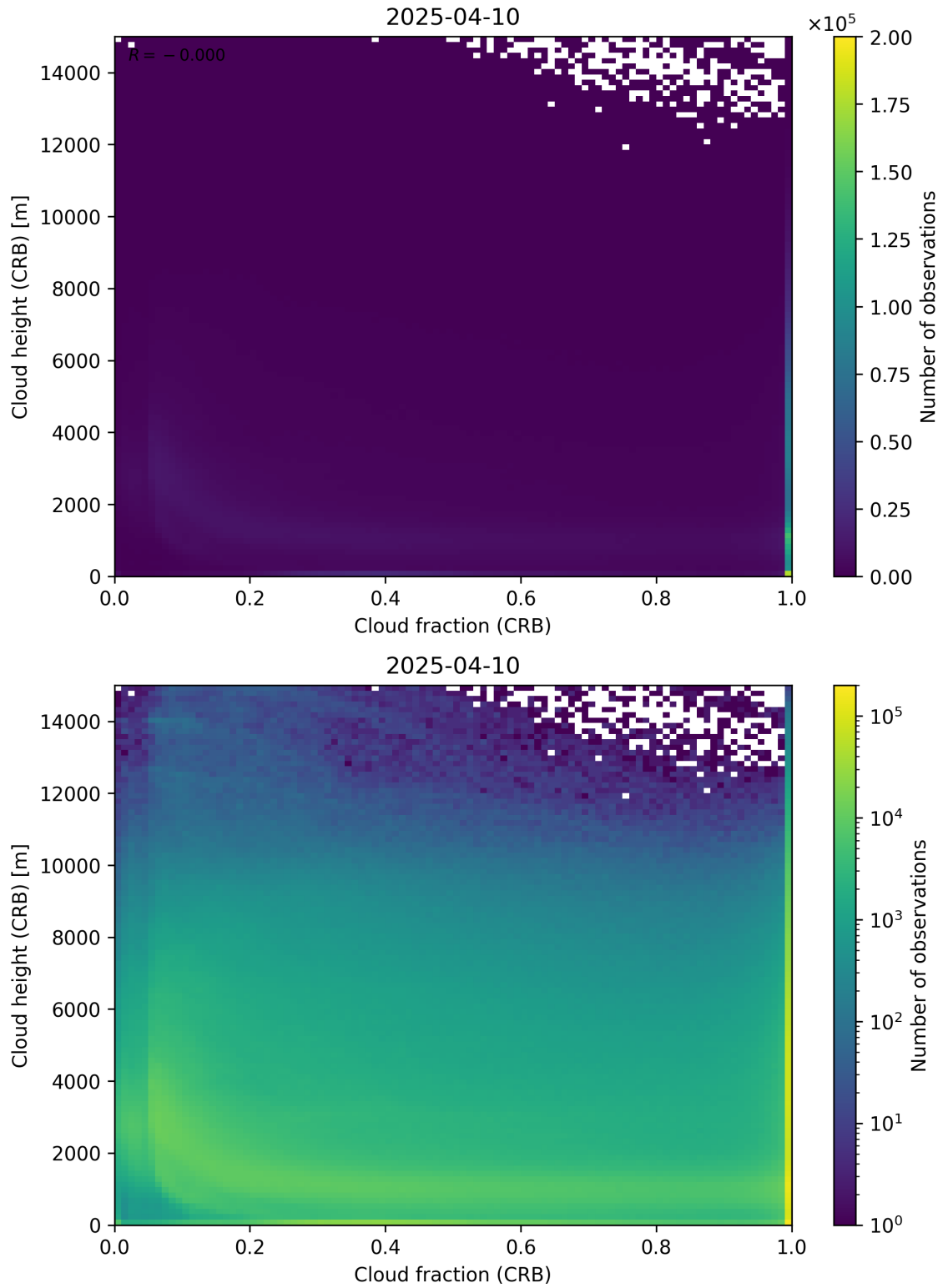
Figure 79: Scatter density plot of “Cloud fraction (CRB)” against “Cloud height (CRB)” for 2025-04-09 to 2025-04-11.
