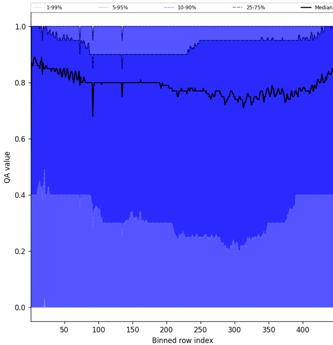
Figure 54: Along track statistics of “QA value” for 2025-04-09 to 2025-04-11
