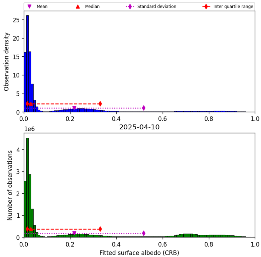
Figure 46: Histogram of “Fitted surface albedo (CRB)” for 2025-04-09 to 2025-04-11
