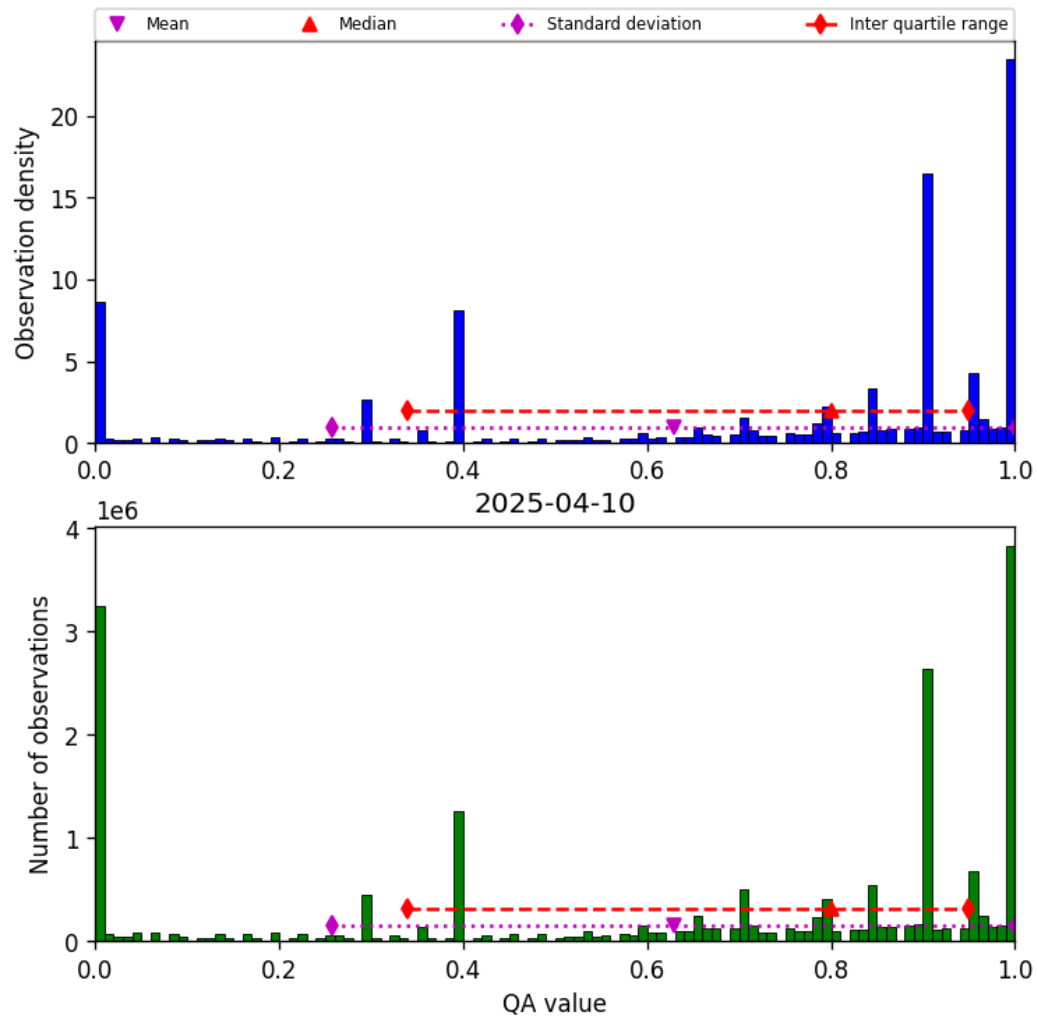
Figure 38: Histogram of “QA value” for 2025-04-09 to 2025-04-11
