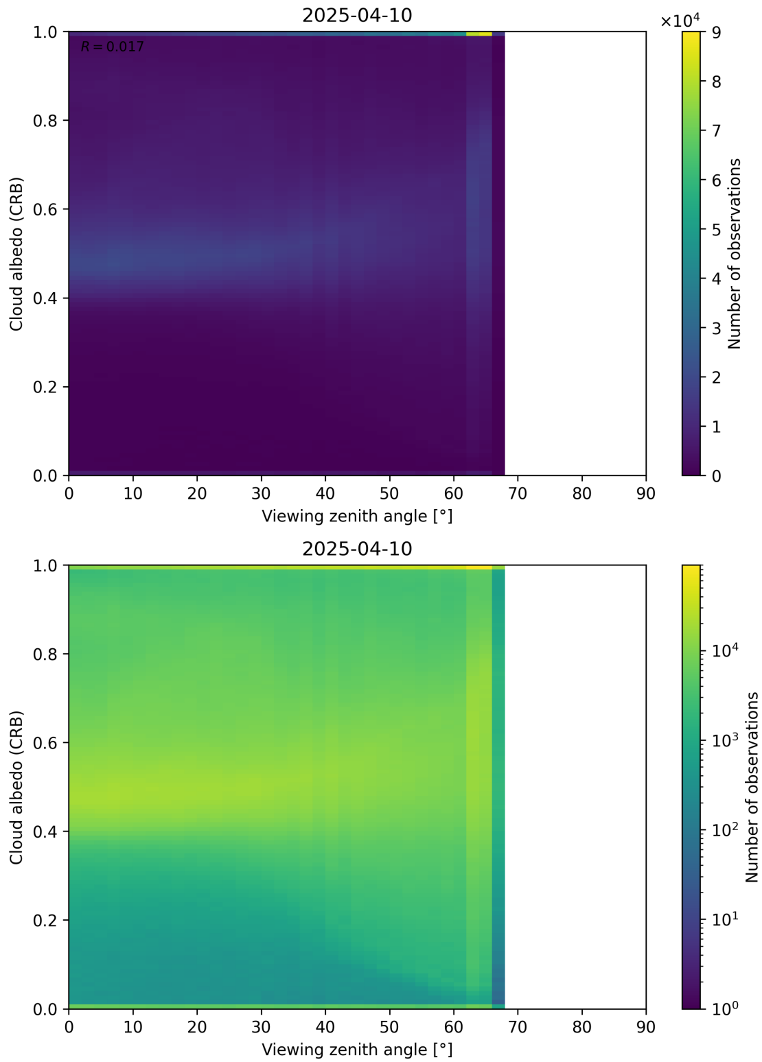
Figure 106: Scatter density plot of “Viewing zenith angle” against “Cloud albedo (CRB)” for 2025-04-09 to 2025-04-11.
