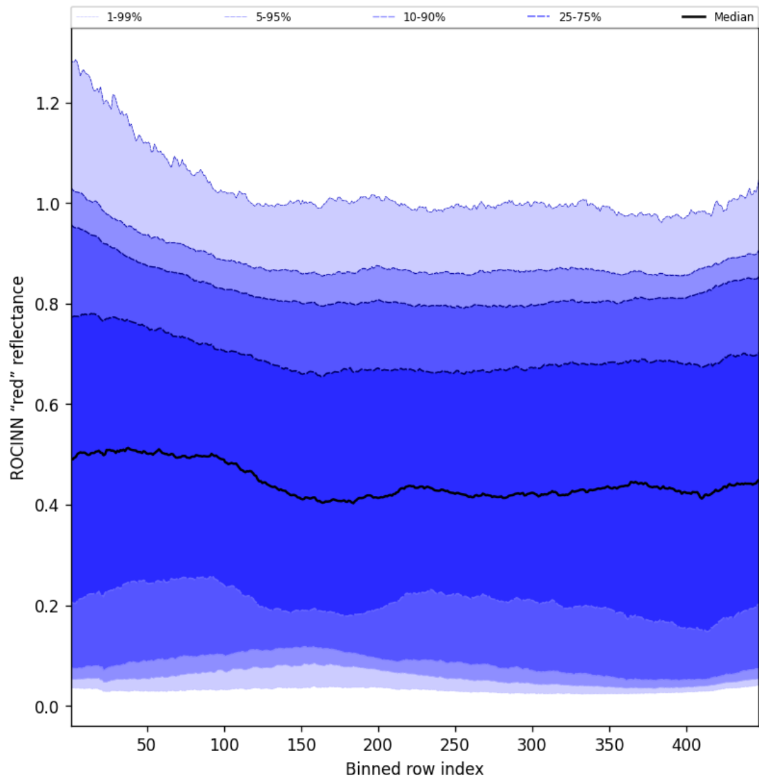
Figure 69: Along track statistics of “ROCINN “red” reflectance” for 2025-04-09 to 2025-04-11
