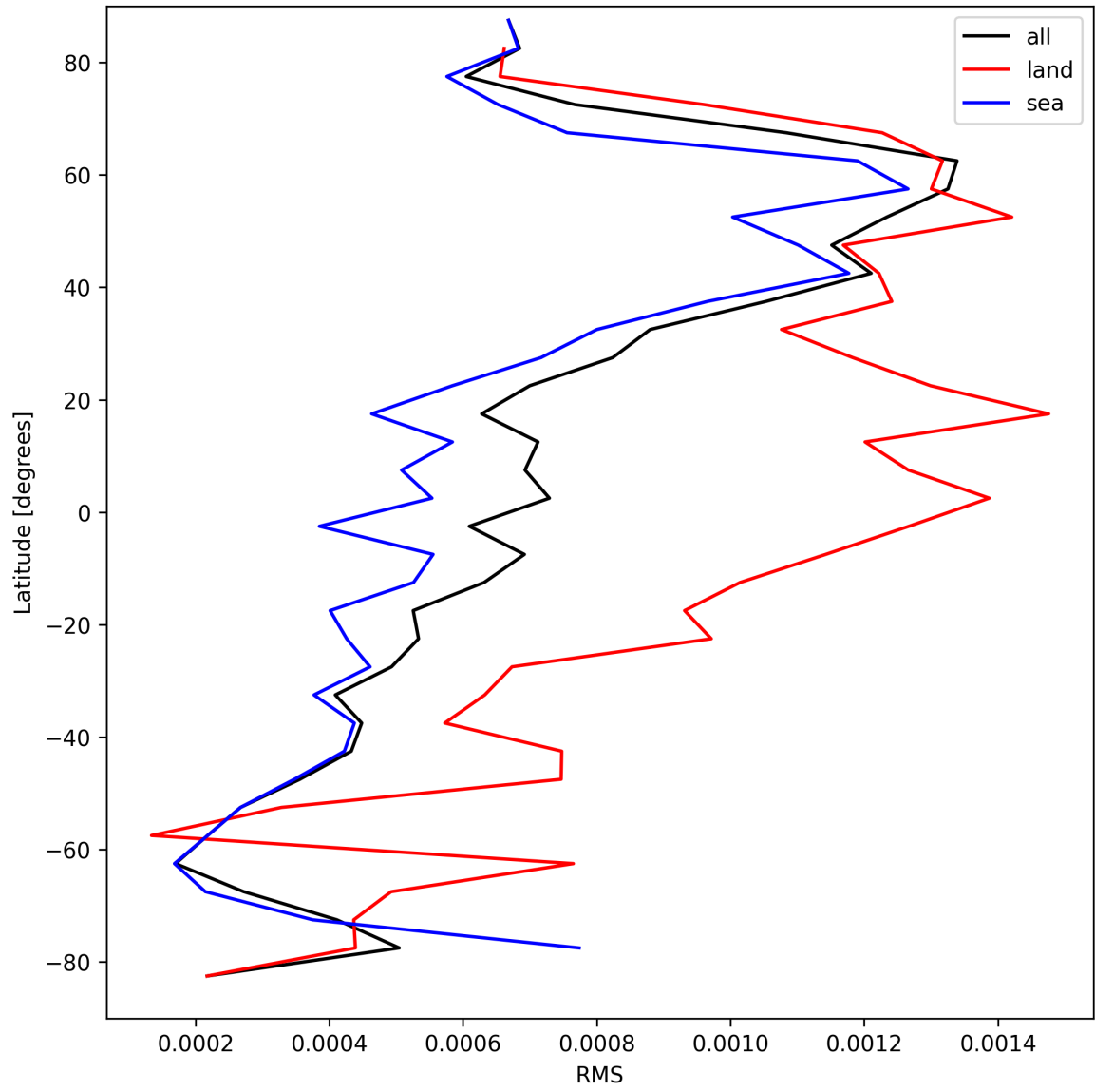
Figure 31: Zonal average of “RMS” for 2025-04-09 to 2025-04-11.
