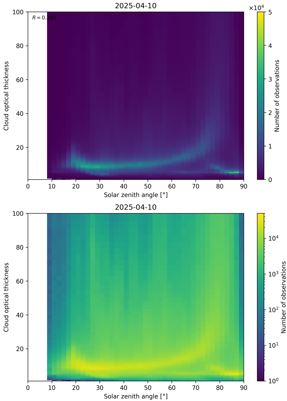
Figure 103: Scatter density plot of “Solar zenith angle” against “Cloud optical thickness” for 2025-04-09 to 2025-04-11.
