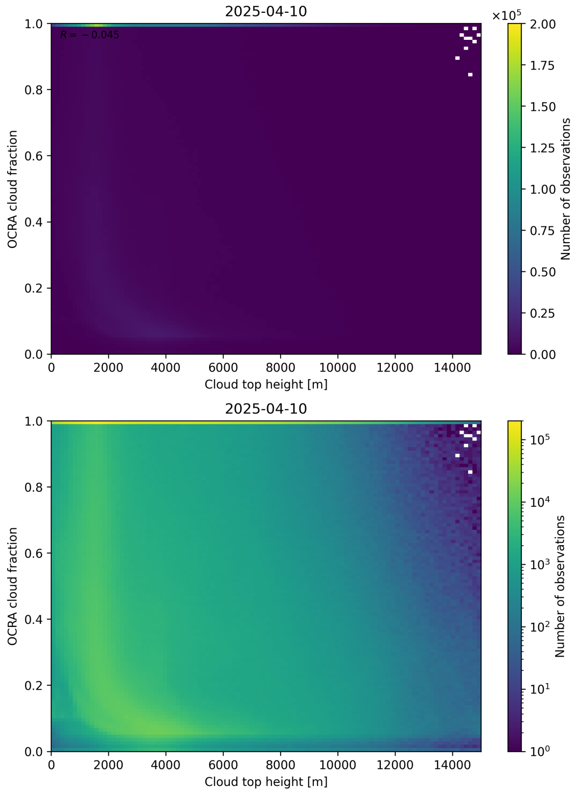
Figure 87: Scatter density plot of “Cloud top height” against “OCRA cloud fraction” for 2025-04-09 to 2025-04-11.
