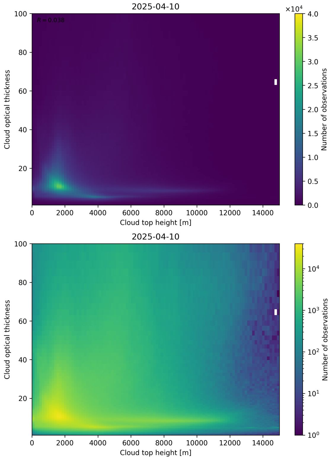
Figure 90: Scatter density plot of “Cloud top height” against “Cloud optical thickness” for 2025-04-09 to 2025-04-11.
