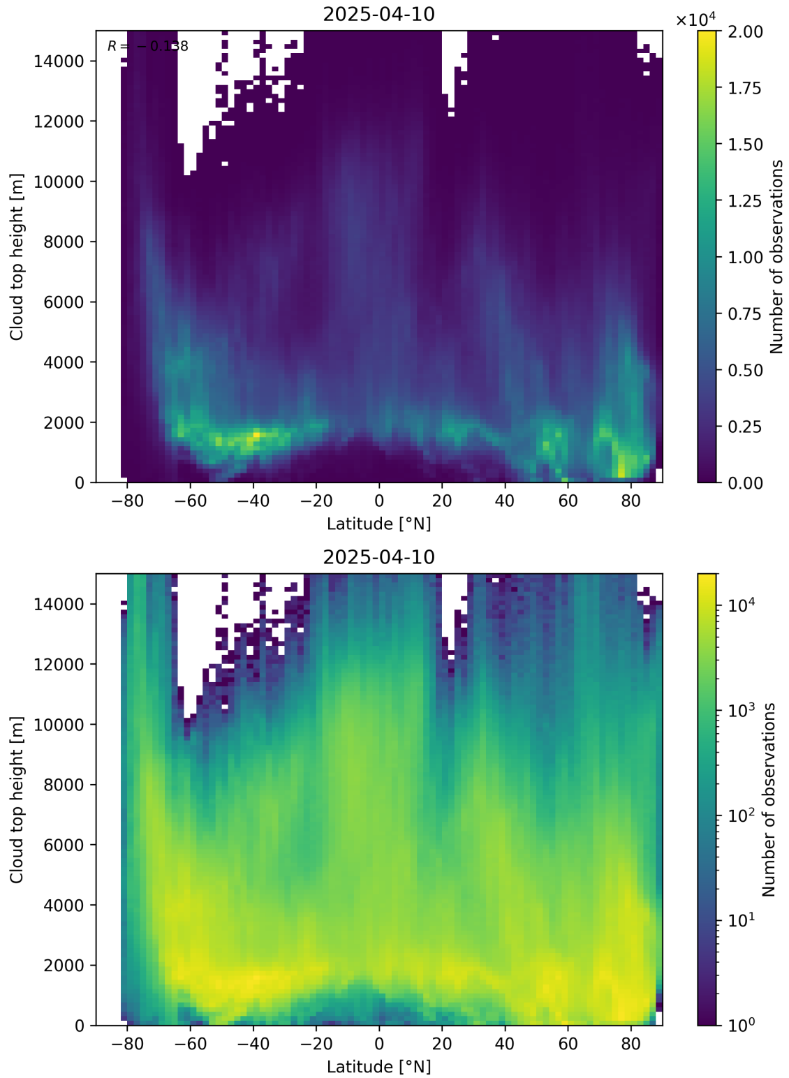
Figure 97: Scatter density plot of “Latitude” against “Cloud top height” for 2025-04-09 to 2025-04-11.
