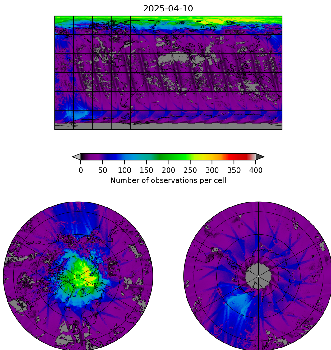
Figure 21: Map of the number of observations for 2025-04-09 to 2025-04-11
