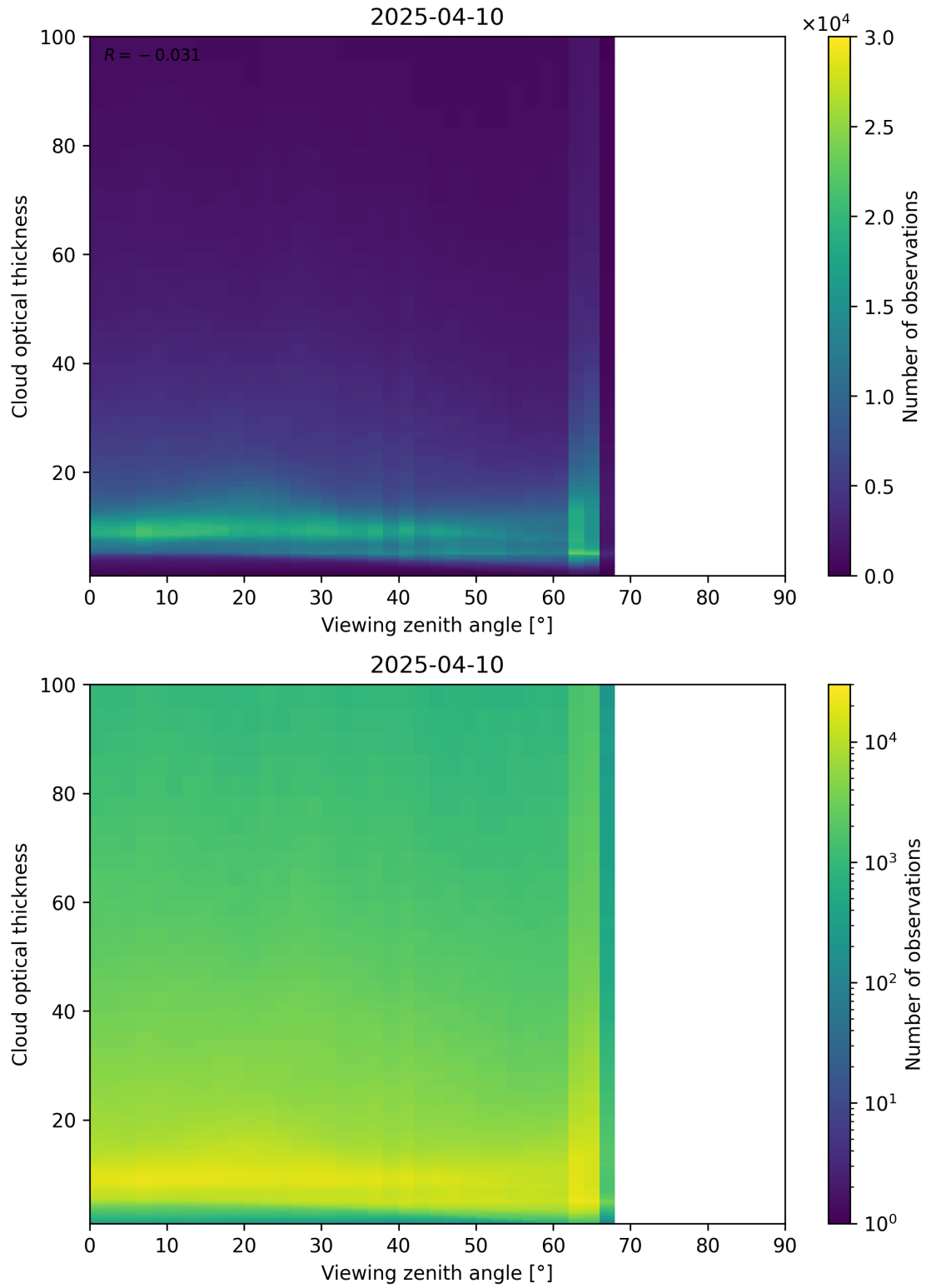
Figure 111: Scatter density plot of “Viewing zenith angle” against “Cloud optical thickness” for 2025-04-09 to 2025-04-11.
