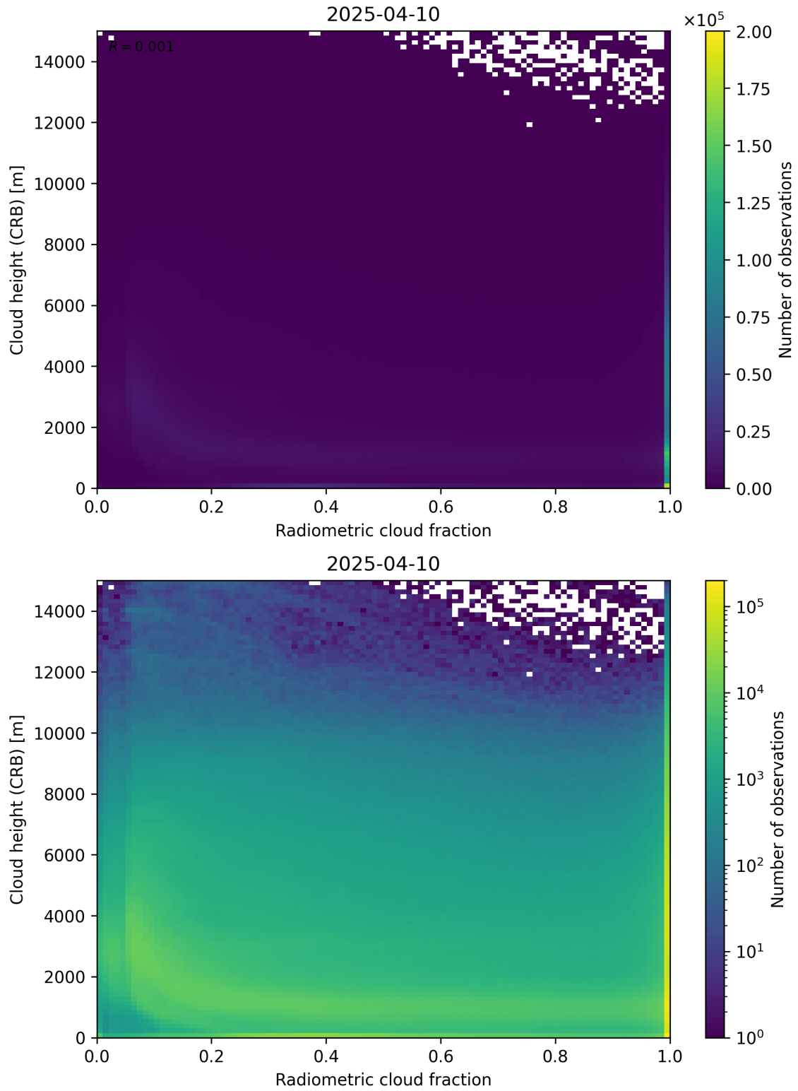
Figure 74: Scatter density plot of “Radiometric cloud fraction” against “Cloud height (CRB)” for 2025-04-09 to 2025-04-11.
