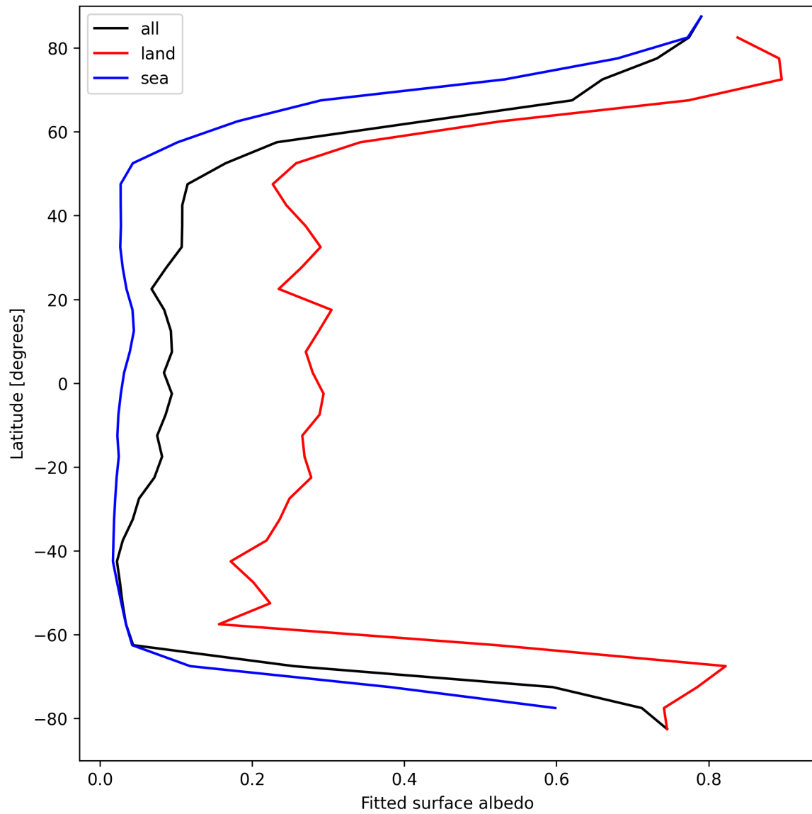
Figure 29: Zonal average of “Fitted surface albedo” for 2025-04-09 to 2025-04-11.
