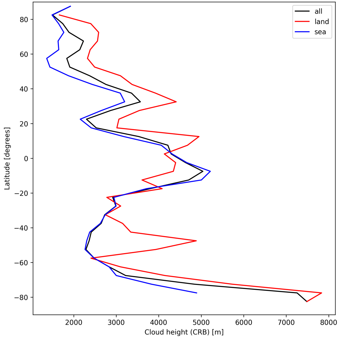
Figure 27: Zonal average of “Cloud height (CRB)” for 2025-04-09 to 2025-04-11.
