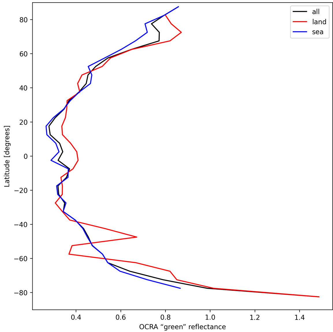
Figure 36: Zonal average of “OCRA “green” reflectance” for 2025-04-09 to 2025-04-11.
