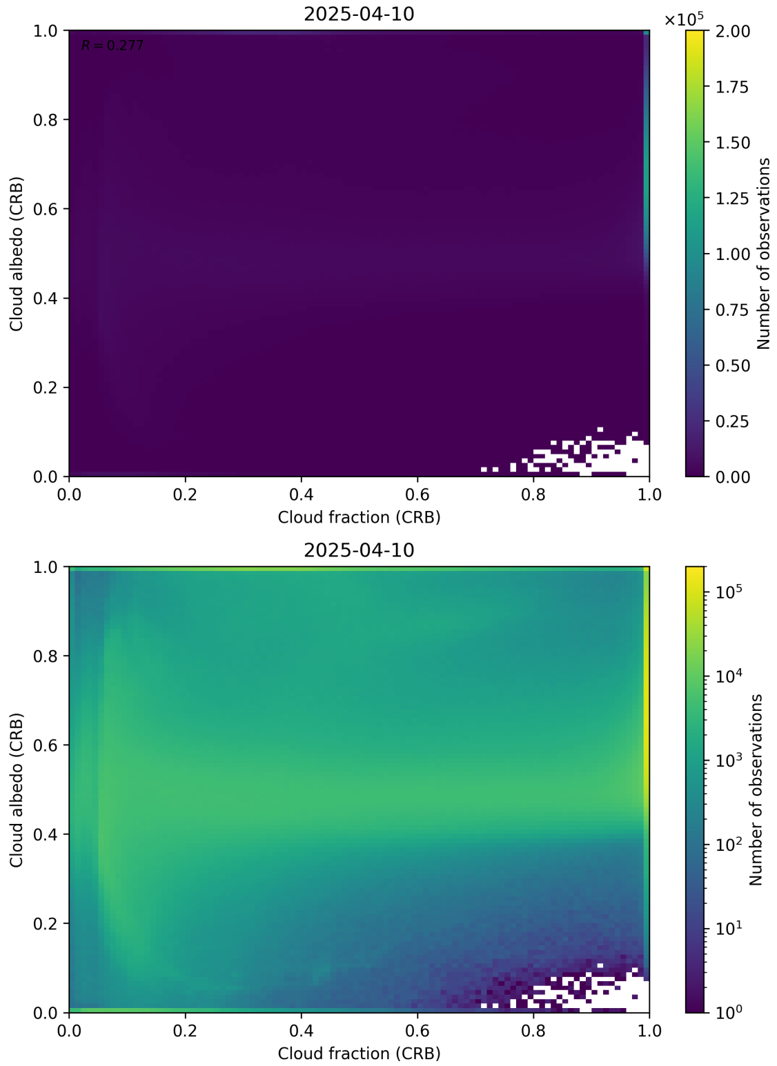
Figure 77: Scatter density plot of “Cloud fraction (CRB)” against “Cloud albedo (CRB)” for 2025-04-09 to 2025-04-11.
