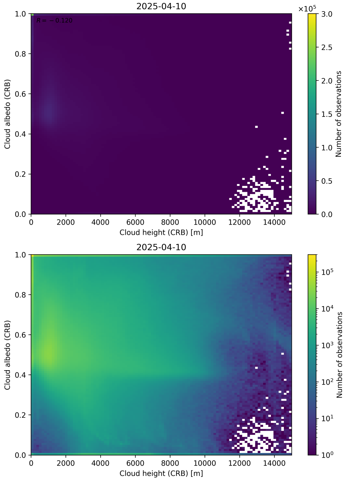
Figure 80: Scatter density plot of “Cloud height (CRB)” against “Cloud albedo (CRB)” for 2025-04-09 to 2025-04-11.
