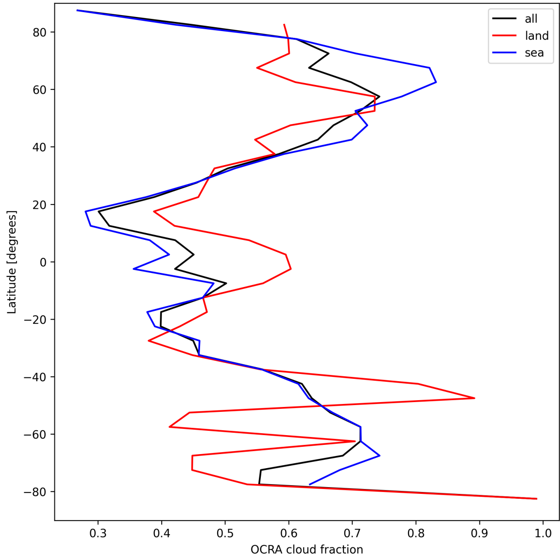
Figure 34: Zonal average of “OCRA cloud fraction” for 2025-04-09 to 2025-04-11.
