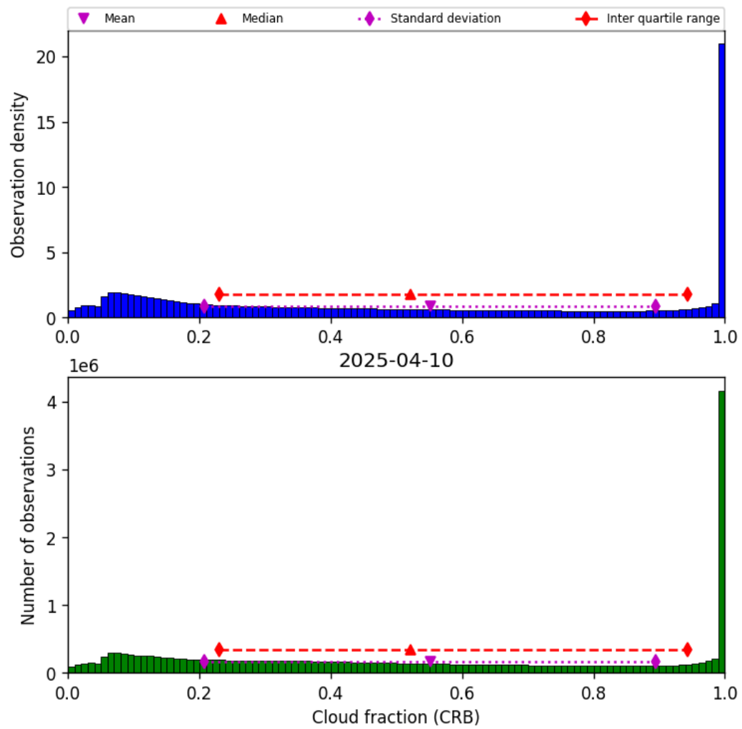
Figure 42: Histogram of “Cloud fraction (CRB)” for 2025-04-09 to 2025-04-11
