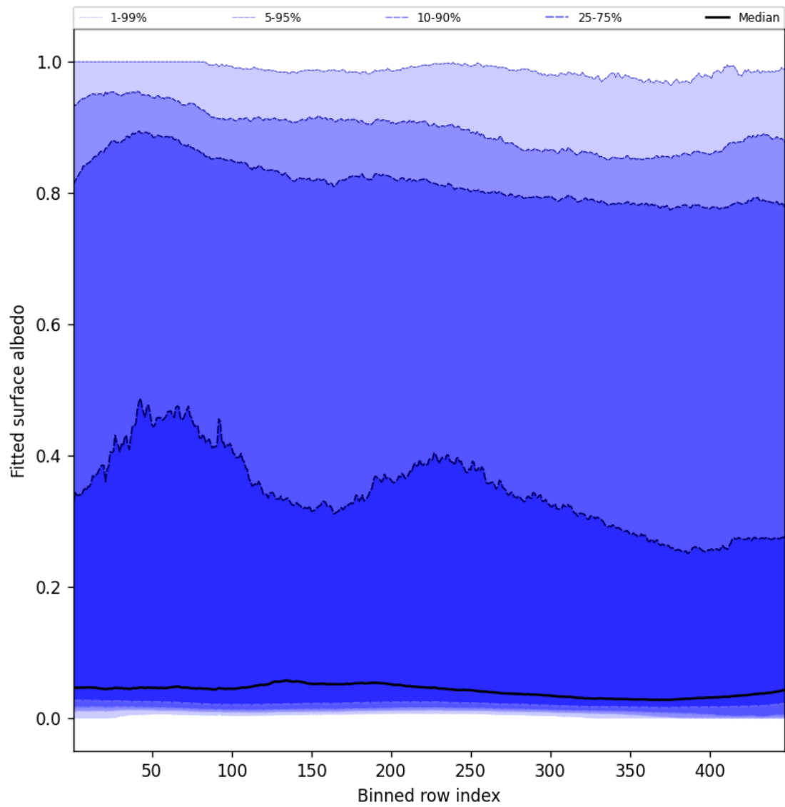
Figure 61: Along track statistics of “Fitted surface albedo” for 2025-04-09 to 2025-04-11
