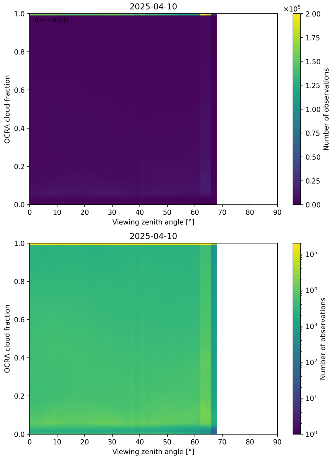
Figure 108: Scatter density plot of “Viewing zenith angle” against “OCRA cloud fraction” for 2025-04-09 to 2025-04-11.
