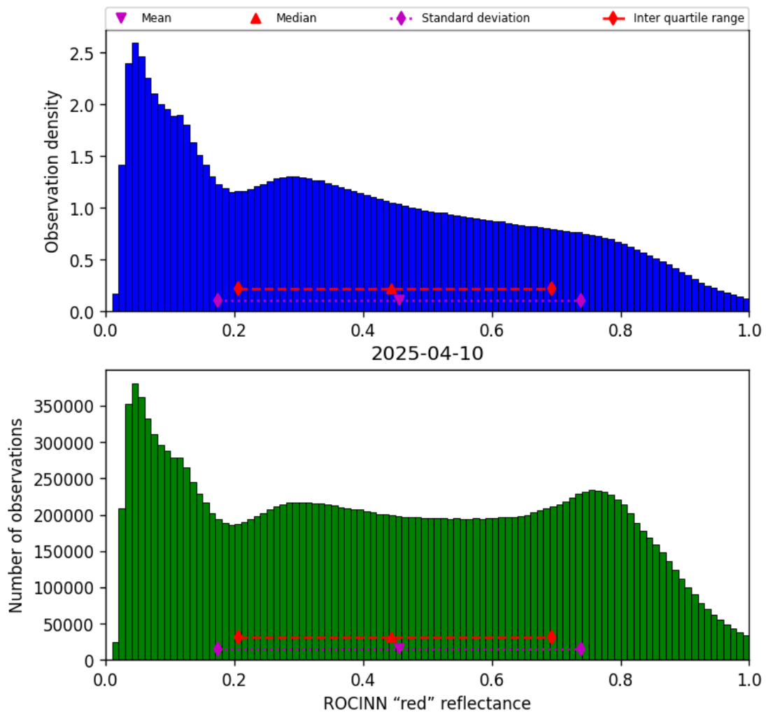
Figure 53: Histogram of “ROCINN “red” reflectance” for 2025-04-09 to 2025-04-11
