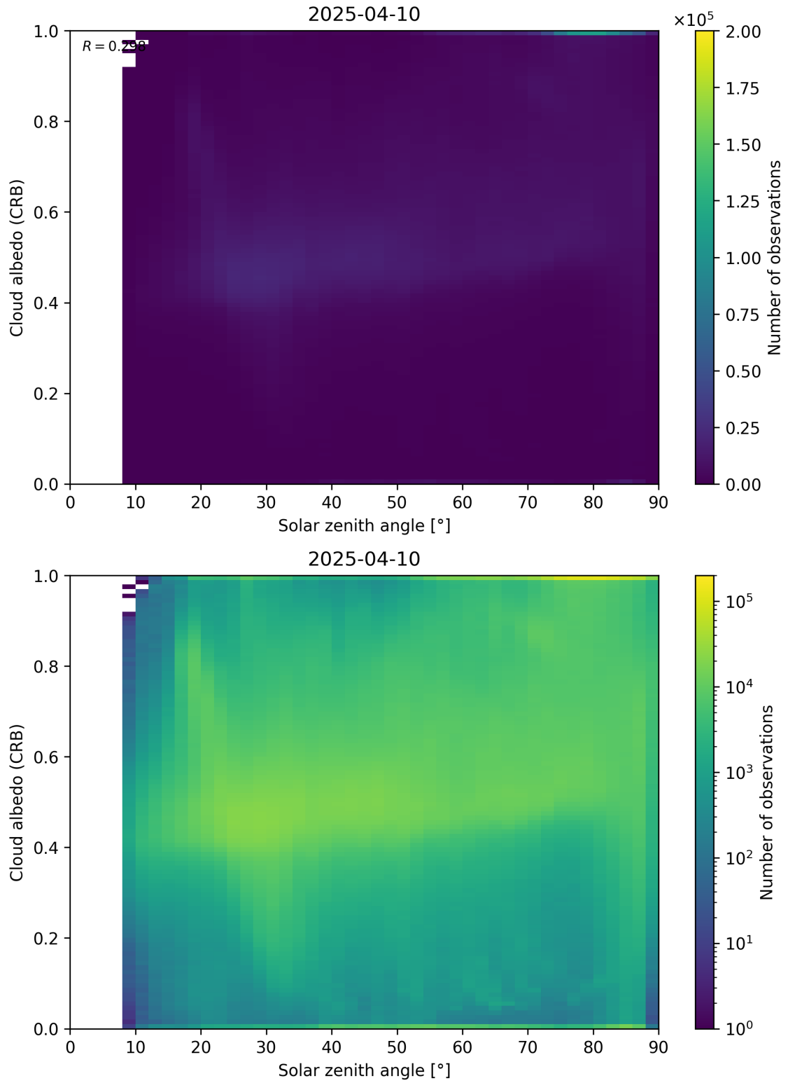
Figure 98: Scatter density plot of “Solar zenith angle” against “Cloud albedo (CRB)” for 2025-04-09 to 2025-04-11.
