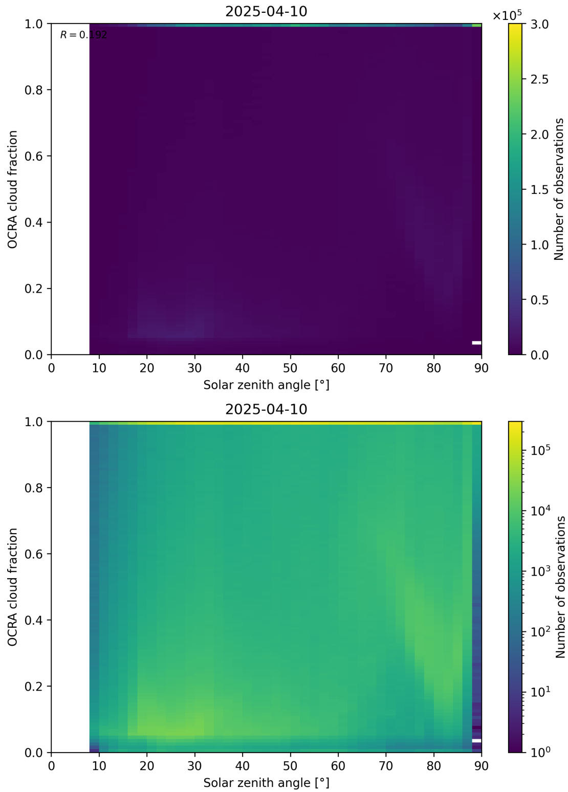
Figure 100: Scatter density plot of “Solar zenith angle” against “OCRA cloud fraction” for 2025-04-09 to 2025-04-11.
