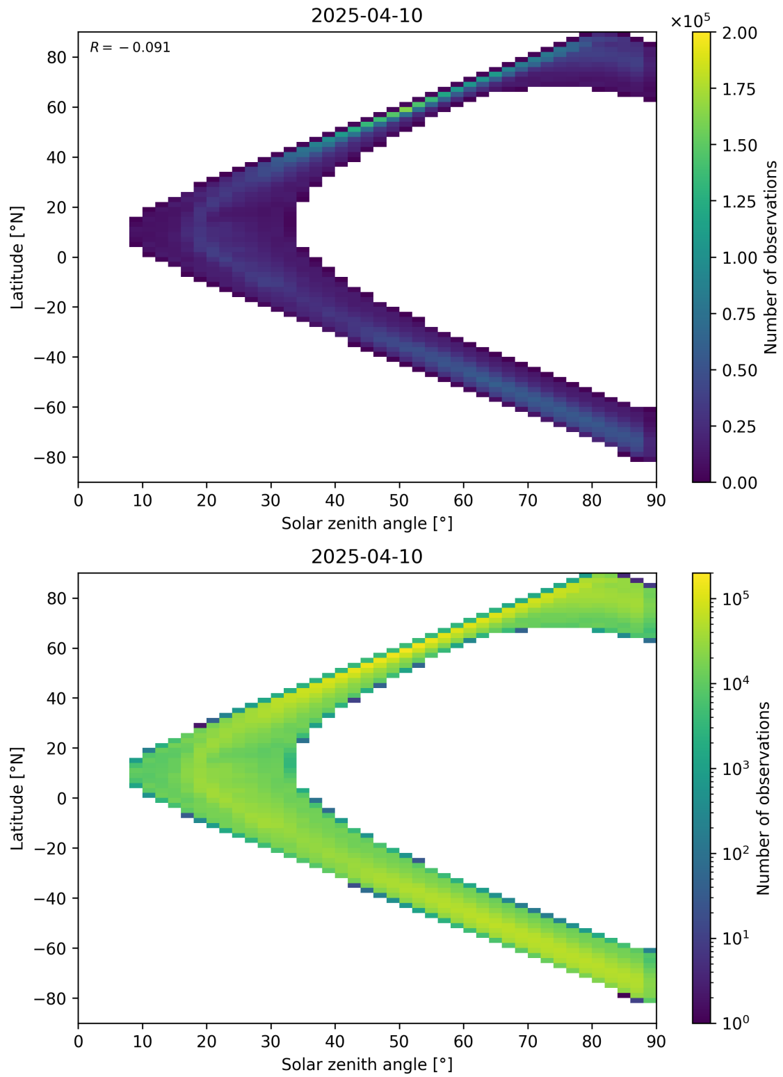
Figure 105: Scatter density plot of “Solar zenith angle” against “Latitude” for 2025-04-09 to 2025-04-11.
