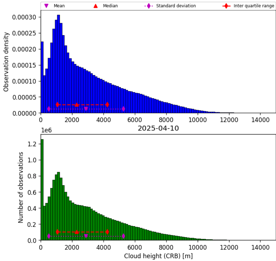
Figure 43: Histogram of “Cloud height (CRB)” for 2025-04-09 to 2025-04-11
