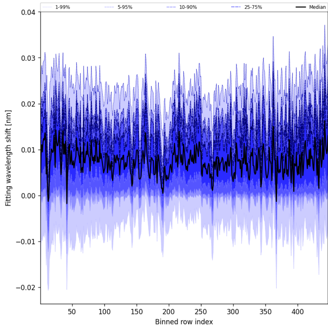
Figure 65: Along track statistics of “Fitting wavelength shift” for 2025-04-09 to 2025-04-11
