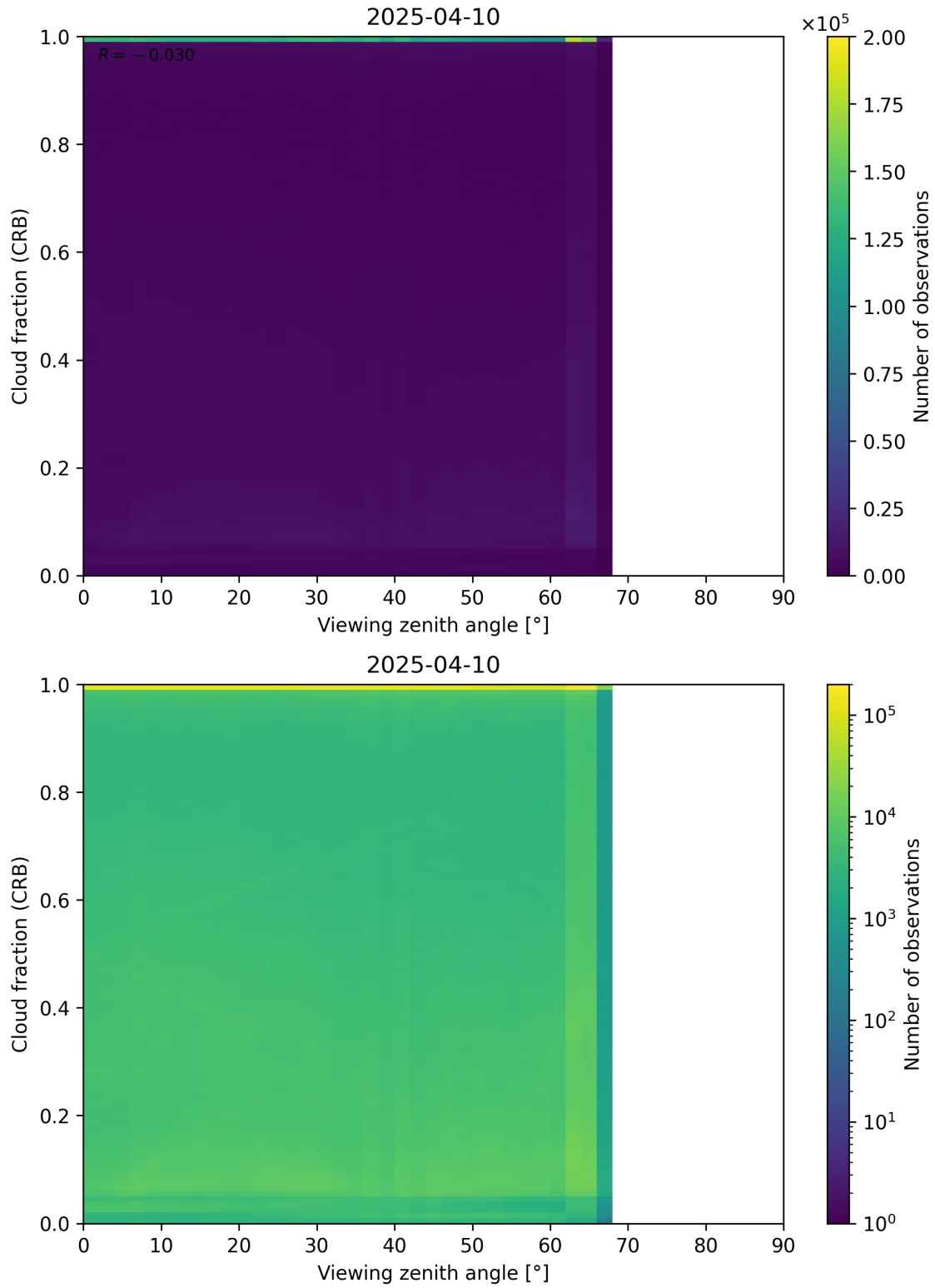
Figure 109: Scatter density plot of “Viewing zenith angle” against “Cloud fraction (CRB)” for 2025-04-09 to 2025-04-11.
