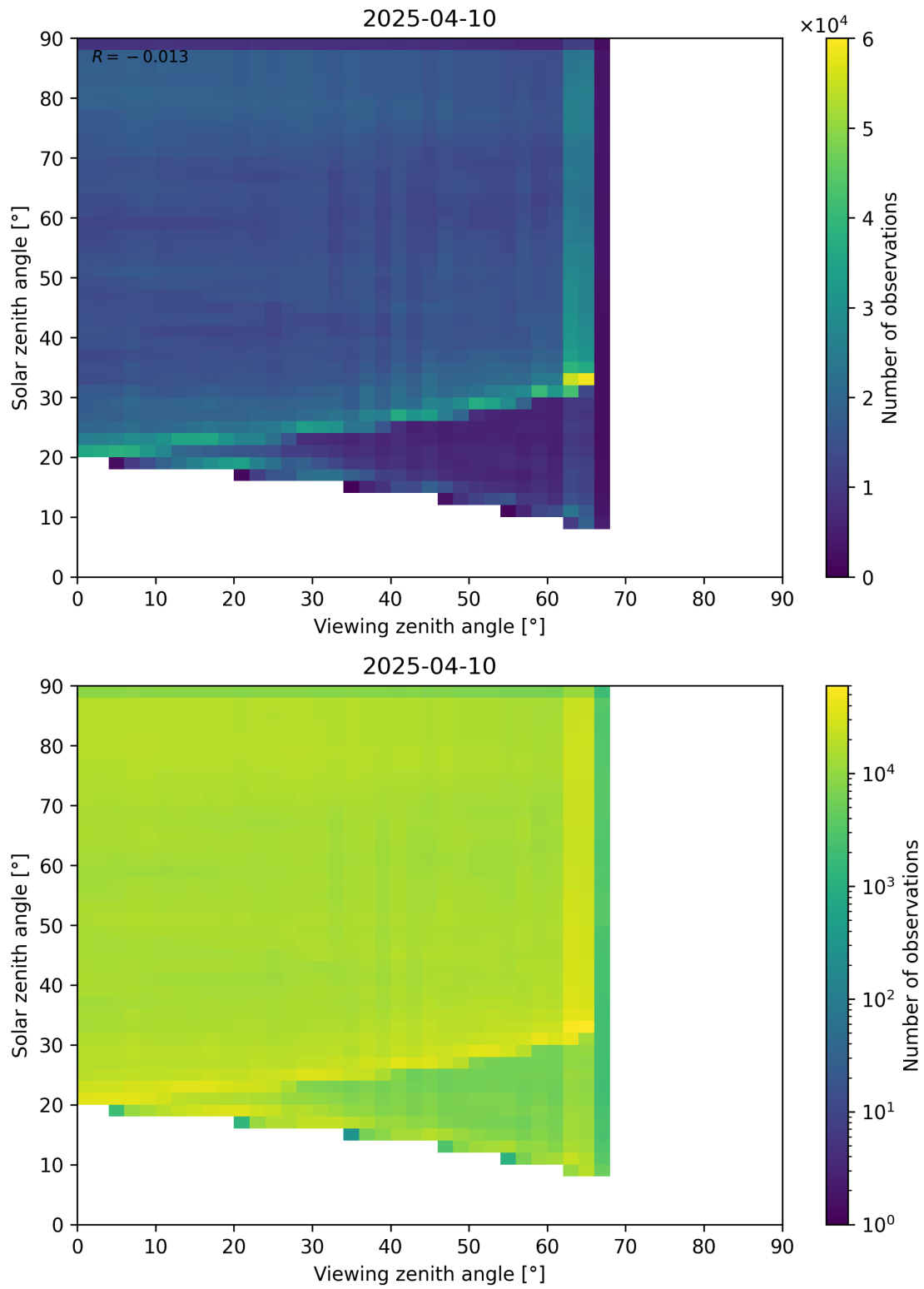
Figure 114: Scatter density plot of “Viewing zenith angle” against “Solar zenith angle” for 2025-04-09 to 2025-04-11.
