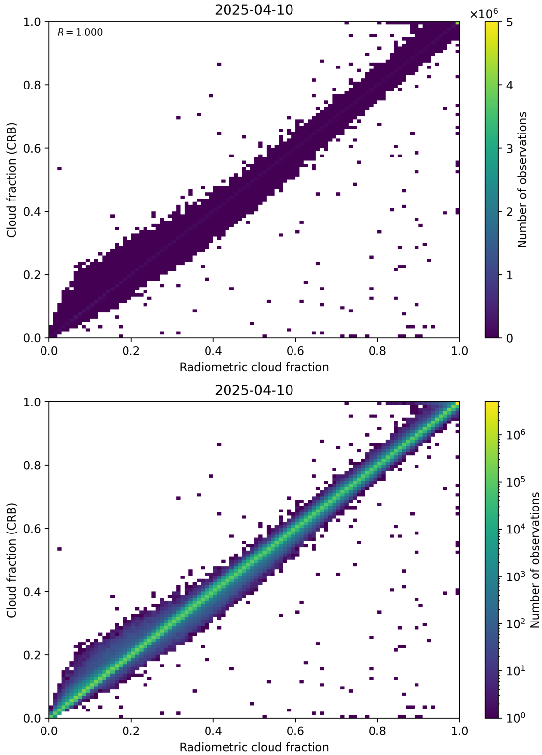
Figure 73: Scatter density plot of “Radiometric cloud fraction” against “Cloud fraction (CRB)” for 2025-04-09 to 2025-04-11.
