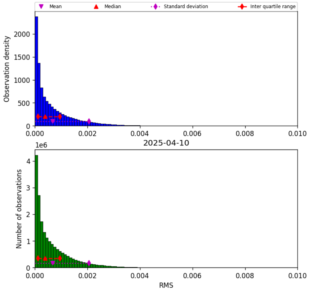
Figure 47: Histogram of “RMS” for 2025-04-09 to 2025-04-11
