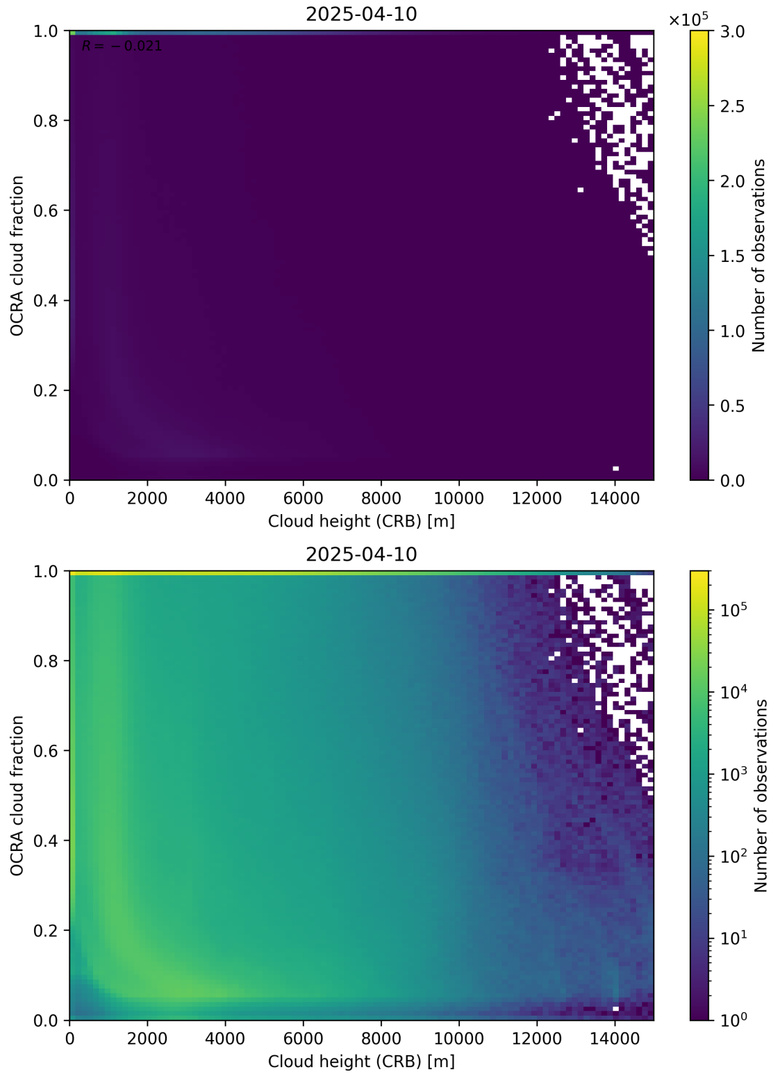
Figure 81: Scatter density plot of “Cloud height (CRB)” against “OCRA cloud fraction” for 2025-04-09 to 2025-04-11.
