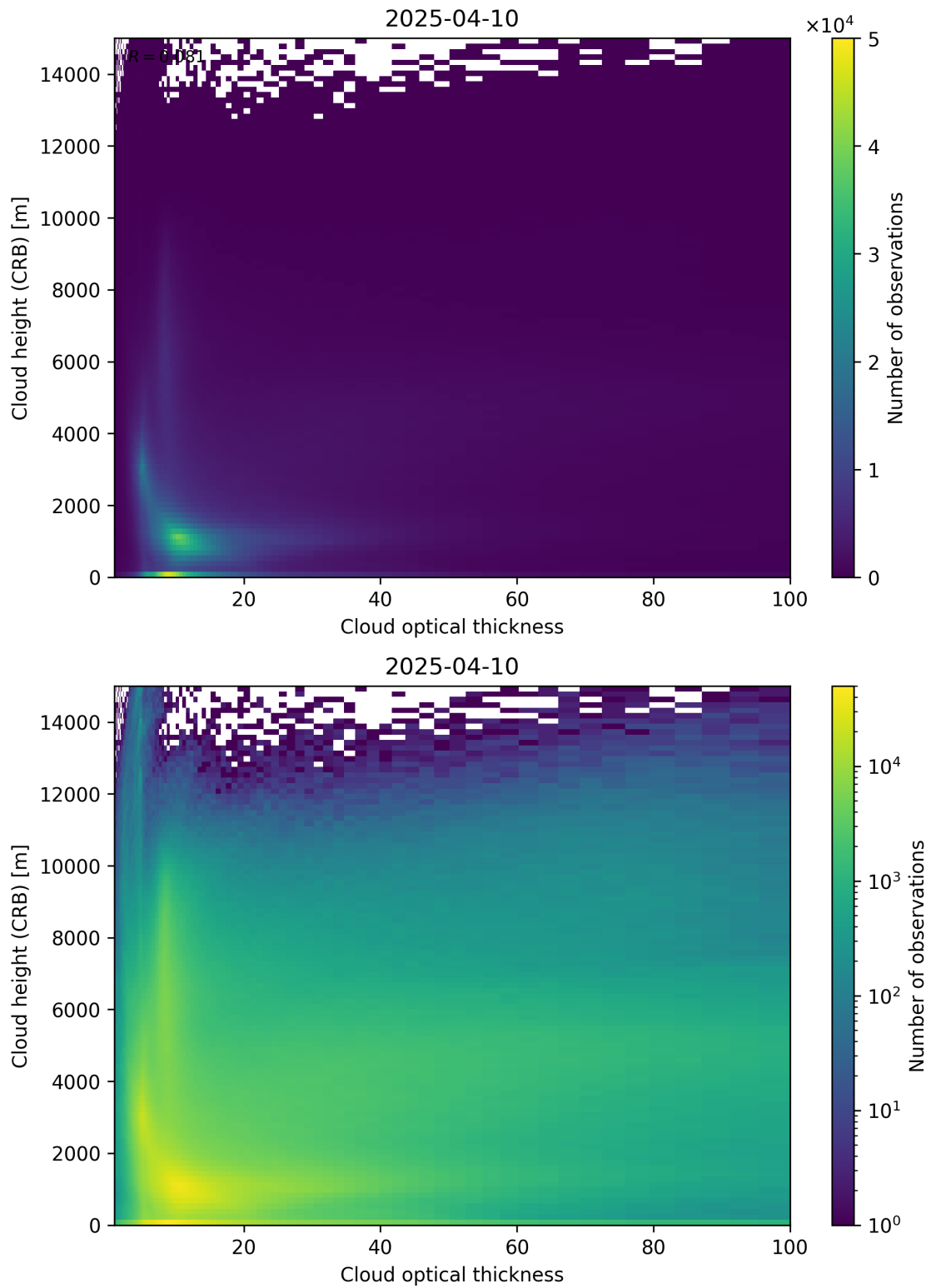
Figure 85: Scatter density plot of “Cloud optical thickness” against “Cloud height (CRB)” for 2025-04-09 to 2025-04-11.
