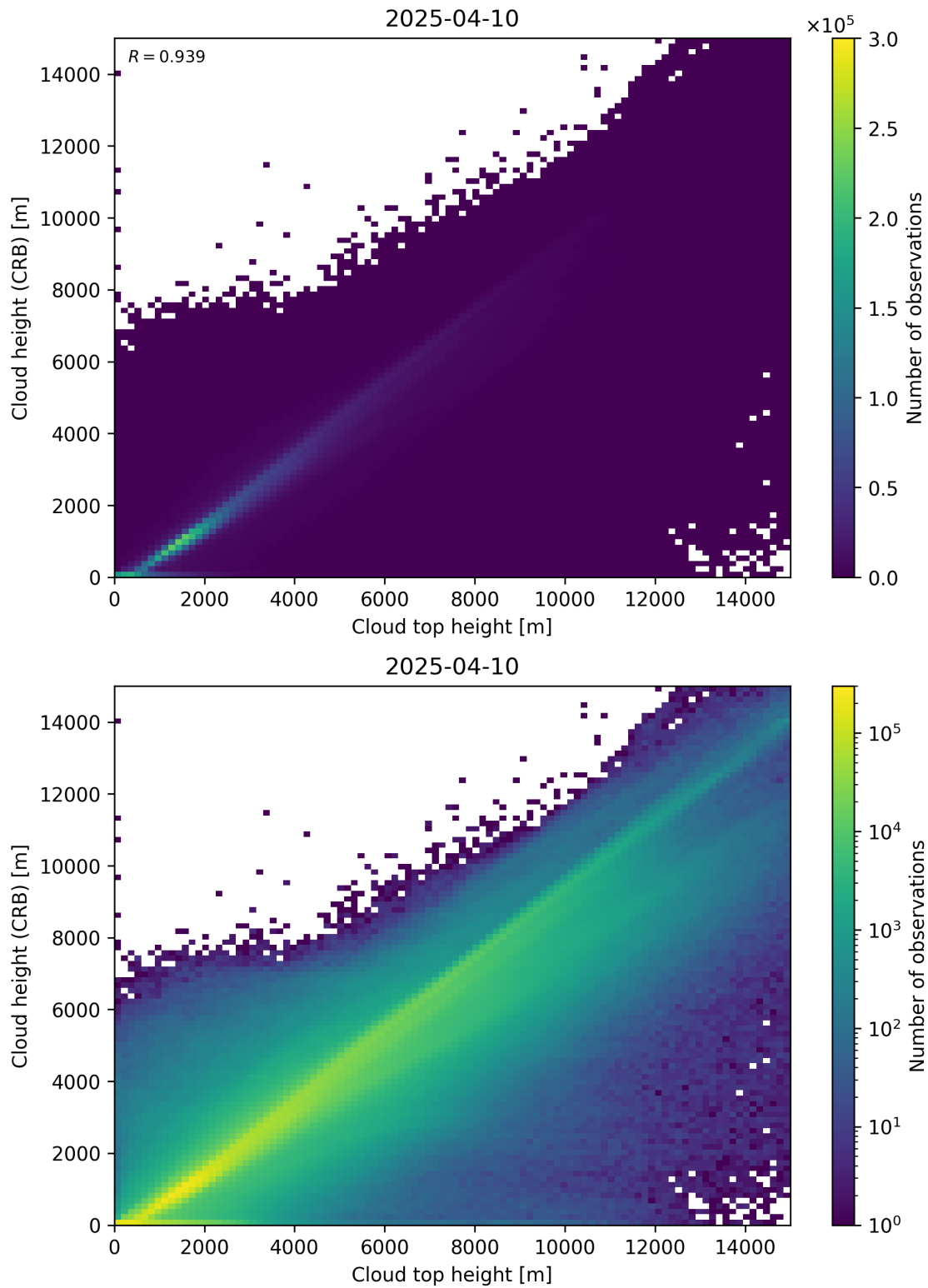
Figure 89: Scatter density plot of “Cloud top height” against “Cloud height (CRB)” for 2025-04-09 to 2025-04-11.
