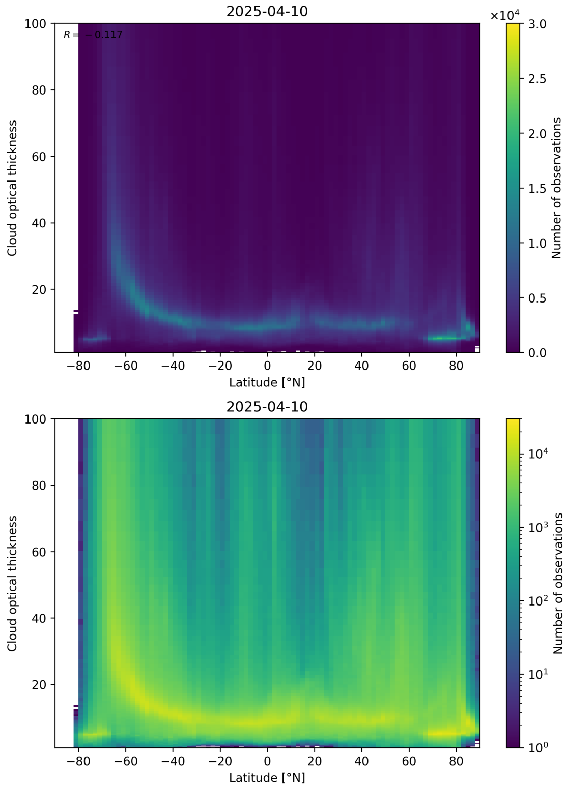
Figure 96: Scatter density plot of “Latitude” against “Cloud optical thickness” for 2025-04-09 to 2025-04-11.
