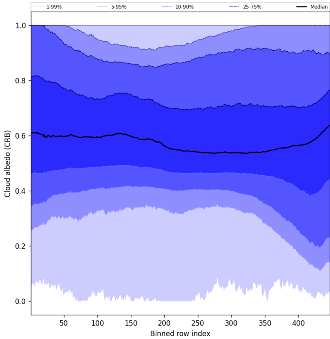
Figure 60: Along track statistics of “Cloud albedo (CRB)” for 2025-04-09 to 2025-04-11
