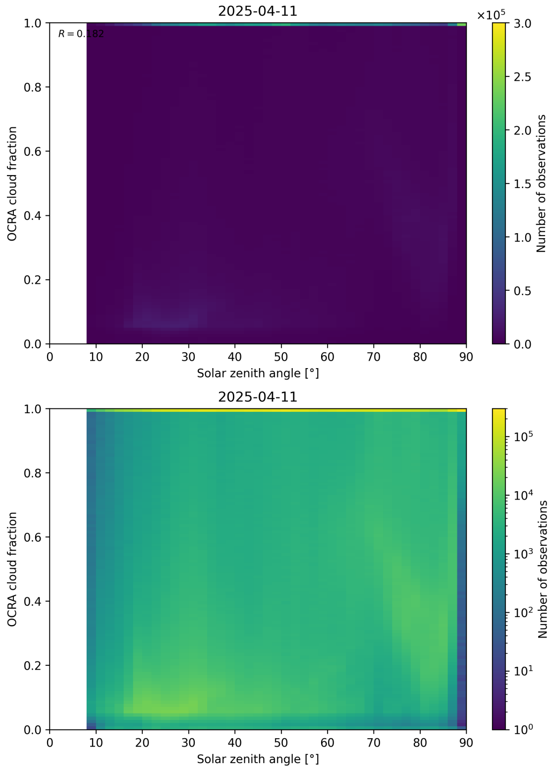
Figure 100: Scatter density plot of “Solar zenith angle” against “OCRA cloud fraction” for 2025-04-10 to 2025-04-12.
