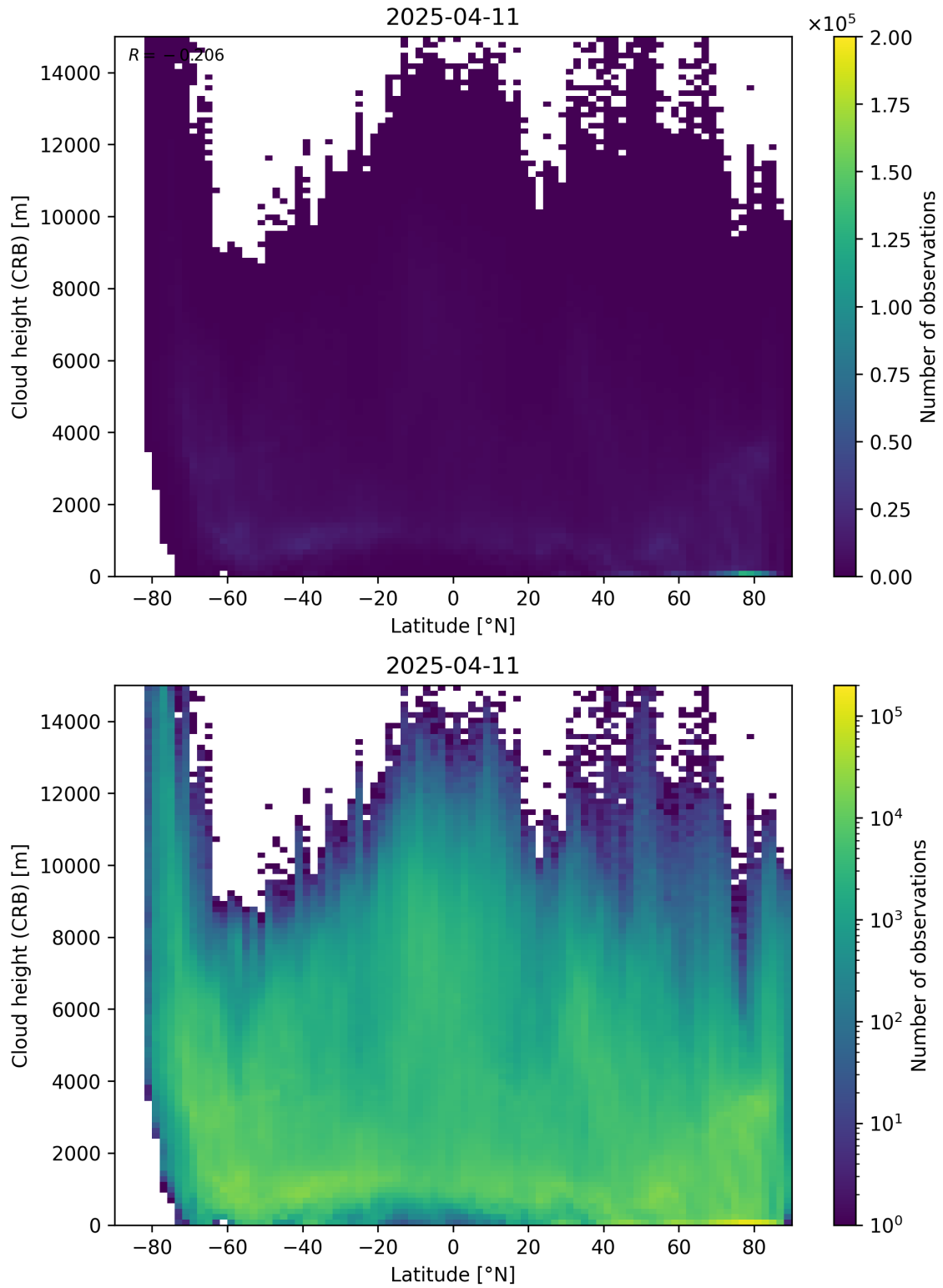
Figure 95: Scatter density plot of “Latitude” against “Cloud height (CRB)” for 2025-04-10 to 2025-04-12.
