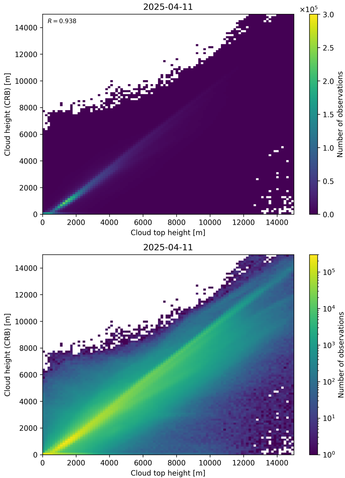
Figure 89: Scatter density plot of “Cloud top height” against “Cloud height (CRB)” for 2025-04-10 to 2025-04-12.
