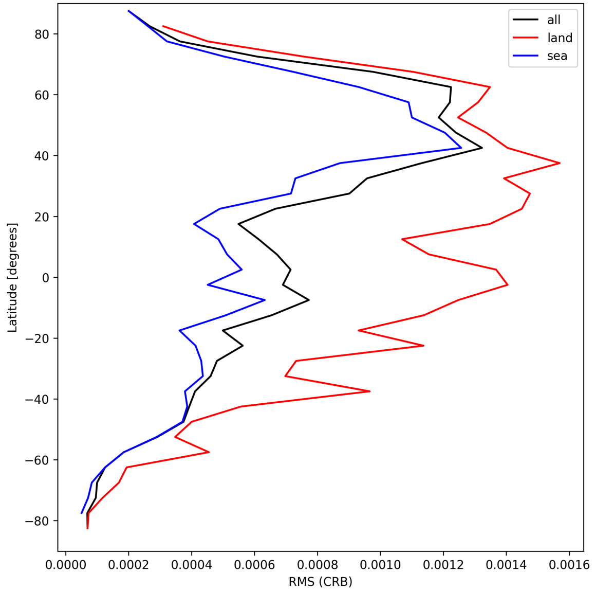
Figure 32: Zonal average of “RMS (CRB)” for 2025-04-10 to 2025-04-12.
