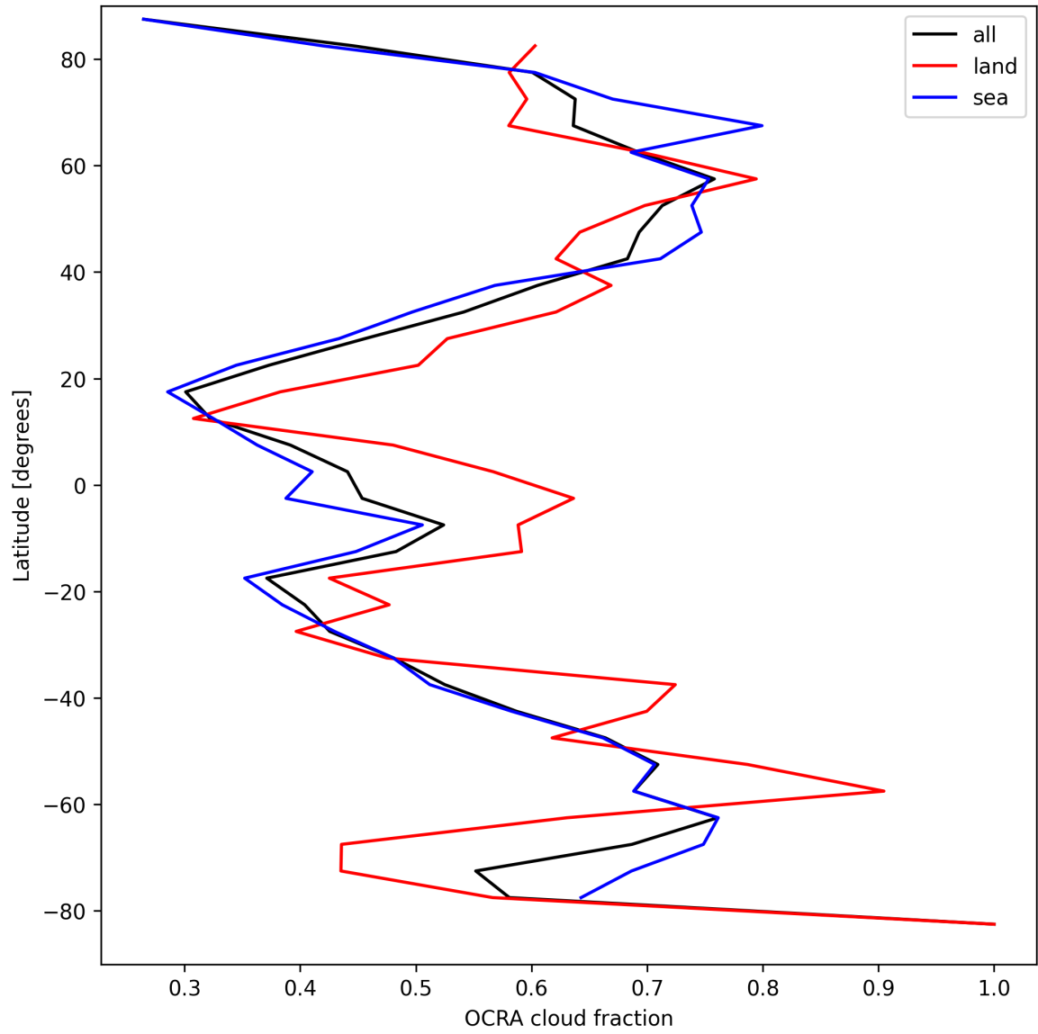
Figure 34: Zonal average of “OCRA cloud fraction” for 2025-04-10 to 2025-04-12.
