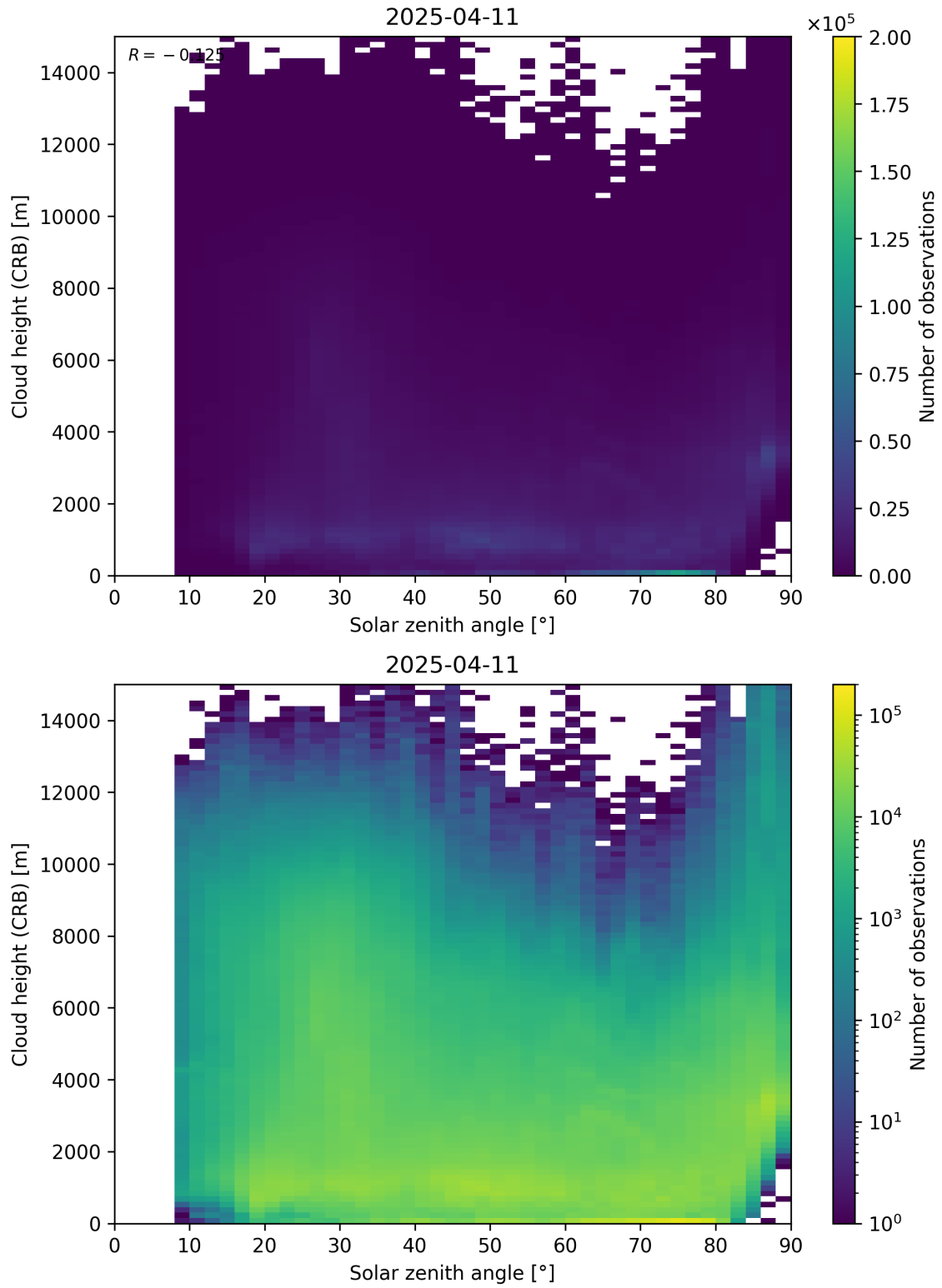
Figure 102: Scatter density plot of “Solar zenith angle” against “Cloud height (CRB)” for 2025-04-10 to 2025-04-12.
