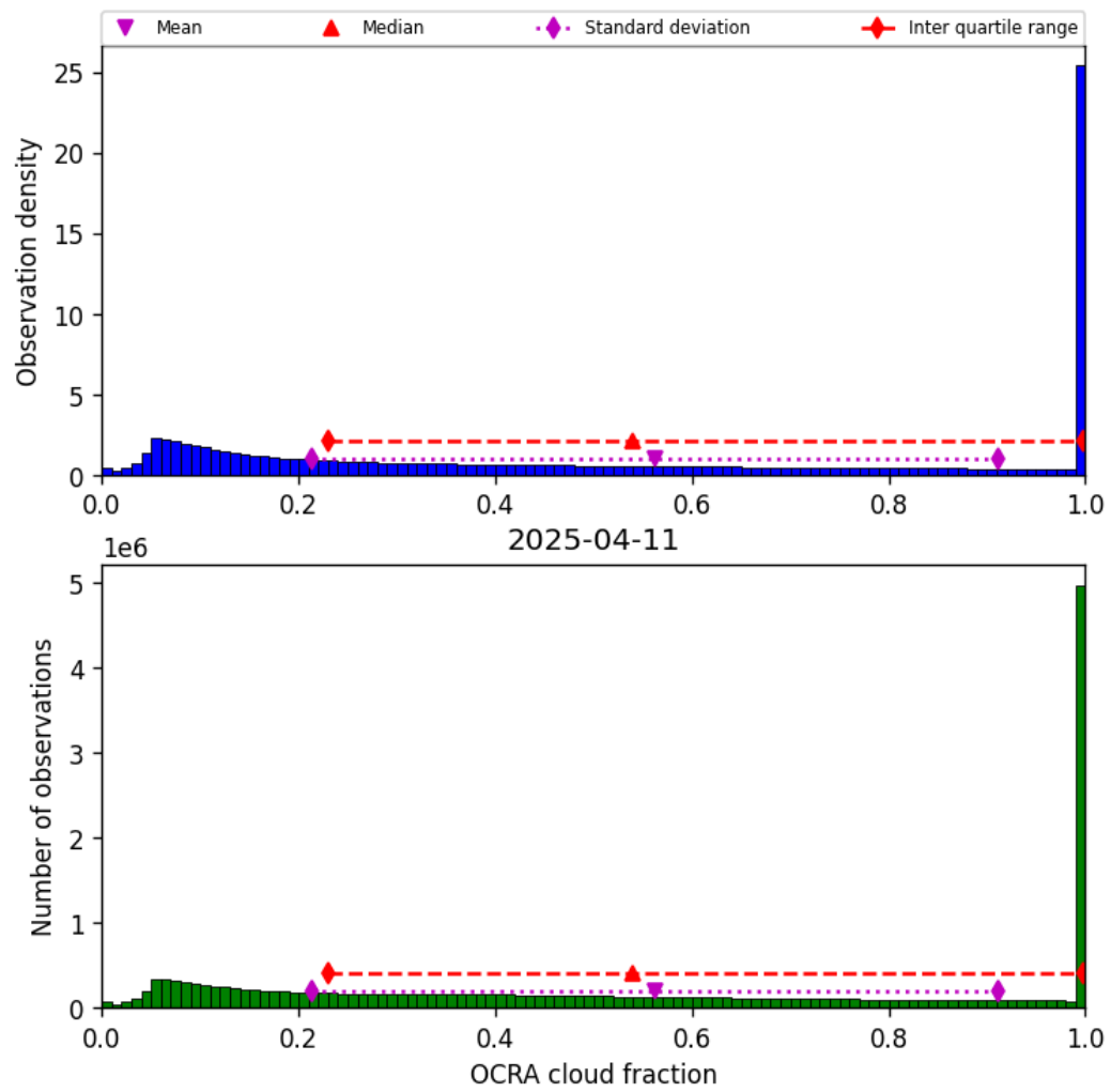
Figure 50: Histogram of “OCRA cloud fraction” for 2025-04-10 to 2025-04-12
