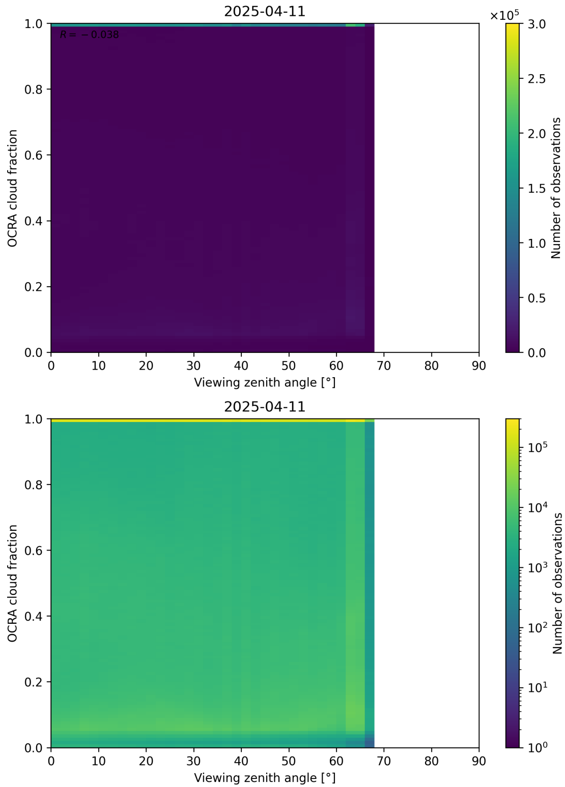
Figure 108: Scatter density plot of “Viewing zenith angle” against “OCRA cloud fraction” for 2025-04-10 to 2025-04-12.
