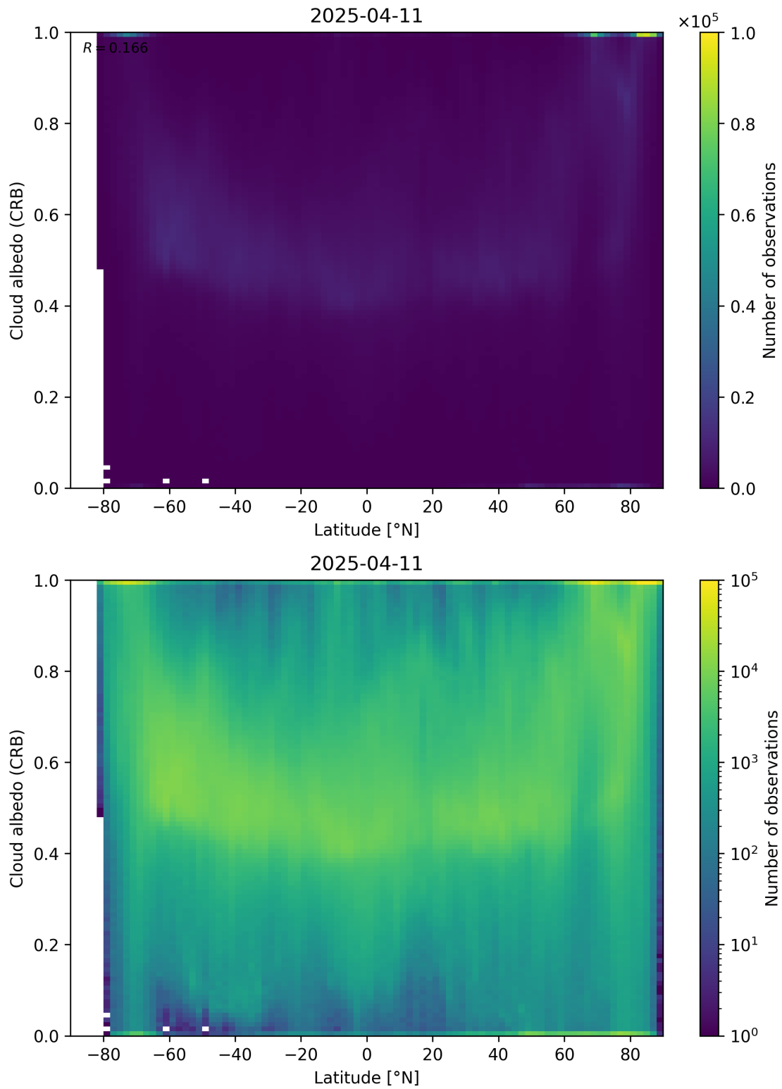
Figure 91: Scatter density plot of “Latitude” against “Cloud albedo (CRB)” for 2025-04-10 to 2025-04-12.
