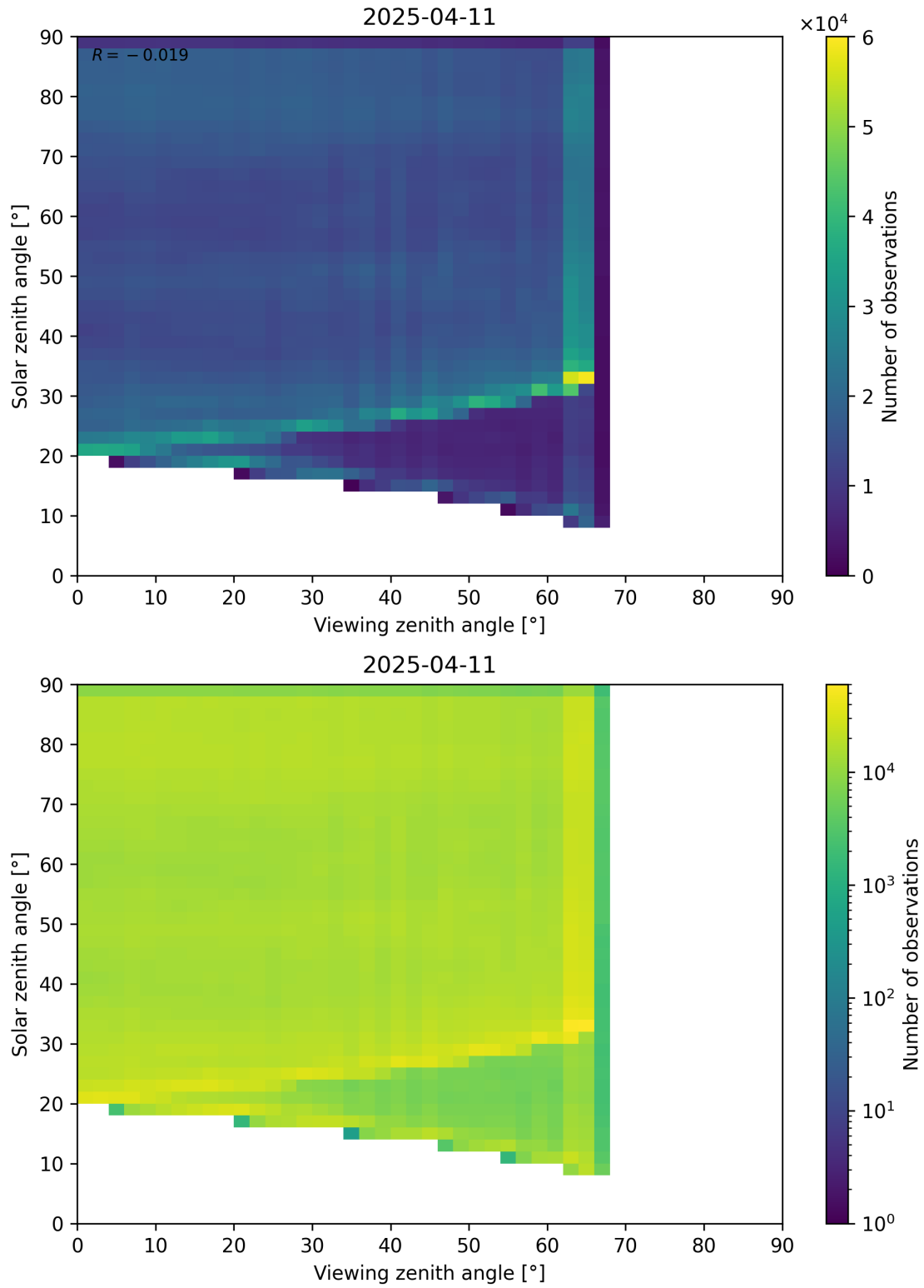
Figure 114: Scatter density plot of “Viewing zenith angle” against “Solar zenith angle” for 2025-04-10 to 2025-04-12.
