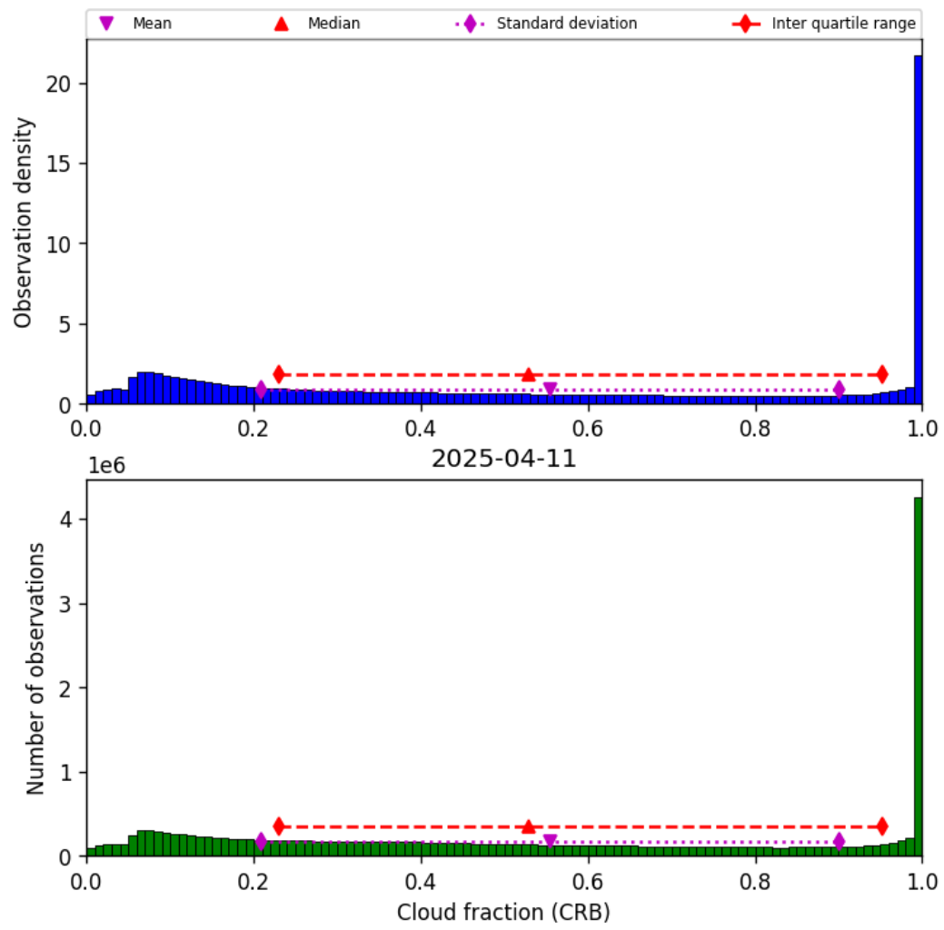
Figure 42: Histogram of “Cloud fraction (CRB)” for 2025-04-10 to 2025-04-12
