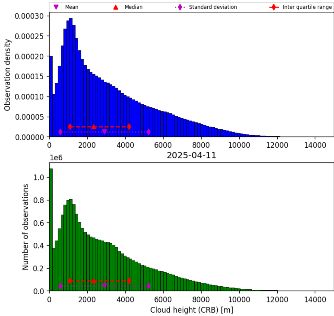
Figure 43: Histogram of “Cloud height (CRB)” for 2025-04-10 to 2025-04-12
