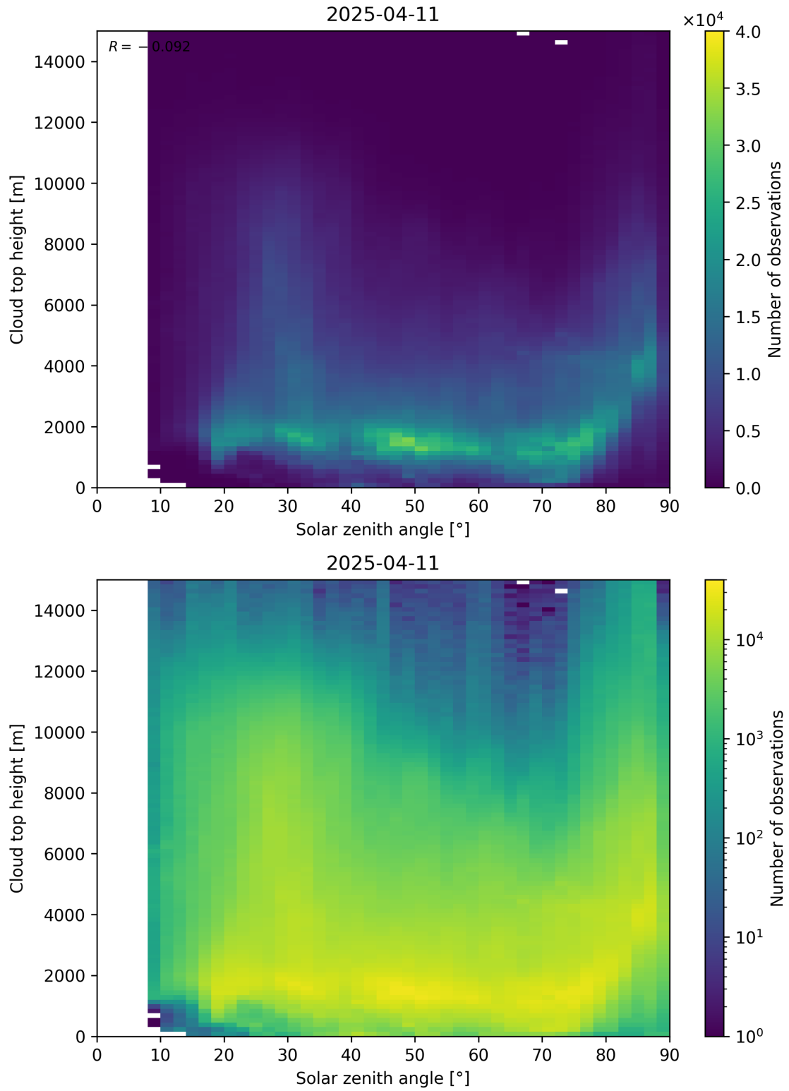
Figure 104: Scatter density plot of “Solar zenith angle” against “Cloud top height” for 2025-04-10 to 2025-04-12.
