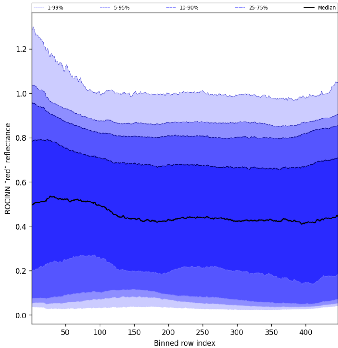
Figure 69: Along track statistics of "ROCINN "red" reflectance" for 2025-04-10 to 2025-04-12
