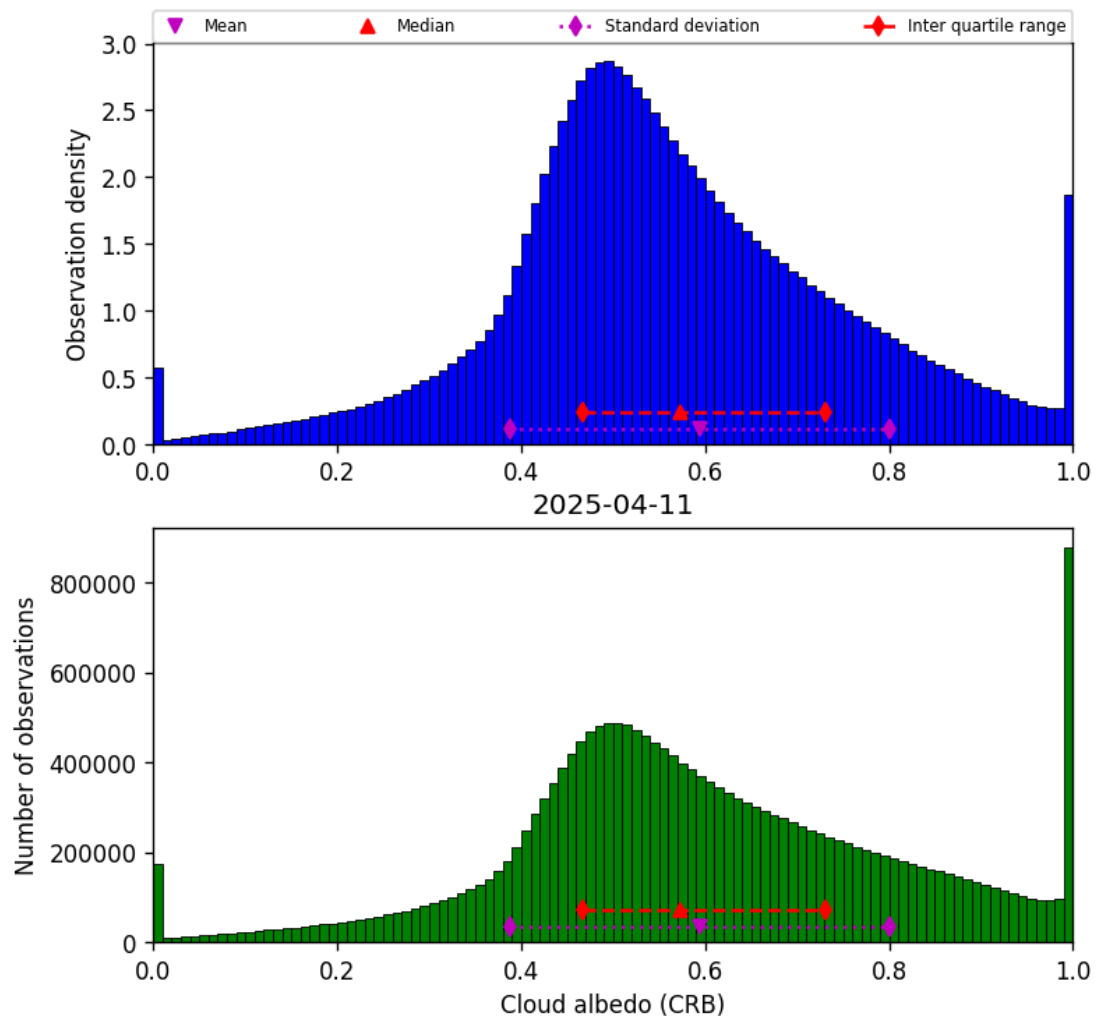
Figure 44: Histogram of “Cloud albedo (CRB)” for 2025-04-10 to 2025-04-12
