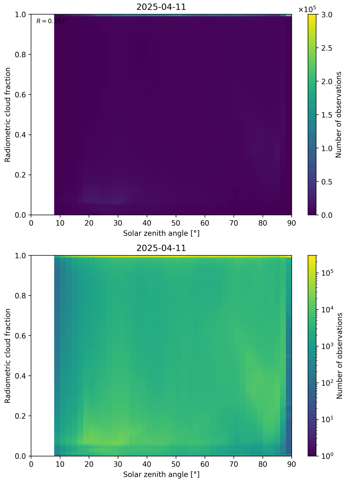
Figure 99: Scatter density plot of “Solar zenith angle” against “Radiometric cloud fraction” for 2025-04-10 to 2025-04-12.
