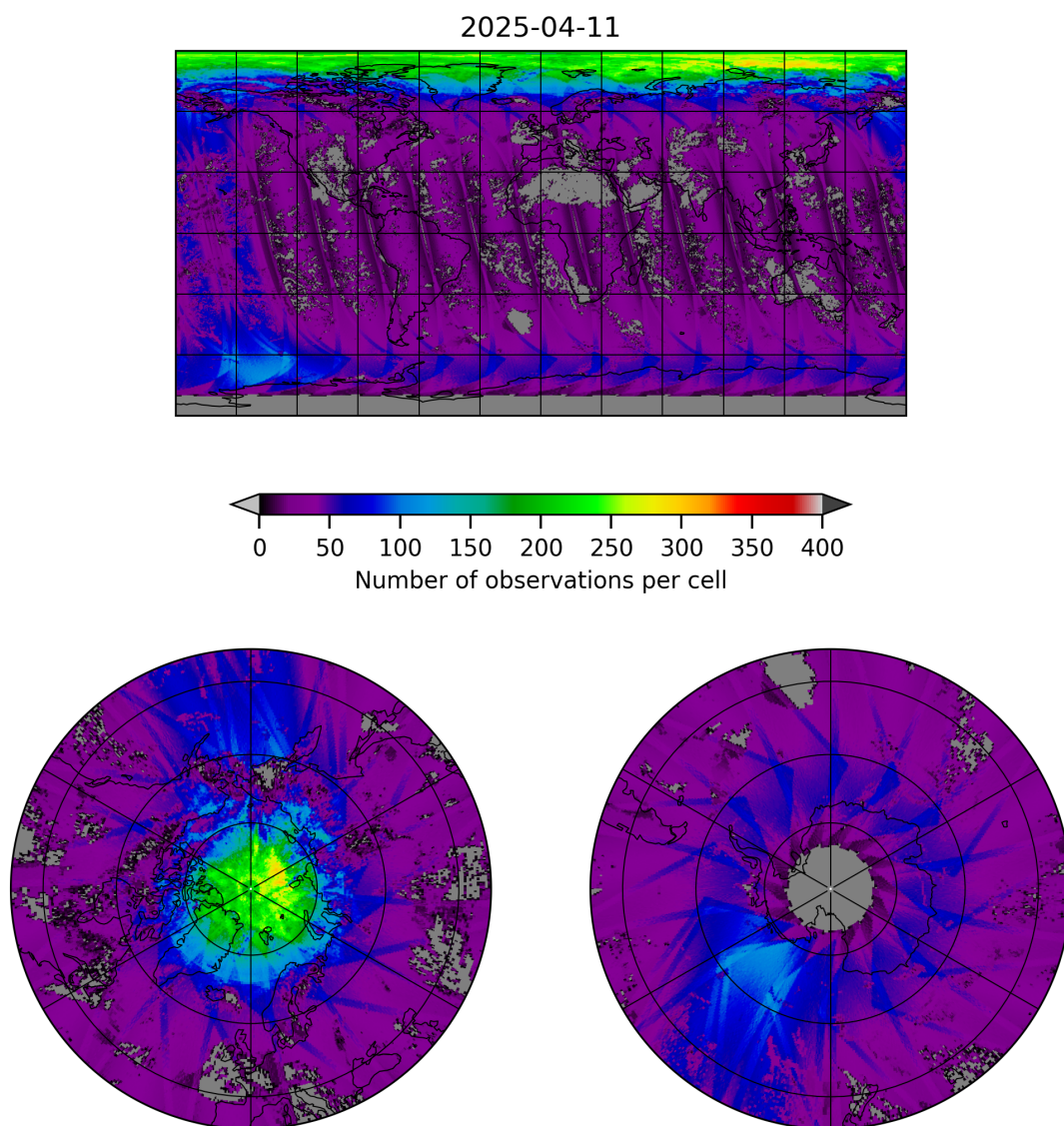
Figure 21: Map of the number of observations for 2025-04-10 to 2025-04-12
