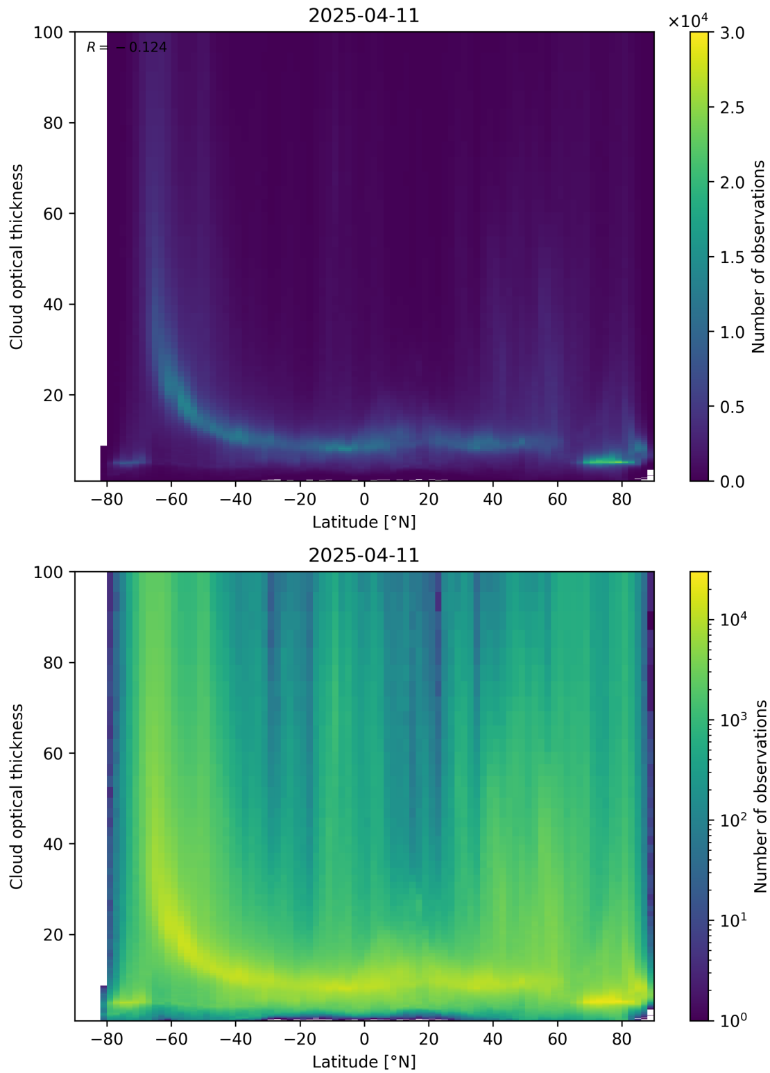
Figure 96: Scatter density plot of “Latitude” against “Cloud optical thickness” for 2025-04-10 to 2025-04-12.
