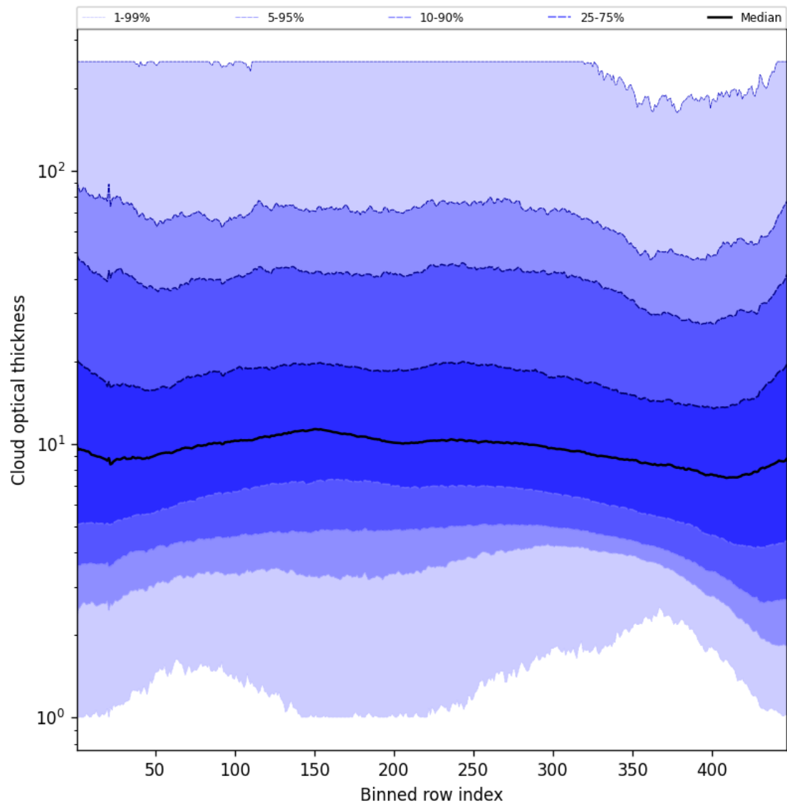
Figure 57: Along track statistics of “Cloud optical thickness” for 2025-04-10 to 2025-04-12
