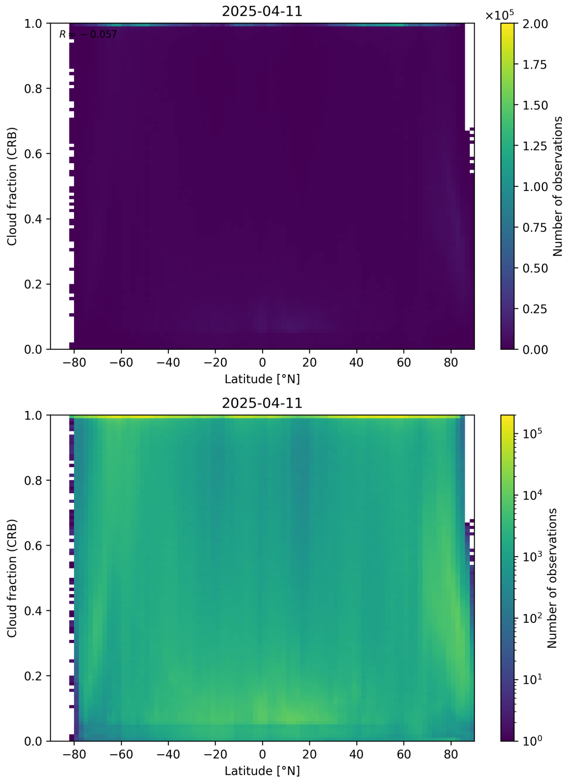
Figure 94: Scatter density plot of “Latitude” against “Cloud fraction (CRB)” for 2025-04-10 to 2025-04-12.
