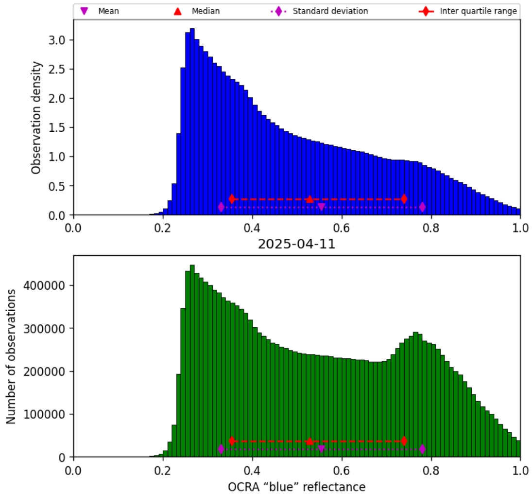
Figure 51: Histogram of “OCRA “blue” reflectance” for 2025-04-10 to 2025-04-12
