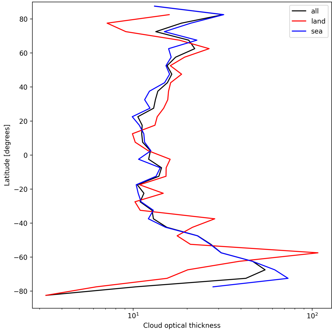
Figure 25: Zonal average of “Cloud optical thickness” for 2025-04-10 to 2025-04-12.
