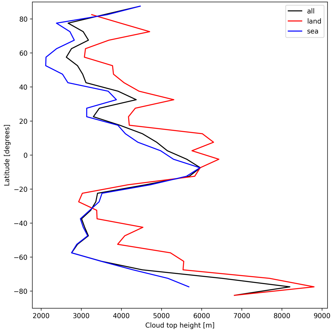
Figure 24: Zonal average of “Cloud top height” for 2025-04-10 to 2025-04-12.
