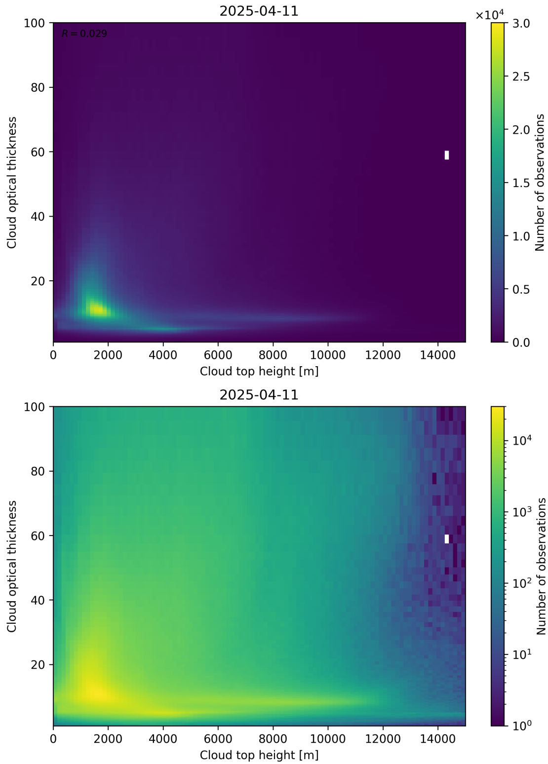
Figure 90: Scatter density plot of “Cloud top height” against “Cloud optical thickness” for 2025-04-10 to 2025-04-12.
