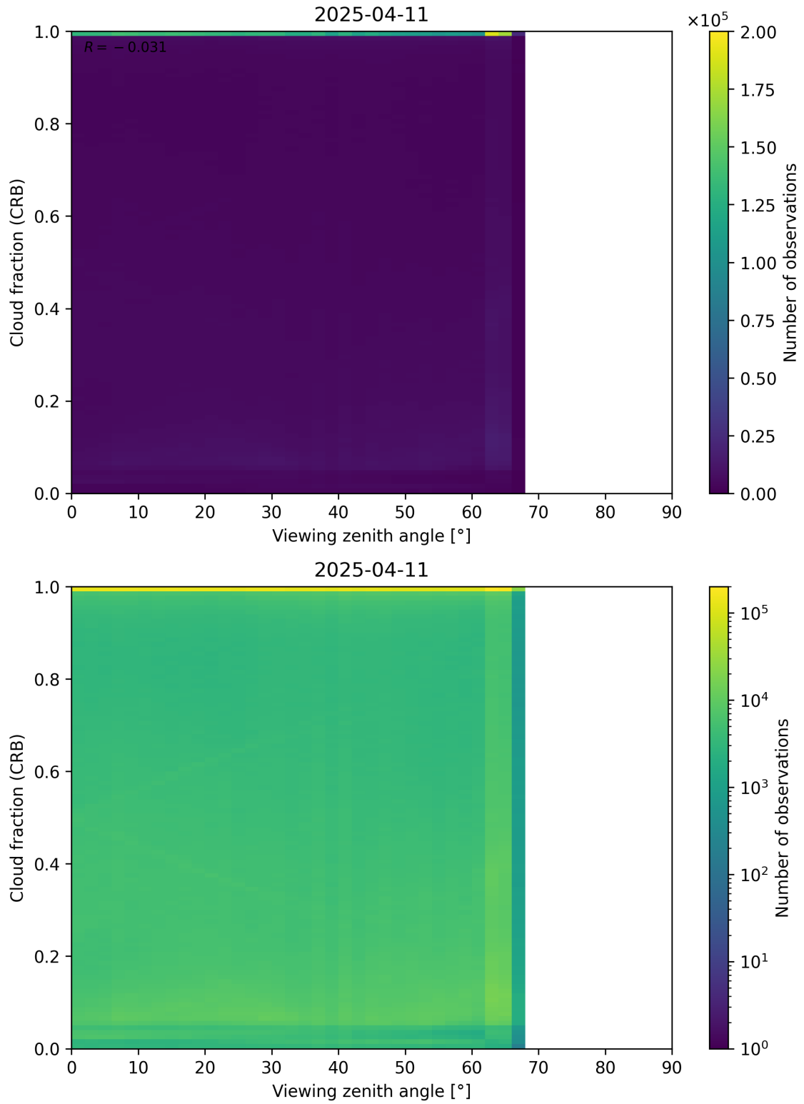
Figure 109: Scatter density plot of “Viewing zenith angle” against “Cloud fraction (CRB)” for 2025-04-10 to 2025-04-12.
