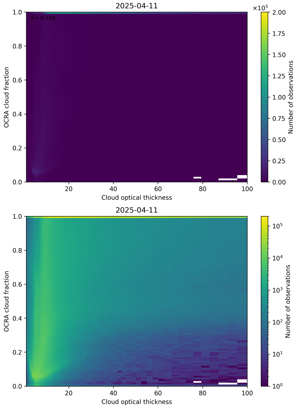
Figure 83: Scatter density plot of “Cloud optical thickness” against “OCRA cloud fraction” for 2025-04-10 to 2025-04-12.
