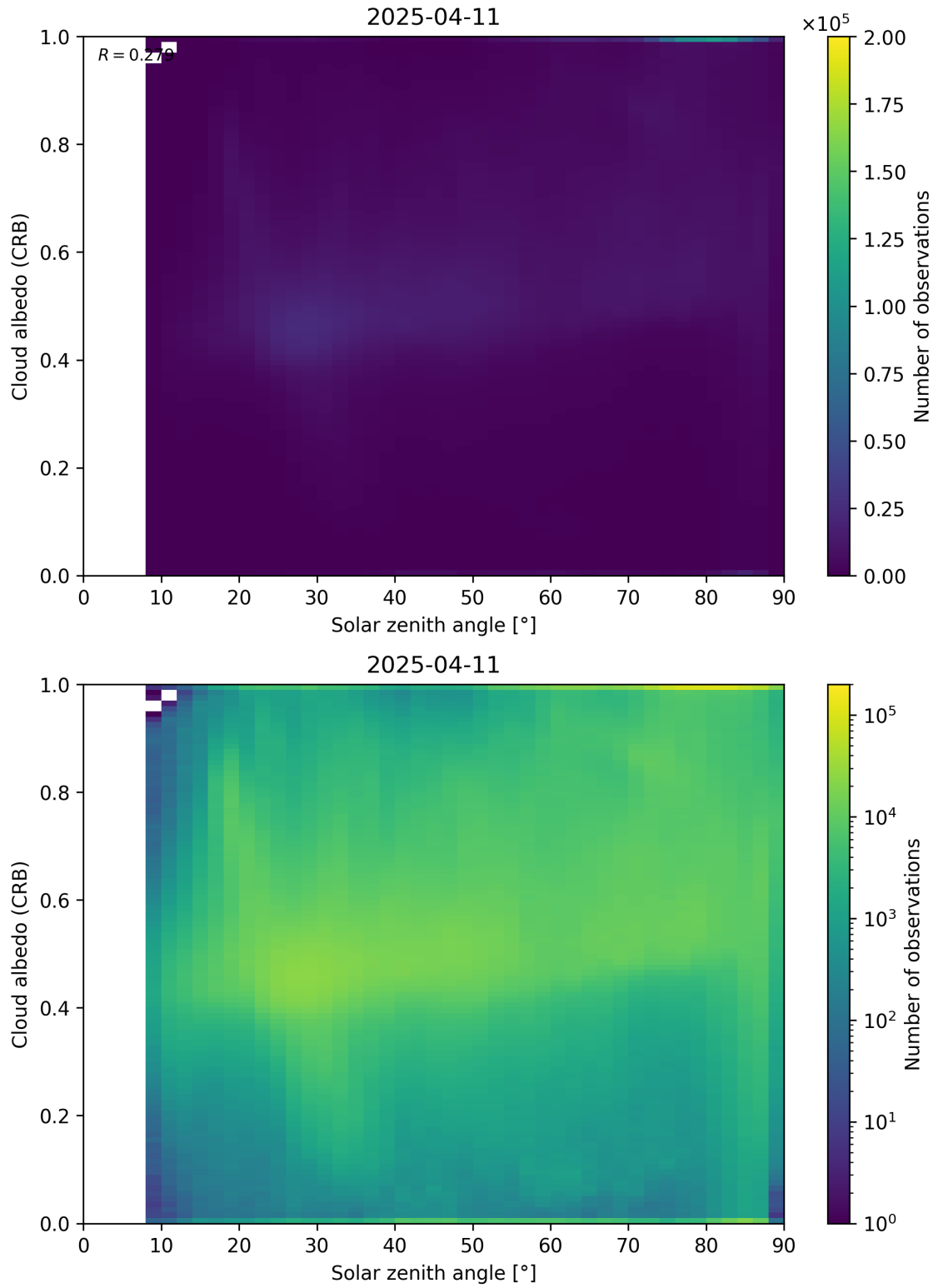
Figure 98: Scatter density plot of “Solar zenith angle” against “Cloud albedo (CRB)” for 2025-04-10 to 2025-04-12.
