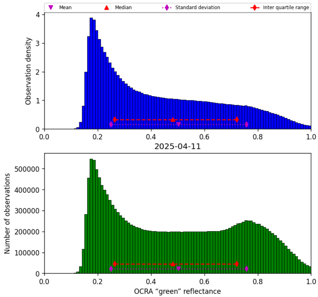
Figure 52: Histogram of “OCRA “green” reflectance” for 2025-04-10 to 2025-04-12
