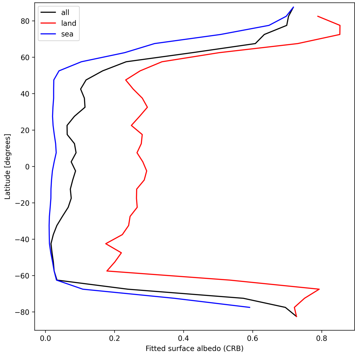
Figure 30: Zonal average of “Fitted surface albedo (CRB)” for 2025-04-10 to 2025-04-12.
