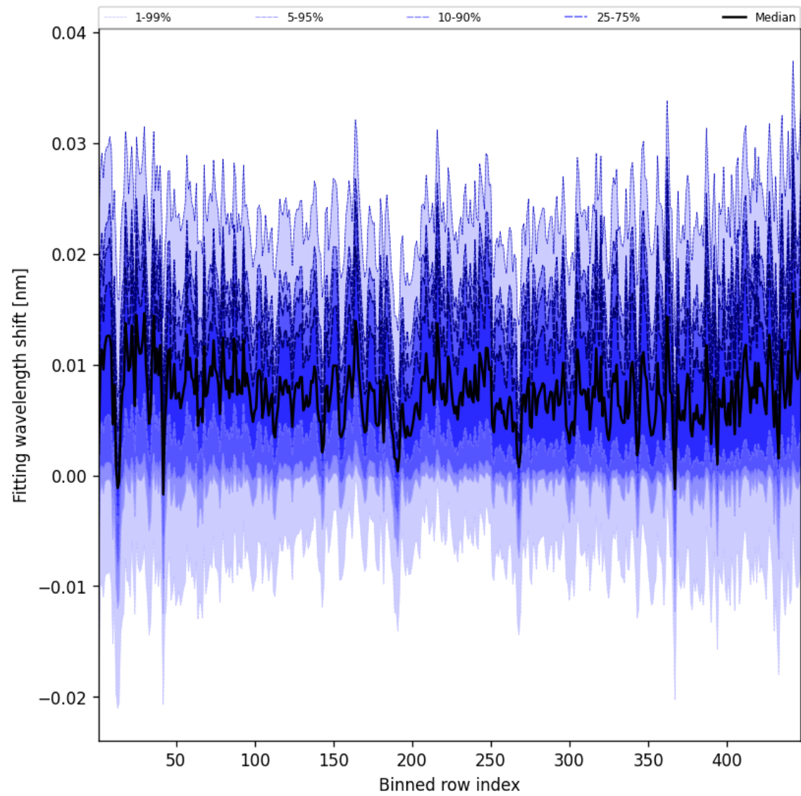
Figure 65: Along track statistics of “Fitting wavelength shift” for 2025-04-10 to 2025-04-12
