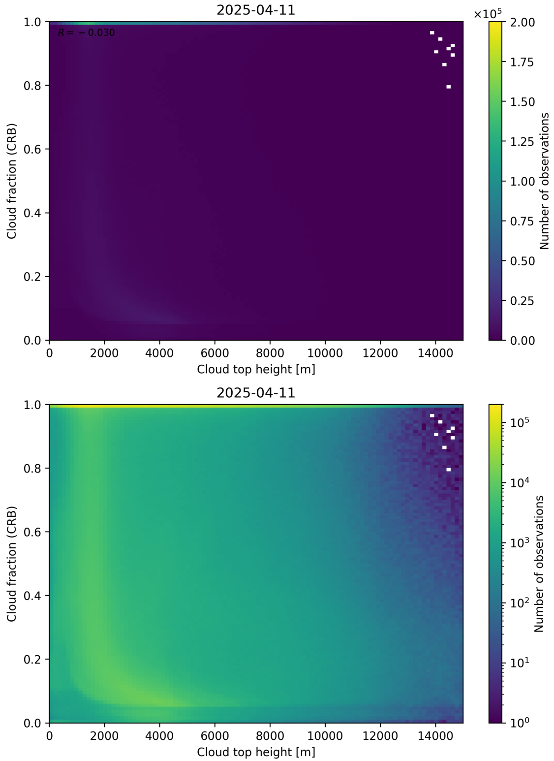
Figure 88: Scatter density plot of “Cloud top height” against “Cloud fraction (CRB)” for 2025-04-10 to 2025-04-12.
