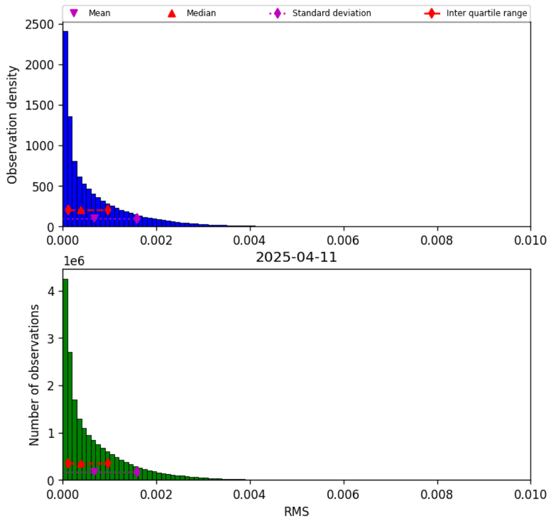
Figure 47: Histogram of “RMS” for 2025-04-10 to 2025-04-12
