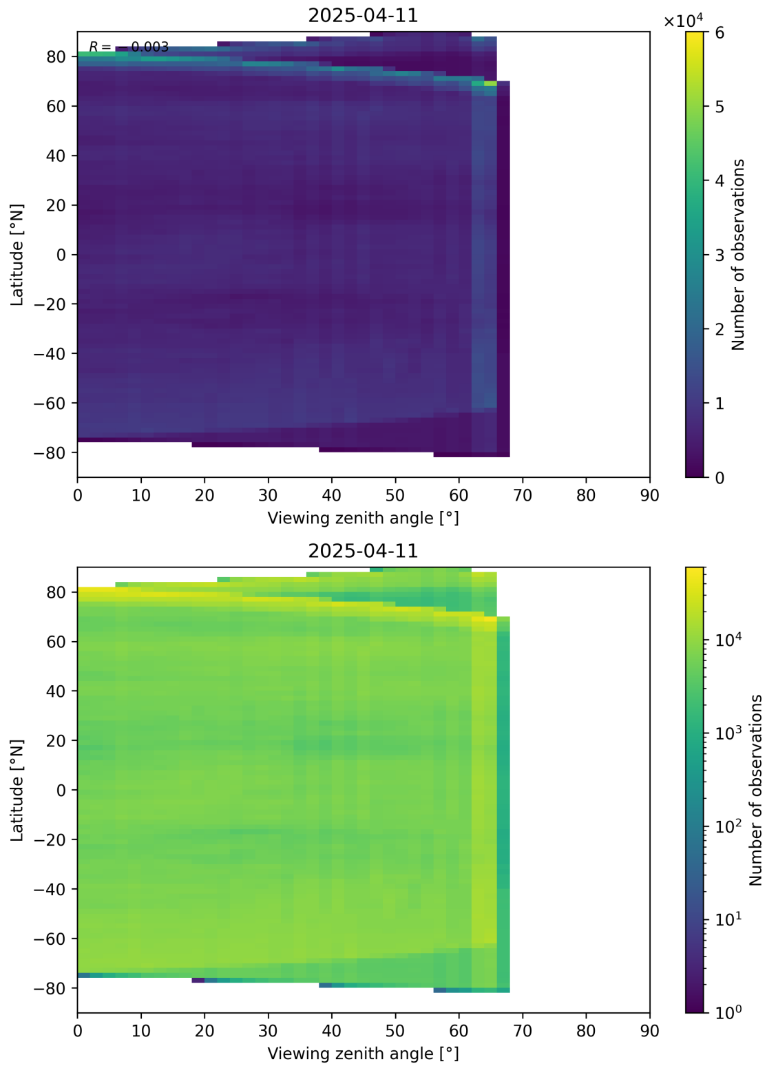
Figure 113: Scatter density plot of “Viewing zenith angle” against “Latitude” for 2025-04-10 to 2025-04-12.
