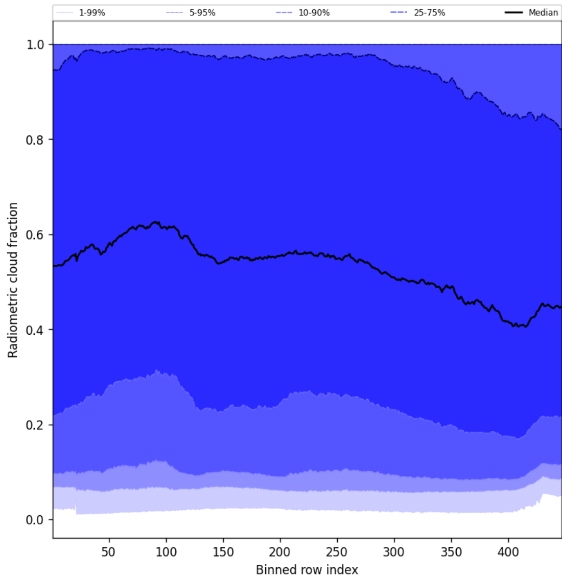
Figure 55: Along track statistics of “Radiometric cloud fraction” for 2025-04-10 to 2025-04-12
