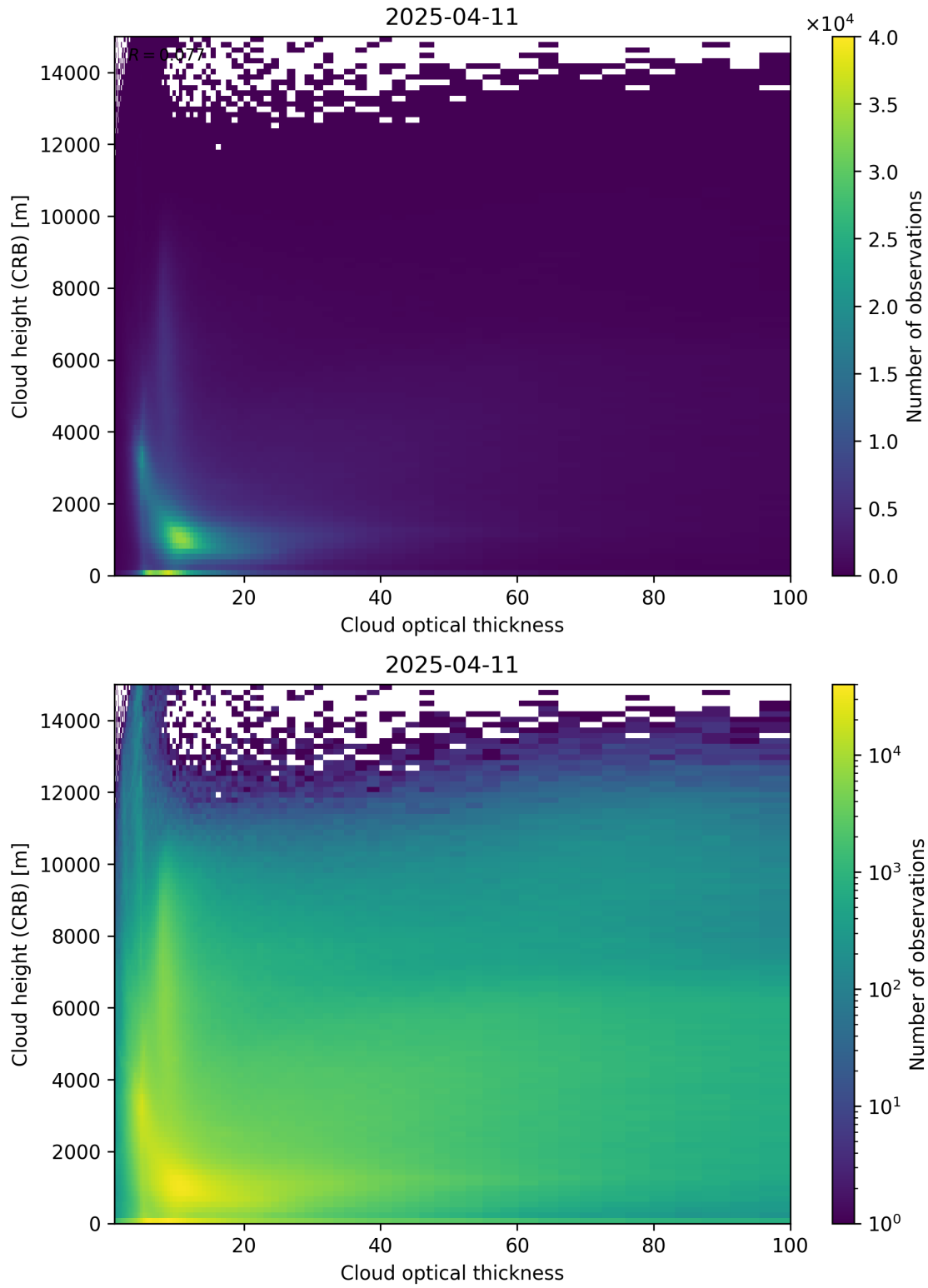
Figure 85: Scatter density plot of “Cloud optical thickness” against “Cloud height (CRB)” for 2025-04-10 to 2025-04-12.
