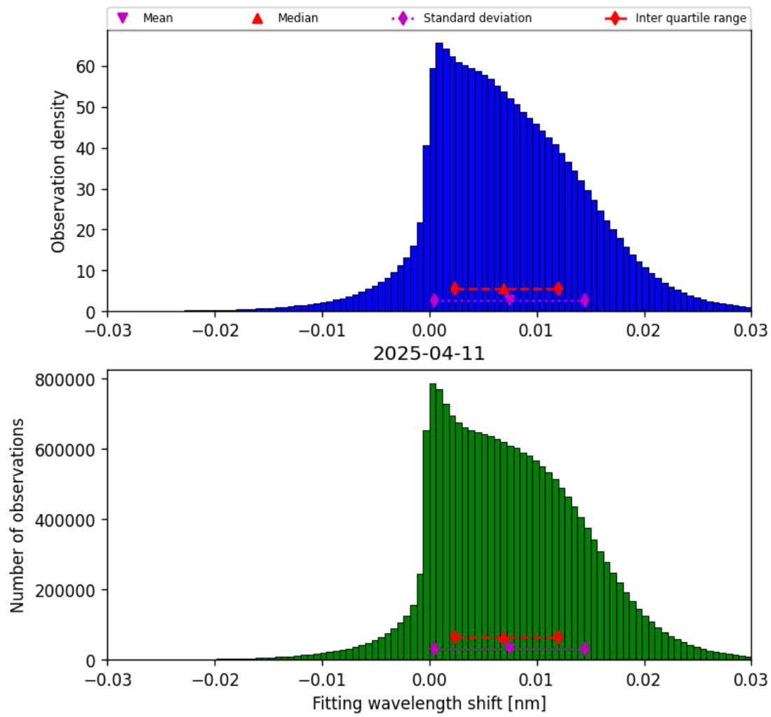
Figure 49: Histogram of “Fitting wavelength shift” for 2025-04-10 to 2025-04-12
