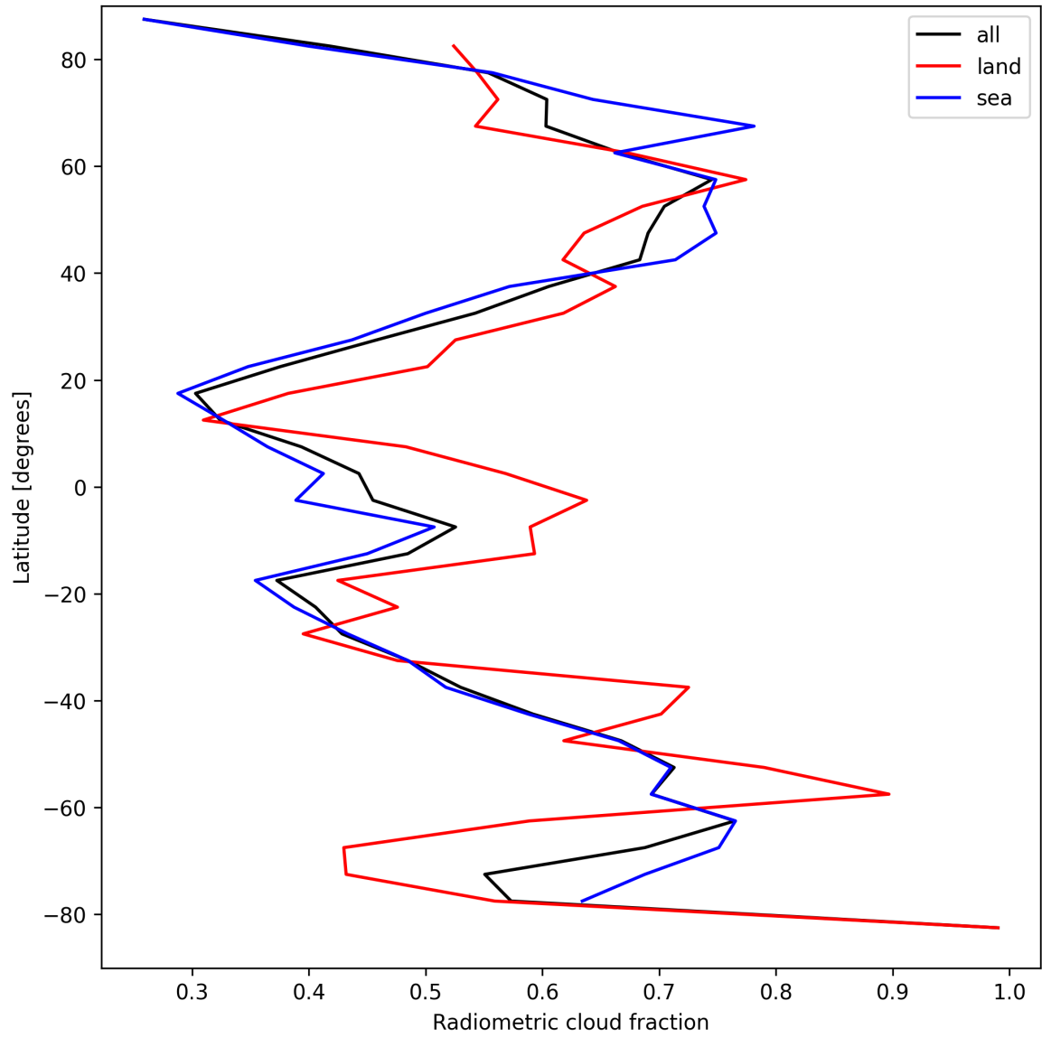
Figure 23: Zonal average of “Radiometric cloud fraction” for 2025-04-10 to 2025-04-12.
