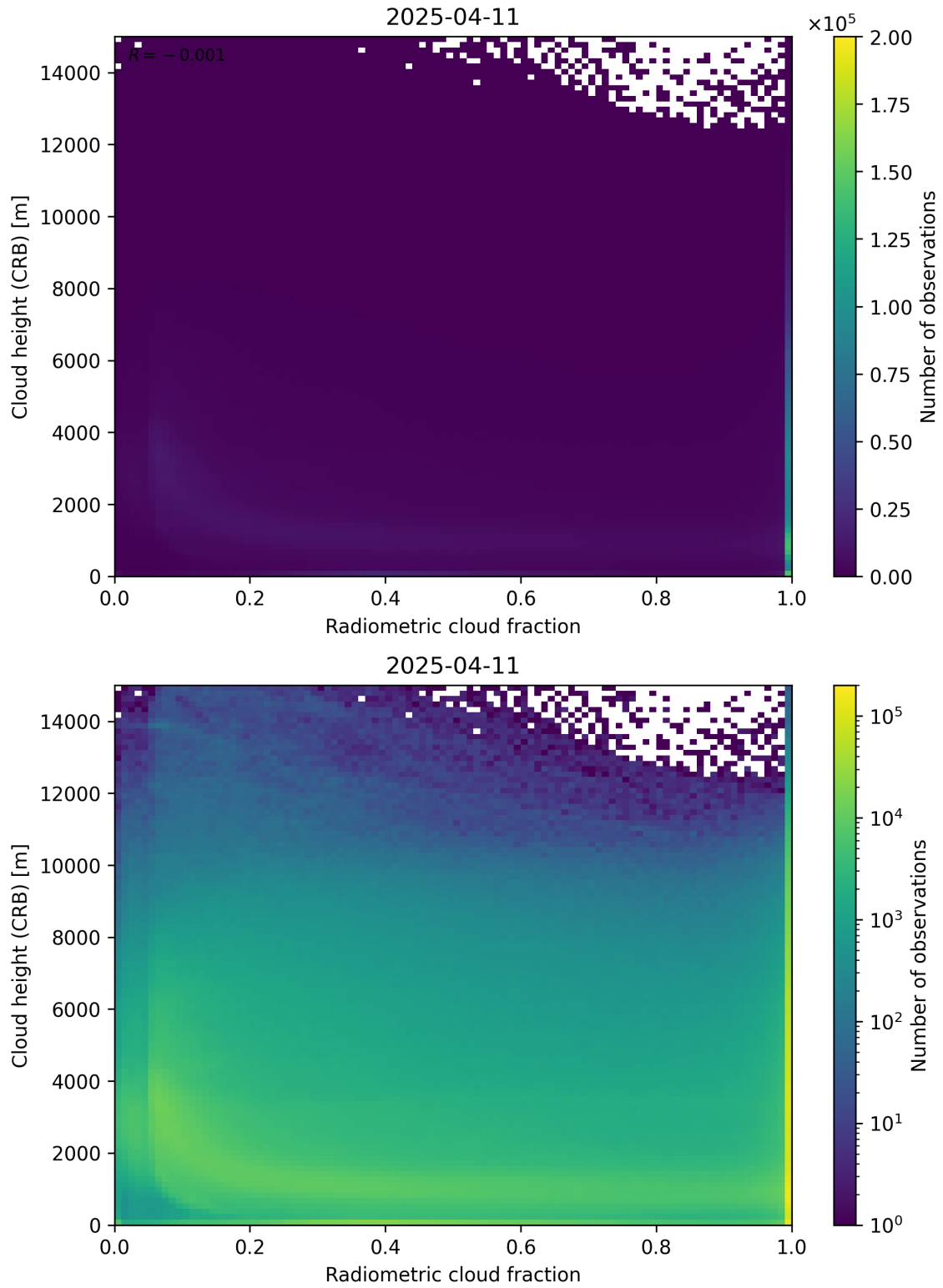
Figure 74: Scatter density plot of “Radiometric cloud fraction” against “Cloud height (CRB)” for 2025-04-10 to 2025-04-12.
