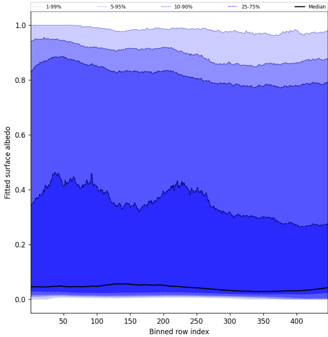
Figure 61: Along track statistics of “Fitted surface albedo” for 2025-04-10 to 2025-04-12
