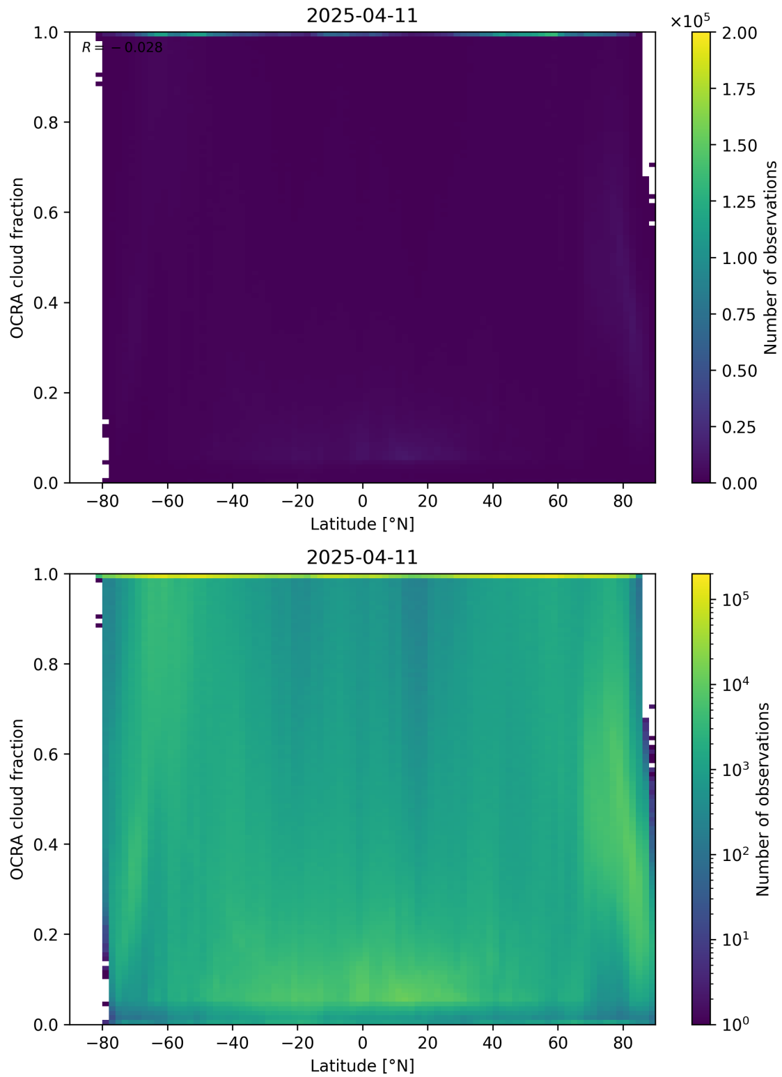
Figure 93: Scatter density plot of “Latitude” against “OCRA cloud fraction” for 2025-04-10 to 2025-04-12.
