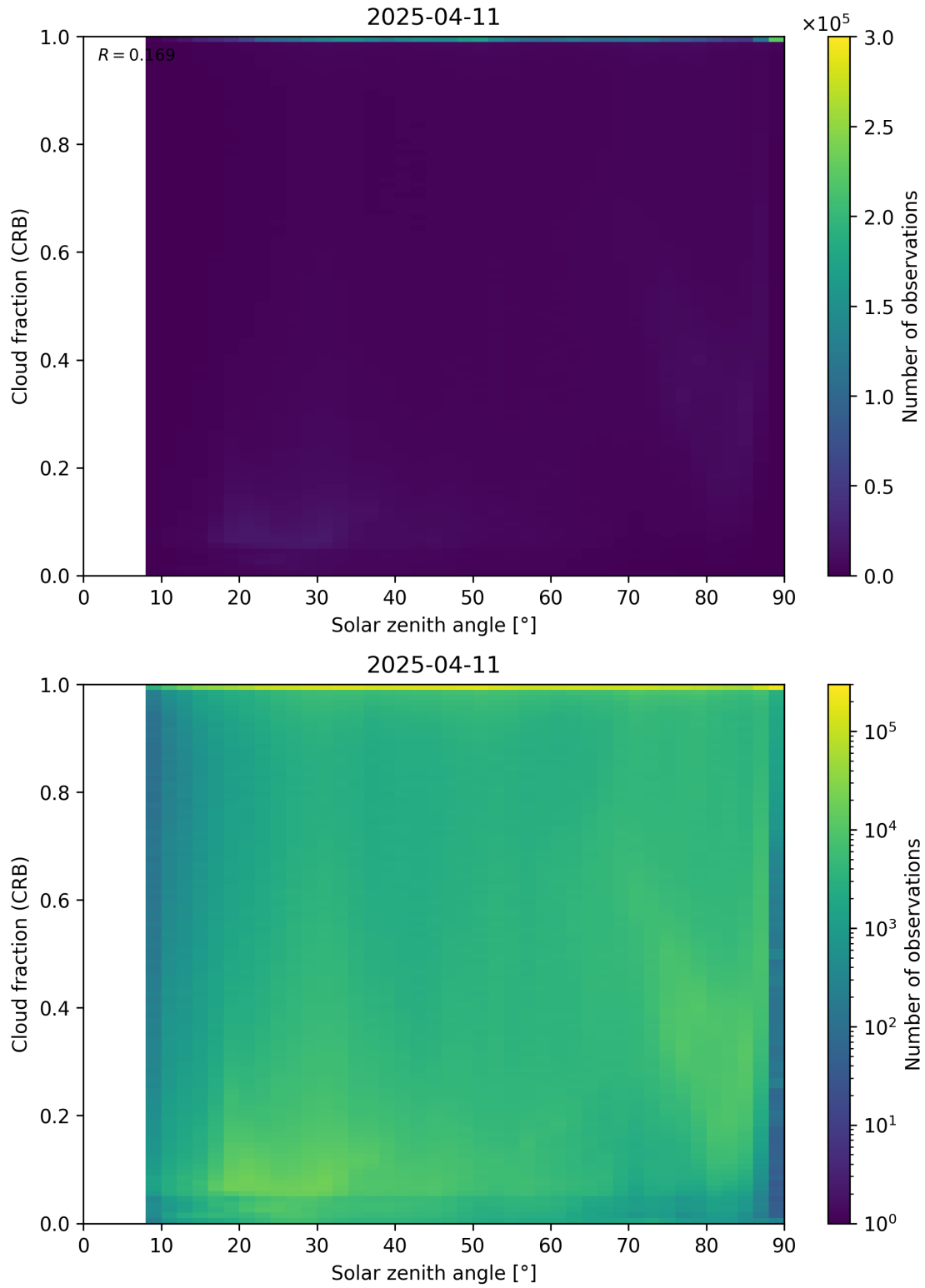
Figure 101: Scatter density plot of “Solar zenith angle” against “Cloud fraction (CRB)” for 2025-04-10 to 2025-04-12.
