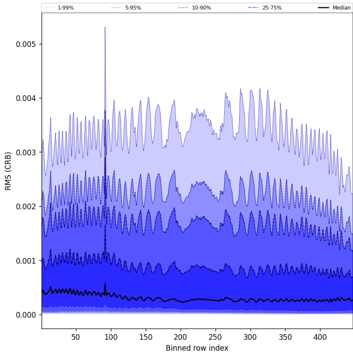
Figure 64: Along track statistics of “RMS (CRB)” for 2025-04-10 to 2025-04-12
