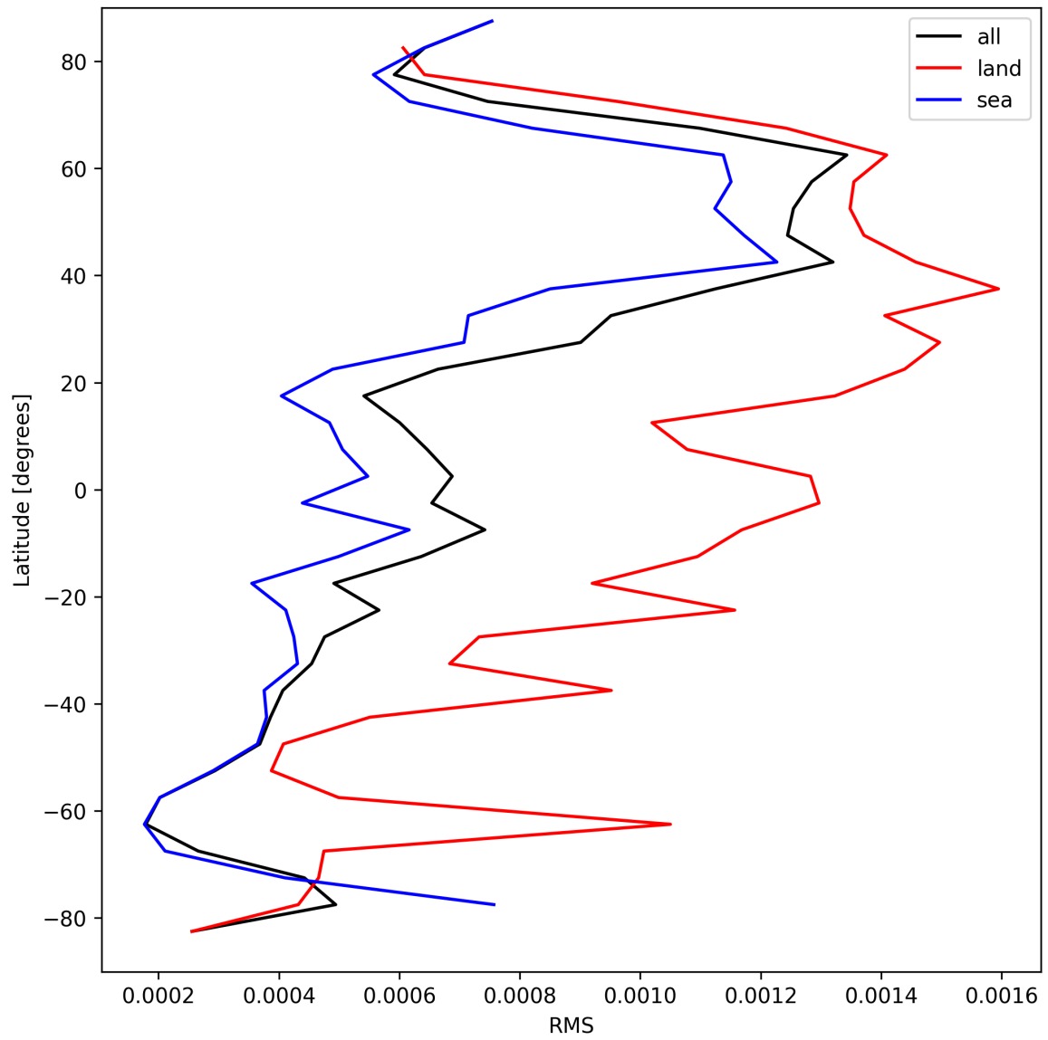
Figure 31: Zonal average of “RMS” for 2025-04-10 to 2025-04-12.
