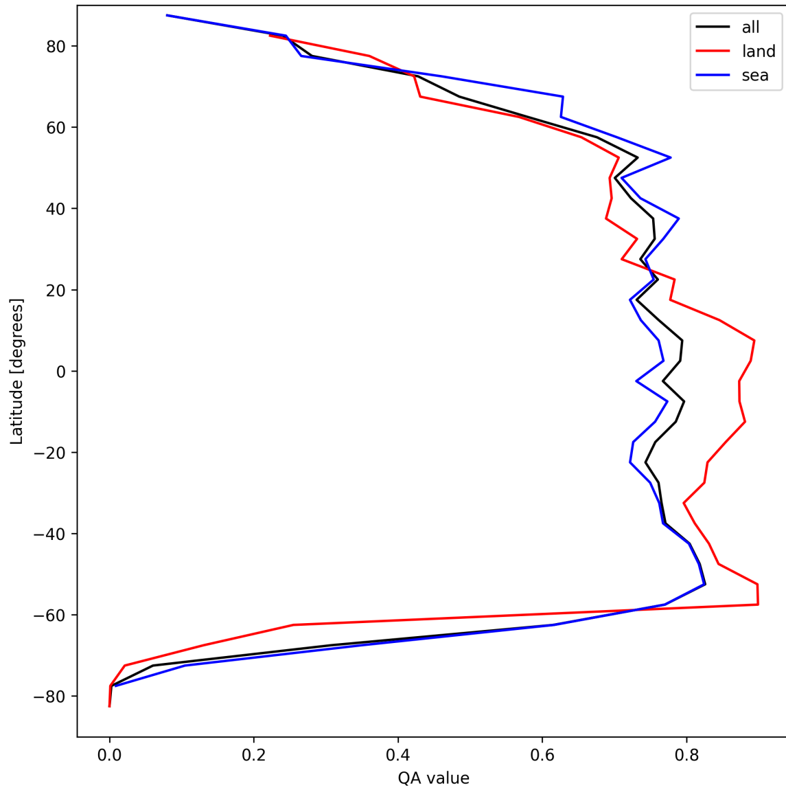
Figure 22: Zonal average of “QA value” for 2025-04-10 to 2025-04-12.
