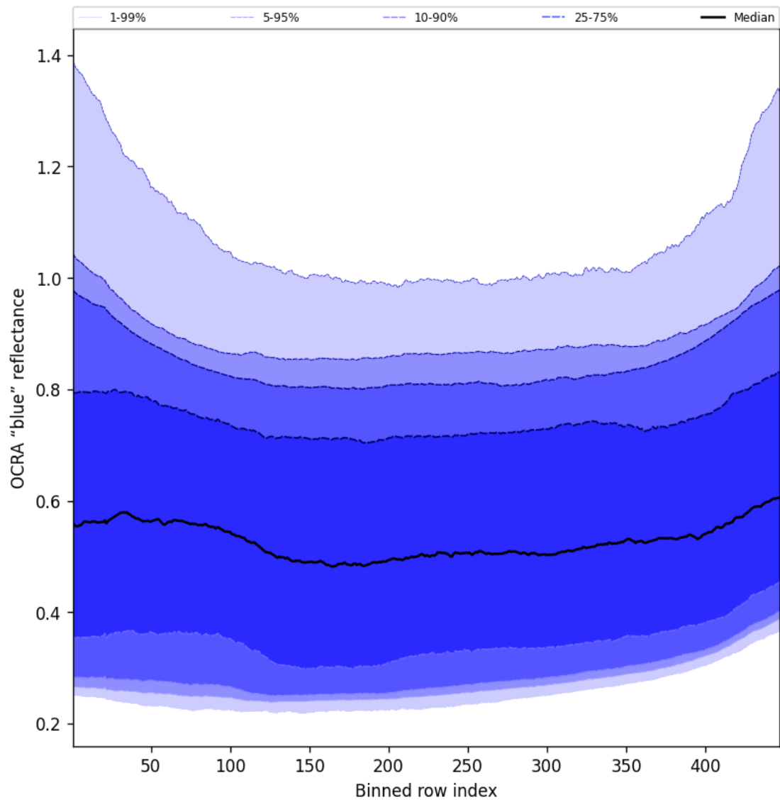
Figure 67: Along track statistics of “OCRA “blue” reflectance” for 2025-04-10 to 2025-04-12
