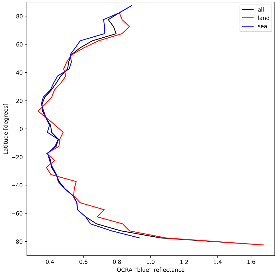
Figure 35: Zonal average of “OCRA “blue” reflectance” for 2025-04-10 to 2025-04-12.
