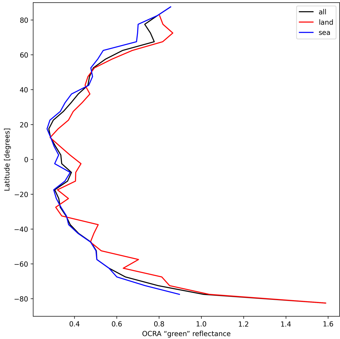
Figure 36: Zonal average of “OCRA “green” reflectance” for 2025-04-10 to 2025-04-12.
