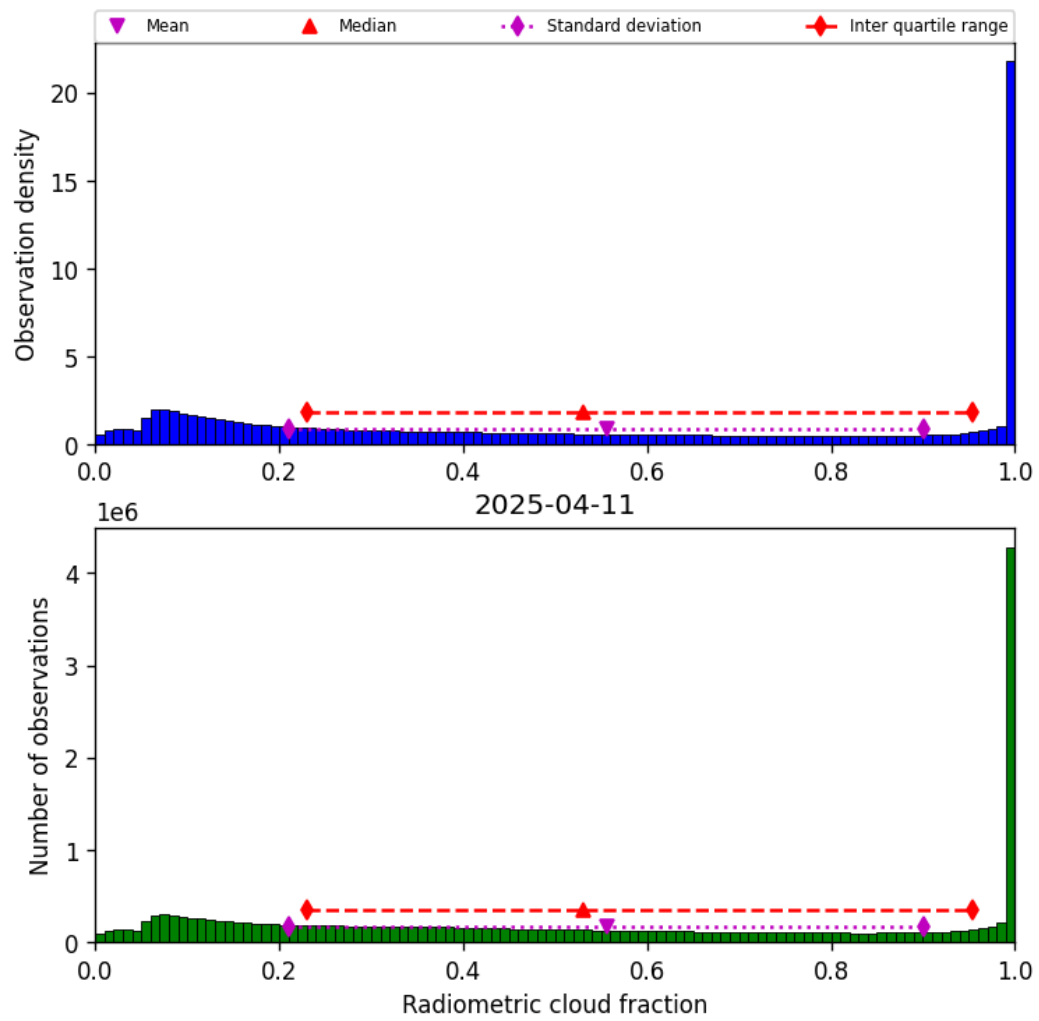
Figure 39: Histogram of “Radiometric cloud fraction” for 2025-04-10 to 2025-04-12
