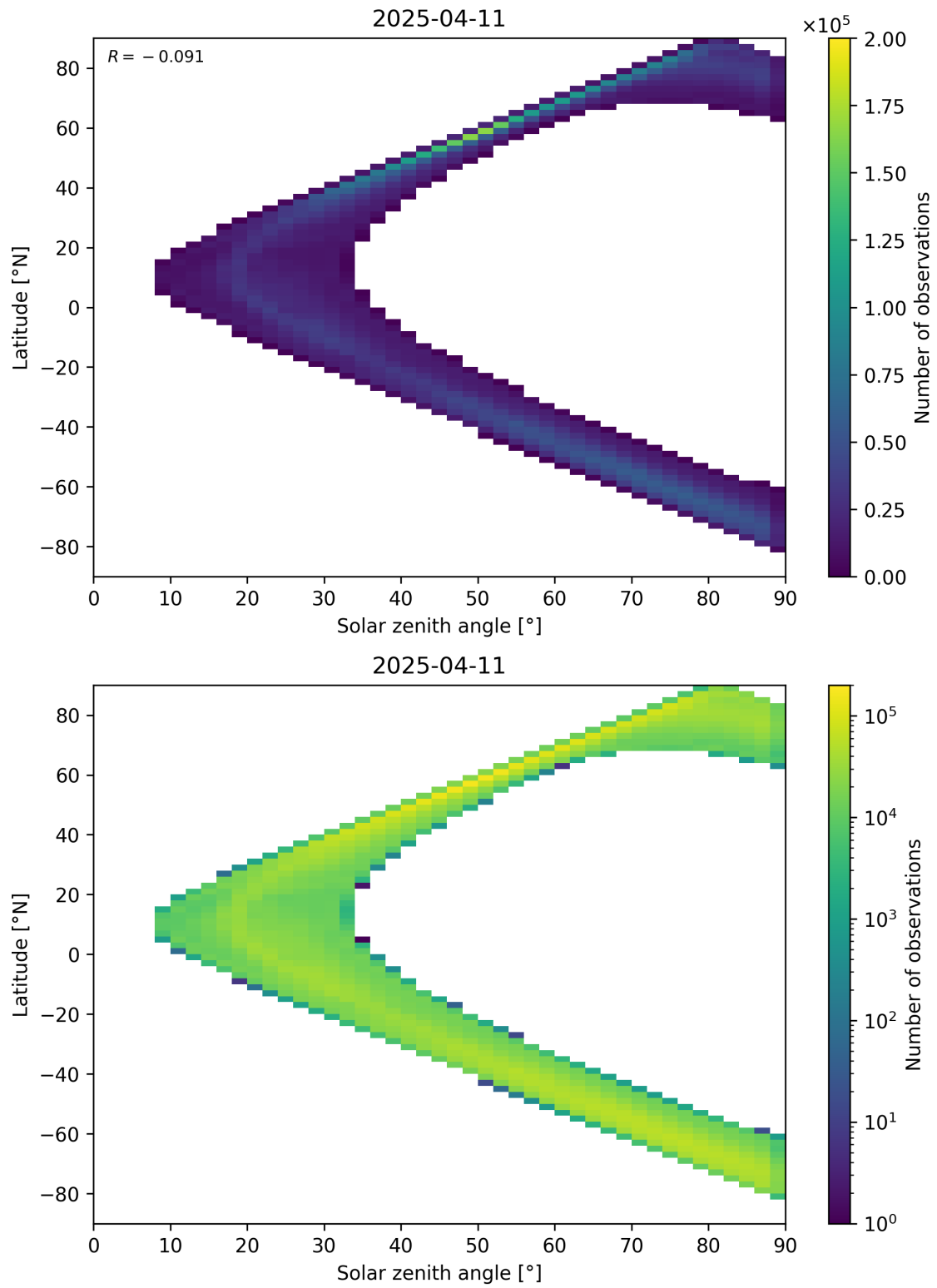
Figure 105: Scatter density plot of “Solar zenith angle” against “Latitude” for 2025-04-10 to 2025-04-12.
