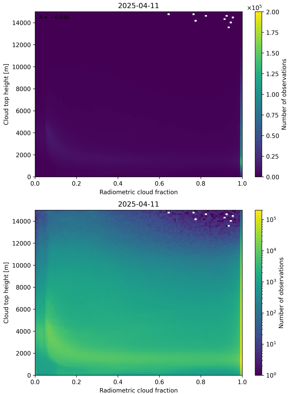
Figure 76: Scatter density plot of “Radiometric cloud fraction” against “Cloud top height” for 2025-04-10 to 2025-04-12.
