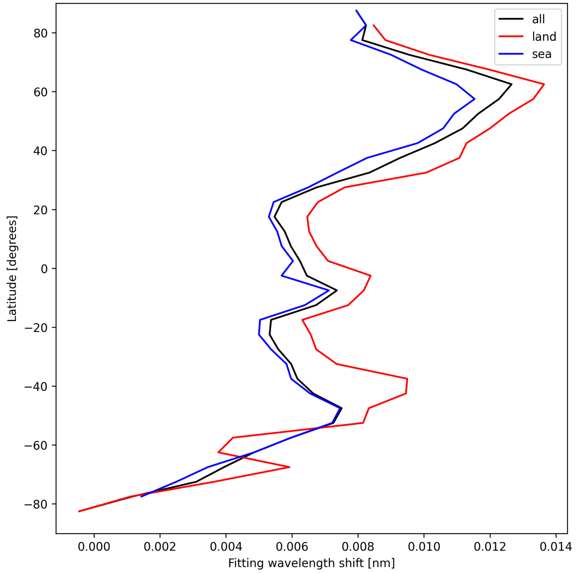
Figure 33: Zonal average of “Fitting wavelength shift” for 2025-04-10 to 2025-04-12.
