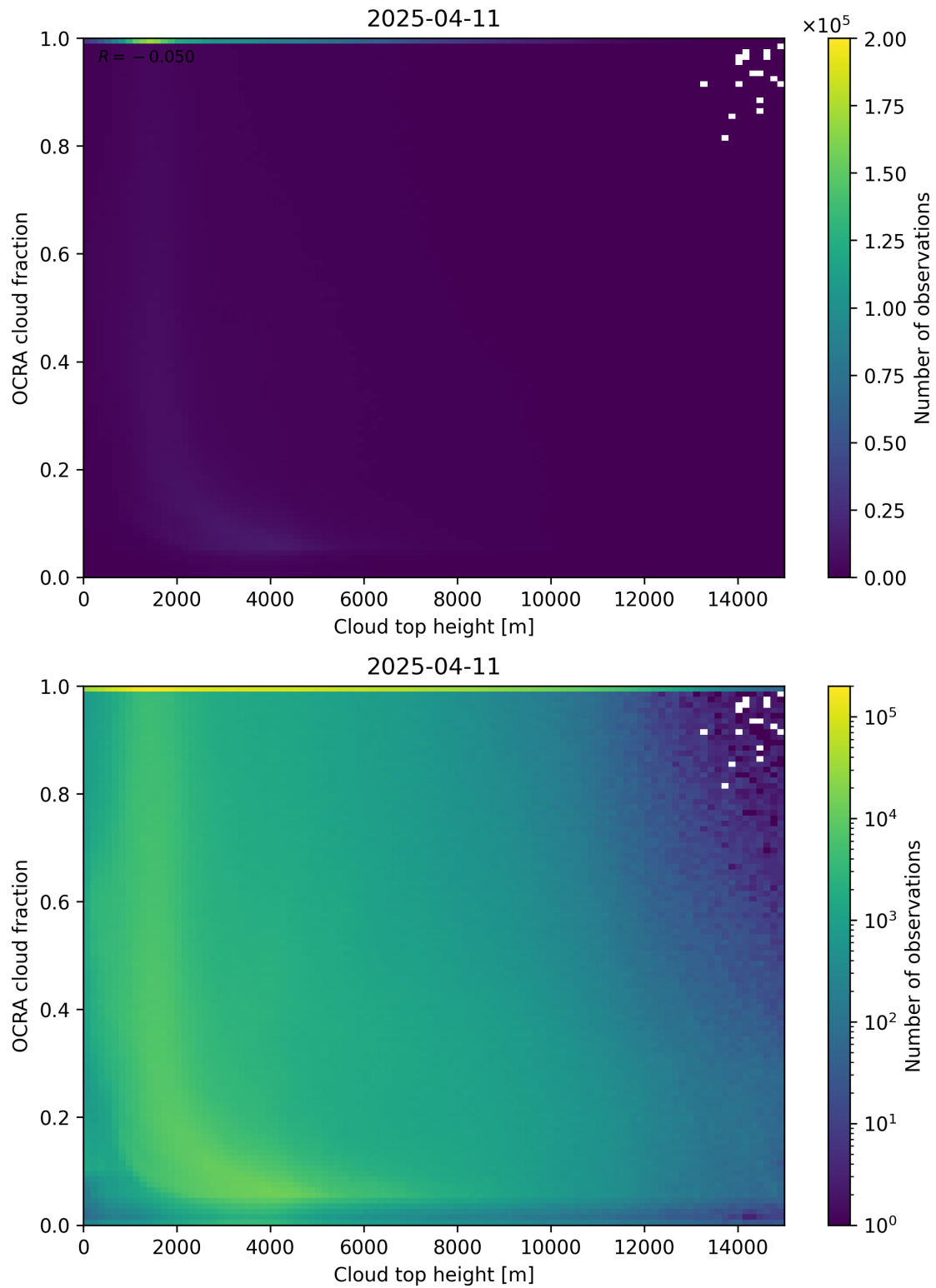
Figure 87: Scatter density plot of “Cloud top height” against “OCRA cloud fraction” for 2025-04-10 to 2025-04-12.
