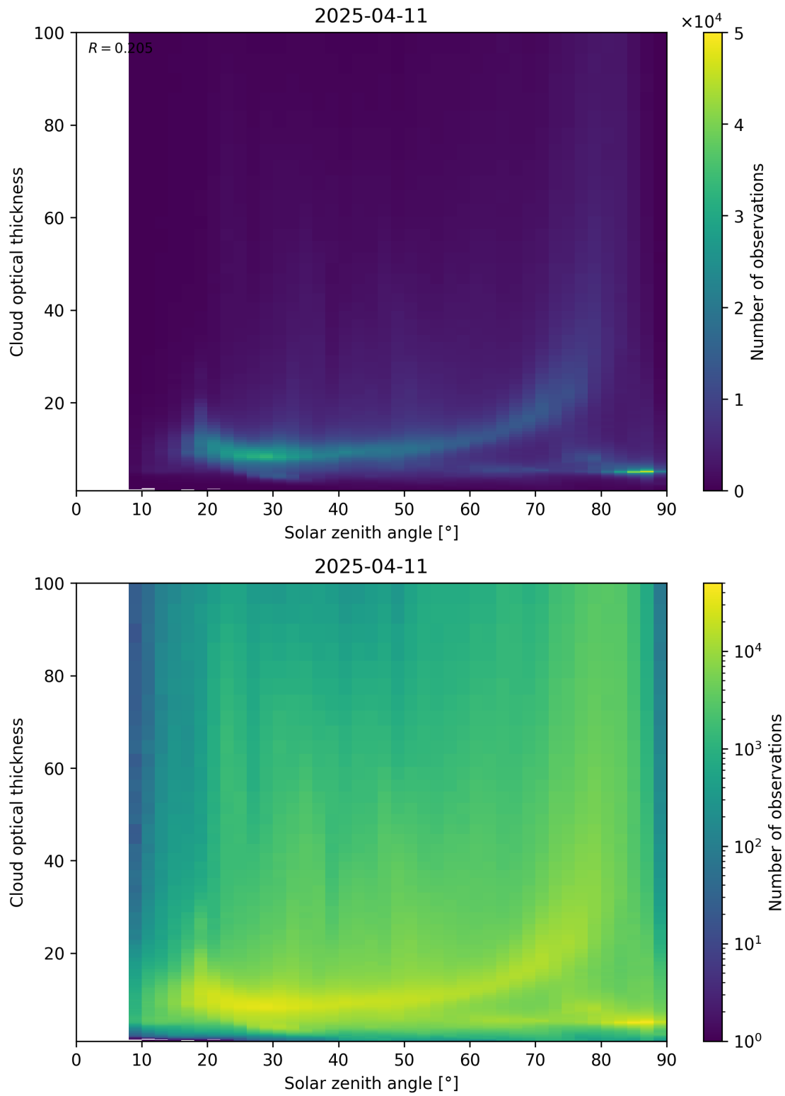
Figure 103: Scatter density plot of “Solar zenith angle” against “Cloud optical thickness” for 2025-04-10 to 2025-04-12.
