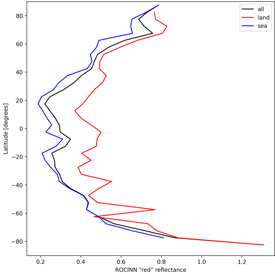
Figure 37: Zonal average of “ROCINN “red” reflectance” for 2025-04-10 to 2025-04-12.
