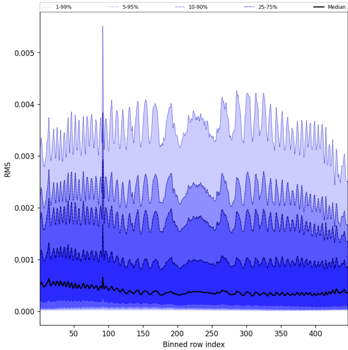
Figure 63: Along track statistics of “RMS” for 2025-04-10 to 2025-04-12
