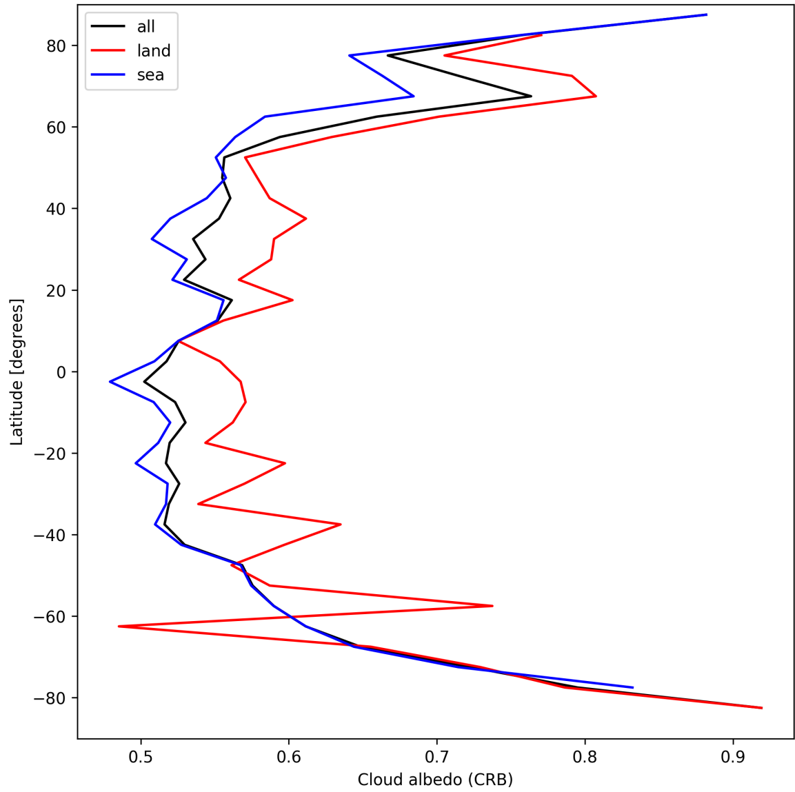
Figure 28: Zonal average of “Cloud albedo (CRB)” for 2025-04-10 to 2025-04-12.
