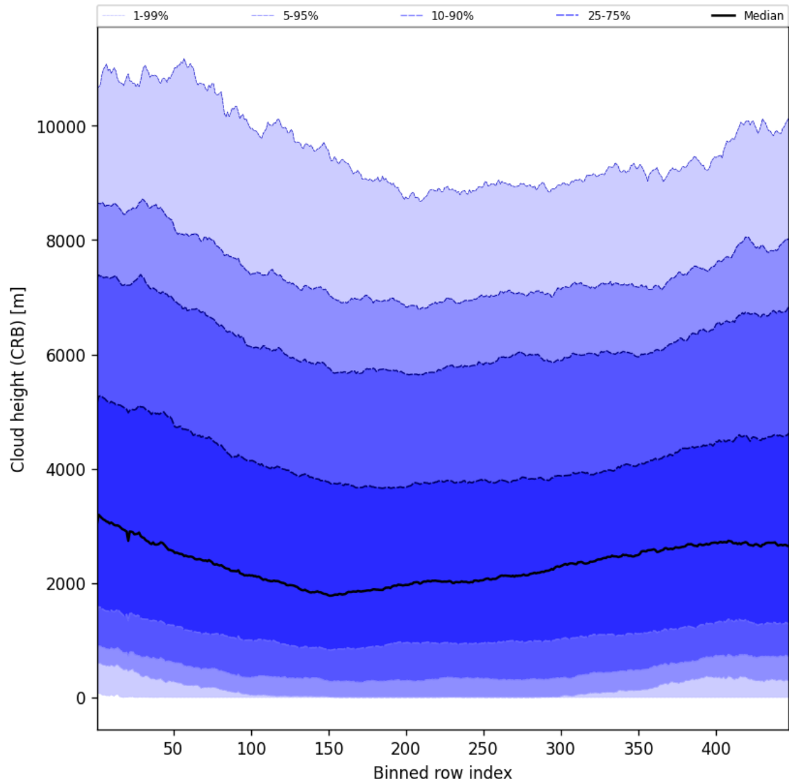
Figure 59: Along track statistics of “Cloud height (CRB)” for 2025-04-10 to 2025-04-12
