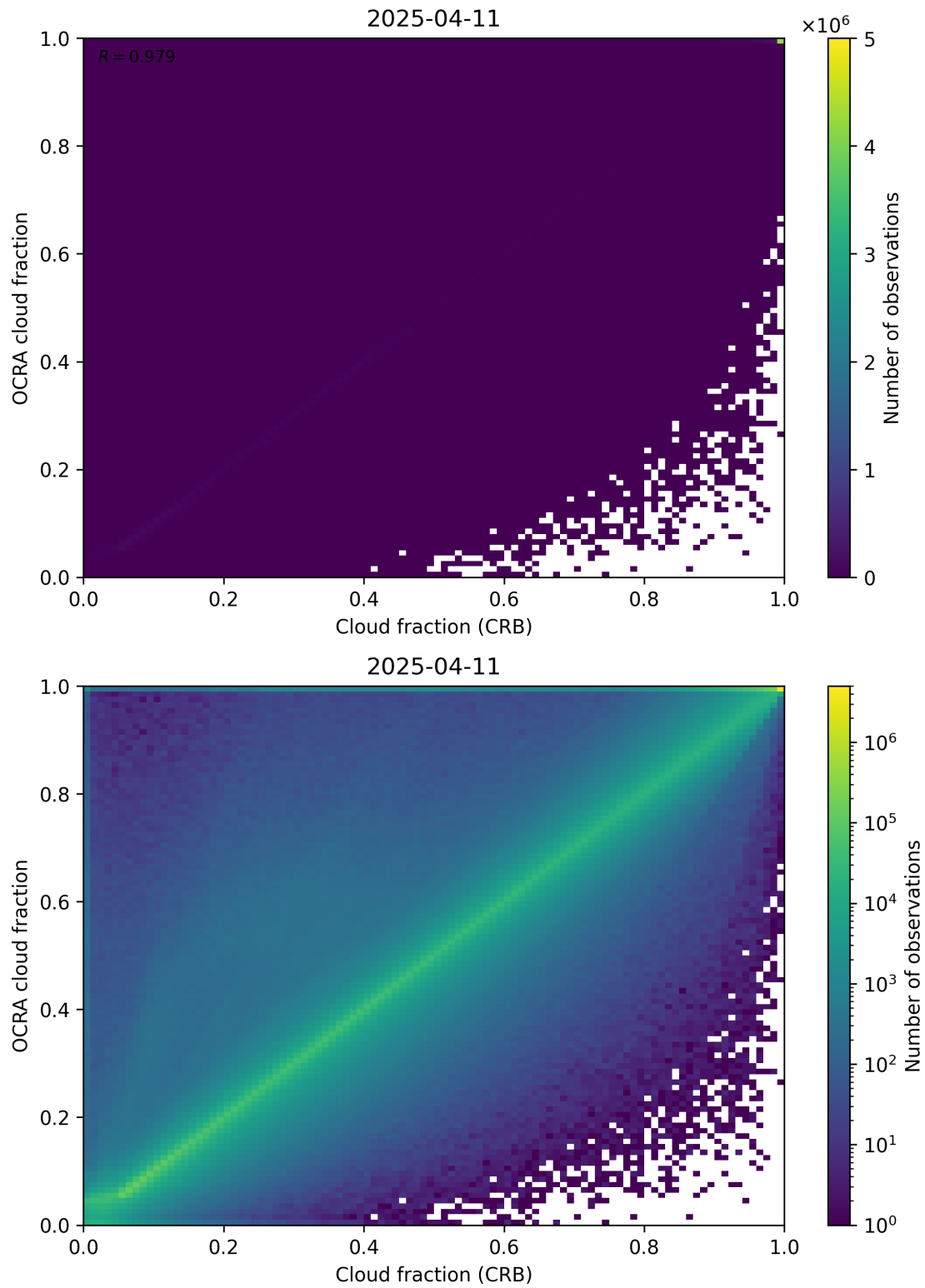
Figure 78: Scatter density plot of “Cloud fraction (CRB)” against “OCRA cloud fraction” for 2025-04-10 to 2025-04-12.
