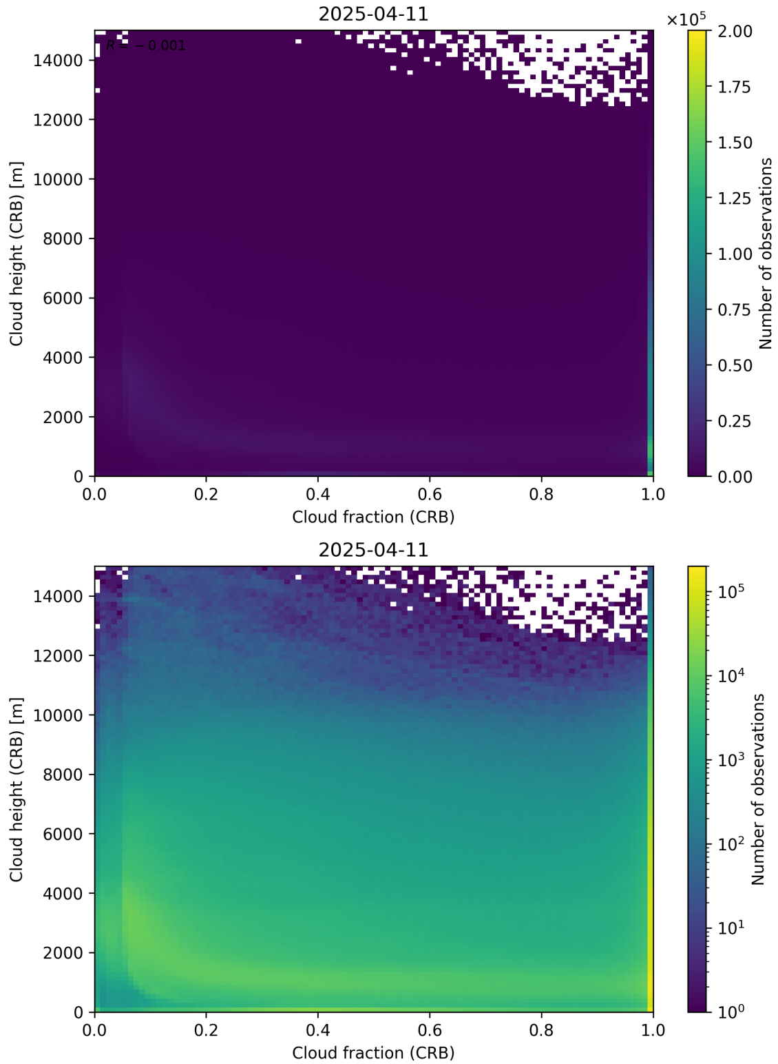
Figure 79: Scatter density plot of “Cloud fraction (CRB)” against “Cloud height (CRB)” for 2025-04-10 to 2025-04-12.
