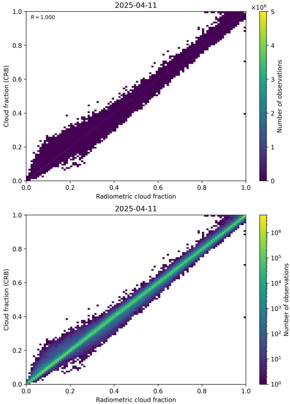
Figure 73: Scatter density plot of “Radiometric cloud fraction” against “Cloud fraction (CRB)” for 2025-04-10 to 2025-04-12.
