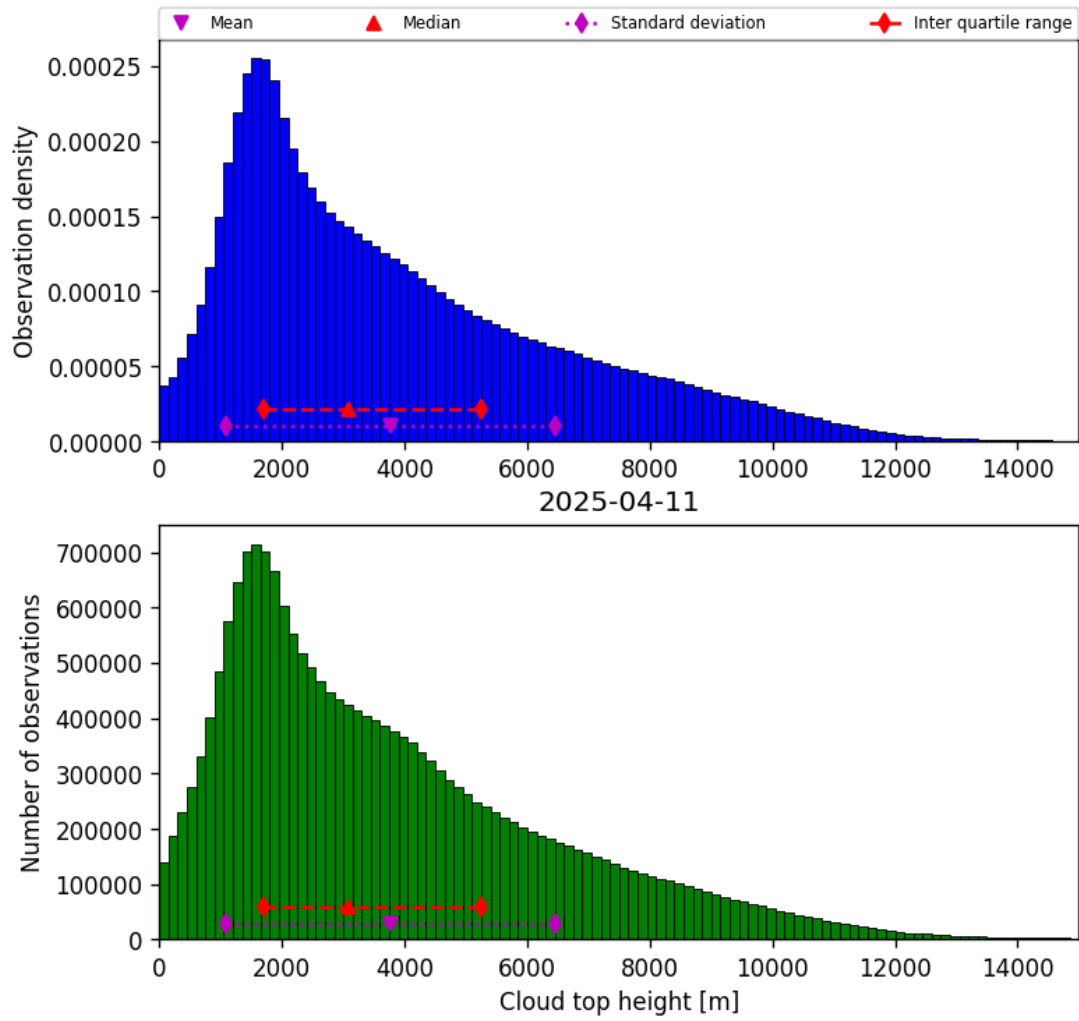
Figure 40: Histogram of “Cloud top height” for 2025-04-10 to 2025-04-12
