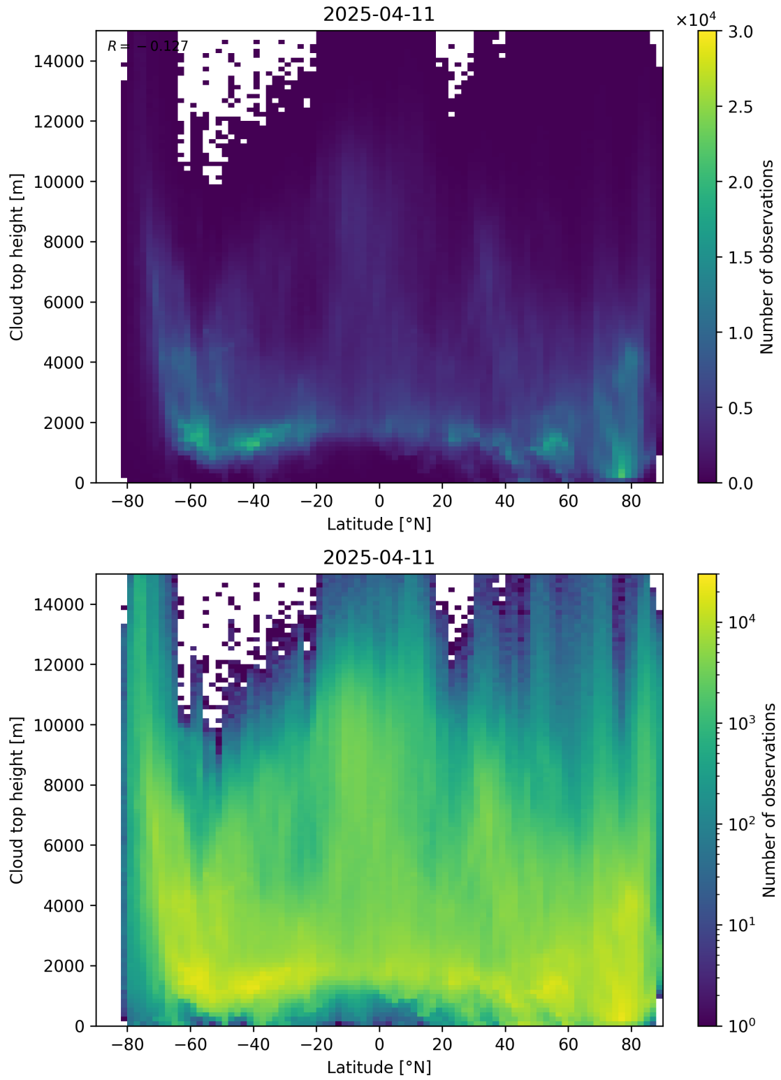
Figure 97: Scatter density plot of “Latitude” against “Cloud top height” for 2025-04-10 to 2025-04-12.
