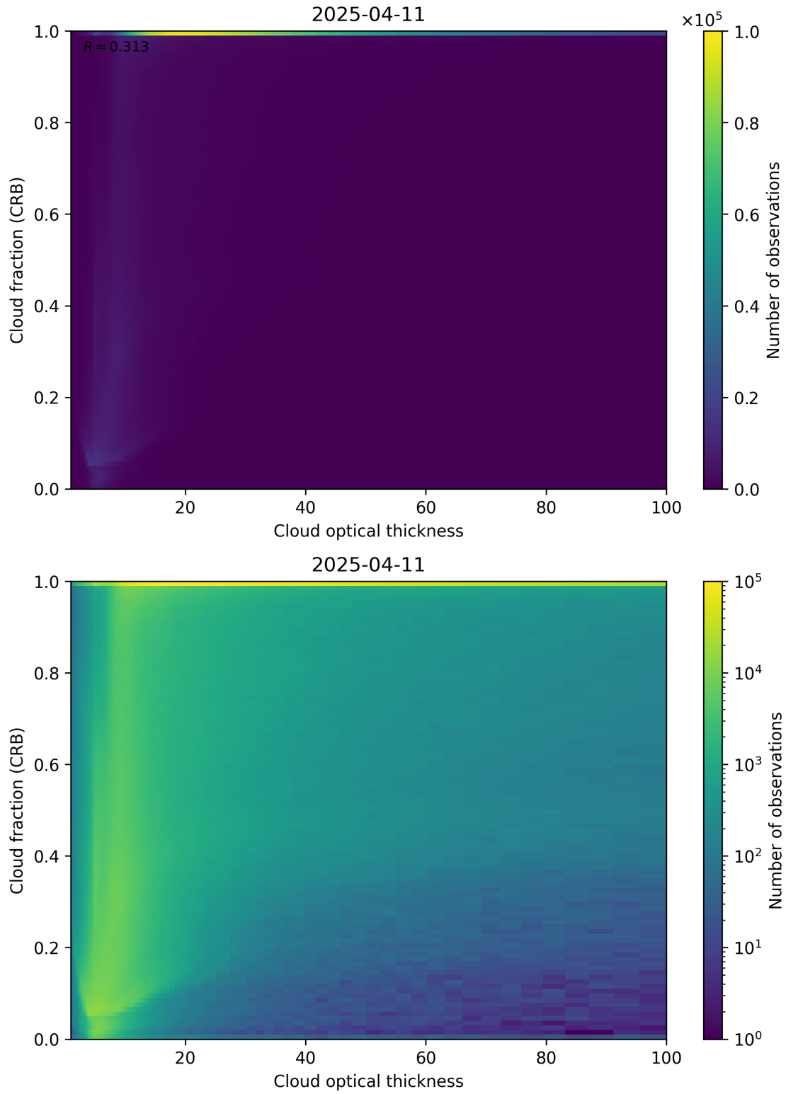
Figure 84: Scatter density plot of “Cloud optical thickness” against “Cloud fraction (CRB)” for 2025-04-10 to 2025-04-12.
