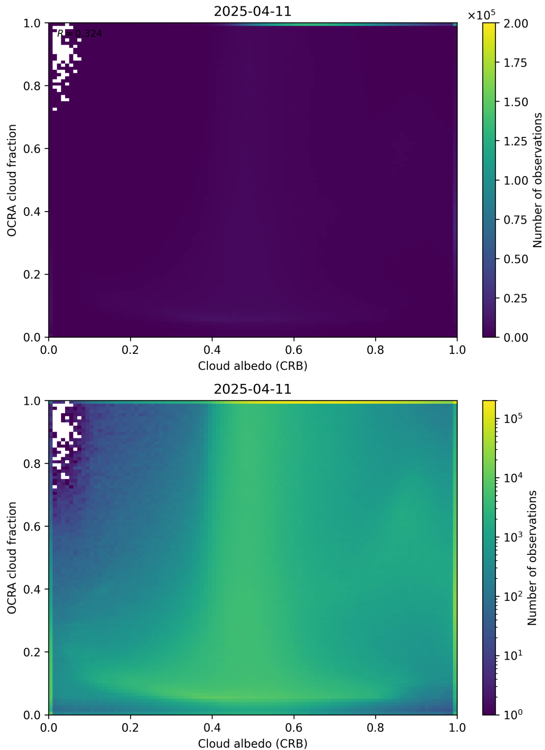
Figure 70: Scatter density plot of “Cloud albedo (CRB)” against “OCRA cloud fraction” for 2025-04-10 to 2025-04-12.
