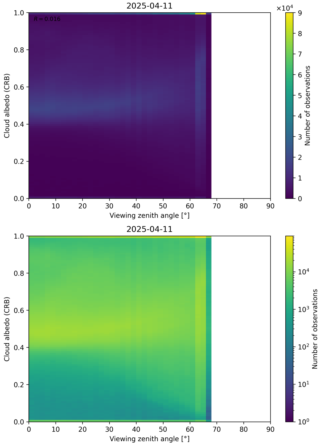
Figure 106: Scatter density plot of “Viewing zenith angle” against “Cloud albedo (CRB)” for 2025-04-10 to 2025-04-12.
