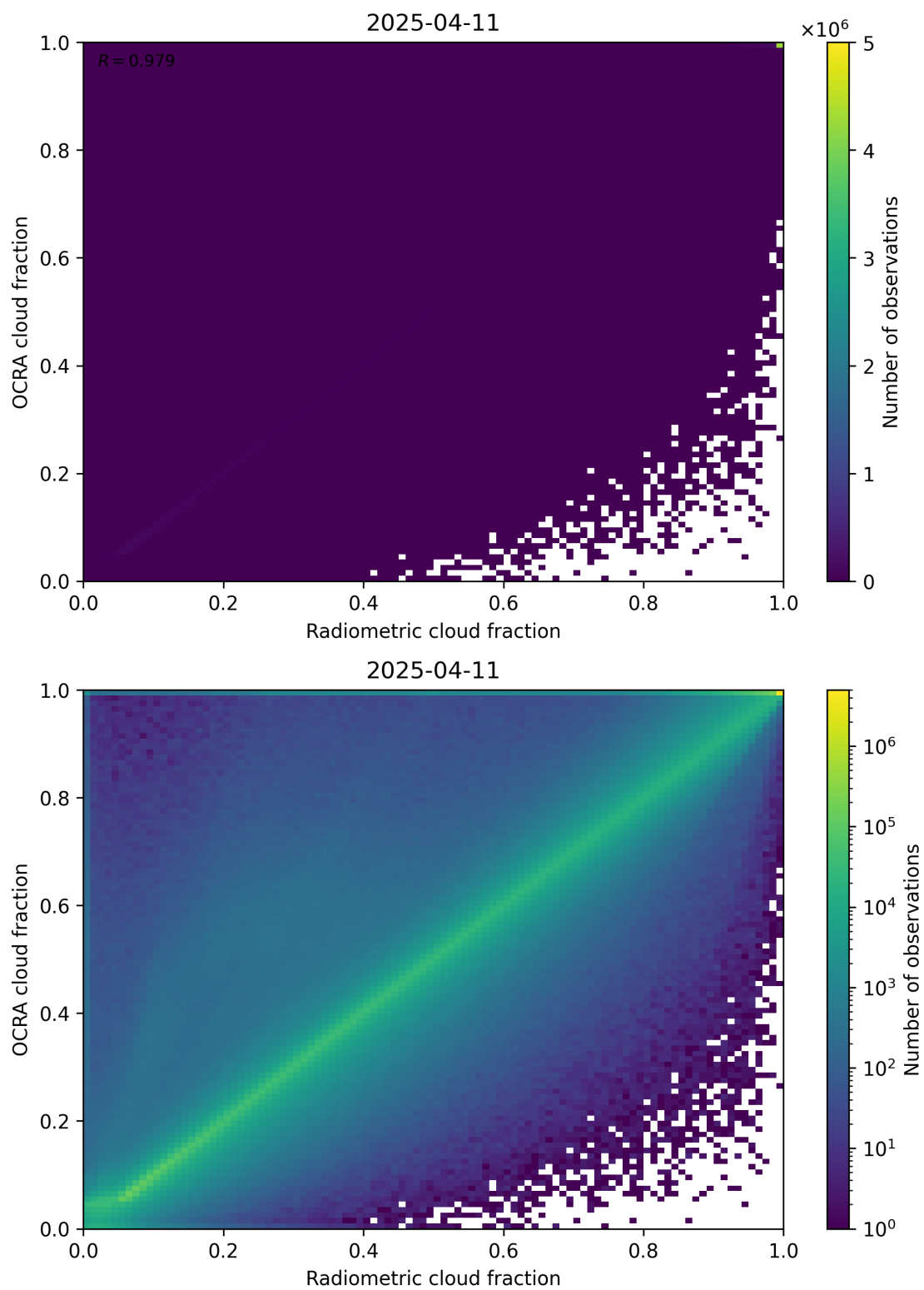
Figure 72: Scatter density plot of “Radiometric cloud fraction” against “OCRA cloud fraction” for 2025-04-10 to 2025-04-12.
