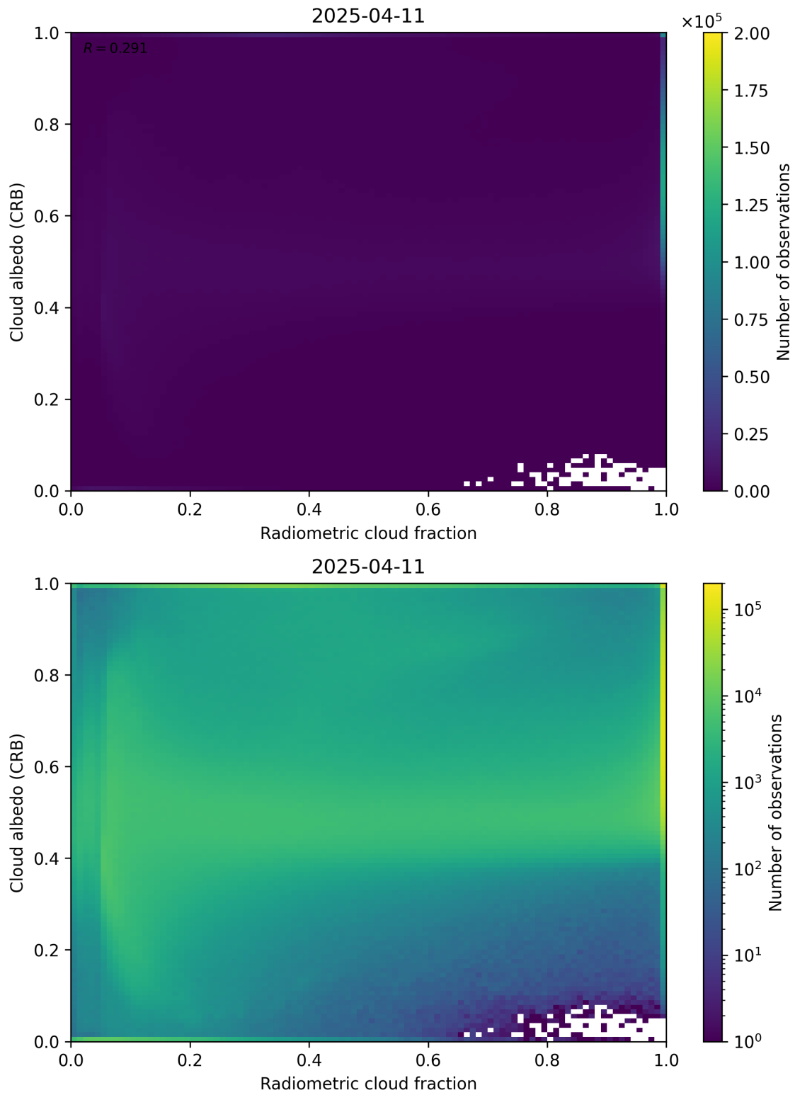
Figure 71: Scatter density plot of “Radiometric cloud fraction” against “Cloud albedo (CRB)” for 2025-04-10 to 2025-04-12.
