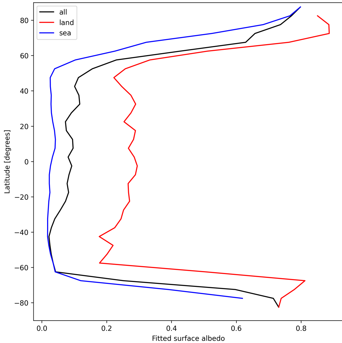
Figure 29: Zonal average of “Fitted surface albedo” for 2025-04-10 to 2025-04-12.
