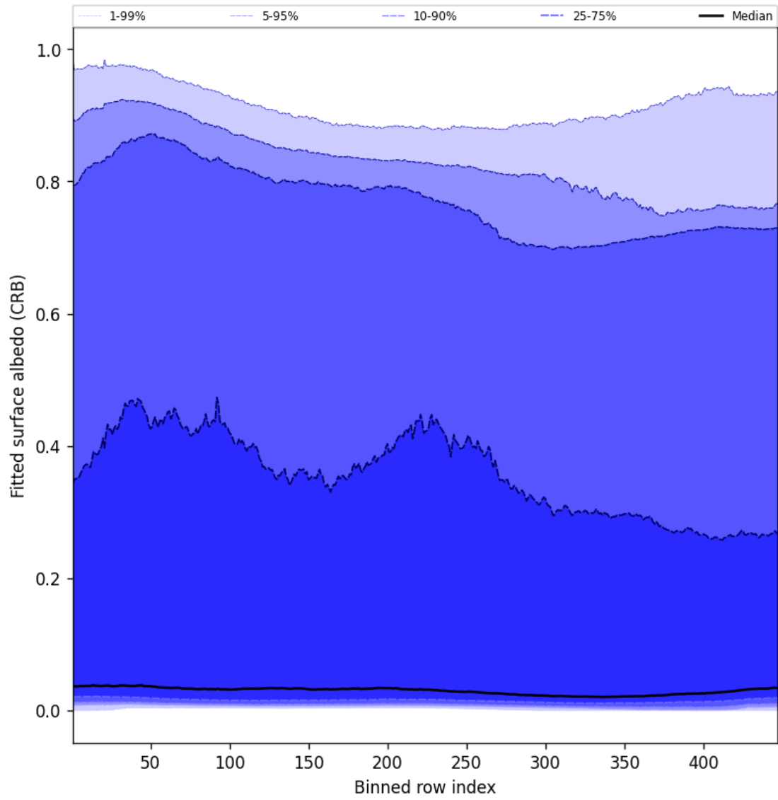
Figure 62: Along track statistics of “Fitted surface albedo (CRB)” for 2025-04-10 to 2025-04-12
