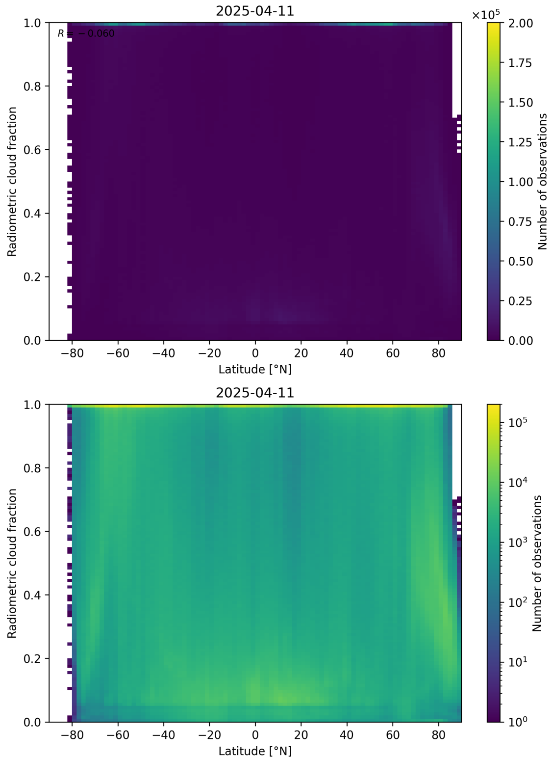
Figure 92: Scatter density plot of “Latitude” against “Radiometric cloud fraction” for 2025-04-10 to 2025-04-12.
