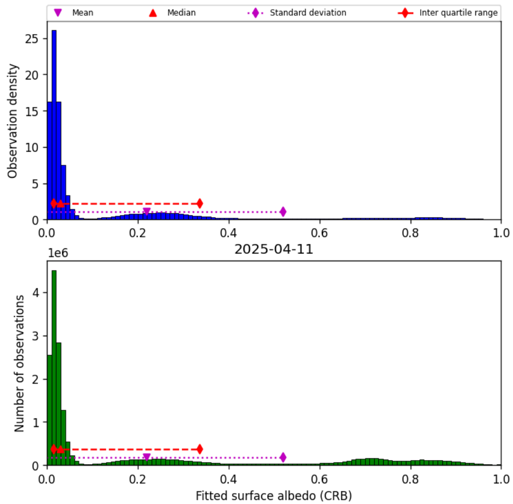
Figure 46: Histogram of “Fitted surface albedo (CRB)” for 2025-04-10 to 2025-04-12
