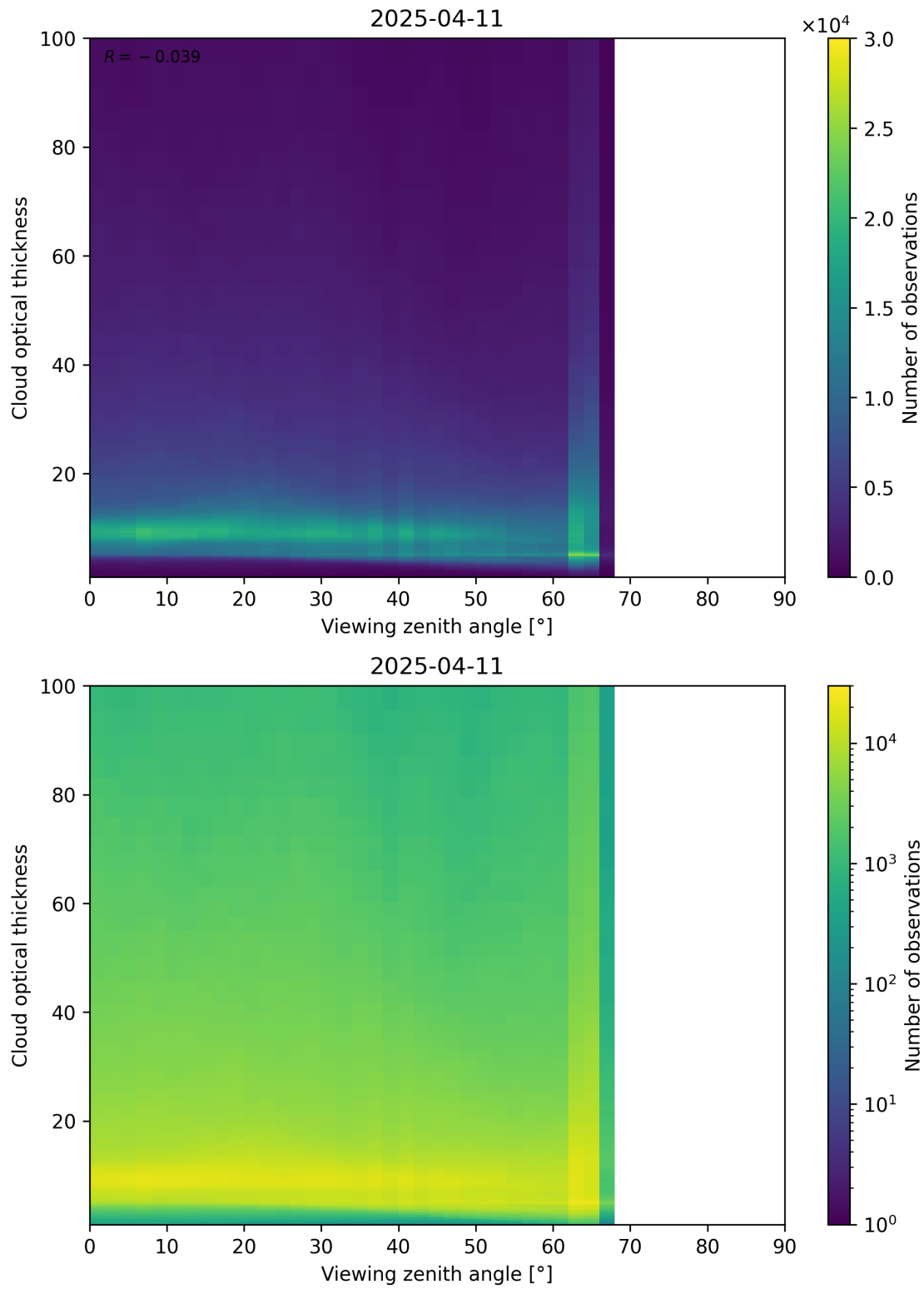
Figure 111: Scatter density plot of “Viewing zenith angle” against “Cloud optical thickness” for 2025-04-10 to 2025-04-12.
