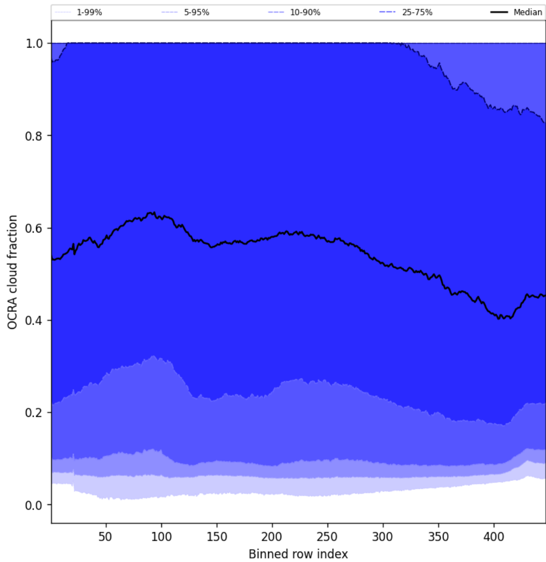
Figure 66: Along track statistics of “OCRA cloud fraction” for 2025-04-10 to 2025-04-12
