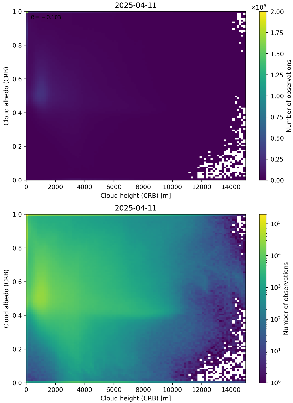
Figure 80: Scatter density plot of “Cloud height (CRB)” against “Cloud albedo (CRB)” for 2025-04-10 to 2025-04-12.
