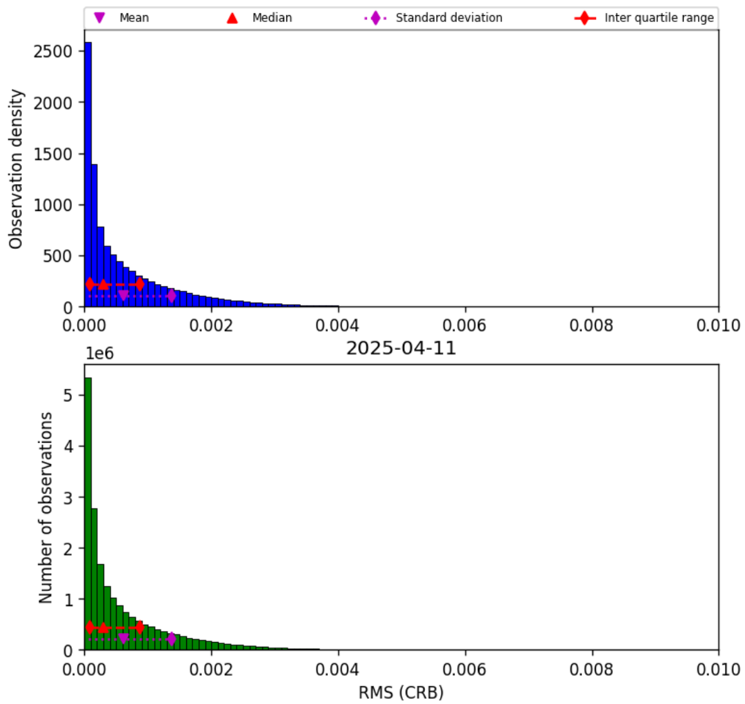
Figure 48: Histogram of “RMS (CRB)” for 2025-04-10 to 2025-04-12
