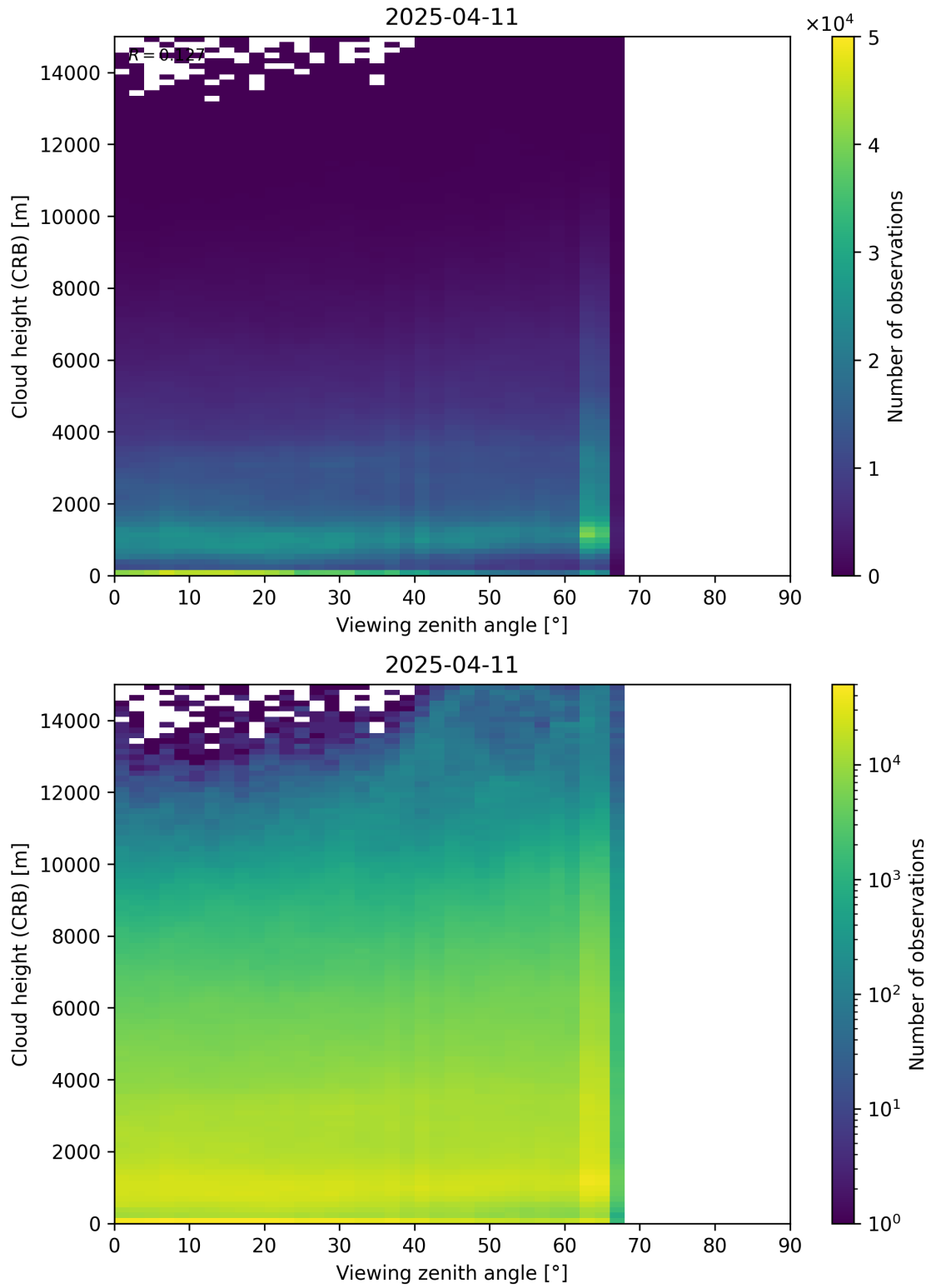
Figure 110: Scatter density plot of “Viewing zenith angle” against “Cloud height (CRB)” for 2025-04-10 to 2025-04-12.
