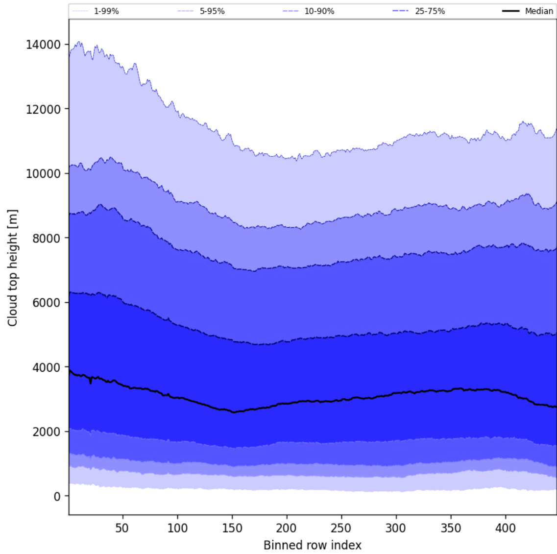
Figure 56: Along track statistics of “Cloud top height” for 2025-04-10 to 2025-04-12
