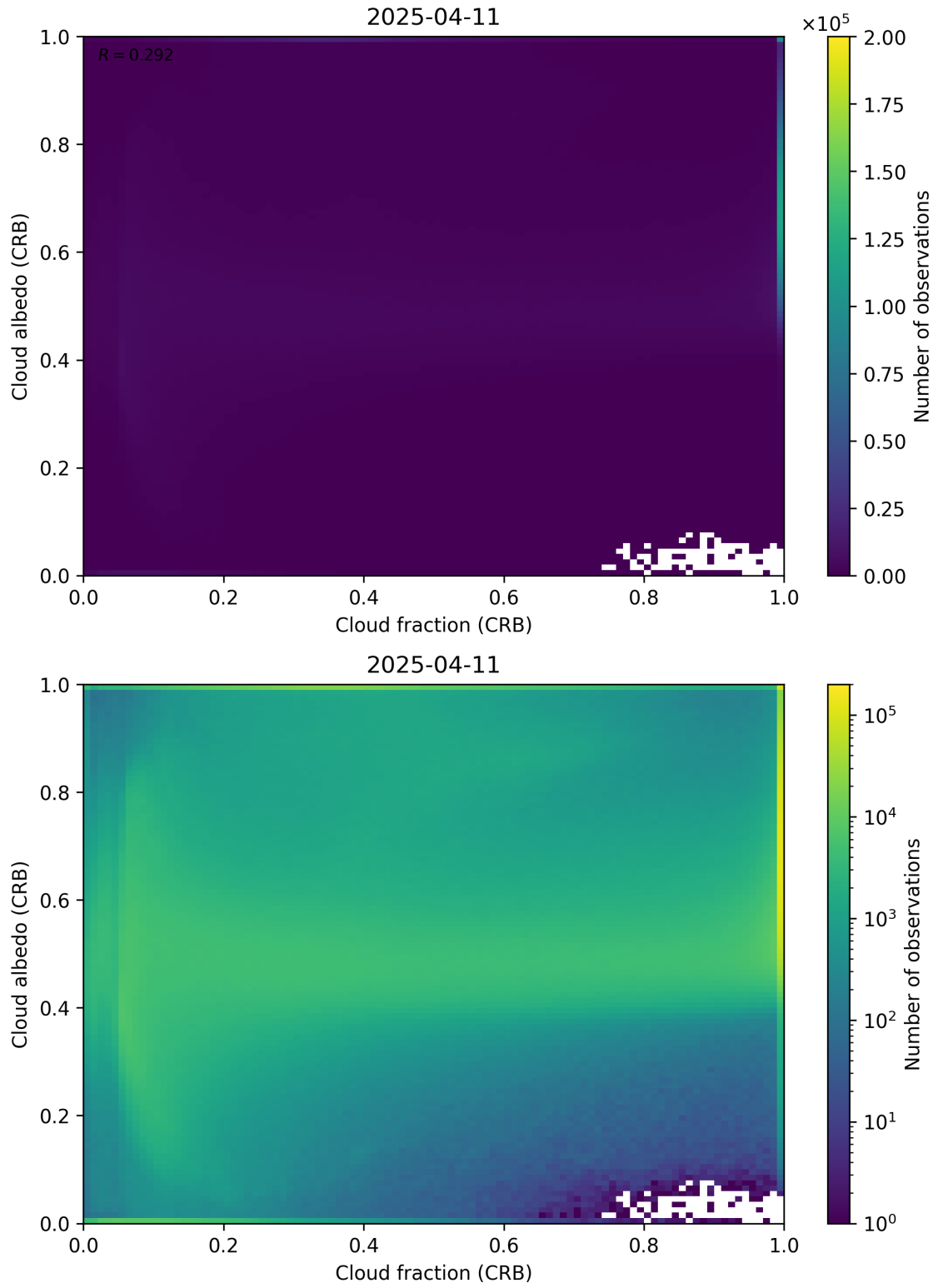
Figure 77: Scatter density plot of “Cloud fraction (CRB)” against “Cloud albedo (CRB)” for 2025-04-10 to 2025-04-12.
