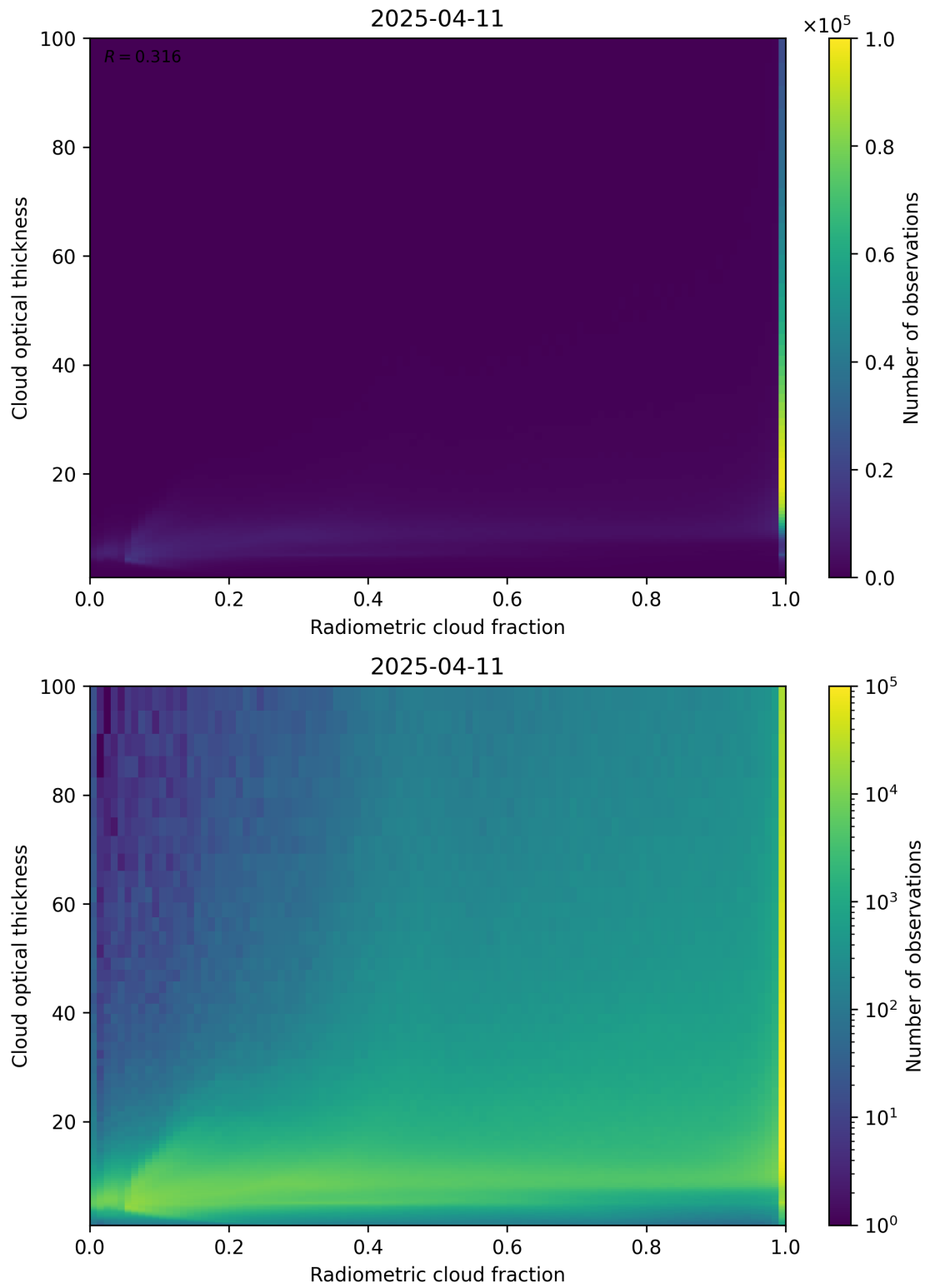
Figure 75: Scatter density plot of “Radiometric cloud fraction” against “Cloud optical thickness” for 2025-04-10 to 2025-04-12.
