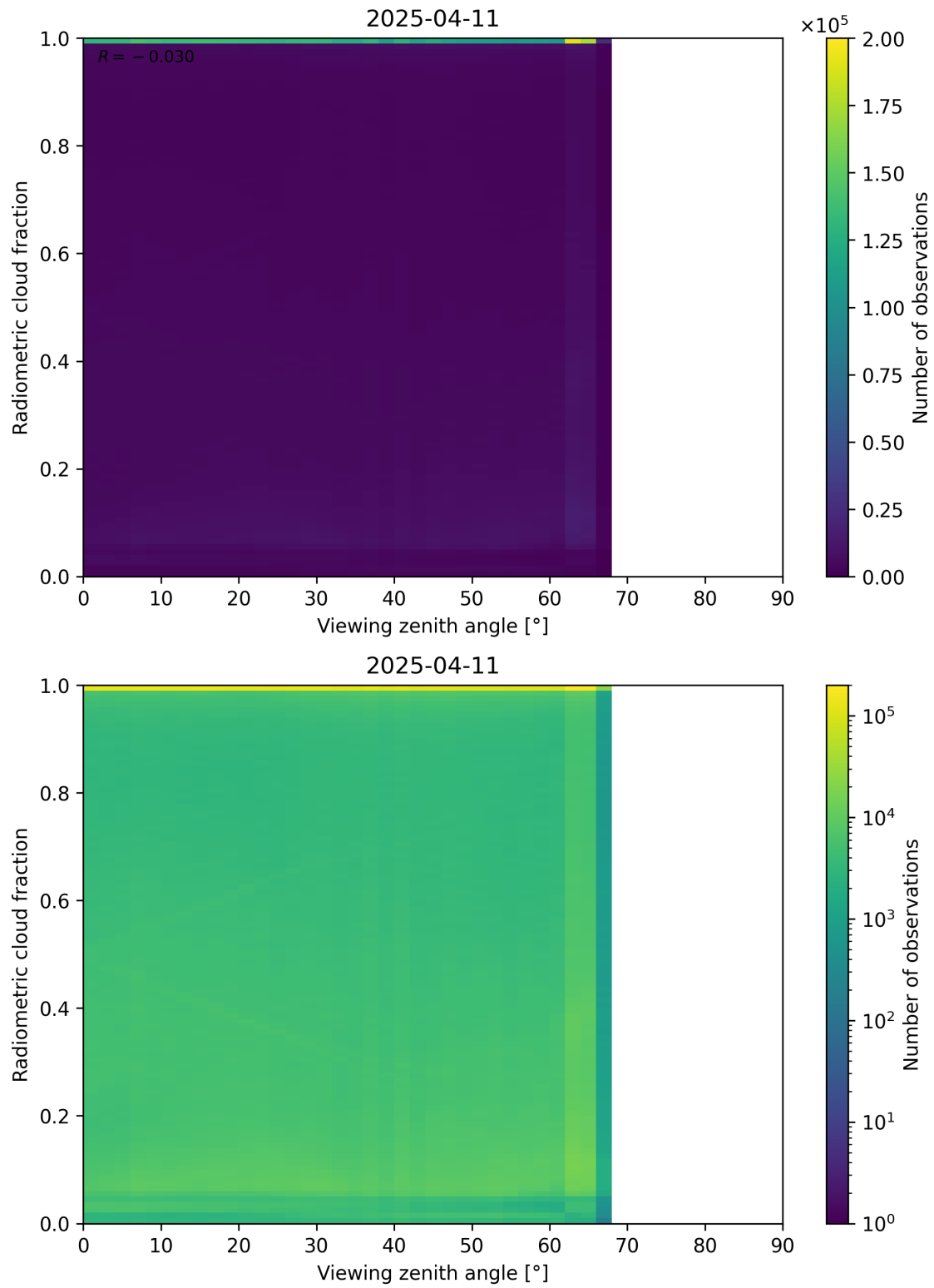
Figure 107: Scatter density plot of “Viewing zenith angle” against “Radiometric cloud fraction” for 2025-04-10 to 2025-04-12.
