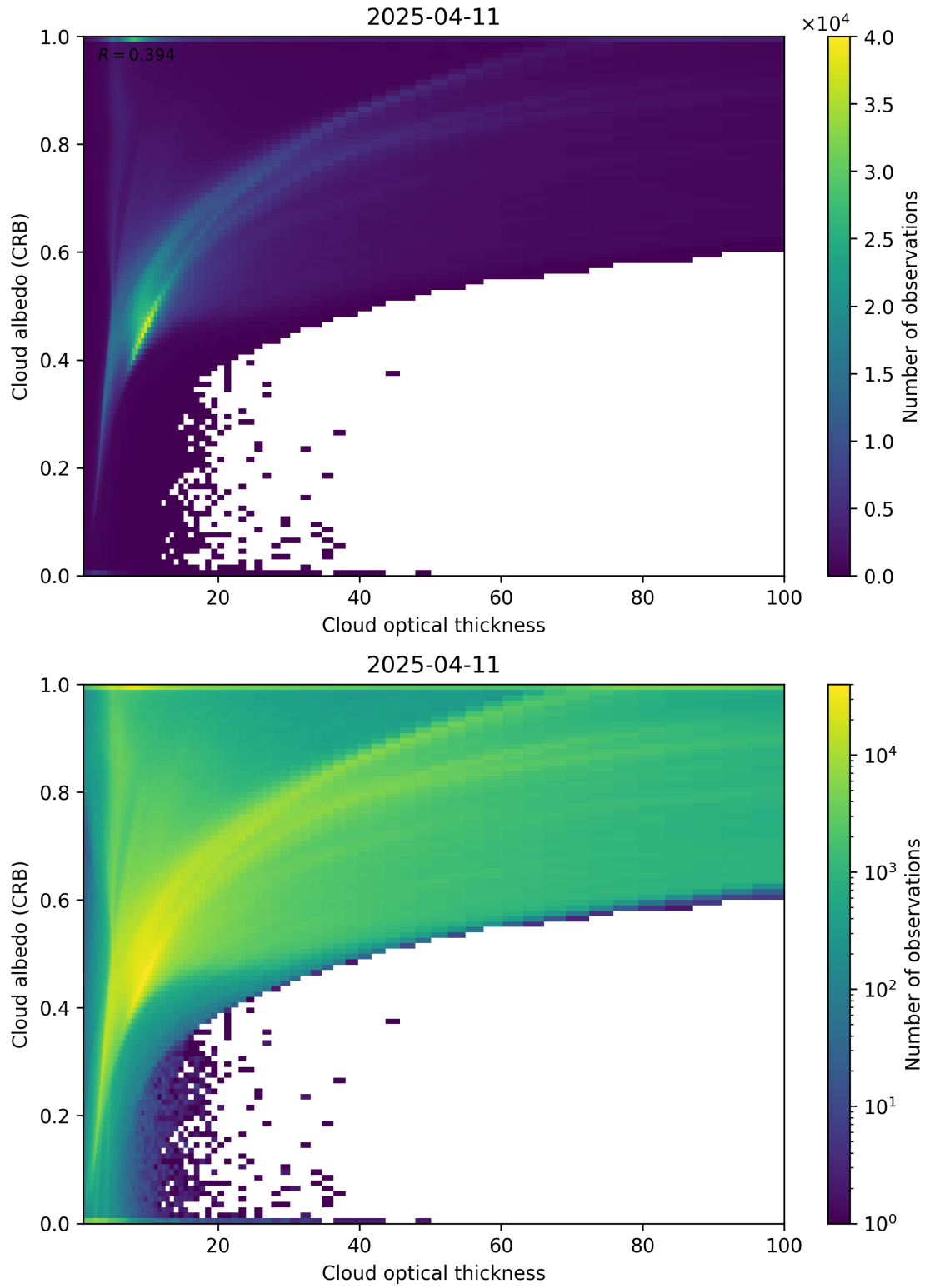
Figure 82: Scatter density plot of “Cloud optical thickness” against “Cloud albedo (CRB)” for 2025-04-10 to 2025-04-12.
