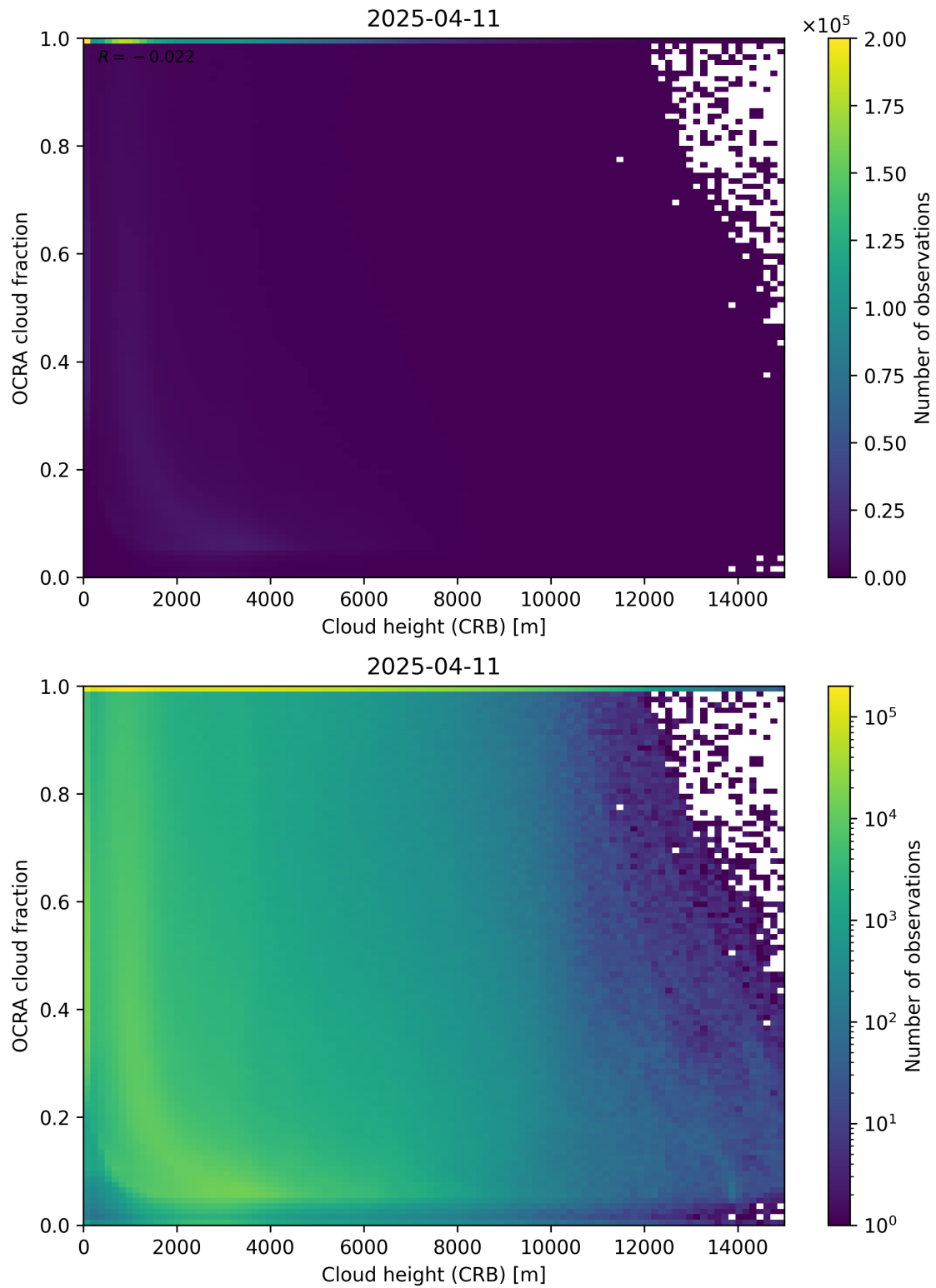
Figure 81: Scatter density plot of “Cloud height (CRB)” against “OCRA cloud fraction” for 2025-04-10 to 2025-04-12.
