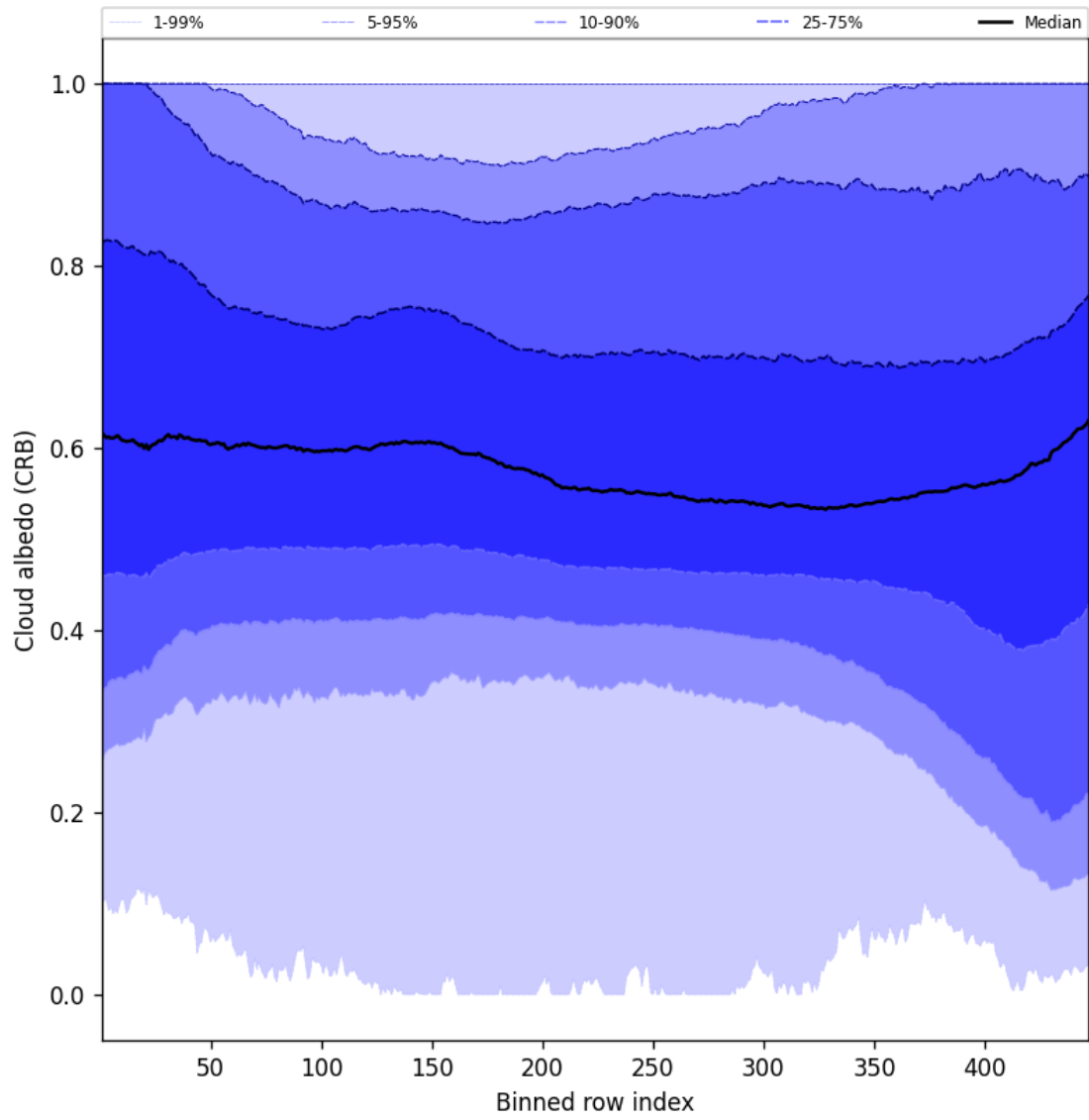
Figure 60: Along track statistics of “Cloud albedo (CRB)” for 2025-04-10 to 2025-04-12
