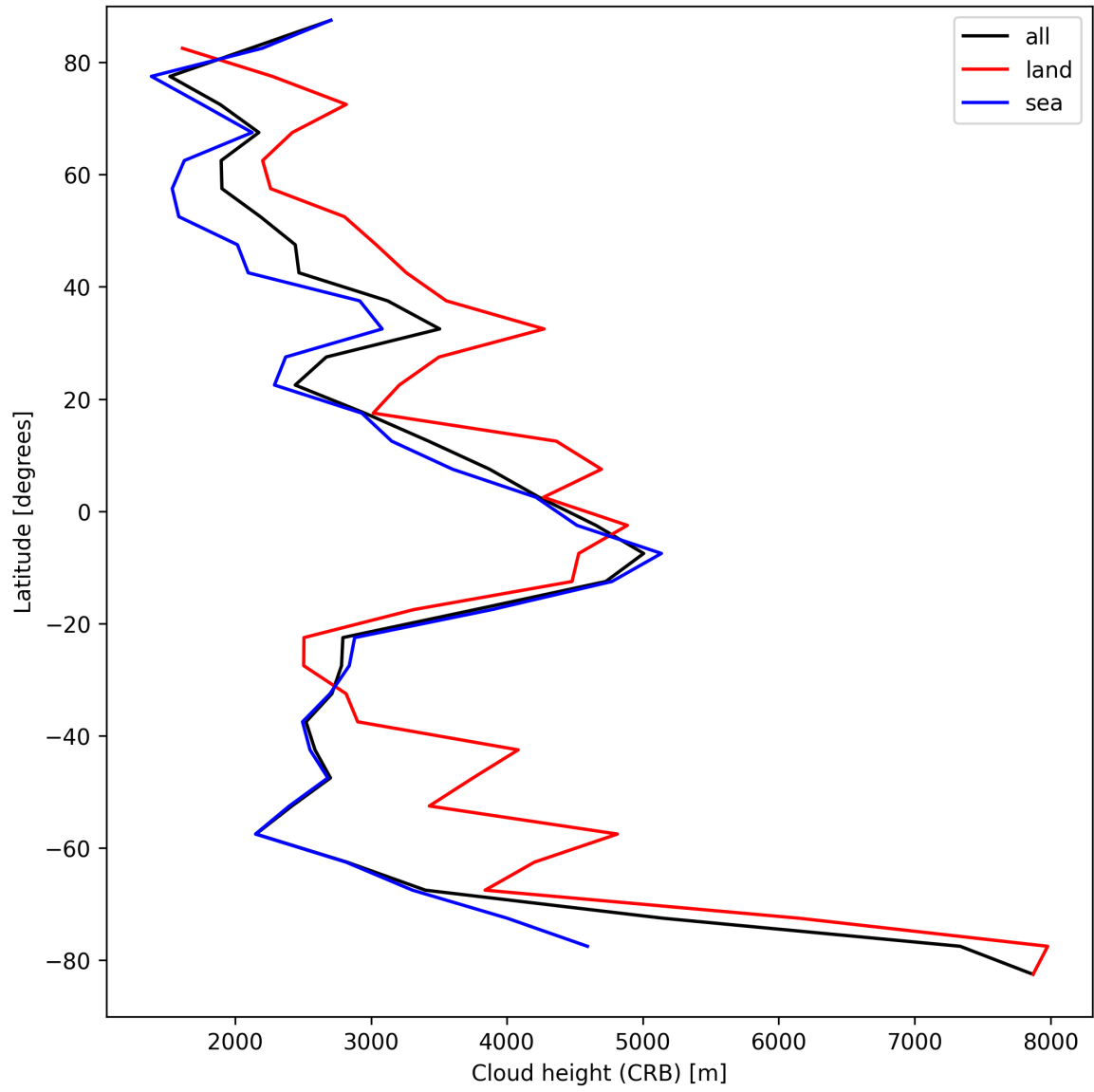
Figure 27: Zonal average of “Cloud height (CRB)” for 2025-04-10 to 2025-04-12.
