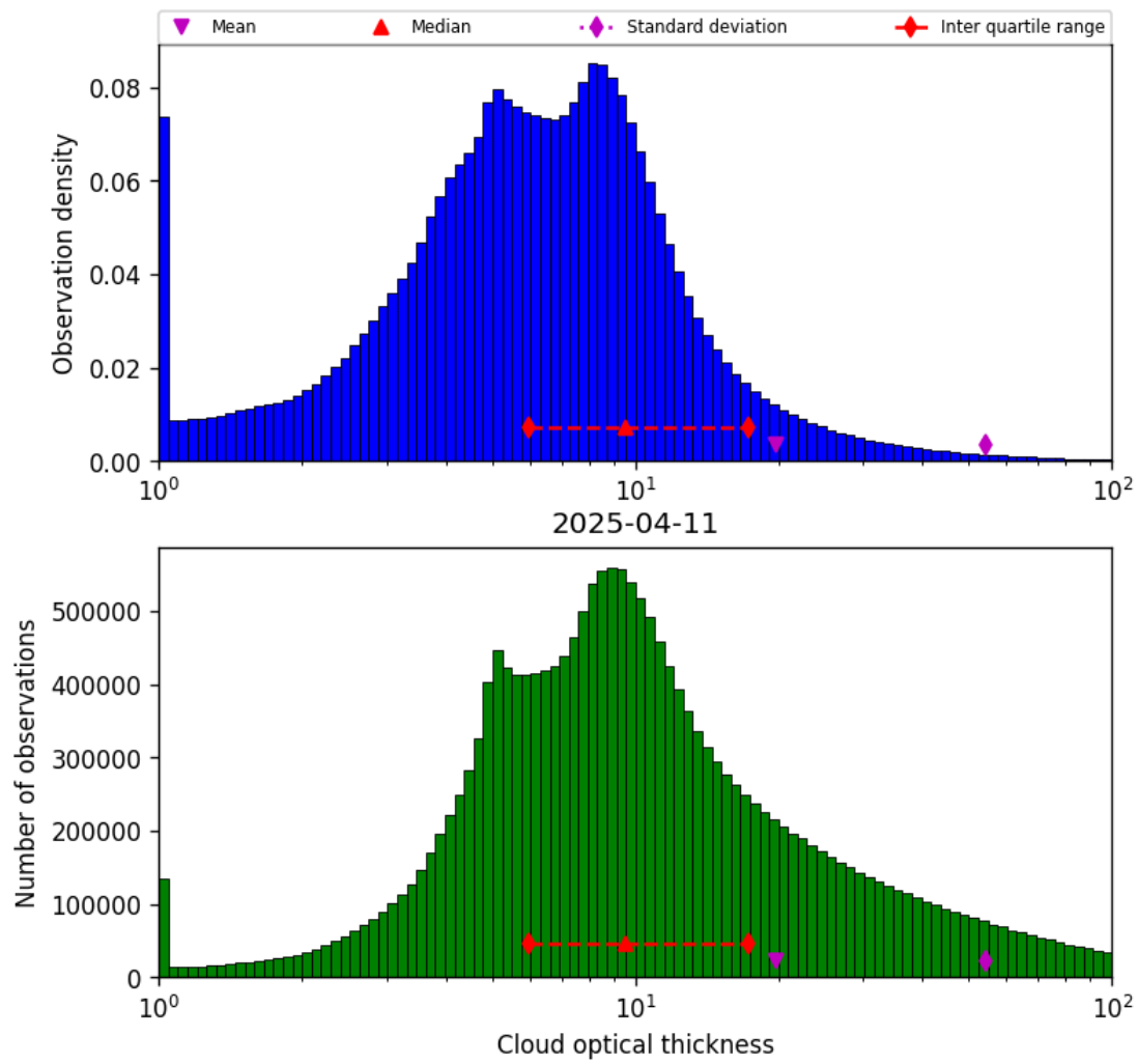
Figure 41: Histogram of “Cloud optical thickness” for 2025-04-10 to 2025-04-12
