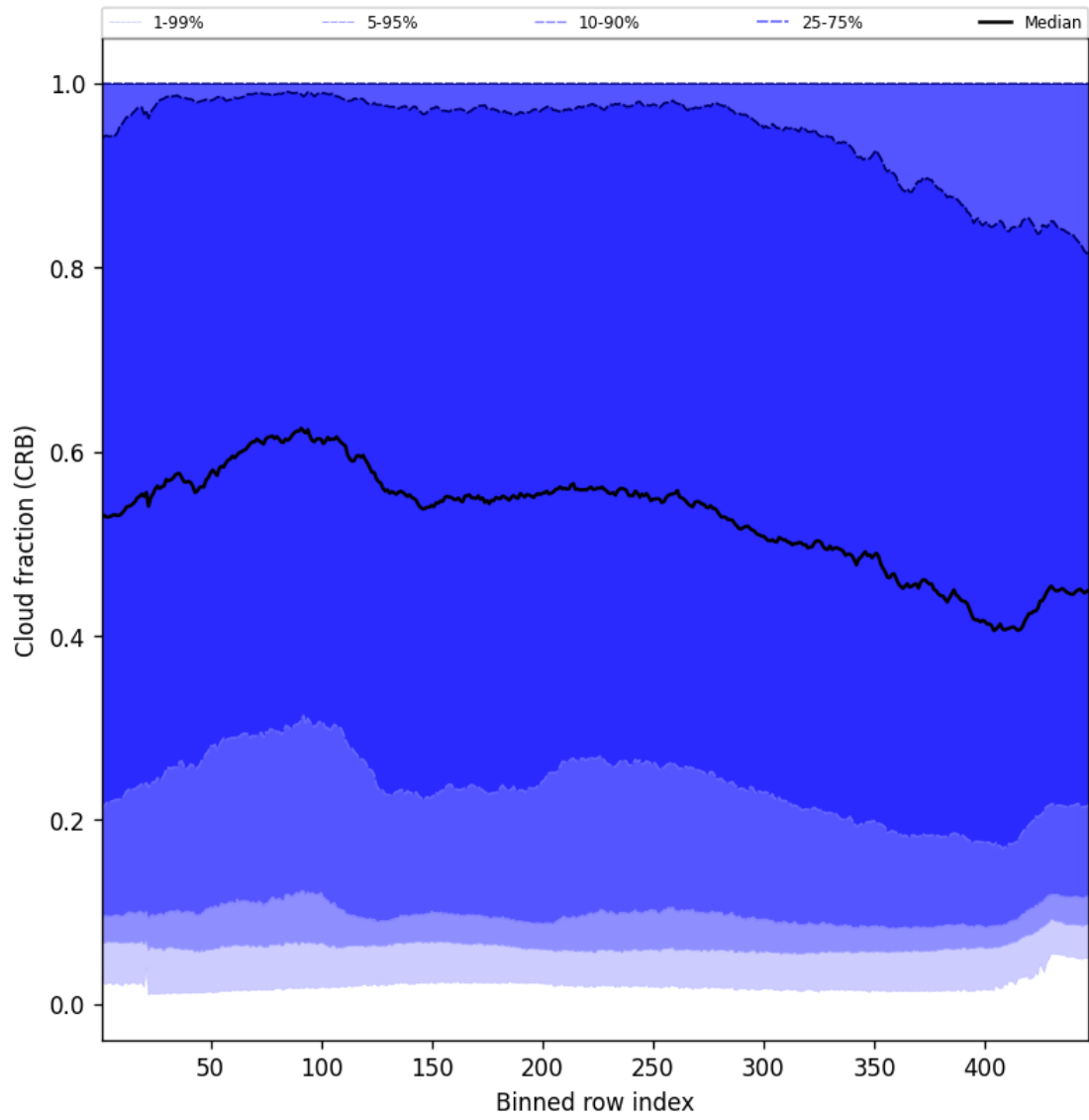
Figure 58: Along track statistics of “Cloud fraction (CRB)” for 2025-04-10 to 2025-04-12
