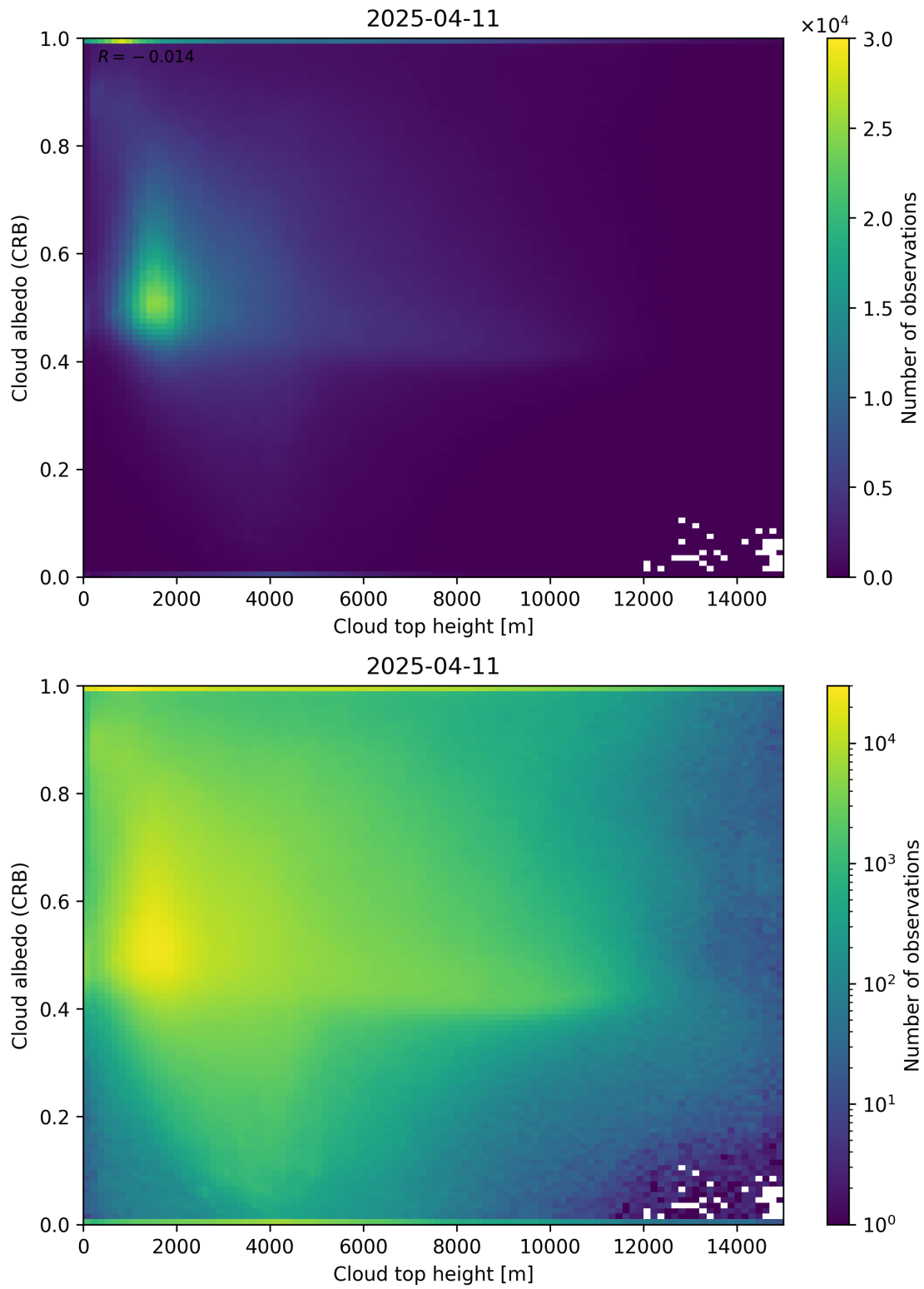
Figure 86: Scatter density plot of “Cloud top height” against “Cloud albedo (CRB)” for 2025-04-10 to 2025-04-12.
