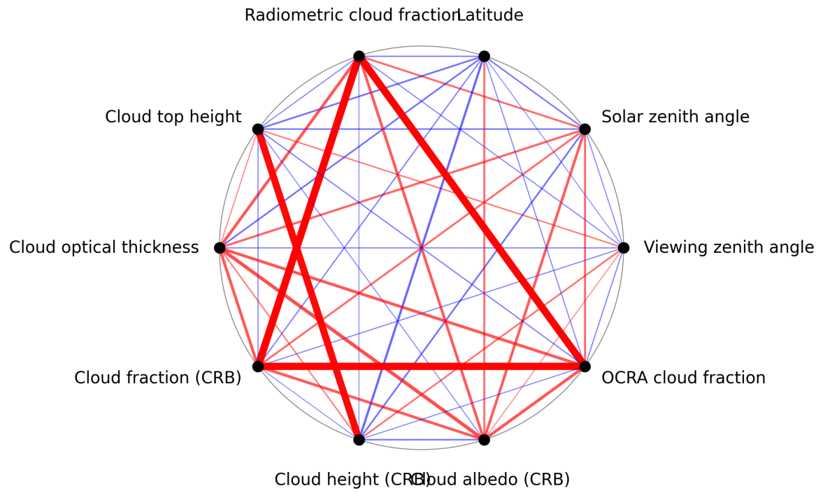
Figure 1: Map of correlation graph for 2025-04-10 to 2025-04-12.
