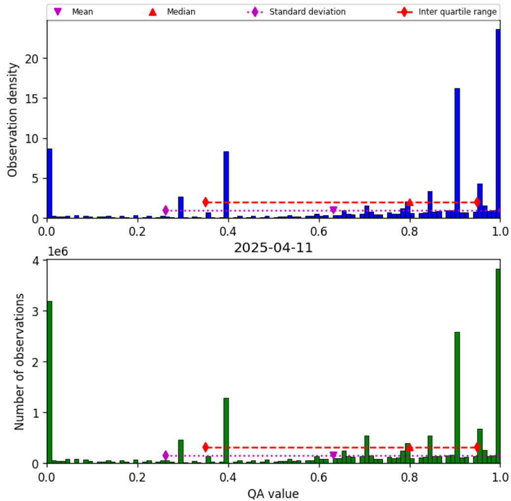
Figure 38: Histogram of “QA value” for 2025-04-10 to 2025-04-12
