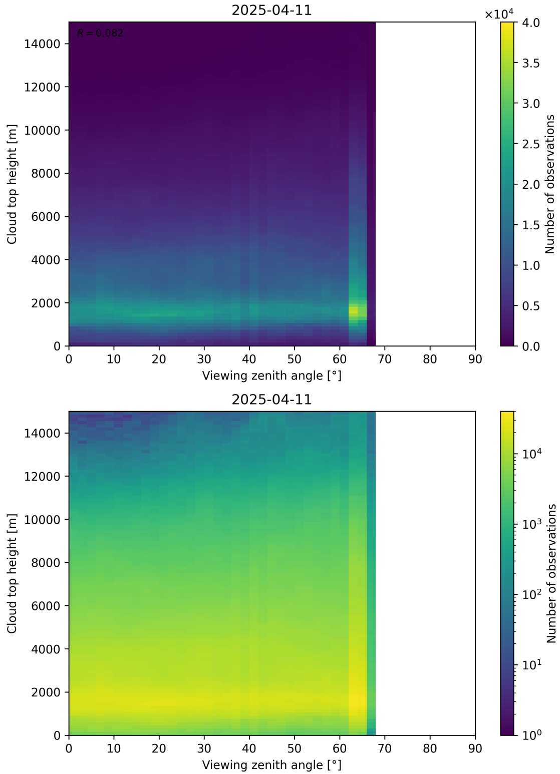
Figure 112: Scatter density plot of “Viewing zenith angle” against “Cloud top height” for 2025-04-10 to 2025-04-12.
