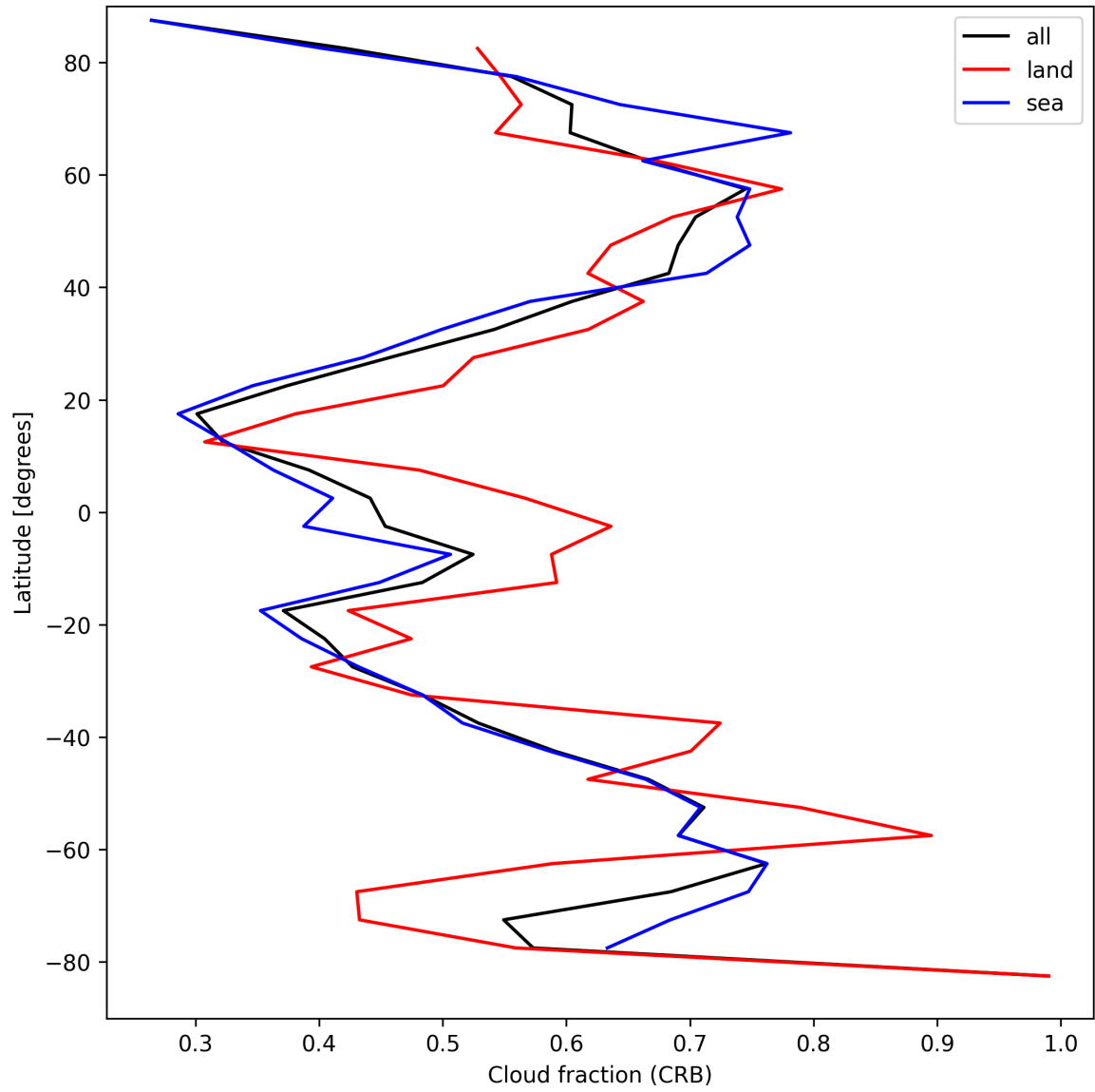
Figure 26: Zonal average of “Cloud fraction (CRB)” for 2025-04-10 to 2025-04-12.
