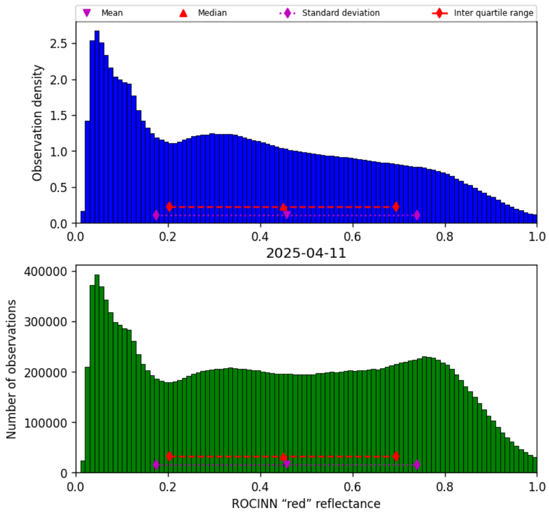
Figure 53: Histogram of “ROCINN “red” reflectance” for 2025-04-10 to 2025-04-12
