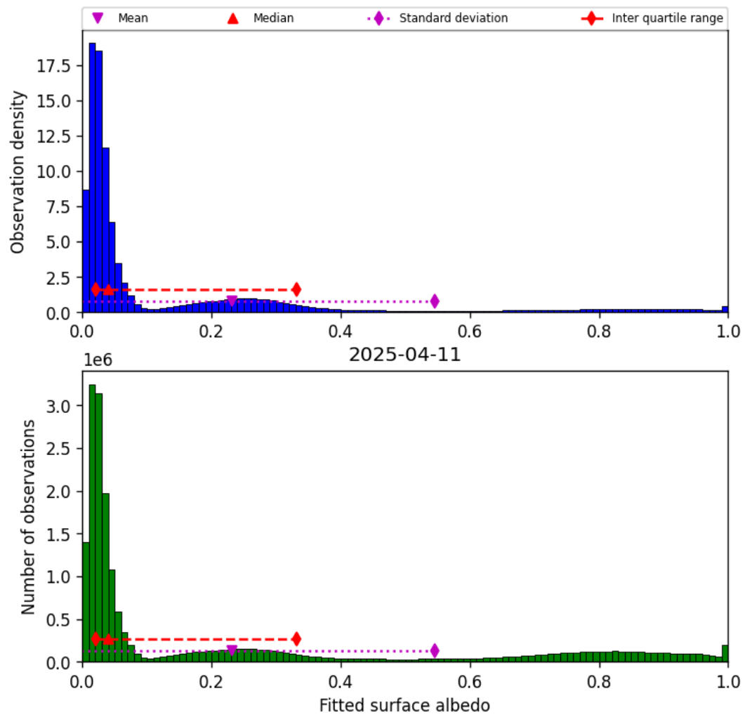
Figure 45: Histogram of “Fitted surface albedo” for 2025-04-10 to 2025-04-12
