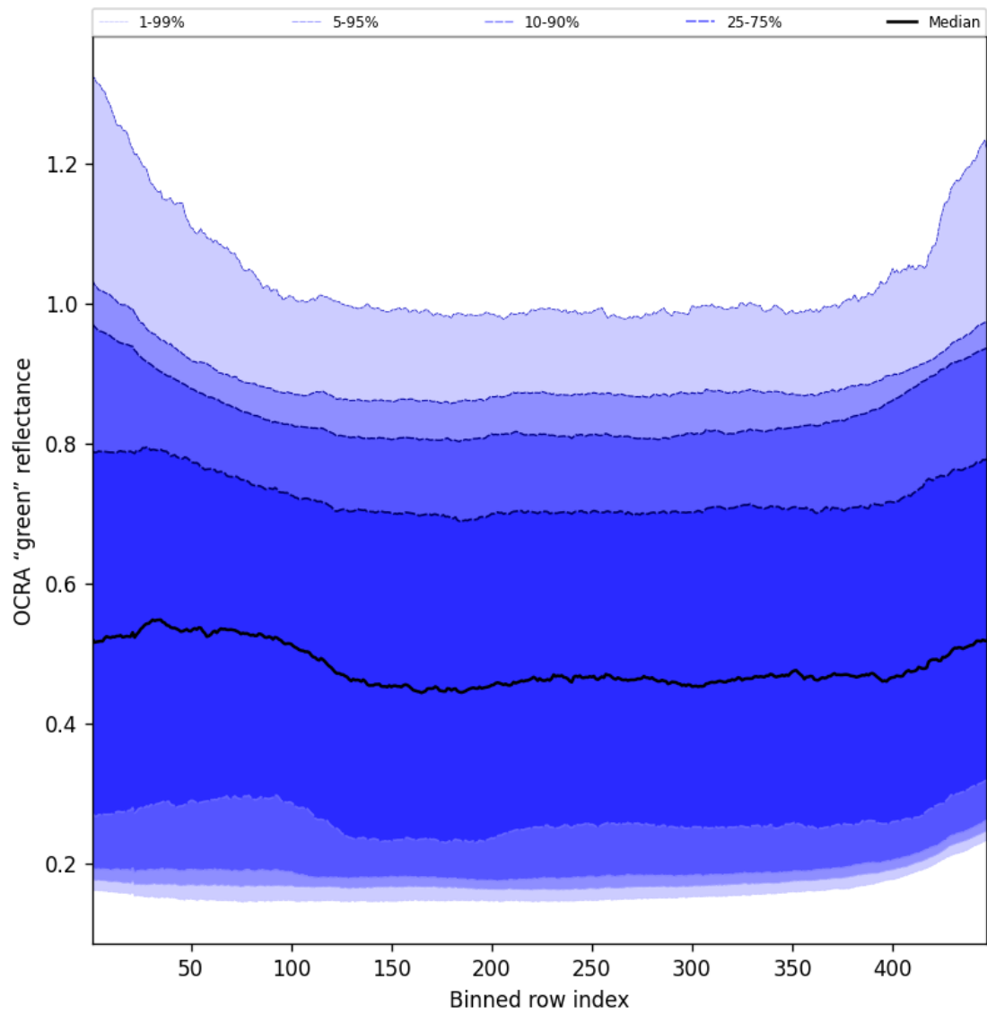
Figure 68: Along track statistics of "OCRA "green" reflectance" for 2025-04-10 to 2025-04-12
