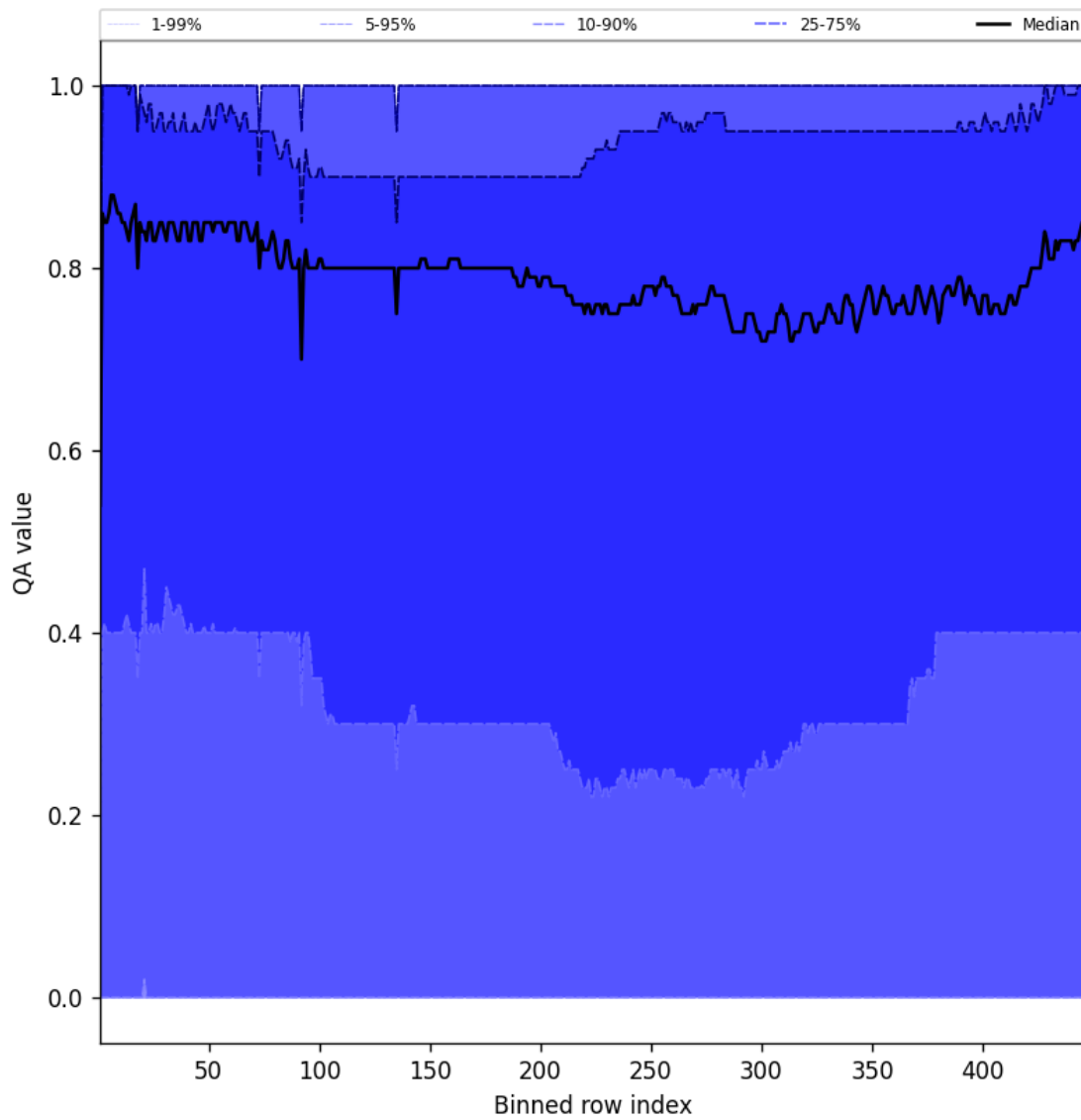
Figure 54: Along track statistics of “QA value” for 2025-04-10 to 2025-04-12
