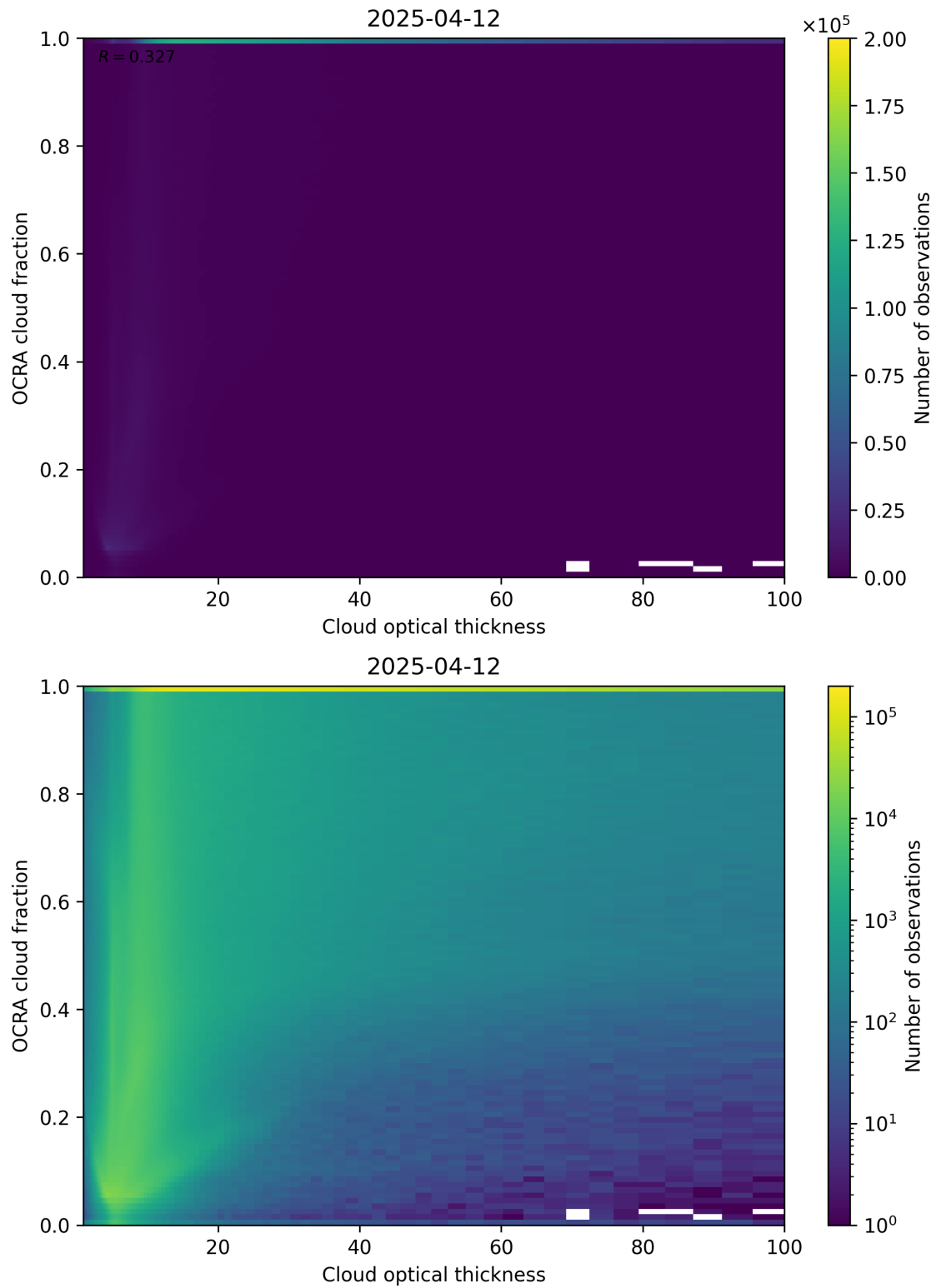
Figure 83: Scatter density plot of “Cloud optical thickness” against “OCRA cloud fraction” for 2025-04-11 to 2025-04-13.
