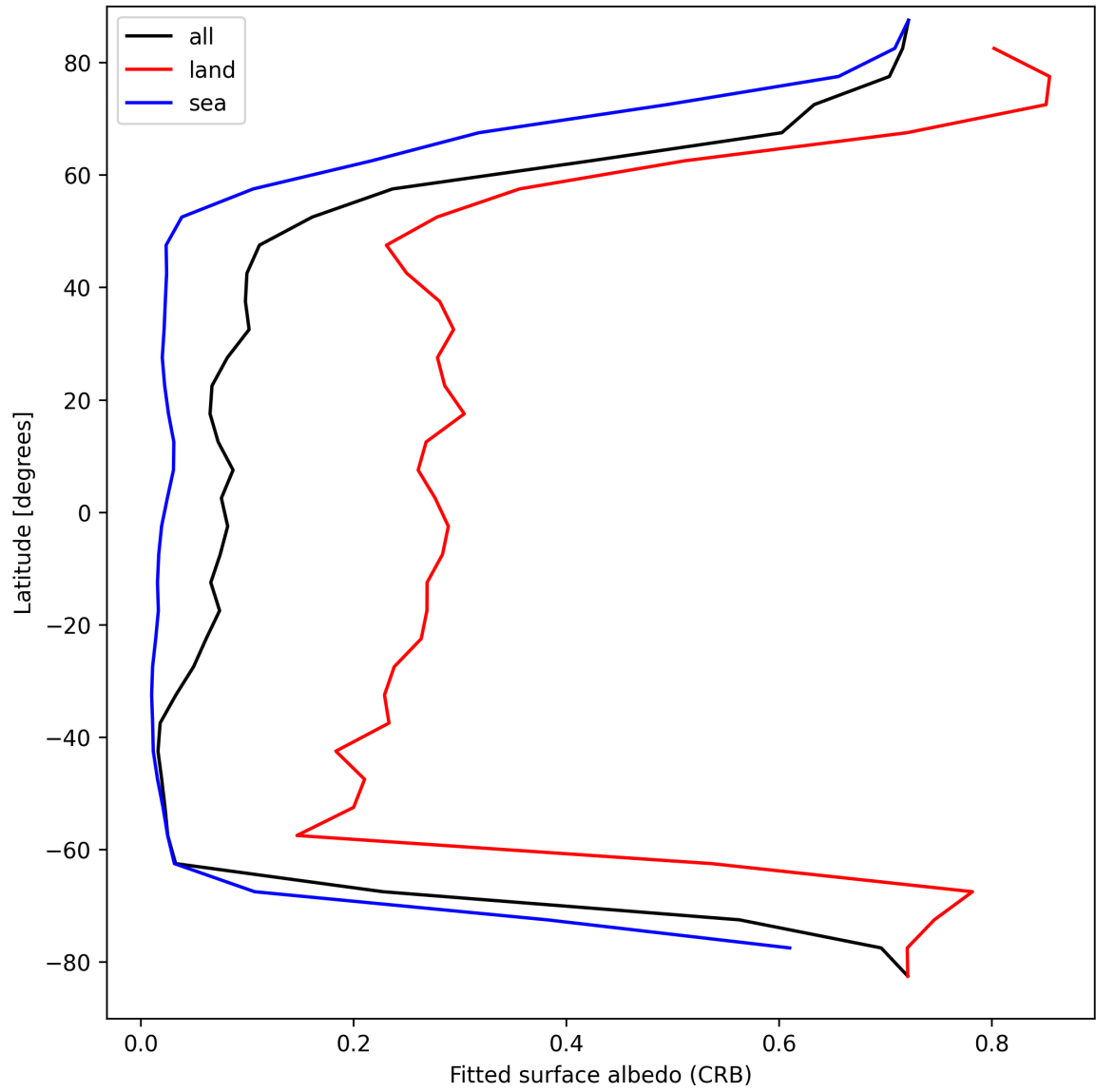
Figure 30: Zonal average of “Fitted surface albedo (CRB)” for 2025-04-11 to 2025-04-13.
