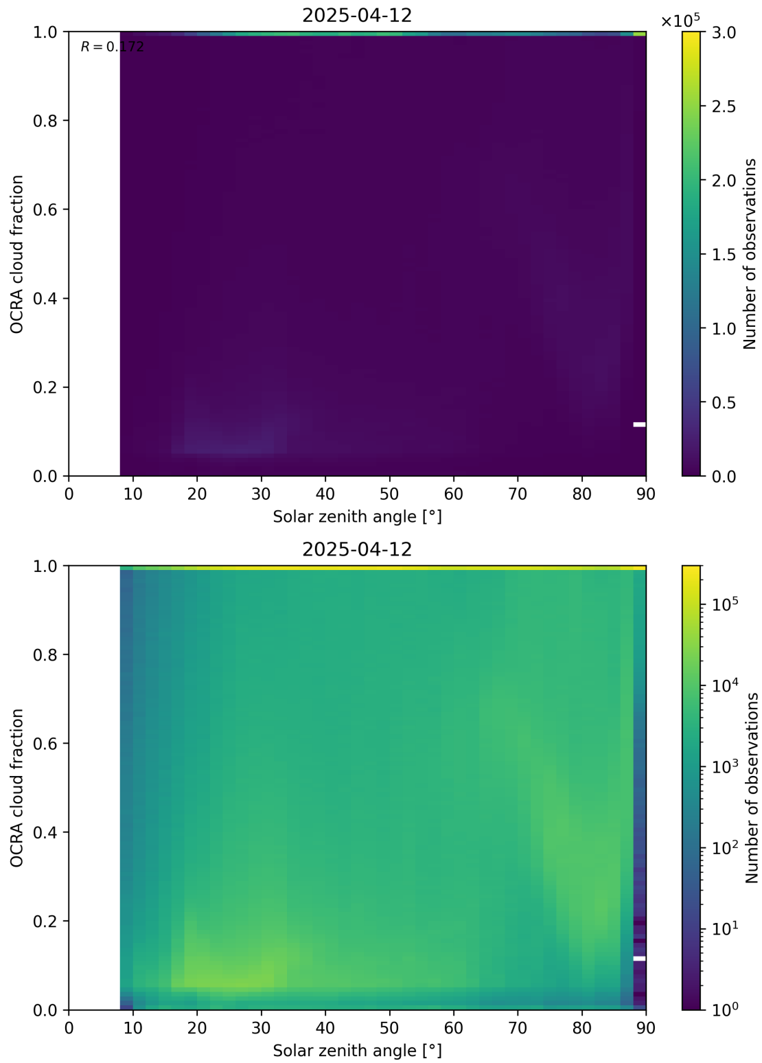
Figure 100: Scatter density plot of “Solar zenith angle” against “OCRA cloud fraction” for 2025-04-11 to 2025-04-13.
