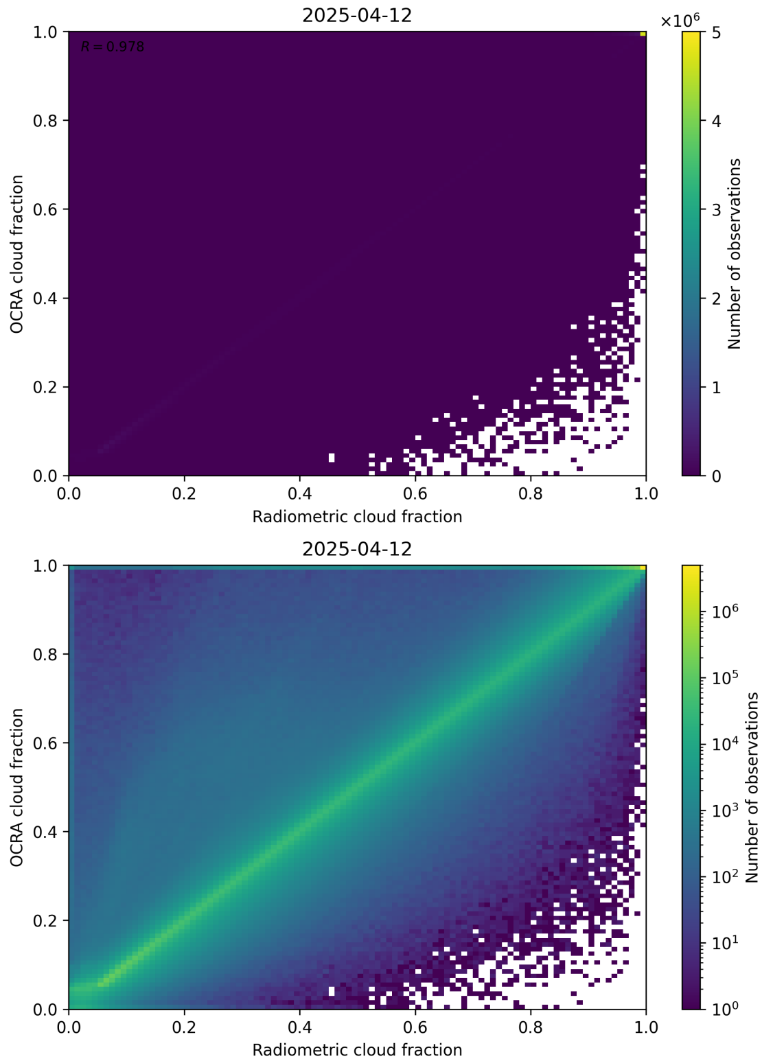
Figure 72: Scatter density plot of “Radiometric cloud fraction” against “OCRA cloud fraction” for 2025-04-11 to 2025-04-13.
