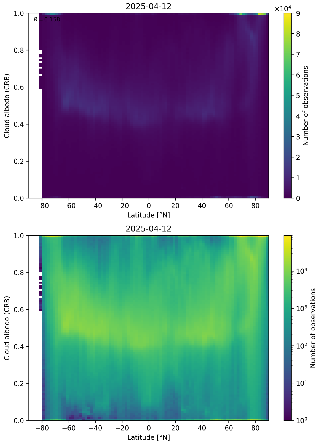
Figure 91: Scatter density plot of “Latitude” against “Cloud albedo (CRB)” for 2025-04-11 to 2025-04-13.
