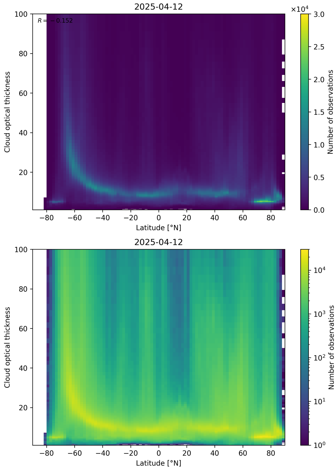
Figure 96: Scatter density plot of “Latitude” against “Cloud optical thickness” for 2025-04-11 to 2025-04-13.
