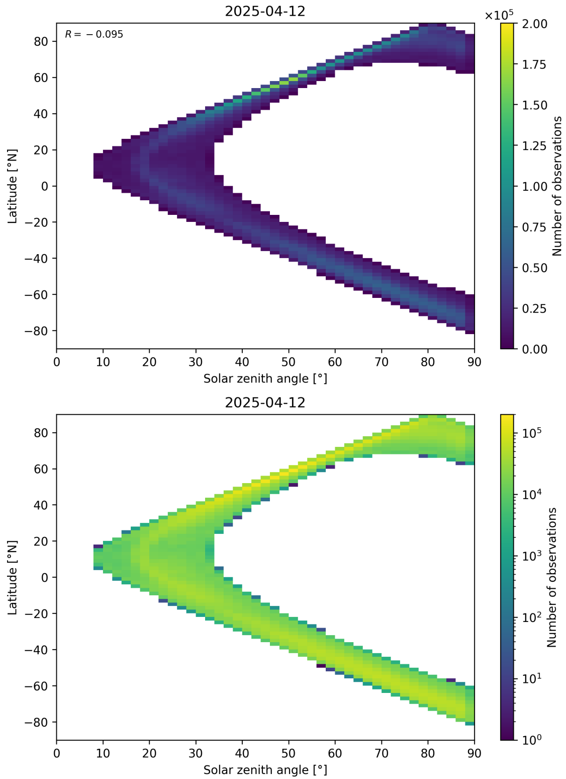
Figure 105: Scatter density plot of “Solar zenith angle” against “Latitude” for 2025-04-11 to 2025-04-13.
