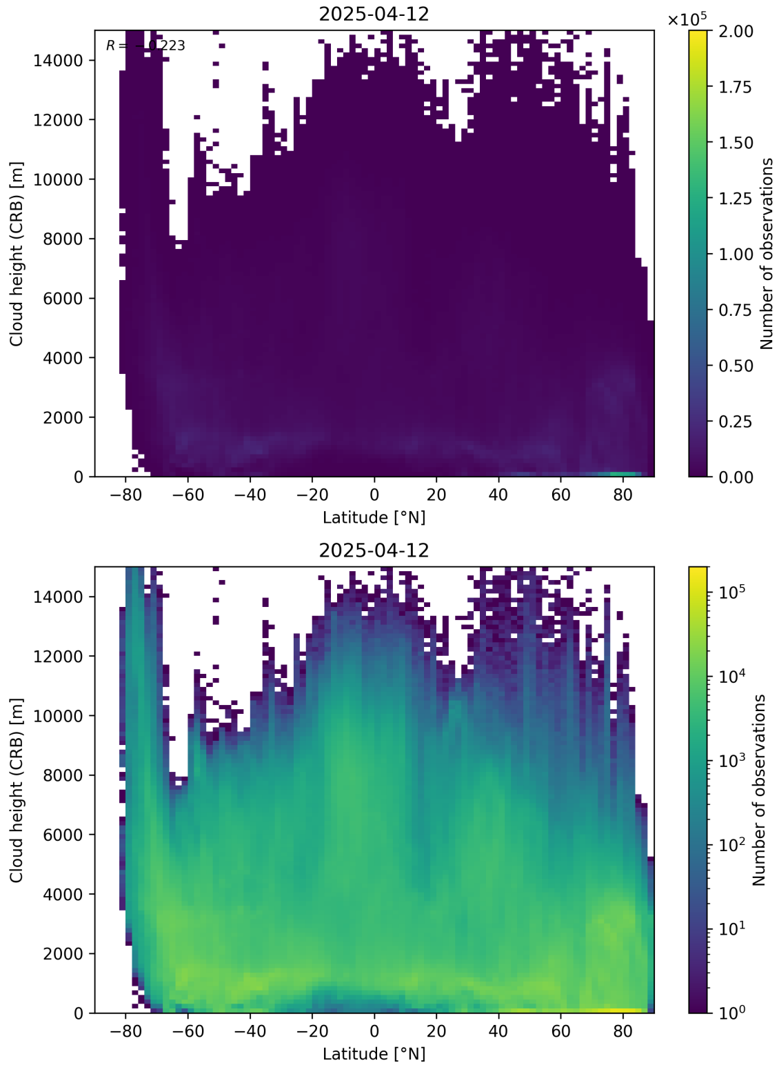
Figure 95: Scatter density plot of “Latitude” against “Cloud height (CRB)” for 2025-04-11 to 2025-04-13.
