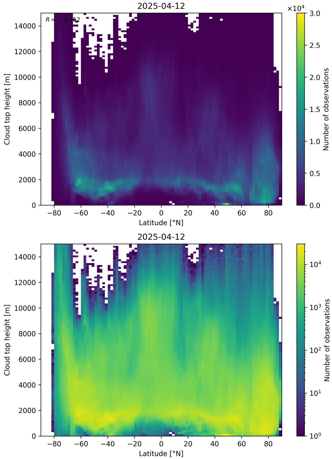
Figure 97: Scatter density plot of “Latitude” against “Cloud top height” for 2025-04-11 to 2025-04-13.
