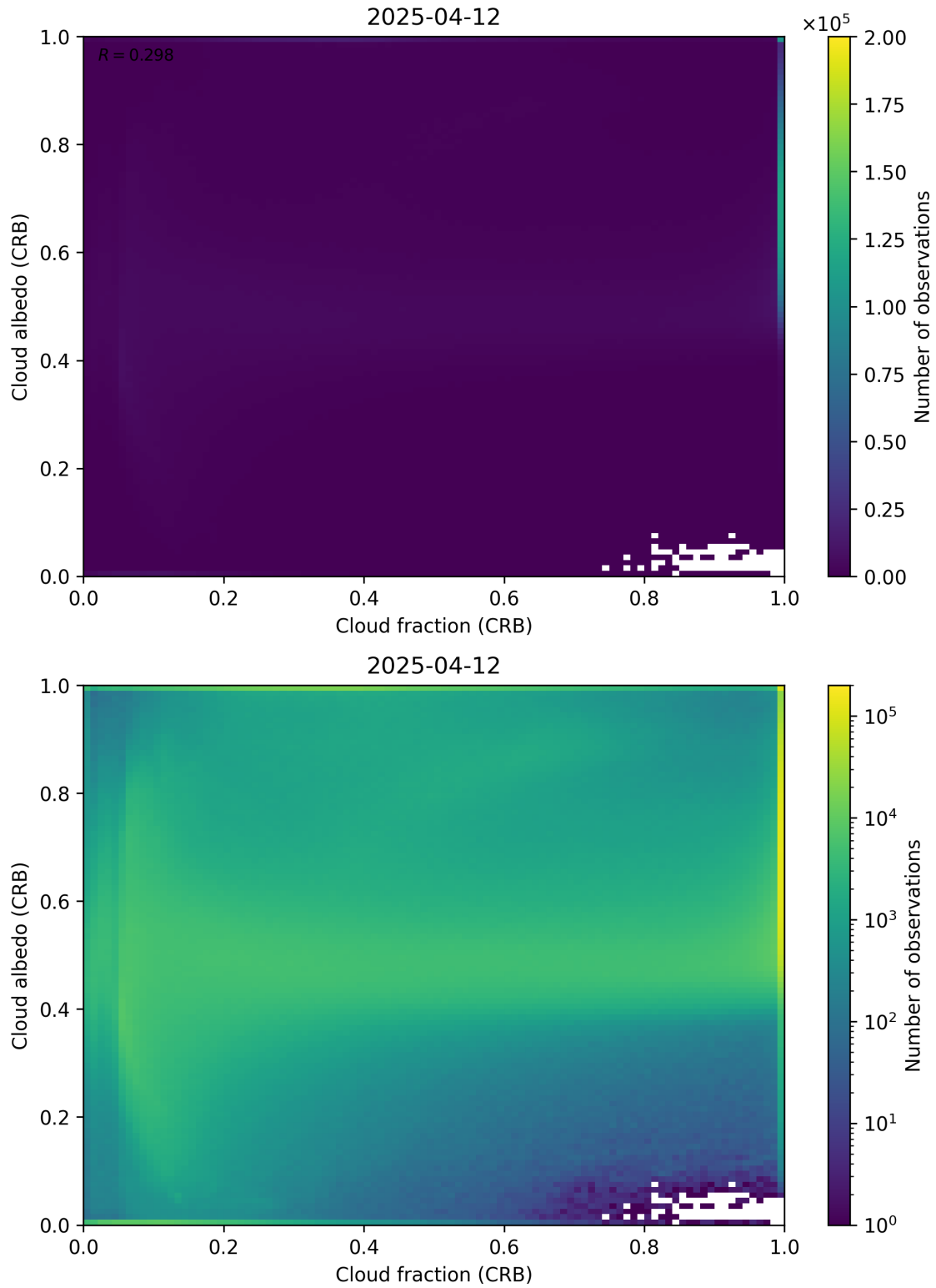
Figure 77: Scatter density plot of “Cloud fraction (CRB)” against “Cloud albedo (CRB)” for 2025-04-11 to 2025-04-13.
