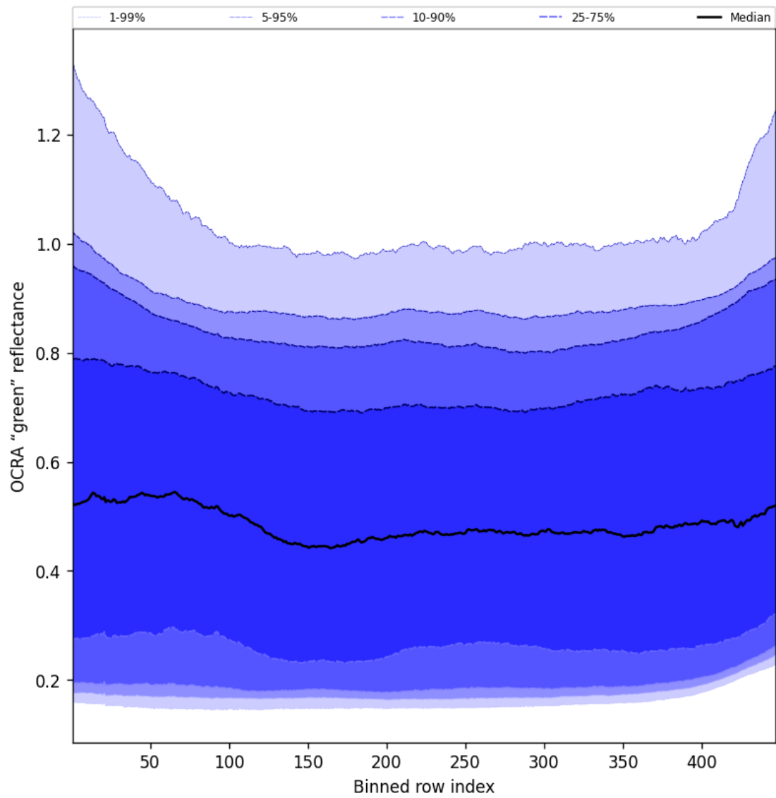
Figure 68: Along track statistics of “OCRA “green” reflectance” for 2025-04-11 to 2025-04-13
