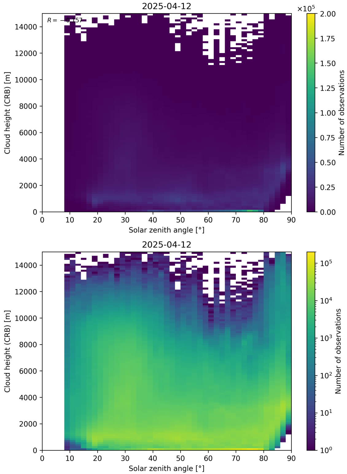
Figure 102: Scatter density plot of “Solar zenith angle” against “Cloud height (CRB)” for 2025-04-11 to 2025-04-13.
