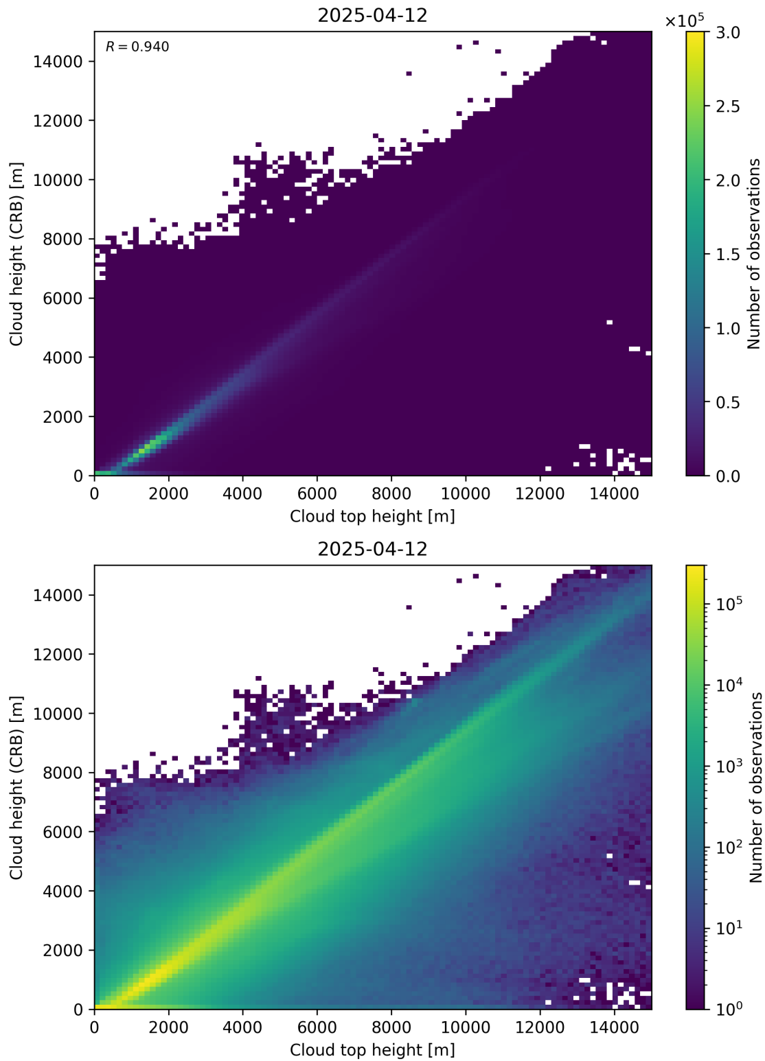
Figure 89: Scatter density plot of “Cloud top height” against “Cloud height (CRB)” for 2025-04-11 to 2025-04-13.
