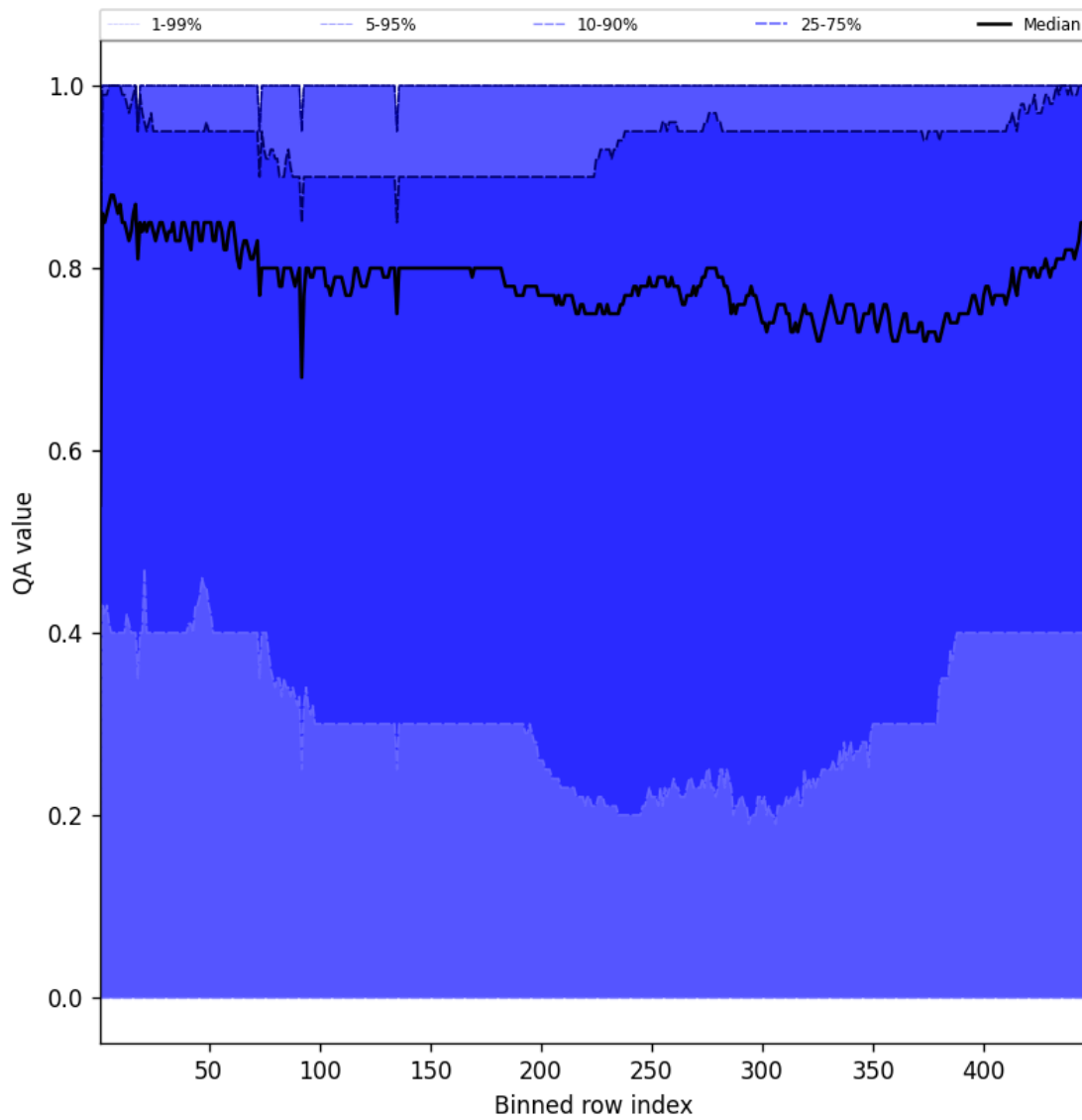
Figure 54: Along track statistics of “QA value” for 2025-04-11 to 2025-04-13
