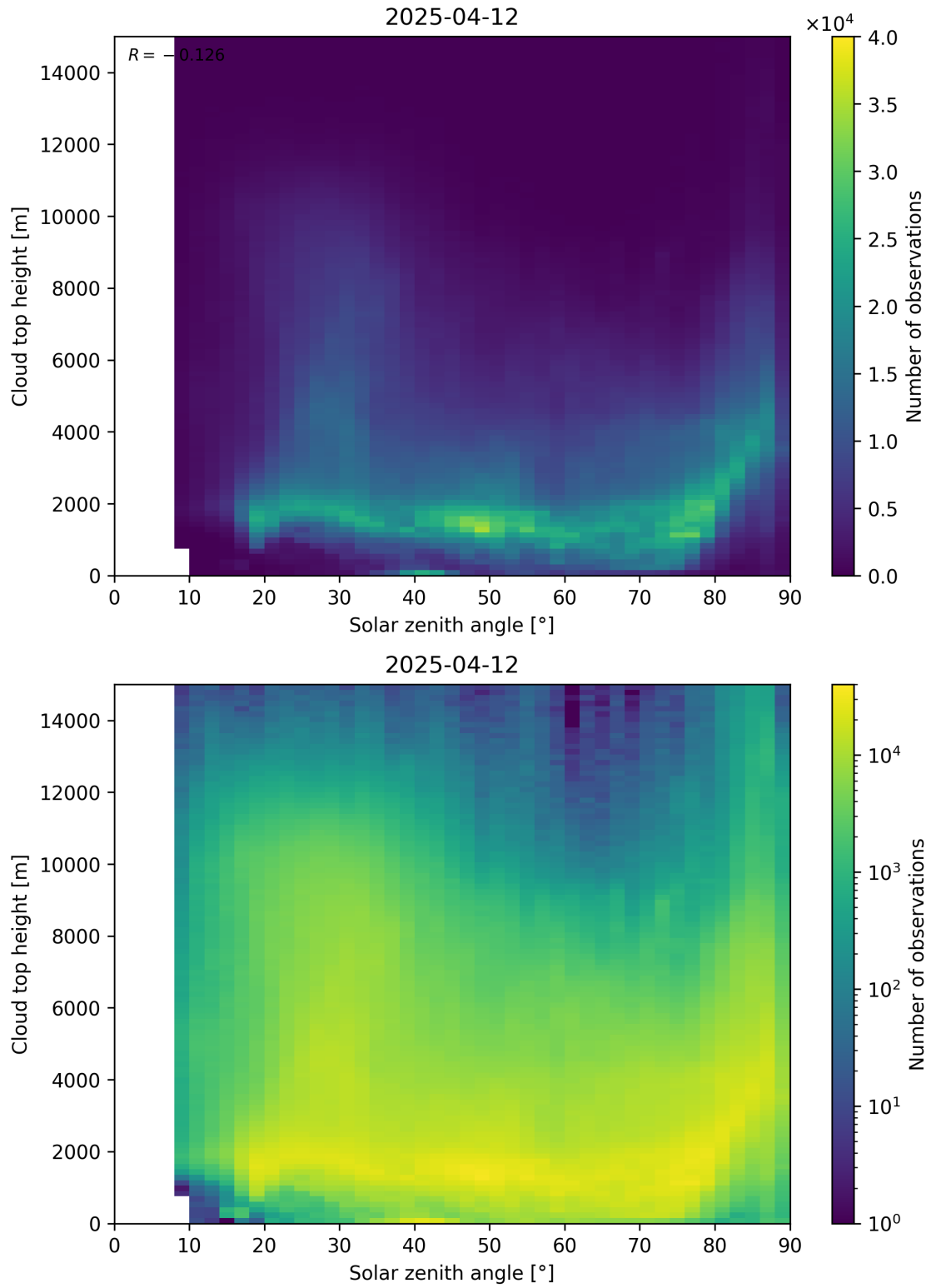
Figure 104: Scatter density plot of “Solar zenith angle” against “Cloud top height” for 2025-04-11 to 2025-04-13.
