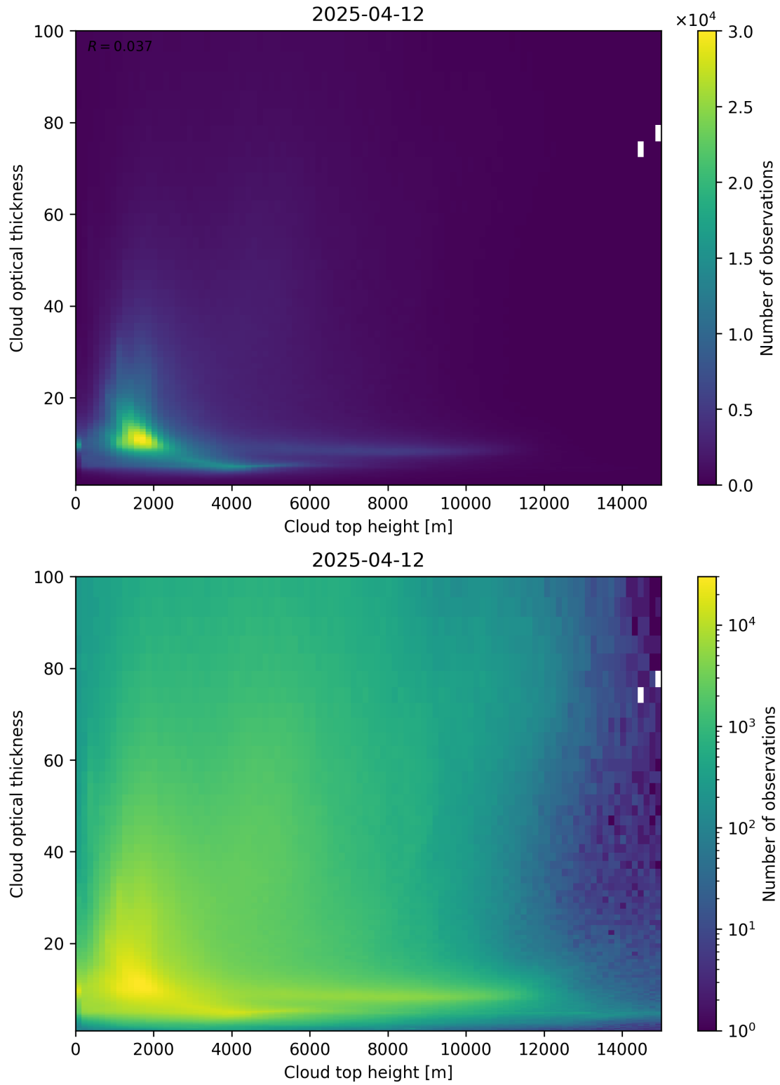
Figure 90: Scatter density plot of “Cloud top height” against “Cloud optical thickness” for 2025-04-11 to 2025-04-13.
