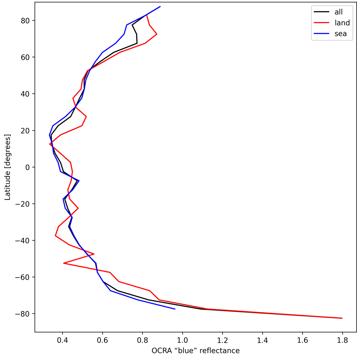
Figure 35: Zonal average of “OCRA “blue” reflectance” for 2025-04-11 to 2025-04-13.
