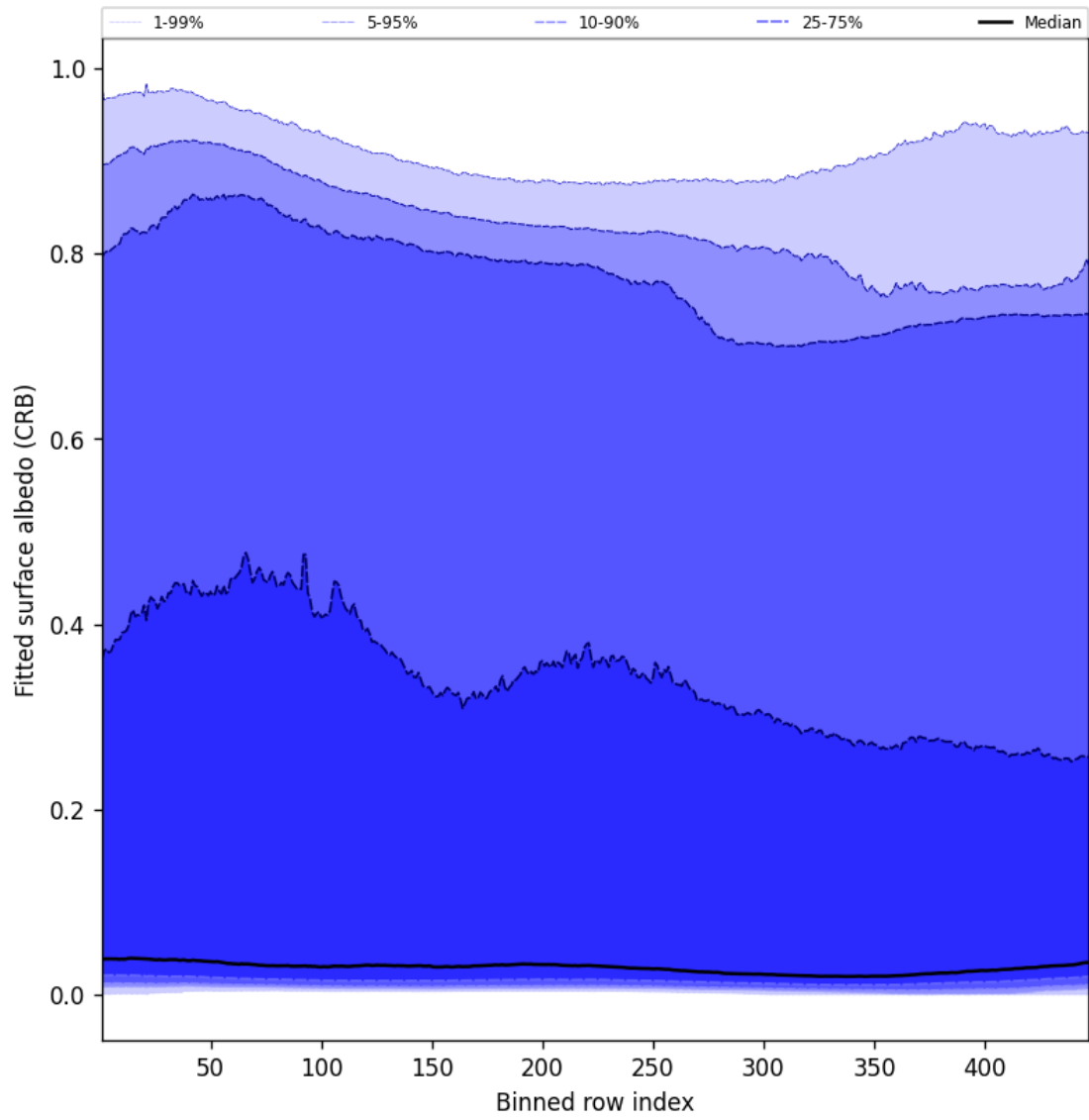
Figure 62: Along track statistics of “Fitted surface albedo (CRB)” for 2025-04-11 to 2025-04-13
