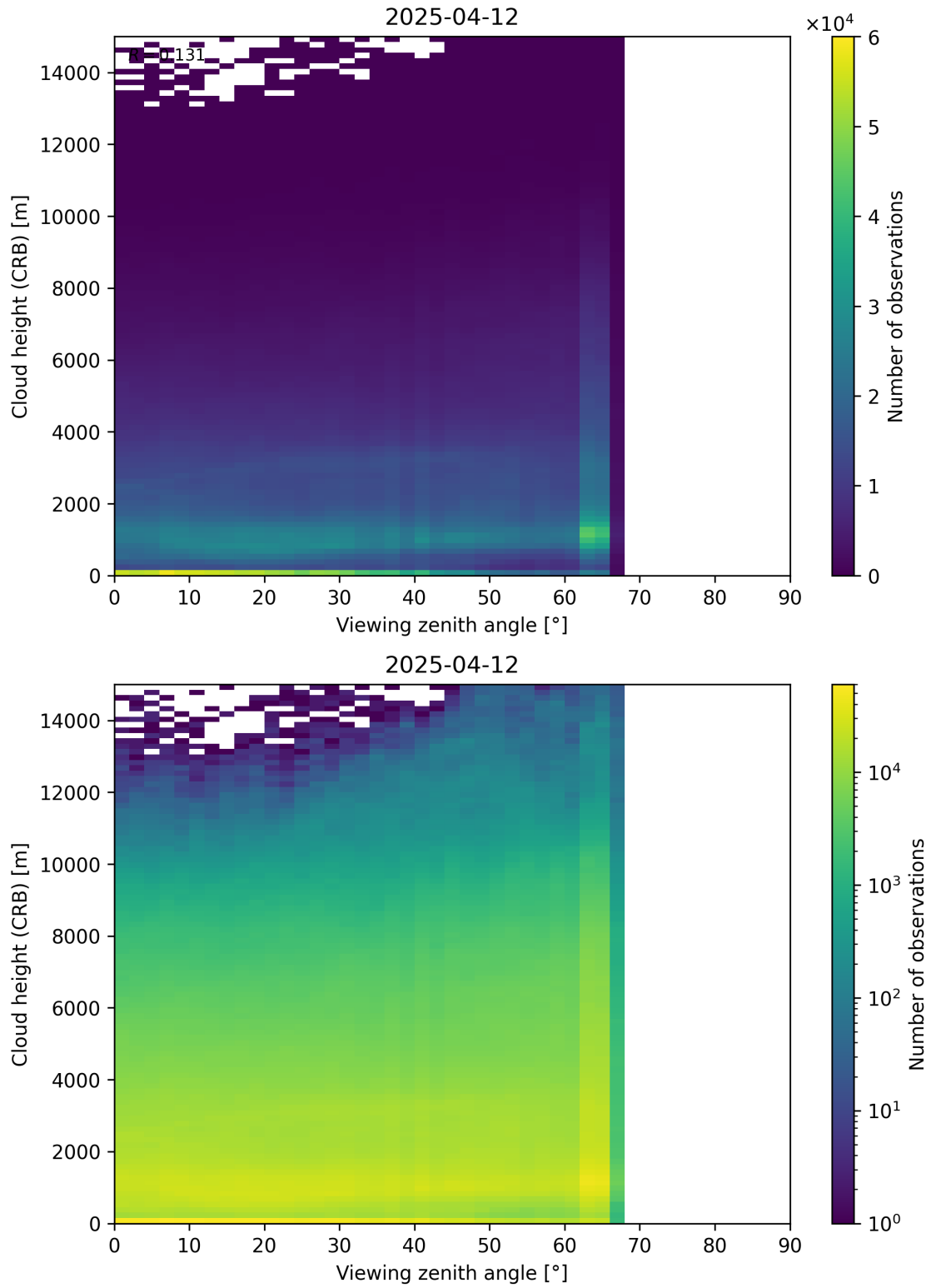
Figure 110: Scatter density plot of “Viewing zenith angle” against “Cloud height (CRB)” for 2025-04-11 to 2025-04-13.
