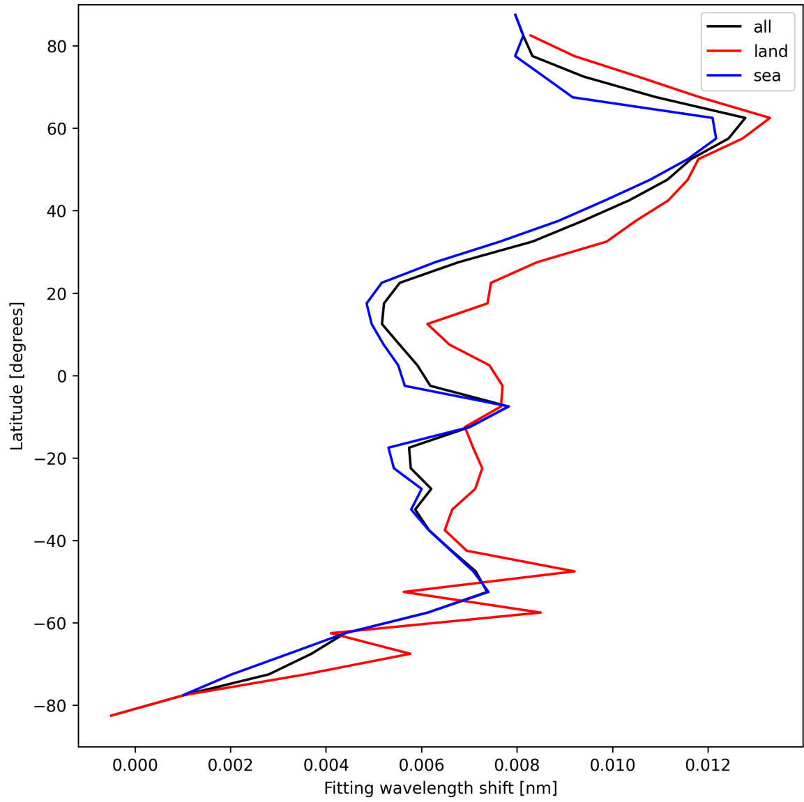
Figure 33: Zonal average of “Fitting wavelength shift” for 2025-04-11 to 2025-04-13.
