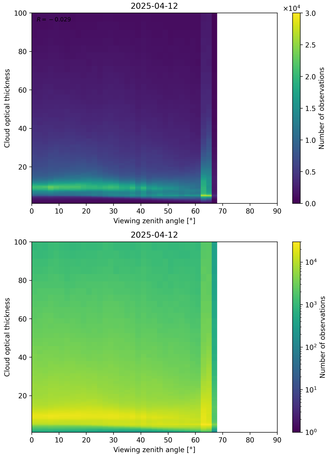
Figure 111: Scatter density plot of “Viewing zenith angle” against “Cloud optical thickness” for 2025-04-11 to 2025-04-13.
