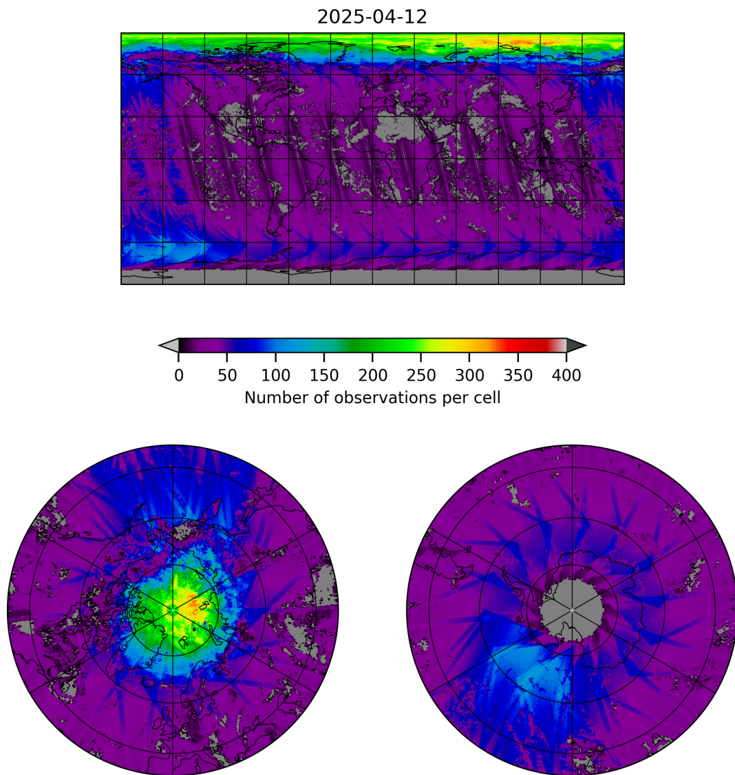
Figure 21: Map of the number of observations for 2025-04-11 to 2025-04-13
