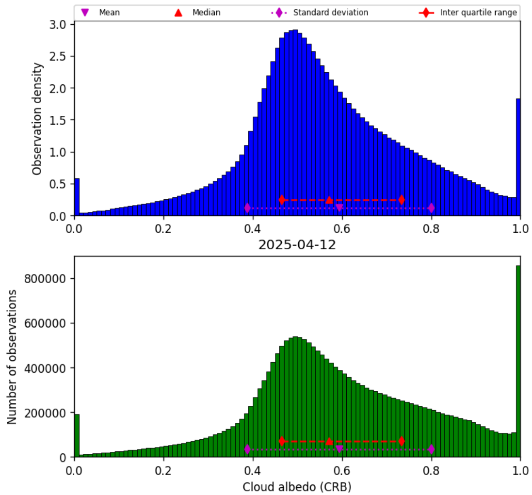
Figure 44: Histogram of “Cloud albedo (CRB)” for 2025-04-11 to 2025-04-13
