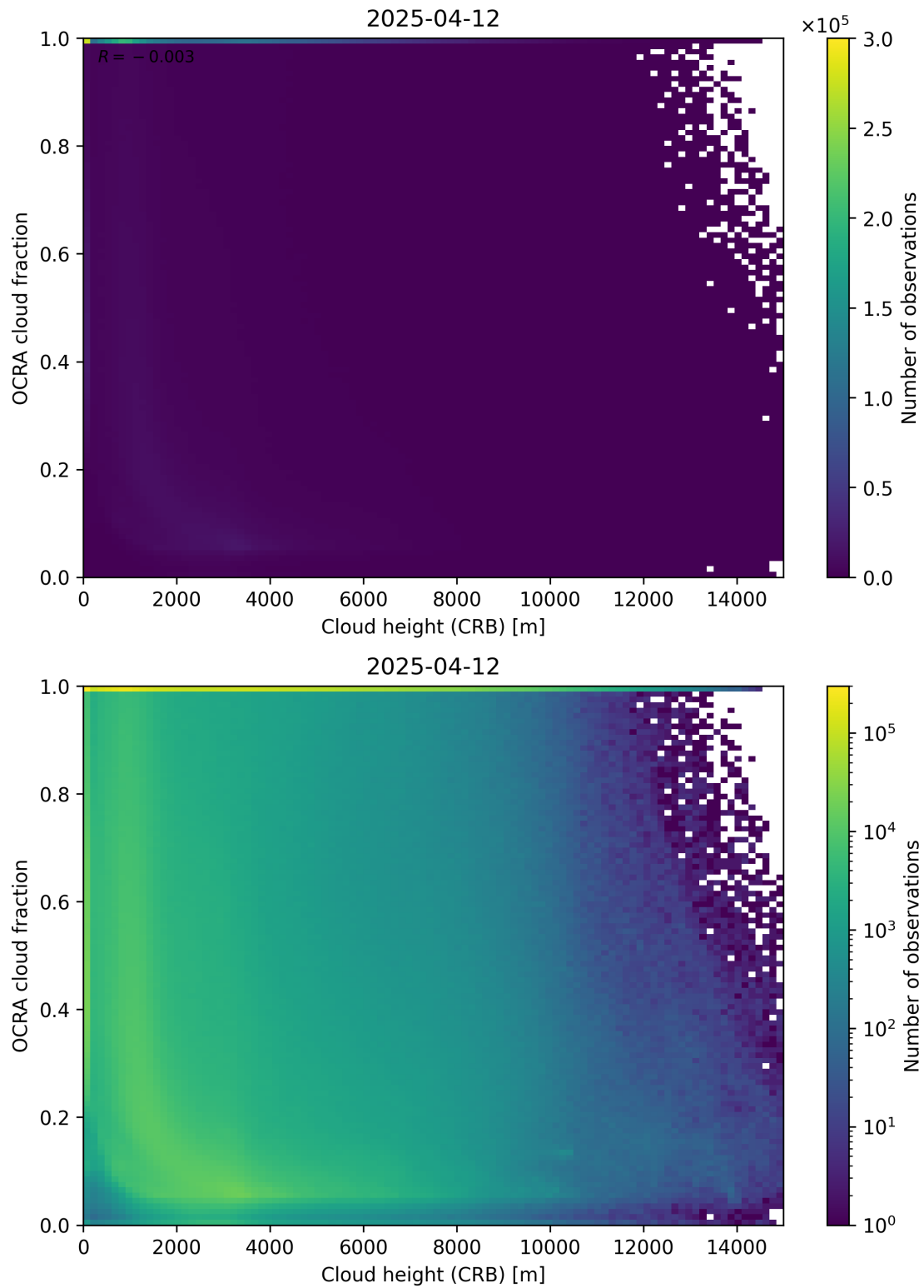
Figure 81: Scatter density plot of “Cloud height (CRB)” against “OCRA cloud fraction” for 2025-04-11 to 2025-04-13.
