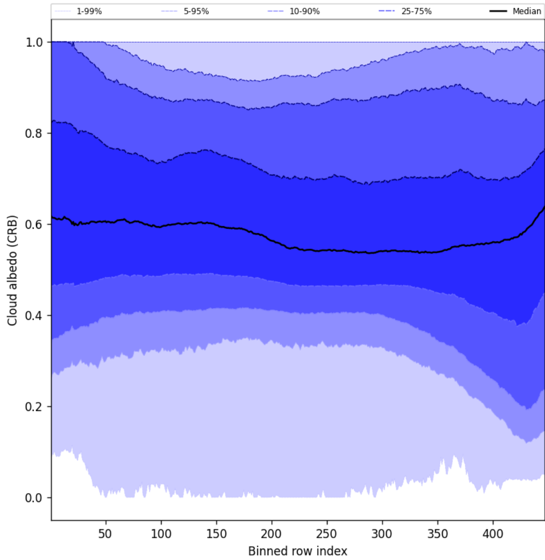
Figure 60: Along track statistics of “Cloud albedo (CRB)” for 2025-04-11 to 2025-04-13
