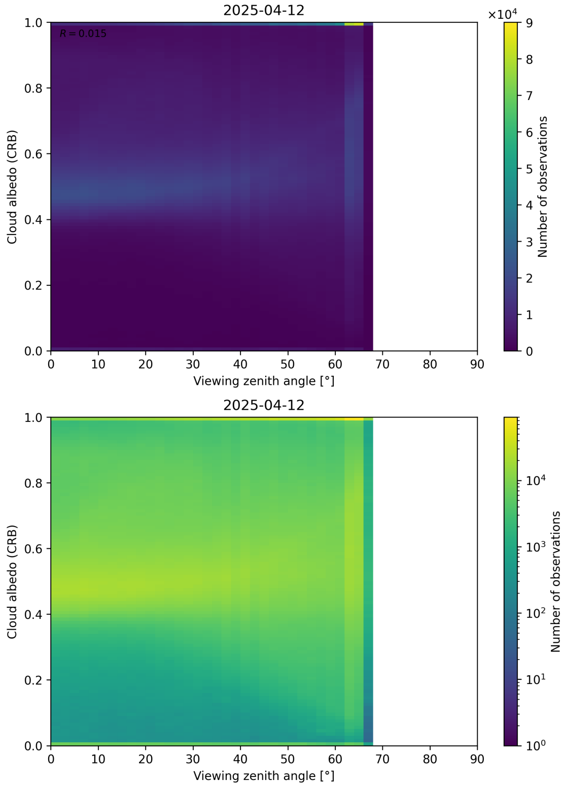
Figure 106: Scatter density plot of “Viewing zenith angle” against “Cloud albedo (CRB)” for 2025-04-11 to 2025-04-13.
