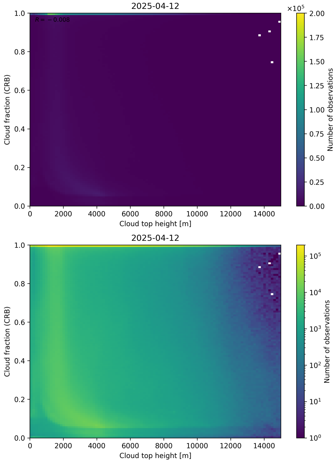
Figure 88: Scatter density plot of “Cloud top height” against “Cloud fraction (CRB)” for 2025-04-11 to 2025-04-13.
