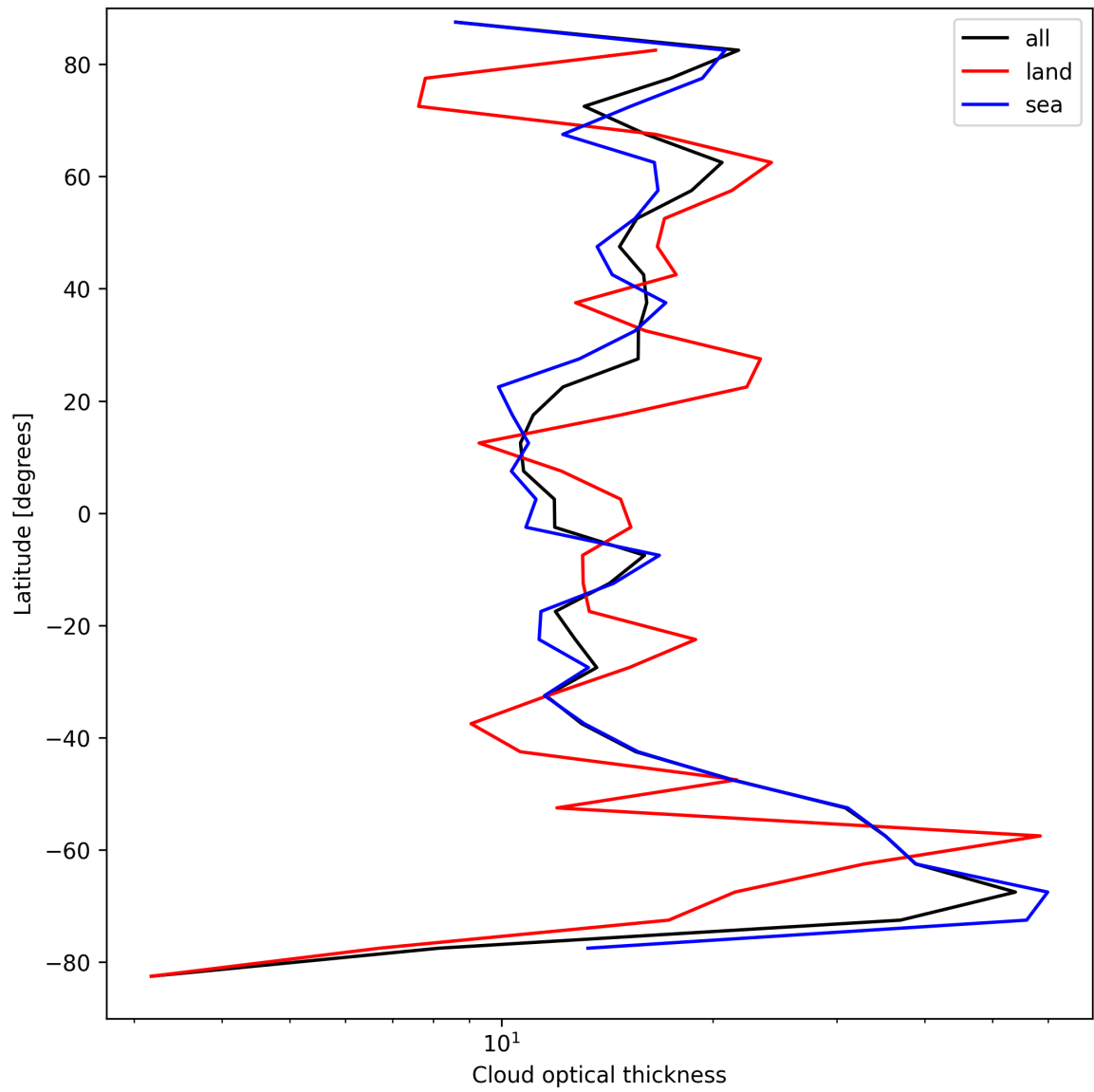
Figure 25: Zonal average of “Cloud optical thickness” for 2025-04-11 to 2025-04-13.
