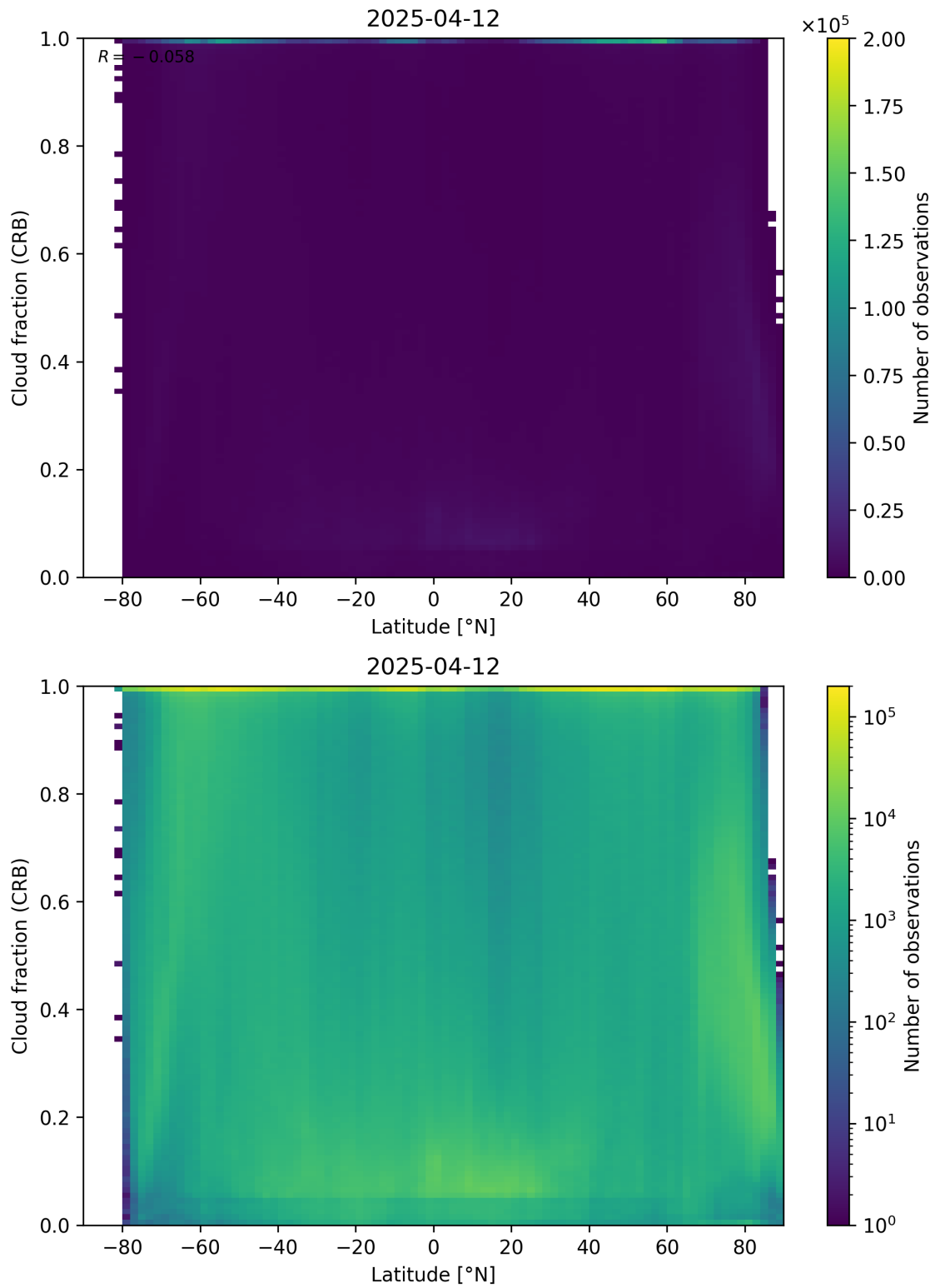
Figure 94: Scatter density plot of “Latitude” against “Cloud fraction (CRB)” for 2025-04-11 to 2025-04-13.
