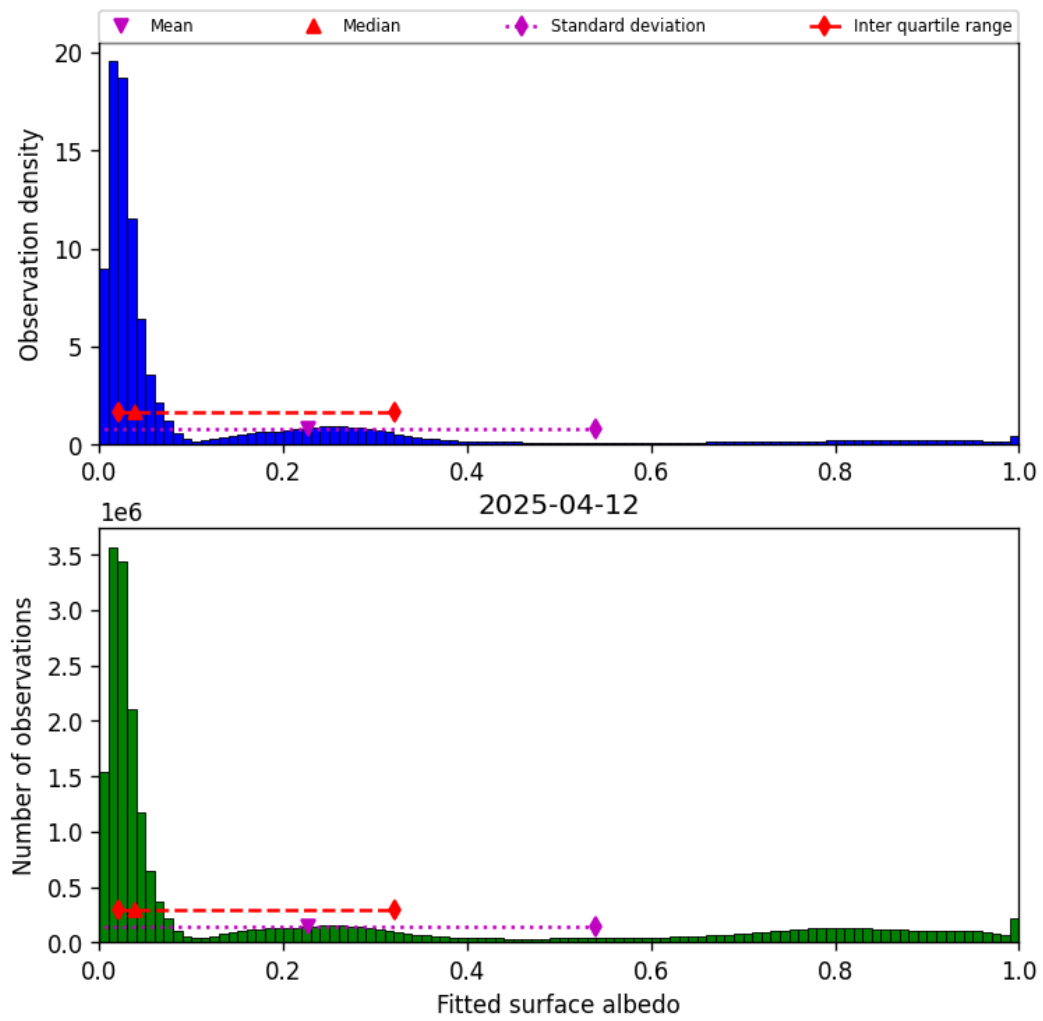
Figure 45: Histogram of “Fitted surface albedo” for 2025-04-11 to 2025-04-13
