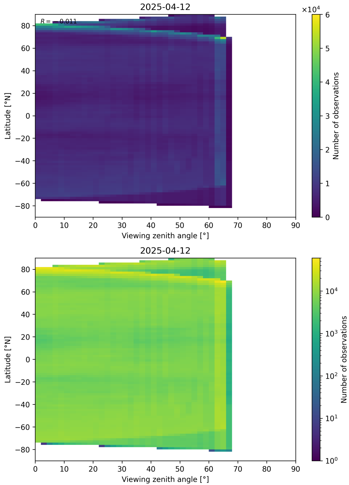
Figure 113: Scatter density plot of “Viewing zenith angle” against “Latitude” for 2025-04-11 to 2025-04-13.
