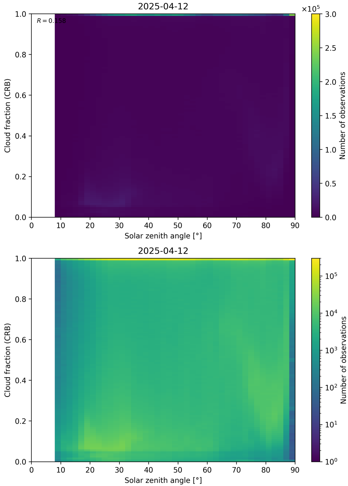
Figure 101: Scatter density plot of “Solar zenith angle” against “Cloud fraction (CRB)” for 2025-04-11 to 2025-04-13.
