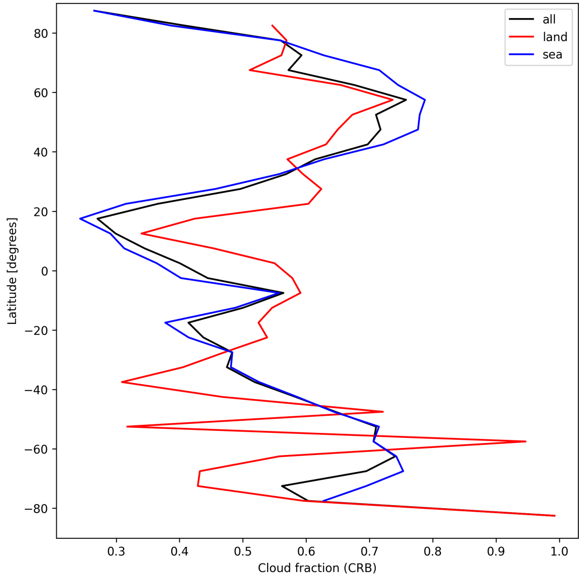
Figure 26: Zonal average of “Cloud fraction (CRB)” for 2025-04-11 to 2025-04-13.
