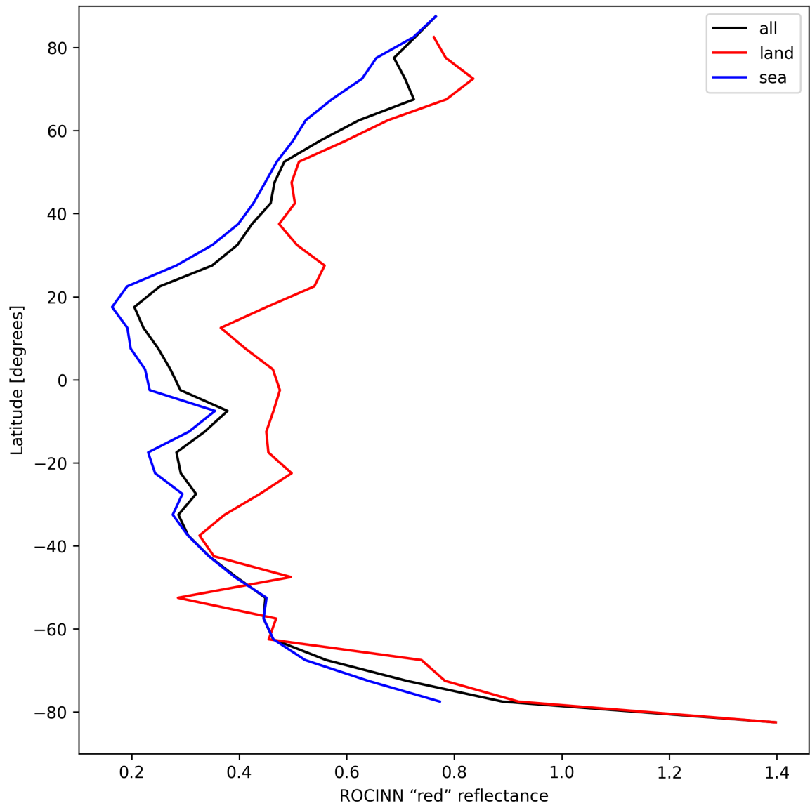
Figure 37: Zonal average of “ROCINN “red” reflectance” for 2025-04-11 to 2025-04-13.
