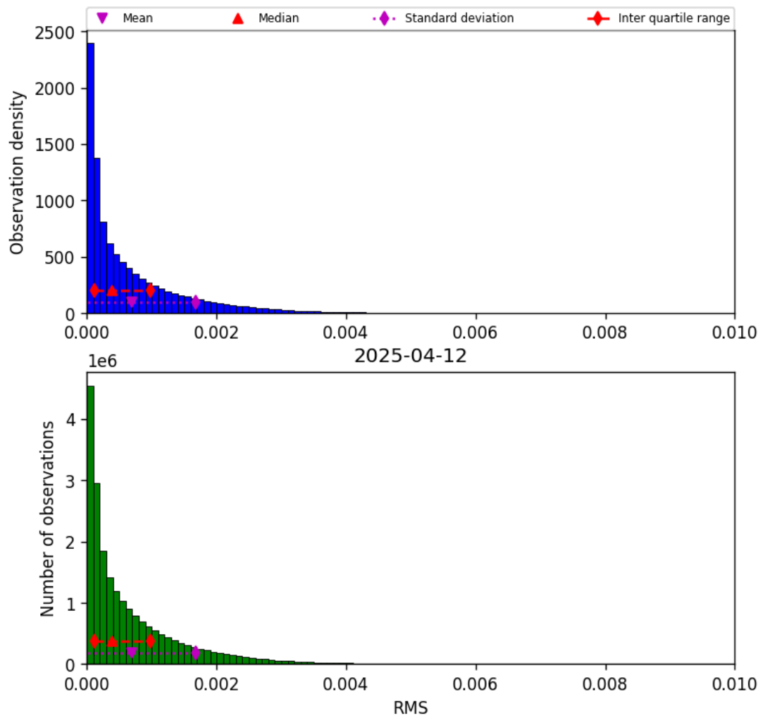
Figure 47: Histogram of “RMS” for 2025-04-11 to 2025-04-13
