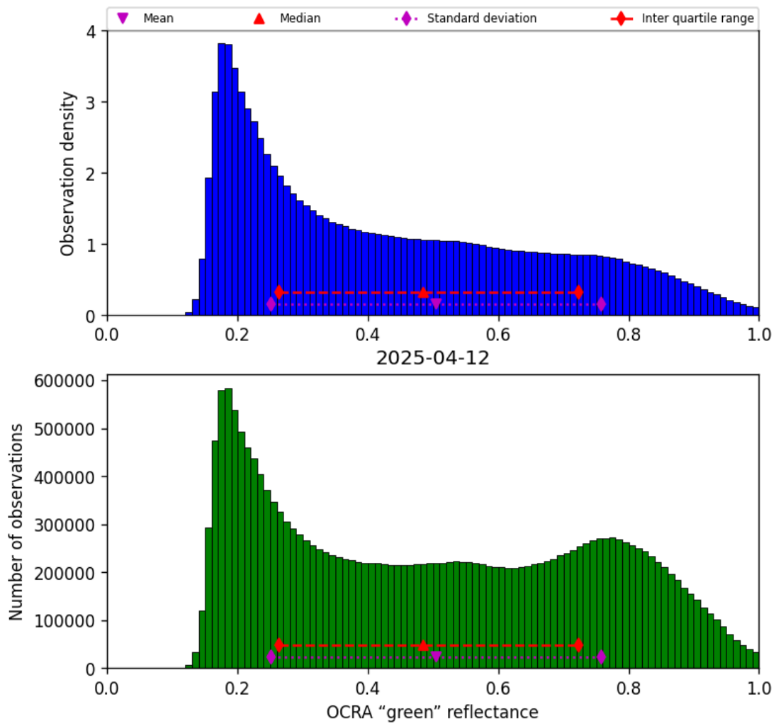
Figure 52: Histogram of “OCRA “green” reflectance” for 2025-04-11 to 2025-04-13
