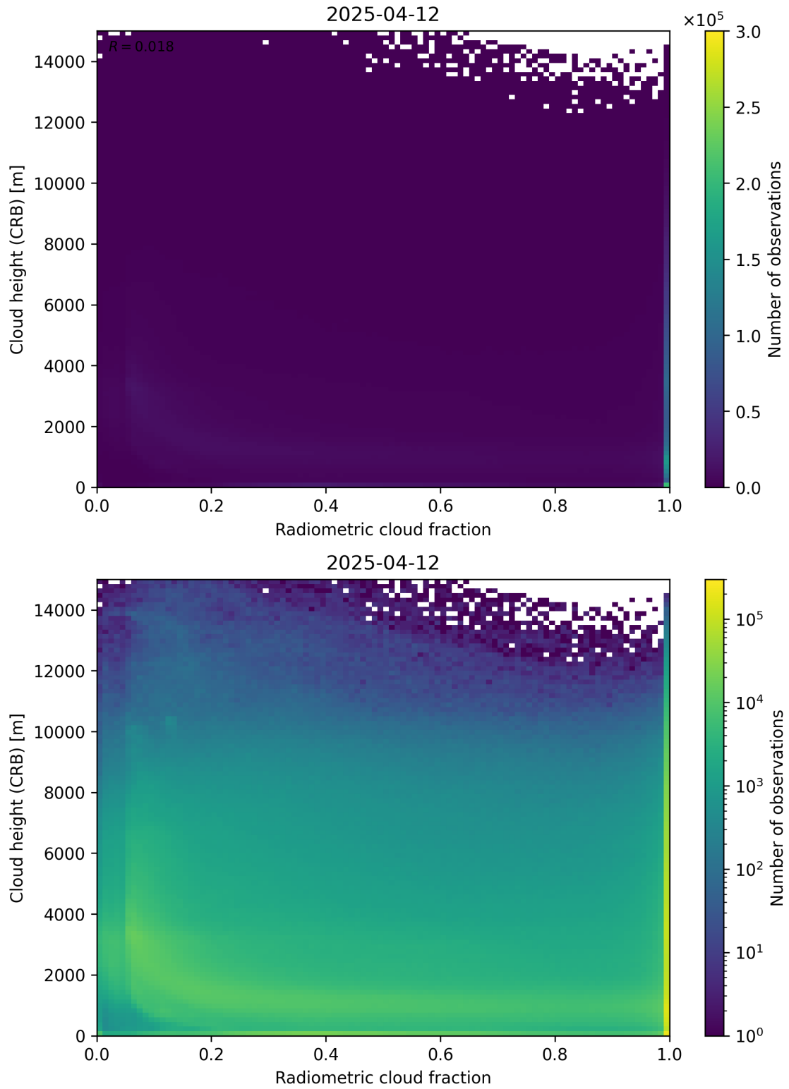
Figure 74: Scatter density plot of “Radiometric cloud fraction” against “Cloud height (CRB)” for 2025-04-11 to 2025-04-13.
