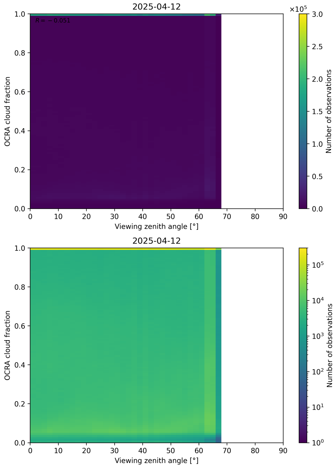
Figure 108: Scatter density plot of “Viewing zenith angle” against “OCRA cloud fraction” for 2025-04-11 to 2025-04-13.
