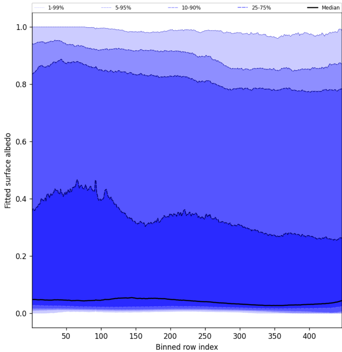
Figure 61: Along track statistics of “Fitted surface albedo” for 2025-04-11 to 2025-04-13
