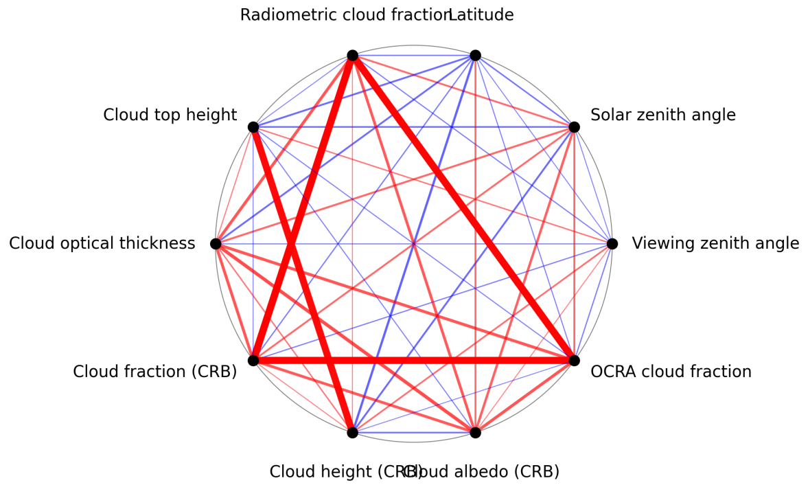
Figure 1: Map of correlation graph for 2025-04-11 to 2025-04-13.
