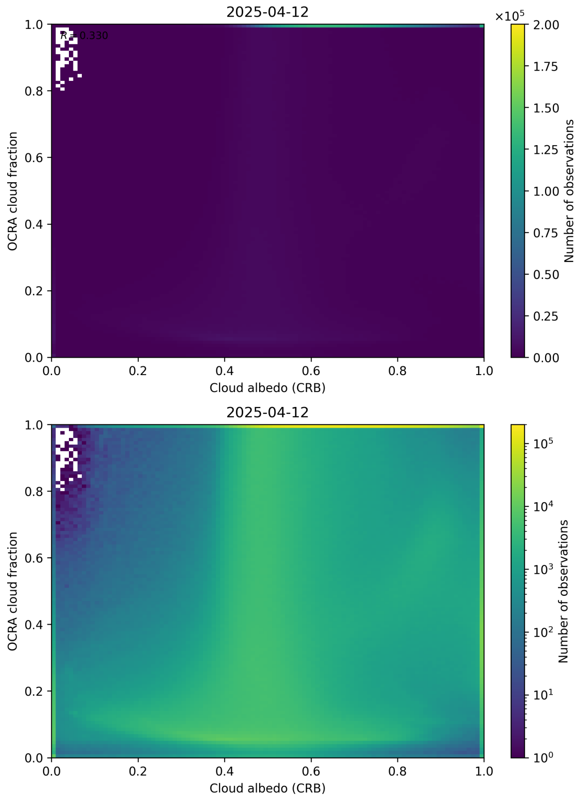
Figure 70: Scatter density plot of “Cloud albedo (CRB)” against “OCRA cloud fraction” for 2025-04-11 to 2025-04-13.
