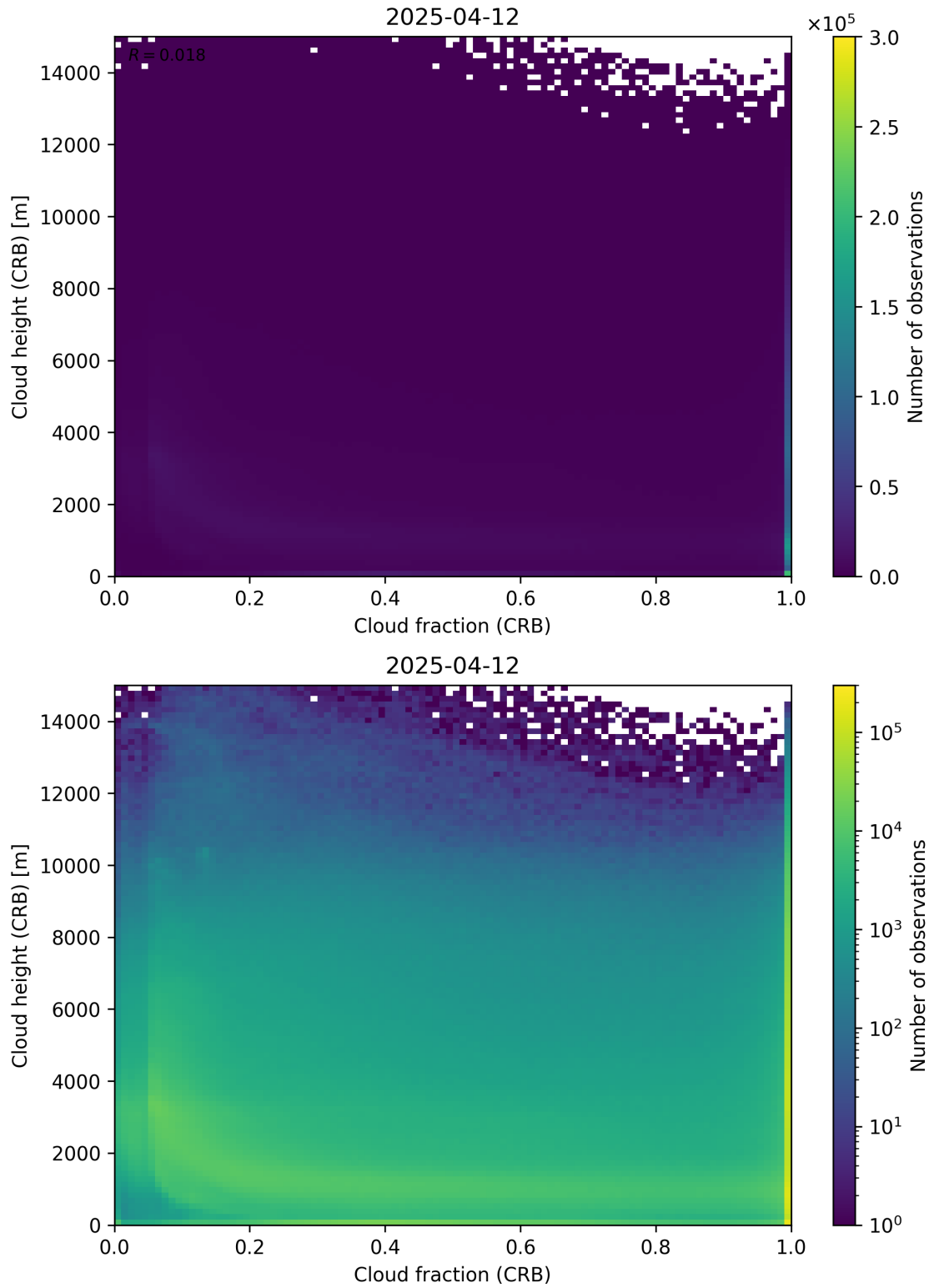
Figure 79: Scatter density plot of “Cloud fraction (CRB)” against “Cloud height (CRB)” for 2025-04-11 to 2025-04-13.
