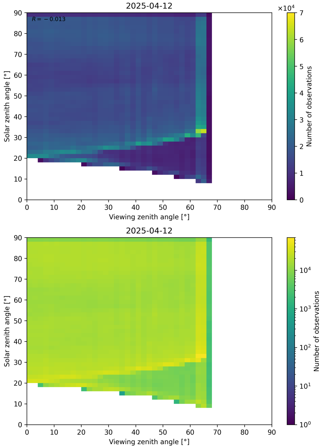
Figure 114: Scatter density plot of “Viewing zenith angle” against “Solar zenith angle” for 2025-04-11 to 2025-04-13.
