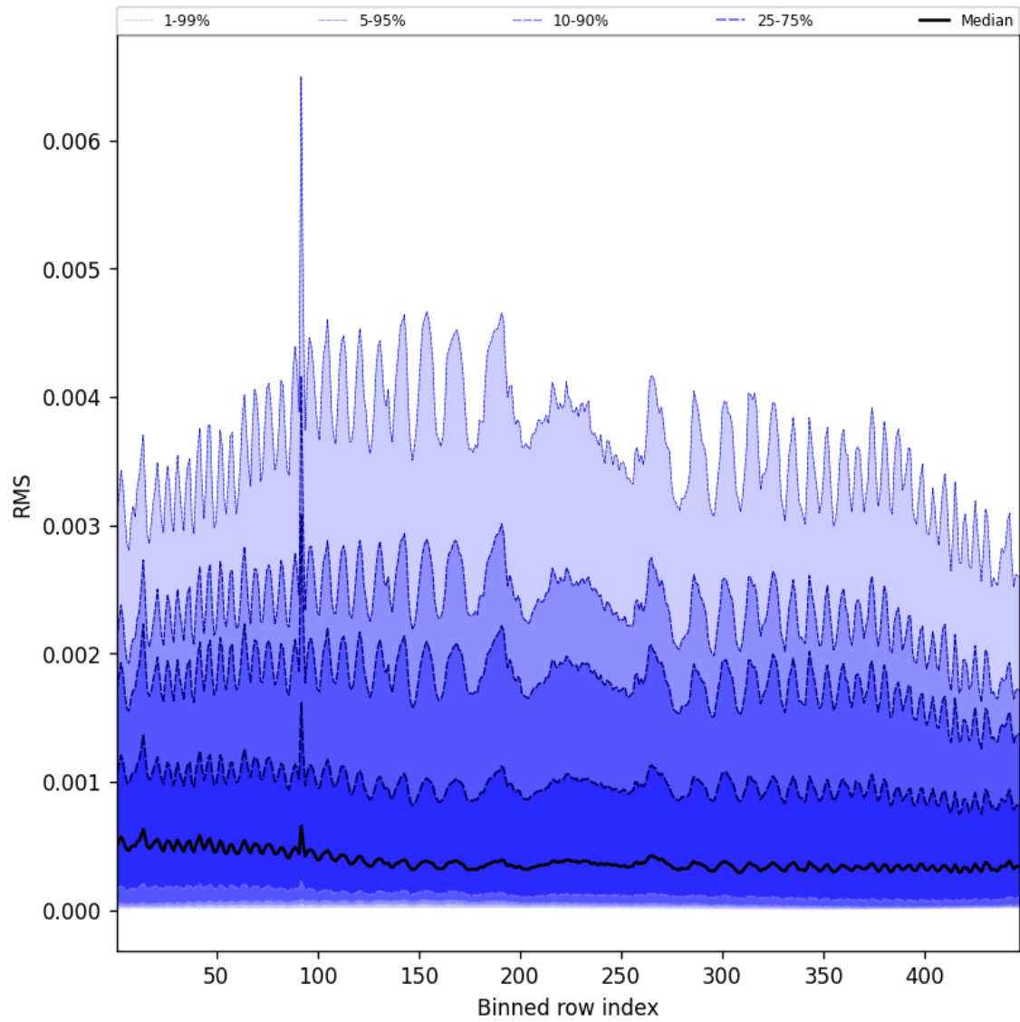
Figure 63: Along track statistics of “RMS” for 2025-04-11 to 2025-04-13
