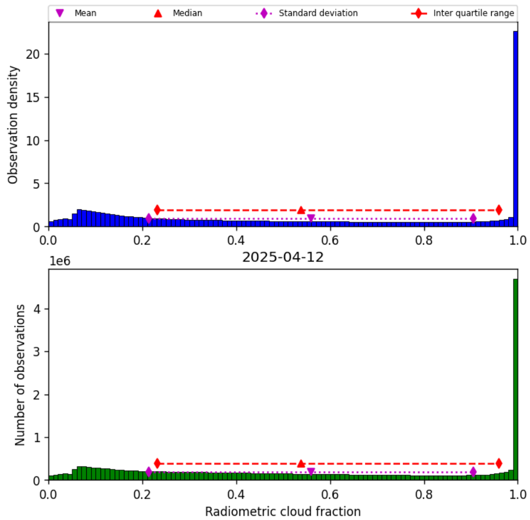
Figure 39: Histogram of “Radiometric cloud fraction” for 2025-04-11 to 2025-04-13
