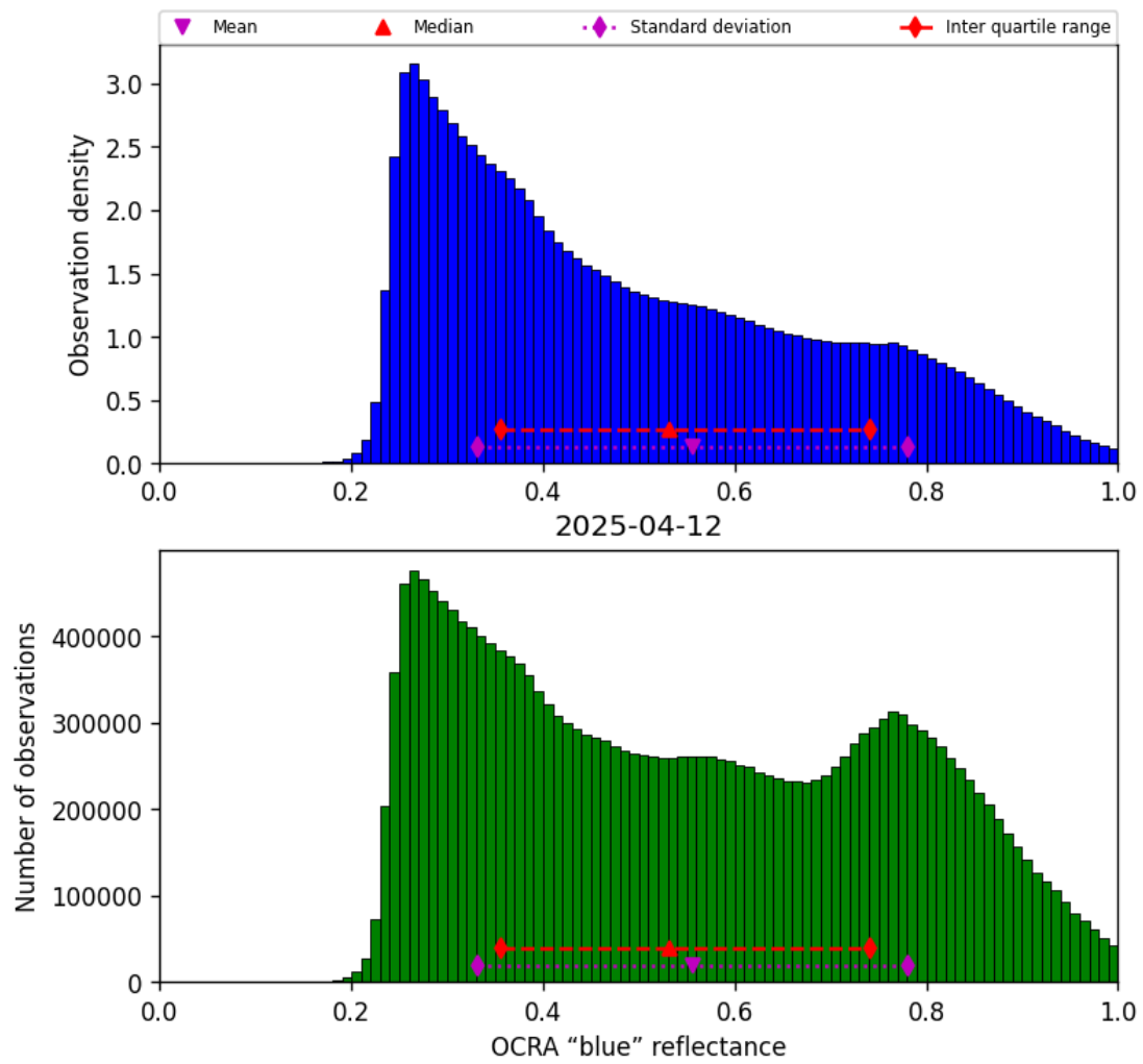
Figure 51: Histogram of “OCRA “blue” reflectance” for 2025-04-11 to 2025-04-13
