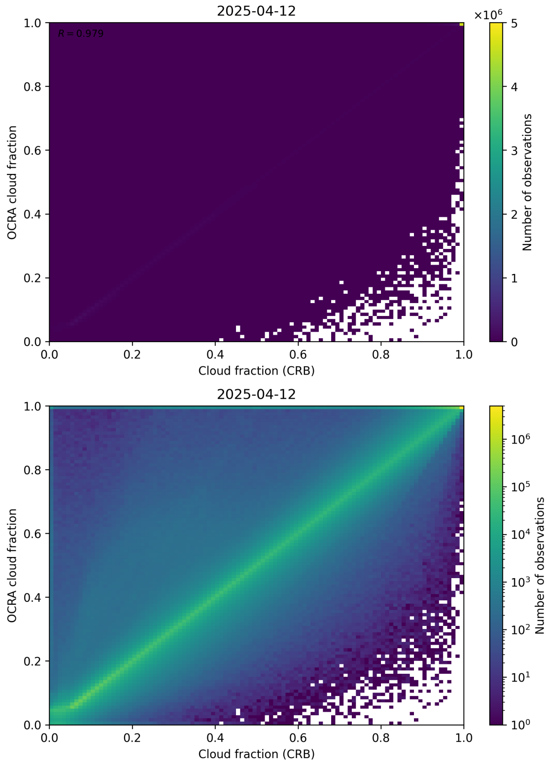
Figure 78: Scatter density plot of “Cloud fraction (CRB)” against “OCRA cloud fraction” for 2025-04-11 to 2025-04-13.
