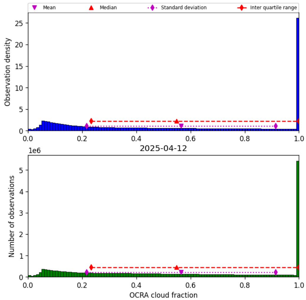
Figure 50: Histogram of “OCRA cloud fraction” for 2025-04-11 to 2025-04-13
