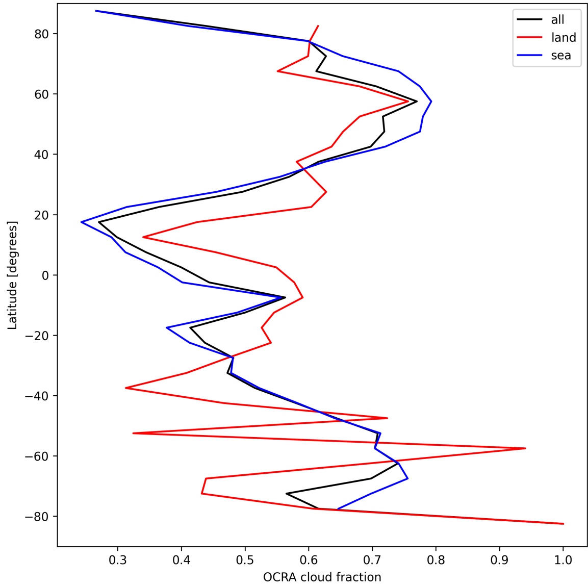
Figure 34: Zonal average of “OCRA cloud fraction” for 2025-04-11 to 2025-04-13.
