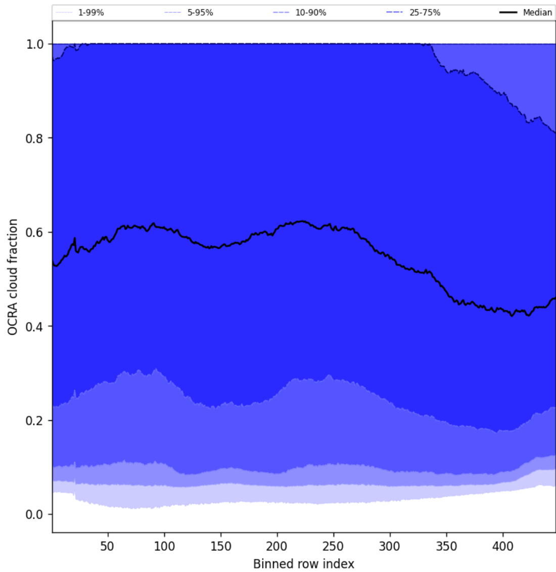
Figure 66: Along track statistics of “OCRA cloud fraction” for 2025-04-11 to 2025-04-13
