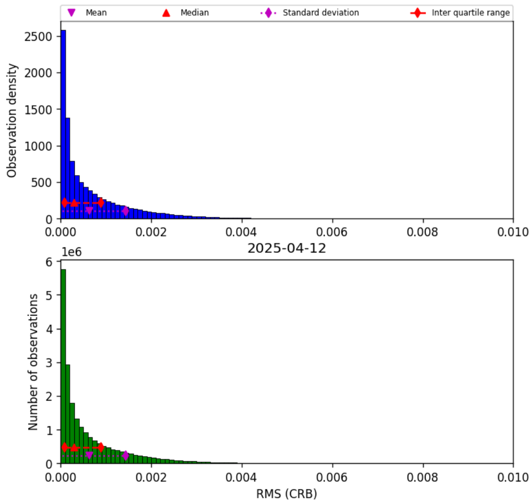
Figure 48: Histogram of “RMS (CRB)” for 2025-04-11 to 2025-04-13
