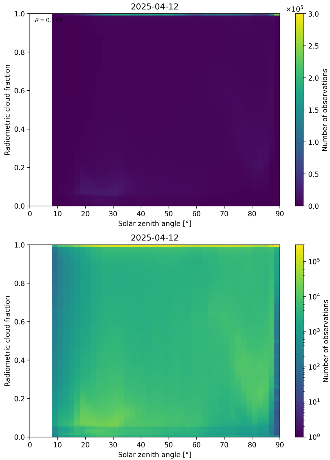
Figure 99: Scatter density plot of “Solar zenith angle” against “Radiometric cloud fraction” for 2025-04-11 to 2025-04-13.
