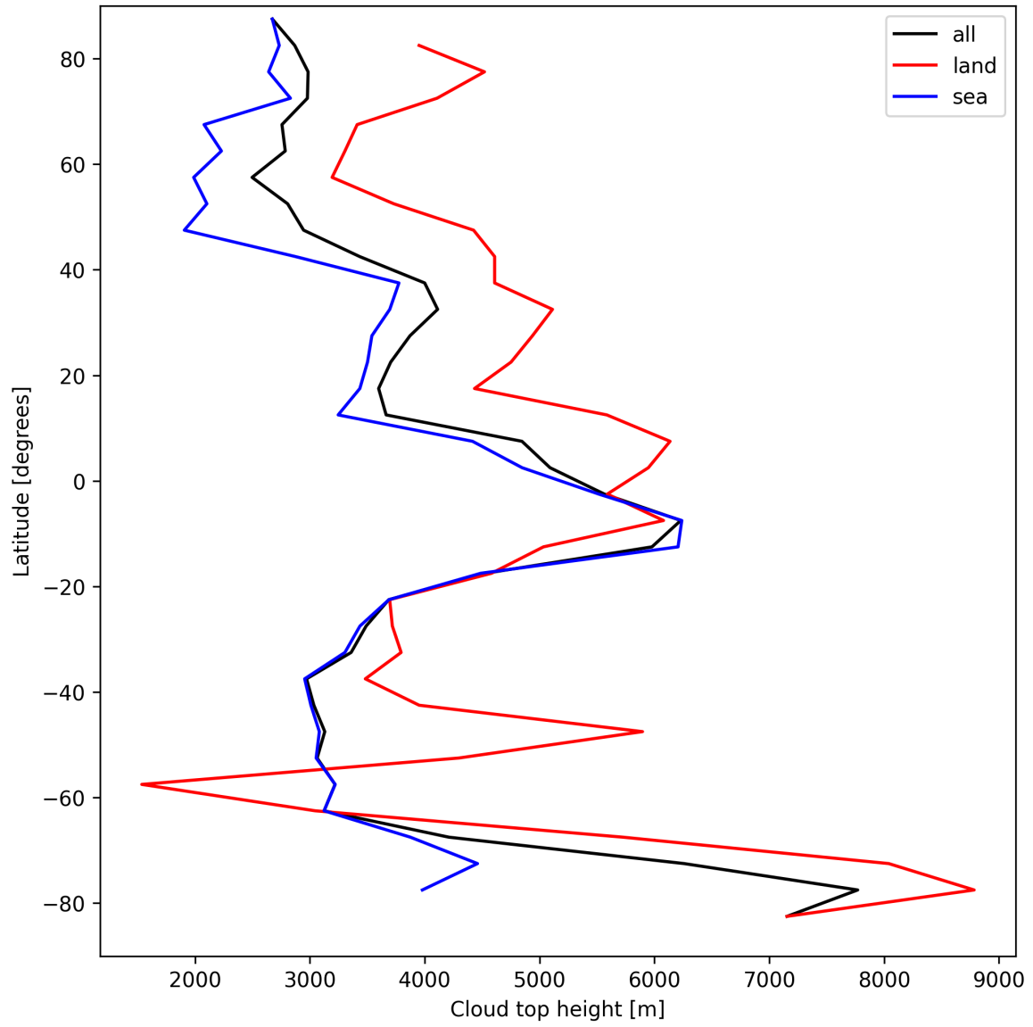
Figure 24: Zonal average of “Cloud top height” for 2025-04-11 to 2025-04-13.
