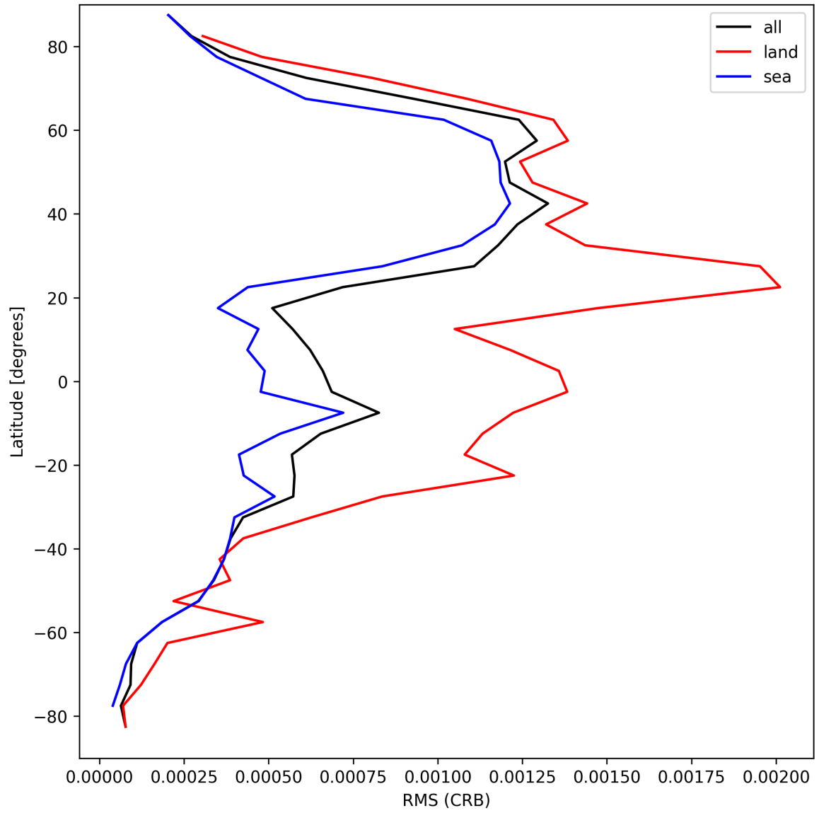
Figure 32: Zonal average of “RMS (CRB)” for 2025-04-11 to 2025-04-13.
