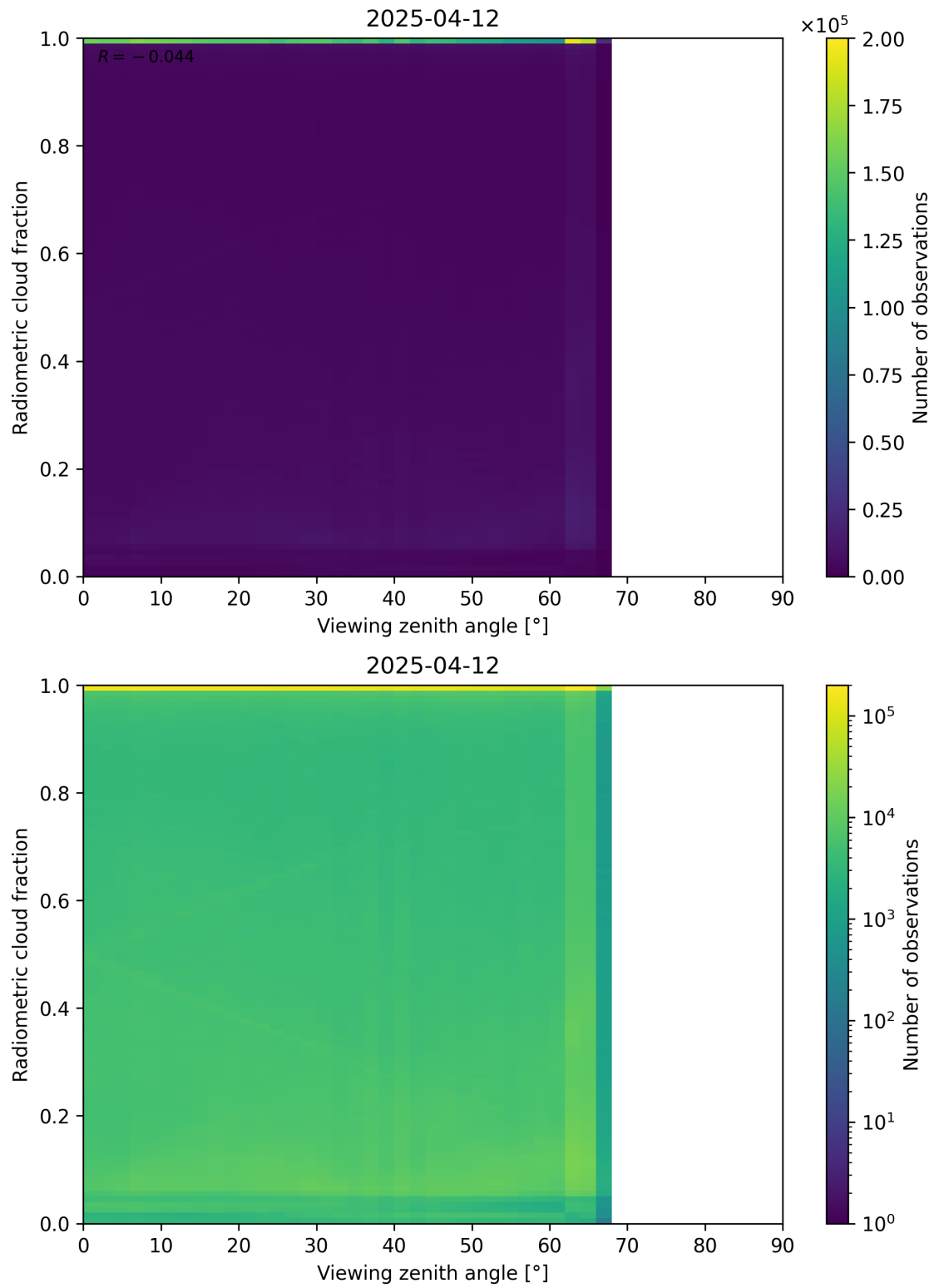
Figure 107: Scatter density plot of “Viewing zenith angle” against “Radiometric cloud fraction” for 2025-04-11 to 2025-04-13.
