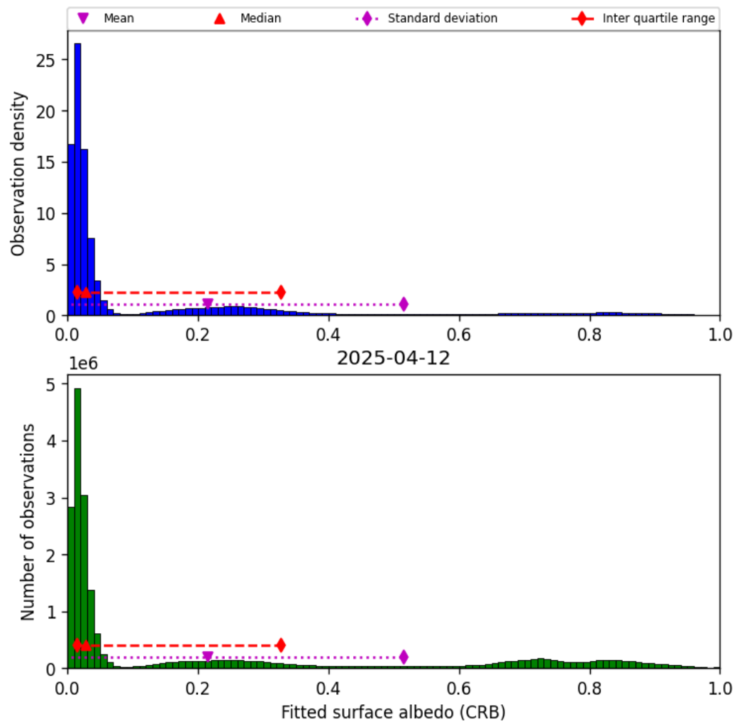
Figure 46: Histogram of “Fitted surface albedo (CRB)” for 2025-04-11 to 2025-04-13
