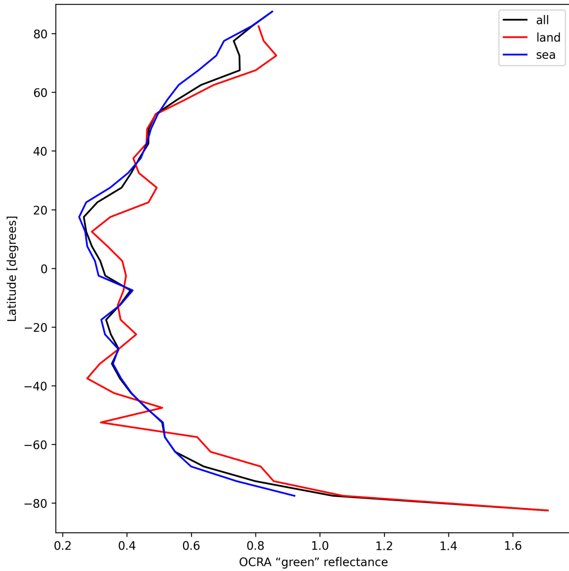
Figure 36: Zonal average of “OCRA “green” reflectance” for 2025-04-11 to 2025-04-13.
