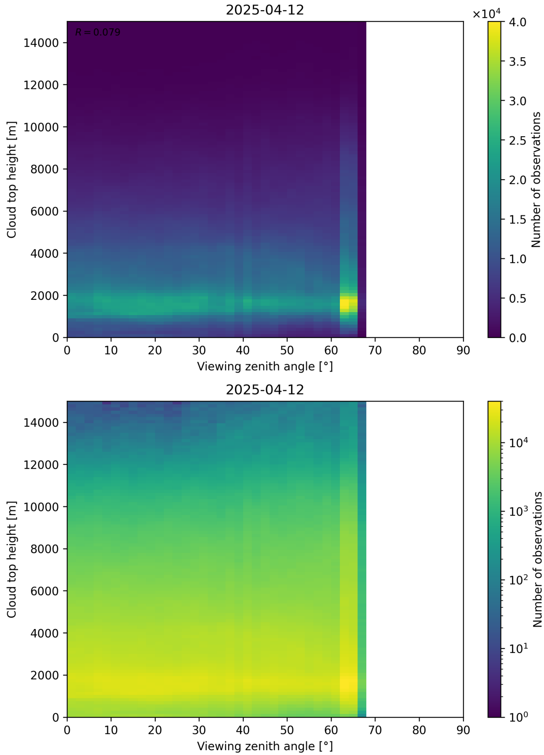
Figure 112: Scatter density plot of “Viewing zenith angle” against “Cloud top height” for 2025-04-11 to 2025-04-13.
