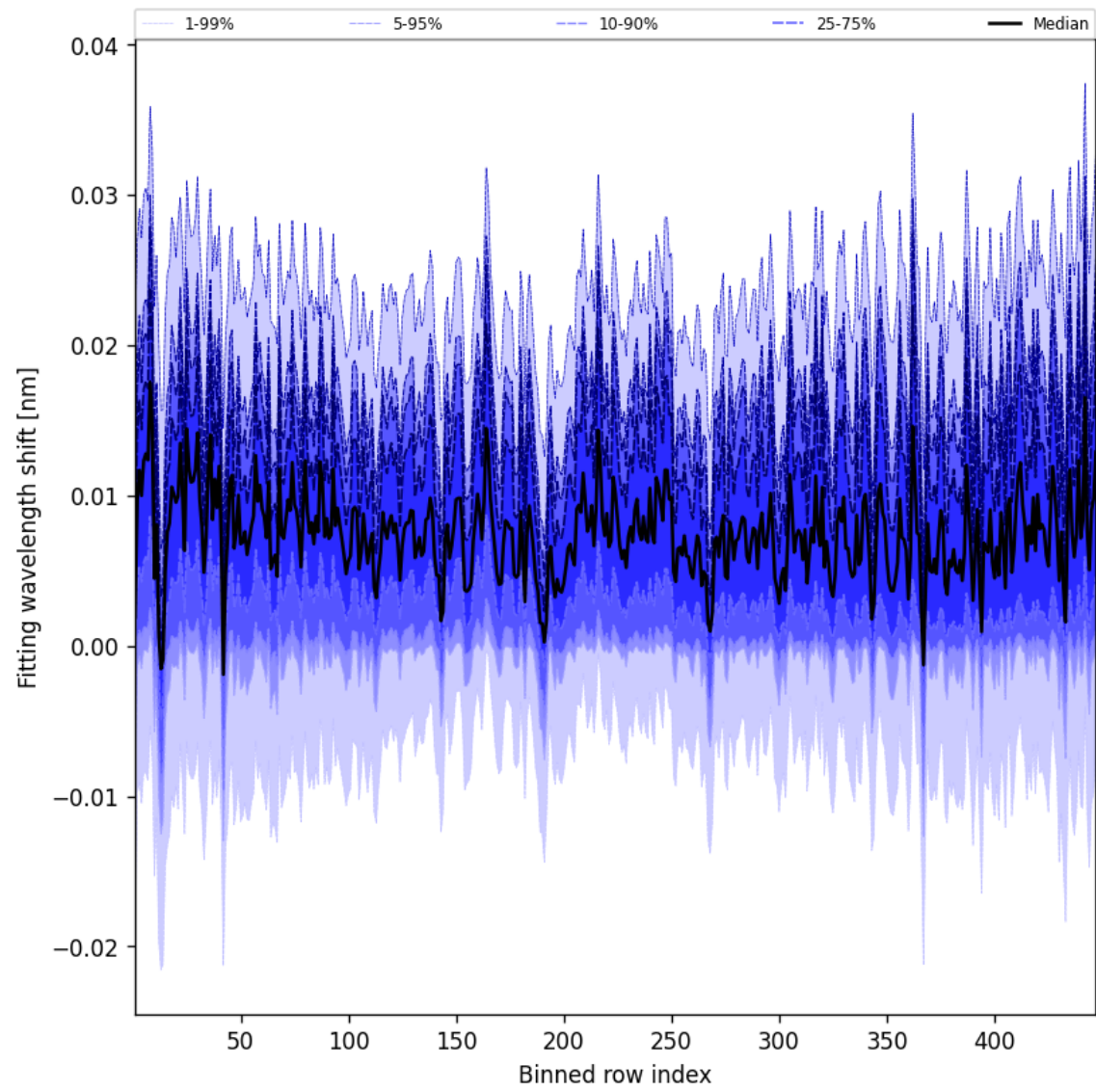
Figure 65: Along track statistics of “Fitting wavelength shift” for 2025-04-11 to 2025-04-13
