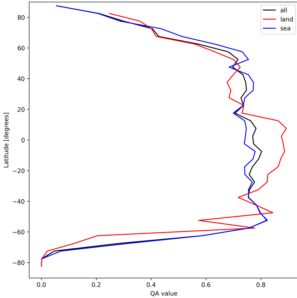
Figure 22: Zonal average of “QA value” for 2025-04-11 to 2025-04-13.
