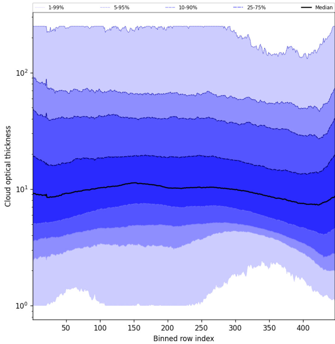
Figure 57: Along track statistics of “Cloud optical thickness” for 2025-04-11 to 2025-04-13
