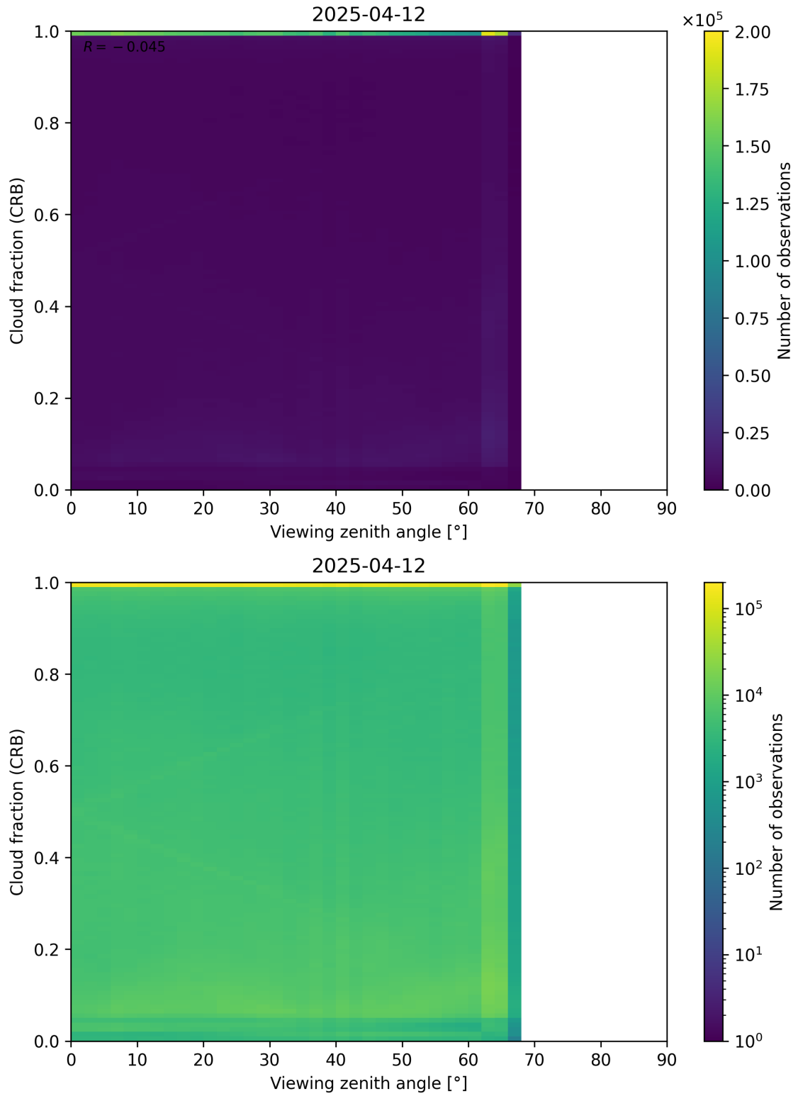
Figure 109: Scatter density plot of “Viewing zenith angle” against “Cloud fraction (CRB)” for 2025-04-11 to 2025-04-13.
