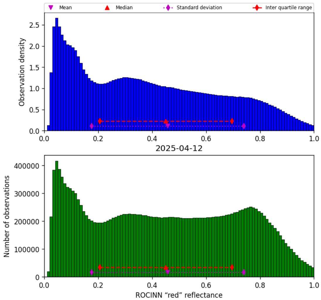
Figure 53: Histogram of “ROCINN “red” reflectance” for 2025-04-11 to 2025-04-13
