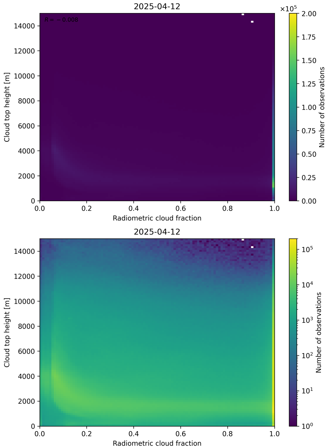
Figure 76: Scatter density plot of “Radiometric cloud fraction” against “Cloud top height” for 2025-04-11 to 2025-04-13.
