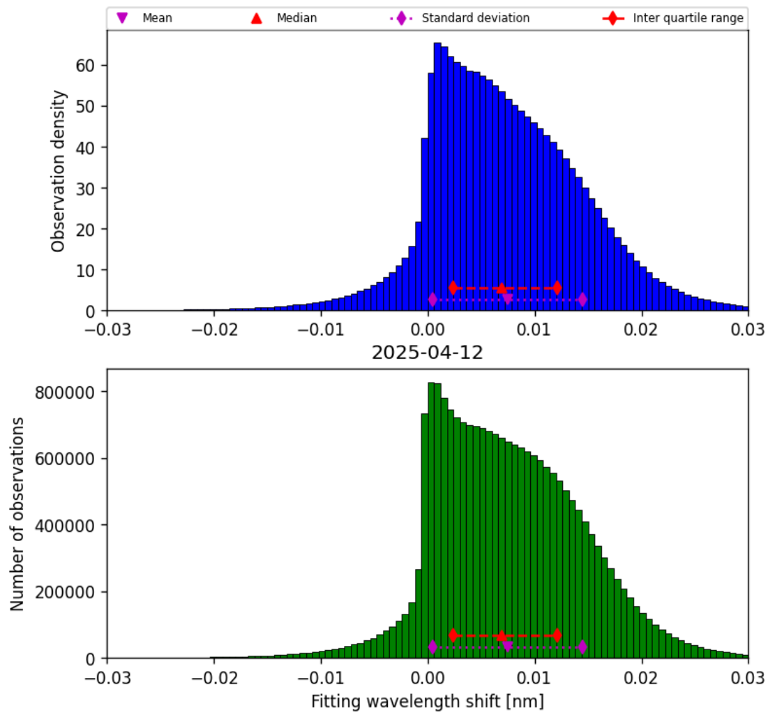
Figure 49: Histogram of “Fitting wavelength shift” for 2025-04-11 to 2025-04-13
