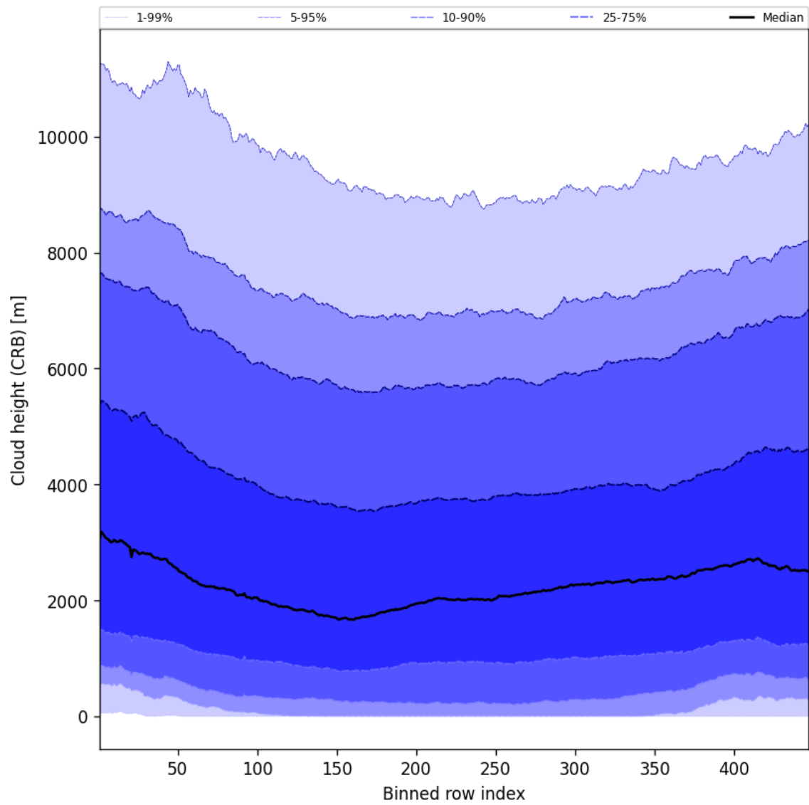
Figure 59: Along track statistics of “Cloud height (CRB)” for 2025-04-11 to 2025-04-13
