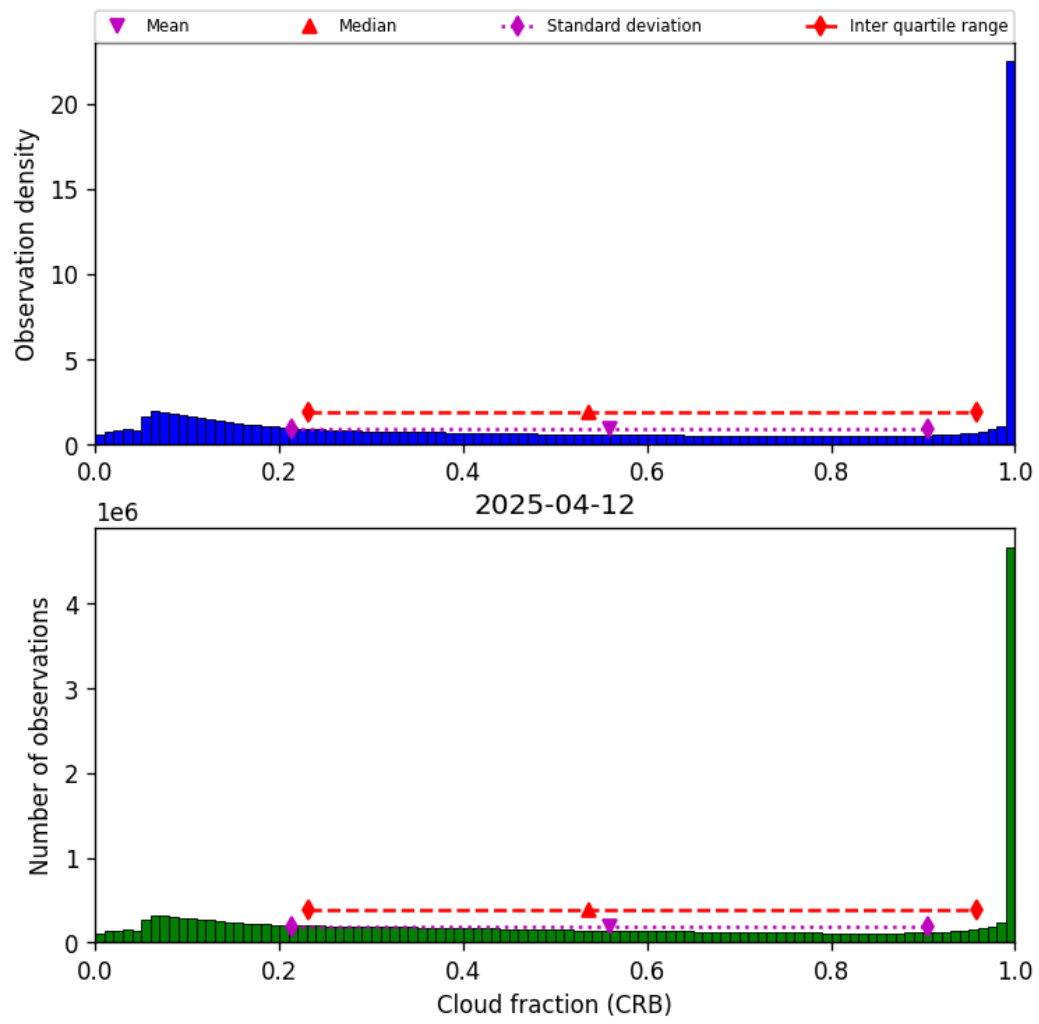
Figure 42: Histogram of “Cloud fraction (CRB)” for 2025-04-11 to 2025-04-13
