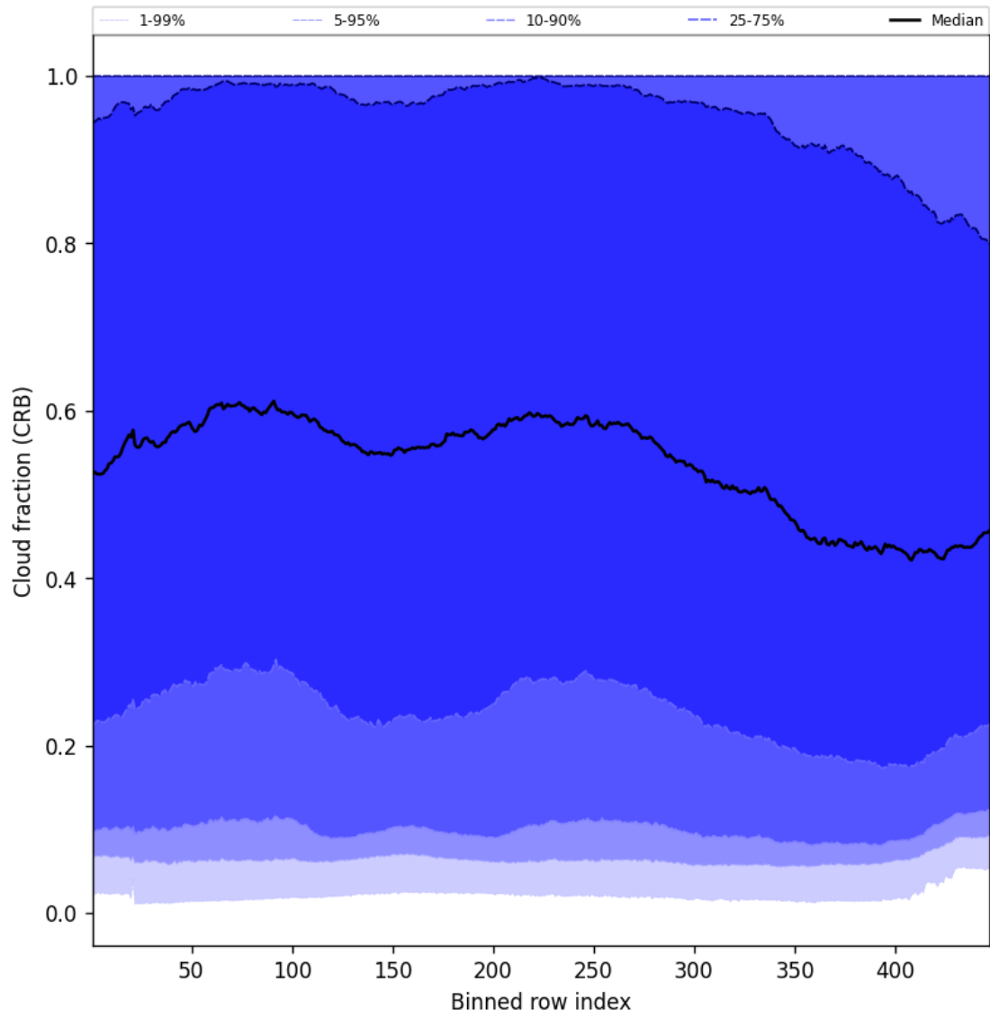
Figure 58: Along track statistics of “Cloud fraction (CRB)” for 2025-04-11 to 2025-04-13
