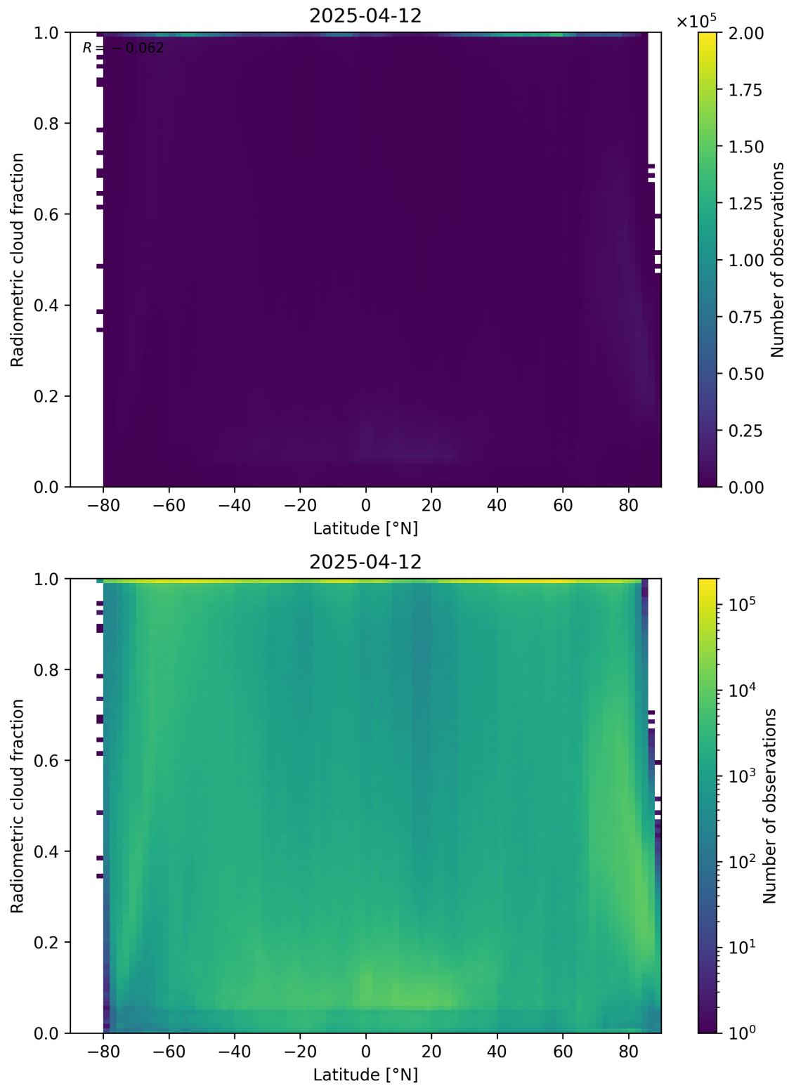
Figure 92: Scatter density plot of “Latitude” against “Radiometric cloud fraction” for 2025-04-11 to 2025-04-13.
