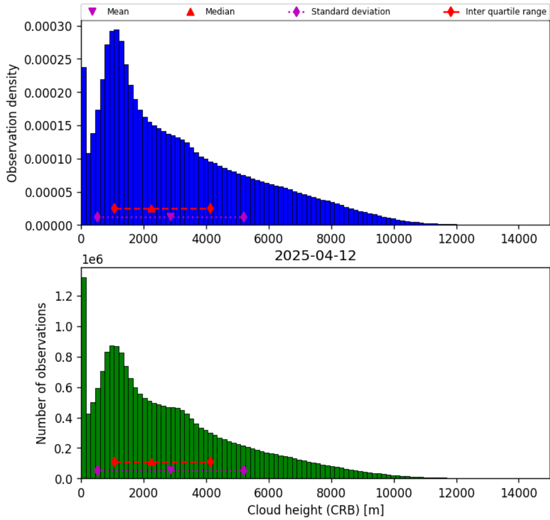
Figure 43: Histogram of “Cloud height (CRB)” for 2025-04-11 to 2025-04-13
