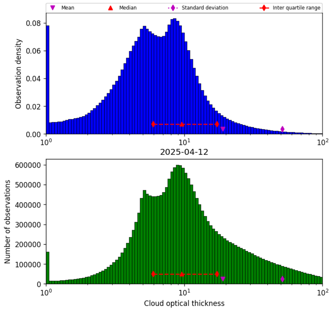
Figure 41: Histogram of “Cloud optical thickness” for 2025-04-11 to 2025-04-13
