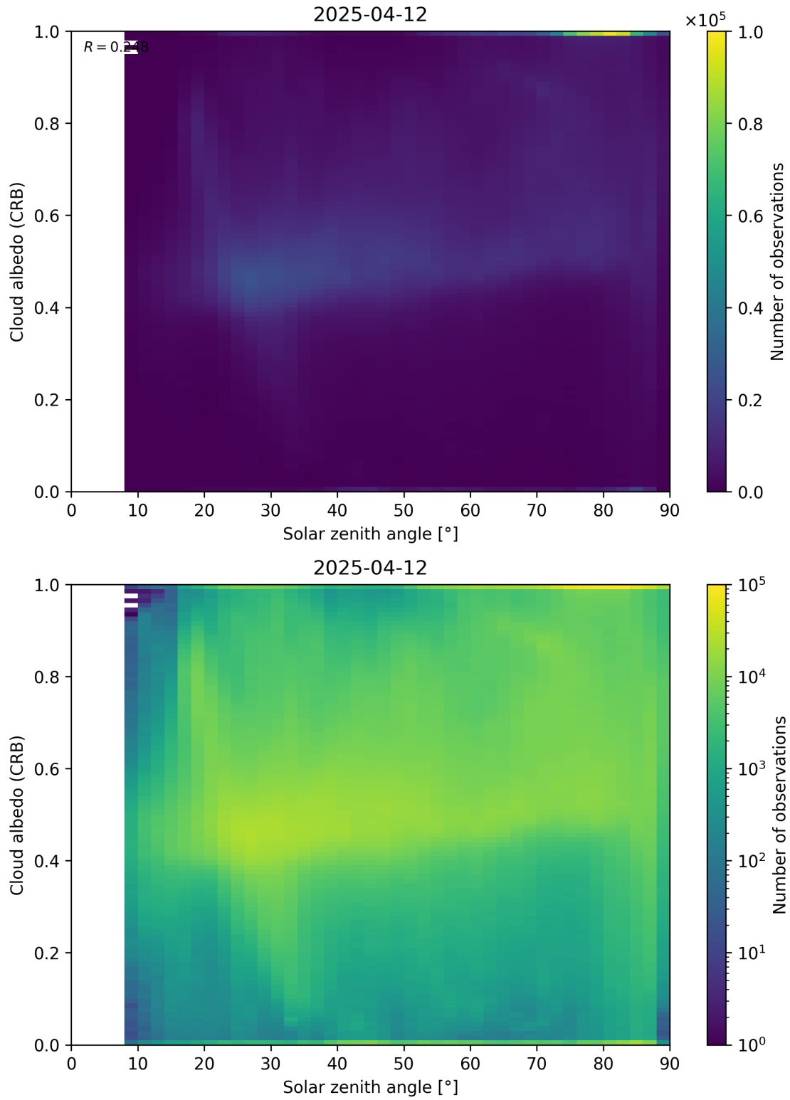
Figure 98: Scatter density plot of “Solar zenith angle” against “Cloud albedo (CRB)” for 2025-04-11 to 2025-04-13.
