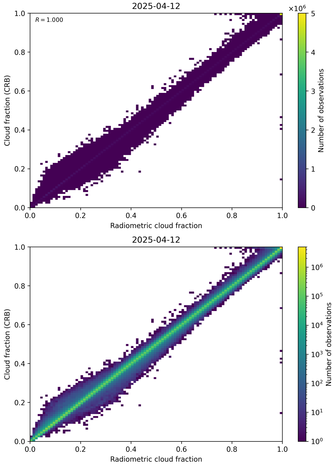
Figure 73: Scatter density plot of “Radiometric cloud fraction” against “Cloud fraction (CRB)” for 2025-04-11 to 2025-04-13.
