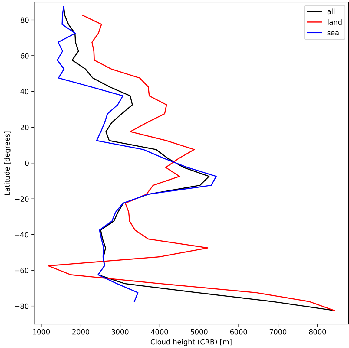
Figure 27: Zonal average of “Cloud height (CRB)” for 2025-04-11 to 2025-04-13.
