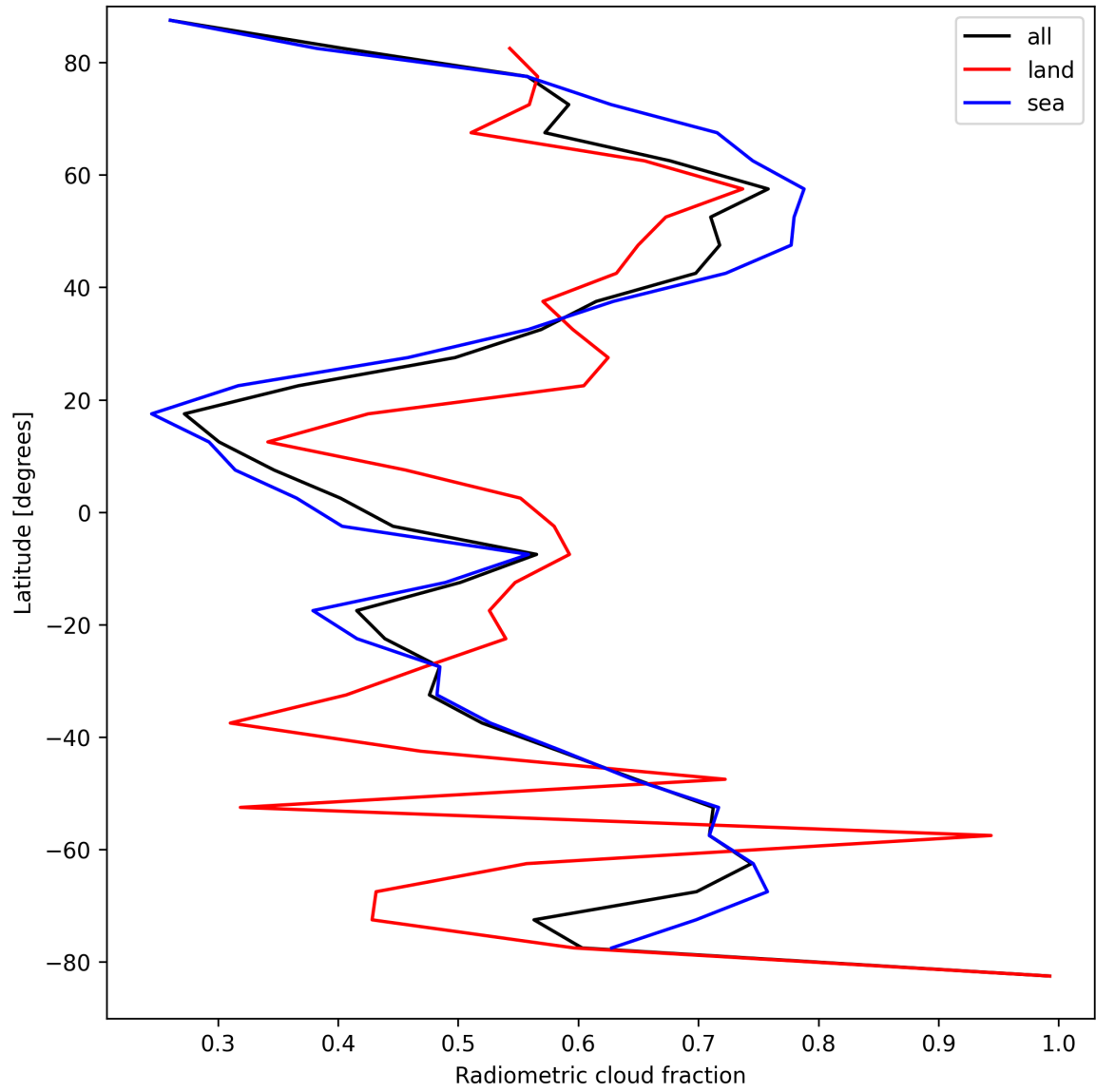
Figure 23: Zonal average of “Radiometric cloud fraction” for 2025-04-11 to 2025-04-13.
