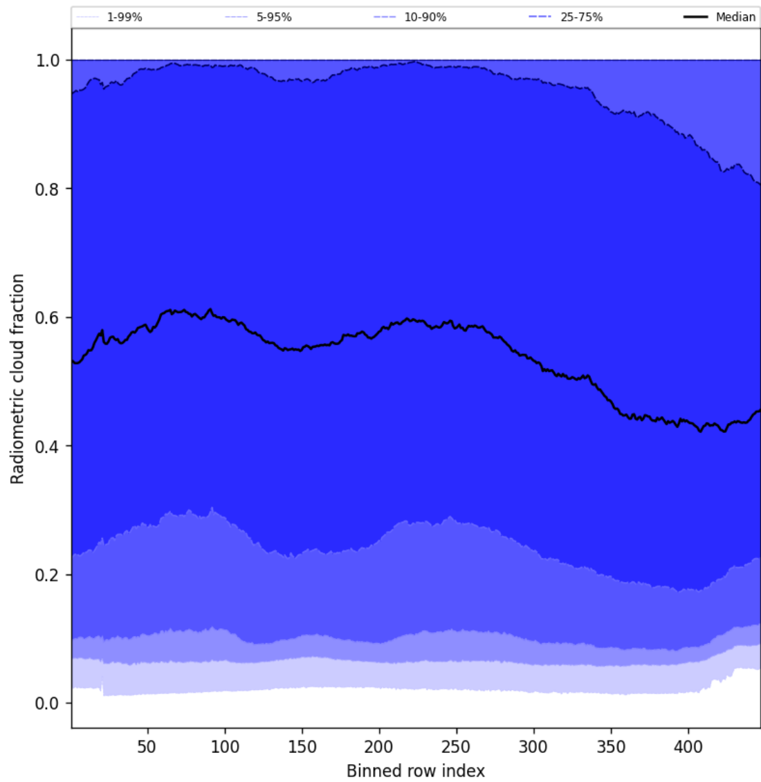
Figure 55: Along track statistics of “Radiometric cloud fraction” for 2025-04-11 to 2025-04-13
