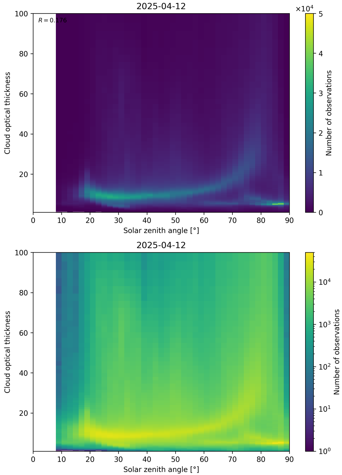
Figure 103: Scatter density plot of “Solar zenith angle” against “Cloud optical thickness” for 2025-04-11 to 2025-04-13.
