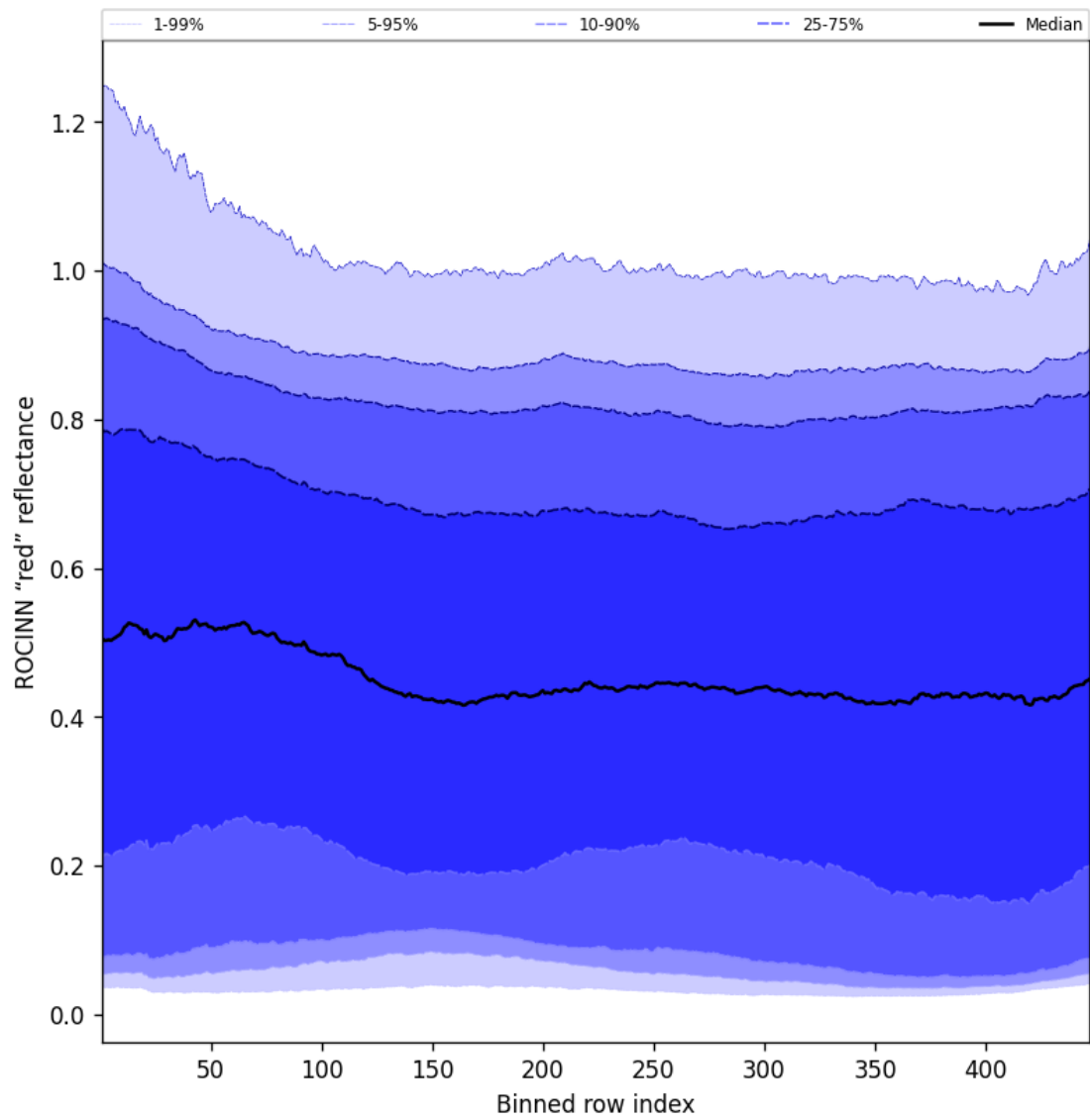
Figure 69: Along track statistics of “ROCINN “red” reflectance” for 2025-04-11 to 2025-04-13
