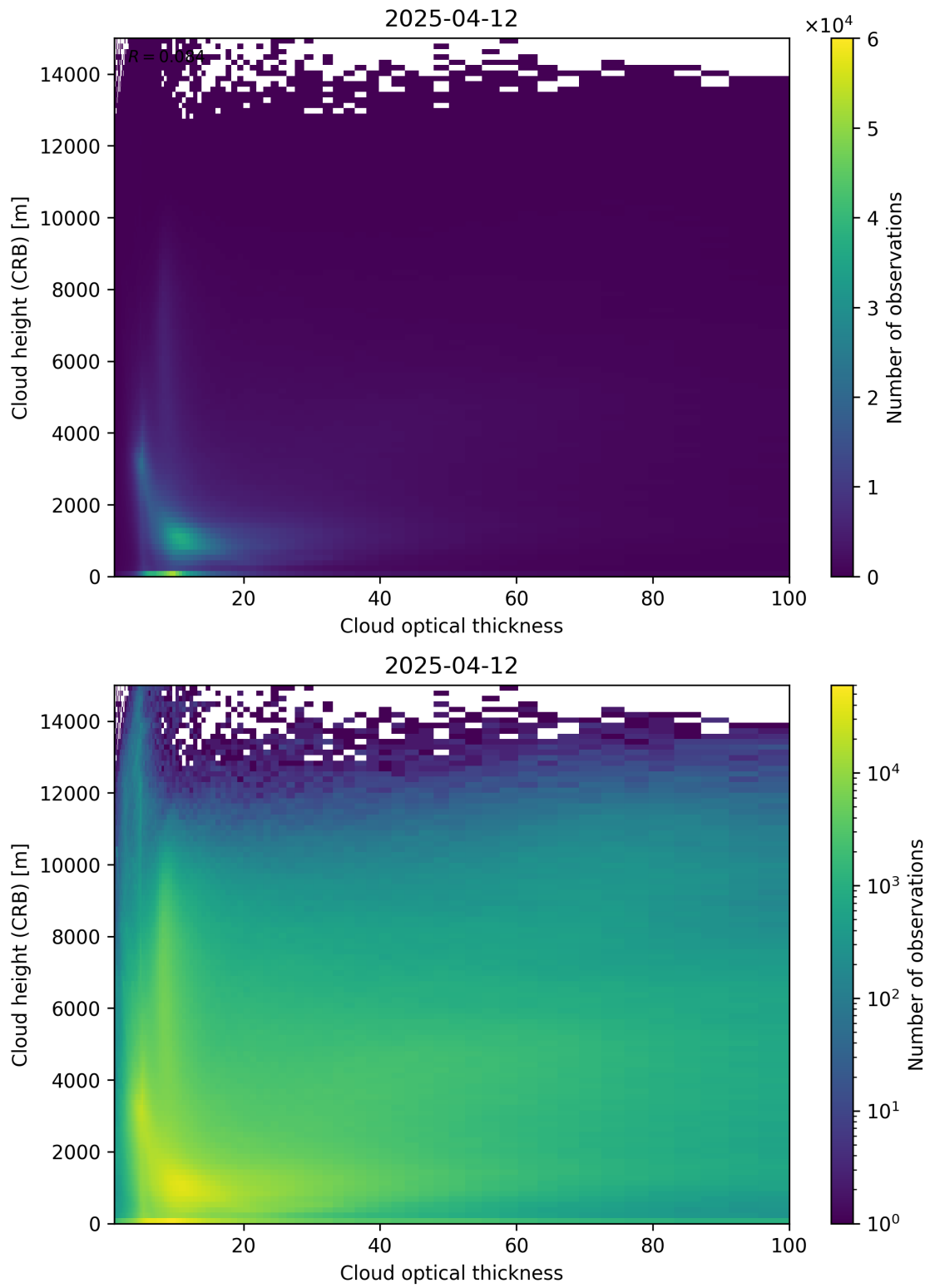
Figure 85: Scatter density plot of “Cloud optical thickness” against “Cloud height (CRB)” for 2025-04-11 to 2025-04-13.
