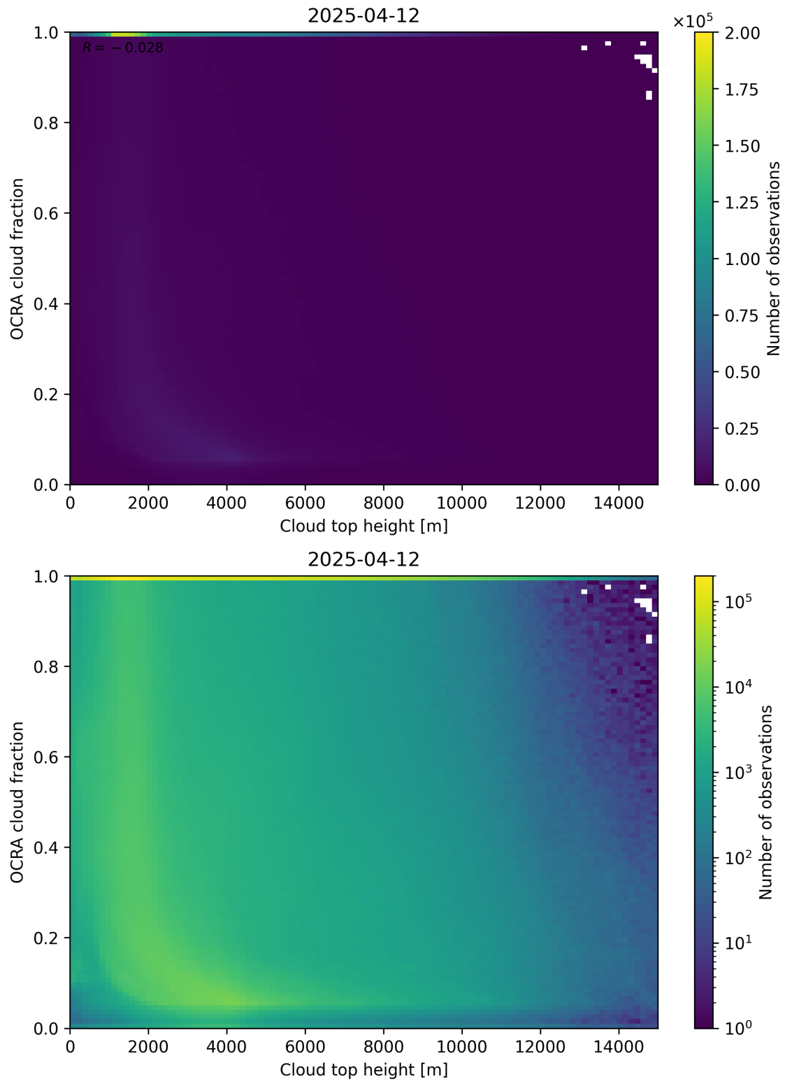
Figure 87: Scatter density plot of “Cloud top height” against “OCRA cloud fraction” for 2025-04-11 to 2025-04-13.
