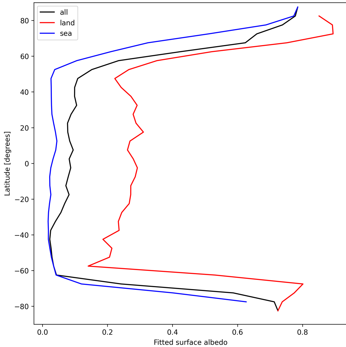
Figure 29: Zonal average of “Fitted surface albedo” for 2025-04-11 to 2025-04-13.
