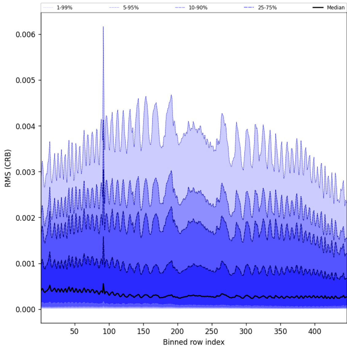
Figure 64: Along track statistics of “RMS (CRB)” for 2025-04-11 to 2025-04-13
