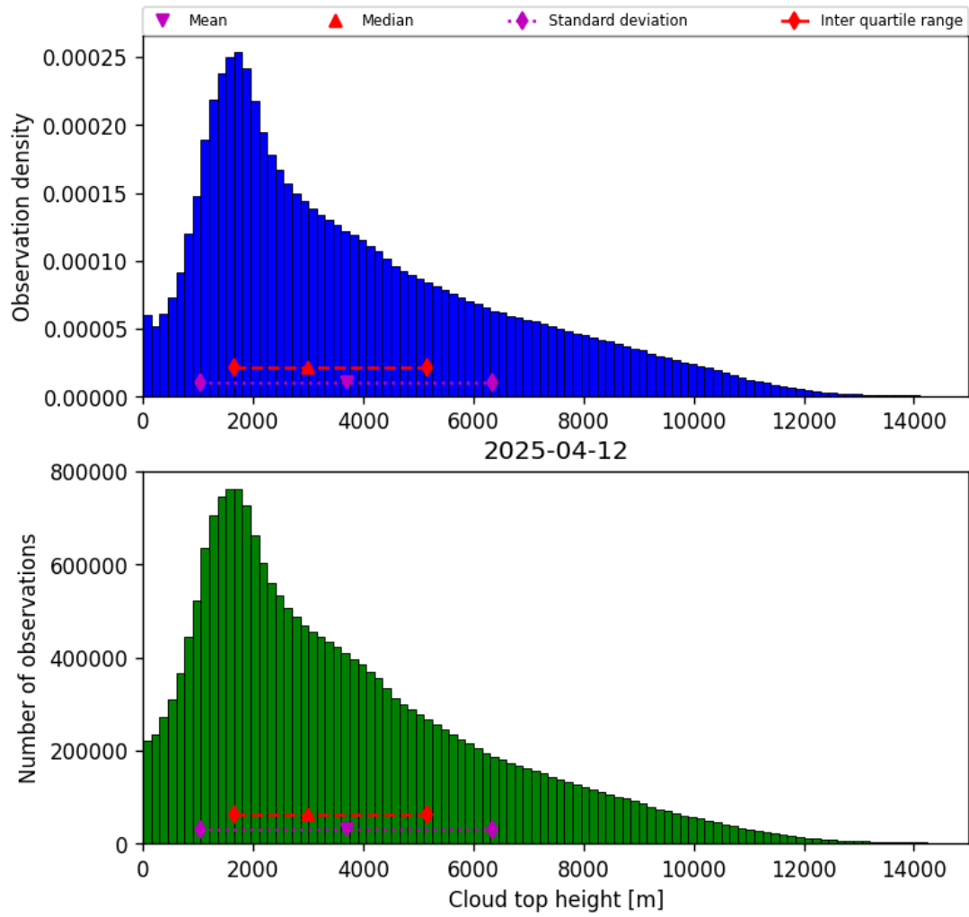
Figure 40: Histogram of “Cloud top height” for 2025-04-11 to 2025-04-13
