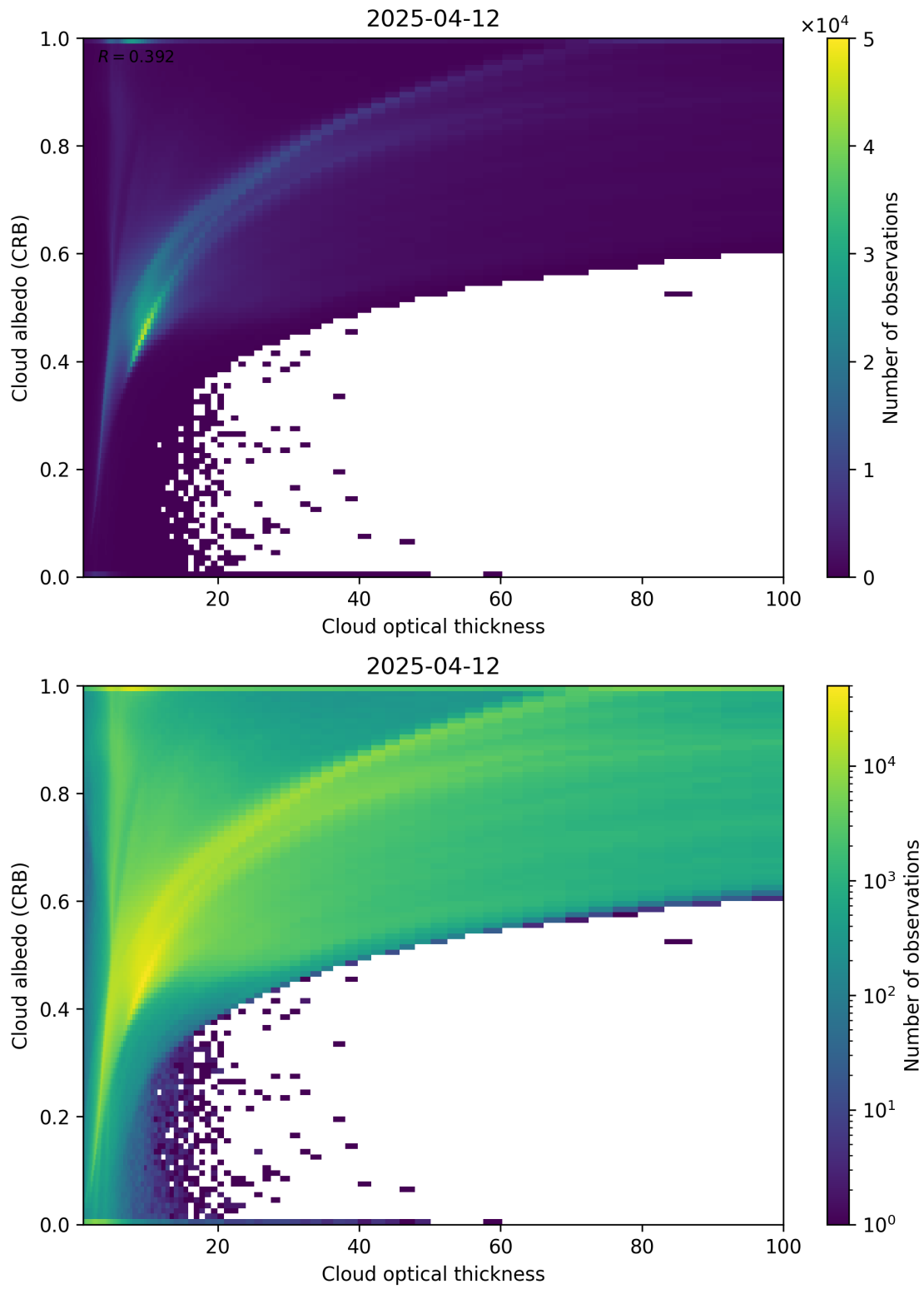
Figure 82: Scatter density plot of “Cloud optical thickness” against “Cloud albedo (CRB)” for 2025-04-11 to 2025-04-13.
