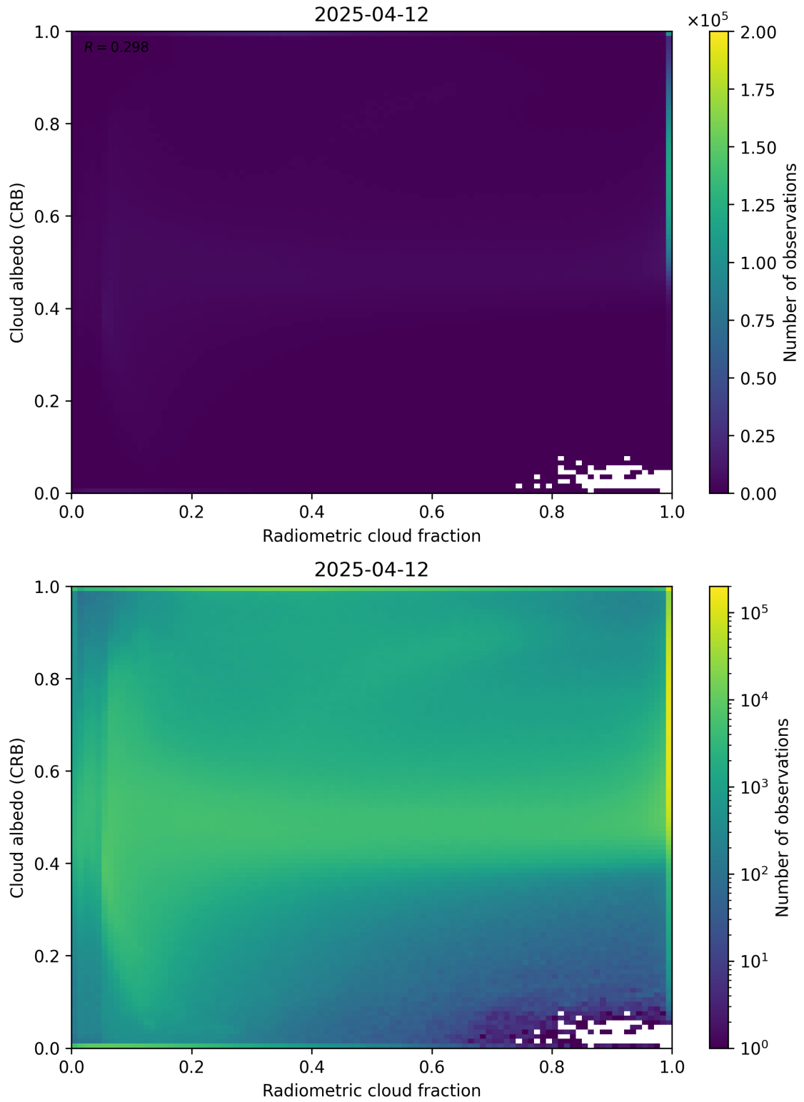
Figure 71: Scatter density plot of “Radiometric cloud fraction” against “Cloud albedo (CRB)” for 2025-04-11 to 2025-04-13.
