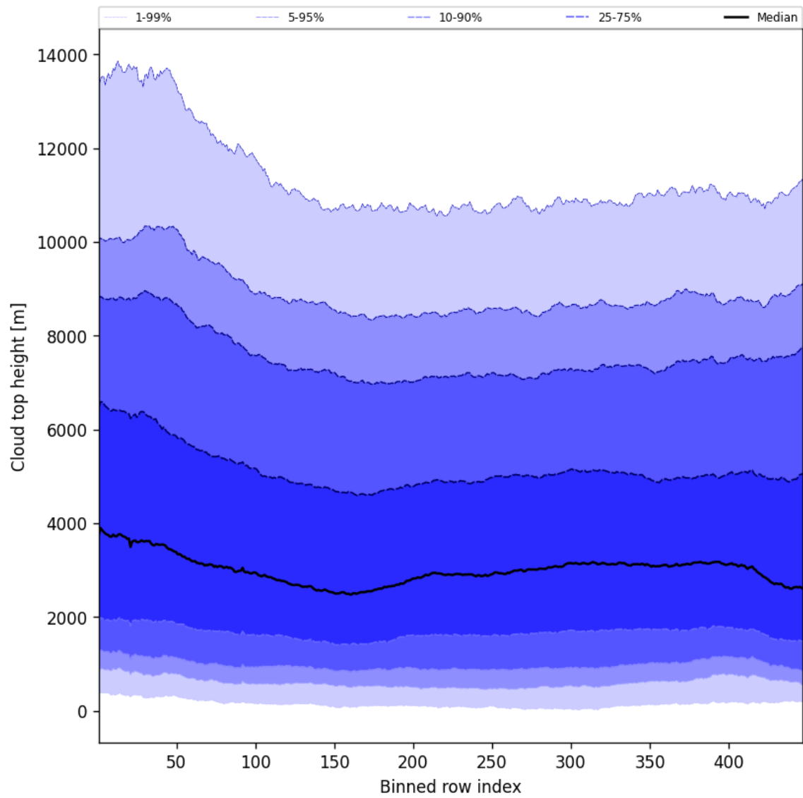
Figure 56: Along track statistics of “Cloud top height” for 2025-04-11 to 2025-04-13
