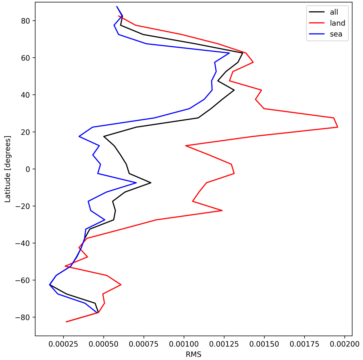
Figure 31: Zonal average of “RMS” for 2025-04-11 to 2025-04-13.
