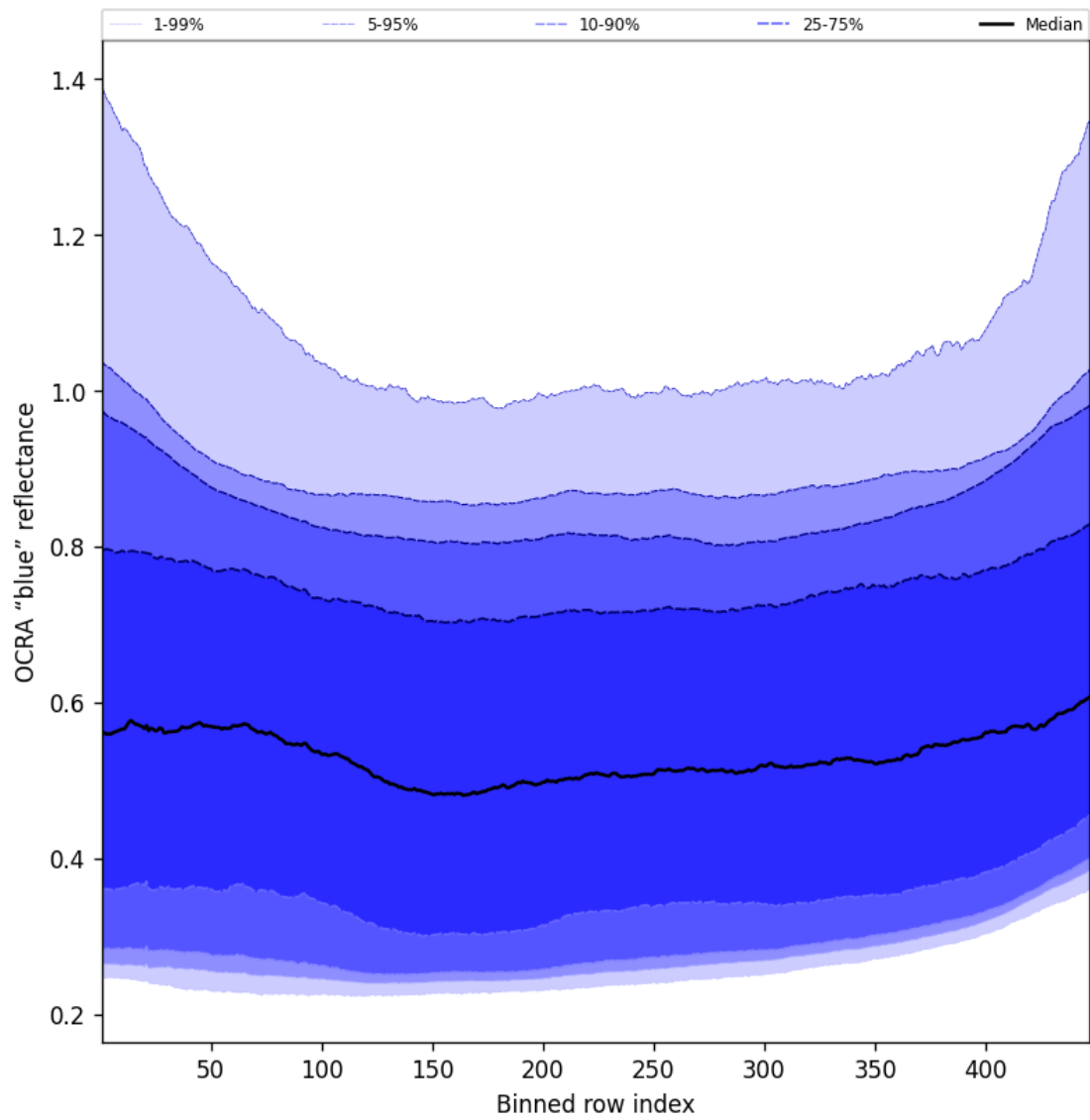
Figure 67: Along track statistics of “OCRA “blue” reflectance” for 2025-04-11 to 2025-04-13
