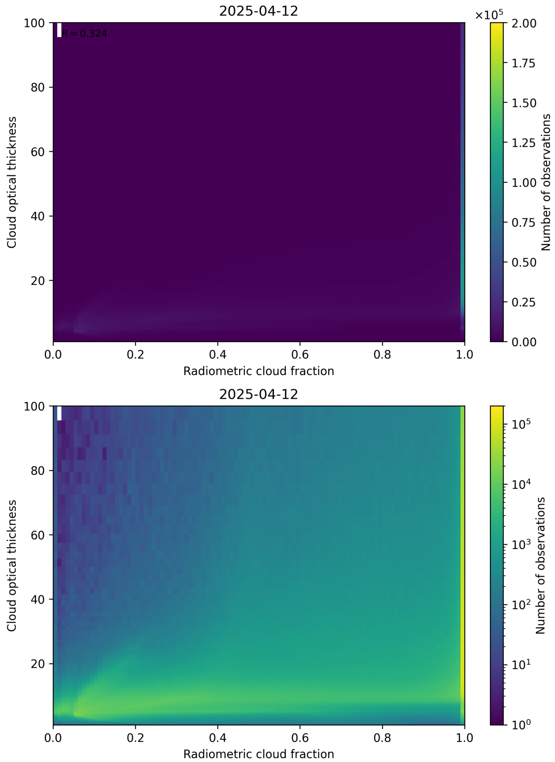
Figure 75: Scatter density plot of “Radiometric cloud fraction” against “Cloud optical thickness” for 2025-04-11 to 2025-04-13.
