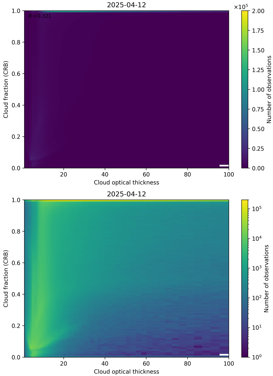
Figure 84: Scatter density plot of “Cloud optical thickness” against “Cloud fraction (CRB)” for 2025-04-11 to 2025-04-13.
