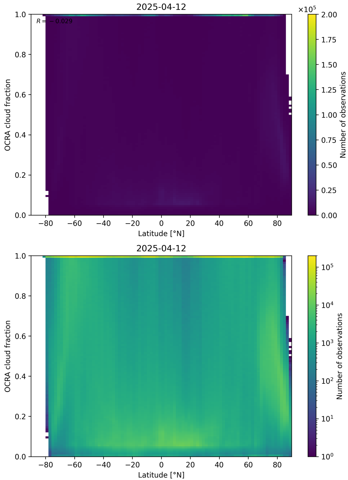
Figure 93: Scatter density plot of “Latitude” against “OCRA cloud fraction” for 2025-04-11 to 2025-04-13.
