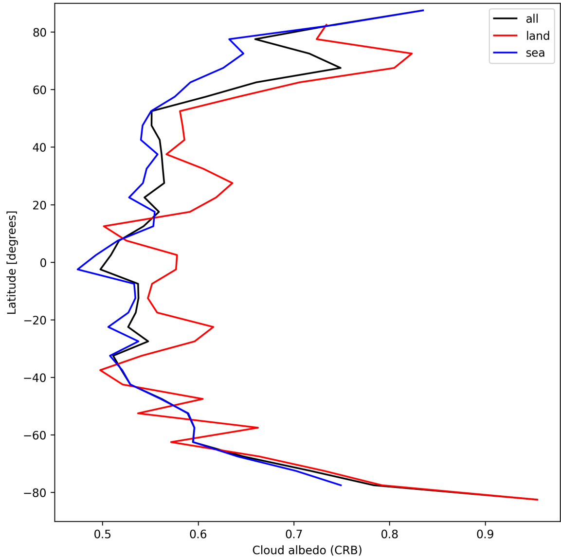
Figure 28: Zonal average of “Cloud albedo (CRB)” for 2025-04-11 to 2025-04-13.
