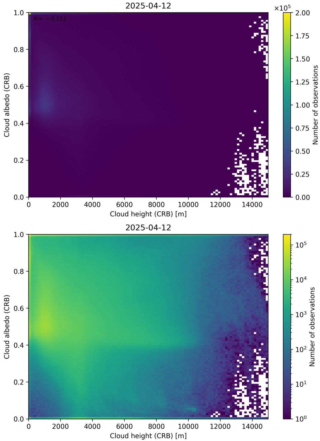
Figure 80: Scatter density plot of “Cloud height (CRB)” against “Cloud albedo (CRB)” for 2025-04-11 to 2025-04-13.
