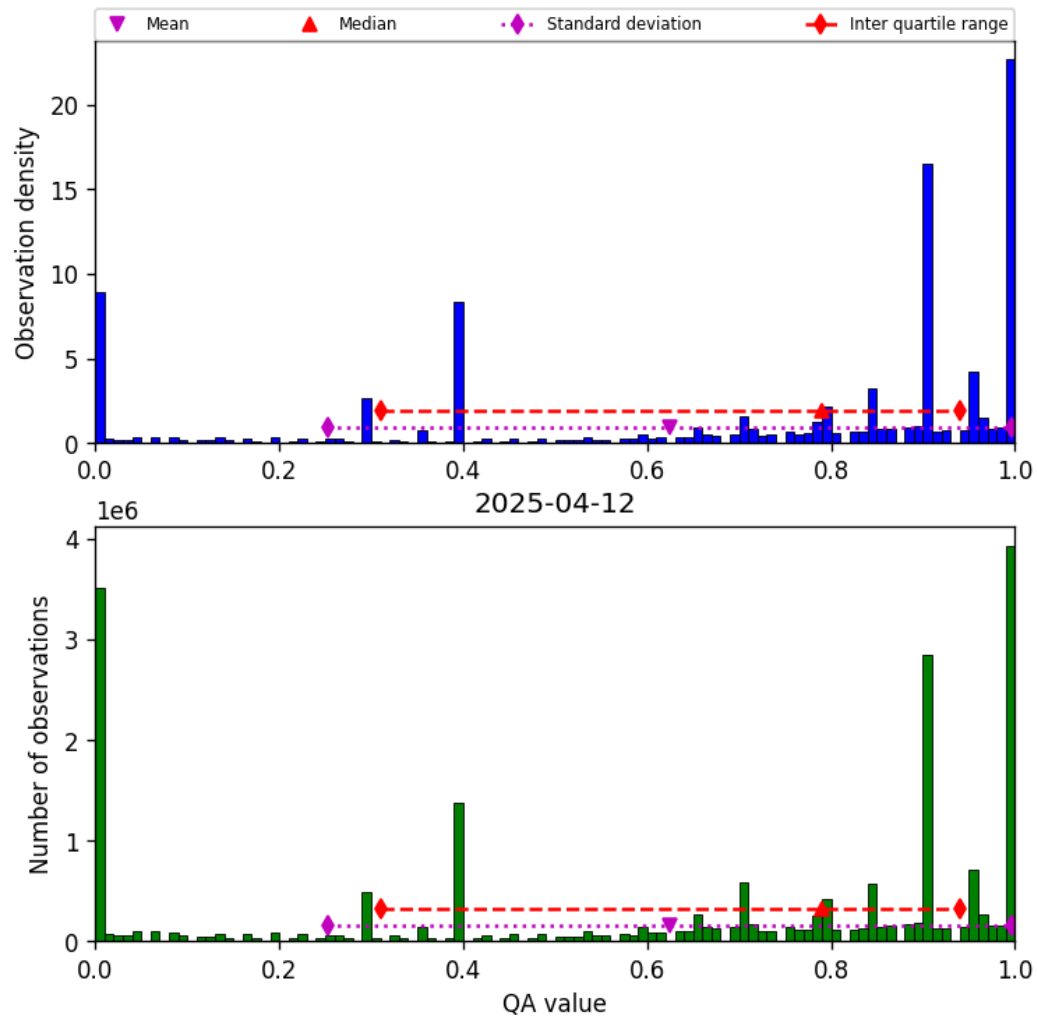
Figure 38: Histogram of “QA value” for 2025-04-11 to 2025-04-13
