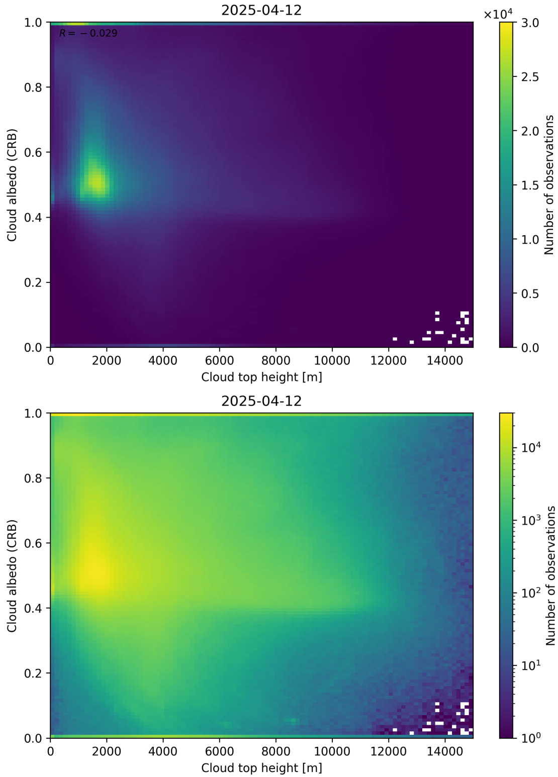
Figure 86: Scatter density plot of “Cloud top height” against “Cloud albedo (CRB)” for 2025-04-11 to 2025-04-13.
