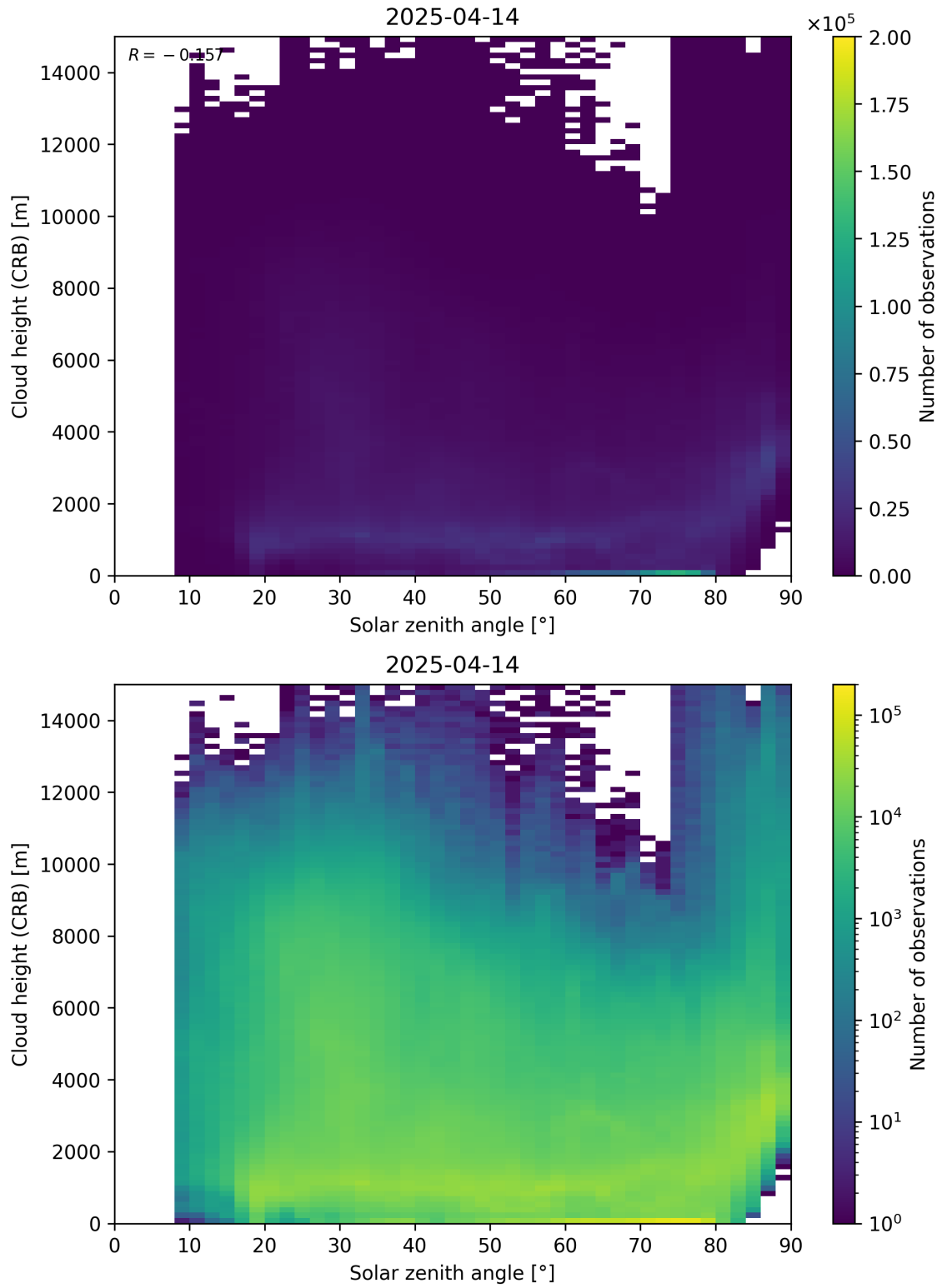
Figure 102: Scatter density plot of “Solar zenith angle” against “Cloud height (CRB)” for 2025-04-13 to 2025-04-15.
