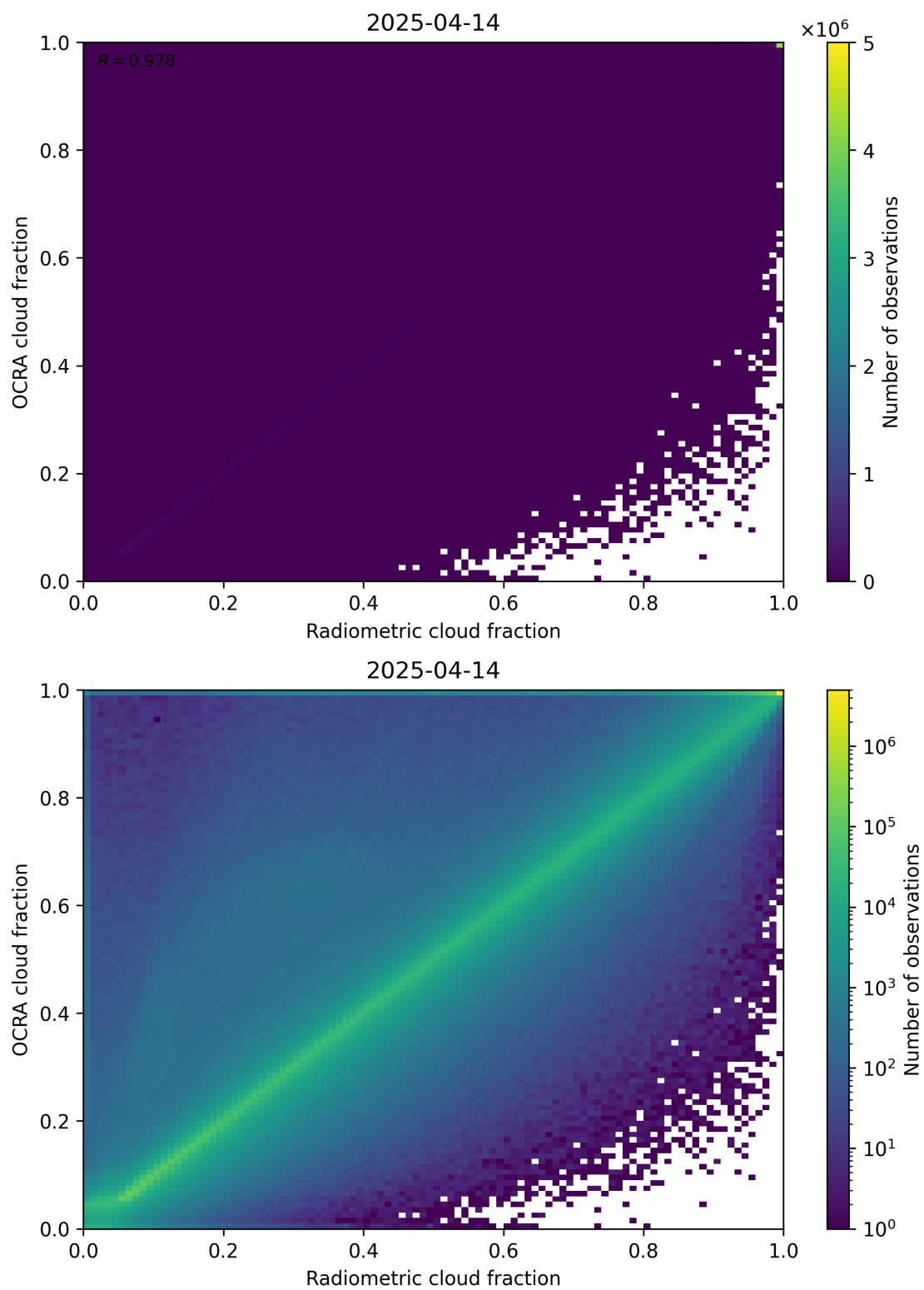
Figure 72: Scatter density plot of “Radiometric cloud fraction” against “OCRA cloud fraction” for 2025-04-13 to 2025-04-15.
