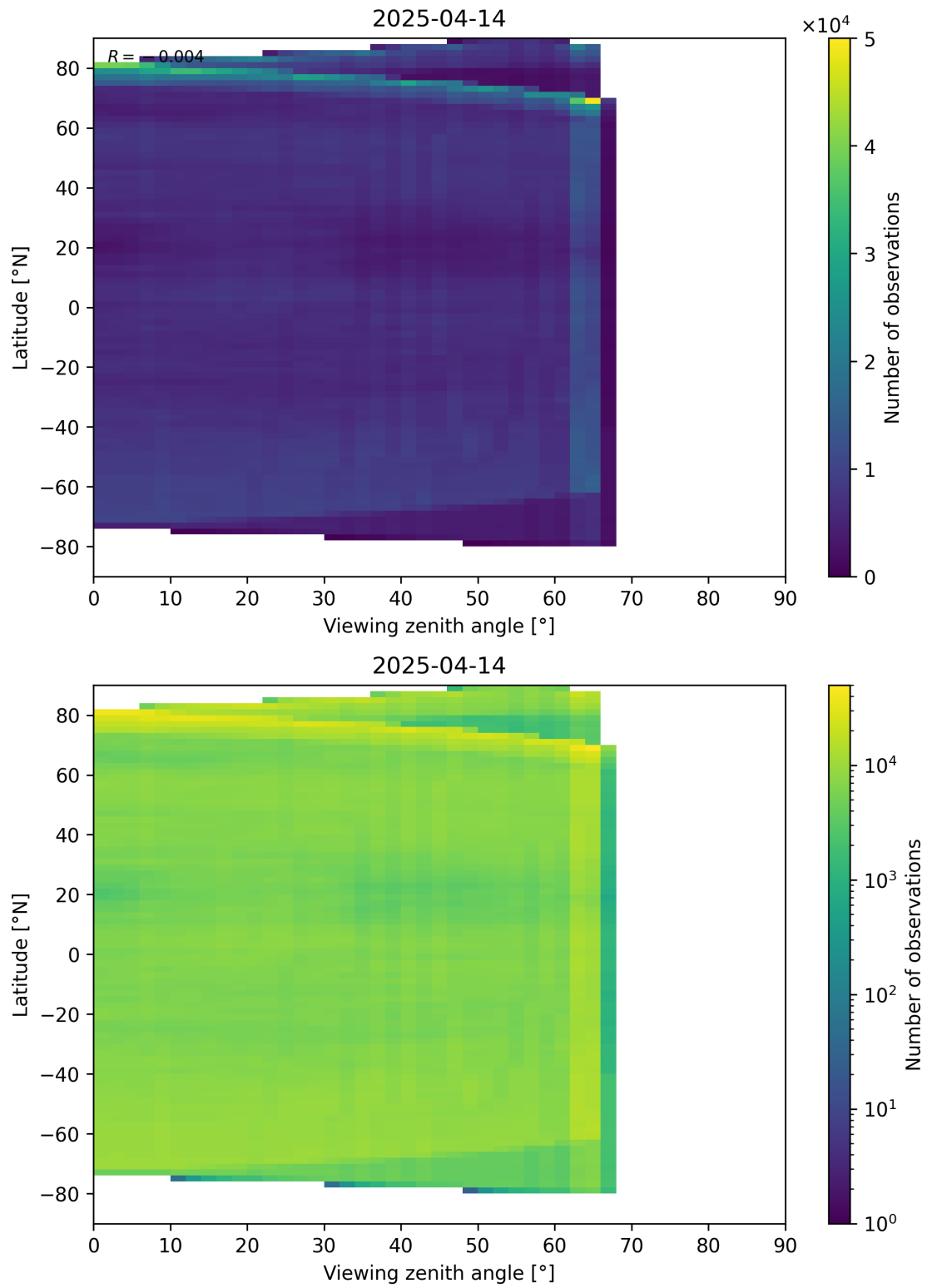
Figure 113: Scatter density plot of “Viewing zenith angle” against “Latitude” for 2025-04-13 to 2025-04-15.
