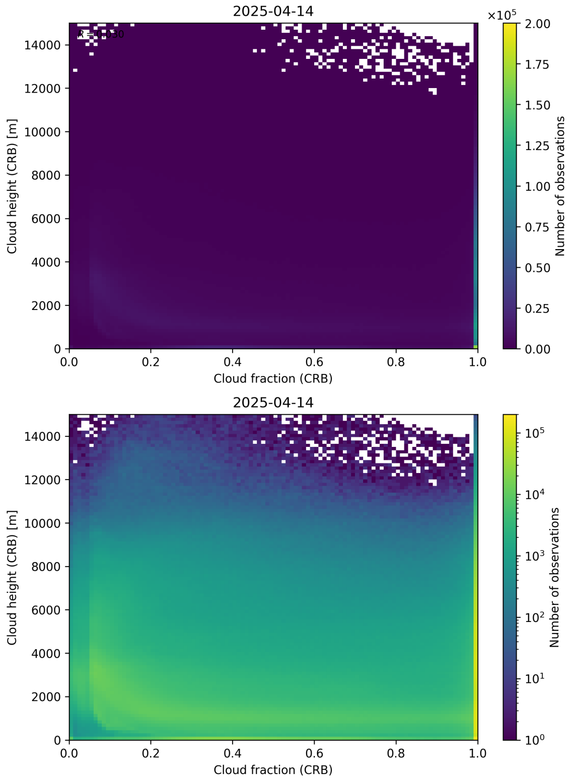
Figure 79: Scatter density plot of “Cloud fraction (CRB)” against “Cloud height (CRB)” for 2025-04-13 to 2025-04-15.
