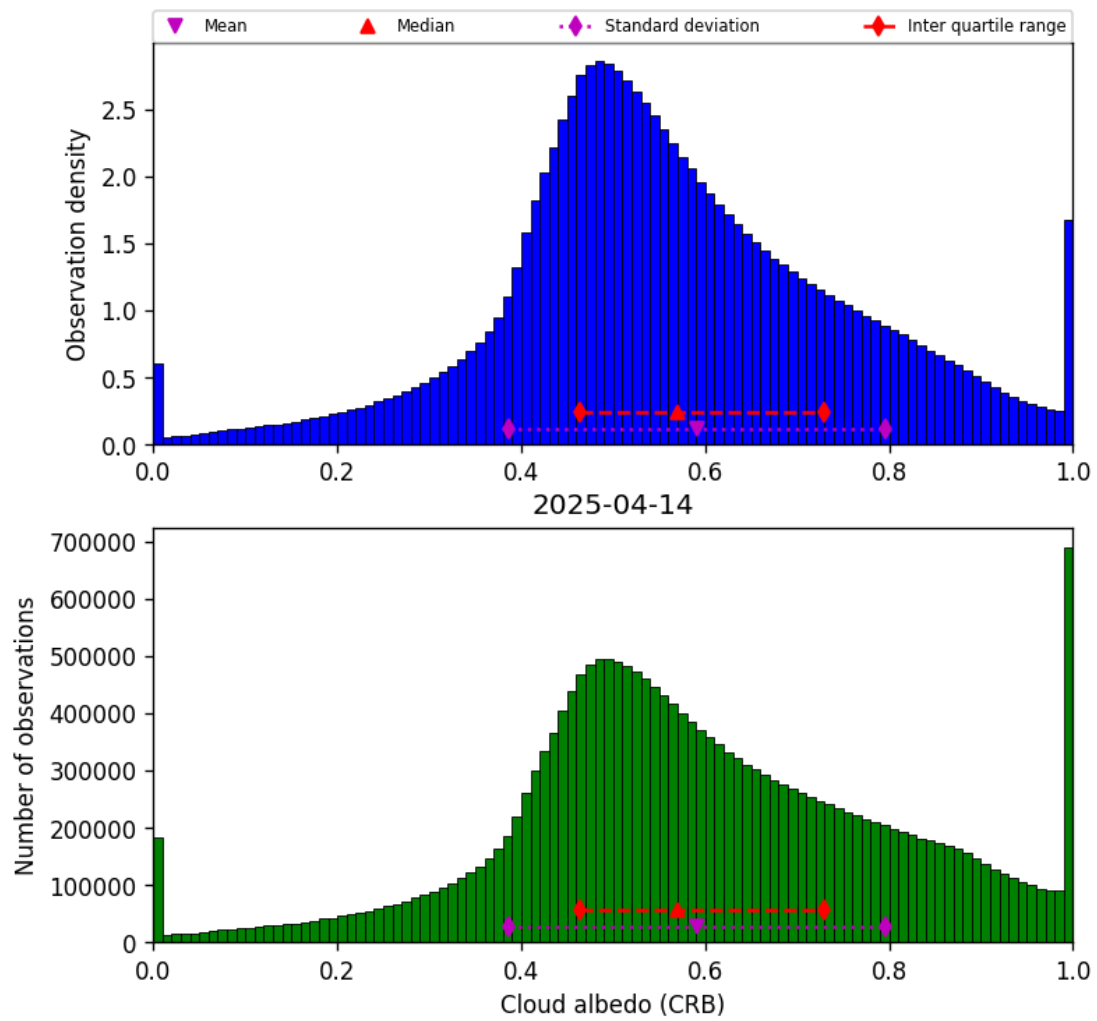
Figure 44: Histogram of “Cloud albedo (CRB)” for 2025-04-13 to 2025-04-15
