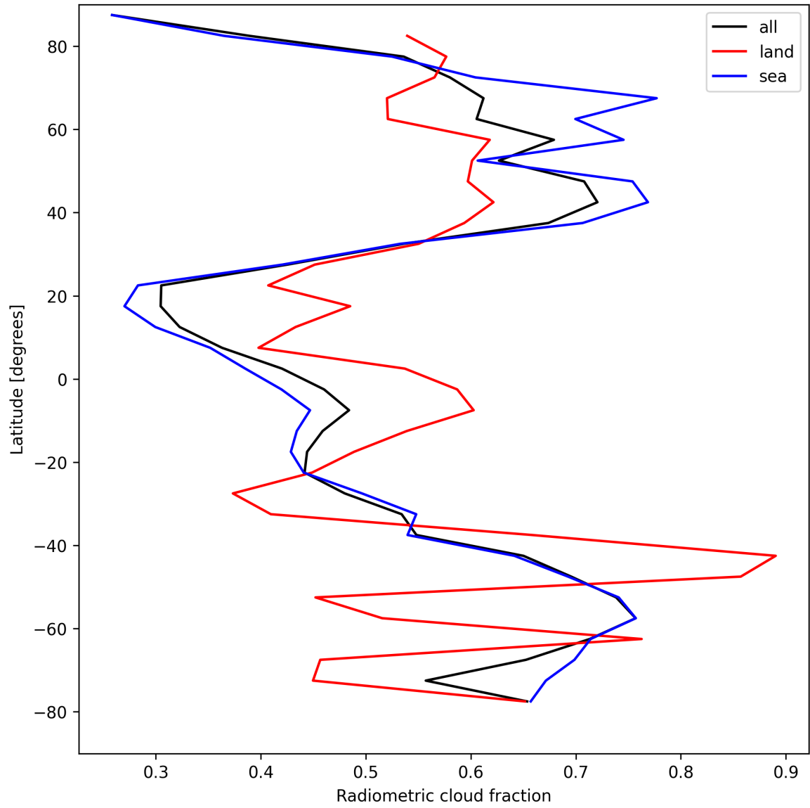
Figure 23: Zonal average of “Radiometric cloud fraction” for 2025-04-13 to 2025-04-15.
