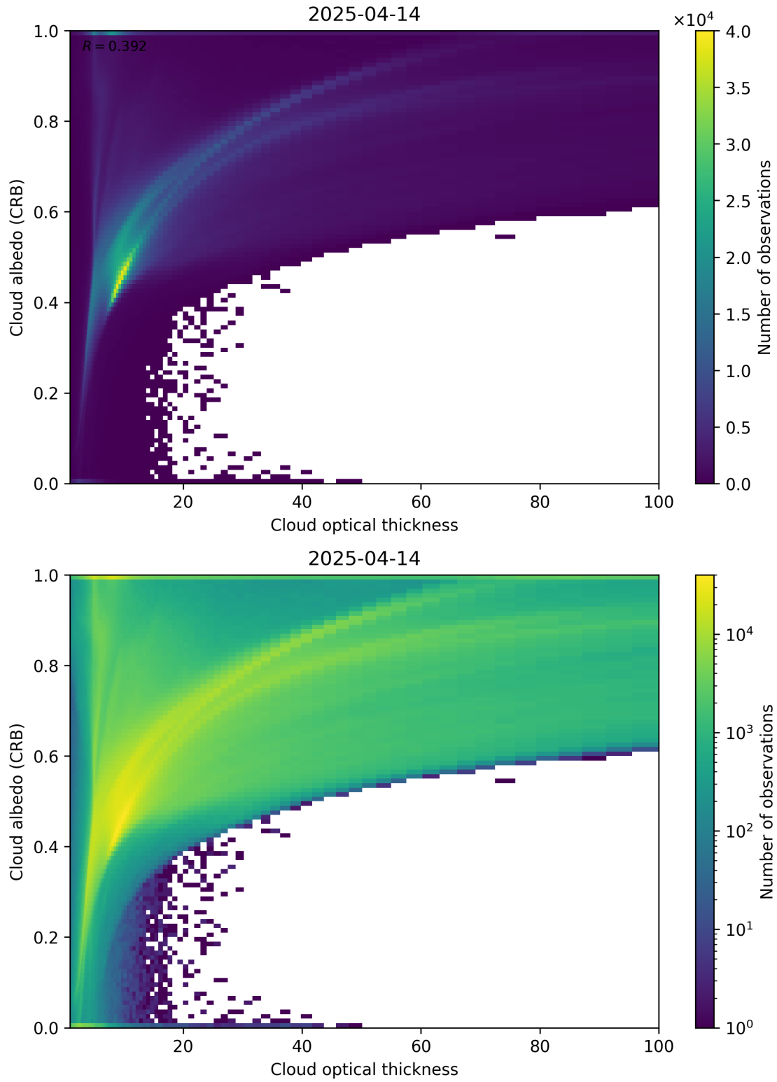
Figure 82: Scatter density plot of “Cloud optical thickness” against “Cloud albedo (CRB)” for 2025-04-13 to 2025-04-15.
