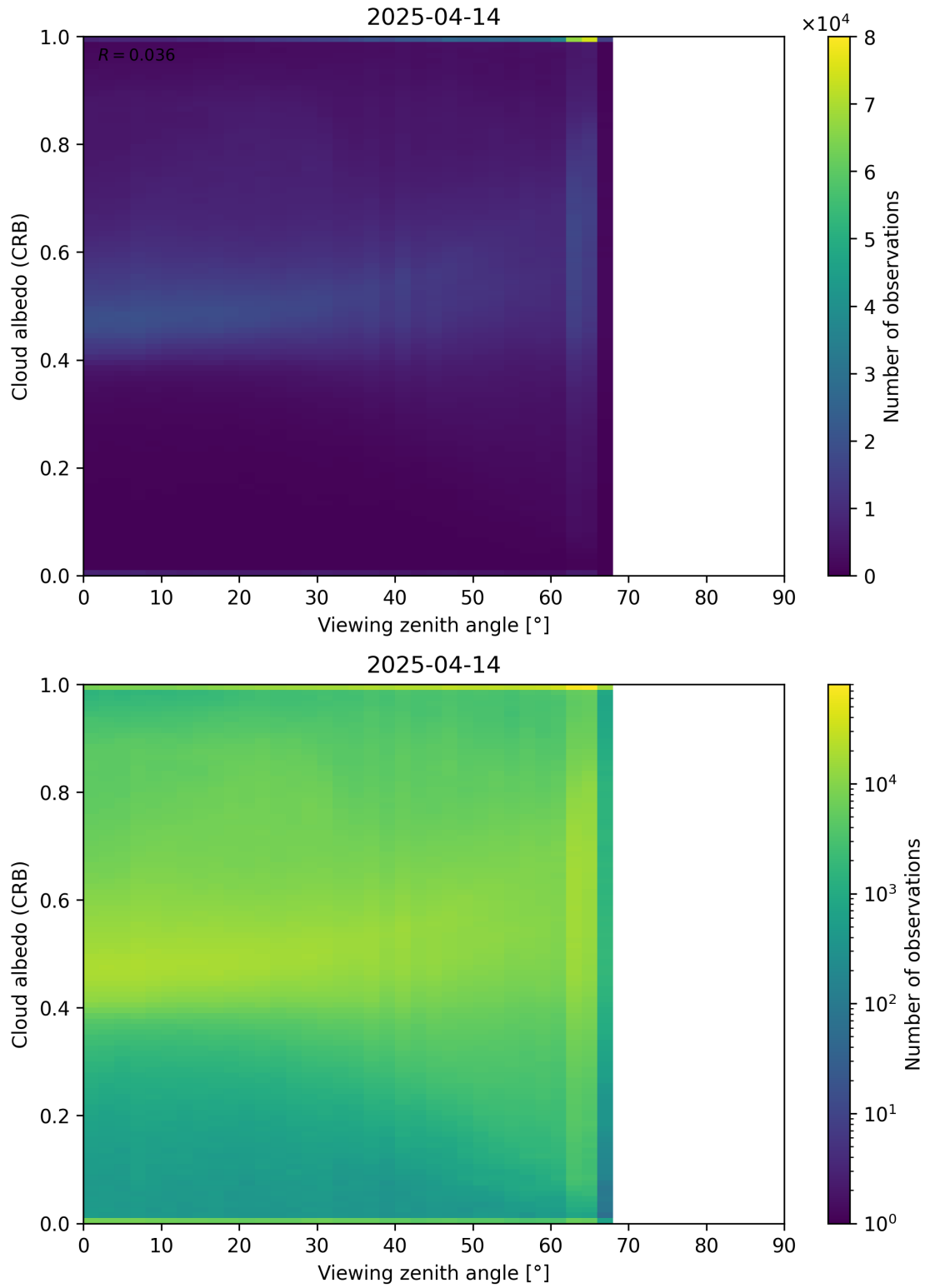
Figure 106: Scatter density plot of “Viewing zenith angle” against “Cloud albedo (CRB)” for 2025-04-13 to 2025-04-15.
