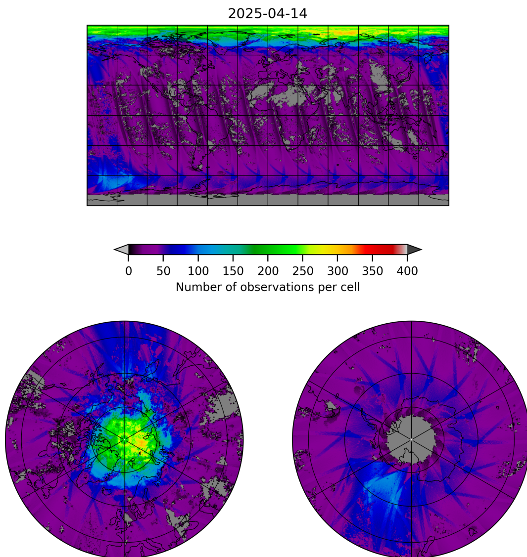
Figure 21: Map of the number of observations for 2025-04-13 to 2025-04-15
