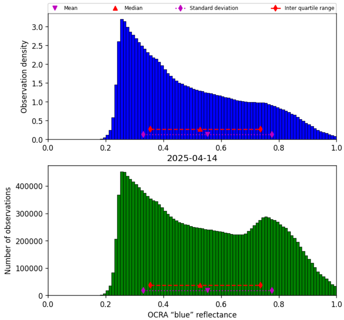
Figure 51: Histogram of “OCRA “blue” reflectance” for 2025-04-13 to 2025-04-15
