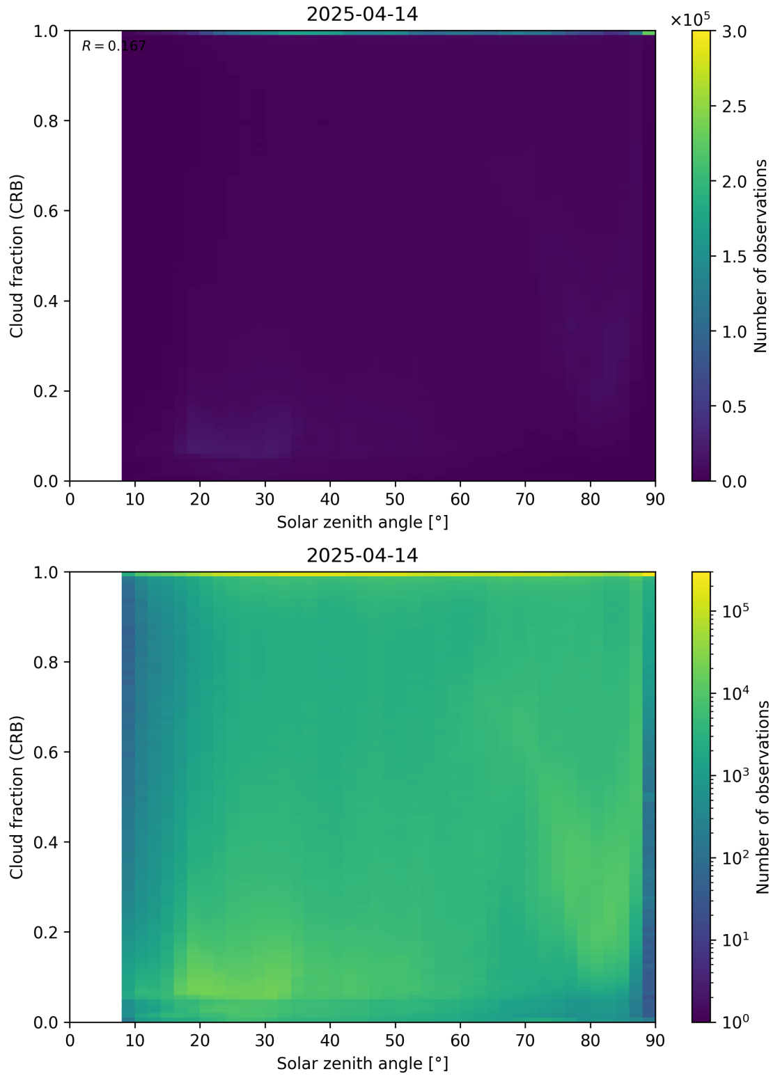
Figure 101: Scatter density plot of “Solar zenith angle” against “Cloud fraction (CRB)” for 2025-04-13 to 2025-04-15.
