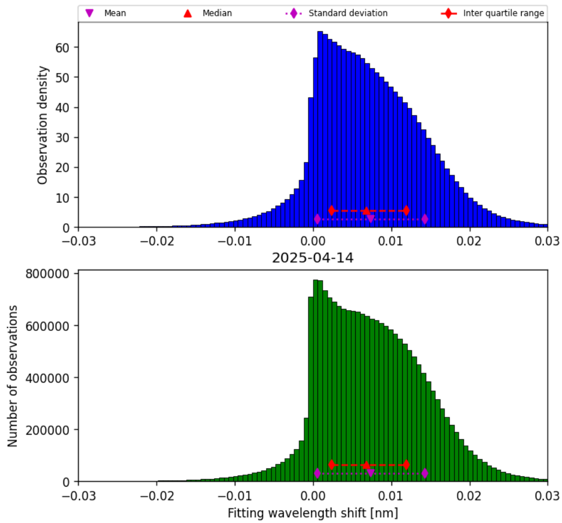
Figure 49: Histogram of “Fitting wavelength shift” for 2025-04-13 to 2025-04-15
