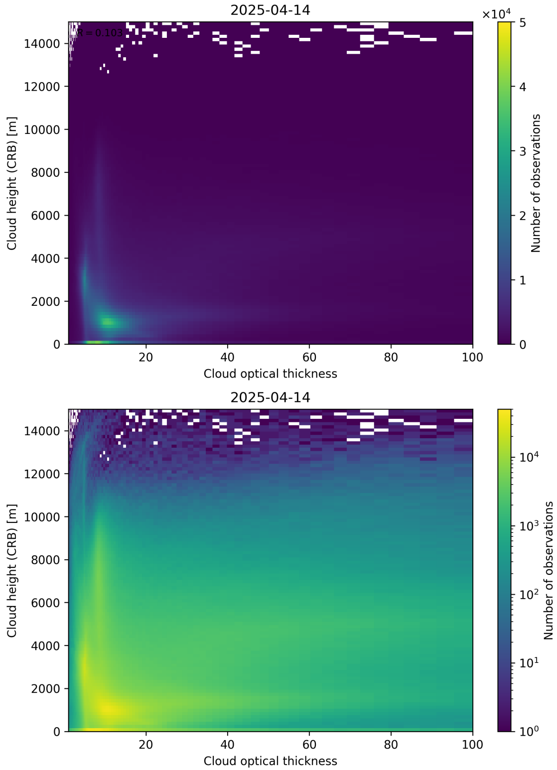
Figure 85: Scatter density plot of “Cloud optical thickness” against “Cloud height (CRB)” for 2025-04-13 to 2025-04-15.
