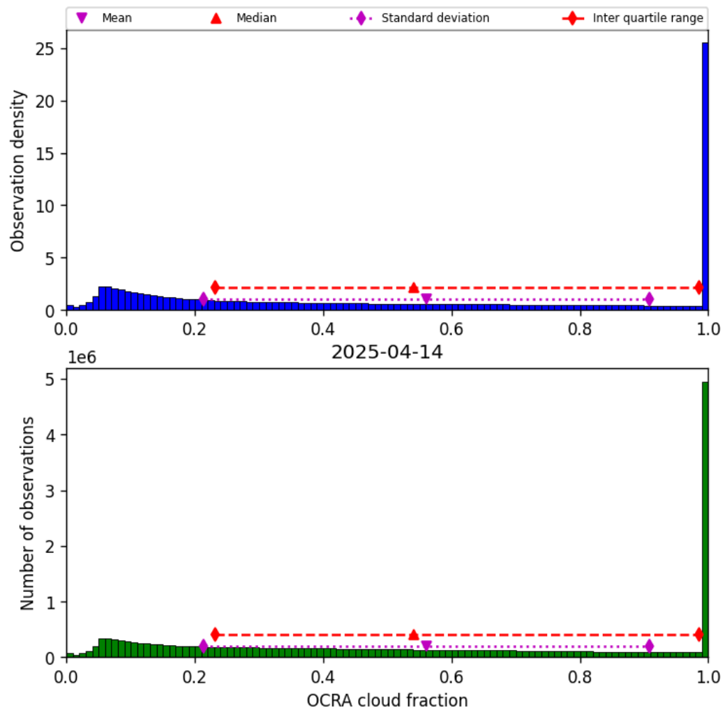
Figure 50: Histogram of “OCRA cloud fraction” for 2025-04-13 to 2025-04-15
