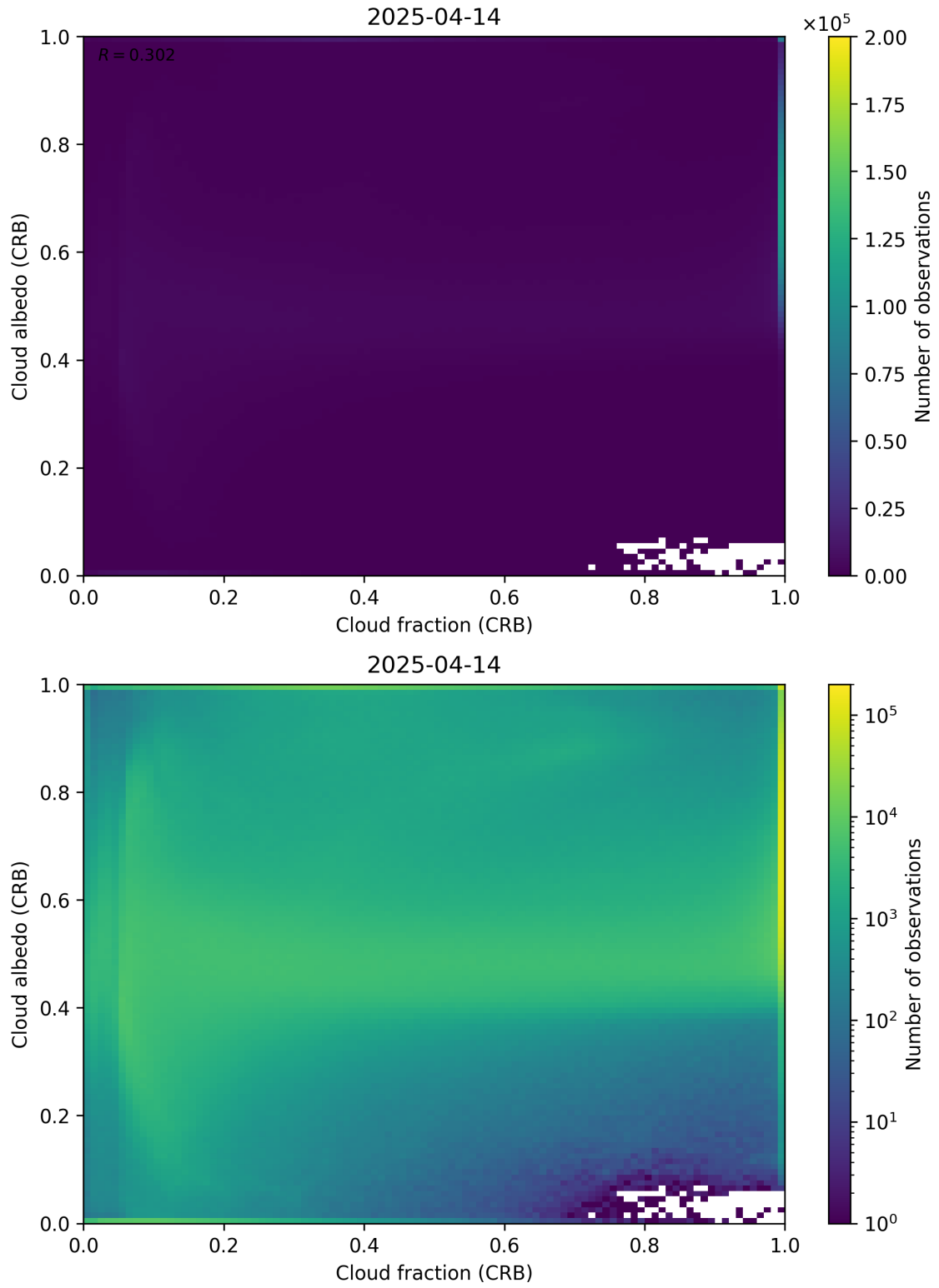
Figure 77: Scatter density plot of “Cloud fraction (CRB)” against “Cloud albedo (CRB)” for 2025-04-13 to 2025-04-15.
