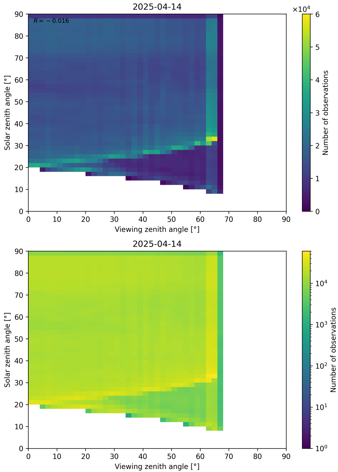
Figure 114: Scatter density plot of “Viewing zenith angle” against “Solar zenith angle” for 2025-04-13 to 2025-04-15.
