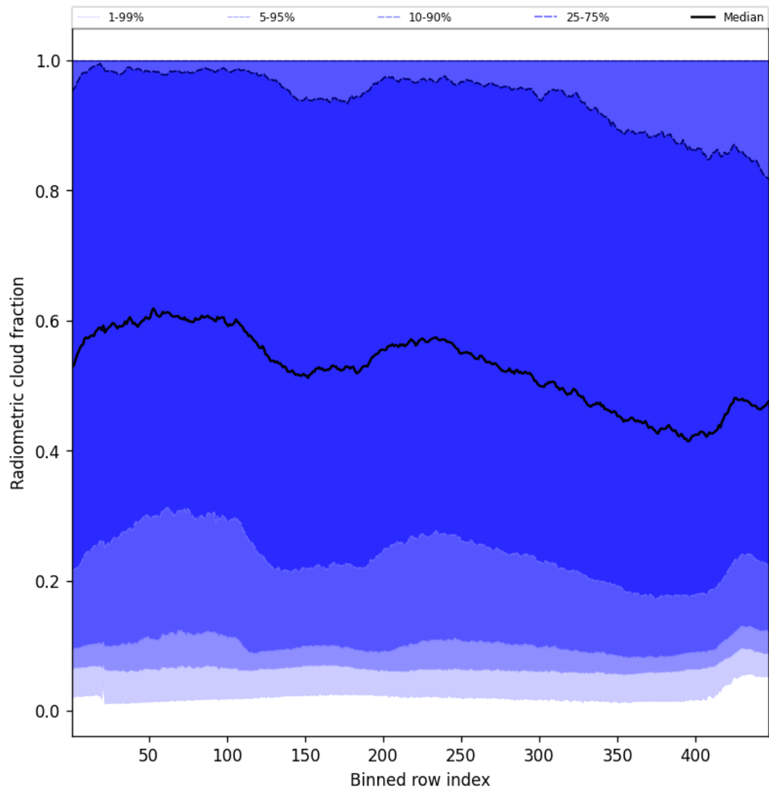
Figure 55: Along track statistics of “Radiometric cloud fraction” for 2025-04-13 to 2025-04-15
