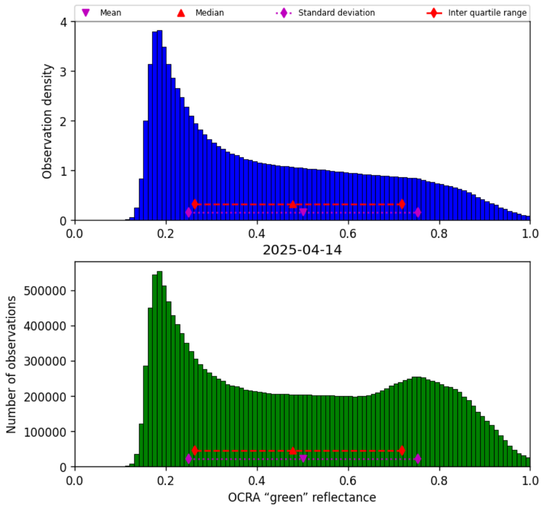
Figure 52: Histogram of “OCRA “green” reflectance” for 2025-04-13 to 2025-04-15
