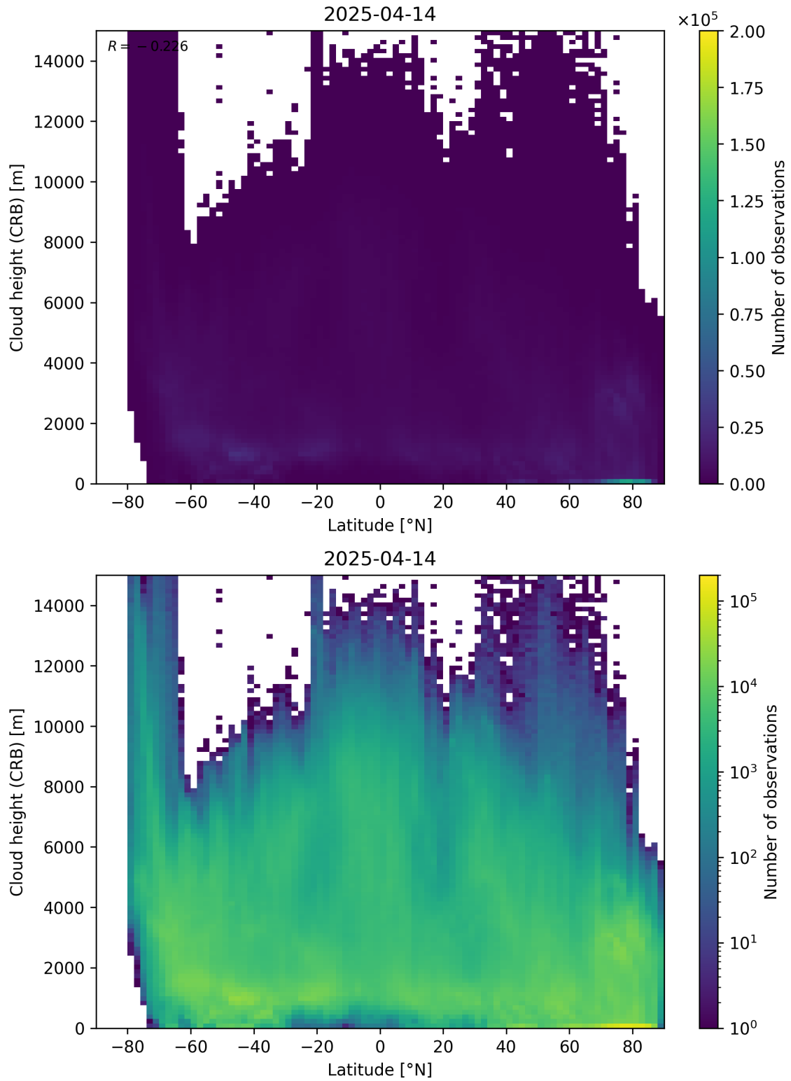
Figure 95: Scatter density plot of “Latitude” against “Cloud height (CRB)” for 2025-04-13 to 2025-04-15.
