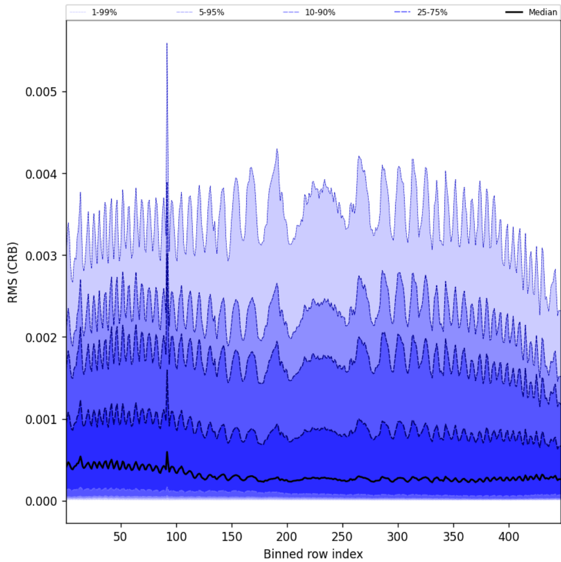
Figure 64: Along track statistics of “RMS (CRB)” for 2025-04-13 to 2025-04-15
