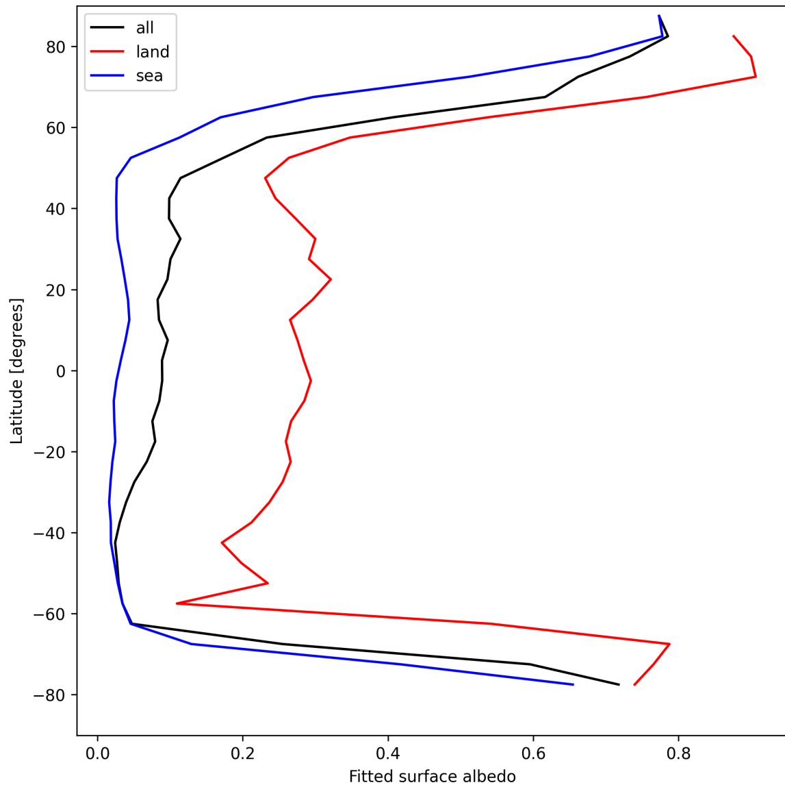
Figure 29: Zonal average of “Fitted surface albedo” for 2025-04-13 to 2025-04-15.
