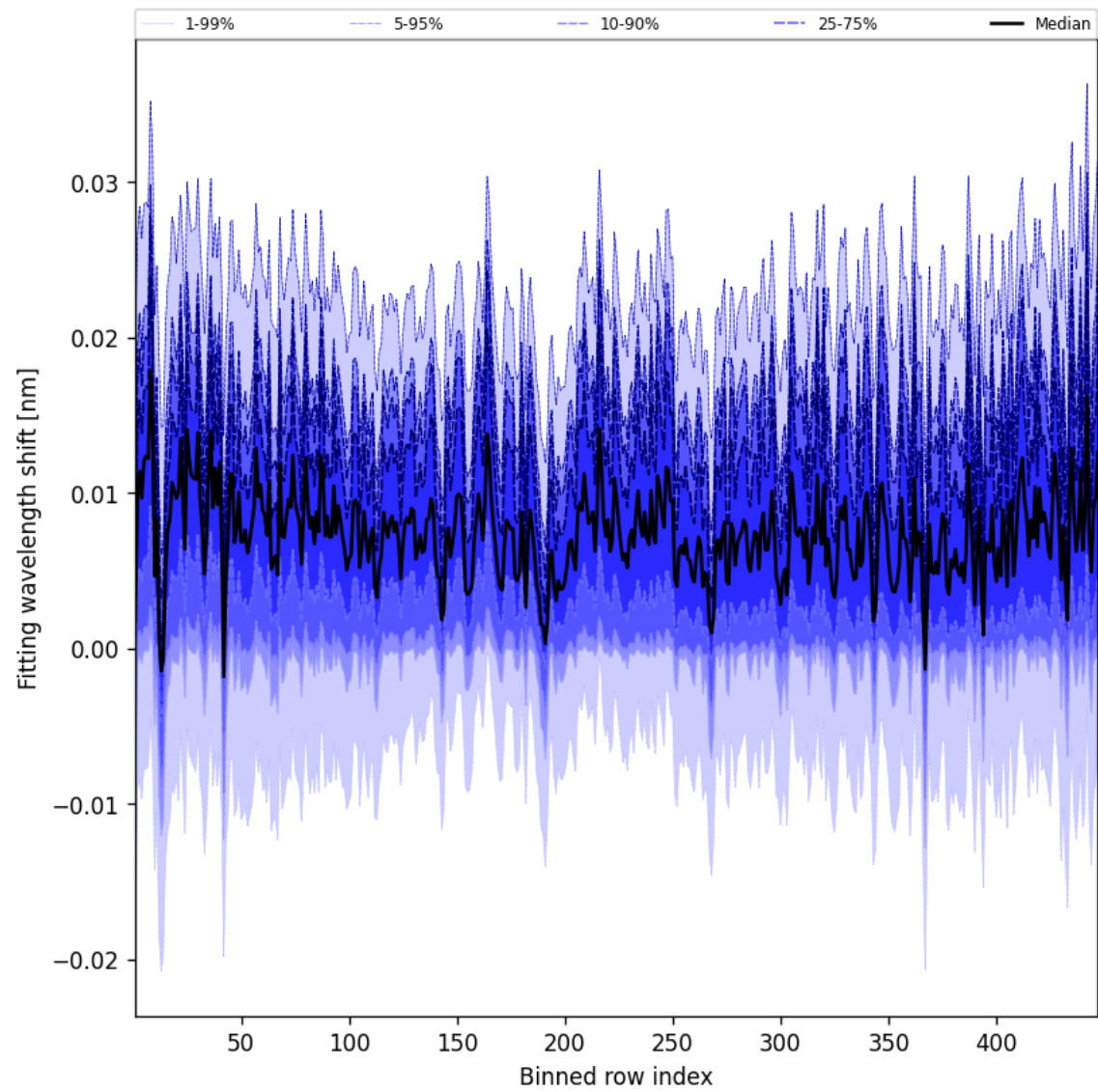
Figure 65: Along track statistics of “Fitting wavelength shift” for 2025-04-13 to 2025-04-15
