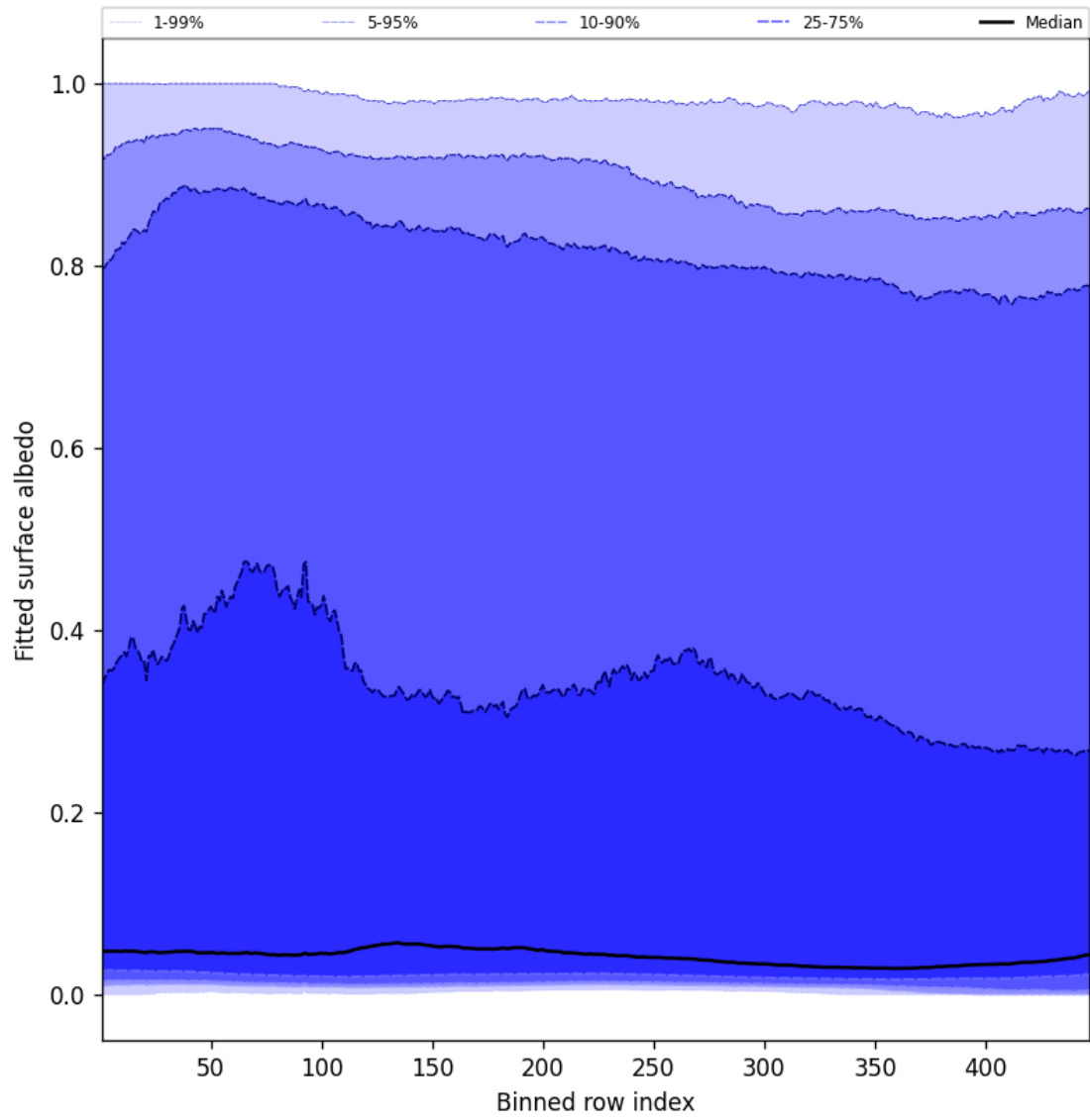
Figure 61: Along track statistics of “Fitted surface albedo” for 2025-04-13 to 2025-04-15
