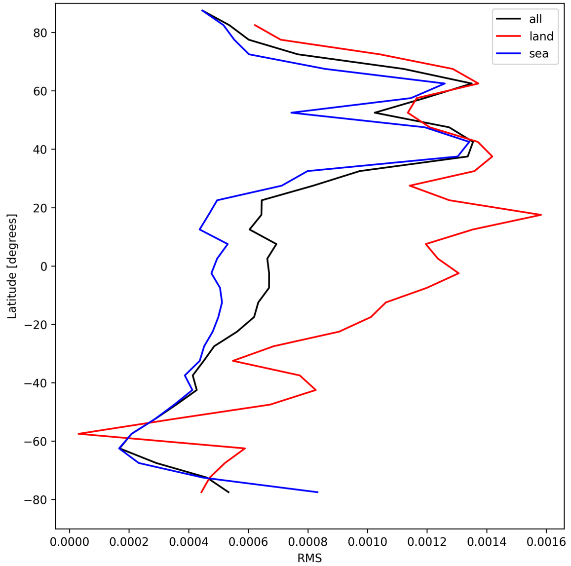
Figure 31: Zonal average of “RMS” for 2025-04-13 to 2025-04-15.
