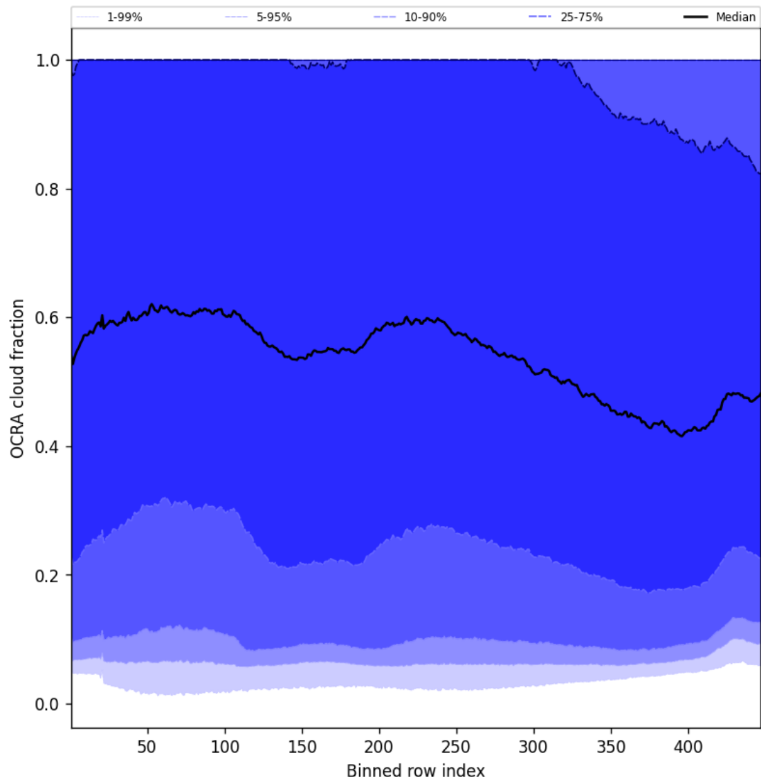
Figure 66: Along track statistics of “OCRA cloud fraction” for 2025-04-13 to 2025-04-15
