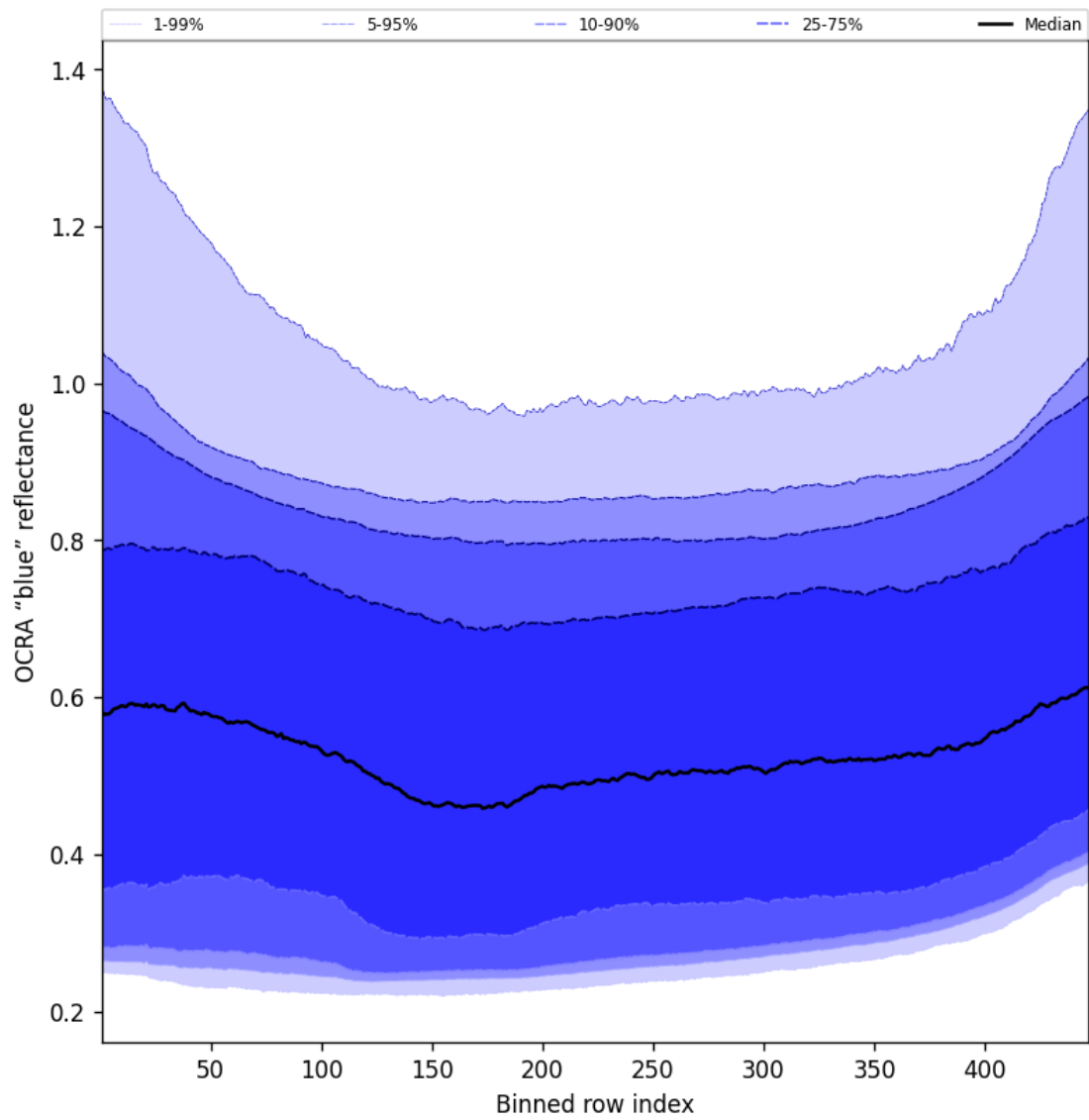
Figure 67: Along track statistics of “OCRA “blue” reflectance” for 2025-04-13 to 2025-04-15
