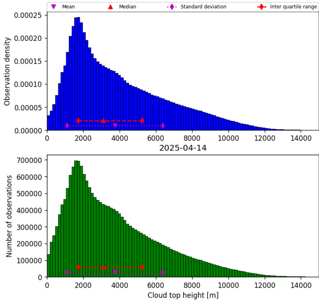
Figure 40: Histogram of “Cloud top height” for 2025-04-13 to 2025-04-15
