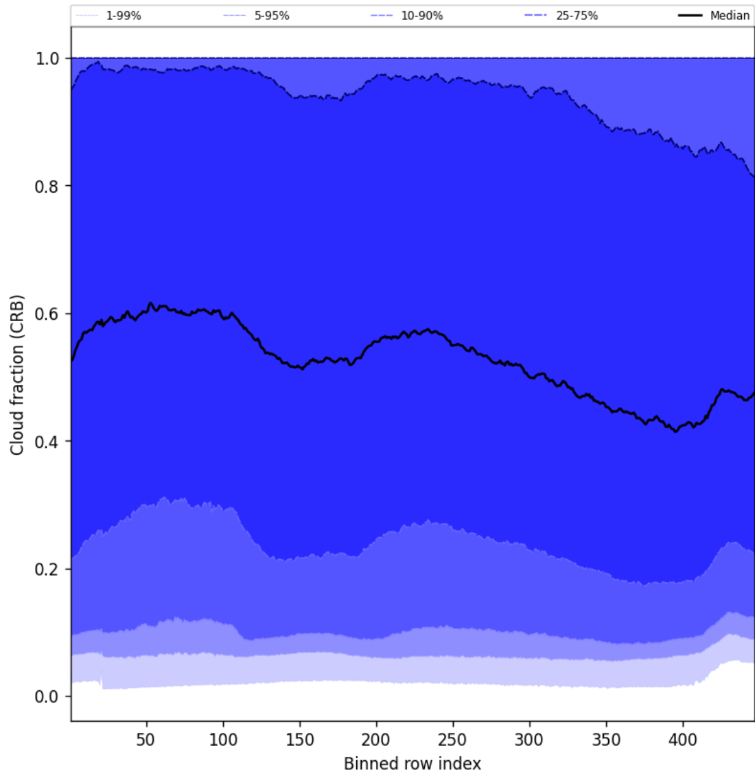
Figure 58: Along track statistics of “Cloud fraction (CRB)” for 2025-04-13 to 2025-04-15
