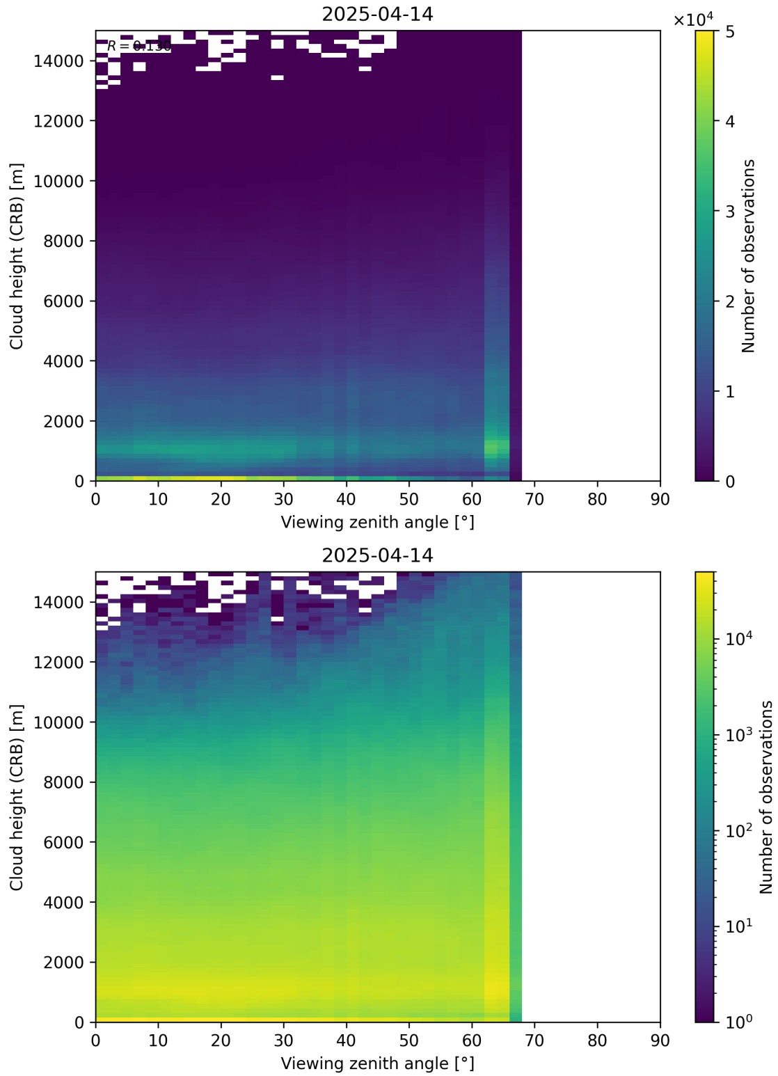
Figure 110: Scatter density plot of “Viewing zenith angle” against “Cloud height (CRB)” for 2025-04-13 to 2025-04-15.
