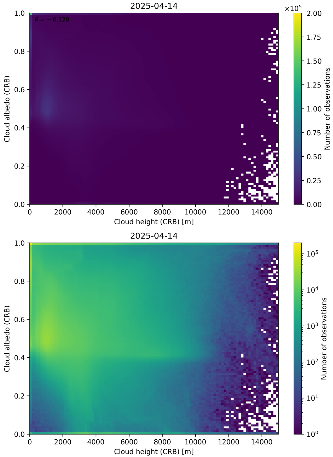
Figure 80: Scatter density plot of “Cloud height (CRB)” against “Cloud albedo (CRB)” for 2025-04-13 to 2025-04-15.
