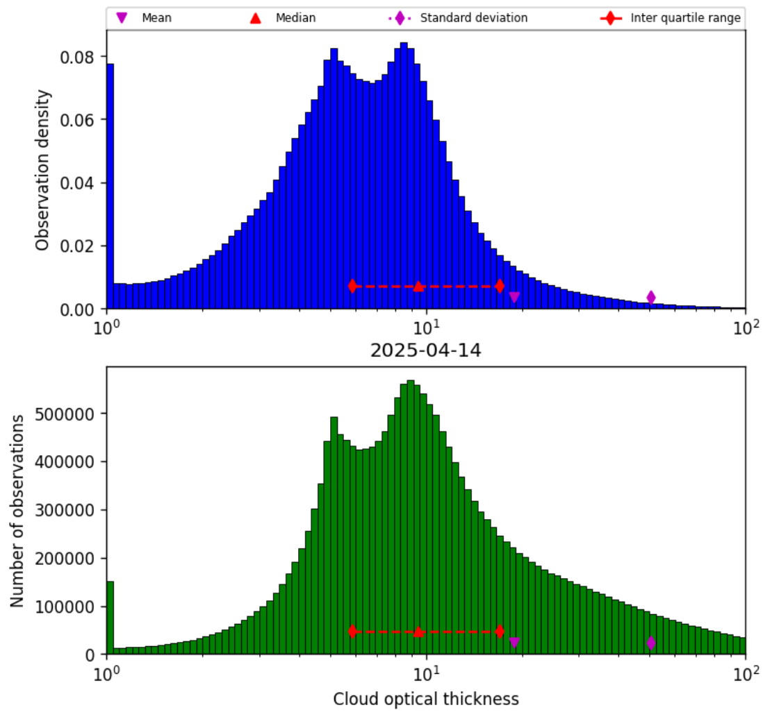
Figure 41: Histogram of “Cloud optical thickness” for 2025-04-13 to 2025-04-15
