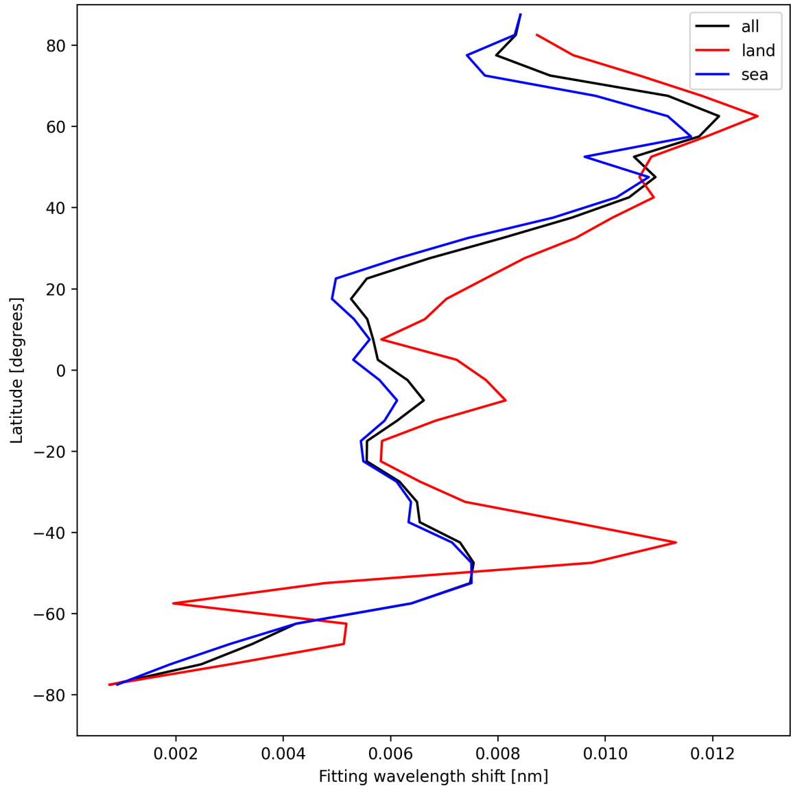
Figure 33: Zonal average of “Fitting wavelength shift” for 2025-04-13 to 2025-04-15.
