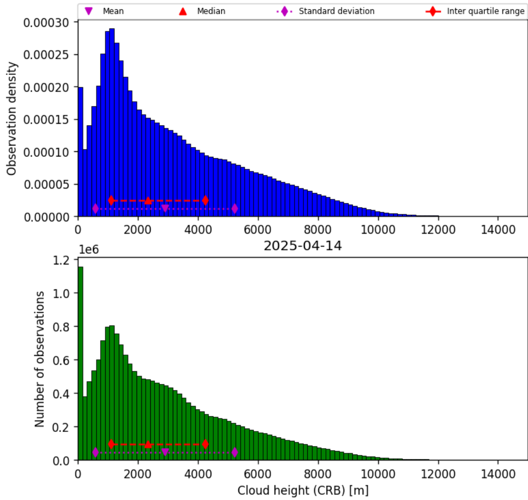
Figure 43: Histogram of “Cloud height (CRB)” for 2025-04-13 to 2025-04-15
