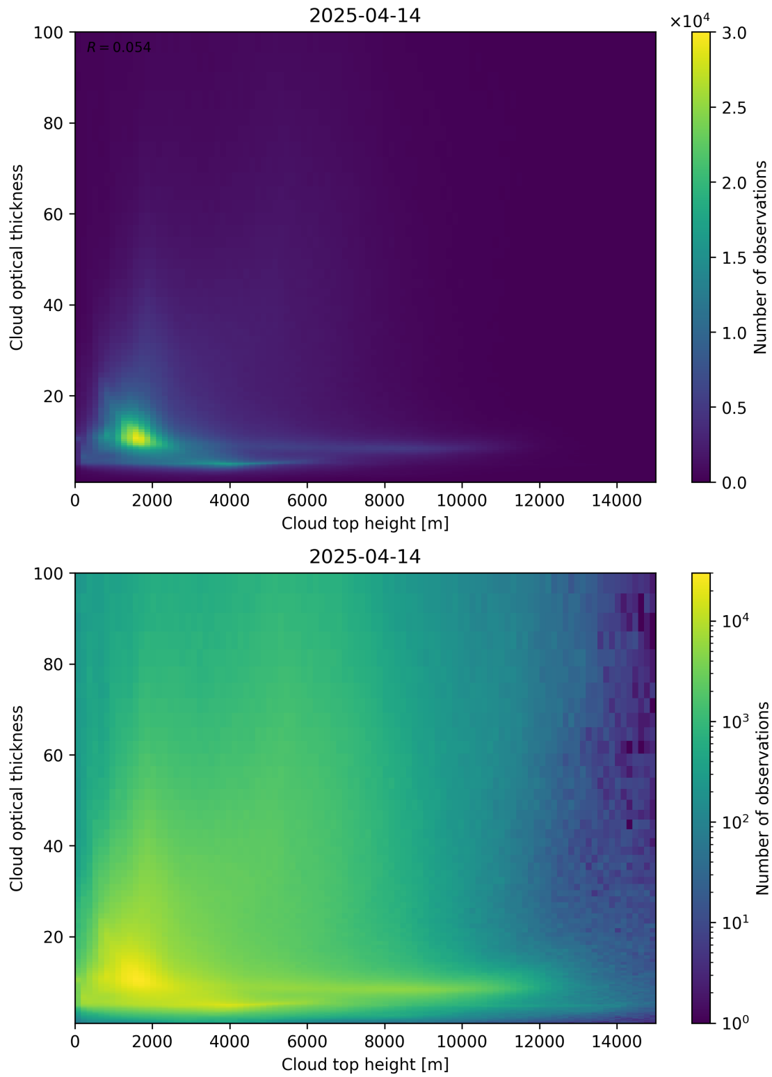
Figure 90: Scatter density plot of “Cloud top height” against “Cloud optical thickness” for 2025-04-13 to 2025-04-15.
