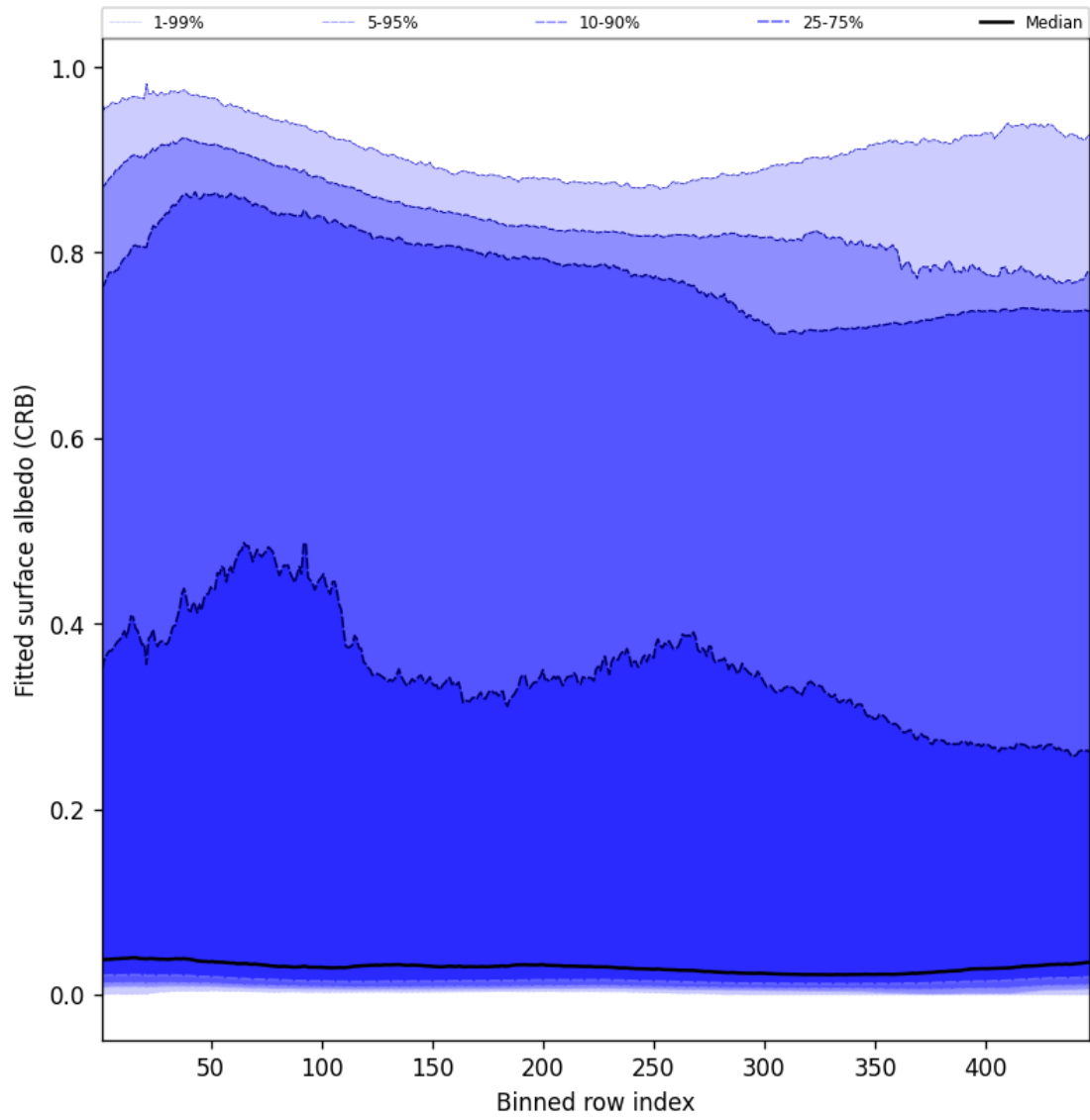
Figure 62: Along track statistics of “Fitted surface albedo (CRB)” for 2025-04-13 to 2025-04-15
