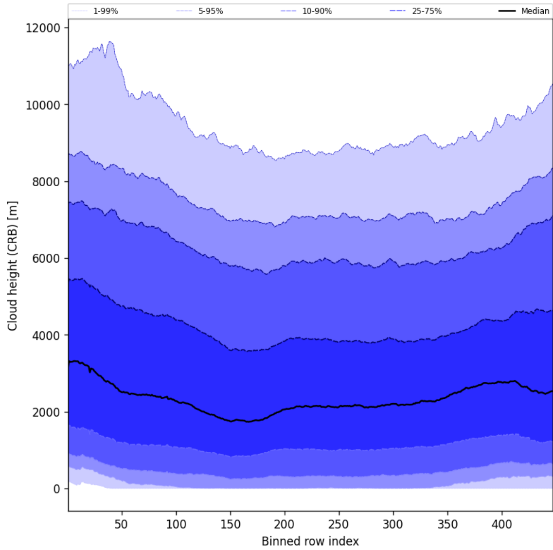
Figure 59: Along track statistics of “Cloud height (CRB)” for 2025-04-13 to 2025-04-15
