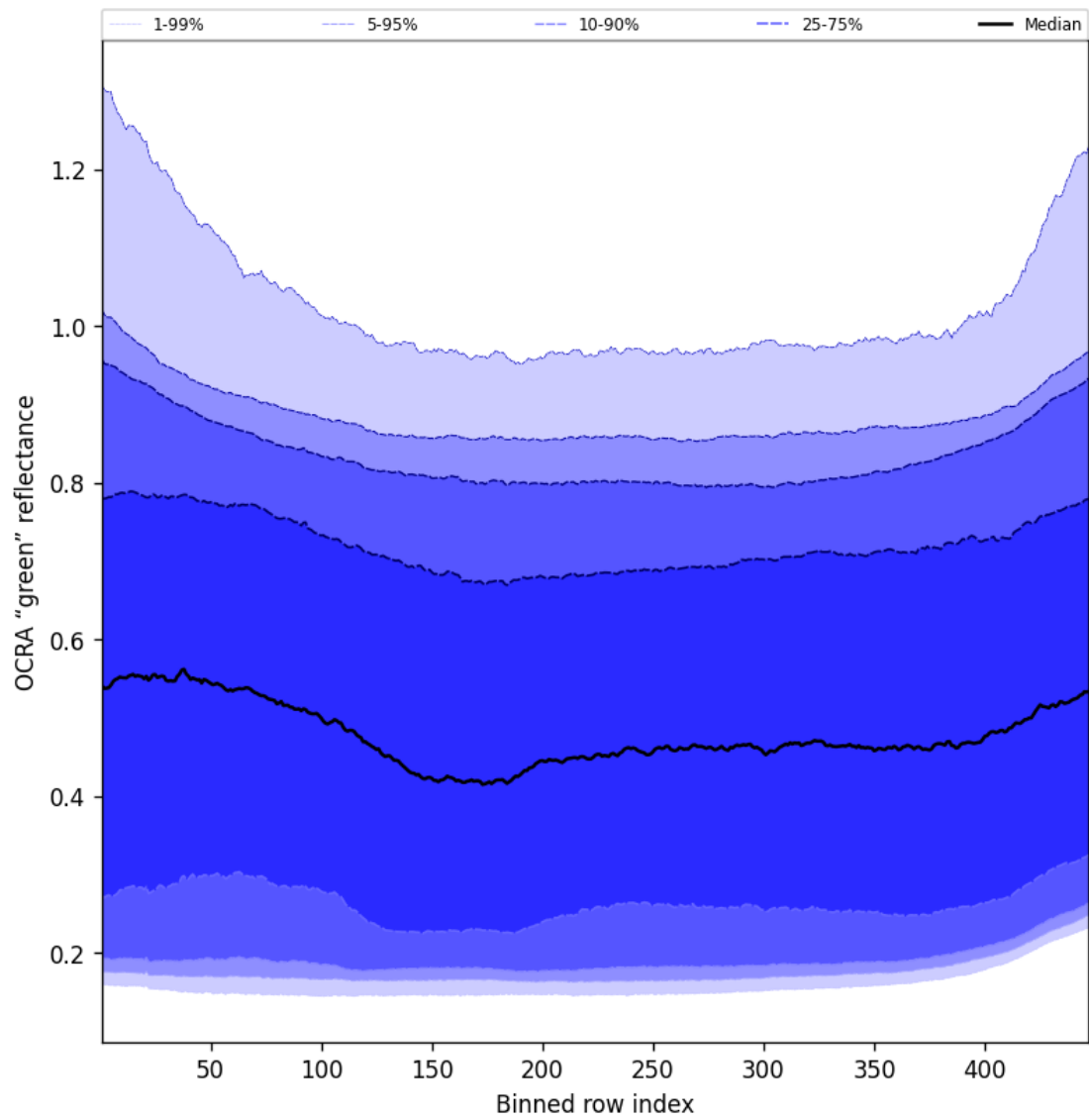
Figure 68: Along track statistics of “OCRA “green” reflectance” for 2025-04-13 to 2025-04-15
