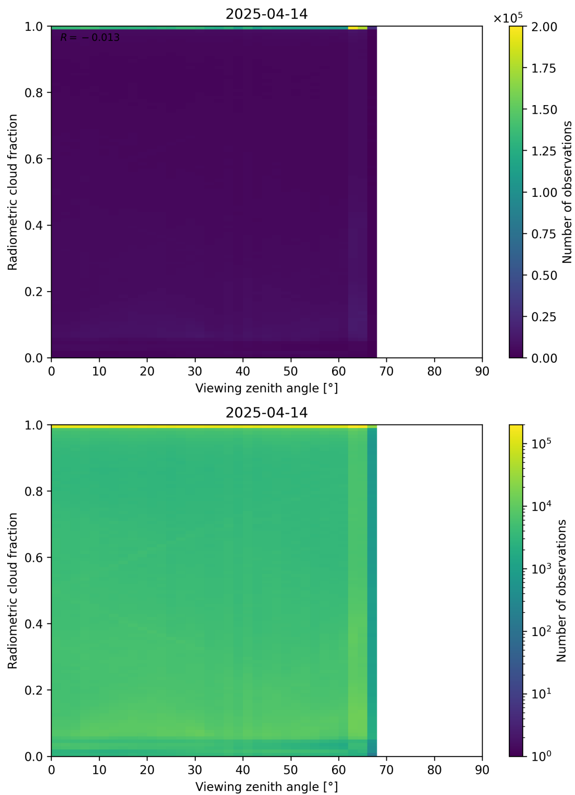
Figure 107: Scatter density plot of “Viewing zenith angle” against “Radiometric cloud fraction” for 2025-04-13 to 2025-04-15.
