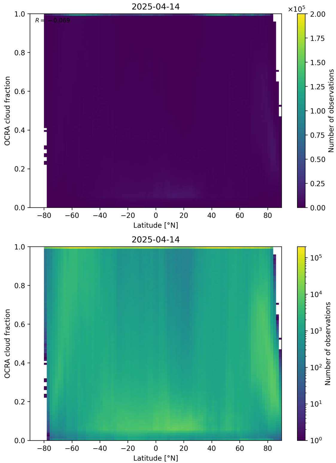
Figure 93: Scatter density plot of “Latitude” against “OCRA cloud fraction” for 2025-04-13 to 2025-04-15.
