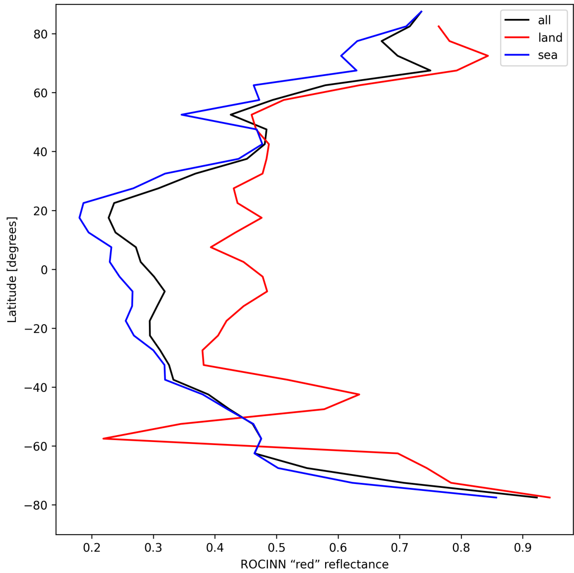
Figure 37: Zonal average of “ROCINN “red” reflectance” for 2025-04-13 to 2025-04-15.
