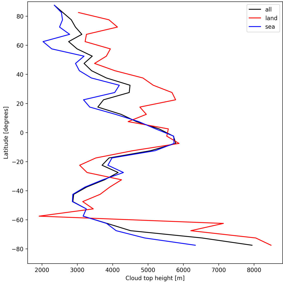
Figure 24: Zonal average of “Cloud top height” for 2025-04-13 to 2025-04-15.
