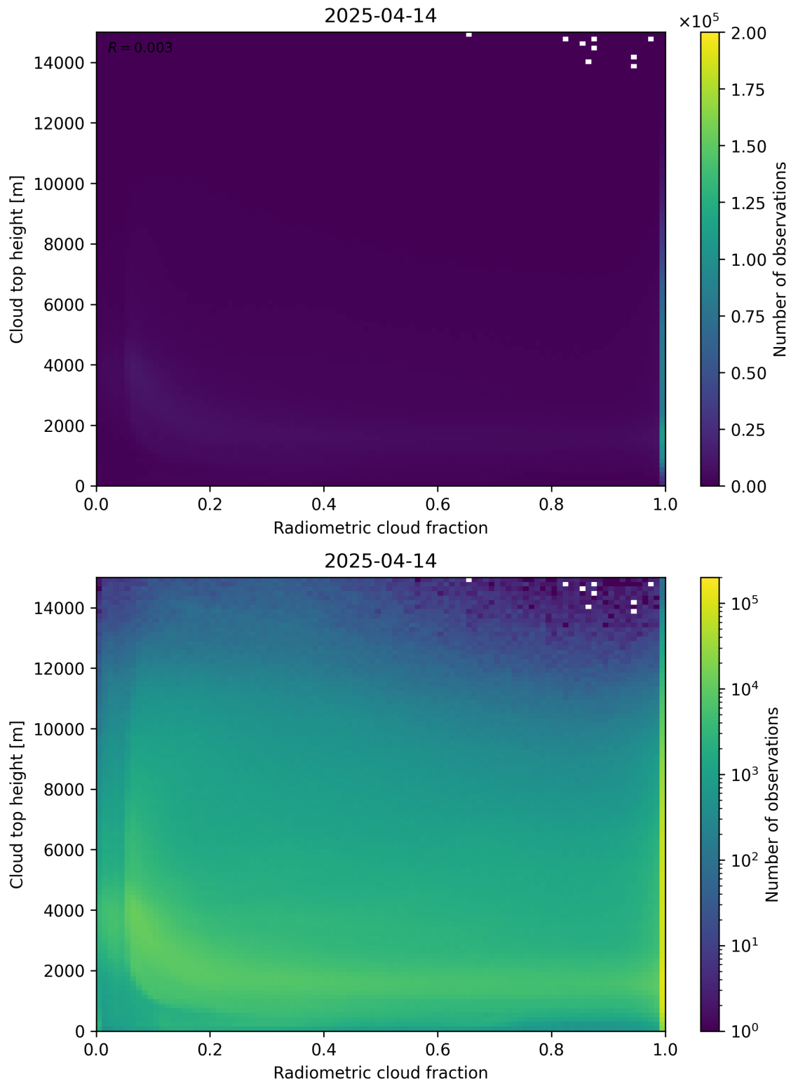
Figure 76: Scatter density plot of “Radiometric cloud fraction” against “Cloud top height” for 2025-04-13 to 2025-04-15.
