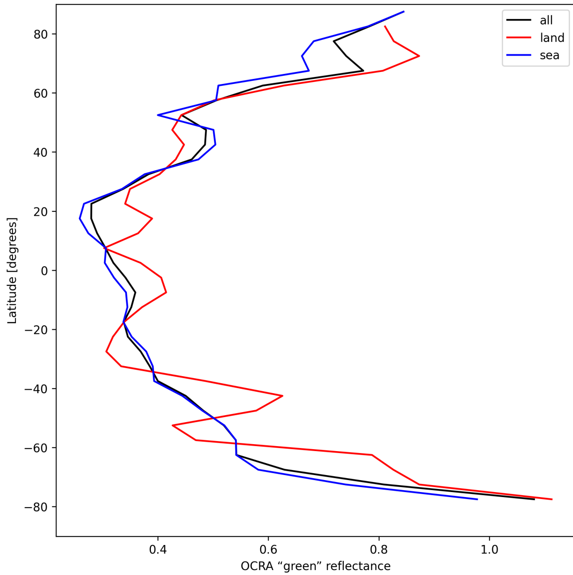
Figure 36: Zonal average of “OCRA “green” reflectance” for 2025-04-13 to 2025-04-15.
