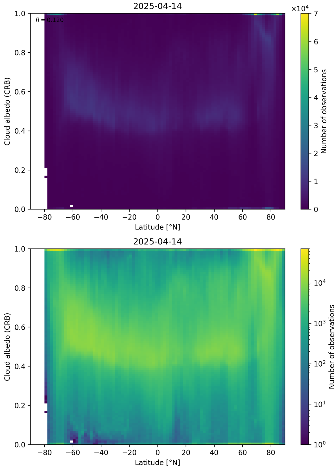
Figure 91: Scatter density plot of “Latitude” against “Cloud albedo (CRB)” for 2025-04-13 to 2025-04-15.
