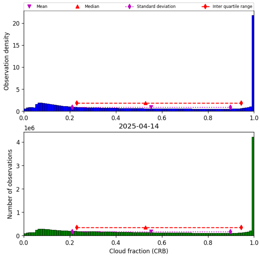
Figure 42: Histogram of “Cloud fraction (CRB)” for 2025-04-13 to 2025-04-15
