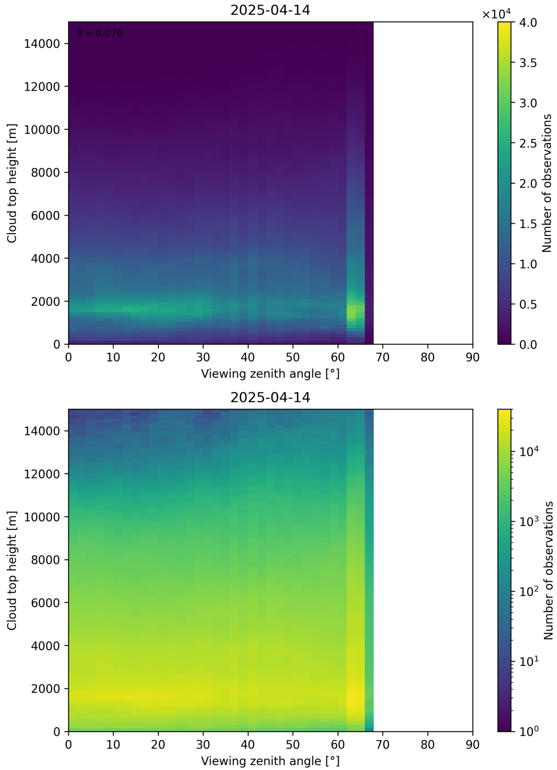
Figure 112: Scatter density plot of “Viewing zenith angle” against “Cloud top height” for 2025-04-13 to 2025-04-15.
