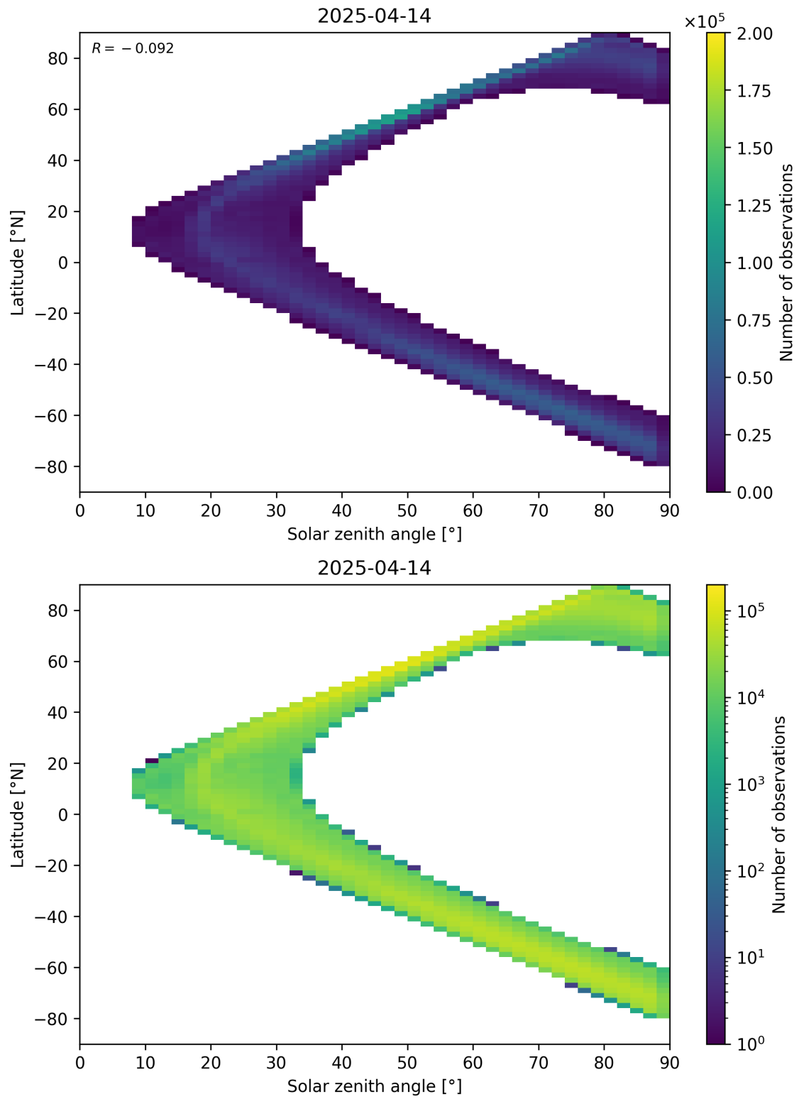
Figure 105: Scatter density plot of “Solar zenith angle” against “Latitude” for 2025-04-13 to 2025-04-15.
