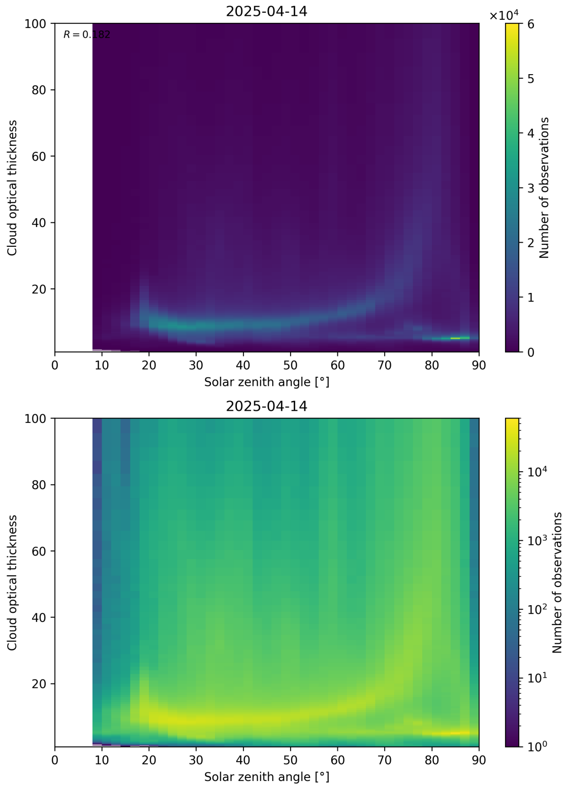
Figure 103: Scatter density plot of “Solar zenith angle” against “Cloud optical thickness” for 2025-04-13 to 2025-04-15.
