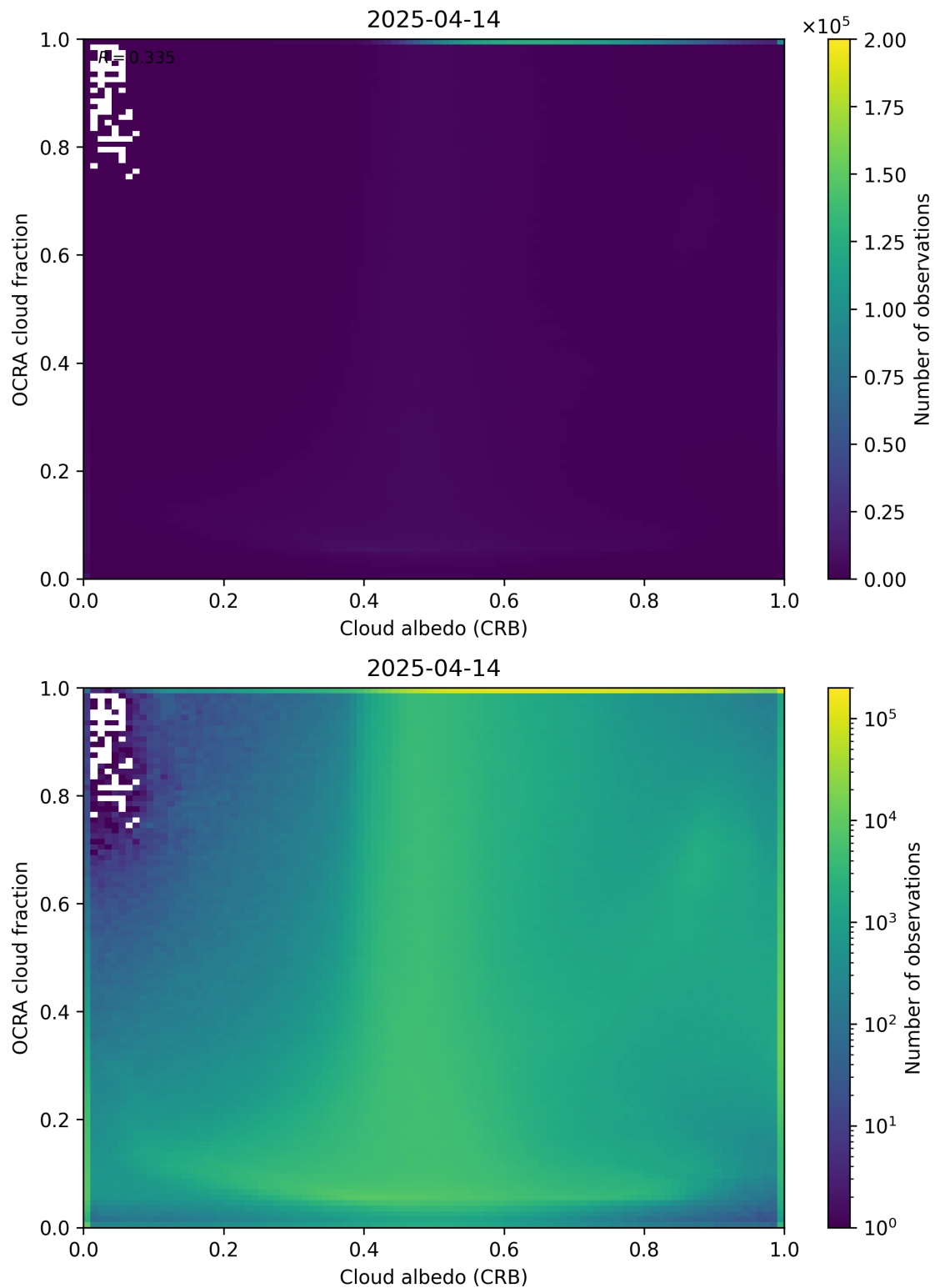
Figure 70: Scatter density plot of “Cloud albedo (CRB)” against “OCRA cloud fraction” for 2025-04-13 to 2025-04-15.
