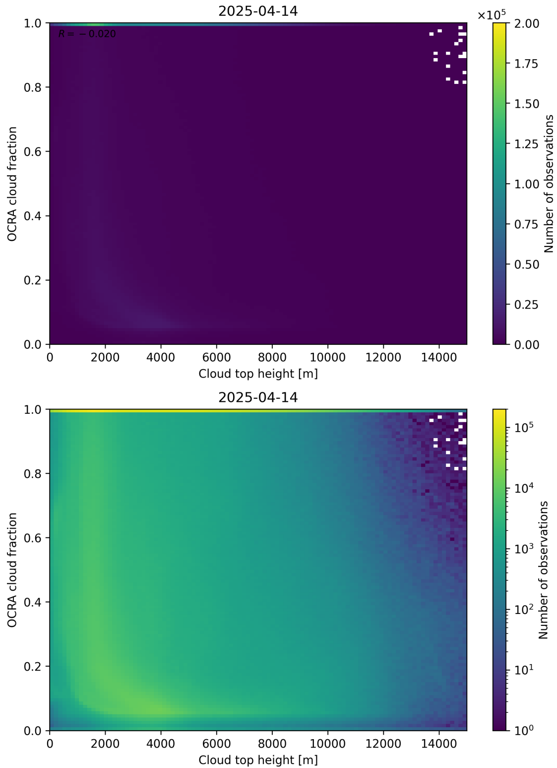
Figure 87: Scatter density plot of “Cloud top height” against “OCRA cloud fraction” for 2025-04-13 to 2025-04-15.
