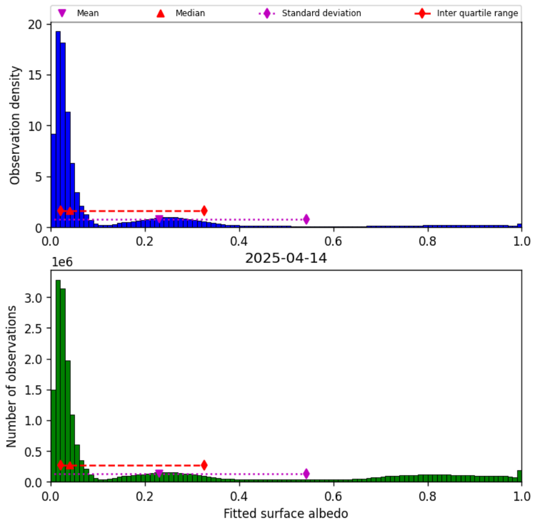
Figure 45: Histogram of “Fitted surface albedo” for 2025-04-13 to 2025-04-15
