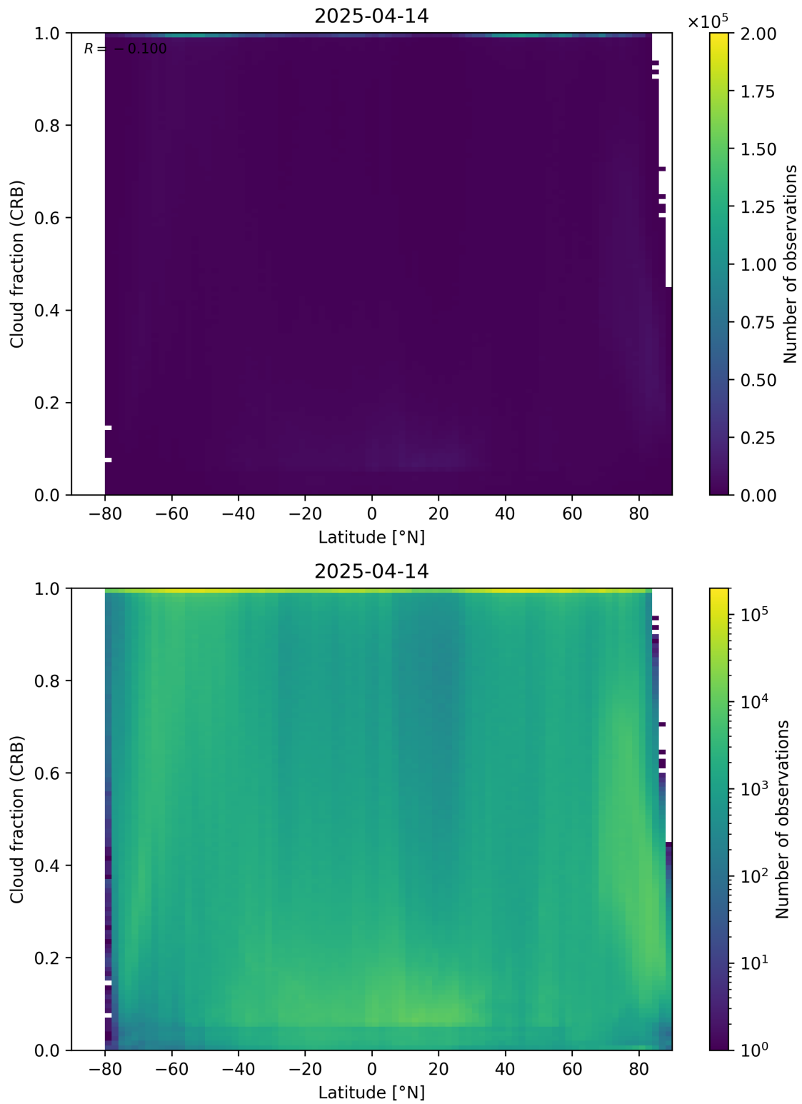
Figure 94: Scatter density plot of “Latitude” against “Cloud fraction (CRB)” for 2025-04-13 to 2025-04-15.
