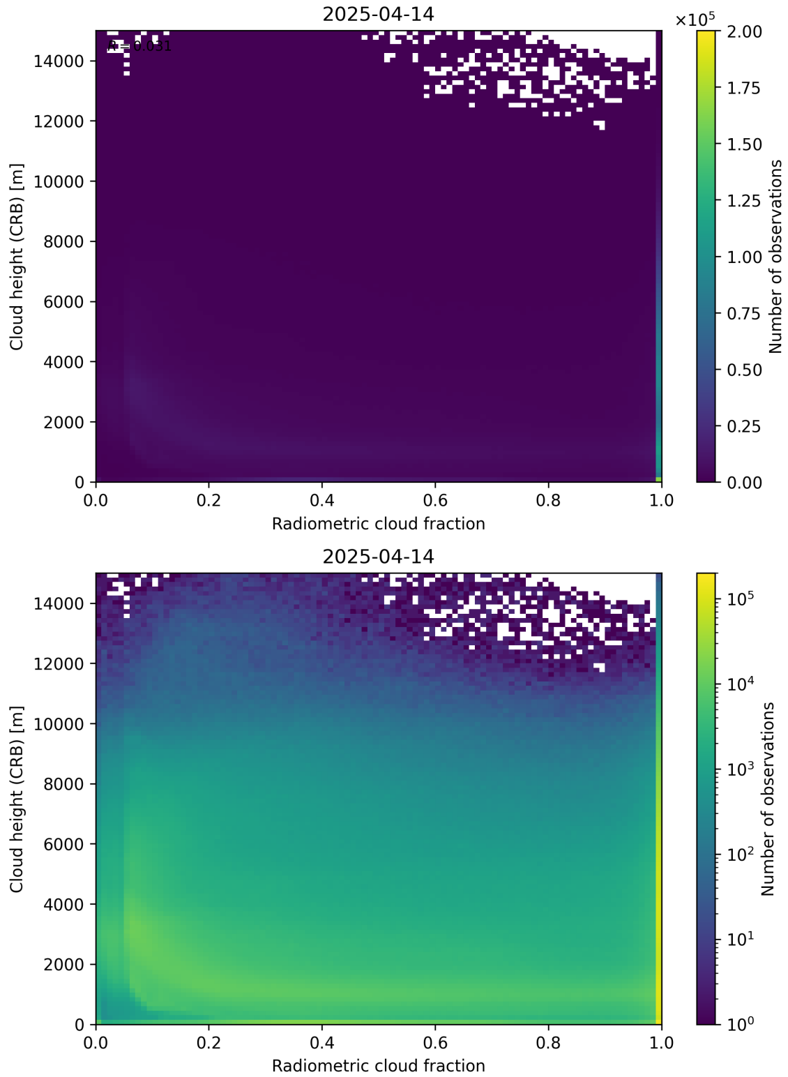
Figure 74: Scatter density plot of “Radiometric cloud fraction” against “Cloud height (CRB)” for 2025-04-13 to 2025-04-15.
