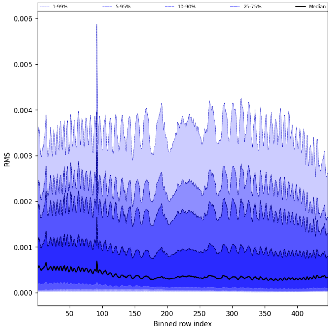
Figure 63: Along track statistics of “RMS” for 2025-04-13 to 2025-04-15
