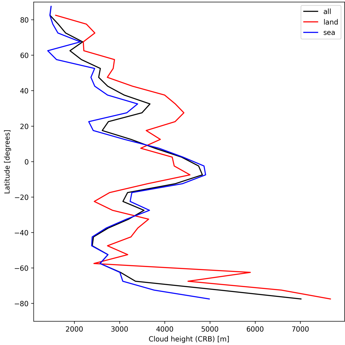
Figure 27: Zonal average of “Cloud height (CRB)” for 2025-04-13 to 2025-04-15.
