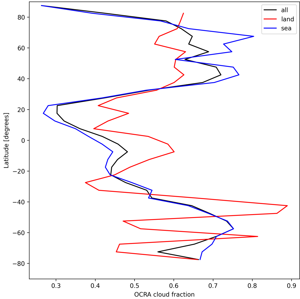
Figure 34: Zonal average of “OCRA cloud fraction” for 2025-04-13 to 2025-04-15.
