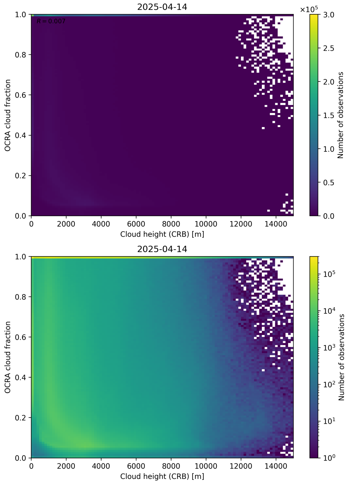
Figure 81: Scatter density plot of “Cloud height (CRB)” against “OCRA cloud fraction” for 2025-04-13 to 2025-04-15.
