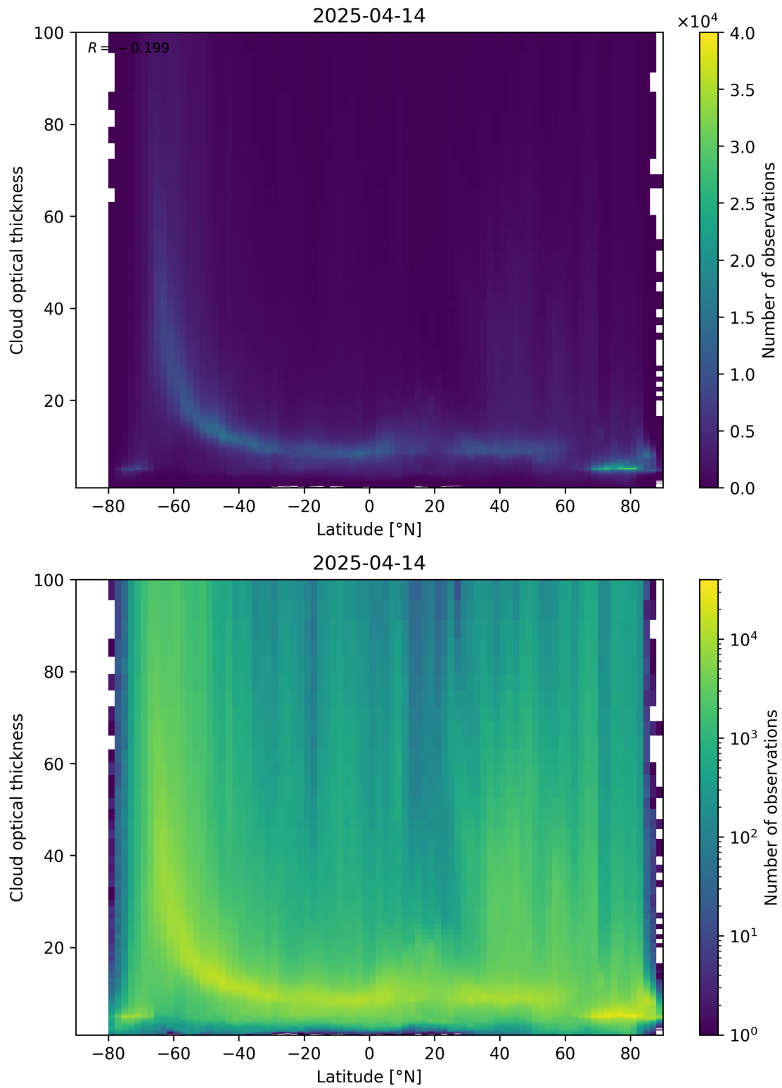
Figure 96: Scatter density plot of “Latitude” against “Cloud optical thickness” for 2025-04-13 to 2025-04-15.
