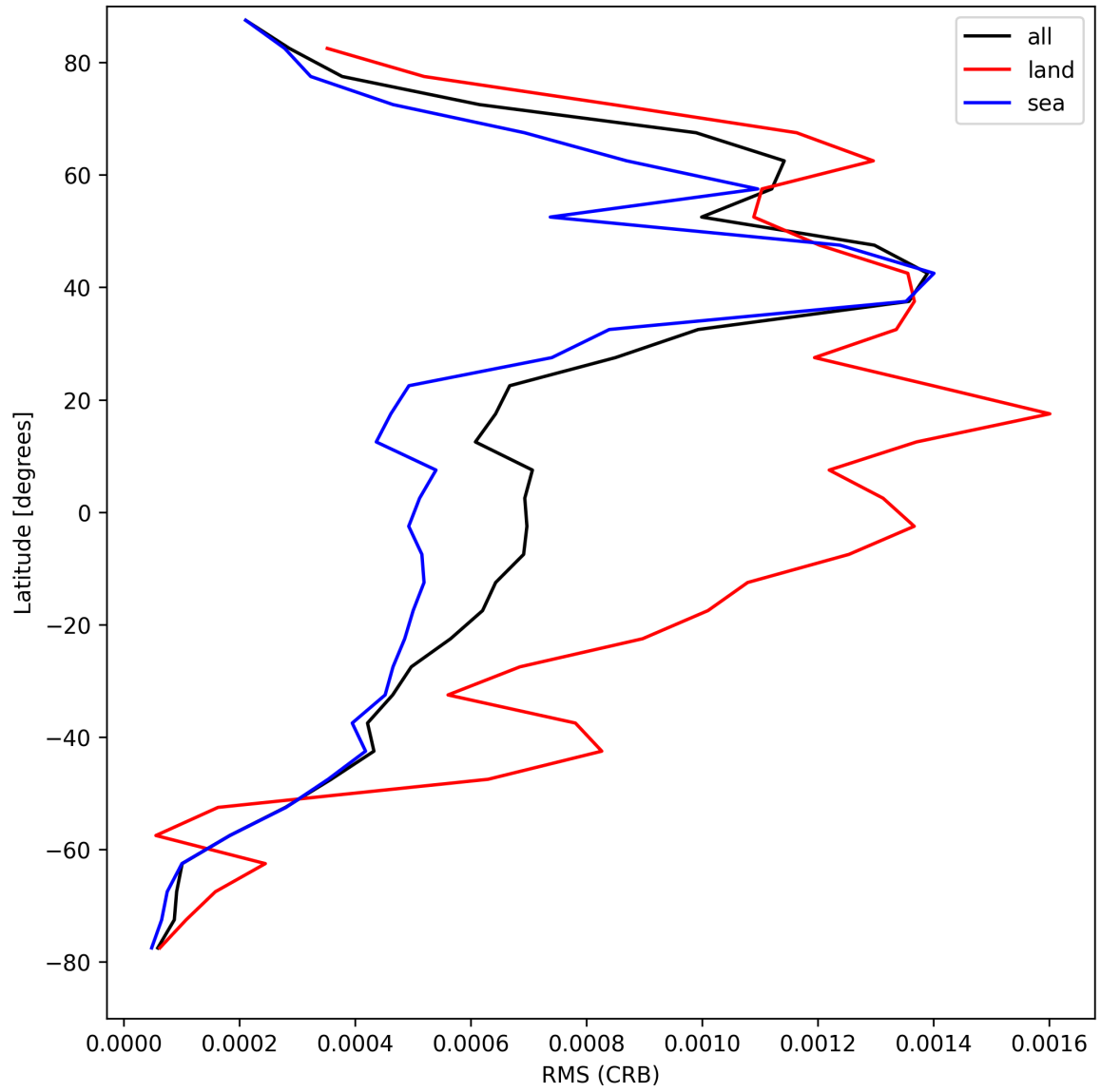
Figure 32: Zonal average of “RMS (CRB)” for 2025-04-13 to 2025-04-15.
