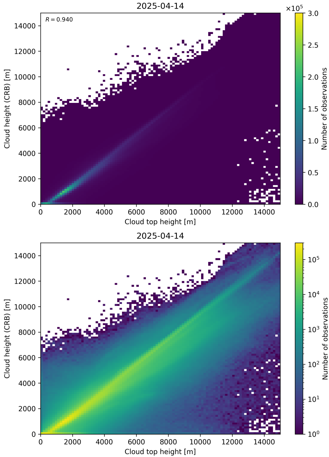
Figure 89: Scatter density plot of “Cloud top height” against “Cloud height (CRB)” for 2025-04-13 to 2025-04-15.
