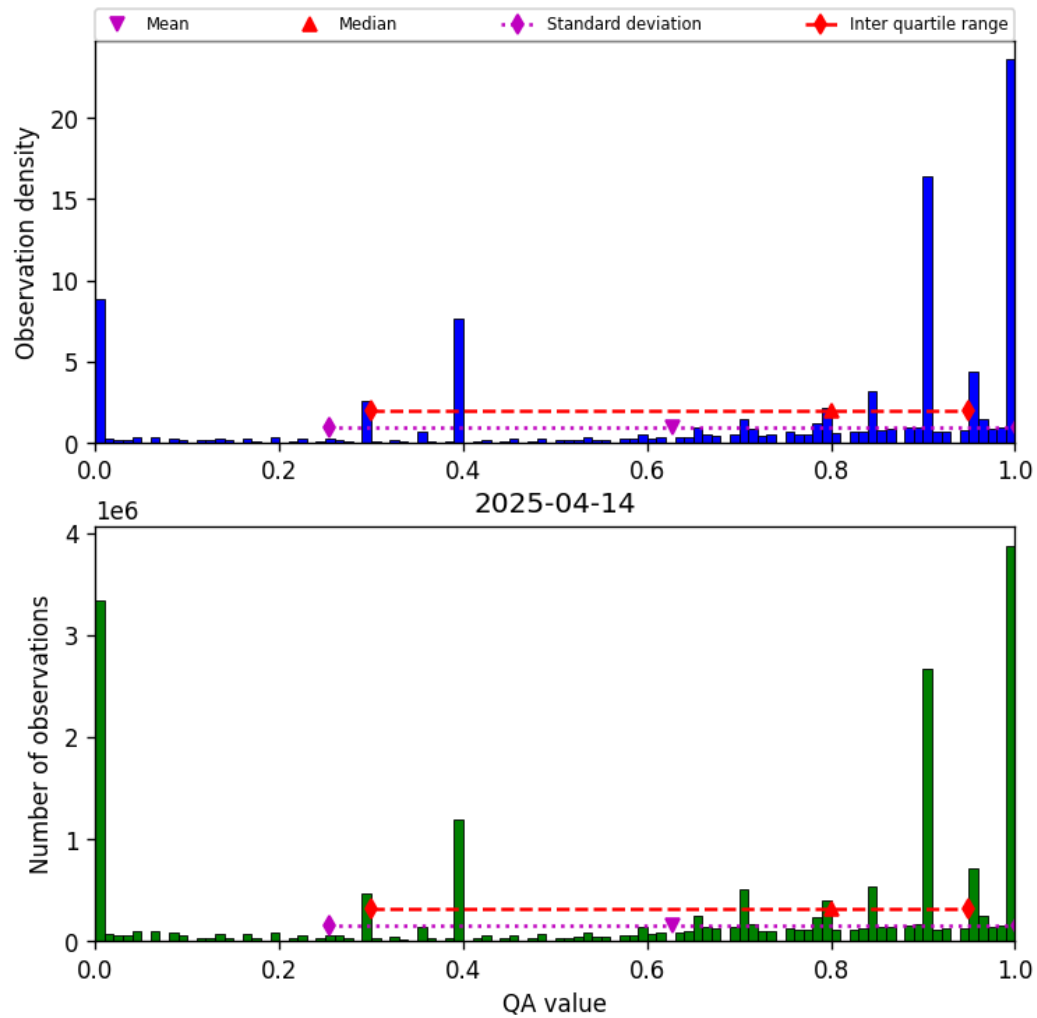
Figure 38: Histogram of “QA value” for 2025-04-13 to 2025-04-15
