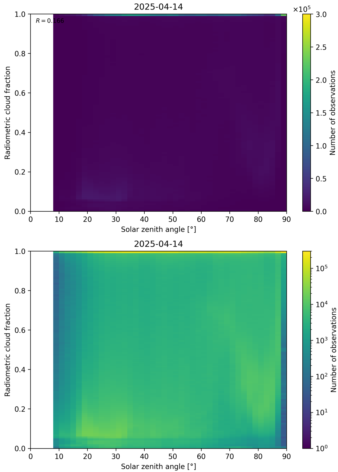
Figure 99: Scatter density plot of “Solar zenith angle” against “Radiometric cloud fraction” for 2025-04-13 to 2025-04-15.
