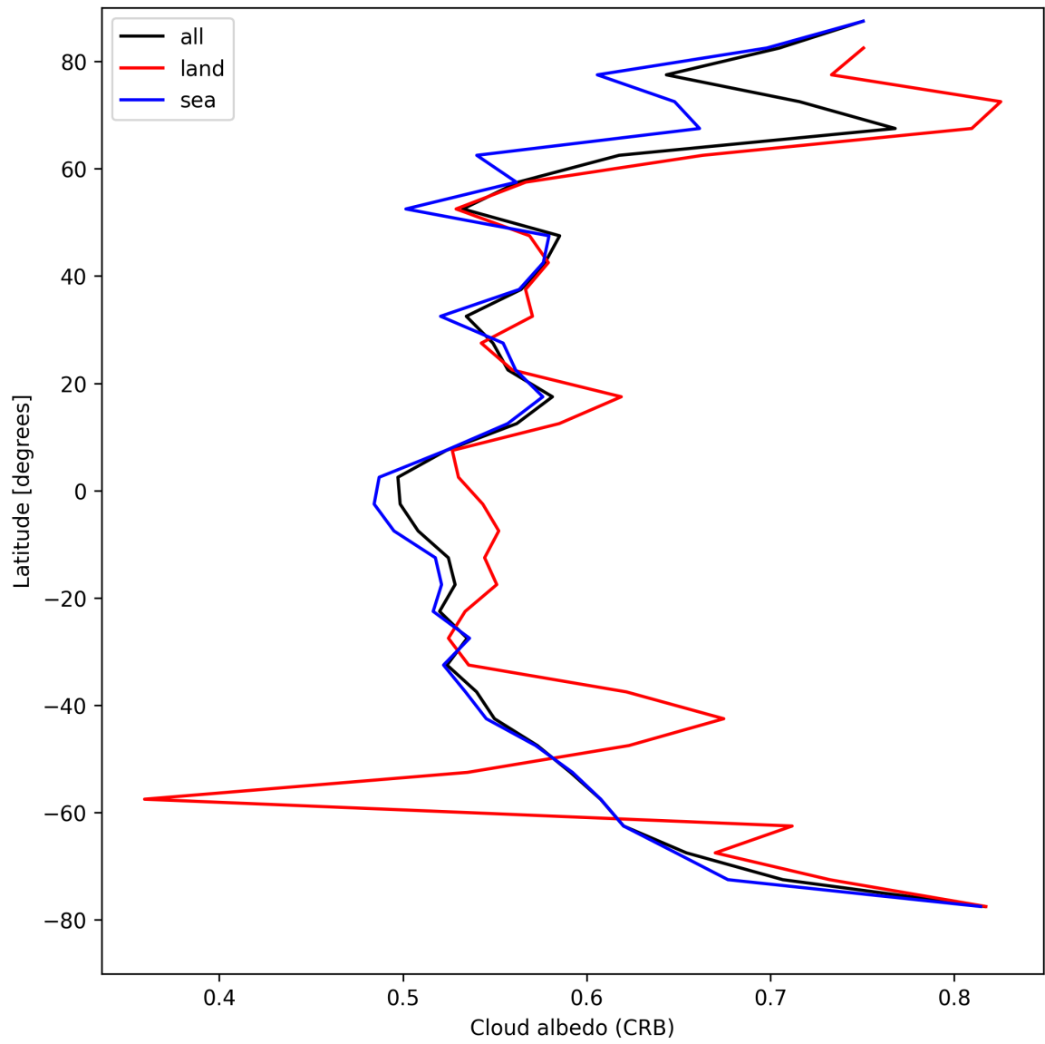
Figure 28: Zonal average of “Cloud albedo (CRB)” for 2025-04-13 to 2025-04-15.
