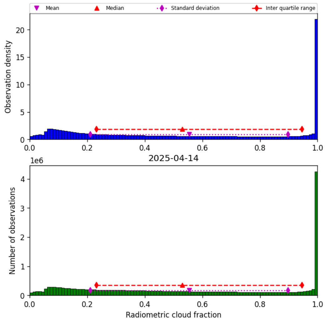
Figure 39: Histogram of “Radiometric cloud fraction” for 2025-04-13 to 2025-04-15
