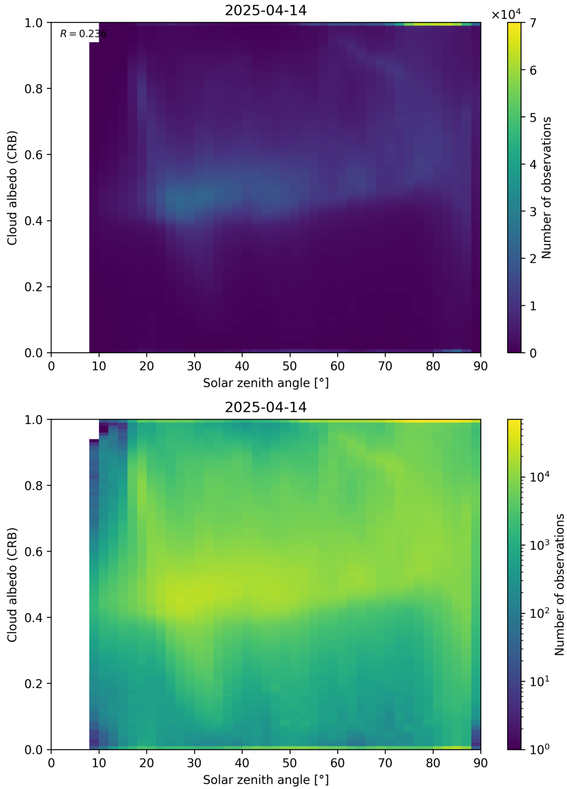
Figure 98: Scatter density plot of “Solar zenith angle” against “Cloud albedo (CRB)” for 2025-04-13 to 2025-04-15.
