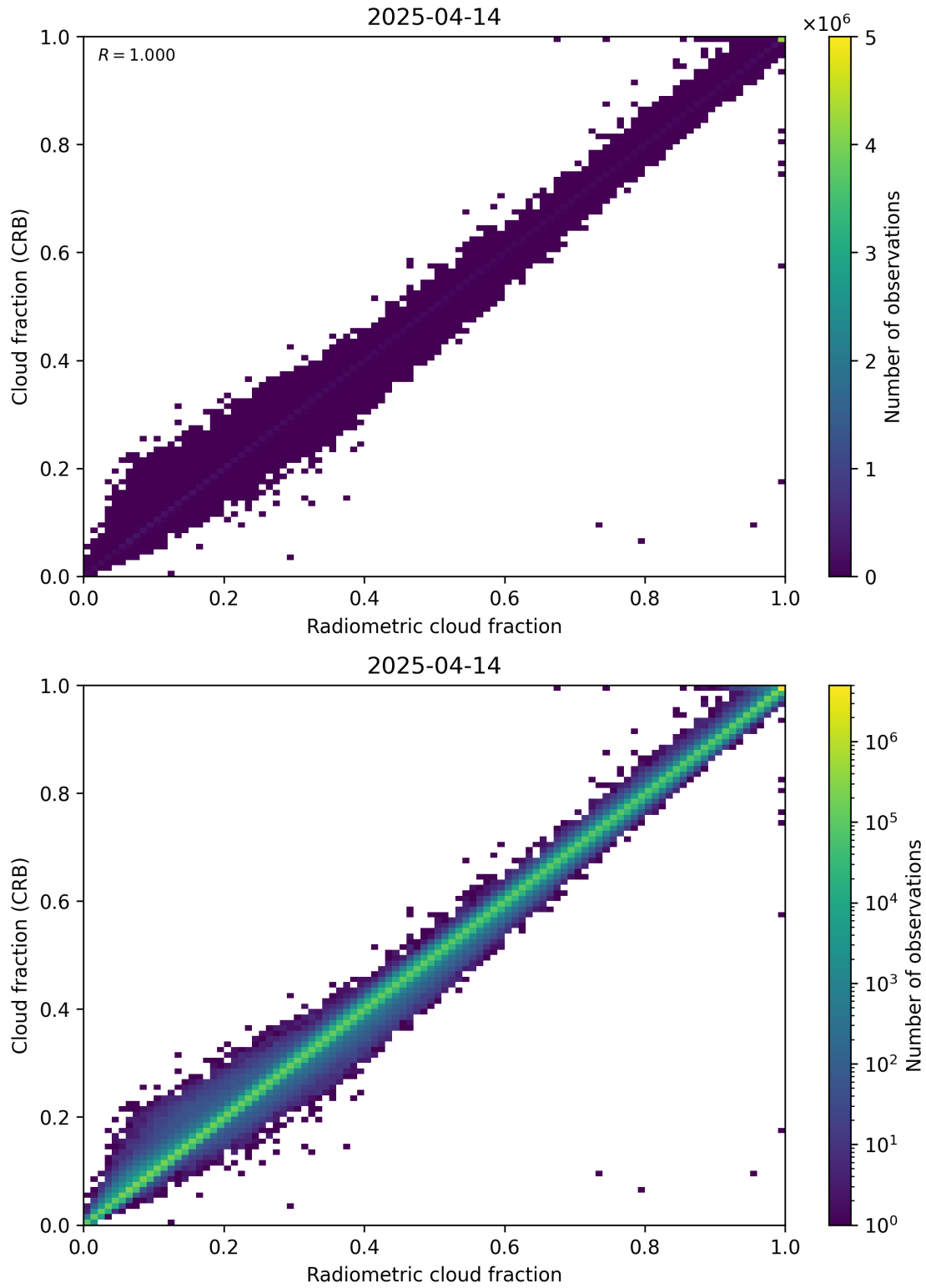
Figure 73: Scatter density plot of “Radiometric cloud fraction” against “Cloud fraction (CRB)” for 2025-04-13 to 2025-04-15.
