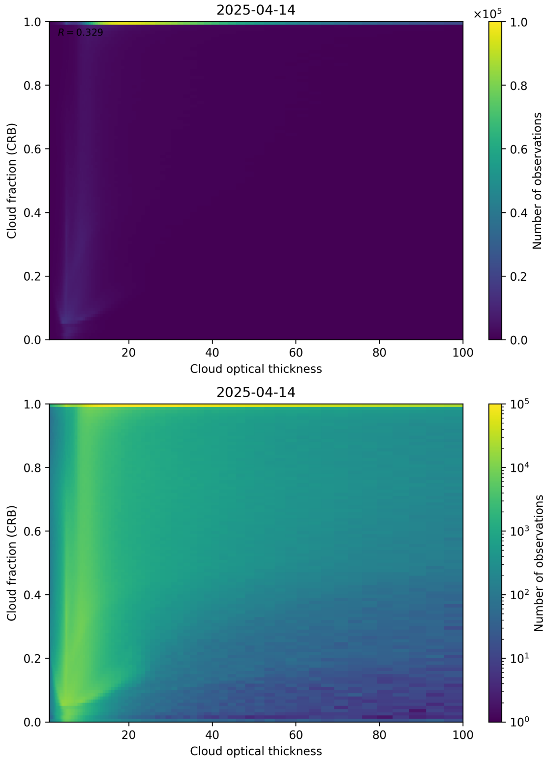
Figure 84: Scatter density plot of “Cloud optical thickness” against “Cloud fraction (CRB)” for 2025-04-13 to 2025-04-15.
