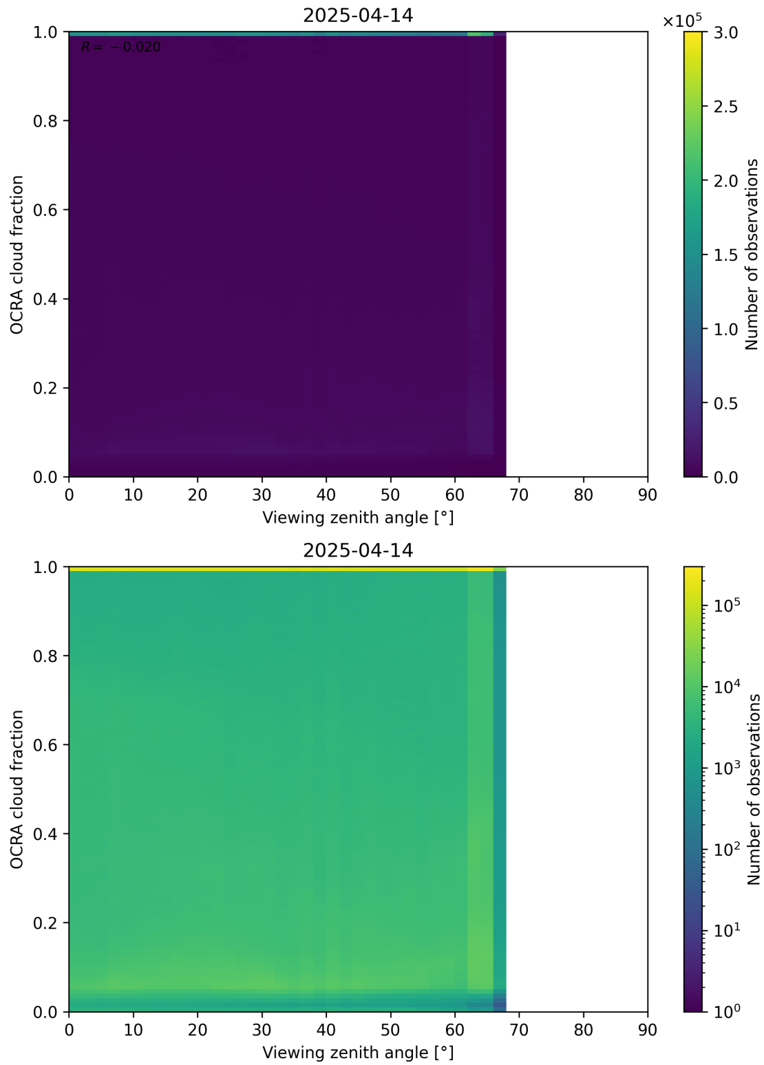
Figure 108: Scatter density plot of “Viewing zenith angle” against “OCRA cloud fraction” for 2025-04-13 to 2025-04-15.
