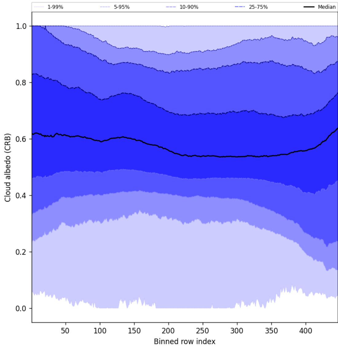
Figure 60: Along track statistics of “Cloud albedo (CRB)” for 2025-04-13 to 2025-04-15
