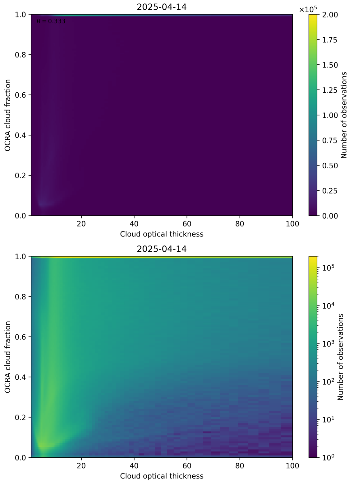
Figure 83: Scatter density plot of “Cloud optical thickness” against “OCRA cloud fraction” for 2025-04-13 to 2025-04-15.
