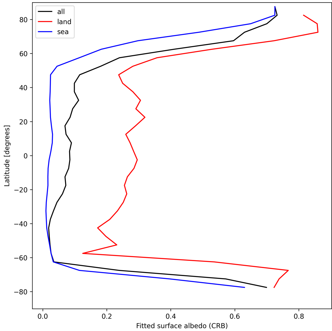
Figure 30: Zonal average of “Fitted surface albedo (CRB)” for 2025-04-13 to 2025-04-15.
