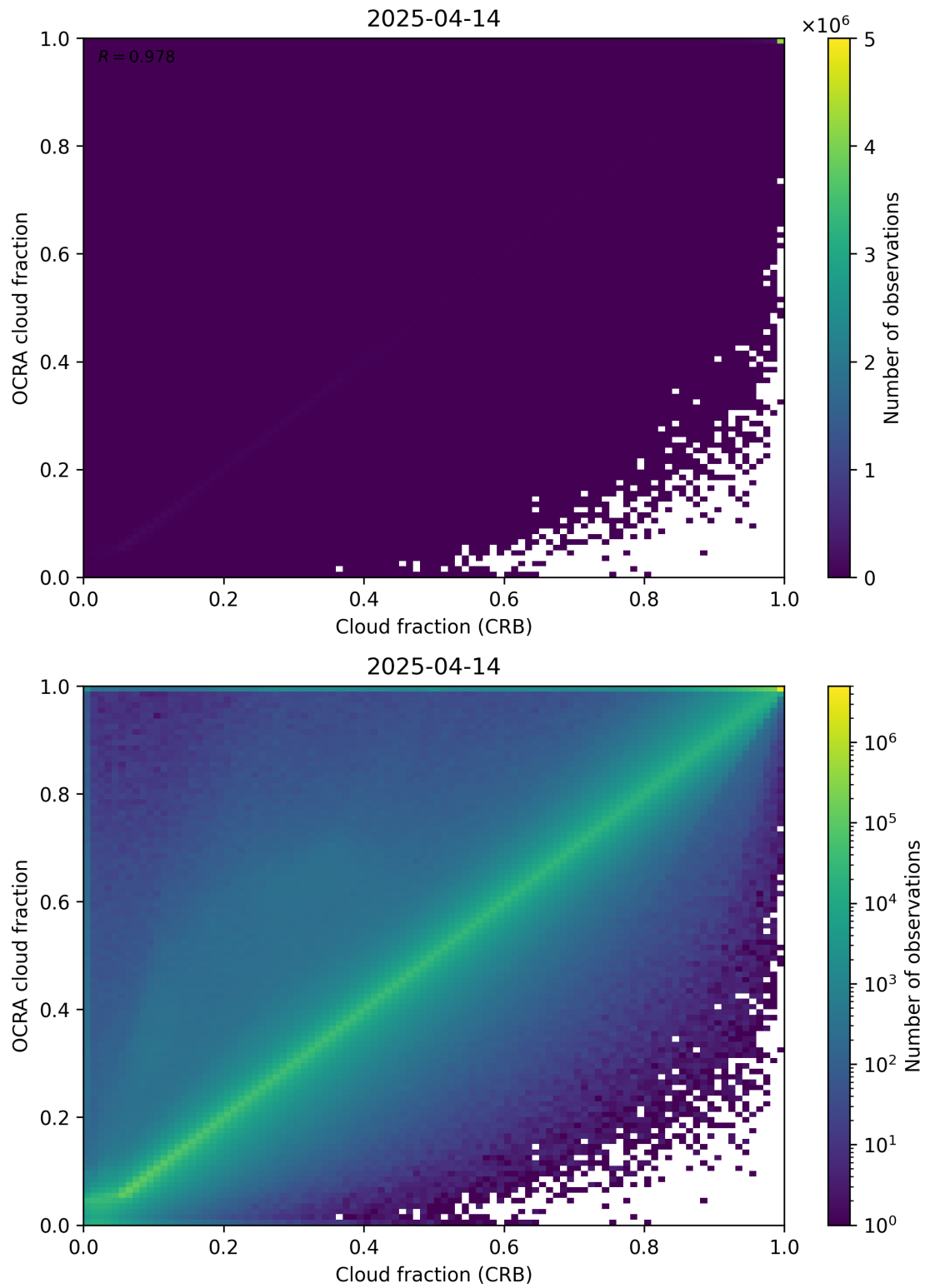
Figure 78: Scatter density plot of “Cloud fraction (CRB)” against “OCRA cloud fraction” for 2025-04-13 to 2025-04-15.
