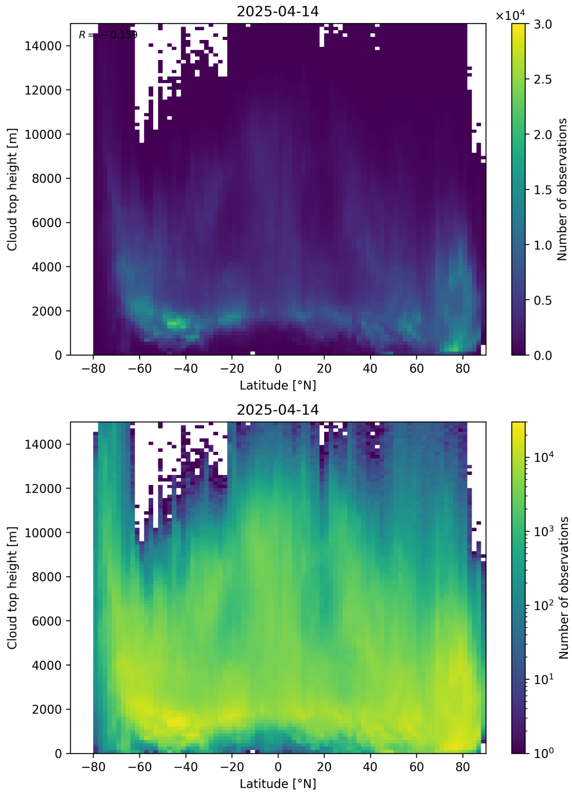
Figure 97: Scatter density plot of “Latitude” against “Cloud top height” for 2025-04-13 to 2025-04-15.
