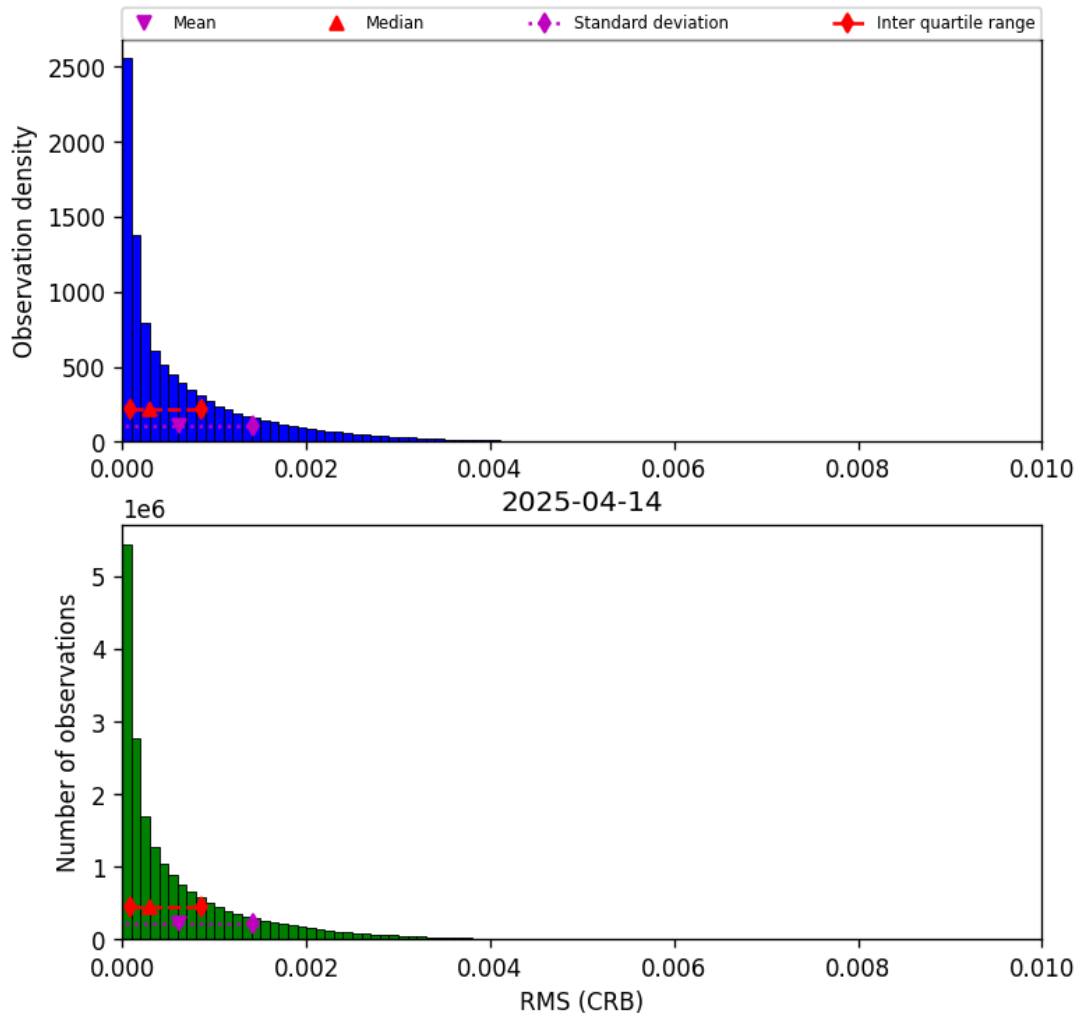
Figure 48: Histogram of “RMS (CRB)” for 2025-04-13 to 2025-04-15
