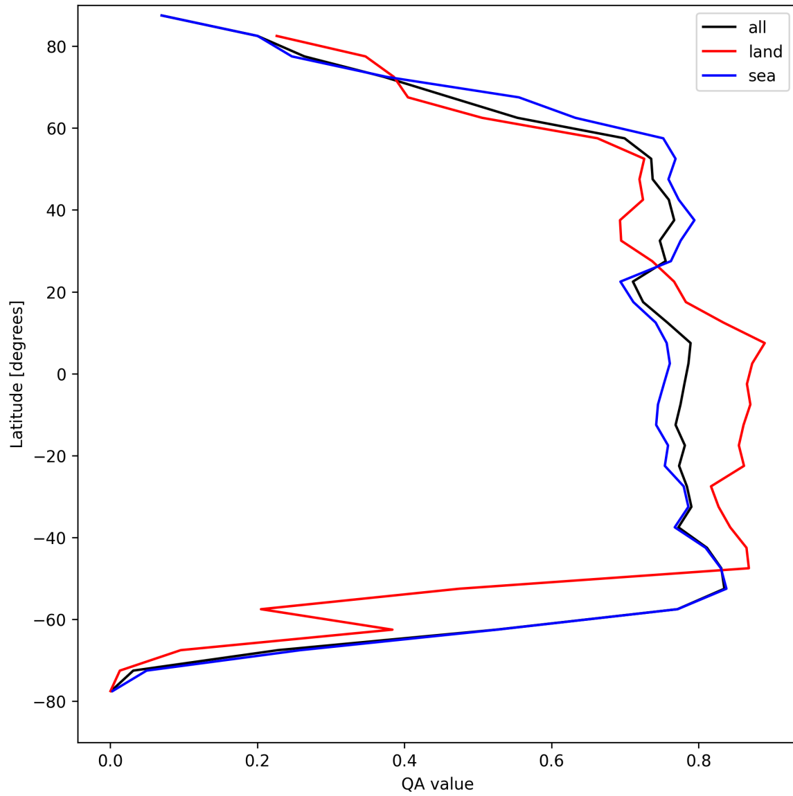
Figure 22: Zonal average of “QA value” for 2025-04-13 to 2025-04-15.
