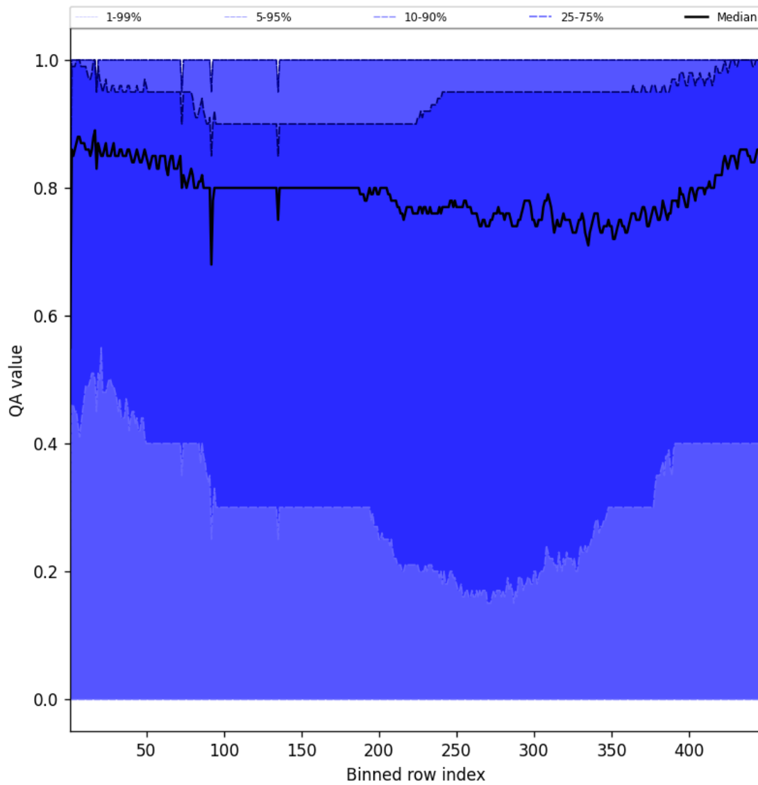
Figure 54: Along track statistics of “QA value” for 2025-04-13 to 2025-04-15
