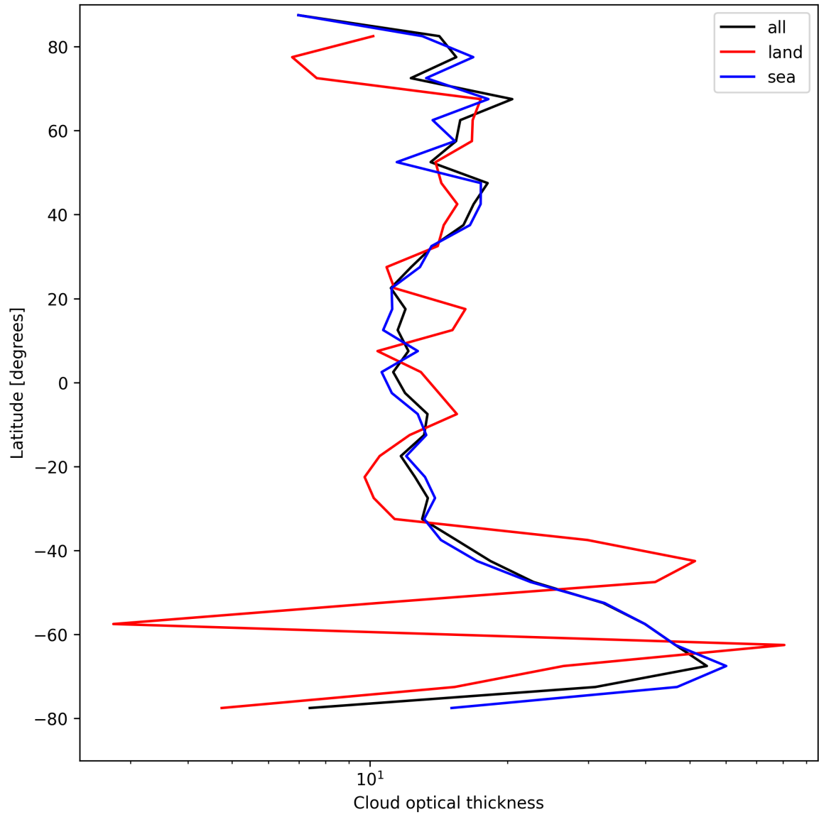
Figure 25: Zonal average of “Cloud optical thickness” for 2025-04-13 to 2025-04-15.
