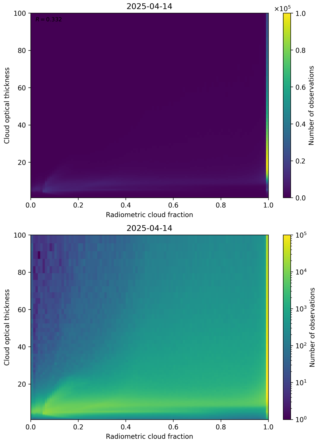
Figure 75: Scatter density plot of “Radiometric cloud fraction” against “Cloud optical thickness” for 2025-04-13 to 2025-04-15.
