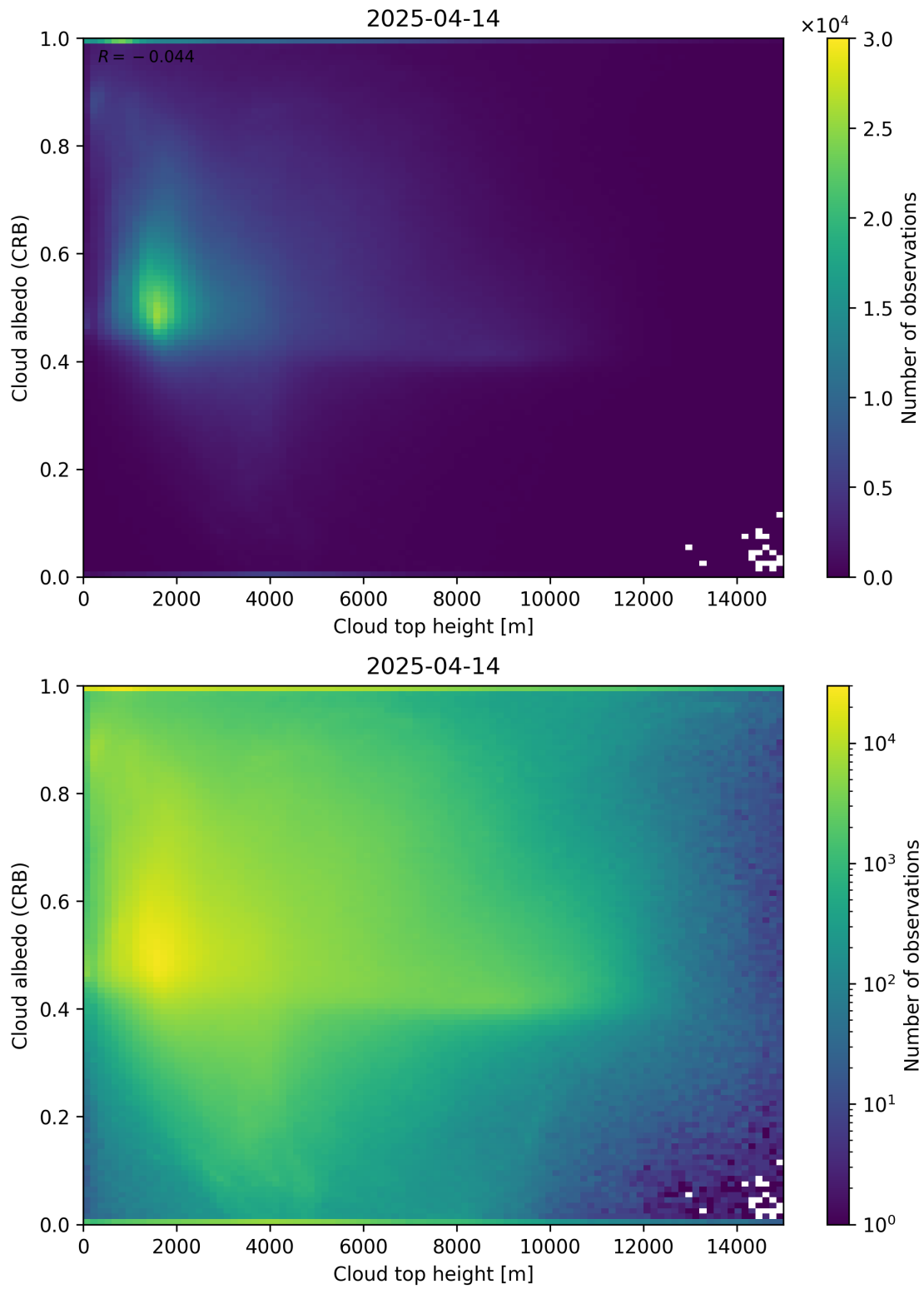
Figure 86: Scatter density plot of “Cloud top height” against “Cloud albedo (CRB)” for 2025-04-13 to 2025-04-15.
