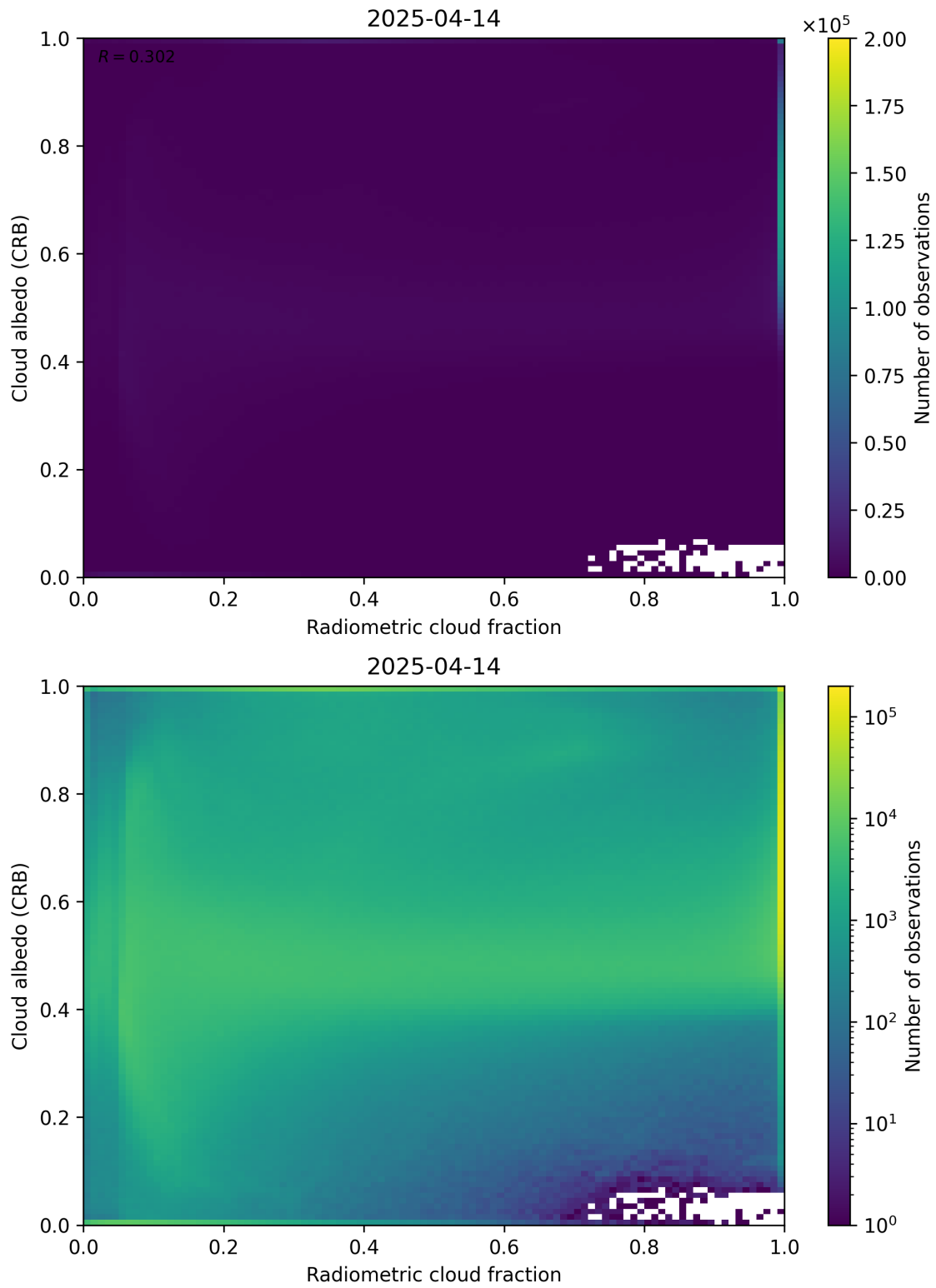
Figure 71: Scatter density plot of “Radiometric cloud fraction” against “Cloud albedo (CRB)” for 2025-04-13 to 2025-04-15.
