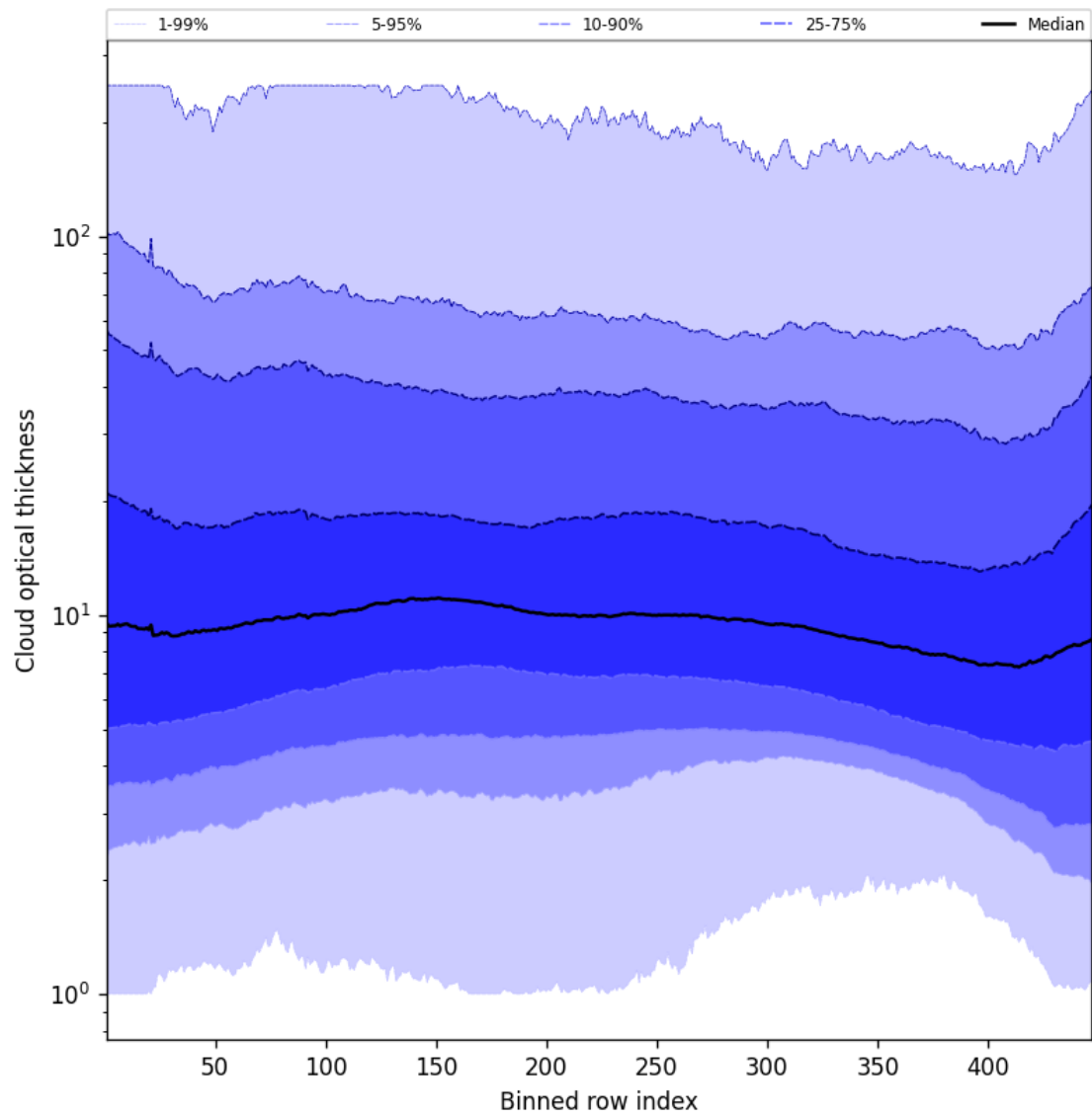
Figure 57: Along track statistics of “Cloud optical thickness” for 2025-04-13 to 2025-04-15
