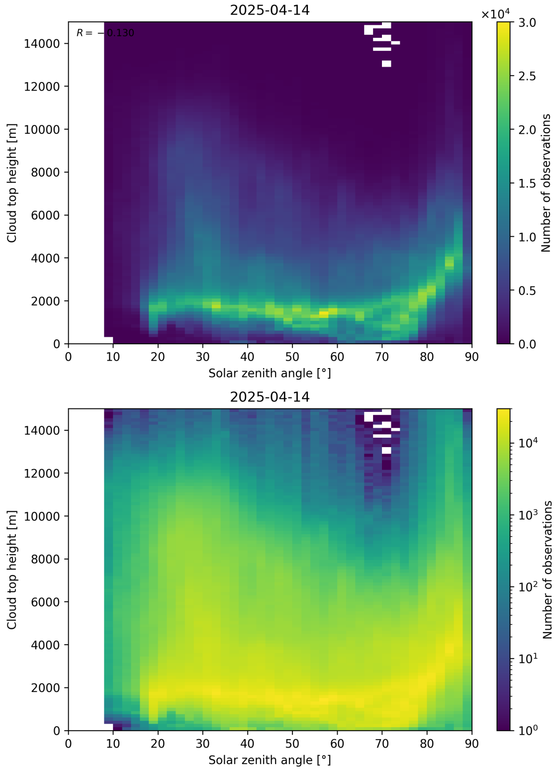
Figure 104: Scatter density plot of “Solar zenith angle” against “Cloud top height” for 2025-04-13 to 2025-04-15.
