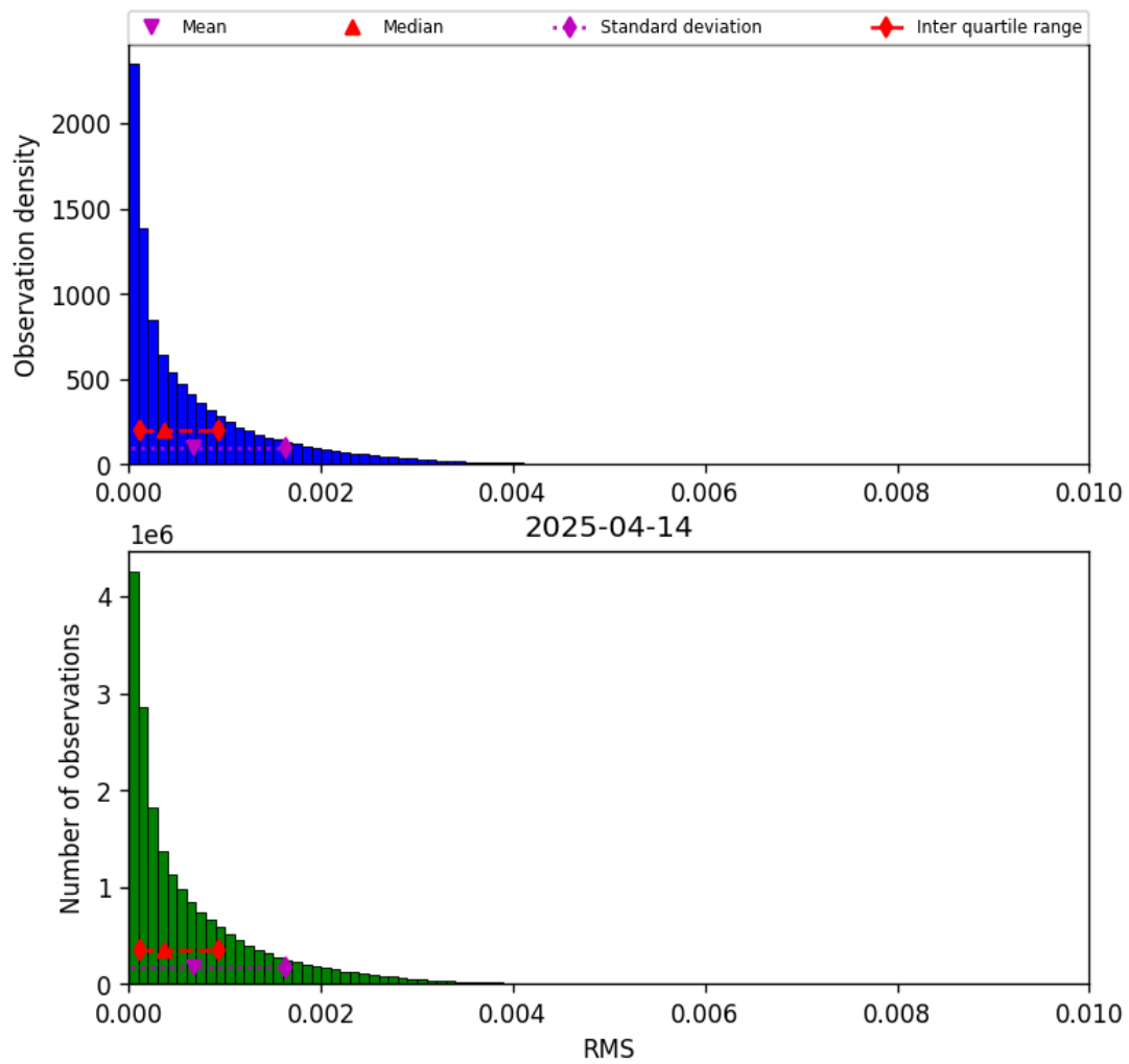
Figure 47: Histogram of “RMS” for 2025-04-13 to 2025-04-15
