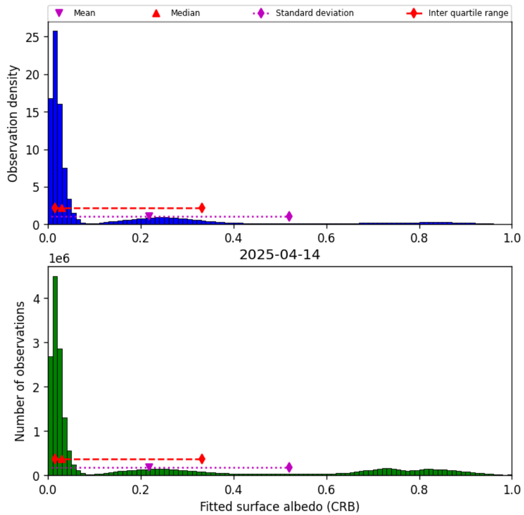
Figure 46: Histogram of “Fitted surface albedo (CRB)” for 2025-04-13 to 2025-04-15
