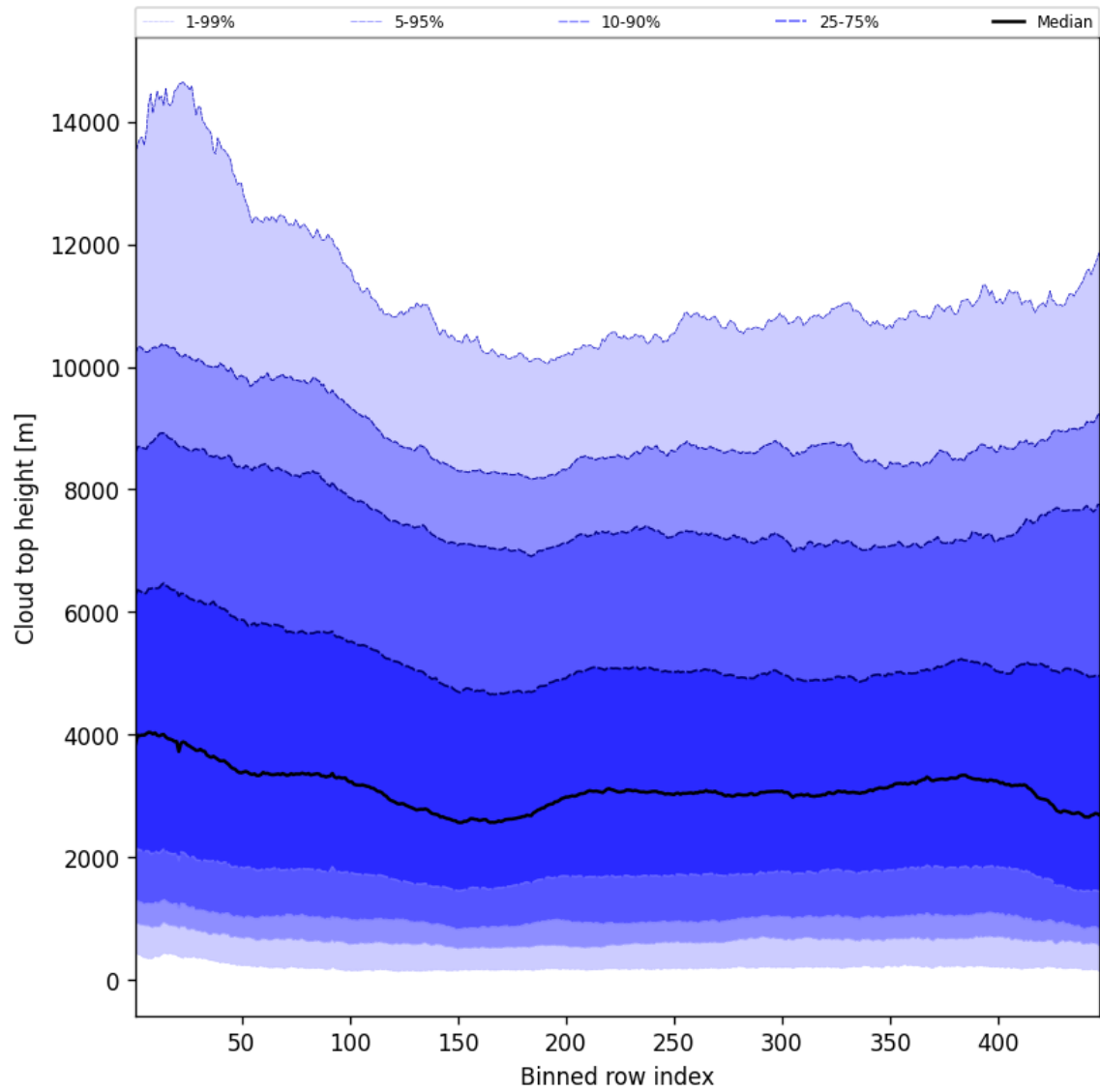
Figure 56: Along track statistics of “Cloud top height” for 2025-04-13 to 2025-04-15
