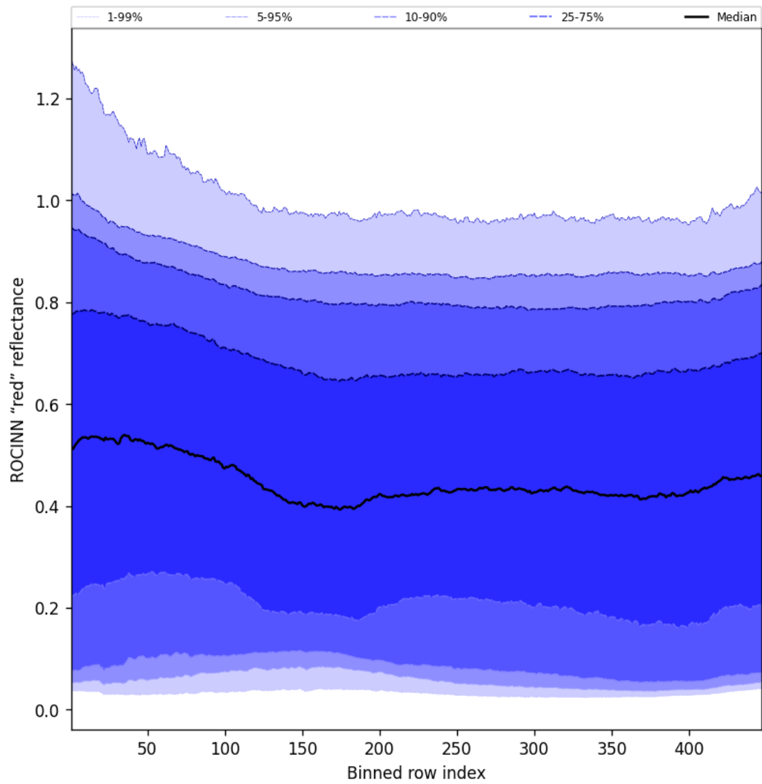
Figure 69: Along track statistics of “ROCINN “red” reflectance” for 2025-04-13 to 2025-04-15
