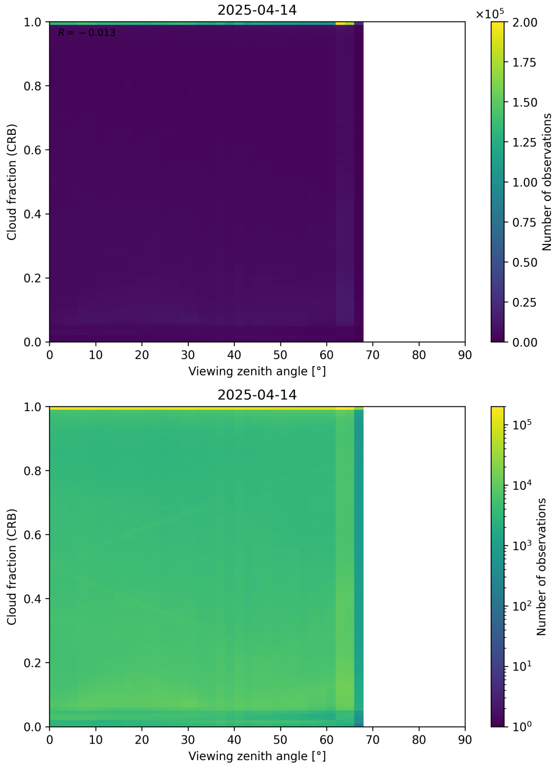
Figure 109: Scatter density plot of “Viewing zenith angle” against “Cloud fraction (CRB)” for 2025-04-13 to 2025-04-15.
