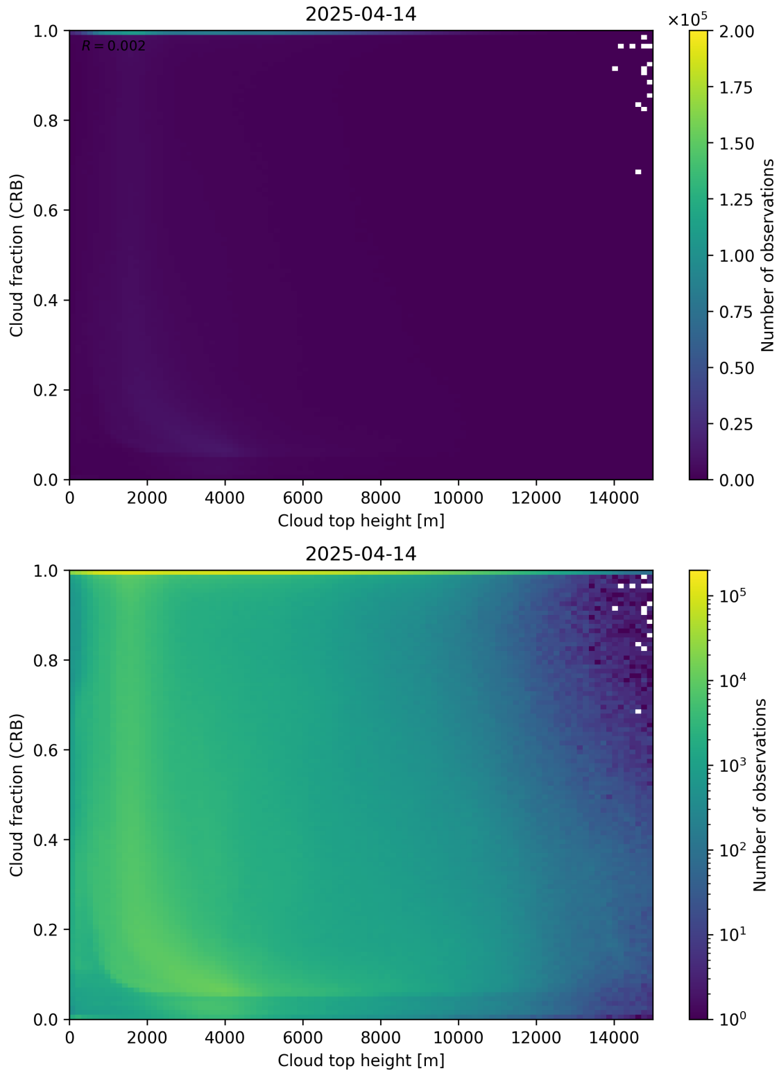
Figure 88: Scatter density plot of “Cloud top height” against “Cloud fraction (CRB)” for 2025-04-13 to 2025-04-15.
