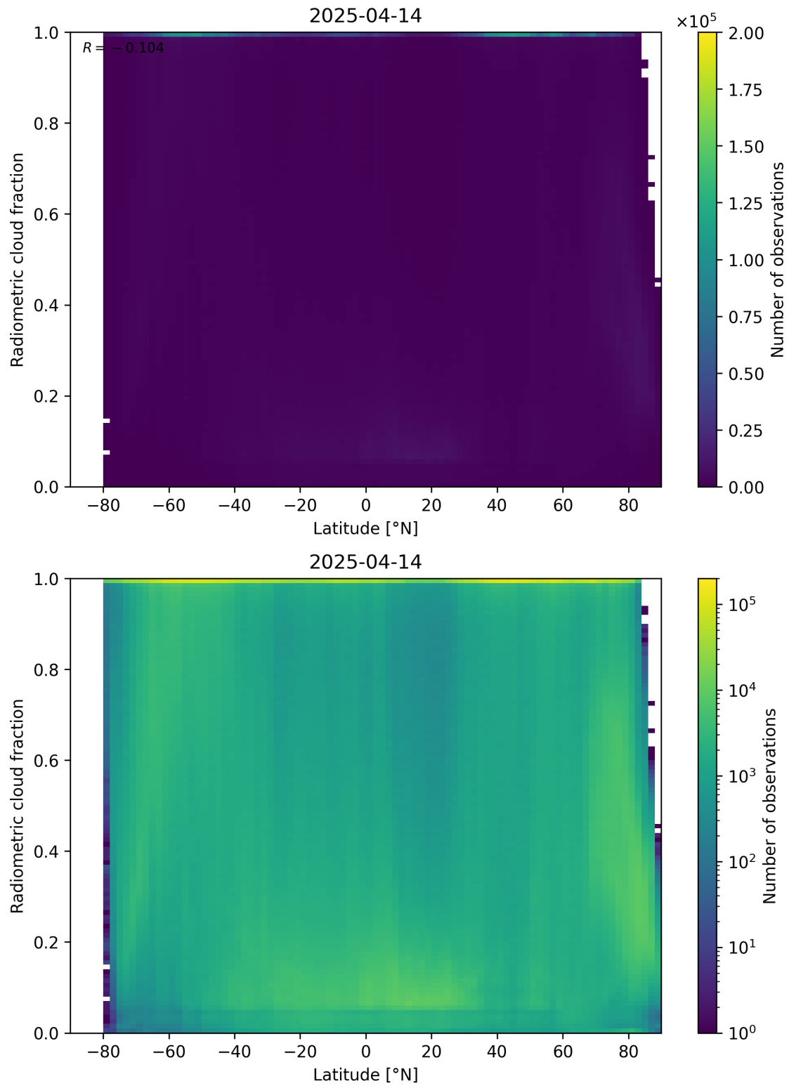
Figure 92: Scatter density plot of “Latitude” against “Radiometric cloud fraction” for 2025-04-13 to 2025-04-15.
