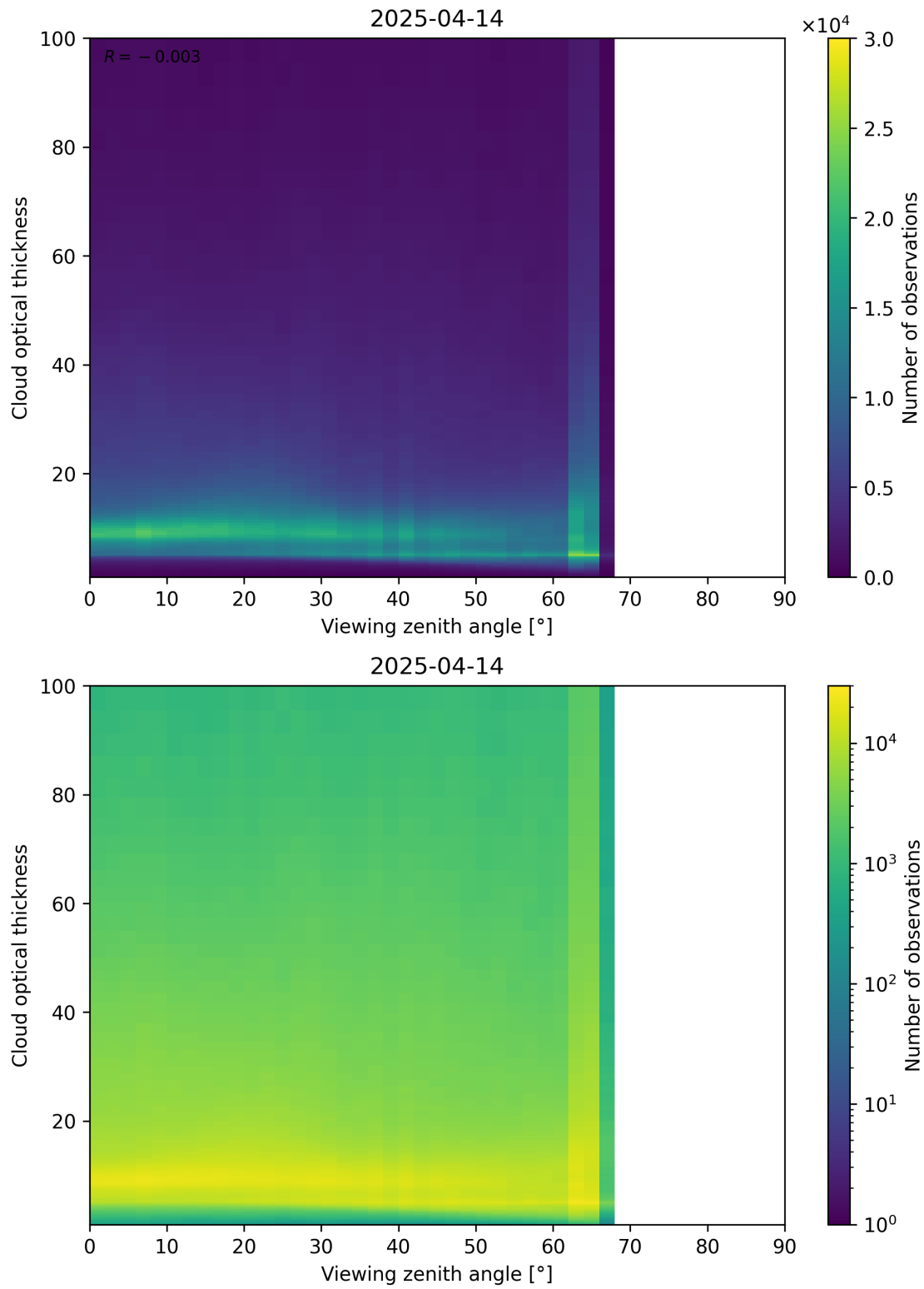
Figure 111: Scatter density plot of “Viewing zenith angle” against “Cloud optical thickness” for 2025-04-13 to 2025-04-15.
