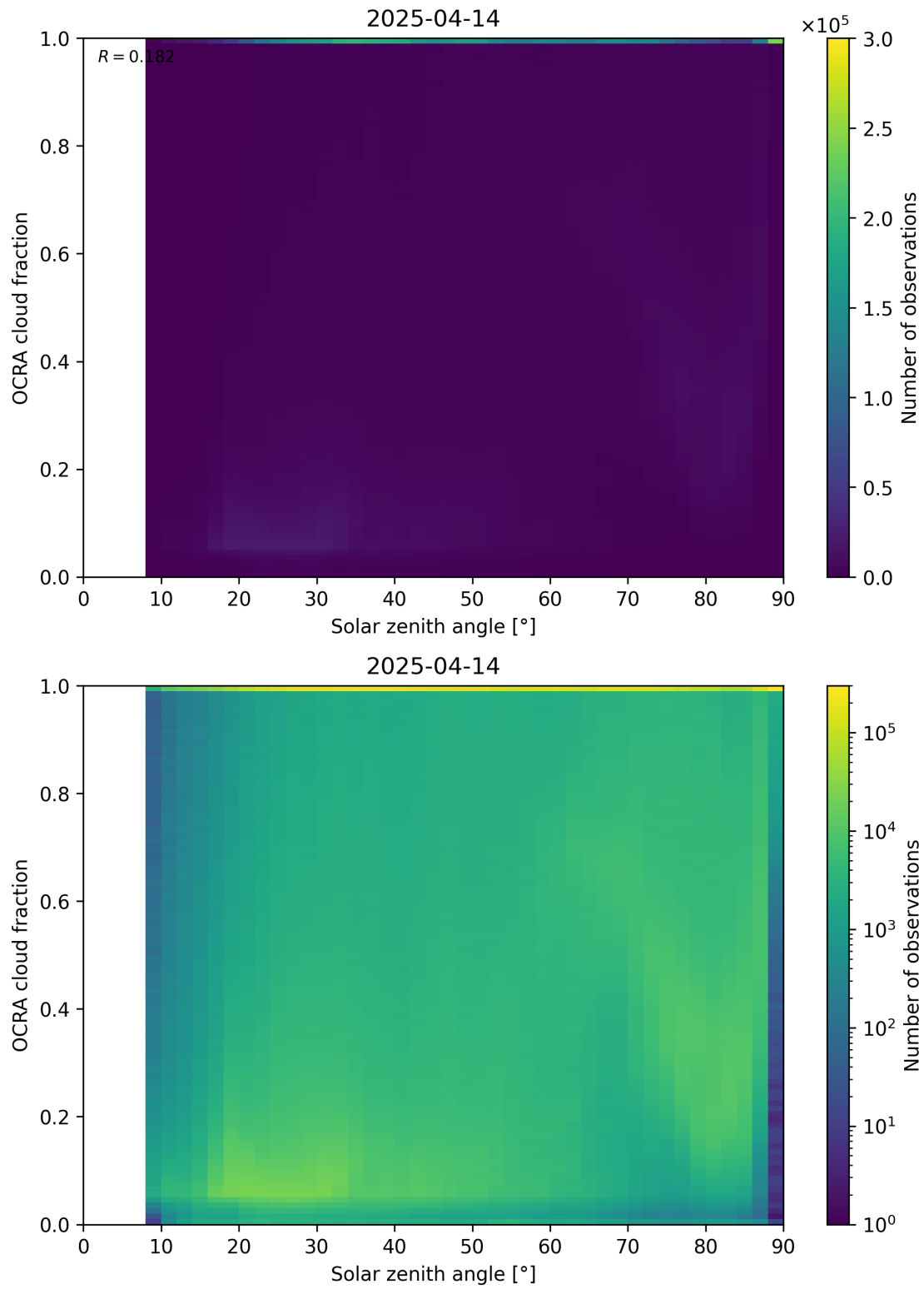
Figure 100: Scatter density plot of “Solar zenith angle” against “OCRA cloud fraction” for 2025-04-13 to 2025-04-15.
