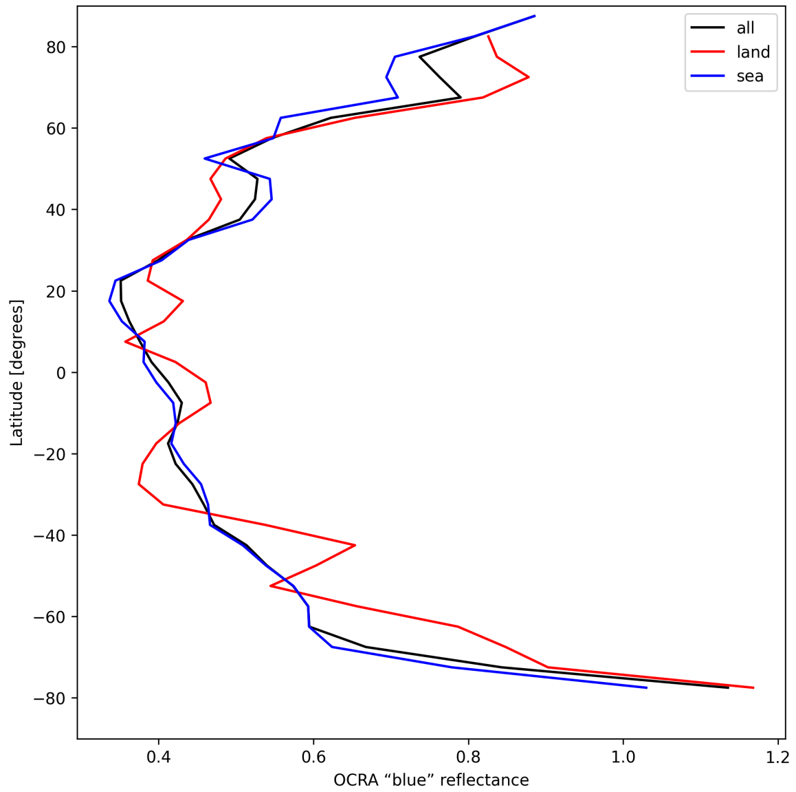
Figure 35: Zonal average of “OCRA “blue” reflectance” for 2025-04-13 to 2025-04-15.
