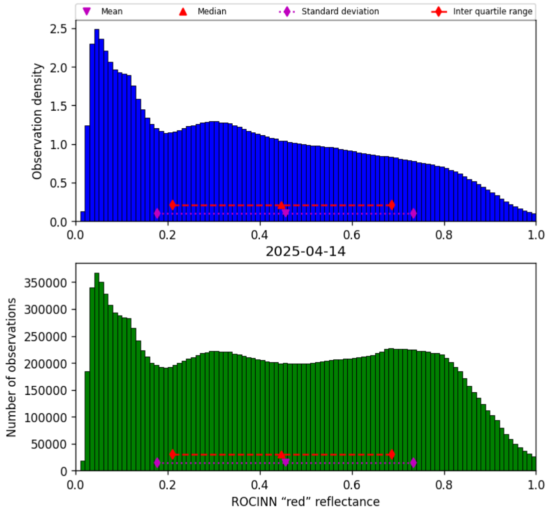
Figure 53: Histogram of “ROCINN “red” reflectance” for 2025-04-13 to 2025-04-15
