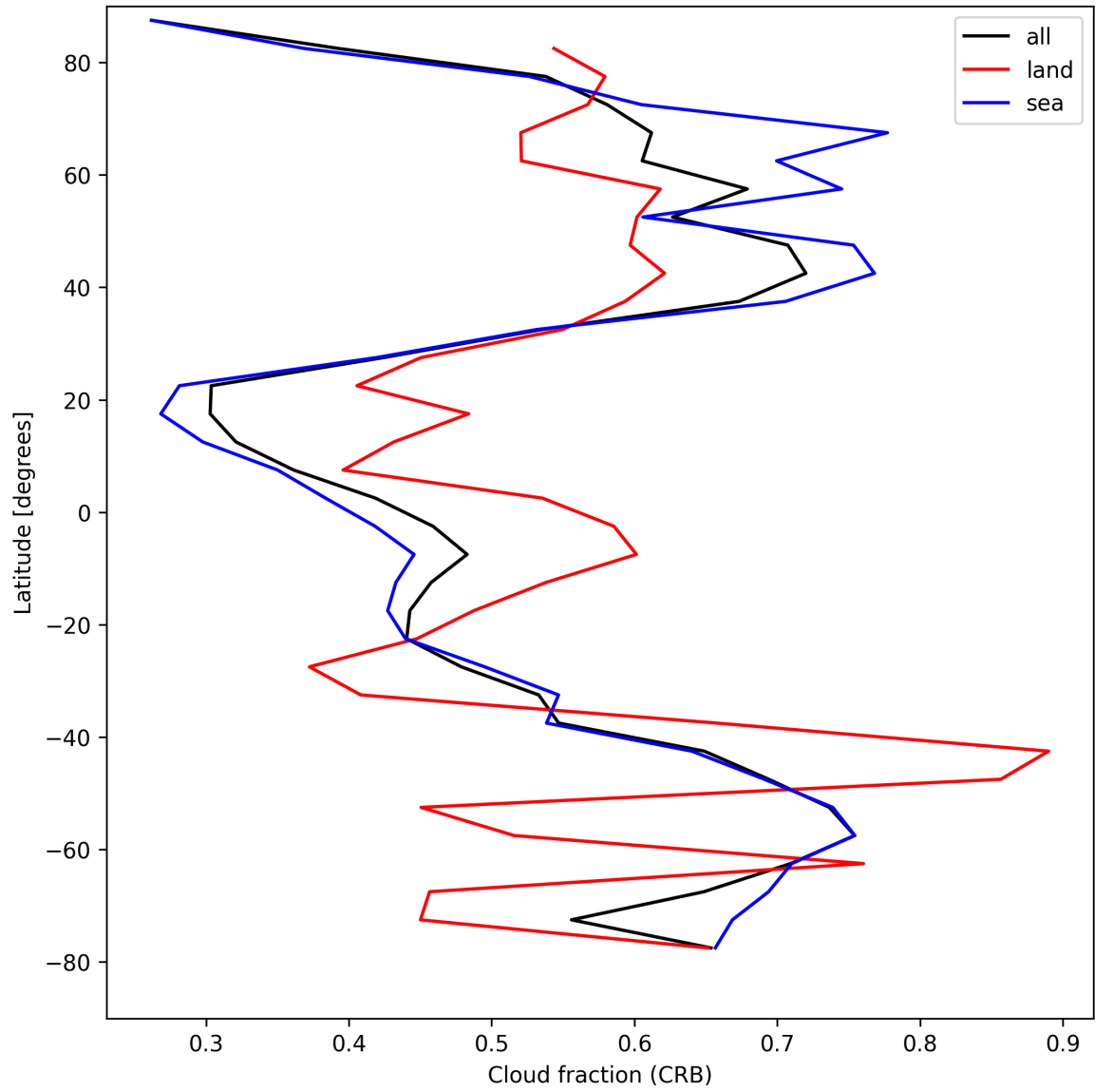
Figure 26: Zonal average of “Cloud fraction (CRB)” for 2025-04-13 to 2025-04-15.
