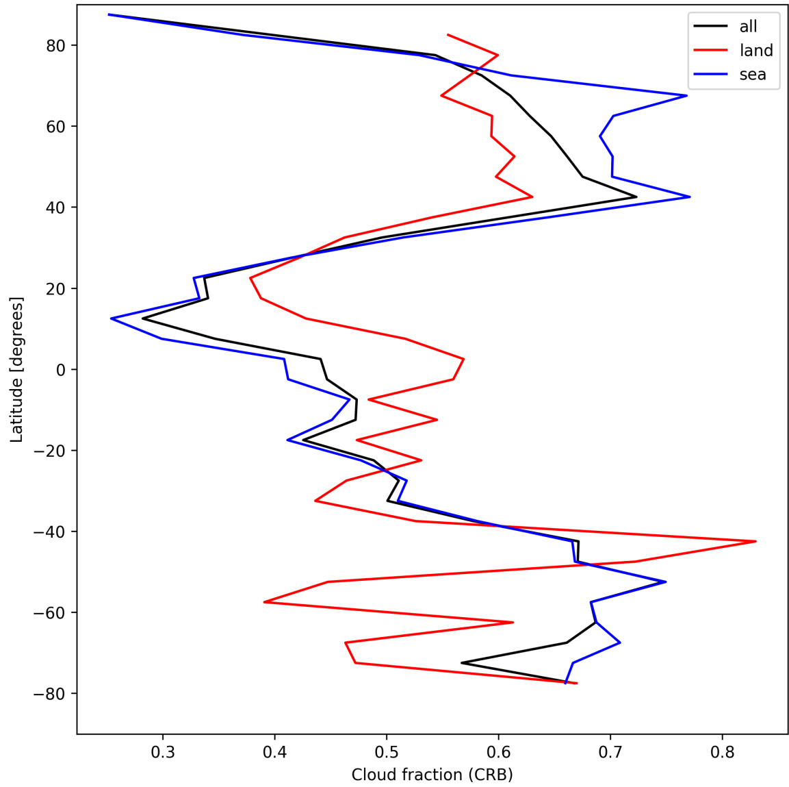
Figure 26: Zonal average of “Cloud fraction (CRB)” for 2025-04-14 to 2025-04-16.
