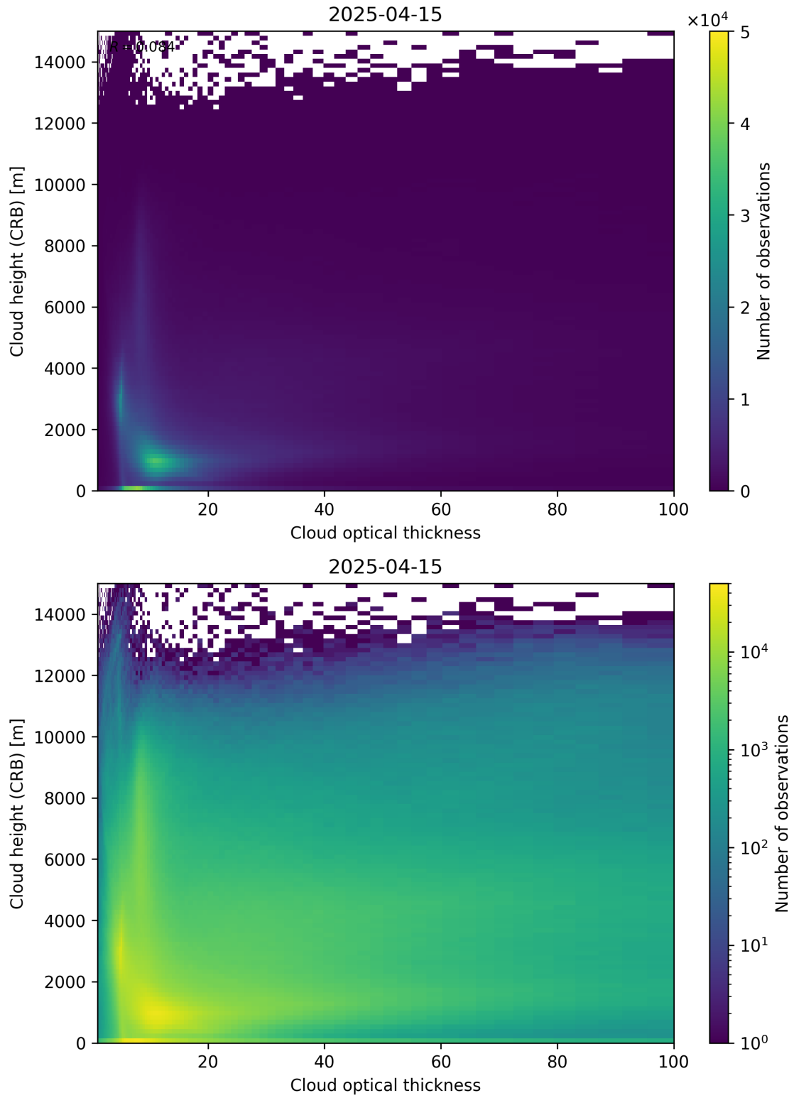
Figure 85: Scatter density plot of “Cloud optical thickness” against “Cloud height (CRB)” for 2025-04-14 to 2025-04-16.
