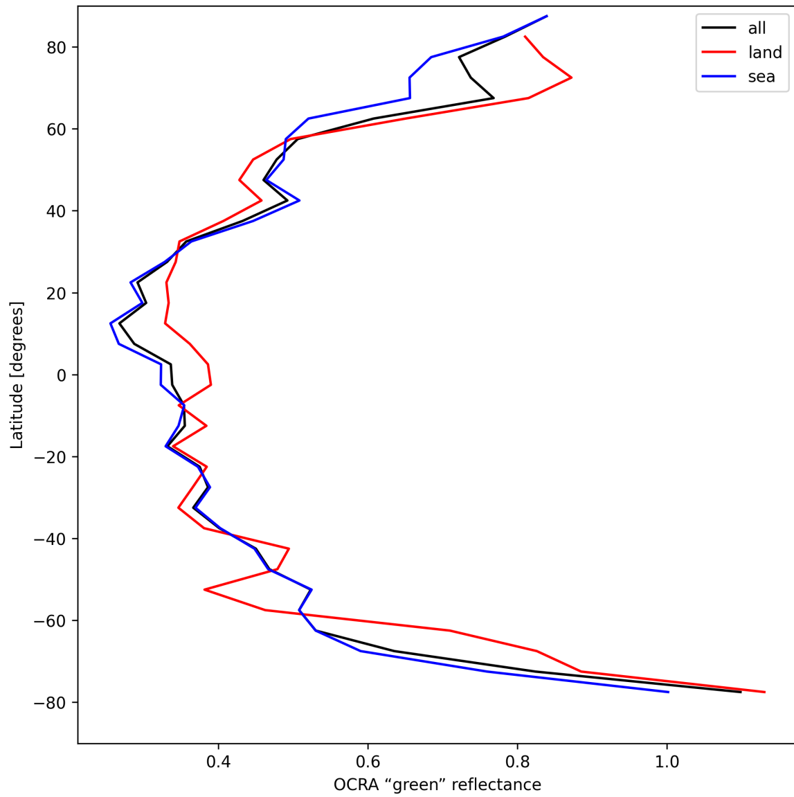
Figure 36: Zonal average of “OCRA “green” reflectance” for 2025-04-14 to 2025-04-16.
