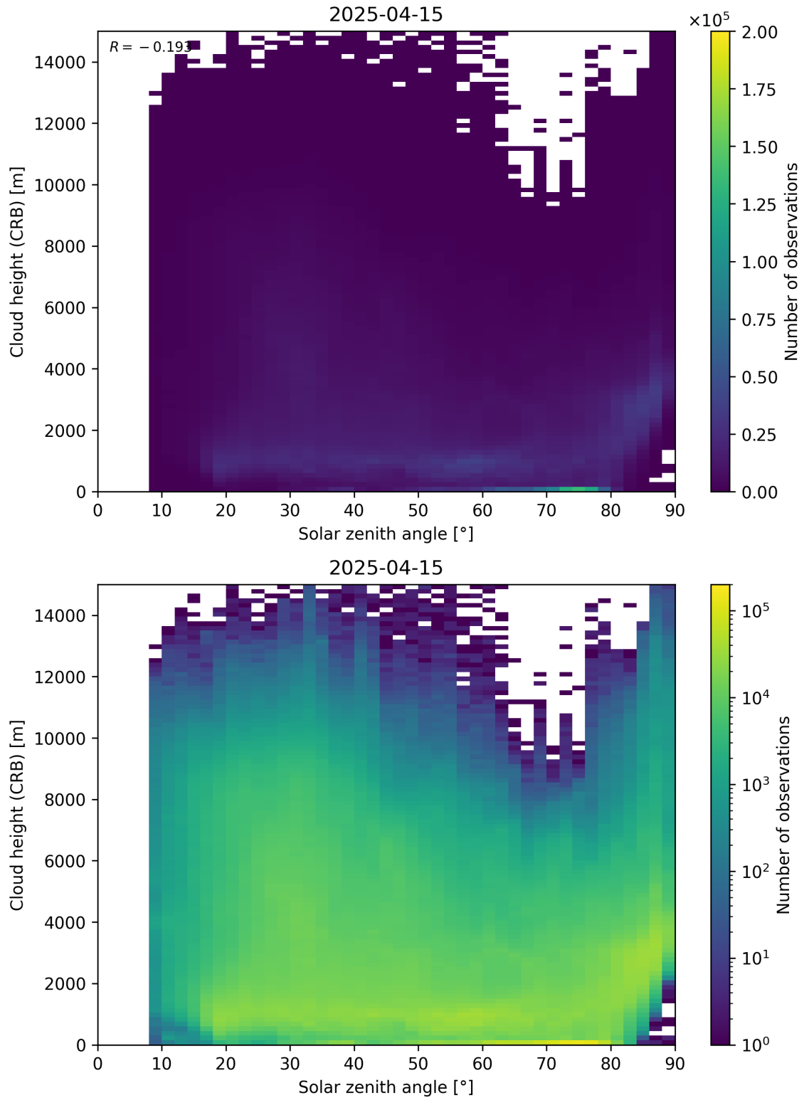
Figure 102: Scatter density plot of “Solar zenith angle” against “Cloud height (CRB)” for 2025-04-14 to 2025-04-16.
