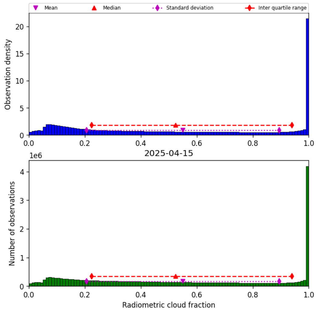
Figure 39: Histogram of “Radiometric cloud fraction” for 2025-04-14 to 2025-04-16
