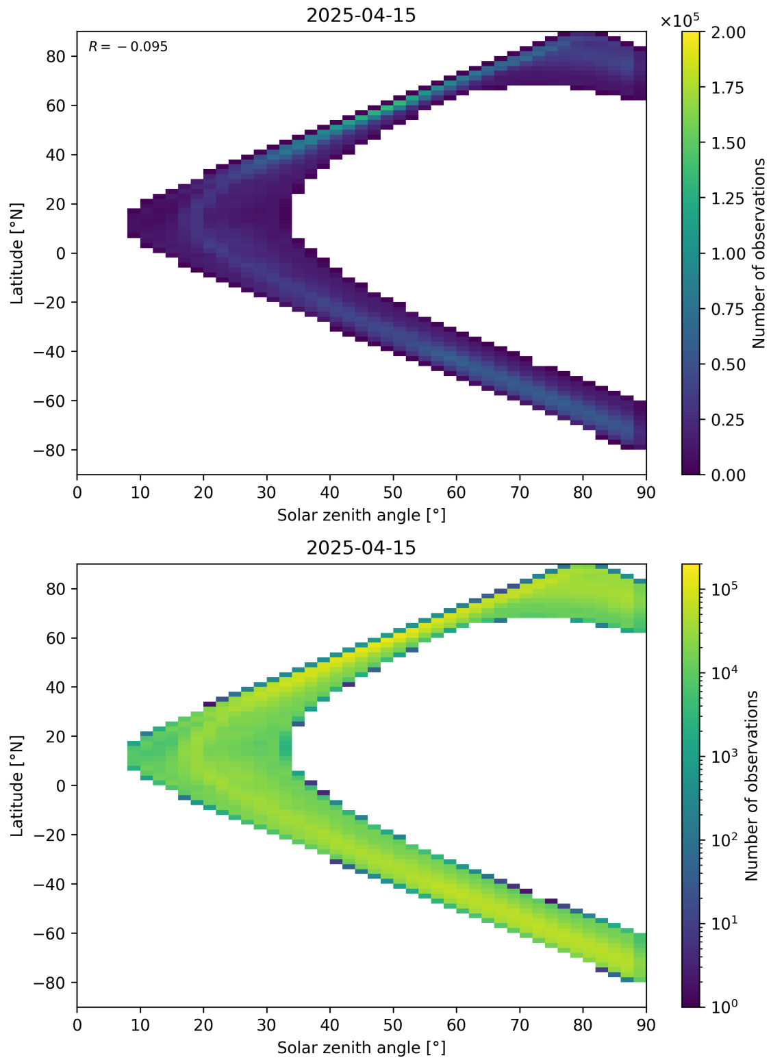
Figure 105: Scatter density plot of “Solar zenith angle” against “Latitude” for 2025-04-14 to 2025-04-16.
