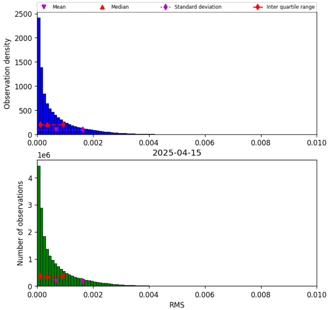
Figure 47: Histogram of “RMS” for 2025-04-14 to 2025-04-16
