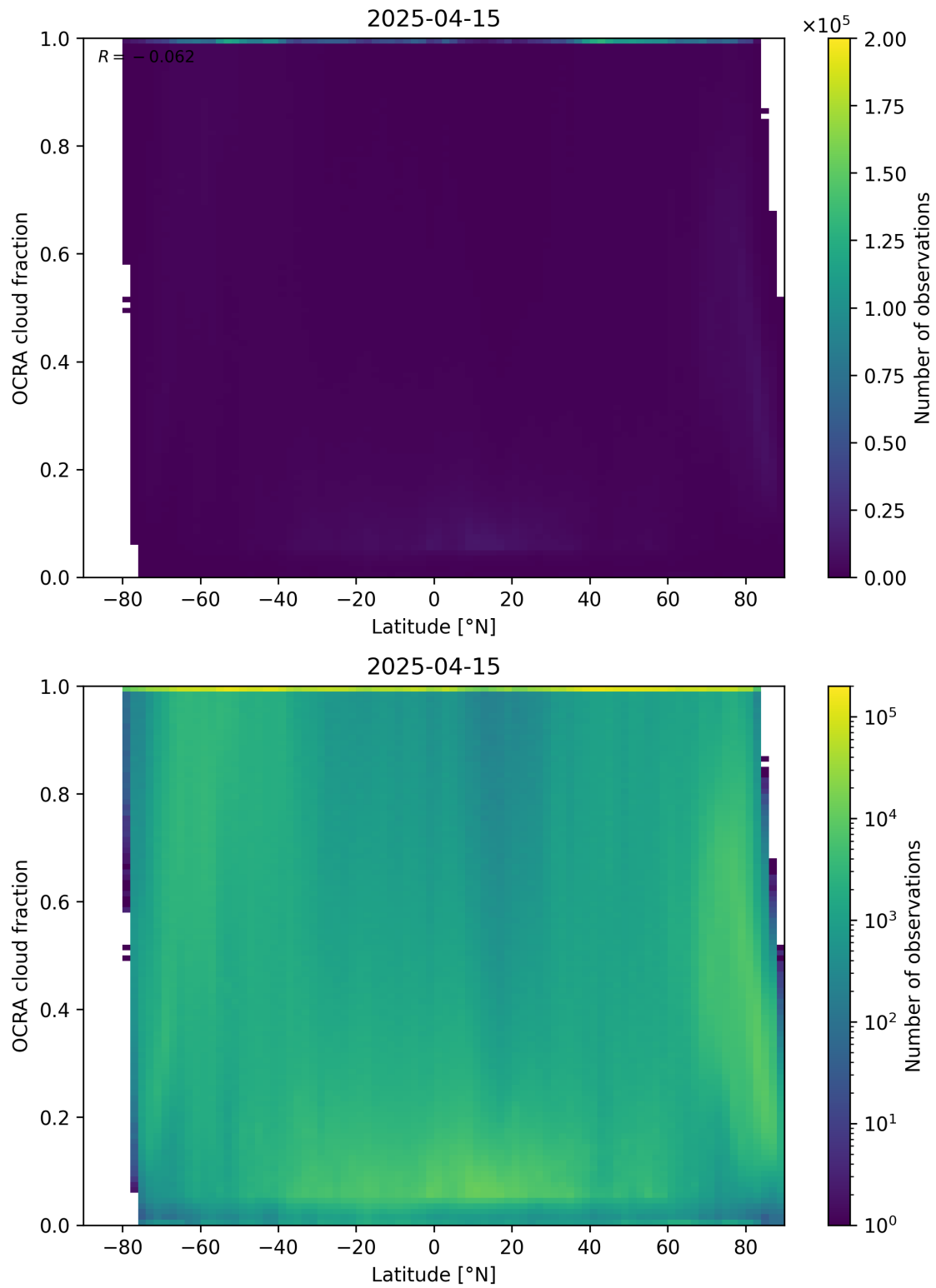
Figure 93: Scatter density plot of “Latitude” against “OCRA cloud fraction” for 2025-04-14 to 2025-04-16.
