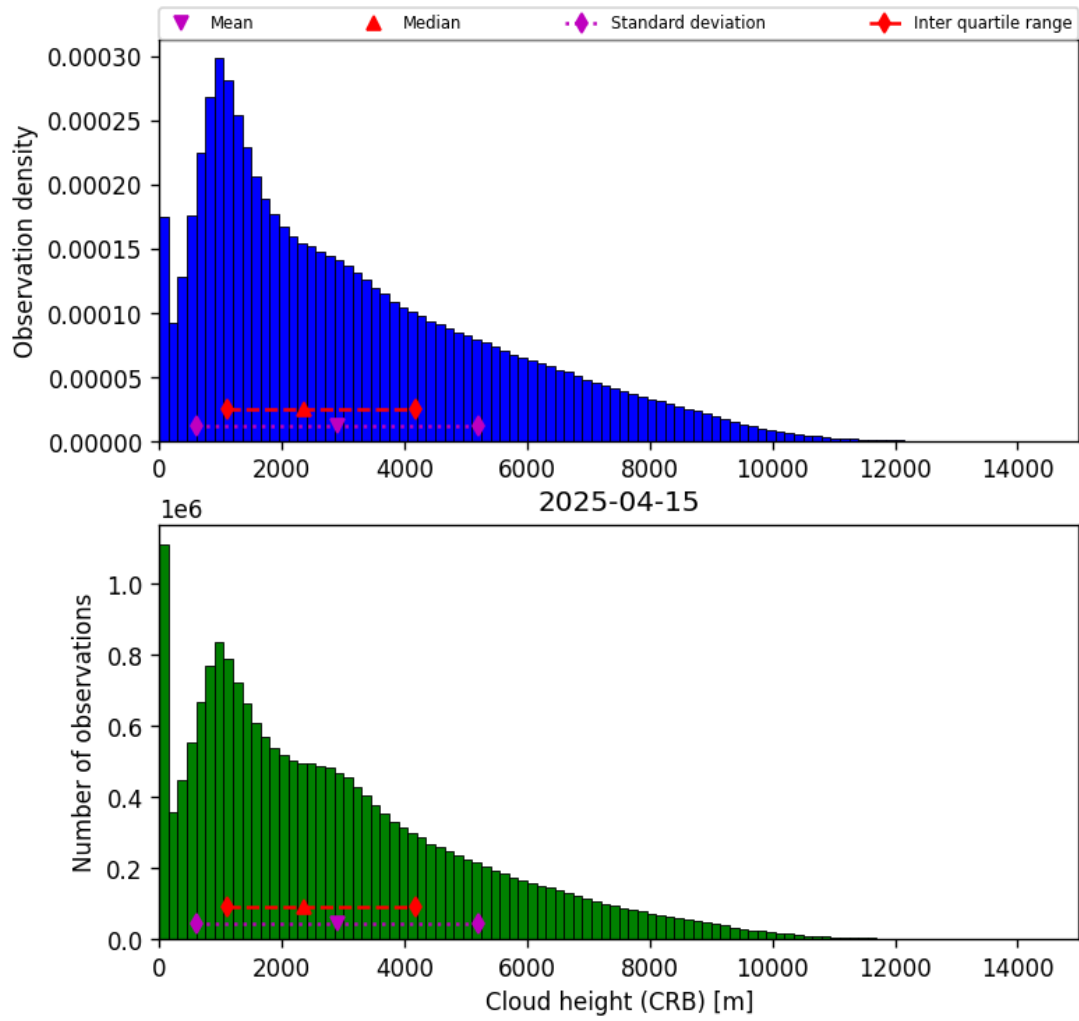
Figure 43: Histogram of “Cloud height (CRB)” for 2025-04-14 to 2025-04-16
