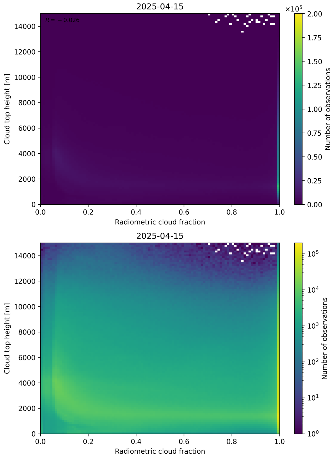
Figure 76: Scatter density plot of “Radiometric cloud fraction” against “Cloud top height” for 2025-04-14 to 2025-04-16.
