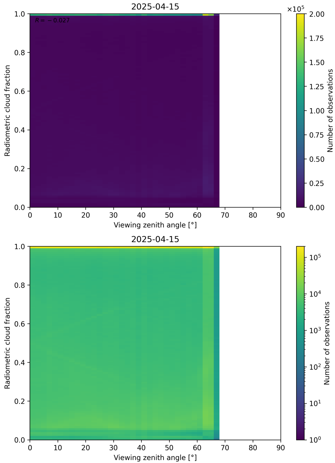
Figure 107: Scatter density plot of “Viewing zenith angle” against “Radiometric cloud fraction” for 2025-04-14 to 2025-04-16.
