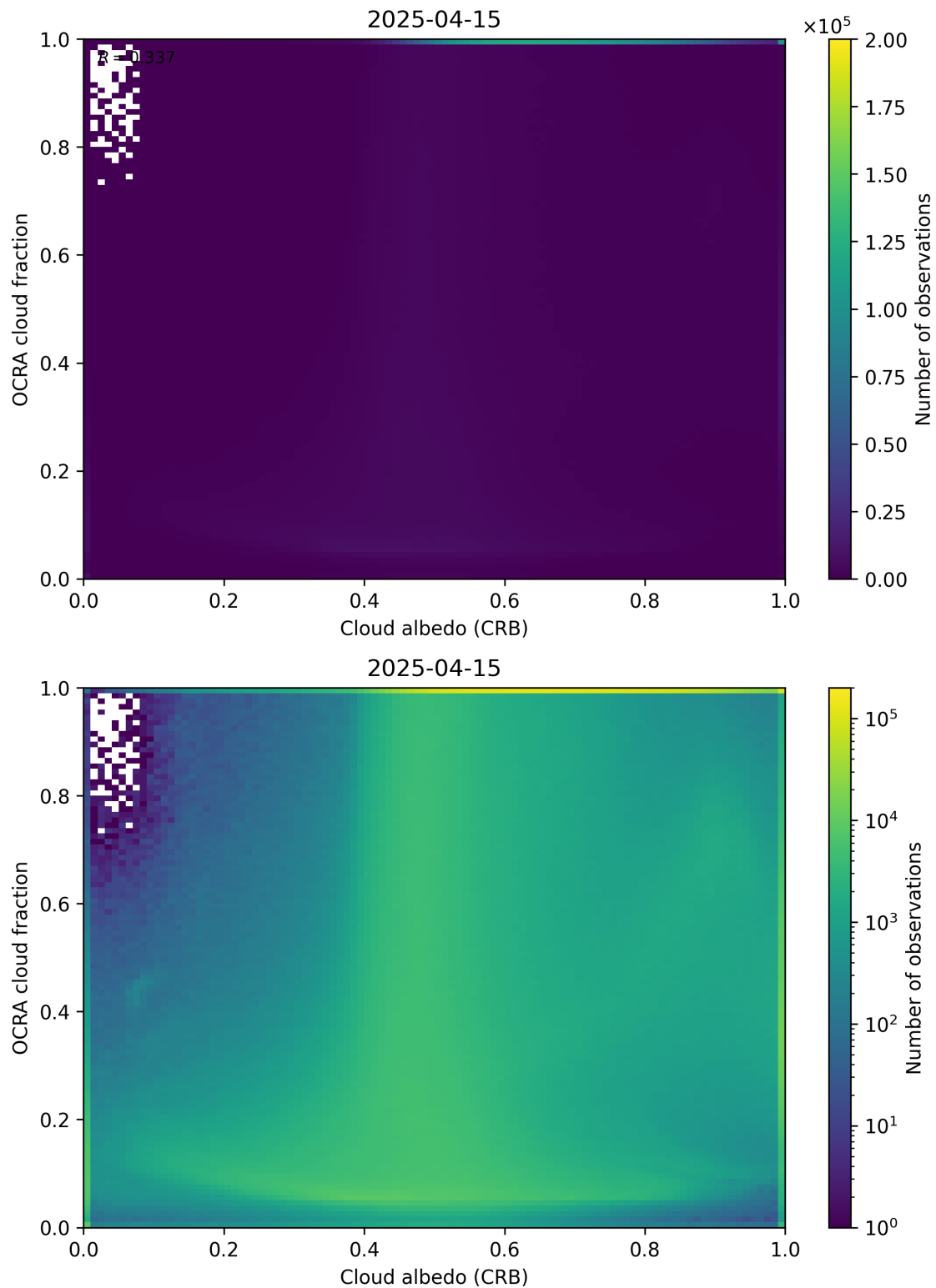
Figure 70: Scatter density plot of “Cloud albedo (CRB)” against “OCRA cloud fraction” for 2025-04-14 to 2025-04-16.
