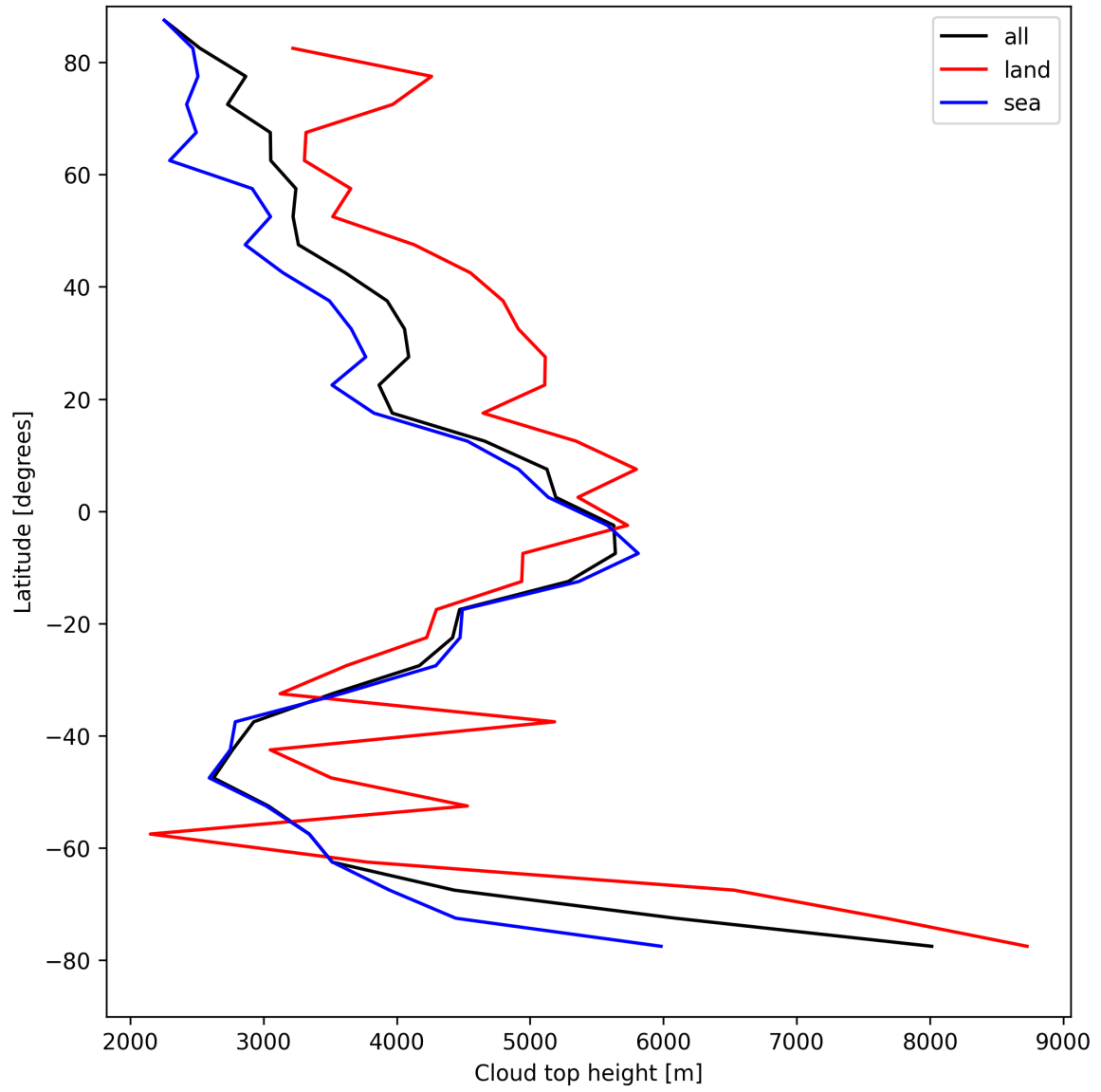
Figure 24: Zonal average of “Cloud top height” for 2025-04-14 to 2025-04-16.
