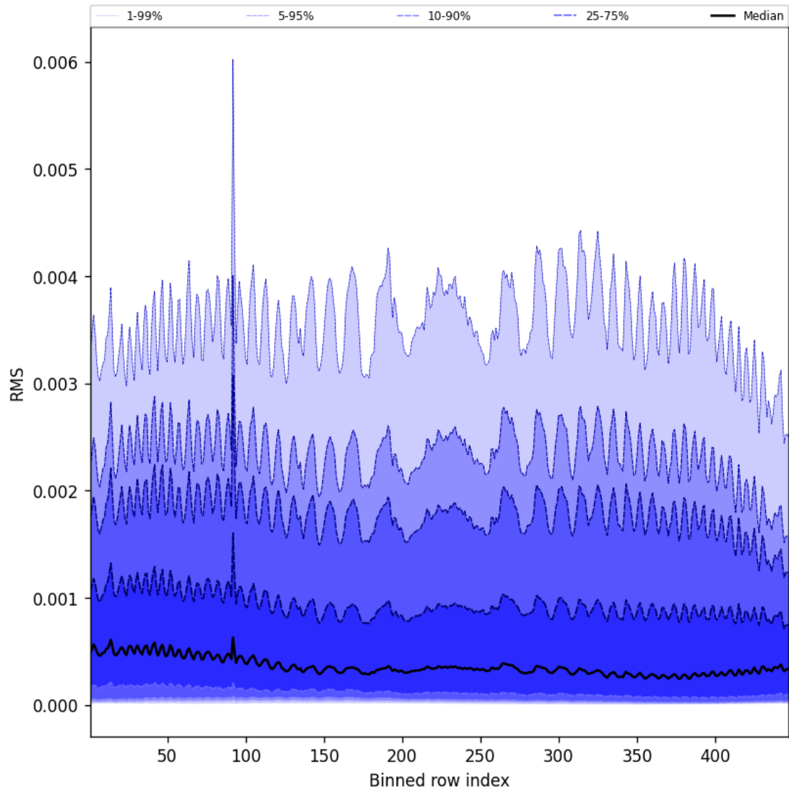
Figure 63: Along track statistics of “RMS” for 2025-04-14 to 2025-04-16
