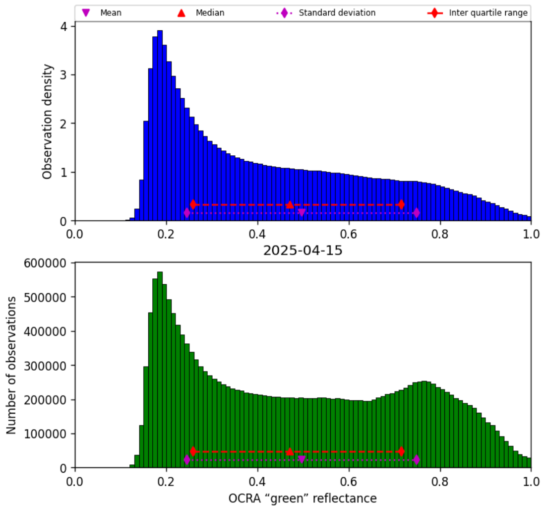
Figure 52: Histogram of “OCRA “green” reflectance” for 2025-04-14 to 2025-04-16
