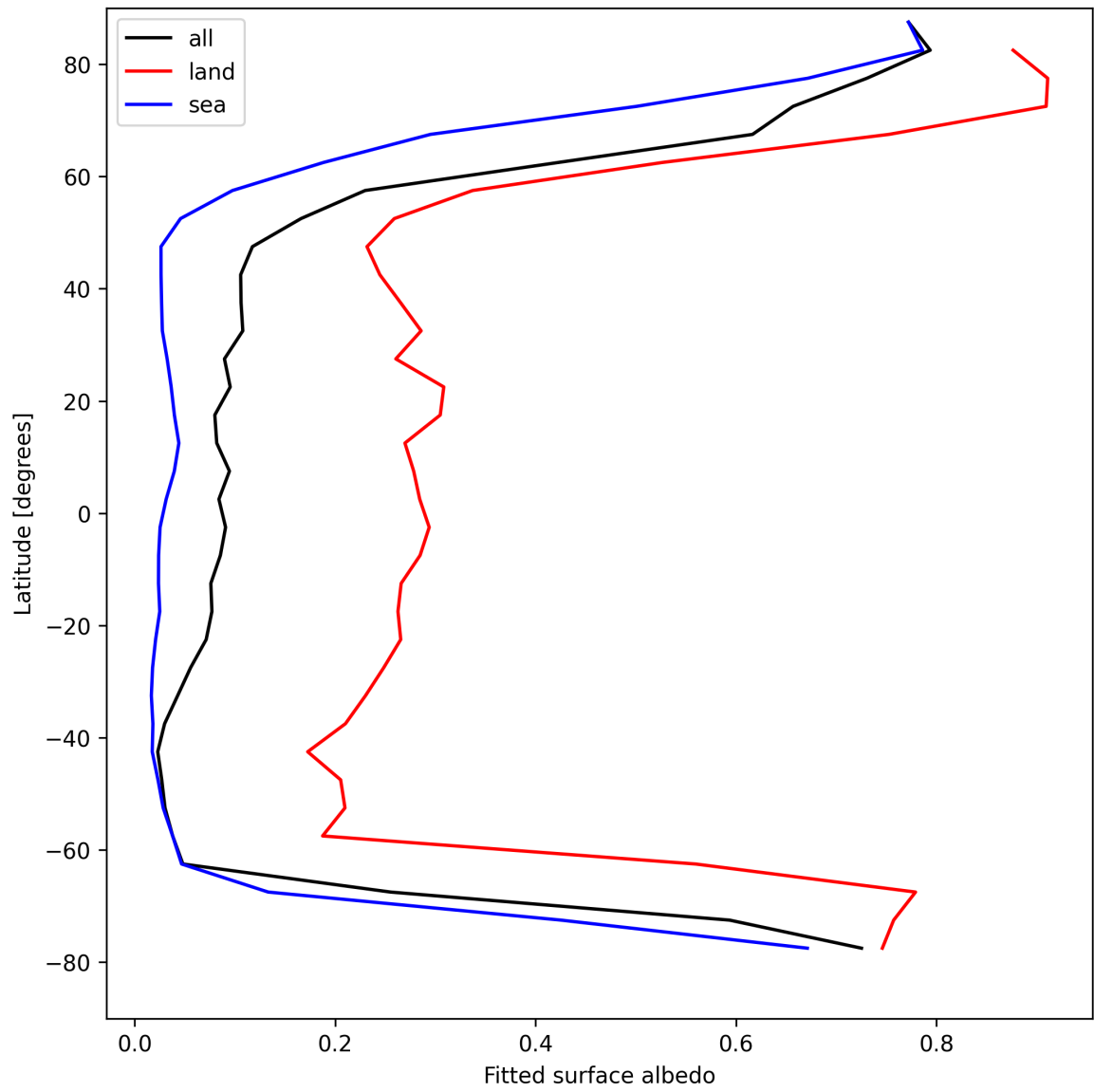
Figure 29: Zonal average of “Fitted surface albedo” for 2025-04-14 to 2025-04-16.
