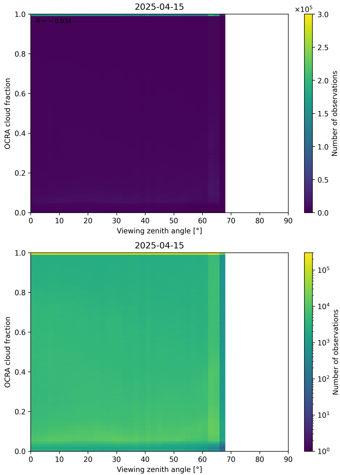
Figure 108: Scatter density plot of “Viewing zenith angle” against “OCRA cloud fraction” for 2025-04-14 to 2025-04-16.
