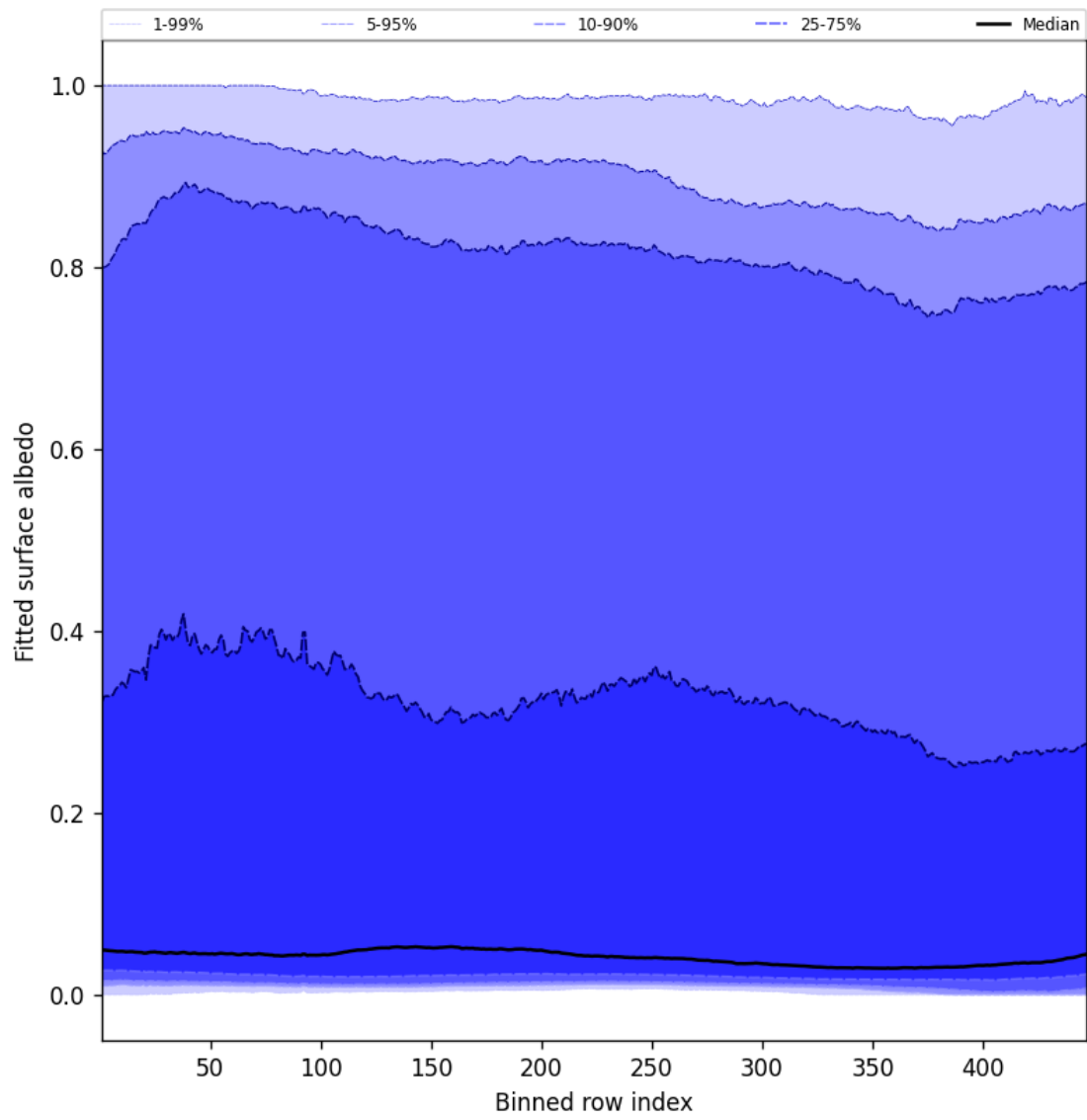
Figure 61: Along track statistics of “Fitted surface albedo” for 2025-04-14 to 2025-04-16
