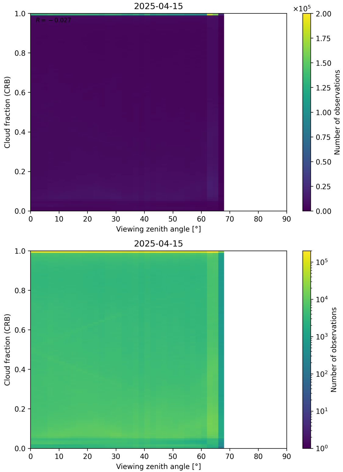
Figure 109: Scatter density plot of “Viewing zenith angle” against “Cloud fraction (CRB)” for 2025-04-14 to 2025-04-16.
