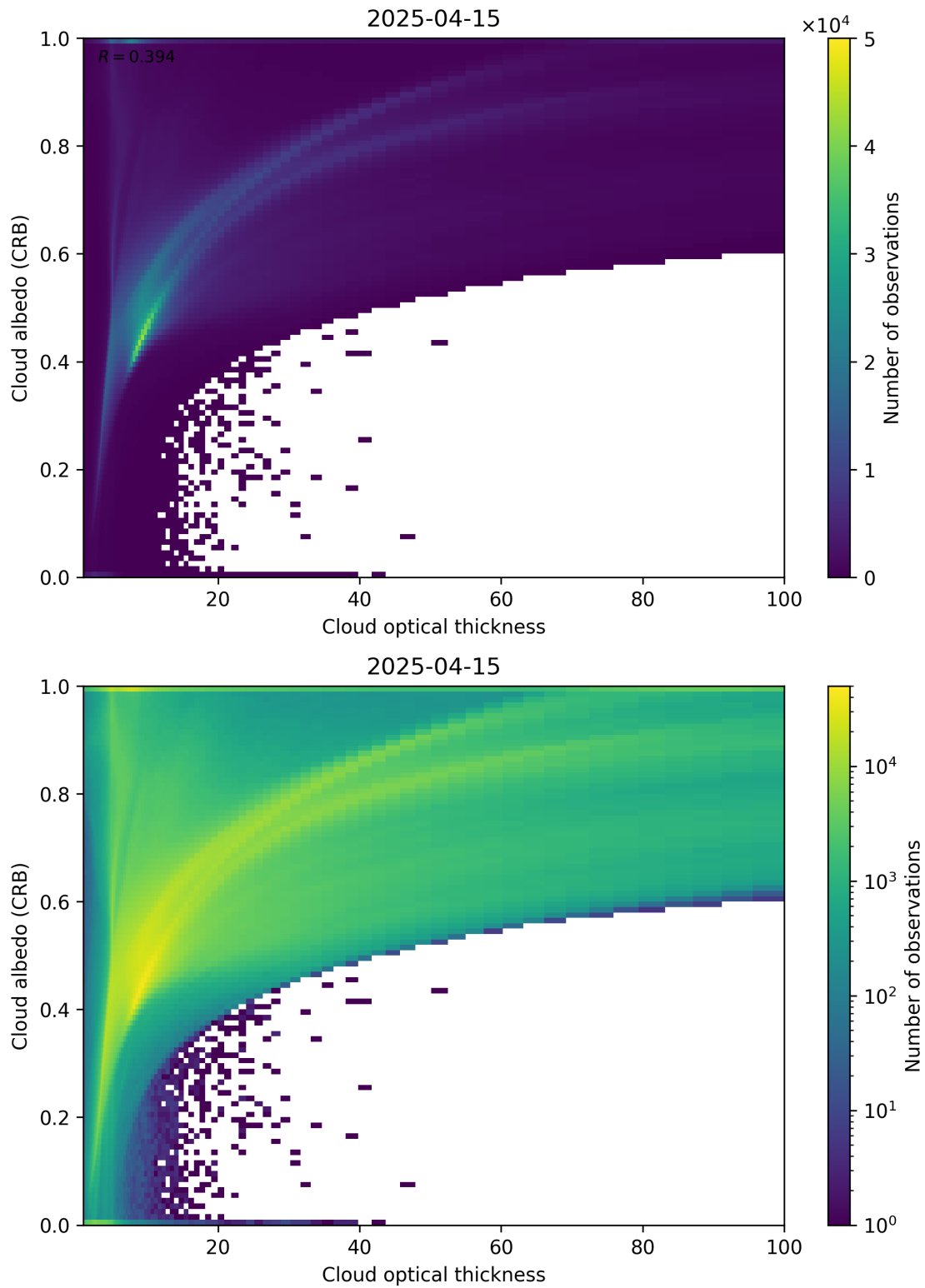
Figure 82: Scatter density plot of “Cloud optical thickness” against “Cloud albedo (CRB)” for 2025-04-14 to 2025-04-16.
