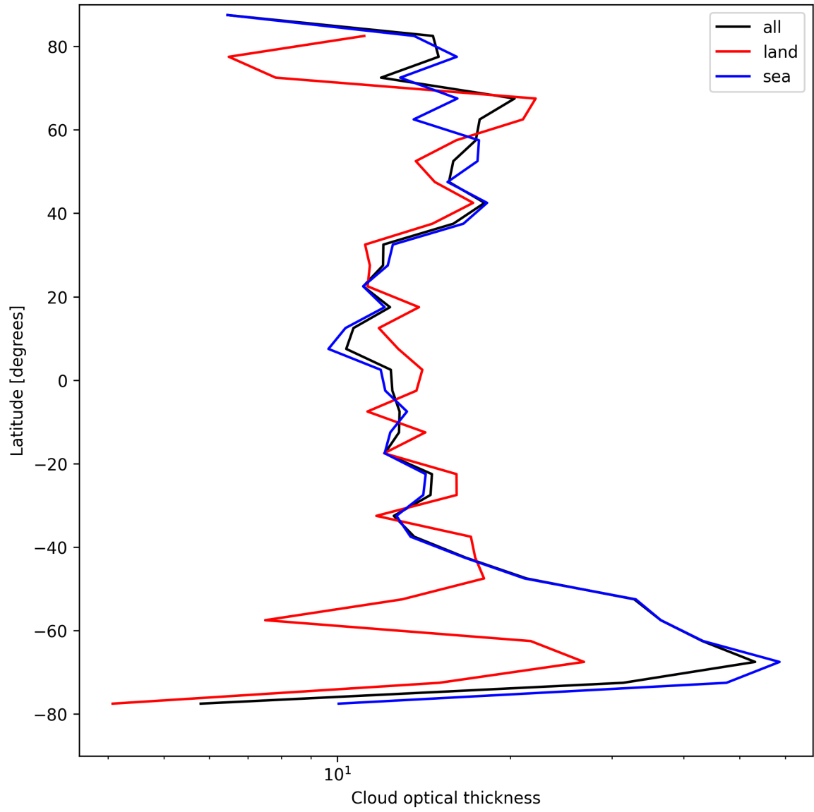
Figure 25: Zonal average of “Cloud optical thickness” for 2025-04-14 to 2025-04-16.
