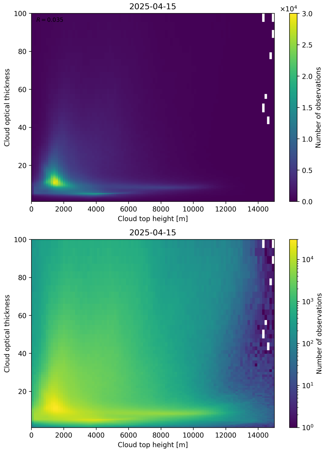
Figure 90: Scatter density plot of “Cloud top height” against “Cloud optical thickness” for 2025-04-14 to 2025-04-16.
