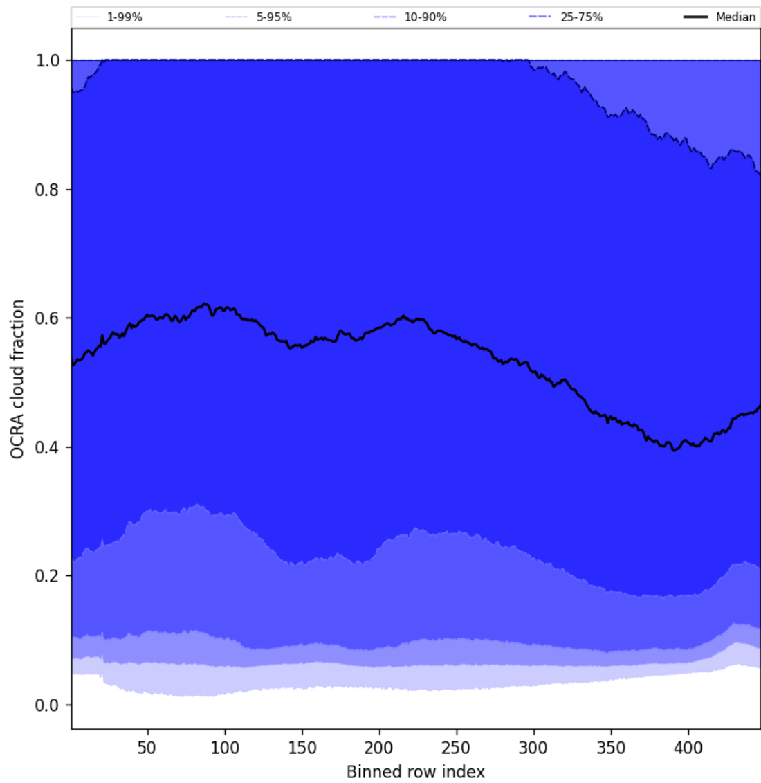
Figure 66: Along track statistics of “OCRA cloud fraction” for 2025-04-14 to 2025-04-16
