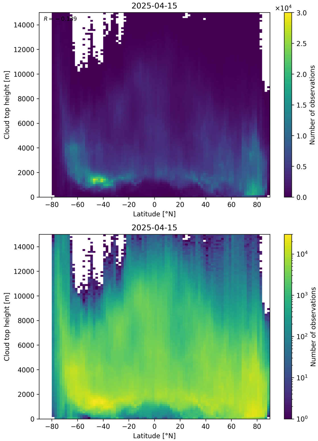
Figure 97: Scatter density plot of “Latitude” against “Cloud top height” for 2025-04-14 to 2025-04-16.
