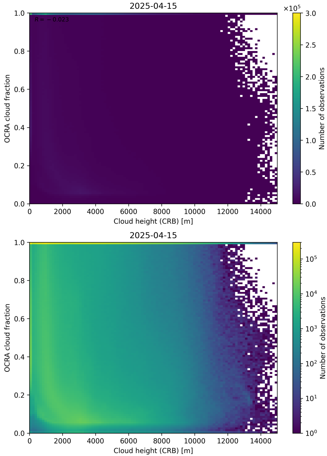
Figure 81: Scatter density plot of “Cloud height (CRB)” against “OCRA cloud fraction” for 2025-04-14 to 2025-04-16.
