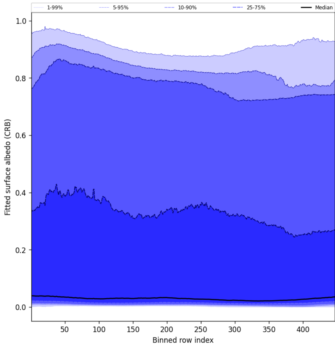
Figure 62: Along track statistics of “Fitted surface albedo (CRB)” for 2025-04-14 to 2025-04-16
