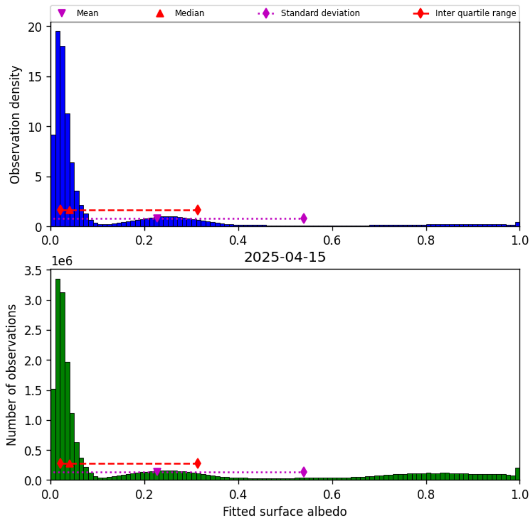
Figure 45: Histogram of “Fitted surface albedo” for 2025-04-14 to 2025-04-16
