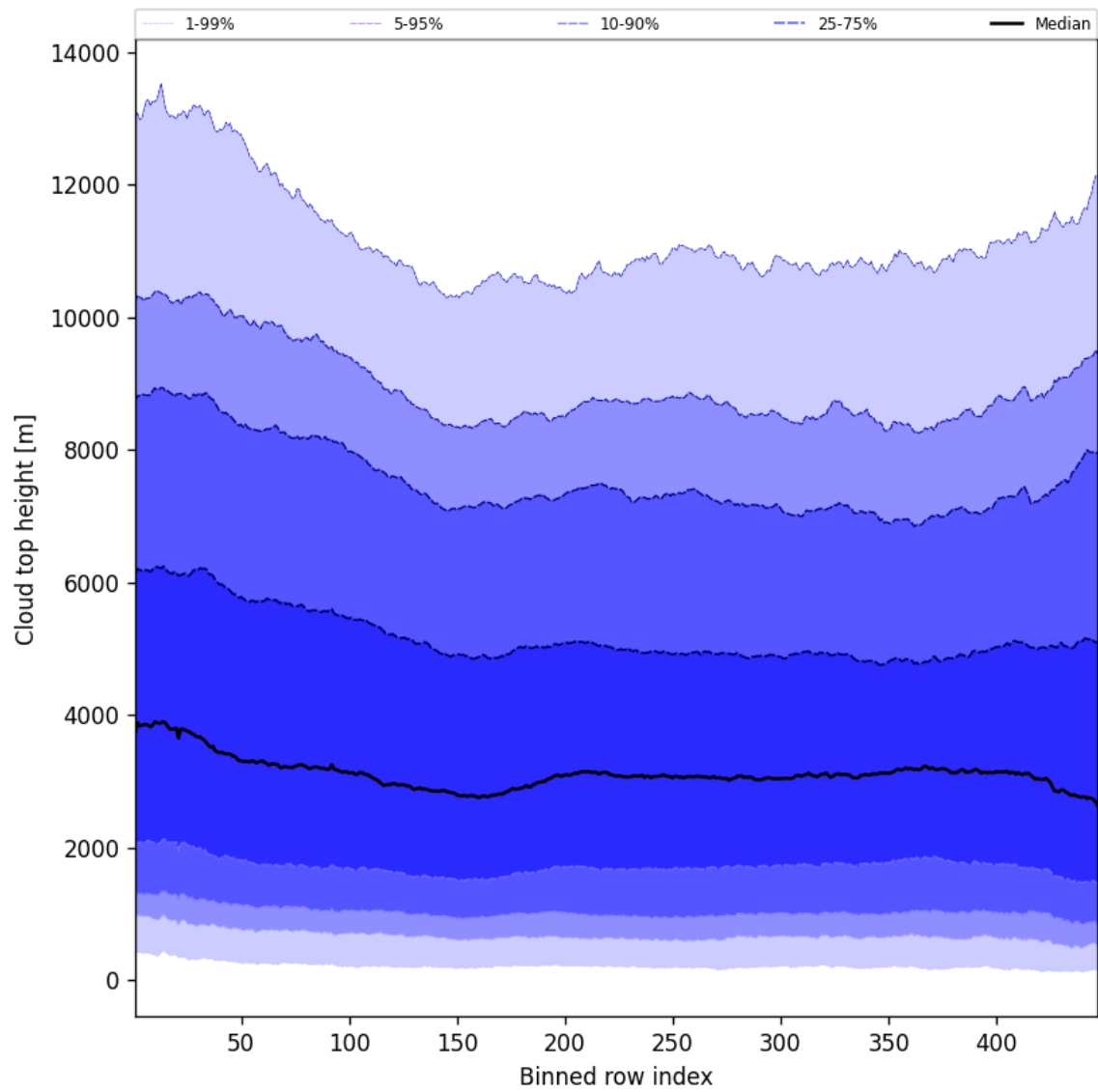
Figure 56: Along track statistics of “Cloud top height” for 2025-04-14 to 2025-04-16
