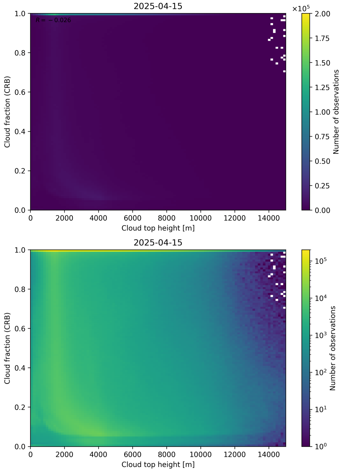
Figure 88: Scatter density plot of “Cloud top height” against “Cloud fraction (CRB)” for 2025-04-14 to 2025-04-16.
