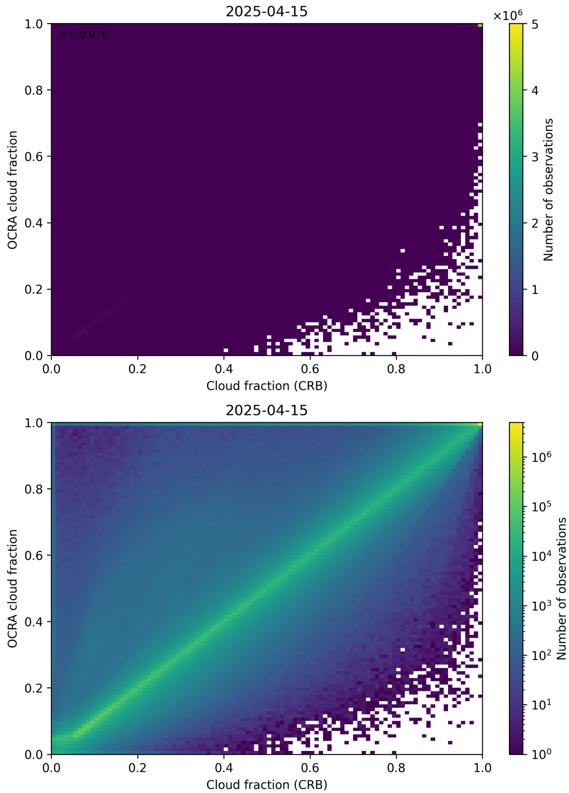
Figure 78: Scatter density plot of “Cloud fraction (CRB)” against “OCRA cloud fraction” for 2025-04-14 to 2025-04-16.
