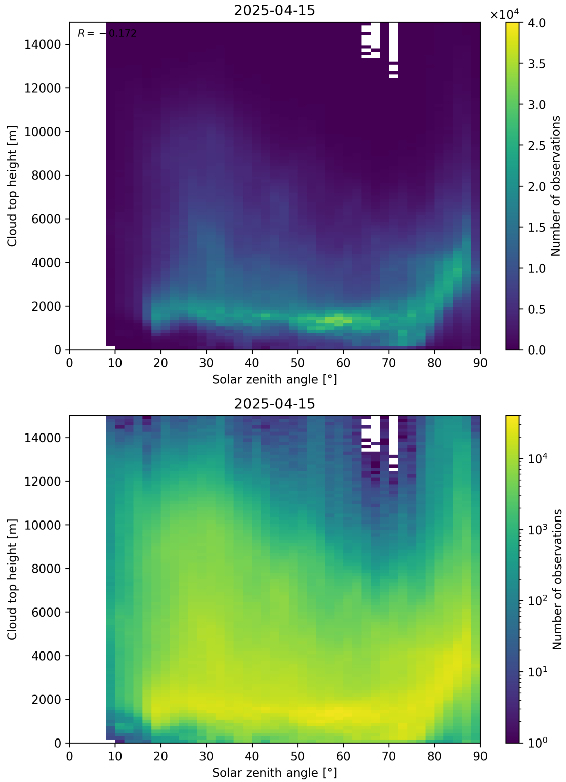
Figure 104: Scatter density plot of “Solar zenith angle” against “Cloud top height” for 2025-04-14 to 2025-04-16.
