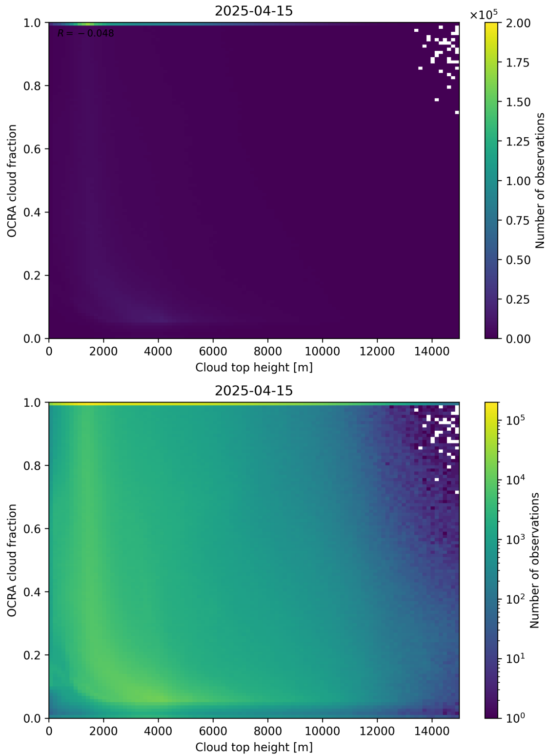
Figure 87: Scatter density plot of “Cloud top height” against “OCRA cloud fraction” for 2025-04-14 to 2025-04-16.
