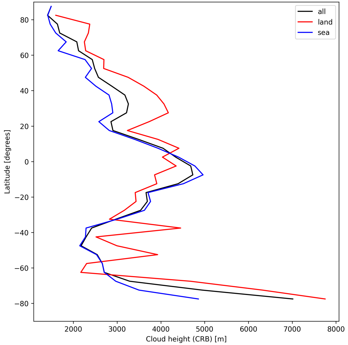
Figure 27: Zonal average of “Cloud height (CRB)” for 2025-04-14 to 2025-04-16.
