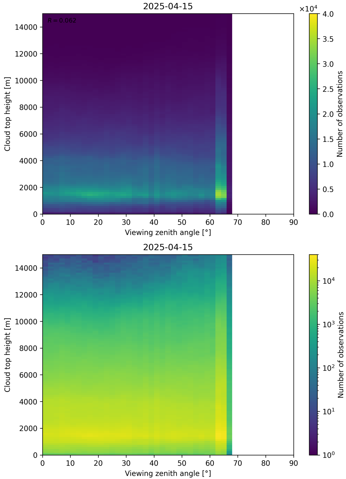
Figure 112: Scatter density plot of “Viewing zenith angle” against “Cloud top height” for 2025-04-14 to 2025-04-16.
