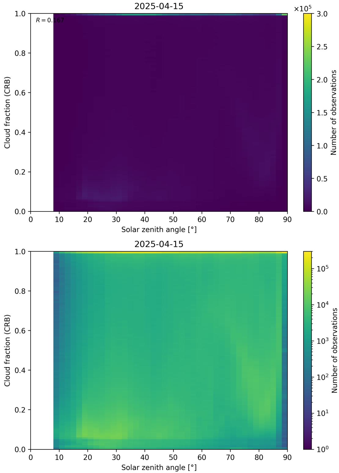
Figure 101: Scatter density plot of “Solar zenith angle” against “Cloud fraction (CRB)” for 2025-04-14 to 2025-04-16.
