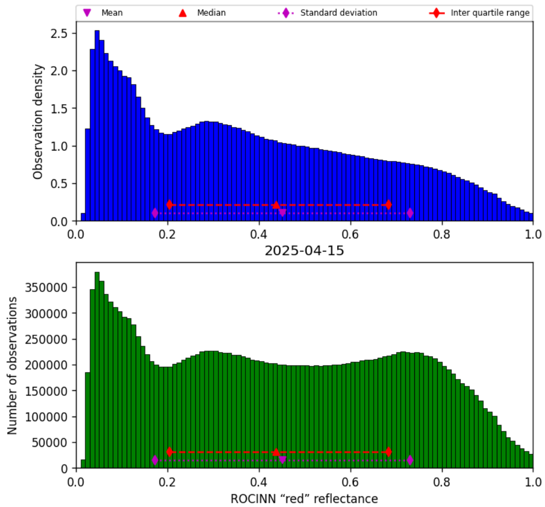
Figure 53: Histogram of “ROCINN “red” reflectance” for 2025-04-14 to 2025-04-16
