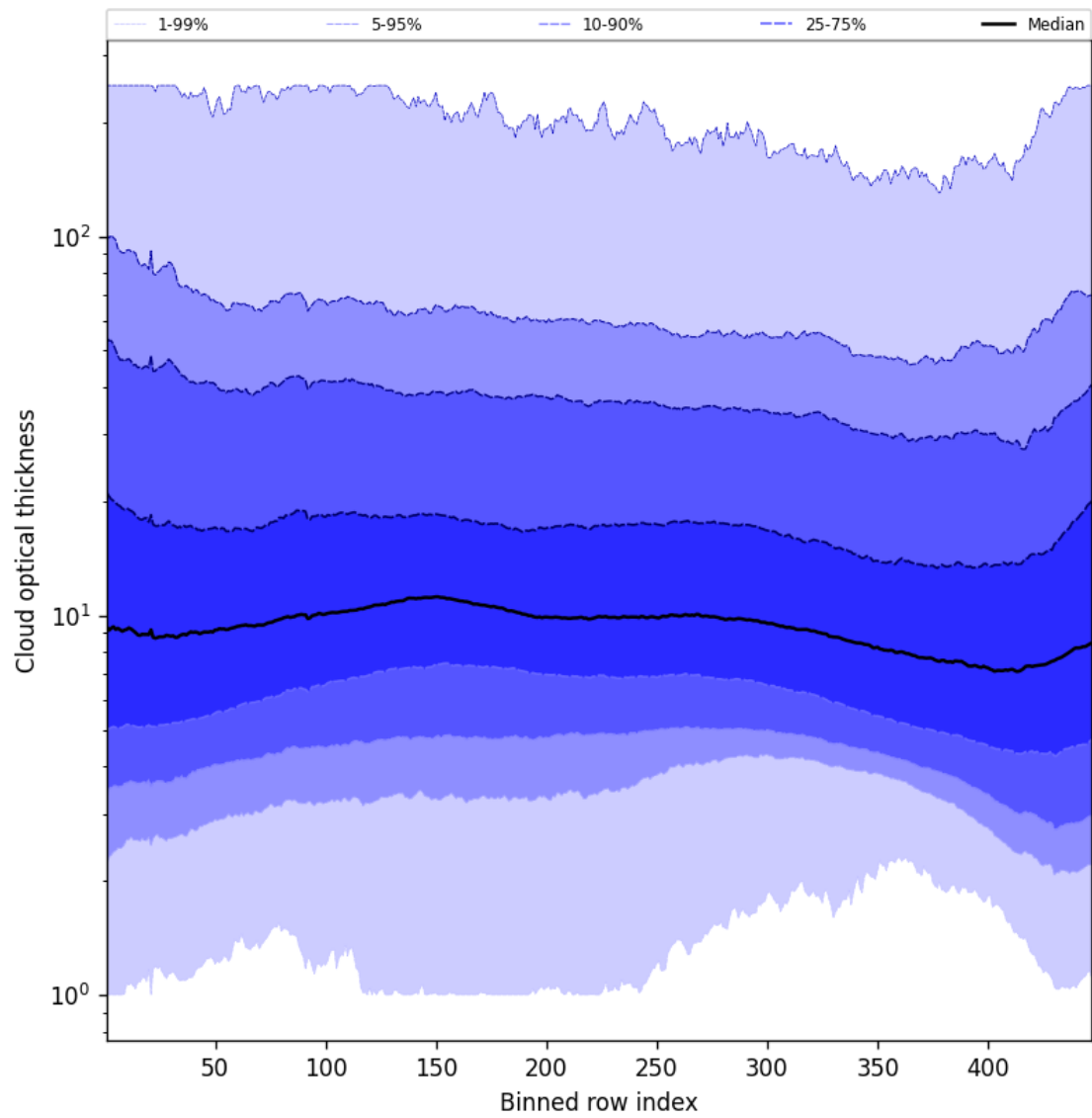
Figure 57: Along track statistics of “Cloud optical thickness” for 2025-04-14 to 2025-04-16
