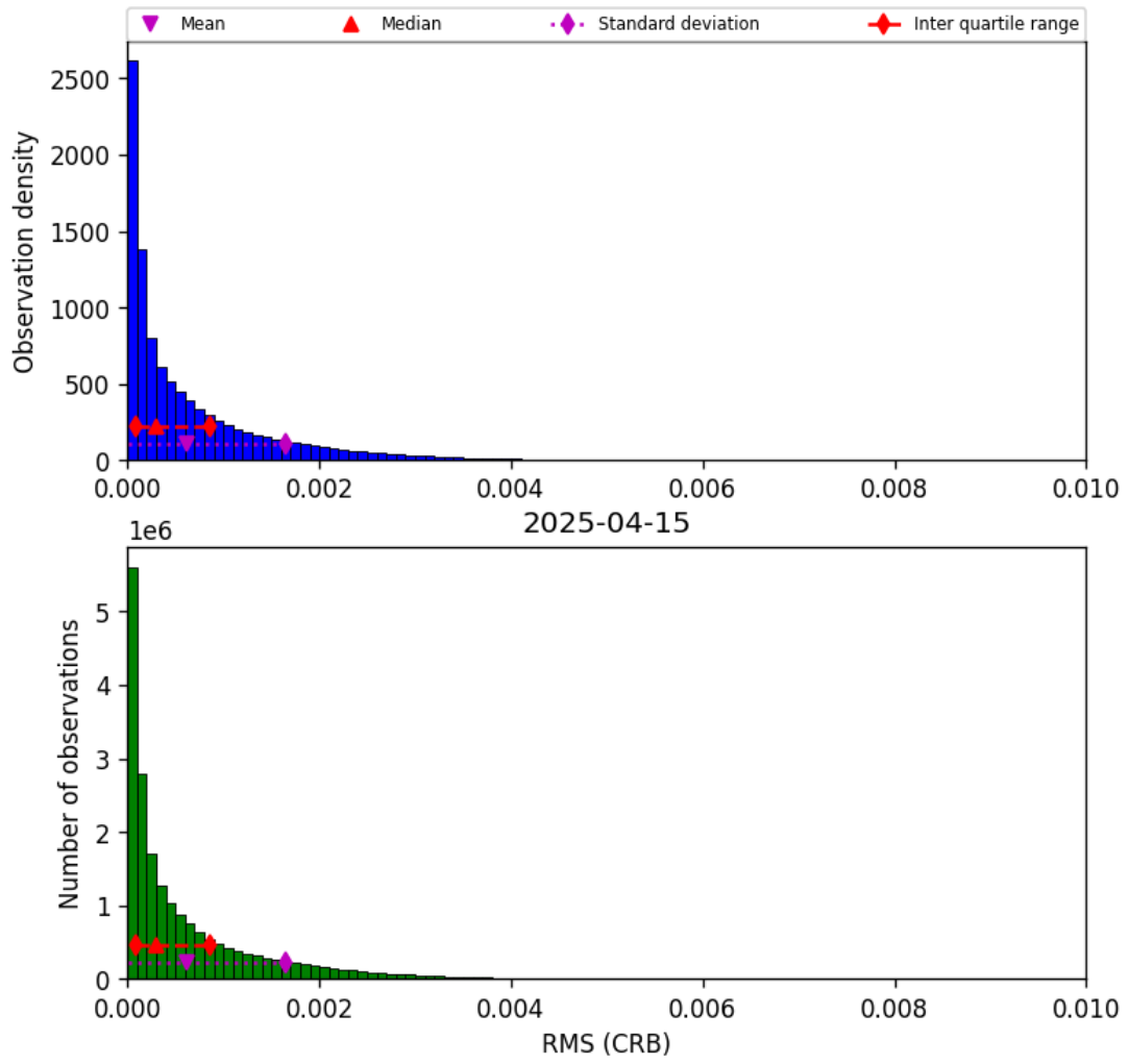
Figure 48: Histogram of “RMS (CRB)” for 2025-04-14 to 2025-04-16
