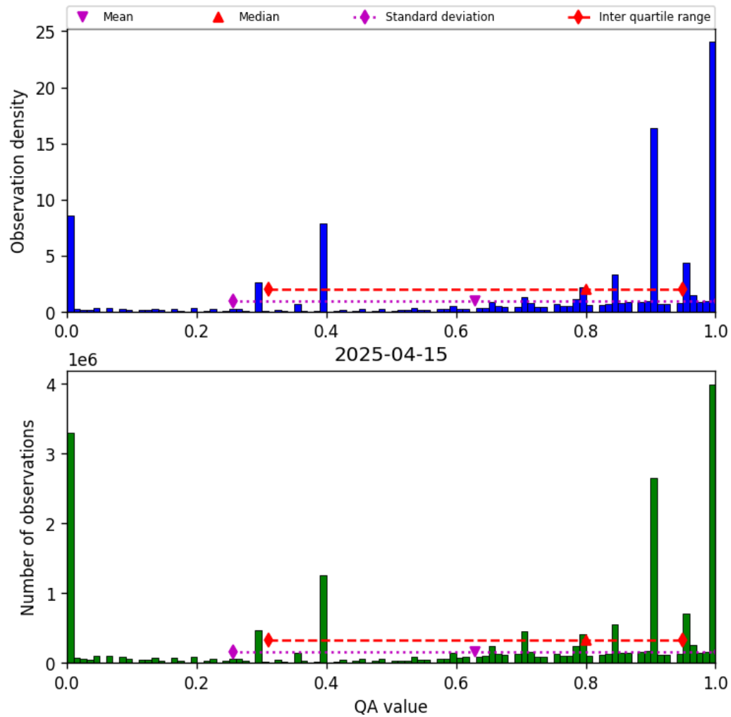
Figure 38: Histogram of “QA value” for 2025-04-14 to 2025-04-16
