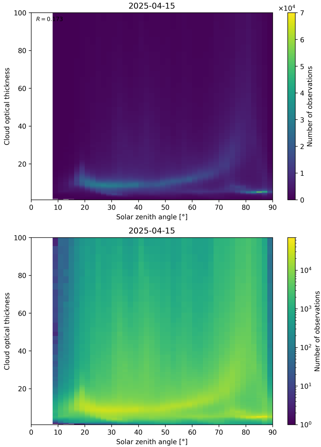
Figure 103: Scatter density plot of “Solar zenith angle” against “Cloud optical thickness” for 2025-04-14 to 2025-04-16.
