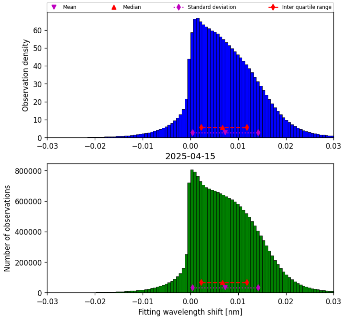
Figure 49: Histogram of “Fitting wavelength shift” for 2025-04-14 to 2025-04-16
