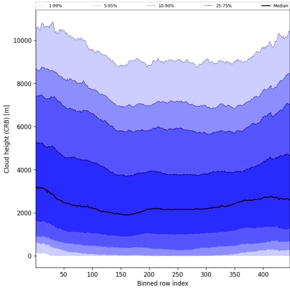
Figure 59: Along track statistics of “Cloud height (CRB)” for 2025-04-14 to 2025-04-16
