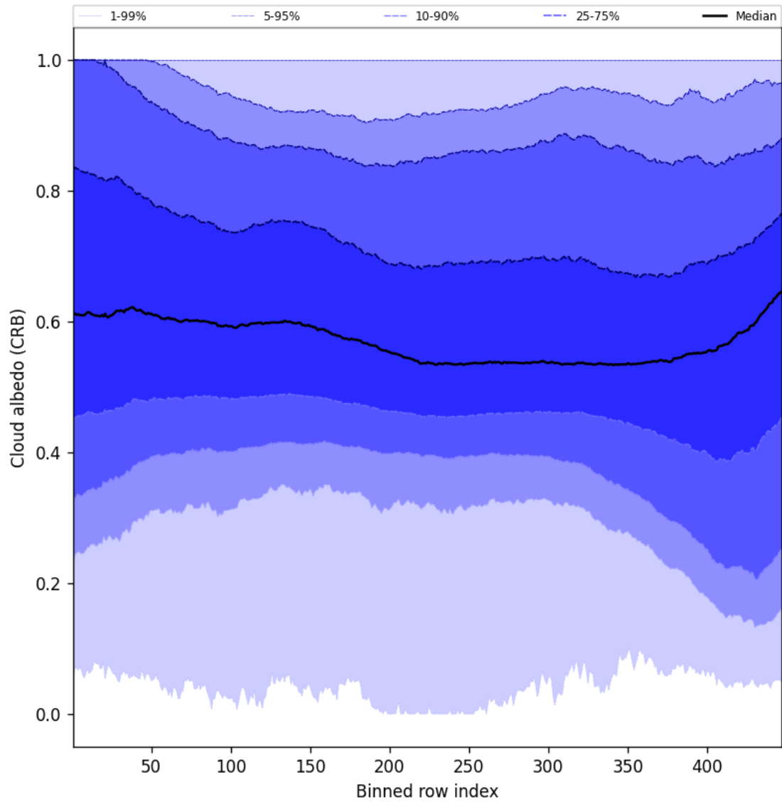
Figure 60: Along track statistics of “Cloud albedo (CRB)” for 2025-04-14 to 2025-04-16
