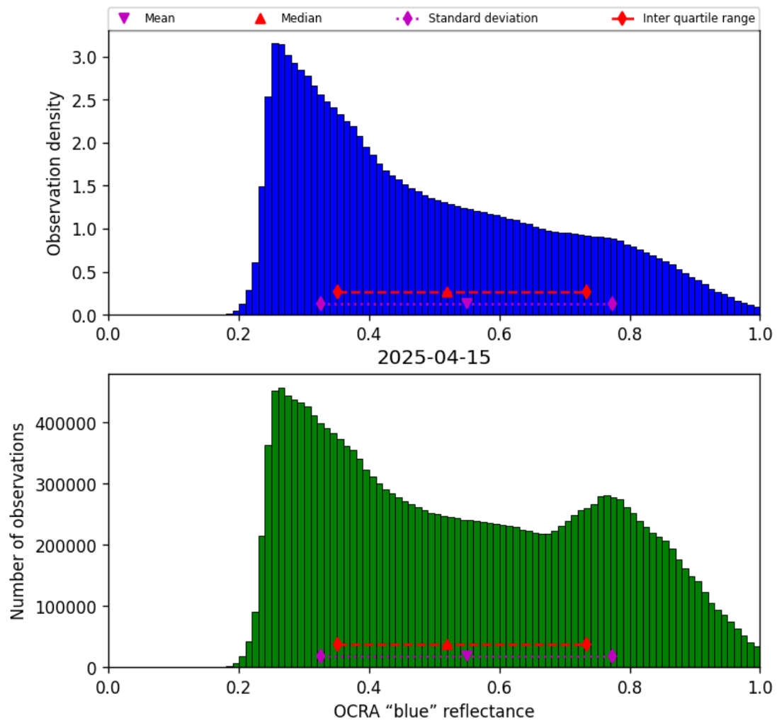
Figure 51: Histogram of “OCRA “blue” reflectance” for 2025-04-14 to 2025-04-16
