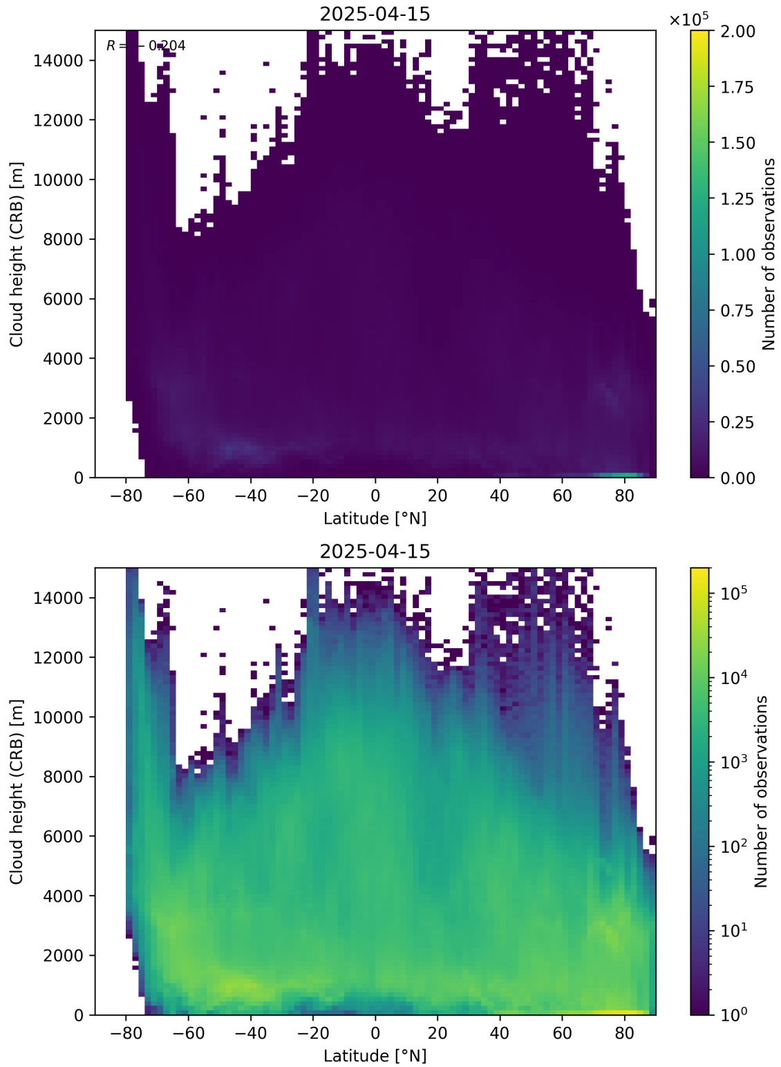
Figure 95: Scatter density plot of “Latitude” against “Cloud height (CRB)” for 2025-04-14 to 2025-04-16.
