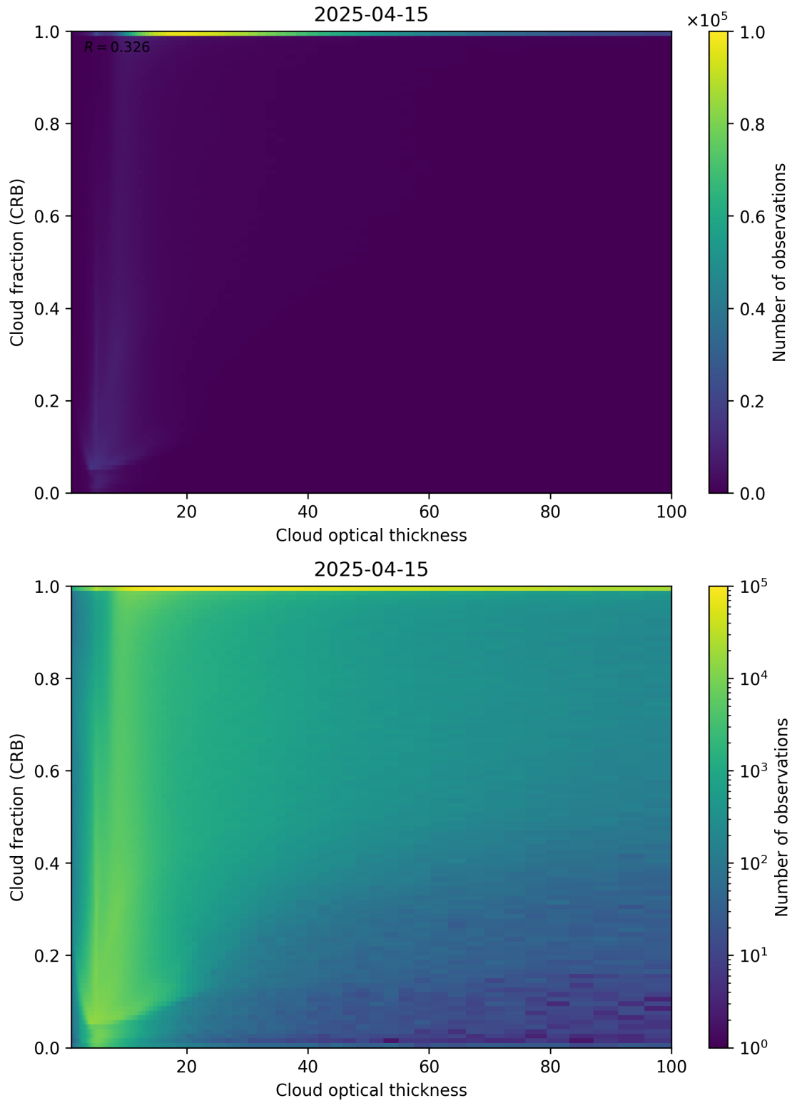
Figure 84: Scatter density plot of “Cloud optical thickness” against “Cloud fraction (CRB)” for 2025-04-14 to 2025-04-16.
