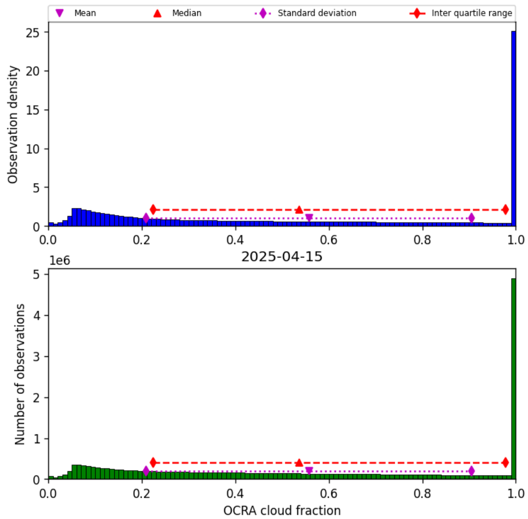
Figure 50: Histogram of “OCRA cloud fraction” for 2025-04-14 to 2025-04-16
