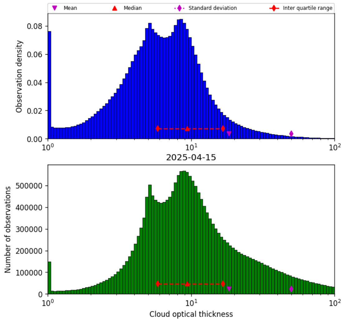
Figure 41: Histogram of “Cloud optical thickness” for 2025-04-14 to 2025-04-16
