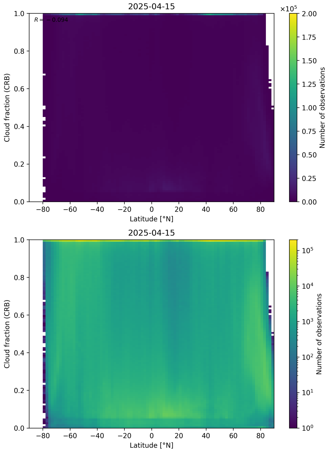
Figure 94: Scatter density plot of “Latitude” against “Cloud fraction (CRB)” for 2025-04-14 to 2025-04-16.
