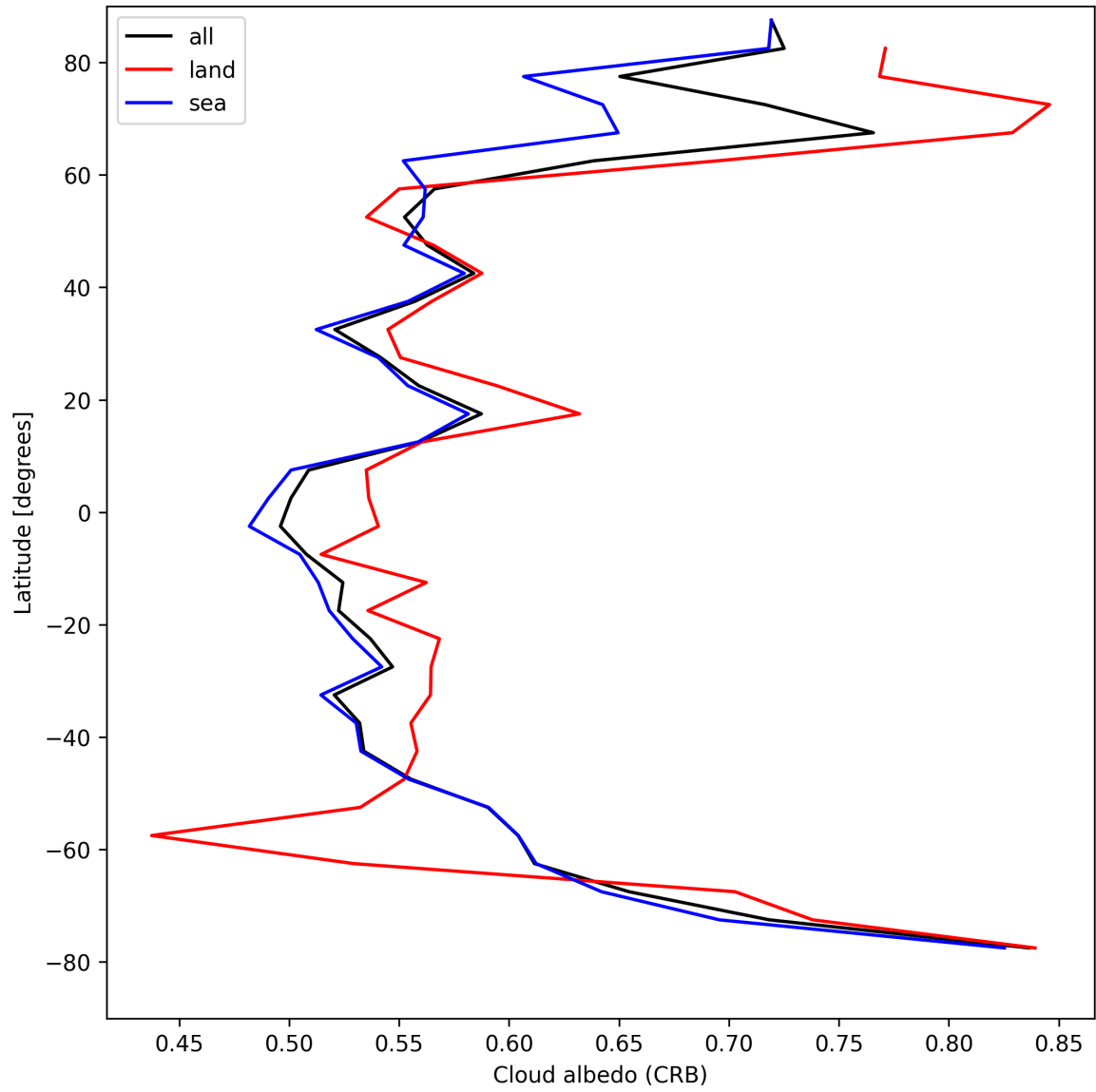
Figure 28: Zonal average of “Cloud albedo (CRB)” for 2025-04-14 to 2025-04-16.
