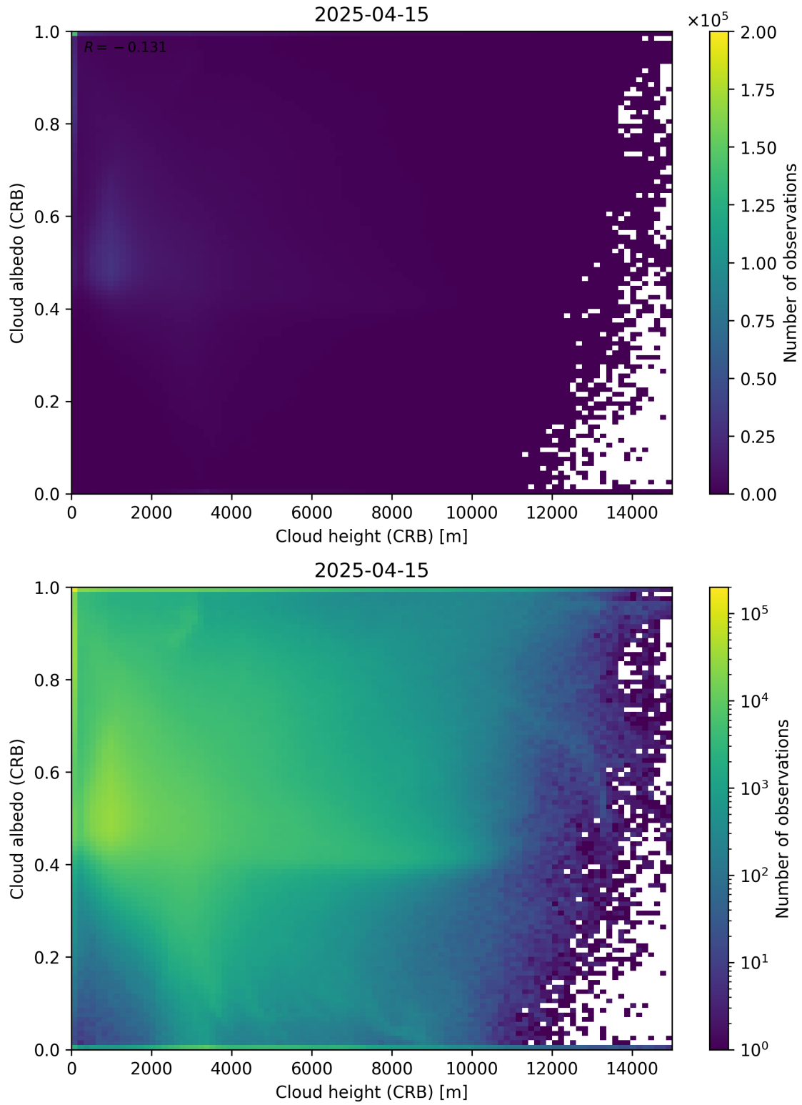
Figure 80: Scatter density plot of “Cloud height (CRB)” against “Cloud albedo (CRB)” for 2025-04-14 to 2025-04-16.
