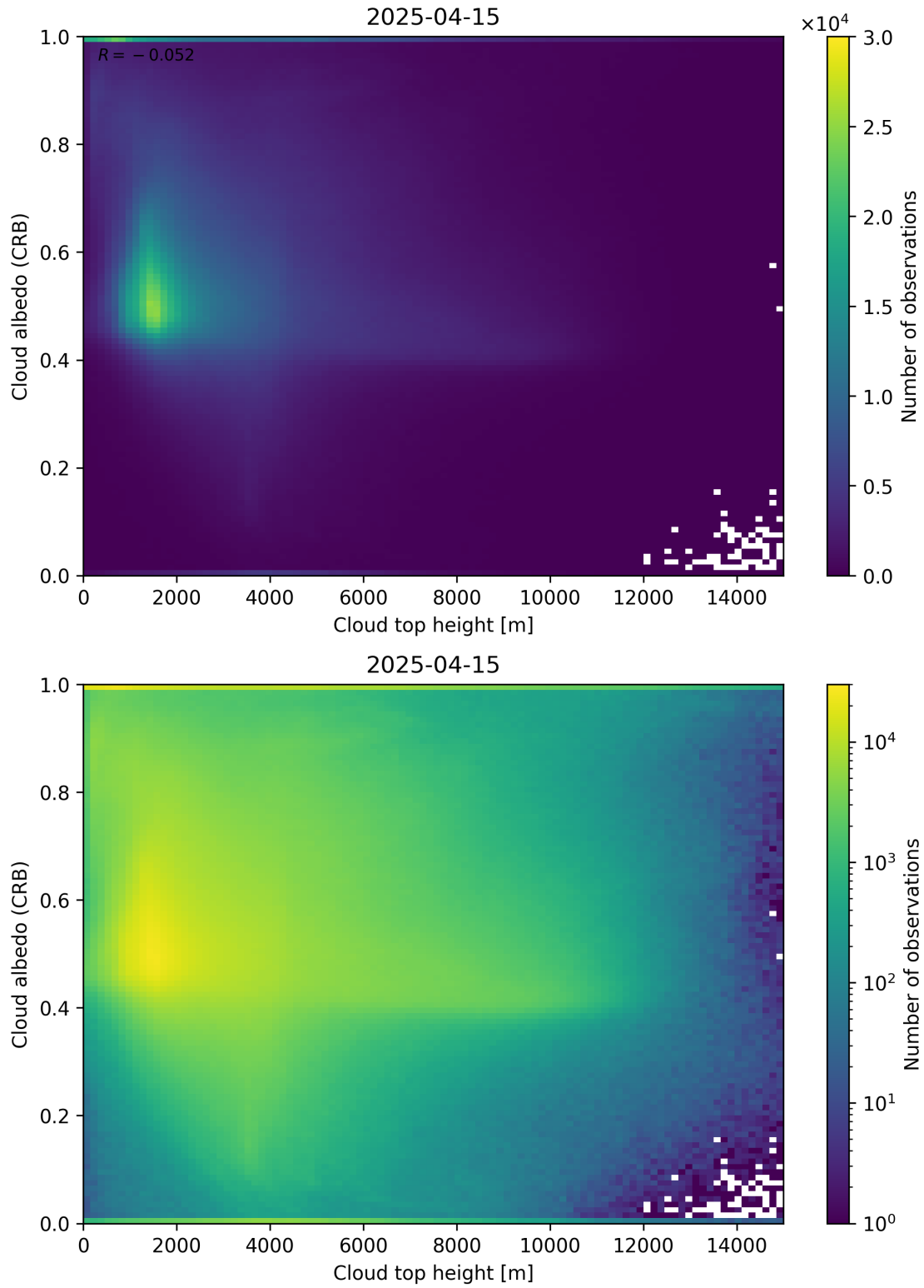
Figure 86: Scatter density plot of “Cloud top height” against “Cloud albedo (CRB)” for 2025-04-14 to 2025-04-16.
