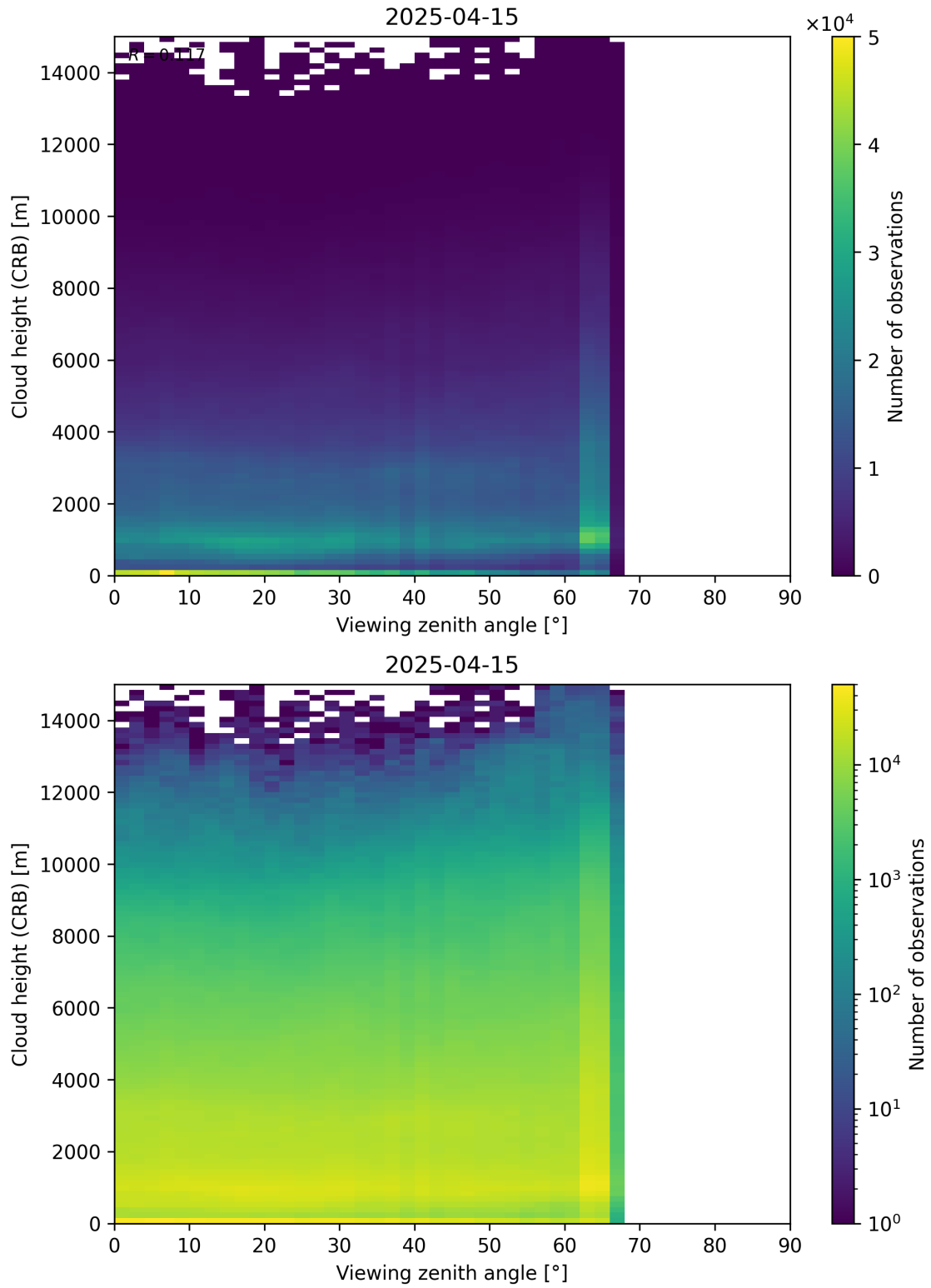
Figure 110: Scatter density plot of “Viewing zenith angle” against “Cloud height (CRB)” for 2025-04-14 to 2025-04-16.
