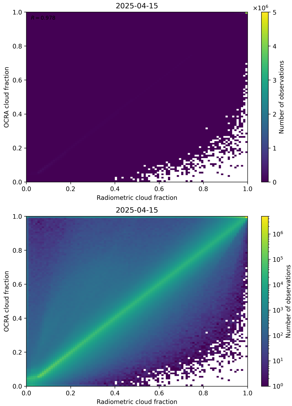
Figure 72: Scatter density plot of “Radiometric cloud fraction” against “OCRA cloud fraction” for 2025-04-14 to 2025-04-16.
