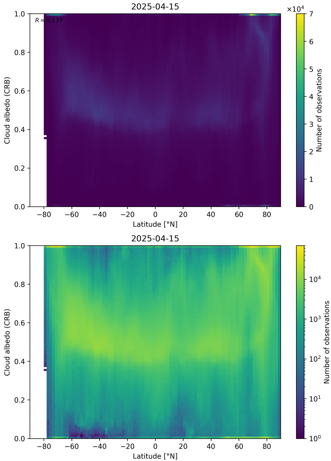
Figure 91: Scatter density plot of “Latitude” against “Cloud albedo (CRB)” for 2025-04-14 to 2025-04-16.
