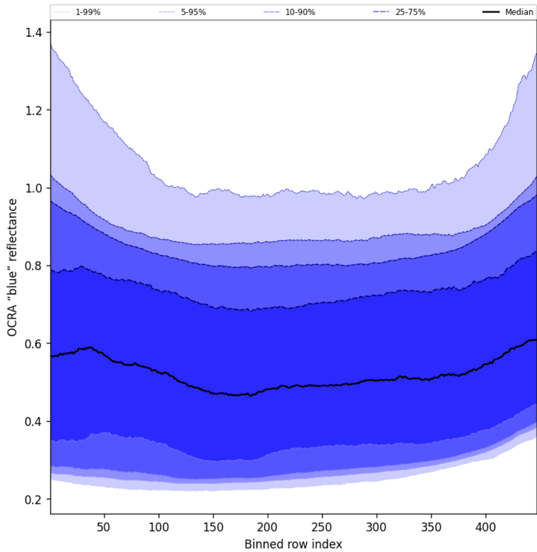
Figure 67: Along track statistics of “OCRA “blue” reflectance” for 2025-04-14 to 2025-04-16
