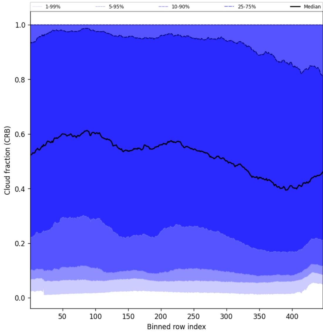
Figure 58: Along track statistics of “Cloud fraction (CRB)” for 2025-04-14 to 2025-04-16
