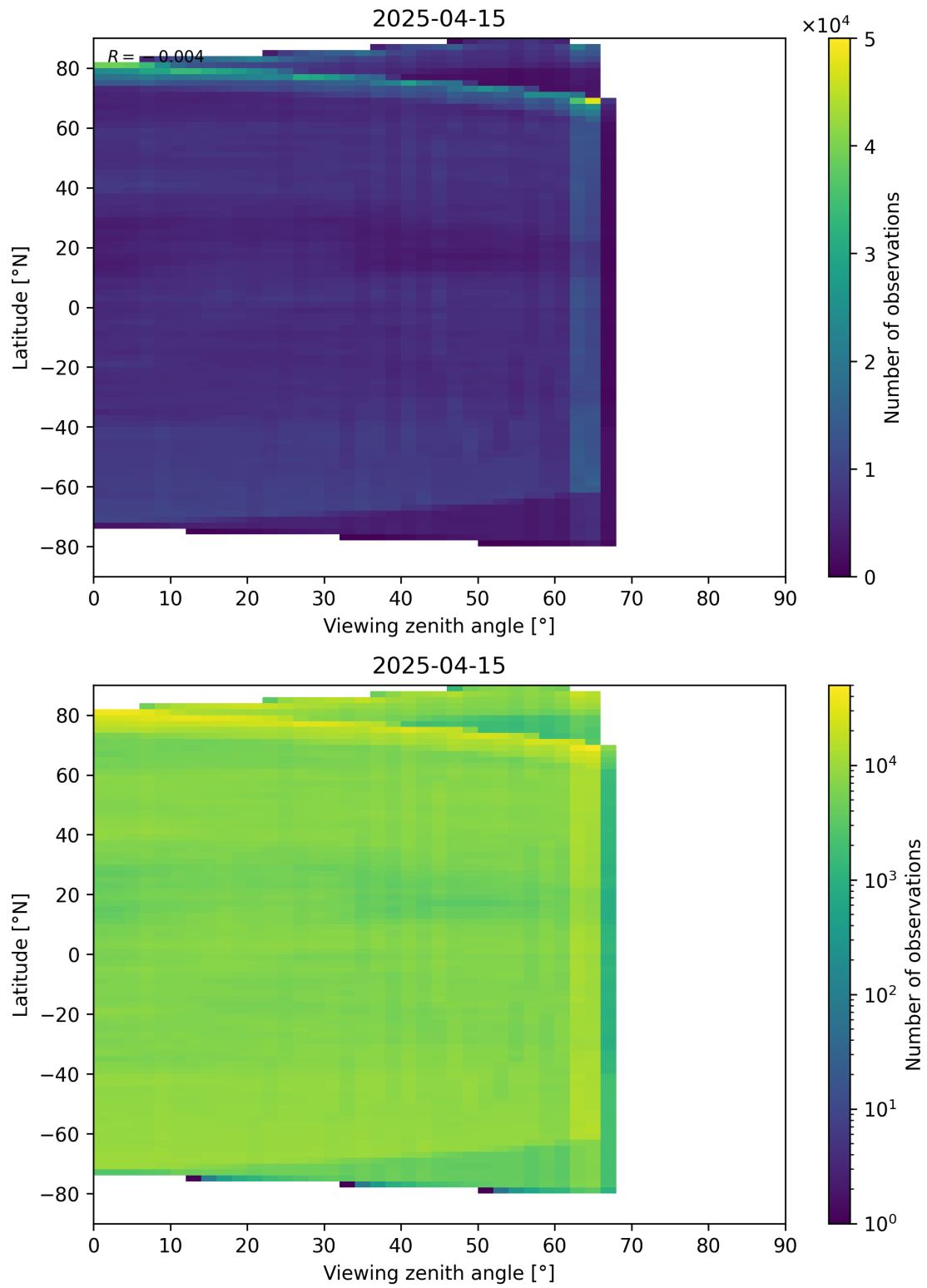
Figure 113: Scatter density plot of “Viewing zenith angle” against “Latitude” for 2025-04-14 to 2025-04-16.
