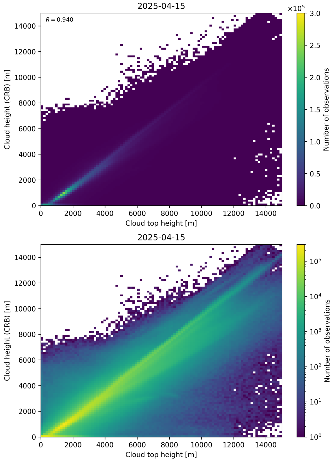
Figure 89: Scatter density plot of “Cloud top height” against “Cloud height (CRB)” for 2025-04-14 to 2025-04-16.
