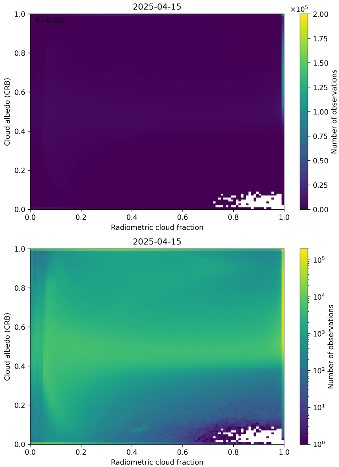
Figure 71: Scatter density plot of “Radiometric cloud fraction” against “Cloud albedo (CRB)” for 2025-04-14 to 2025-04-16.
