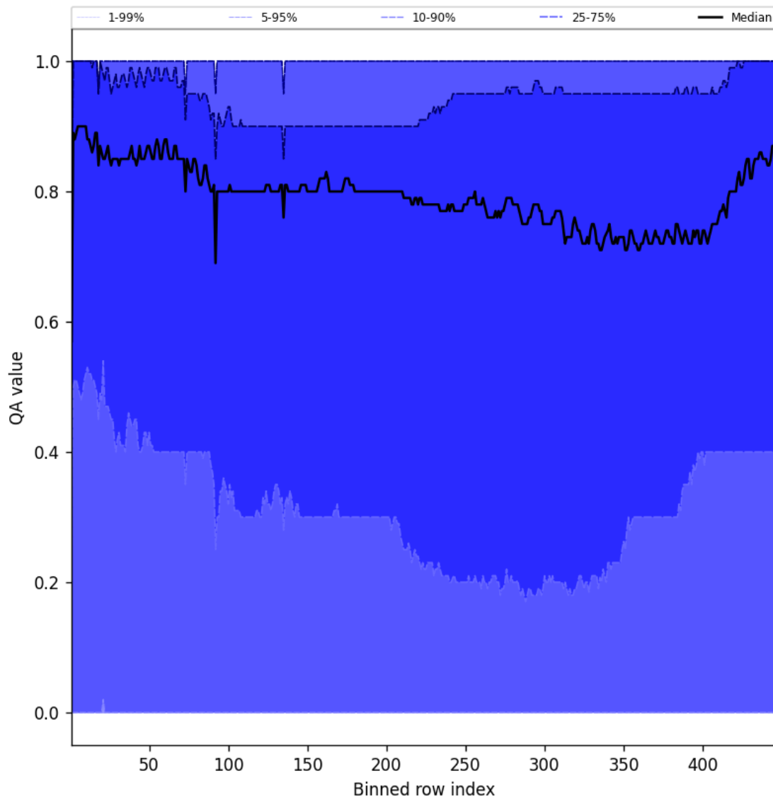
Figure 54: Along track statistics of "QA value" for 2025-04-14 to 2025-04-16
