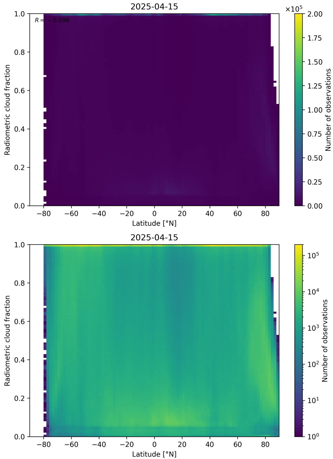
Figure 92: Scatter density plot of “Latitude” against “Radiometric cloud fraction” for 2025-04-14 to 2025-04-16.
