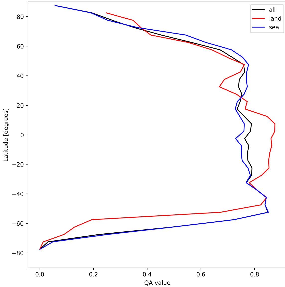
Figure 22: Zonal average of “QA value” for 2025-04-14 to 2025-04-16.
