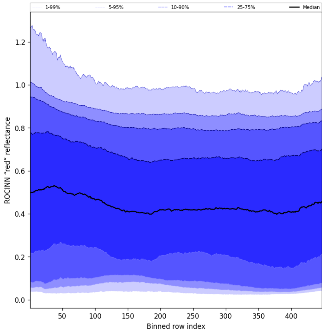
Figure 69: Along track statistics of “ROCINN “red” reflectance” for 2025-04-14 to 2025-04-16
