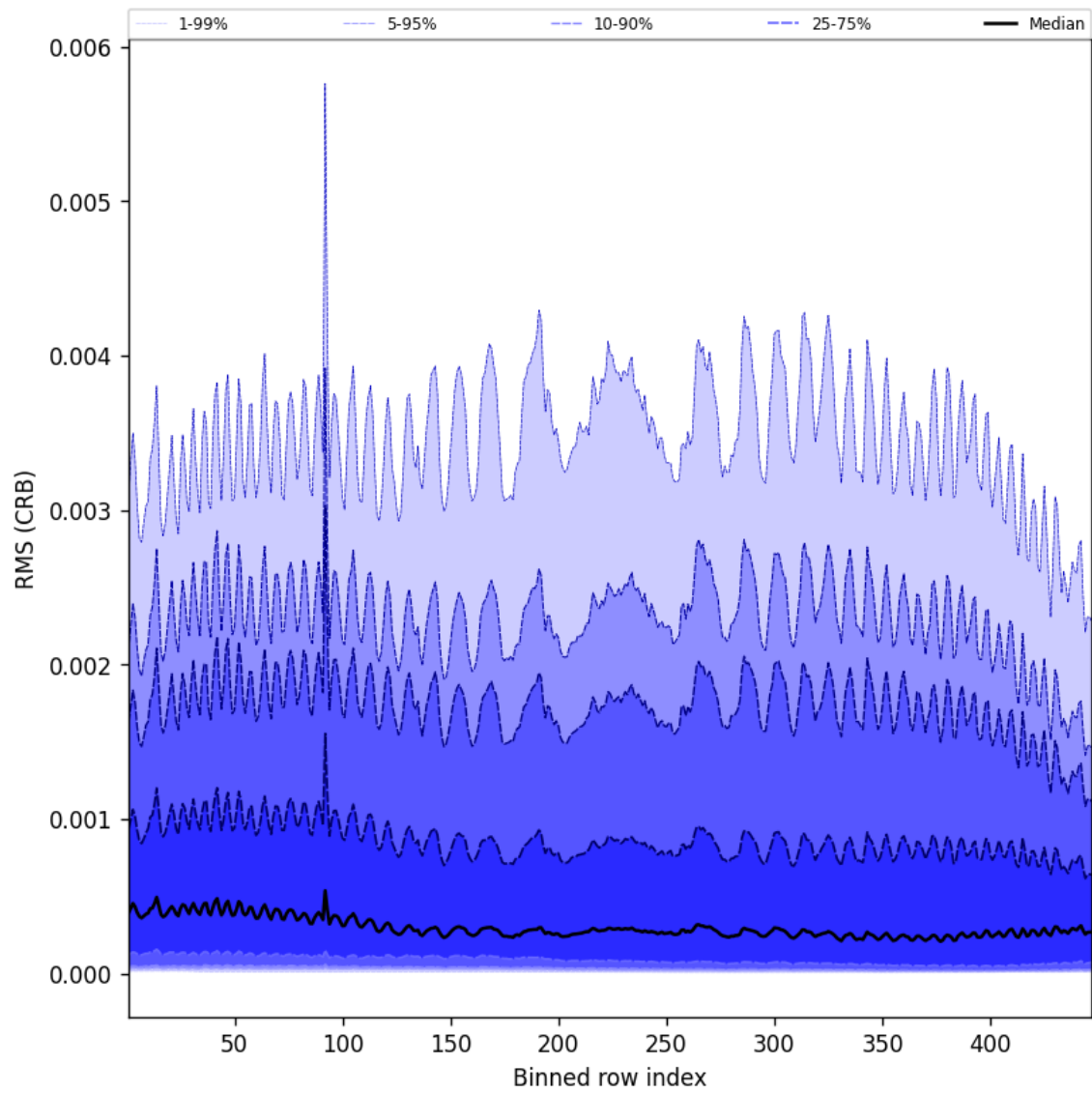
Figure 64: Along track statistics of "RMS (CRB)" for 2025-04-14 to 2025-04-16
