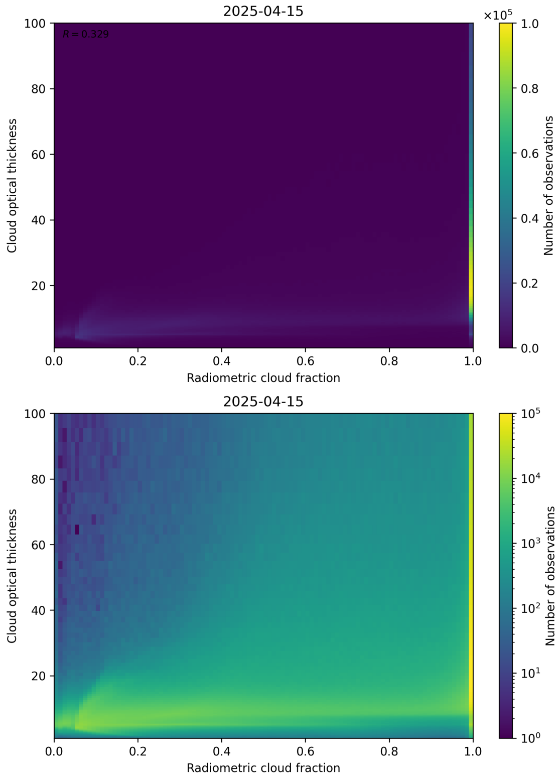
Figure 75: Scatter density plot of “Radiometric cloud fraction” against “Cloud optical thickness” for 2025-04-14 to 2025-04-16.
