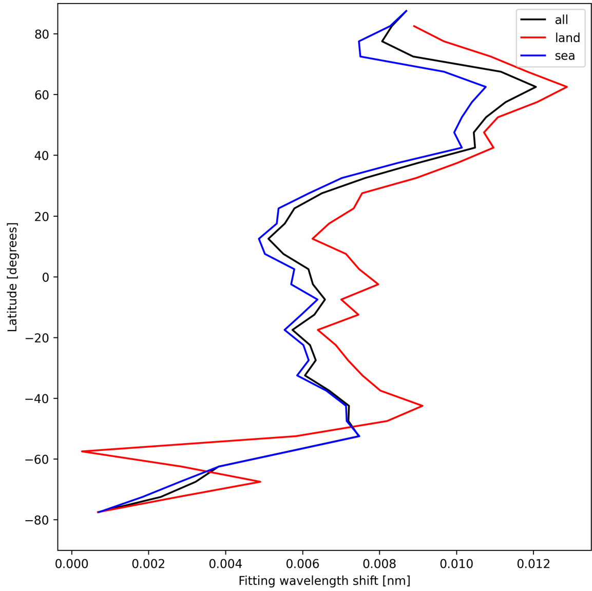
Figure 33: Zonal average of “Fitting wavelength shift” for 2025-04-14 to 2025-04-16.
