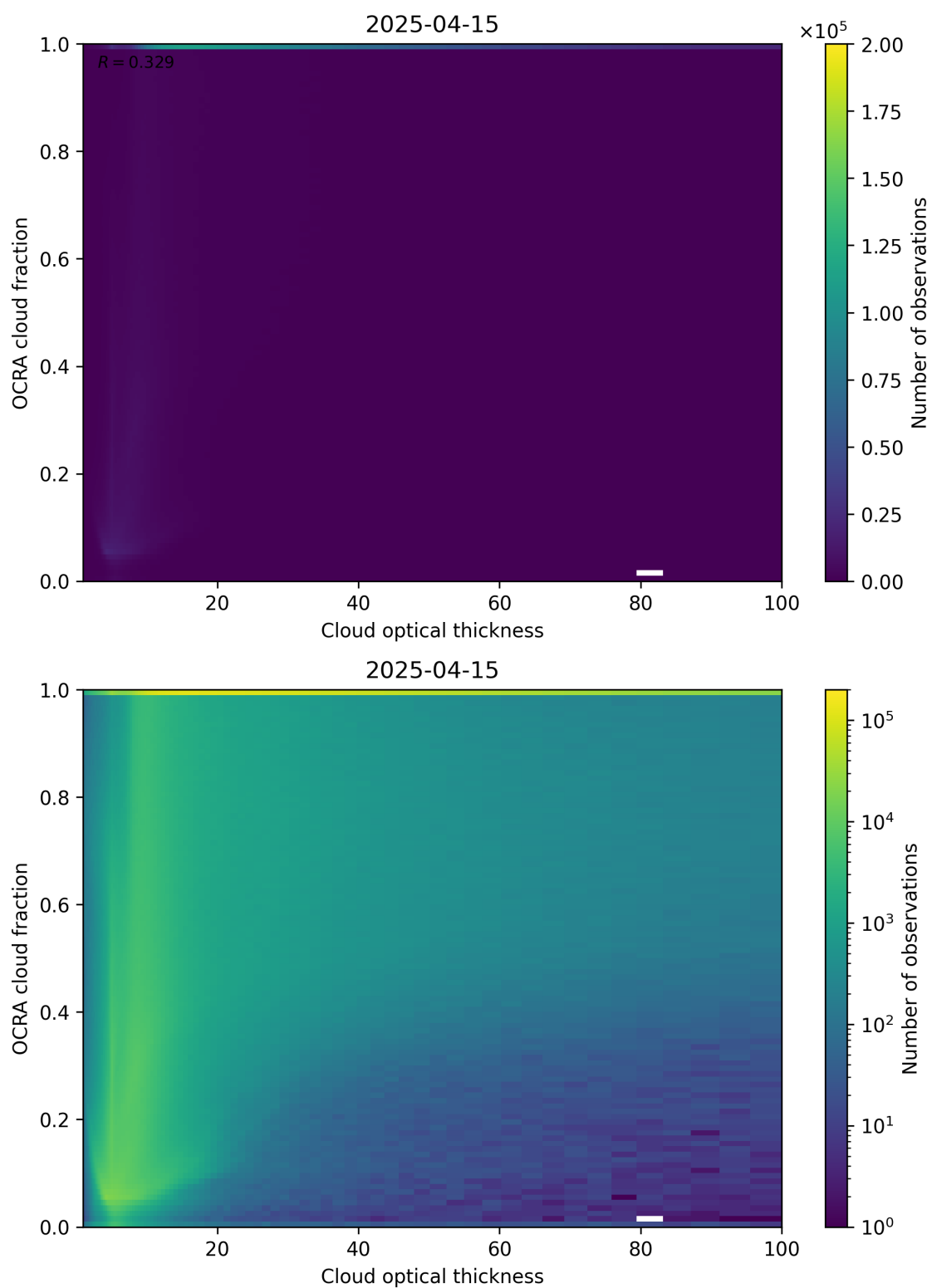
Figure 83: Scatter density plot of “Cloud optical thickness” against “OCRA cloud fraction” for 2025-04-14 to 2025-04-16.
