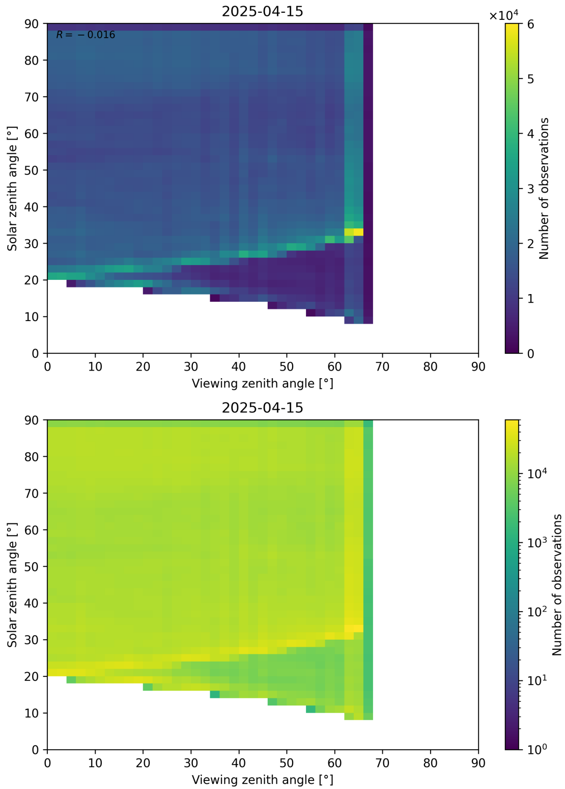
Figure 114: Scatter density plot of “Viewing zenith angle” against “Solar zenith angle” for 2025-04-14 to 2025-04-16.
