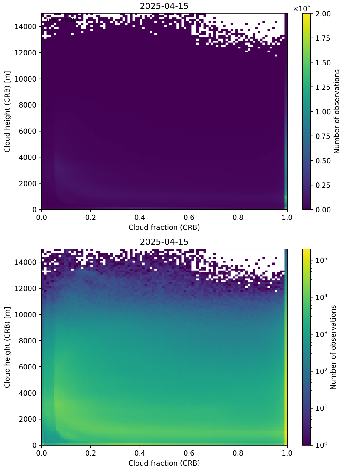
Figure 79: Scatter density plot of “Cloud fraction (CRB)” against “Cloud height (CRB)” for 2025-04-14 to 2025-04-16.
