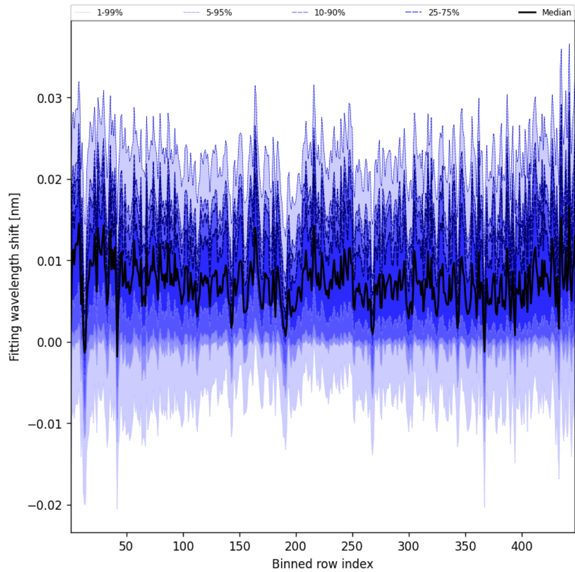
Figure 65: Along track statistics of “Fitting wavelength shift” for 2025-04-14 to 2025-04-16
