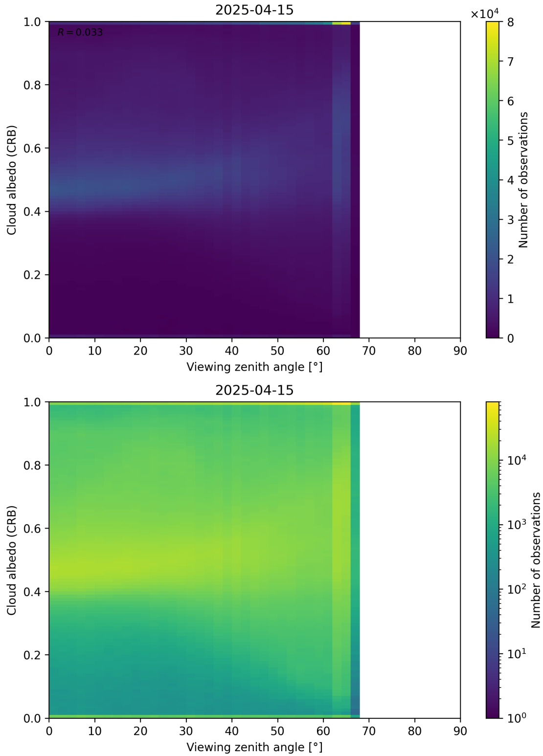
Figure 106: Scatter density plot of “Viewing zenith angle” against “Cloud albedo (CRB)” for 2025-04-14 to 2025-04-16.
