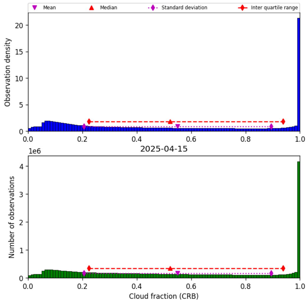
Figure 42: Histogram of “Cloud fraction (CRB)” for 2025-04-14 to 2025-04-16
