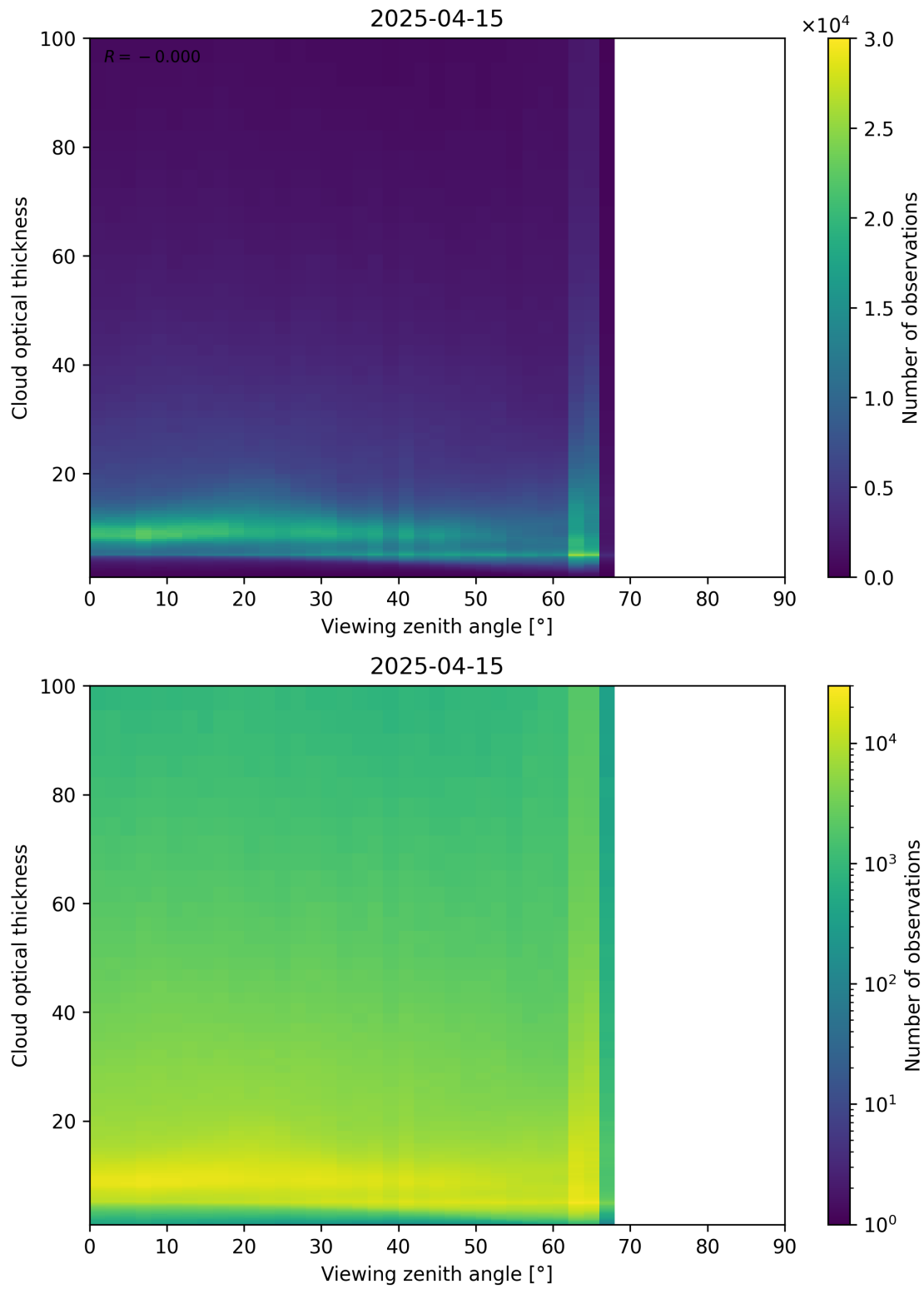
Figure 111: Scatter density plot of “Viewing zenith angle” against “Cloud optical thickness” for 2025-04-14 to 2025-04-16.
