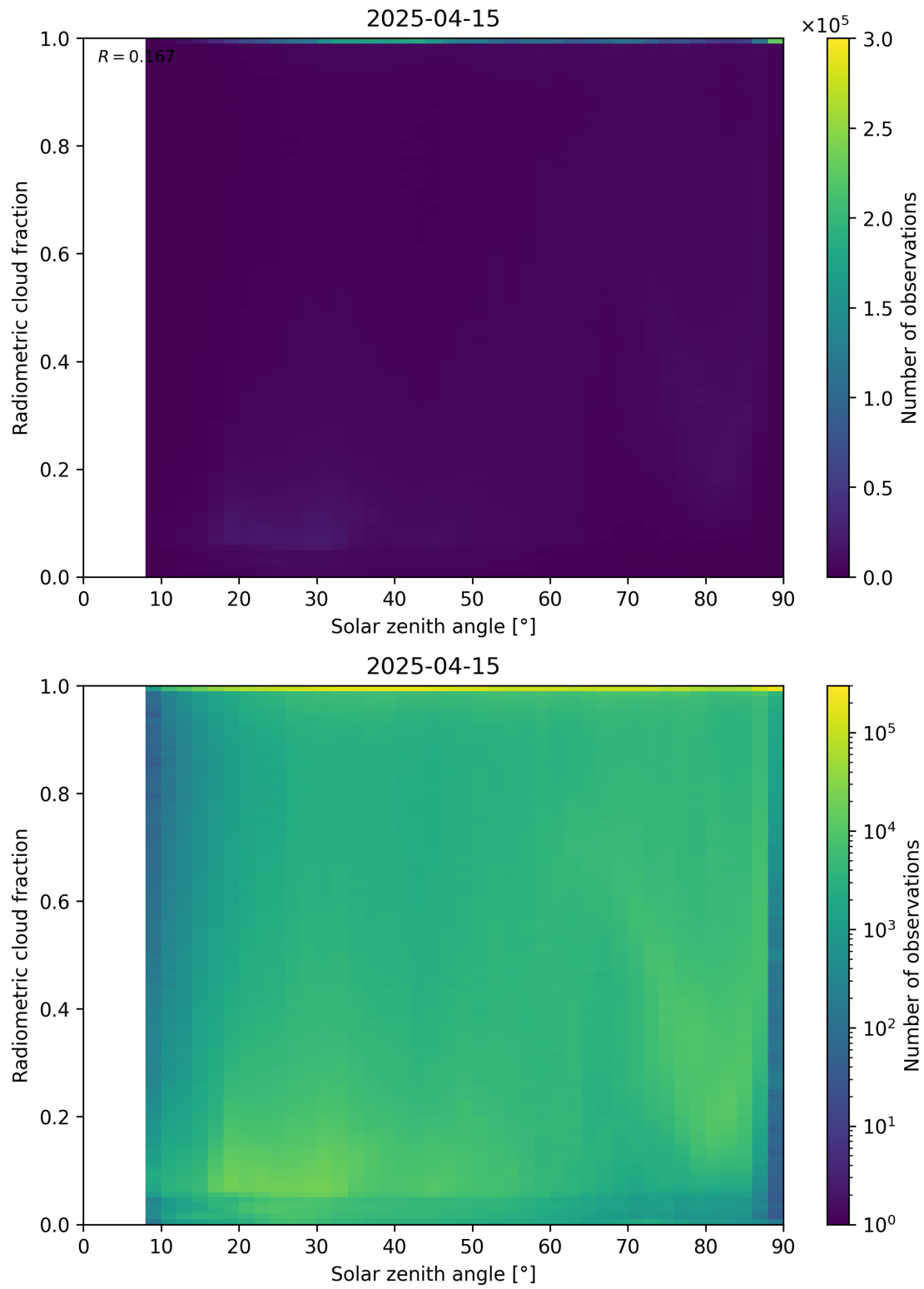
Figure 99: Scatter density plot of “Solar zenith angle” against “Radiometric cloud fraction” for 2025-04-14 to 2025-04-16.
