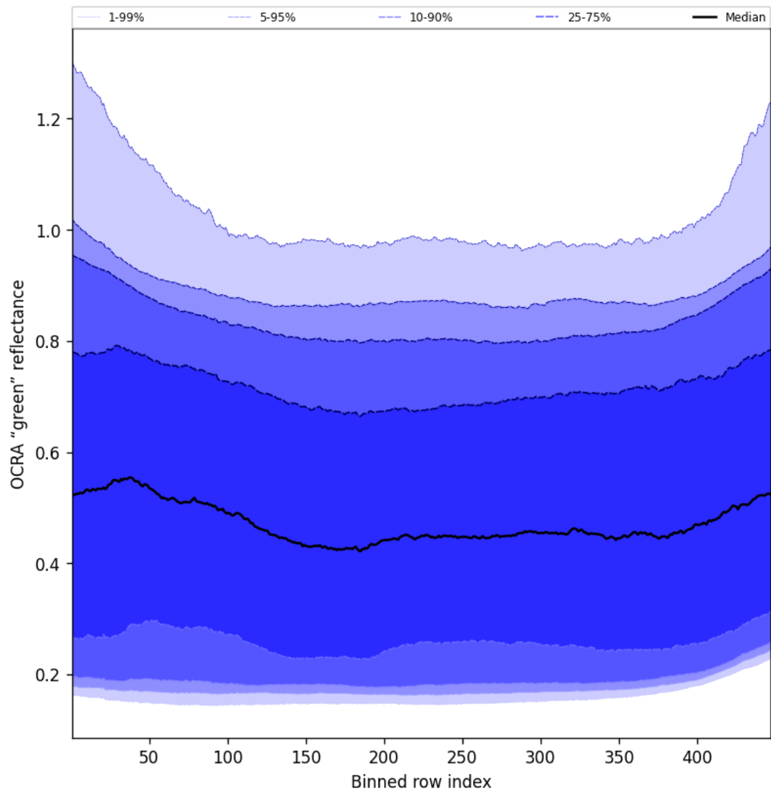
Figure 68: Along track statistics of “OCRA “green” reflectance” for 2025-04-14 to 2025-04-16
