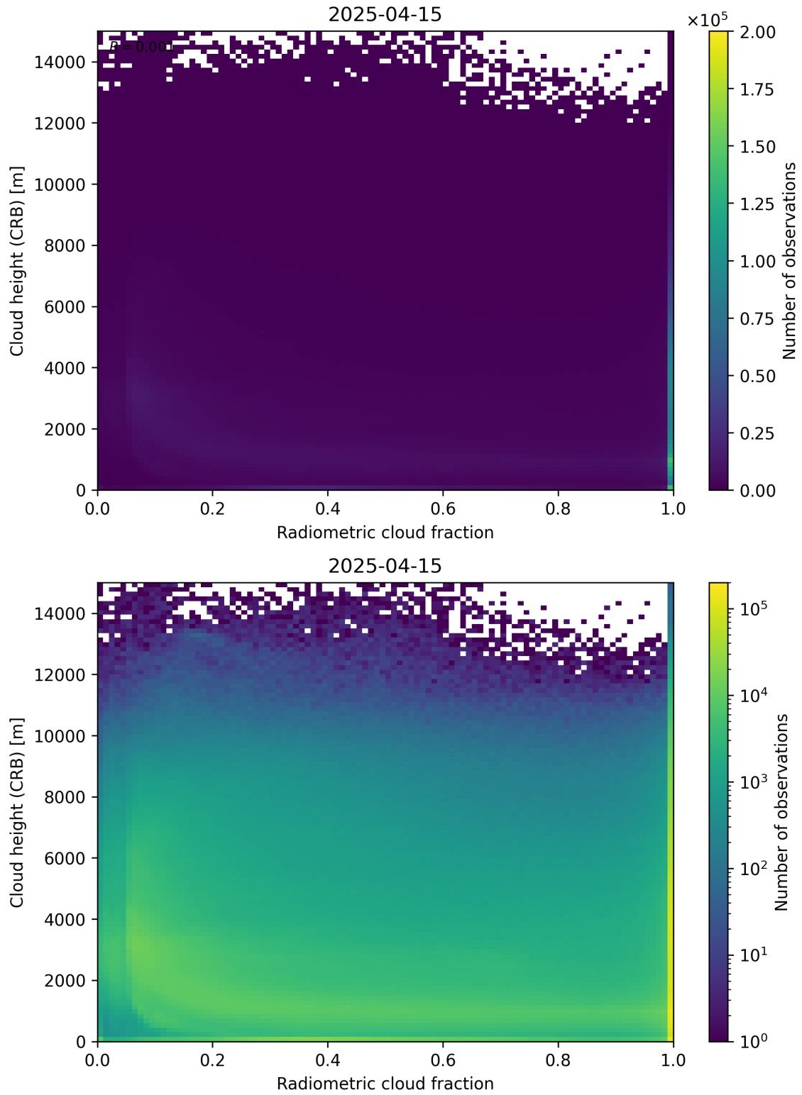
Figure 74: Scatter density plot of “Radiometric cloud fraction” against “Cloud height (CRB)” for 2025-04-14 to 2025-04-16.
