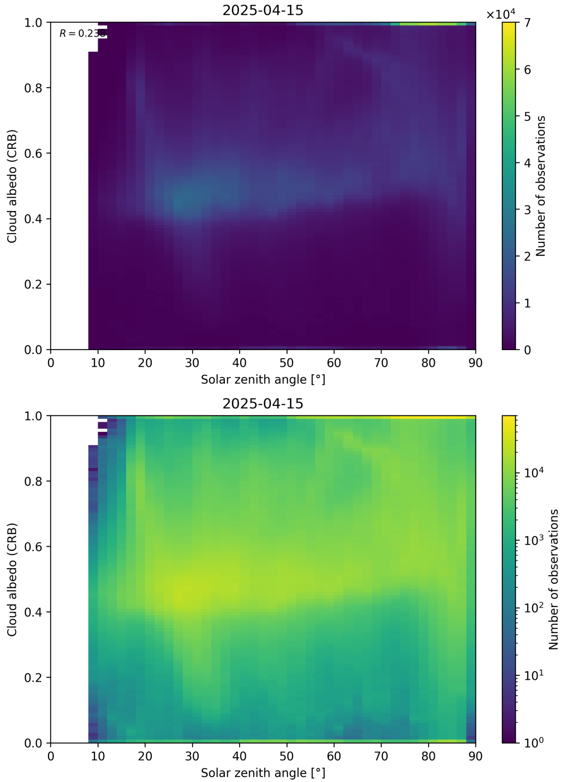
Figure 98: Scatter density plot of “Solar zenith angle” against “Cloud albedo (CRB)” for 2025-04-14 to 2025-04-16.
