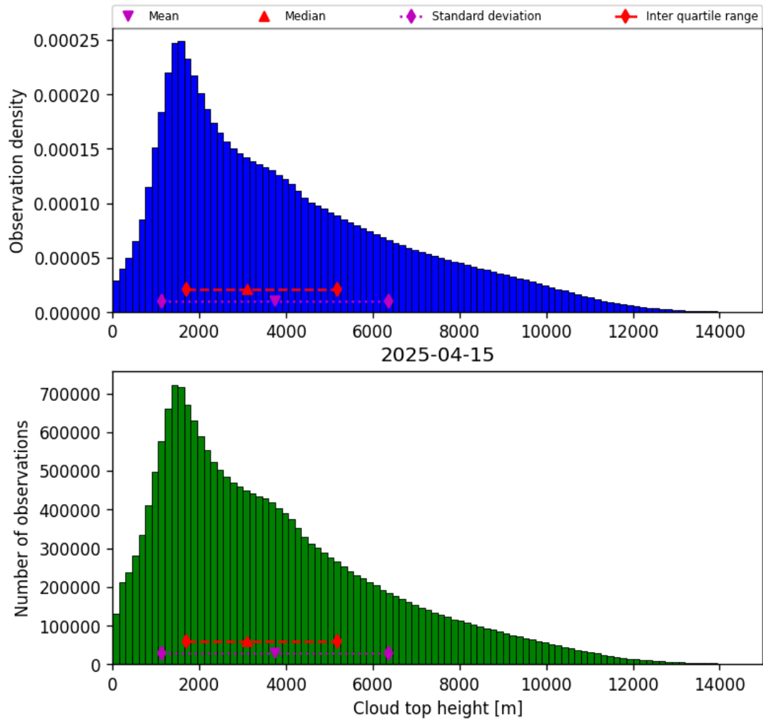
Figure 40: Histogram of “Cloud top height” for 2025-04-14 to 2025-04-16
