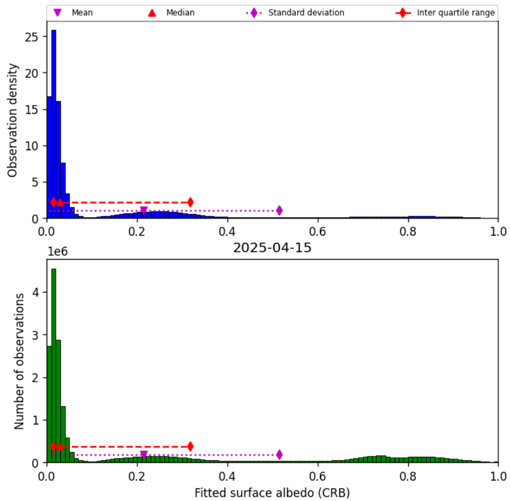
Figure 46: Histogram of “Fitted surface albedo (CRB)” for 2025-04-14 to 2025-04-16
