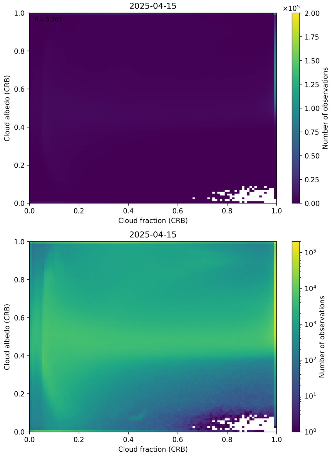
Figure 77: Scatter density plot of “Cloud fraction (CRB)” against “Cloud albedo (CRB)” for 2025-04-14 to 2025-04-16.
