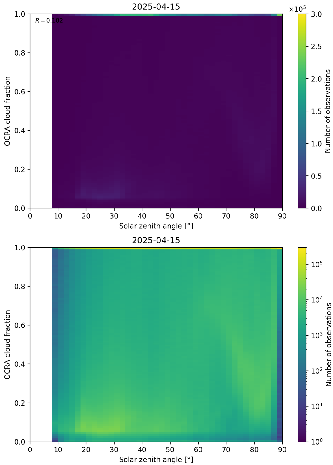
Figure 100: Scatter density plot of “Solar zenith angle” against “OCRA cloud fraction” for 2025-04-14 to 2025-04-16.
