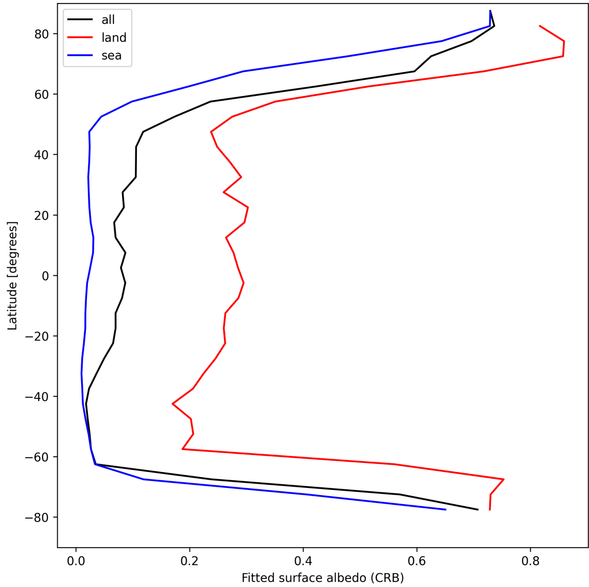
Figure 30: Zonal average of “Fitted surface albedo (CRB)” for 2025-04-14 to 2025-04-16.
