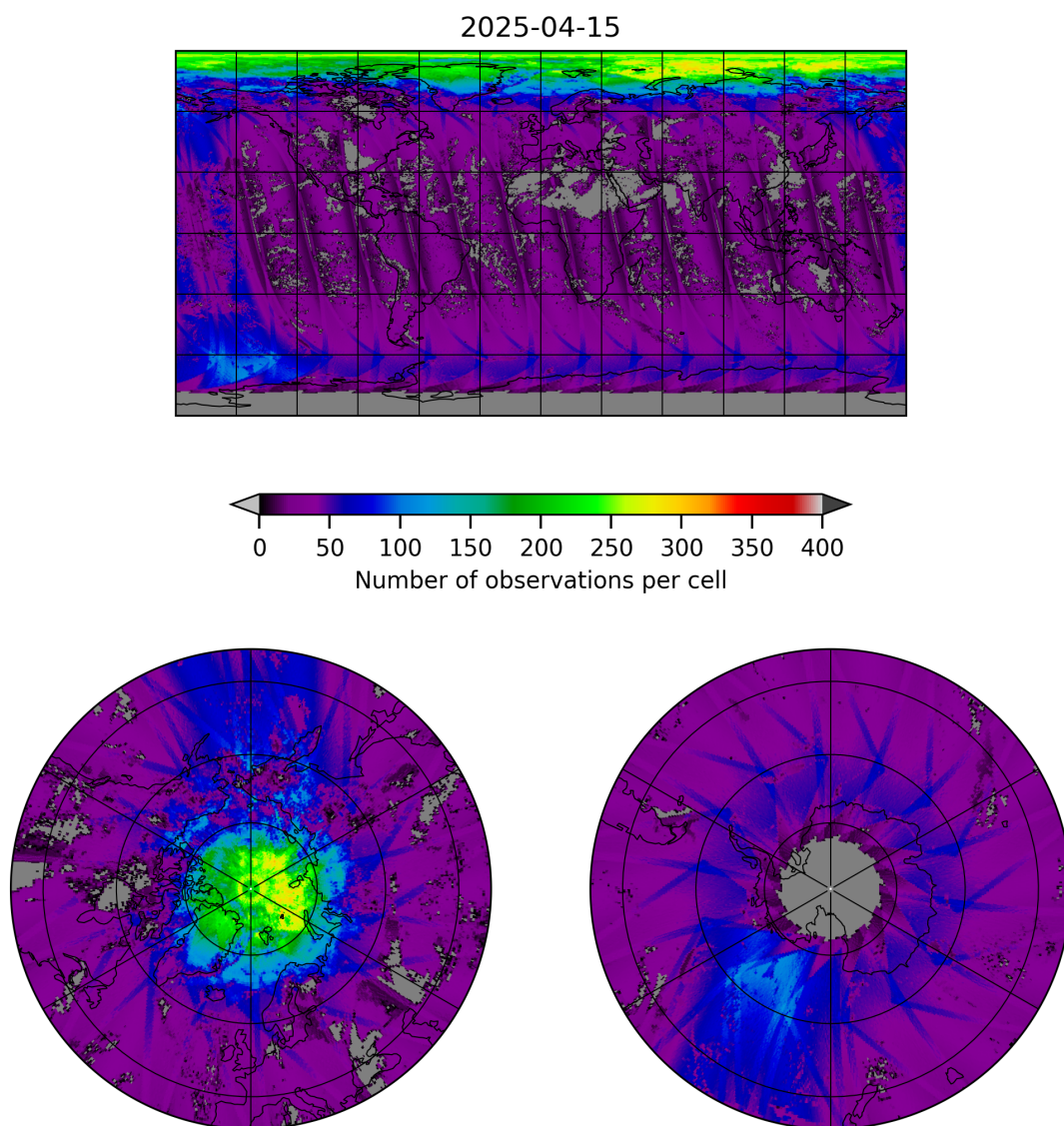
Figure 21: Map of the number of observations for 2025-04-14 to 2025-04-16
