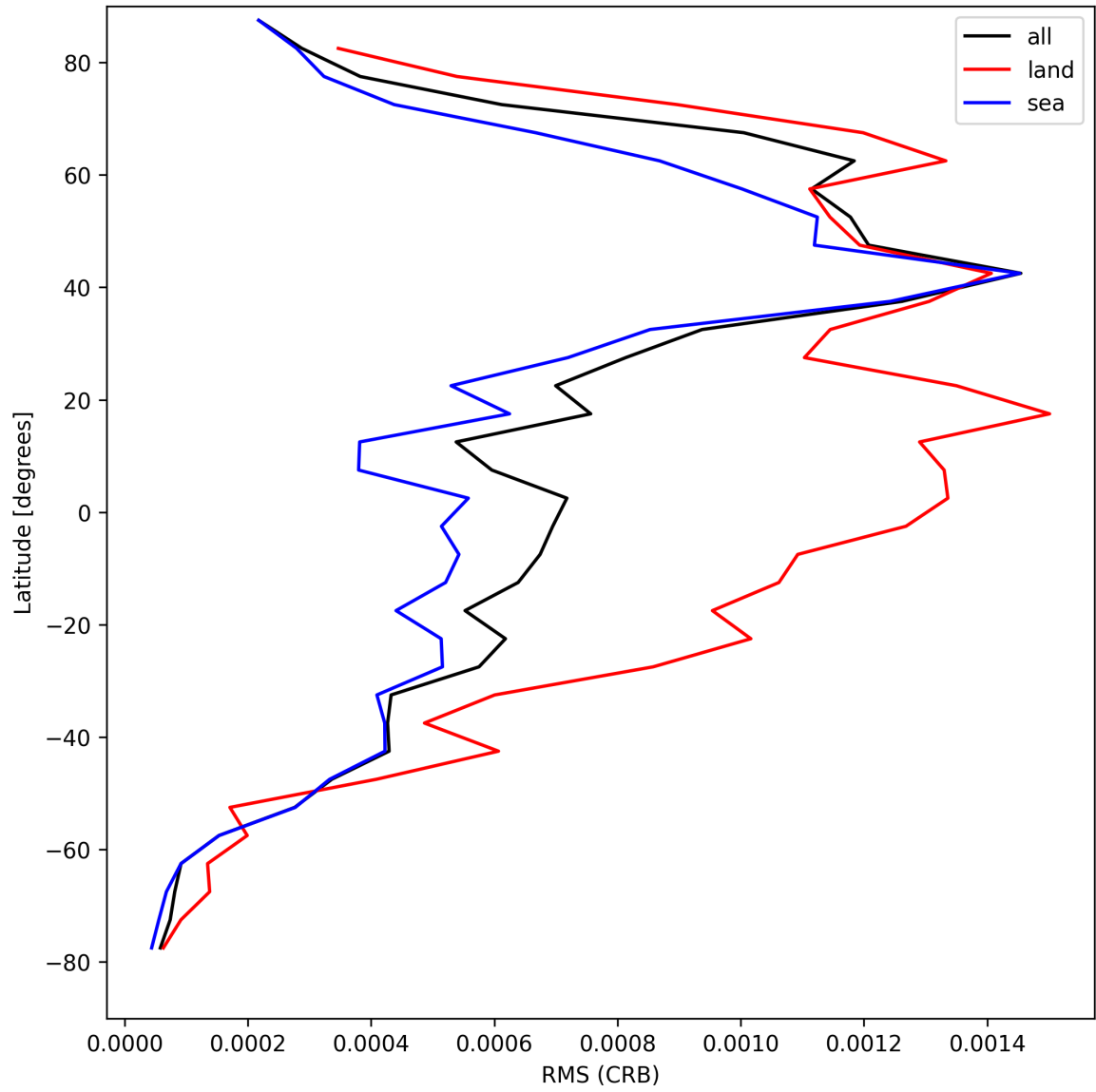
Figure 32: Zonal average of “RMS (CRB)” for 2025-04-14 to 2025-04-16.
