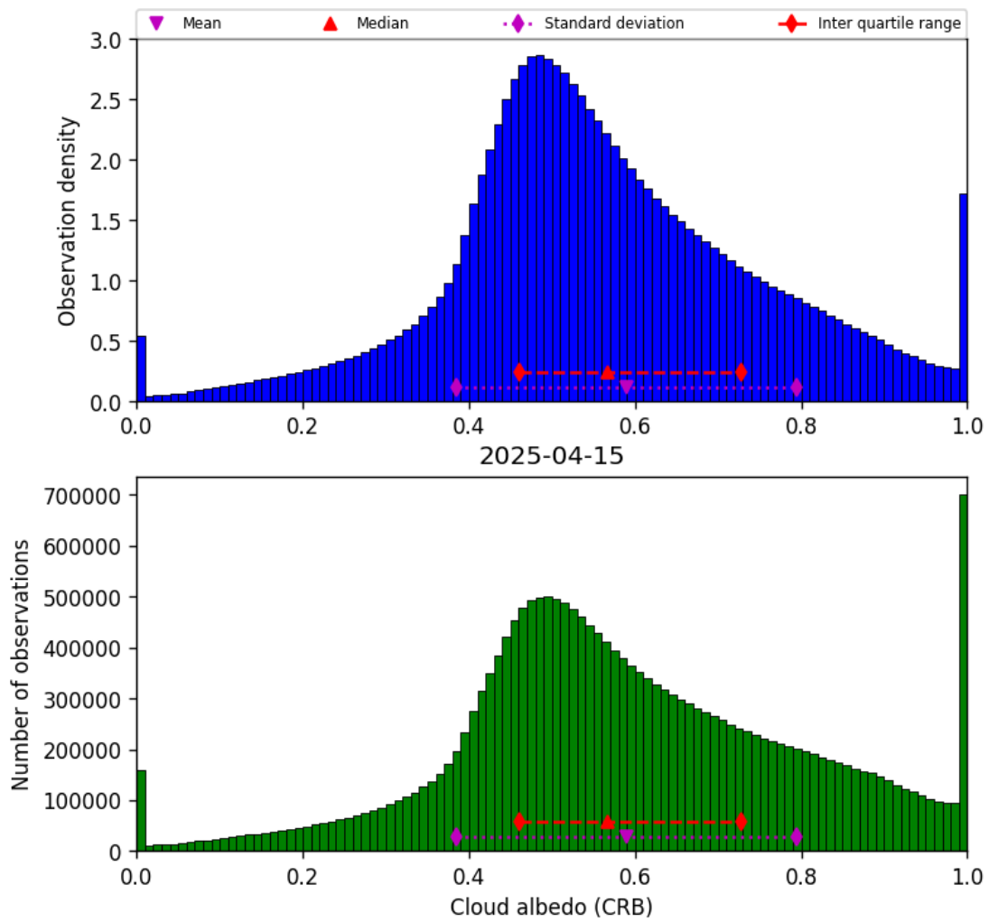
Figure 44: Histogram of “Cloud albedo (CRB)” for 2025-04-14 to 2025-04-16
