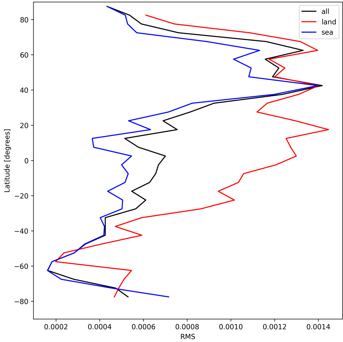
Figure 31: Zonal average of “RMS” for 2025-04-14 to 2025-04-16.
