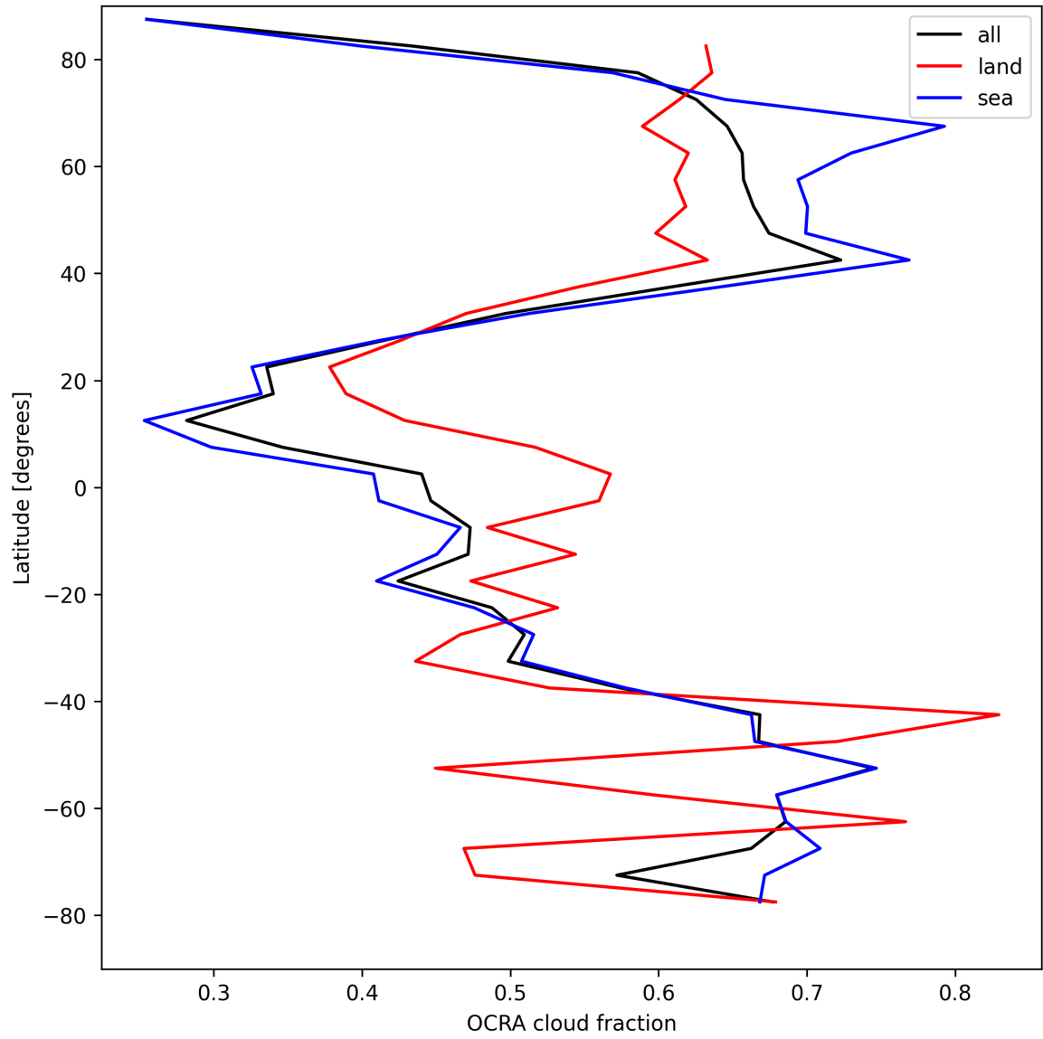
Figure 34: Zonal average of “OCRA cloud fraction” for 2025-04-14 to 2025-04-16.
