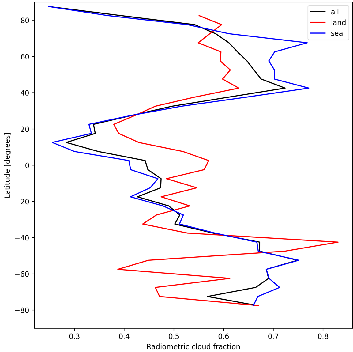
Figure 23: Zonal average of “Radiometric cloud fraction” for 2025-04-14 to 2025-04-16.
