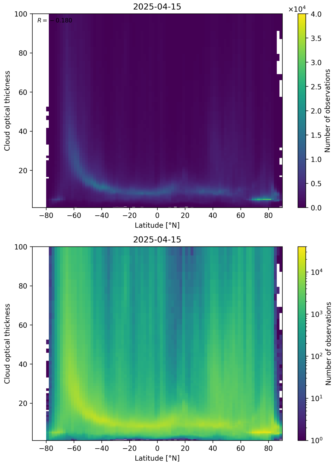
Figure 96: Scatter density plot of “Latitude” against “Cloud optical thickness” for 2025-04-14 to 2025-04-16.
