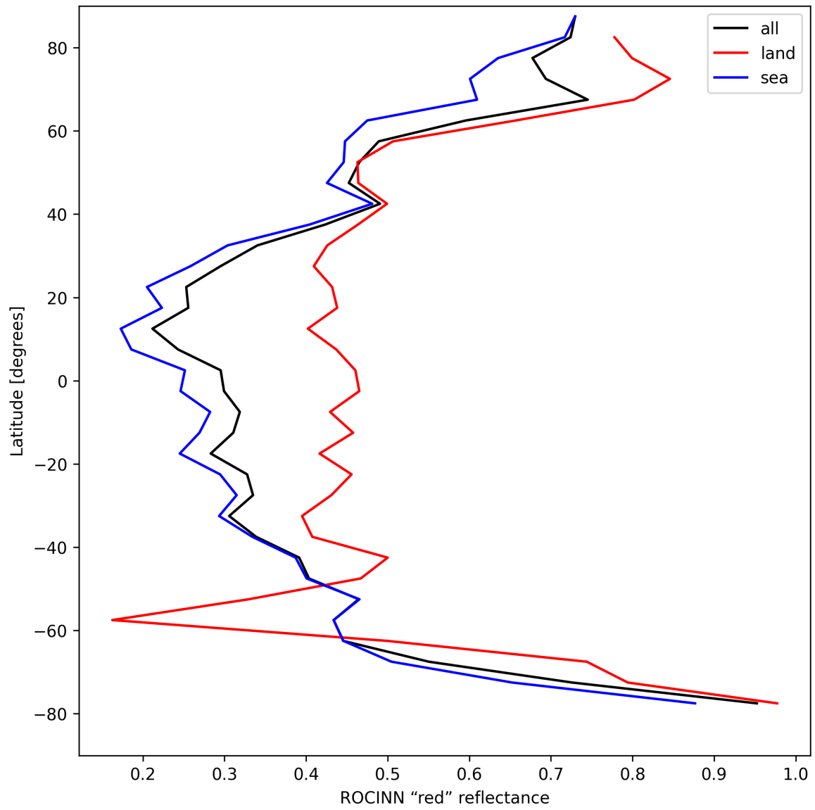
Figure 37: Zonal average of “ROCINN “red” reflectance” for 2025-04-14 to 2025-04-16.
