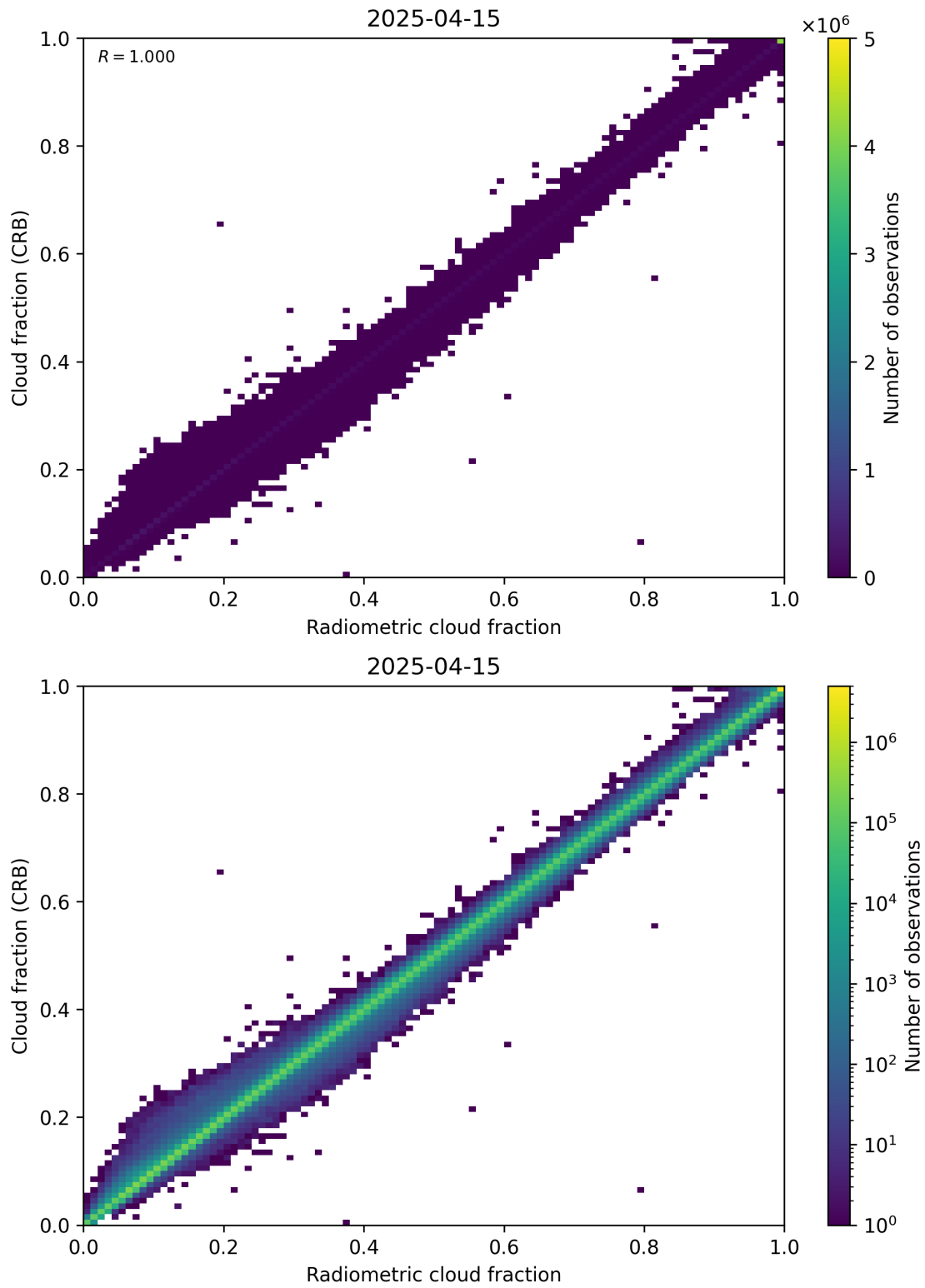
Figure 73: Scatter density plot of “Radiometric cloud fraction” against “Cloud fraction (CRB)” for 2025-04-14 to 2025-04-16.
