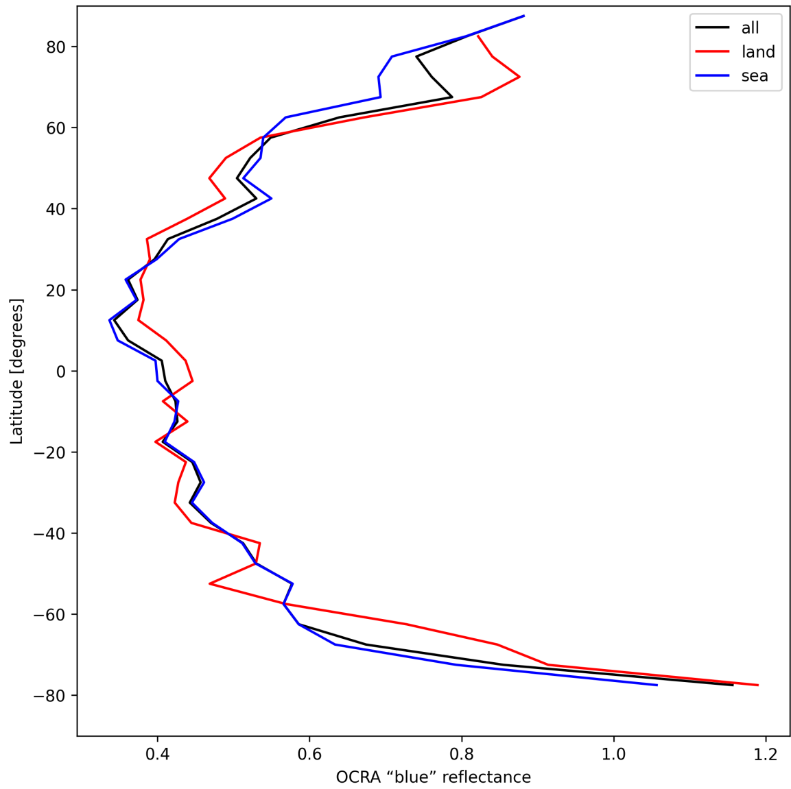
Figure 35: Zonal average of “OCRA “blue” reflectance” for 2025-04-14 to 2025-04-16.
