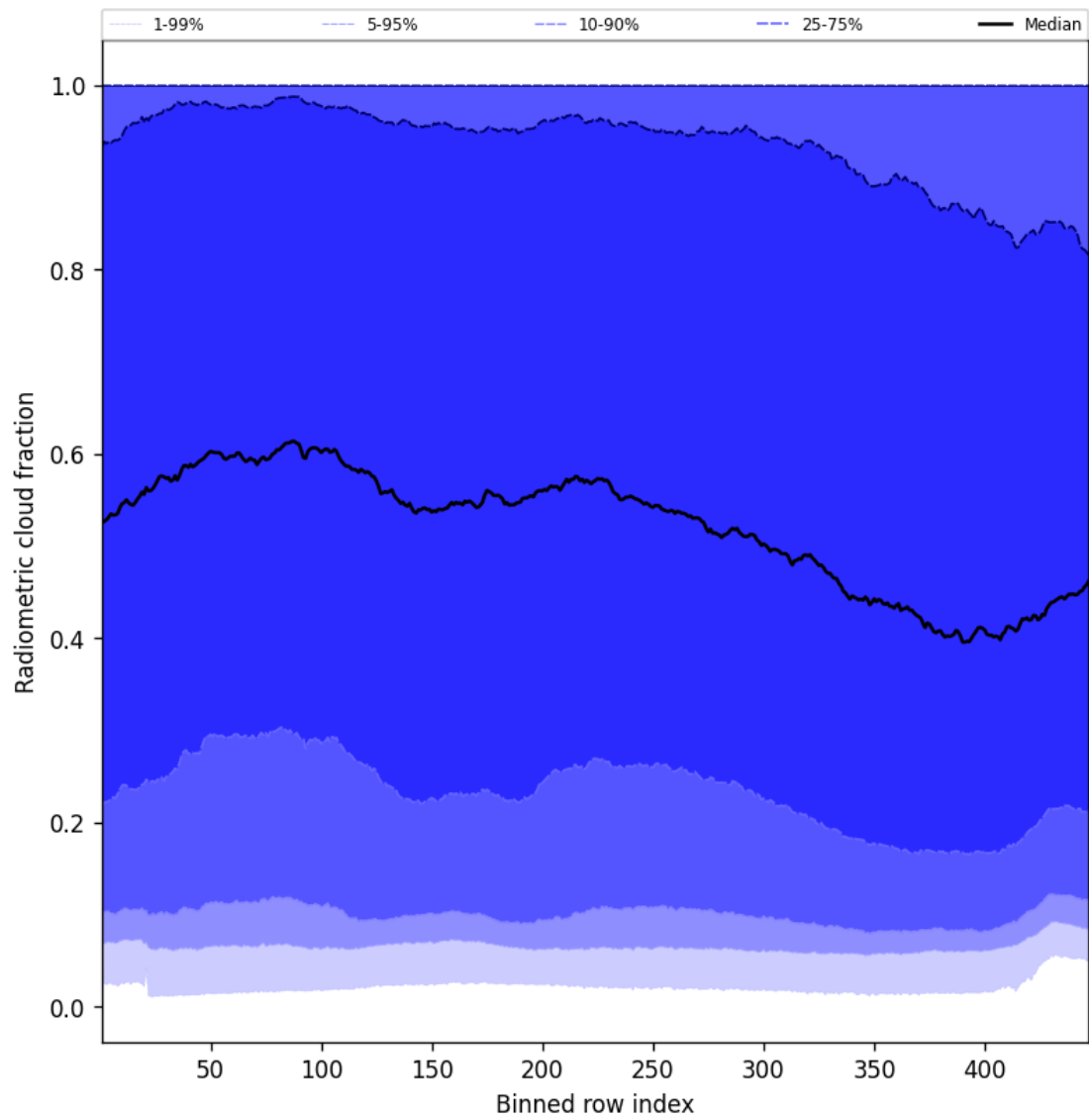
Figure 55: Along track statistics of “Radiometric cloud fraction” for 2025-04-14 to 2025-04-16
