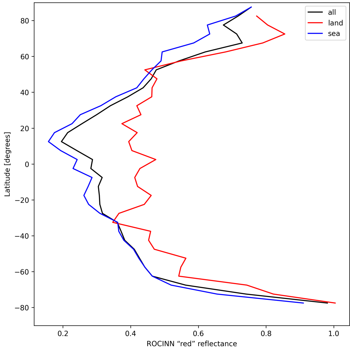
Figure 37: Zonal average of “ROCINN “red” reflectance” for 2025-04-15 to 2025-04-17.
