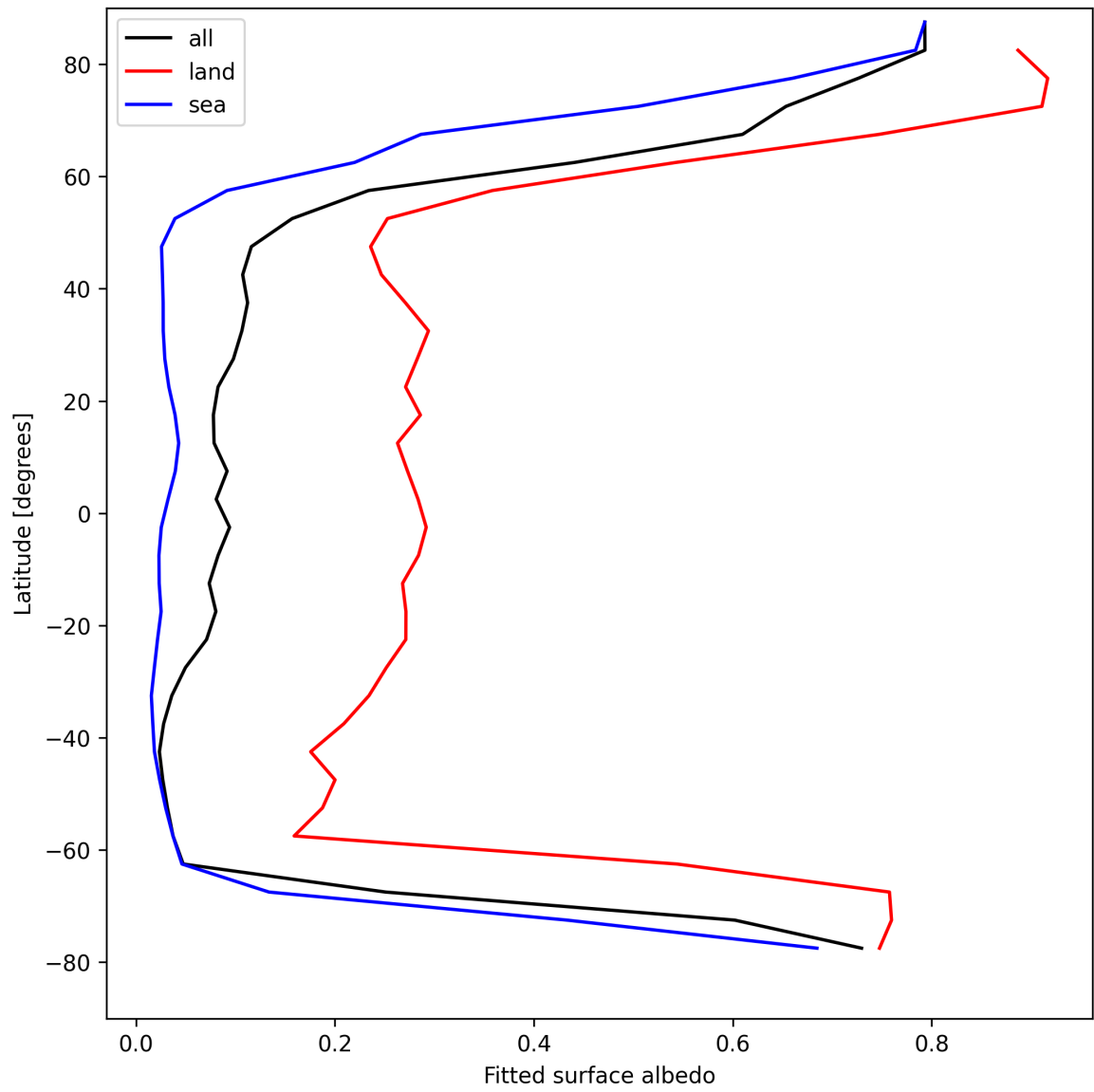
Figure 29: Zonal average of “Fitted surface albedo” for 2025-04-15 to 2025-04-17.
