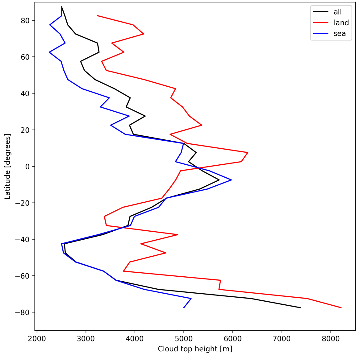
Figure 24: Zonal average of “Cloud top height” for 2025-04-15 to 2025-04-17.
