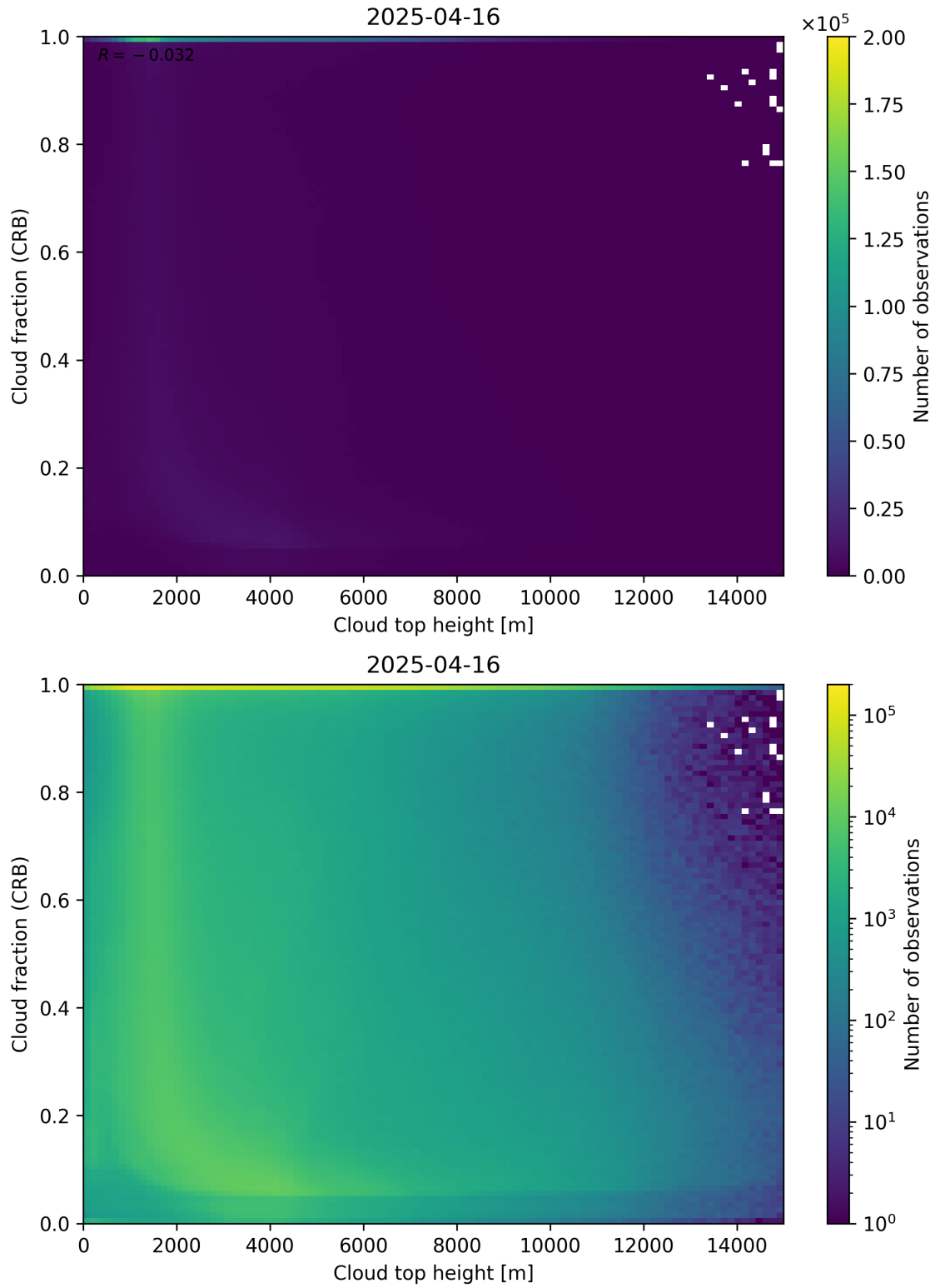
Figure 88: Scatter density plot of “Cloud top height” against “Cloud fraction (CRB)” for 2025-04-15 to 2025-04-17.
