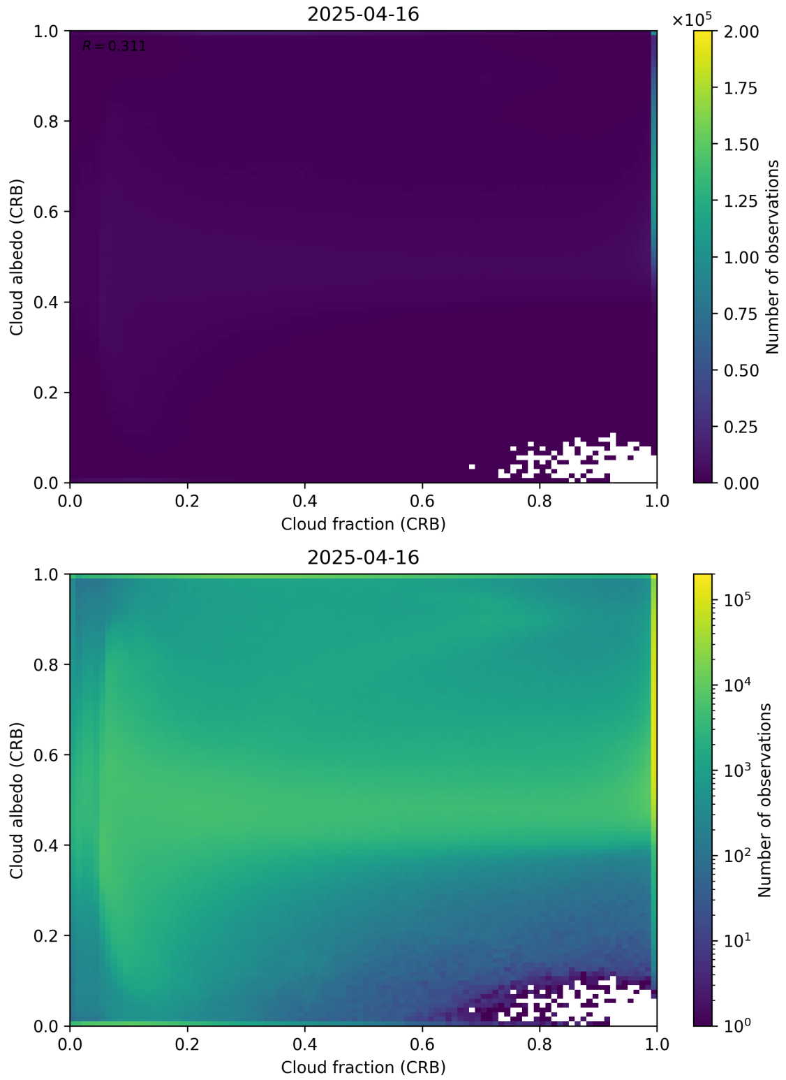
Figure 77: Scatter density plot of “Cloud fraction (CRB)” against “Cloud albedo (CRB)” for 2025-04-15 to 2025-04-17.
