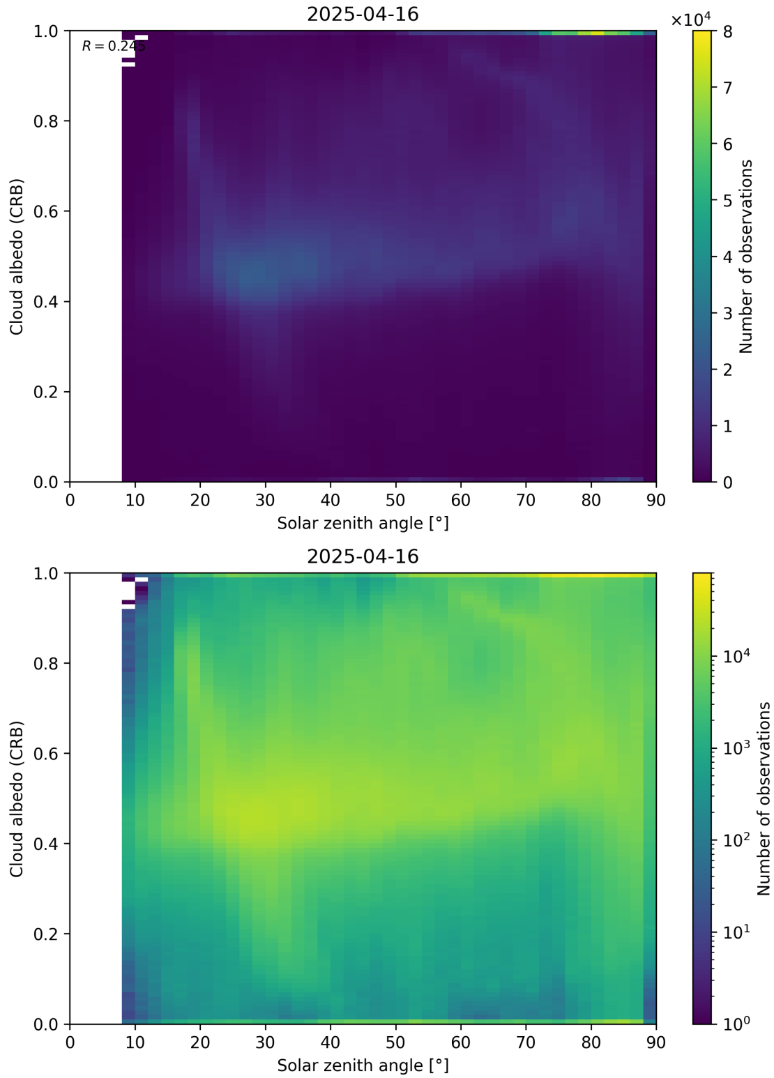
Figure 98: Scatter density plot of “Solar zenith angle” against “Cloud albedo (CRB)” for 2025-04-15 to 2025-04-17.
