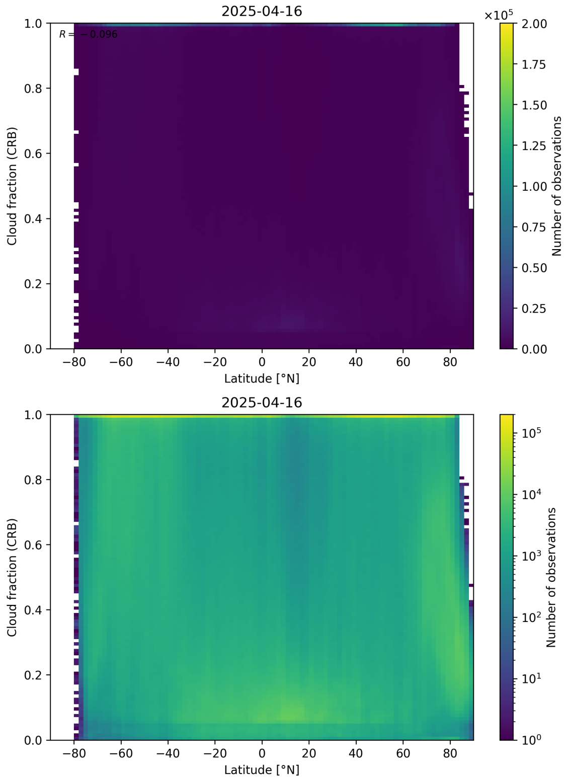
Figure 94: Scatter density plot of “Latitude” against “Cloud fraction (CRB)” for 2025-04-15 to 2025-04-17.
