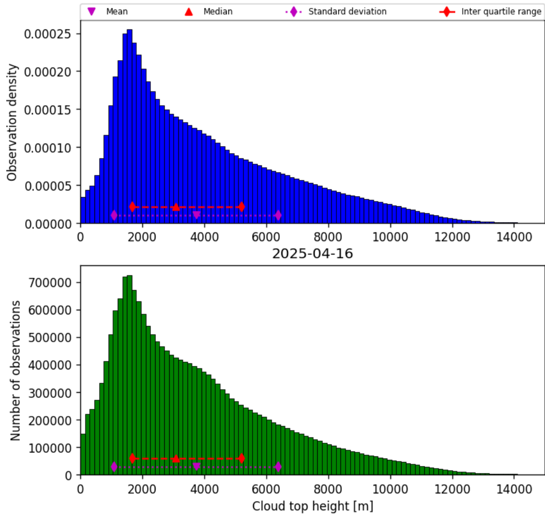
Figure 40: Histogram of “Cloud top height” for 2025-04-15 to 2025-04-17
