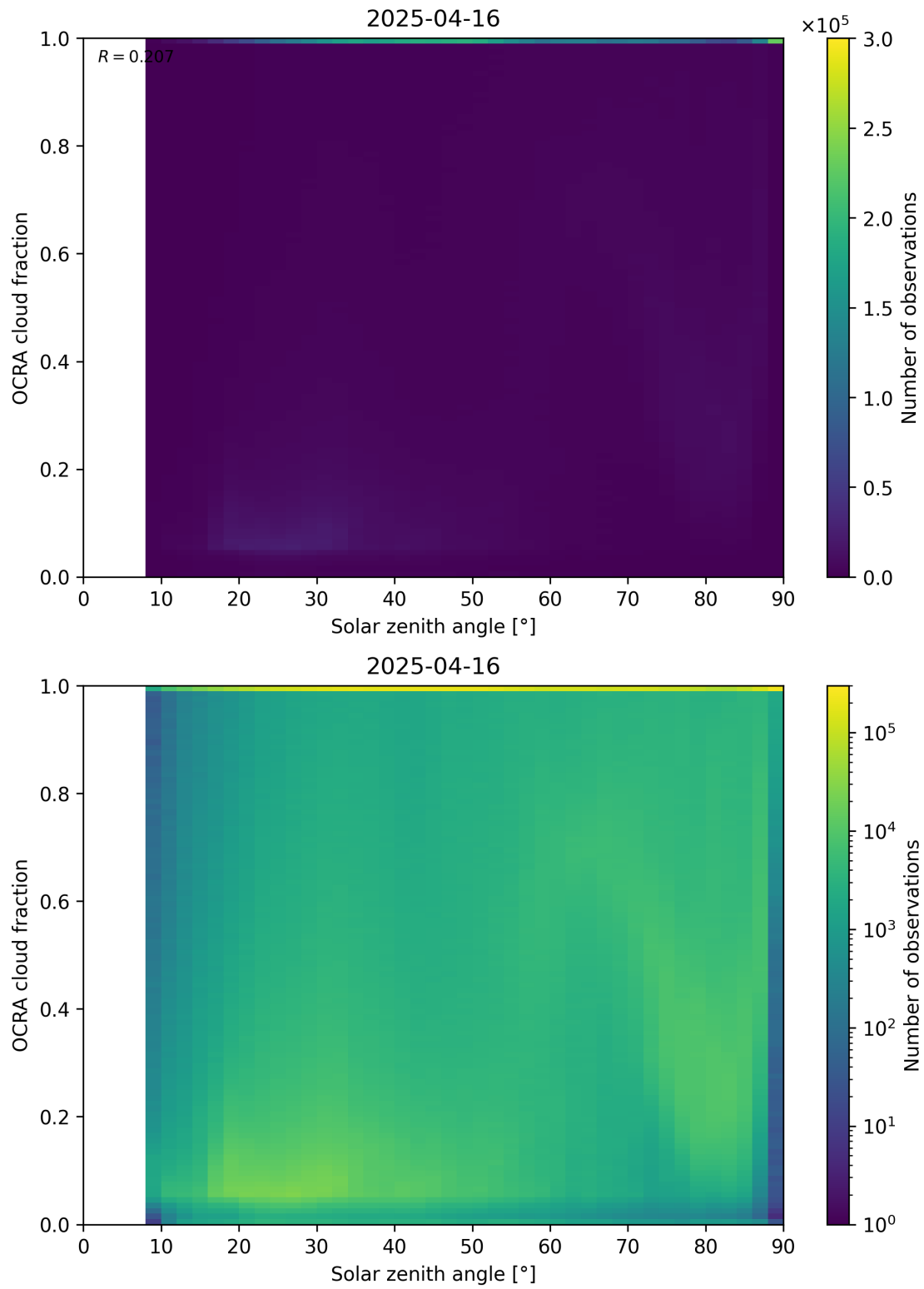
Figure 100: Scatter density plot of “Solar zenith angle” against “OCRA cloud fraction” for 2025-04-15 to 2025-04-17.
