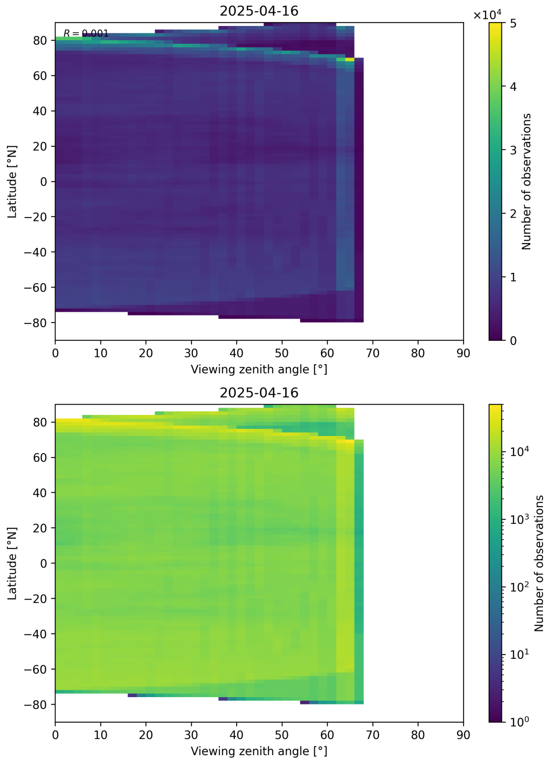
Figure 113: Scatter density plot of “Viewing zenith angle” against “Latitude” for 2025-04-15 to 2025-04-17.
