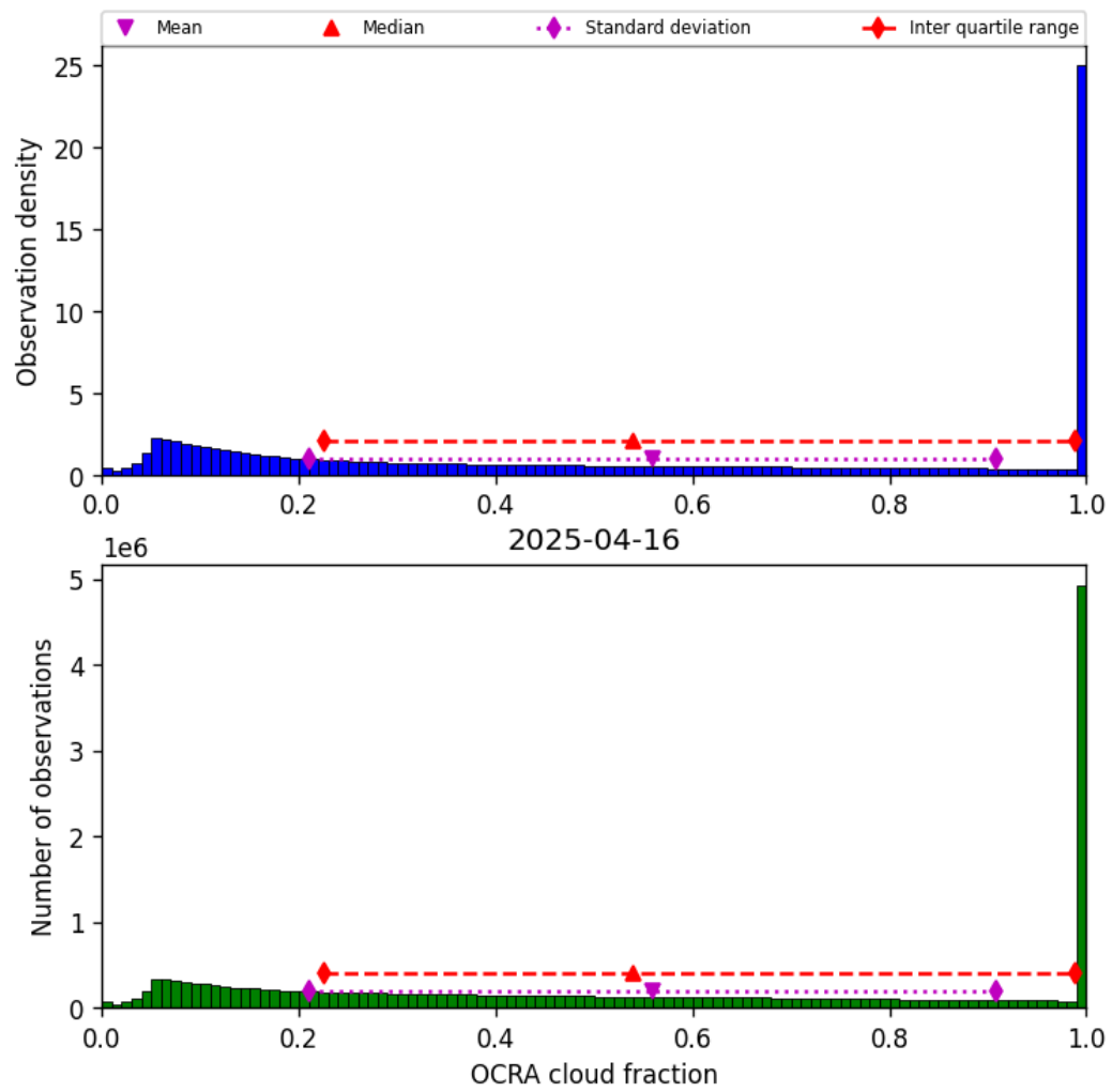
Figure 50: Histogram of “OCRA cloud fraction” for 2025-04-15 to 2025-04-17
