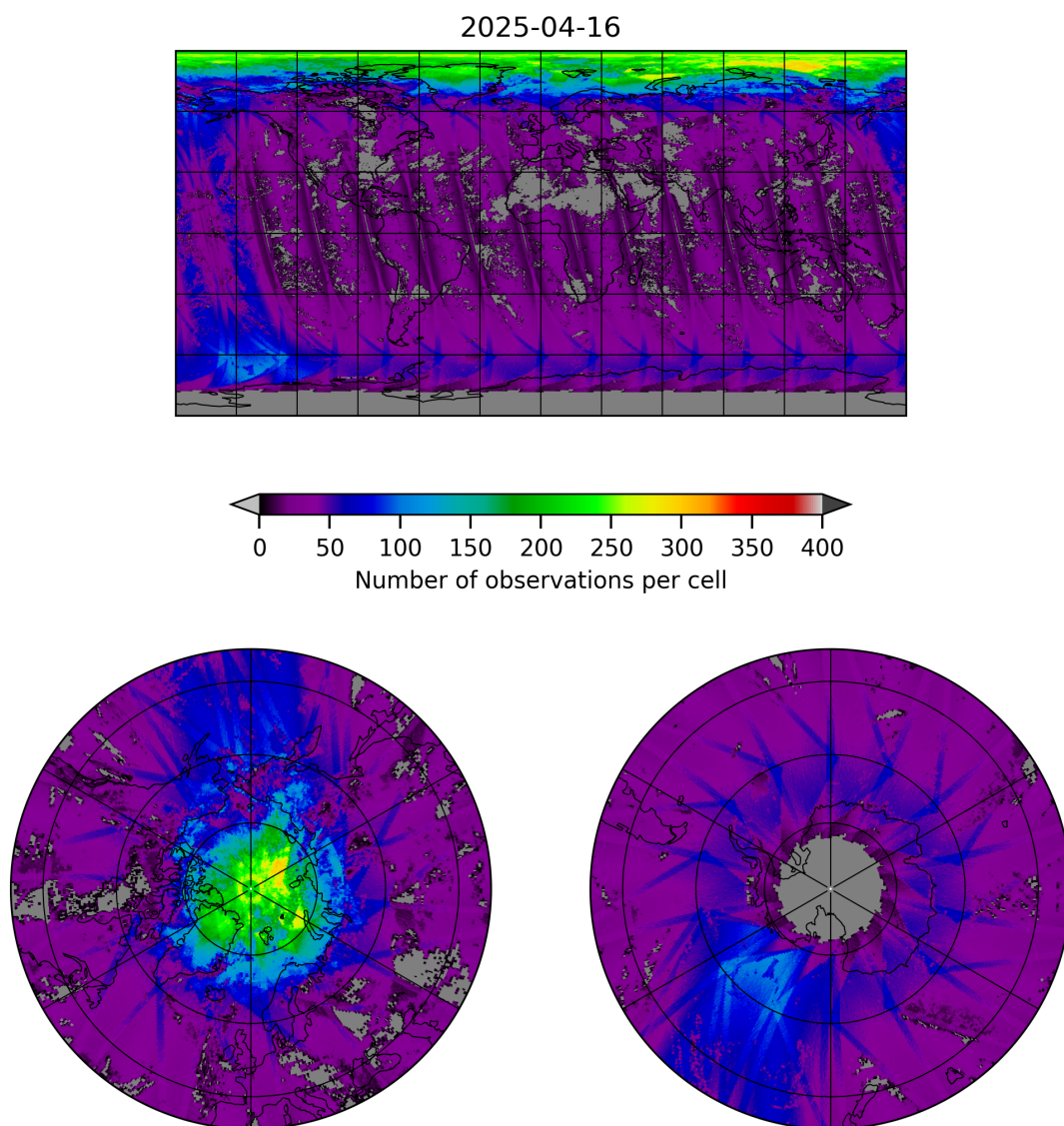
Figure 21: Map of the number of observations for 2025-04-15 to 2025-04-17
