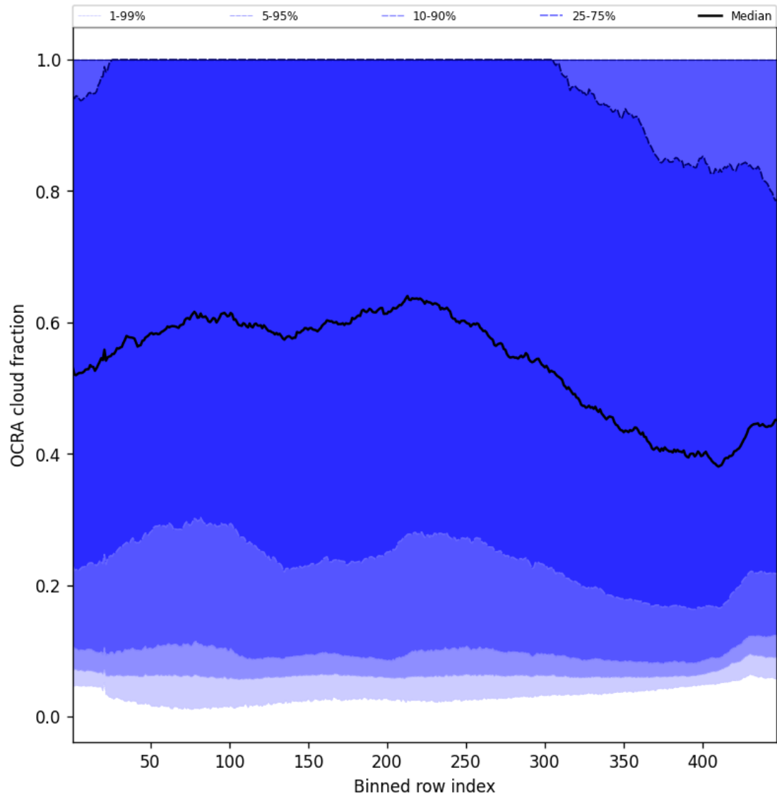
Figure 66: Along track statistics of “OCRA cloud fraction” for 2025-04-15 to 2025-04-17
