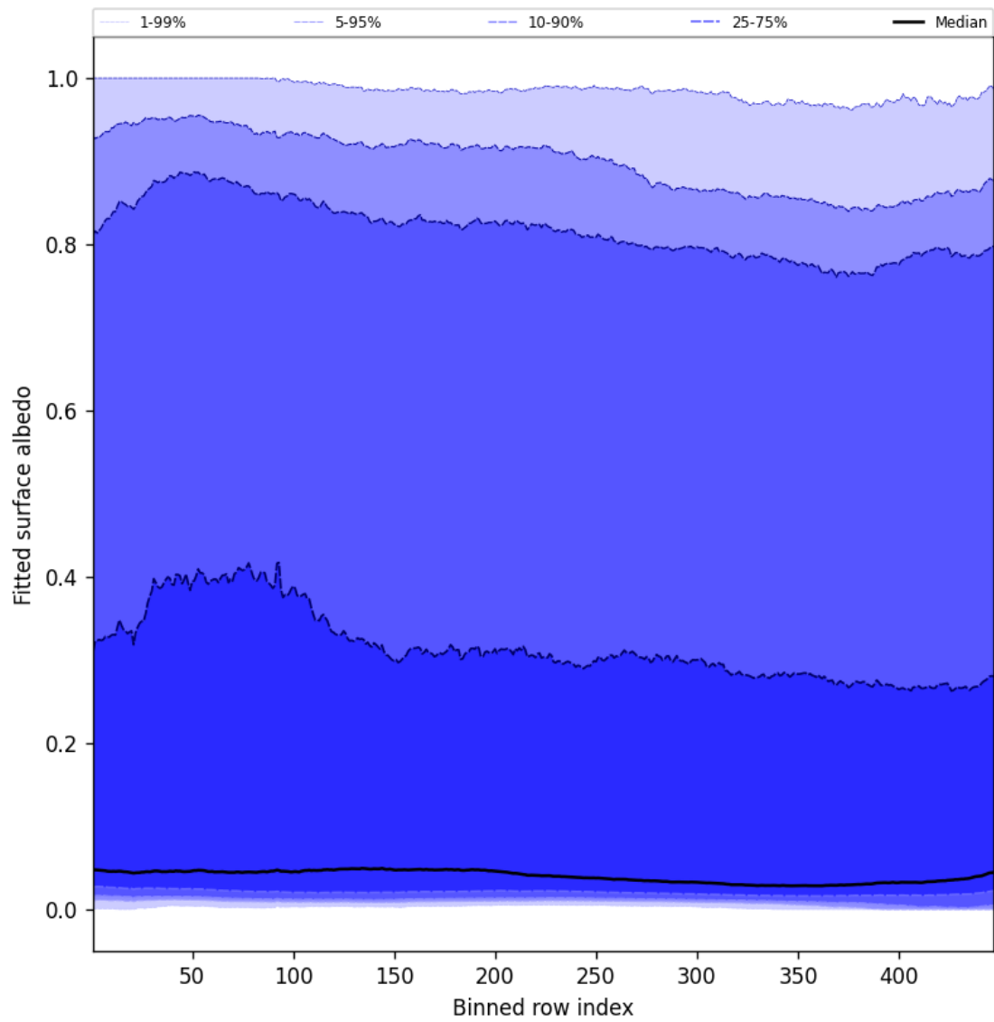
Figure 61: Along track statistics of “Fitted surface albedo” for 2025-04-15 to 2025-04-17
