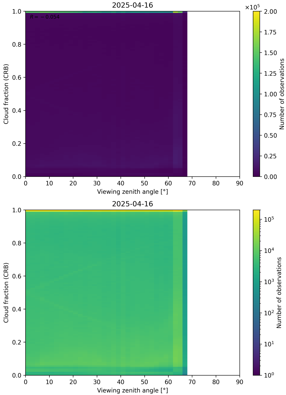
Figure 109: Scatter density plot of “Viewing zenith angle” against “Cloud fraction (CRB)” for 2025-04-15 to 2025-04-17.
