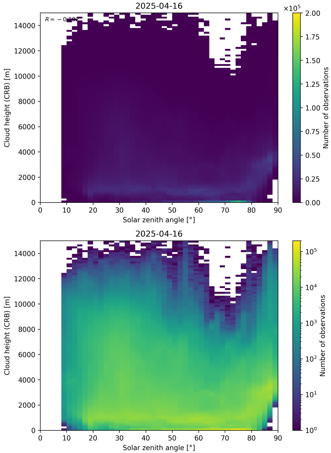
Figure 102: Scatter density plot of “Solar zenith angle” against “Cloud height (CRB)” for 2025-04-15 to 2025-04-17.
