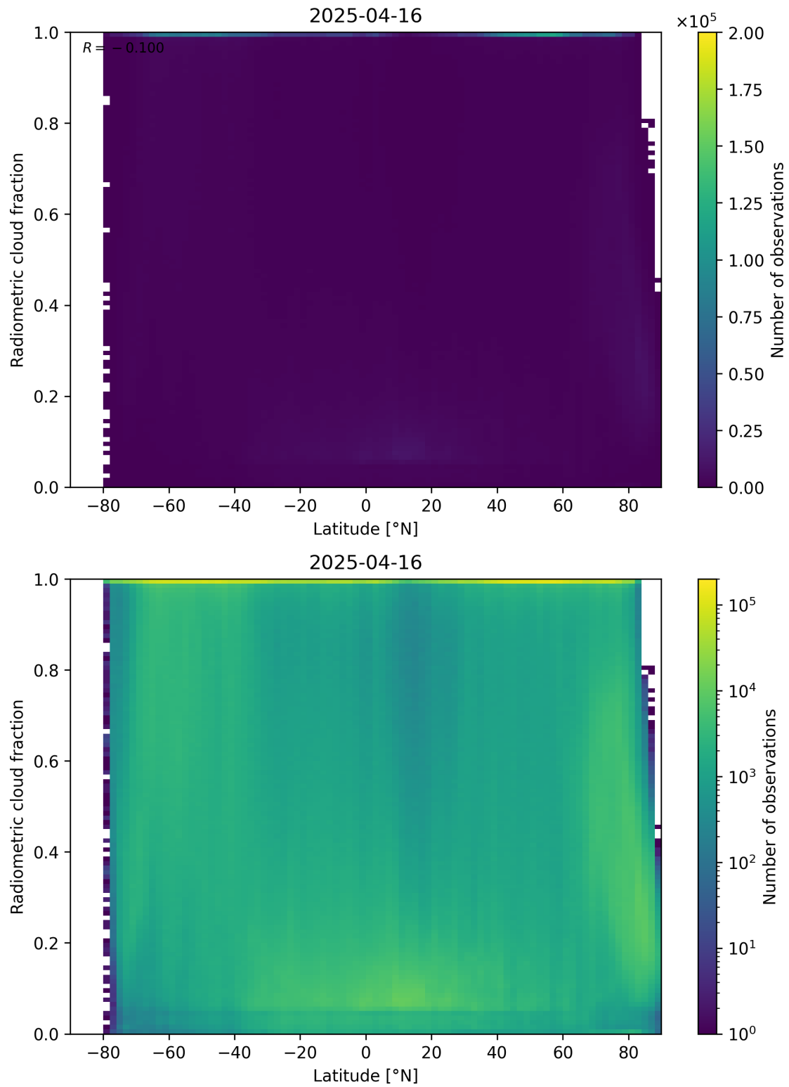
Figure 92: Scatter density plot of “Latitude” against “Radiometric cloud fraction” for 2025-04-15 to 2025-04-17.
