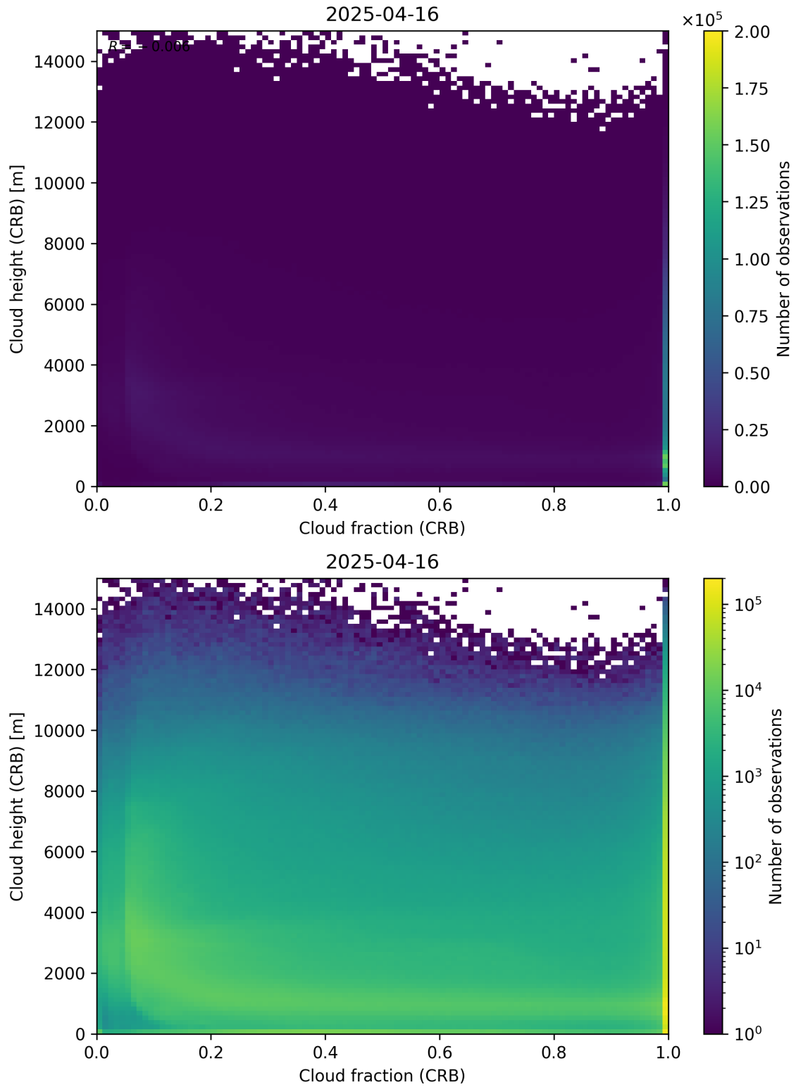
Figure 79: Scatter density plot of “Cloud fraction (CRB)” against “Cloud height (CRB)” for 2025-04-15 to 2025-04-17.
