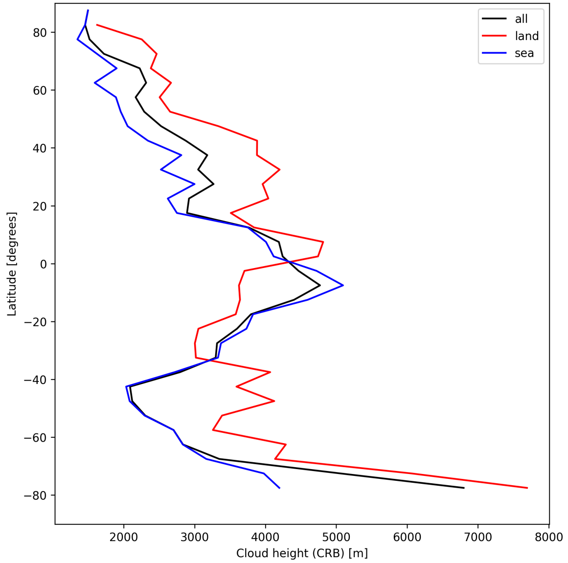
Figure 27: Zonal average of “Cloud height (CRB)” for 2025-04-15 to 2025-04-17.
