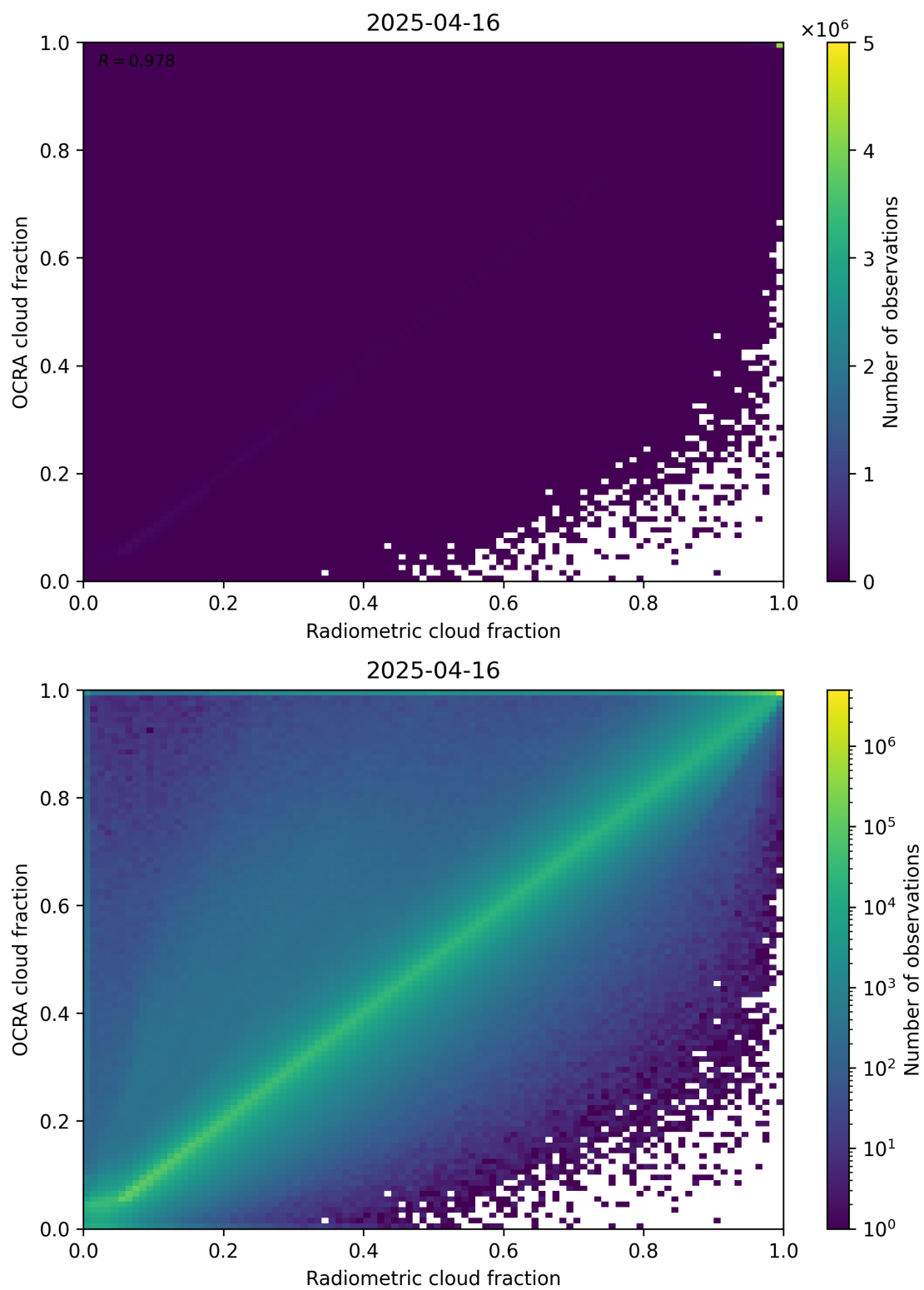
Figure 72: Scatter density plot of “Radiometric cloud fraction” against “OCRA cloud fraction” for 2025-04-15 to 2025-04-17.
