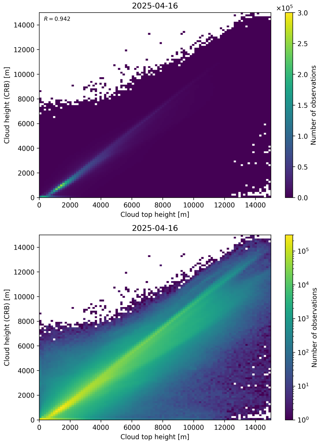
Figure 89: Scatter density plot of “Cloud top height” against “Cloud height (CRB)” for 2025-04-15 to 2025-04-17.
