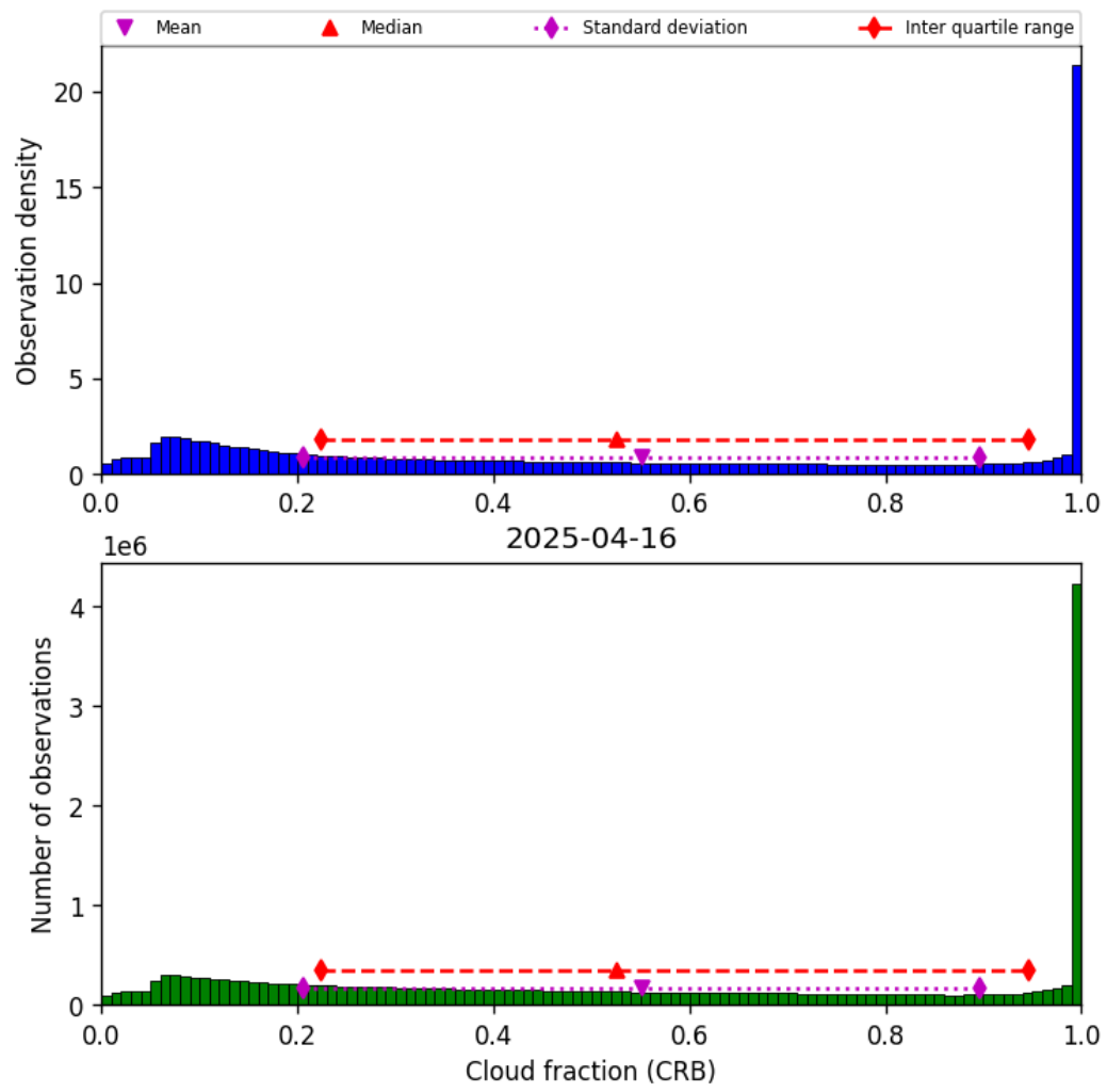
Figure 42: Histogram of “Cloud fraction (CRB)” for 2025-04-15 to 2025-04-17
