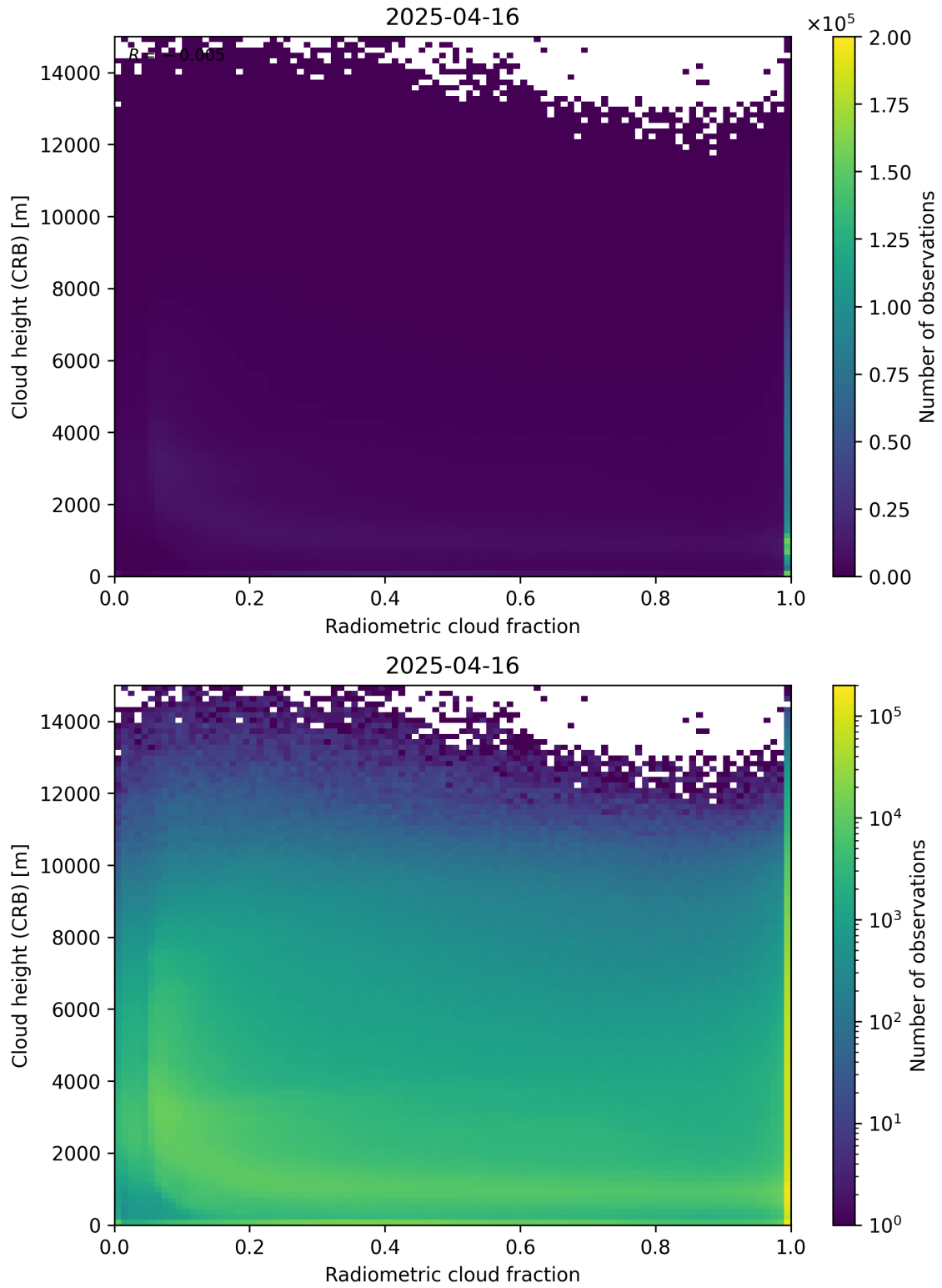
Figure 74: Scatter density plot of “Radiometric cloud fraction” against “Cloud height (CRB)” for 2025-04-15 to 2025-04-17.
