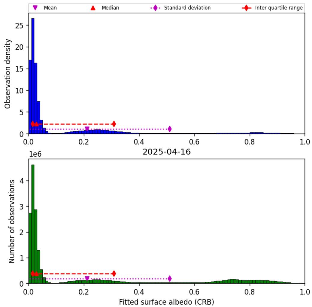
Figure 46: Histogram of “Fitted surface albedo (CRB)” for 2025-04-15 to 2025-04-17
