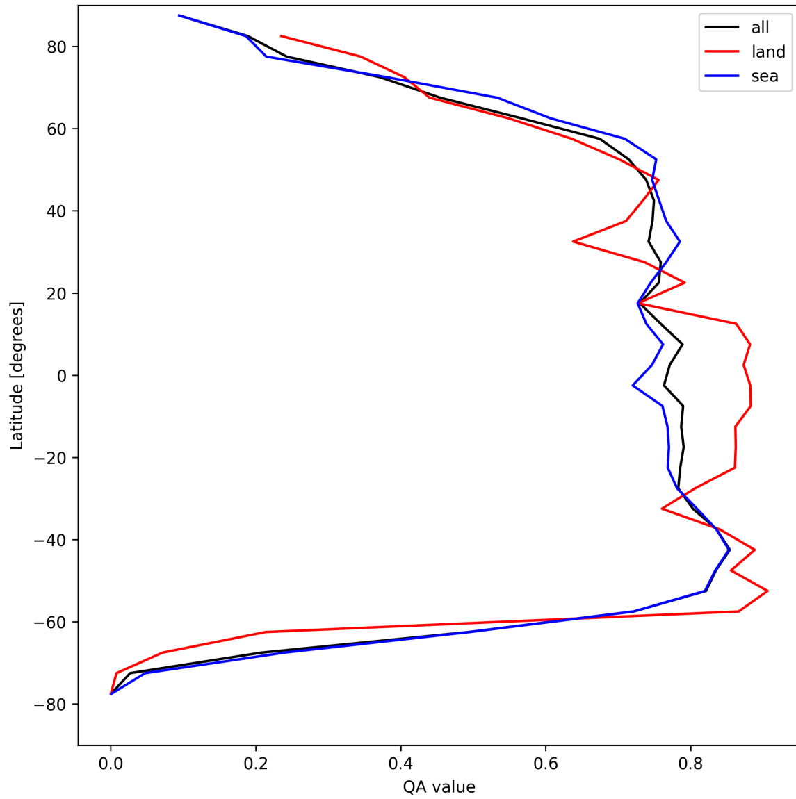
Figure 22: Zonal average of “QA value” for 2025-04-15 to 2025-04-17.
