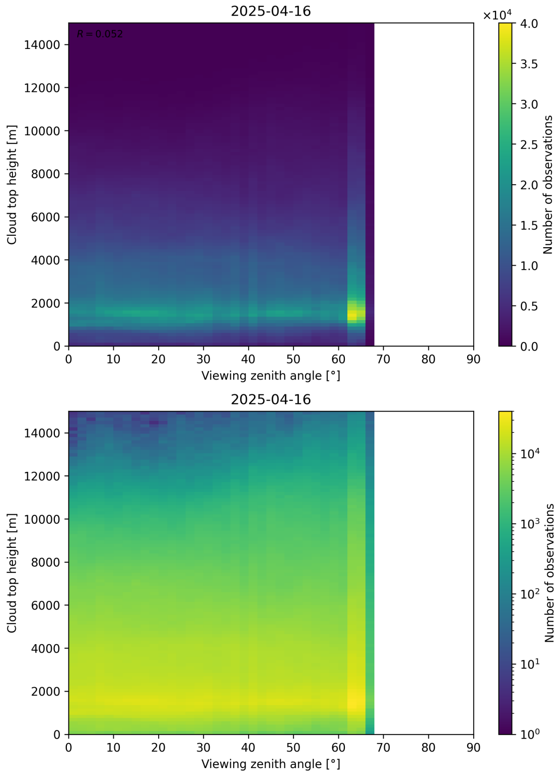
Figure 112: Scatter density plot of “Viewing zenith angle” against “Cloud top height” for 2025-04-15 to 2025-04-17.
