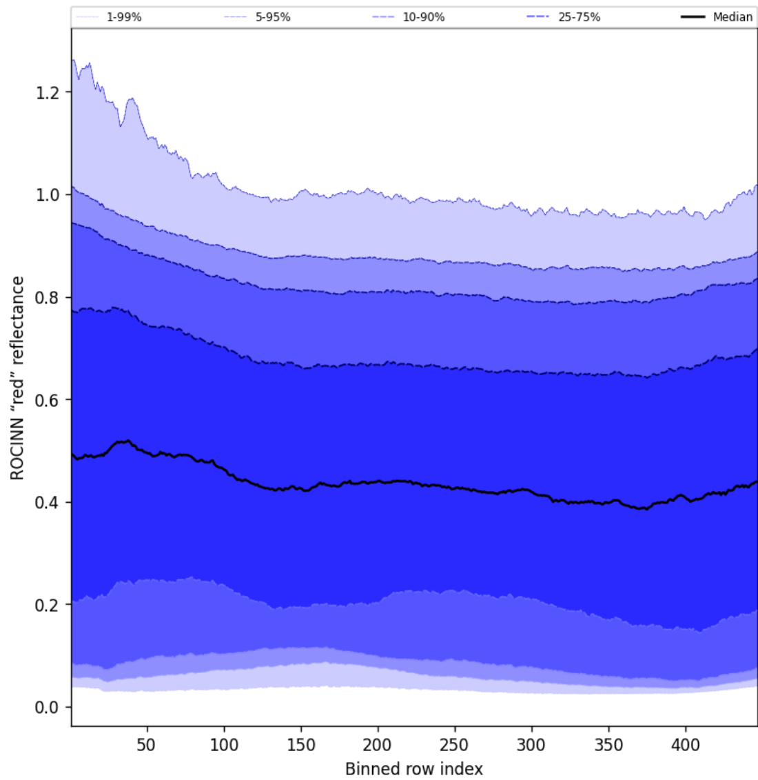
Figure 69: Along track statistics of “ROCINN “red” reflectance” for 2025-04-15 to 2025-04-17
