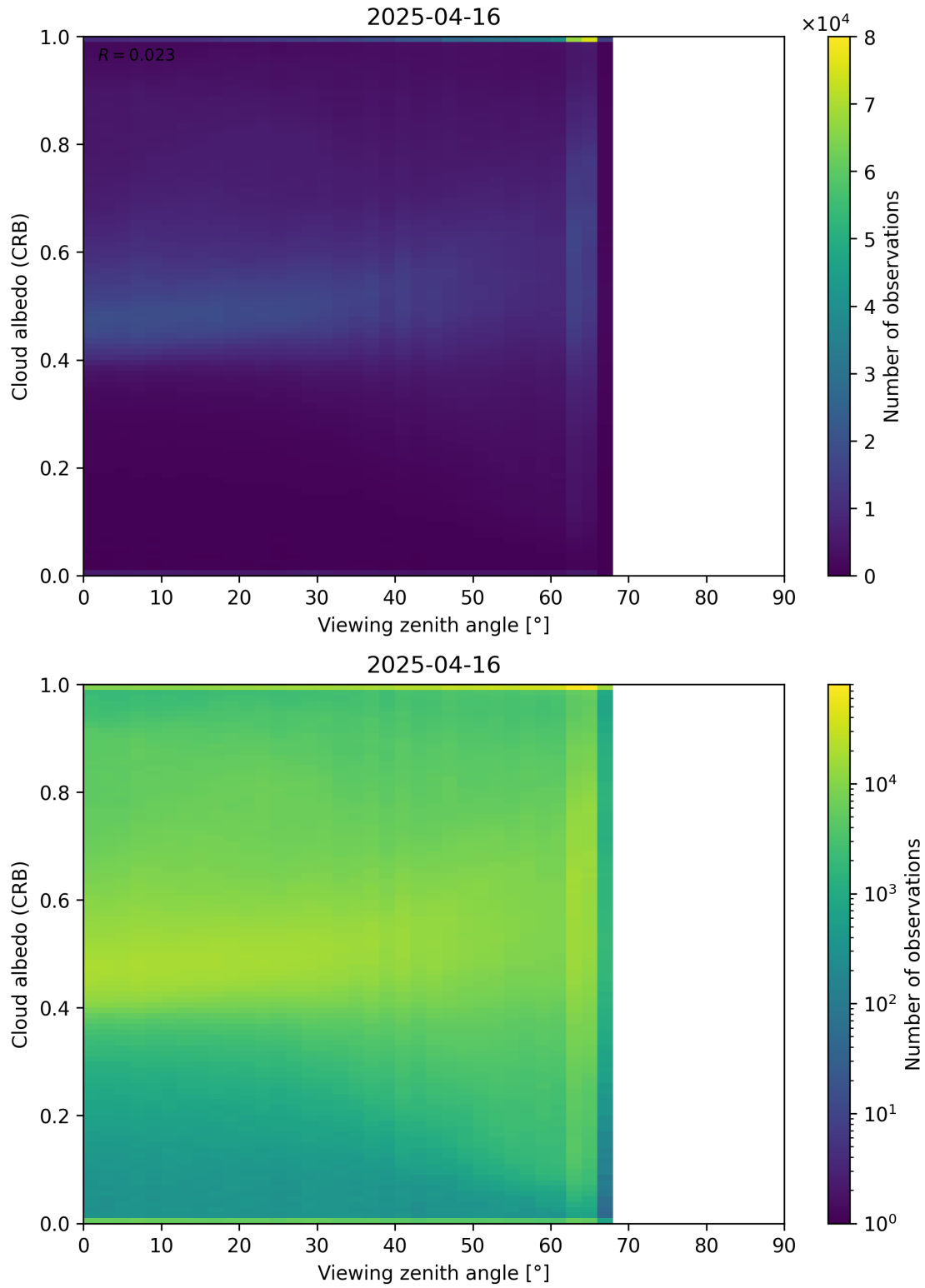
Figure 106: Scatter density plot of “Viewing zenith angle” against “Cloud albedo (CRB)” for 2025-04-15 to 2025-04-17.
