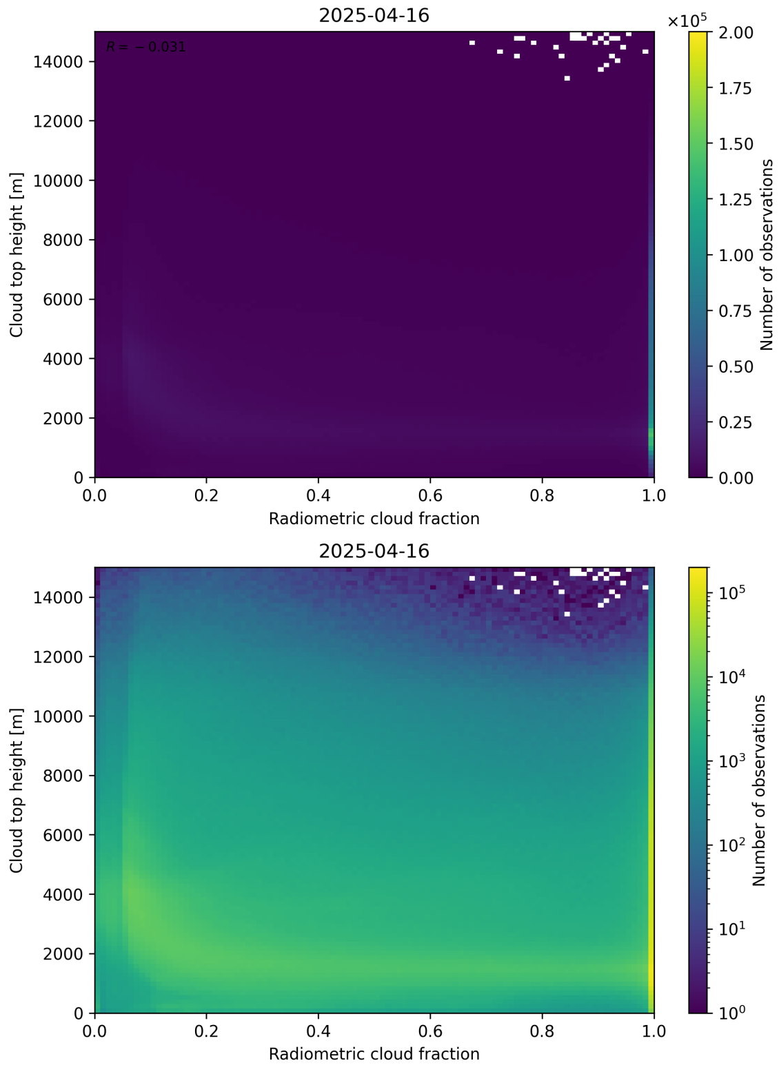
Figure 76: Scatter density plot of “Radiometric cloud fraction” against “Cloud top height” for 2025-04-15 to 2025-04-17.
