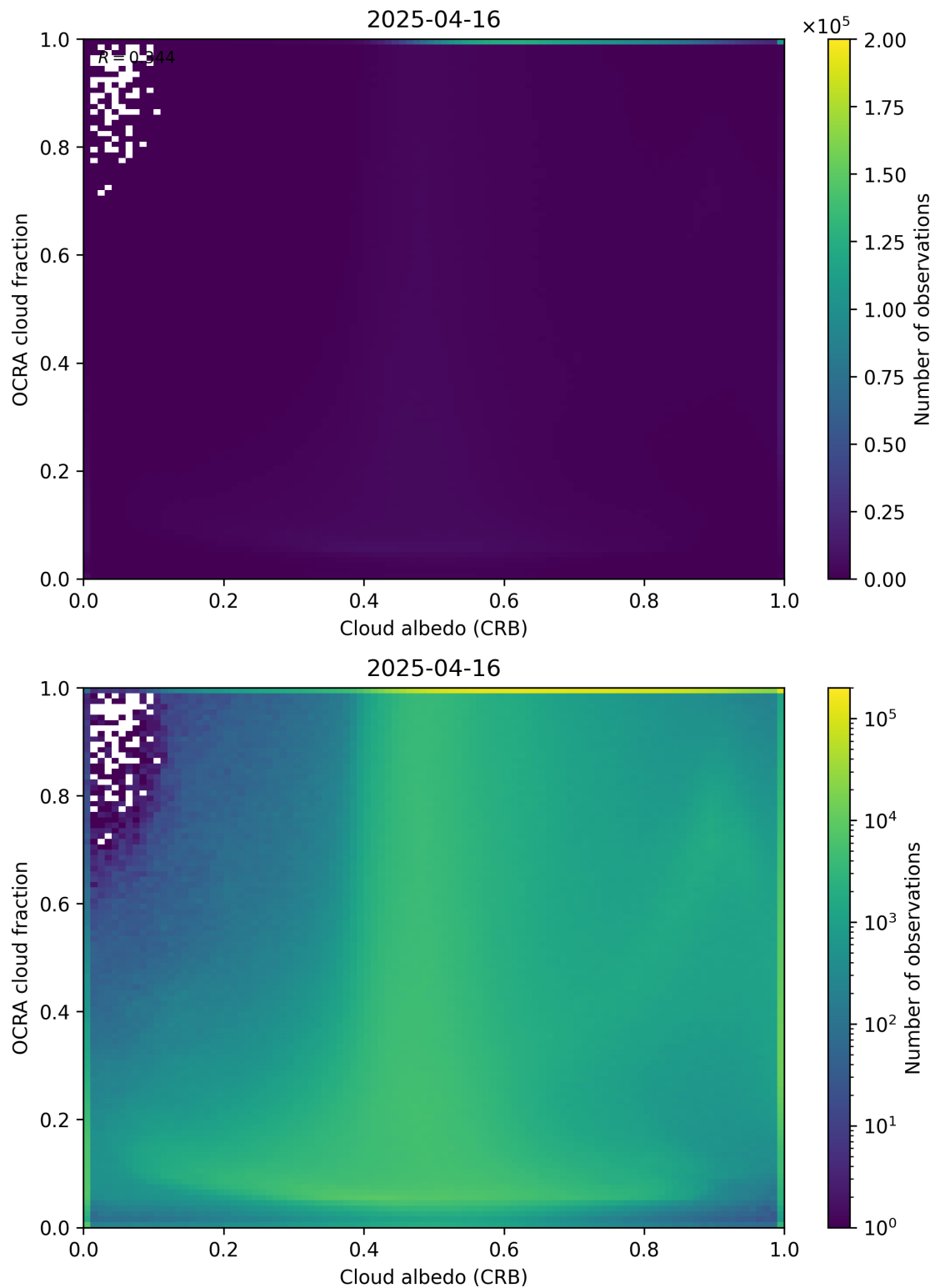
Figure 70: Scatter density plot of “Cloud albedo (CRB)” against “OCRA cloud fraction” for 2025-04-15 to 2025-04-17.
