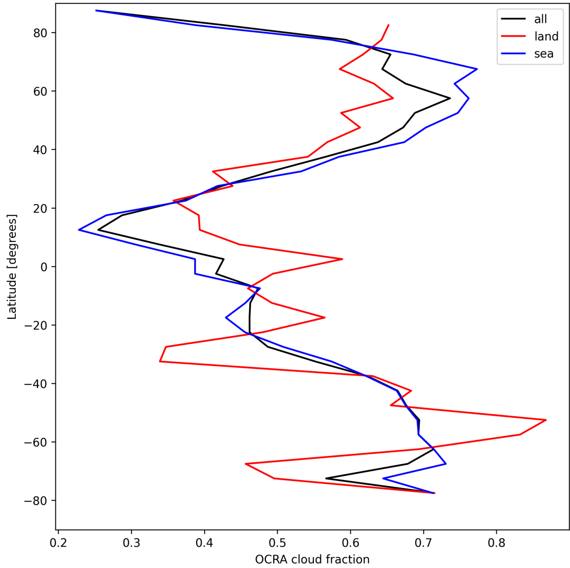
Figure 34: Zonal average of “OCRA cloud fraction” for 2025-04-15 to 2025-04-17.
