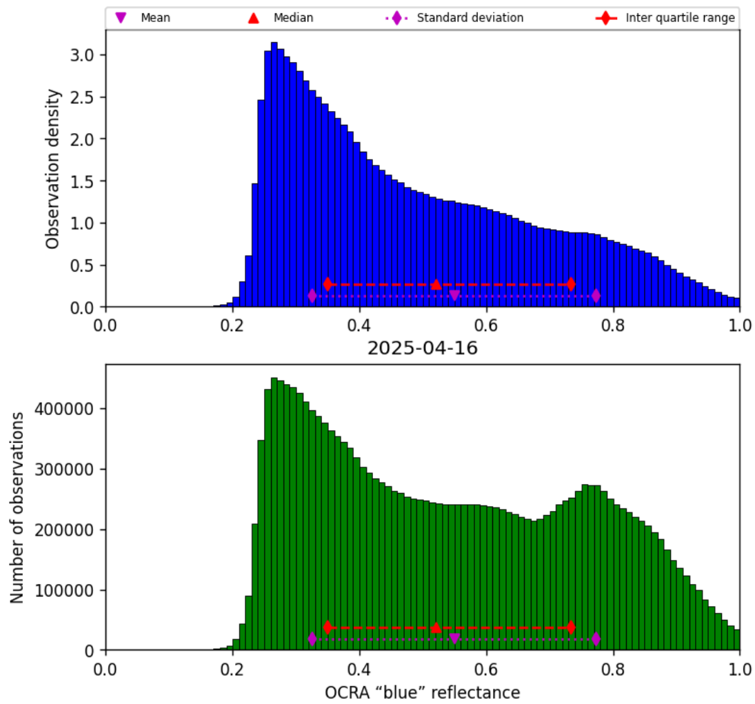
Figure 51: Histogram of “OCRA “blue” reflectance” for 2025-04-15 to 2025-04-17
