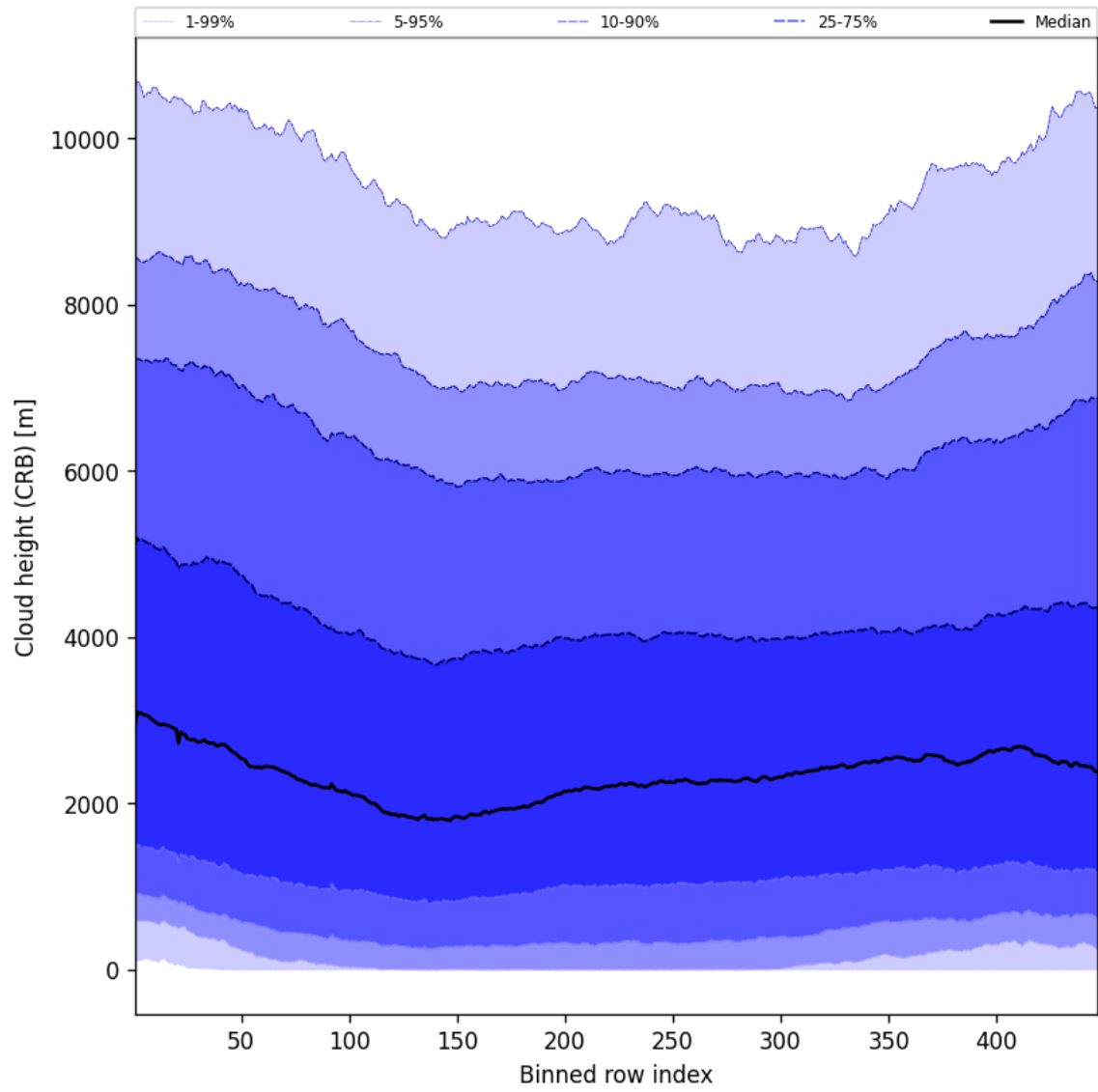
Figure 59: Along track statistics of “Cloud height (CRB)” for 2025-04-15 to 2025-04-17
