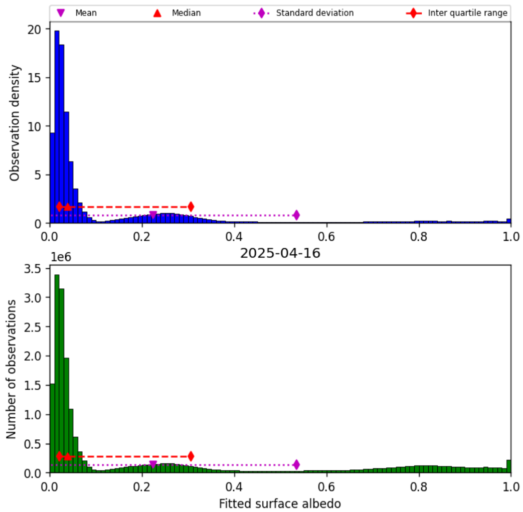
Figure 45: Histogram of “Fitted surface albedo” for 2025-04-15 to 2025-04-17
