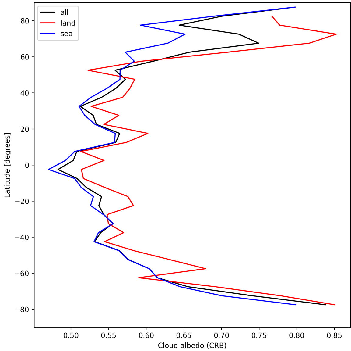
Figure 28: Zonal average of “Cloud albedo (CRB)” for 2025-04-15 to 2025-04-17.
