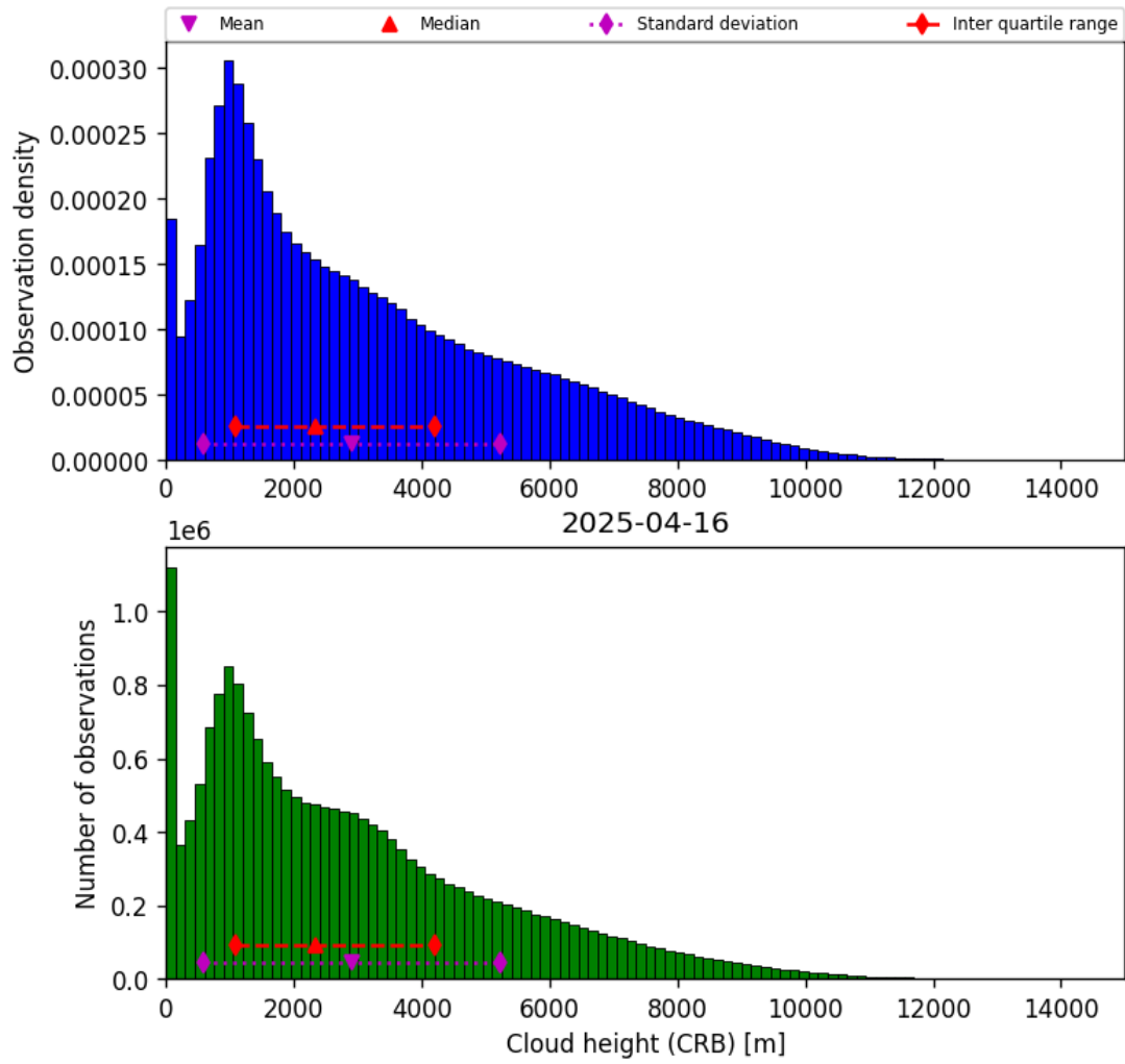
Figure 43: Histogram of “Cloud height (CRB)” for 2025-04-15 to 2025-04-17
