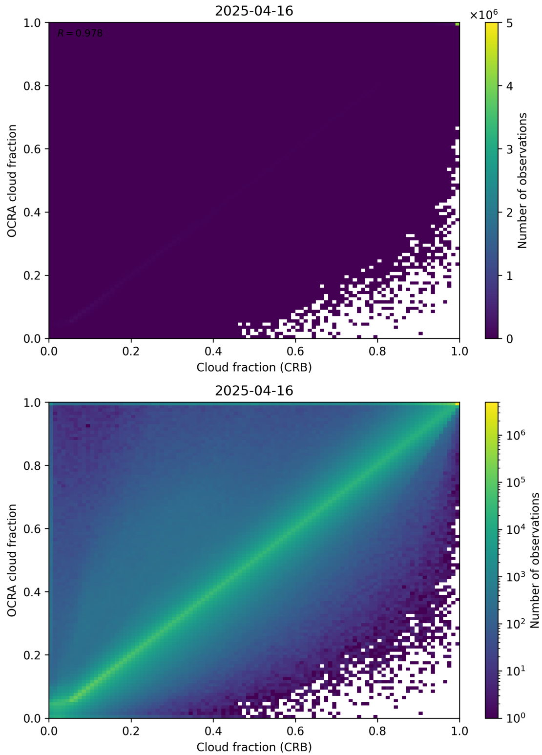
Figure 78: Scatter density plot of “Cloud fraction (CRB)” against “OCRA cloud fraction” for 2025-04-15 to 2025-04-17.
