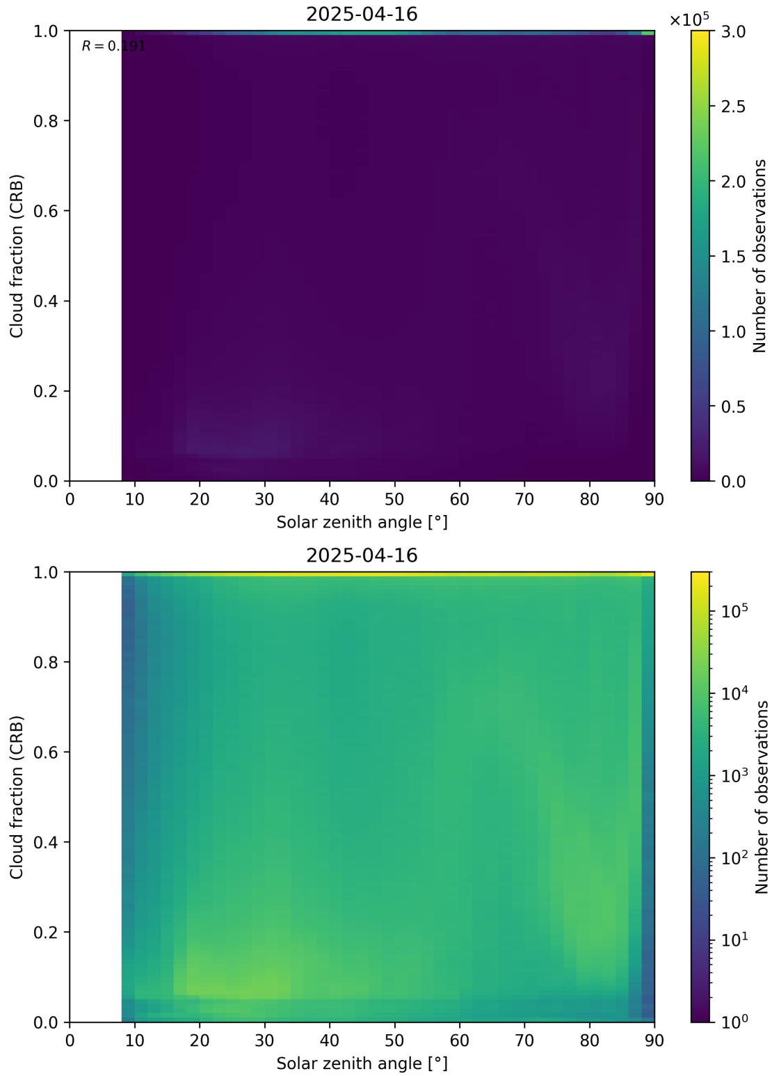
Figure 101: Scatter density plot of “Solar zenith angle” against “Cloud fraction (CRB)” for 2025-04-15 to 2025-04-17.
