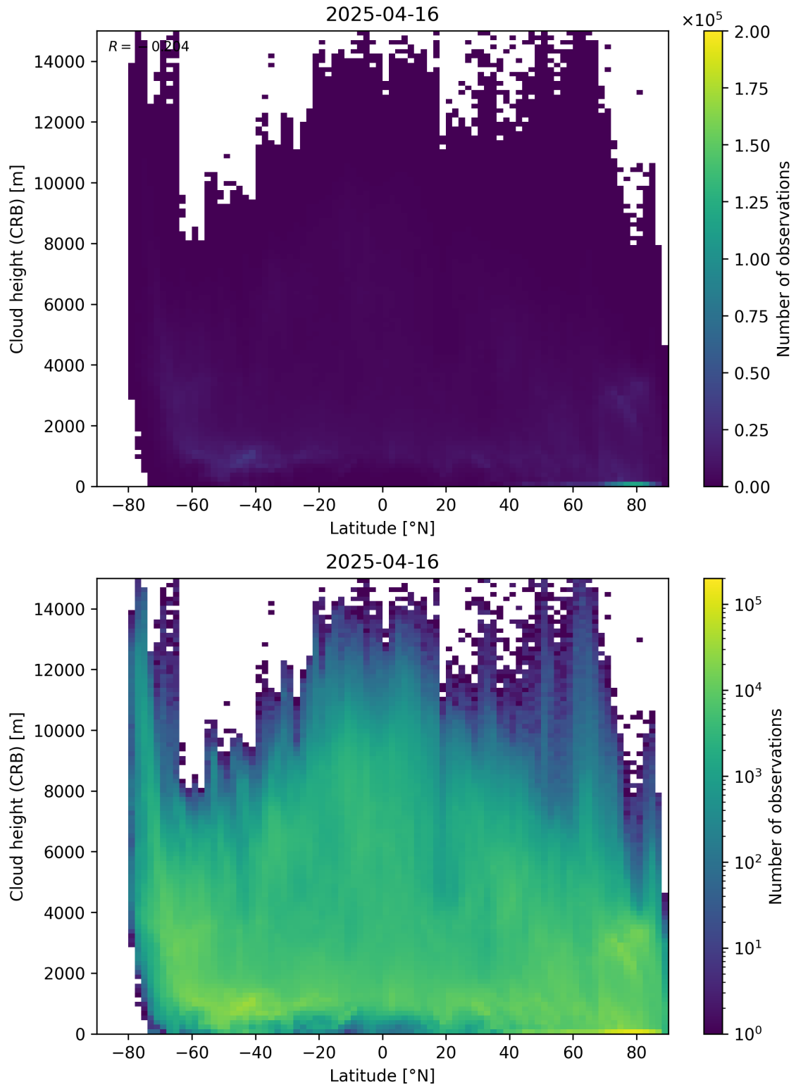
Figure 95: Scatter density plot of “Latitude” against “Cloud height (CRB)” for 2025-04-15 to 2025-04-17.
