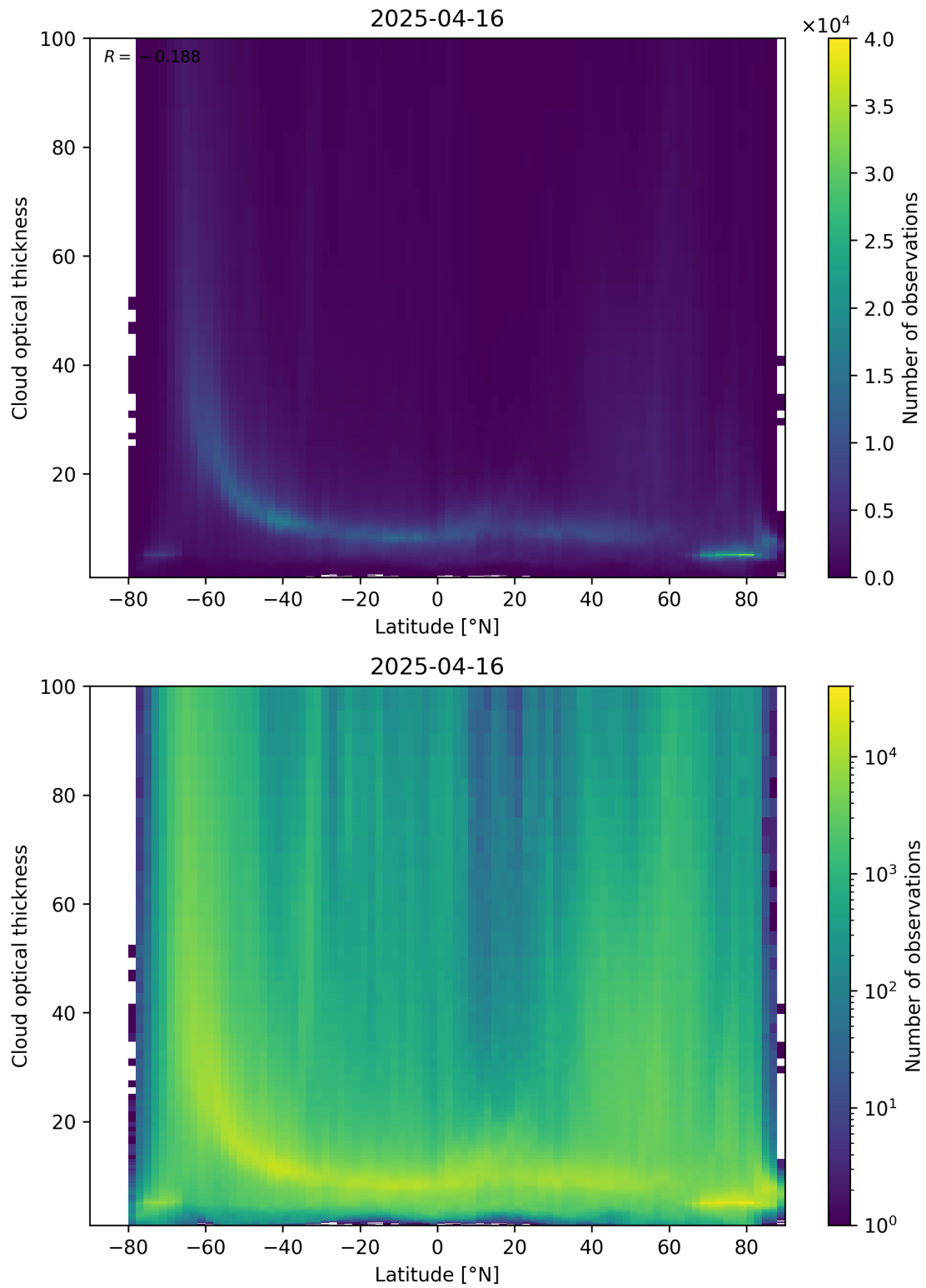
Figure 96: Scatter density plot of “Latitude” against “Cloud optical thickness” for 2025-04-15 to 2025-04-17.
