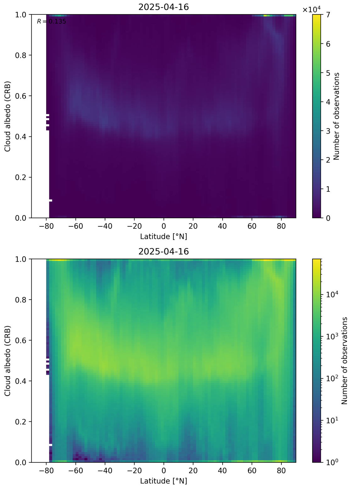
Figure 91: Scatter density plot of “Latitude” against “Cloud albedo (CRB)” for 2025-04-15 to 2025-04-17.
