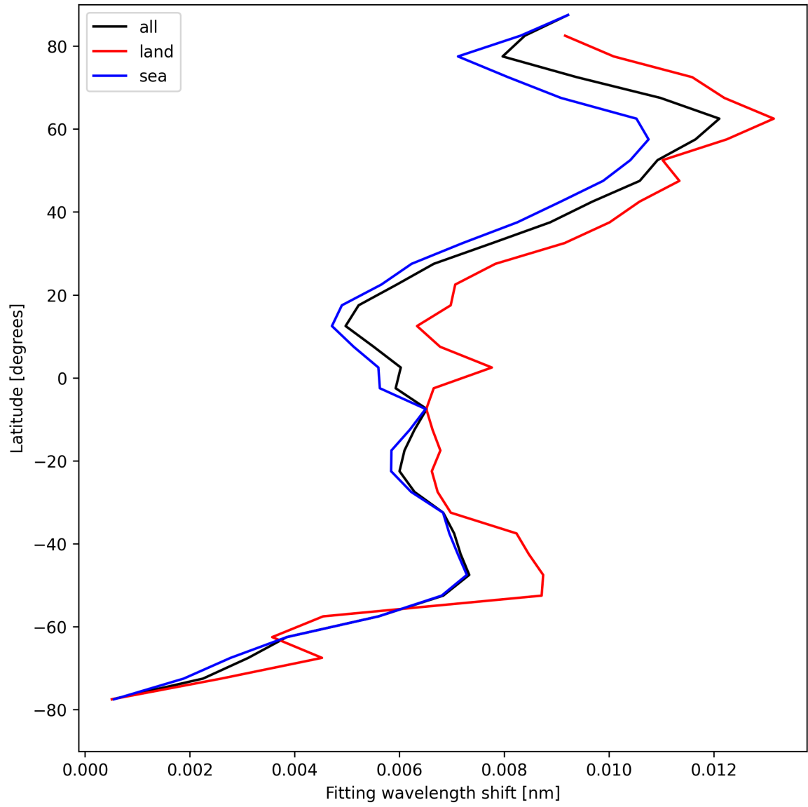
Figure 33: Zonal average of “Fitting wavelength shift” for 2025-04-15 to 2025-04-17.
