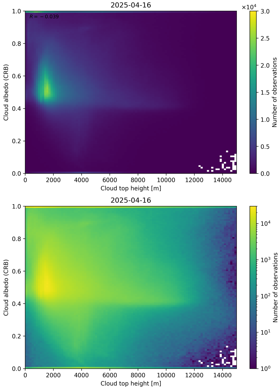
Figure 86: Scatter density plot of “Cloud top height” against “Cloud albedo (CRB)” for 2025-04-15 to 2025-04-17.
