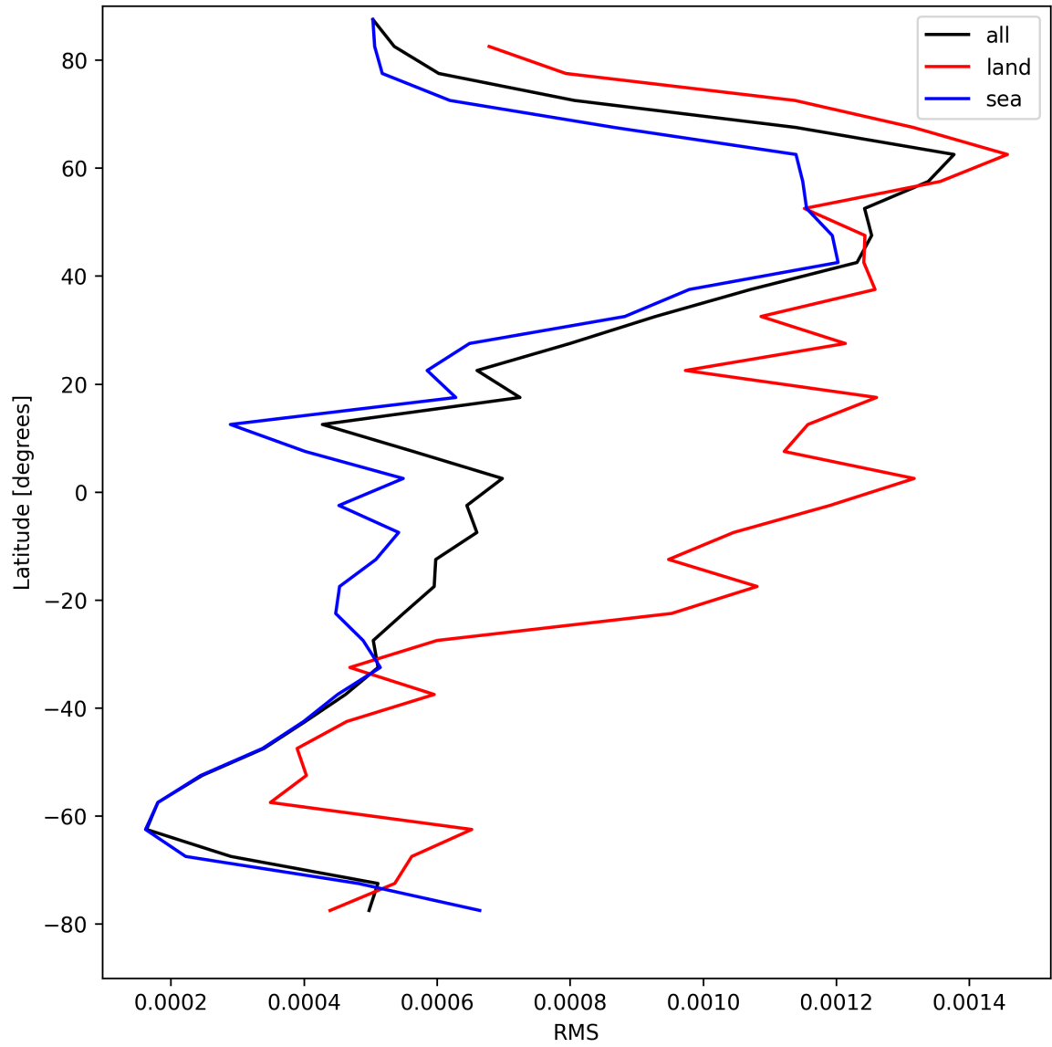
Figure 31: Zonal average of “RMS” for 2025-04-15 to 2025-04-17.
