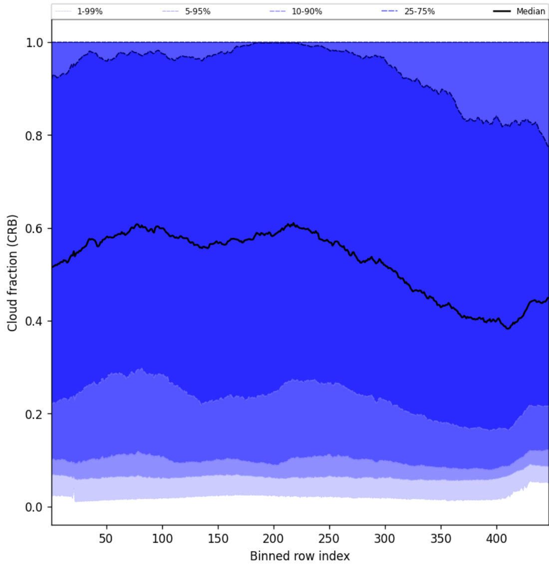
Figure 58: Along track statistics of “Cloud fraction (CRB)” for 2025-04-15 to 2025-04-17
