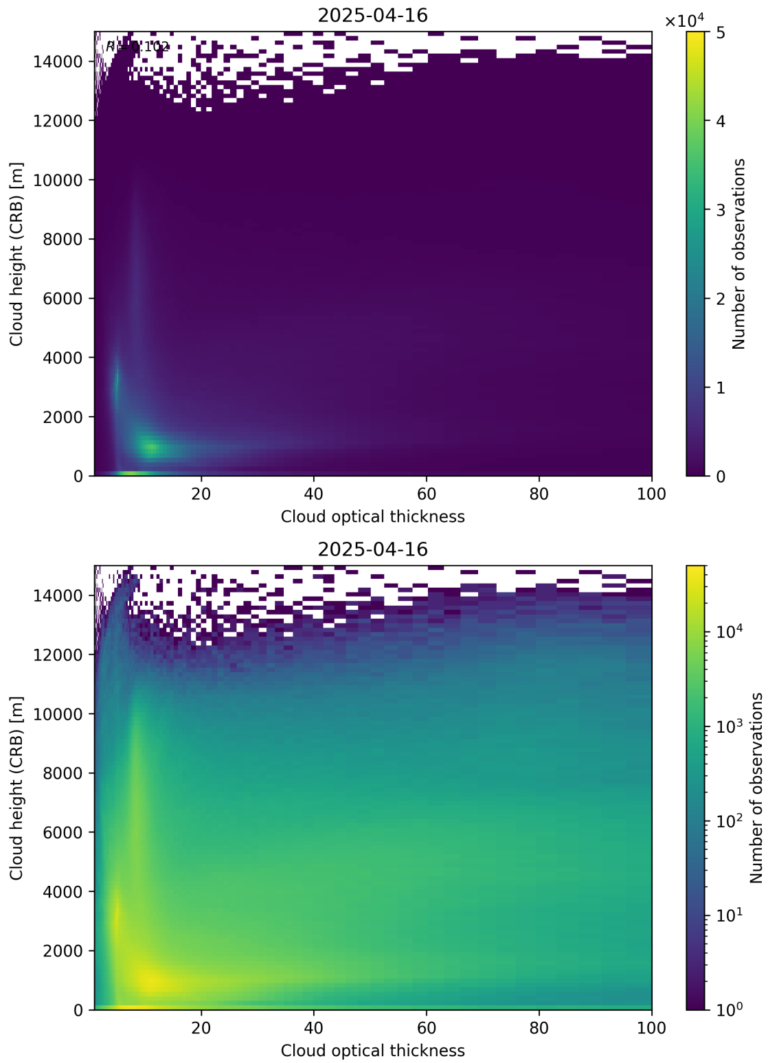
Figure 85: Scatter density plot of “Cloud optical thickness” against “Cloud height (CRB)” for 2025-04-15 to 2025-04-17.
