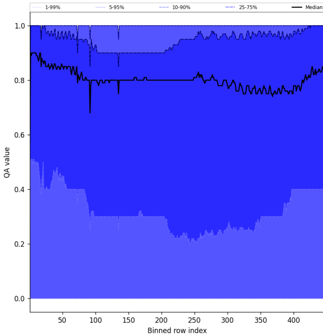
Figure 54: Along track statistics of “QA value” for 2025-04-15 to 2025-04-17
