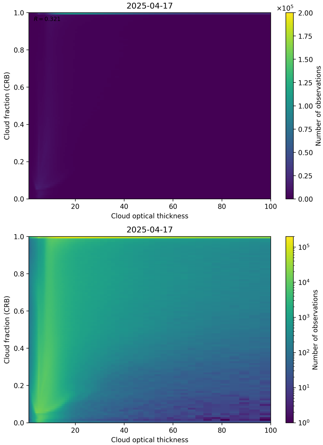
Figure 84: Scatter density plot of “Cloud optical thickness” against “Cloud fraction (CRB)” for 2025-04-16 to 2025-04-18.
