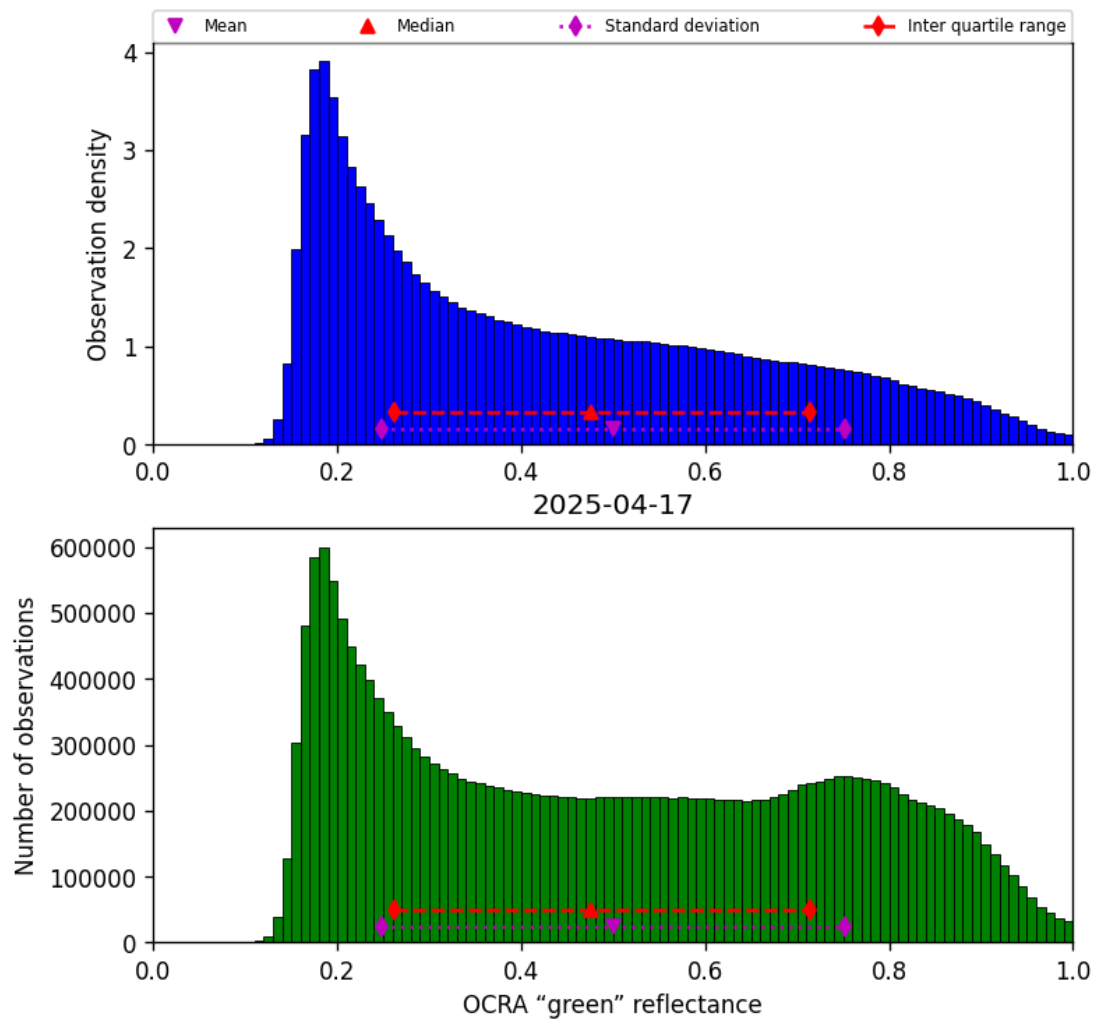
Figure 52: Histogram of “OCRA “green” reflectance” for 2025-04-16 to 2025-04-18
