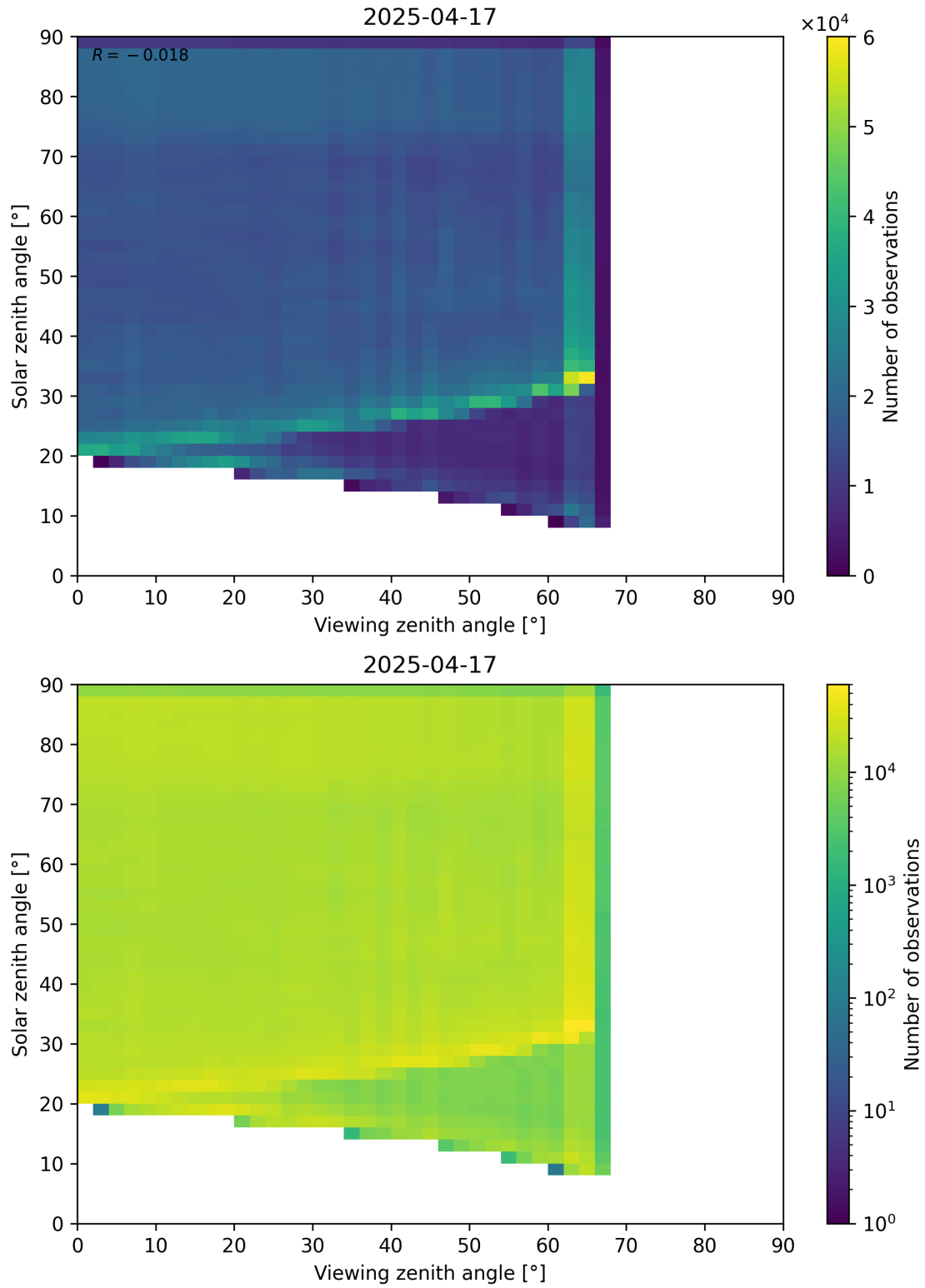
Figure 114: Scatter density plot of “Viewing zenith angle” against “Solar zenith angle” for 2025-04-16 to 2025-04-18.
