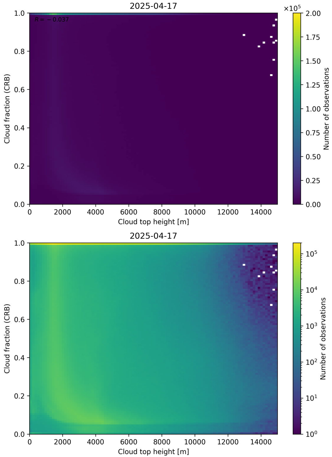
Figure 88: Scatter density plot of “Cloud top height” against “Cloud fraction (CRB)” for 2025-04-16 to 2025-04-18.
