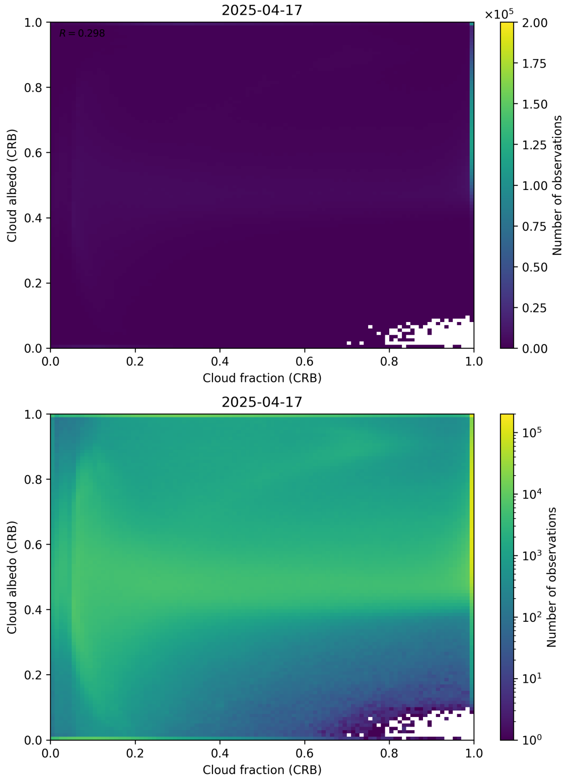
Figure 77: Scatter density plot of “Cloud fraction (CRB)” against “Cloud albedo (CRB)” for 2025-04-16 to 2025-04-18.
