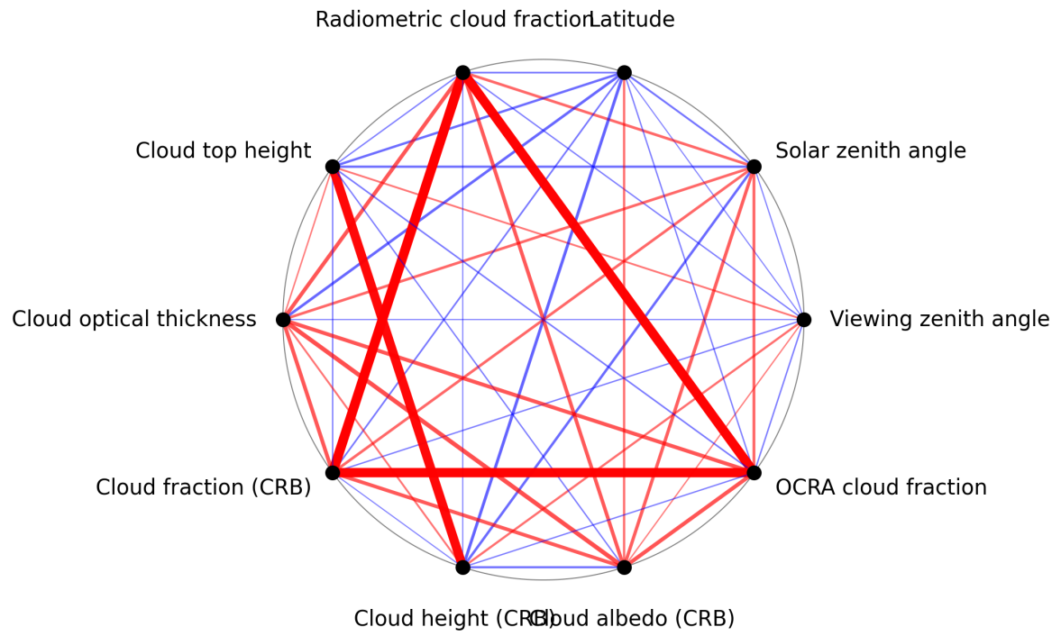
Figure 1: Map of correlation graph for 2025-04-16 to 2025-04-18.
