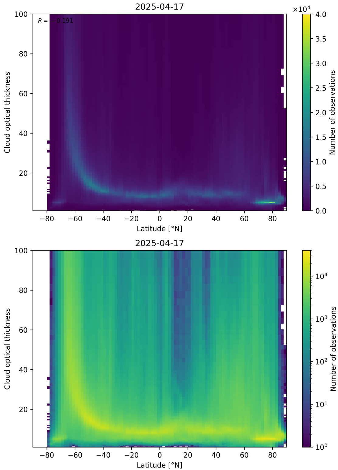
Figure 96: Scatter density plot of “Latitude” against “Cloud optical thickness” for 2025-04-16 to 2025-04-18.
