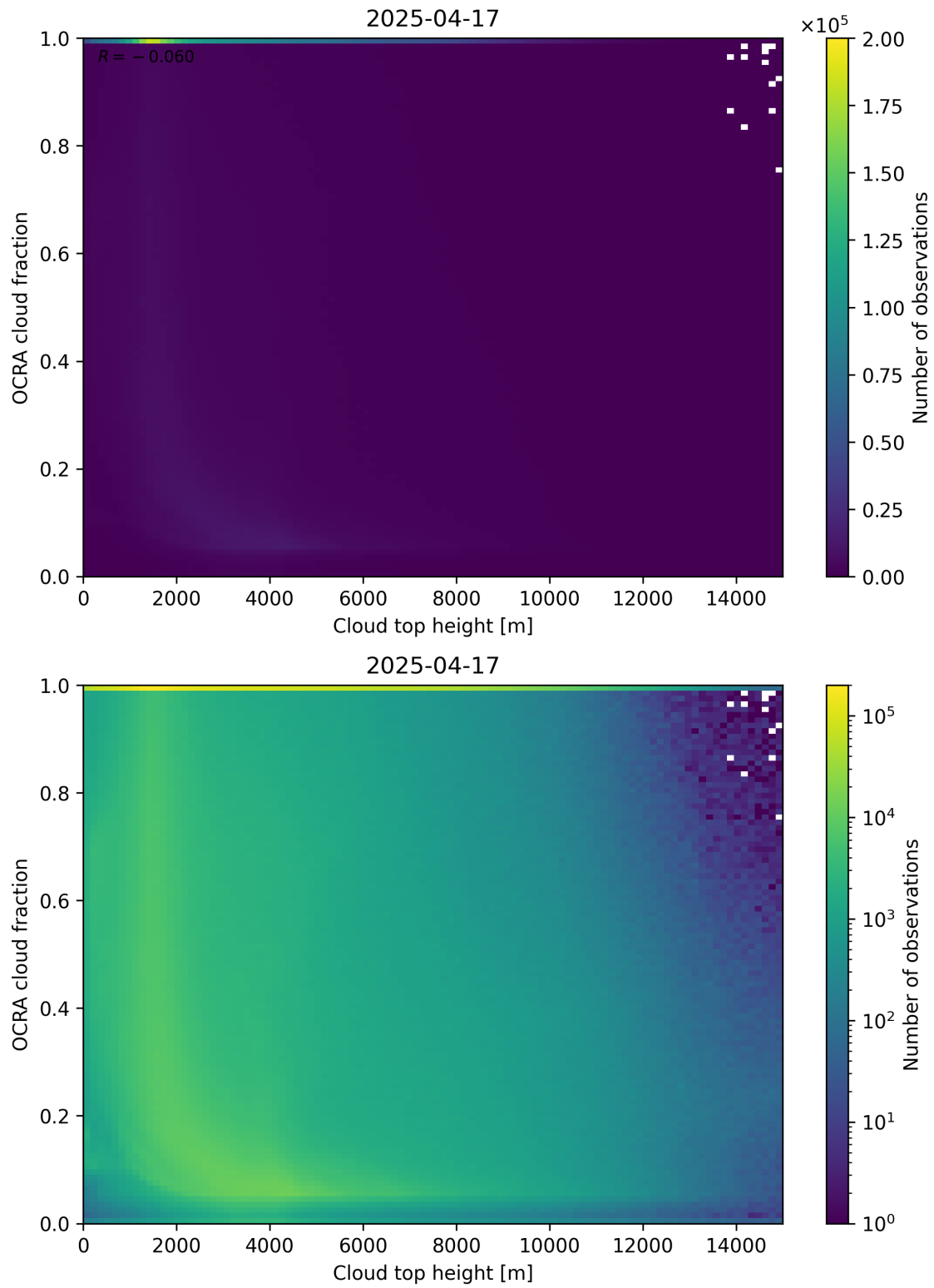
Figure 87: Scatter density plot of “Cloud top height” against “OCRA cloud fraction” for 2025-04-16 to 2025-04-18.
