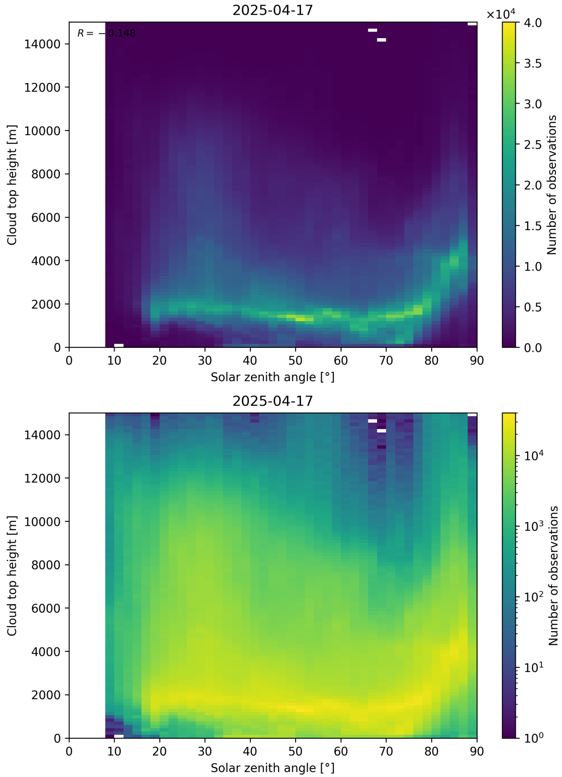
Figure 104: Scatter density plot of “Solar zenith angle” against “Cloud top height” for 2025-04-16 to 2025-04-18.
