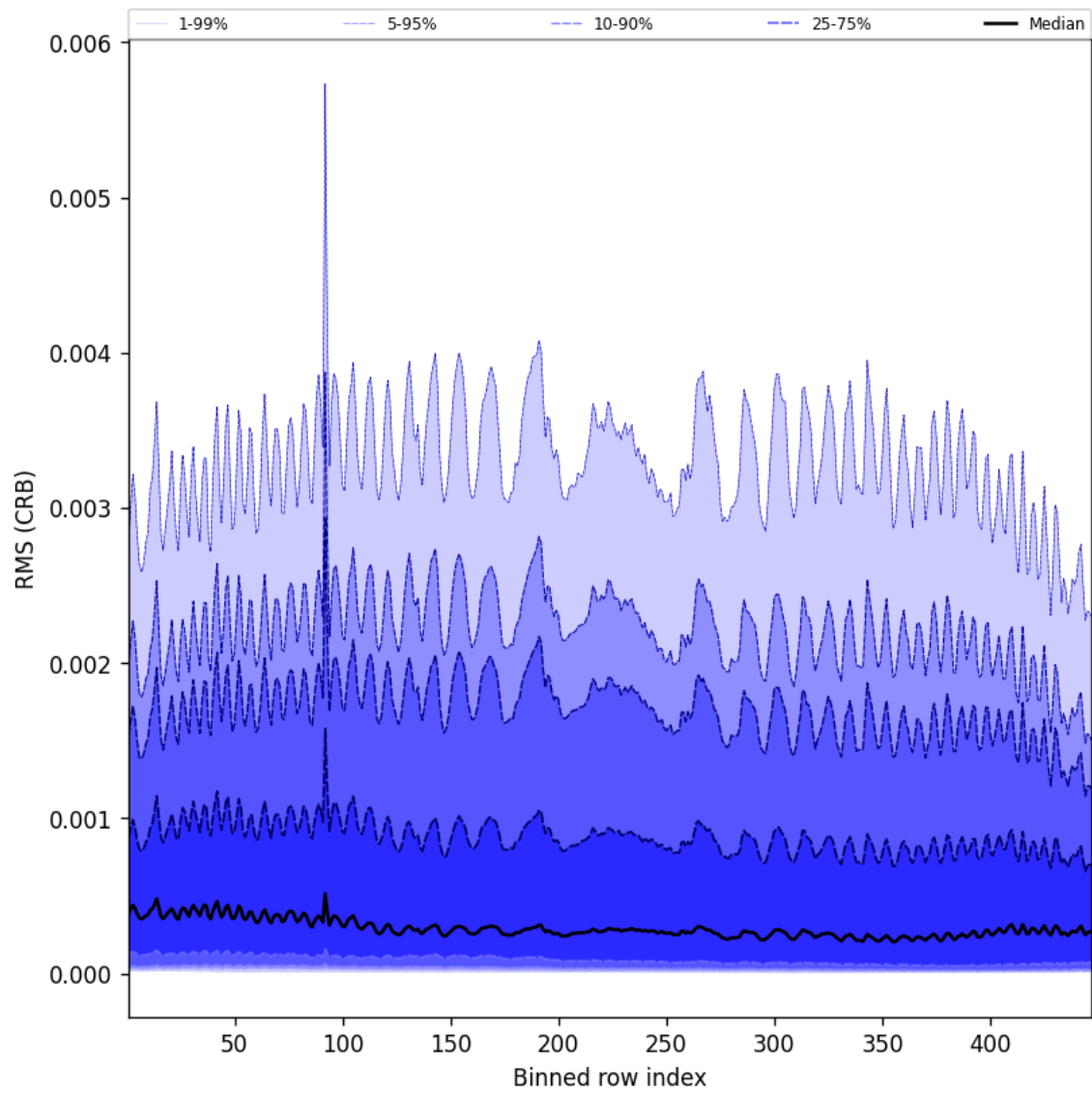
Figure 64: Along track statistics of “RMS (CRB)” for 2025-04-16 to 2025-04-18
