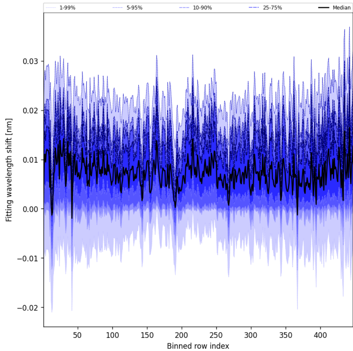
Figure 65: Along track statistics of “Fitting wavelength shift” for 2025-04-16 to 2025-04-18
