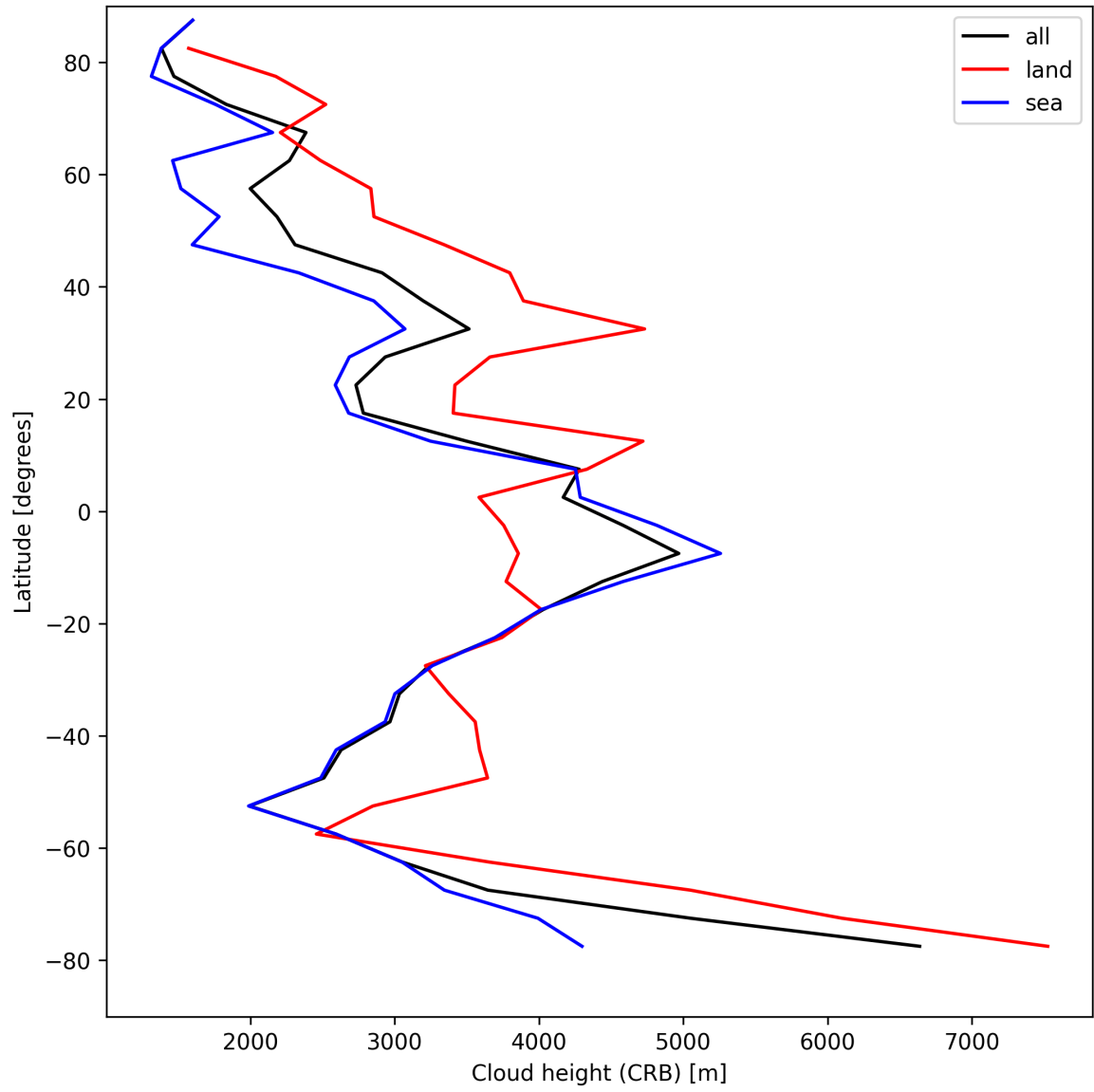
Figure 27: Zonal average of “Cloud height (CRB)” for 2025-04-16 to 2025-04-18.
