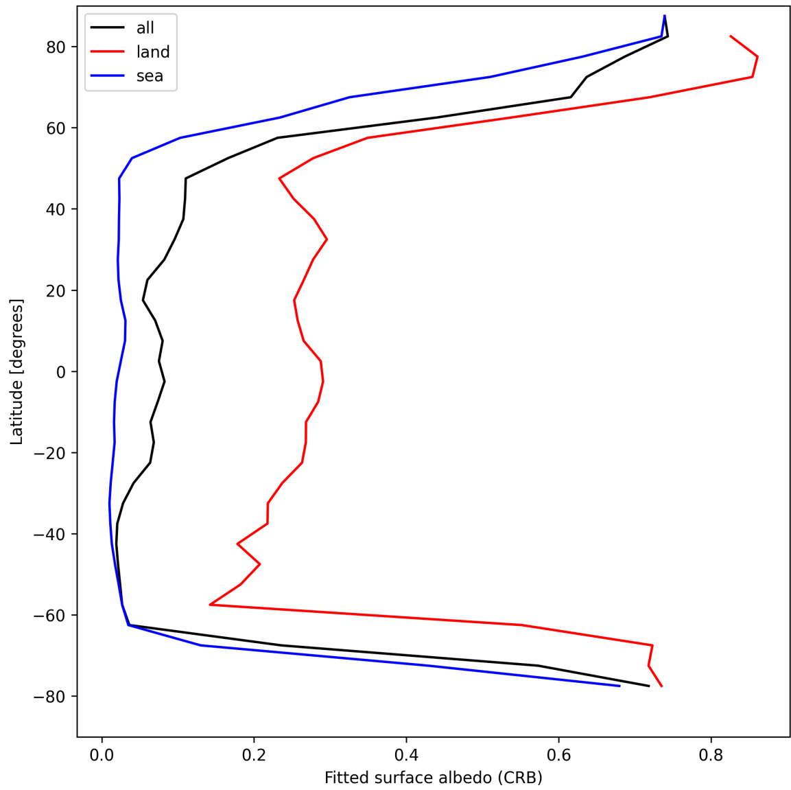
Figure 30: Zonal average of “Fitted surface albedo (CRB)” for 2025-04-16 to 2025-04-18.
