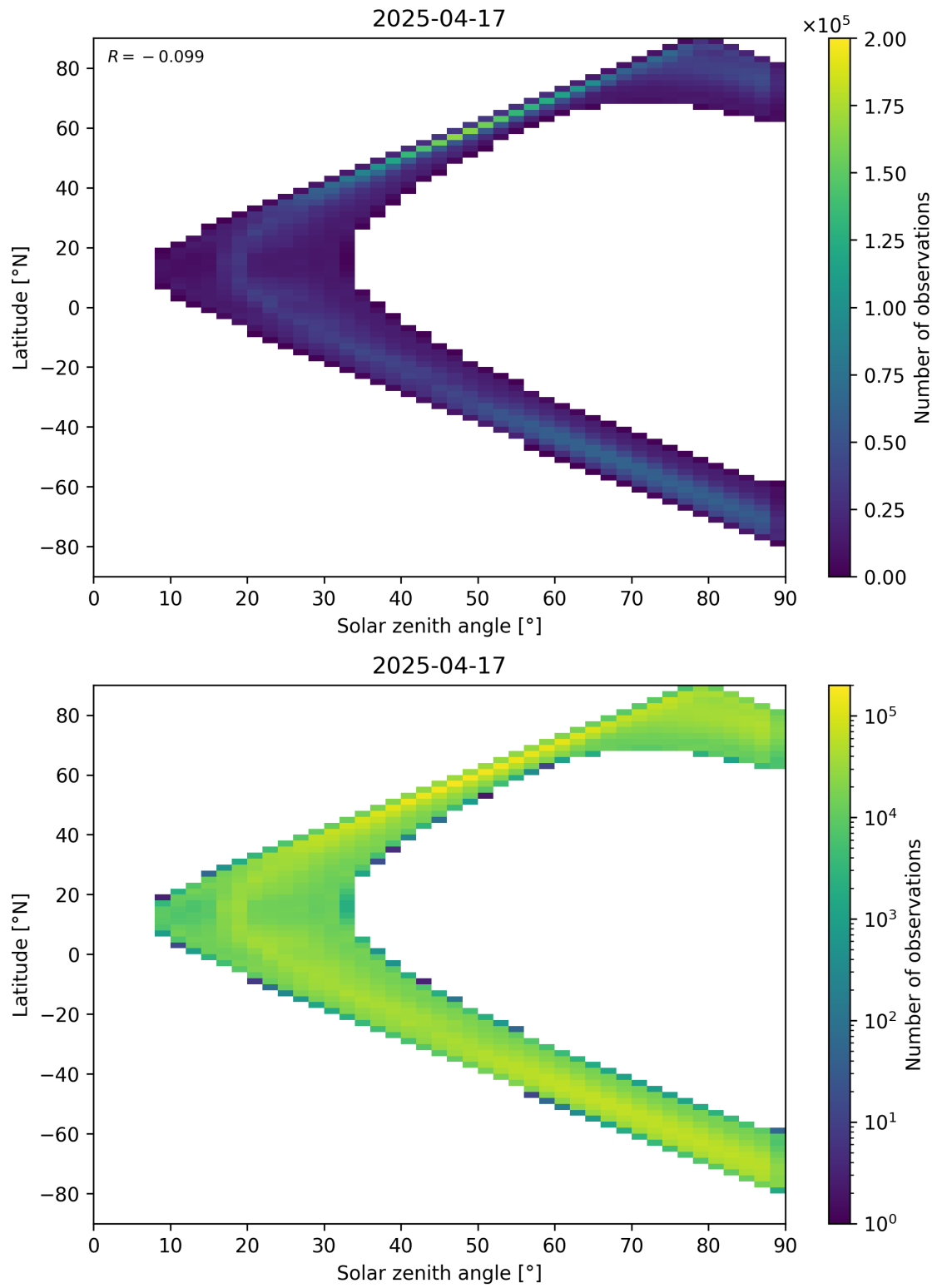
Figure 105: Scatter density plot of “Solar zenith angle” against “Latitude” for 2025-04-16 to 2025-04-18.
