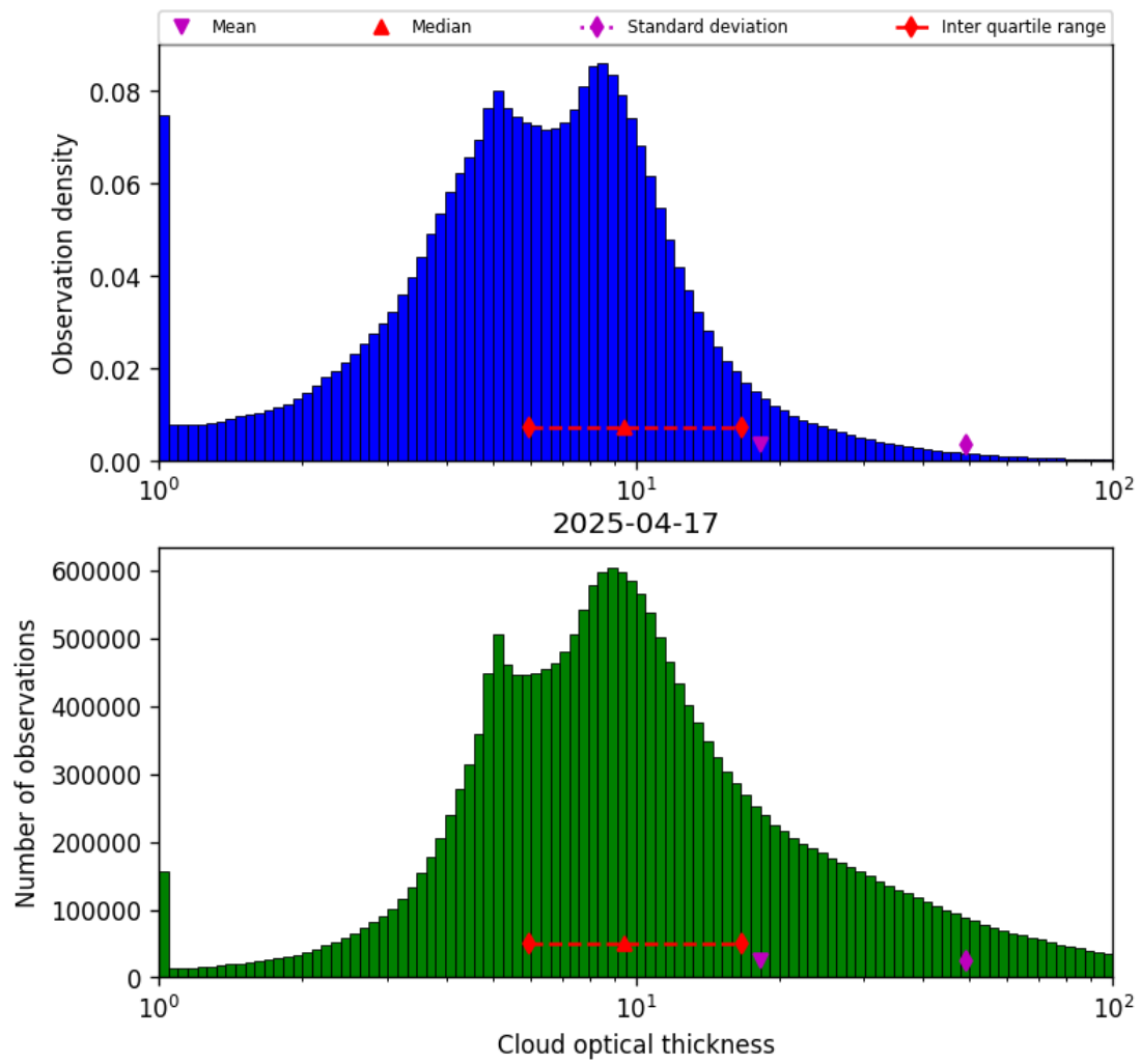
Figure 41: Histogram of “Cloud optical thickness” for 2025-04-16 to 2025-04-18
