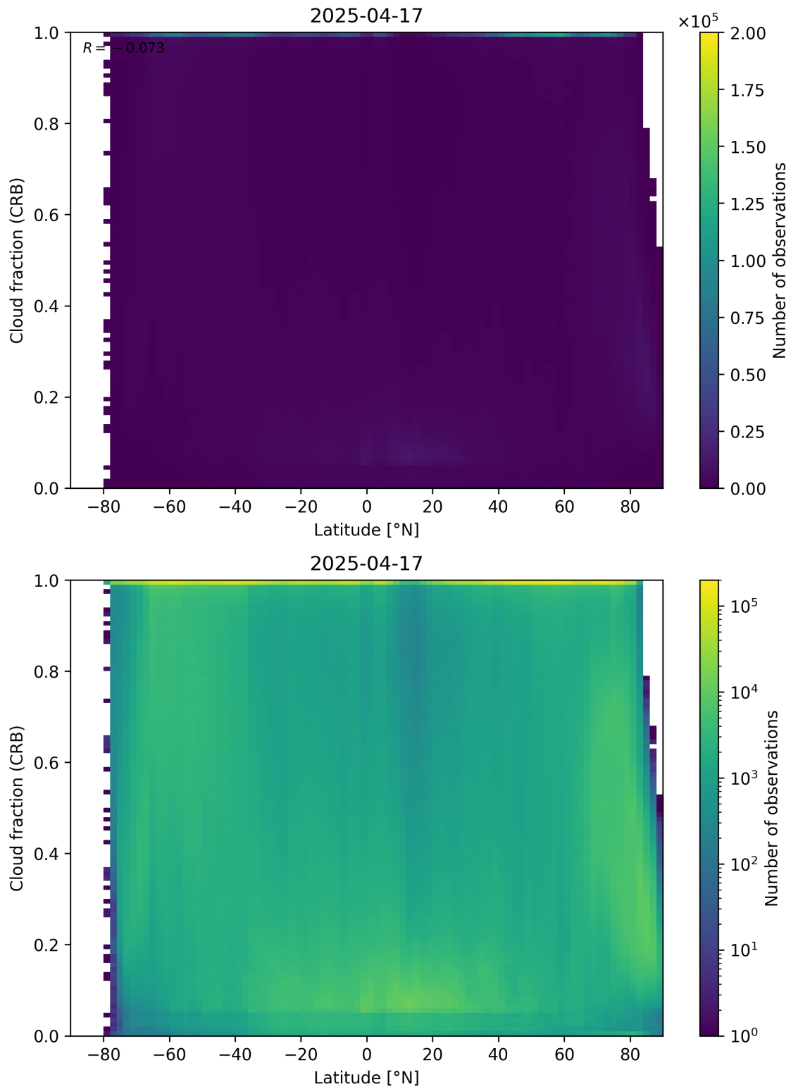
Figure 94: Scatter density plot of “Latitude” against “Cloud fraction (CRB)” for 2025-04-16 to 2025-04-18.
