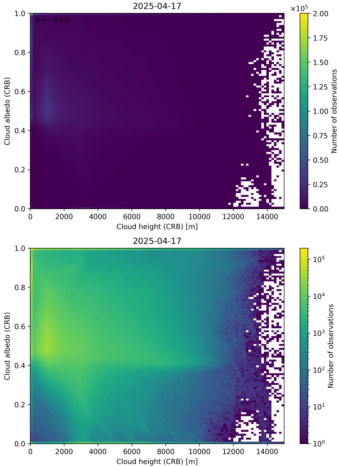
Figure 80: Scatter density plot of “Cloud height (CRB)” against “Cloud albedo (CRB)” for 2025-04-16 to 2025-04-18.
