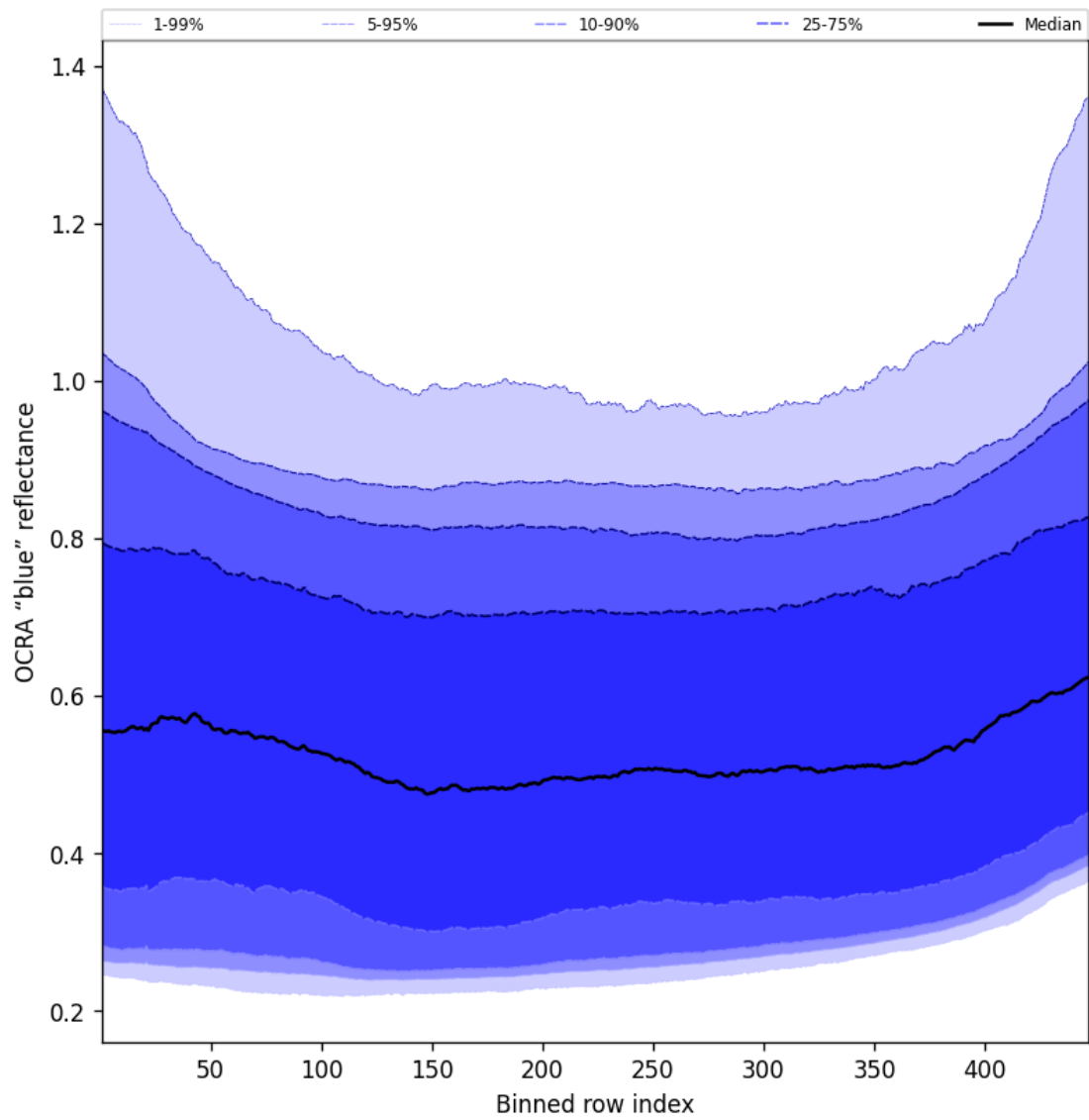
Figure 67: Along track statistics of “OCRA “blue” reflectance” for 2025-04-16 to 2025-04-18
