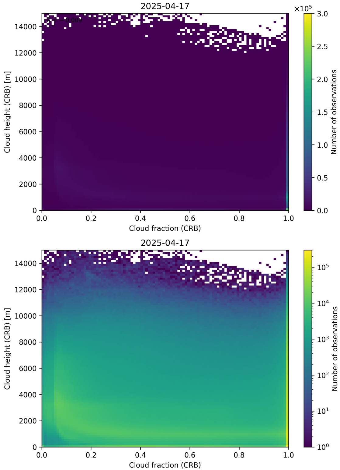
Figure 79: Scatter density plot of “Cloud fraction (CRB)” against “Cloud height (CRB)” for 2025-04-16 to 2025-04-18.
