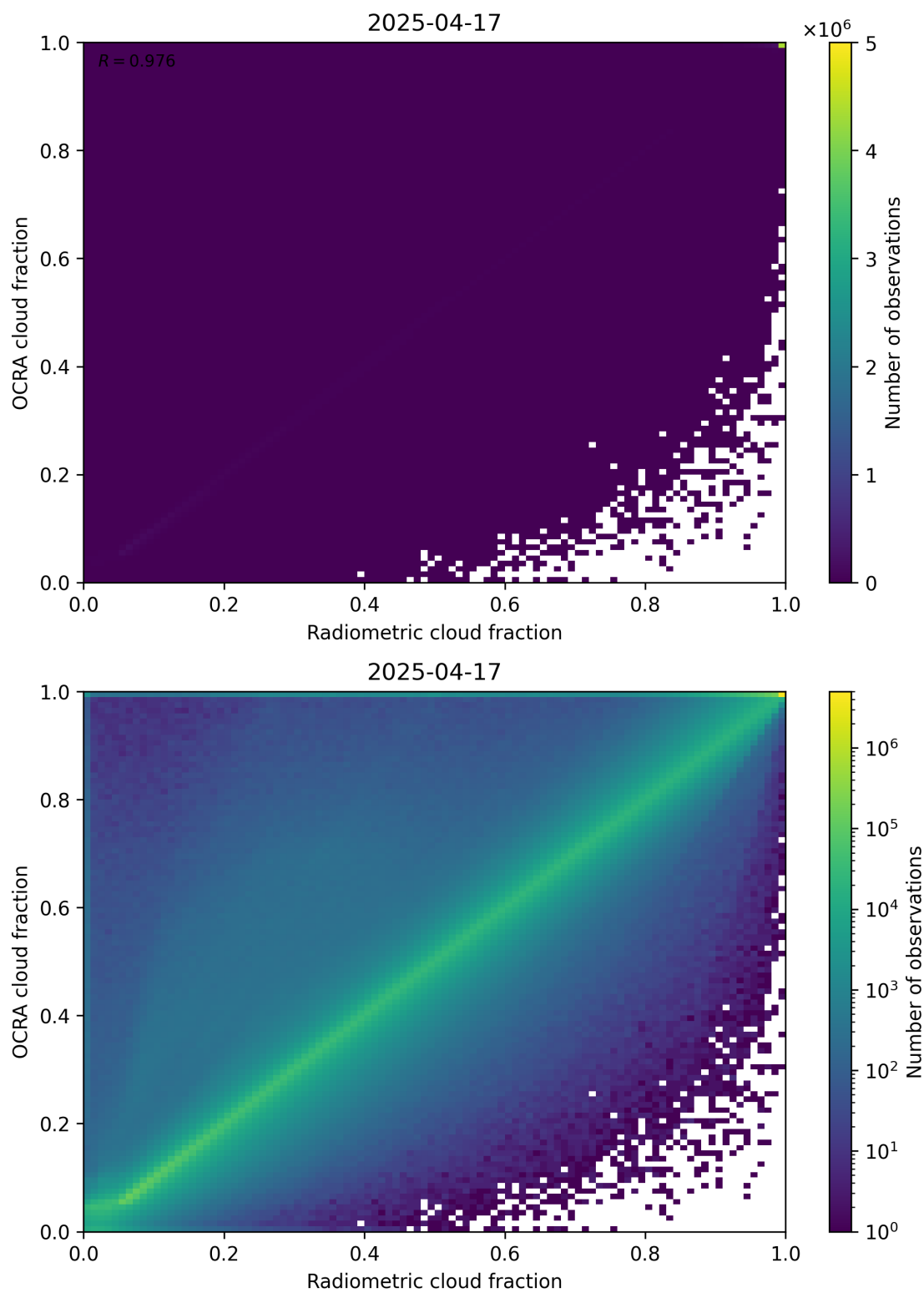
Figure 72: Scatter density plot of “Radiometric cloud fraction” against “OCRA cloud fraction” for 2025-04-16 to 2025-04-18.
