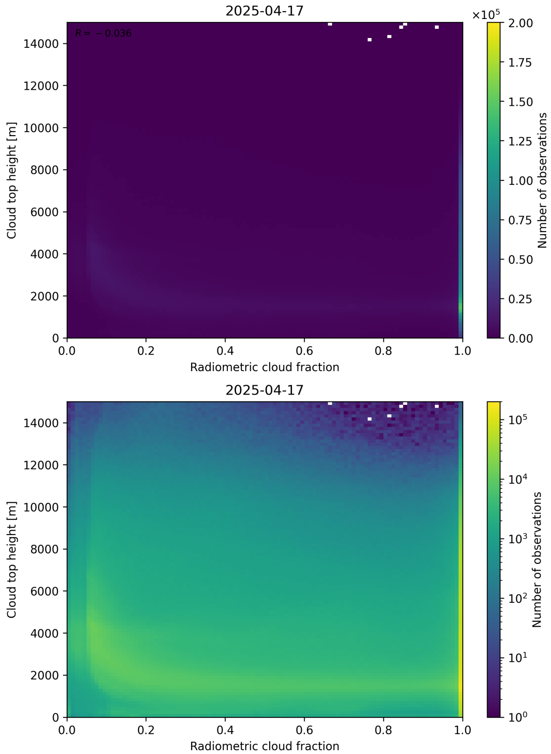
Figure 76: Scatter density plot of “Radiometric cloud fraction” against “Cloud top height” for 2025-04-16 to 2025-04-18.
