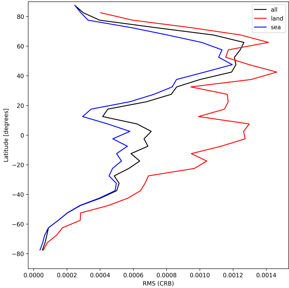
Figure 32: Zonal average of “RMS (CRB)” for 2025-04-16 to 2025-04-18.
