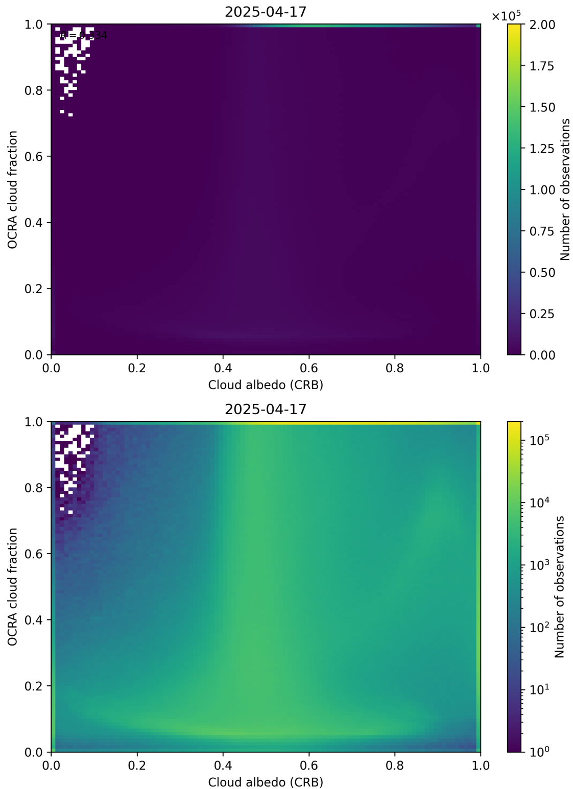
Figure 70: Scatter density plot of “Cloud albedo (CRB)” against “OCRA cloud fraction” for 2025-04-16 to 2025-04-18.
