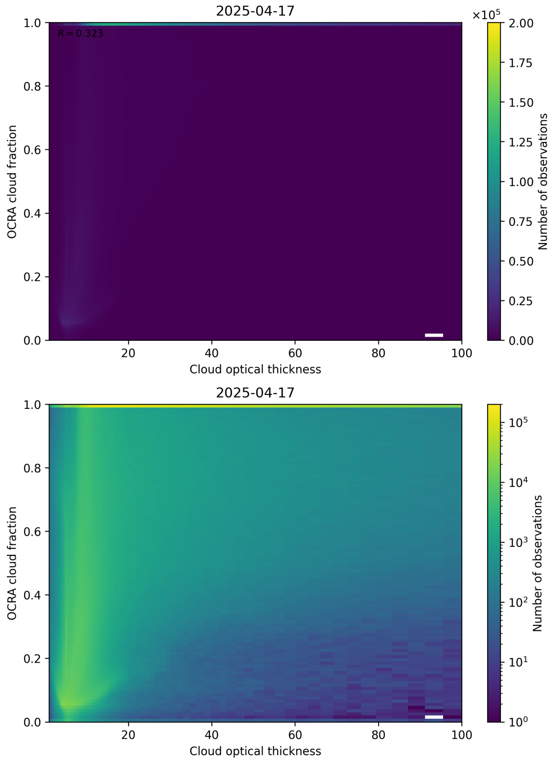
Figure 83: Scatter density plot of “Cloud optical thickness” against “OCRA cloud fraction” for 2025-04-16 to 2025-04-18.
