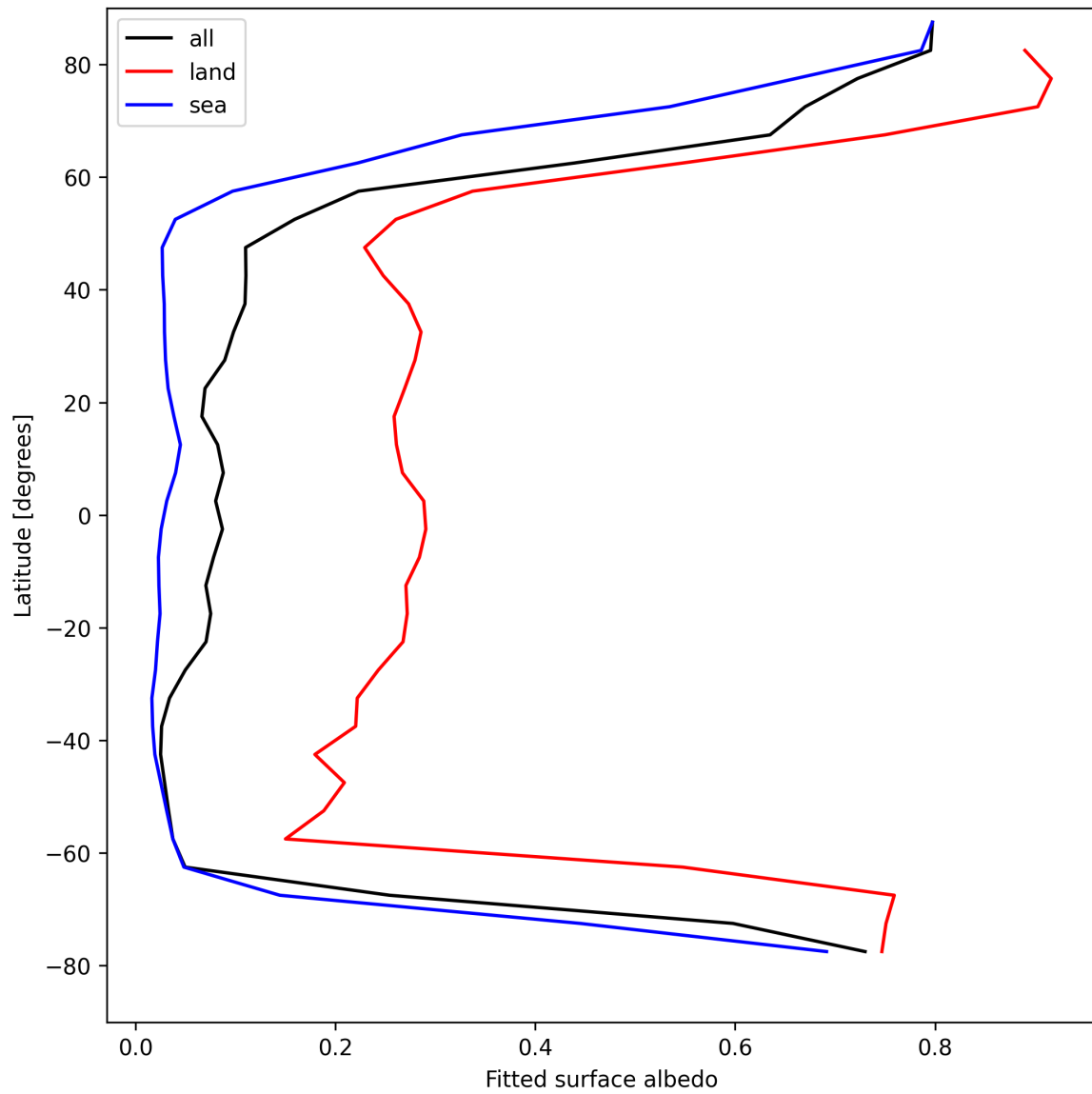
Figure 29: Zonal average of “Fitted surface albedo” for 2025-04-16 to 2025-04-18.
