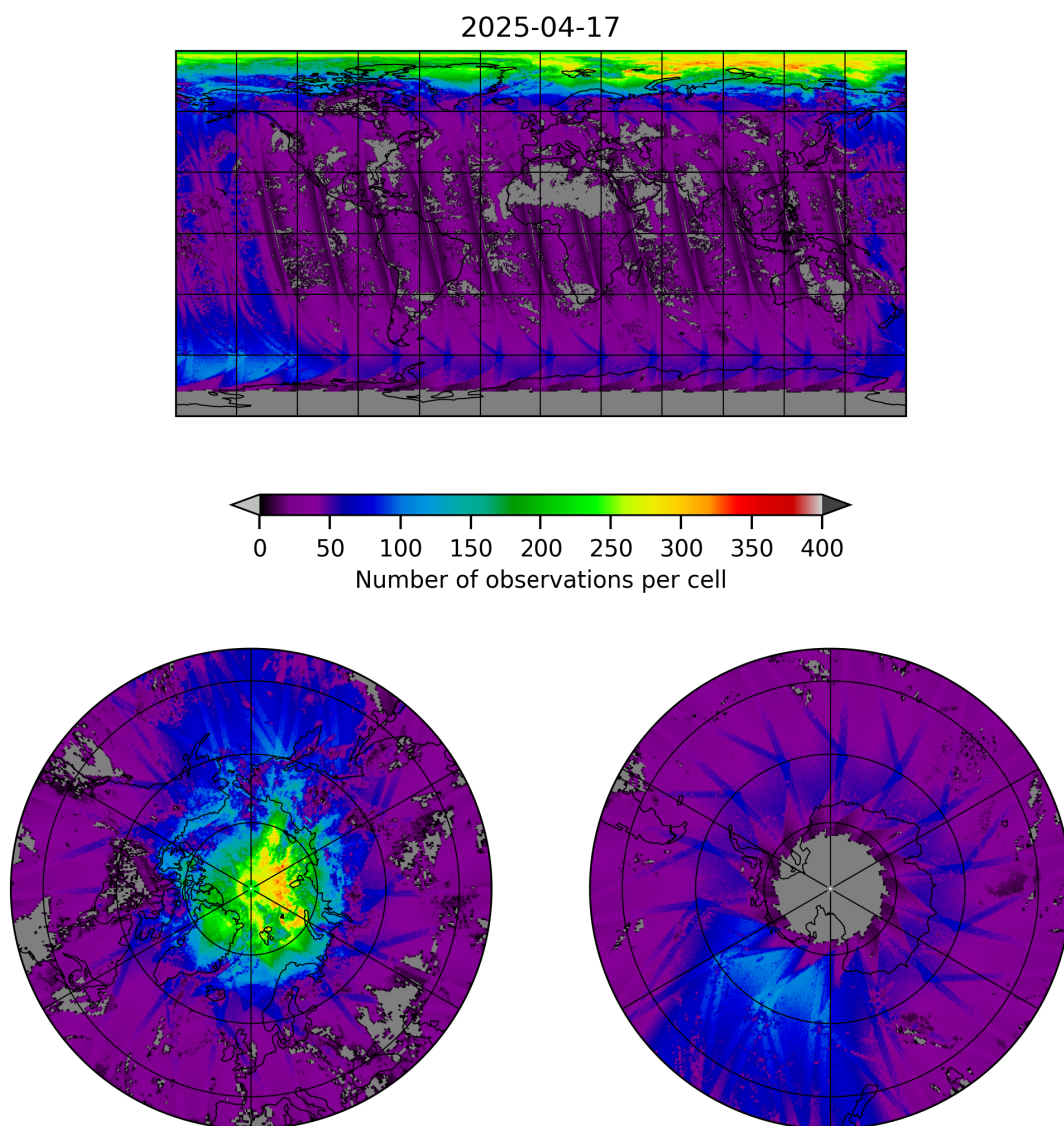
Figure 21: Map of the number of observations for 2025-04-16 to 2025-04-18
