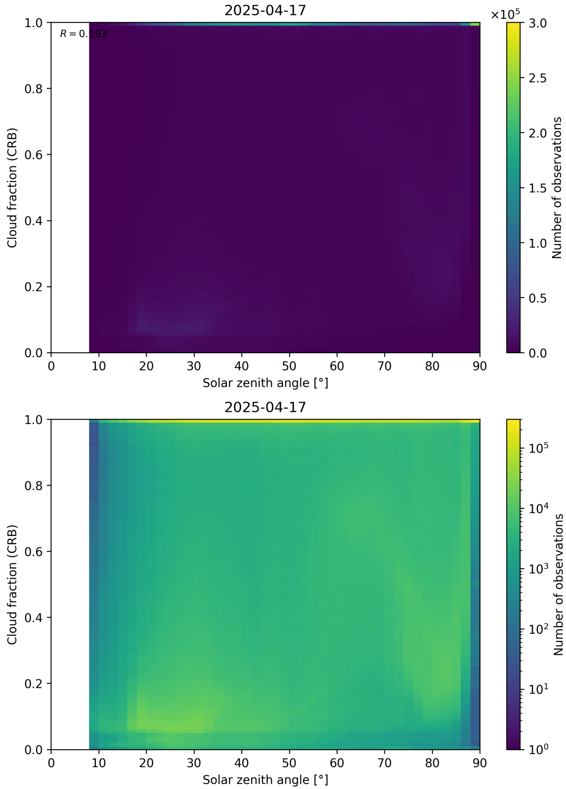
Figure 101: Scatter density plot of “Solar zenith angle” against “Cloud fraction (CRB)” for 2025-04-16 to 2025-04-18.
