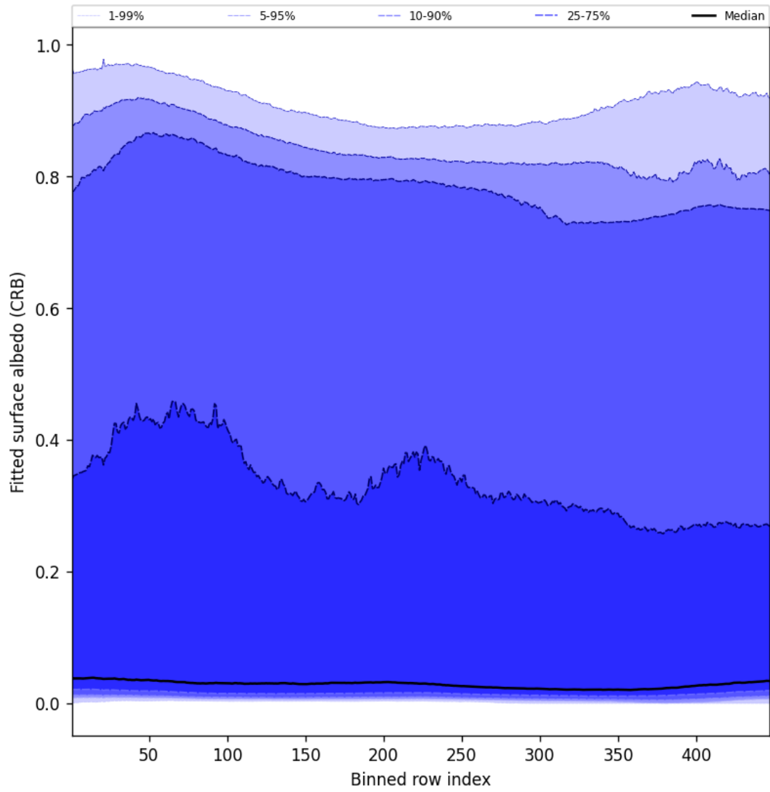
Figure 62: Along track statistics of “Fitted surface albedo (CRB)” for 2025-04-16 to 2025-04-18
