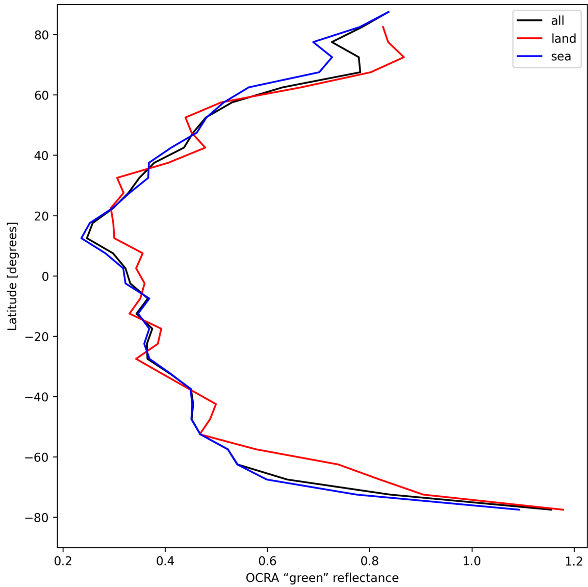
Figure 36: Zonal average of “OCRA “green” reflectance” for 2025-04-16 to 2025-04-18.
