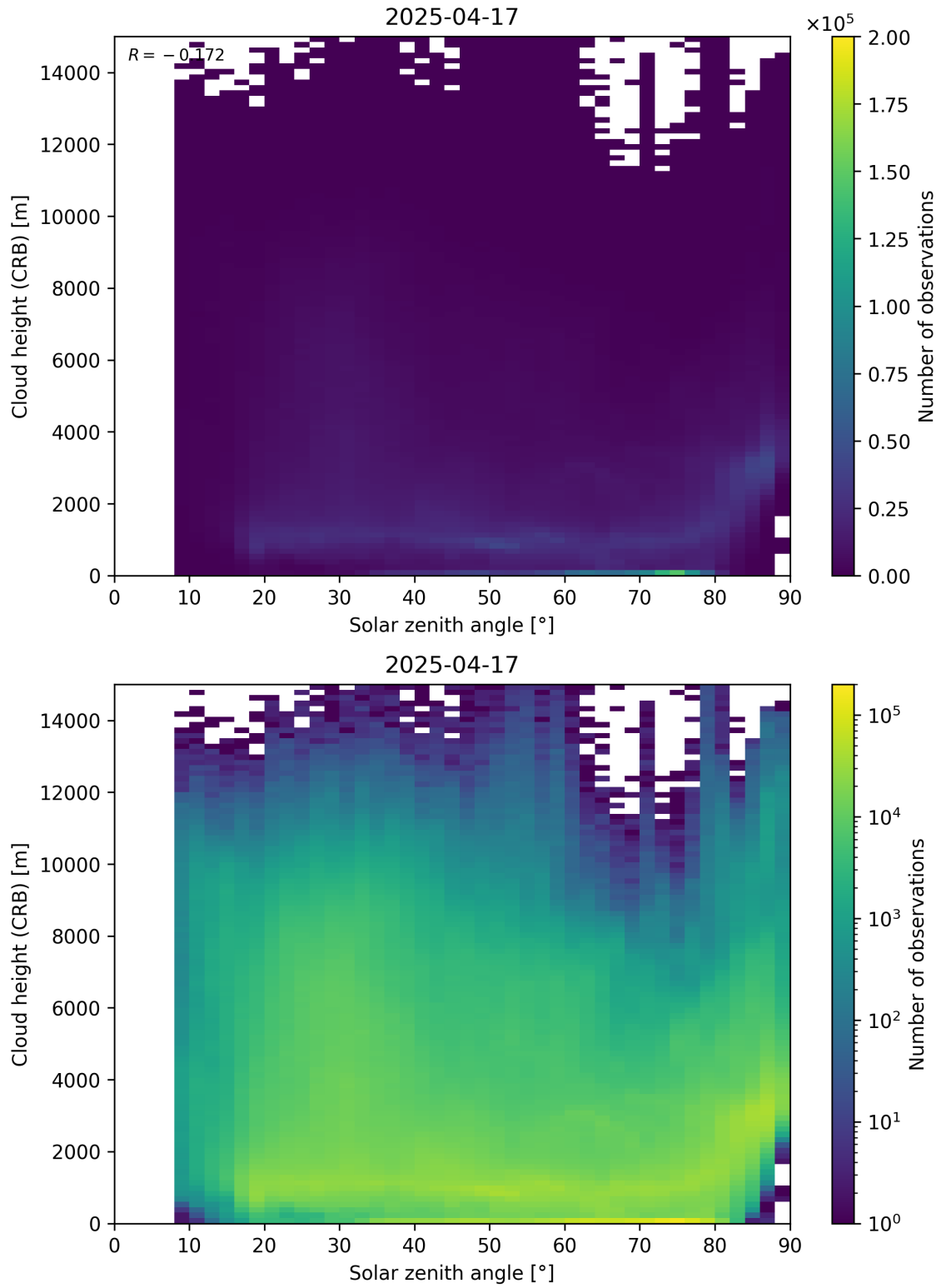
Figure 102: Scatter density plot of “Solar zenith angle” against “Cloud height (CRB)” for 2025-04-16 to 2025-04-18.
