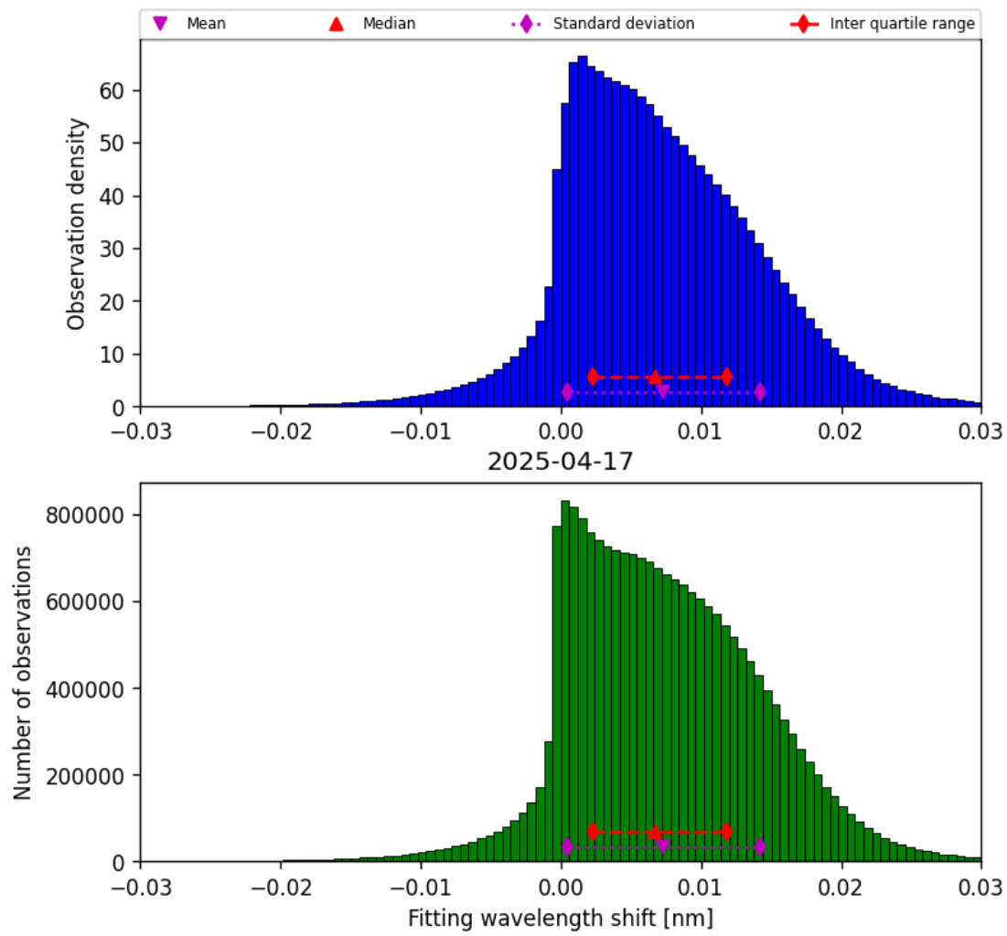
Figure 49: Histogram of “Fitting wavelength shift” for 2025-04-16 to 2025-04-18
