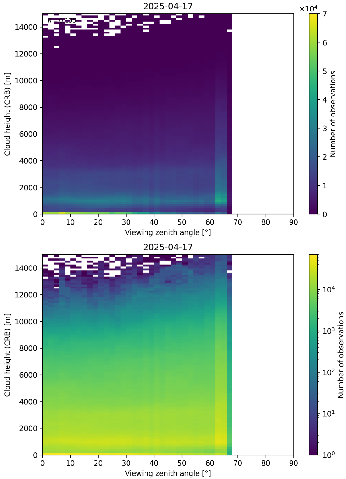
Figure 110: Scatter density plot of “Viewing zenith angle” against “Cloud height (CRB)” for 2025-04-16 to 2025-04-18.
