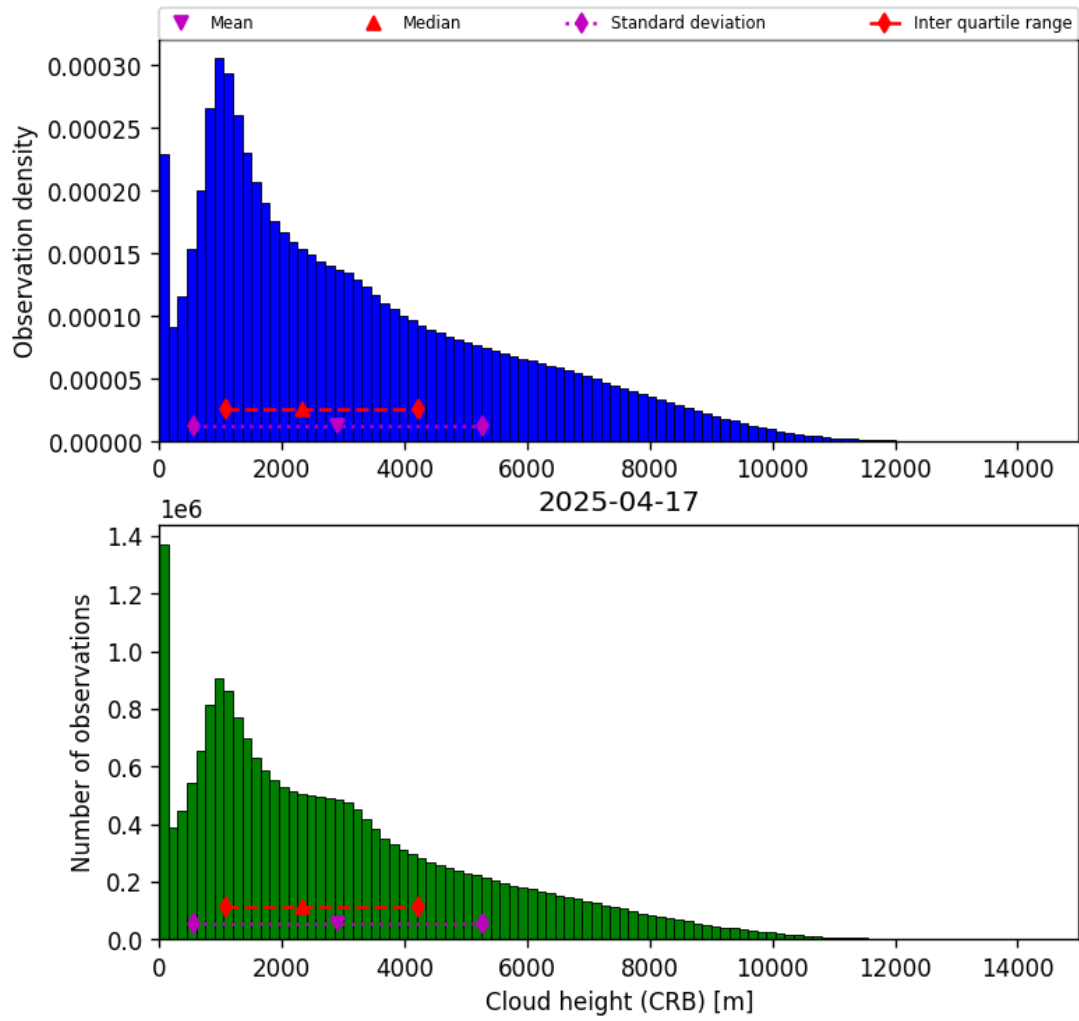
Figure 43: Histogram of “Cloud height (CRB)” for 2025-04-16 to 2025-04-18
