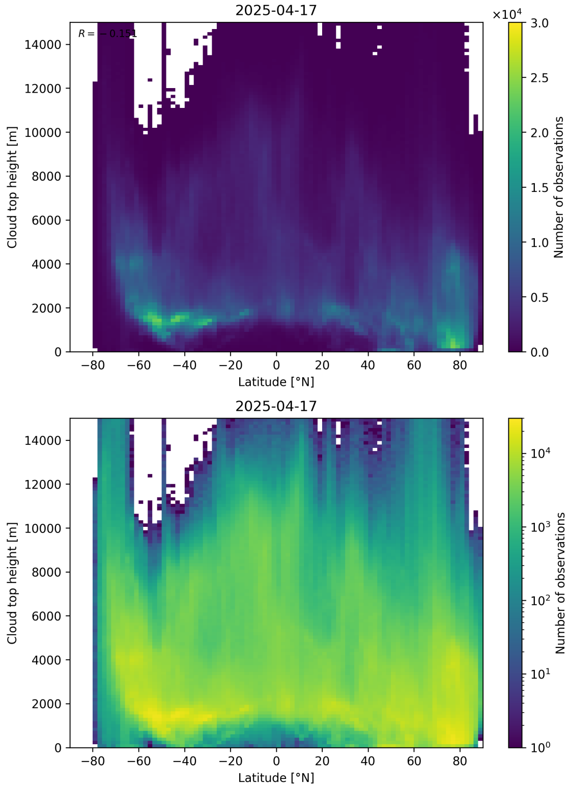
Figure 97: Scatter density plot of “Latitude” against “Cloud top height” for 2025-04-16 to 2025-04-18.
