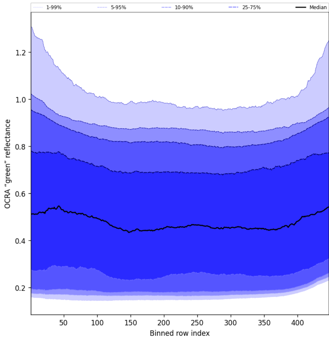
Figure 68: Along track statistics of “OCRA “green” reflectance” for 2025-04-16 to 2025-04-18
