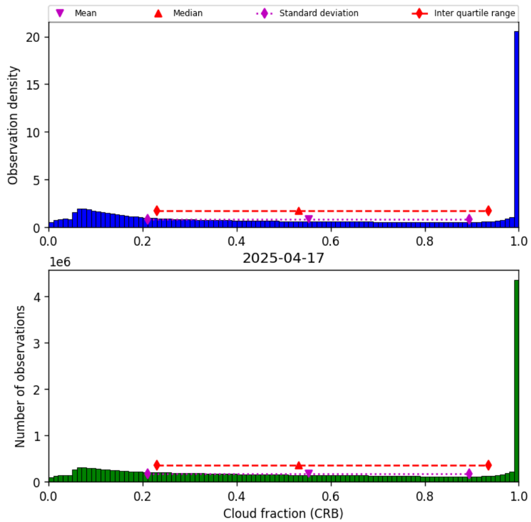
Figure 42: Histogram of “Cloud fraction (CRB)” for 2025-04-16 to 2025-04-18
