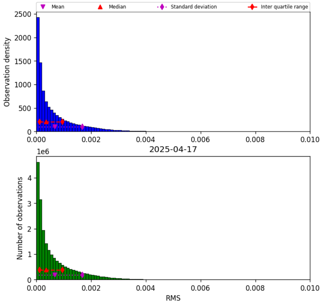
Figure 47: Histogram of “RMS” for 2025-04-16 to 2025-04-18
