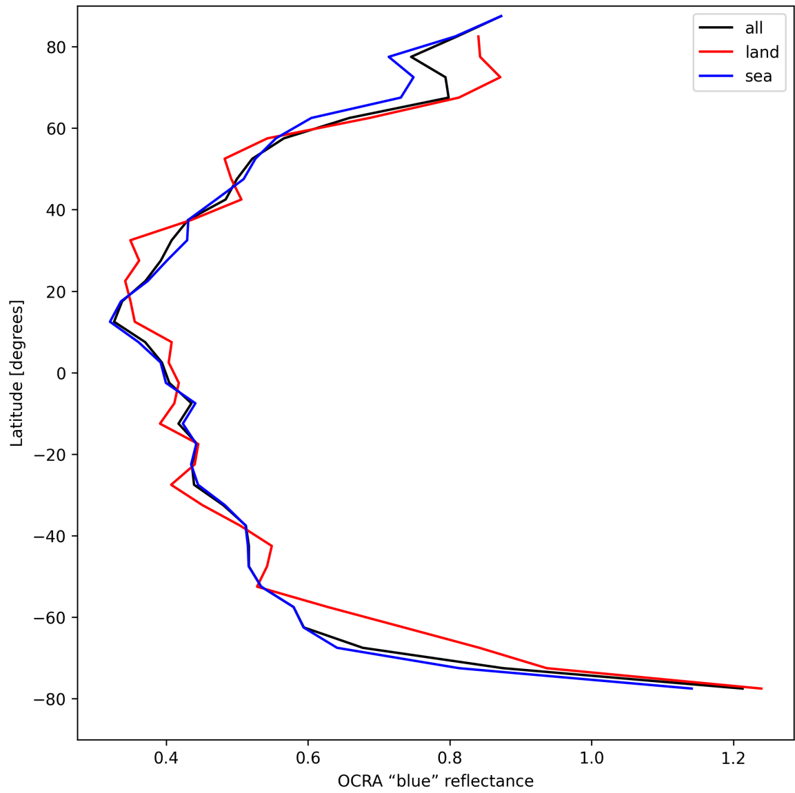
Figure 35: Zonal average of "OCRA "blue" reflectance" for 2025-04-16 to 2025-04-18.
