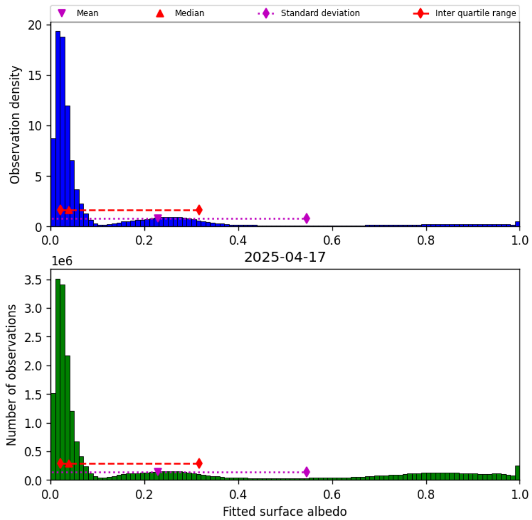
Figure 45: Histogram of “Fitted surface albedo” for 2025-04-16 to 2025-04-18
