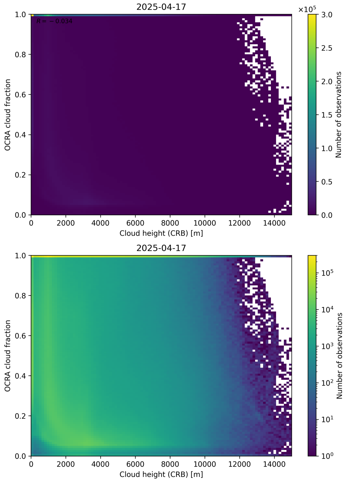
Figure 81: Scatter density plot of “Cloud height (CRB)” against “OCRA cloud fraction” for 2025-04-16 to 2025-04-18.
