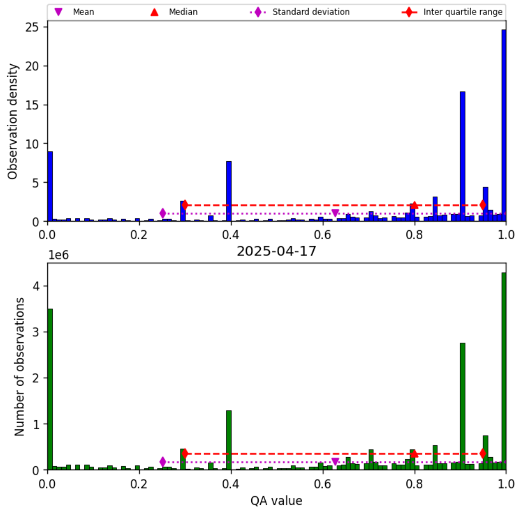
Figure 38: Histogram of “QA value” for 2025-04-16 to 2025-04-18
