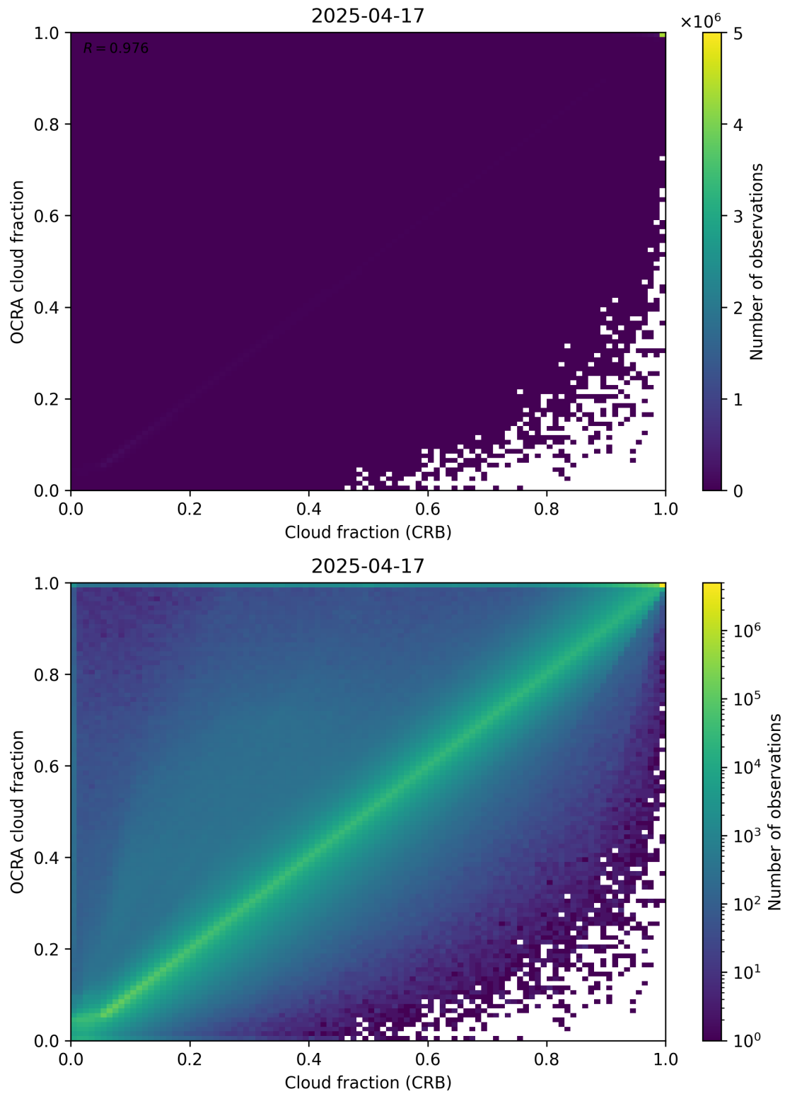
Figure 78: Scatter density plot of “Cloud fraction (CRB)” against “OCRA cloud fraction” for 2025-04-16 to 2025-04-18.
