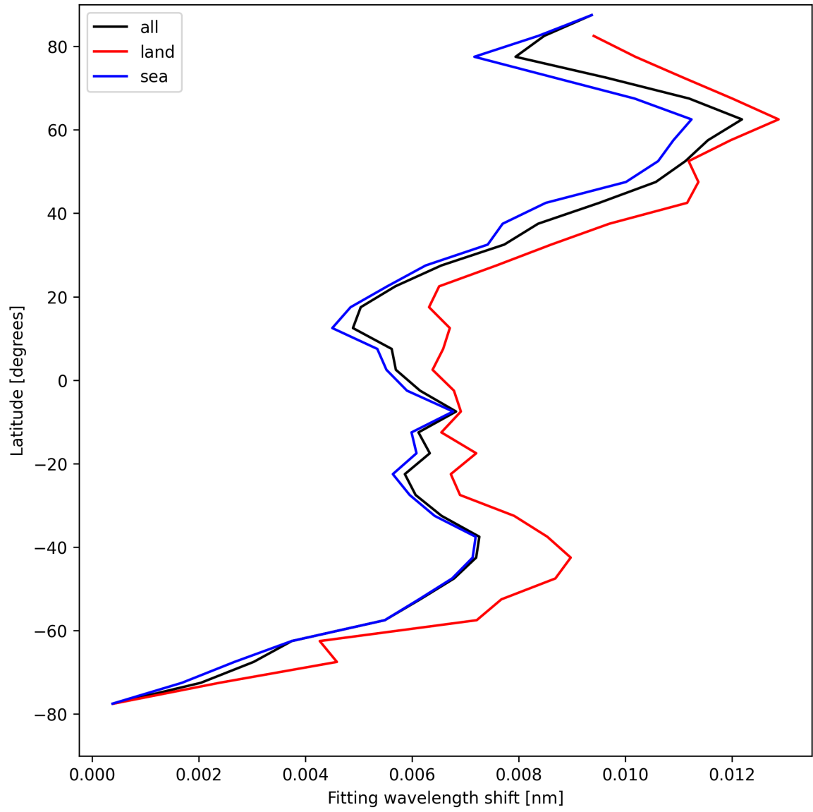
Figure 33: Zonal average of “Fitting wavelength shift” for 2025-04-16 to 2025-04-18.
