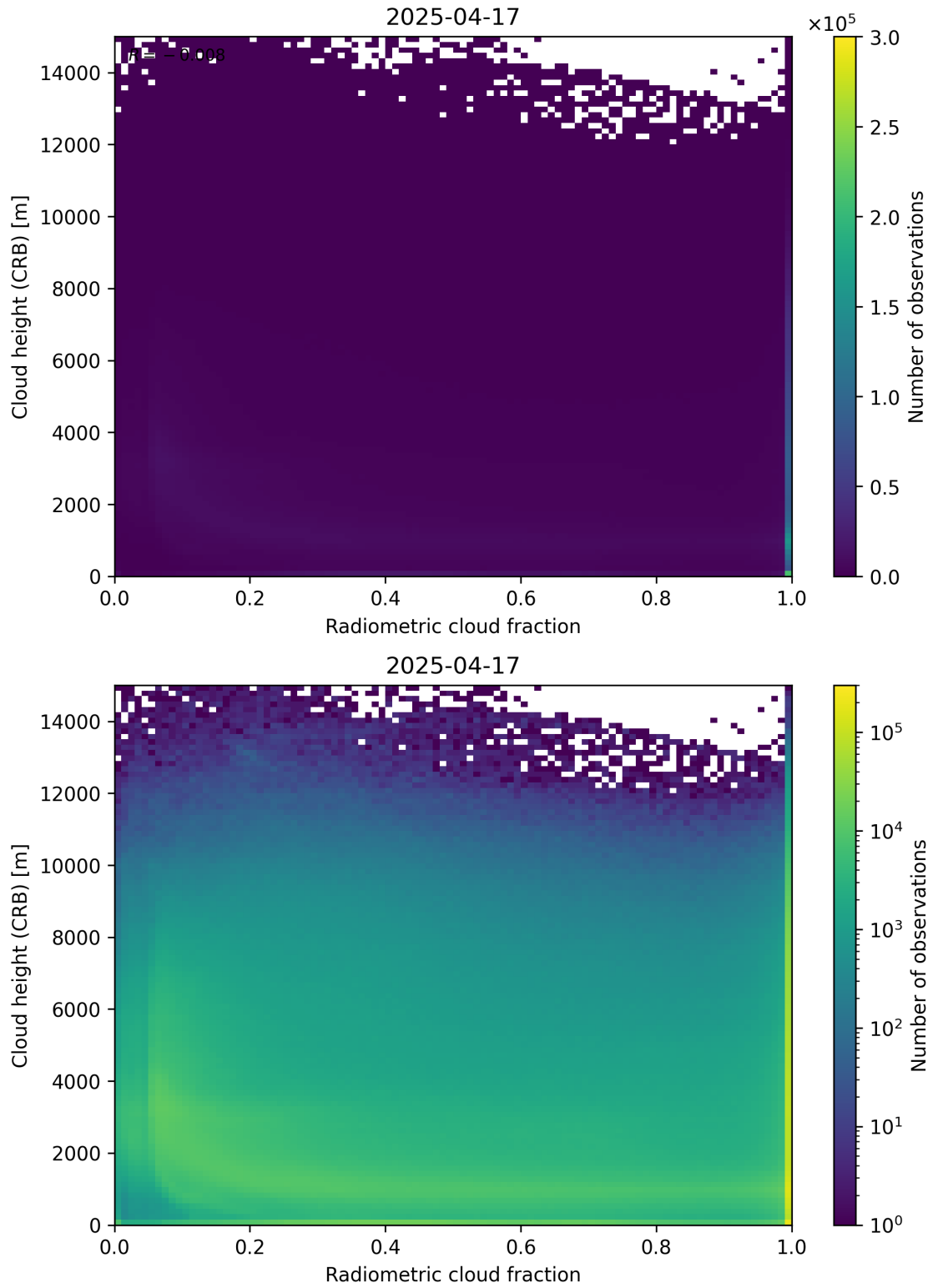
Figure 74: Scatter density plot of “Radiometric cloud fraction” against “Cloud height (CRB)” for 2025-04-16 to 2025-04-18.
