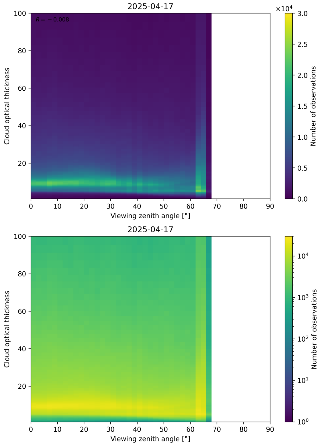
Figure 111: Scatter density plot of “Viewing zenith angle” against “Cloud optical thickness” for 2025-04-16 to 2025-04-18.
