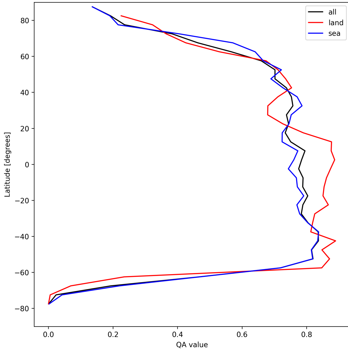
Figure 22: Zonal average of “QA value” for 2025-04-16 to 2025-04-18.
