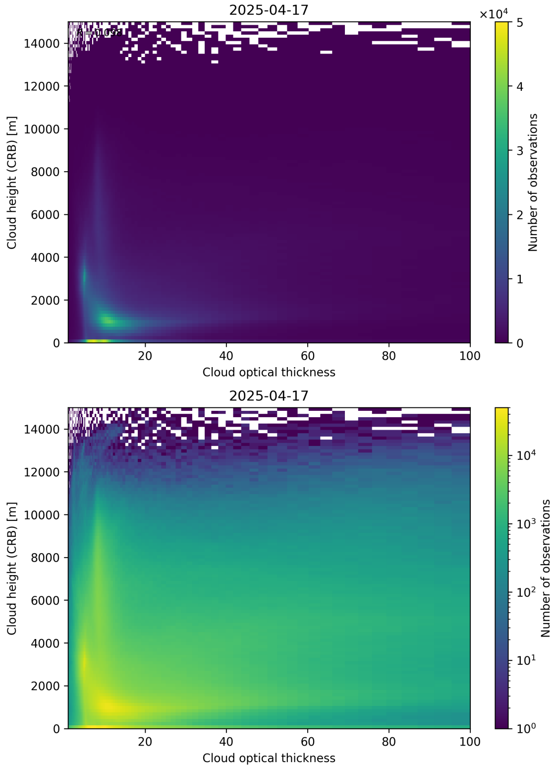
Figure 85: Scatter density plot of “Cloud optical thickness” against “Cloud height (CRB)” for 2025-04-16 to 2025-04-18.
