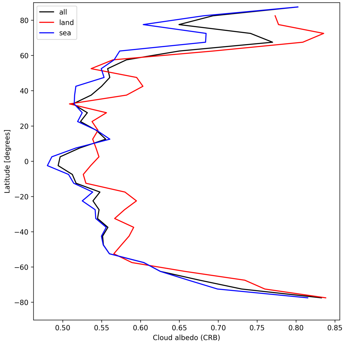
Figure 28: Zonal average of “Cloud albedo (CRB)” for 2025-04-16 to 2025-04-18.
