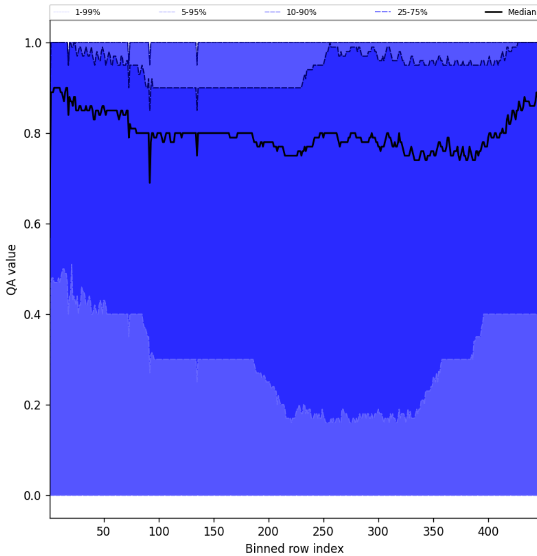
Figure 54: Along track statistics of “QA value” for 2025-04-16 to 2025-04-18
