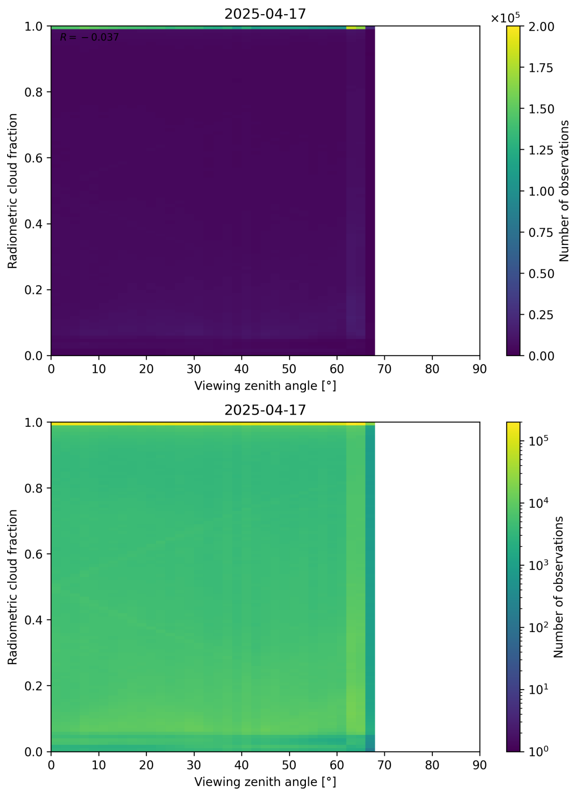
Figure 107: Scatter density plot of “Viewing zenith angle” against “Radiometric cloud fraction” for 2025-04-16 to 2025-04-18.
