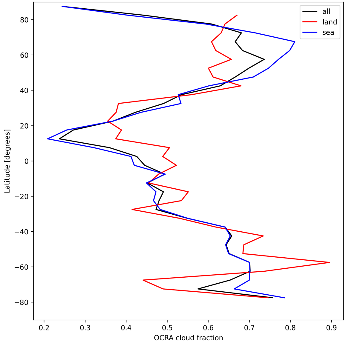
Figure 34: Zonal average of “OCRA cloud fraction” for 2025-04-16 to 2025-04-18.
