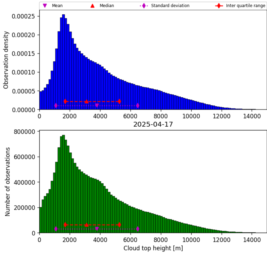
Figure 40: Histogram of “Cloud top height” for 2025-04-16 to 2025-04-18
