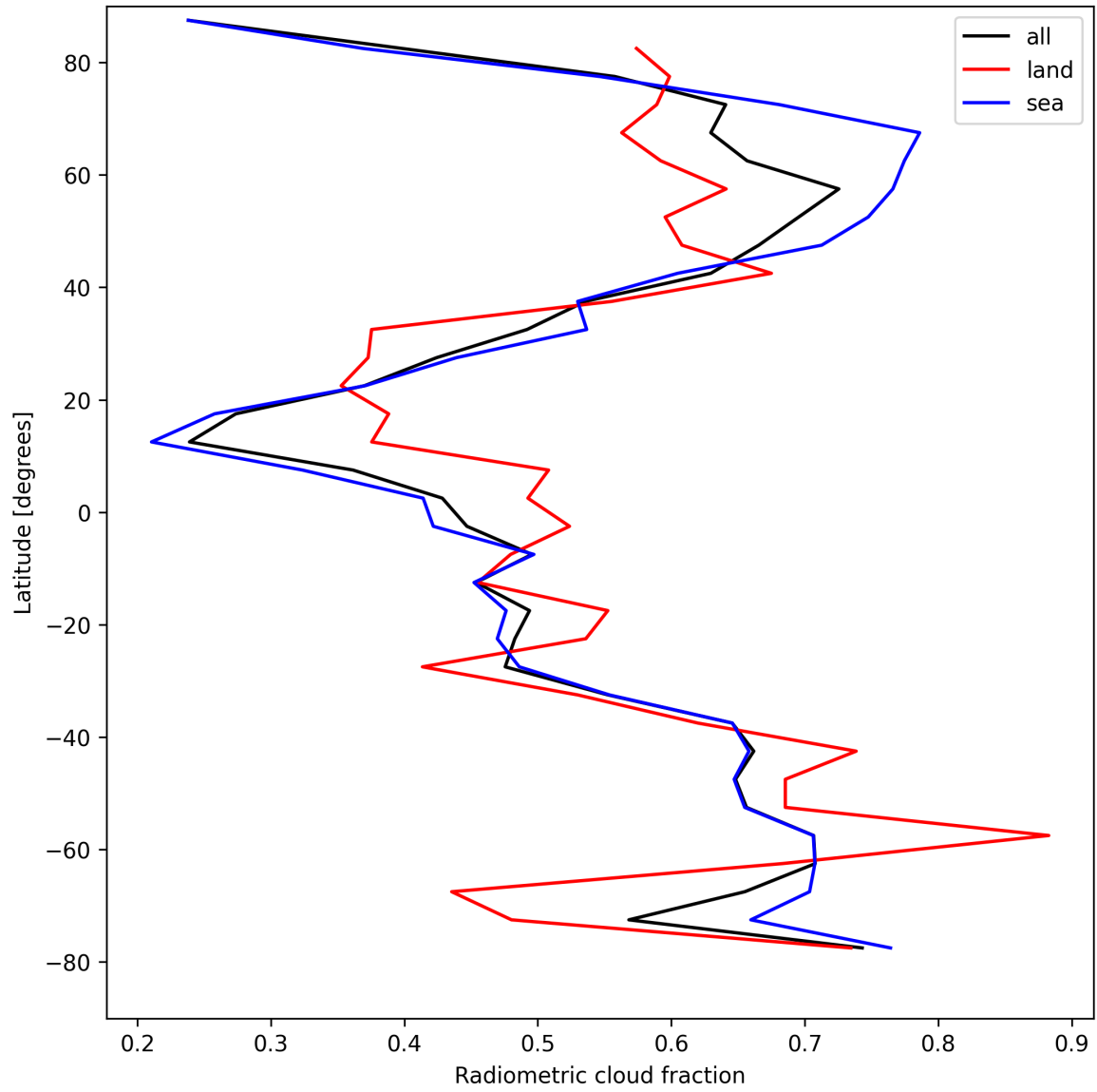
Figure 23: Zonal average of “Radiometric cloud fraction” for 2025-04-16 to 2025-04-18.
