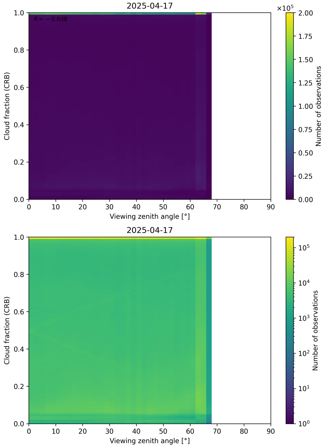
Figure 109: Scatter density plot of “Viewing zenith angle” against “Cloud fraction (CRB)” for 2025-04-16 to 2025-04-18.
