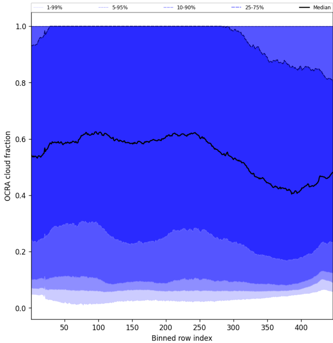
Figure 66: Along track statistics of “OCRA cloud fraction” for 2025-04-16 to 2025-04-18
