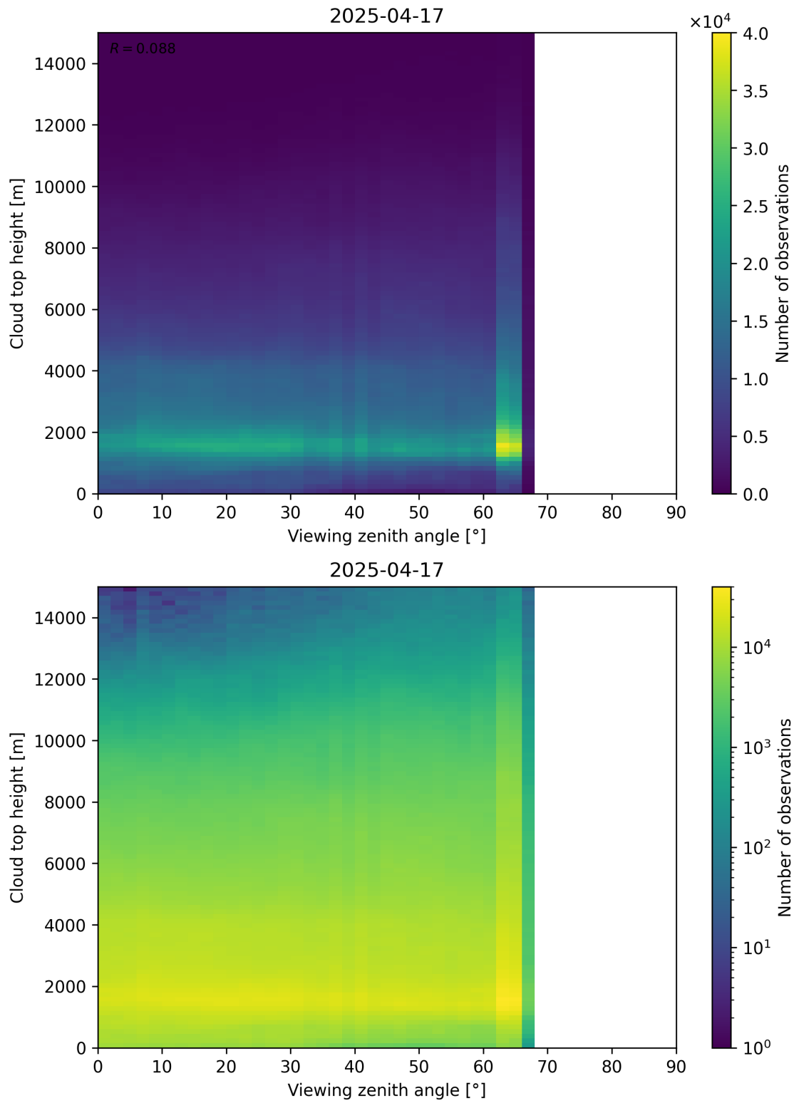
Figure 112: Scatter density plot of “Viewing zenith angle” against “Cloud top height” for 2025-04-16 to 2025-04-18.
