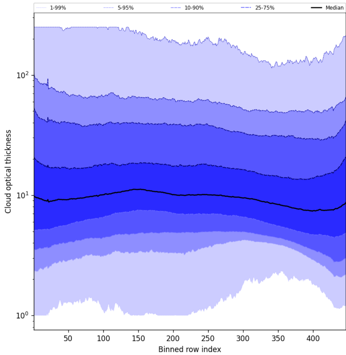
Figure 57: Along track statistics of “Cloud optical thickness” for 2025-04-16 to 2025-04-18
