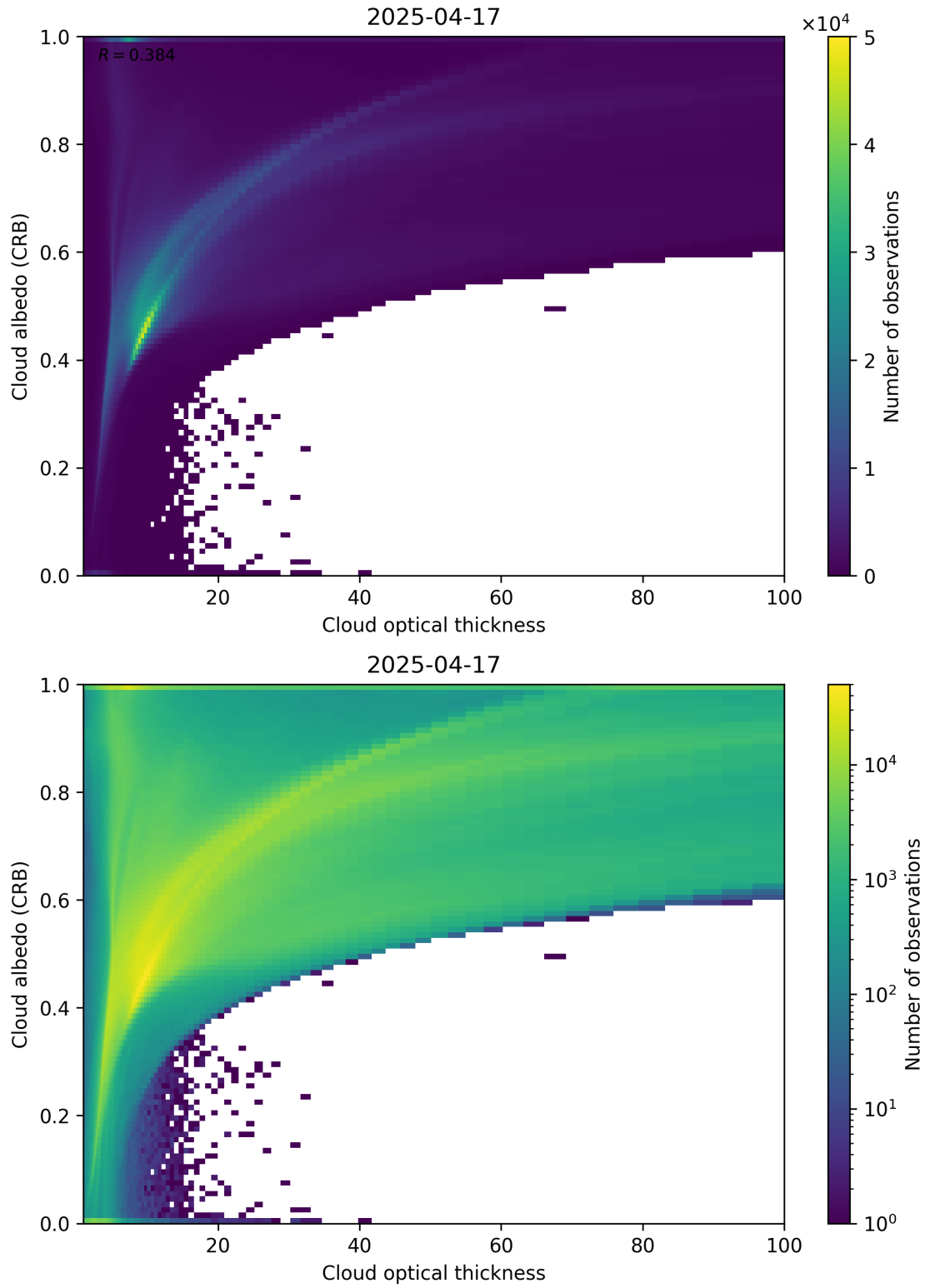
Figure 82: Scatter density plot of “Cloud optical thickness” against “Cloud albedo (CRB)” for 2025-04-16 to 2025-04-18.
