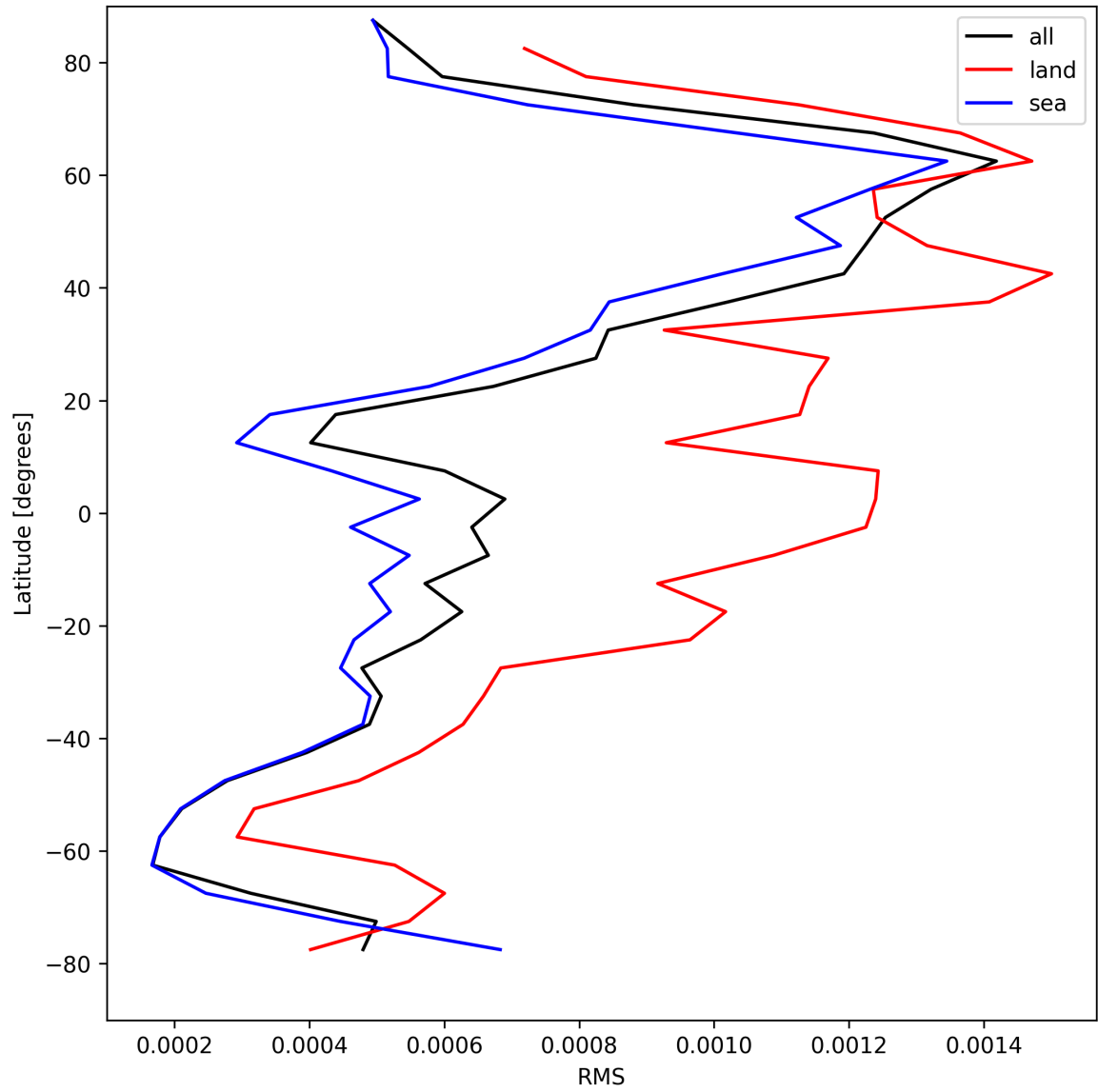
Figure 31: Zonal average of “RMS” for 2025-04-16 to 2025-04-18.
