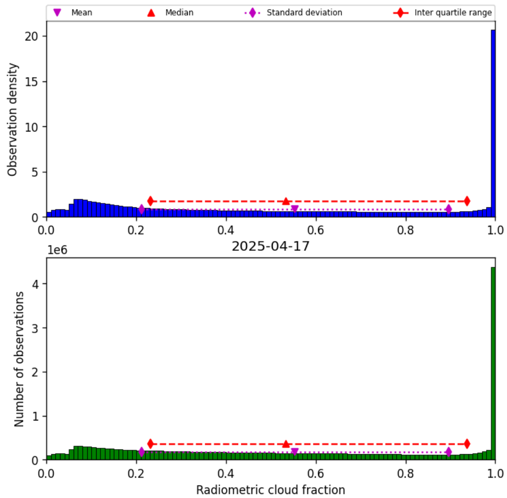
Figure 39: Histogram of “Radiometric cloud fraction” for 2025-04-16 to 2025-04-18
