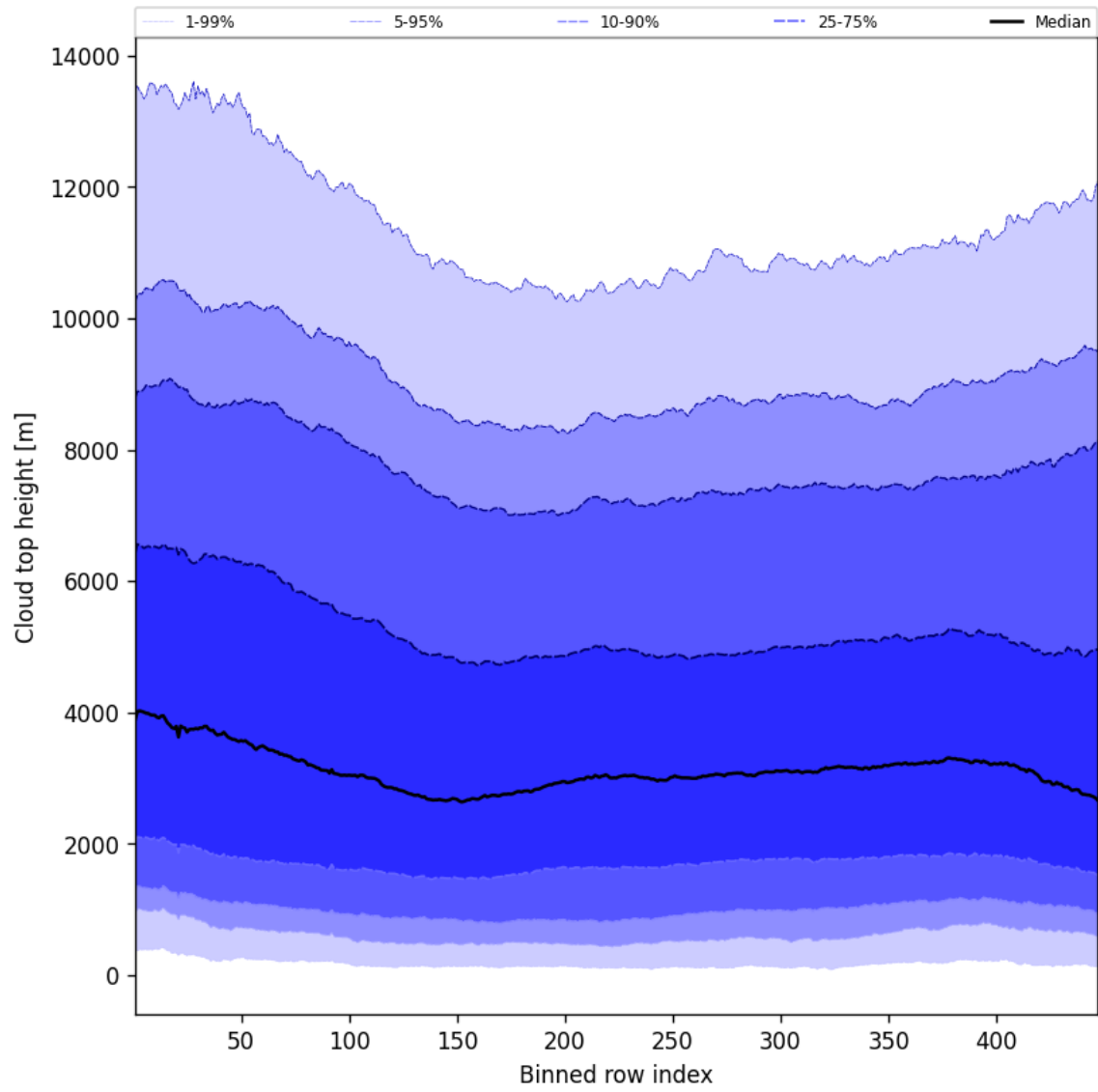
Figure 56: Along track statistics of “Cloud top height” for 2025-04-16 to 2025-04-18
