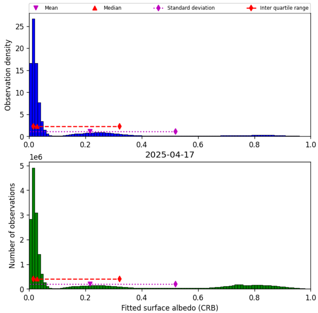
Figure 46: Histogram of “Fitted surface albedo (CRB)” for 2025-04-16 to 2025-04-18
