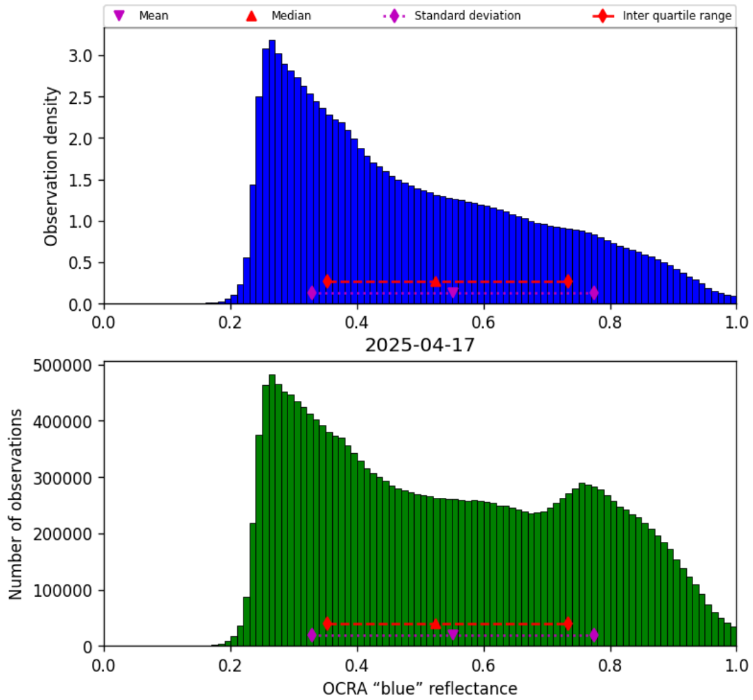
Figure 51: Histogram of “OCRA “blue” reflectance” for 2025-04-16 to 2025-04-18
