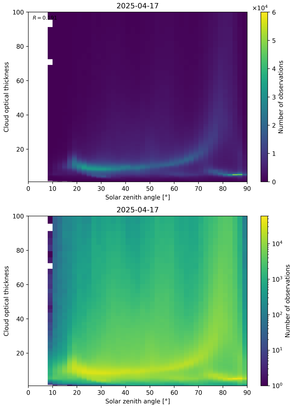
Figure 103: Scatter density plot of “Solar zenith angle” against “Cloud optical thickness” for 2025-04-16 to 2025-04-18.
