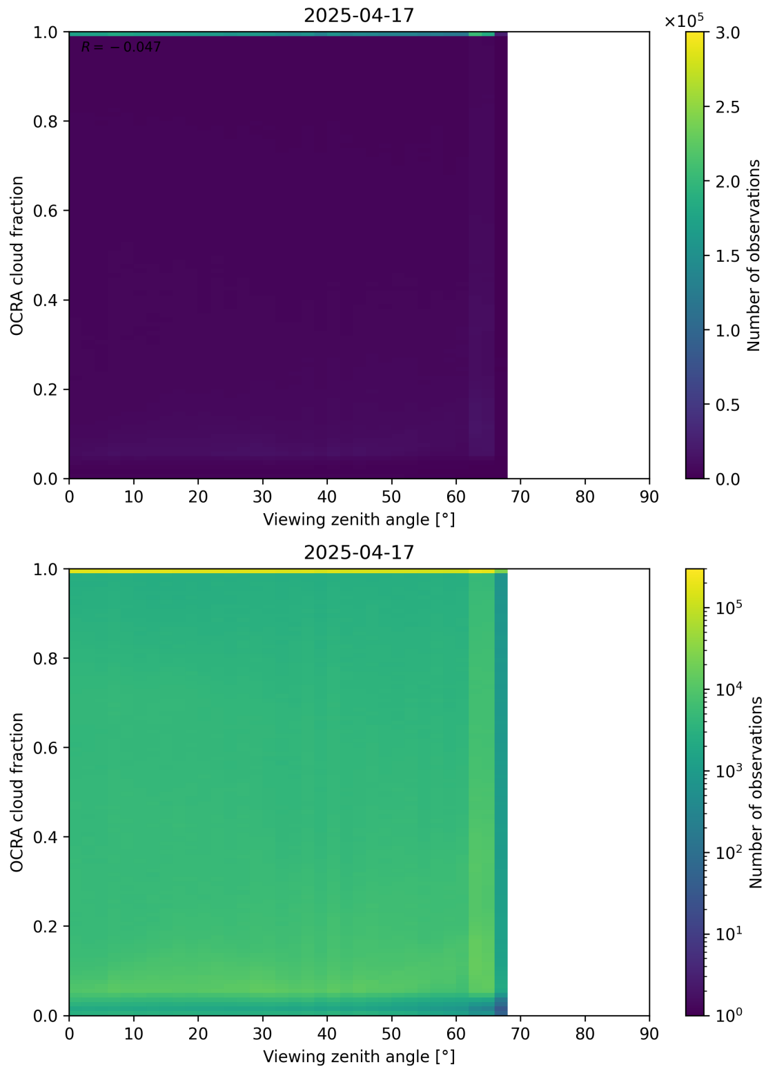
Figure 108: Scatter density plot of “Viewing zenith angle” against “OCRA cloud fraction” for 2025-04-16 to 2025-04-18.
