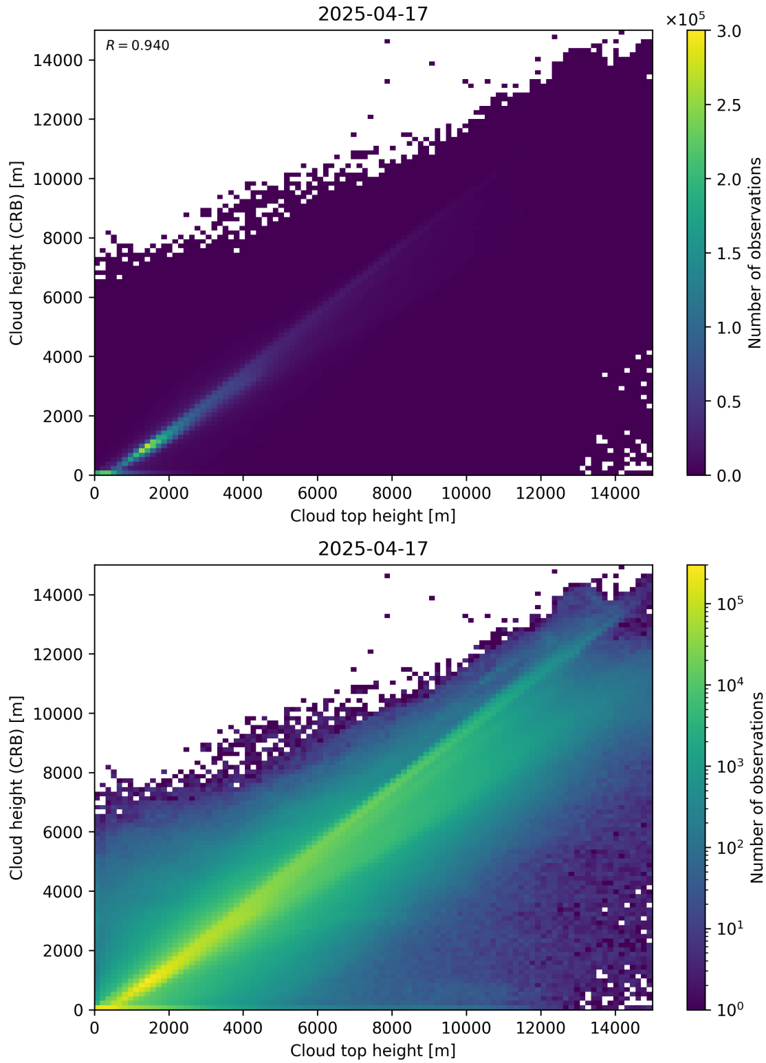
Figure 89: Scatter density plot of “Cloud top height” against “Cloud height (CRB)” for 2025-04-16 to 2025-04-18.
