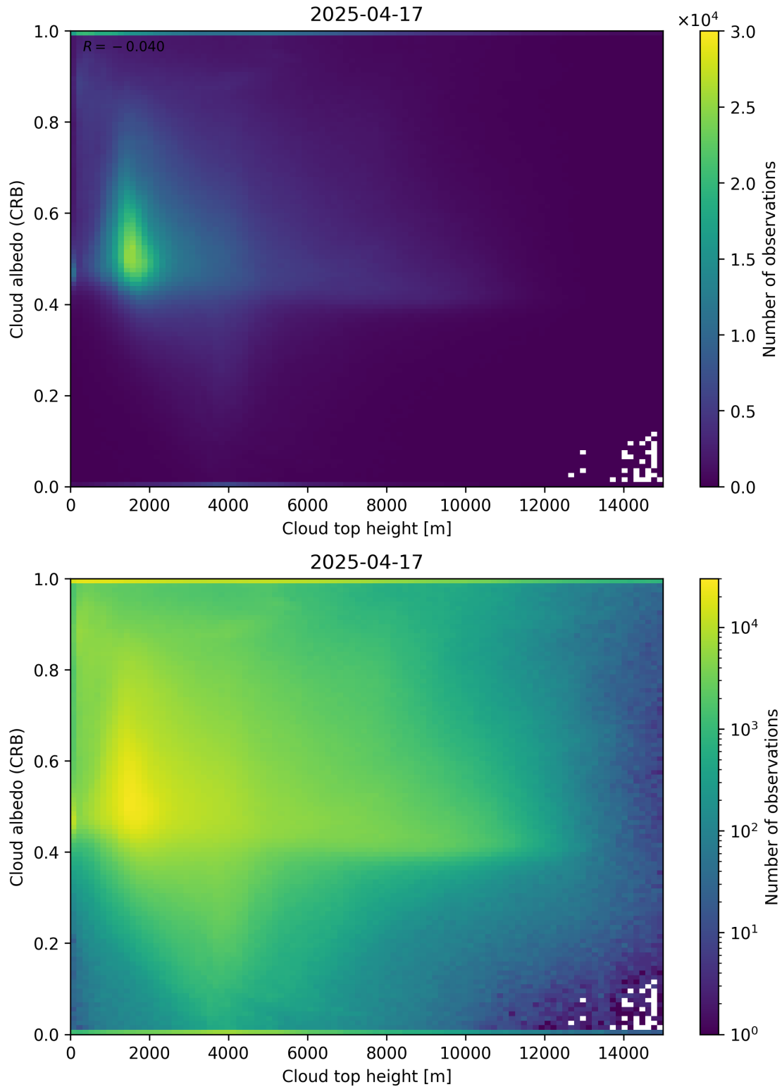
Figure 86: Scatter density plot of “Cloud top height” against “Cloud albedo (CRB)” for 2025-04-16 to 2025-04-18.
