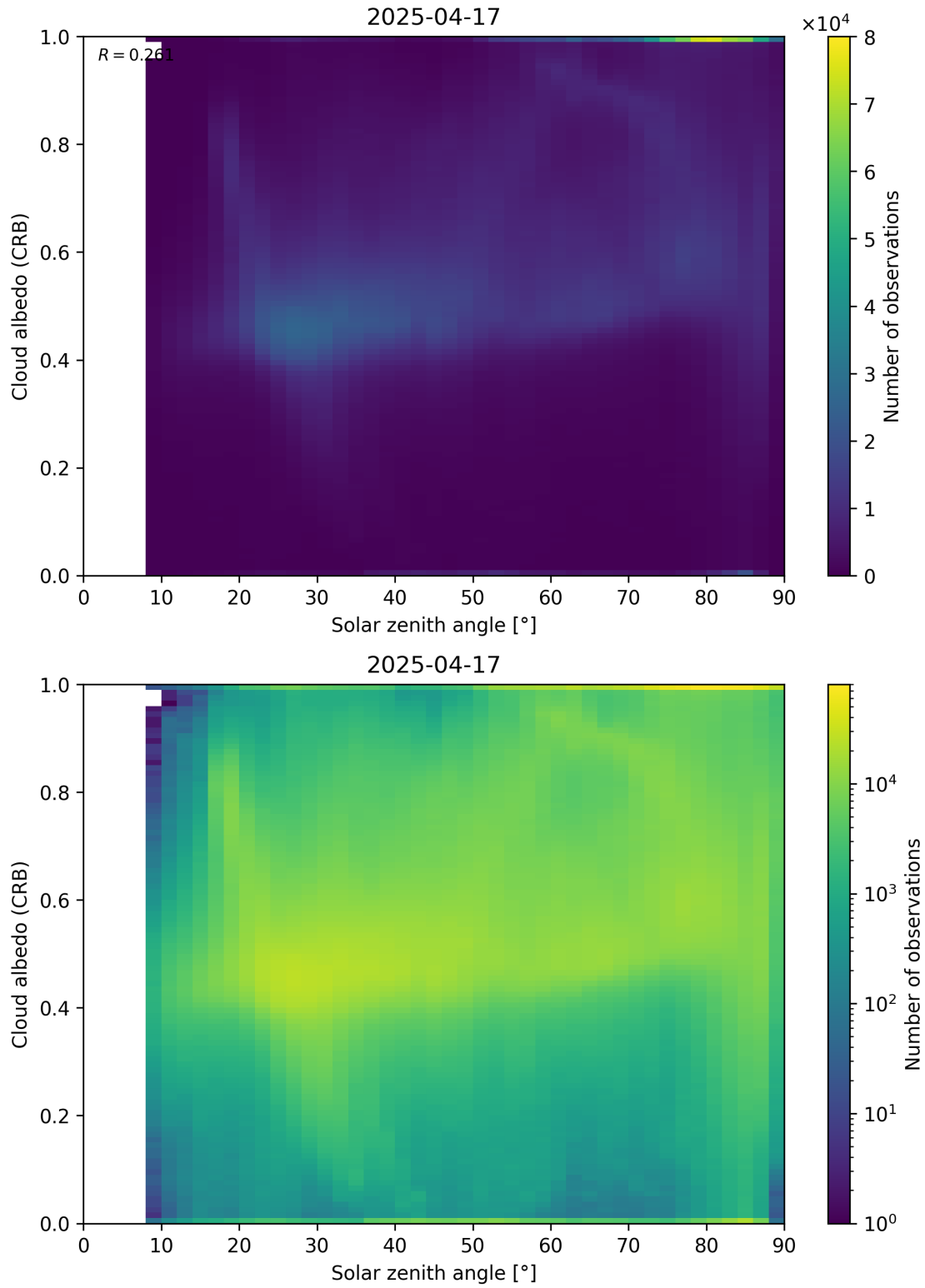
Figure 98: Scatter density plot of “Solar zenith angle” against “Cloud albedo (CRB)” for 2025-04-16 to 2025-04-18.
