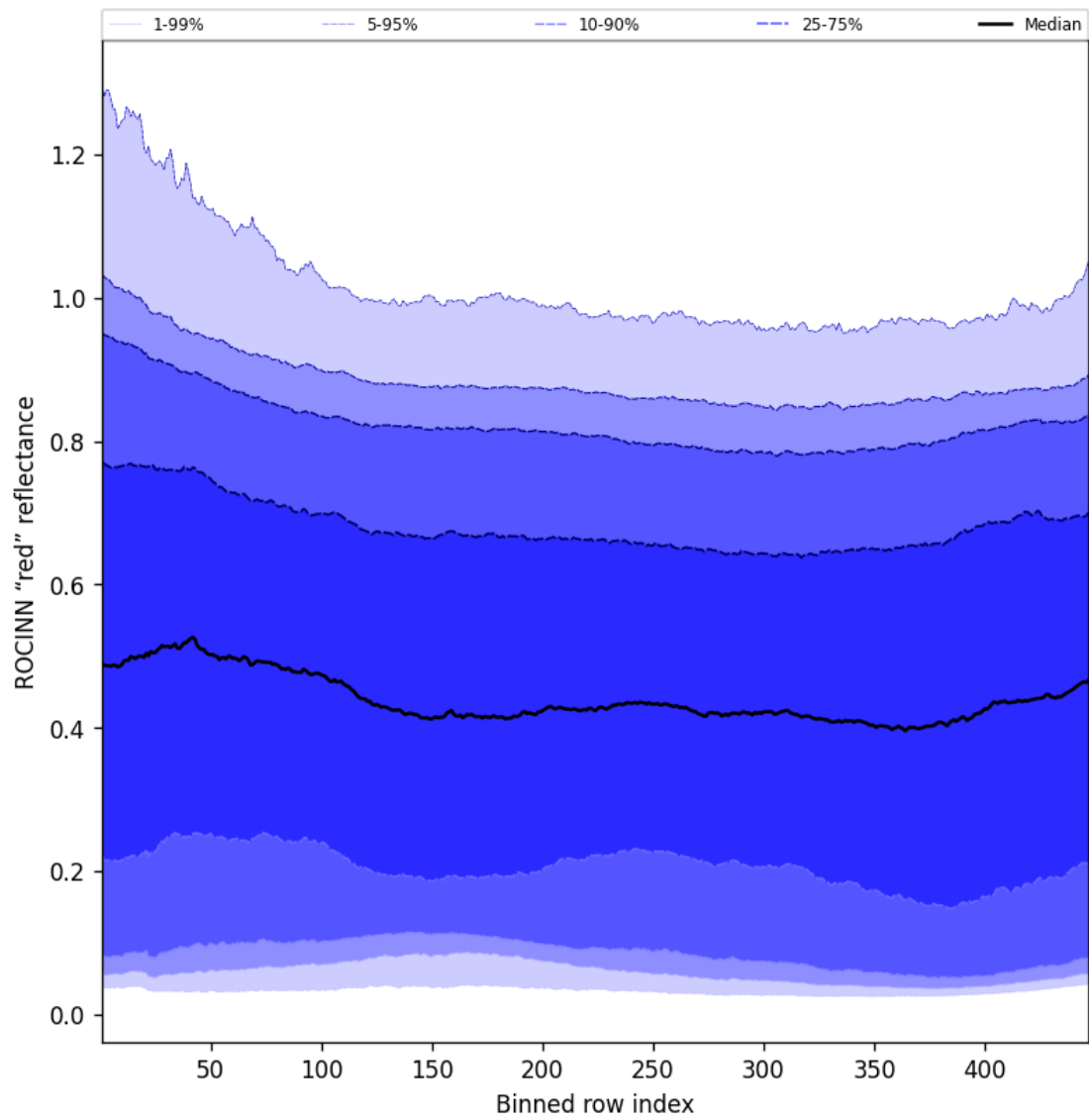
Figure 69: Along track statistics of “ROCINN “red” reflectance” for 2025-04-16 to 2025-04-18
