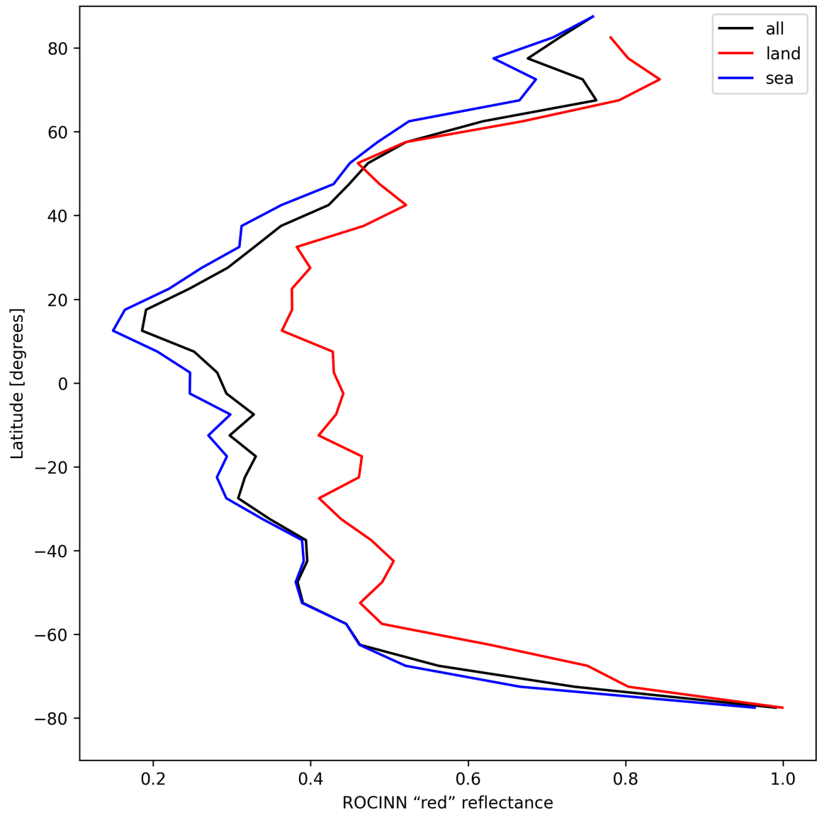
Figure 37: Zonal average of “ROCINN “red” reflectance” for 2025-04-16 to 2025-04-18.
