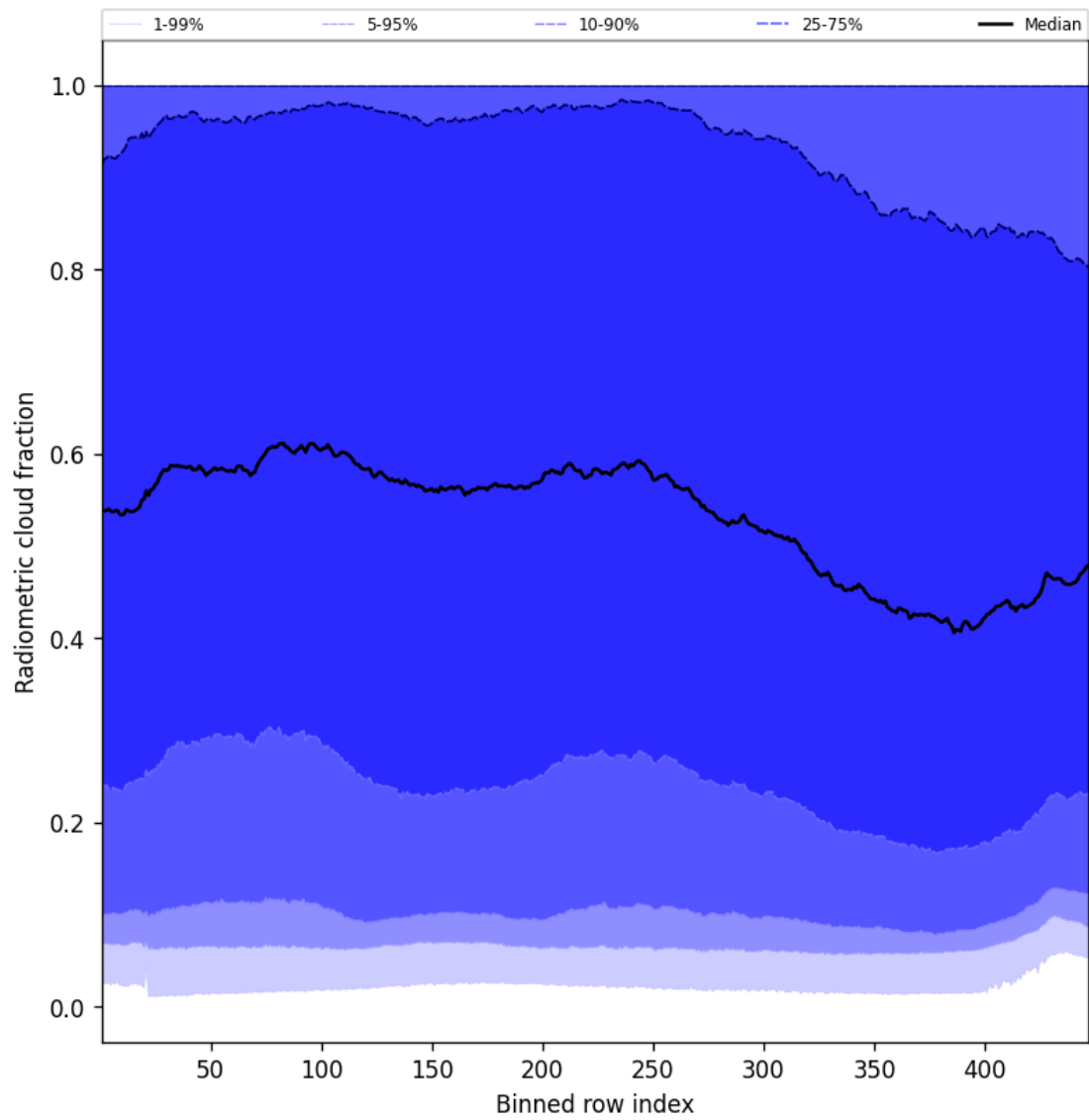
Figure 55: Along track statistics of “Radiometric cloud fraction” for 2025-04-16 to 2025-04-18
