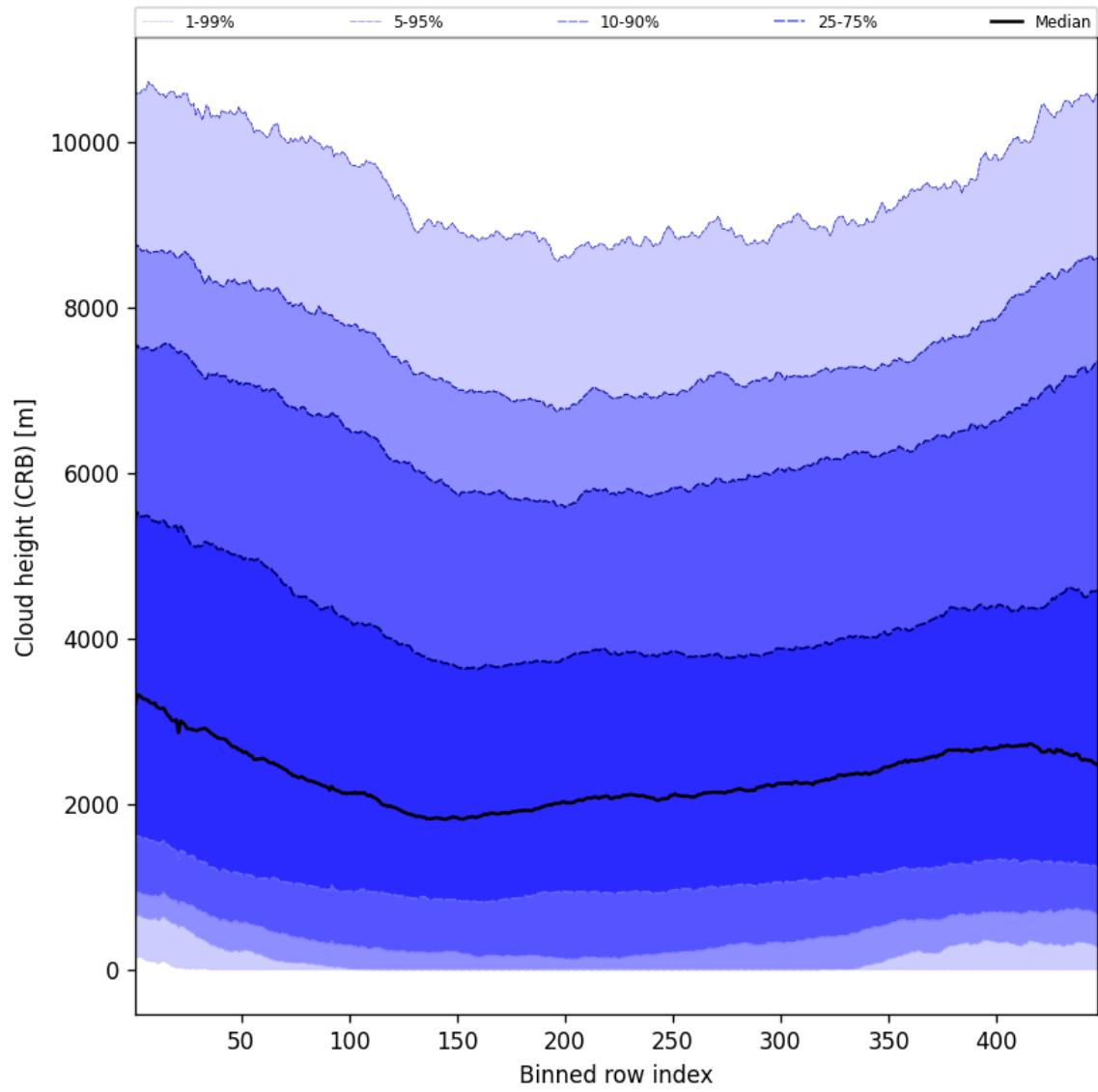
Figure 59: Along track statistics of “Cloud height (CRB)” for 2025-04-16 to 2025-04-18
