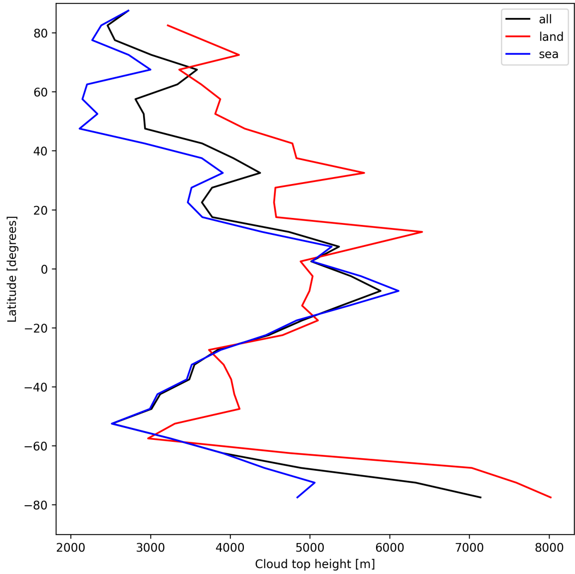
Figure 24: Zonal average of “Cloud top height” for 2025-04-16 to 2025-04-18.
