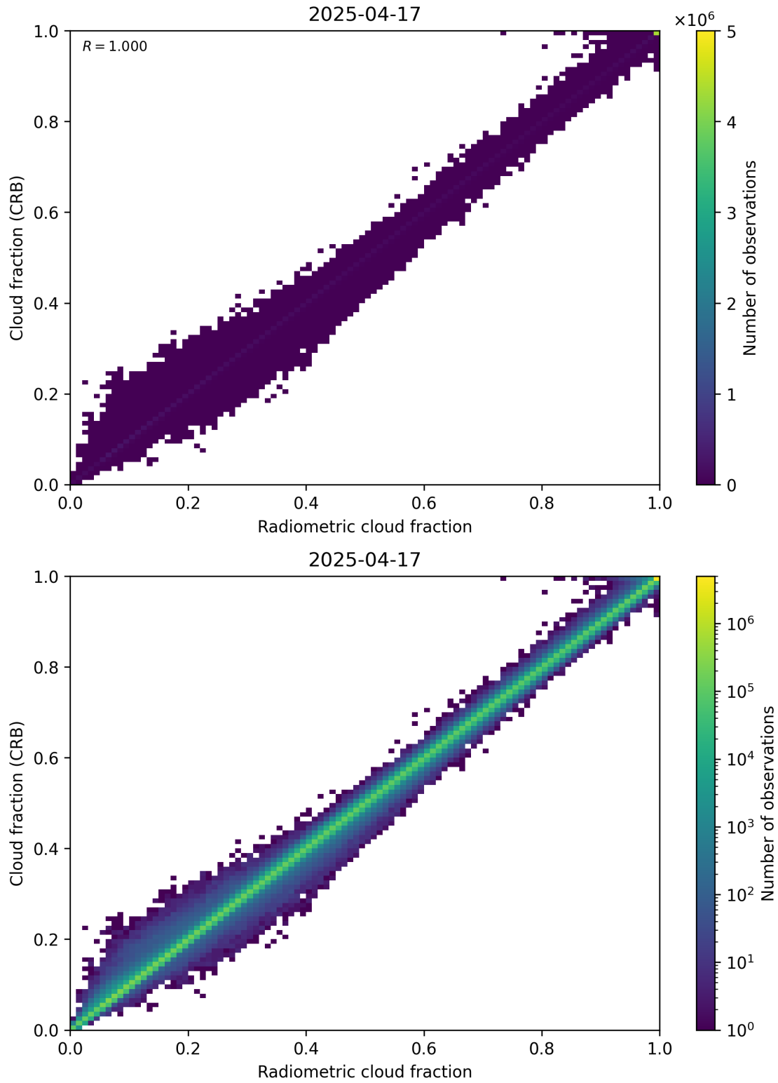
Figure 73: Scatter density plot of “Radiometric cloud fraction” against “Cloud fraction (CRB)” for 2025-04-16 to 2025-04-18.
