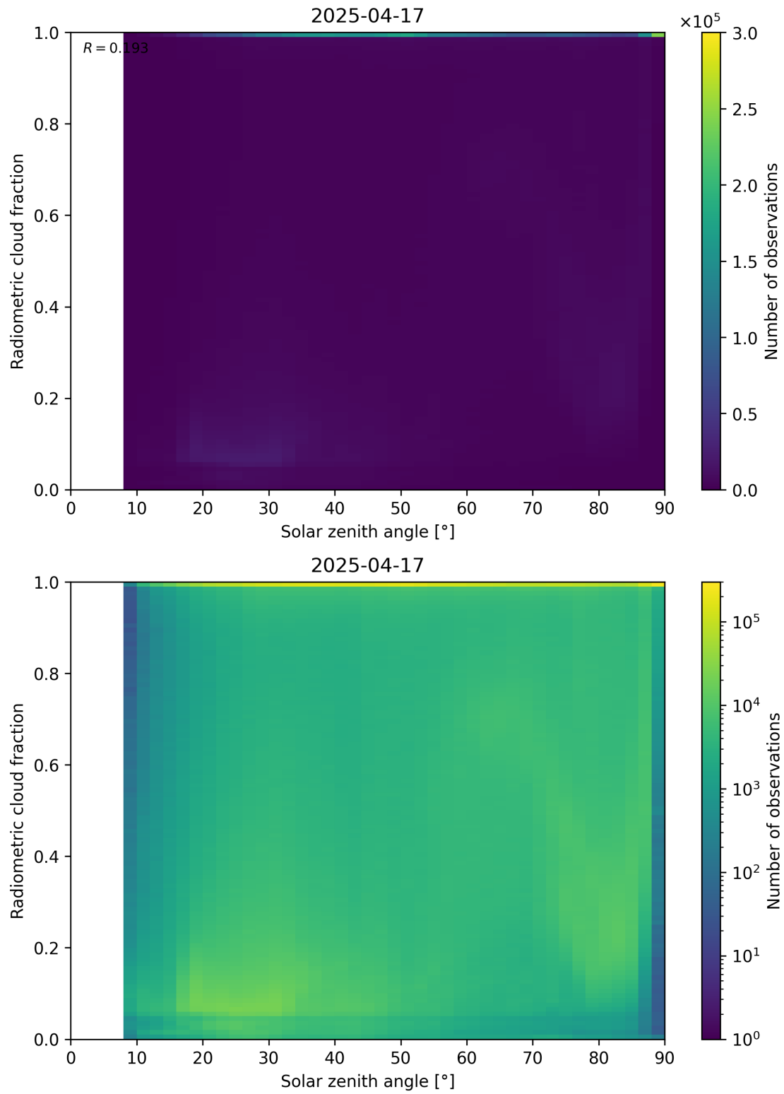
Figure 99: Scatter density plot of “Solar zenith angle” against “Radiometric cloud fraction” for 2025-04-16 to 2025-04-18.
