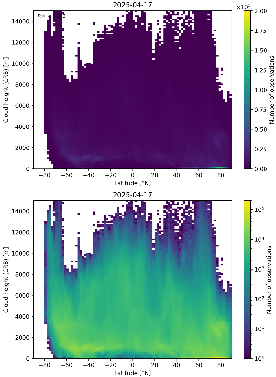
Figure 95: Scatter density plot of “Latitude” against “Cloud height (CRB)” for 2025-04-16 to 2025-04-18.
