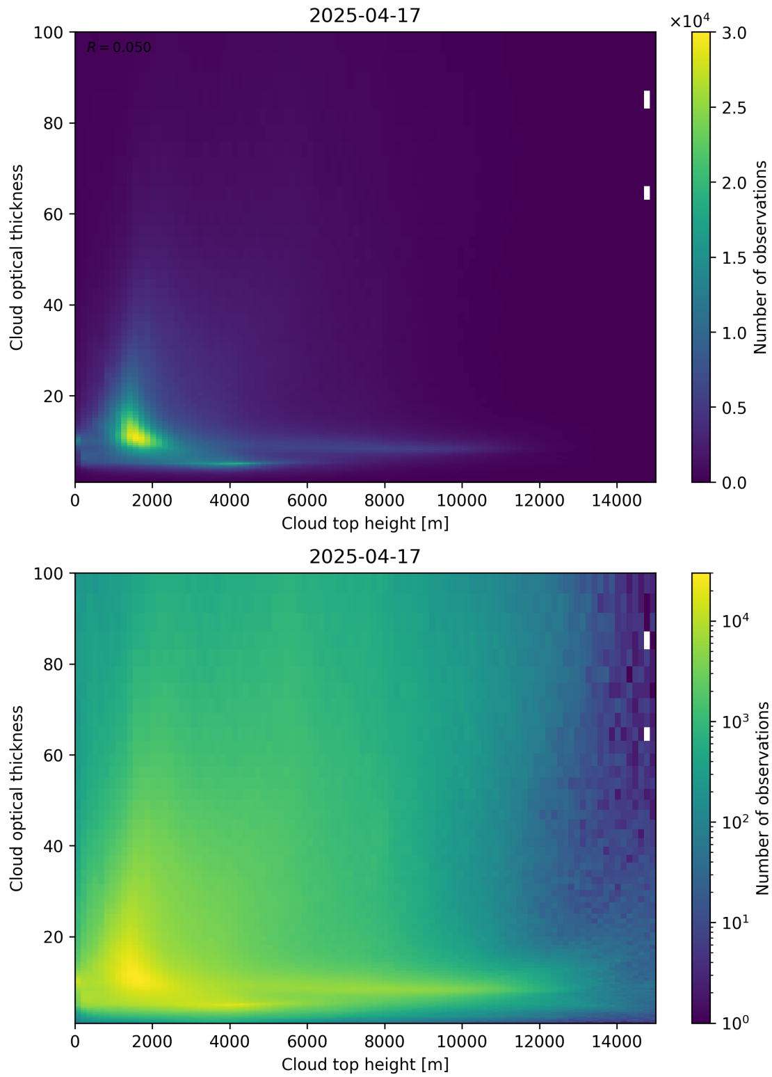
Figure 90: Scatter density plot of “Cloud top height” against “Cloud optical thickness” for 2025-04-16 to 2025-04-18.
