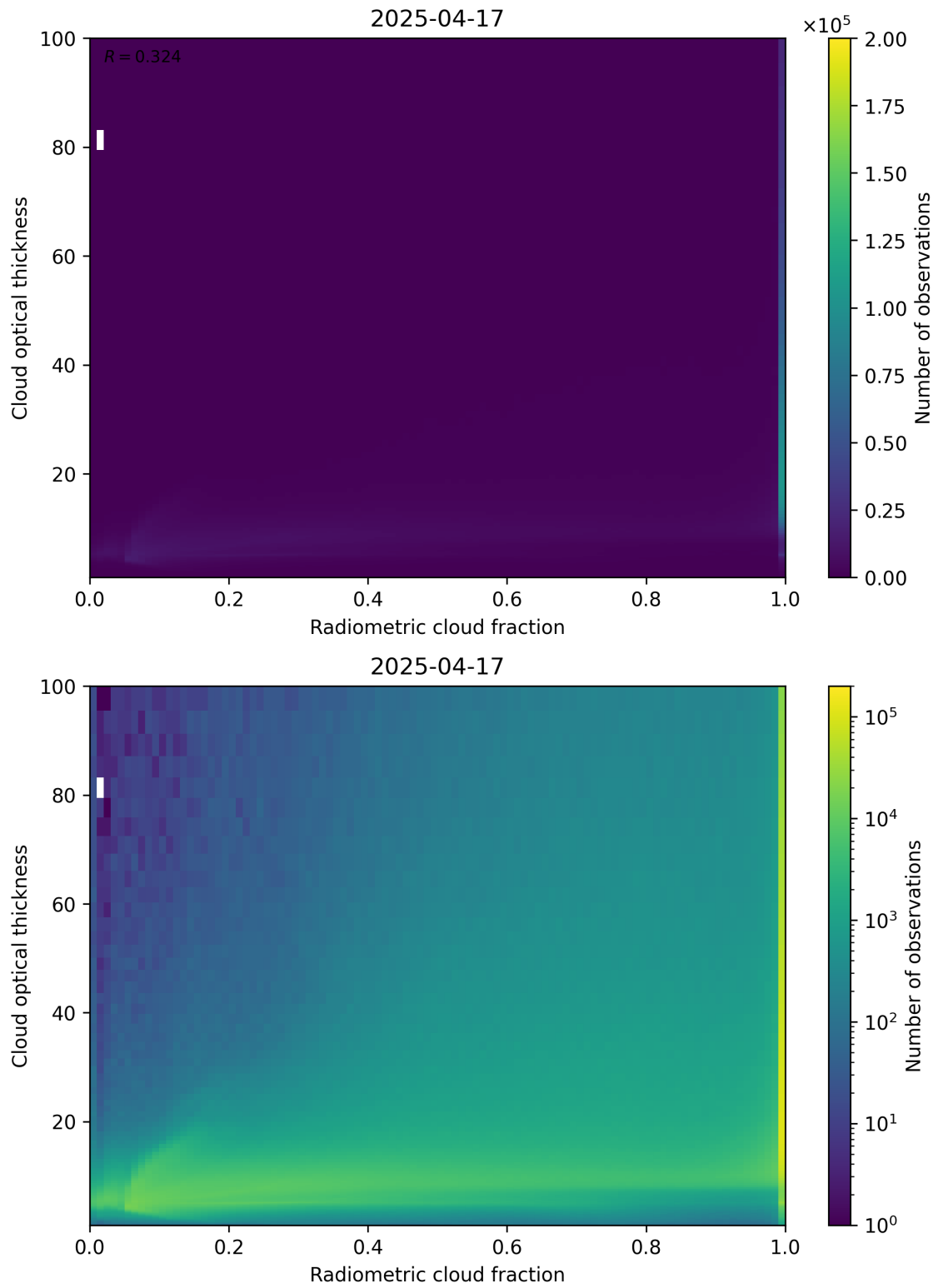
Figure 75: Scatter density plot of “Radiometric cloud fraction” against “Cloud optical thickness” for 2025-04-16 to 2025-04-18.
