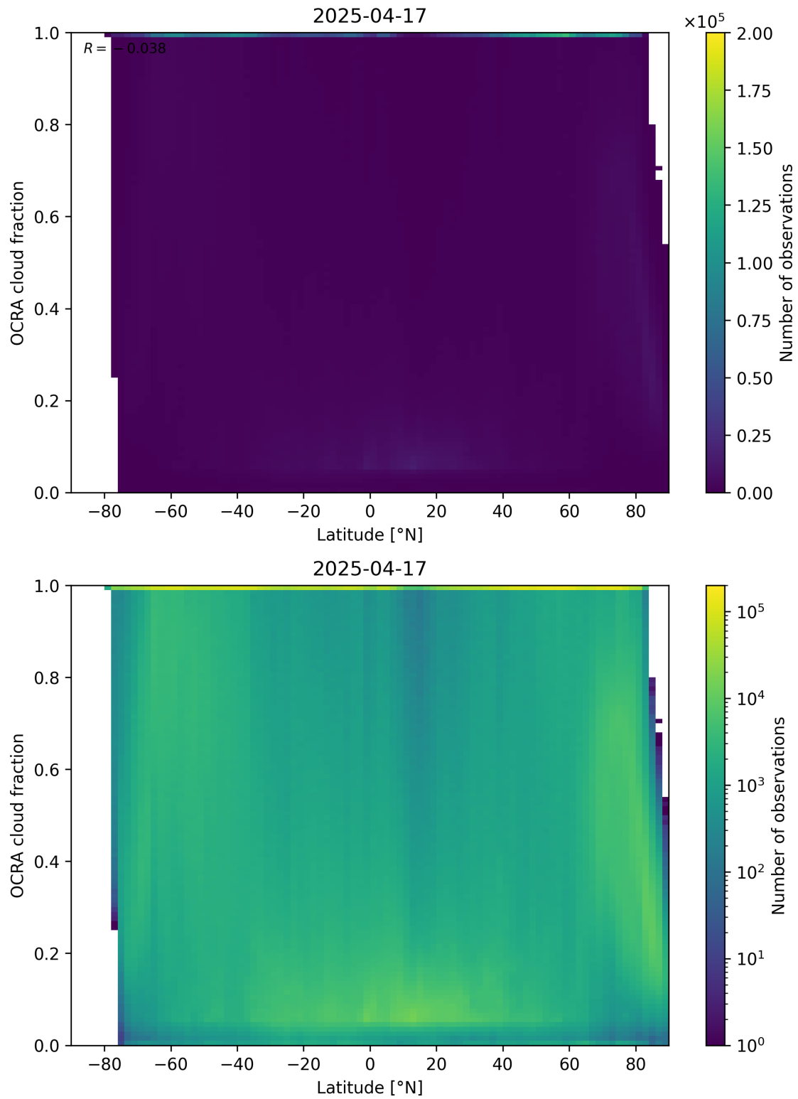
Figure 93: Scatter density plot of “Latitude” against “OCRA cloud fraction” for 2025-04-16 to 2025-04-18.
