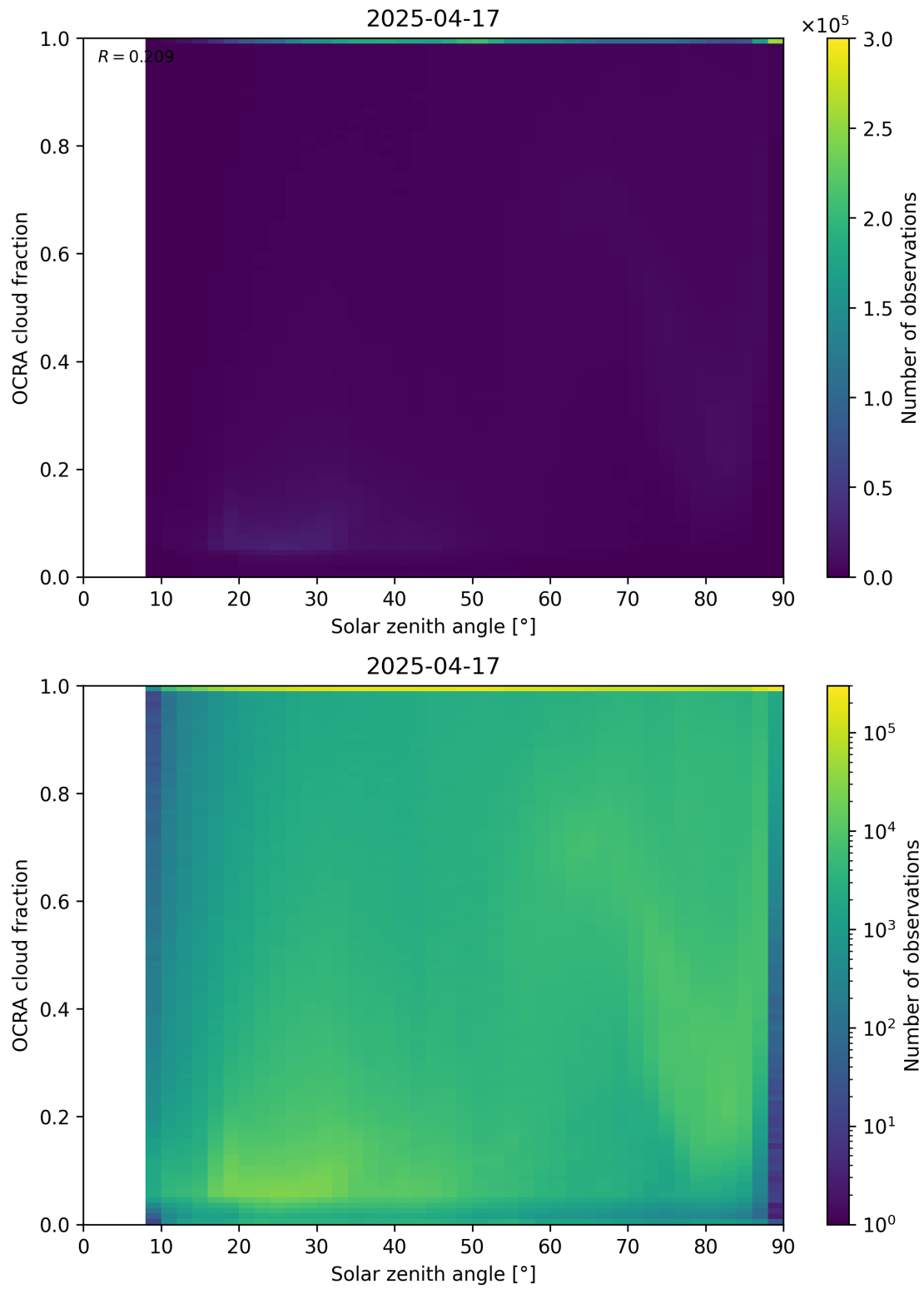
Figure 100: Scatter density plot of “Solar zenith angle” against “OCRA cloud fraction” for 2025-04-16 to 2025-04-18.
