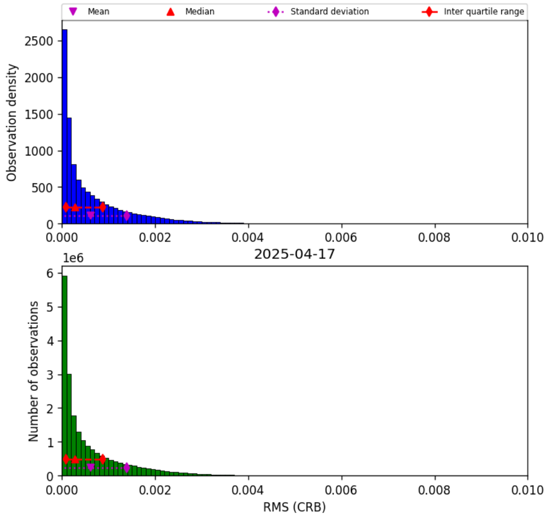
Figure 48: Histogram of “RMS (CRB)” for 2025-04-16 to 2025-04-18
