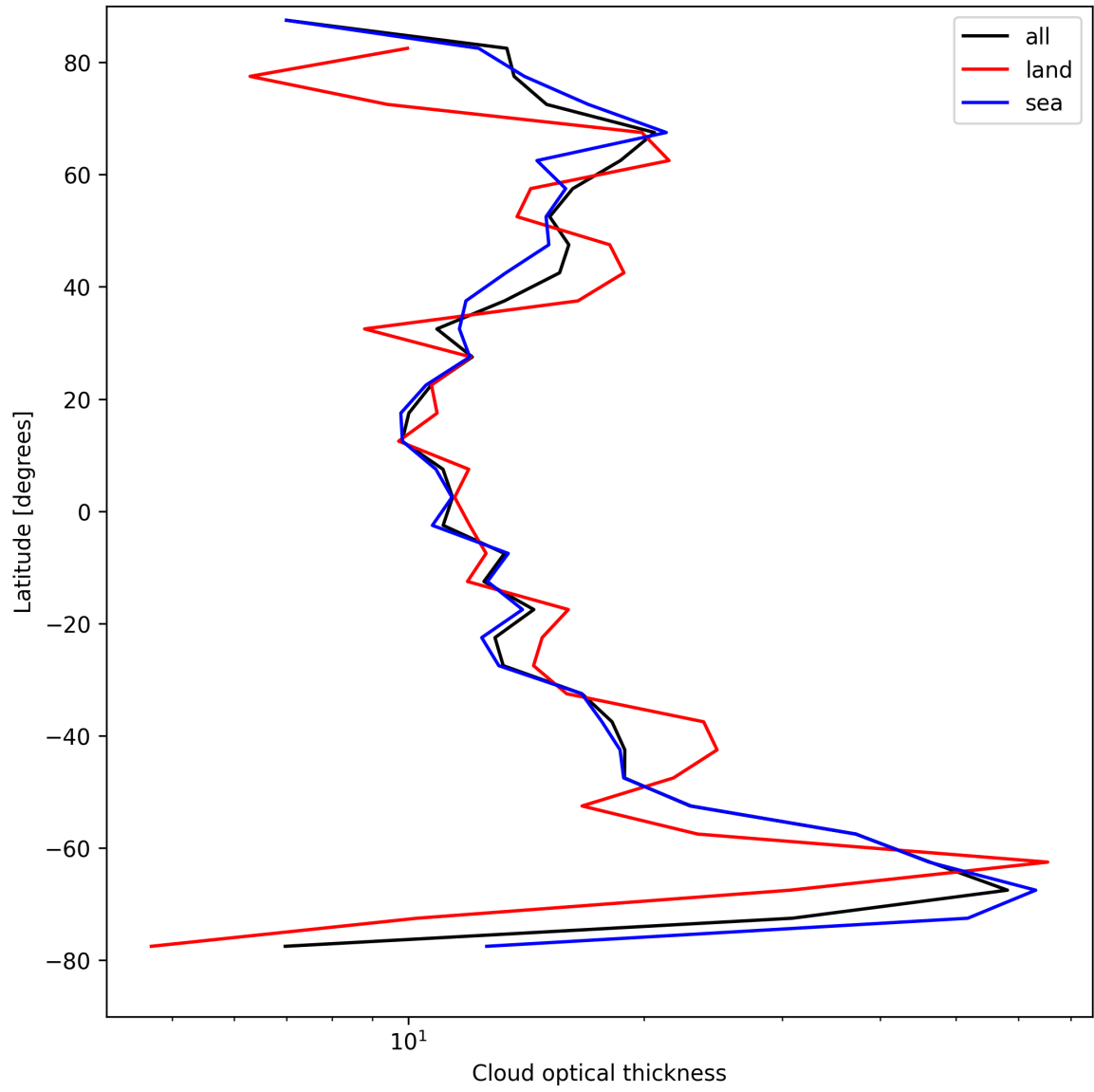
Figure 25: Zonal average of “Cloud optical thickness” for 2025-04-16 to 2025-04-18.
