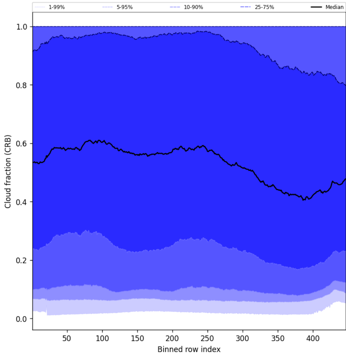
Figure 58: Along track statistics of “Cloud fraction (CRB)” for 2025-04-16 to 2025-04-18
