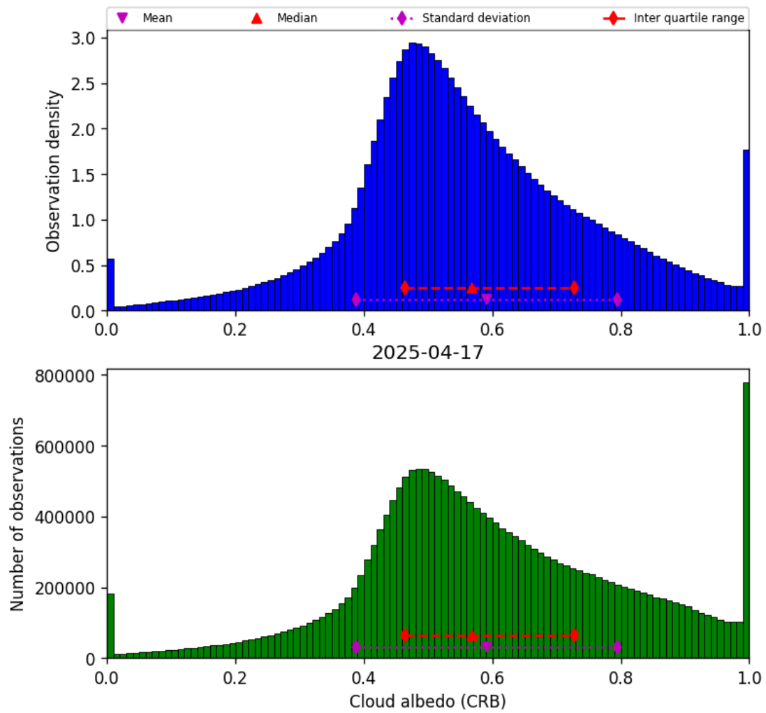
Figure 44: Histogram of “Cloud albedo (CRB)” for 2025-04-16 to 2025-04-18
