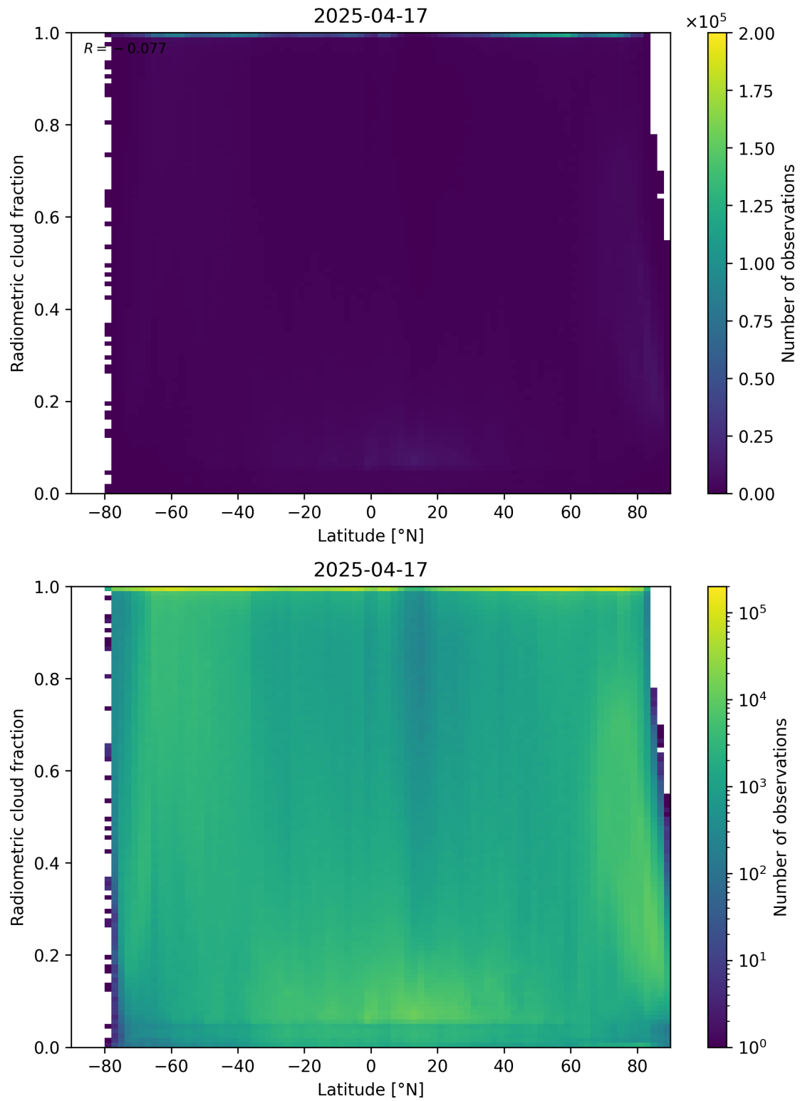
Figure 92: Scatter density plot of “Latitude” against “Radiometric cloud fraction” for 2025-04-16 to 2025-04-18.
