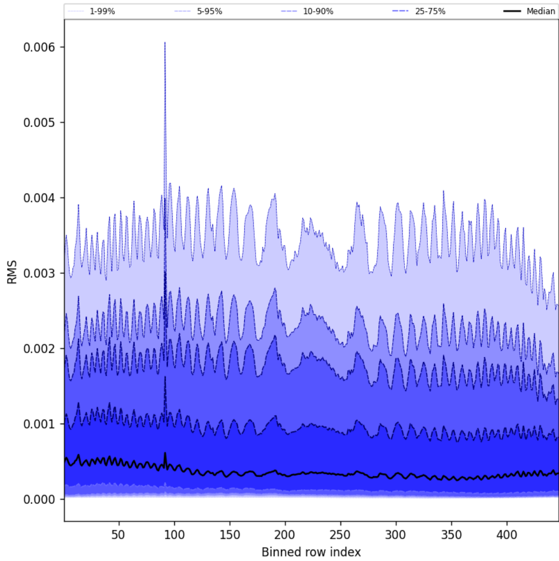
Figure 63: Along track statistics of “RMS” for 2025-04-16 to 2025-04-18
