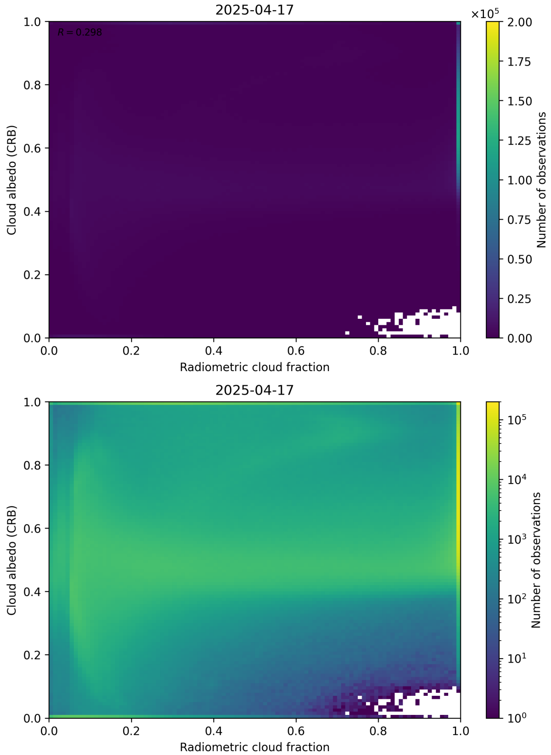
Figure 71: Scatter density plot of “Radiometric cloud fraction” against “Cloud albedo (CRB)” for 2025-04-16 to 2025-04-18.
