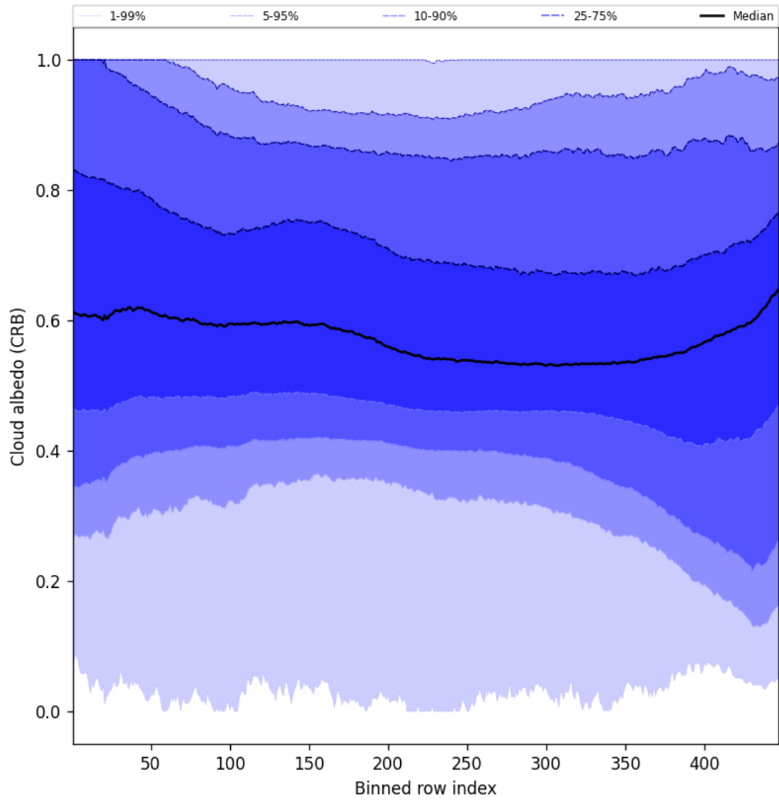
Figure 60: Along track statistics of “Cloud albedo (CRB)” for 2025-04-16 to 2025-04-18
