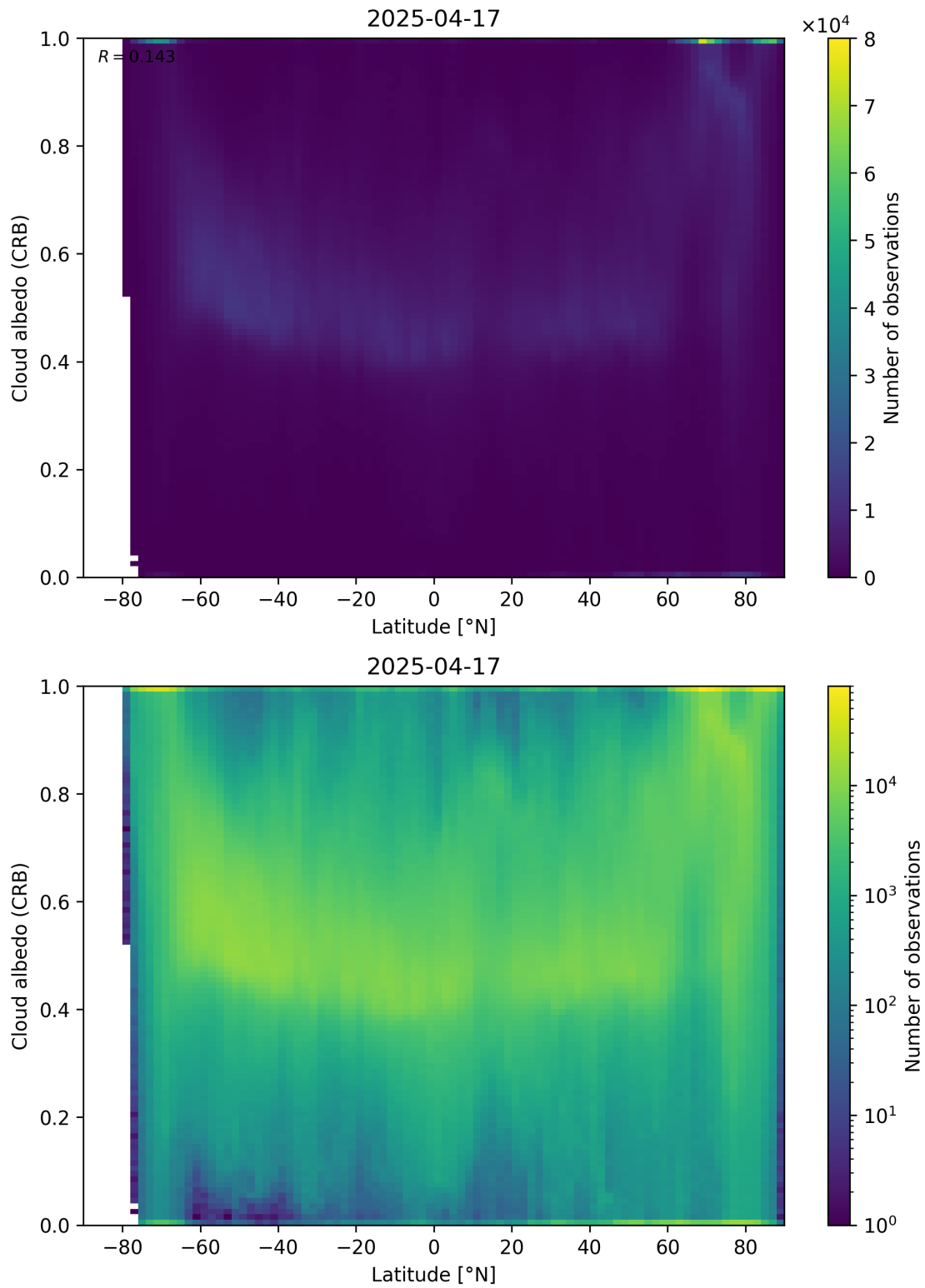
Figure 91: Scatter density plot of “Latitude” against “Cloud albedo (CRB)” for 2025-04-16 to 2025-04-18.
