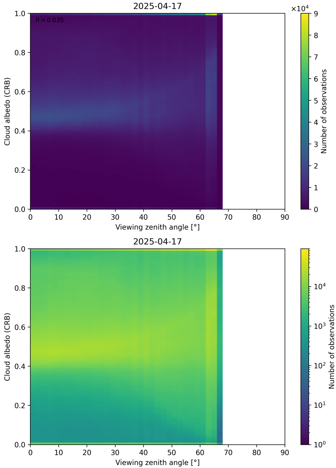
Figure 106: Scatter density plot of “Viewing zenith angle” against “Cloud albedo (CRB)” for 2025-04-16 to 2025-04-18.
