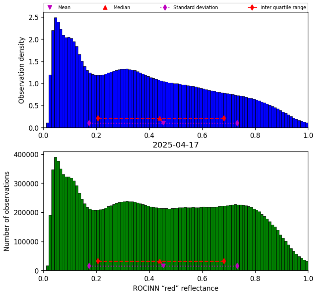
Figure 53: Histogram of “ROCINN “red” reflectance” for 2025-04-16 to 2025-04-18
