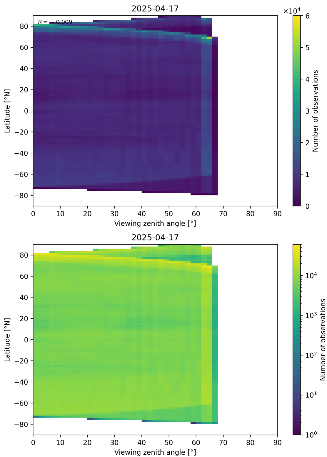
Figure 113: Scatter density plot of “Viewing zenith angle” against “Latitude” for 2025-04-16 to 2025-04-18.
