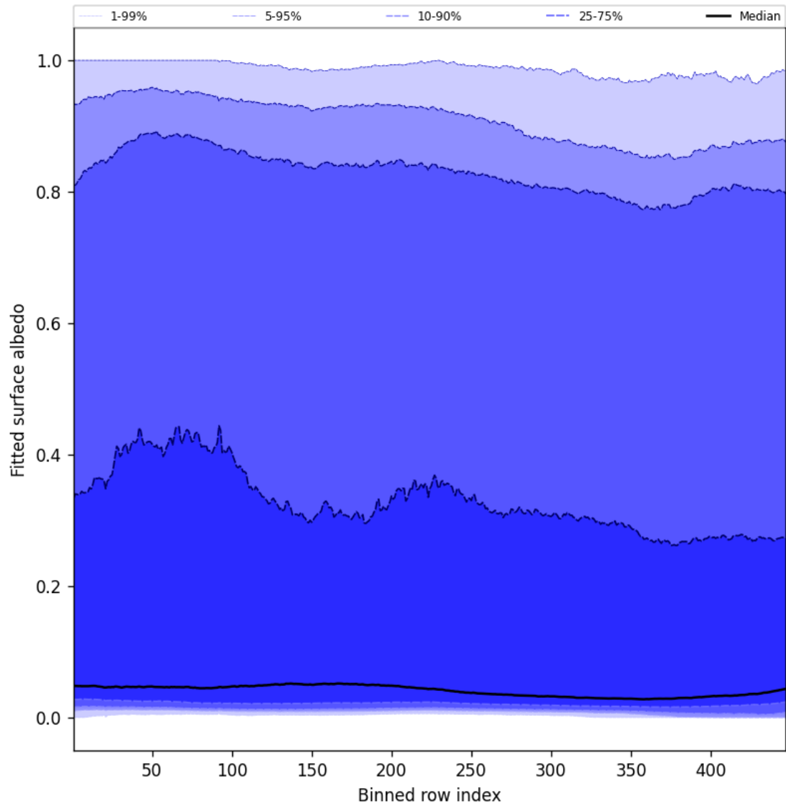
Figure 61: Along track statistics of “Fitted surface albedo” for 2025-04-16 to 2025-04-18
