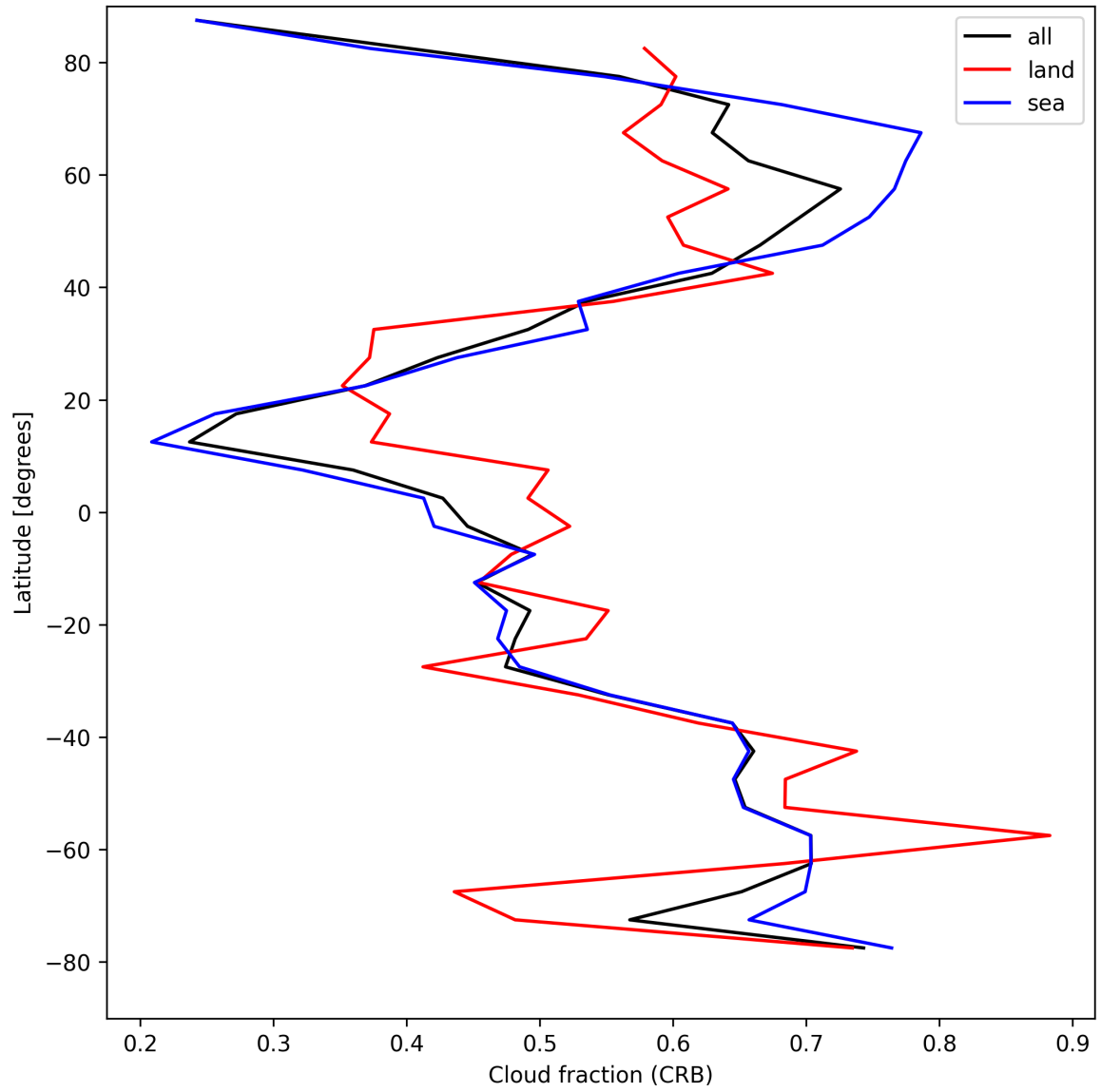
Figure 26: Zonal average of “Cloud fraction (CRB)” for 2025-04-16 to 2025-04-18.
