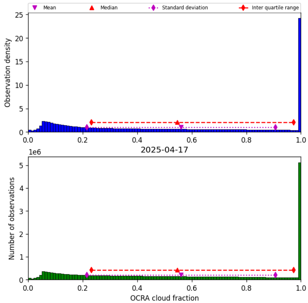
Figure 50: Histogram of “OCRA cloud fraction” for 2025-04-16 to 2025-04-18
