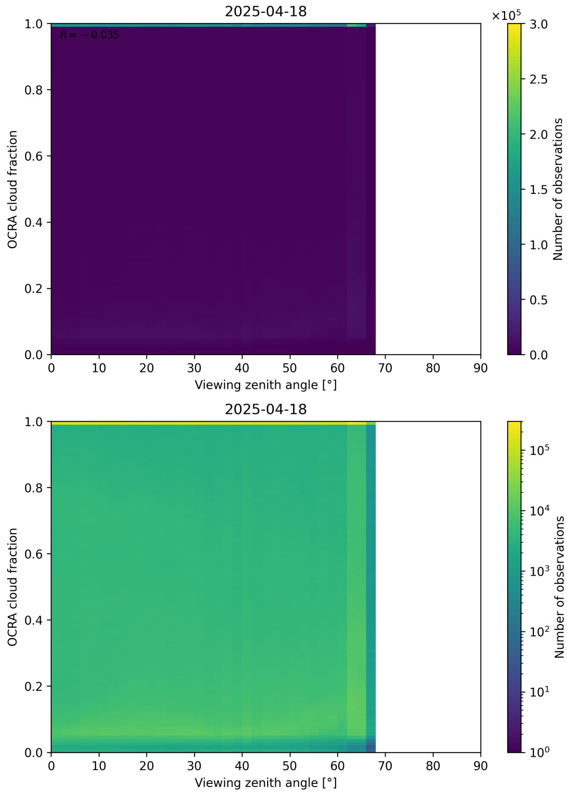
Figure 108: Scatter density plot of “Viewing zenith angle” against “OCRA cloud fraction” for 2025-04-18 to 2025-04-19.
