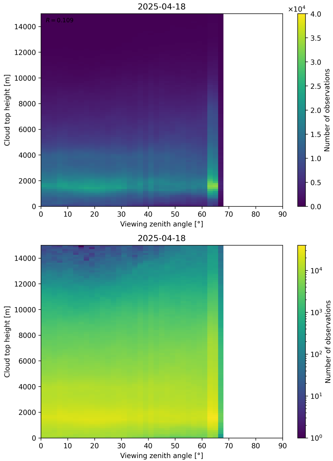
Figure 112: Scatter density plot of “Viewing zenith angle” against “Cloud top height” for 2025-04-18 to 2025-04-19.
