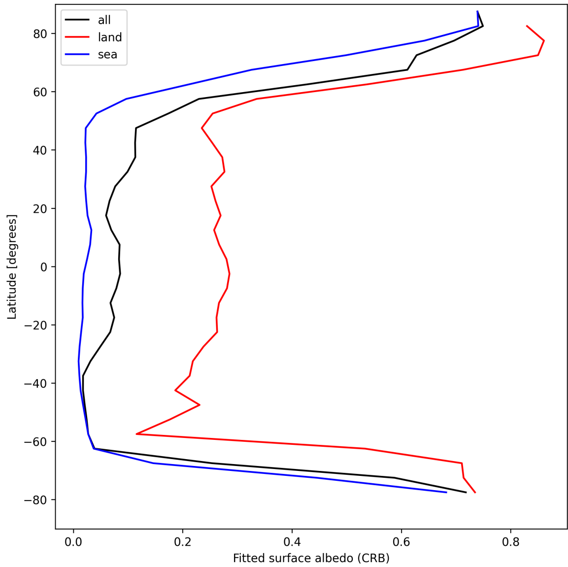
Figure 30: Zonal average of “Fitted surface albedo (CRB)” for 2025-04-18 to 2025-04-19.
