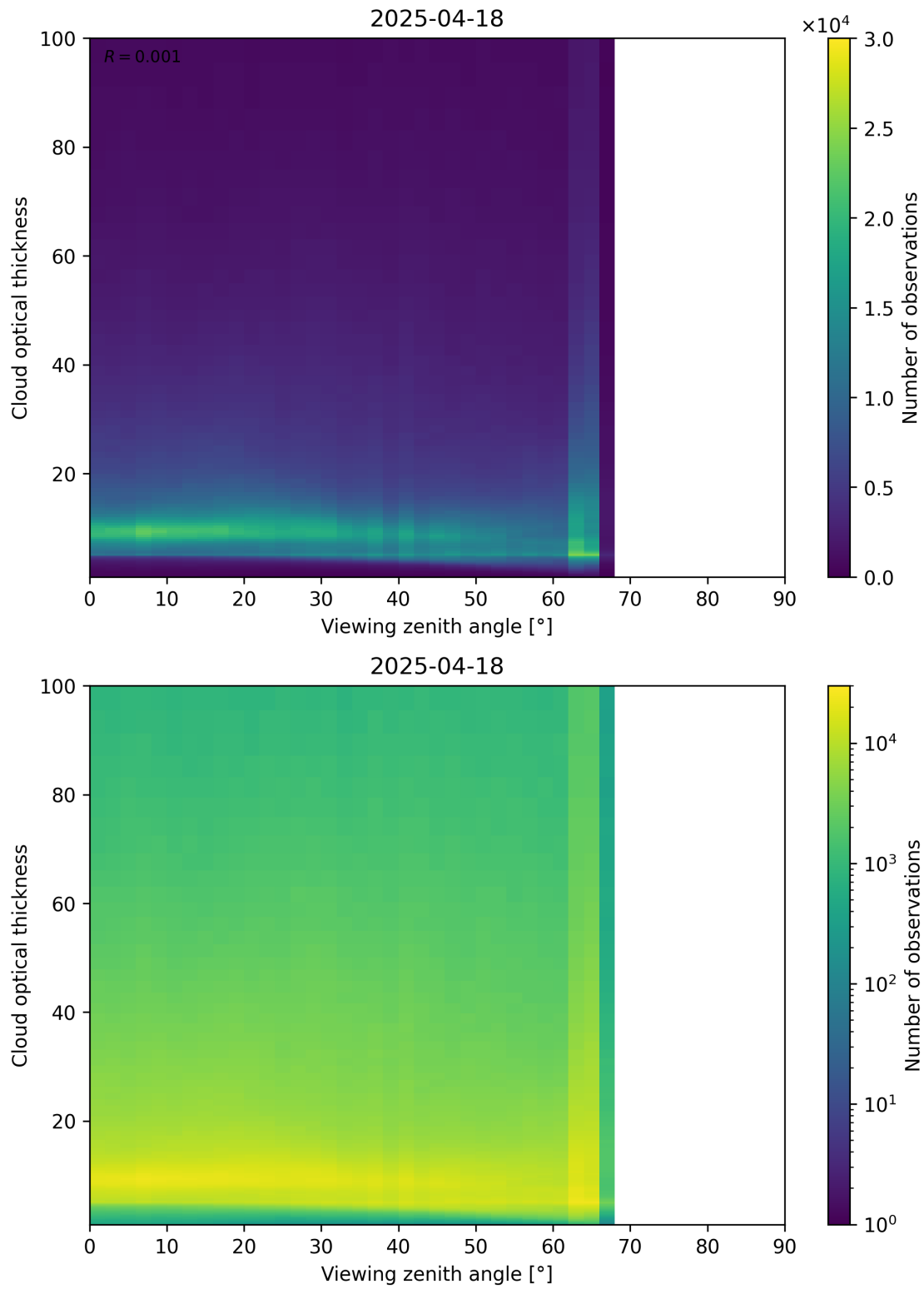
Figure 111: Scatter density plot of “Viewing zenith angle” against “Cloud optical thickness” for 2025-04-18 to 2025-04-19.
