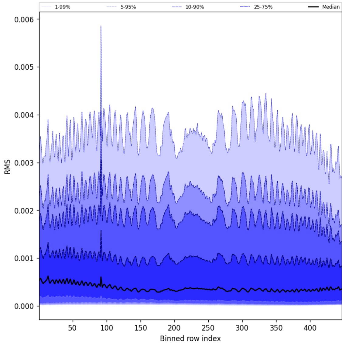
Figure 63: Along track statistics of “RMS” for 2025-04-18 to 2025-04-19
