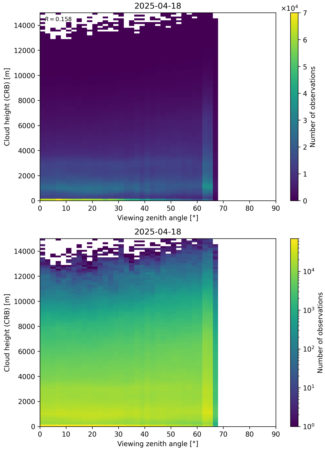
Figure 110: Scatter density plot of “Viewing zenith angle” against “Cloud height (CRB)” for 2025-04-18 to 2025-04-19.
