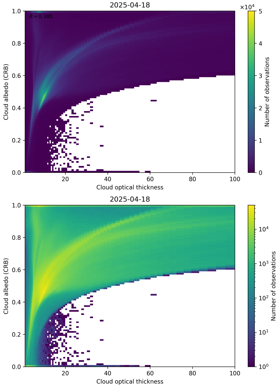
Figure 82: Scatter density plot of “Cloud optical thickness” against “Cloud albedo (CRB)” for 2025-04-18 to 2025-04-19.
