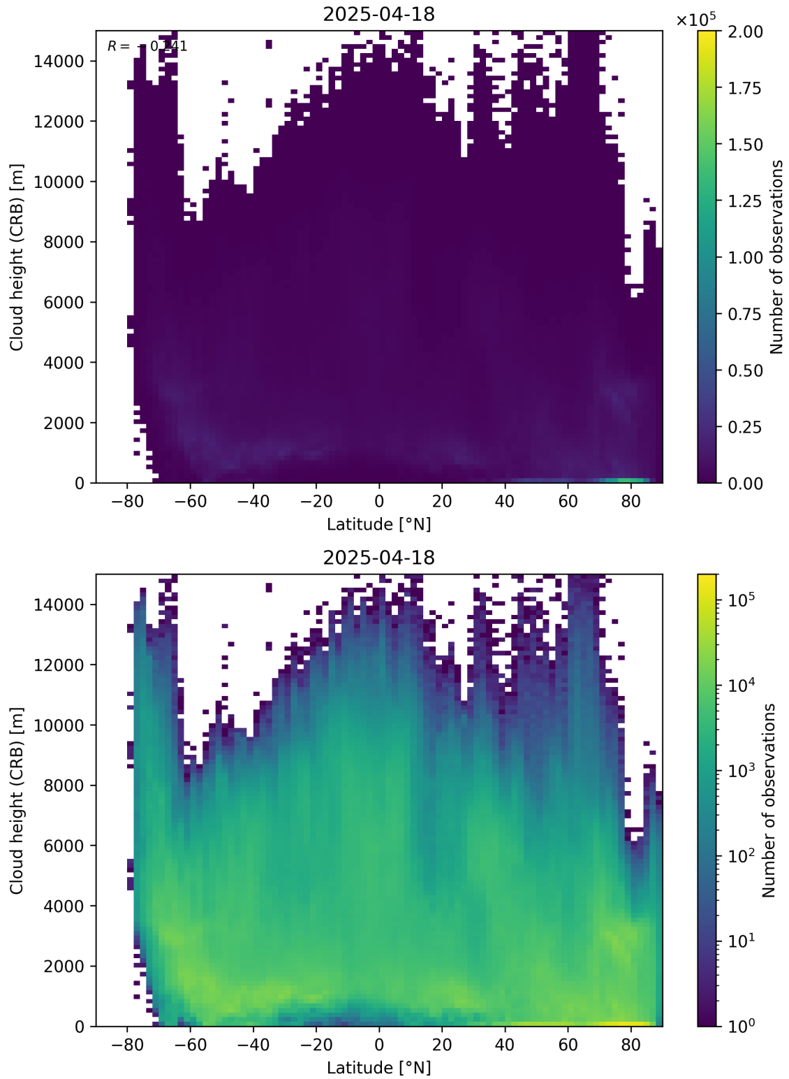
Figure 95: Scatter density plot of “Latitude” against “Cloud height (CRB)” for 2025-04-18 to 2025-04-19.
