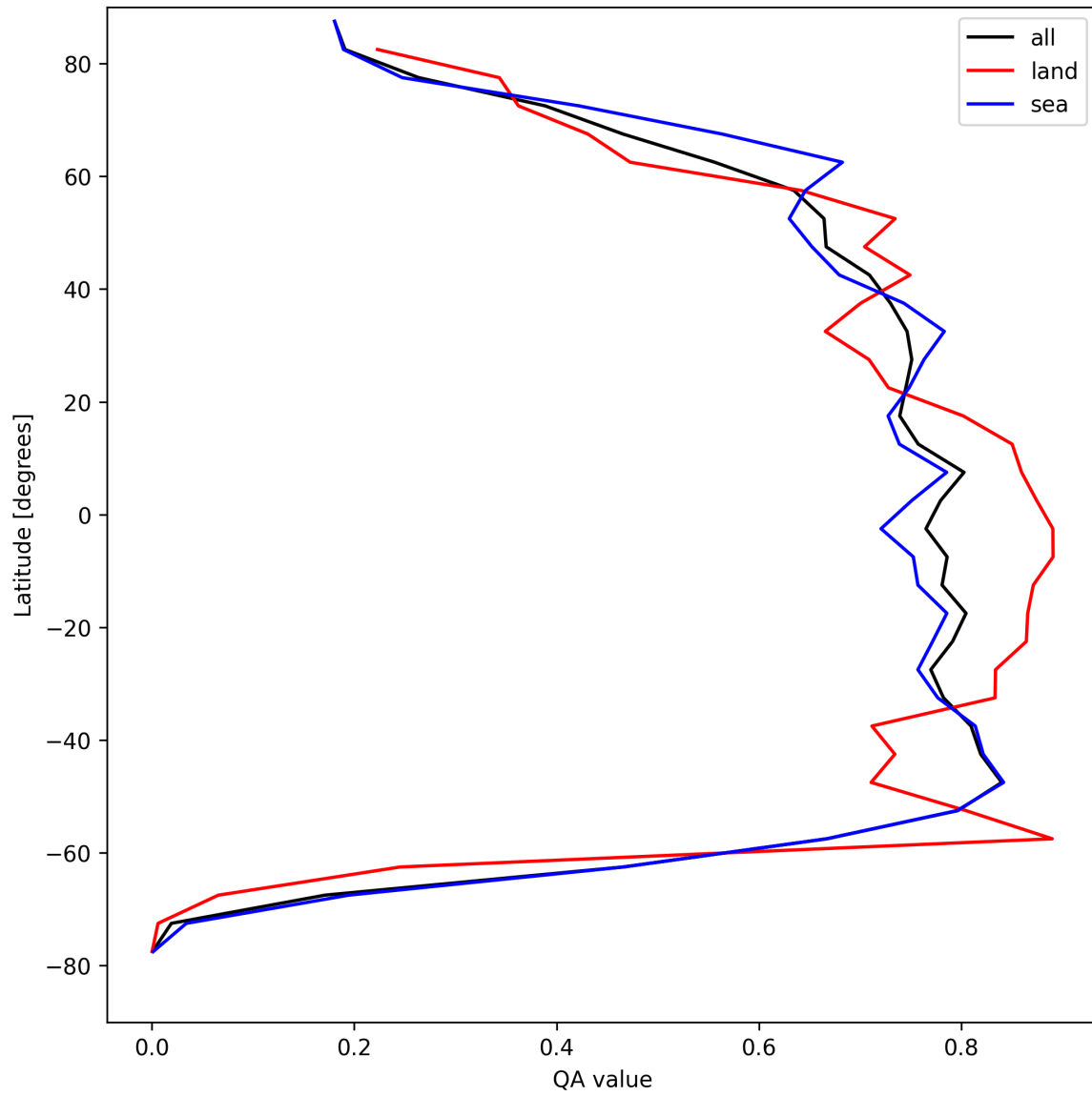
Figure 22: Zonal average of “QA value” for 2025-04-18 to 2025-04-19.
