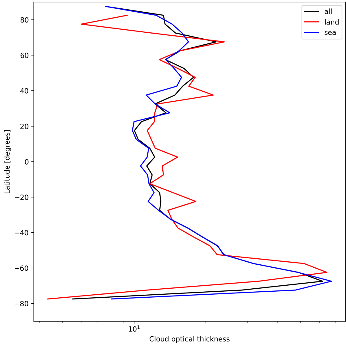
Figure 25: Zonal average of “Cloud optical thickness” for 2025-04-18 to 2025-04-19.
