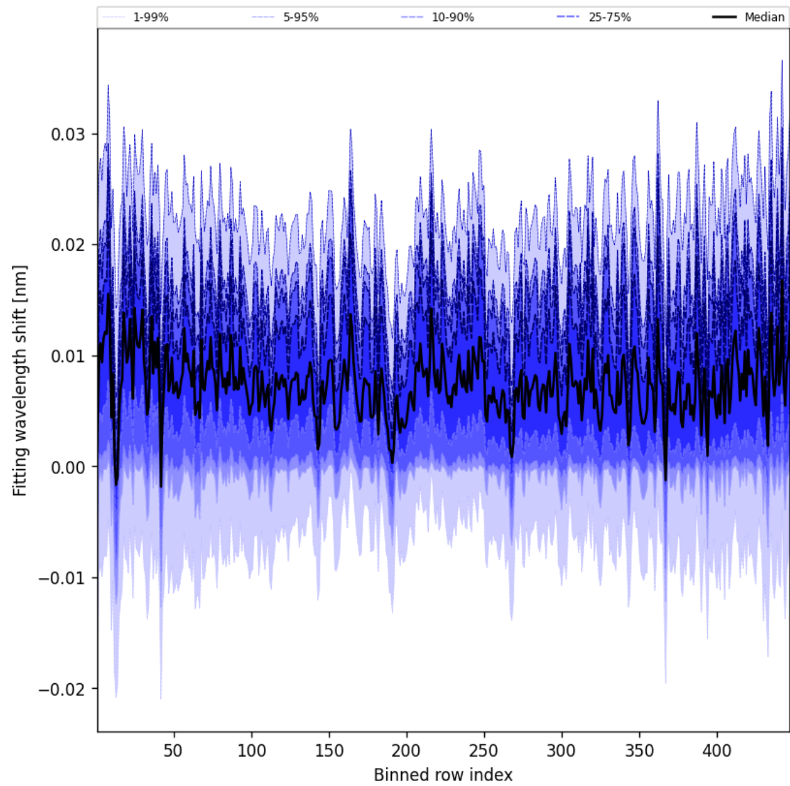
Figure 65: Along track statistics of “Fitting wavelength shift” for 2025-04-18 to 2025-04-19
