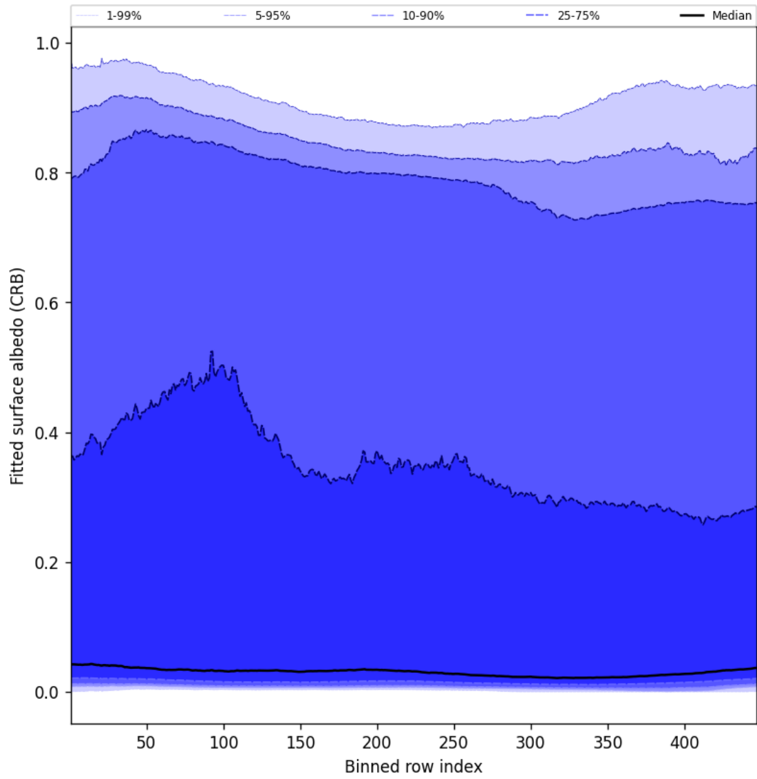
Figure 62: Along track statistics of “Fitted surface albedo (CRB)” for 2025-04-18 to 2025-04-19
