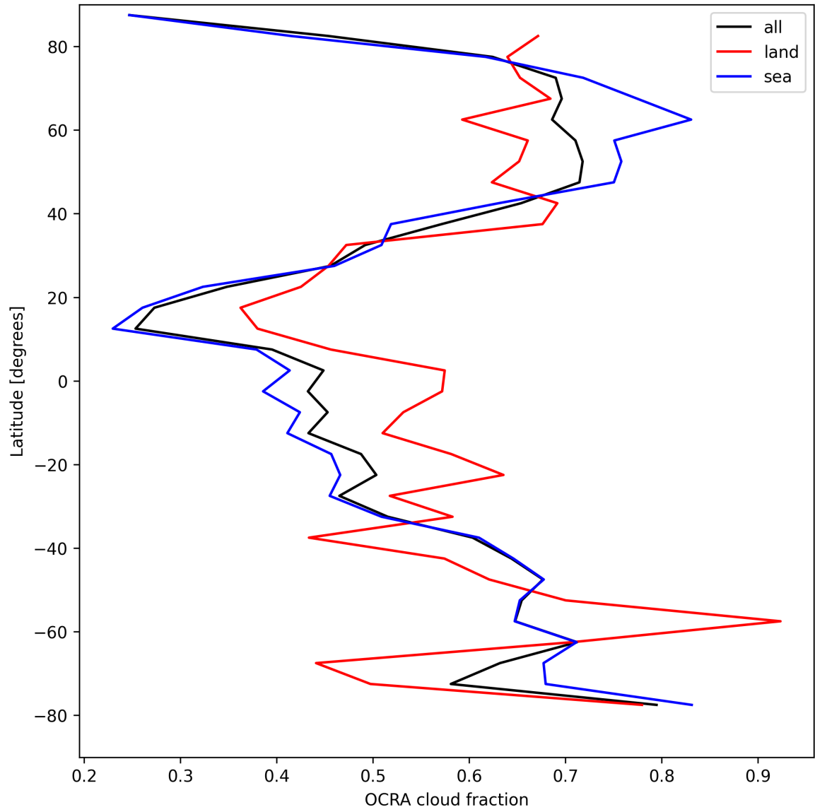
Figure 34: Zonal average of “OCRA cloud fraction” for 2025-04-18 to 2025-04-19.
