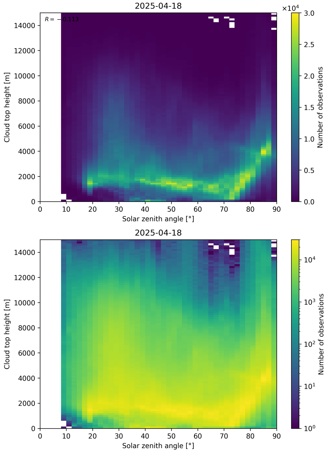
Figure 104: Scatter density plot of “Solar zenith angle” against “Cloud top height” for 2025-04-18 to 2025-04-19.
