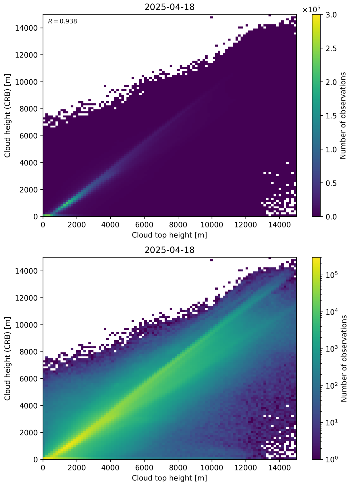
Figure 89: Scatter density plot of “Cloud top height” against “Cloud height (CRB)” for 2025-04-18 to 2025-04-19.
