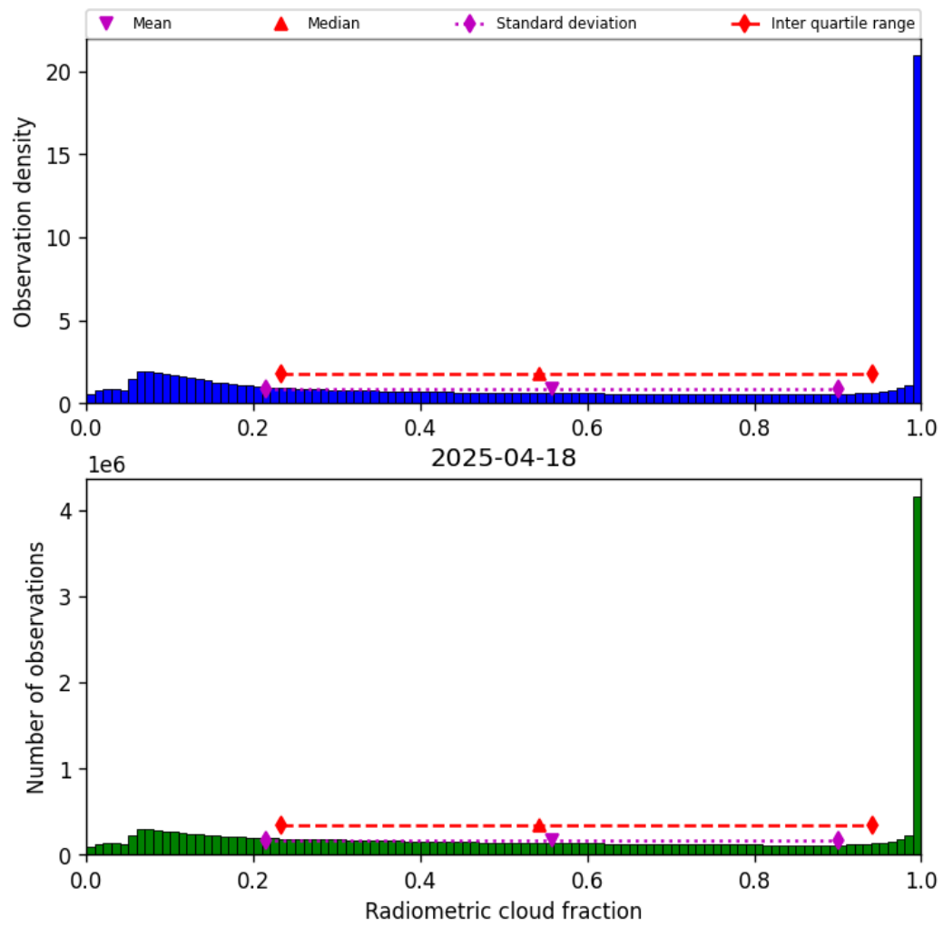
Figure 39: Histogram of “Radiometric cloud fraction” for 2025-04-18 to 2025-04-19
