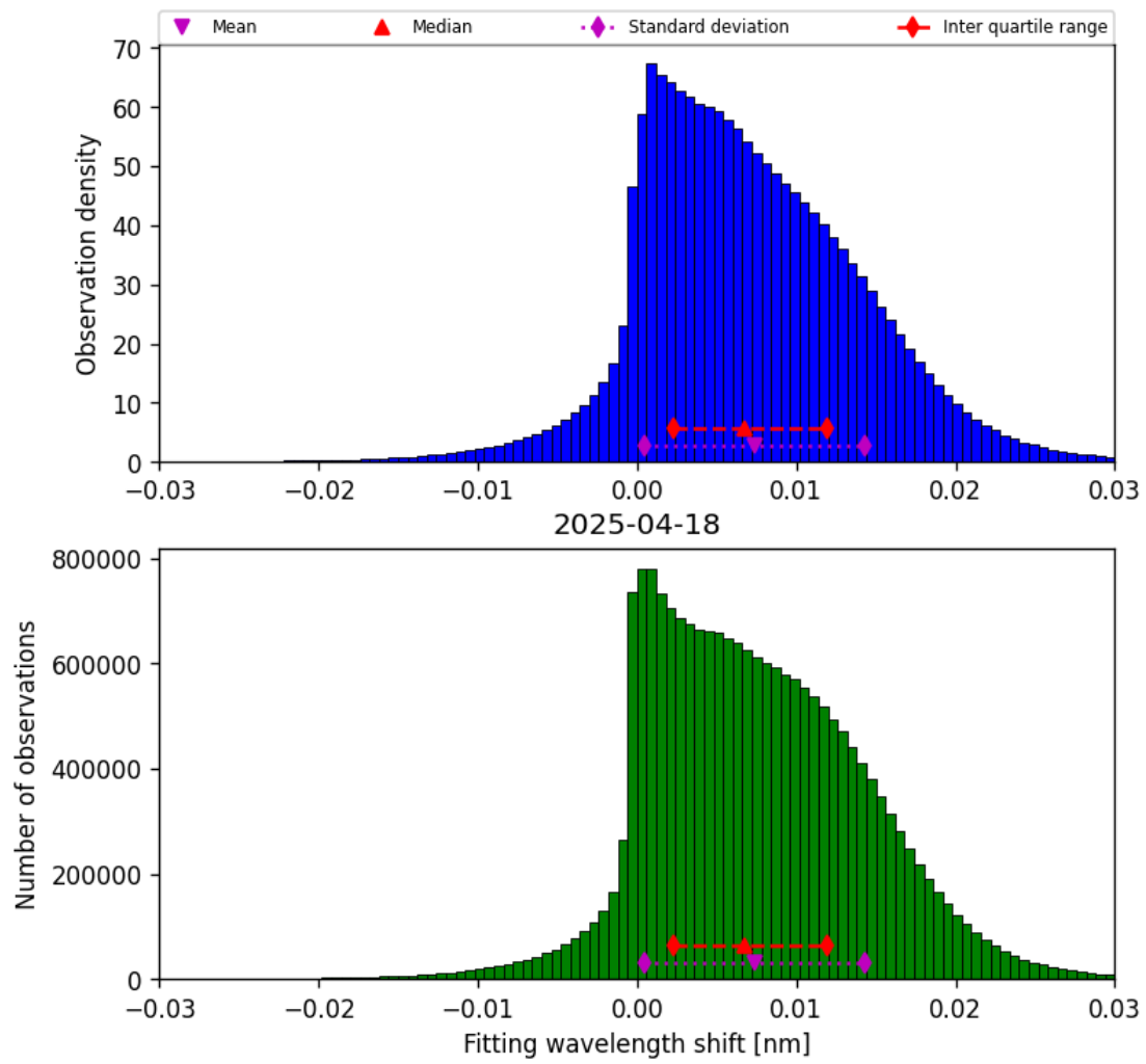
Figure 49: Histogram of “Fitting wavelength shift” for 2025-04-18 to 2025-04-19
