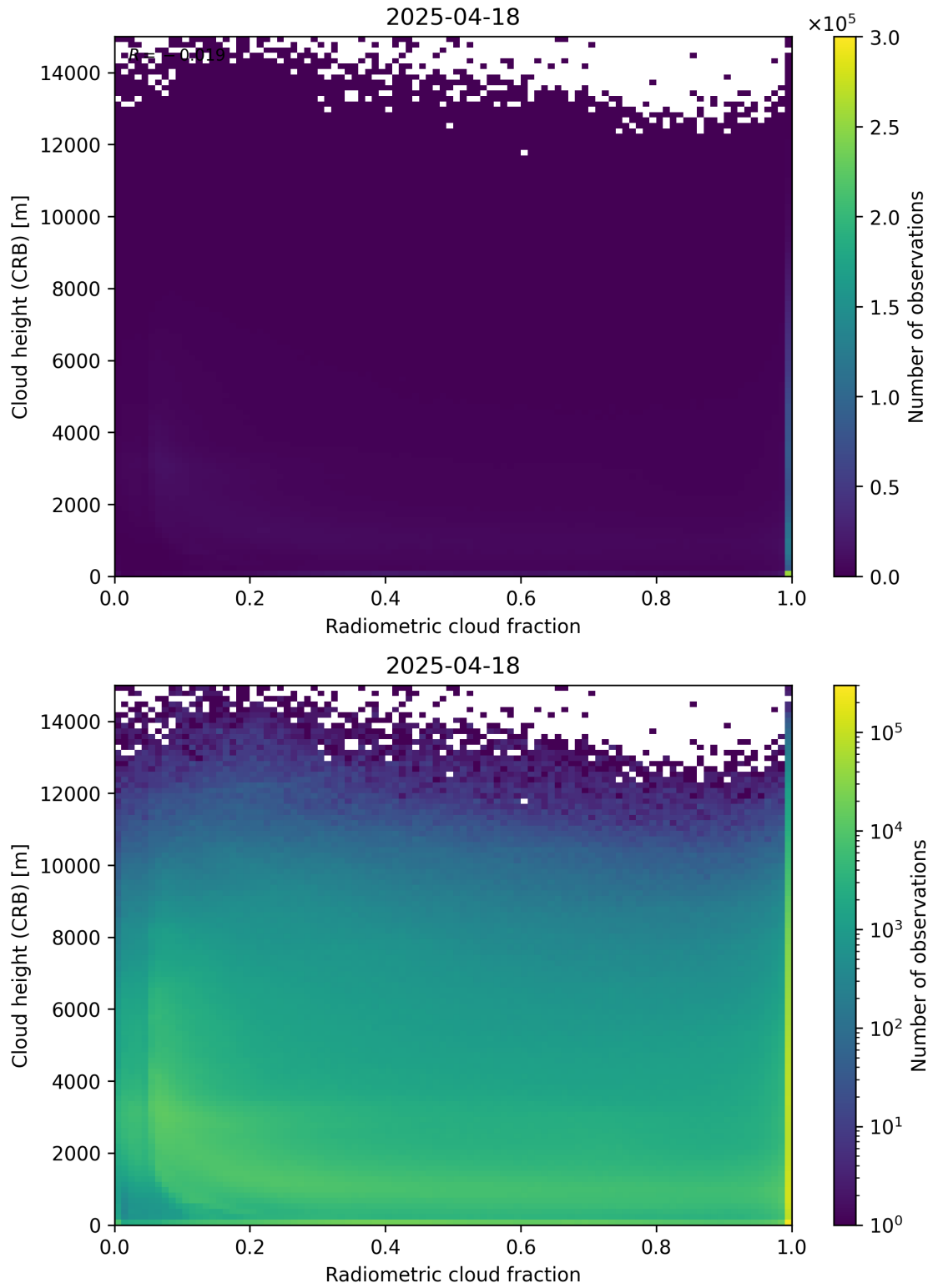
Figure 74: Scatter density plot of “Radiometric cloud fraction” against “Cloud height (CRB)” for 2025-04-18 to 2025-04-19.
