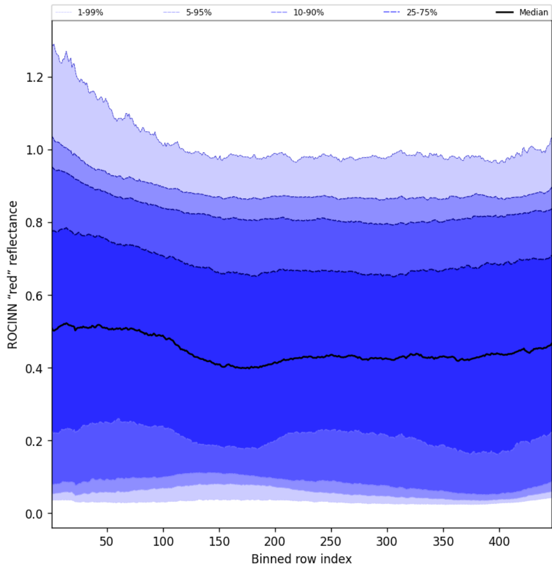
Figure 69: Along track statistics of “ROCINN “red” reflectance” for 2025-04-18 to 2025-04-19
