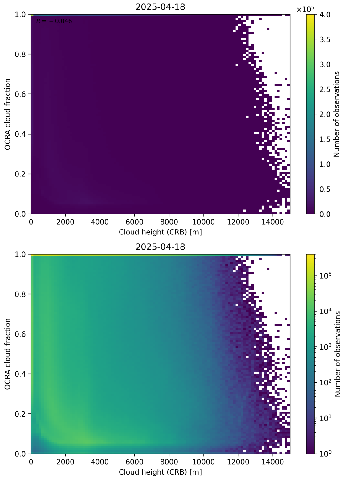
Figure 81: Scatter density plot of “Cloud height (CRB)” against “OCRA cloud fraction” for 2025-04-18 to 2025-04-19.
