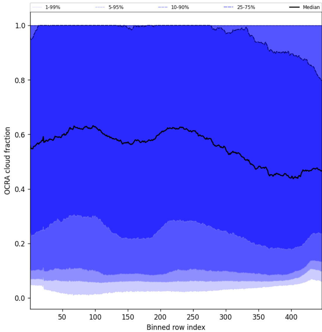
Figure 66: Along track statistics of “OCRA cloud fraction” for 2025-04-18 to 2025-04-19
