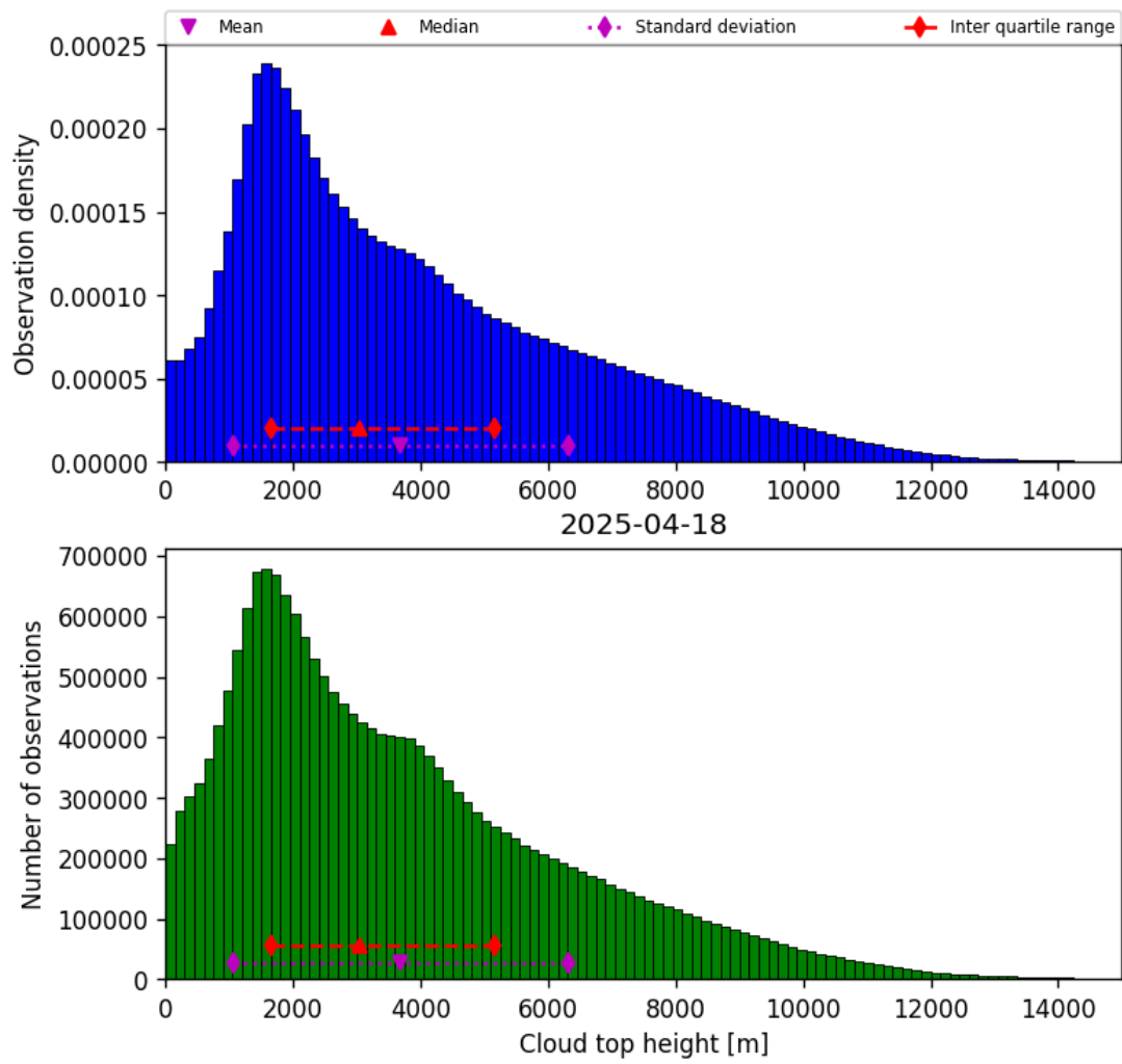
Figure 40: Histogram of “Cloud top height” for 2025-04-18 to 2025-04-19
