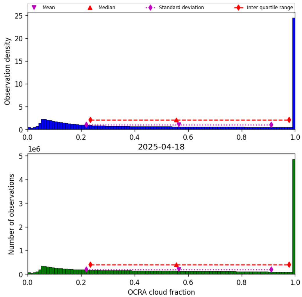
Figure 50: Histogram of “OCRA cloud fraction” for 2025-04-18 to 2025-04-19
