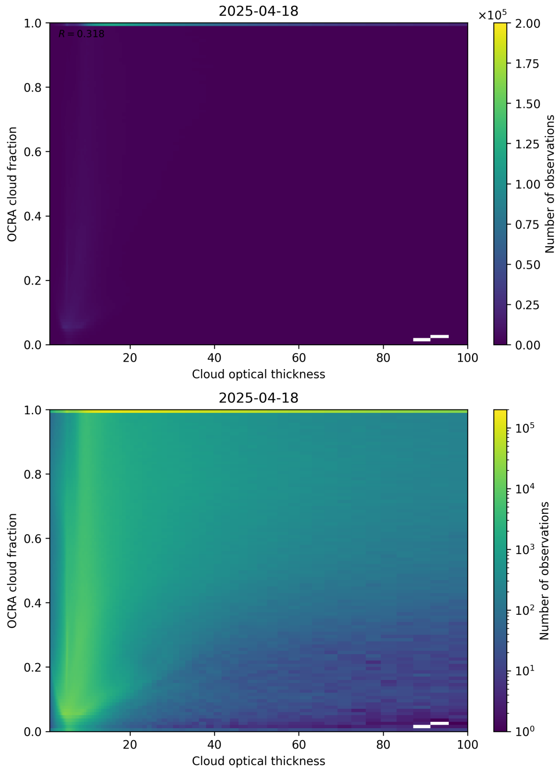
Figure 83: Scatter density plot of “Cloud optical thickness” against “OCRA cloud fraction” for 2025-04-18 to 2025-04-19.
