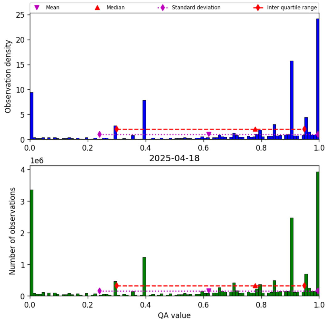
Figure 38: Histogram of “QA value” for 2025-04-18 to 2025-04-19
