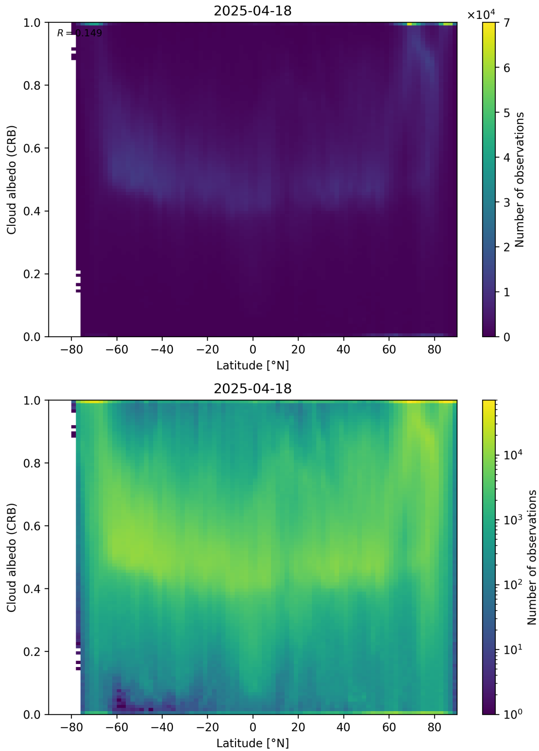
Figure 91: Scatter density plot of “Latitude” against “Cloud albedo (CRB)” for 2025-04-18 to 2025-04-19.
