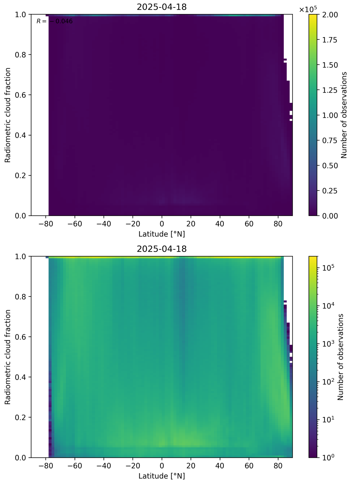
Figure 92: Scatter density plot of “Latitude” against “Radiometric cloud fraction” for 2025-04-18 to 2025-04-19.
