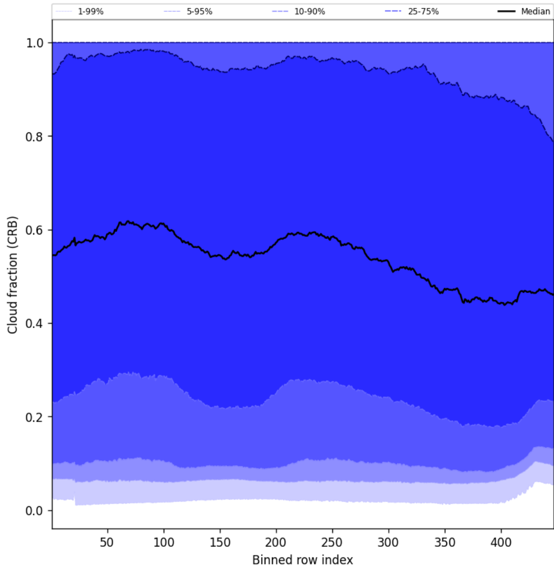
Figure 58: Along track statistics of “Cloud fraction (CRB)” for 2025-04-18 to 2025-04-19
