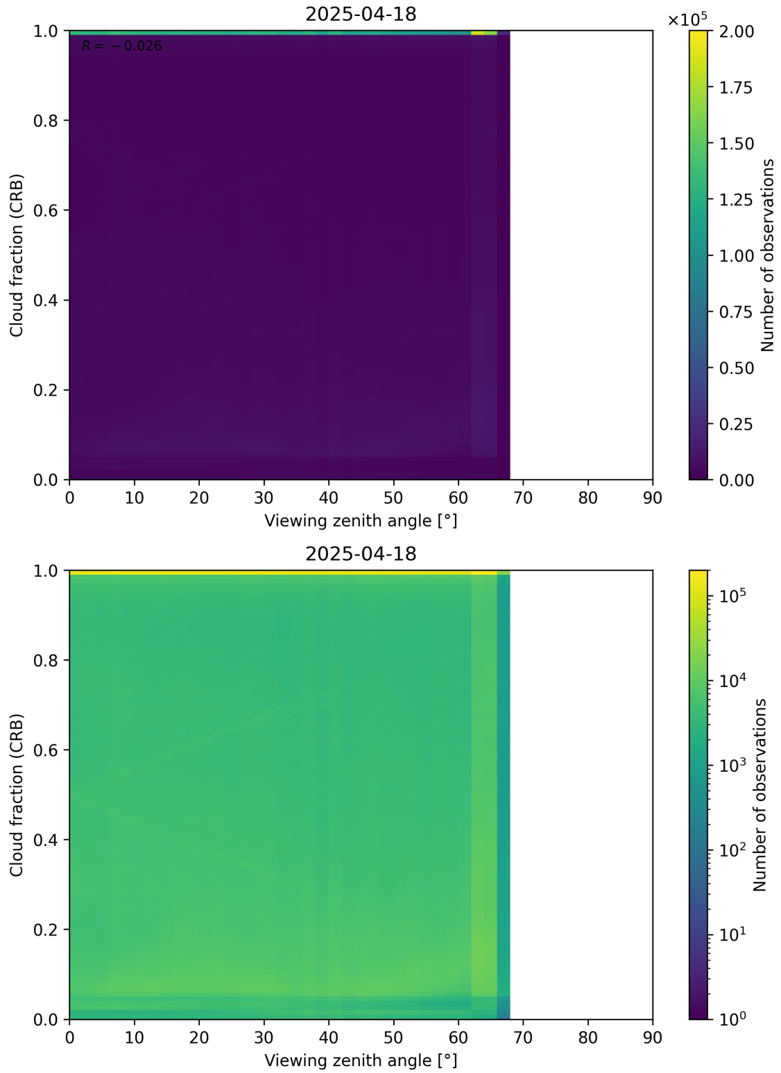
Figure 109: Scatter density plot of “Viewing zenith angle” against “Cloud fraction (CRB)” for 2025-04-18 to 2025-04-19.
