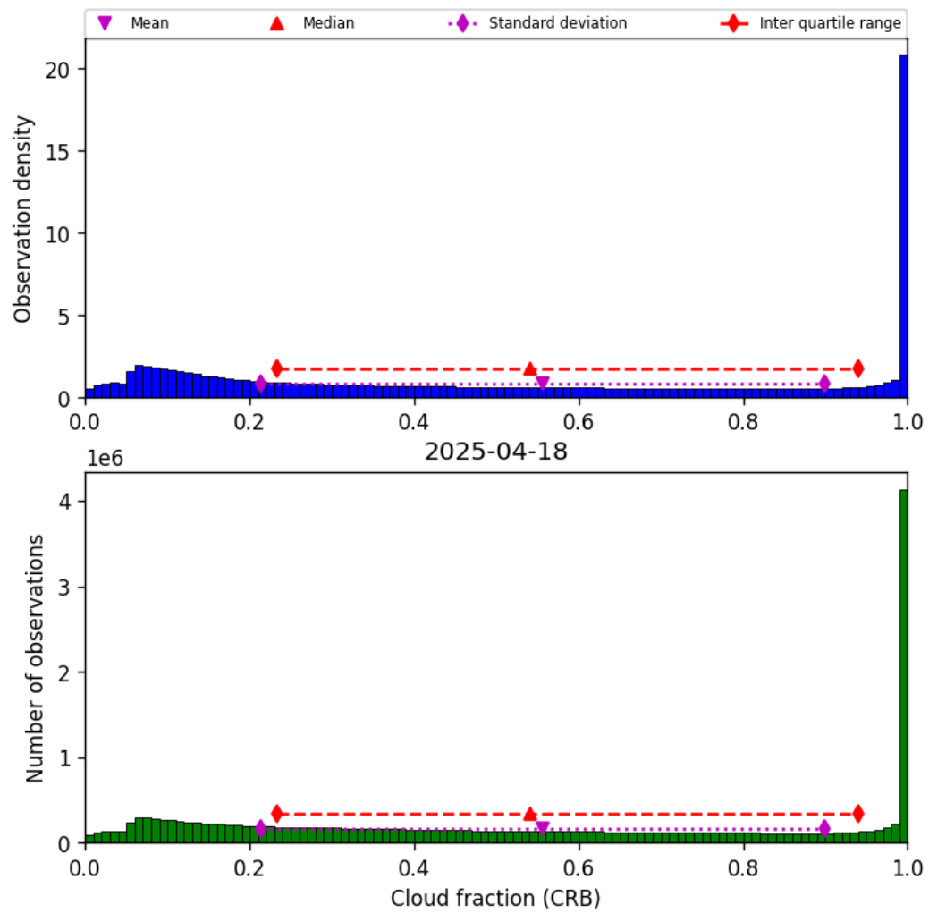
Figure 42: Histogram of “Cloud fraction (CRB)” for 2025-04-18 to 2025-04-19
