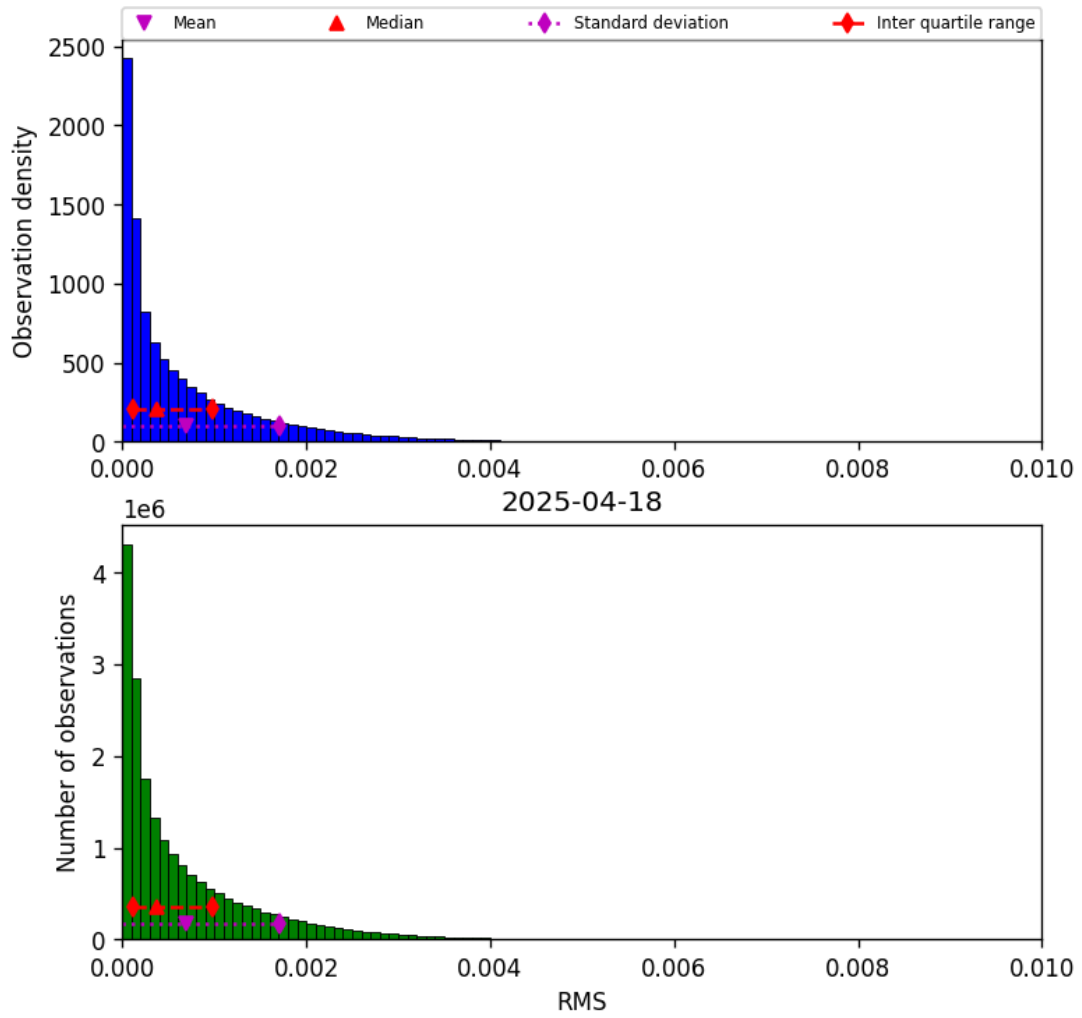
Figure 47: Histogram of “RMS” for 2025-04-18 to 2025-04-19
