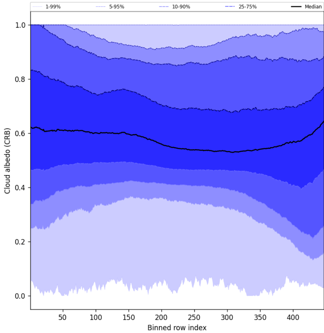
Figure 60: Along track statistics of “Cloud albedo (CRB)” for 2025-04-18 to 2025-04-19
