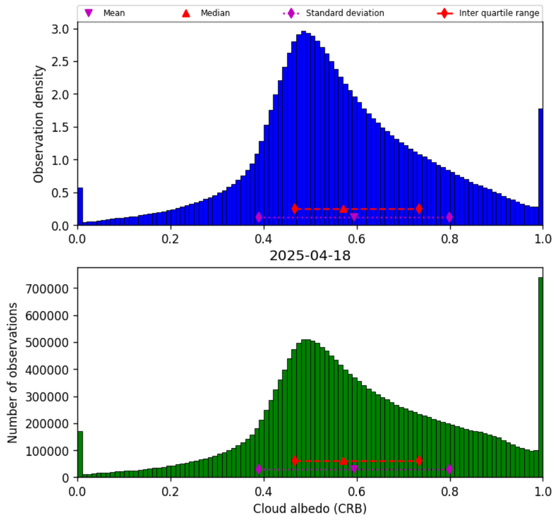
Figure 44: Histogram of “Cloud albedo (CRB)” for 2025-04-18 to 2025-04-19
