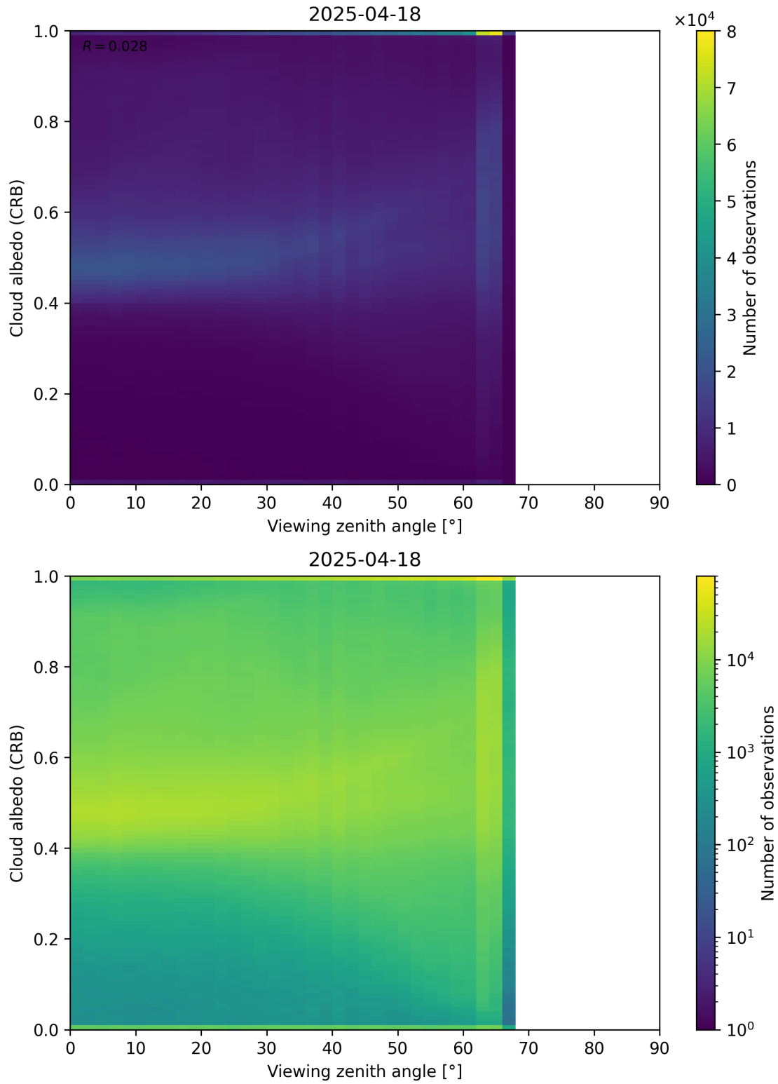
Figure 106: Scatter density plot of “Viewing zenith angle” against “Cloud albedo (CRB)” for 2025-04-18 to 2025-04-19.
