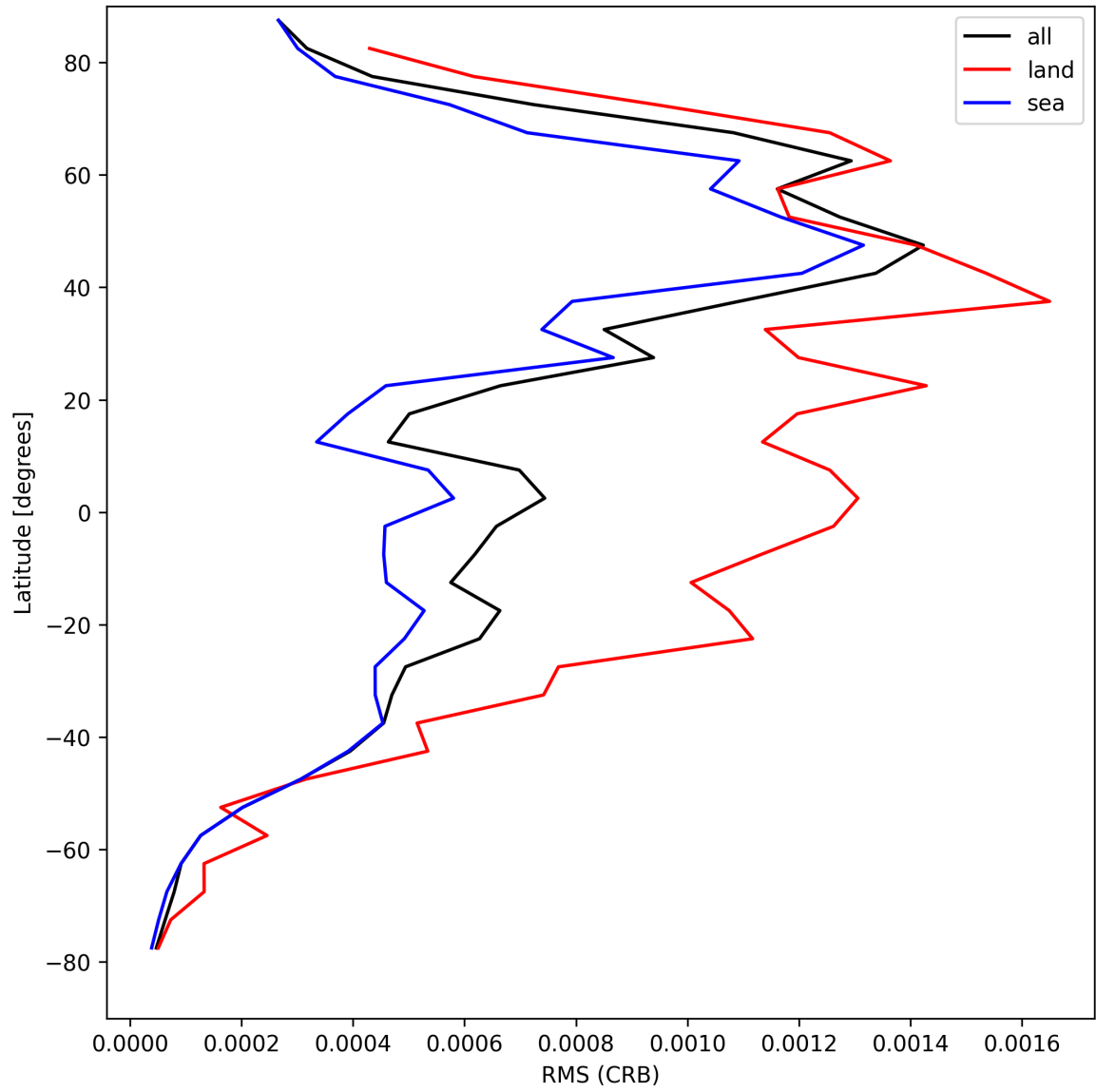
Figure 32: Zonal average of “RMS (CRB)” for 2025-04-18 to 2025-04-19.
