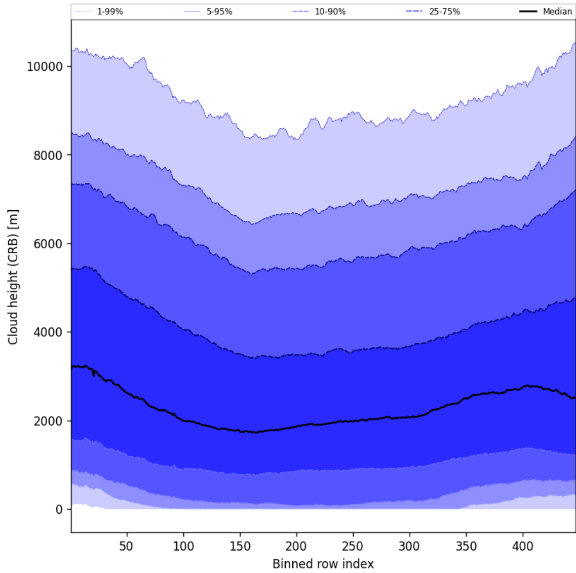
Figure 59: Along track statistics of “Cloud height (CRB)” for 2025-04-18 to 2025-04-19
