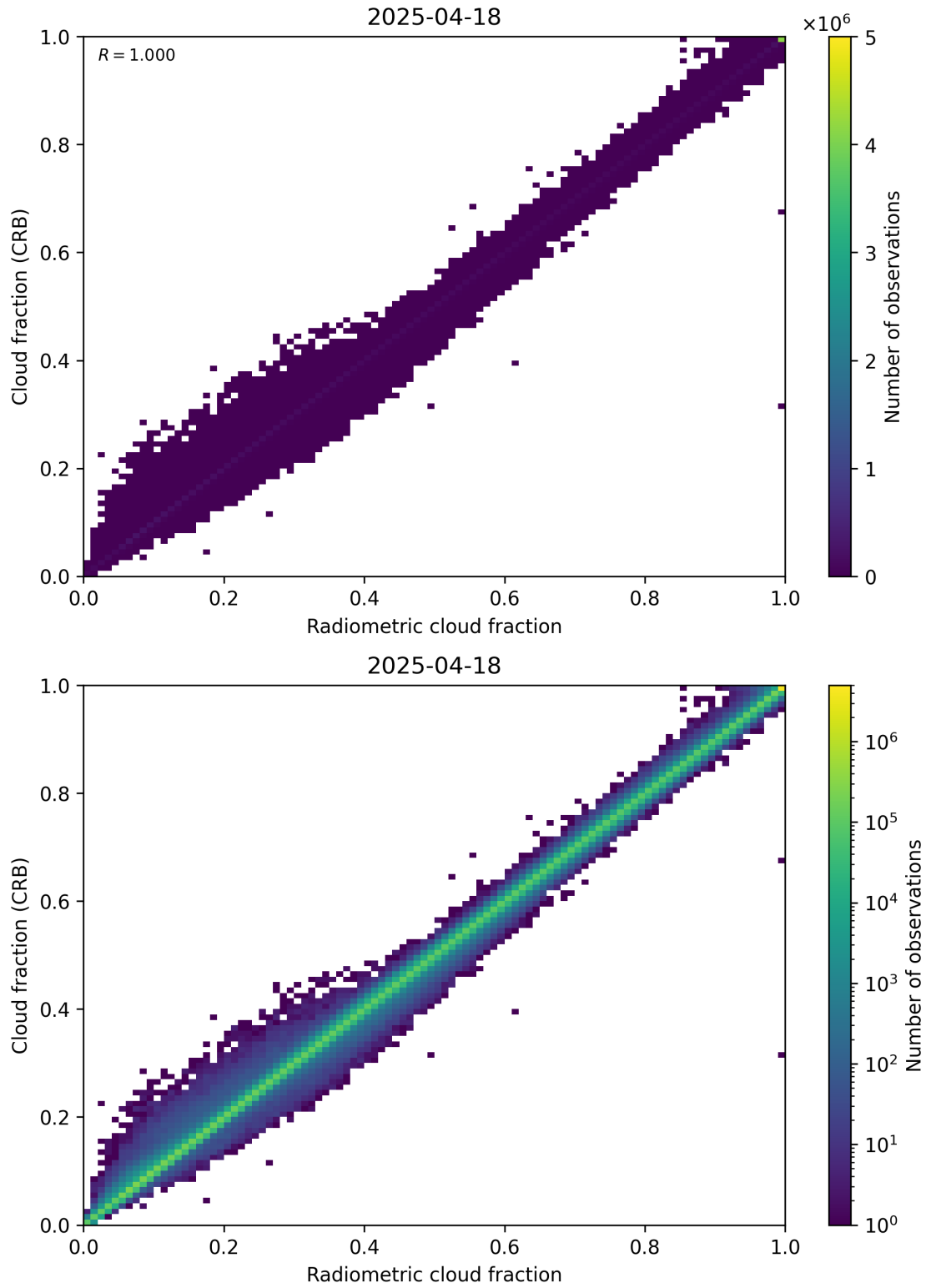
Figure 73: Scatter density plot of “Radiometric cloud fraction” against “Cloud fraction (CRB)” for 2025-04-18 to 2025-04-19.
