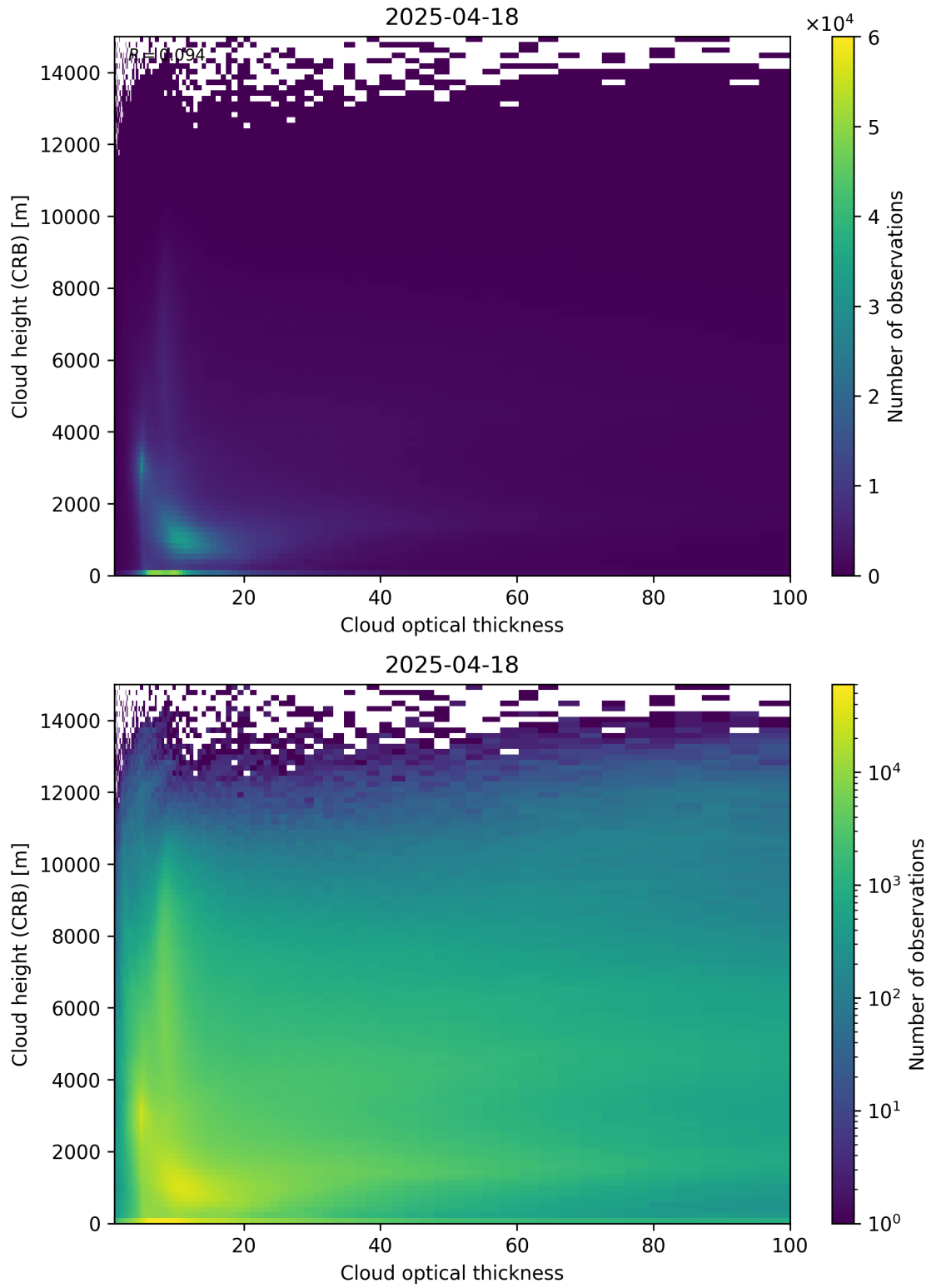
Figure 85: Scatter density plot of “Cloud optical thickness” against “Cloud height (CRB)” for 2025-04-18 to 2025-04-19.
