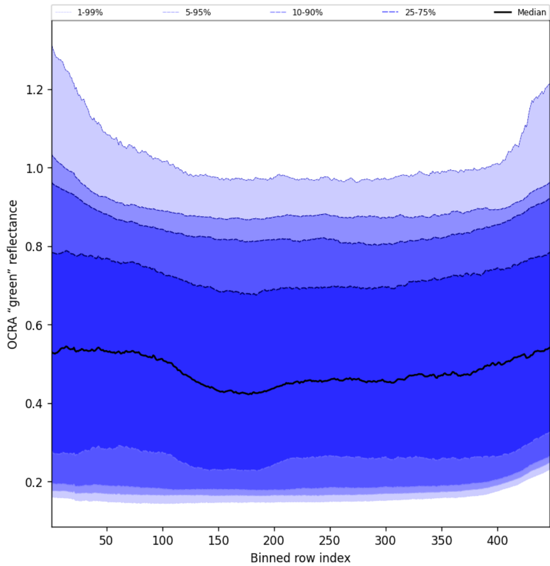
Figure 68: Along track statistics of “OCRA “green” reflectance” for 2025-04-18 to 2025-04-19
