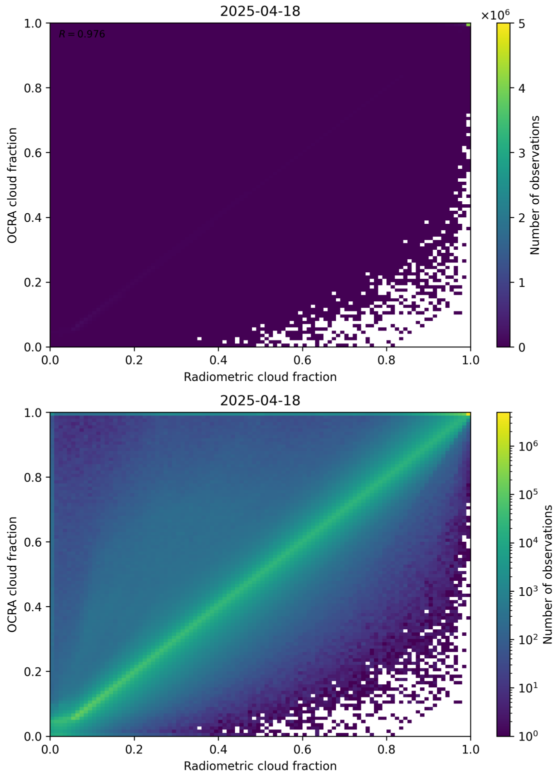
Figure 72: Scatter density plot of “Radiometric cloud fraction” against “OCRA cloud fraction” for 2025-04-18 to 2025-04-19.
