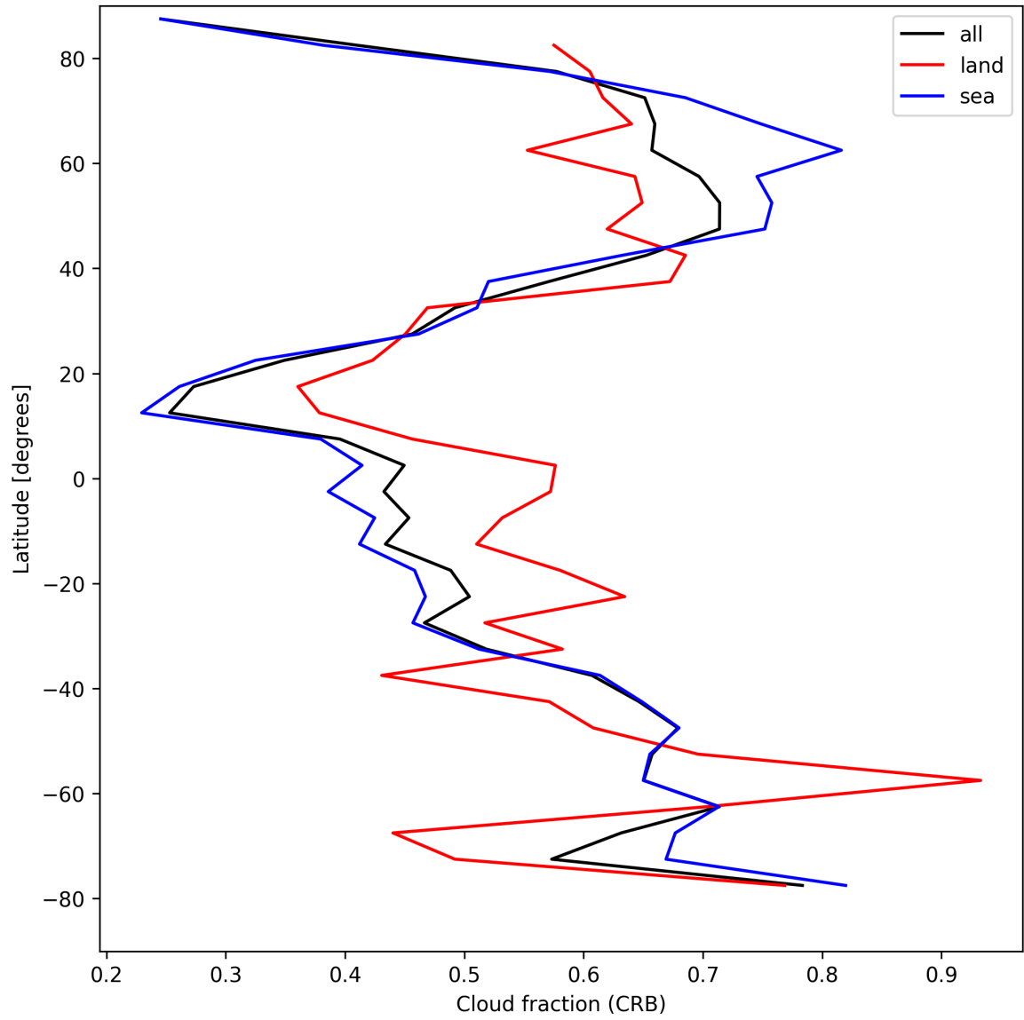
Figure 26: Zonal average of “Cloud fraction (CRB)” for 2025-04-18 to 2025-04-19.
