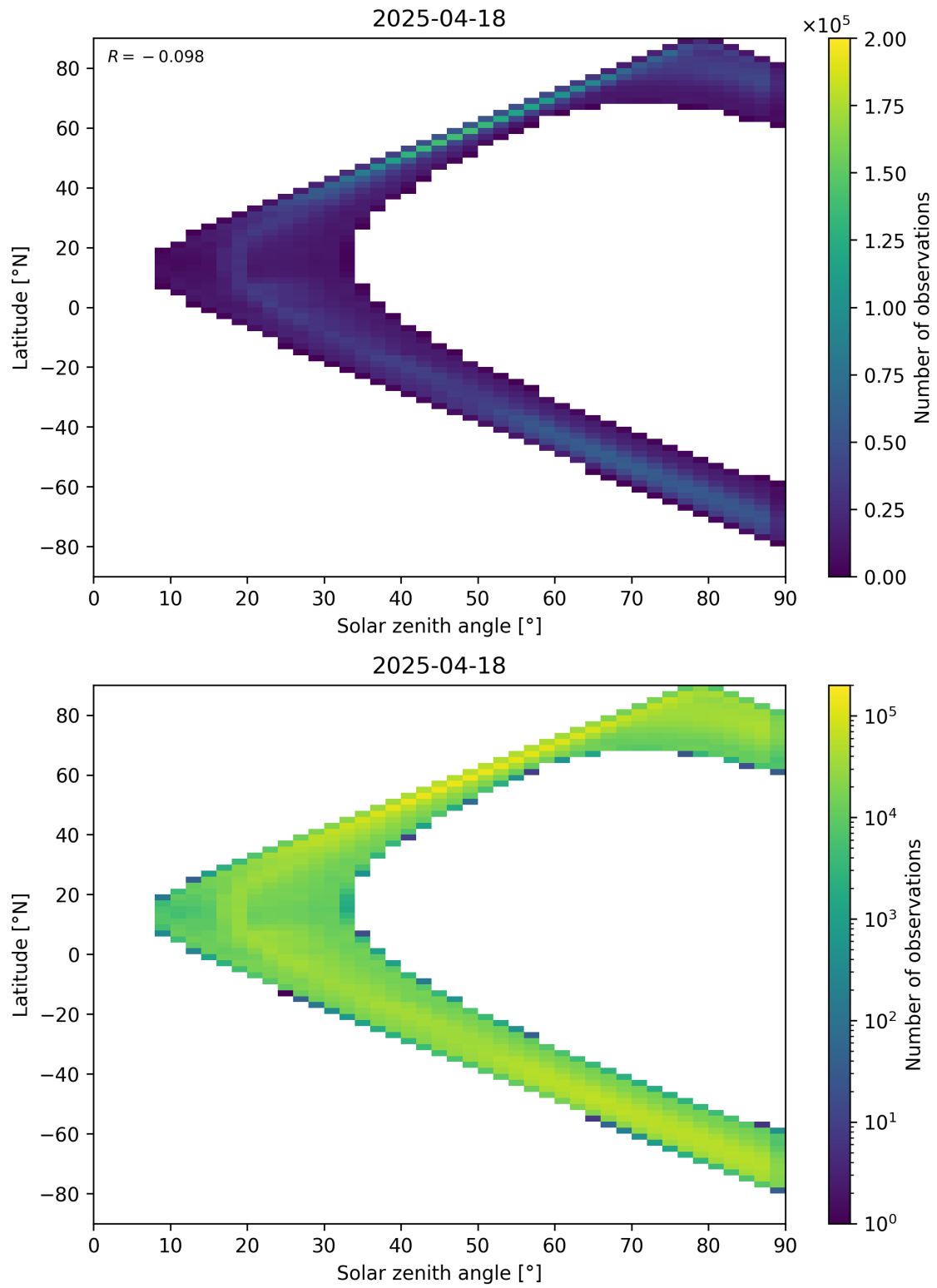
Figure 105: Scatter density plot of “Solar zenith angle” against “Latitude” for 2025-04-18 to 2025-04-19.
