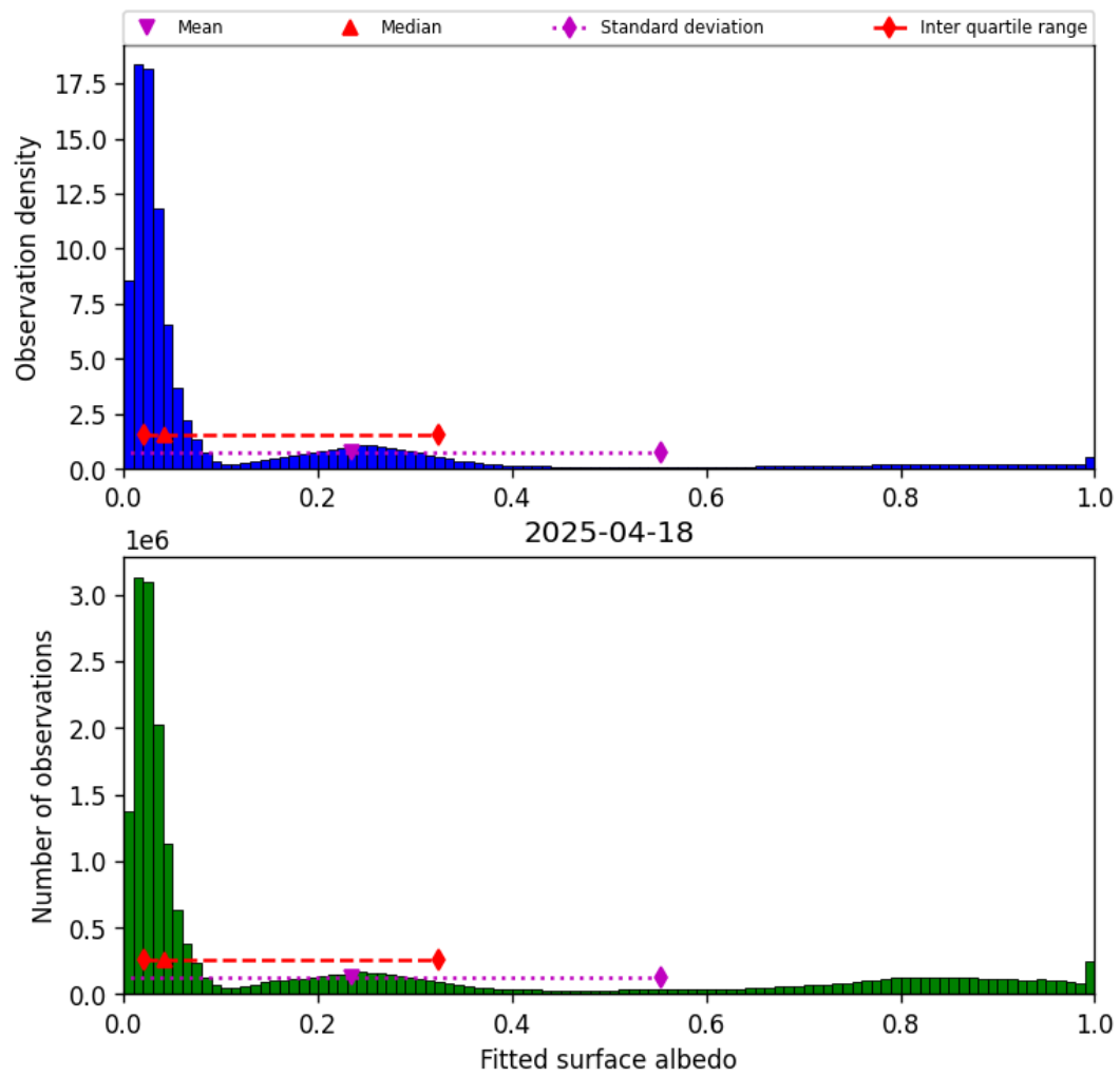
Figure 45: Histogram of “Fitted surface albedo” for 2025-04-18 to 2025-04-19
