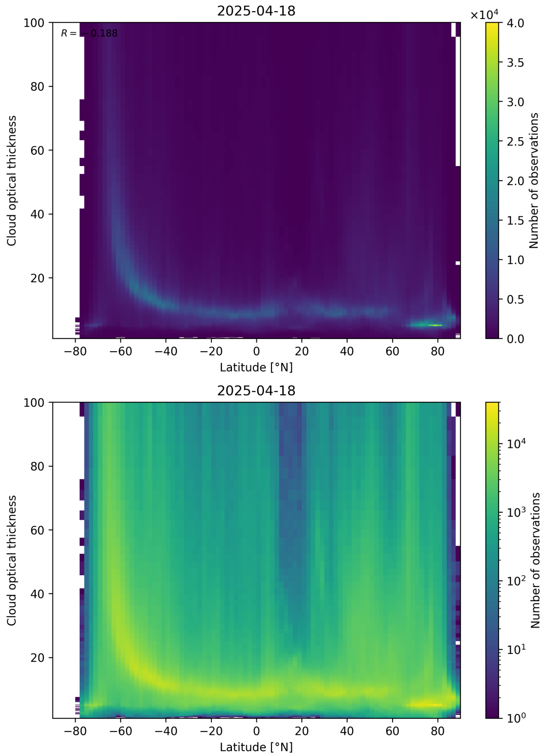
Figure 96: Scatter density plot of “Latitude” against “Cloud optical thickness” for 2025-04-18 to 2025-04-19.
