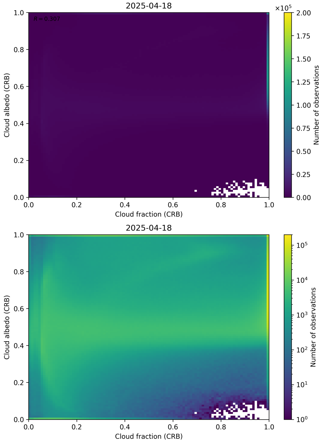
Figure 77: Scatter density plot of “Cloud fraction (CRB)” against “Cloud albedo (CRB)” for 2025-04-18 to 2025-04-19.
