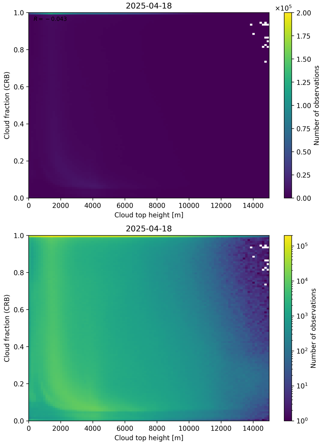
Figure 88: Scatter density plot of “Cloud top height” against “Cloud fraction (CRB)” for 2025-04-18 to 2025-04-19.
