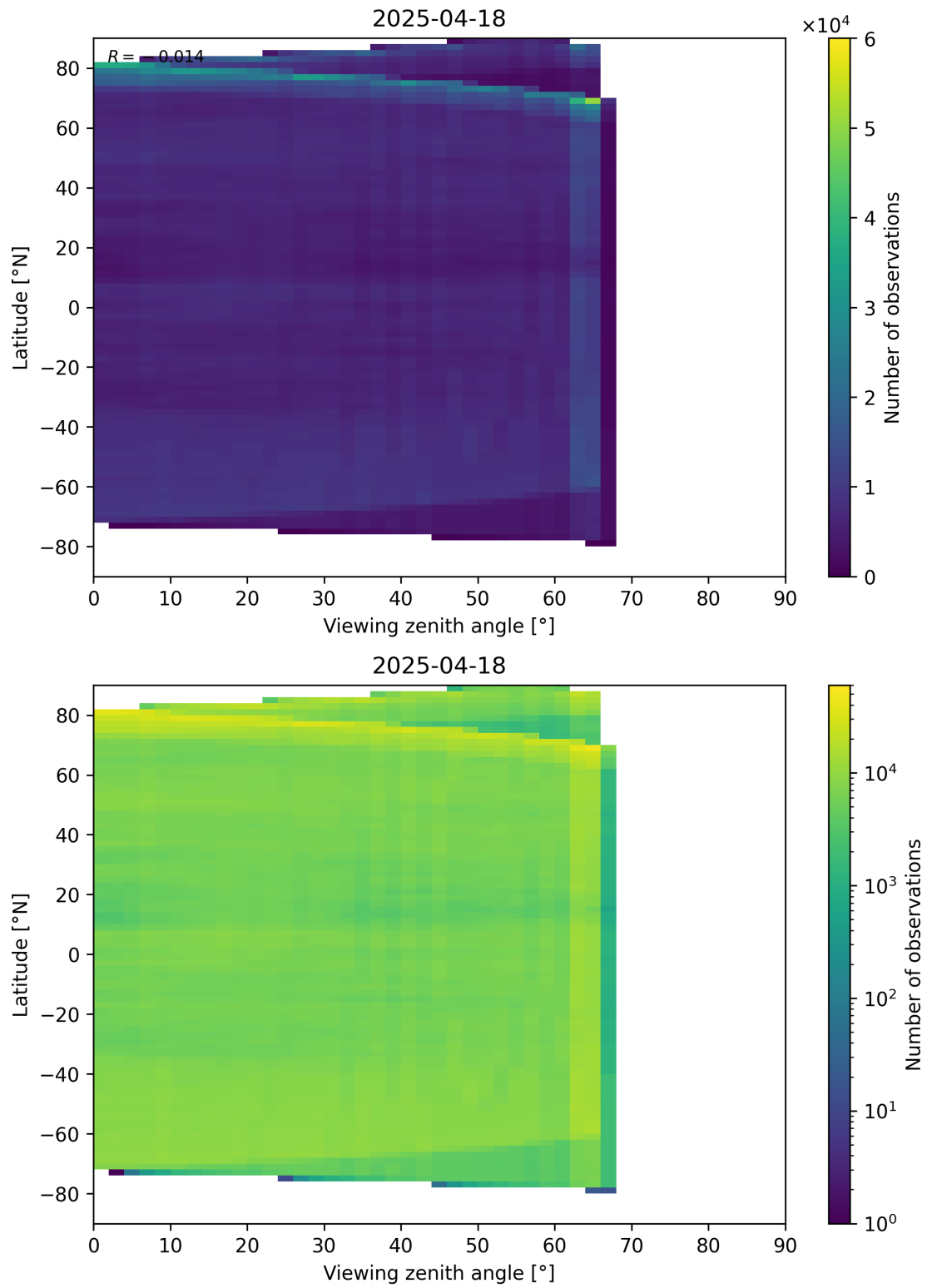
Figure 113: Scatter density plot of “Viewing zenith angle” against “Latitude” for 2025-04-18 to 2025-04-19.
