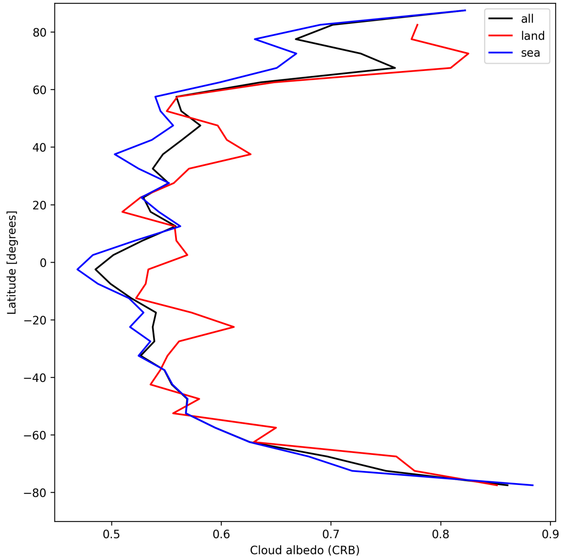
Figure 28: Zonal average of “Cloud albedo (CRB)” for 2025-04-18 to 2025-04-19.
