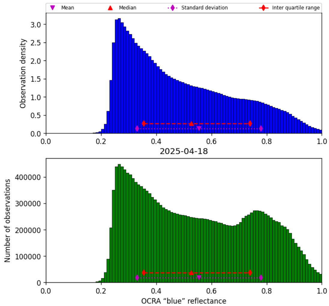
Figure 51: Histogram of “OCRA “blue” reflectance” for 2025-04-18 to 2025-04-19
