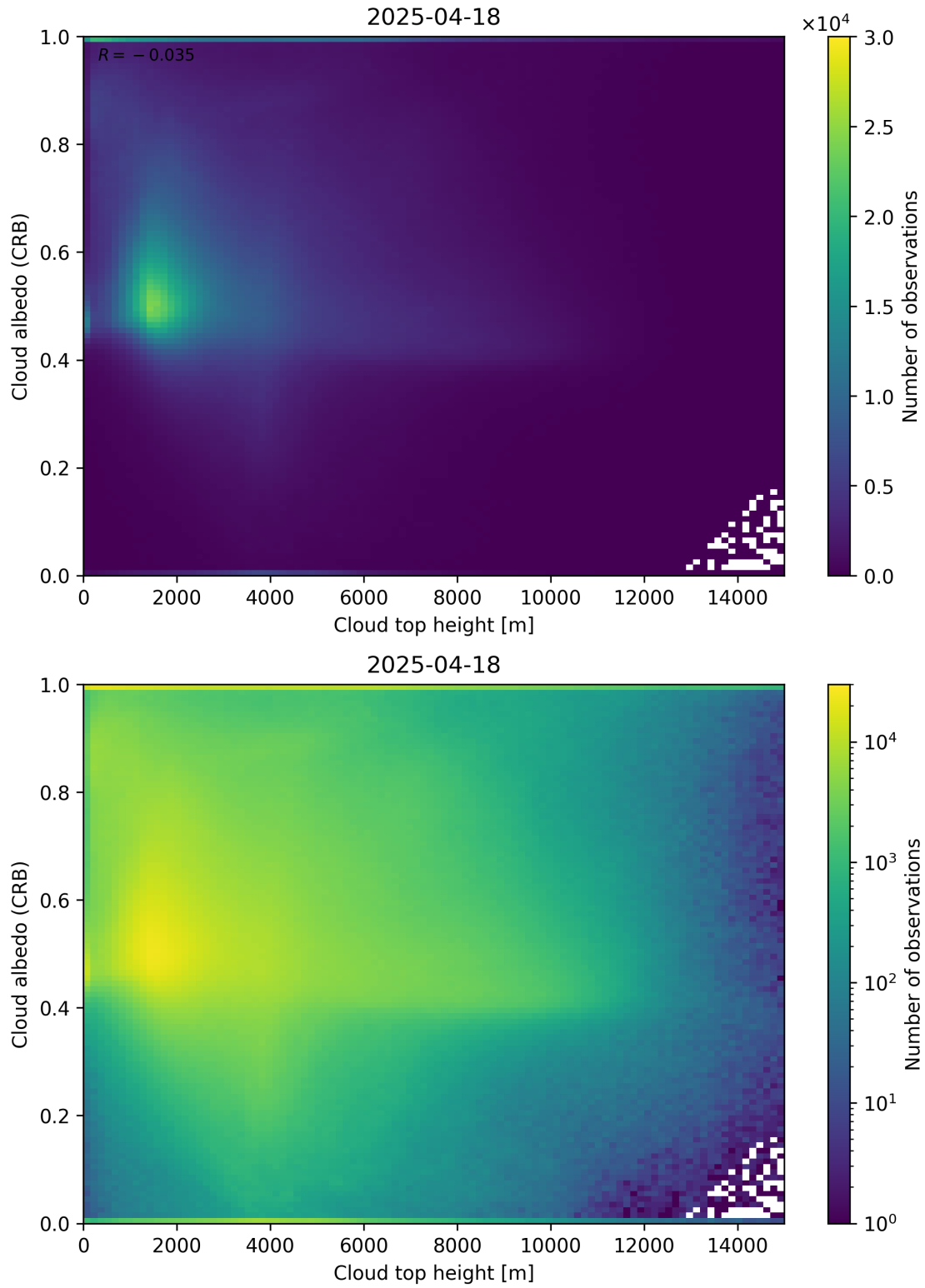
Figure 86: Scatter density plot of “Cloud top height” against “Cloud albedo (CRB)” for 2025-04-18 to 2025-04-19.
