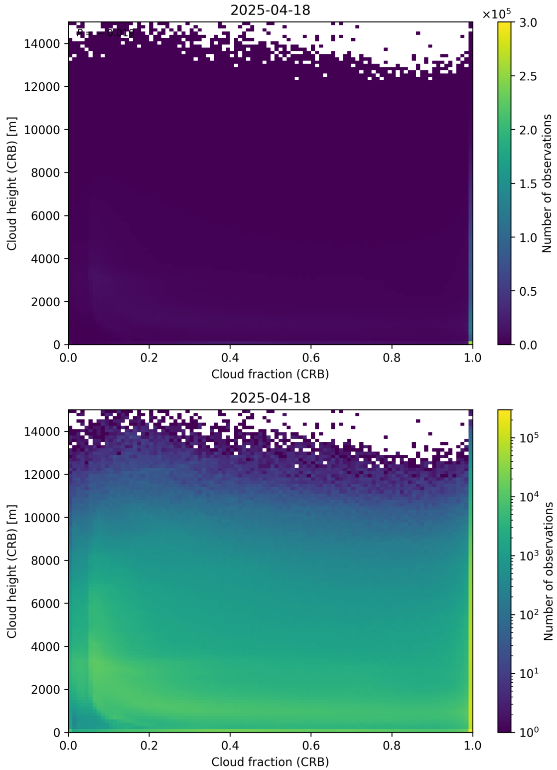
Figure 79: Scatter density plot of “Cloud fraction (CRB)” against “Cloud height (CRB)” for 2025-04-18 to 2025-04-19.
