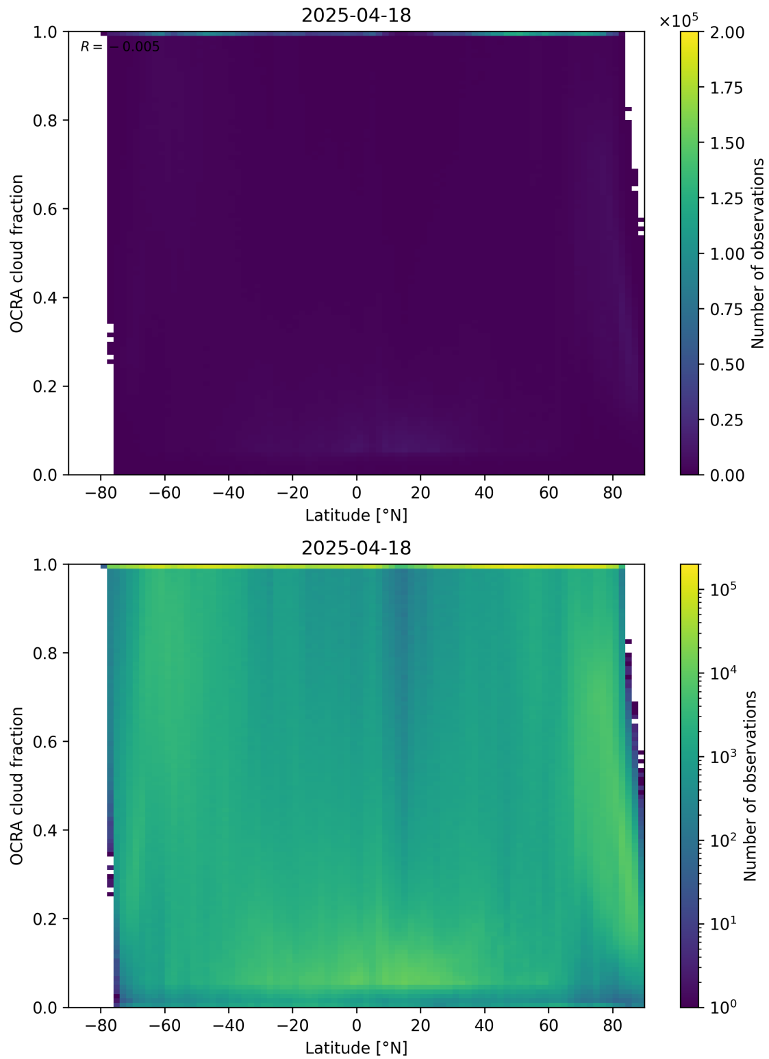
Figure 93: Scatter density plot of “Latitude” against “OCRA cloud fraction” for 2025-04-18 to 2025-04-19.
