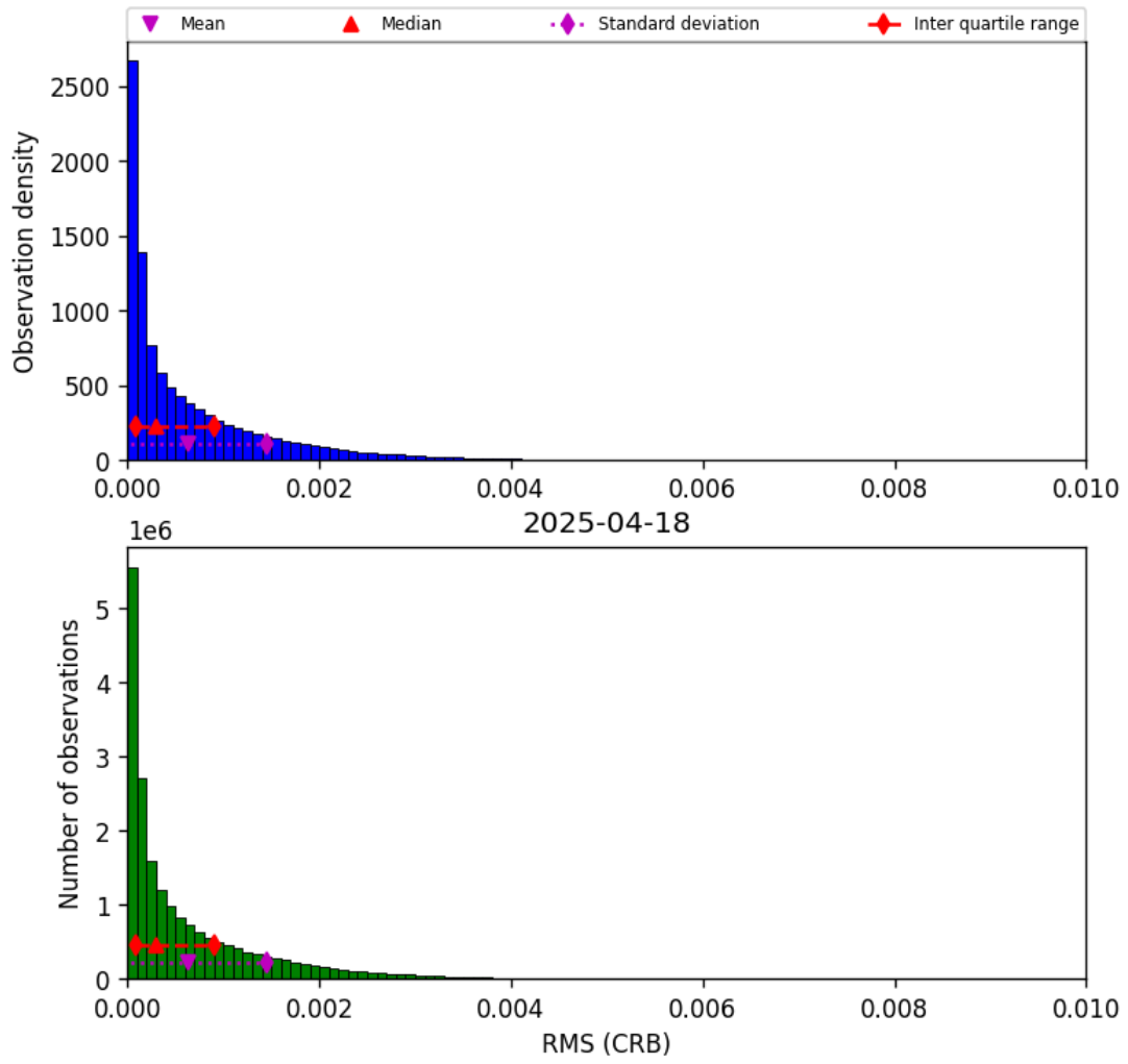
Figure 48: Histogram of “RMS (CRB)” for 2025-04-18 to 2025-04-19
