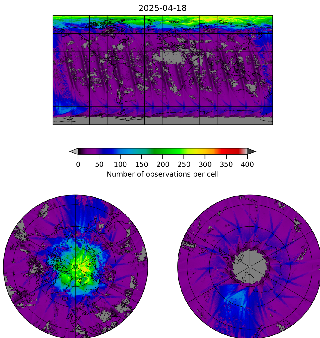
Figure 21: Map of the number of observations for 2025-04-18 to 2025-04-19
