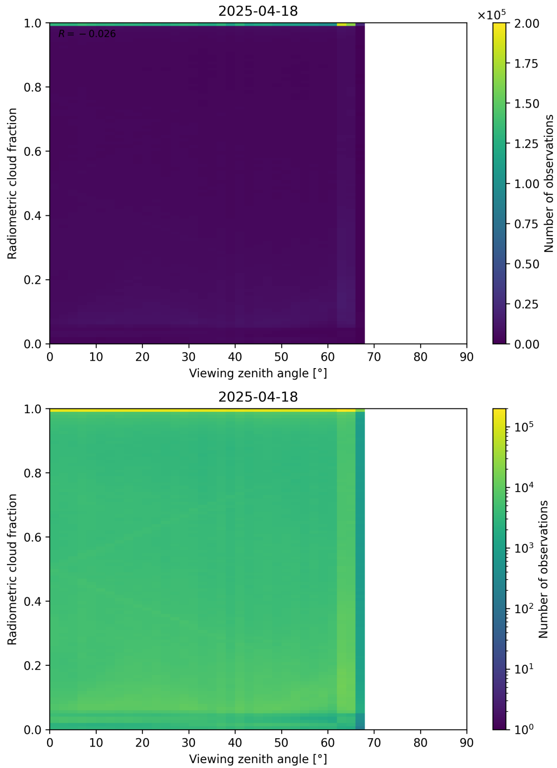
Figure 107: Scatter density plot of “Viewing zenith angle” against “Radiometric cloud fraction” for 2025-04-18 to 2025-04-19.
