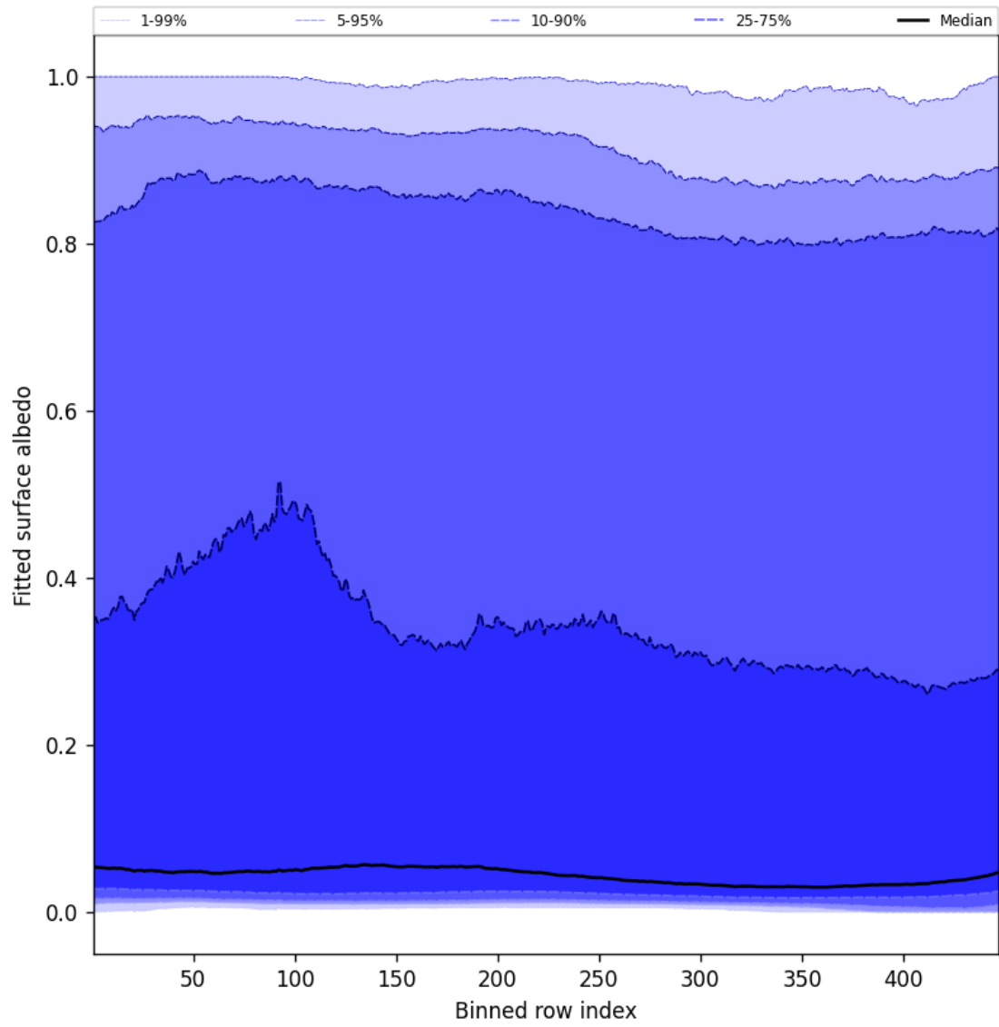
Figure 61: Along track statistics of “Fitted surface albedo” for 2025-04-18 to 2025-04-19
