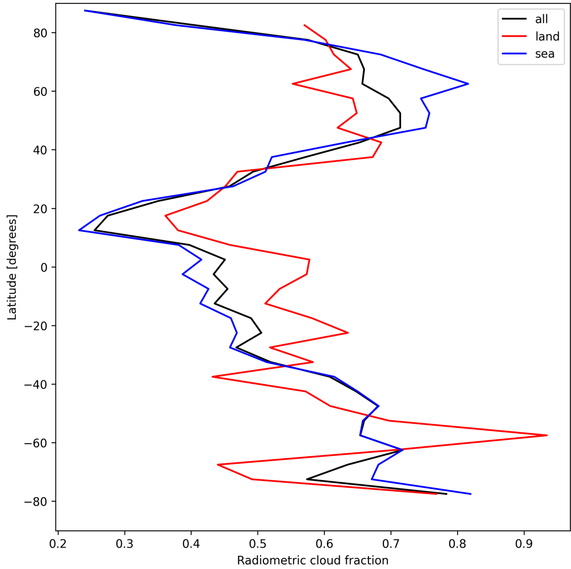
Figure 23: Zonal average of “Radiometric cloud fraction” for 2025-04-18 to 2025-04-19.
