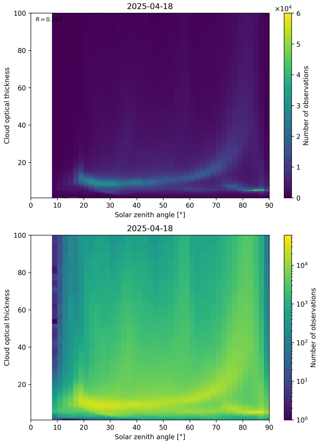
Figure 103: Scatter density plot of “Solar zenith angle” against “Cloud optical thickness” for 2025-04-18 to 2025-04-19.
