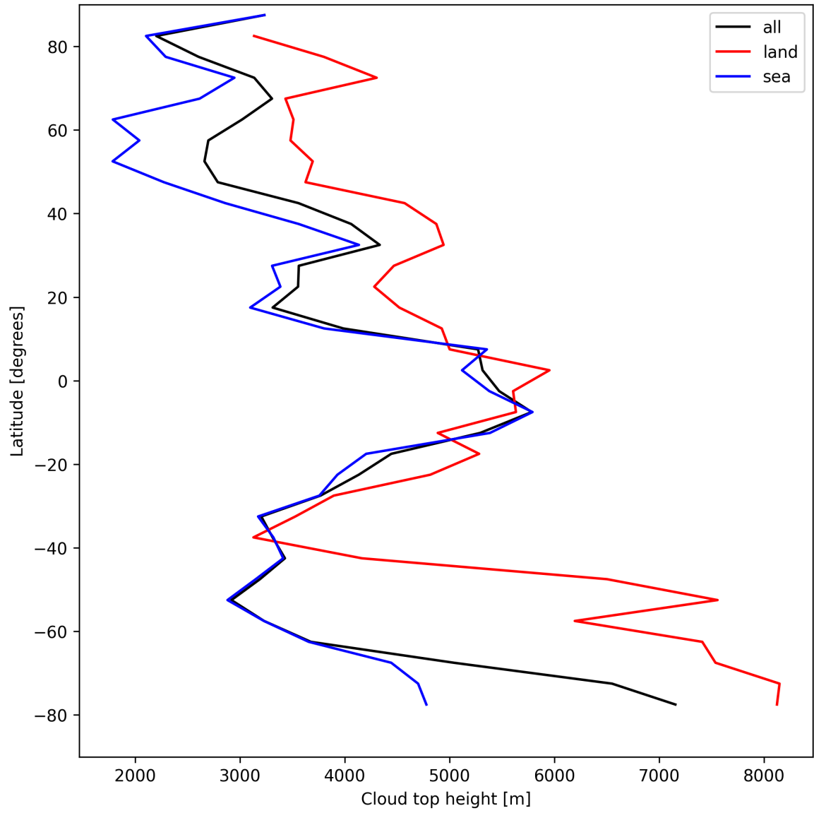
Figure 24: Zonal average of “Cloud top height” for 2025-04-18 to 2025-04-19.
