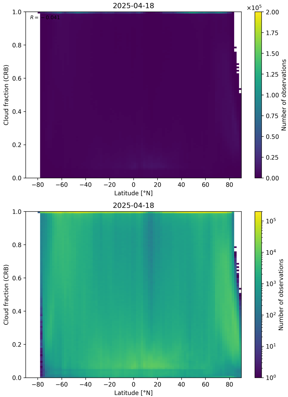
Figure 94: Scatter density plot of “Latitude” against “Cloud fraction (CRB)” for 2025-04-18 to 2025-04-19.
