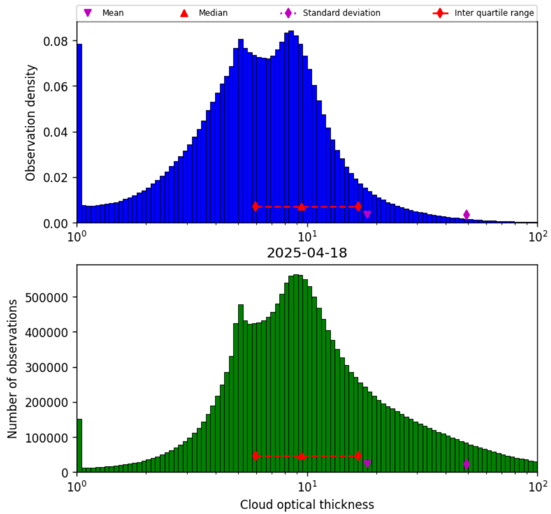
Figure 41: Histogram of “Cloud optical thickness” for 2025-04-18 to 2025-04-19
