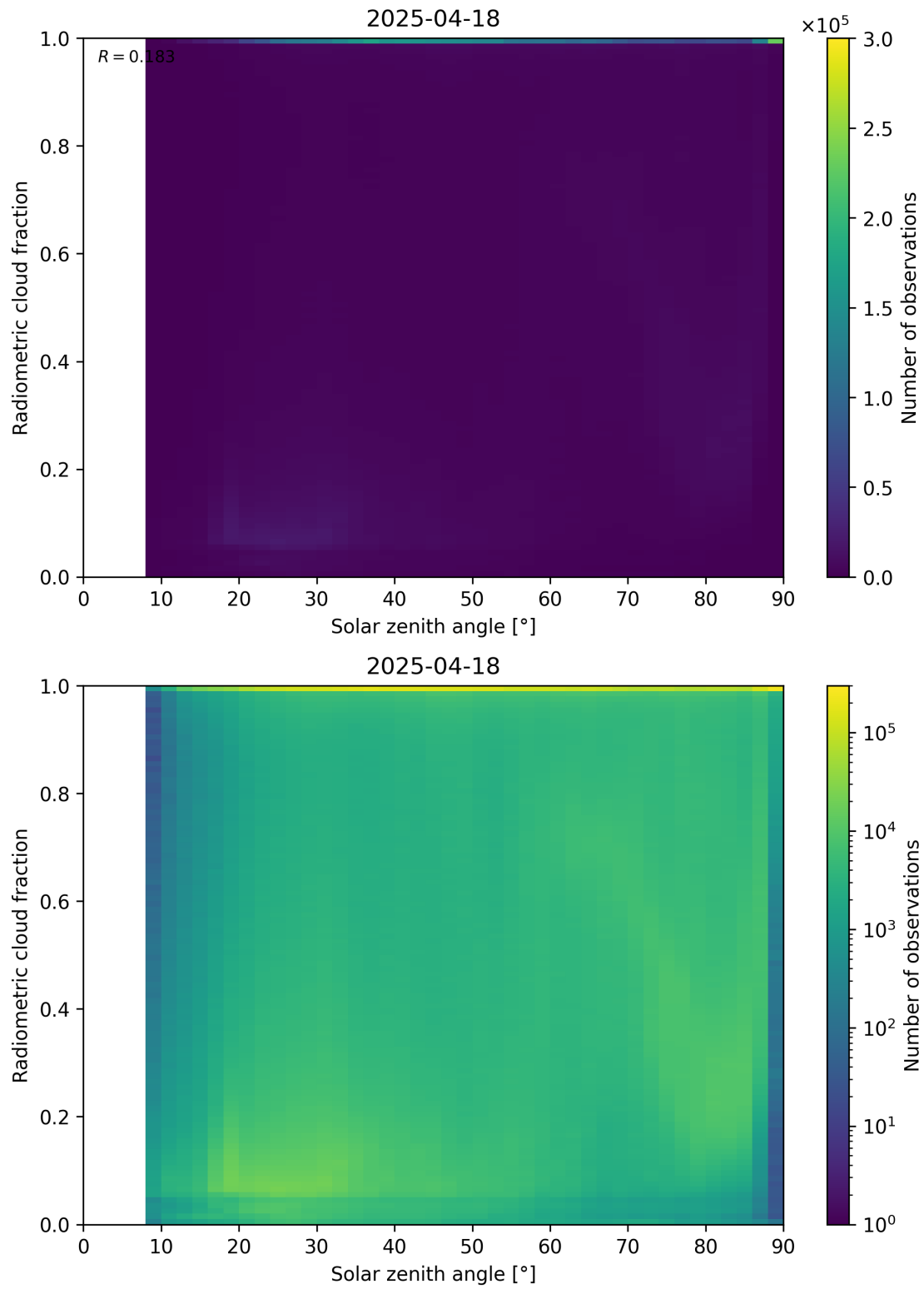
Figure 99: Scatter density plot of “Solar zenith angle” against “Radiometric cloud fraction” for 2025-04-18 to 2025-04-19.
