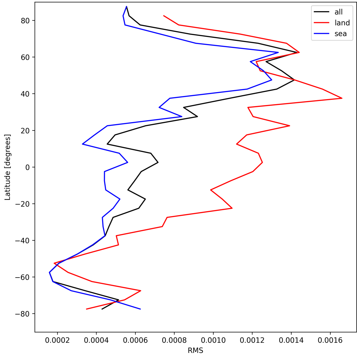
Figure 31: Zonal average of “RMS” for 2025-04-18 to 2025-04-19.
