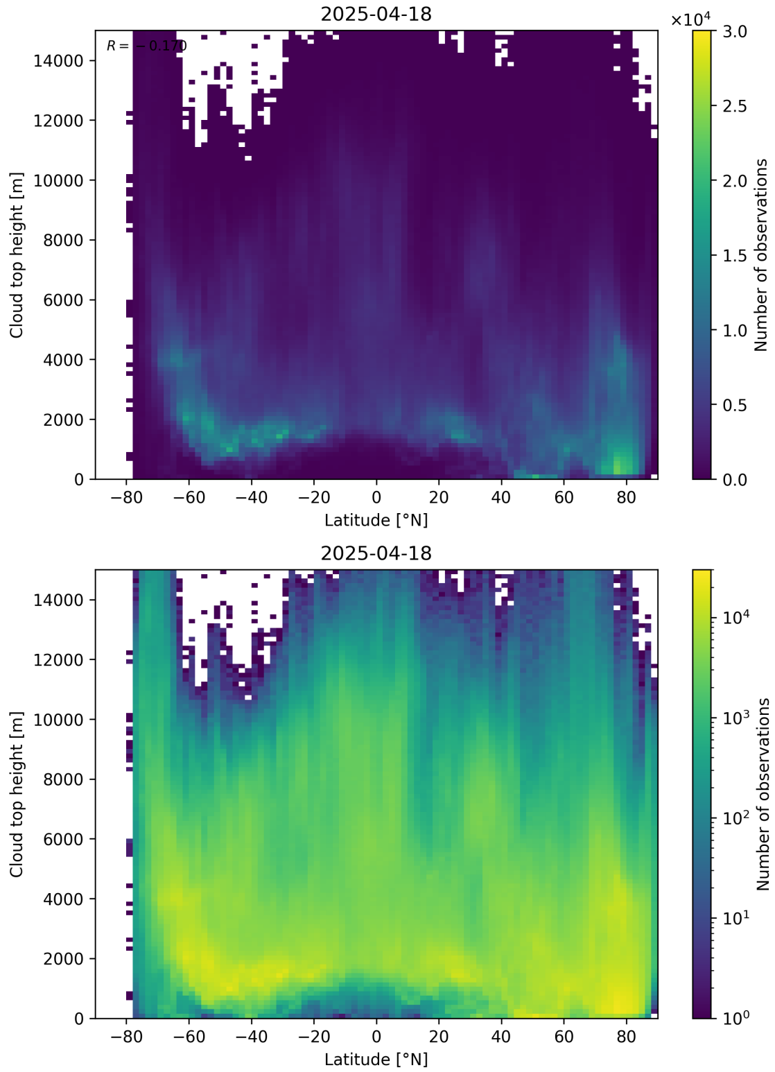
Figure 97: Scatter density plot of “Latitude” against “Cloud top height” for 2025-04-18 to 2025-04-19.
