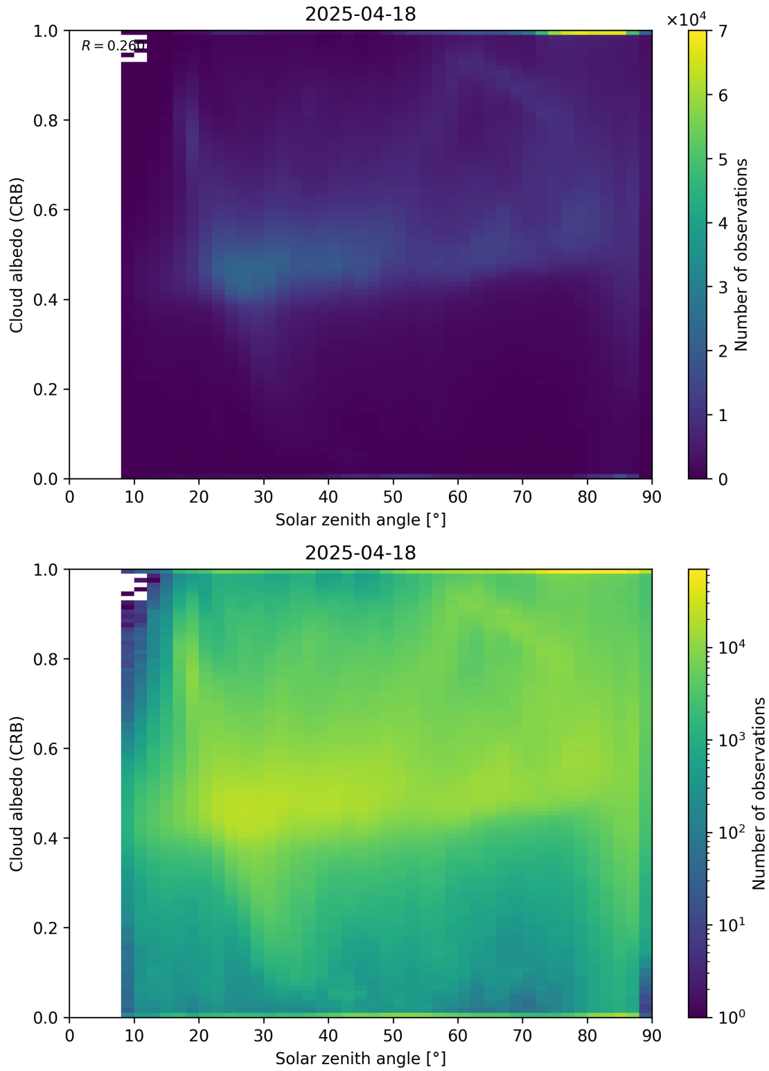
Figure 98: Scatter density plot of “Solar zenith angle” against “Cloud albedo (CRB)” for 2025-04-18 to 2025-04-19.
