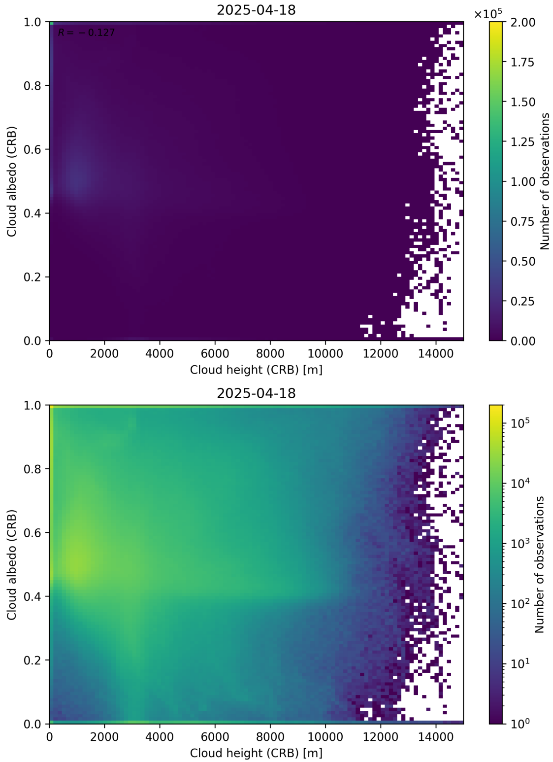
Figure 80: Scatter density plot of “Cloud height (CRB)” against “Cloud albedo (CRB)” for 2025-04-18 to 2025-04-19.
