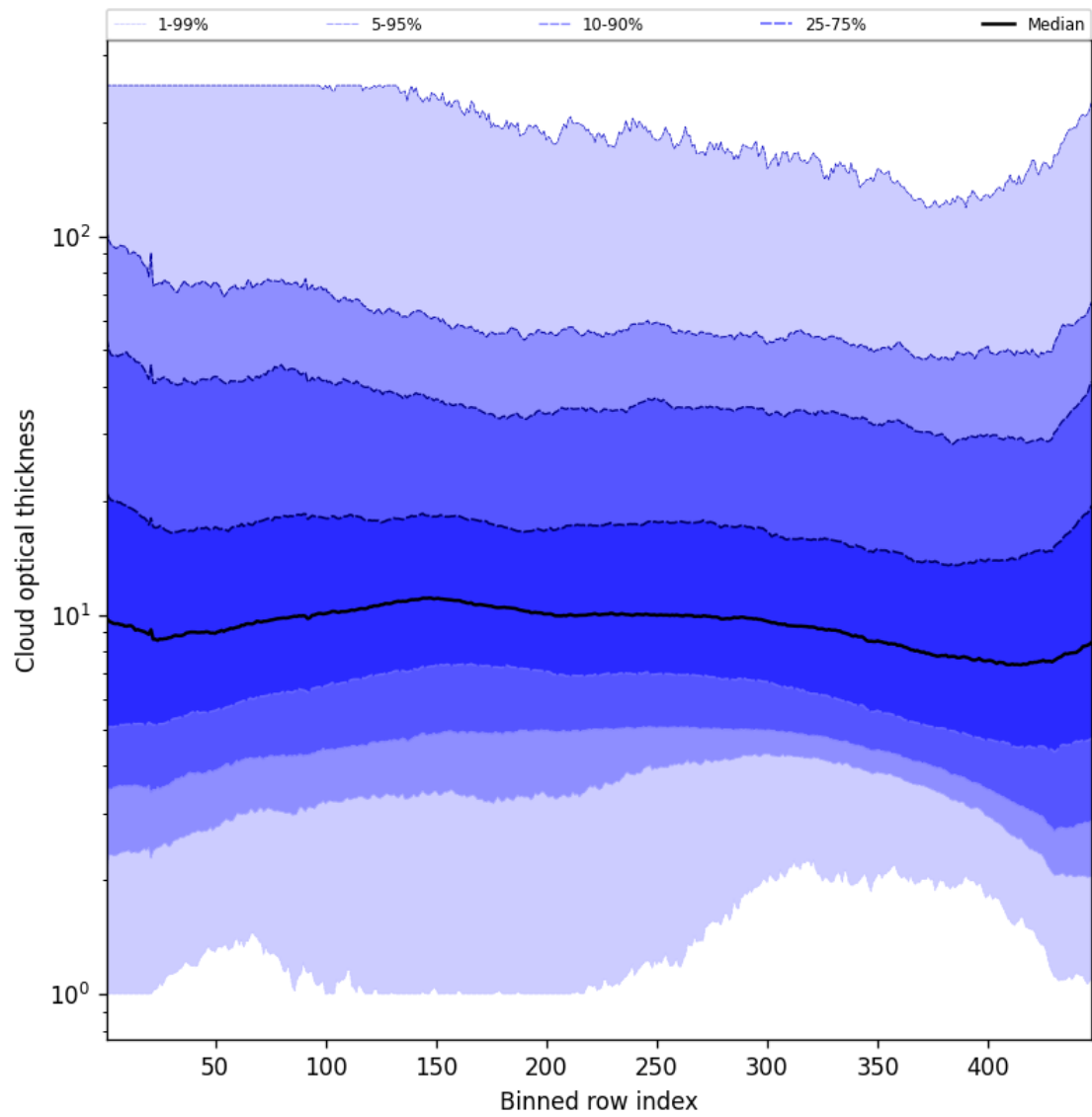
Figure 57: Along track statistics of “Cloud optical thickness” for 2025-04-18 to 2025-04-19
