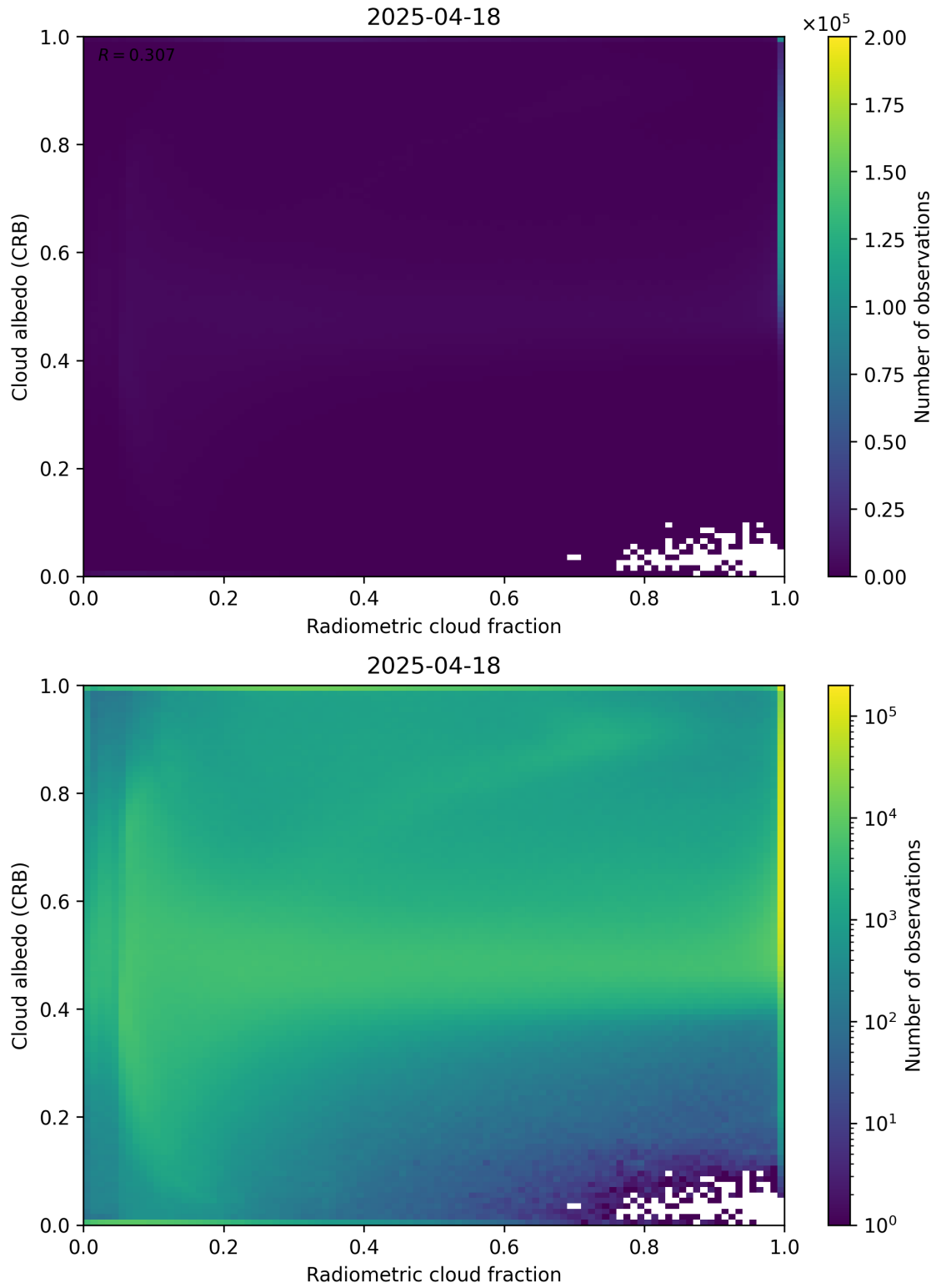
Figure 71: Scatter density plot of “Radiometric cloud fraction” against “Cloud albedo (CRB)” for 2025-04-18 to 2025-04-19.
