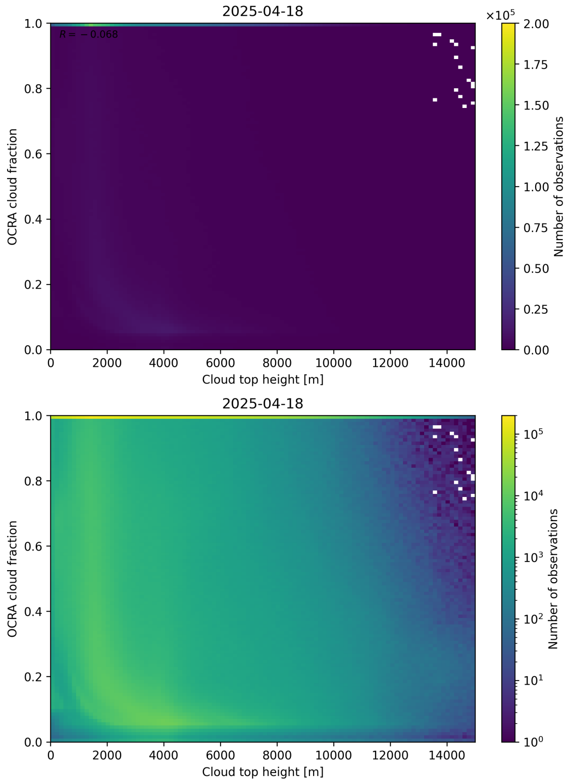
Figure 87: Scatter density plot of “Cloud top height” against “OCRA cloud fraction” for 2025-04-18 to 2025-04-19.
