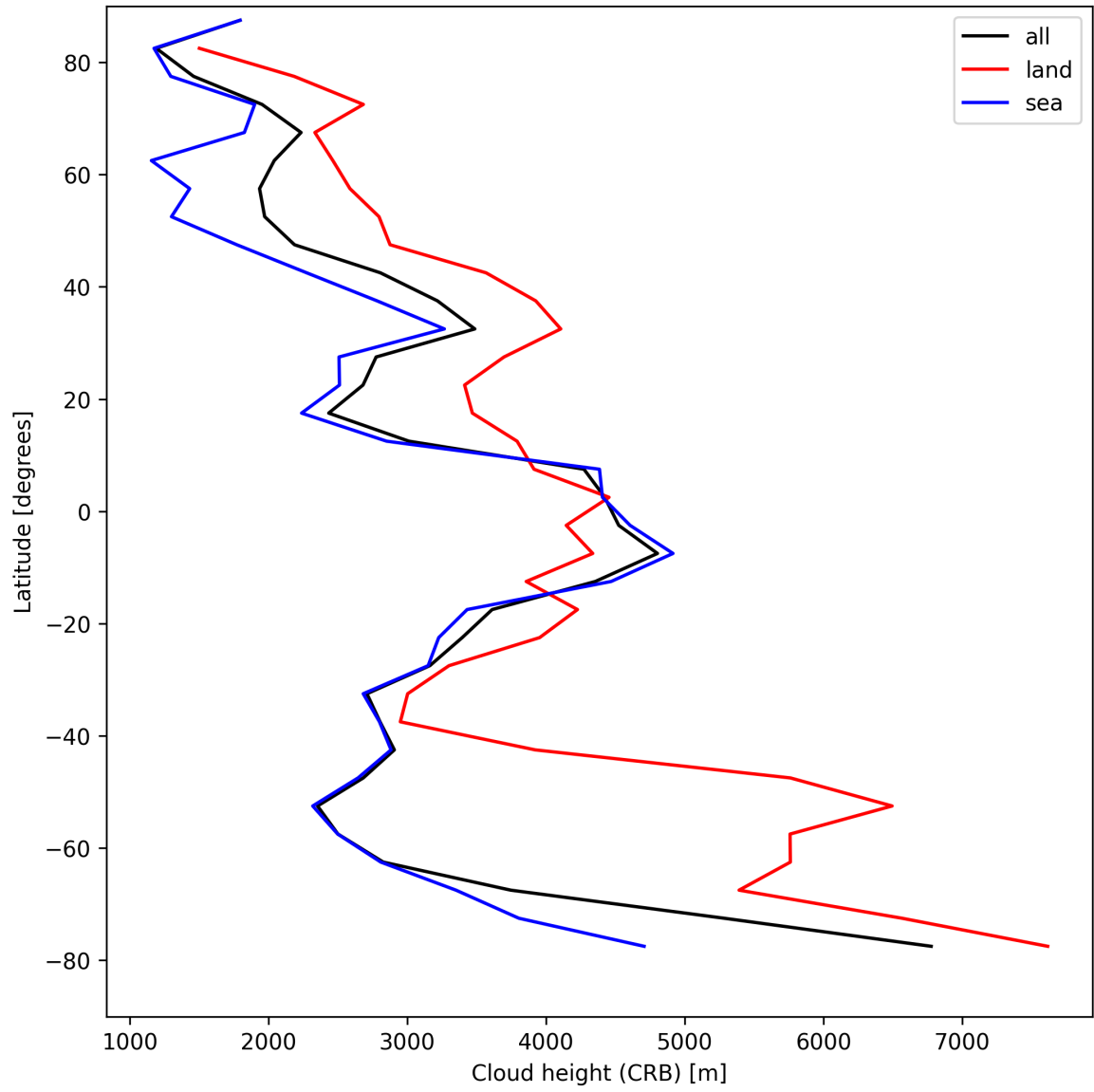
Figure 27: Zonal average of “Cloud height (CRB)” for 2025-04-18 to 2025-04-19.
