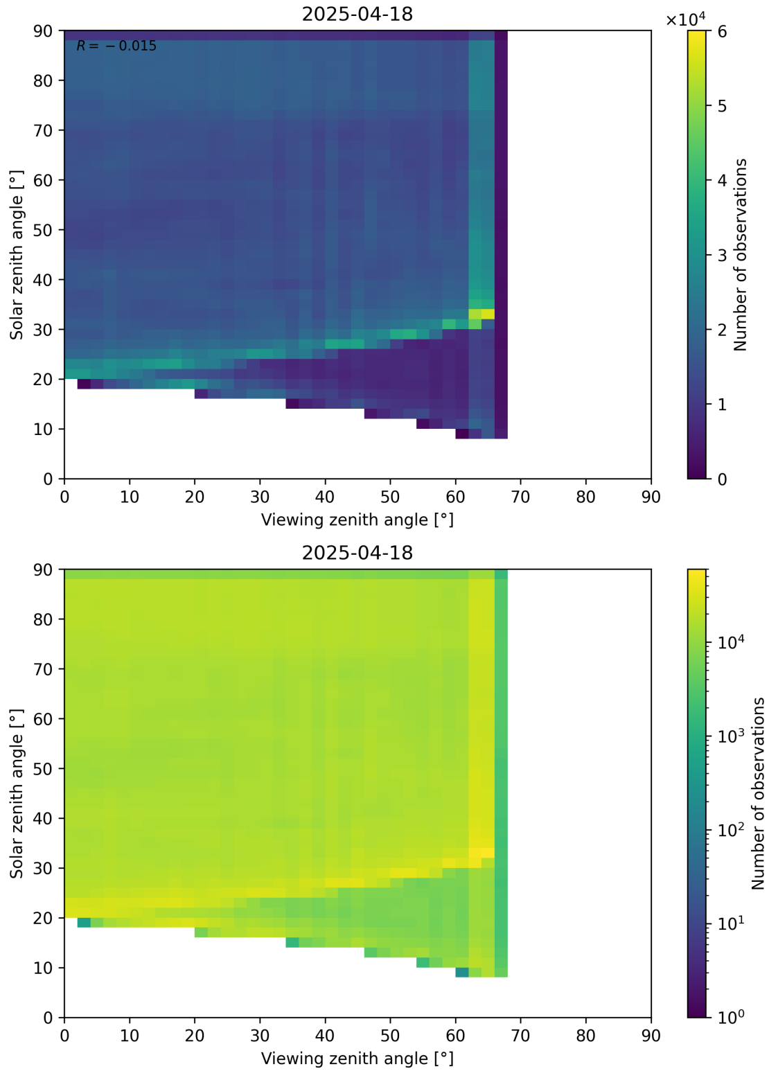
Figure 114: Scatter density plot of “Viewing zenith angle” against “Solar zenith angle” for 2025-04-18 to 2025-04-19.
