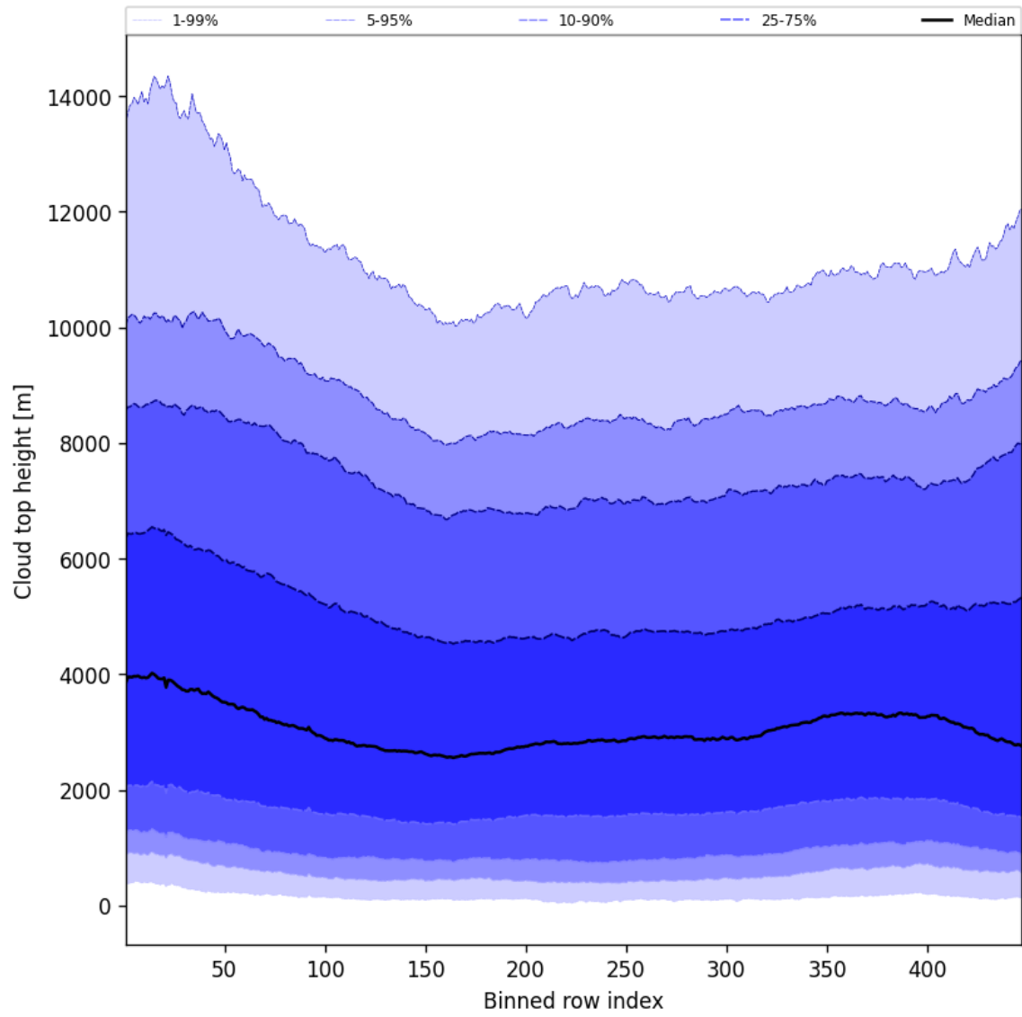
Figure 56: Along track statistics of “Cloud top height” for 2025-04-18 to 2025-04-19
