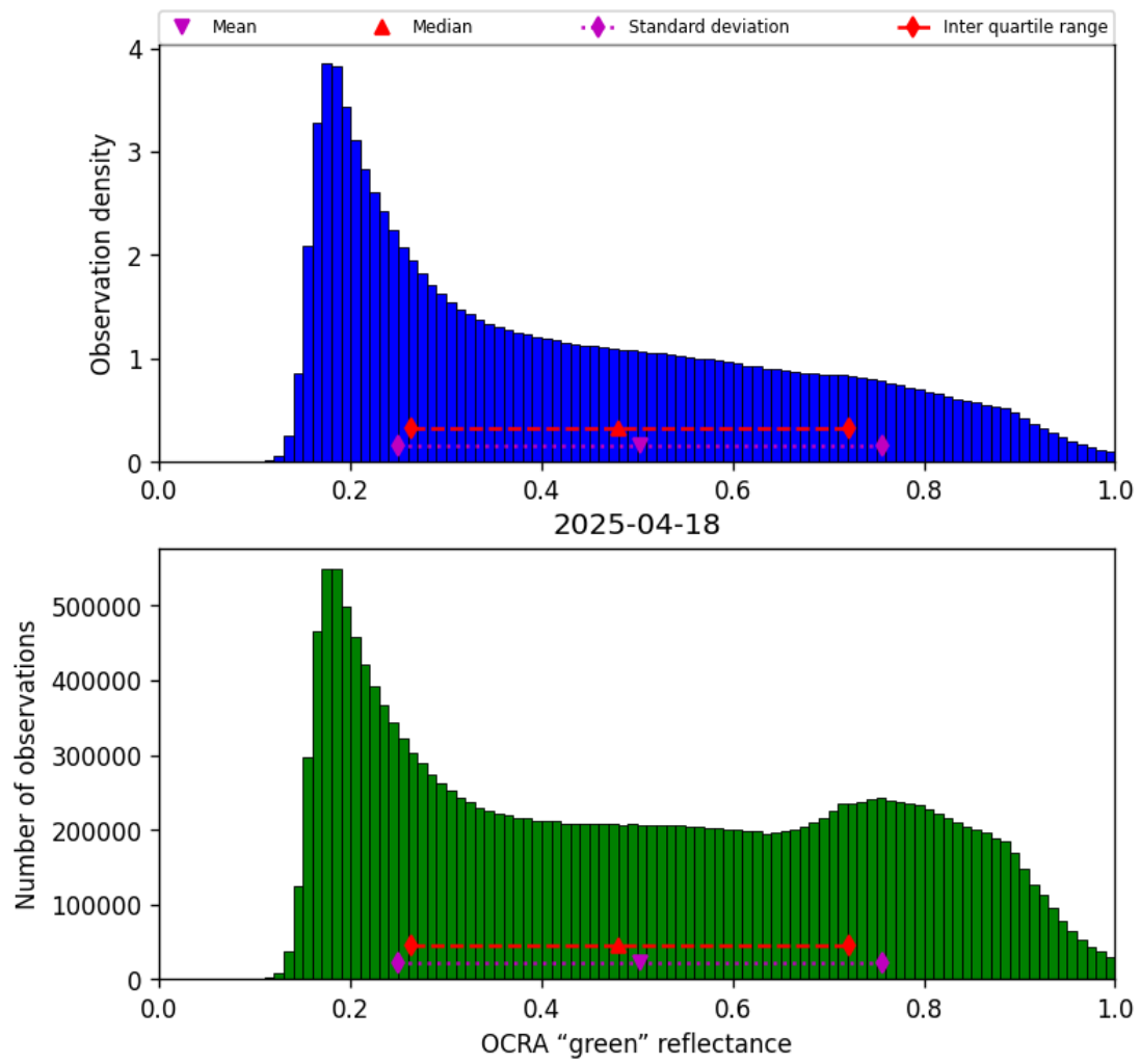
Figure 52: Histogram of “OCRA “green” reflectance” for 2025-04-18 to 2025-04-19
