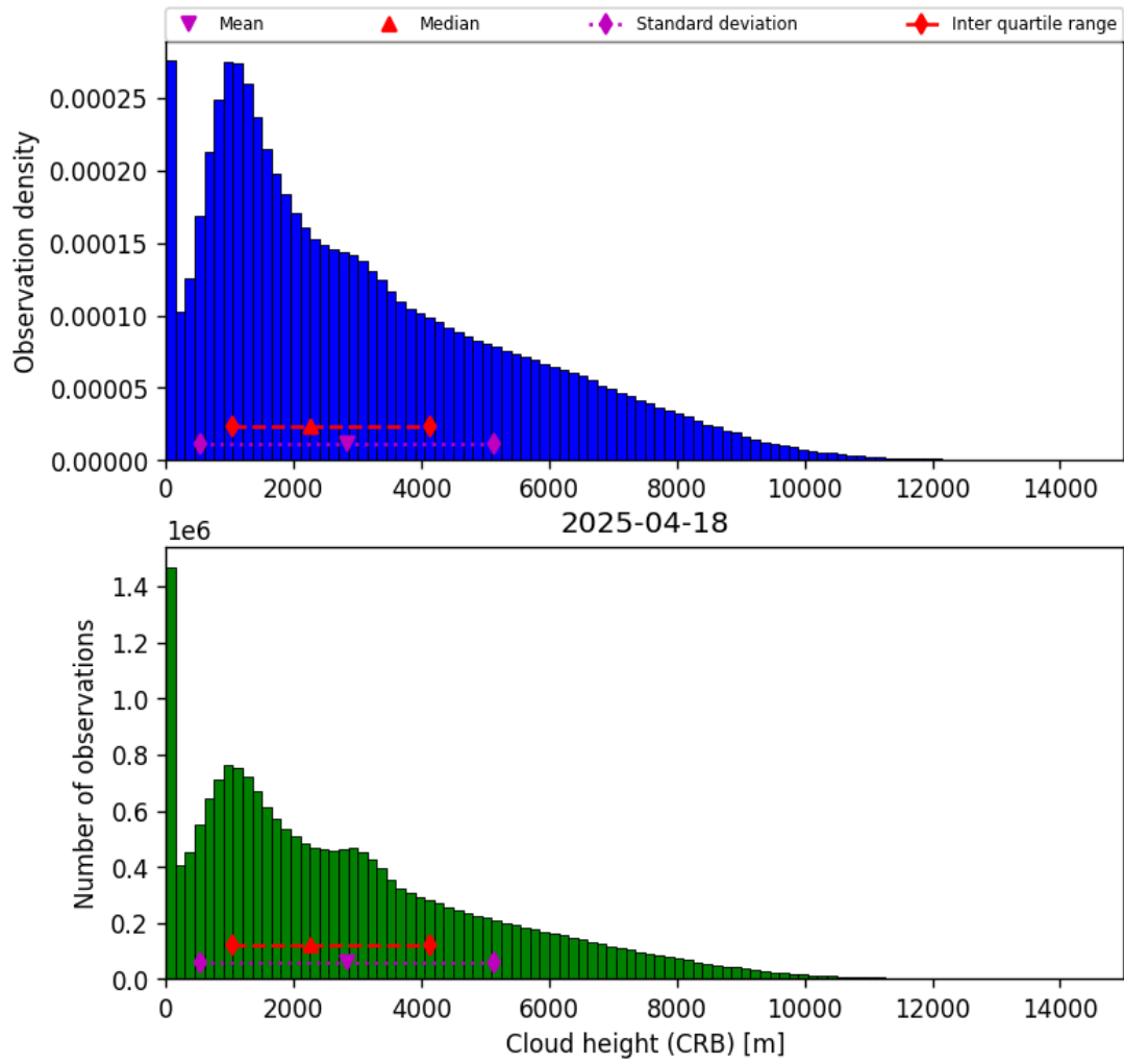
Figure 43: Histogram of “Cloud height (CRB)” for 2025-04-18 to 2025-04-19
