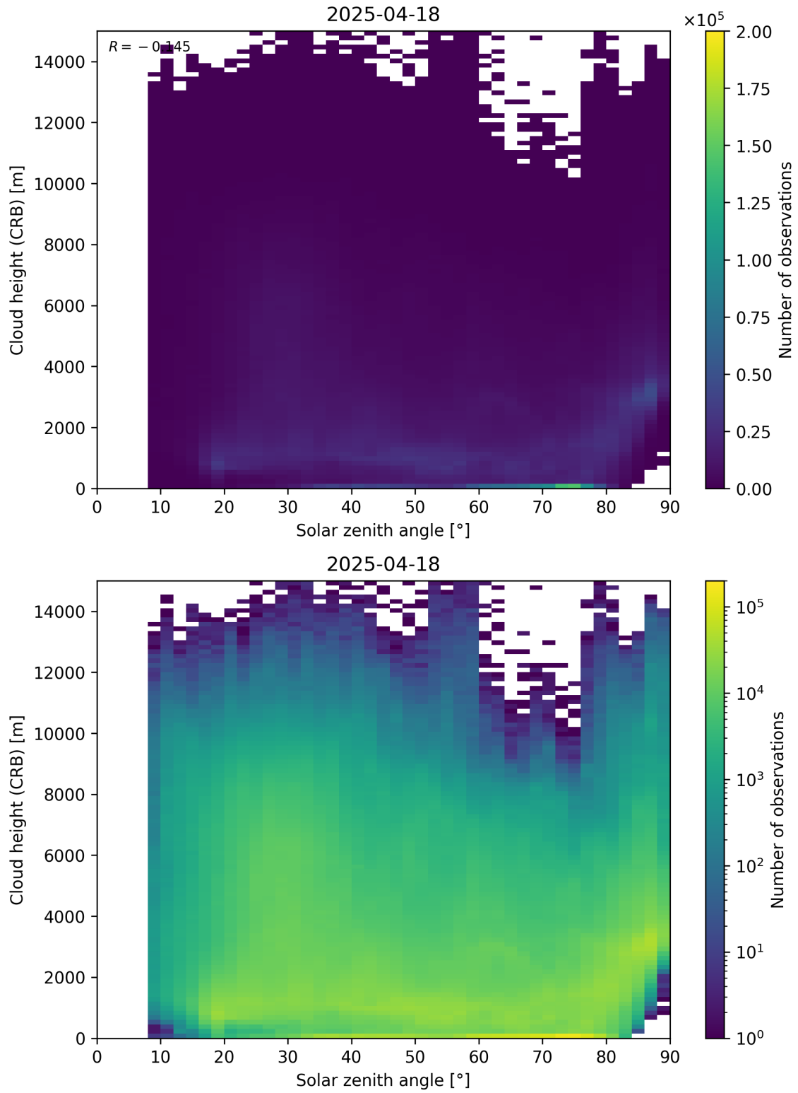
Figure 102: Scatter density plot of “Solar zenith angle” against “Cloud height (CRB)” for 2025-04-18 to 2025-04-19.
