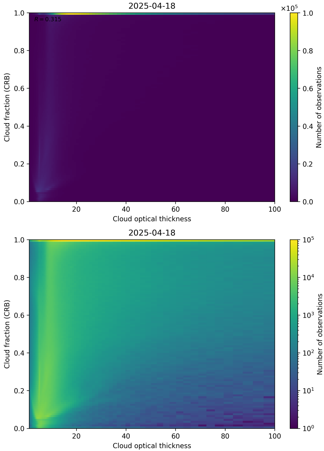
Figure 84: Scatter density plot of “Cloud optical thickness” against “Cloud fraction (CRB)” for 2025-04-18 to 2025-04-19.
