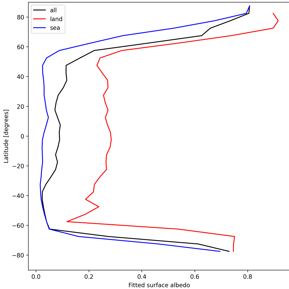
Figure 29: Zonal average of “Fitted surface albedo” for 2025-04-18 to 2025-04-19.
