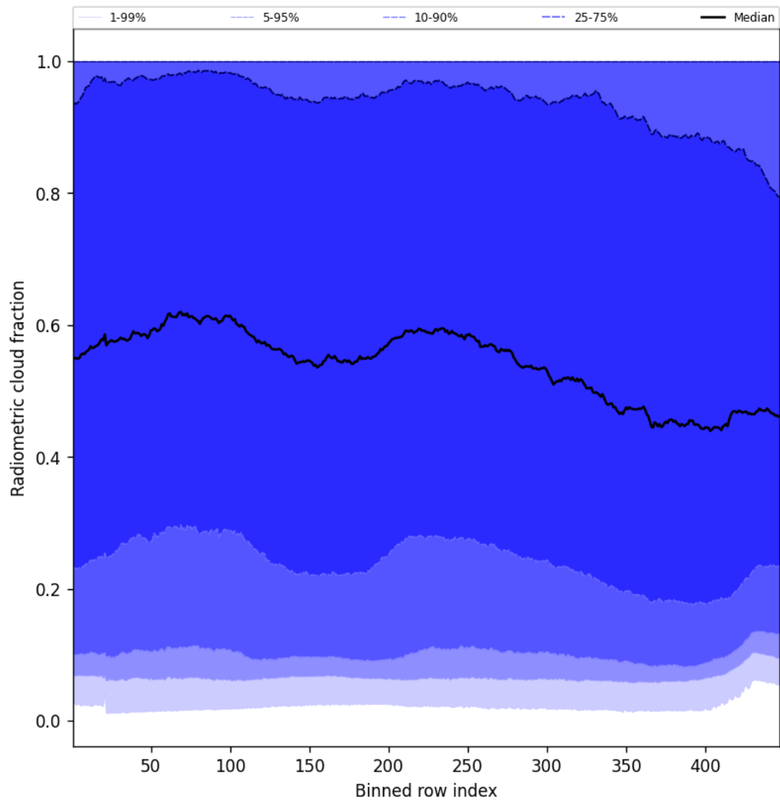
Figure 55: Along track statistics of “Radiometric cloud fraction” for 2025-04-18 to 2025-04-19
