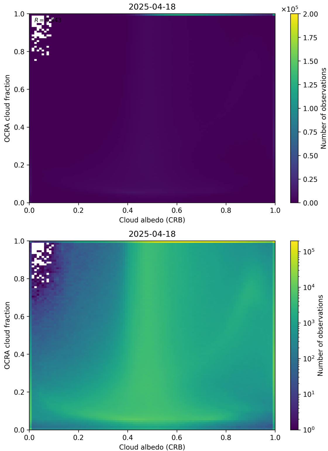
Figure 70: Scatter density plot of “Cloud albedo (CRB)” against “OCRA cloud fraction” for 2025-04-18 to 2025-04-19.
