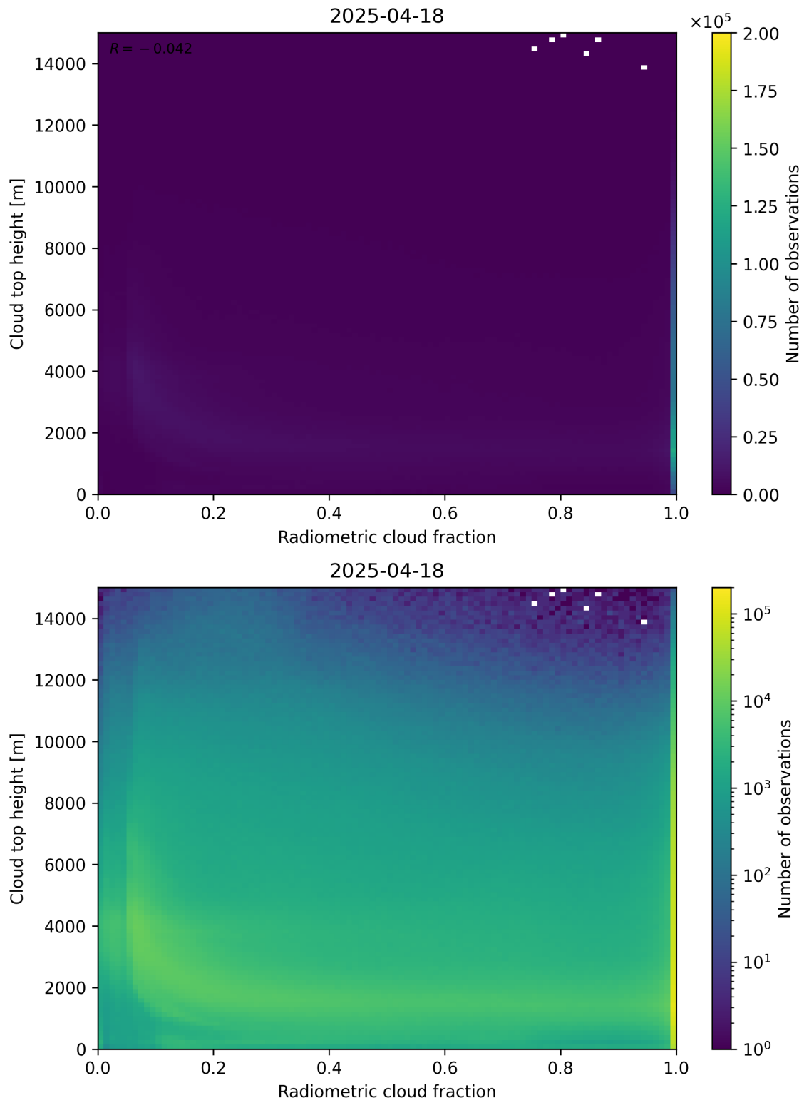
Figure 76: Scatter density plot of “Radiometric cloud fraction” against “Cloud top height” for 2025-04-18 to 2025-04-19.
