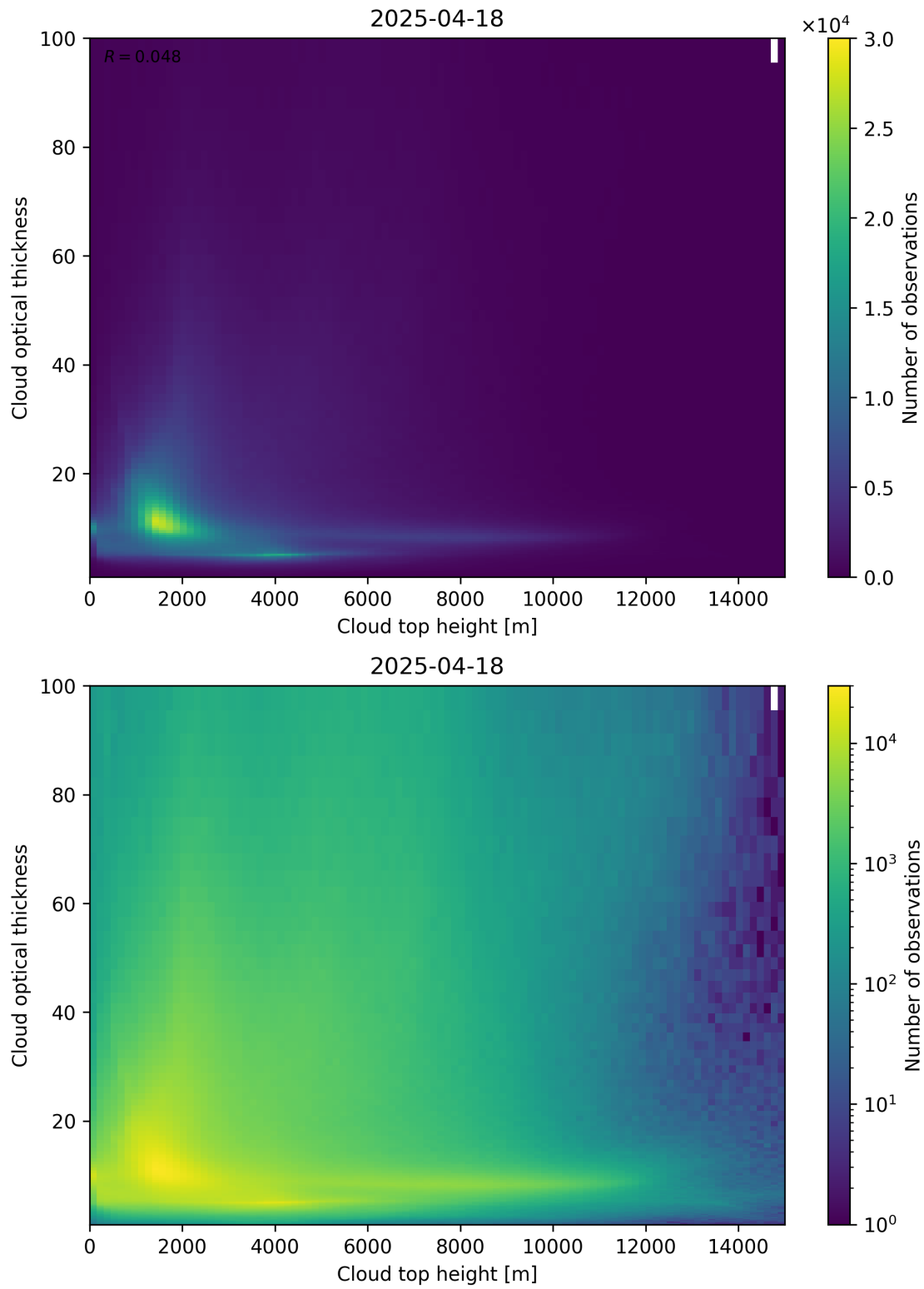
Figure 90: Scatter density plot of “Cloud top height” against “Cloud optical thickness” for 2025-04-18 to 2025-04-19.
