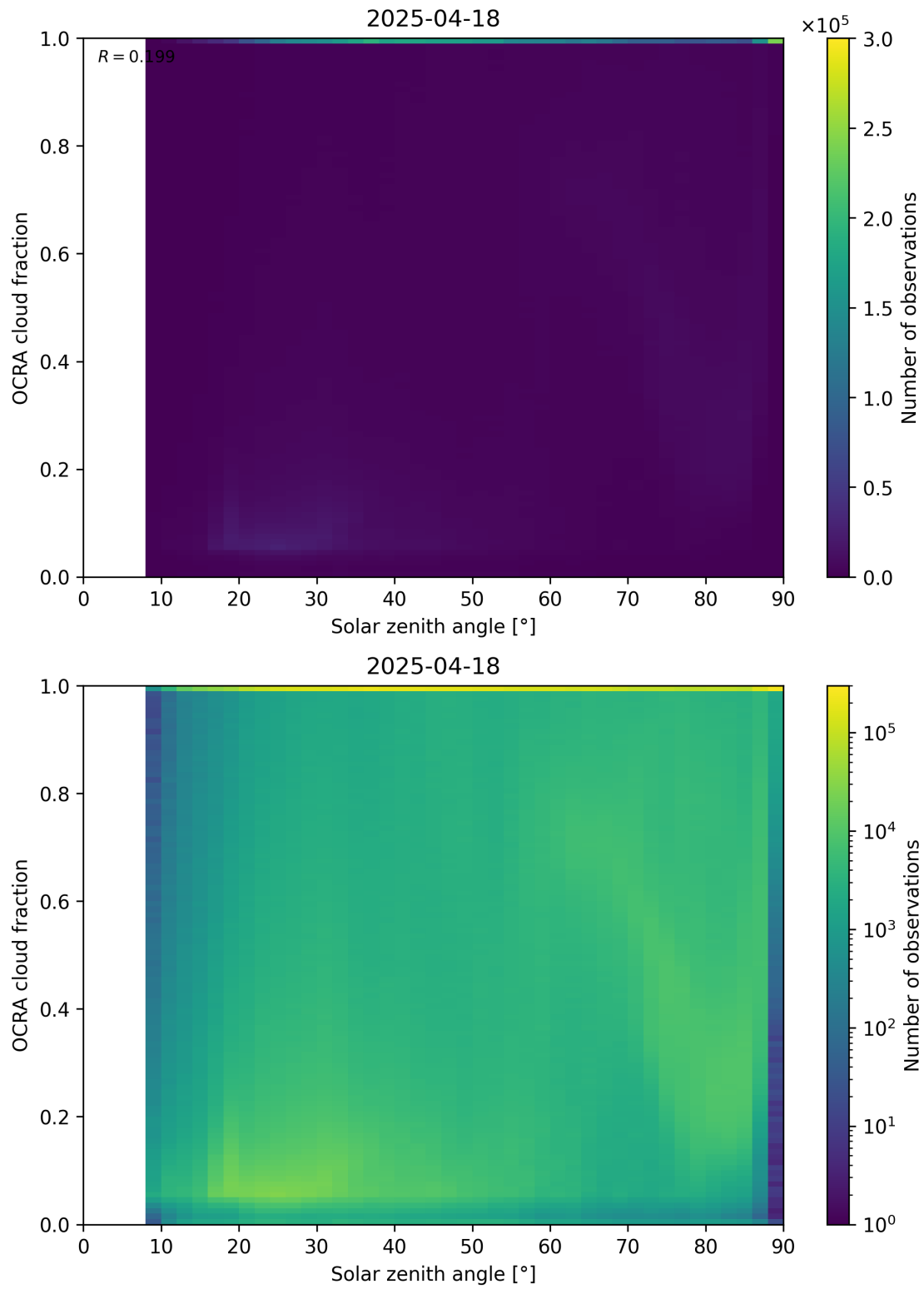
Figure 100: Scatter density plot of “Solar zenith angle” against “OCRA cloud fraction” for 2025-04-18 to 2025-04-19.
