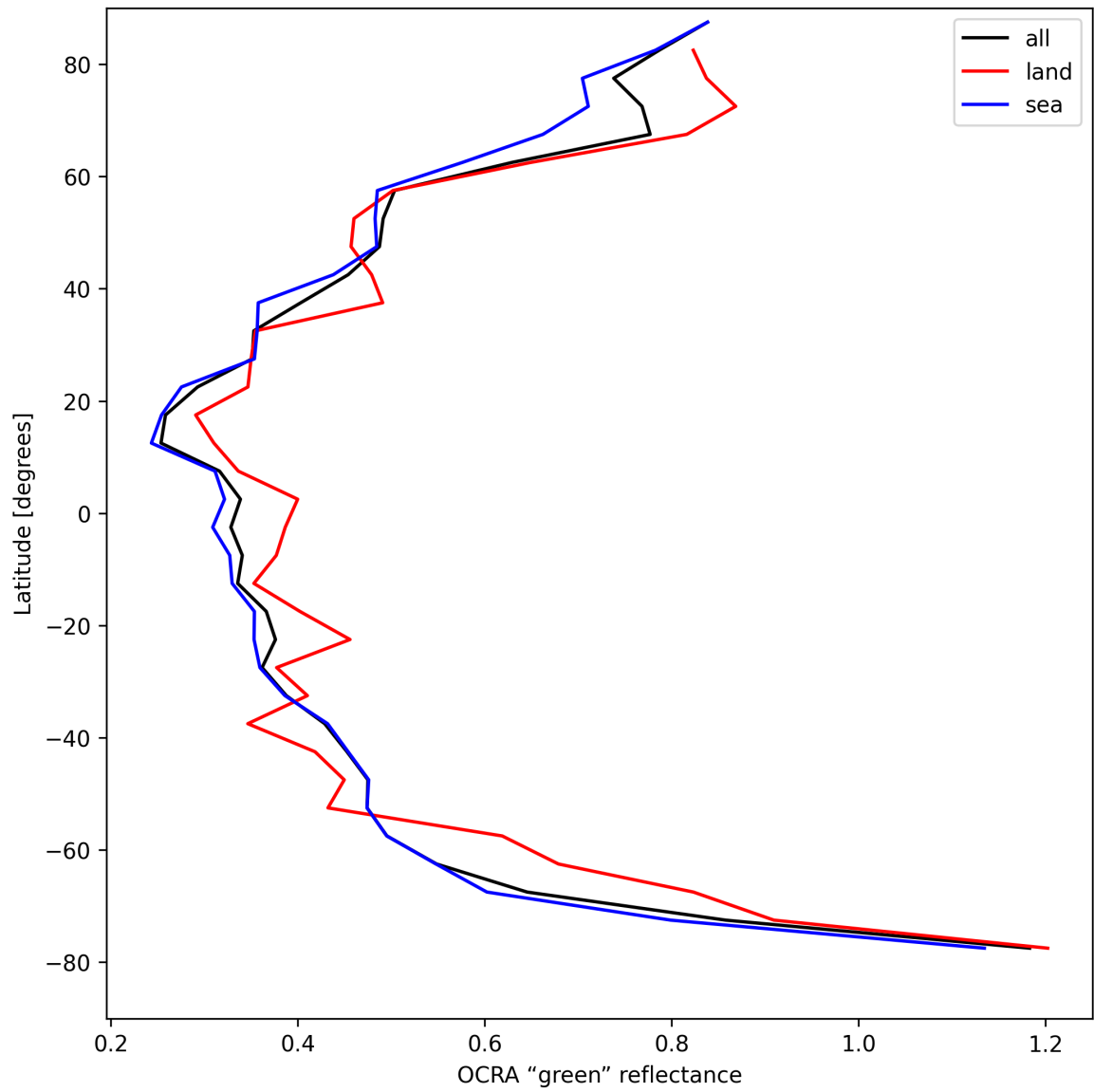
Figure 36: Zonal average of “OCRA “green” reflectance” for 2025-04-18 to 2025-04-19.
