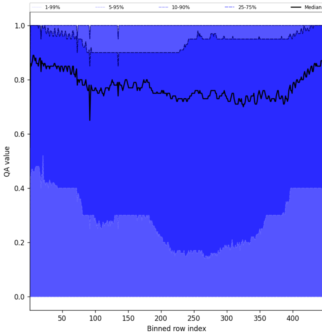
Figure 54: Along track statistics of "QA value" for 2025-04-18 to 2025-04-19
