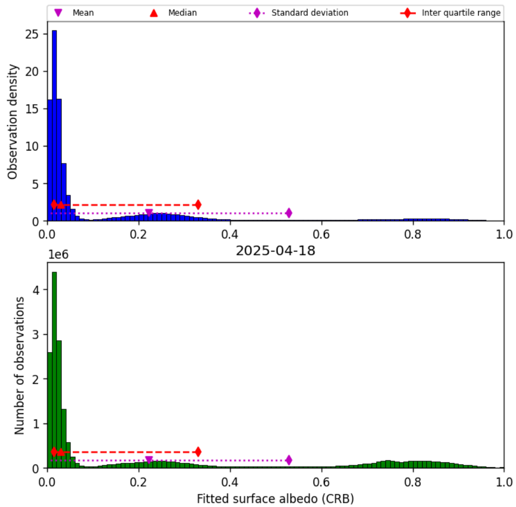
Figure 46: Histogram of “Fitted surface albedo (CRB)” for 2025-04-18 to 2025-04-19
