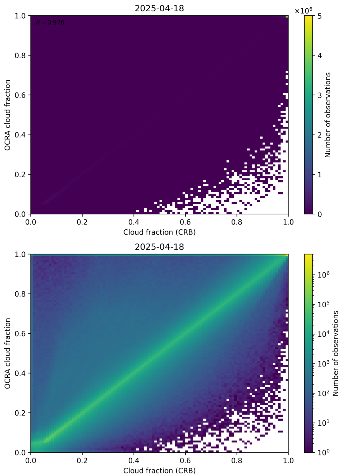
Figure 78: Scatter density plot of “Cloud fraction (CRB)” against “OCRA cloud fraction” for 2025-04-18 to 2025-04-19.
