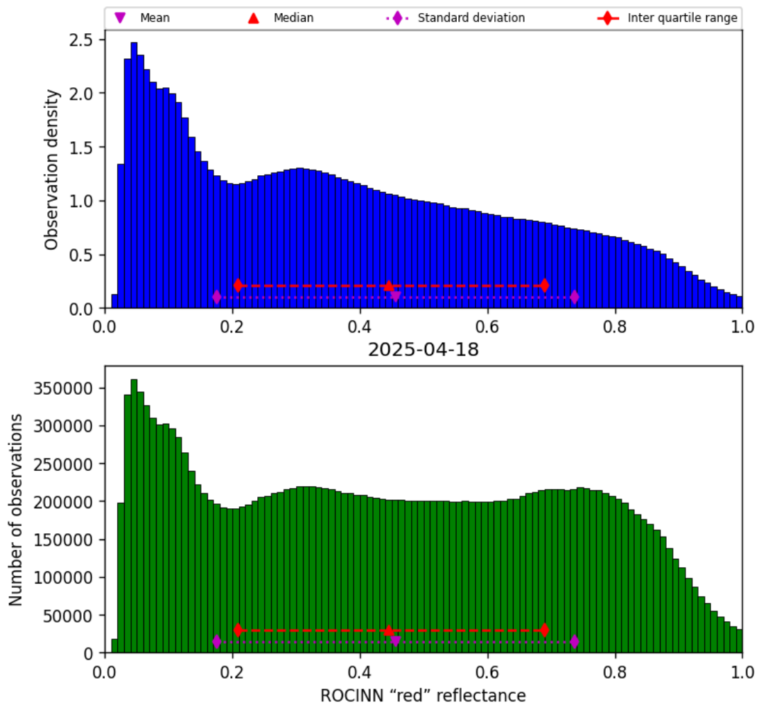
Figure 53: Histogram of “ROCINN “red” reflectance” for 2025-04-18 to 2025-04-19
