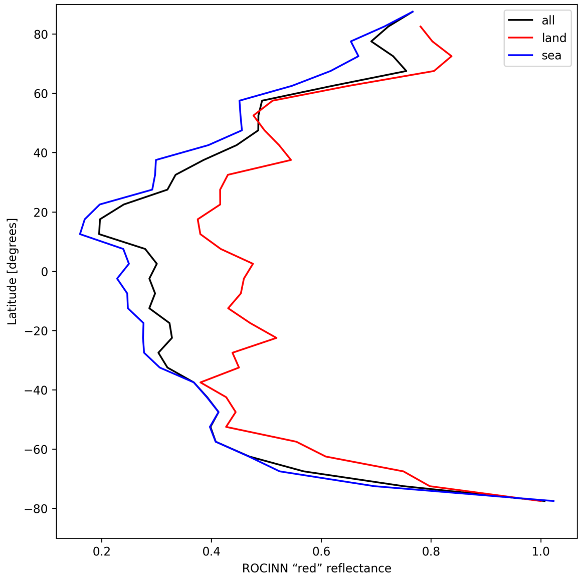
Figure 37: Zonal average of “ROCINN “red” reflectance” for 2025-04-18 to 2025-04-19.
