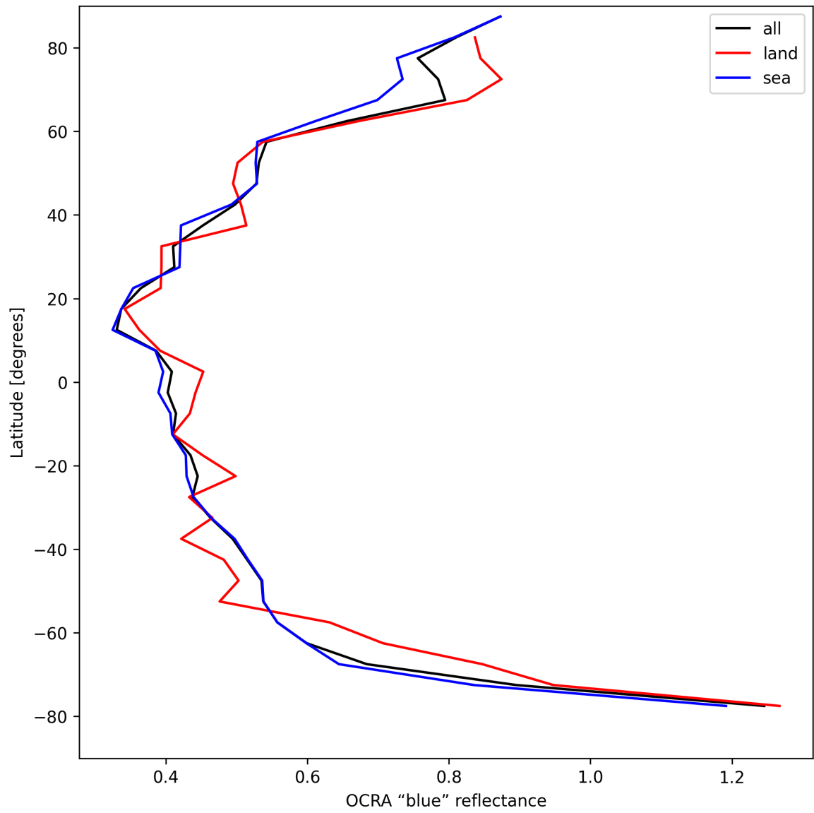
Figure 35: Zonal average of “OCRA “blue” reflectance” for 2025-04-18 to 2025-04-19.
