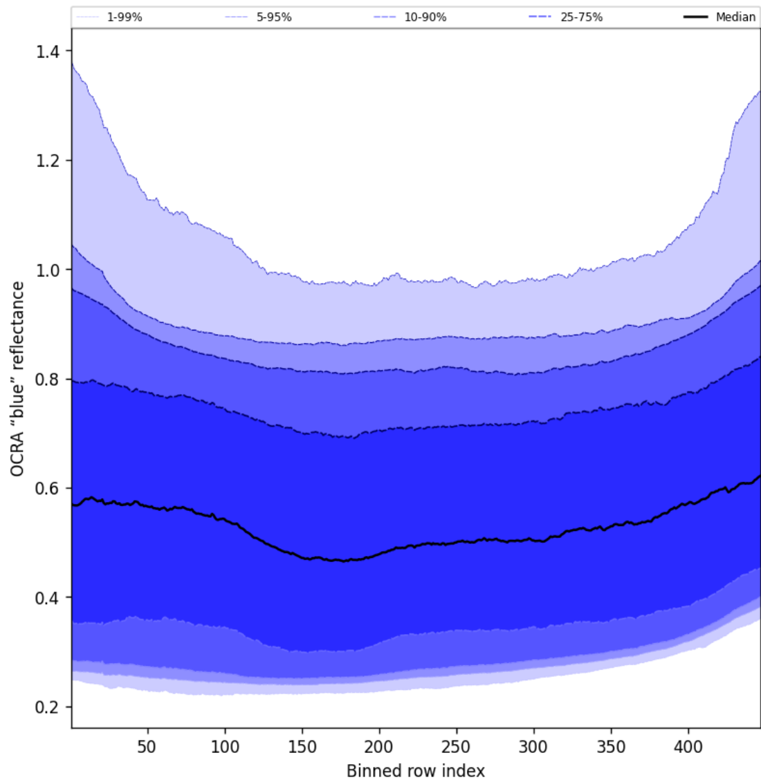
Figure 67: Along track statistics of “OCRA “blue” reflectance” for 2025-04-18 to 2025-04-19
