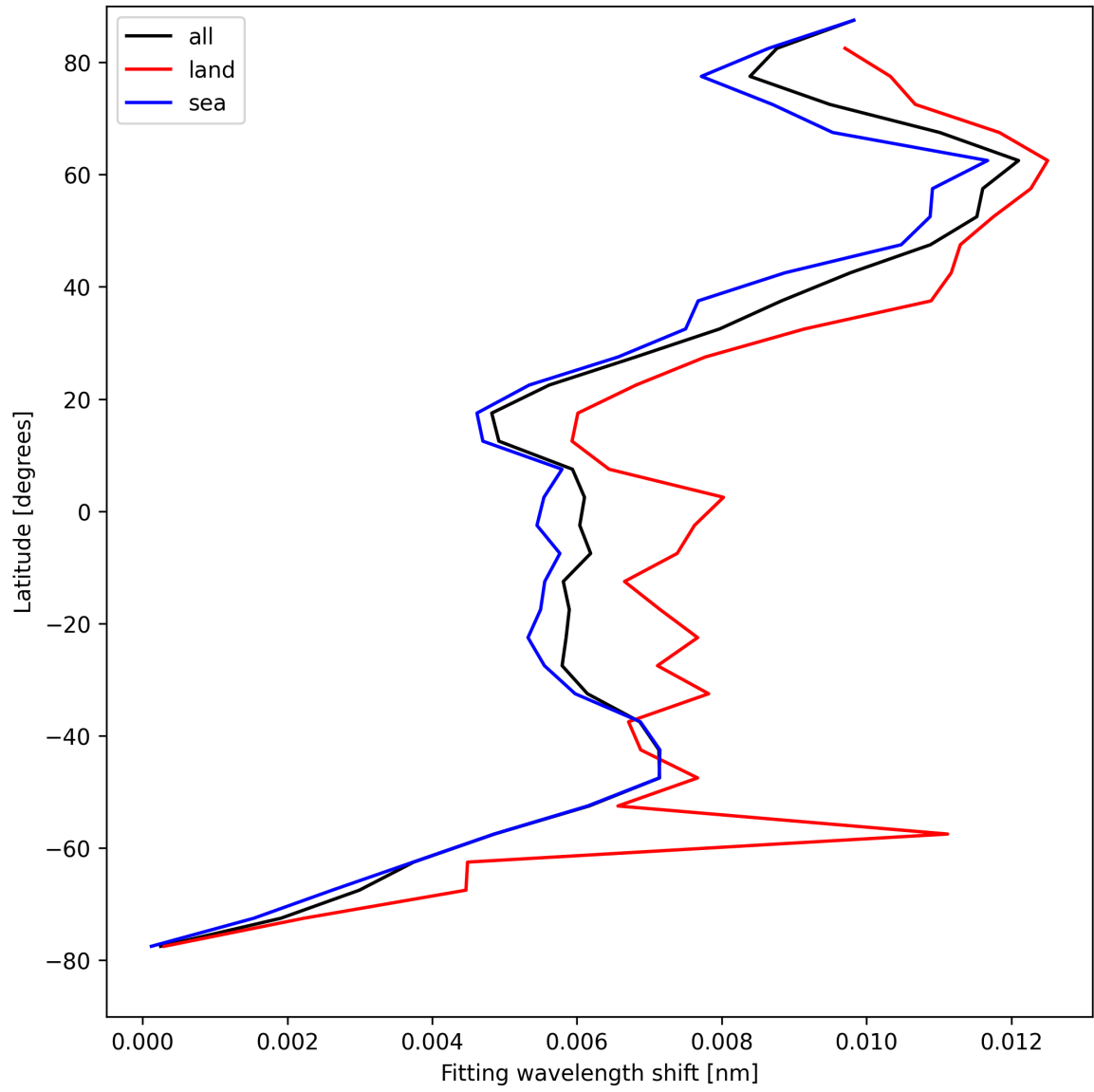
Figure 33: Zonal average of “Fitting wavelength shift” for 2025-04-18 to 2025-04-19.
