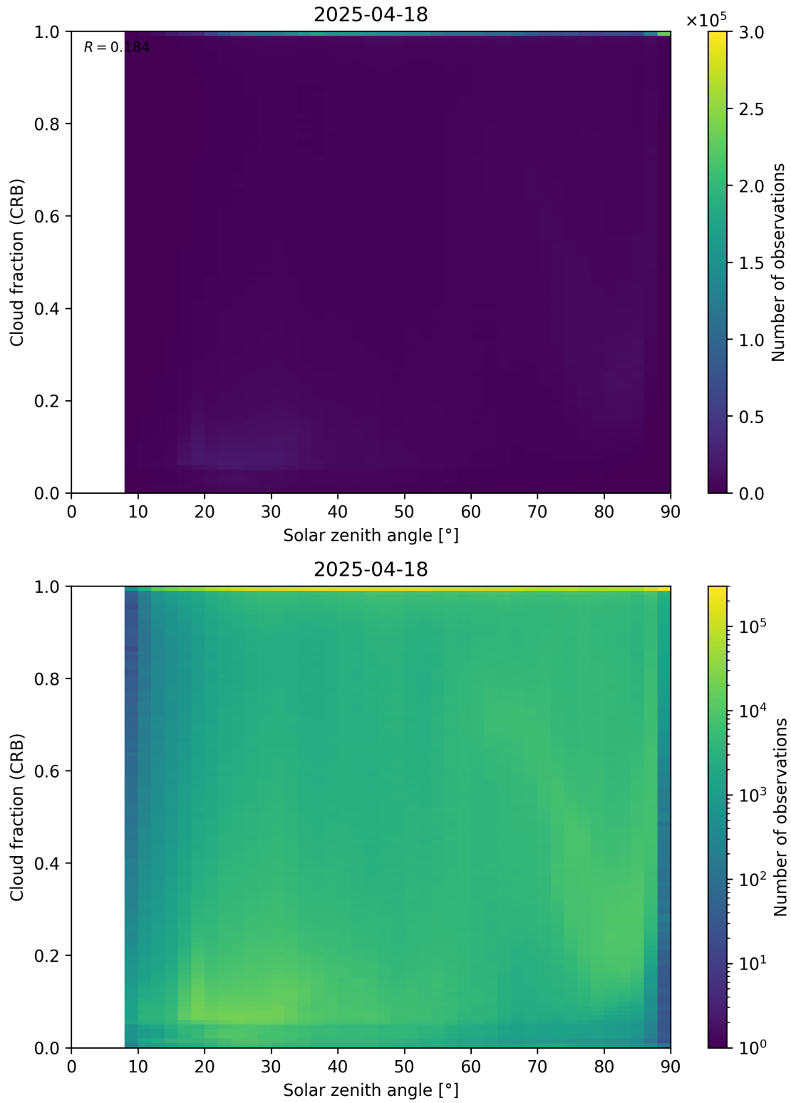
Figure 101: Scatter density plot of “Solar zenith angle” against “Cloud fraction (CRB)” for 2025-04-18 to 2025-04-19.
