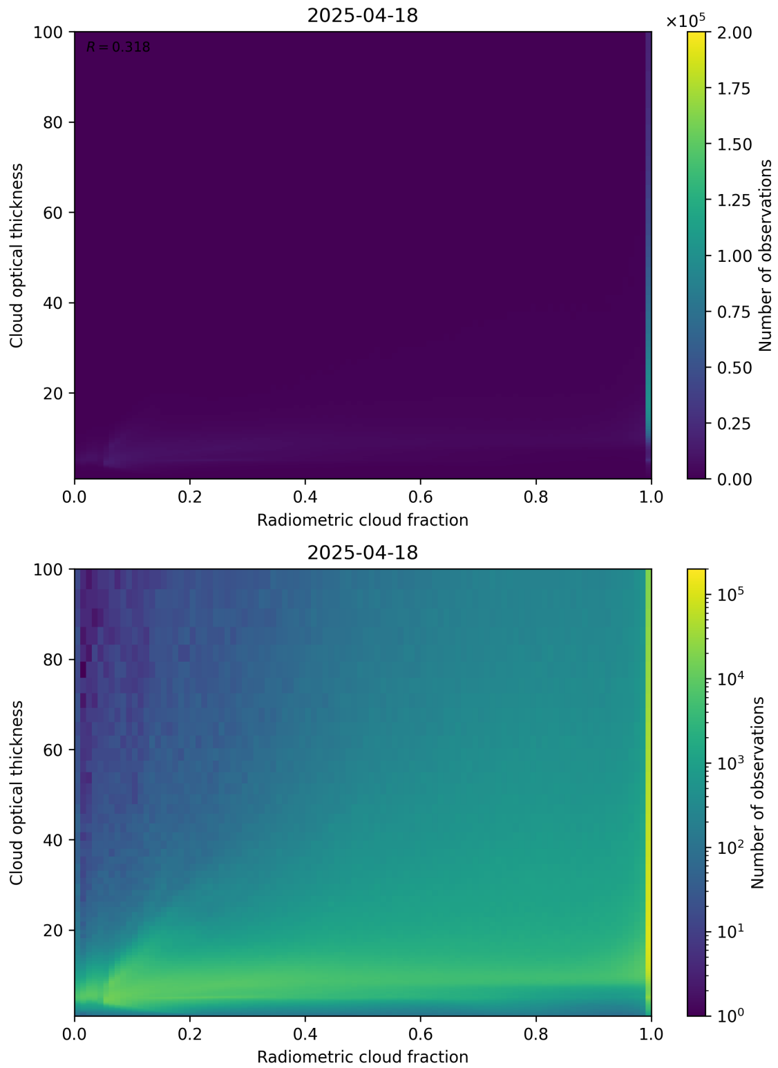
Figure 75: Scatter density plot of “Radiometric cloud fraction” against “Cloud optical thickness” for 2025-04-18 to 2025-04-19.
