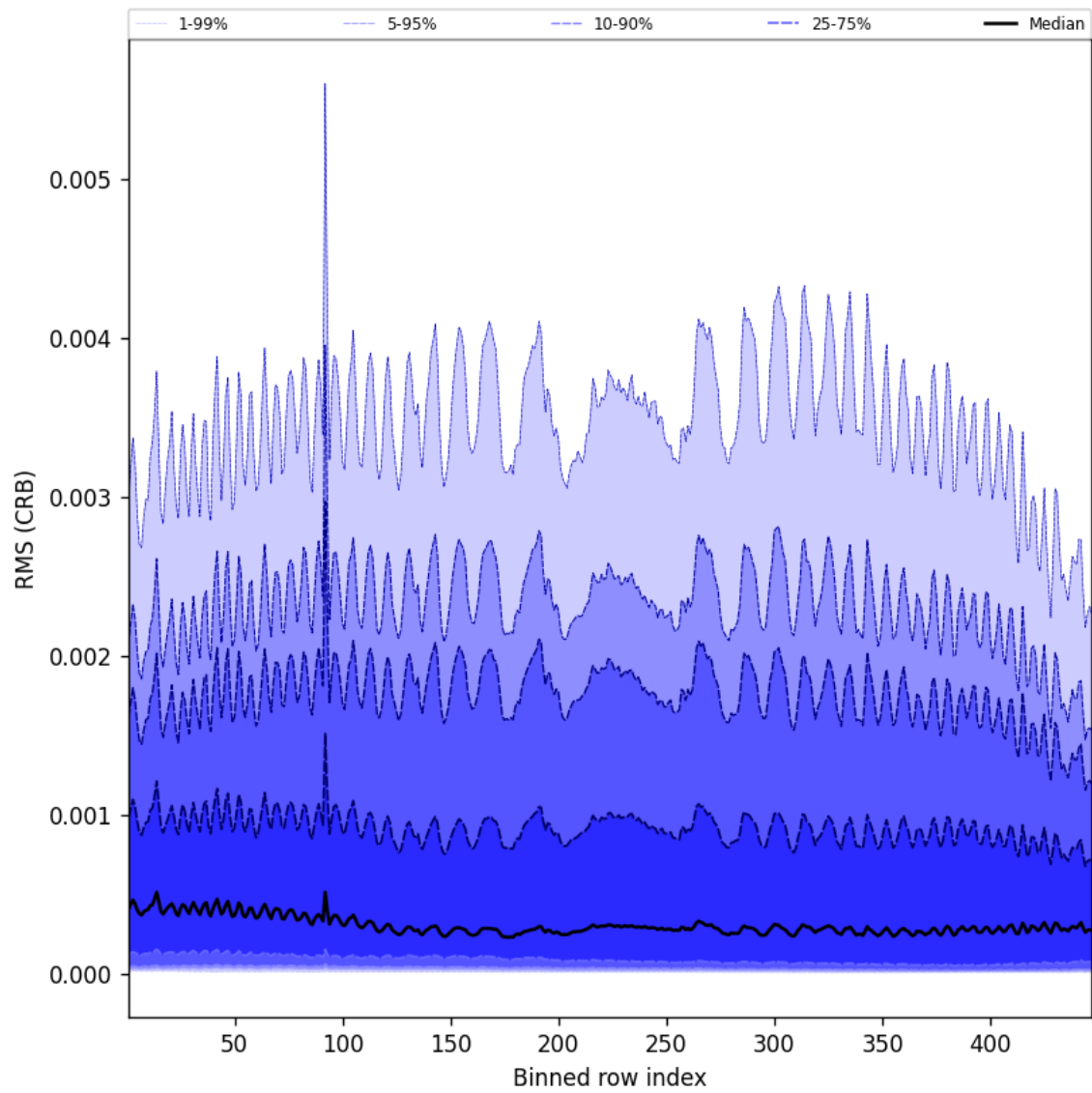
Figure 64: Along track statistics of “RMS (CRB)” for 2025-04-18 to 2025-04-19
