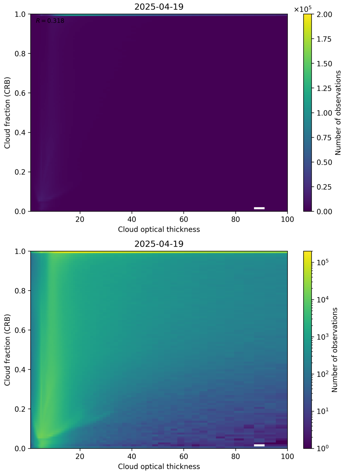
Figure 84: Scatter density plot of “Cloud optical thickness” against “Cloud fraction (CRB)” for 2025-04-19 to 2025-04-20.
