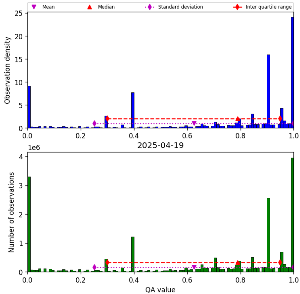
Figure 38: Histogram of “QA value” for 2025-04-19 to 2025-04-20
