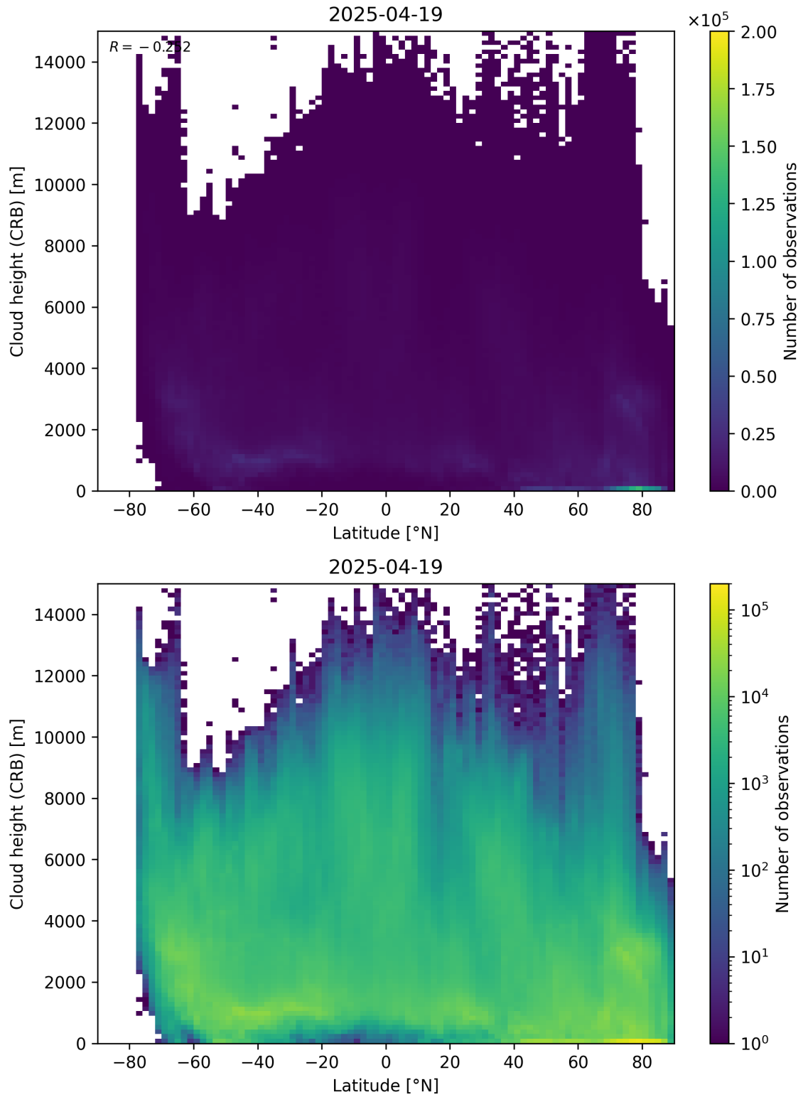
Figure 95: Scatter density plot of “Latitude” against “Cloud height (CRB)” for 2025-04-19 to 2025-04-20.
