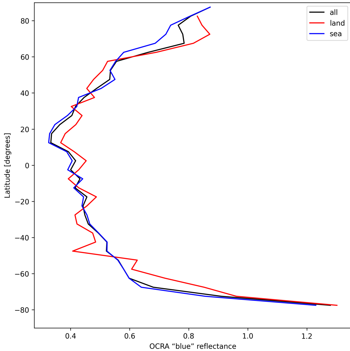
Figure 35: Zonal average of “OCRA “blue” reflectance” for 2025-04-19 to 2025-04-20.
