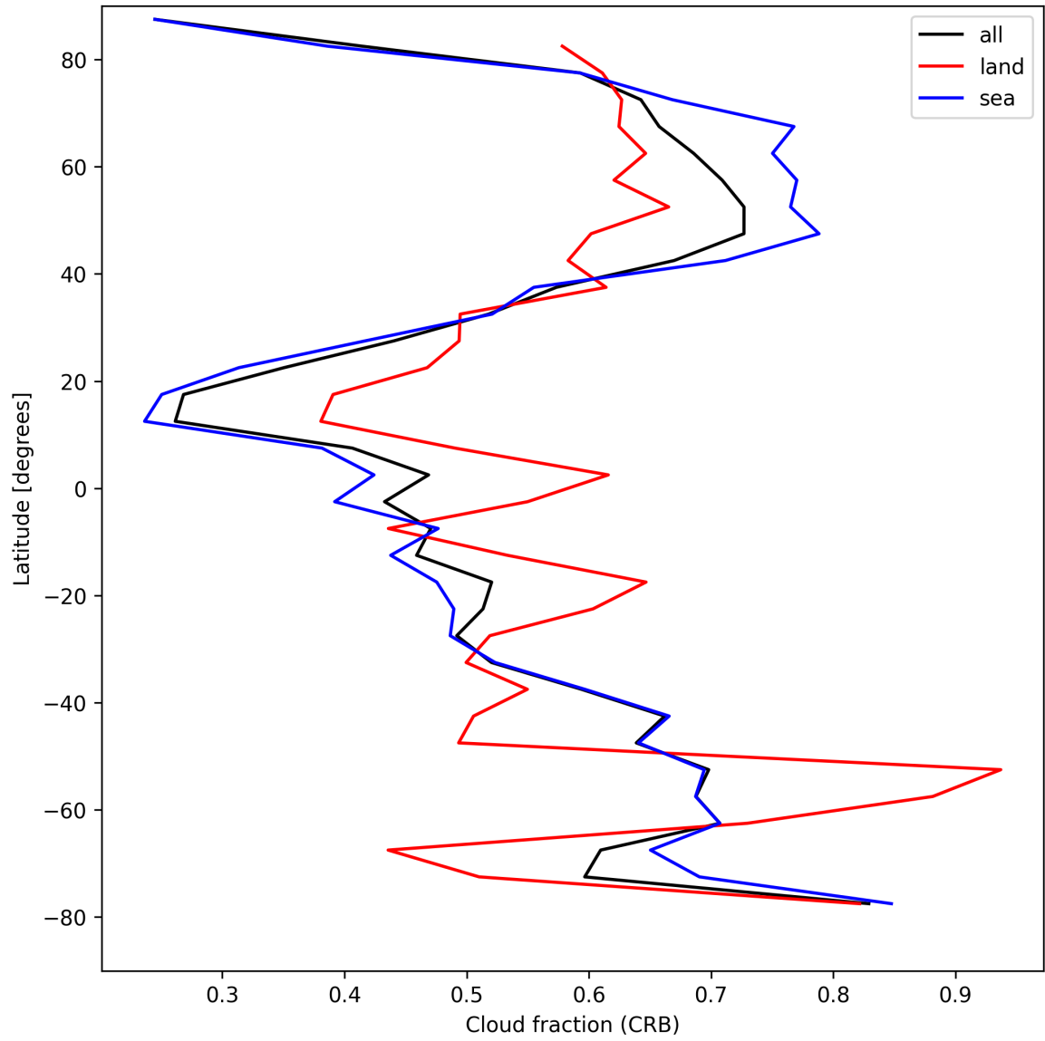
Figure 26: Zonal average of “Cloud fraction (CRB)” for 2025-04-19 to 2025-04-20.
