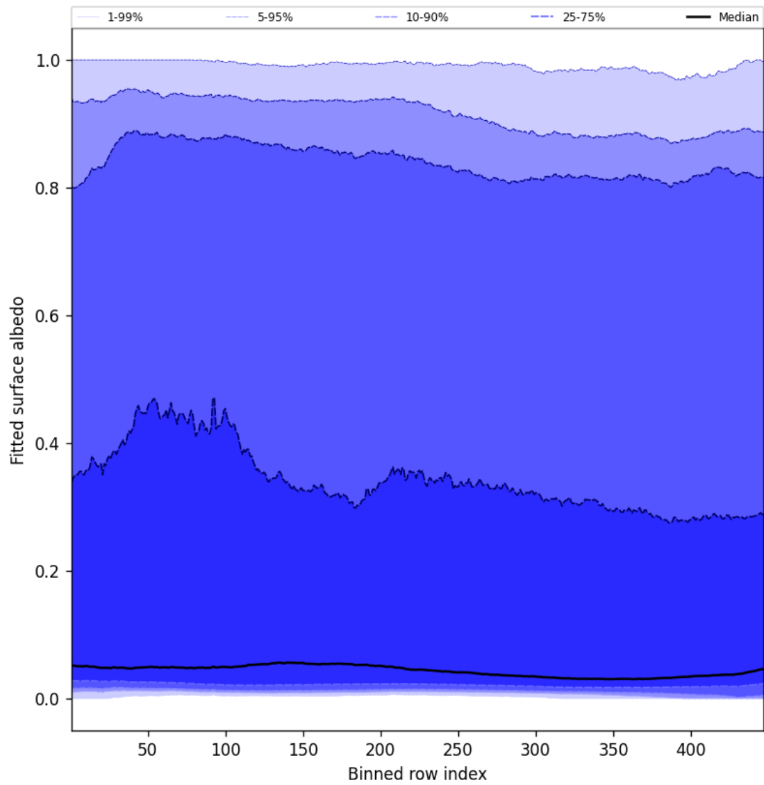
Figure 61: Along track statistics of “Fitted surface albedo” for 2025-04-19 to 2025-04-20
