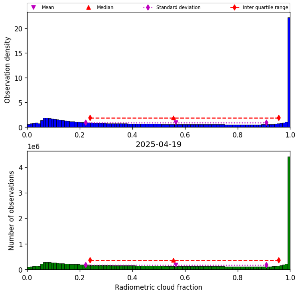
Figure 39: Histogram of “Radiometric cloud fraction” for 2025-04-19 to 2025-04-20
