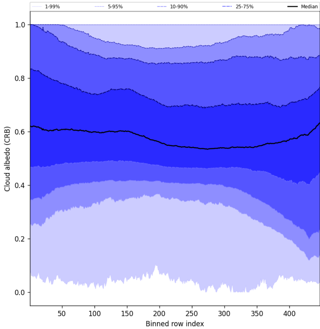
Figure 60: Along track statistics of “Cloud albedo (CRB)” for 2025-04-19 to 2025-04-20
