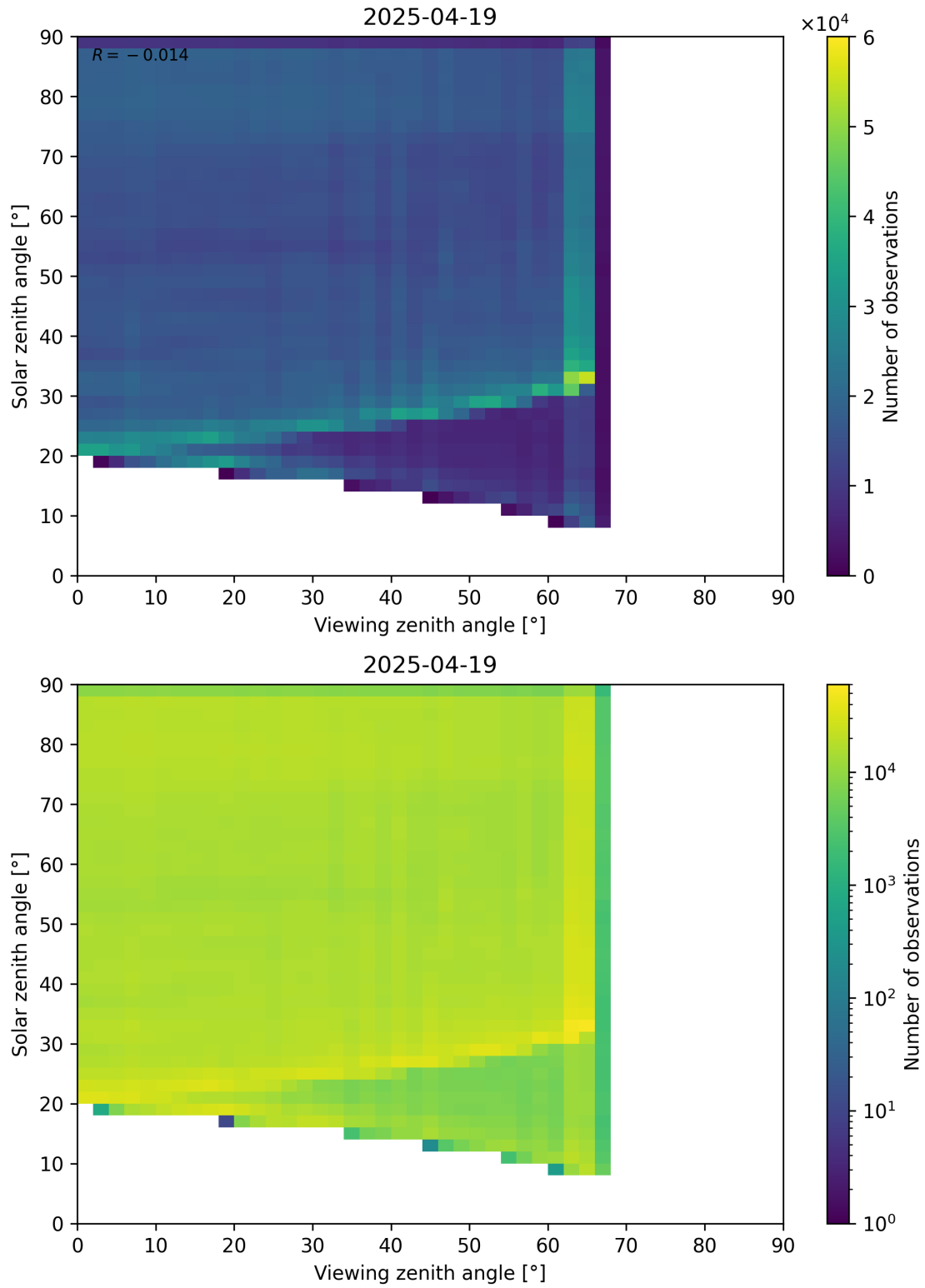
Figure 114: Scatter density plot of “Viewing zenith angle” against “Solar zenith angle” for 2025-04-19 to 2025-04-20.
