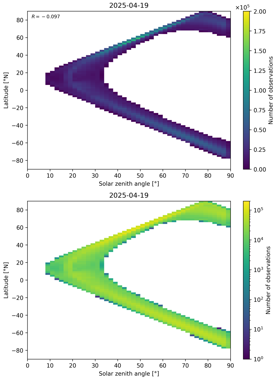
Figure 105: Scatter density plot of “Solar zenith angle” against “Latitude” for 2025-04-19 to 2025-04-20.
