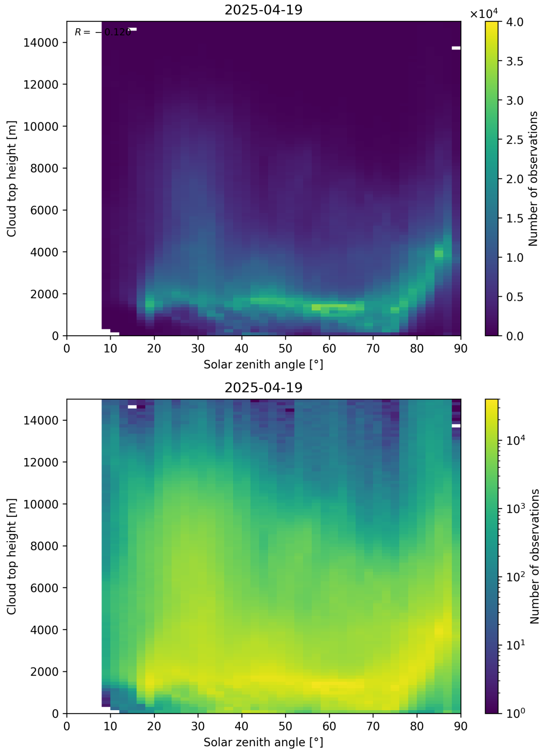
Figure 104: Scatter density plot of “Solar zenith angle” against “Cloud top height” for 2025-04-19 to 2025-04-20.
