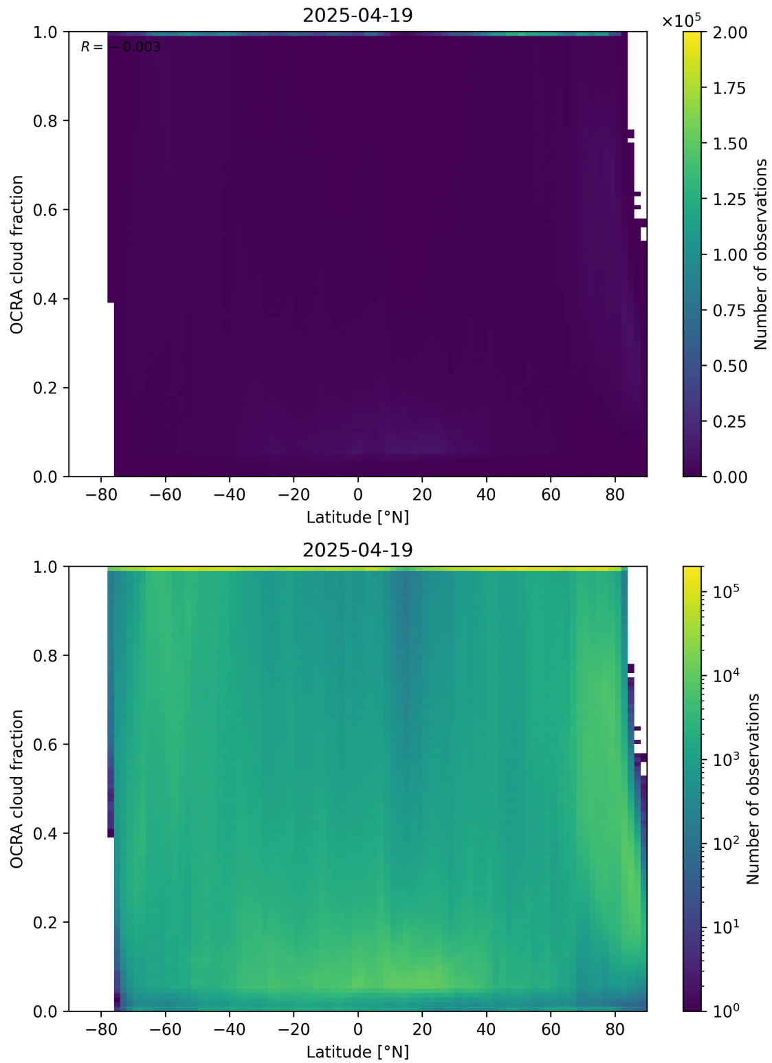
Figure 93: Scatter density plot of “Latitude” against “OCRA cloud fraction” for 2025-04-19 to 2025-04-20.
