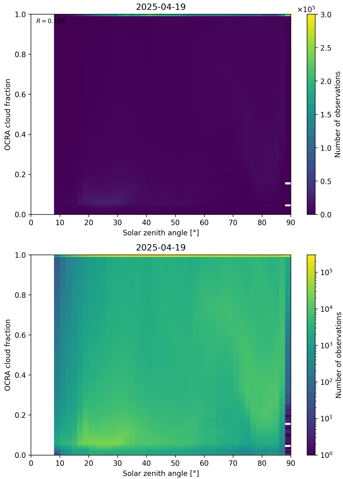
Figure 100: Scatter density plot of “Solar zenith angle” against “OCRA cloud fraction” for 2025-04-19 to 2025-04-20.
