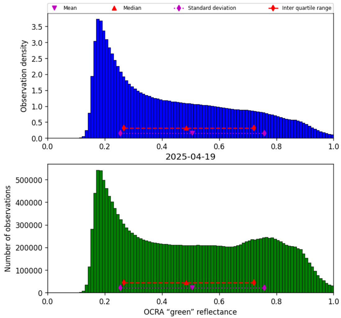
Figure 52: Histogram of “OCRA “green” reflectance” for 2025-04-19 to 2025-04-20
