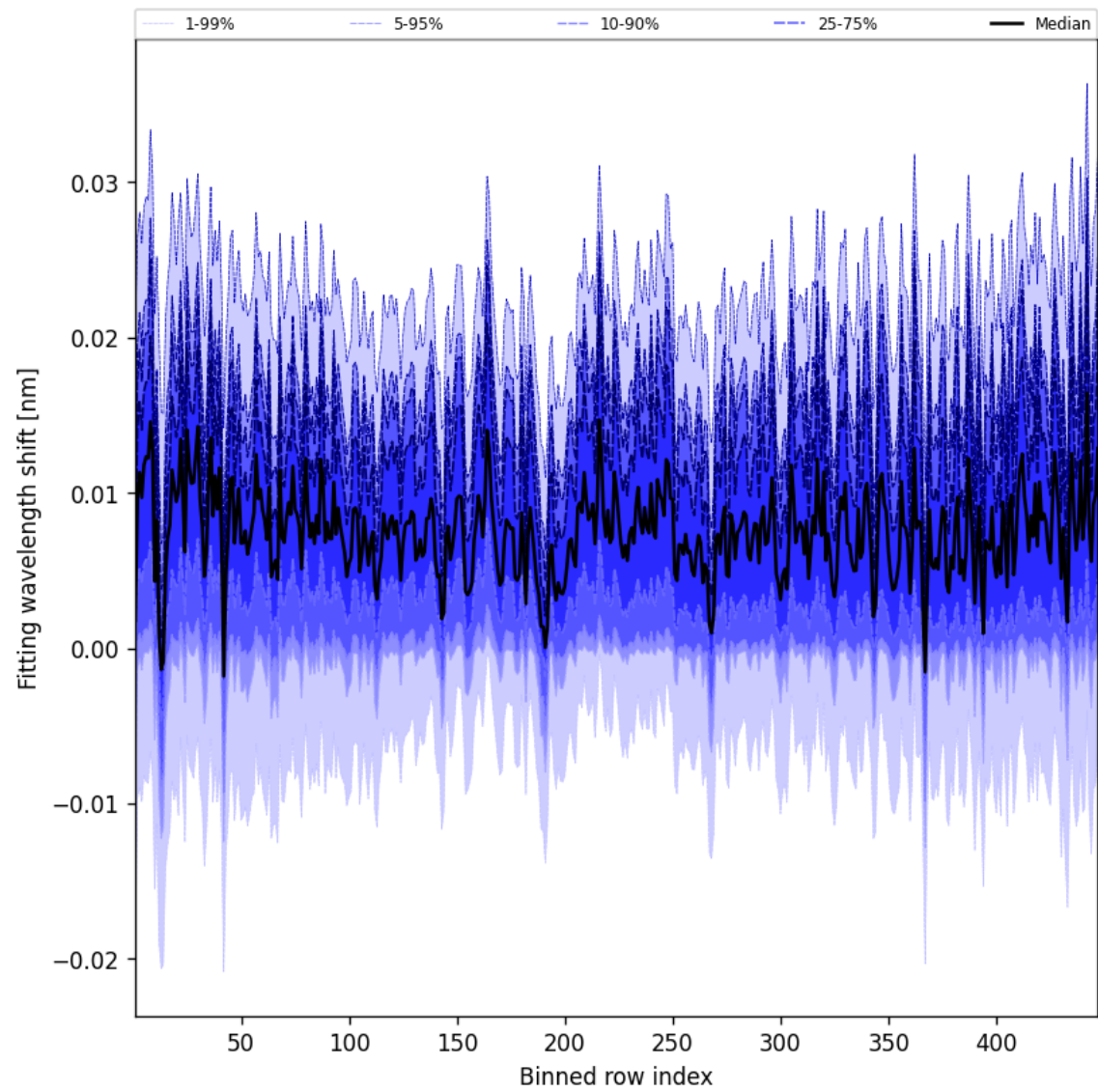
Figure 65: Along track statistics of “Fitting wavelength shift” for 2025-04-19 to 2025-04-20
