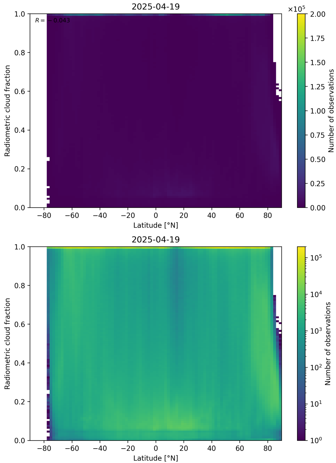
Figure 92: Scatter density plot of “Latitude” against “Radiometric cloud fraction” for 2025-04-19 to 2025-04-20.
