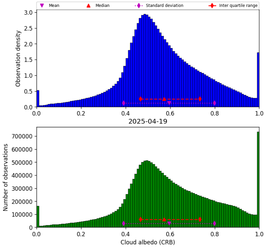
Figure 44: Histogram of “Cloud albedo (CRB)” for 2025-04-19 to 2025-04-20
