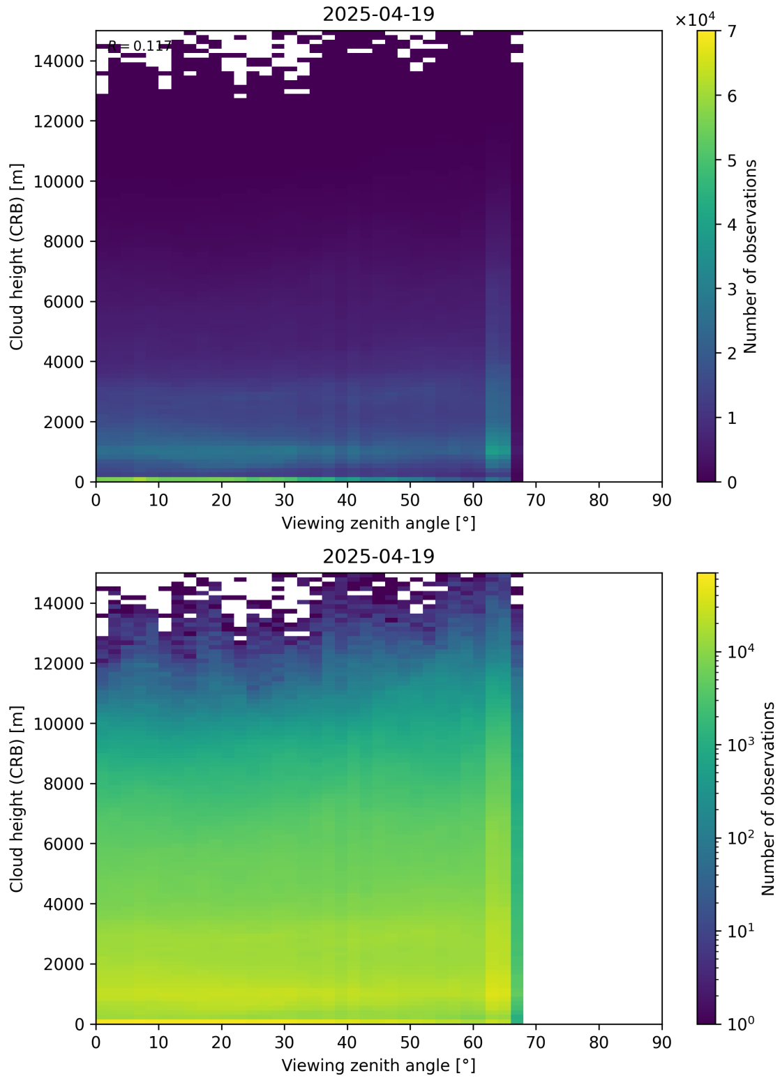
Figure 110: Scatter density plot of “Viewing zenith angle” against “Cloud height (CRB)” for 2025-04-19 to 2025-04-20.
