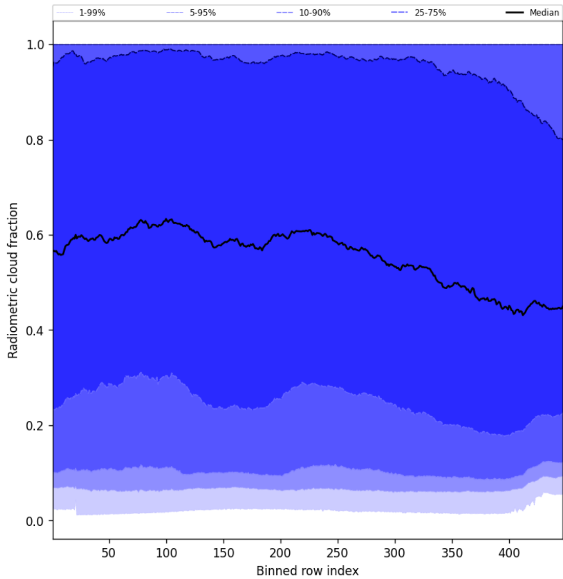
Figure 55: Along track statistics of “Radiometric cloud fraction” for 2025-04-19 to 2025-04-20
