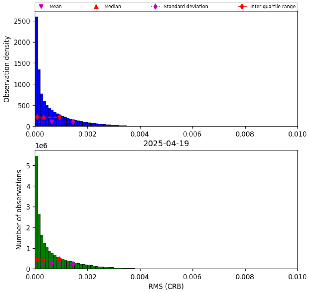
Figure 48: Histogram of “RMS (CRB)” for 2025-04-19 to 2025-04-20
