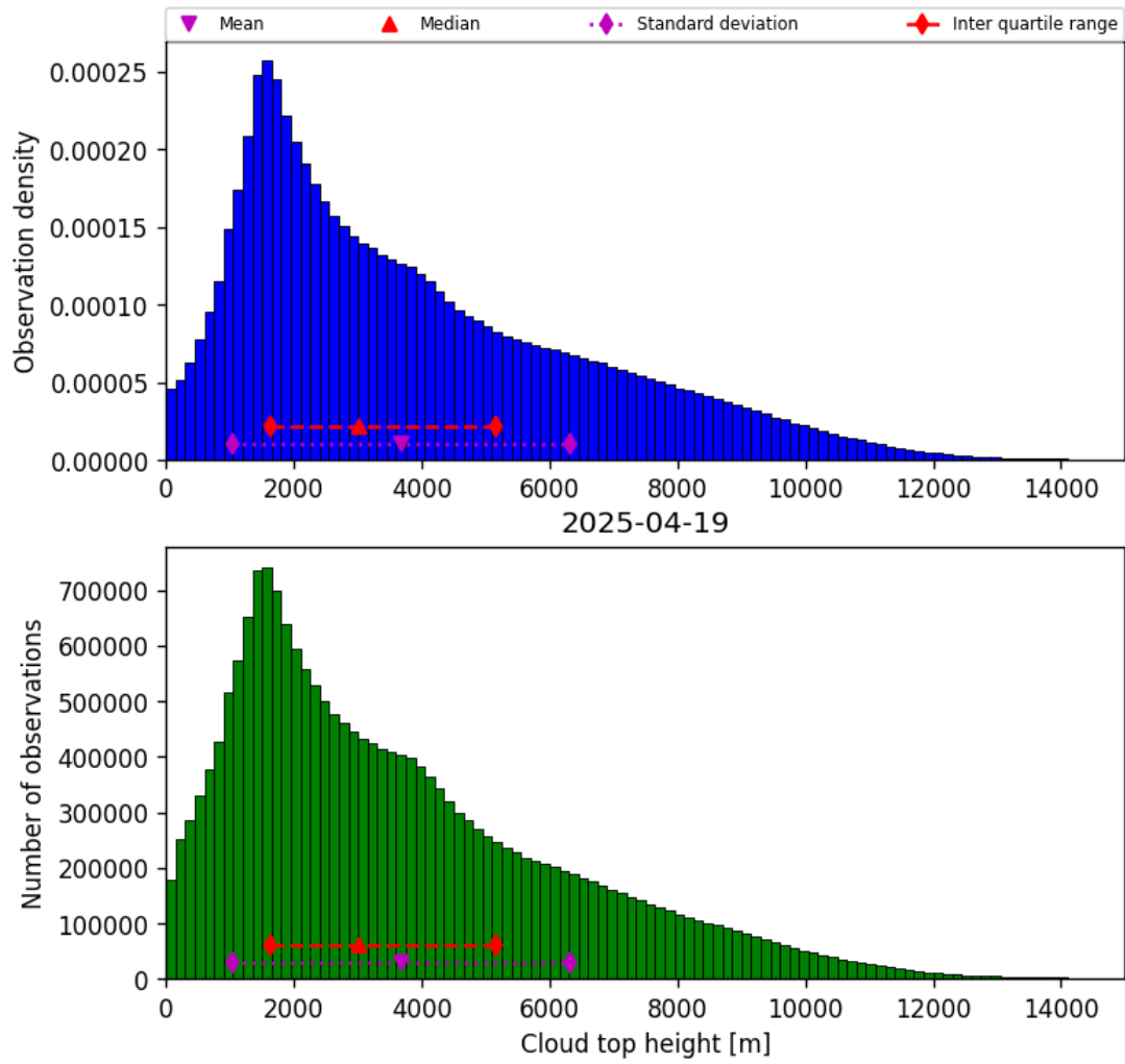
Figure 40: Histogram of “Cloud top height” for 2025-04-19 to 2025-04-20
