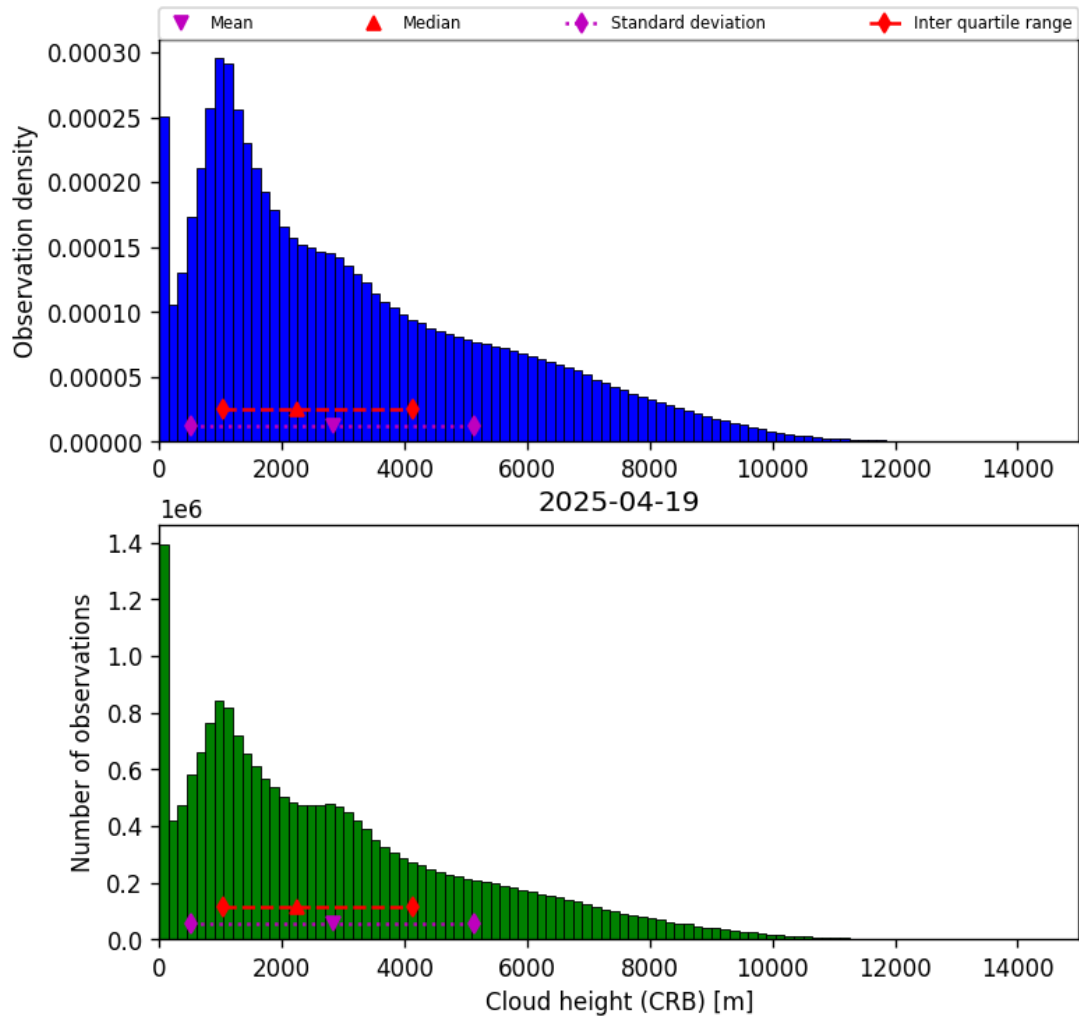
Figure 43: Histogram of “Cloud height (CRB)” for 2025-04-19 to 2025-04-20
