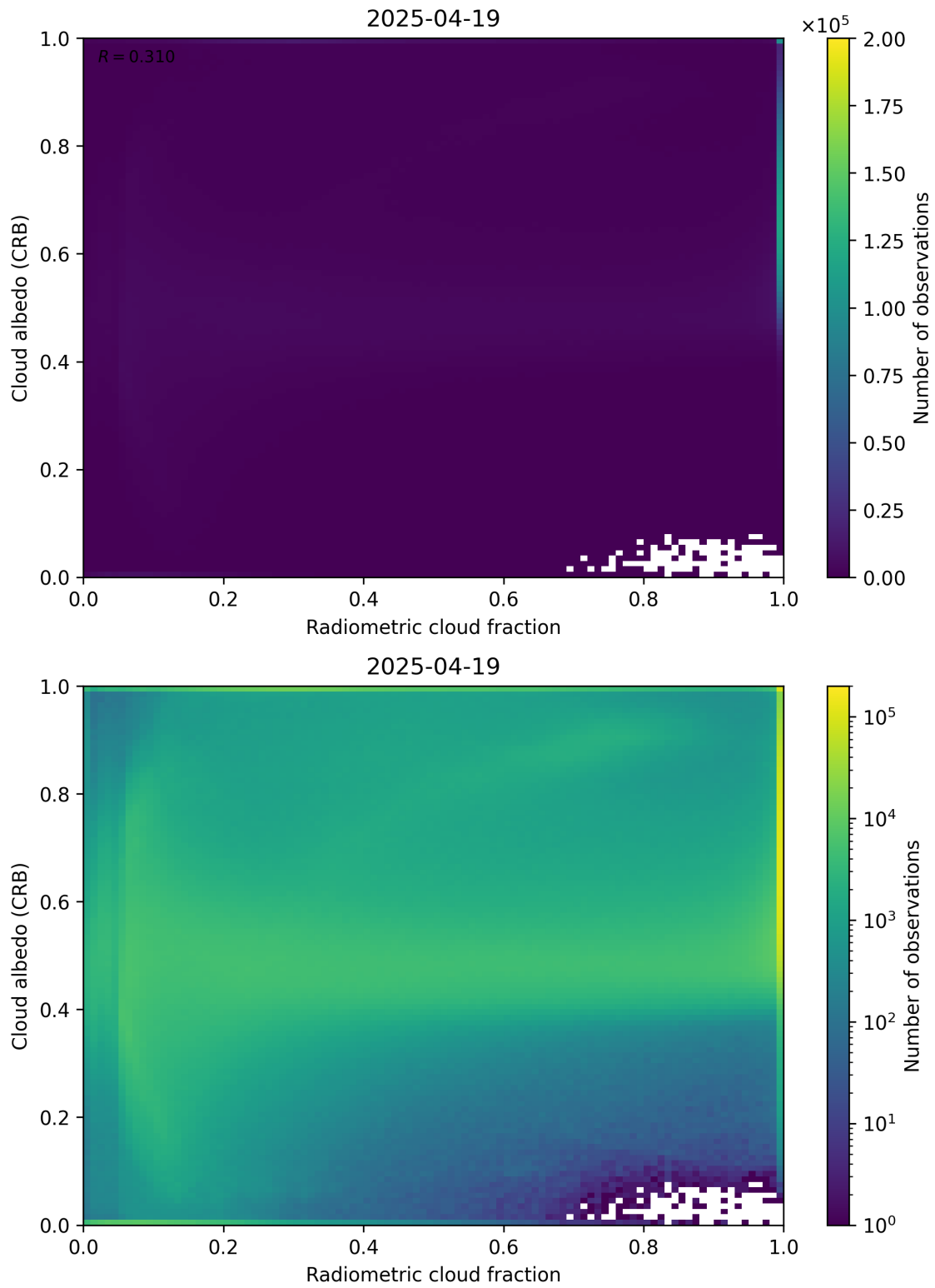
Figure 71: Scatter density plot of “Radiometric cloud fraction” against “Cloud albedo (CRB)” for 2025-04-19 to 2025-04-20.
