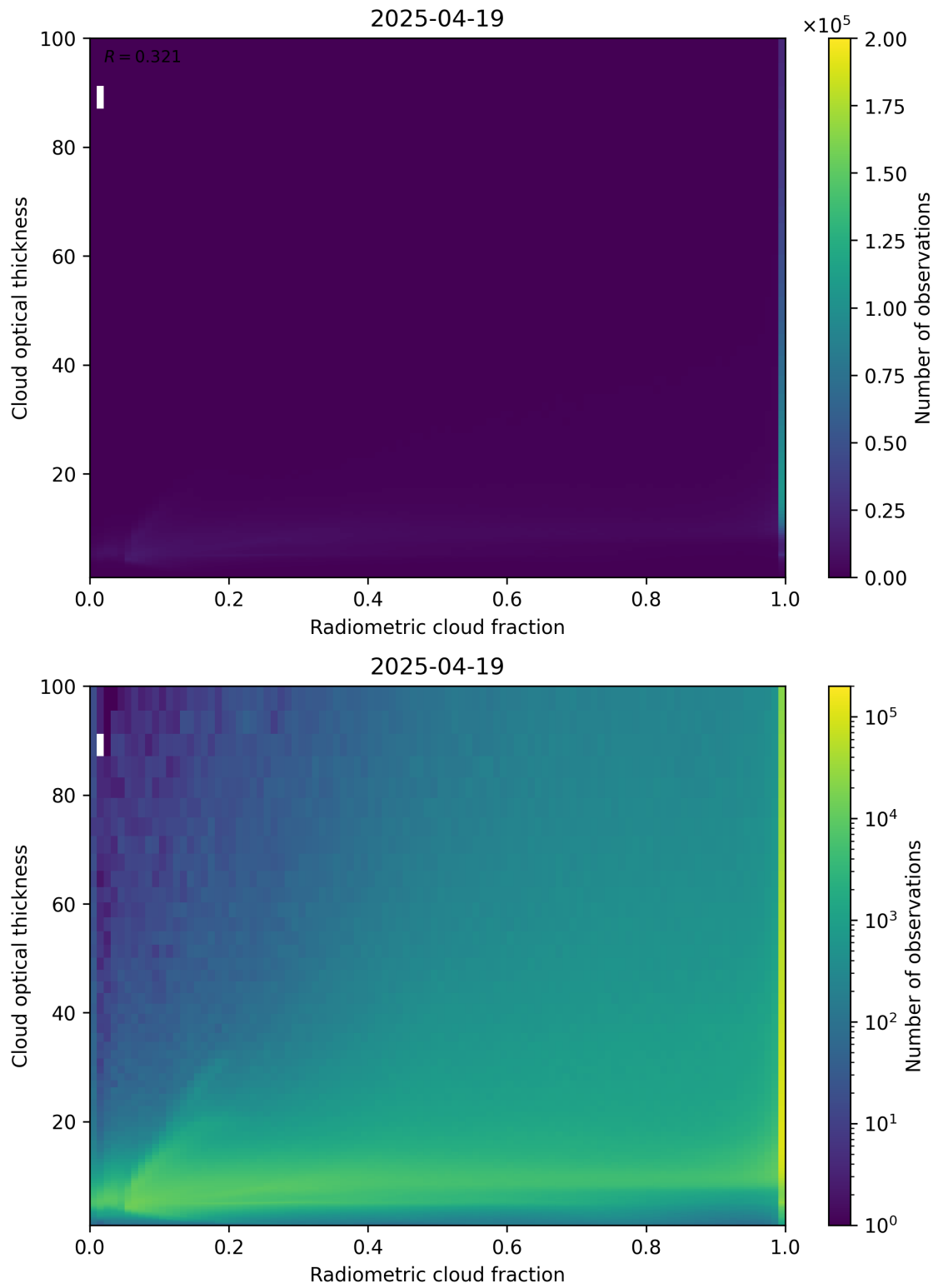
Figure 75: Scatter density plot of “Radiometric cloud fraction” against “Cloud optical thickness” for 2025-04-19 to 2025-04-20.
