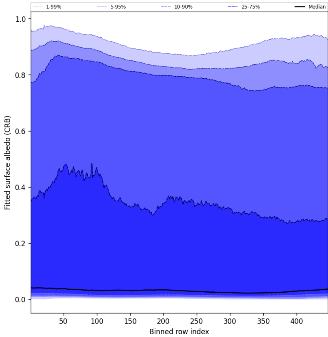
Figure 62: Along track statistics of “Fitted surface albedo (CRB)” for 2025-04-19 to 2025-04-20
