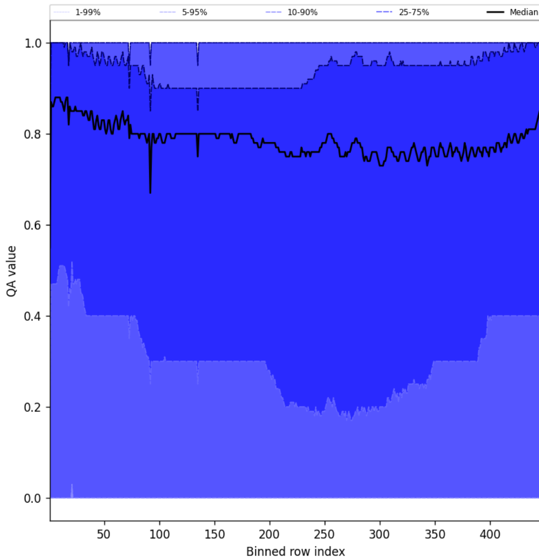
Figure 54: Along track statistics of “QA value” for 2025-04-19 to 2025-04-20
