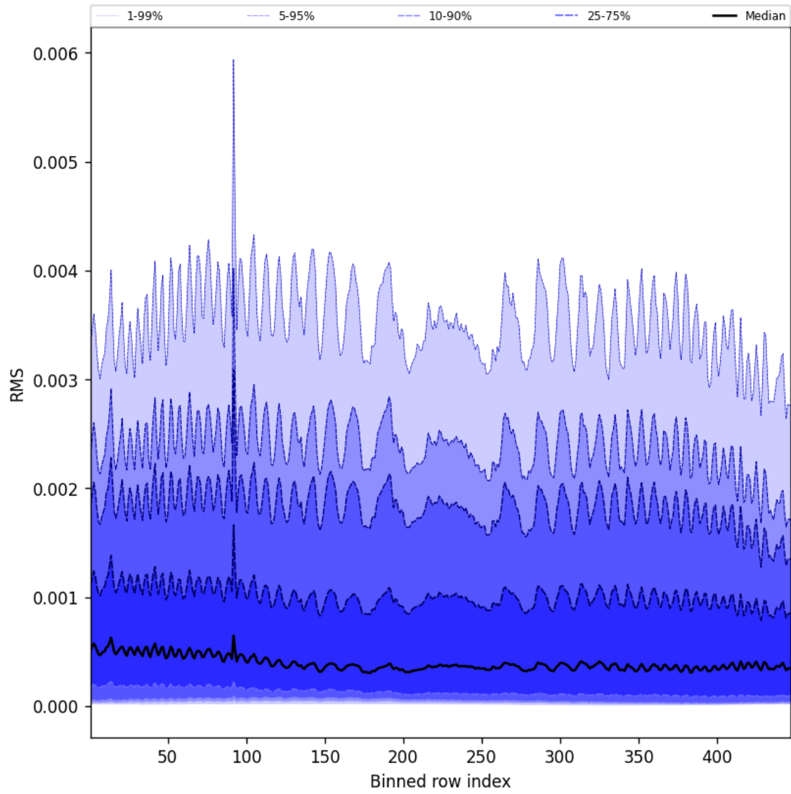
Figure 63: Along track statistics of “RMS” for 2025-04-19 to 2025-04-20
