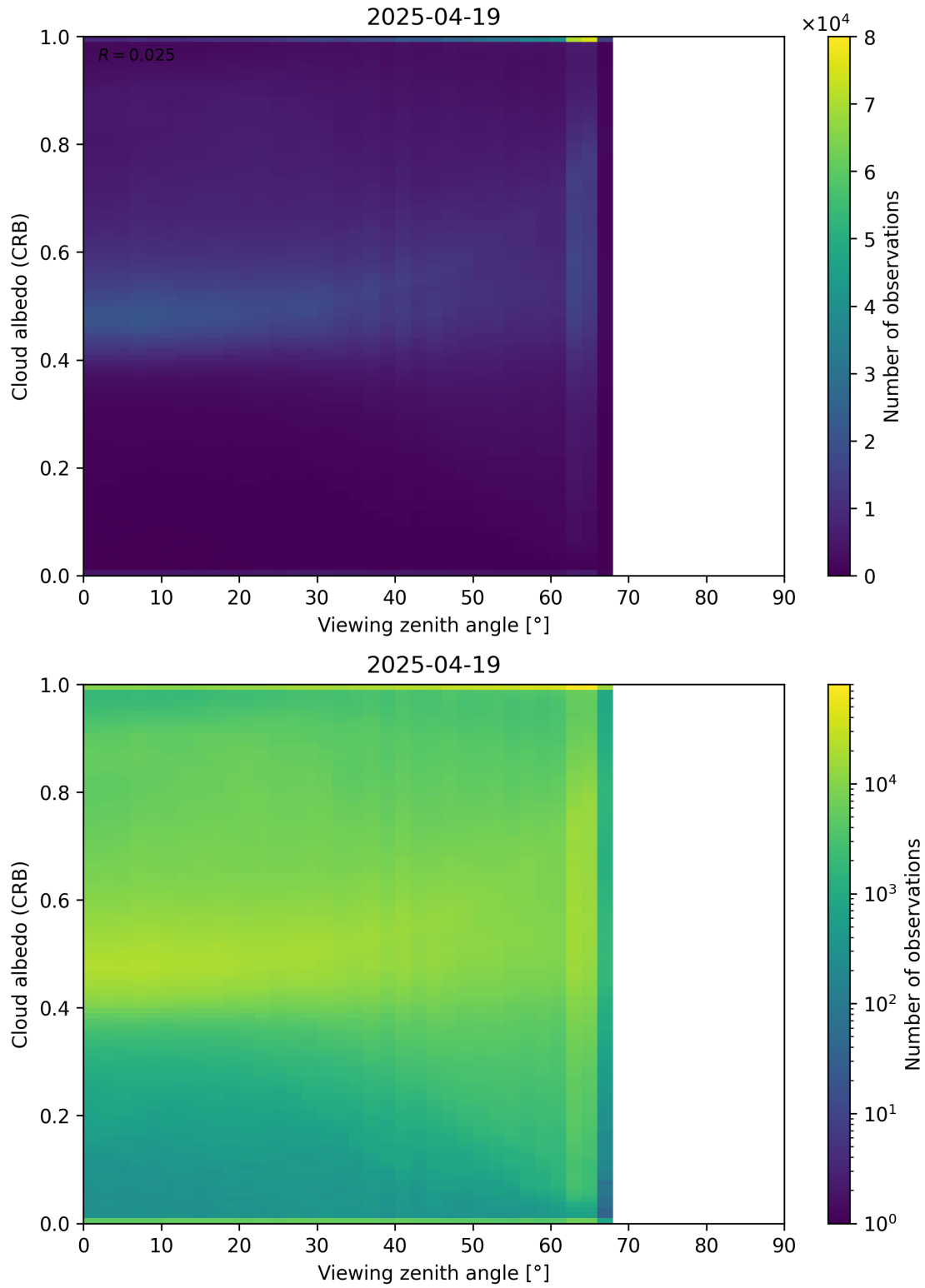
Figure 106: Scatter density plot of “Viewing zenith angle” against “Cloud albedo (CRB)” for 2025-04-19 to 2025-04-20.
