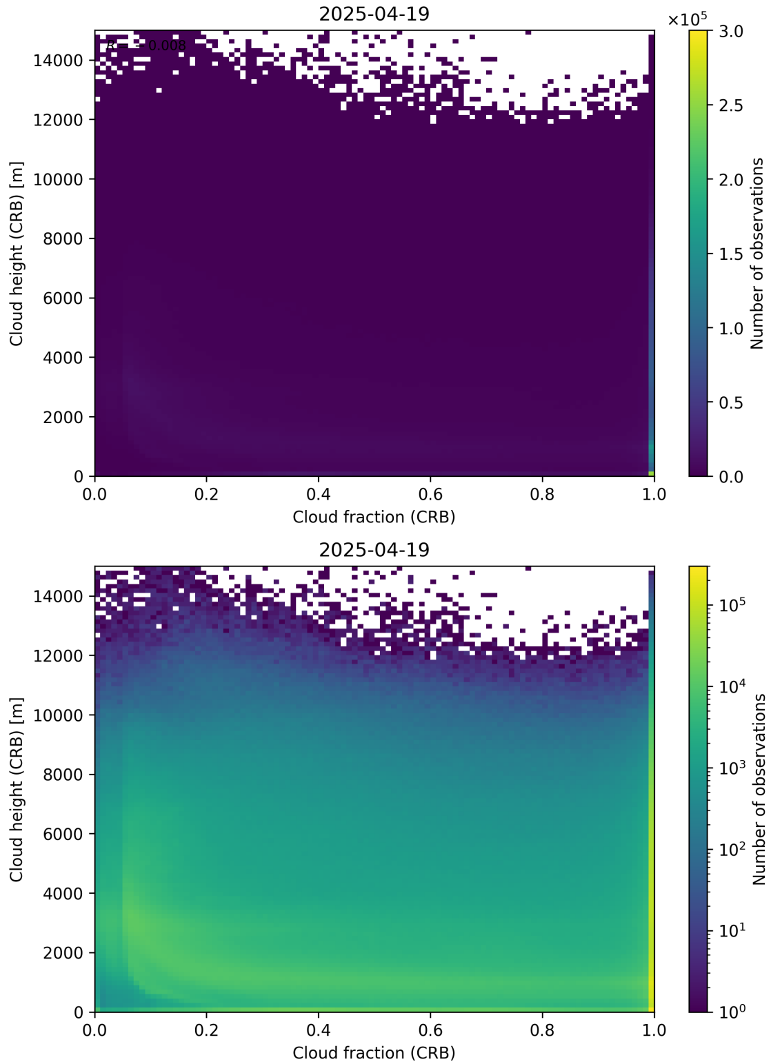
Figure 79: Scatter density plot of “Cloud fraction (CRB)” against “Cloud height (CRB)” for 2025-04-19 to 2025-04-20.
