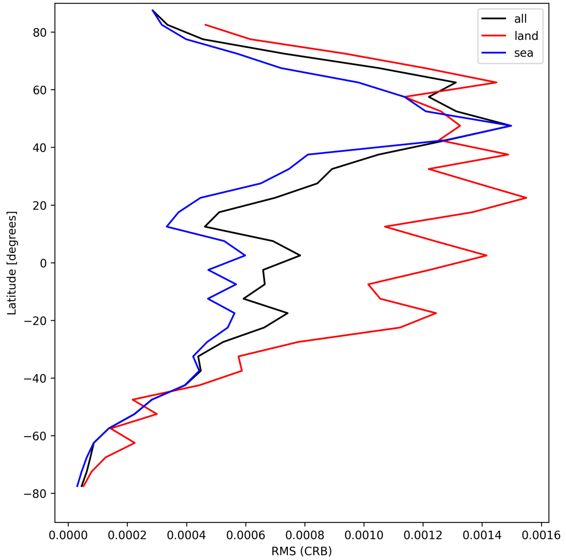
Figure 32: Zonal average of “RMS (CRB)” for 2025-04-19 to 2025-04-20.
