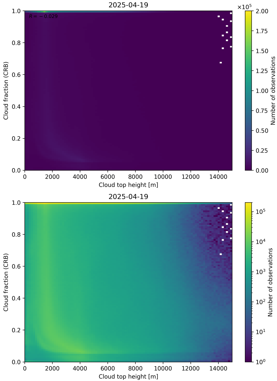
Figure 88: Scatter density plot of “Cloud top height” against “Cloud fraction (CRB)” for 2025-04-19 to 2025-04-20.
