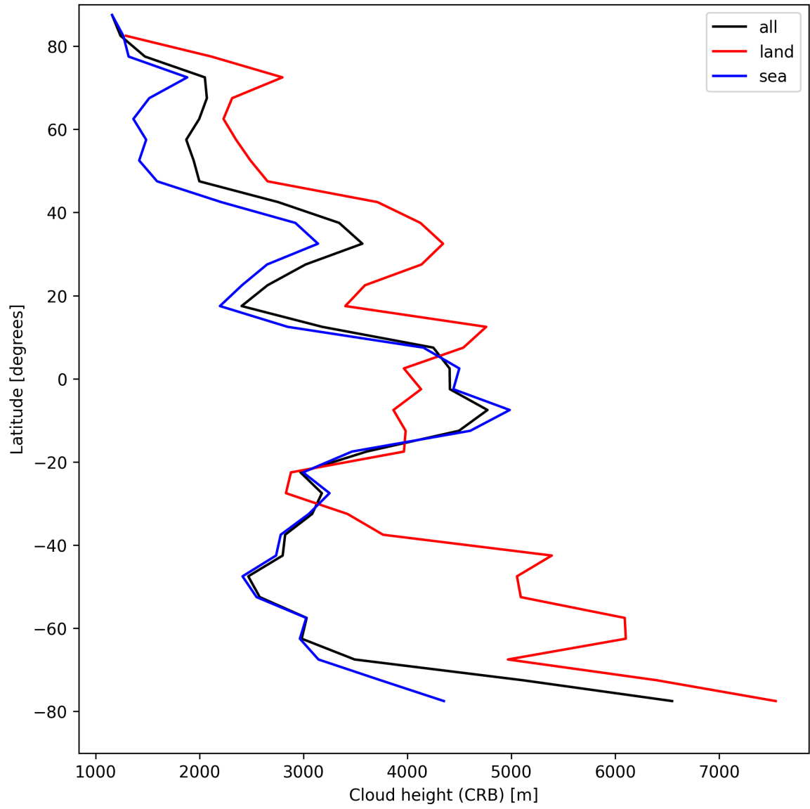
Figure 27: Zonal average of “Cloud height (CRB)” for 2025-04-19 to 2025-04-20.
