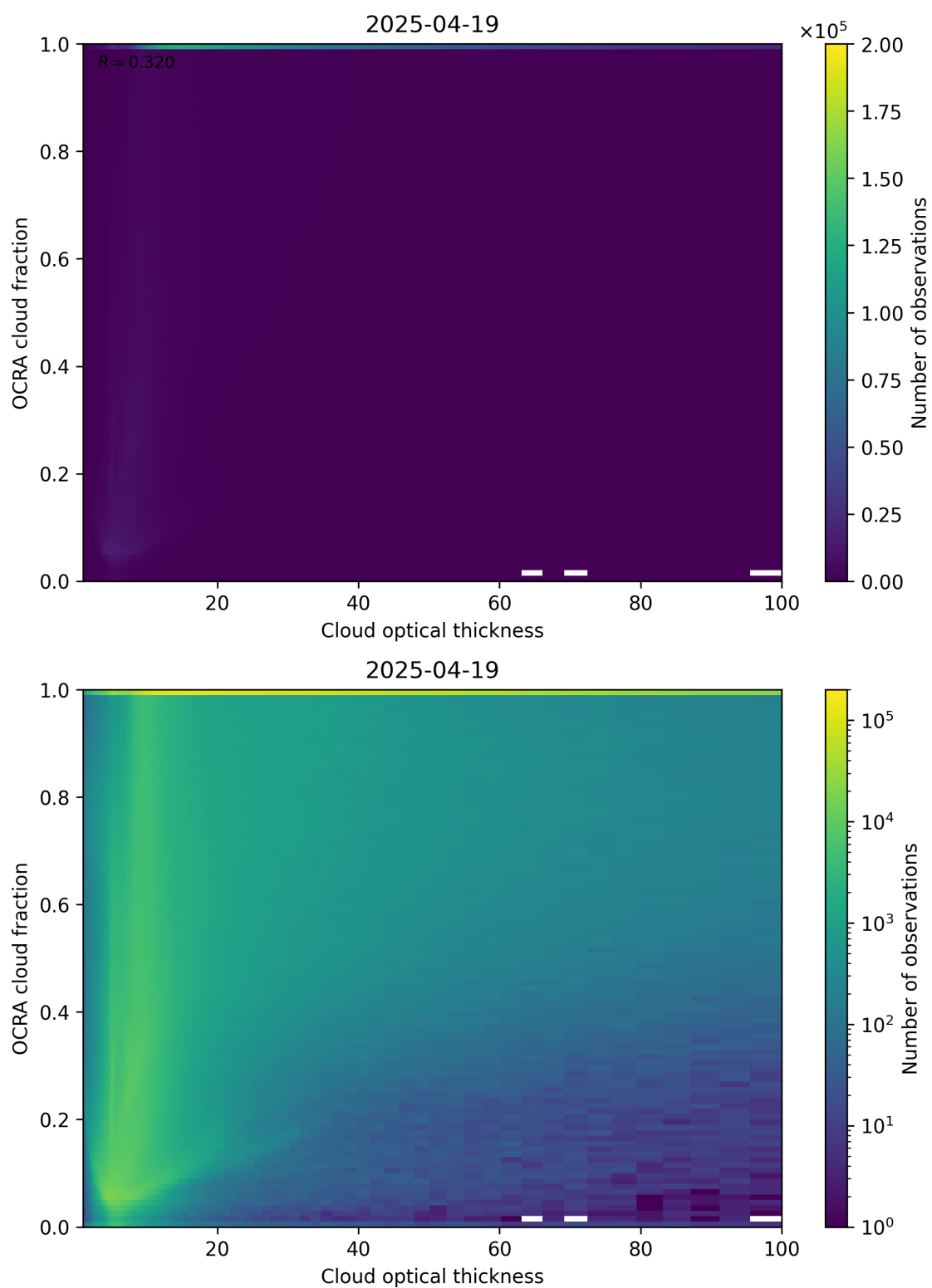
Figure 83: Scatter density plot of “Cloud optical thickness” against “OCRA cloud fraction” for 2025-04-19 to 2025-04-20.
