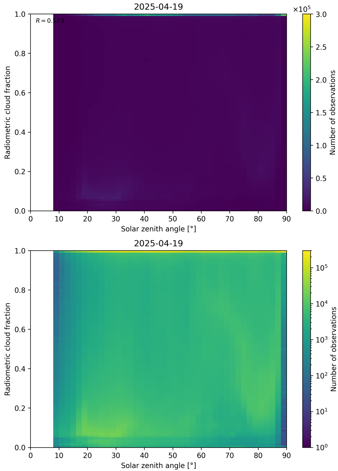
Figure 99: Scatter density plot of “Solar zenith angle” against “Radiometric cloud fraction” for 2025-04-19 to 2025-04-20.
