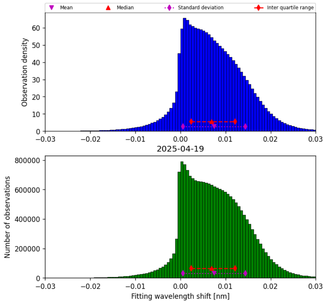
Figure 49: Histogram of “Fitting wavelength shift” for 2025-04-19 to 2025-04-20
