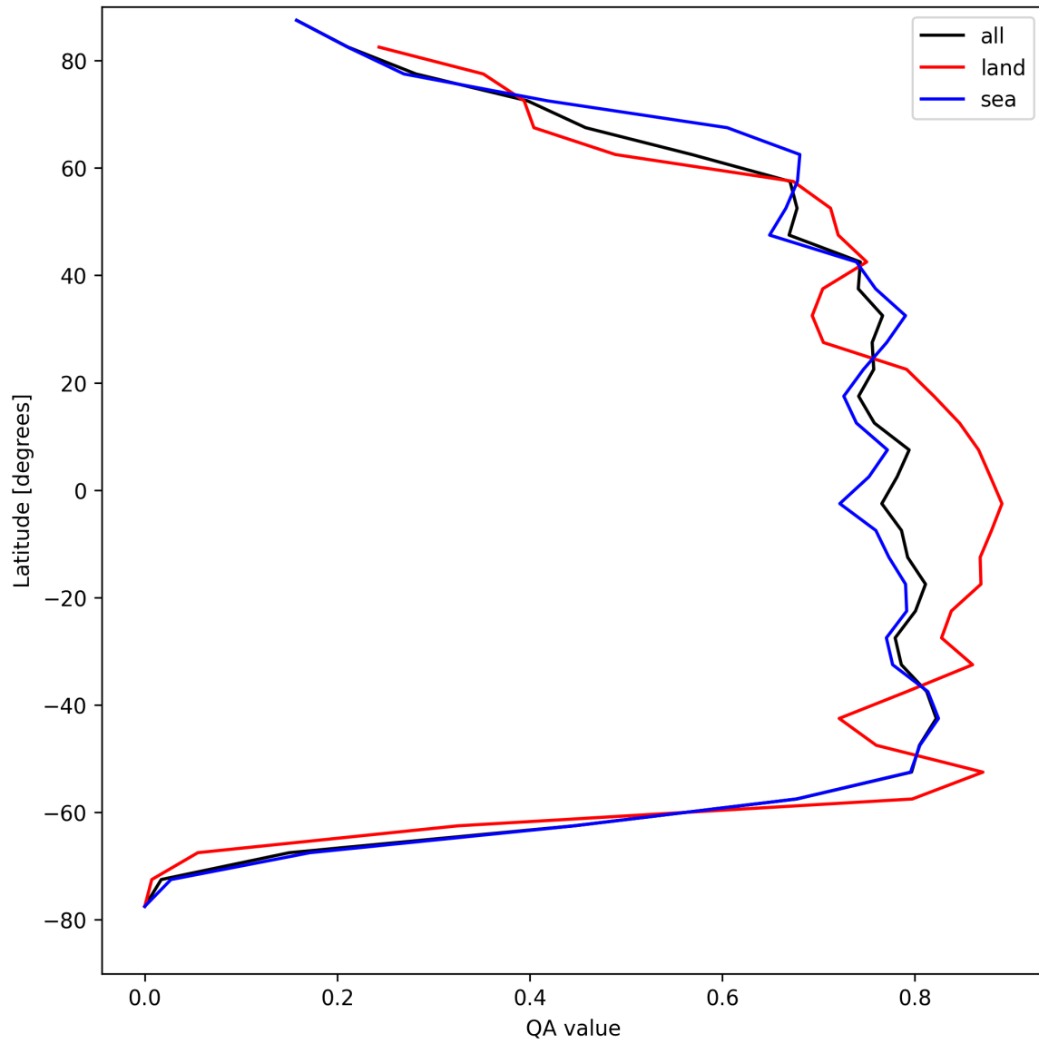
Figure 22: Zonal average of “QA value” for 2025-04-19 to 2025-04-20.
