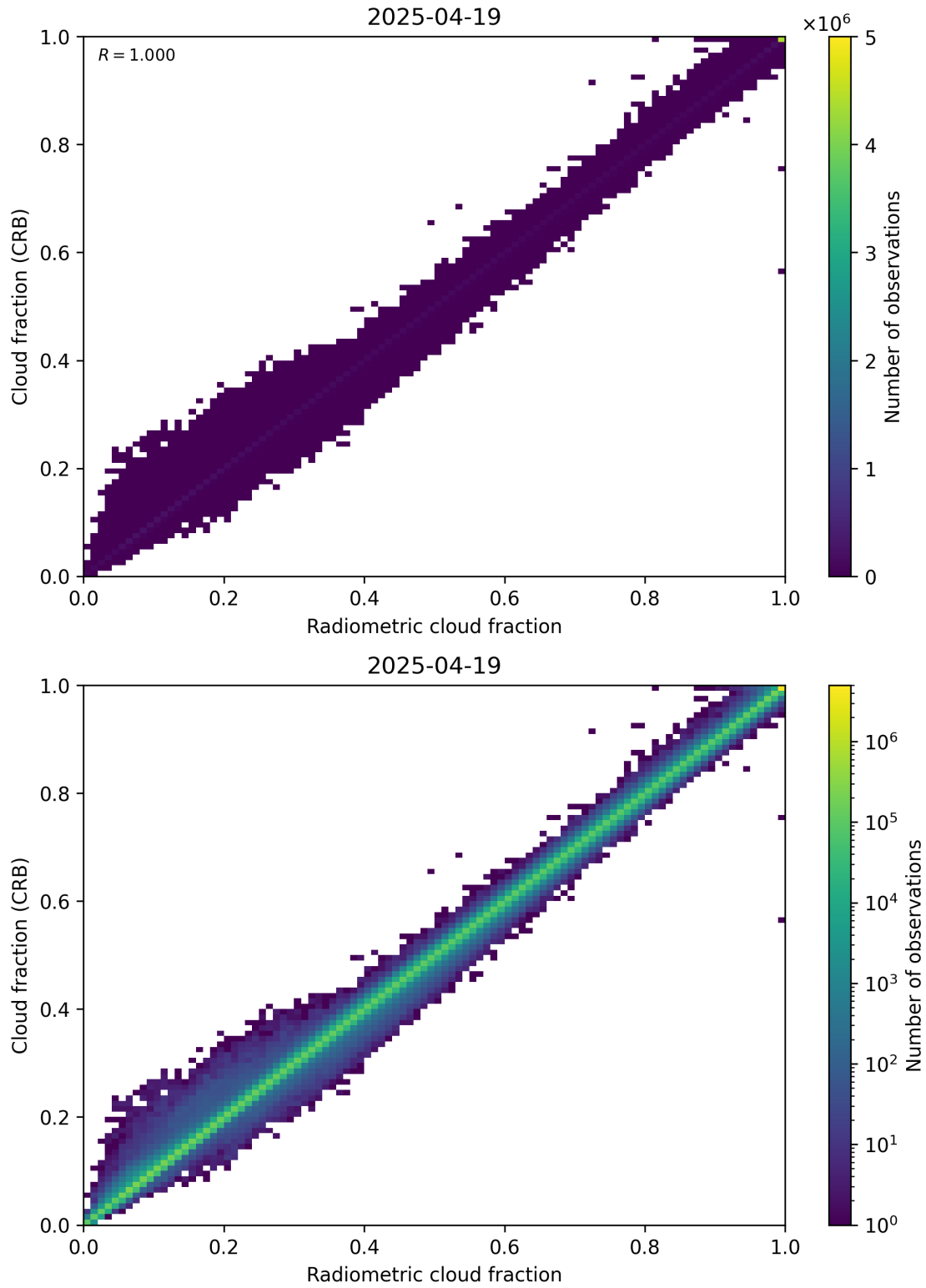
Figure 73: Scatter density plot of “Radiometric cloud fraction” against “Cloud fraction (CRB)” for 2025-04-19 to 2025-04-20.
