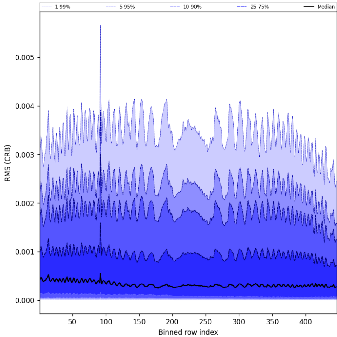
Figure 64: Along track statistics of “RMS (CRB)” for 2025-04-19 to 2025-04-20
