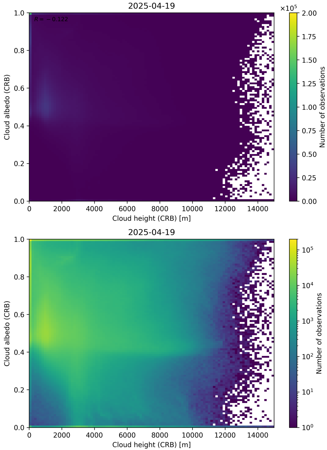
Figure 80: Scatter density plot of “Cloud height (CRB)” against “Cloud albedo (CRB)” for 2025-04-19 to 2025-04-20.
