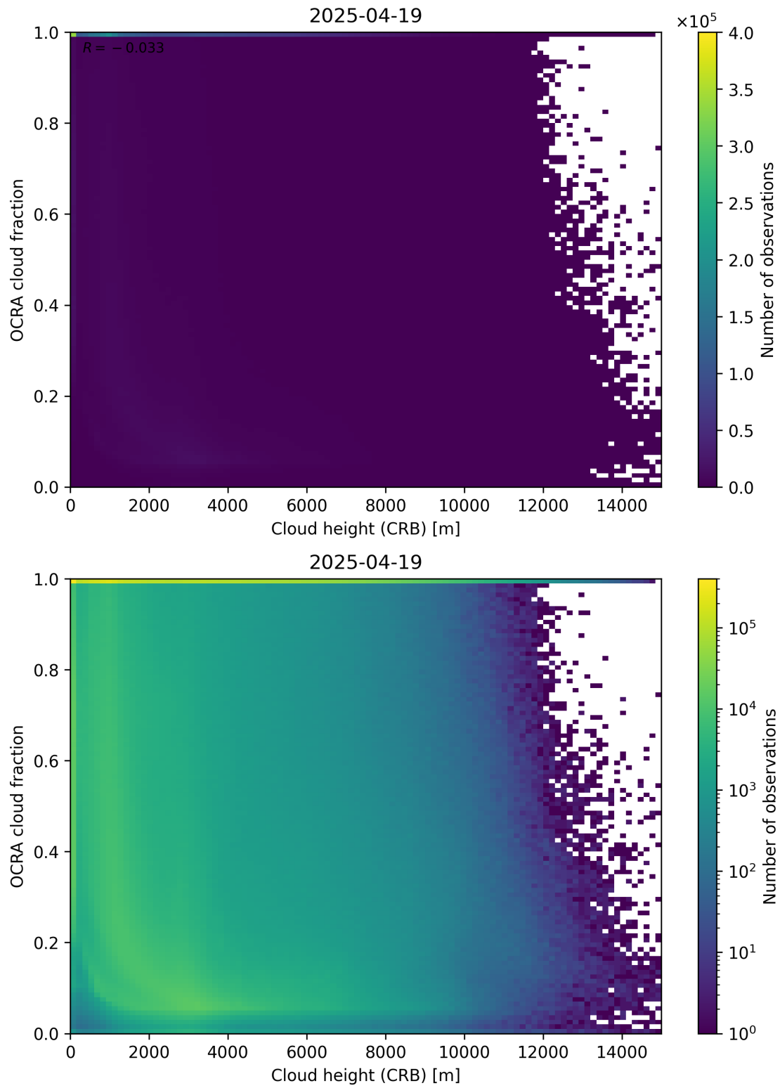
Figure 81: Scatter density plot of “Cloud height (CRB)” against “OCRA cloud fraction” for 2025-04-19 to 2025-04-20.
