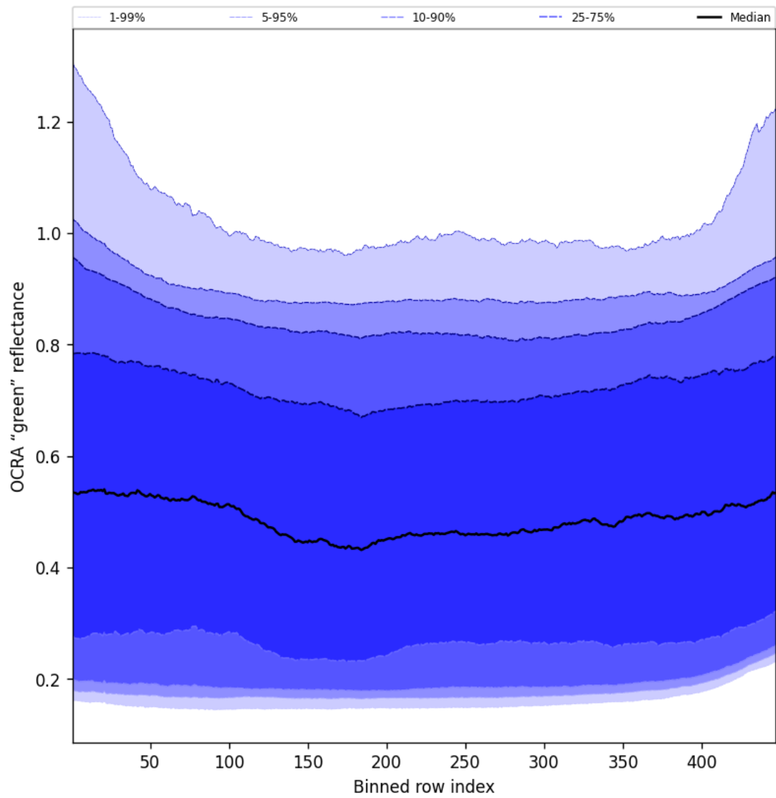
Figure 68: Along track statistics of “OCRA “green” reflectance” for 2025-04-19 to 2025-04-20
