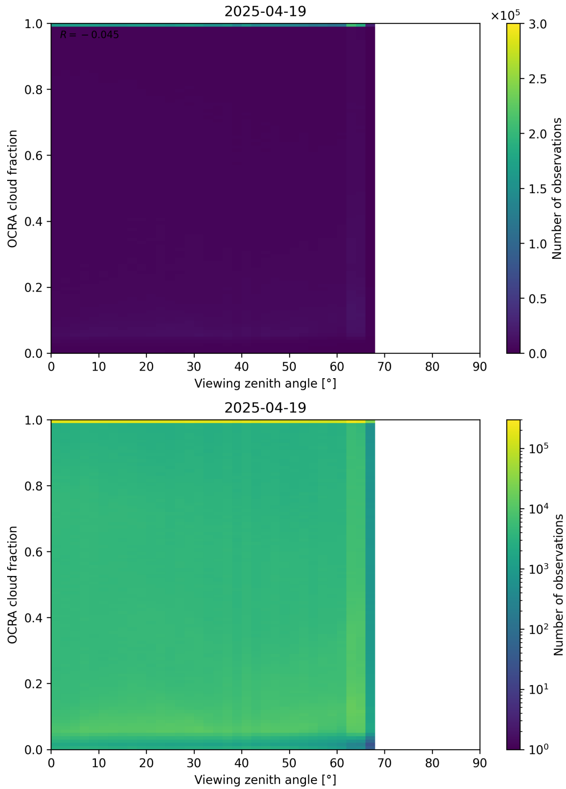
Figure 108: Scatter density plot of “Viewing zenith angle” against “OCRA cloud fraction” for 2025-04-19 to 2025-04-20.
