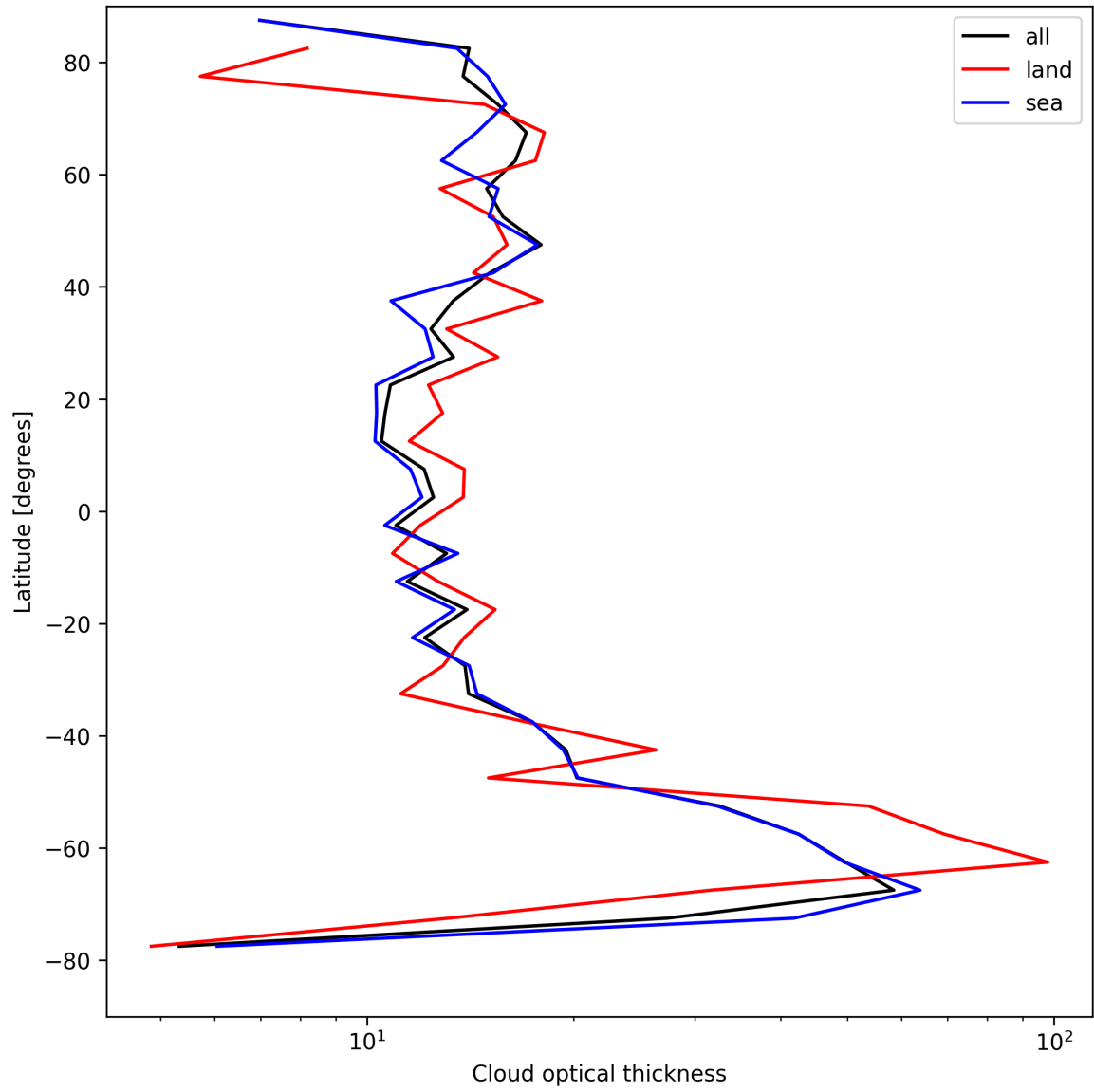
Figure 25: Zonal average of “Cloud optical thickness” for 2025-04-19 to 2025-04-20.
