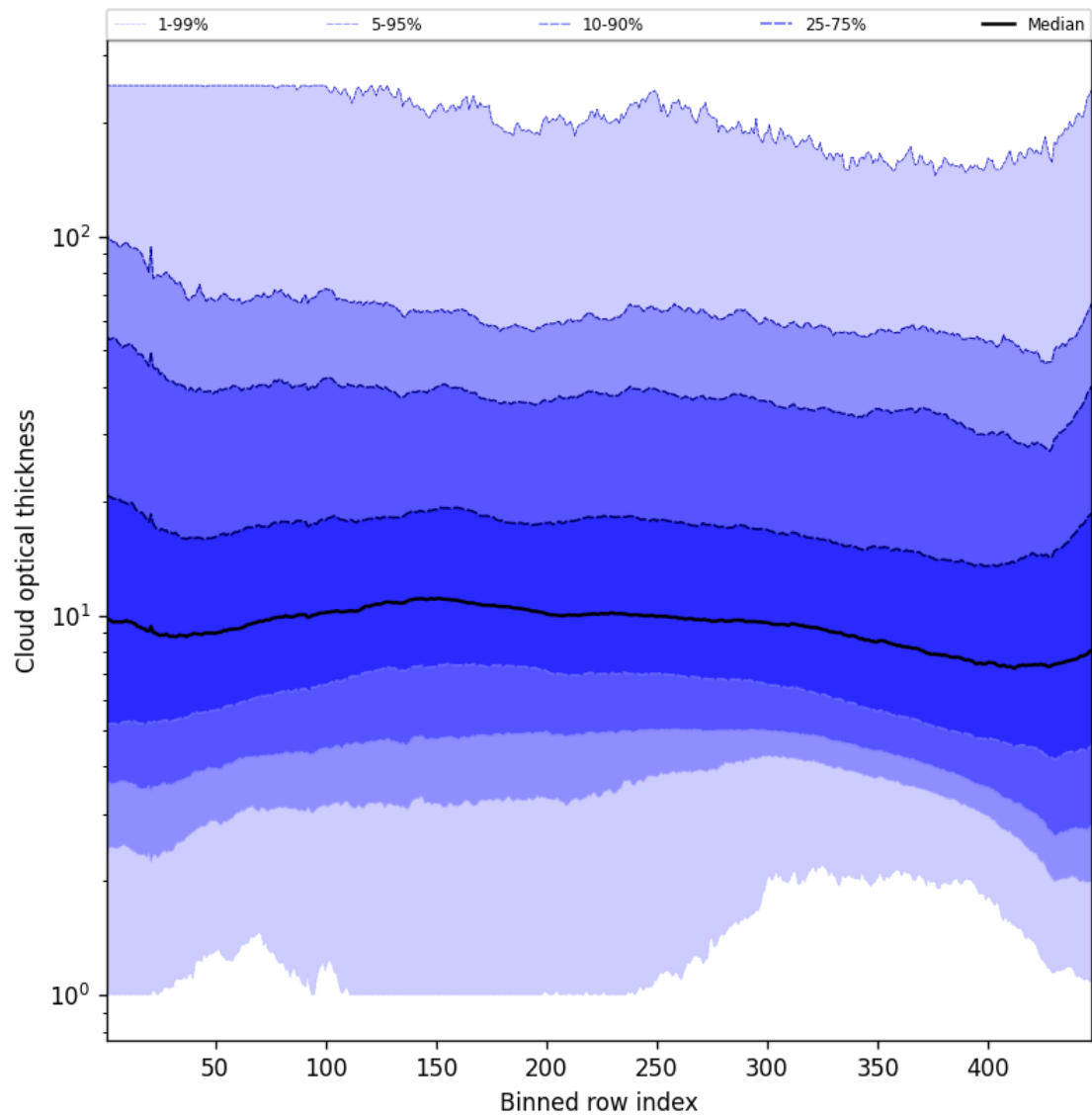
Figure 57: Along track statistics of “Cloud optical thickness” for 2025-04-19 to 2025-04-20
