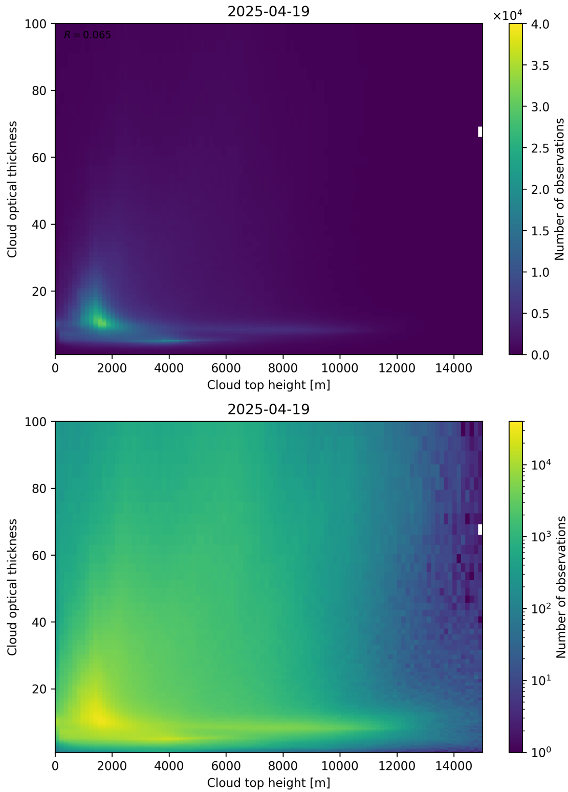
Figure 90: Scatter density plot of “Cloud top height” against “Cloud optical thickness” for 2025-04-19 to 2025-04-20.
