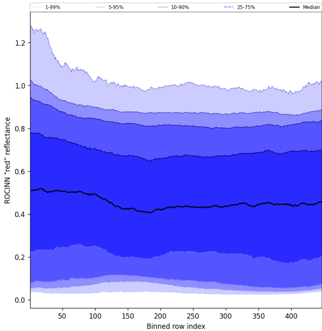
Figure 69: Along track statistics of "ROCINN "red" reflectance" for 2025-04-19 to 2025-04-20
