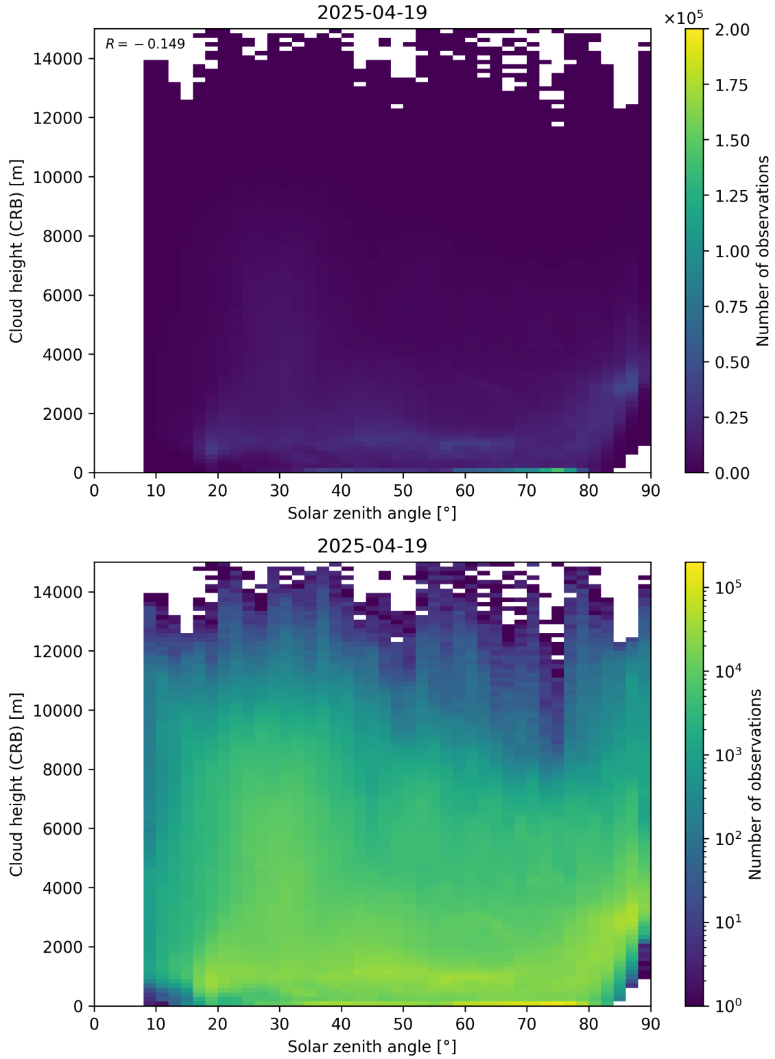
Figure 102: Scatter density plot of “Solar zenith angle” against “Cloud height (CRB)” for 2025-04-19 to 2025-04-20.
