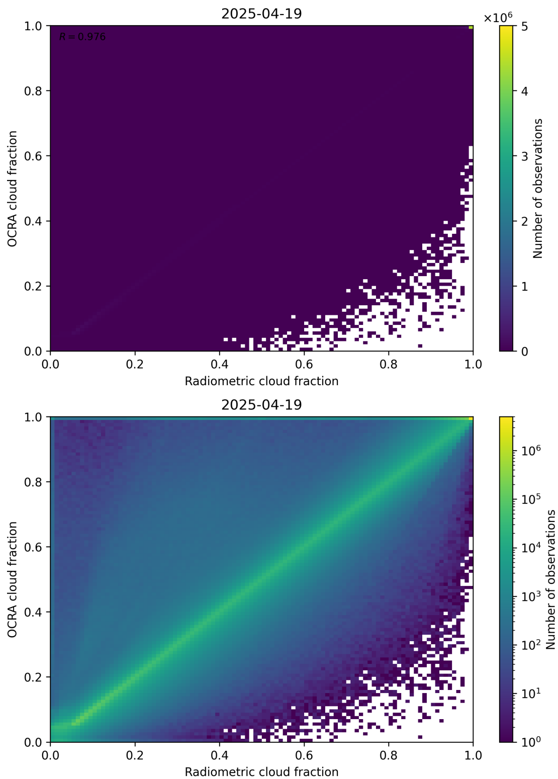
Figure 72: Scatter density plot of “Radiometric cloud fraction” against “OCRA cloud fraction” for 2025-04-19 to 2025-04-20.
