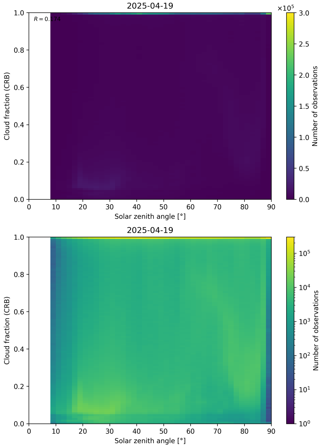
Figure 101: Scatter density plot of “Solar zenith angle” against “Cloud fraction (CRB)” for 2025-04-19 to 2025-04-20.
