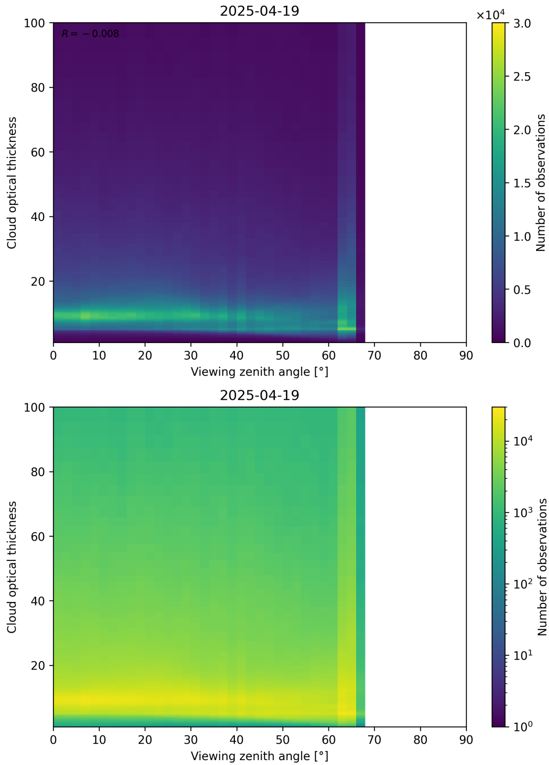
Figure 111: Scatter density plot of “Viewing zenith angle” against “Cloud optical thickness” for 2025-04-19 to 2025-04-20.
