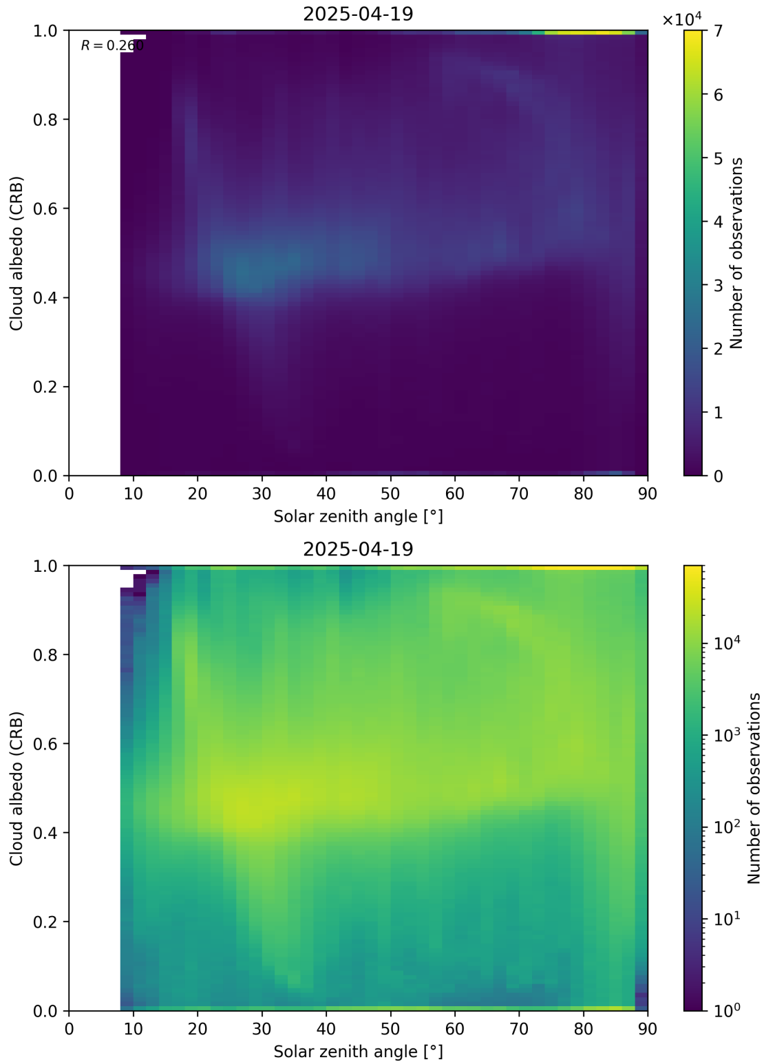
Figure 98: Scatter density plot of “Solar zenith angle” against “Cloud albedo (CRB)” for 2025-04-19 to 2025-04-20.
