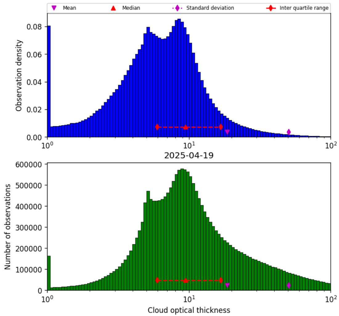
Figure 41: Histogram of “Cloud optical thickness” for 2025-04-19 to 2025-04-20
