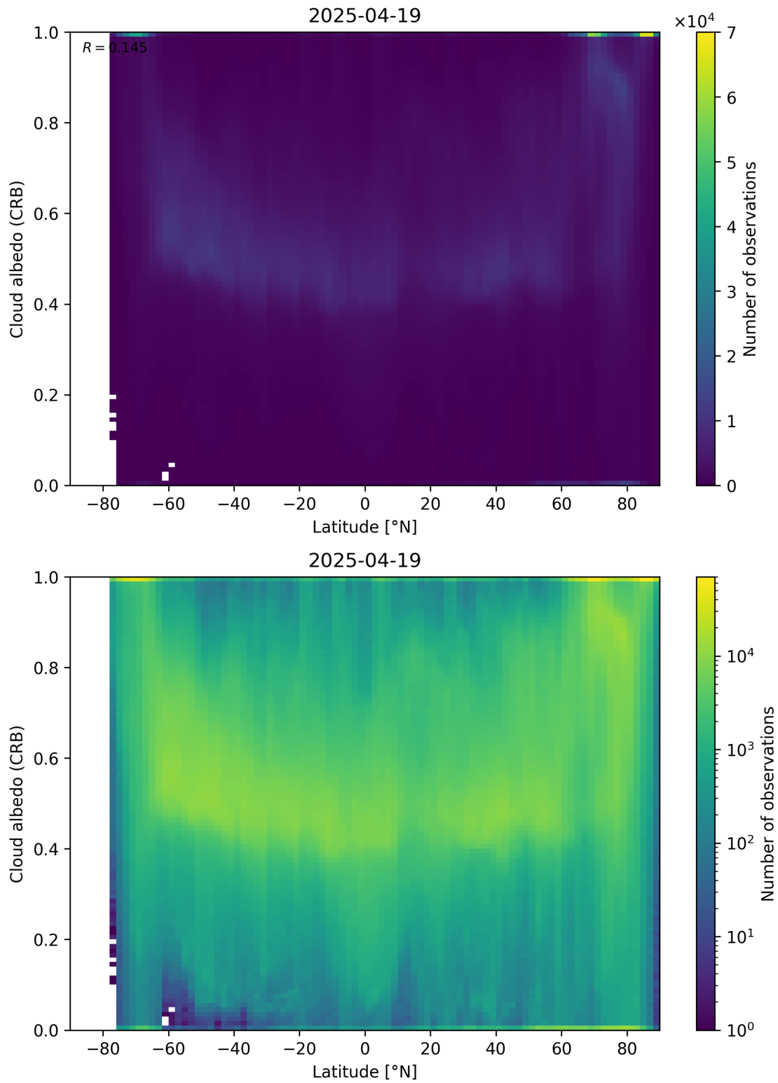
Figure 91: Scatter density plot of “Latitude” against “Cloud albedo (CRB)” for 2025-04-19 to 2025-04-20.
