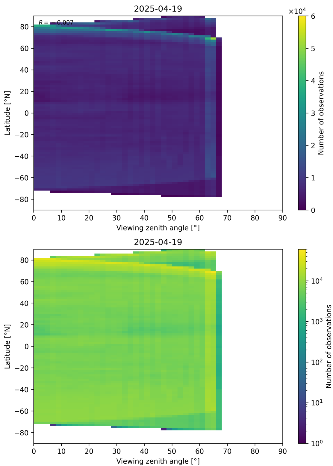
Figure 113: Scatter density plot of “Viewing zenith angle” against “Latitude” for 2025-04-19 to 2025-04-20.
