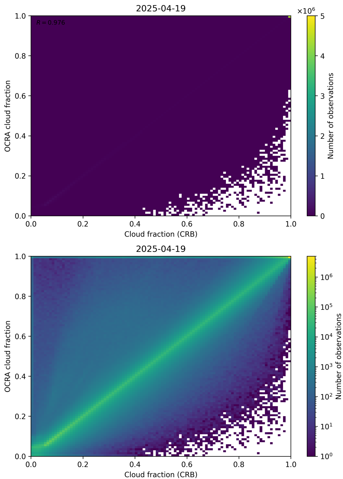
Figure 78: Scatter density plot of “Cloud fraction (CRB)” against “OCRA cloud fraction” for 2025-04-19 to 2025-04-20.
