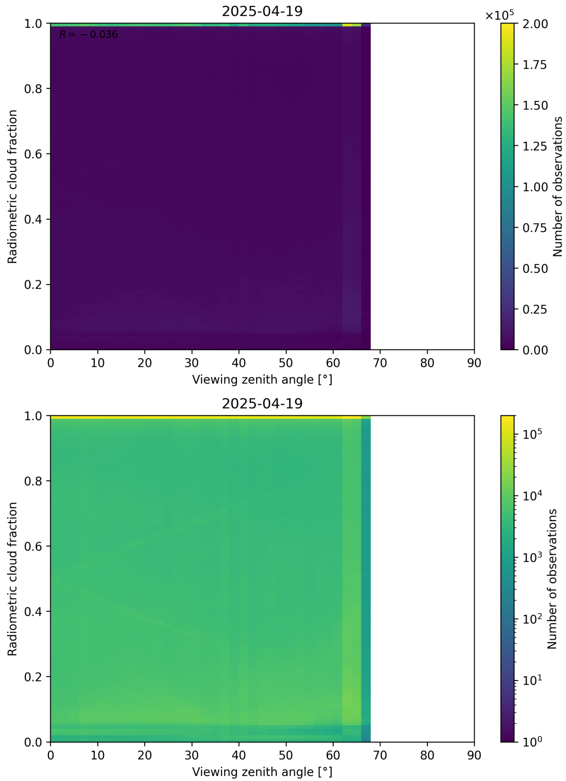
Figure 107: Scatter density plot of “Viewing zenith angle” against “Radiometric cloud fraction” for 2025-04-19 to 2025-04-20.
