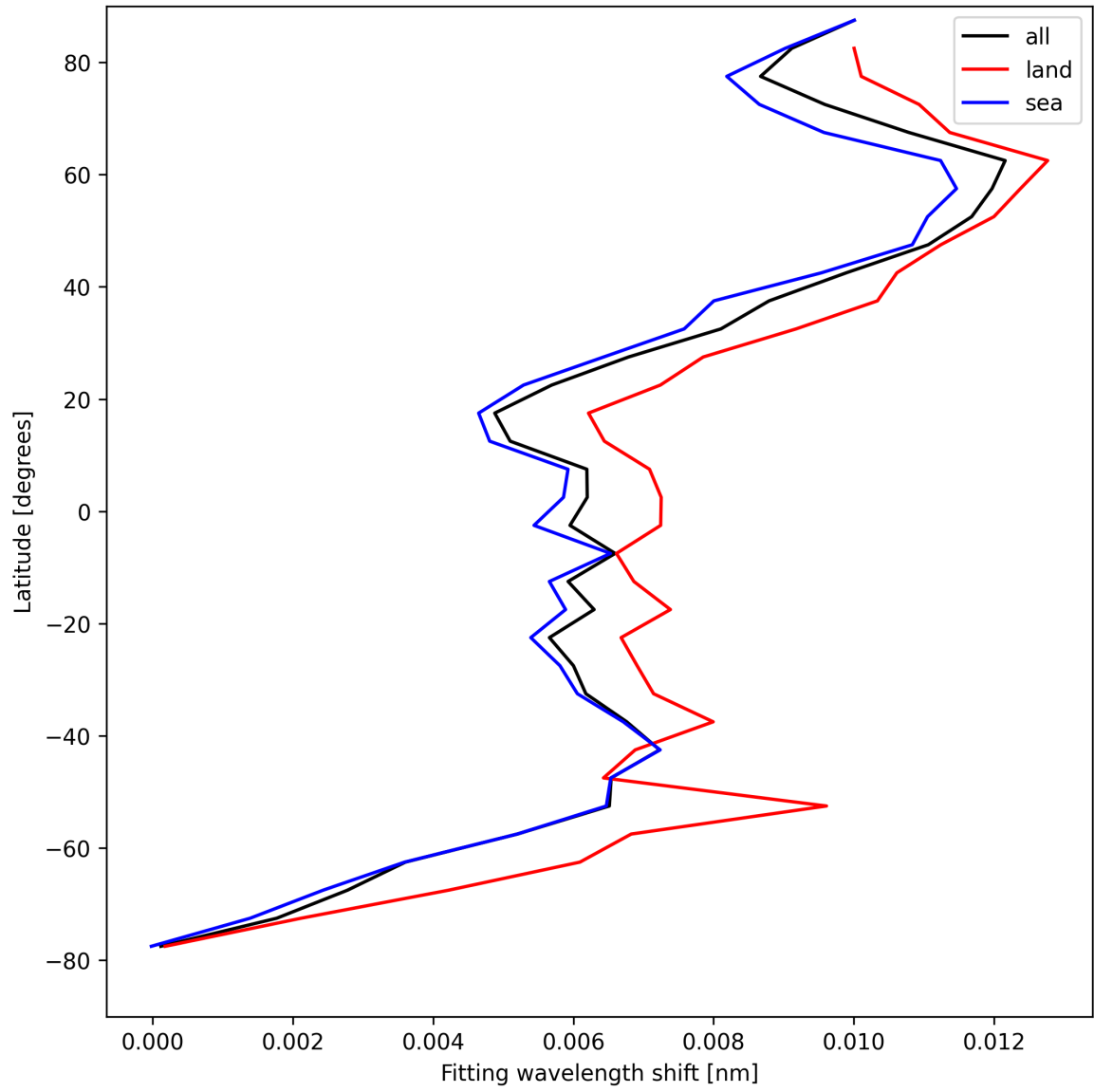
Figure 33: Zonal average of “Fitting wavelength shift” for 2025-04-19 to 2025-04-20.
