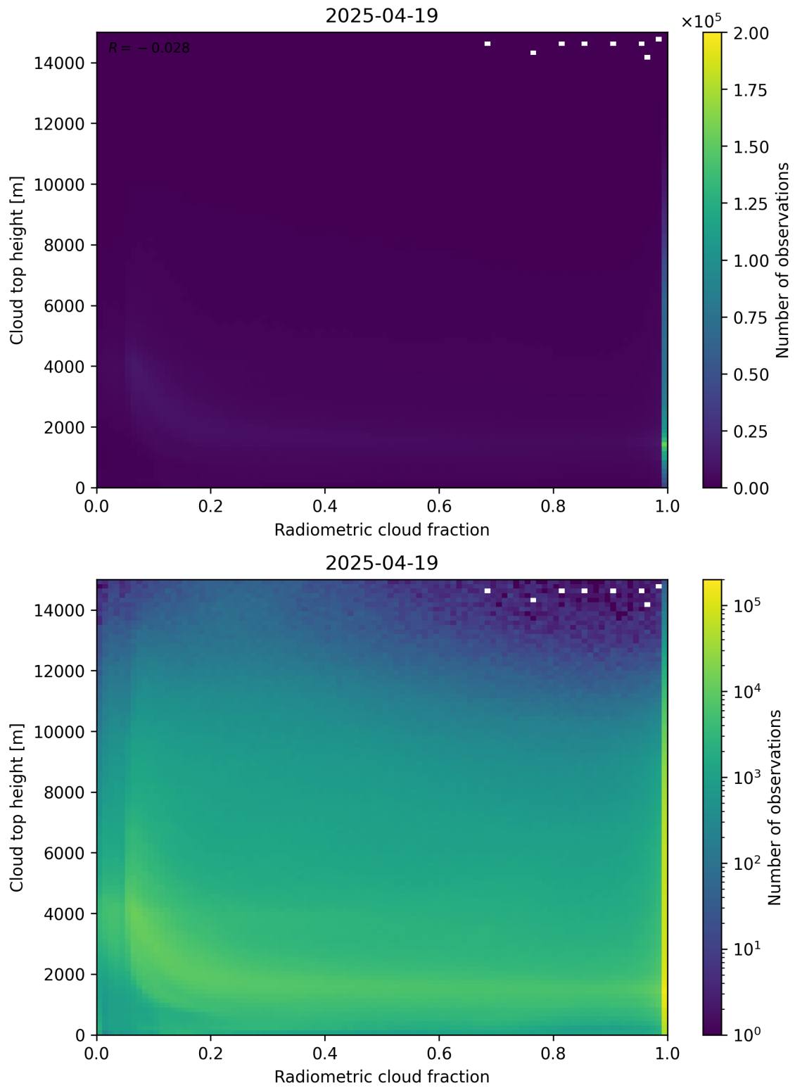
Figure 76: Scatter density plot of “Radiometric cloud fraction” against “Cloud top height” for 2025-04-19 to 2025-04-20.
