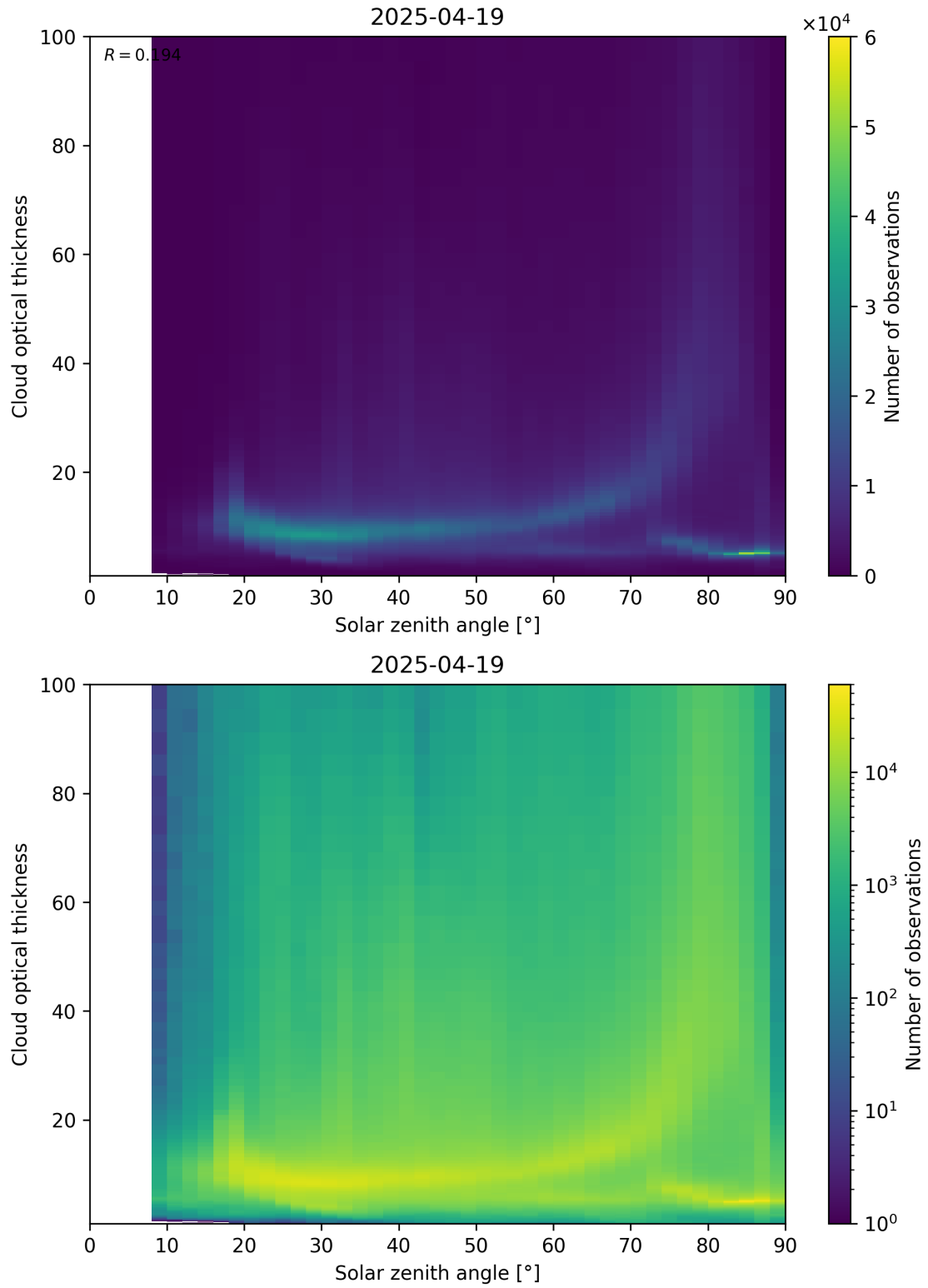
Figure 103: Scatter density plot of “Solar zenith angle” against “Cloud optical thickness” for 2025-04-19 to 2025-04-20.
