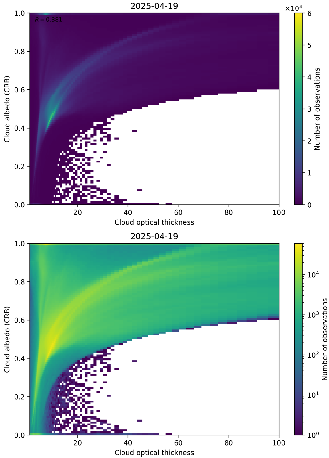
Figure 82: Scatter density plot of “Cloud optical thickness” against “Cloud albedo (CRB)” for 2025-04-19 to 2025-04-20.
