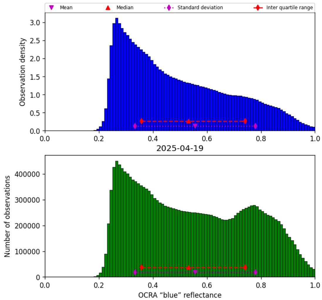
Figure 51: Histogram of “OCRA “blue” reflectance” for 2025-04-19 to 2025-04-20
