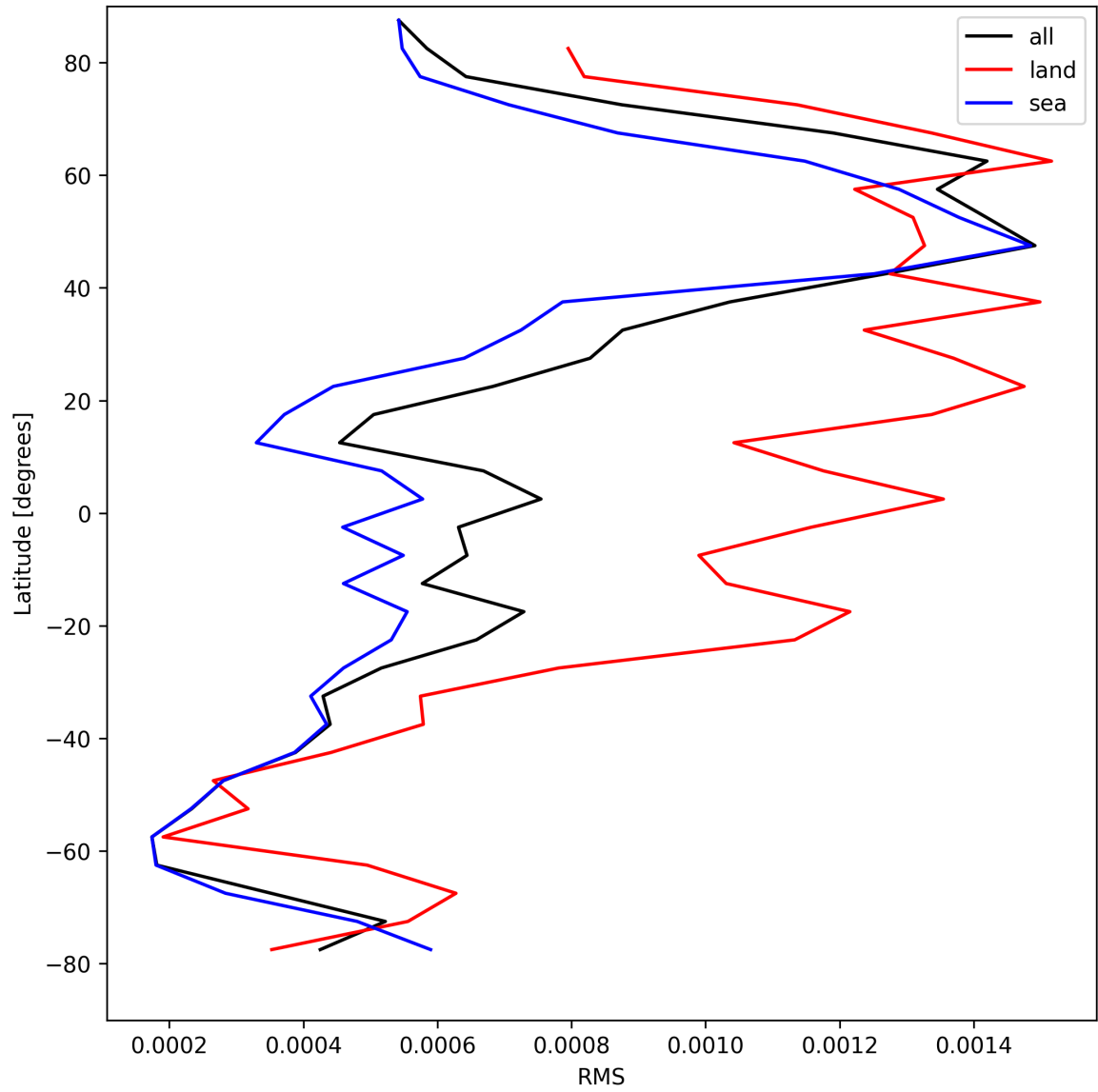
Figure 31: Zonal average of “RMS” for 2025-04-19 to 2025-04-20.
