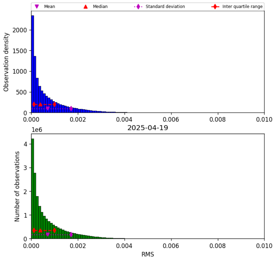
Figure 47: Histogram of “RMS” for 2025-04-19 to 2025-04-20
