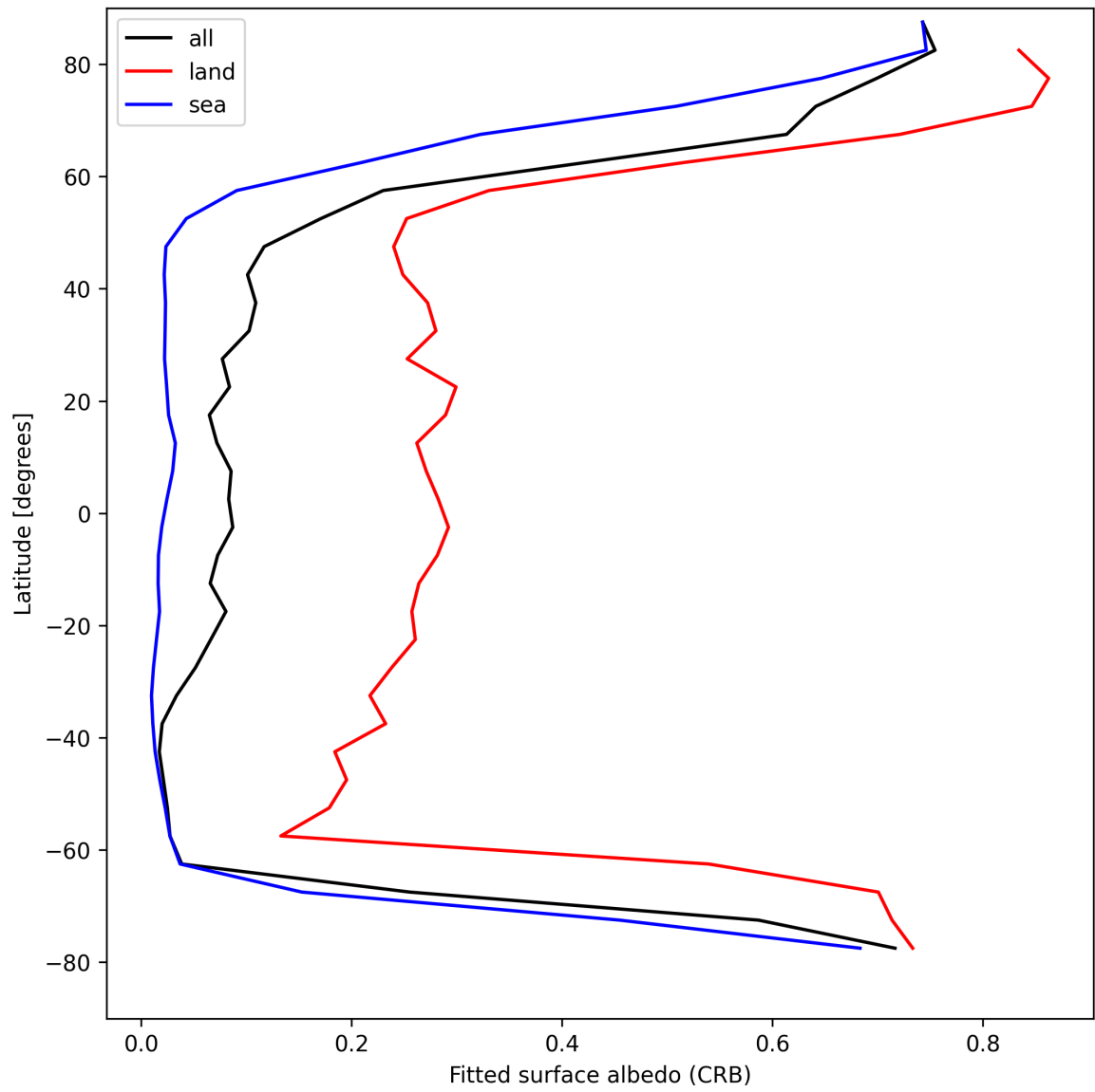
Figure 30: Zonal average of “Fitted surface albedo (CRB)” for 2025-04-19 to 2025-04-20.
