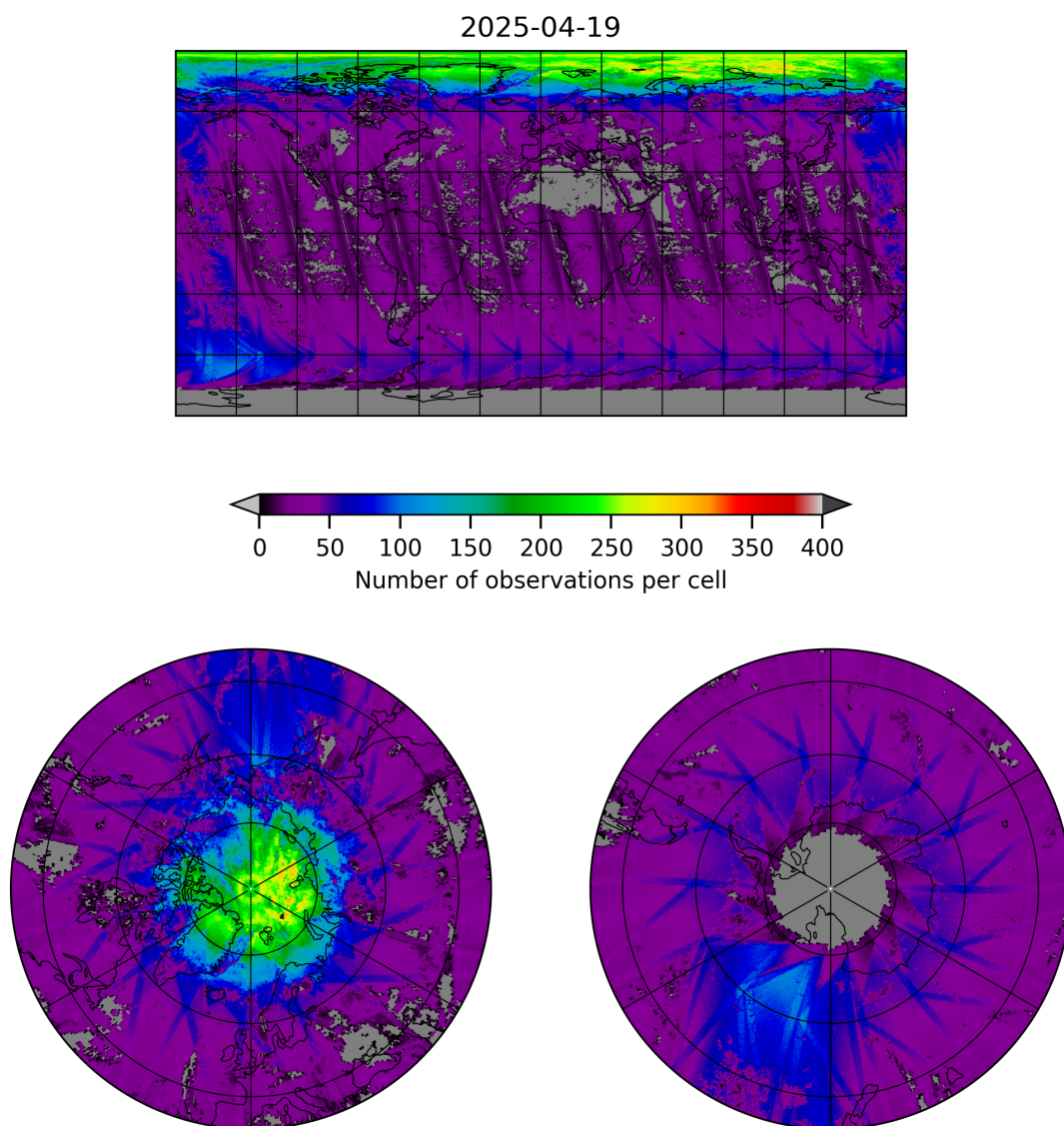
Figure 21: Map of the number of observations for 2025-04-19 to 2025-04-20
