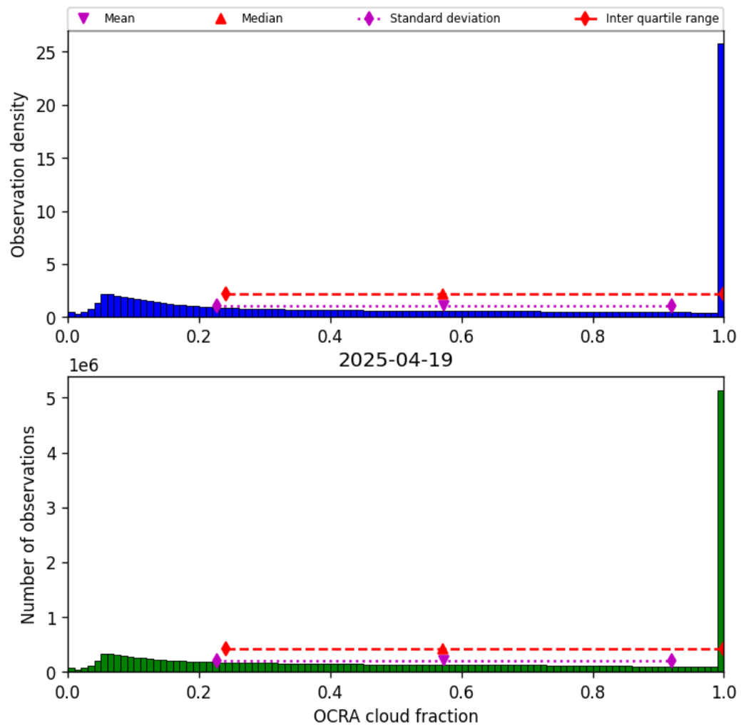
Figure 50: Histogram of “OCRA cloud fraction” for 2025-04-19 to 2025-04-20
