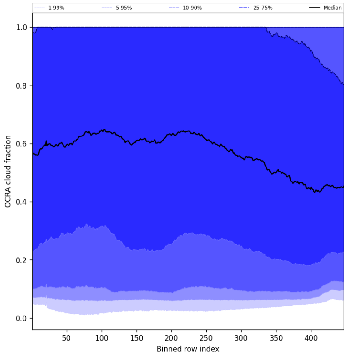
Figure 66: Along track statistics of “OCRA cloud fraction” for 2025-04-19 to 2025-04-20
