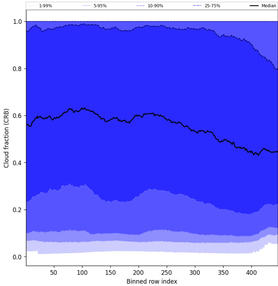
Figure 58: Along track statistics of “Cloud fraction (CRB)” for 2025-04-19 to 2025-04-20
