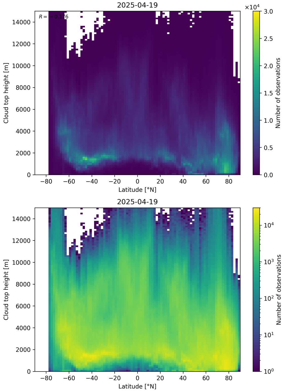
Figure 97: Scatter density plot of “Latitude” against “Cloud top height” for 2025-04-19 to 2025-04-20.
