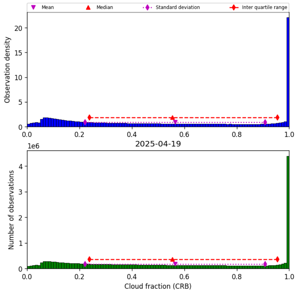
Figure 42: Histogram of “Cloud fraction (CRB)” for 2025-04-19 to 2025-04-20
