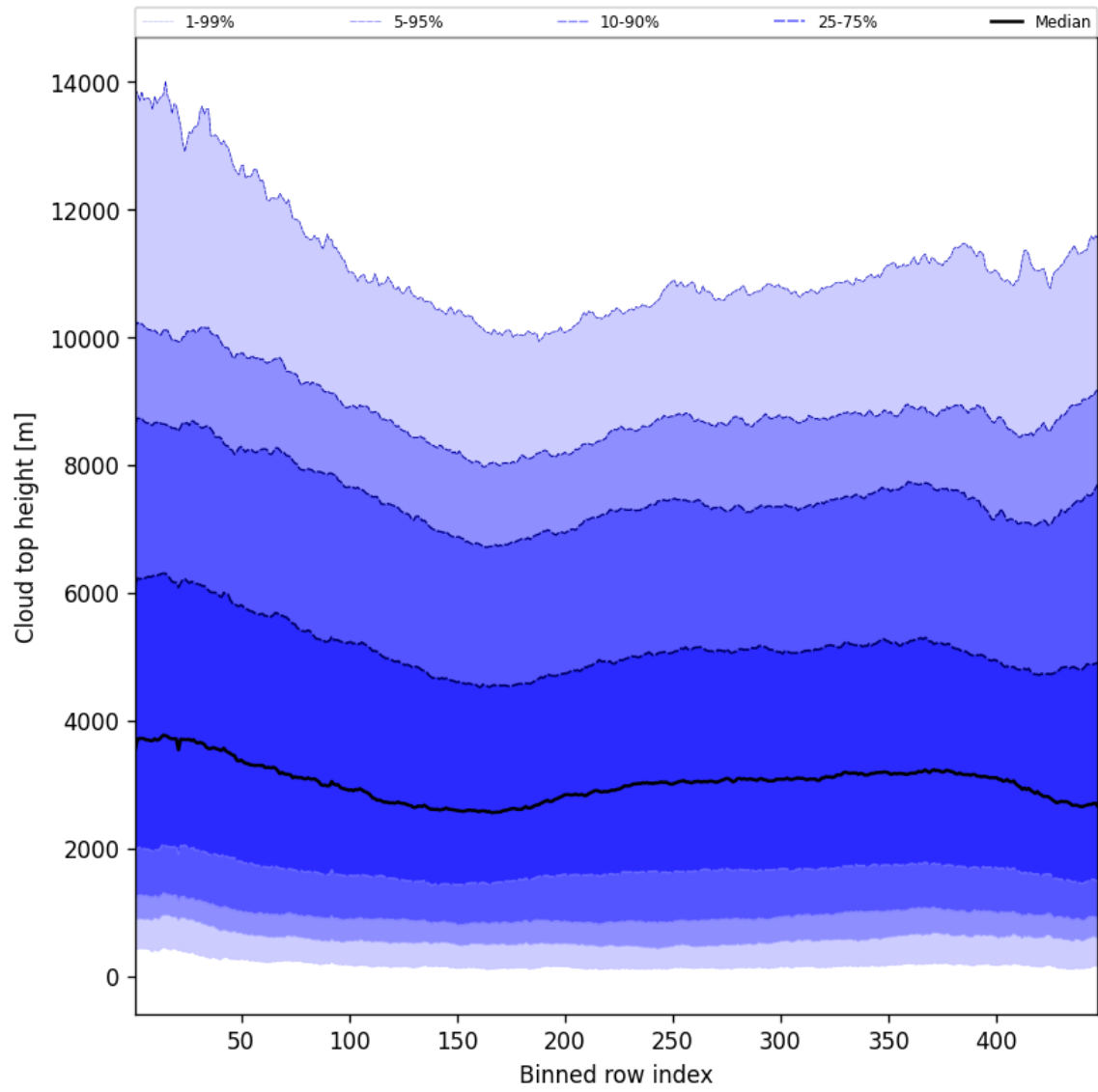
Figure 56: Along track statistics of “Cloud top height” for 2025-04-19 to 2025-04-20
