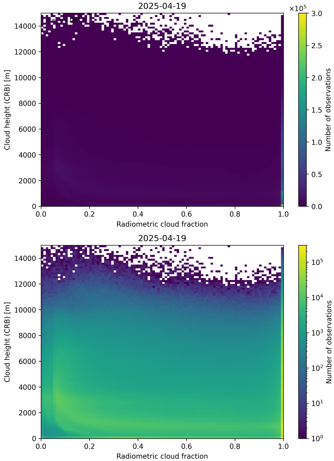
Figure 74: Scatter density plot of “Radiometric cloud fraction” against “Cloud height (CRB)” for 2025-04-19 to 2025-04-20.
