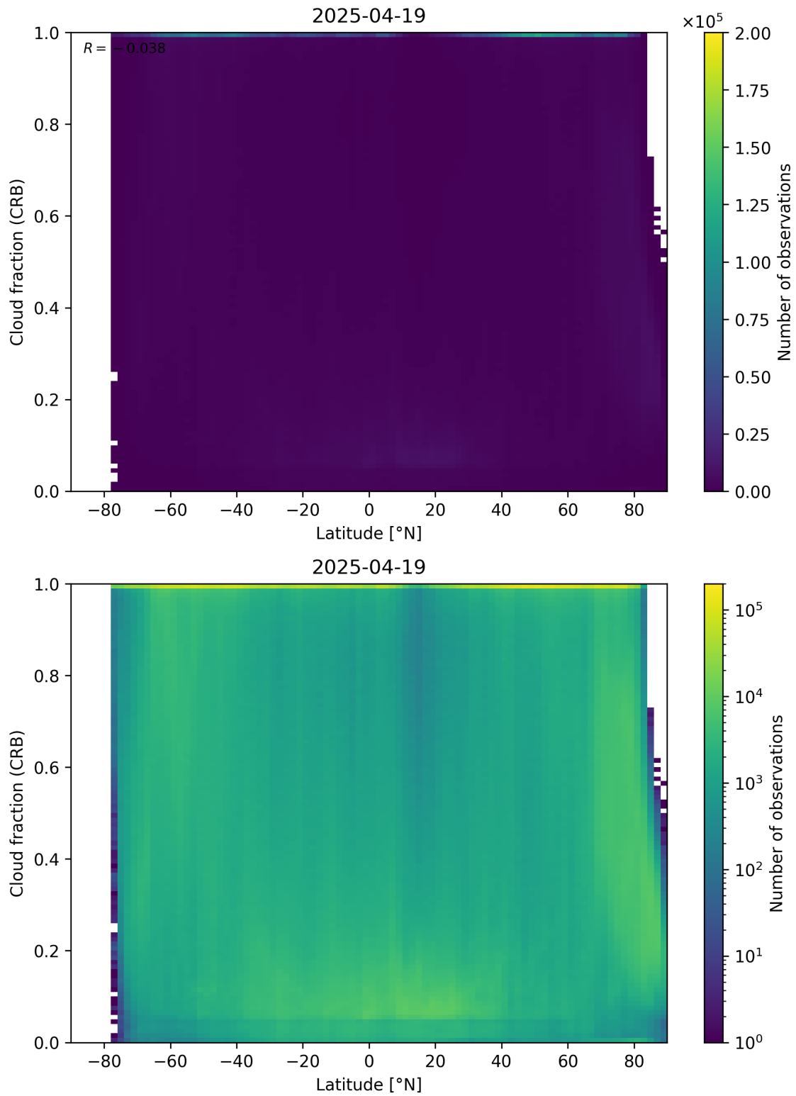
Figure 94: Scatter density plot of “Latitude” against “Cloud fraction (CRB)” for 2025-04-19 to 2025-04-20.
