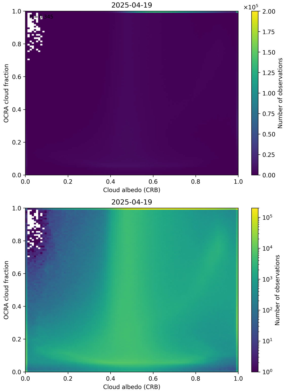
Figure 70: Scatter density plot of “Cloud albedo (CRB)” against “OCRA cloud fraction” for 2025-04-19 to 2025-04-20.
