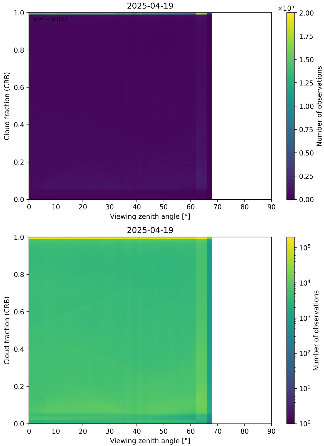
Figure 109: Scatter density plot of “Viewing zenith angle” against “Cloud fraction (CRB)” for 2025-04-19 to 2025-04-20.
