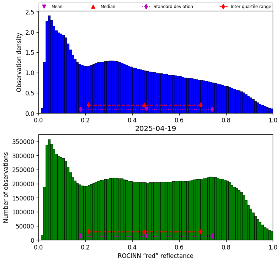
Figure 53: Histogram of “ROCINN “red” reflectance” for 2025-04-19 to 2025-04-20
