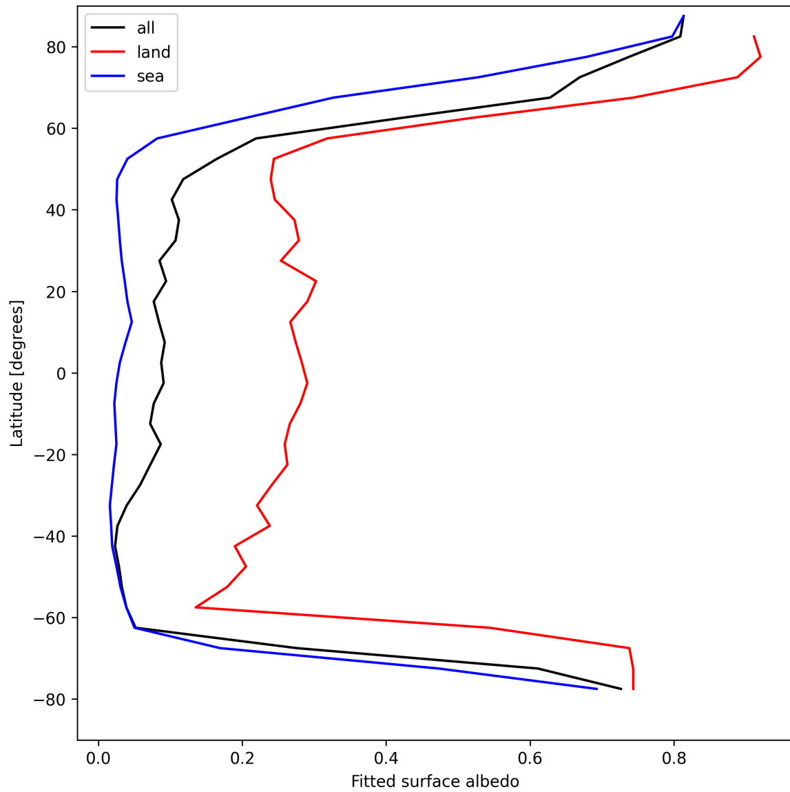
Figure 29: Zonal average of “Fitted surface albedo” for 2025-04-19 to 2025-04-20.
