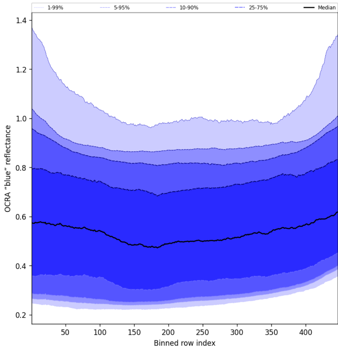
Figure 67: Along track statistics of “OCRA “blue” reflectance” for 2025-04-19 to 2025-04-20
