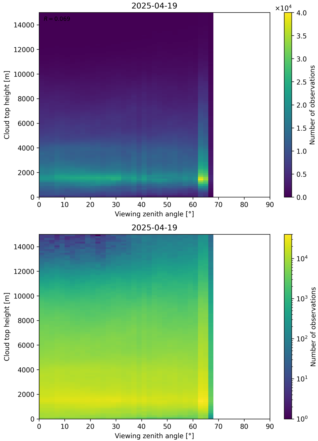
Figure 112: Scatter density plot of “Viewing zenith angle” against “Cloud top height” for 2025-04-19 to 2025-04-20.
