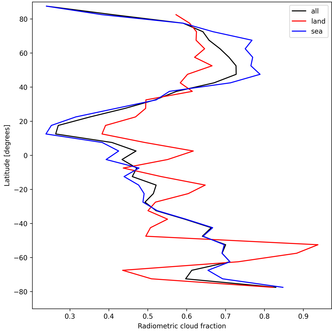
Figure 23: Zonal average of “Radiometric cloud fraction” for 2025-04-19 to 2025-04-20.
