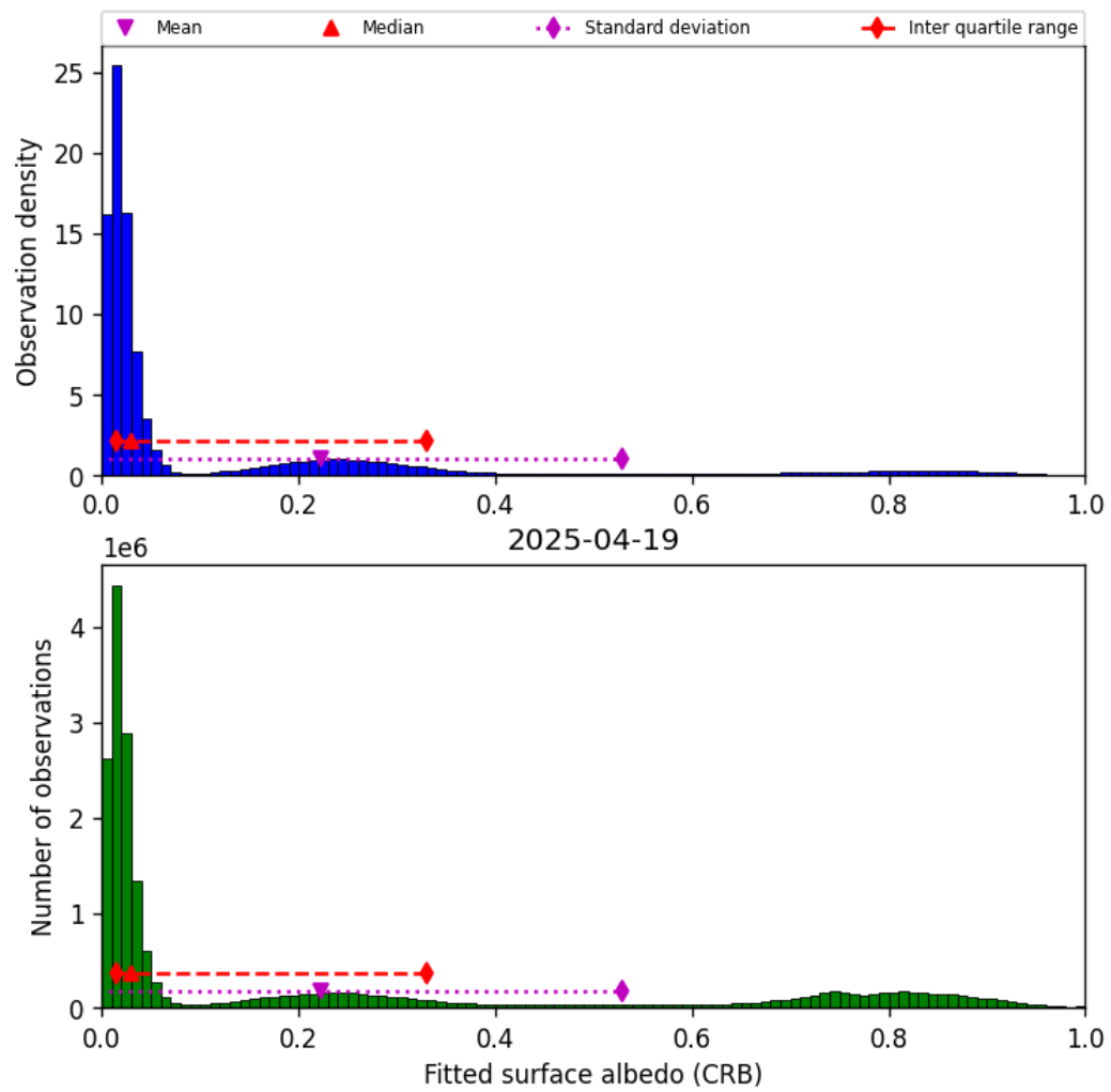
Figure 46: Histogram of “Fitted surface albedo (CRB)” for 2025-04-19 to 2025-04-20
