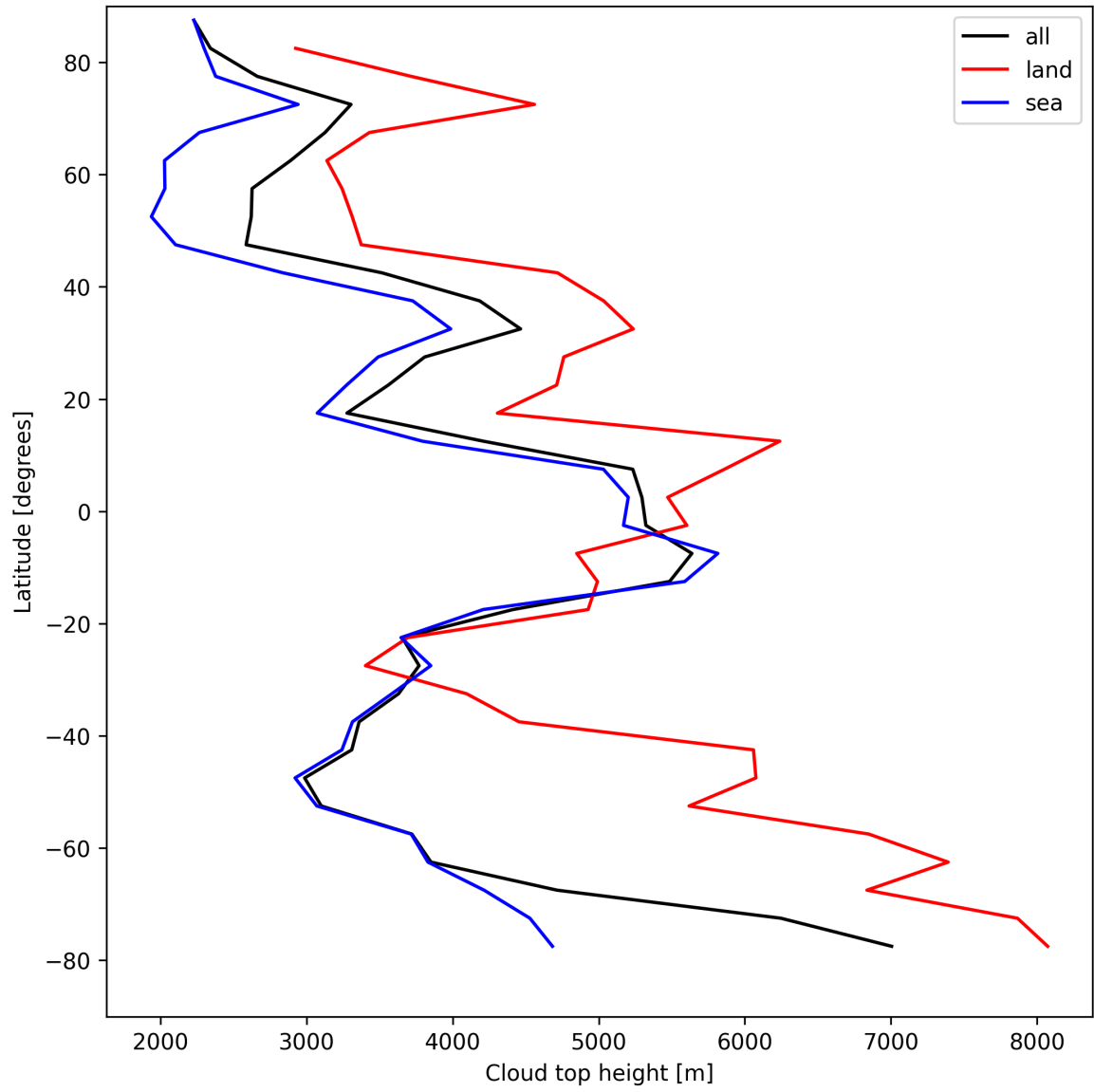
Figure 24: Zonal average of “Cloud top height” for 2025-04-19 to 2025-04-20.
