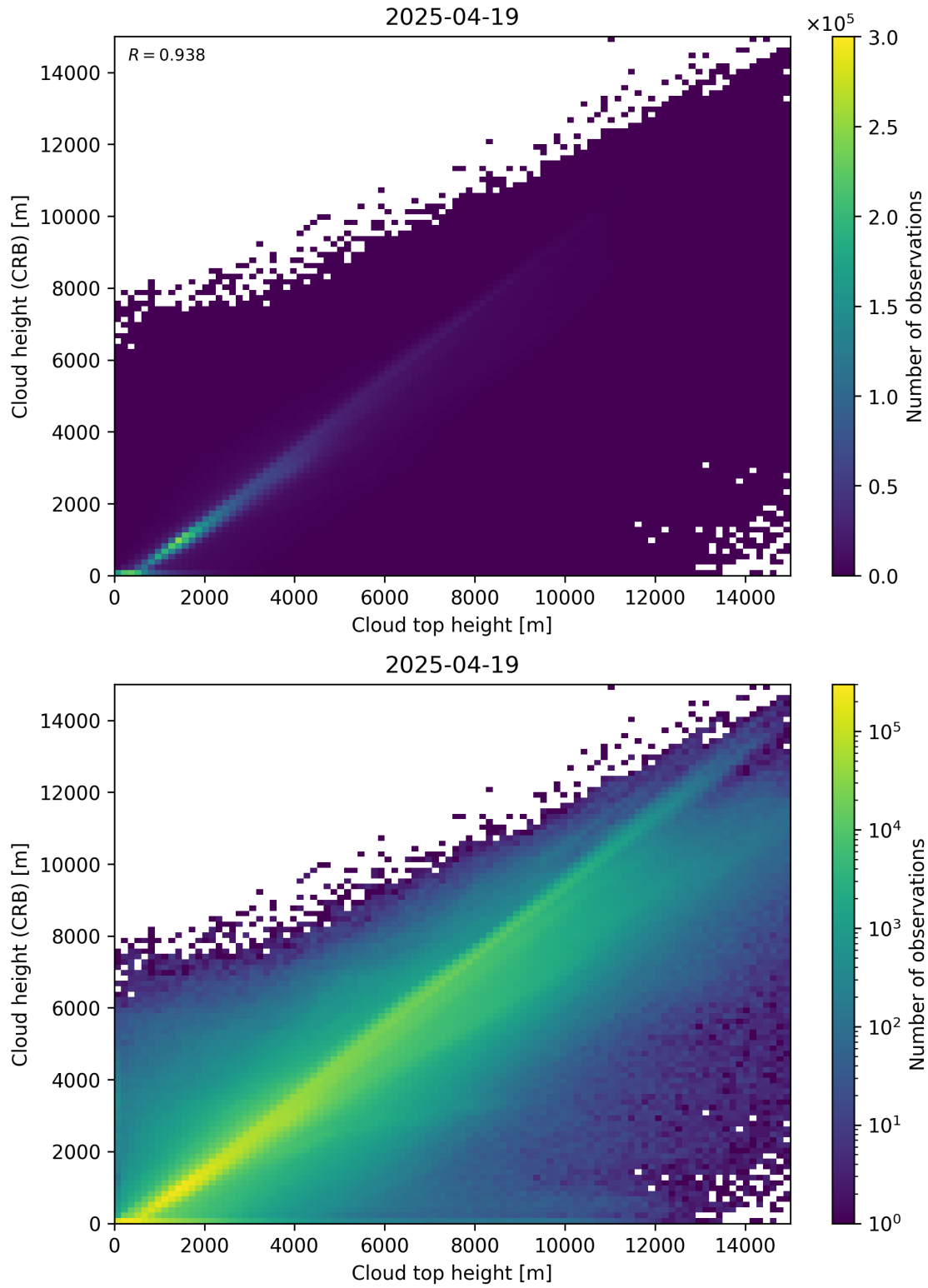
Figure 89: Scatter density plot of “Cloud top height” against “Cloud height (CRB)” for 2025-04-19 to 2025-04-20.
