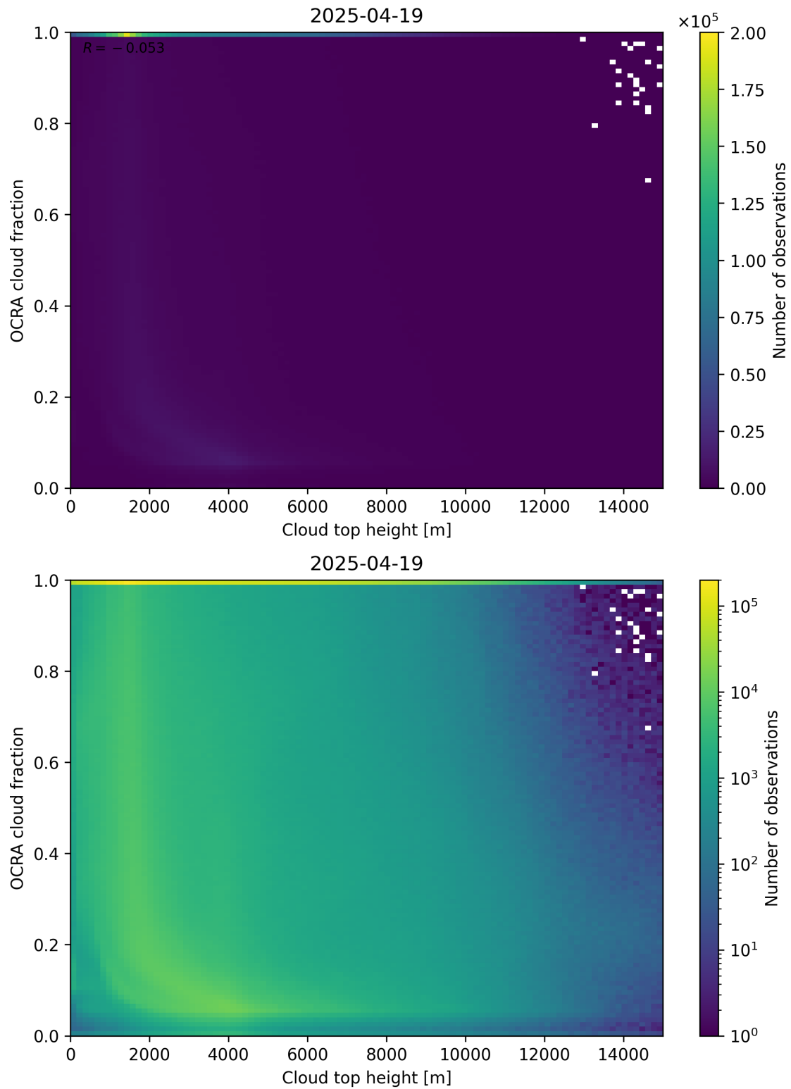
Figure 87: Scatter density plot of “Cloud top height” against “OCRA cloud fraction” for 2025-04-19 to 2025-04-20.
