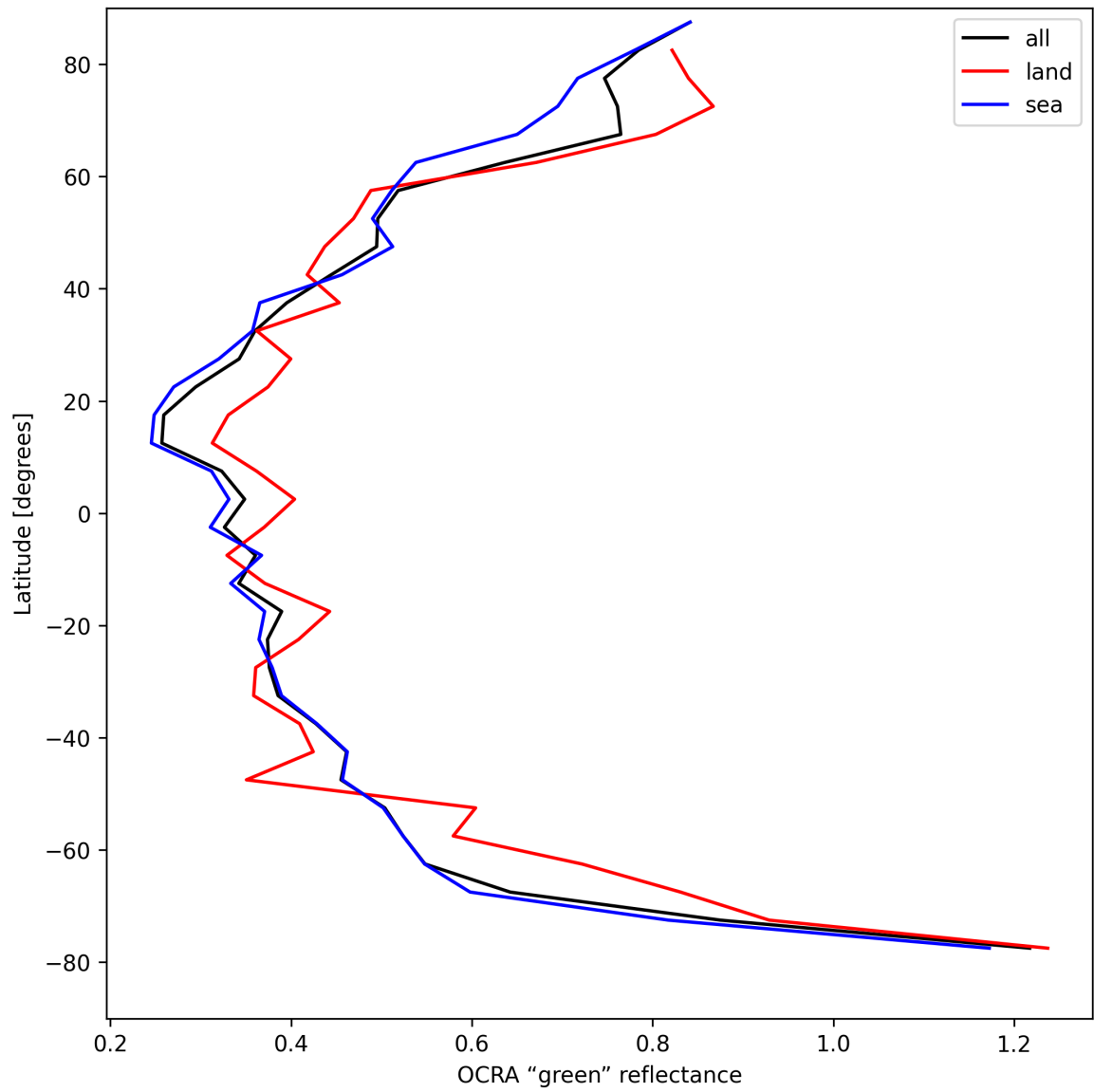
Figure 36: Zonal average of “OCRA “green” reflectance” for 2025-04-19 to 2025-04-20.
