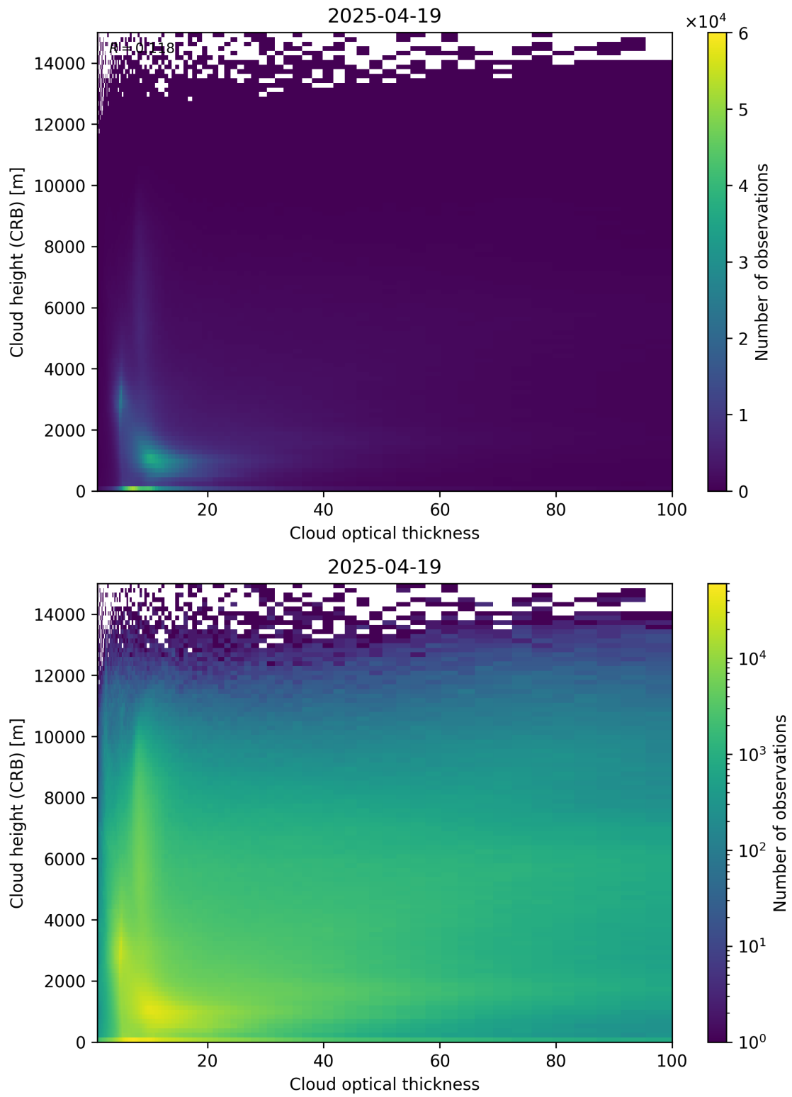
Figure 85: Scatter density plot of “Cloud optical thickness” against “Cloud height (CRB)” for 2025-04-19 to 2025-04-20.
