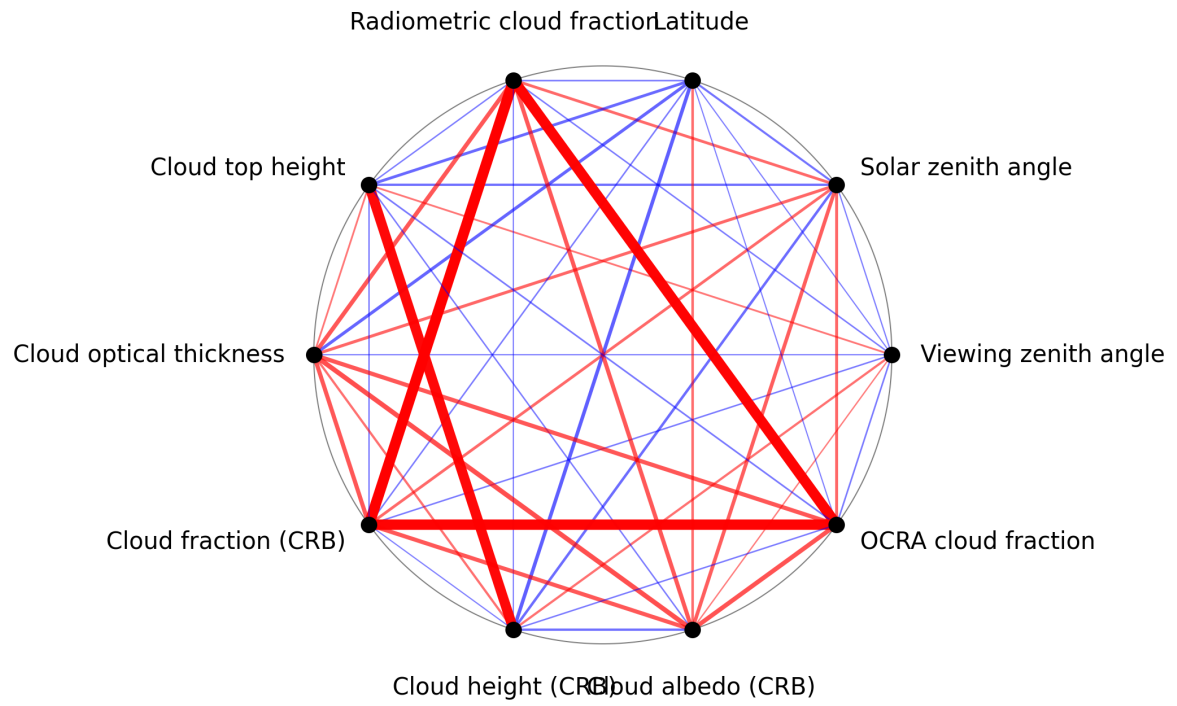
Figure 1: Map of correlation graph for 2025-04-19 to 2025-04-20.
