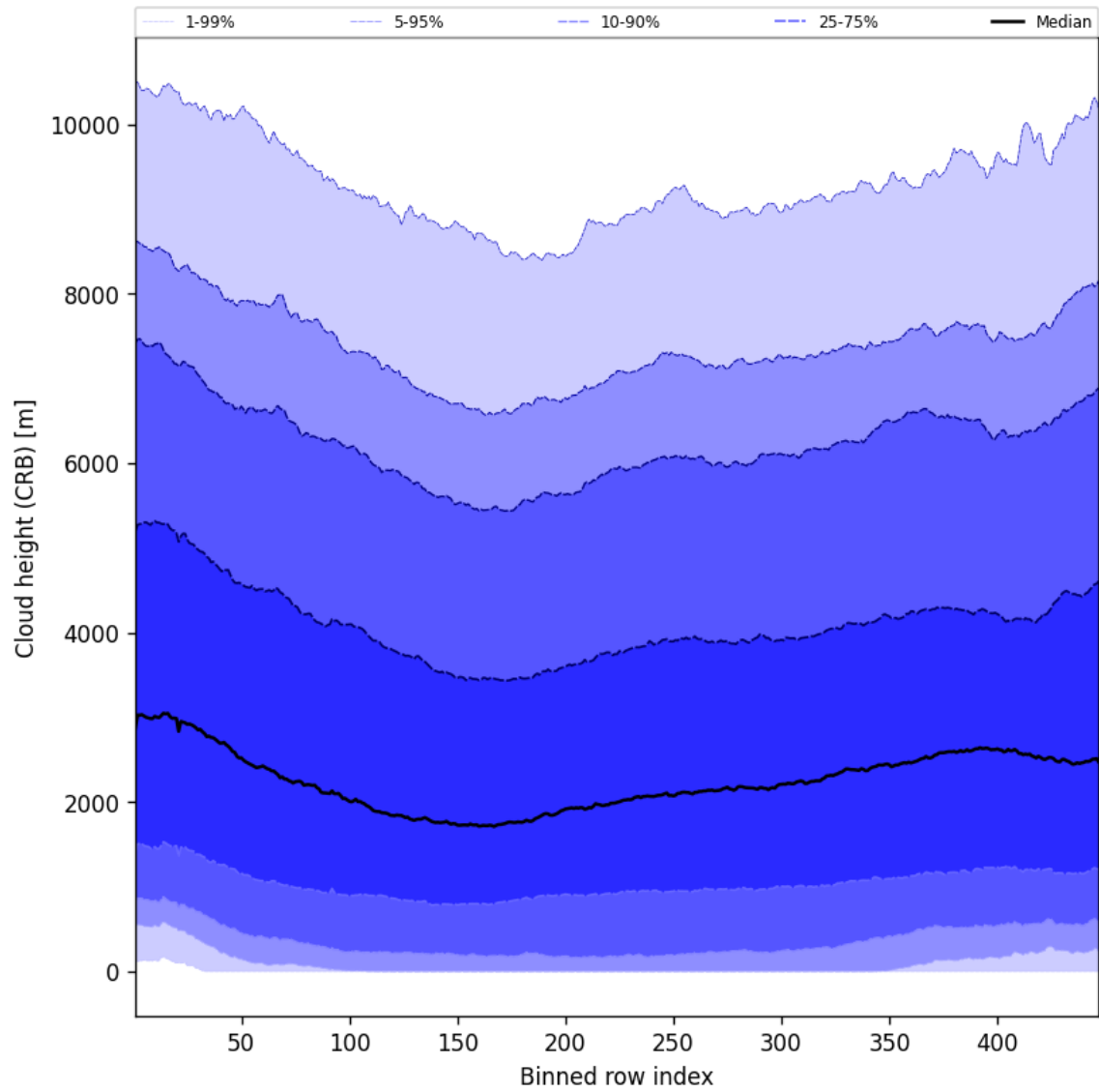
Figure 59: Along track statistics of “Cloud height (CRB)” for 2025-04-19 to 2025-04-20
