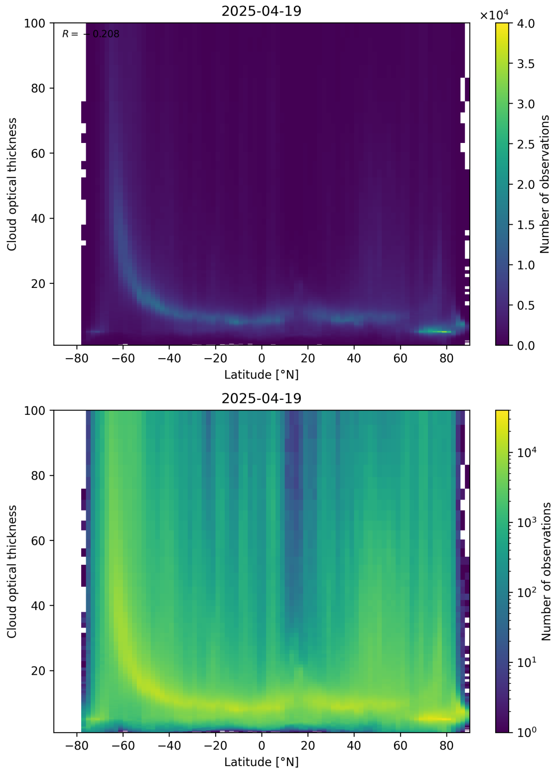
Figure 96: Scatter density plot of “Latitude” against “Cloud optical thickness” for 2025-04-19 to 2025-04-20.
