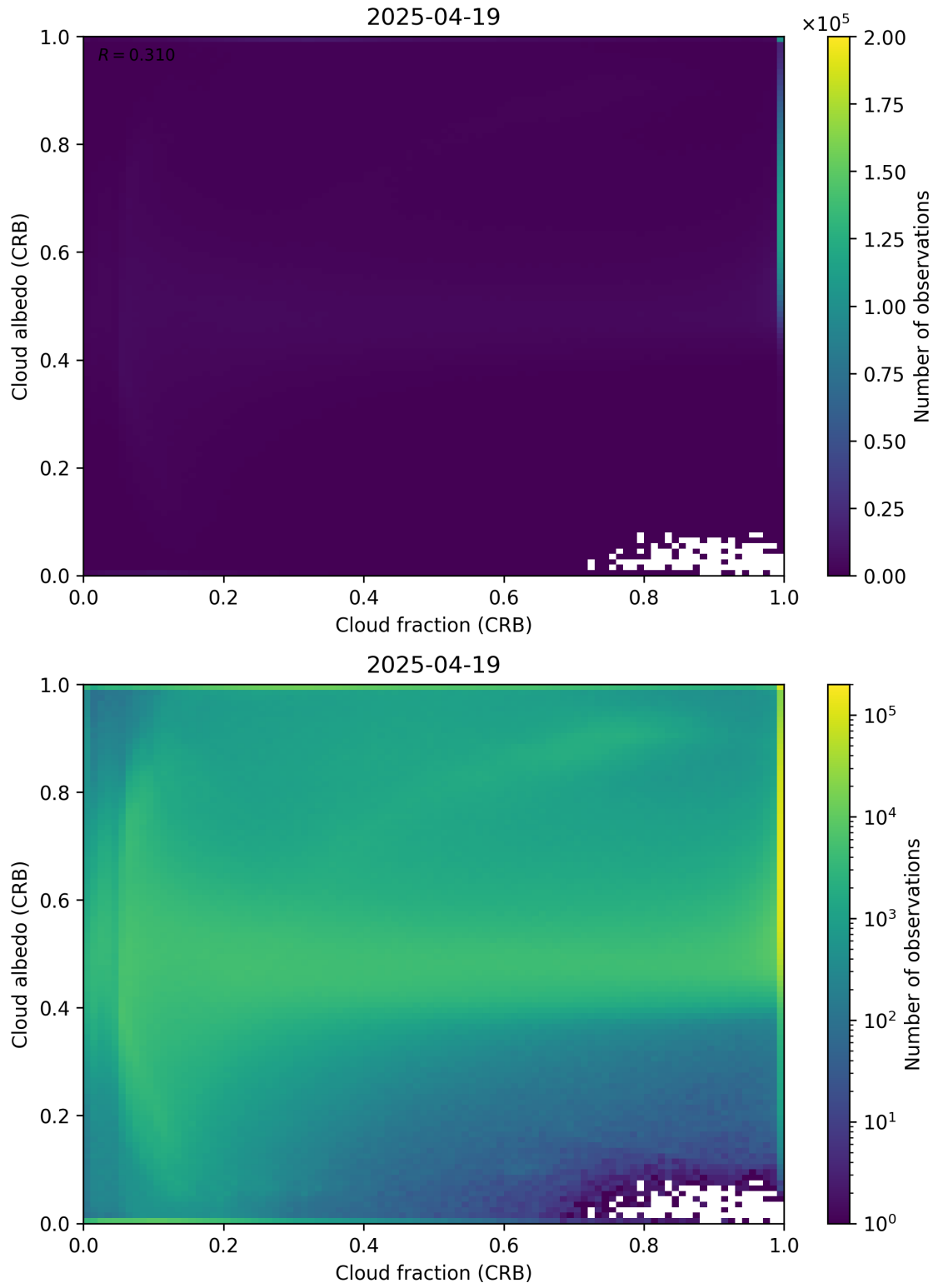
Figure 77: Scatter density plot of “Cloud fraction (CRB)” against “Cloud albedo (CRB)” for 2025-04-19 to 2025-04-20.
