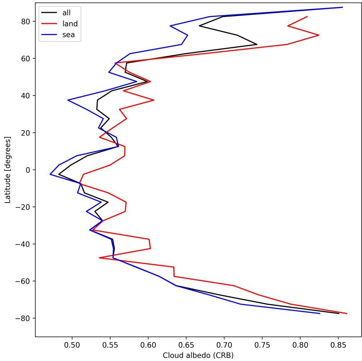
Figure 28: Zonal average of “Cloud albedo (CRB)” for 2025-04-19 to 2025-04-20.
