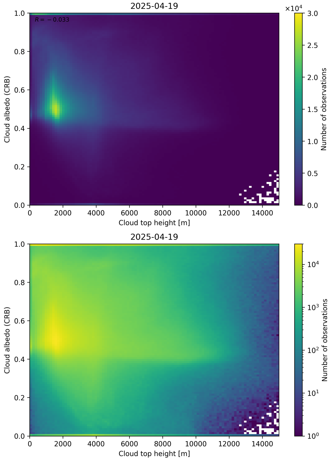
Figure 86: Scatter density plot of “Cloud top height” against “Cloud albedo (CRB)” for 2025-04-19 to 2025-04-20.
