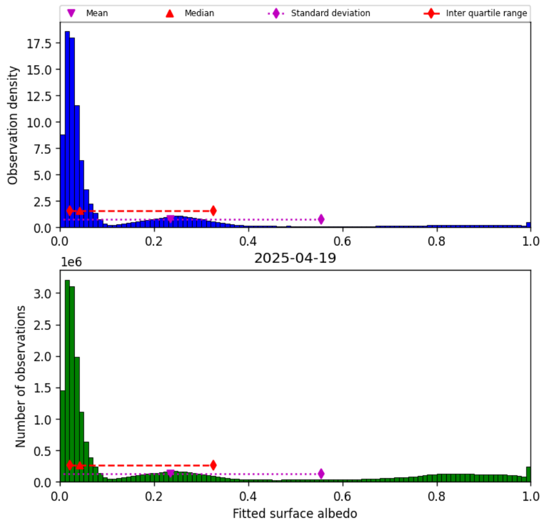
Figure 45: Histogram of “Fitted surface albedo” for 2025-04-19 to 2025-04-20
