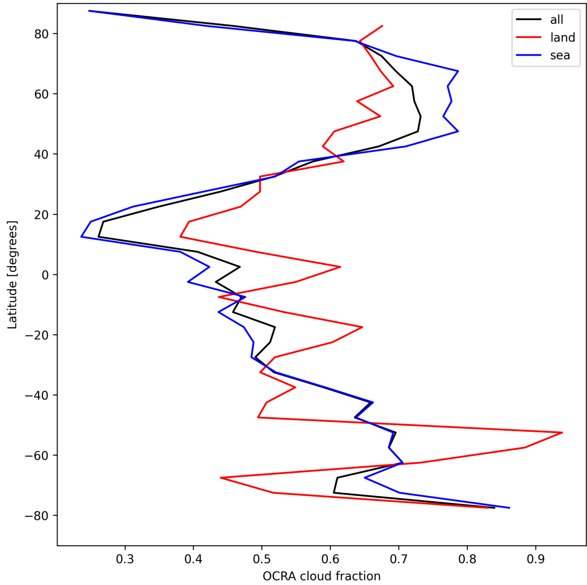
Figure 34: Zonal average of “OCRA cloud fraction” for 2025-04-19 to 2025-04-20.
