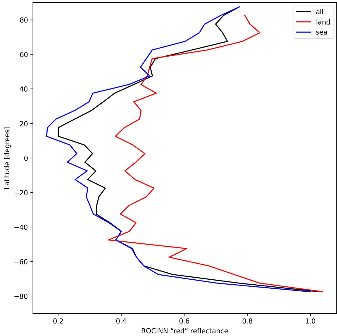
Figure 37: Zonal average of “ROCINN “red” reflectance” for 2025-04-19 to 2025-04-20.
