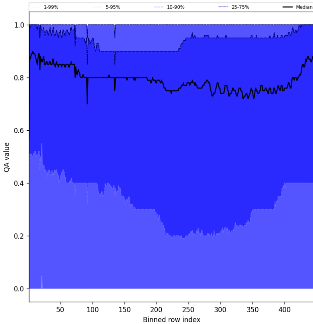
Figure 54: Along track statistics of “QA value” for 2025-04-19 to 2025-04-21
