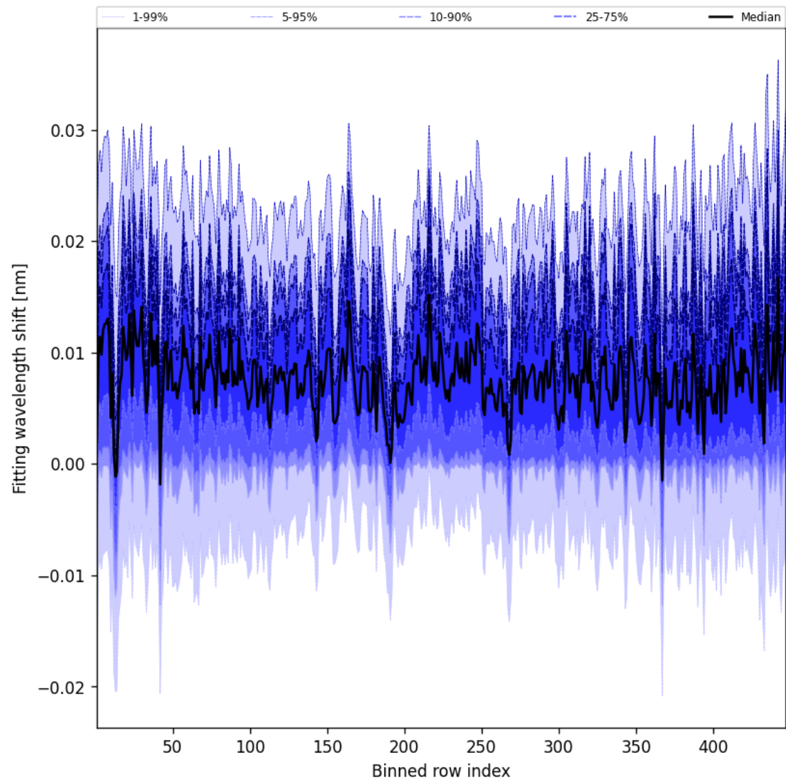
Figure 65: Along track statistics of “Fitting wavelength shift” for 2025-04-19 to 2025-04-21
