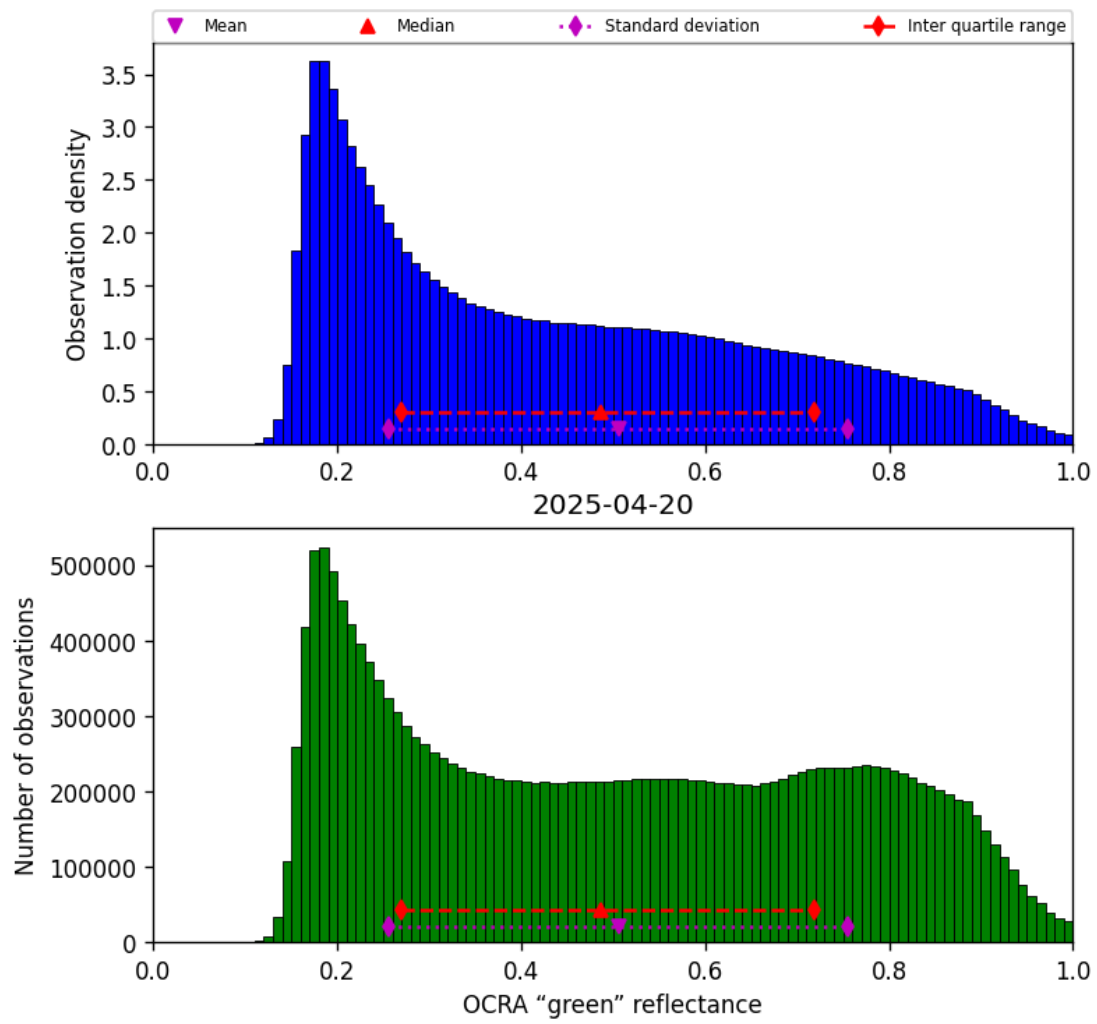
Figure 52: Histogram of “OCRA “green” reflectance” for 2025-04-19 to 2025-04-21
