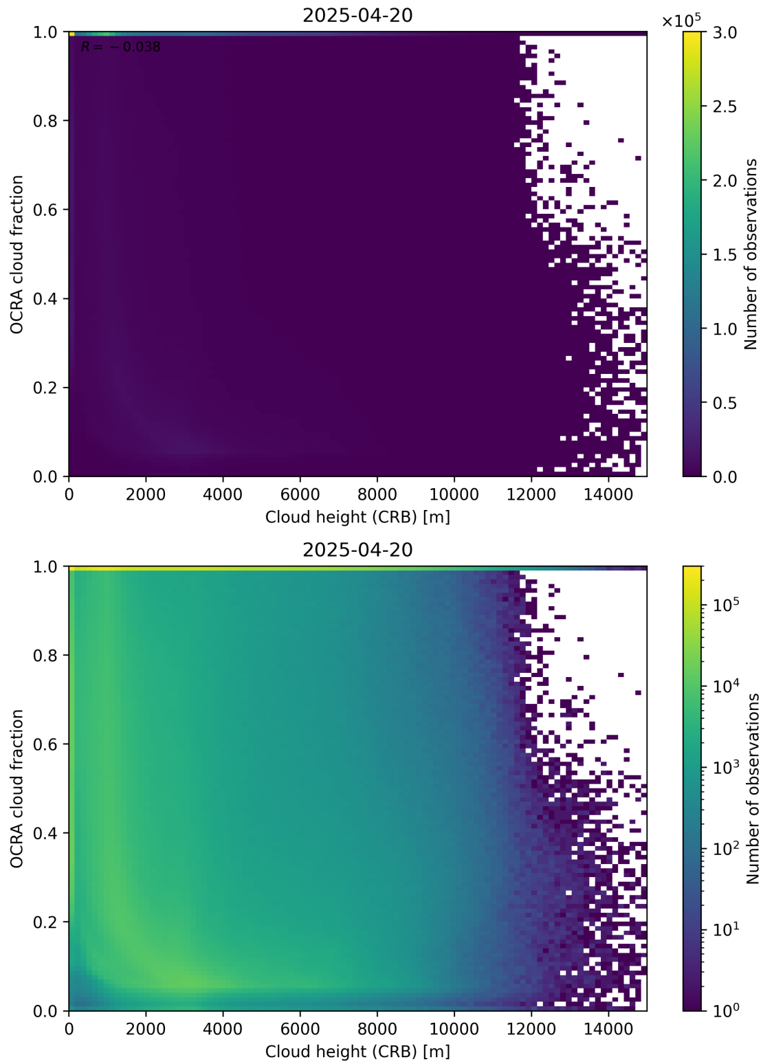
Figure 81: Scatter density plot of “Cloud height (CRB)” against “OCRA cloud fraction” for 2025-04-19 to 2025-04-21.
