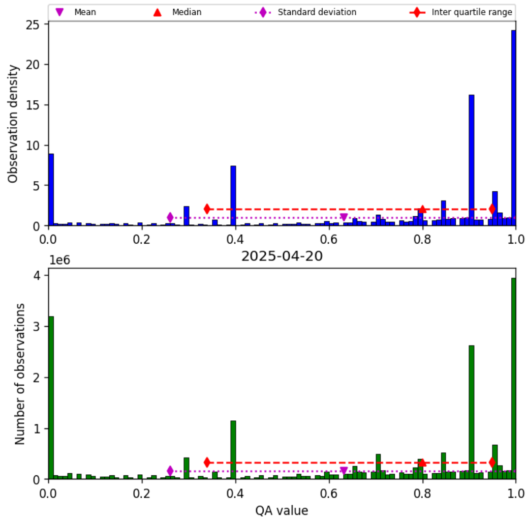
Figure 38: Histogram of “QA value” for 2025-04-19 to 2025-04-21
