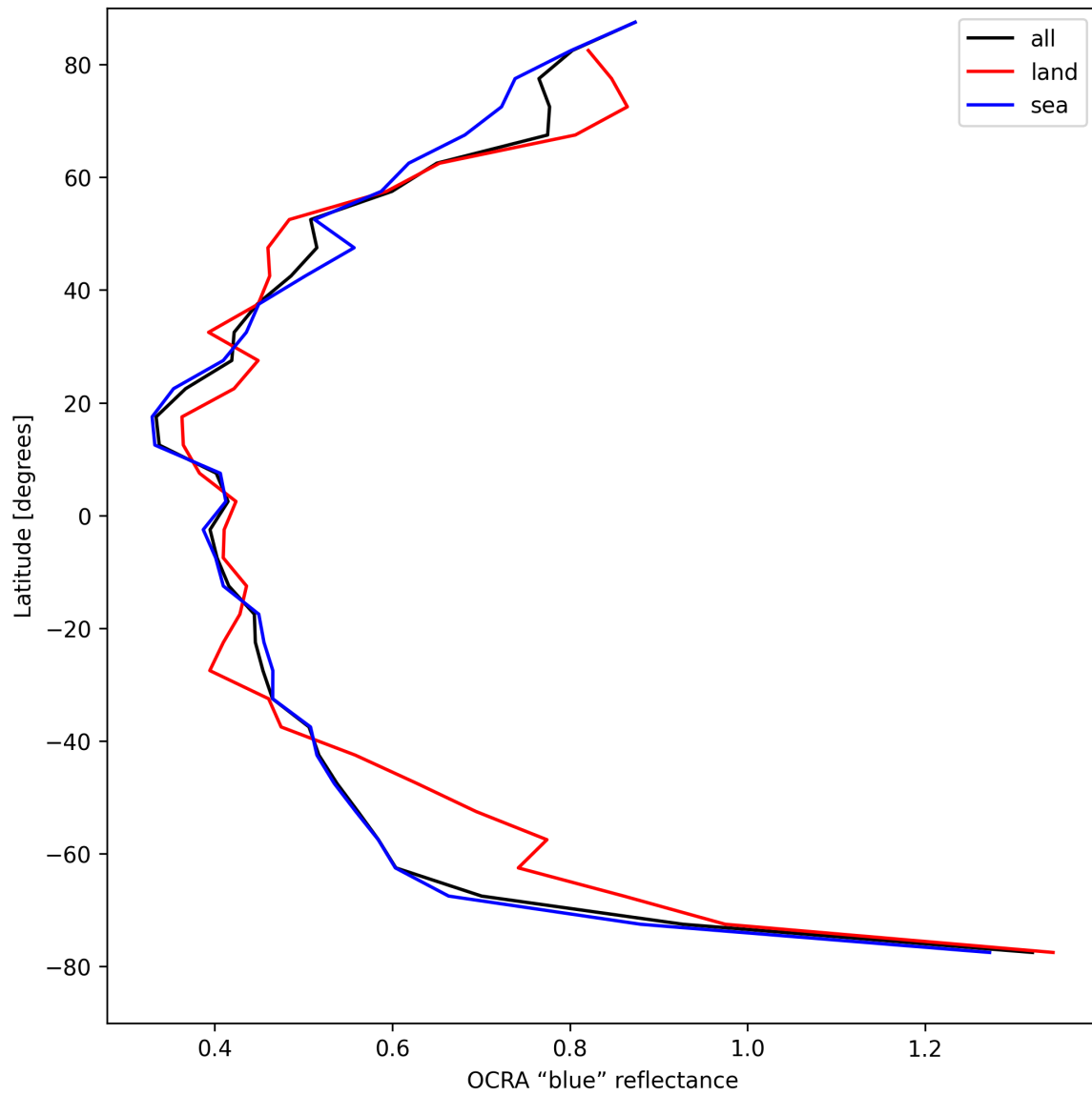
Figure 35: Zonal average of “OCRA “blue” reflectance” for 2025-04-19 to 2025-04-21.
