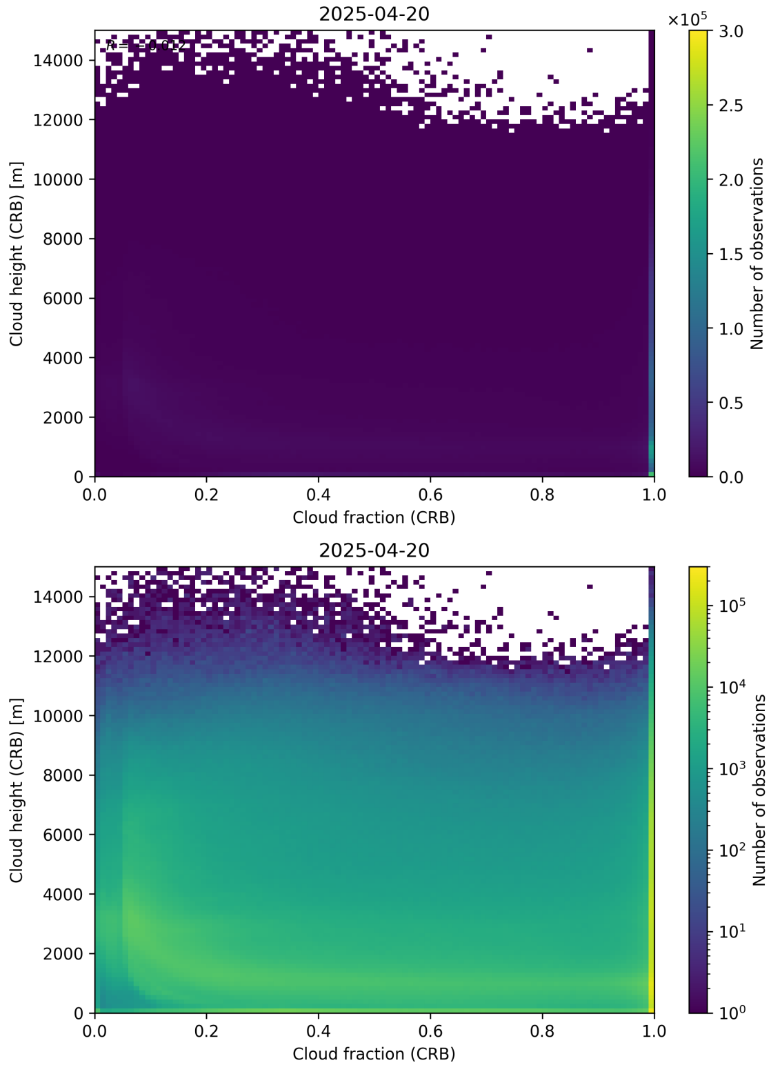
Figure 79: Scatter density plot of “Cloud fraction (CRB)” against “Cloud height (CRB)” for 2025-04-19 to 2025-04-21.
