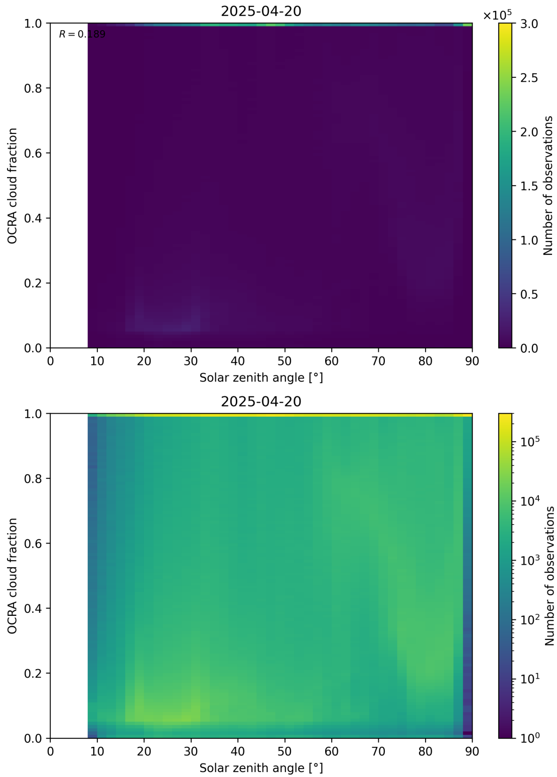
Figure 100: Scatter density plot of “Solar zenith angle” against “OCRA cloud fraction” for 2025-04-19 to 2025-04-21.
