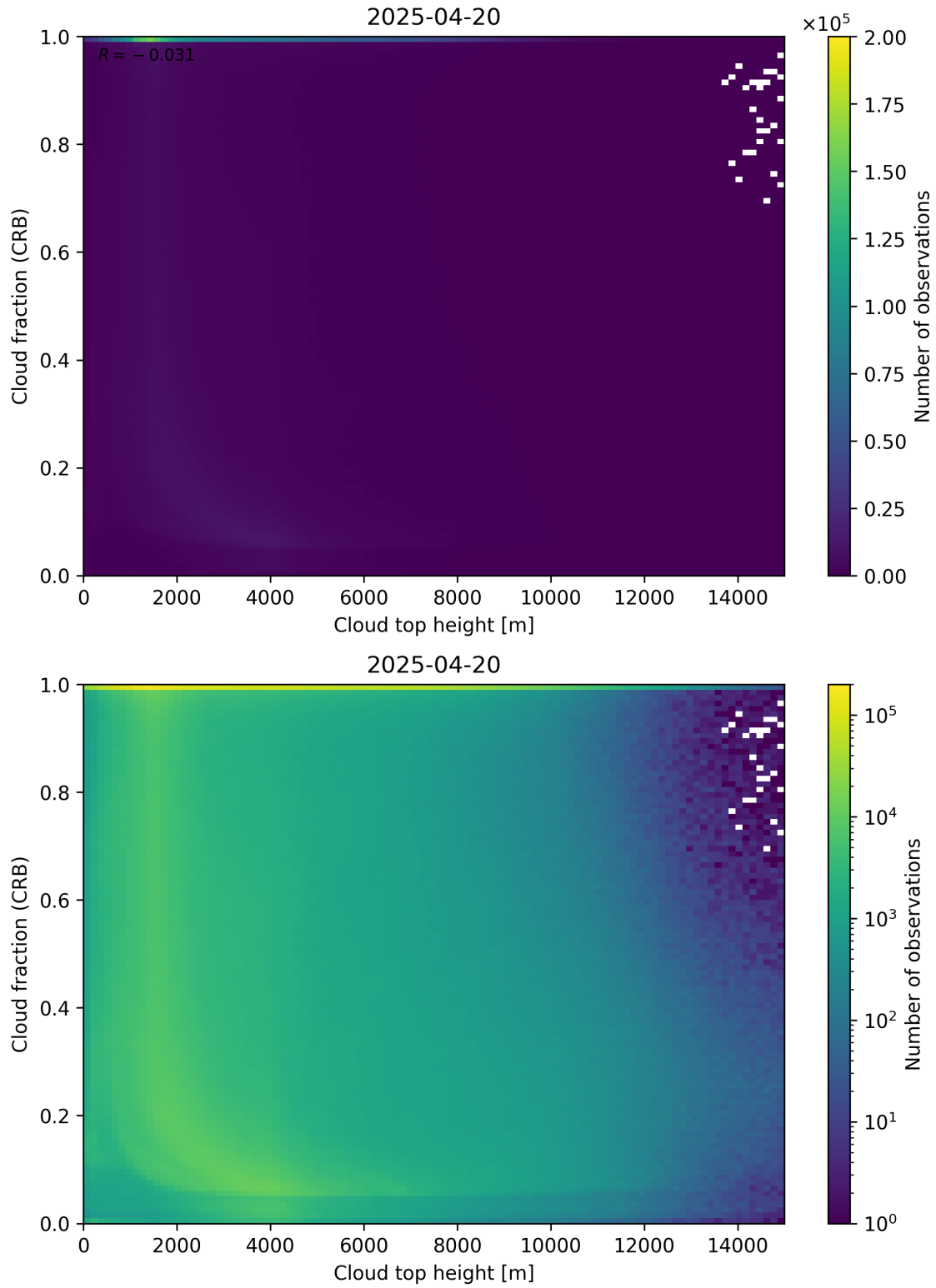
Figure 88: Scatter density plot of “Cloud top height” against “Cloud fraction (CRB)” for 2025-04-19 to 2025-04-21.
