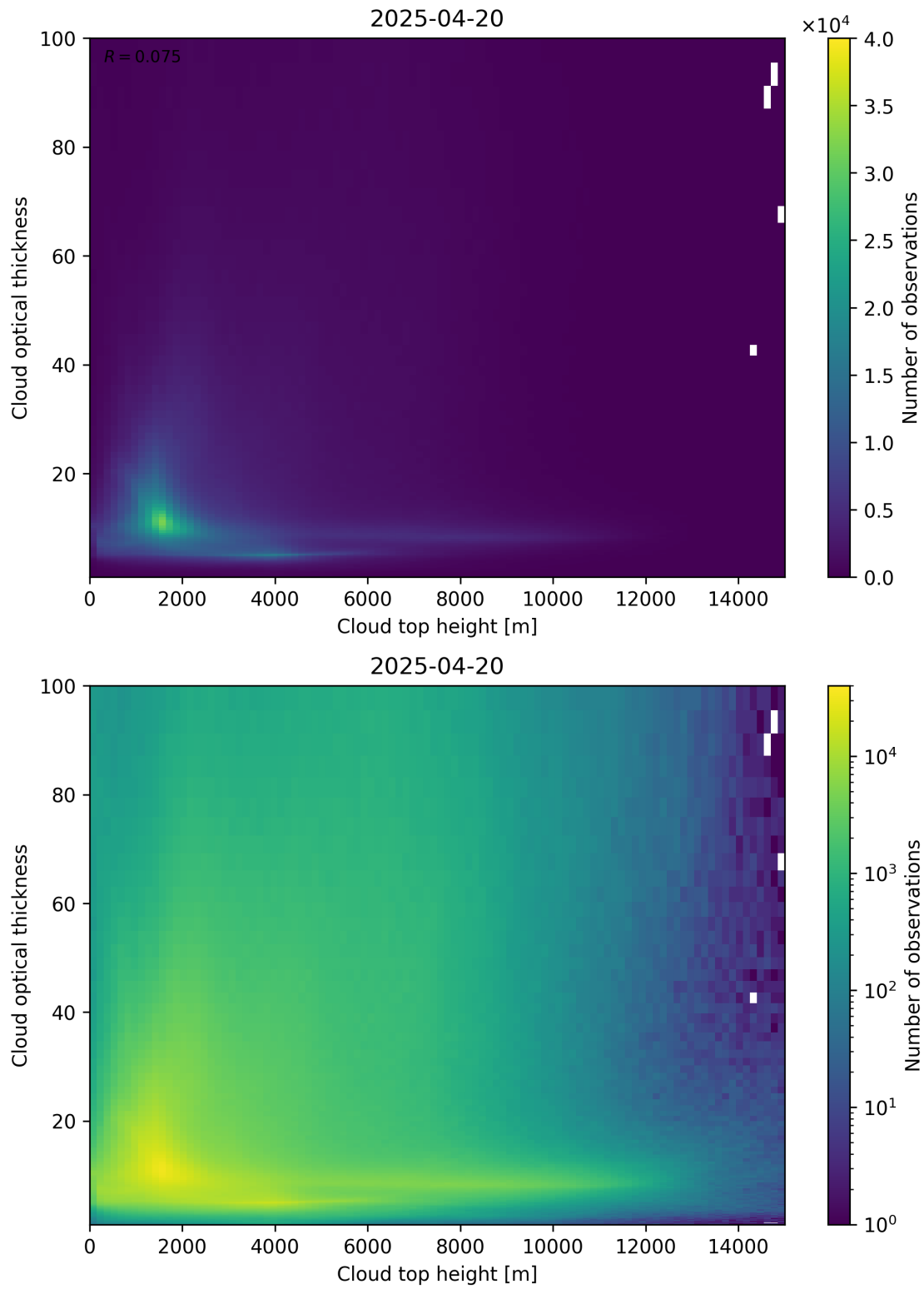
Figure 90: Scatter density plot of “Cloud top height” against “Cloud optical thickness” for 2025-04-19 to 2025-04-21.
