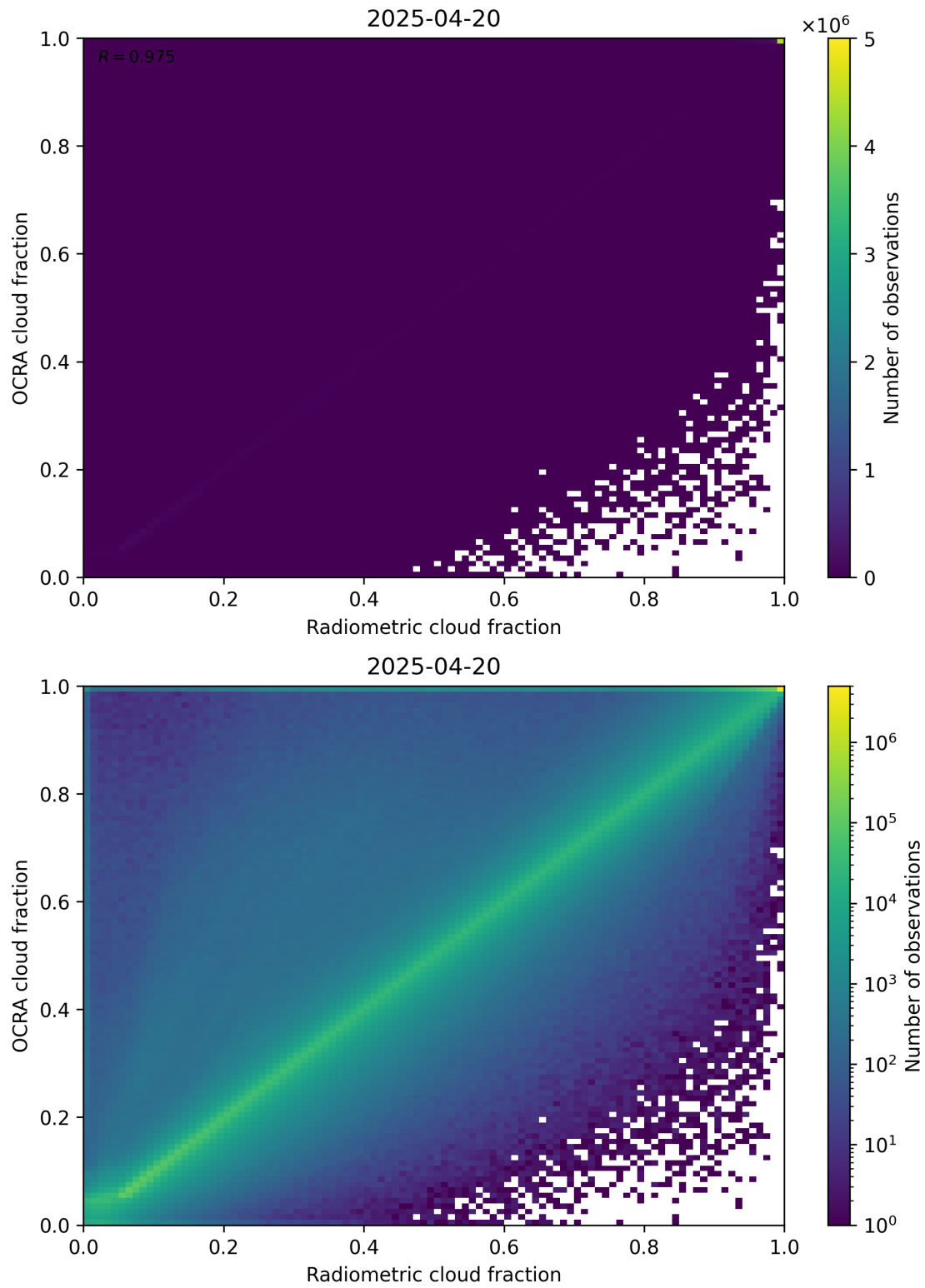
Figure 72: Scatter density plot of “Radiometric cloud fraction” against “OCRA cloud fraction” for 2025-04-19 to 2025-04-21.
