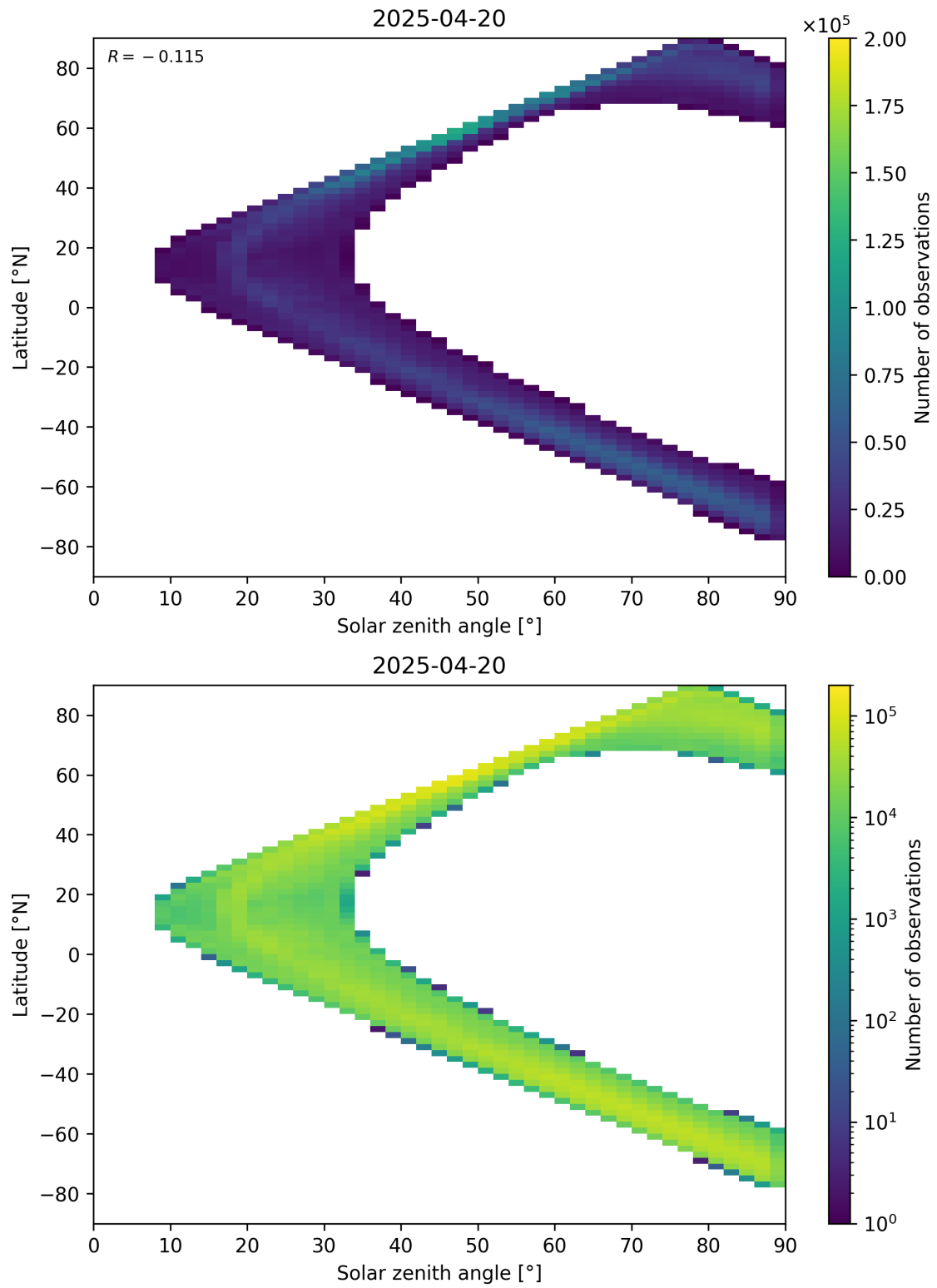
Figure 105: Scatter density plot of “Solar zenith angle” against “Latitude” for 2025-04-19 to 2025-04-21.
