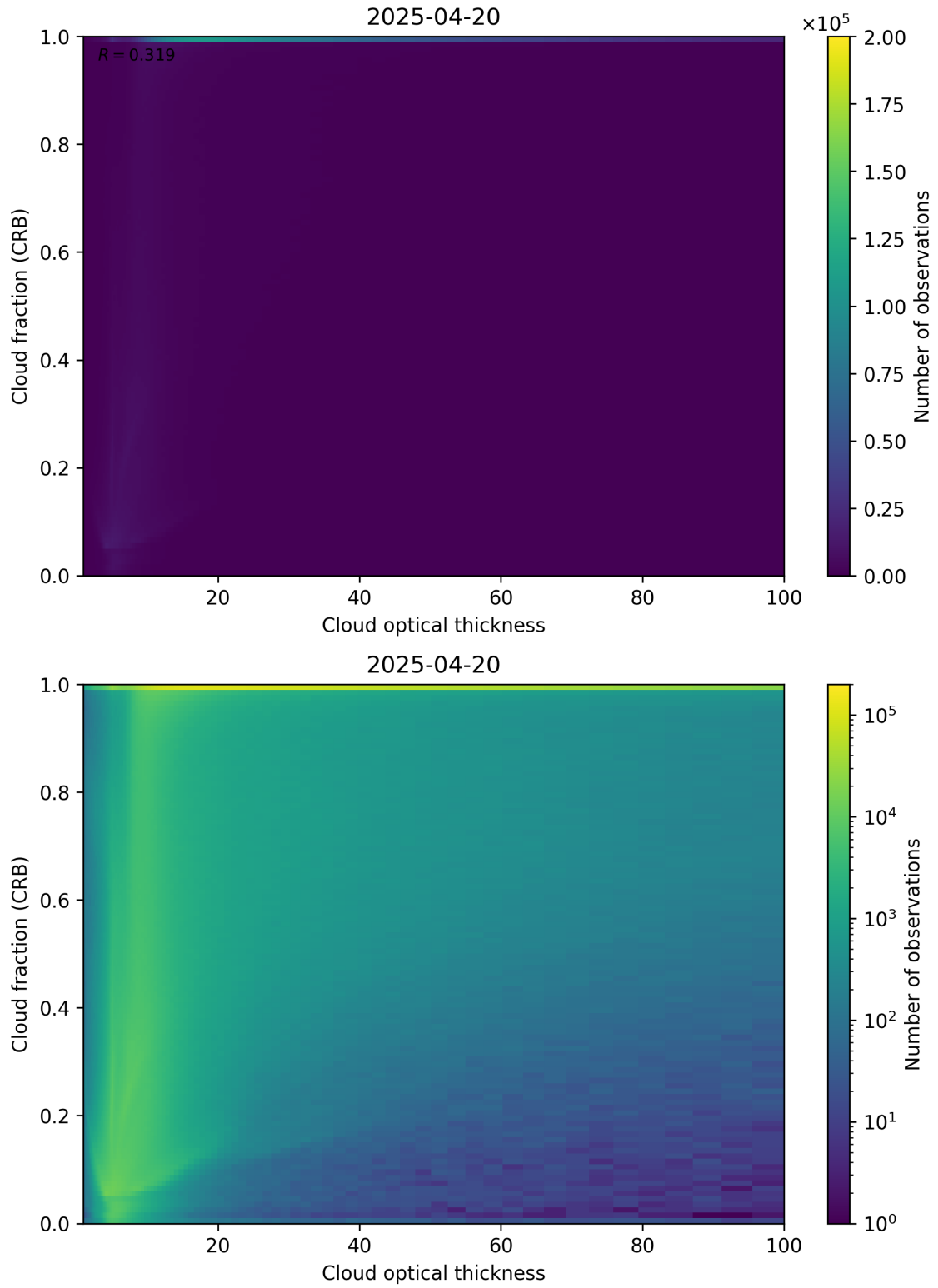
Figure 84: Scatter density plot of “Cloud optical thickness” against “Cloud fraction (CRB)” for 2025-04-19 to 2025-04-21.
