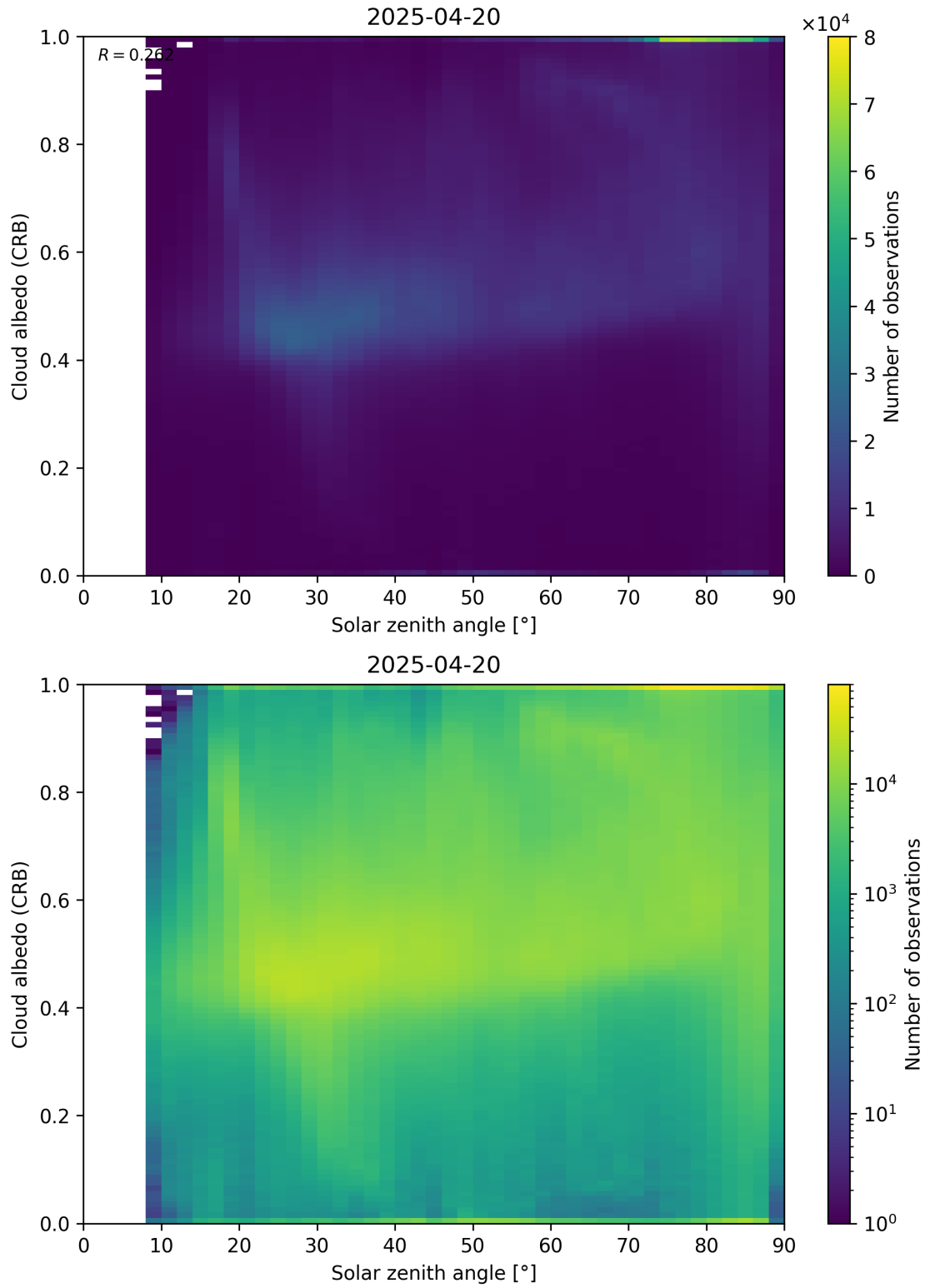
Figure 98: Scatter density plot of “Solar zenith angle” against “Cloud albedo (CRB)” for 2025-04-19 to 2025-04-21.
