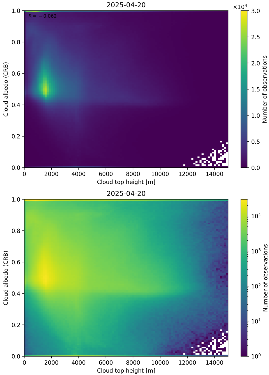
Figure 86: Scatter density plot of “Cloud top height” against “Cloud albedo (CRB)” for 2025-04-19 to 2025-04-21.
