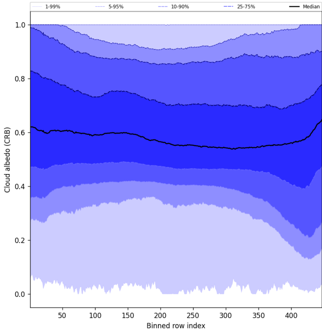
Figure 60: Along track statistics of “Cloud albedo (CRB)” for 2025-04-19 to 2025-04-21
