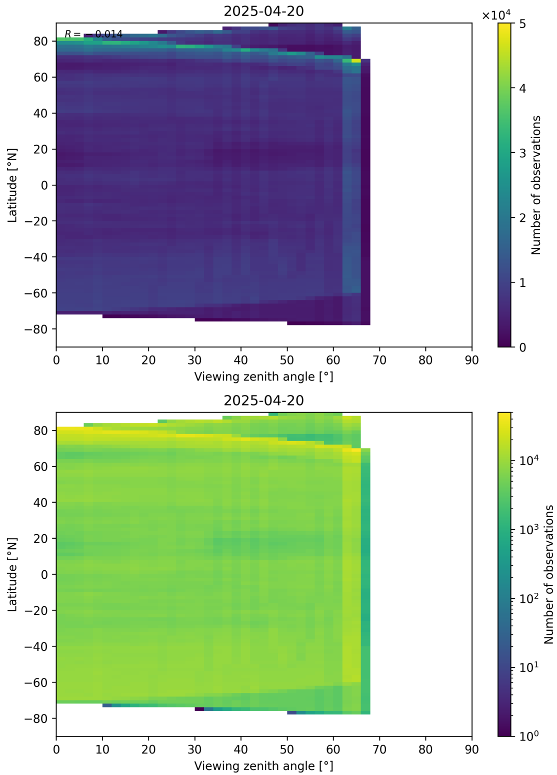
Figure 113: Scatter density plot of “Viewing zenith angle” against “Latitude” for 2025-04-19 to 2025-04-21.
