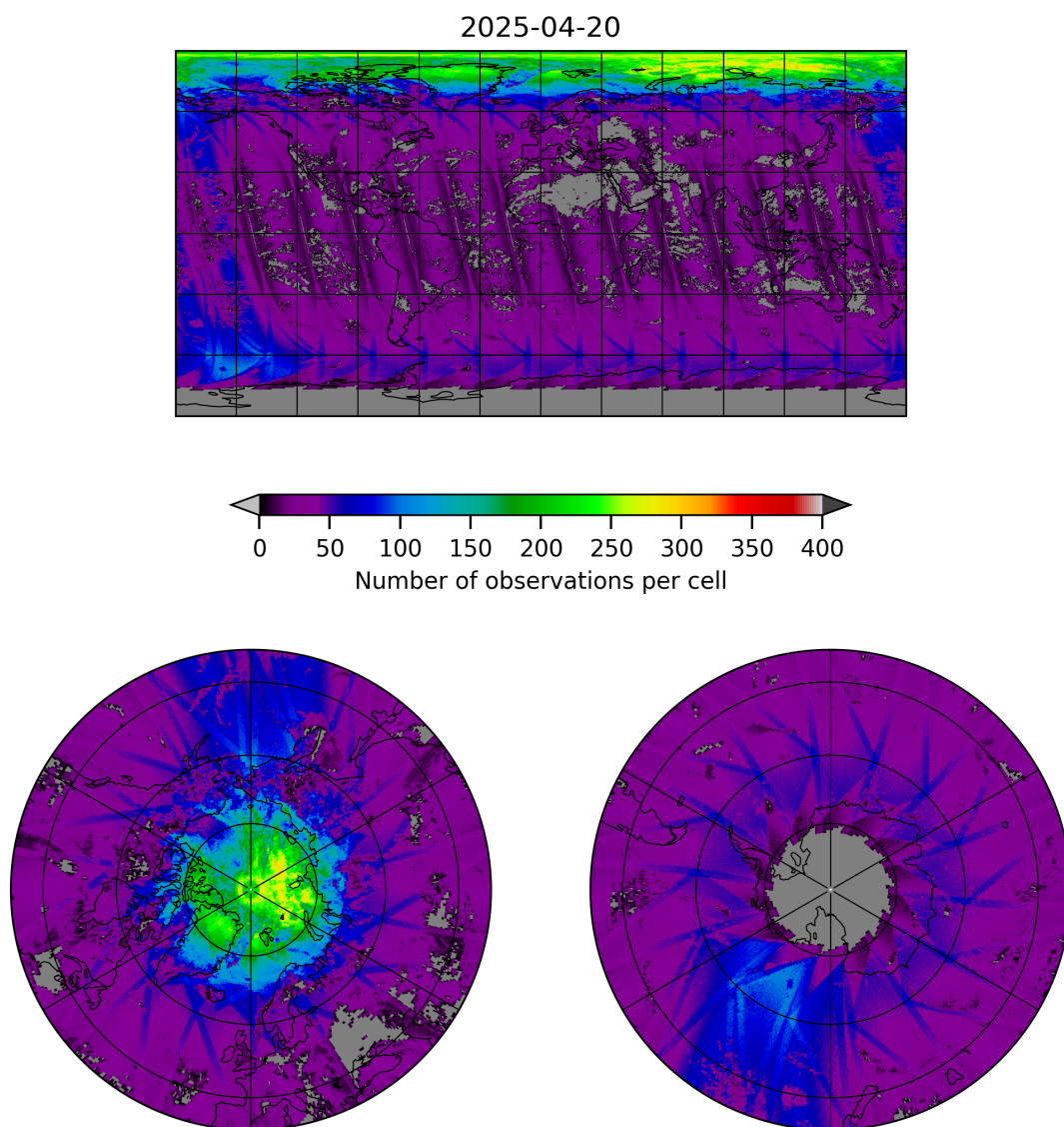
Figure 21: Map of the number of observations for 2025-04-19 to 2025-04-21
