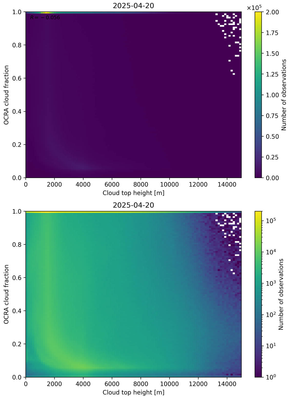
Figure 87: Scatter density plot of “Cloud top height” against “OCRA cloud fraction” for 2025-04-19 to 2025-04-21.
