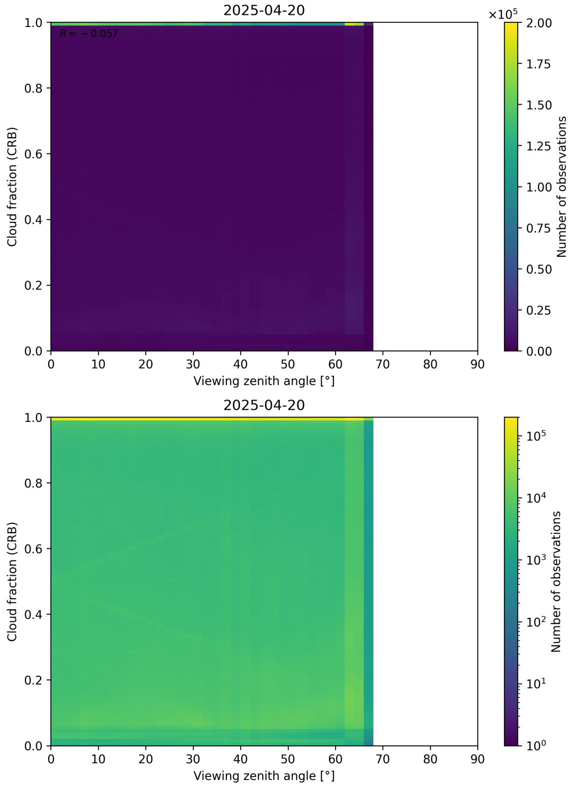
Figure 109: Scatter density plot of “Viewing zenith angle” against “Cloud fraction (CRB)” for 2025-04-19 to 2025-04-21.
