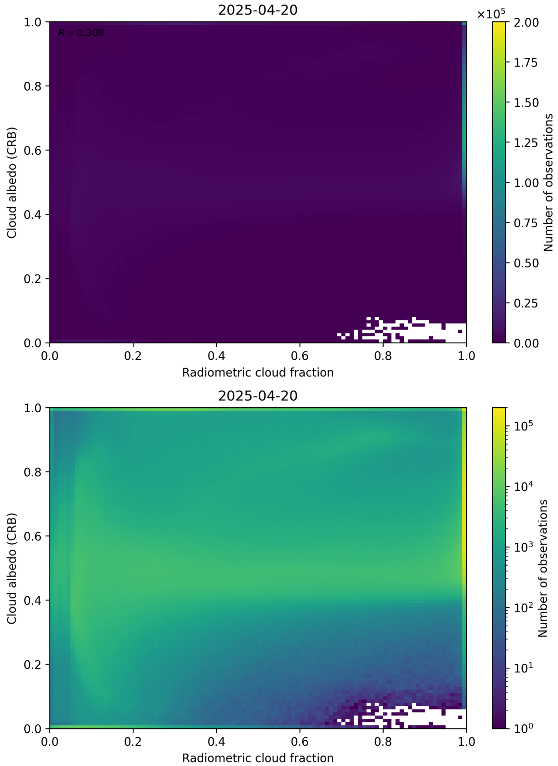
Figure 71: Scatter density plot of “Radiometric cloud fraction” against “Cloud albedo (CRB)” for 2025-04-19 to 2025-04-21.
