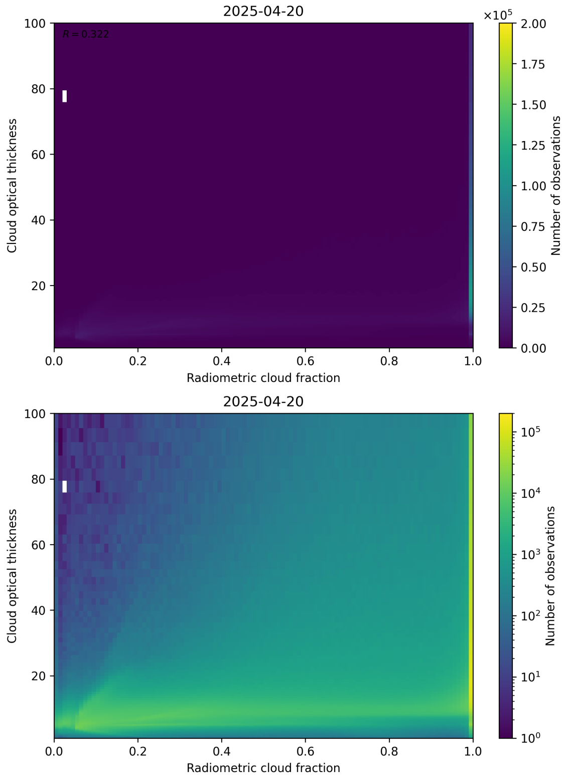
Figure 75: Scatter density plot of “Radiometric cloud fraction” against “Cloud optical thickness” for 2025-04-19 to 2025-04-21.
