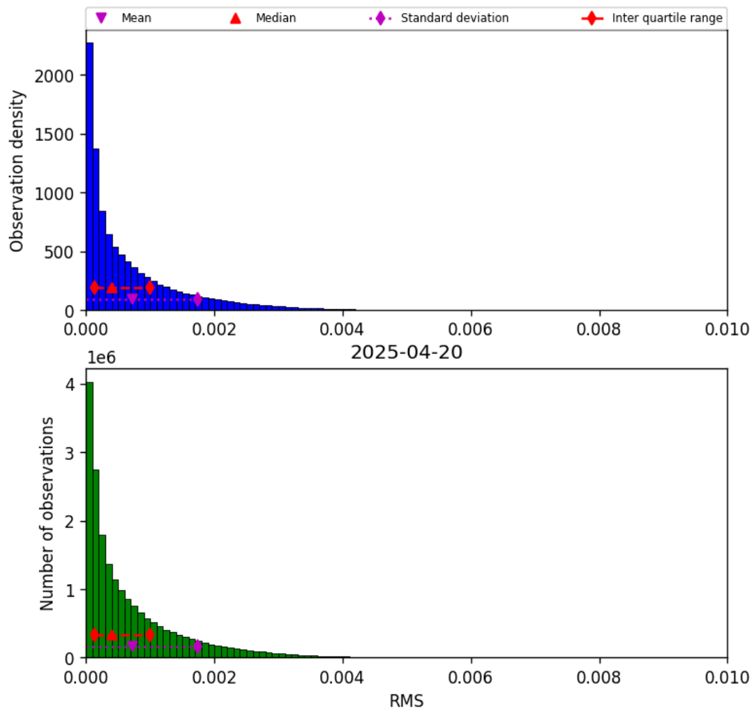
Figure 47: Histogram of “RMS” for 2025-04-19 to 2025-04-21
