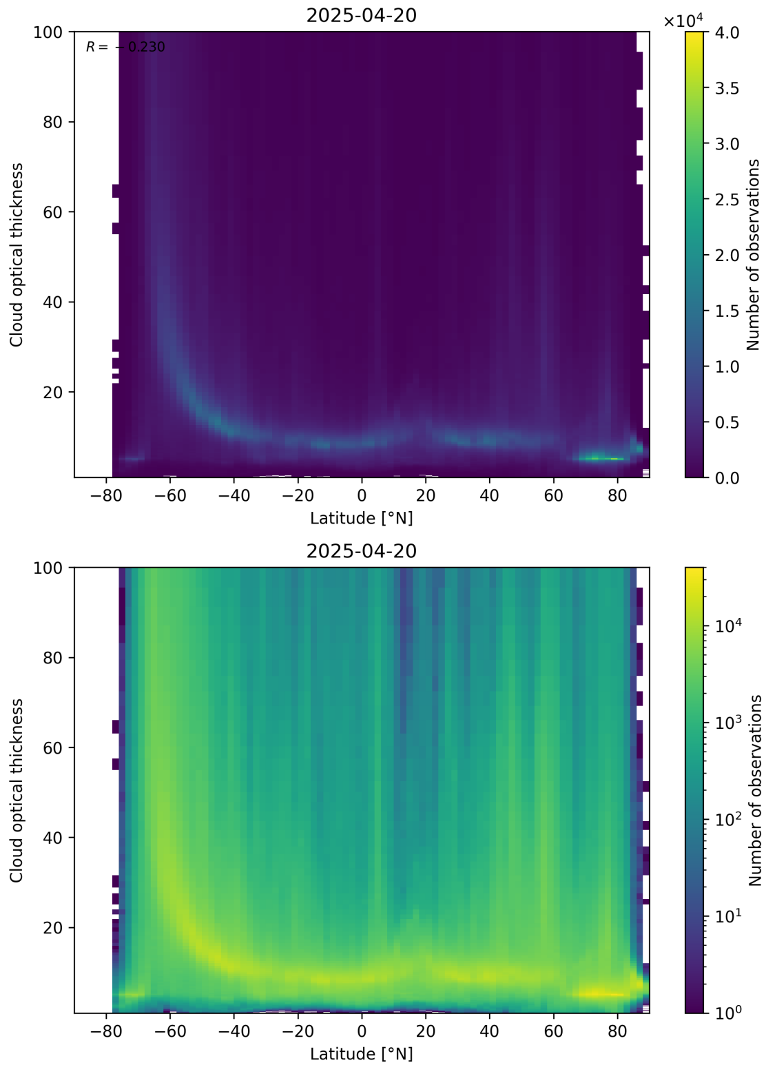
Figure 96: Scatter density plot of “Latitude” against “Cloud optical thickness” for 2025-04-19 to 2025-04-21.
