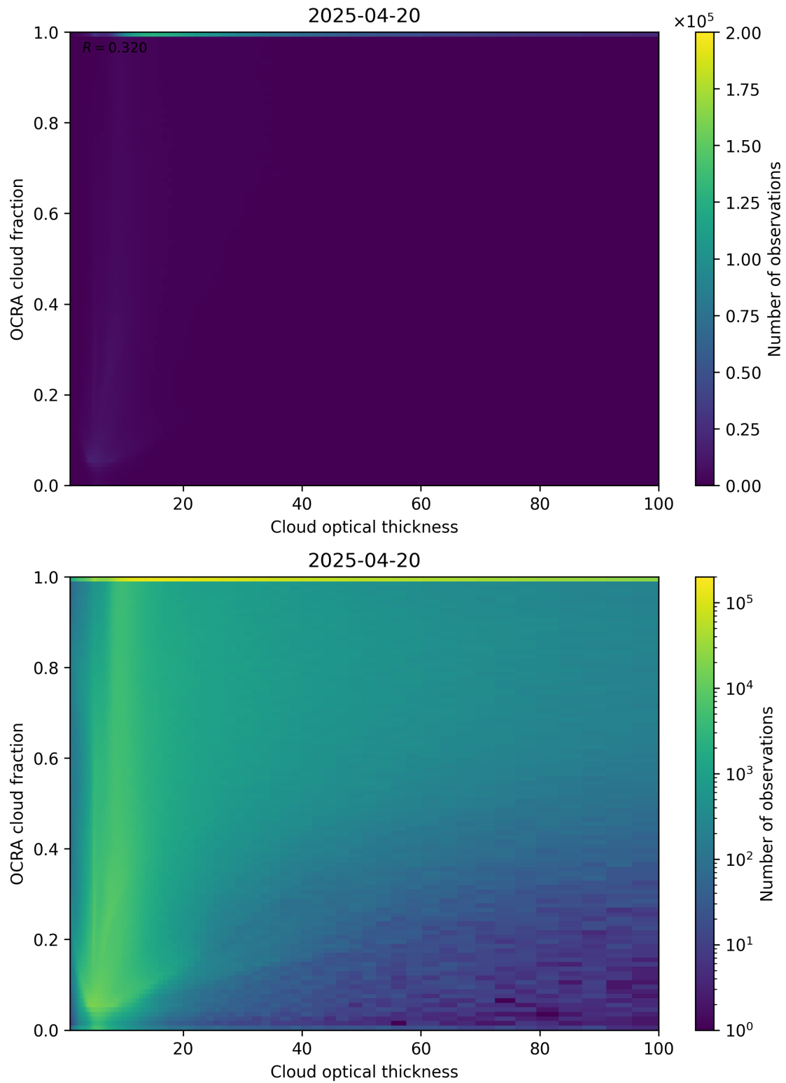
Figure 83: Scatter density plot of “Cloud optical thickness” against “OCRA cloud fraction” for 2025-04-19 to 2025-04-21.
