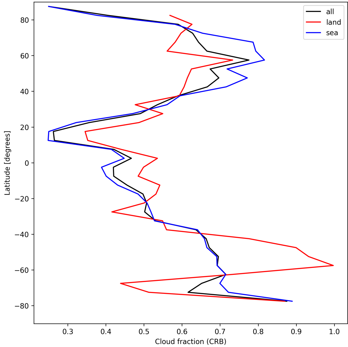
Figure 26: Zonal average of “Cloud fraction (CRB)” for 2025-04-19 to 2025-04-21.
