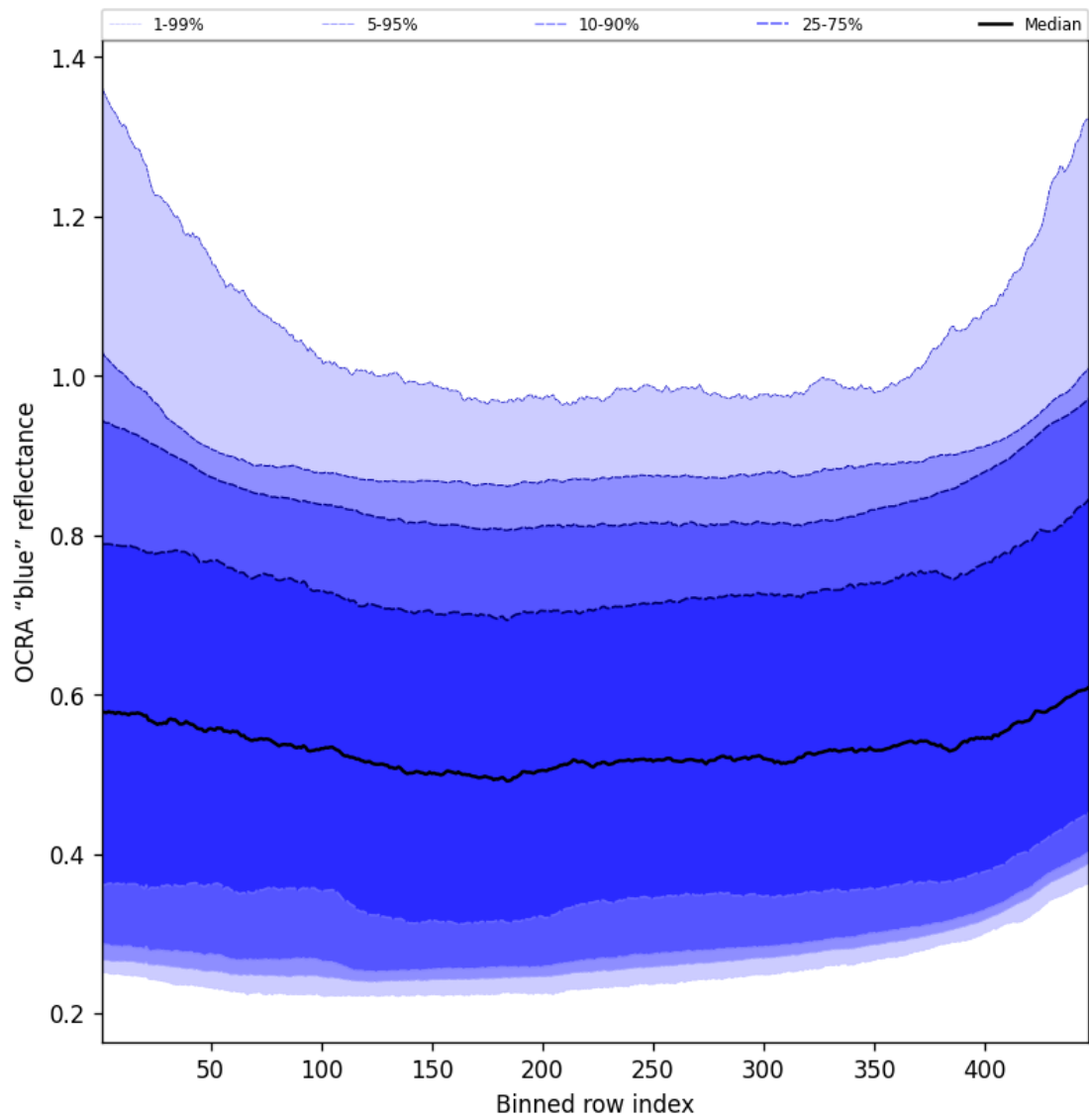
Figure 67: Along track statistics of “OCRA “blue” reflectance” for 2025-04-19 to 2025-04-21
