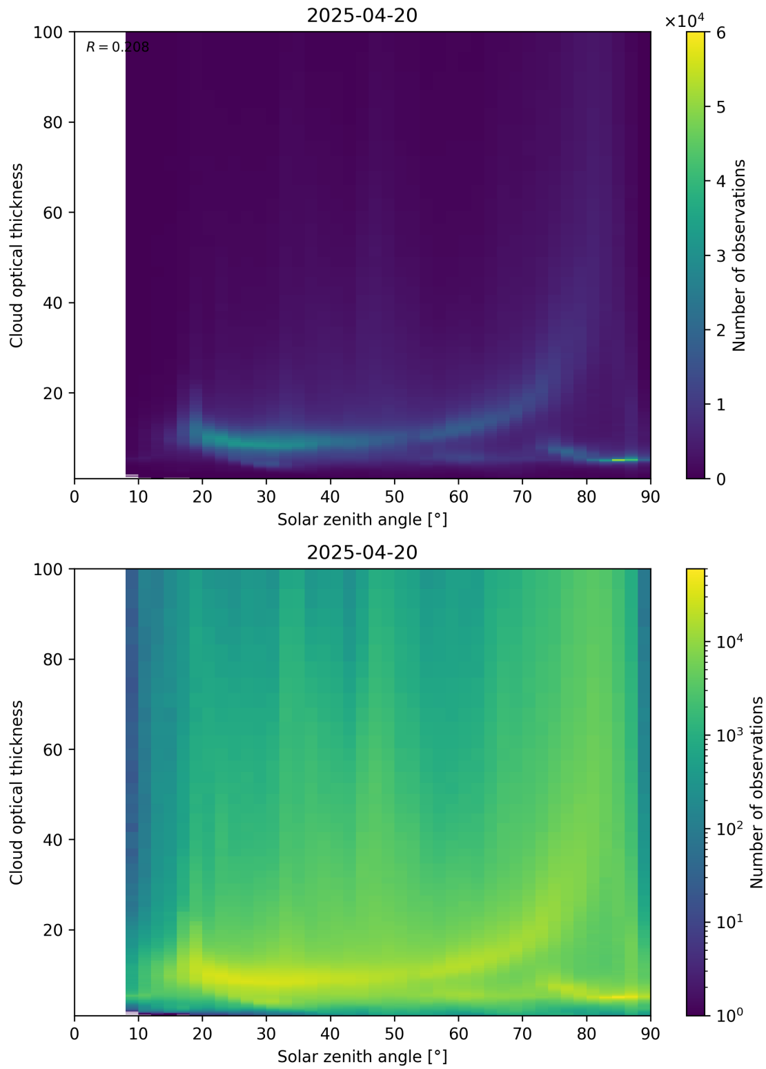
Figure 103: Scatter density plot of “Solar zenith angle” against “Cloud optical thickness” for 2025-04-19 to 2025-04-21.
