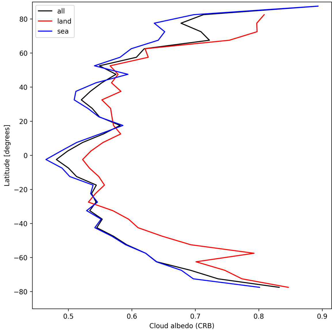
Figure 28: Zonal average of “Cloud albedo (CRB)” for 2025-04-19 to 2025-04-21.
