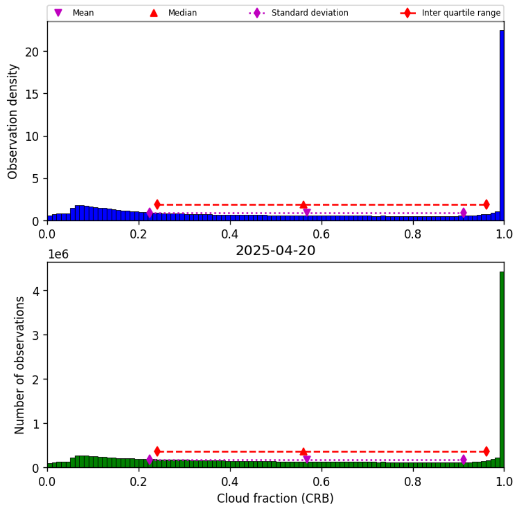
Figure 42: Histogram of “Cloud fraction (CRB)” for 2025-04-19 to 2025-04-21
