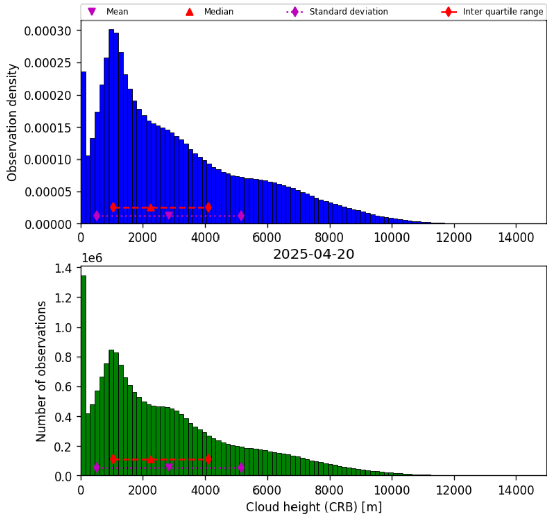
Figure 43: Histogram of “Cloud height (CRB)” for 2025-04-19 to 2025-04-21
