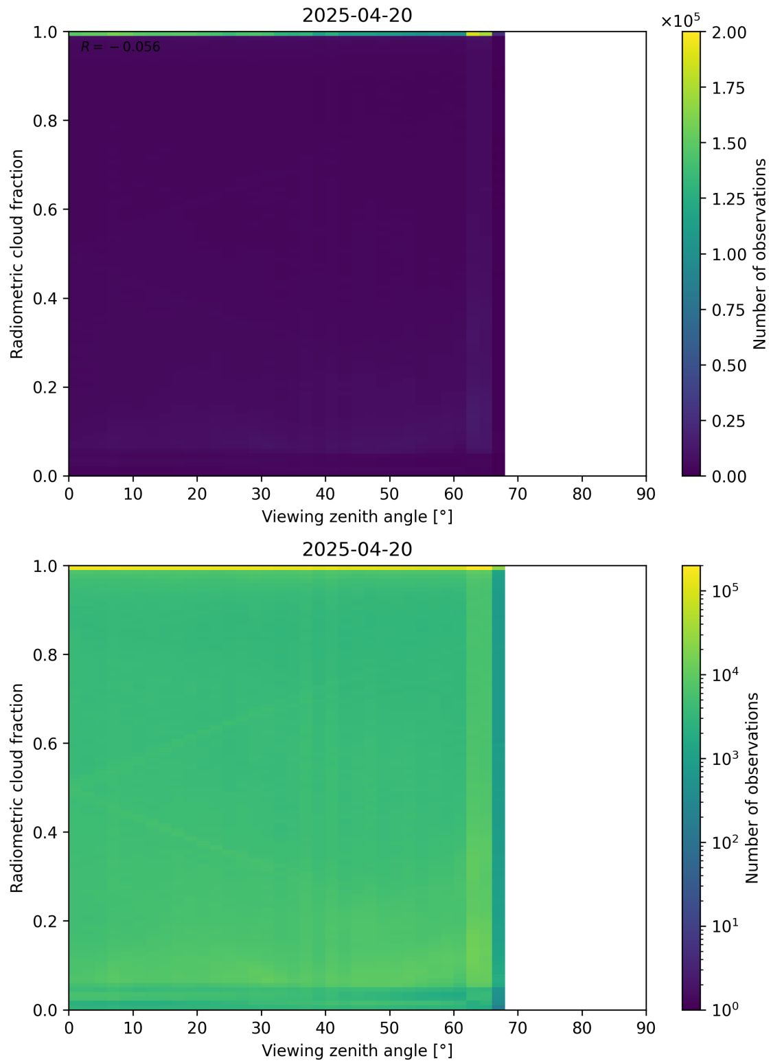
Figure 107: Scatter density plot of “Viewing zenith angle” against “Radiometric cloud fraction” for 2025-04-19 to 2025-04-21.
