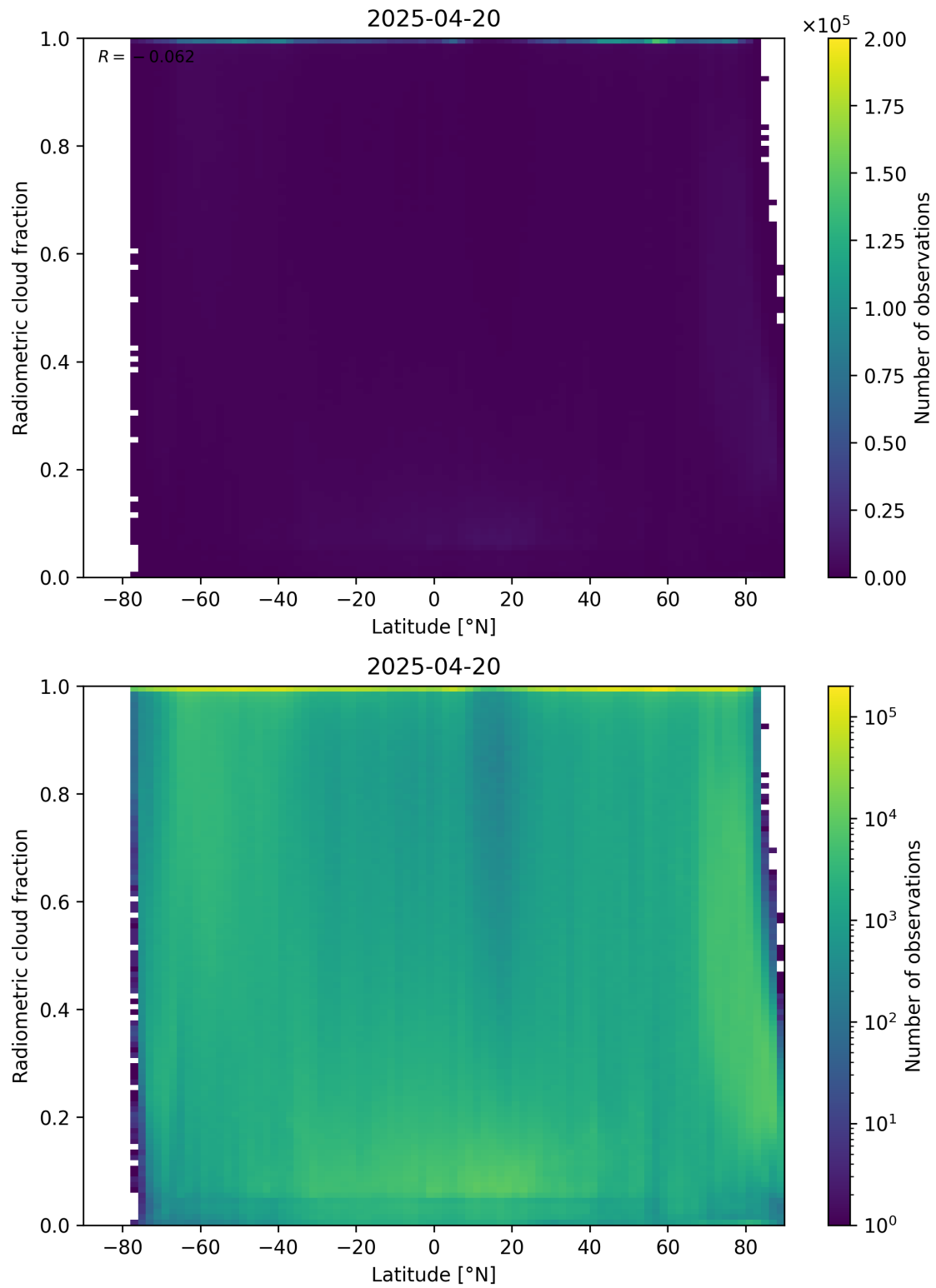
Figure 92: Scatter density plot of “Latitude” against “Radiometric cloud fraction” for 2025-04-19 to 2025-04-21.
