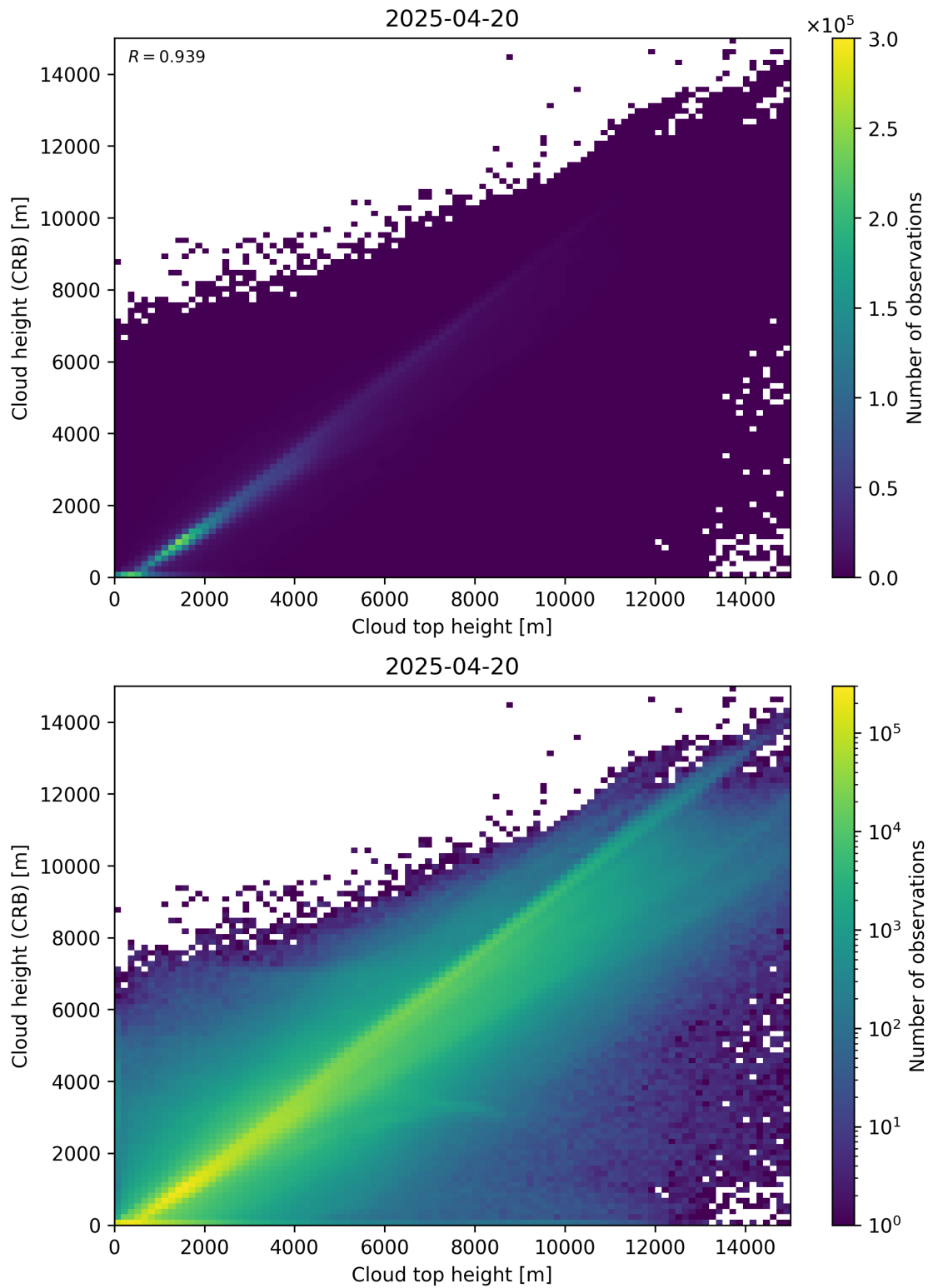
Figure 89: Scatter density plot of “Cloud top height” against “Cloud height (CRB)” for 2025-04-19 to 2025-04-21.
