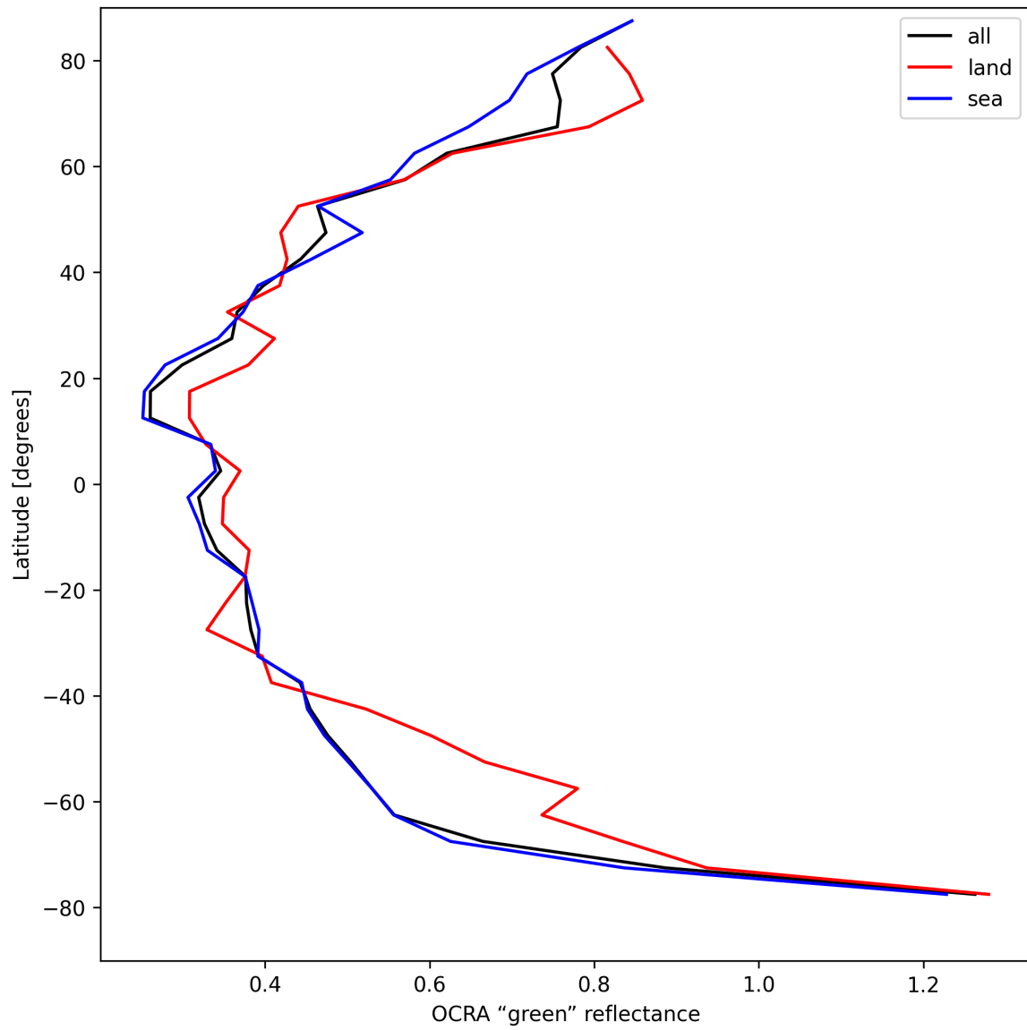
Figure 36: Zonal average of “OCRA “green” reflectance” for 2025-04-19 to 2025-04-21.
