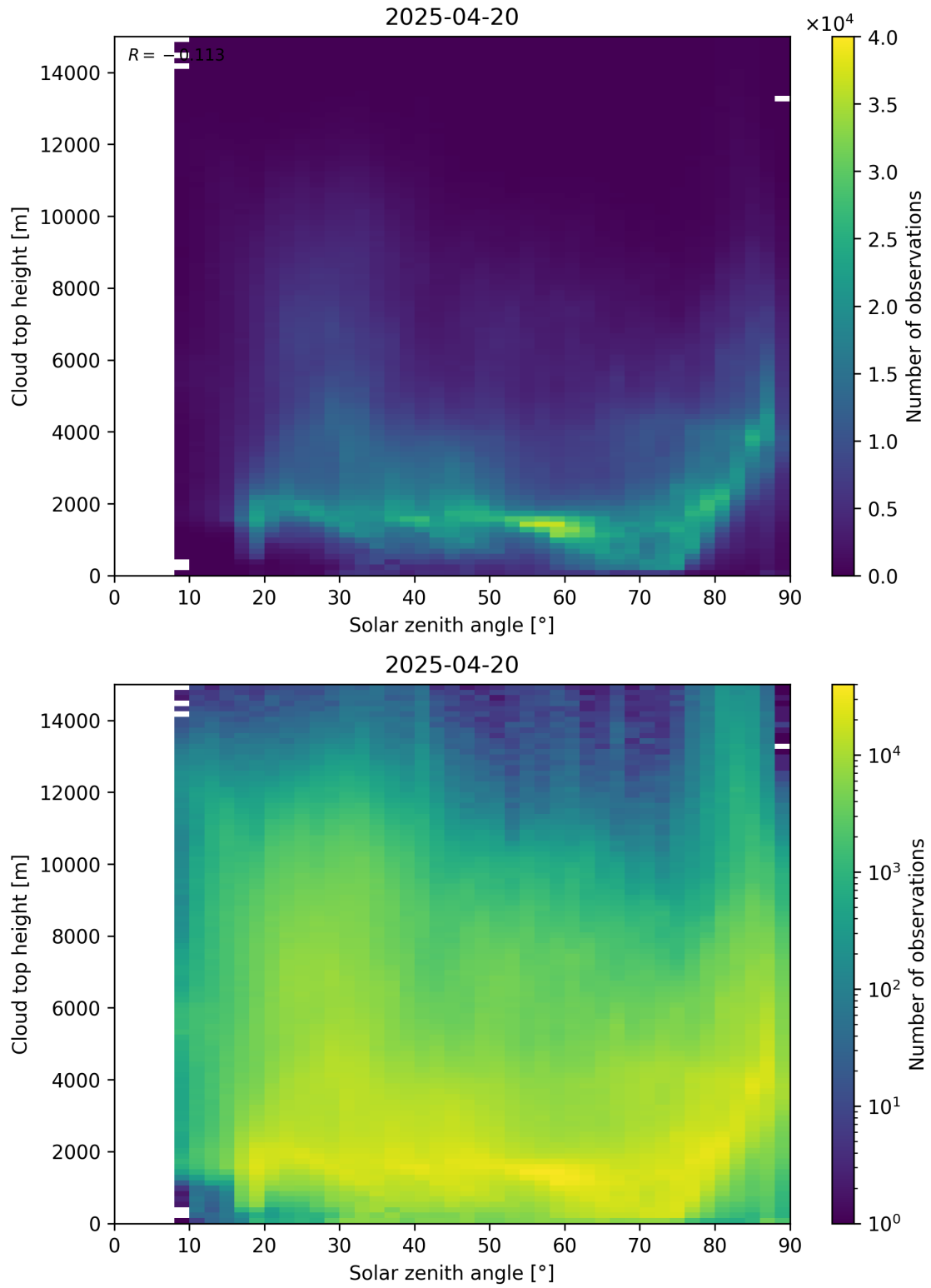
Figure 104: Scatter density plot of “Solar zenith angle” against “Cloud top height” for 2025-04-19 to 2025-04-21.
