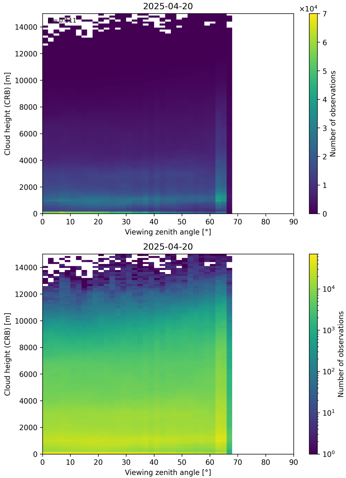
Figure 110: Scatter density plot of “Viewing zenith angle” against “Cloud height (CRB)” for 2025-04-19 to 2025-04-21.
