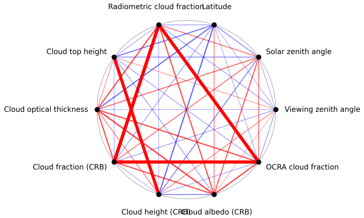
Figure 1: Map of correlation graph for 2025-04-19 to 2025-04-21.
