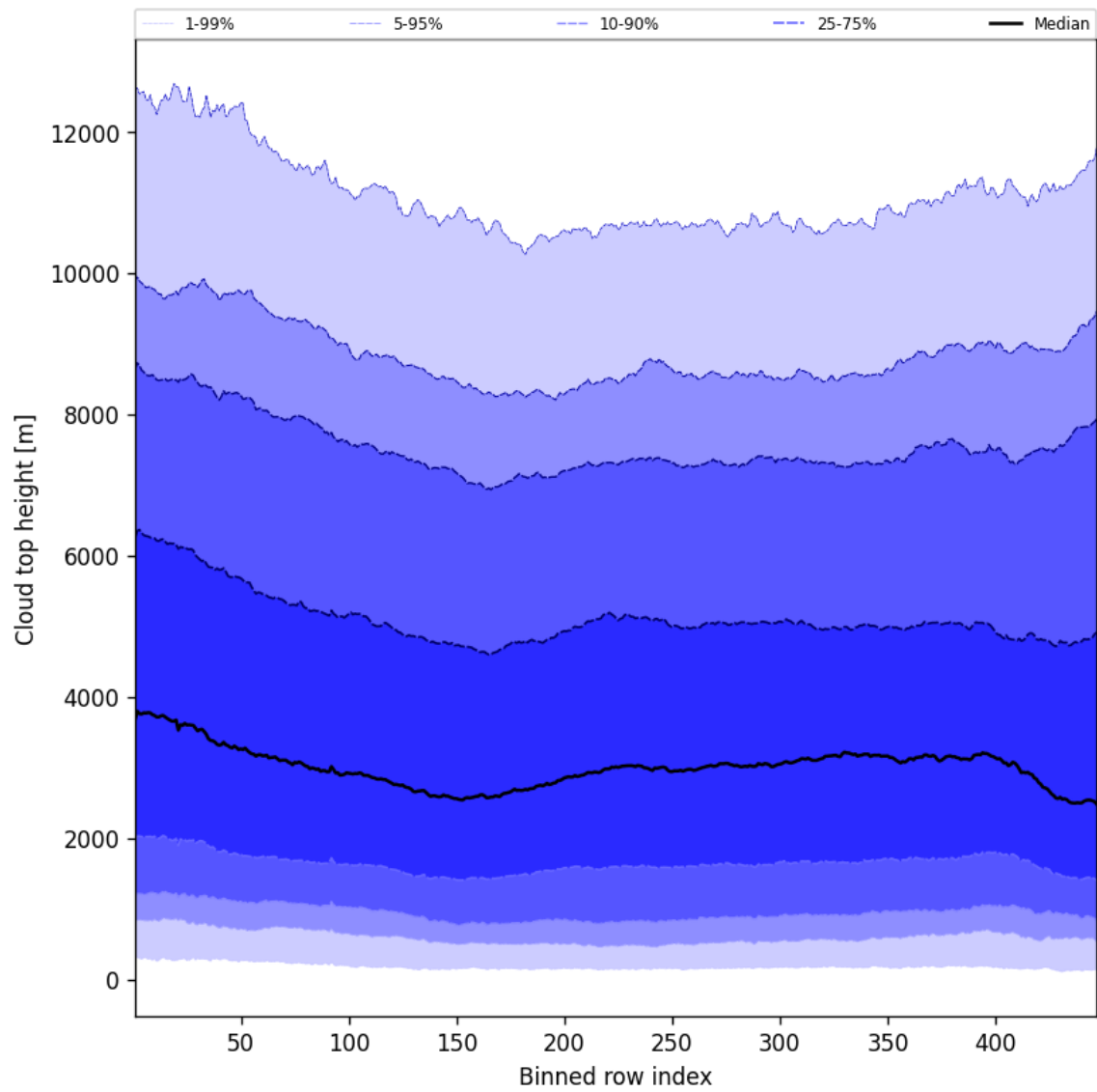
Figure 56: Along track statistics of “Cloud top height” for 2025-04-19 to 2025-04-21
