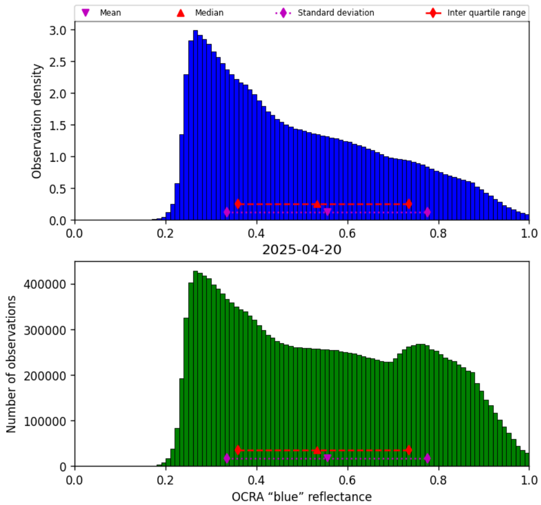
Figure 51: Histogram of “OCRA “blue” reflectance” for 2025-04-19 to 2025-04-21
