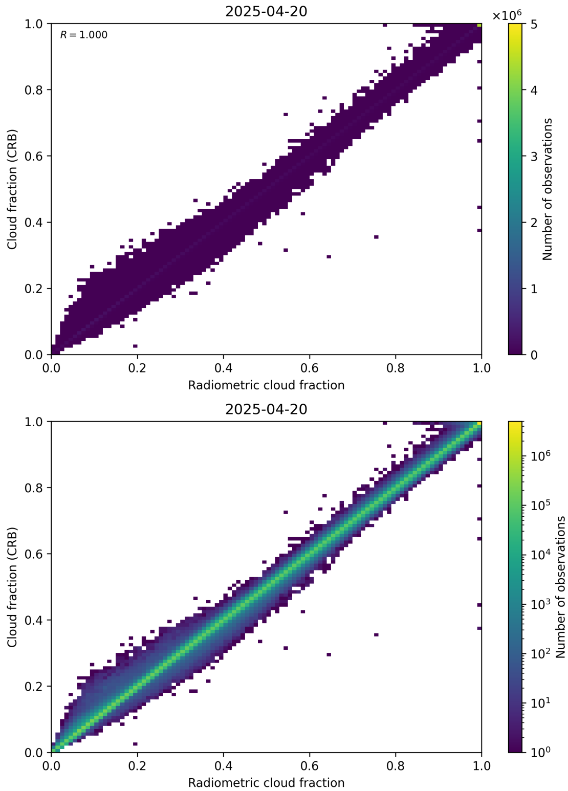
Figure 73: Scatter density plot of “Radiometric cloud fraction” against “Cloud fraction (CRB)” for 2025-04-19 to 2025-04-21.
