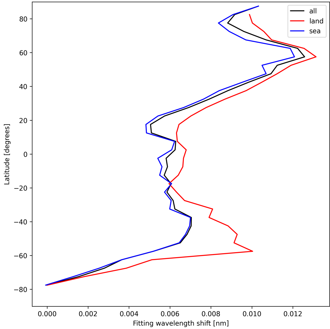
Figure 33: Zonal average of “Fitting wavelength shift” for 2025-04-19 to 2025-04-21.
