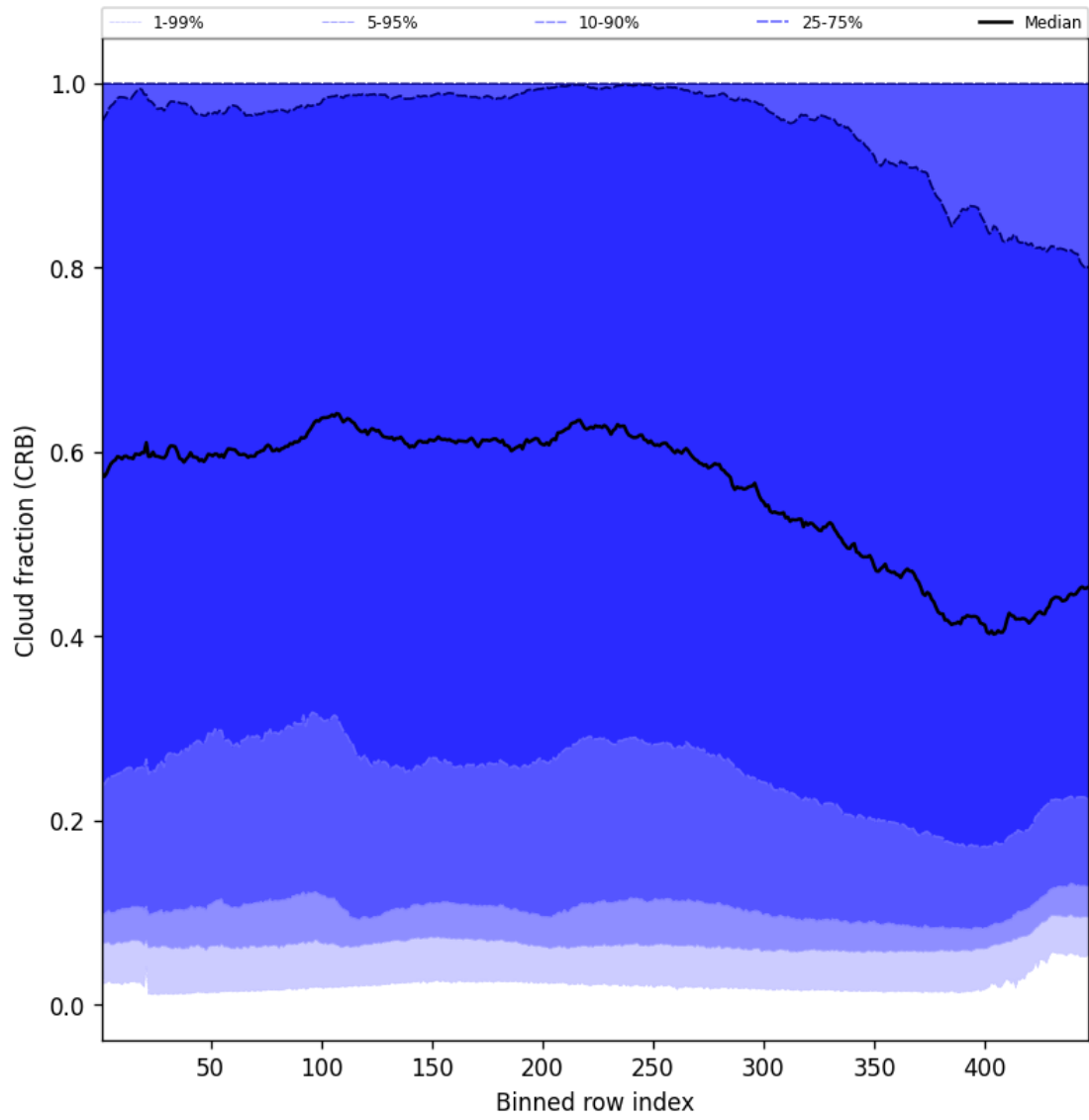
Figure 58: Along track statistics of “Cloud fraction (CRB)” for 2025-04-19 to 2025-04-21
