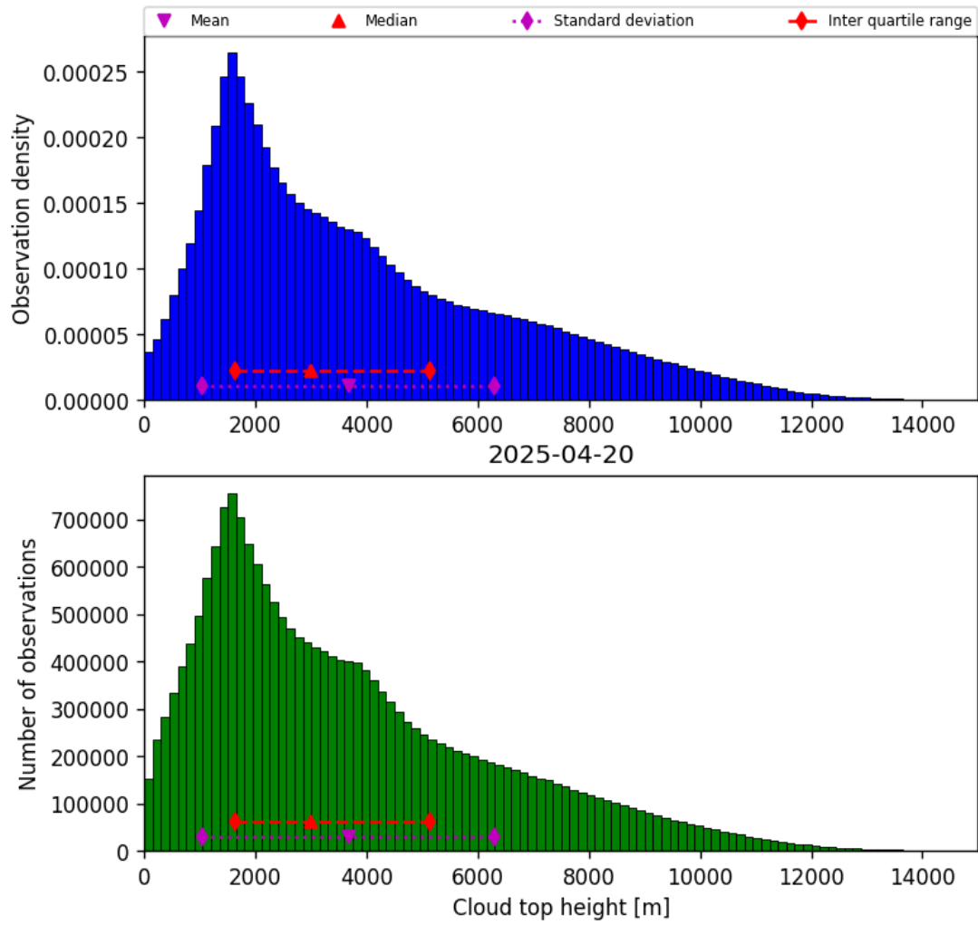
Figure 40: Histogram of “Cloud top height” for 2025-04-19 to 2025-04-21
