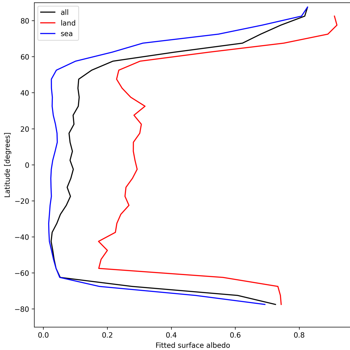
Figure 29: Zonal average of “Fitted surface albedo” for 2025-04-19 to 2025-04-21.
