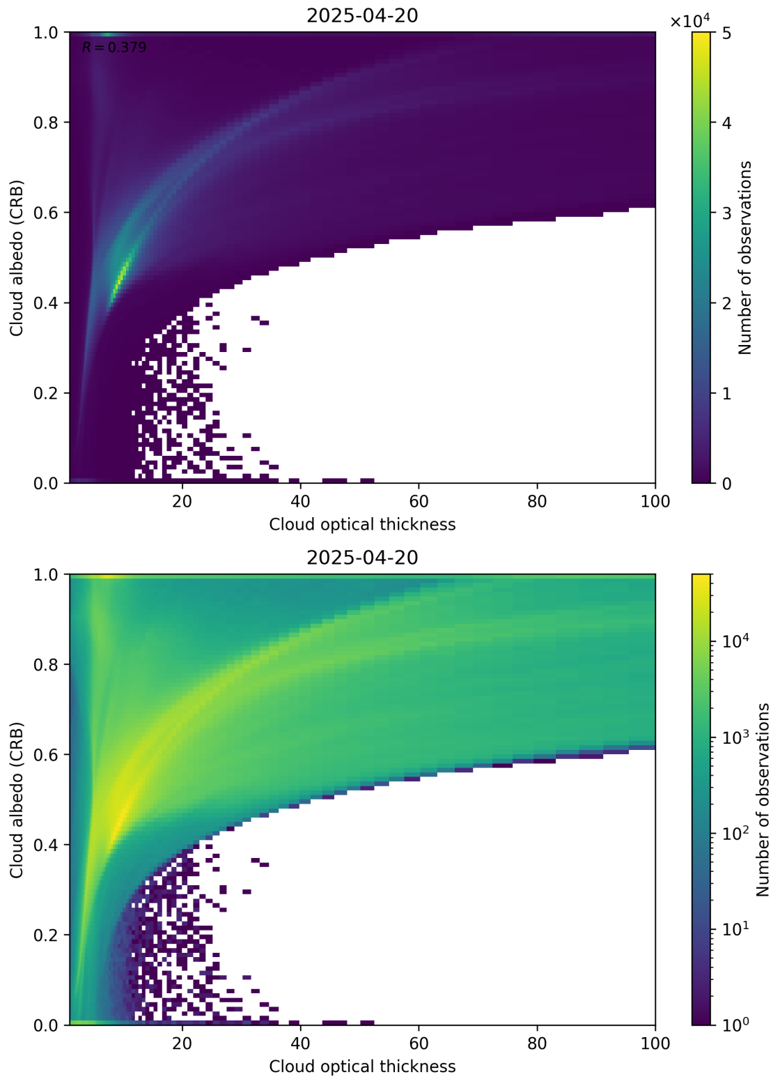
Figure 82: Scatter density plot of “Cloud optical thickness” against “Cloud albedo (CRB)” for 2025-04-19 to 2025-04-21.
