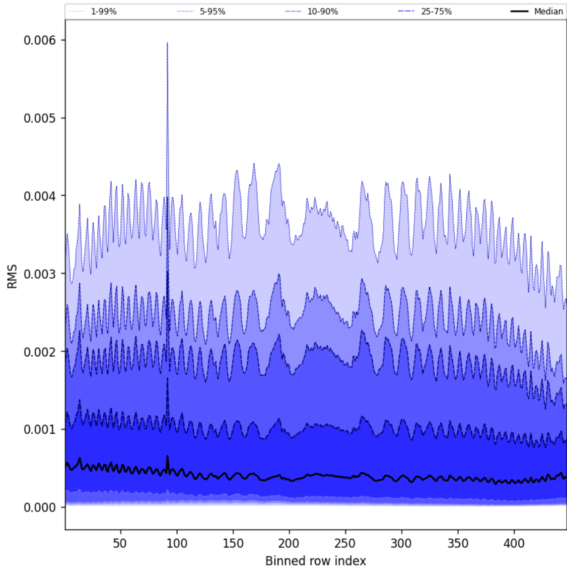
Figure 63: Along track statistics of “RMS” for 2025-04-19 to 2025-04-21
