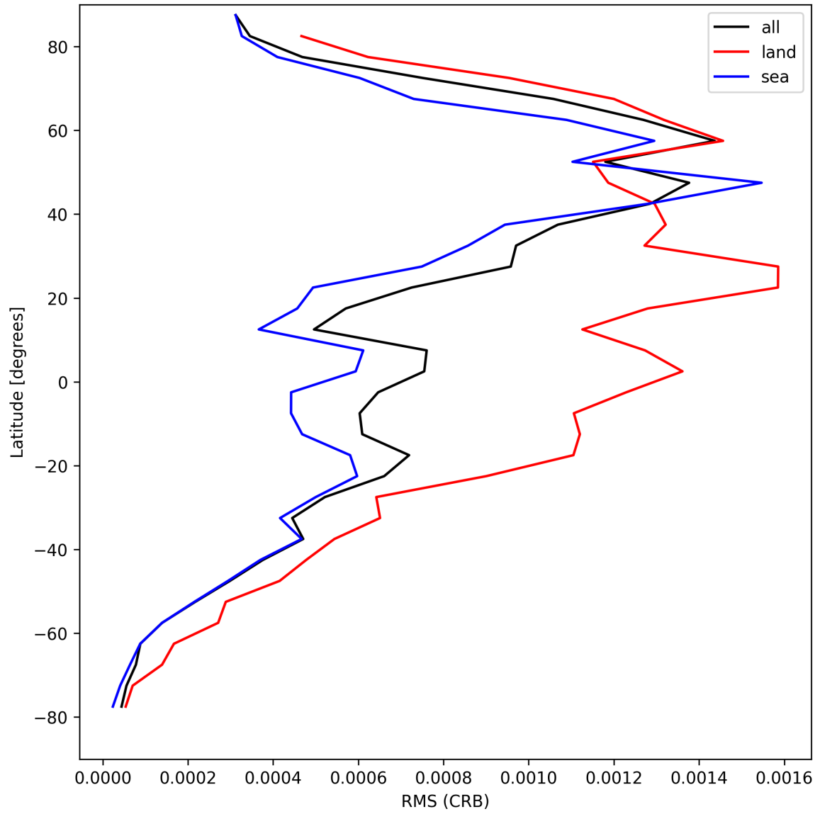
Figure 32: Zonal average of “RMS (CRB)” for 2025-04-19 to 2025-04-21.
