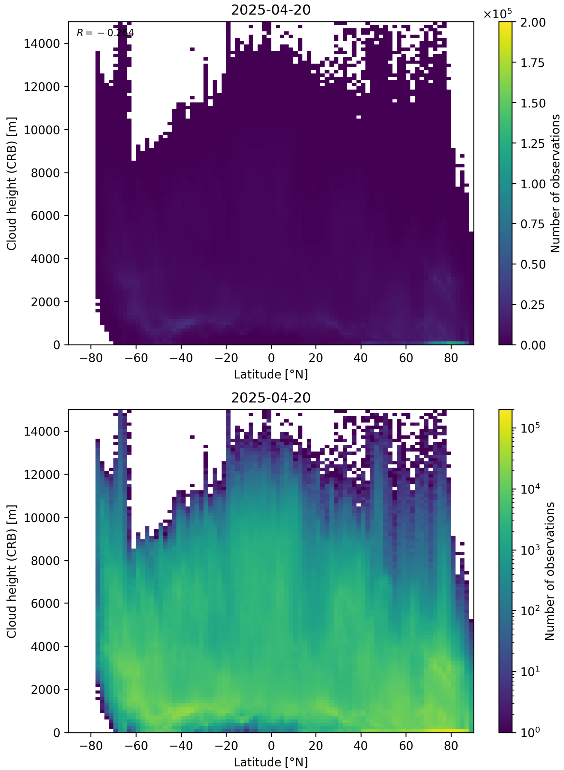
Figure 95: Scatter density plot of “Latitude” against “Cloud height (CRB)” for 2025-04-19 to 2025-04-21.
