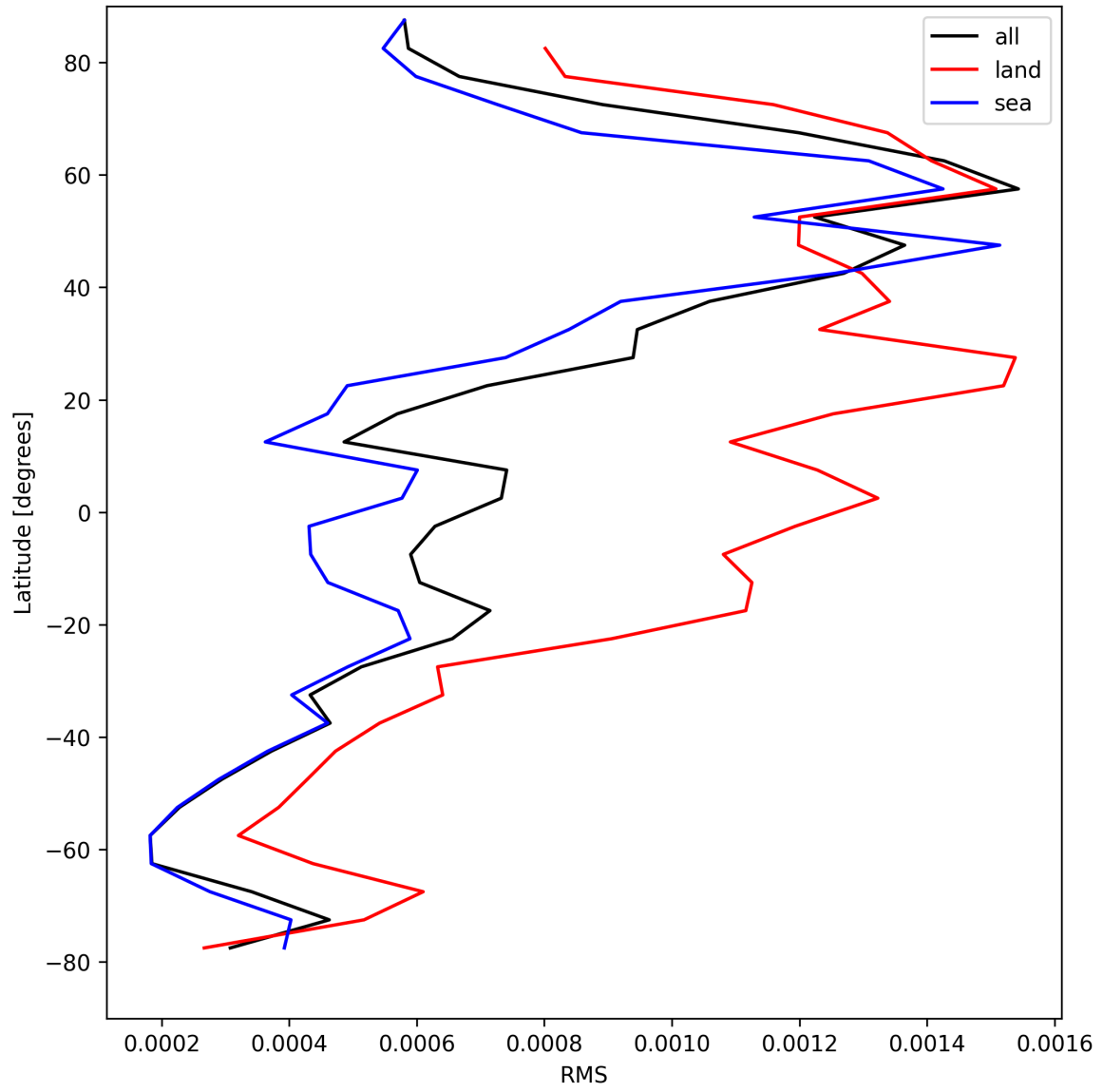
Figure 31: Zonal average of “RMS” for 2025-04-19 to 2025-04-21.
