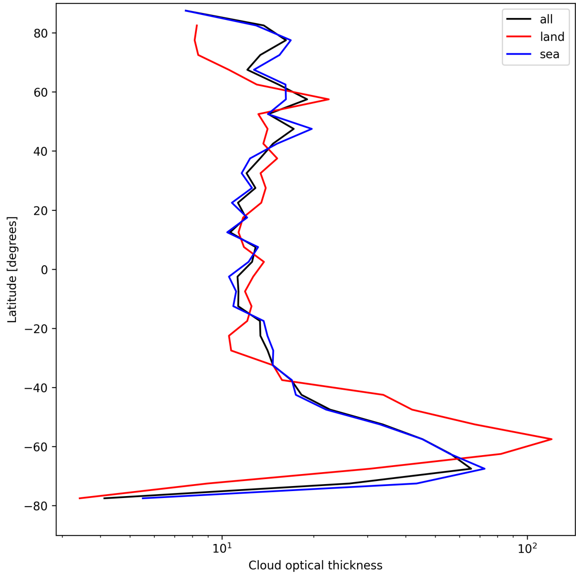
Figure 25: Zonal average of “Cloud optical thickness” for 2025-04-19 to 2025-04-21.
