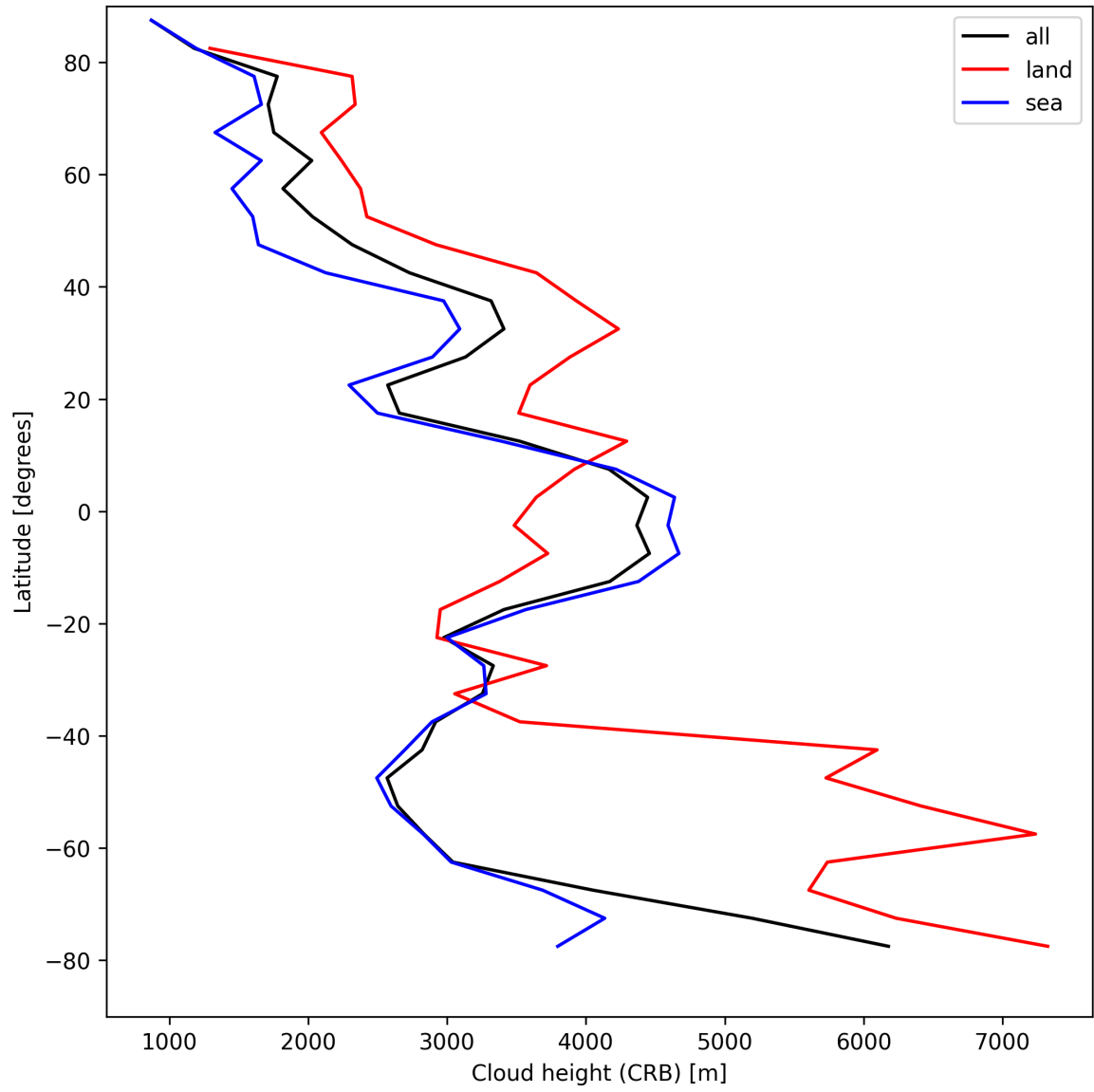
Figure 27: Zonal average of “Cloud height (CRB)” for 2025-04-19 to 2025-04-21.
