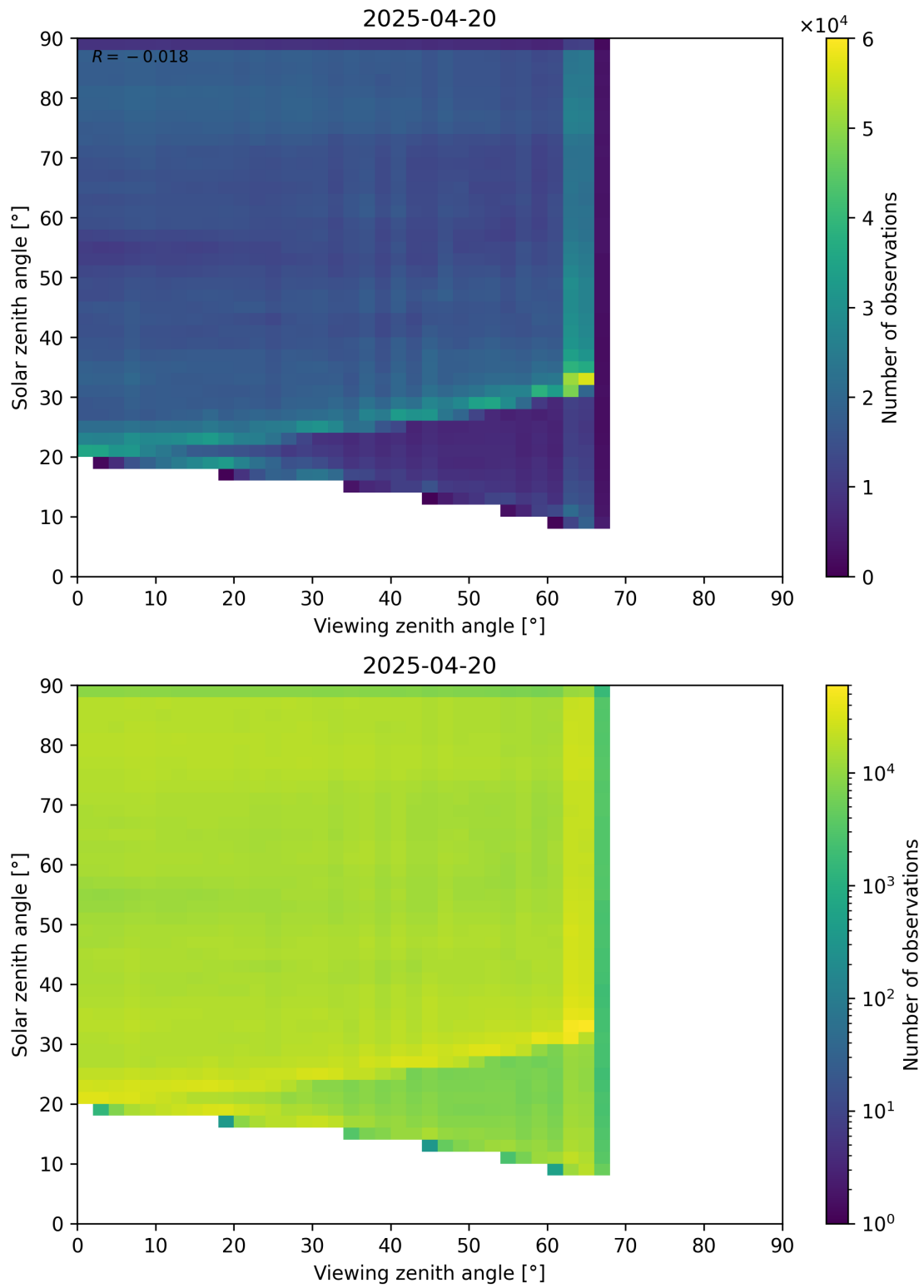
Figure 114: Scatter density plot of “Viewing zenith angle” against “Solar zenith angle” for 2025-04-19 to 2025-04-21.
