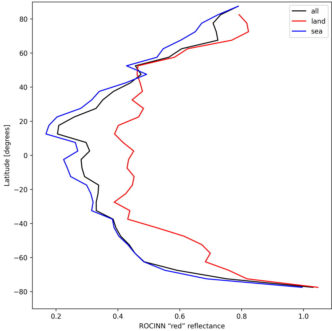
Figure 37: Zonal average of “ROCINN “red” reflectance” for 2025-04-19 to 2025-04-21.
