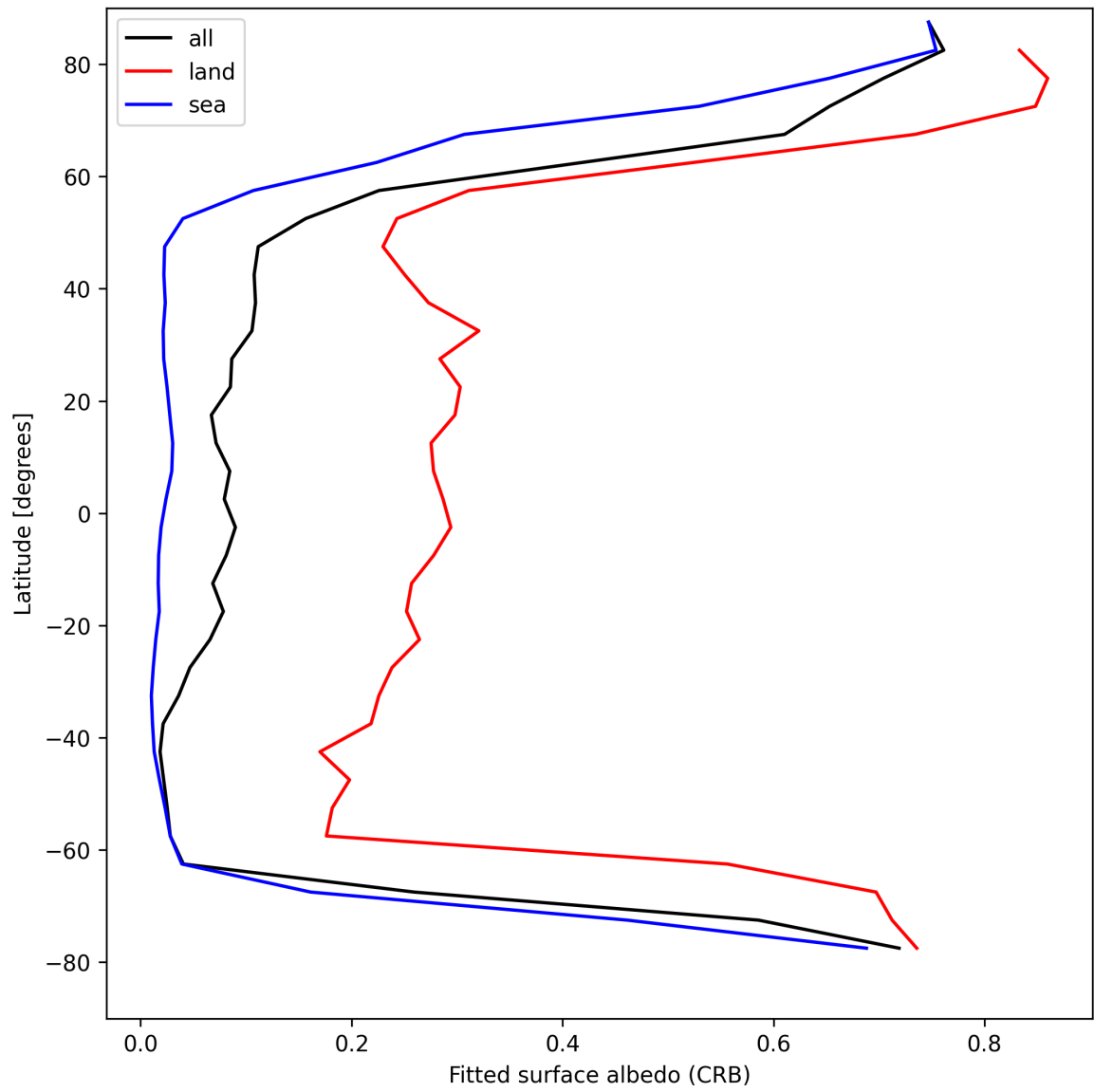
Figure 30: Zonal average of “Fitted surface albedo (CRB)” for 2025-04-19 to 2025-04-21.
