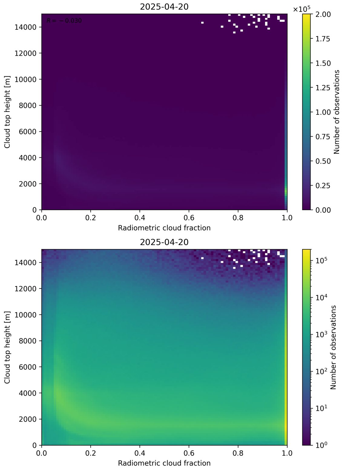
Figure 76: Scatter density plot of “Radiometric cloud fraction” against “Cloud top height” for 2025-04-19 to 2025-04-21.
