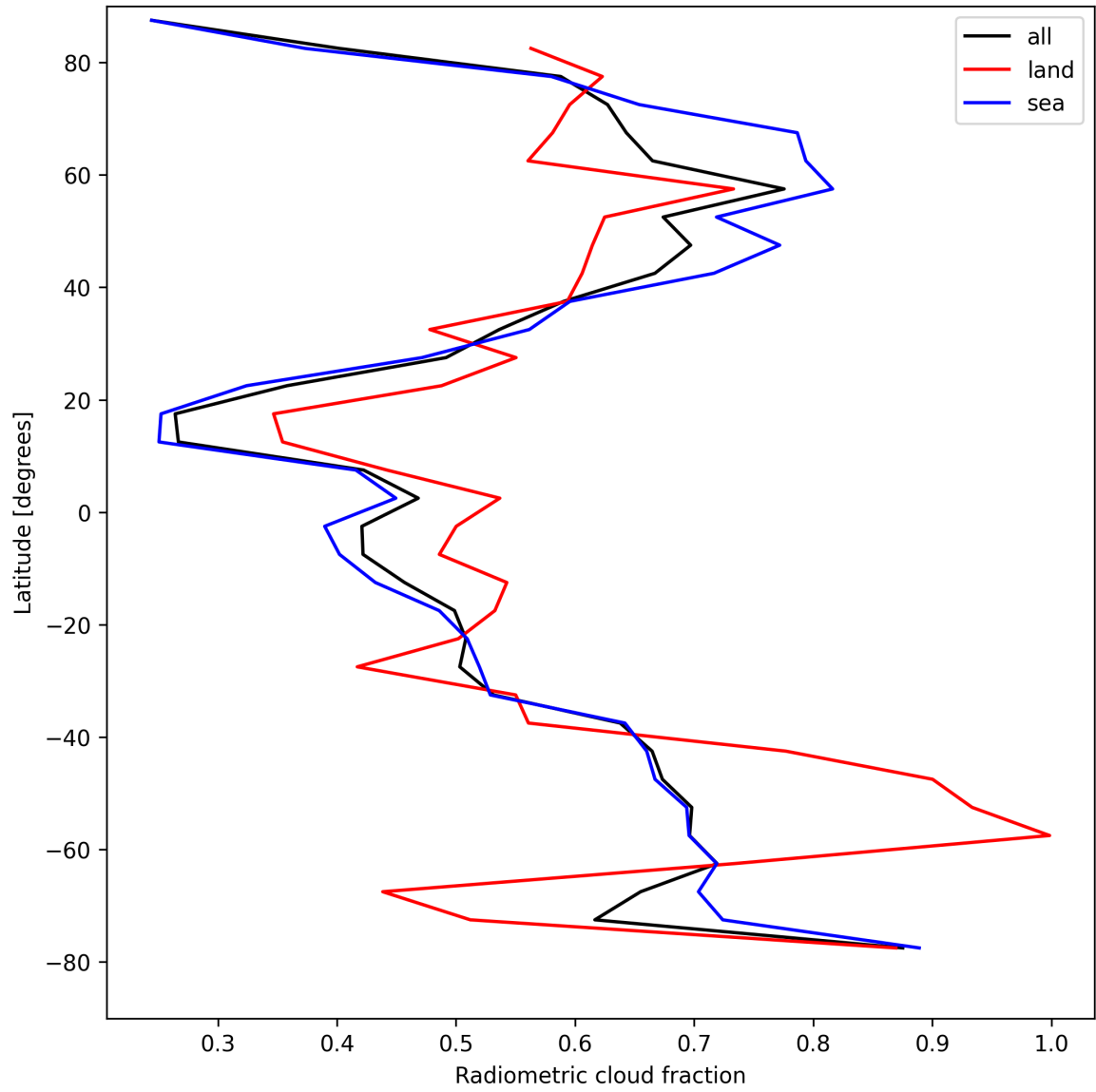
Figure 23: Zonal average of “Radiometric cloud fraction” for 2025-04-19 to 2025-04-21.
