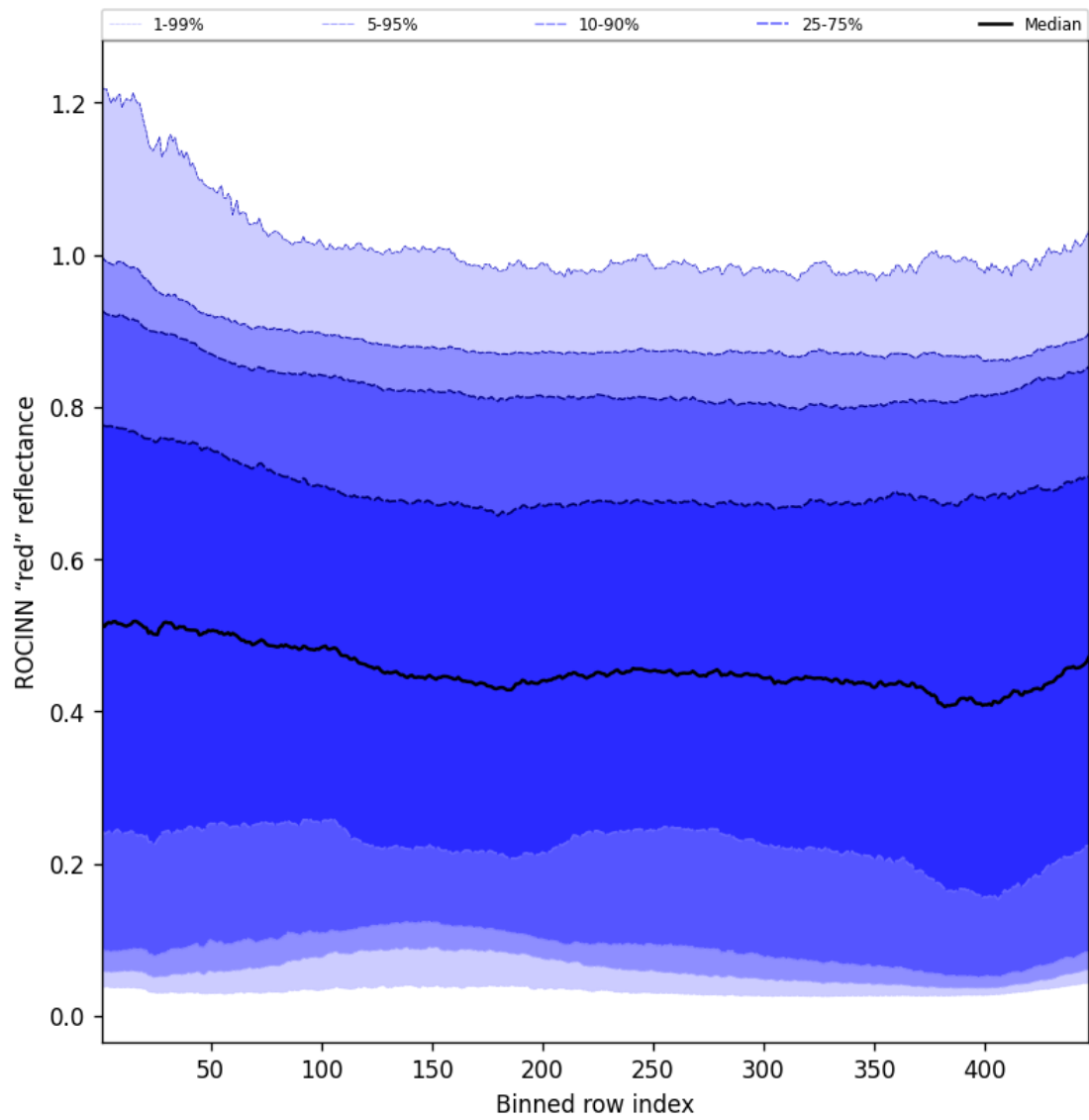
Figure 69: Along track statistics of "ROCINN "red" reflectance" for 2025-04-19 to 2025-04-21
