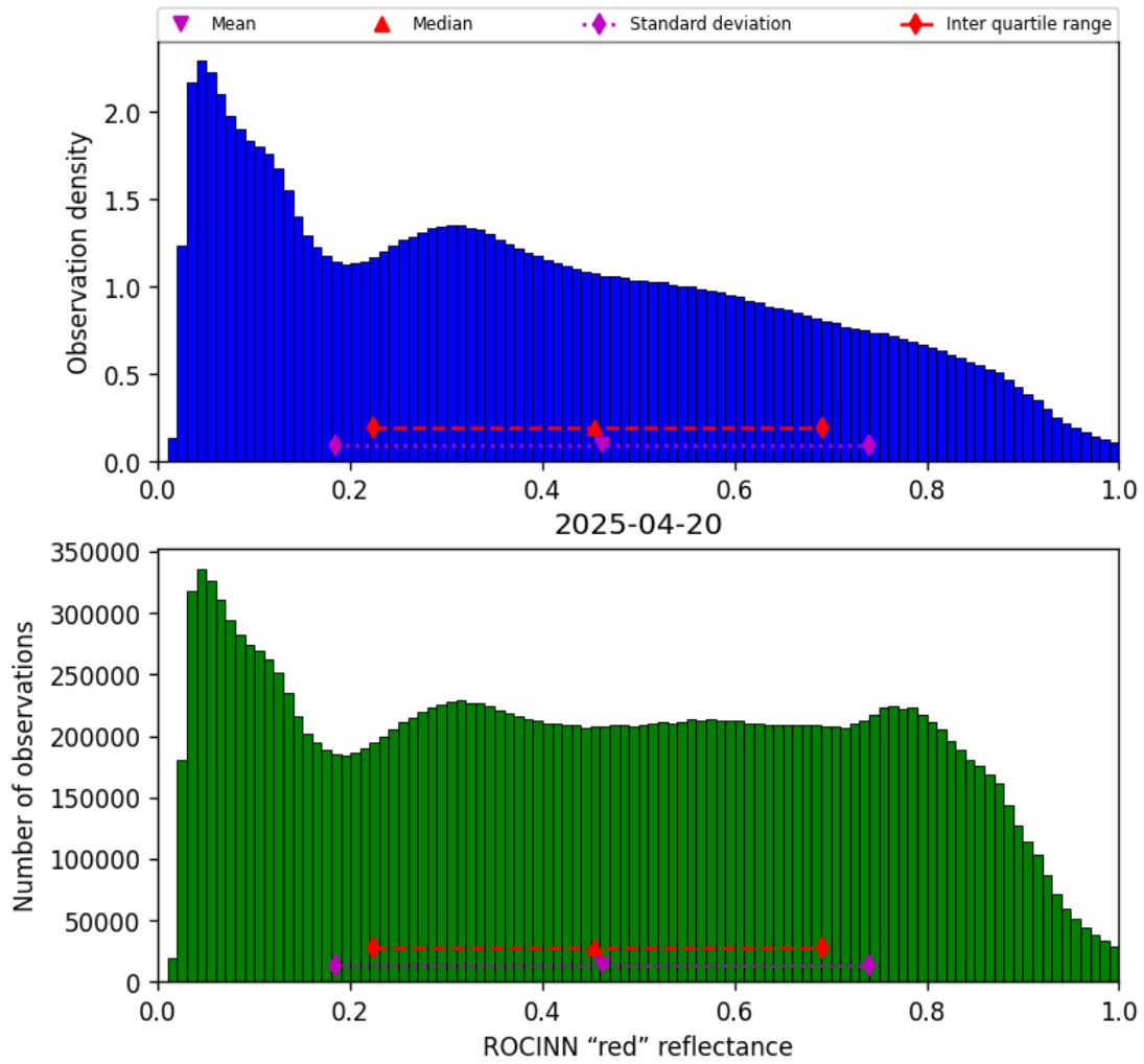
Figure 53: Histogram of “ROCINN “red” reflectance” for 2025-04-19 to 2025-04-21
