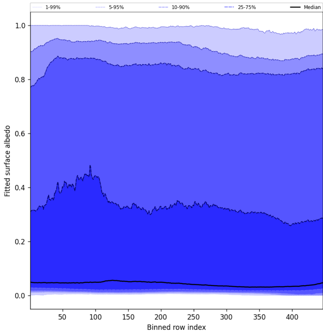
Figure 61: Along track statistics of “Fitted surface albedo” for 2025-04-19 to 2025-04-21
