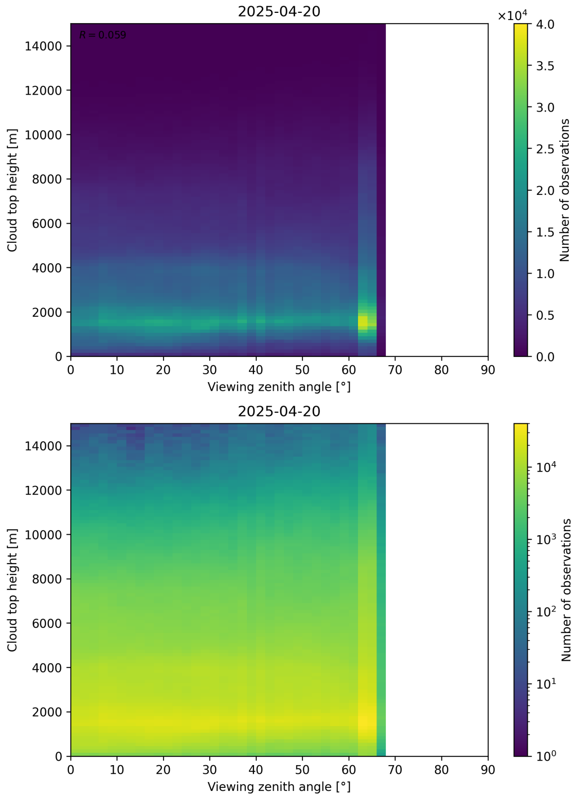
Figure 112: Scatter density plot of “Viewing zenith angle” against “Cloud top height” for 2025-04-19 to 2025-04-21.
