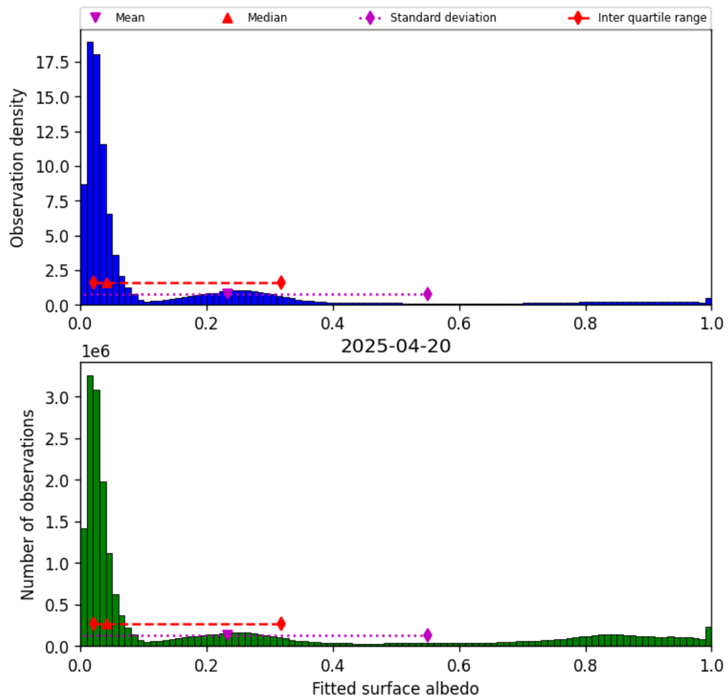
Figure 45: Histogram of “Fitted surface albedo” for 2025-04-19 to 2025-04-21
