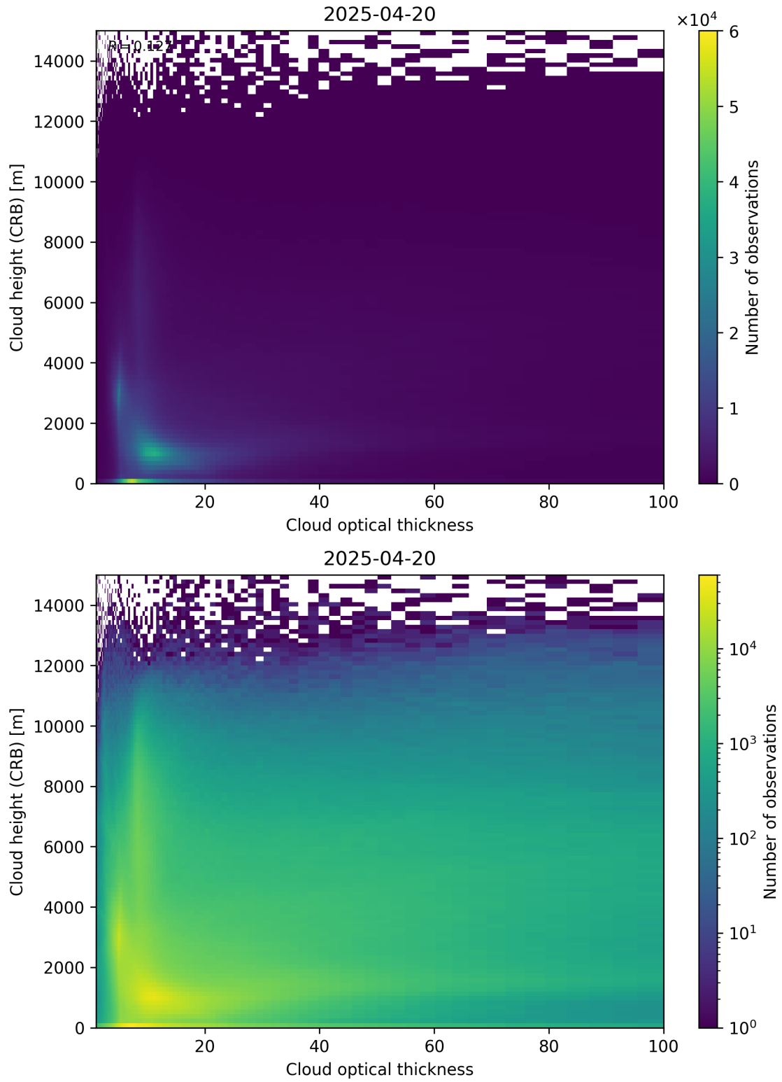
Figure 85: Scatter density plot of “Cloud optical thickness” against “Cloud height (CRB)” for 2025-04-19 to 2025-04-21.
