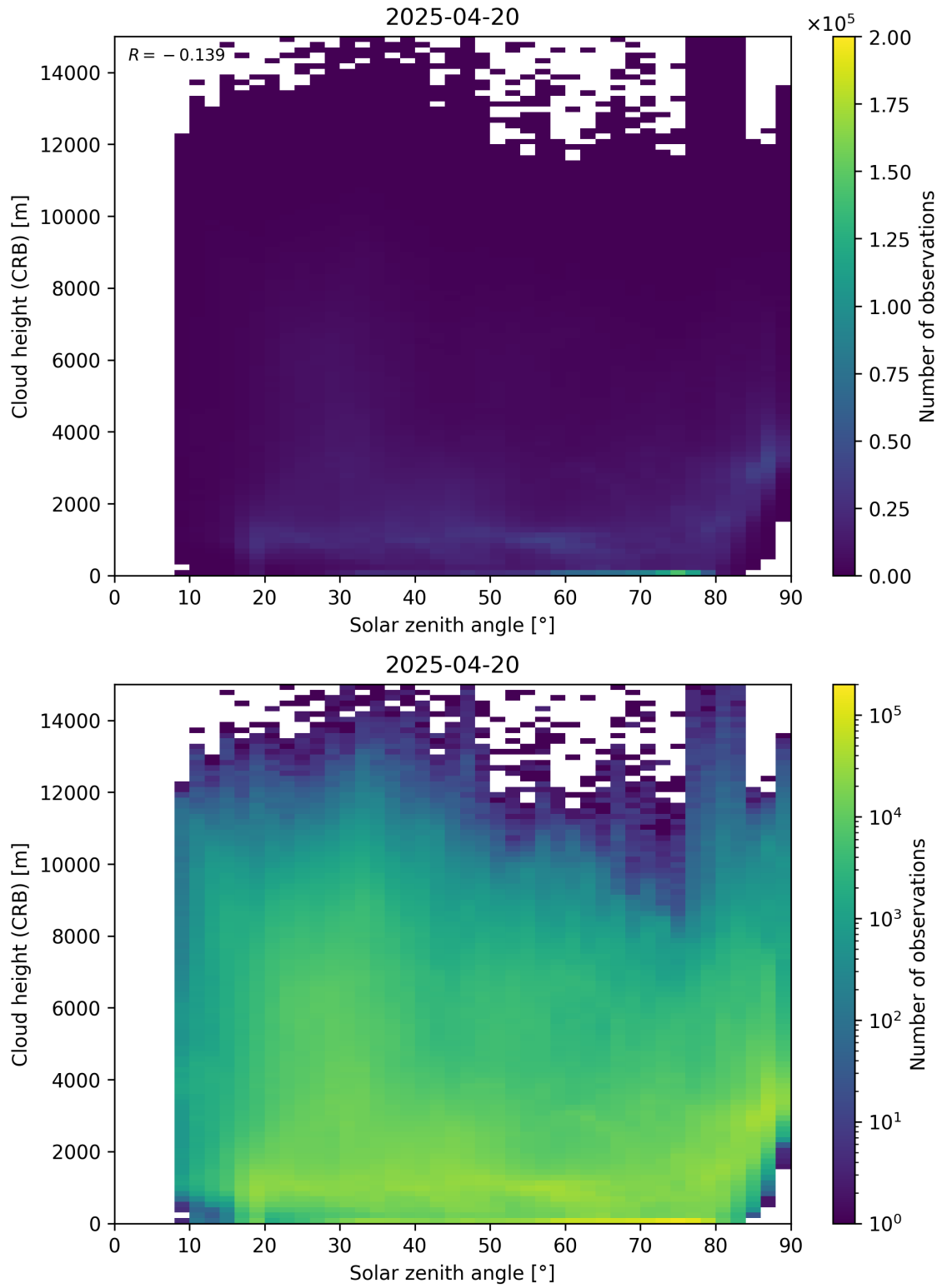
Figure 102: Scatter density plot of “Solar zenith angle” against “Cloud height (CRB)” for 2025-04-19 to 2025-04-21.
