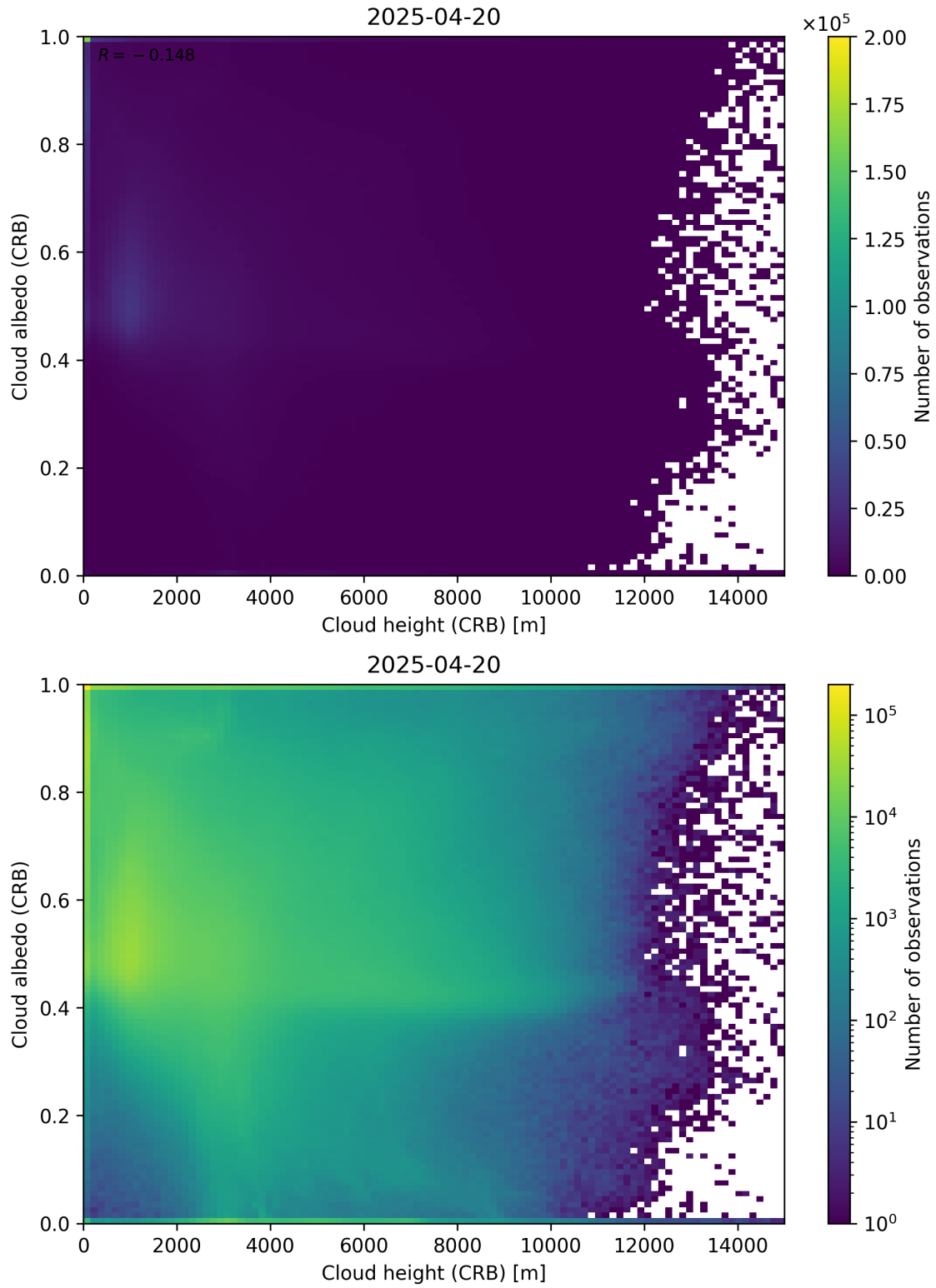
Figure 80: Scatter density plot of “Cloud height (CRB)” against “Cloud albedo (CRB)” for 2025-04-19 to 2025-04-21.
