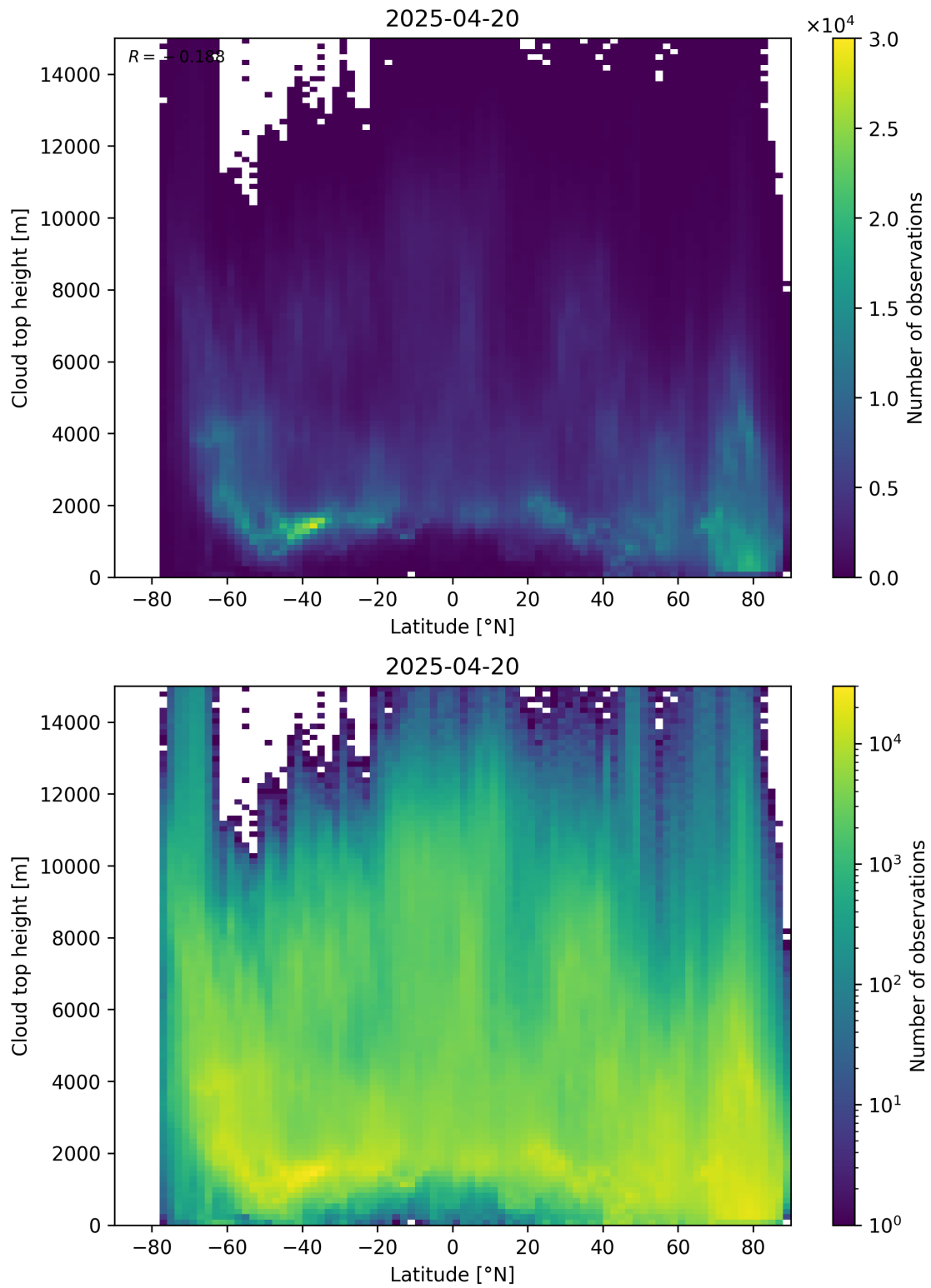
Figure 97: Scatter density plot of “Latitude” against “Cloud top height” for 2025-04-19 to 2025-04-21.
