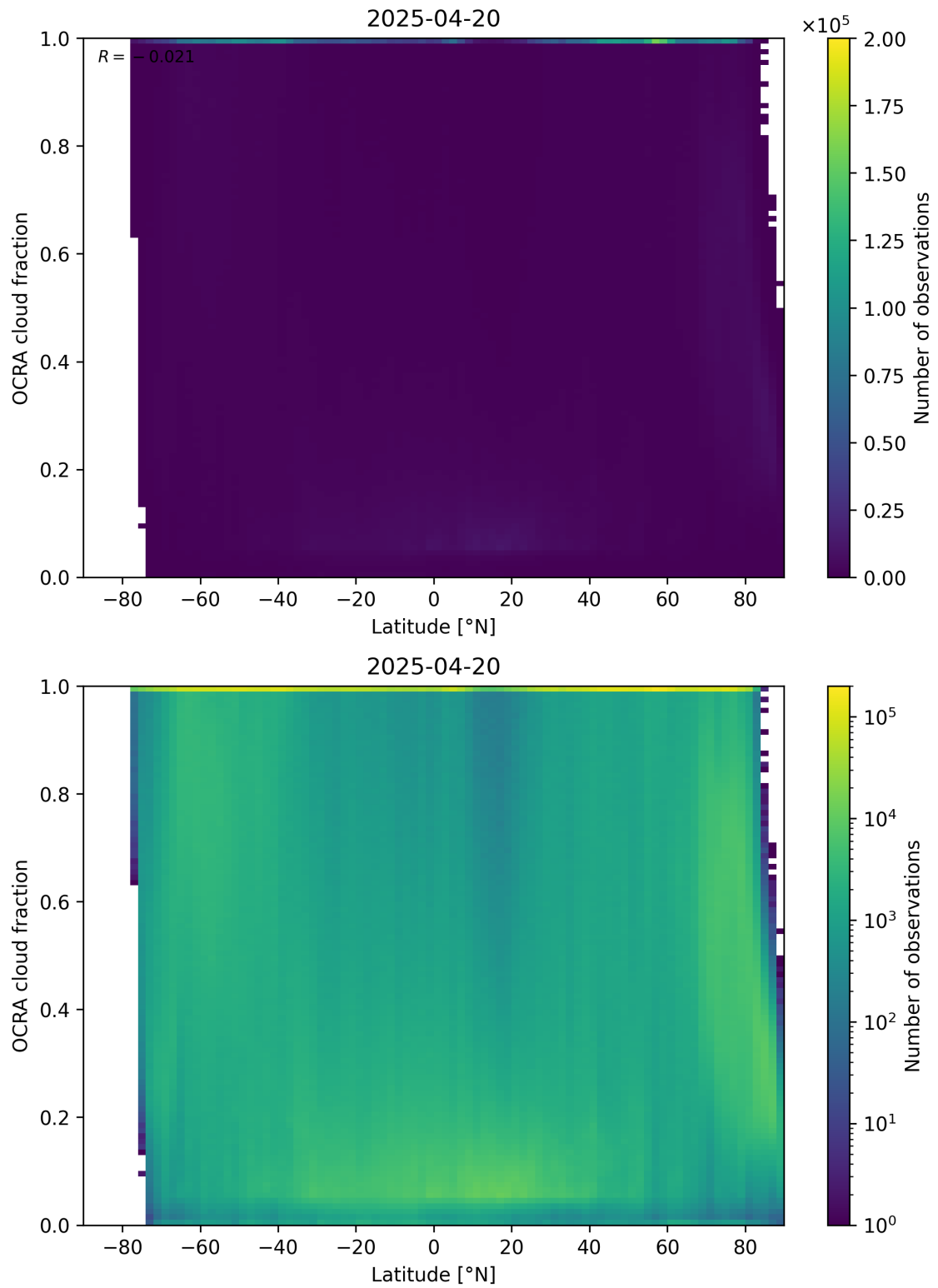
Figure 93: Scatter density plot of “Latitude” against “OCRA cloud fraction” for 2025-04-19 to 2025-04-21.
