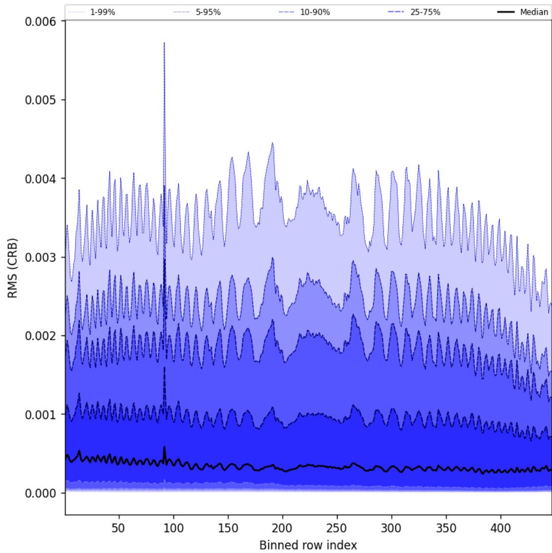
Figure 64: Along track statistics of “RMS (CRB)” for 2025-04-19 to 2025-04-21
