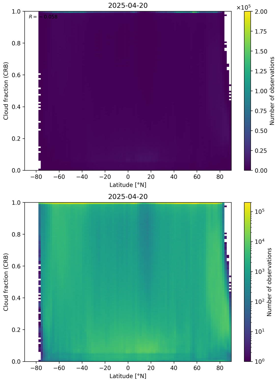
Figure 94: Scatter density plot of “Latitude” against “Cloud fraction (CRB)” for 2025-04-19 to 2025-04-21.
