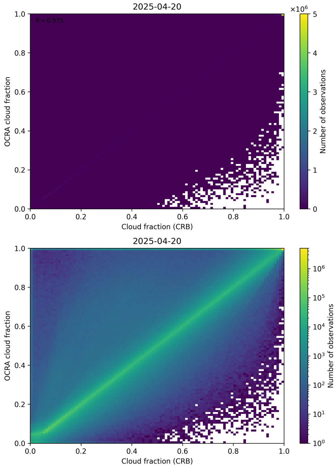
Figure 78: Scatter density plot of “Cloud fraction (CRB)” against “OCRA cloud fraction” for 2025-04-19 to 2025-04-21.
