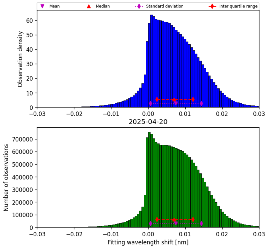
Figure 49: Histogram of “Fitting wavelength shift” for 2025-04-19 to 2025-04-21
