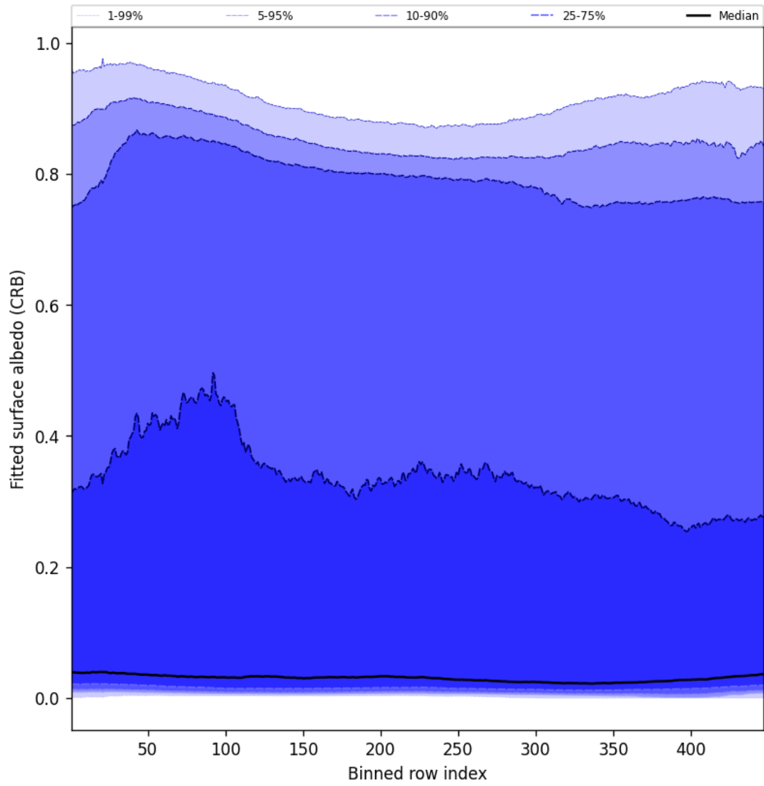
Figure 62: Along track statistics of “Fitted surface albedo (CRB)” for 2025-04-19 to 2025-04-21
