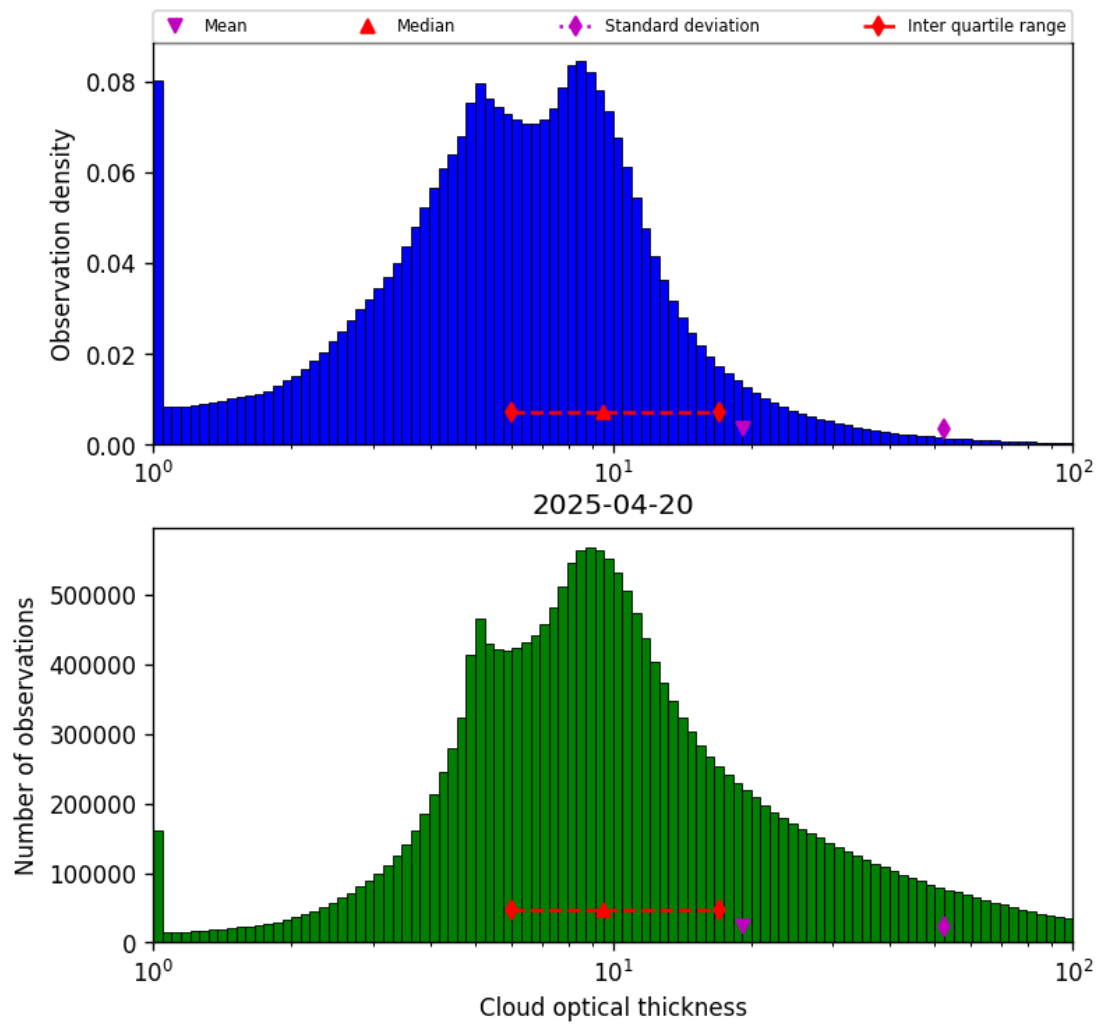
Figure 41: Histogram of “Cloud optical thickness” for 2025-04-19 to 2025-04-21
