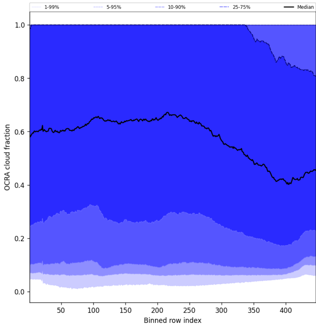
Figure 66: Along track statistics of “OCRA cloud fraction” for 2025-04-19 to 2025-04-21
