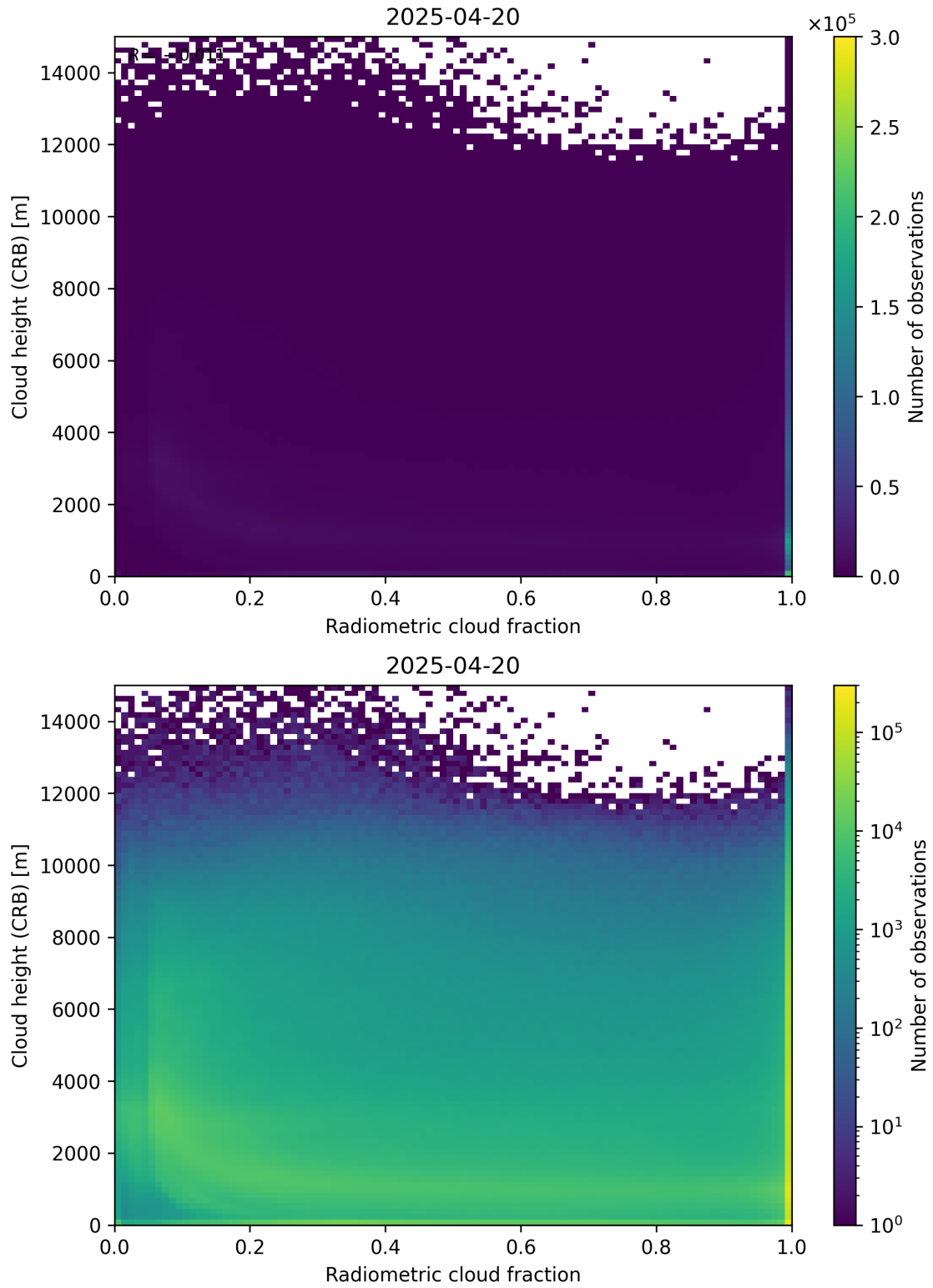
Figure 74: Scatter density plot of “Radiometric cloud fraction” against “Cloud height (CRB)” for 2025-04-19 to 2025-04-21.
