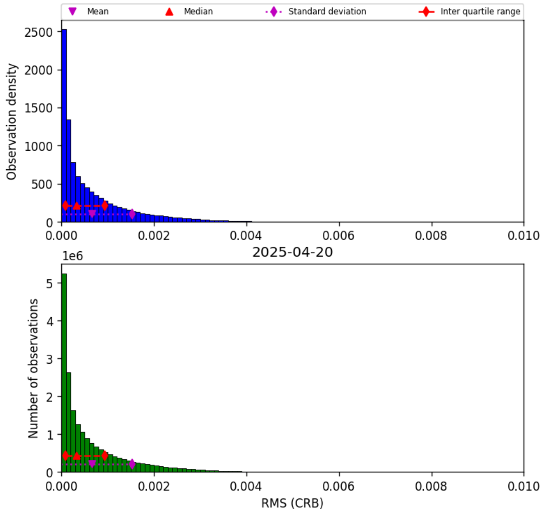
Figure 48: Histogram of “RMS (CRB)” for 2025-04-19 to 2025-04-21
