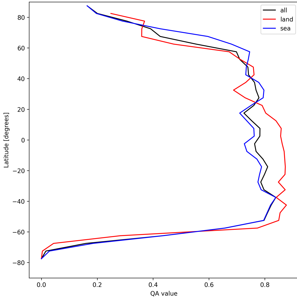
Figure 22: Zonal average of “QA value” for 2025-04-19 to 2025-04-21.
