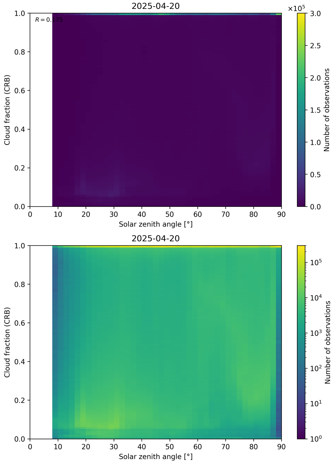
Figure 101: Scatter density plot of “Solar zenith angle” against “Cloud fraction (CRB)” for 2025-04-19 to 2025-04-21.
