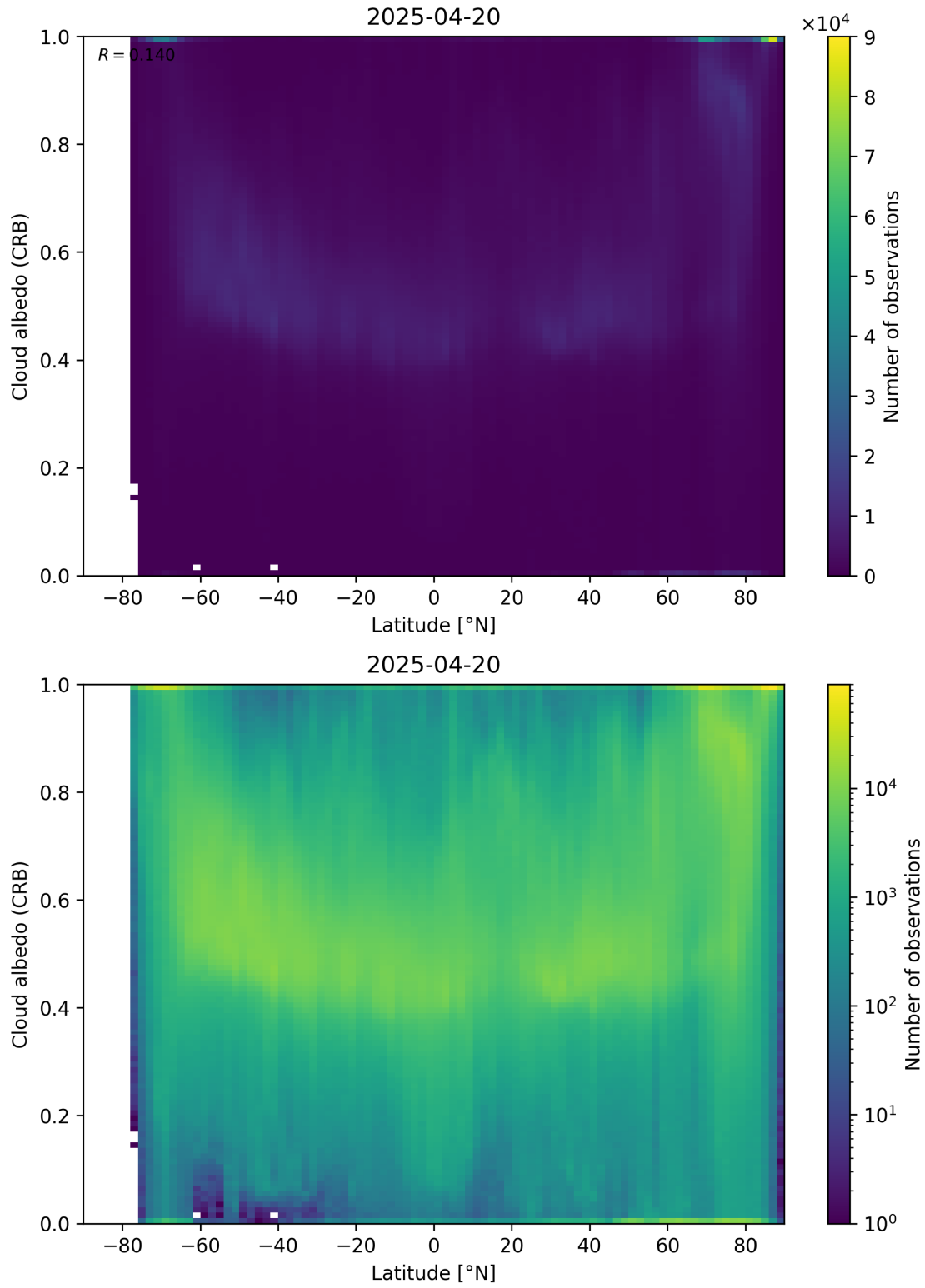
Figure 91: Scatter density plot of “Latitude” against “Cloud albedo (CRB)” for 2025-04-19 to 2025-04-21.
