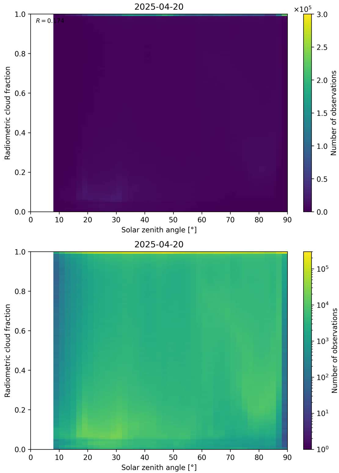
Figure 99: Scatter density plot of “Solar zenith angle” against “Radiometric cloud fraction” for 2025-04-19 to 2025-04-21.
