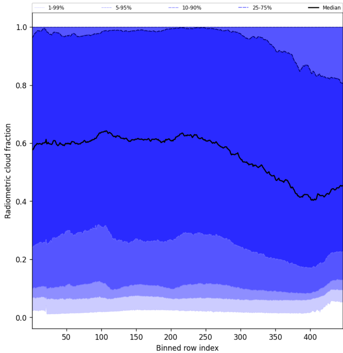
Figure 55: Along track statistics of “Radiometric cloud fraction” for 2025-04-19 to 2025-04-21
