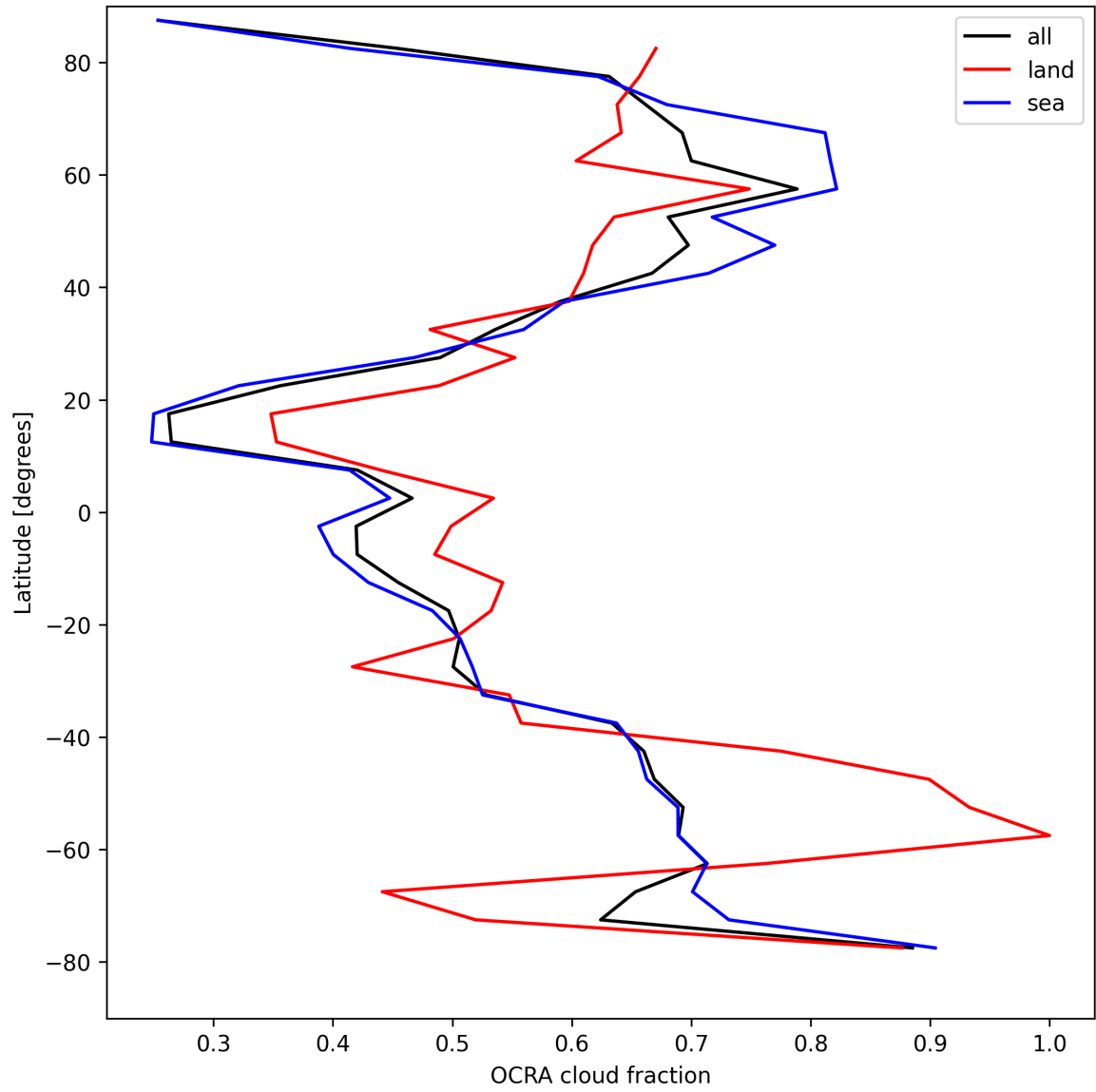
Figure 34: Zonal average of “OCRA cloud fraction” for 2025-04-19 to 2025-04-21.
