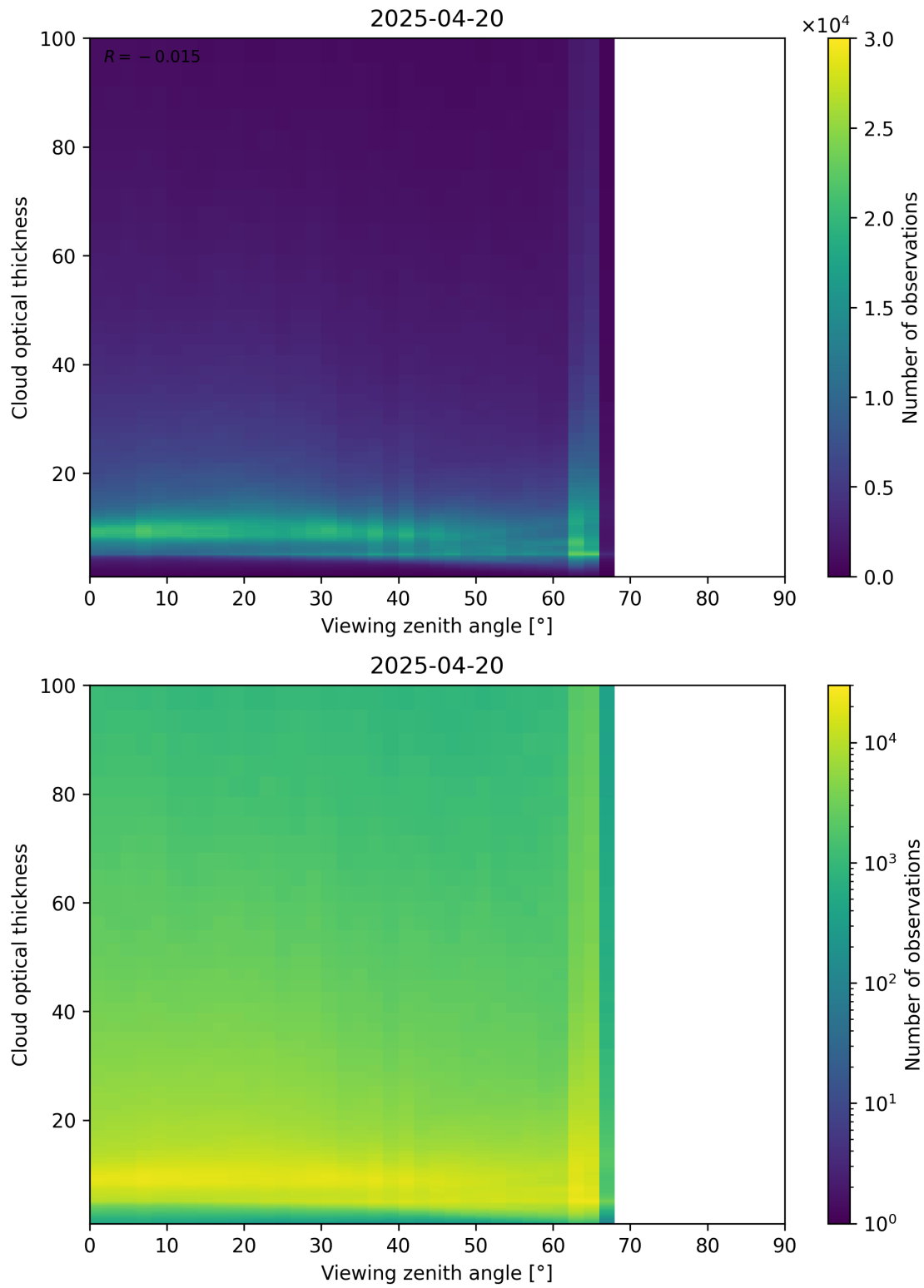
Figure 111: Scatter density plot of “Viewing zenith angle” against “Cloud optical thickness” for 2025-04-19 to 2025-04-21.
