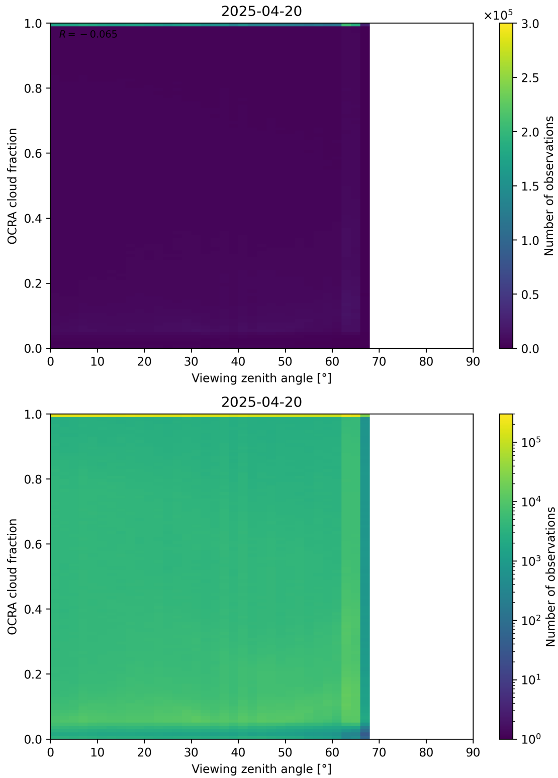
Figure 108: Scatter density plot of “Viewing zenith angle” against “OCRA cloud fraction” for 2025-04-19 to 2025-04-21.
