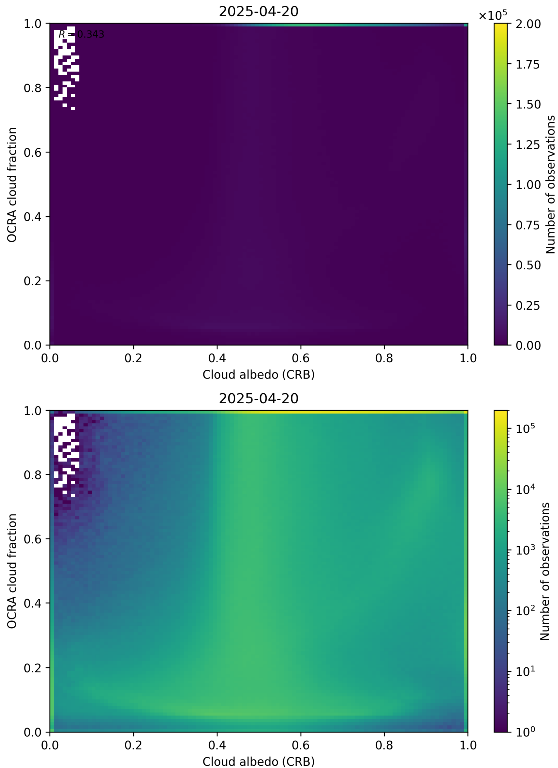
Figure 70: Scatter density plot of “Cloud albedo (CRB)” against “OCRA cloud fraction” for 2025-04-19 to 2025-04-21.
