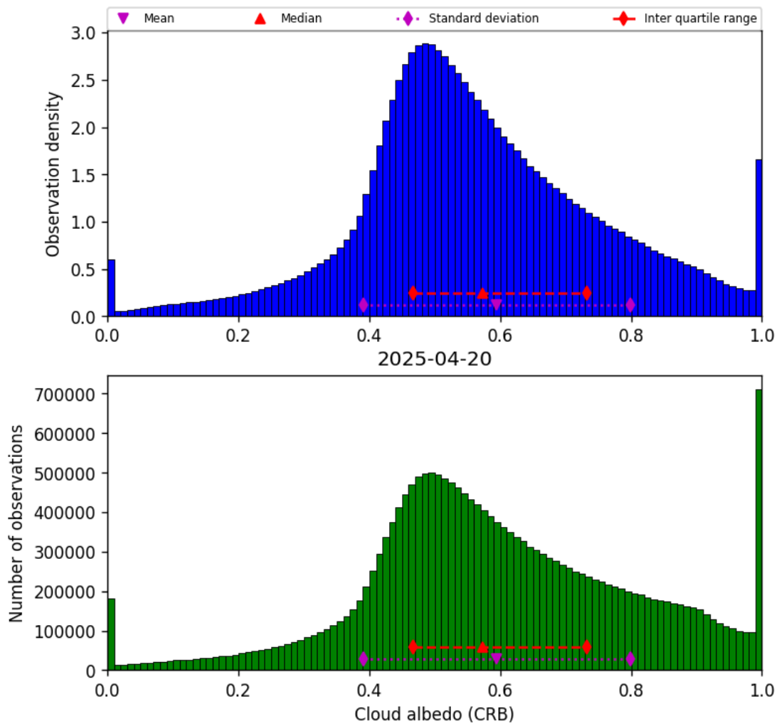
Figure 44: Histogram of “Cloud albedo (CRB)” for 2025-04-19 to 2025-04-21
