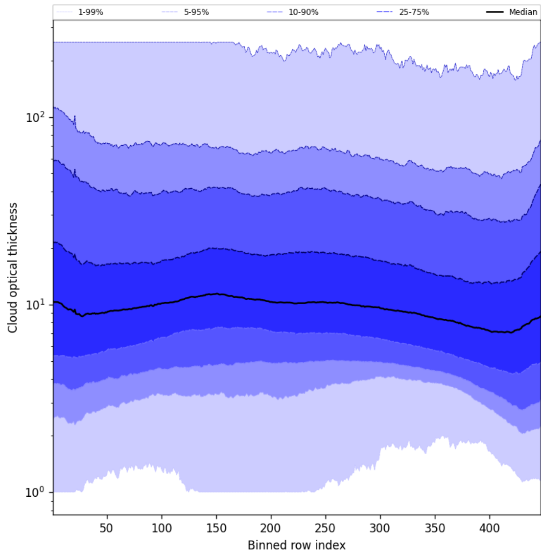
Figure 57: Along track statistics of “Cloud optical thickness” for 2025-04-19 to 2025-04-21
