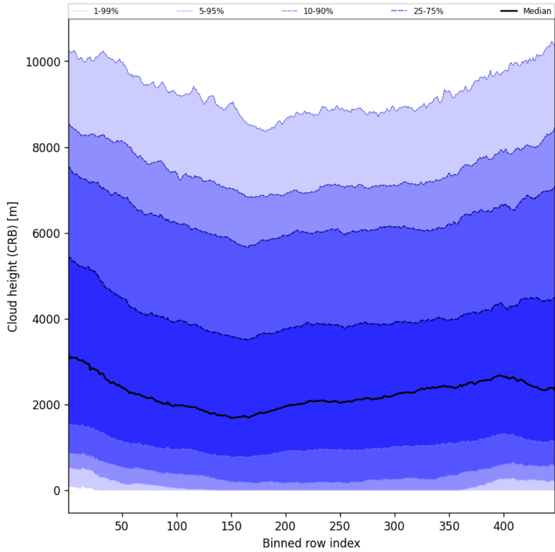
Figure 59: Along track statistics of “Cloud height (CRB)” for 2025-04-19 to 2025-04-21
