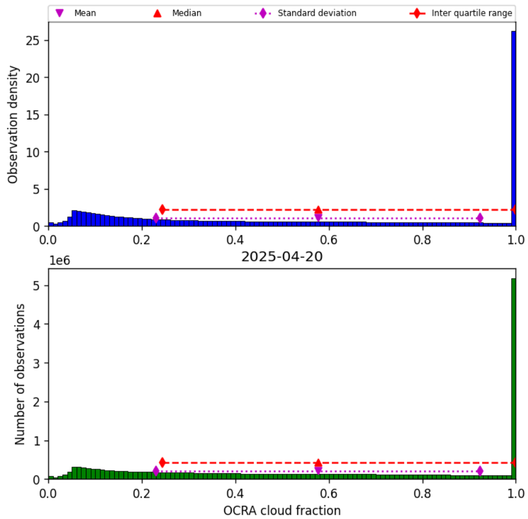
Figure 50: Histogram of “OCRA cloud fraction” for 2025-04-19 to 2025-04-21
