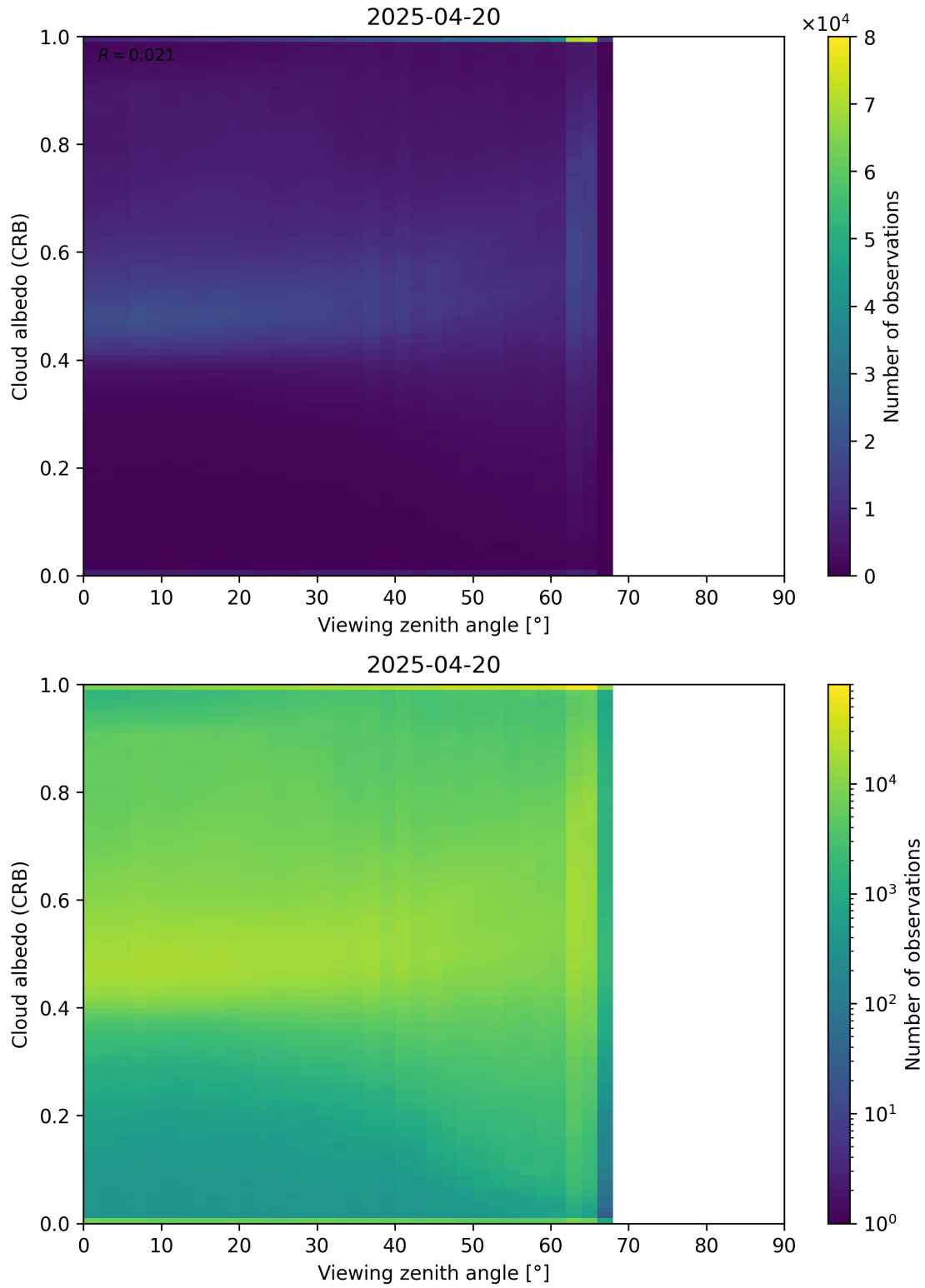
Figure 106: Scatter density plot of “Viewing zenith angle” against “Cloud albedo (CRB)” for 2025-04-19 to 2025-04-21.
