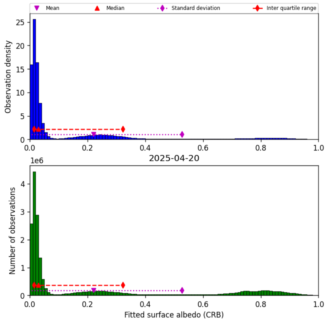
Figure 46: Histogram of “Fitted surface albedo (CRB)” for 2025-04-19 to 2025-04-21
