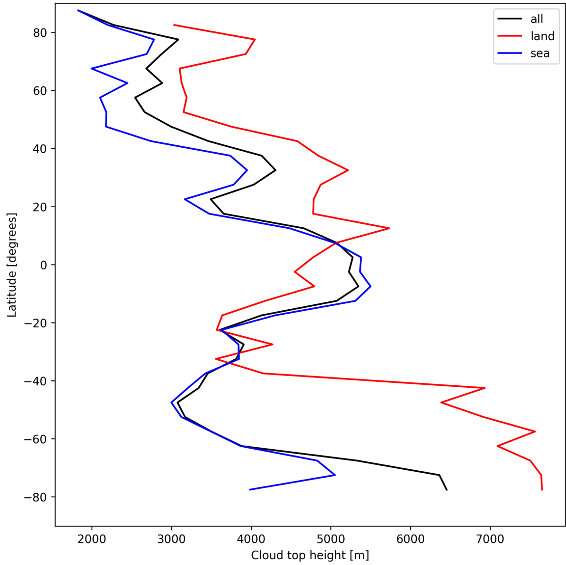
Figure 24: Zonal average of “Cloud top height” for 2025-04-19 to 2025-04-21.
