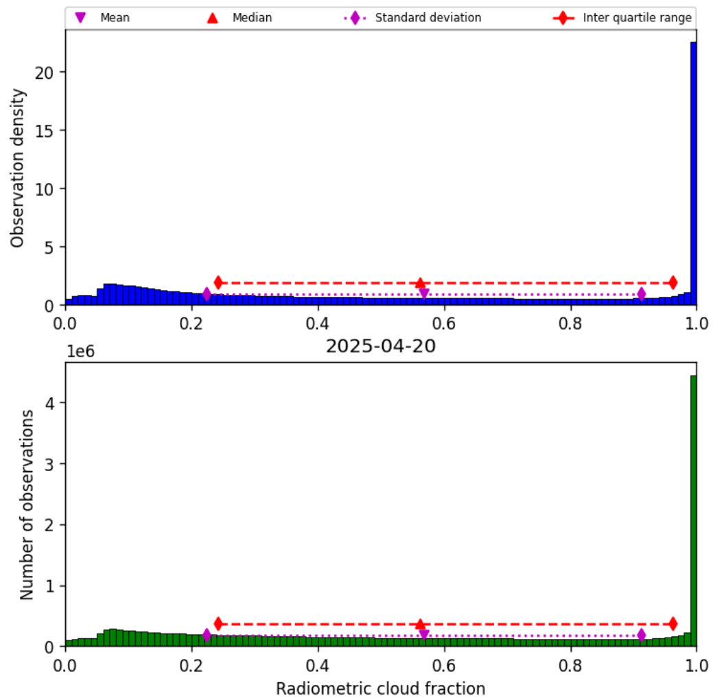
Figure 39: Histogram of “Radiometric cloud fraction” for 2025-04-19 to 2025-04-21
