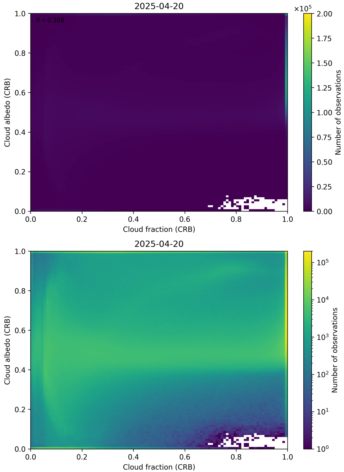
Figure 77: Scatter density plot of “Cloud fraction (CRB)” against “Cloud albedo (CRB)” for 2025-04-19 to 2025-04-21.
