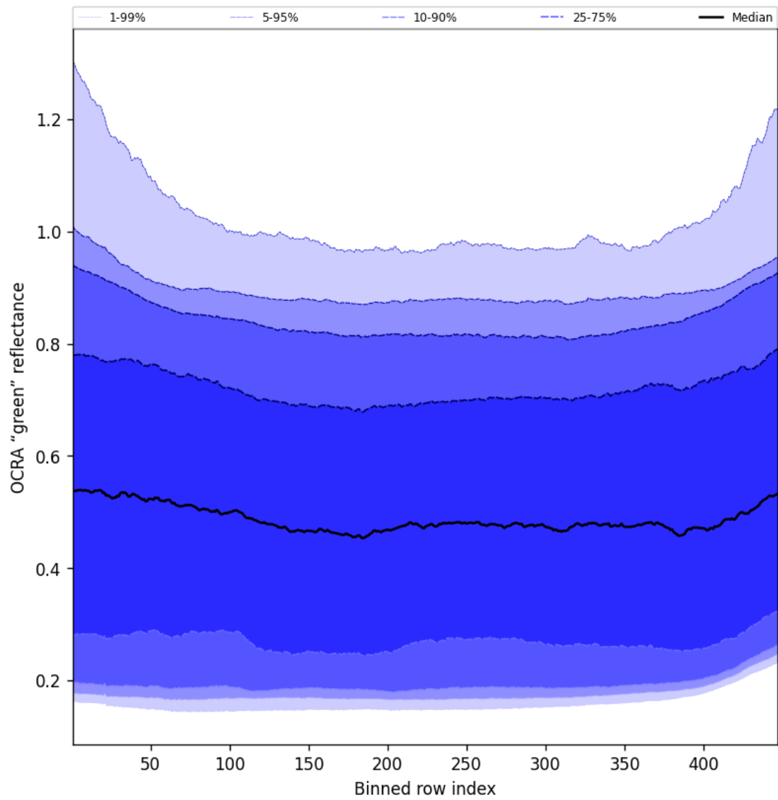
Figure 68: Along track statistics of "OCRA "green" reflectance" for 2025-04-19 to 2025-04-21
