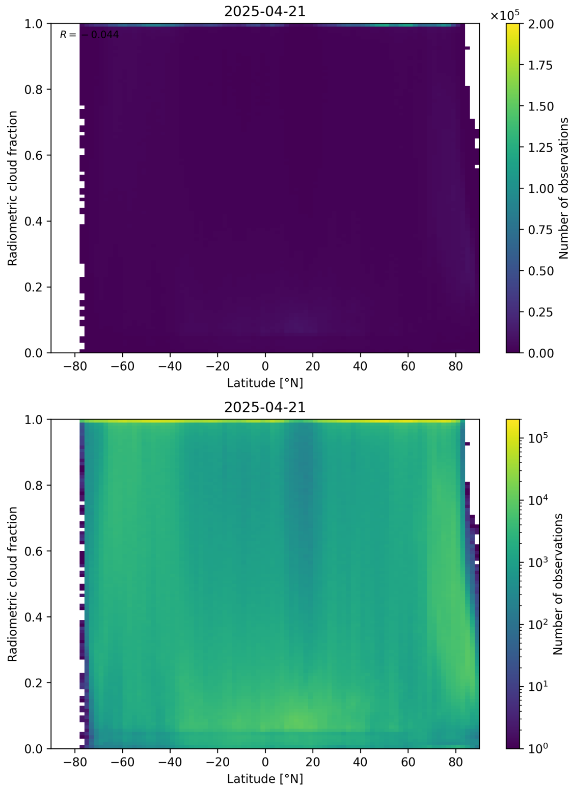
Figure 92: Scatter density plot of “Latitude” against “Radiometric cloud fraction” for 2025-04-20 to 2025-04-22.
