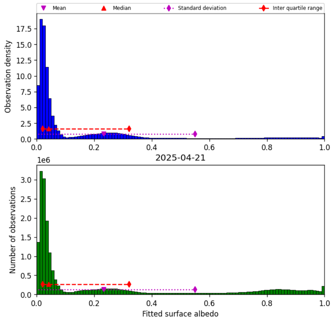
Figure 45: Histogram of “Fitted surface albedo” for 2025-04-20 to 2025-04-22
