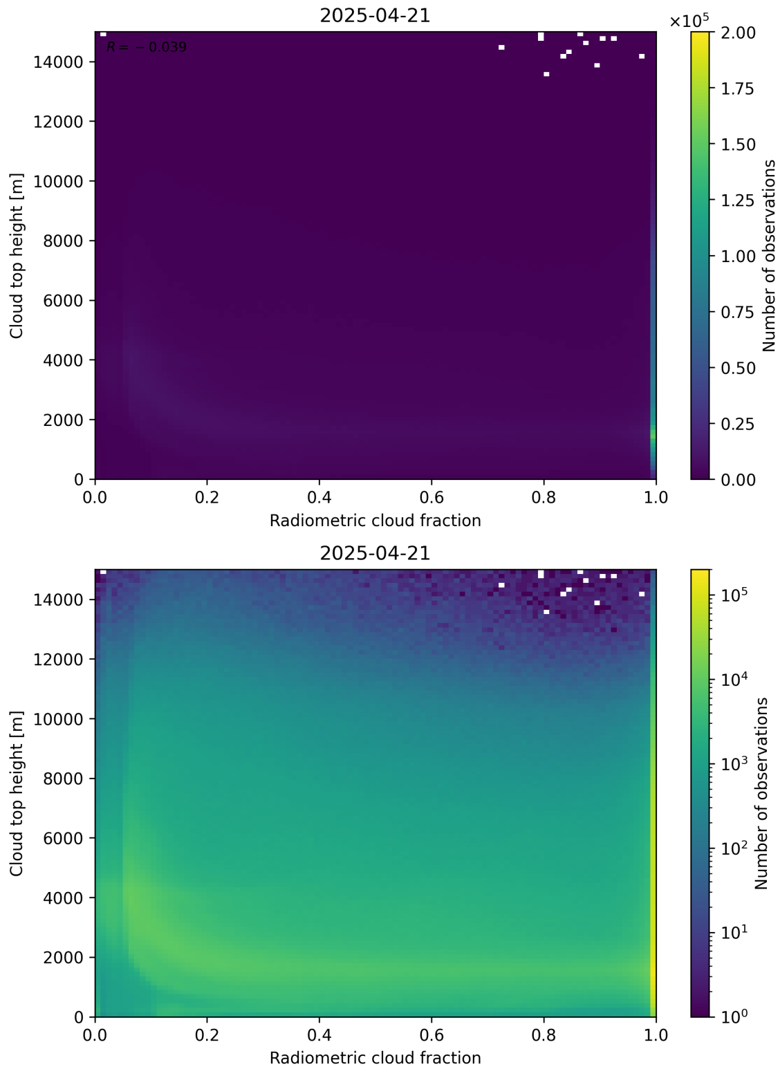
Figure 76: Scatter density plot of “Radiometric cloud fraction” against “Cloud top height” for 2025-04-20 to 2025-04-22.
