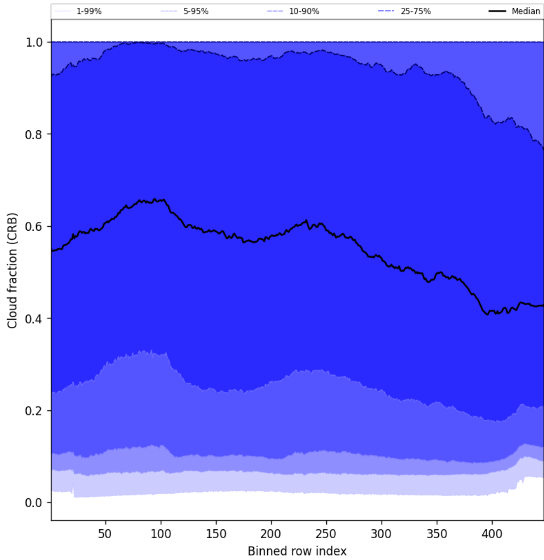
Figure 58: Along track statistics of “Cloud fraction (CRB)” for 2025-04-20 to 2025-04-22
