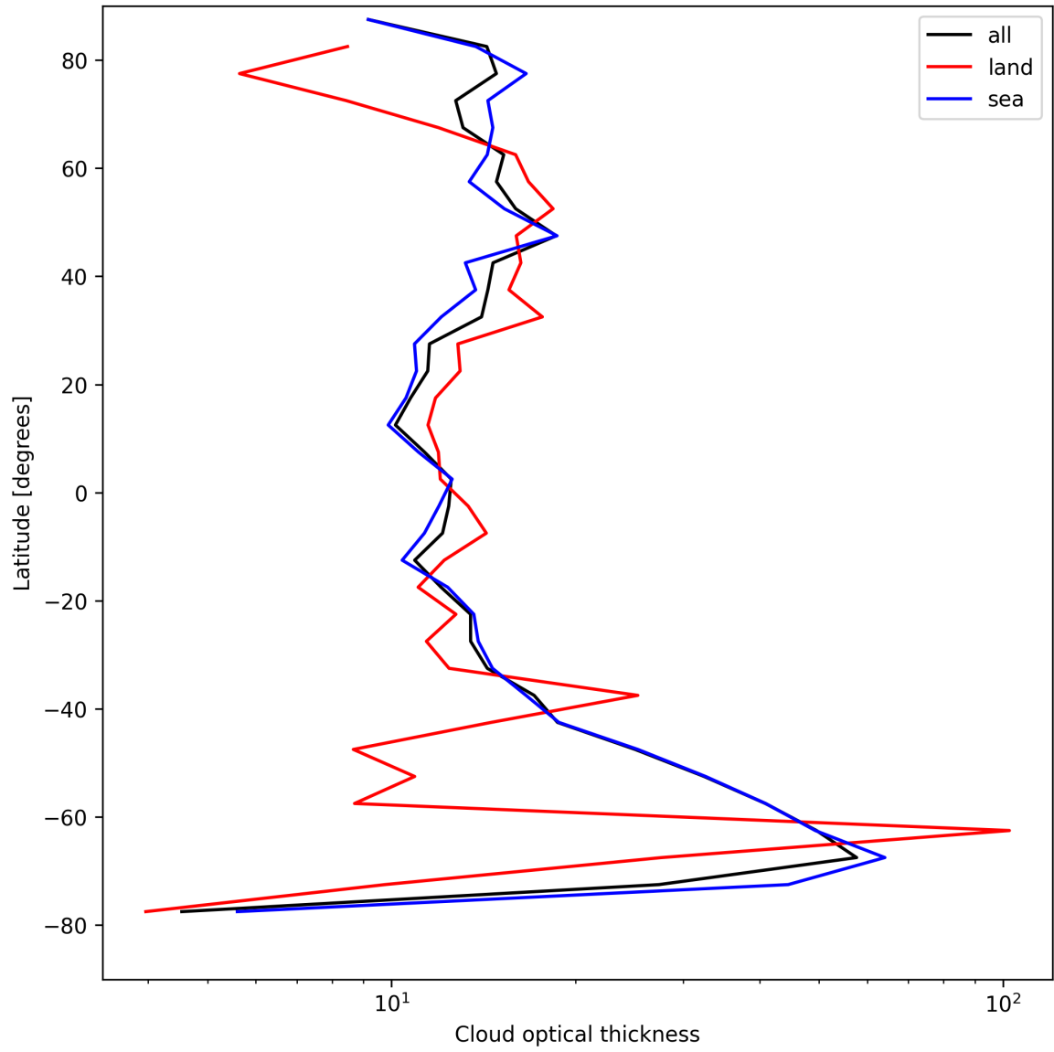
Figure 25: Zonal average of “Cloud optical thickness” for 2025-04-20 to 2025-04-22.
