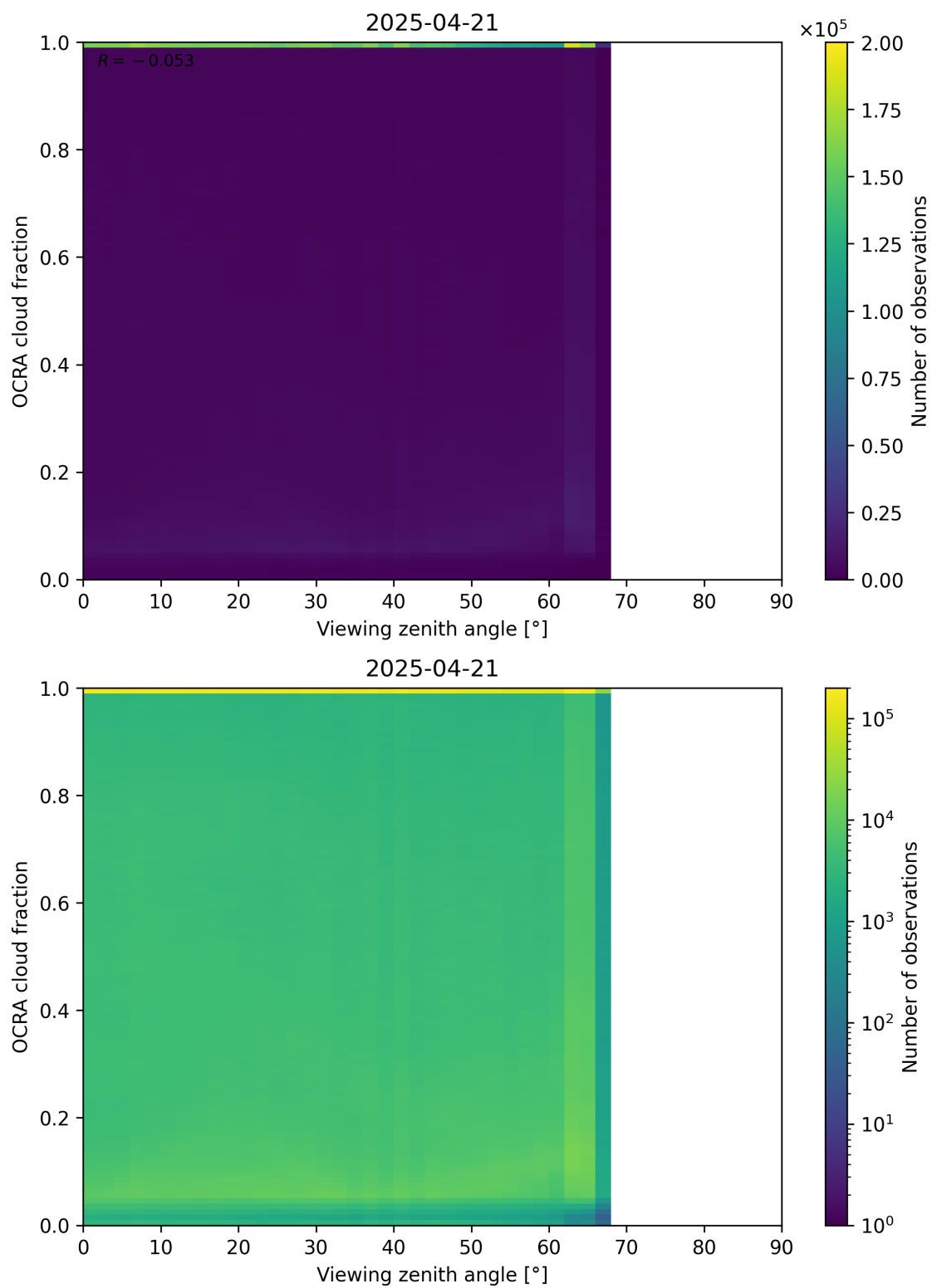
Figure 108: Scatter density plot of “Viewing zenith angle” against “OCRA cloud fraction” for 2025-04-20 to 2025-04-22.
