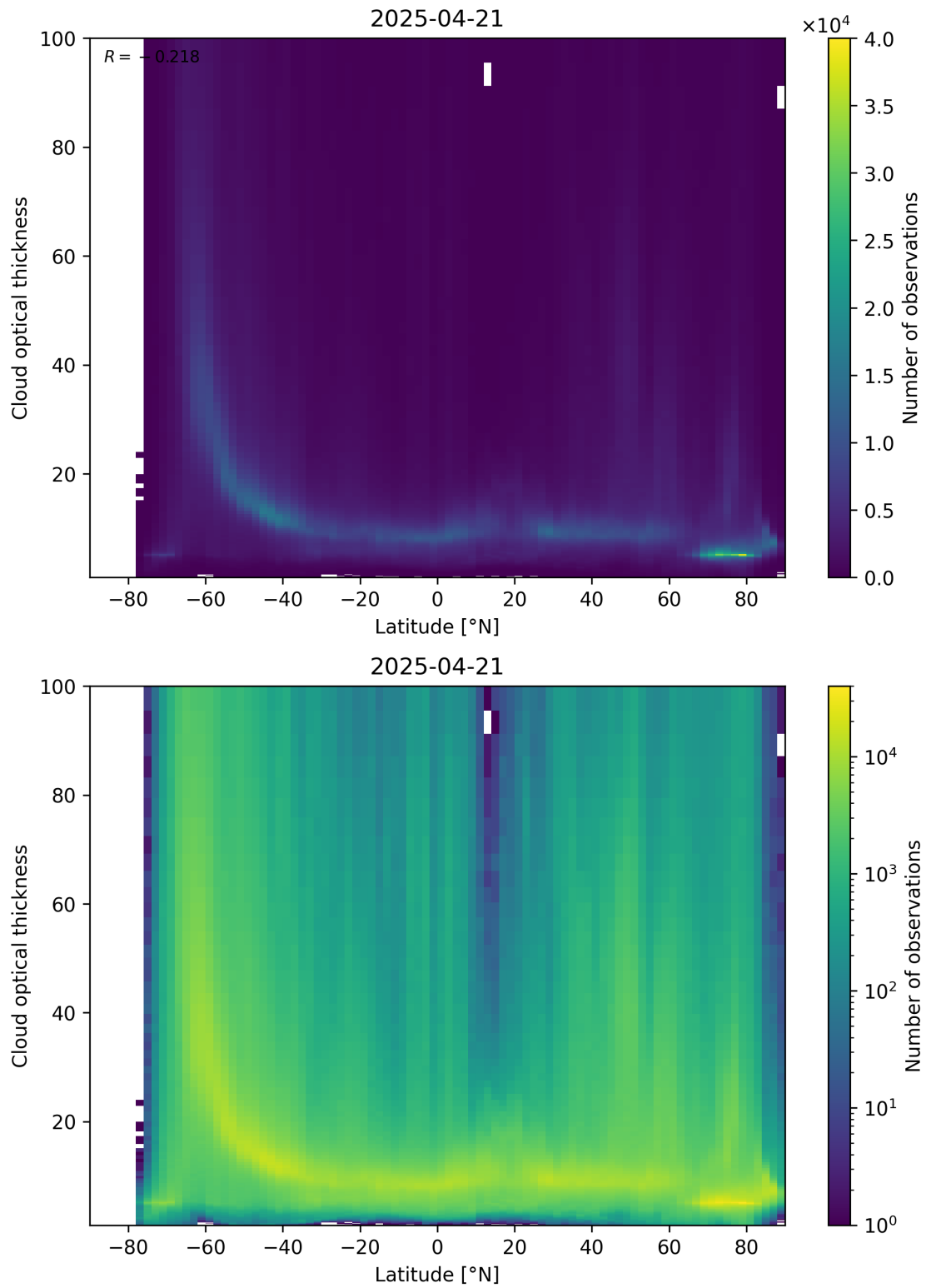
Figure 96: Scatter density plot of “Latitude” against “Cloud optical thickness” for 2025-04-20 to 2025-04-22.
