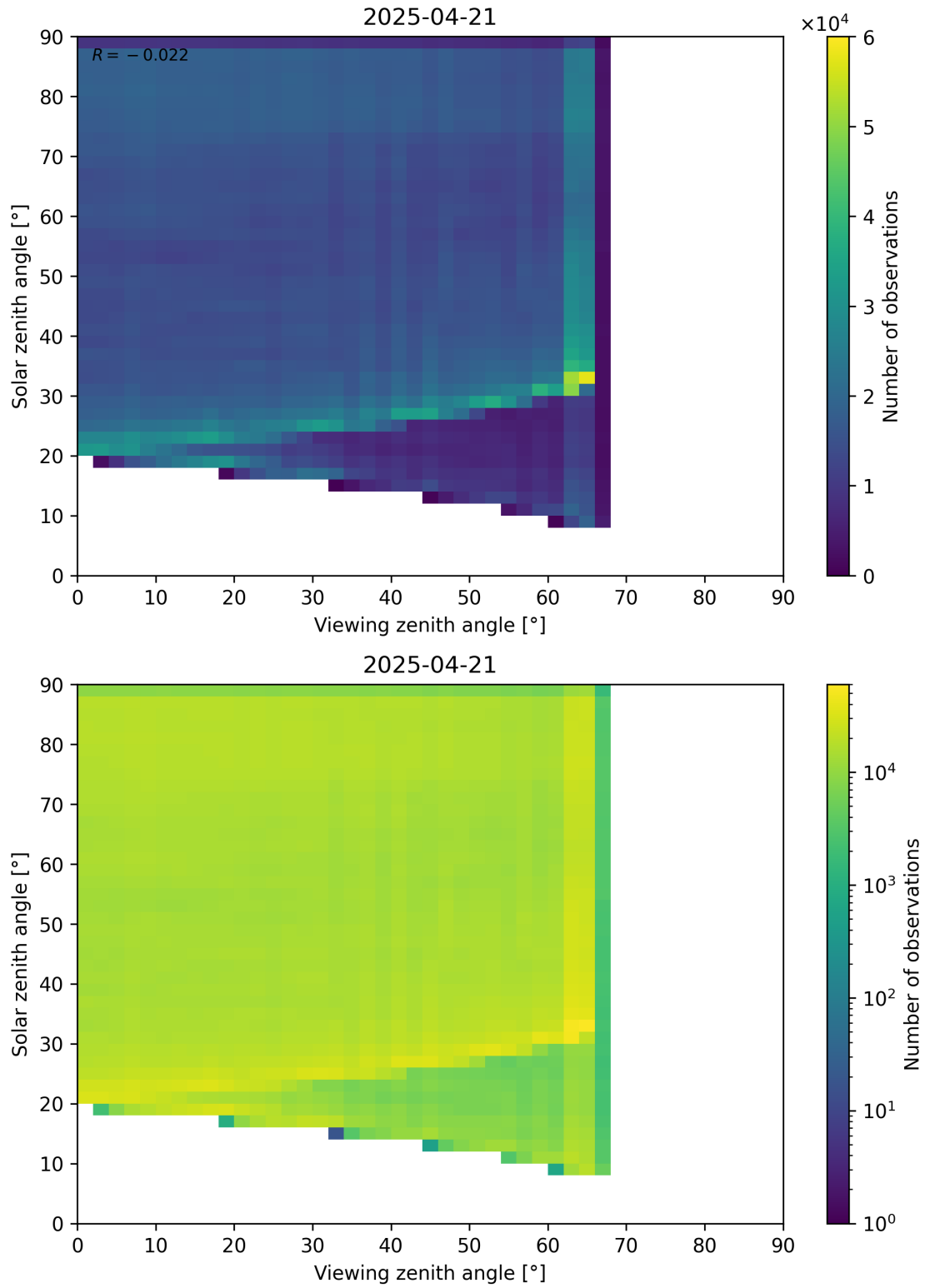
Figure 114: Scatter density plot of “Viewing zenith angle” against “Solar zenith angle” for 2025-04-20 to 2025-04-22.
