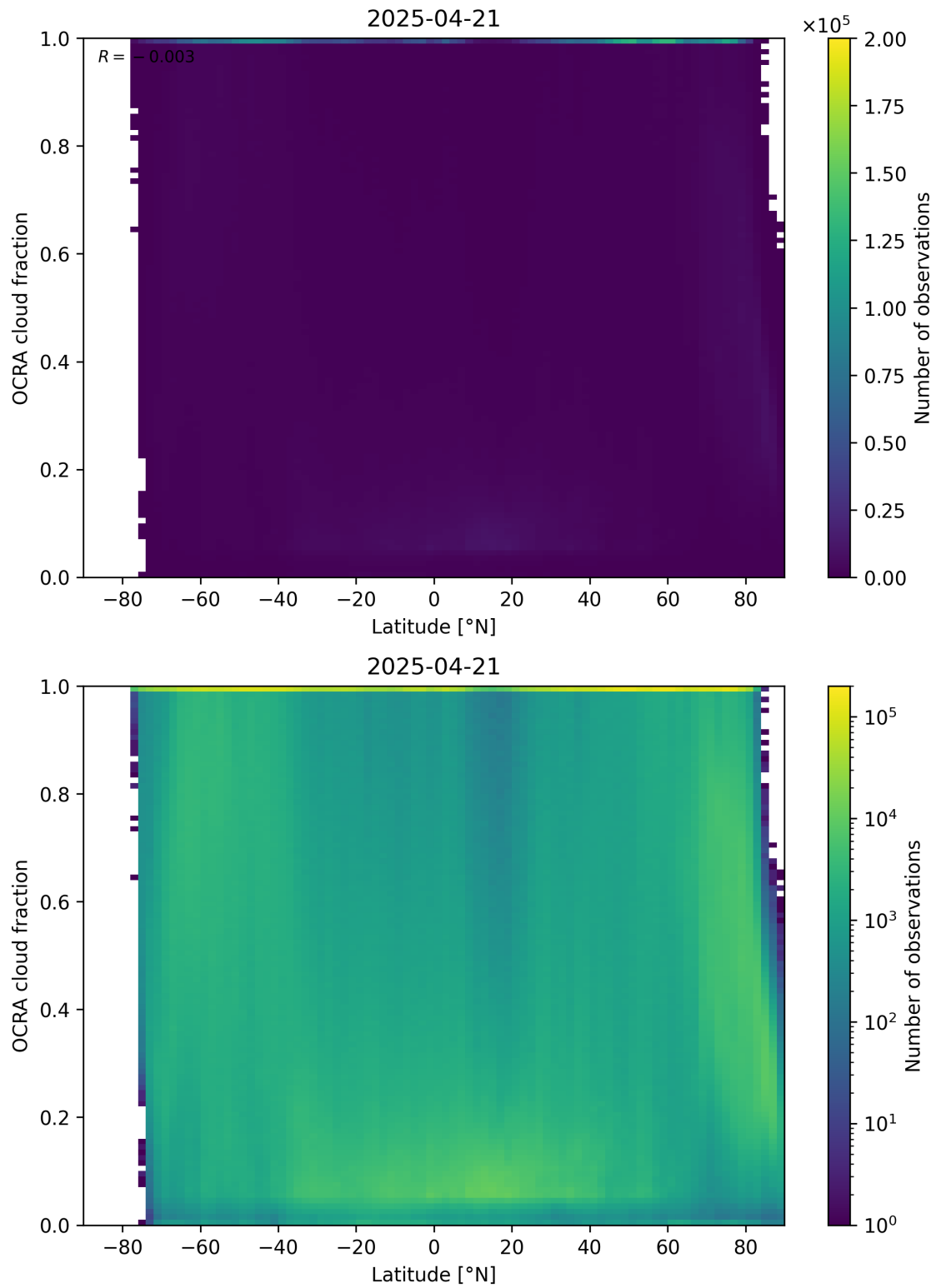
Figure 93: Scatter density plot of “Latitude” against “OCRA cloud fraction” for 2025-04-20 to 2025-04-22.
