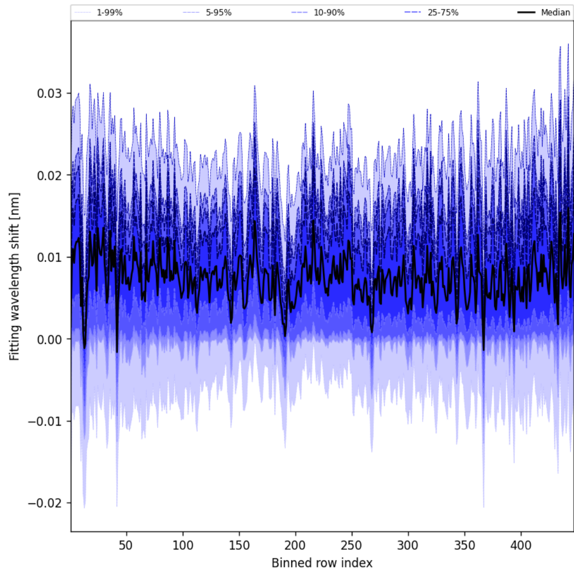
Figure 65: Along track statistics of “Fitting wavelength shift” for 2025-04-20 to 2025-04-22
