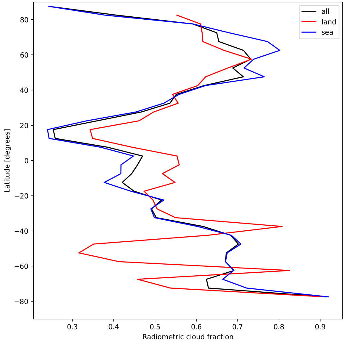
Figure 23: Zonal average of “Radiometric cloud fraction” for 2025-04-20 to 2025-04-22.
