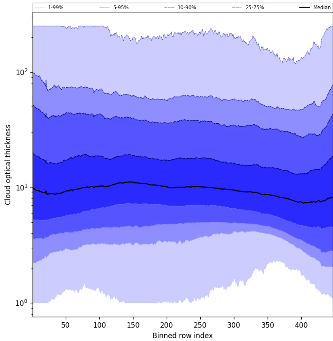
Figure 57: Along track statistics of “Cloud optical thickness” for 2025-04-20 to 2025-04-22
