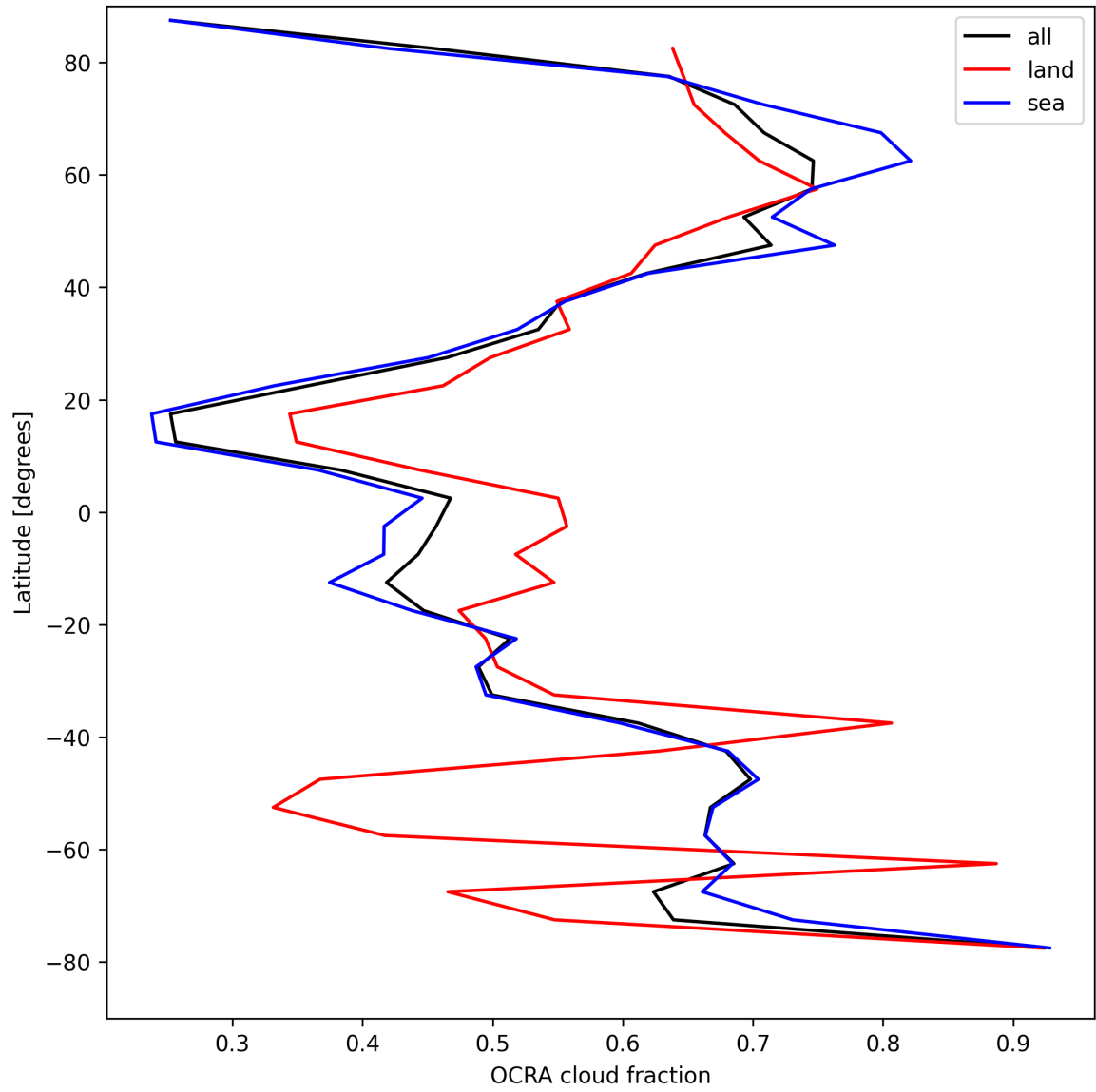
Figure 34: Zonal average of “OCRA cloud fraction” for 2025-04-20 to 2025-04-22.
