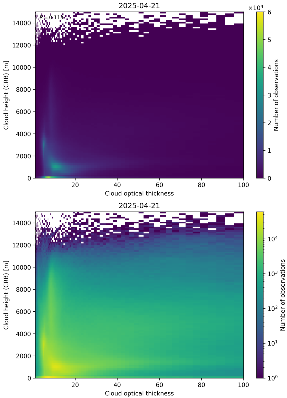
Figure 85: Scatter density plot of “Cloud optical thickness” against “Cloud height (CRB)” for 2025-04-20 to 2025-04-22.
