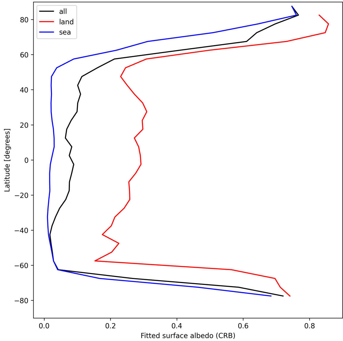
Figure 30: Zonal average of “Fitted surface albedo (CRB)” for 2025-04-20 to 2025-04-22.
