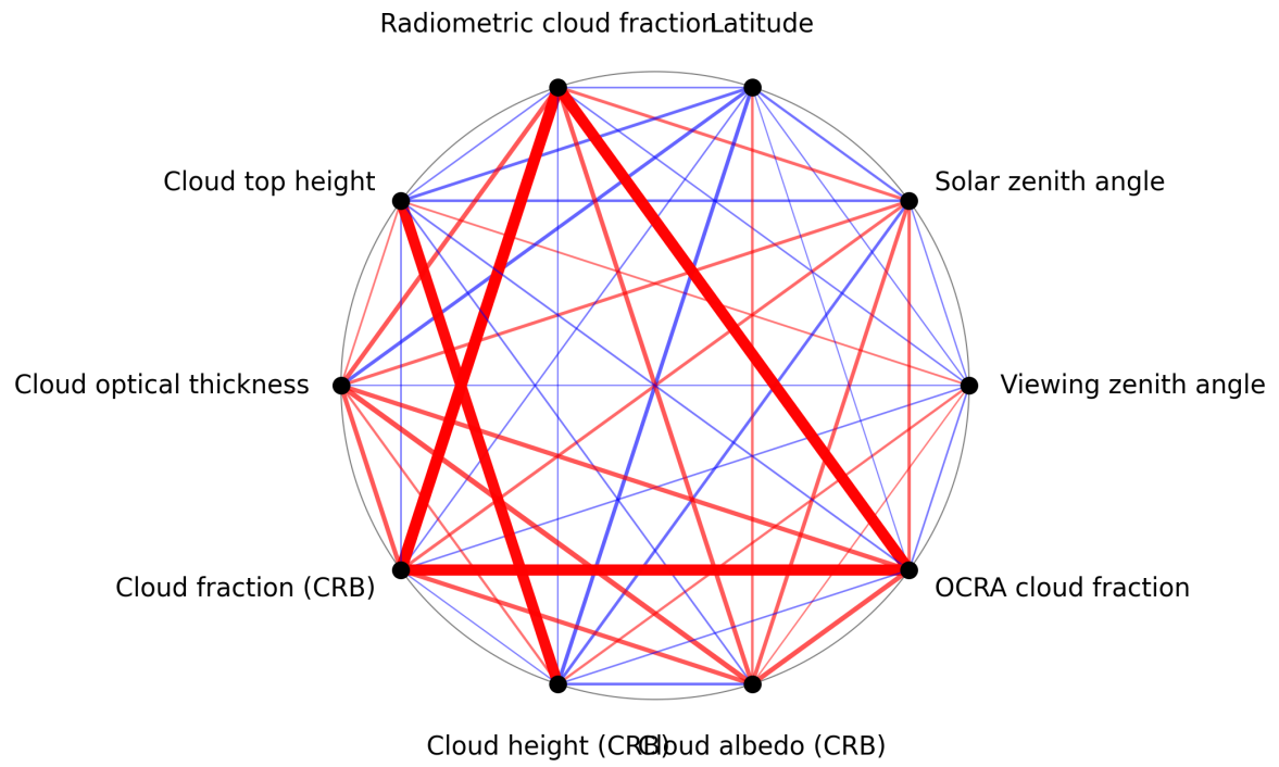
Figure 1: Map of correlation graph for 2025-04-20 to 2025-04-22.
