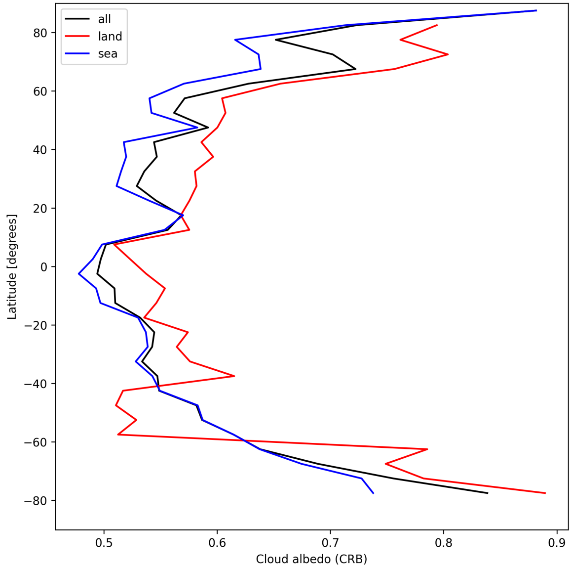
Figure 28: Zonal average of “Cloud albedo (CRB)” for 2025-04-20 to 2025-04-22.
