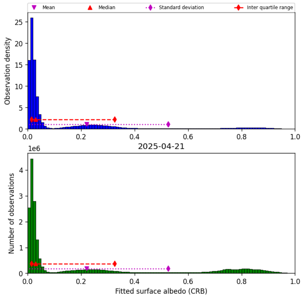
Figure 46: Histogram of “Fitted surface albedo (CRB)” for 2025-04-20 to 2025-04-22
