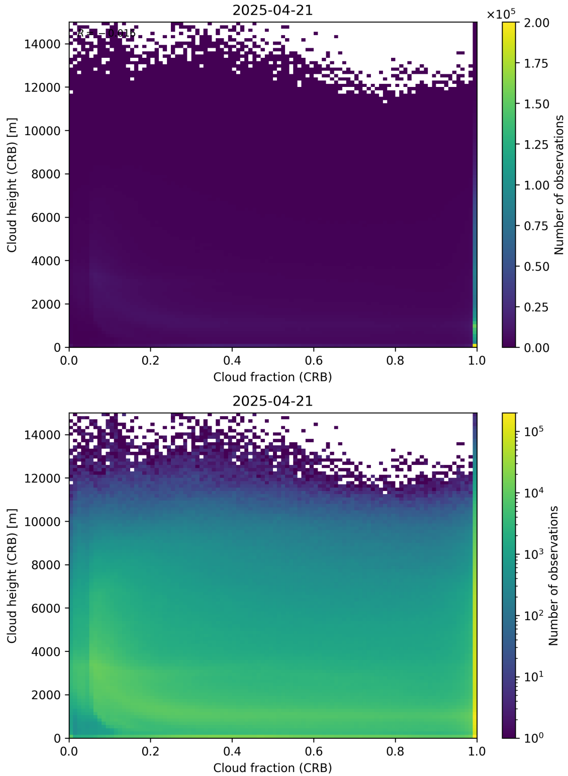
Figure 79: Scatter density plot of “Cloud fraction (CRB)” against “Cloud height (CRB)” for 2025-04-20 to 2025-04-22.
