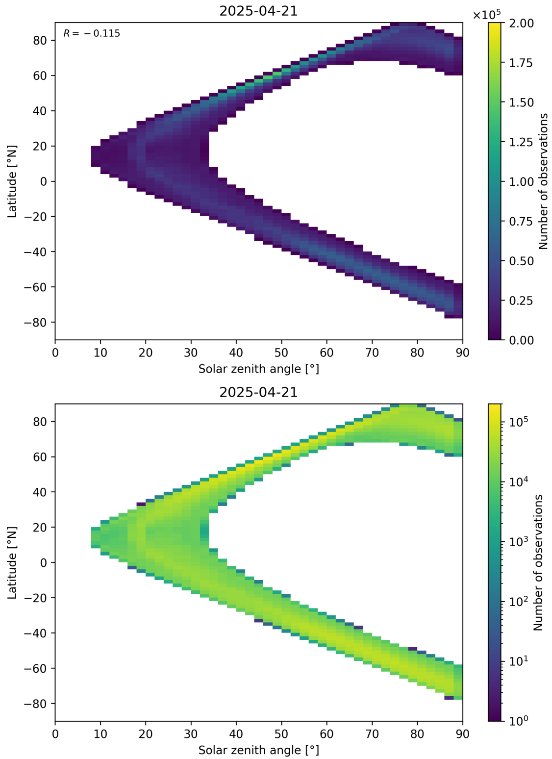
Figure 105: Scatter density plot of “Solar zenith angle” against “Latitude” for 2025-04-20 to 2025-04-22.
