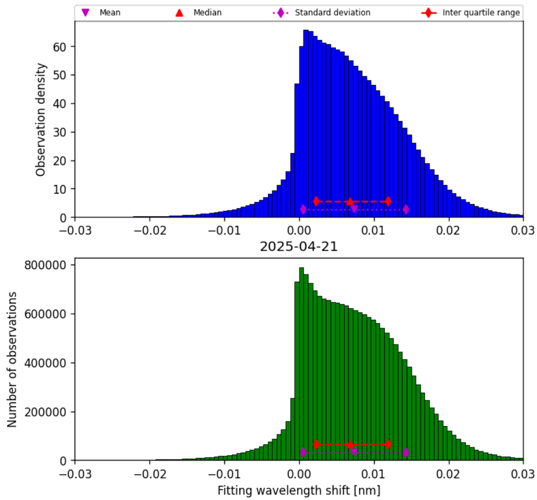
Figure 49: Histogram of “Fitting wavelength shift” for 2025-04-20 to 2025-04-22
