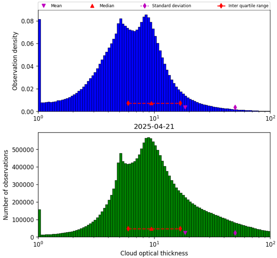
Figure 41: Histogram of “Cloud optical thickness” for 2025-04-20 to 2025-04-22
