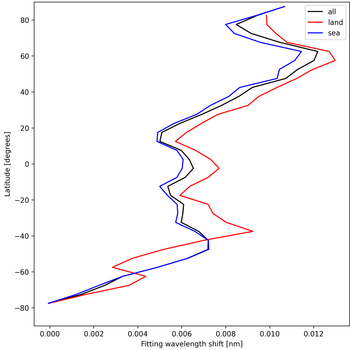
Figure 33: Zonal average of “Fitting wavelength shift” for 2025-04-20 to 2025-04-22.
