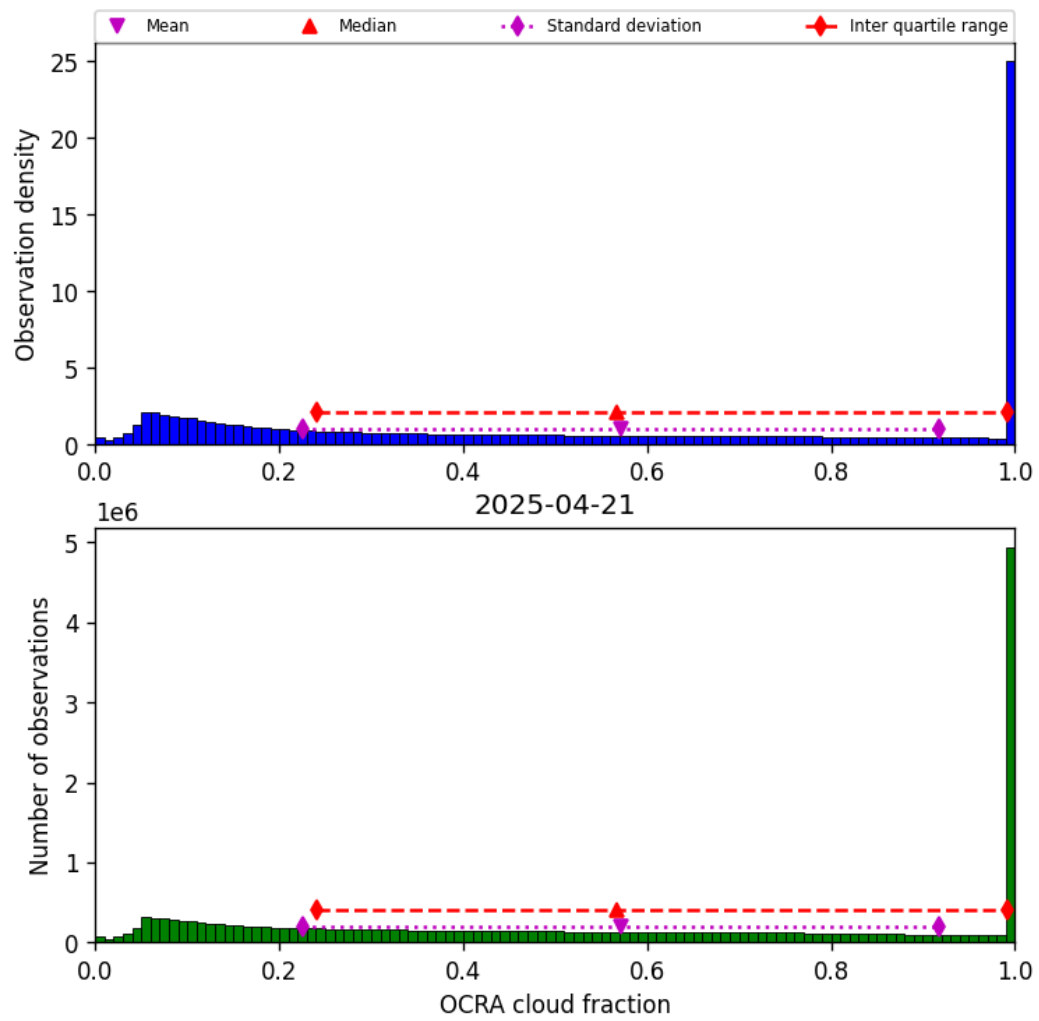
Figure 50: Histogram of “OCRA cloud fraction” for 2025-04-20 to 2025-04-22
