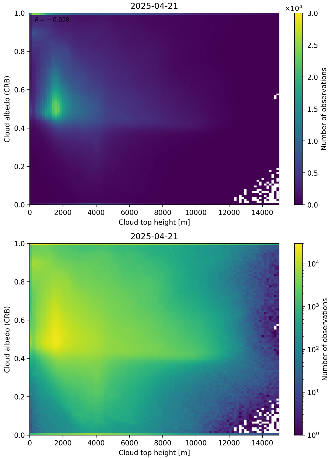
Figure 86: Scatter density plot of “Cloud top height” against “Cloud albedo (CRB)” for 2025-04-20 to 2025-04-22.
