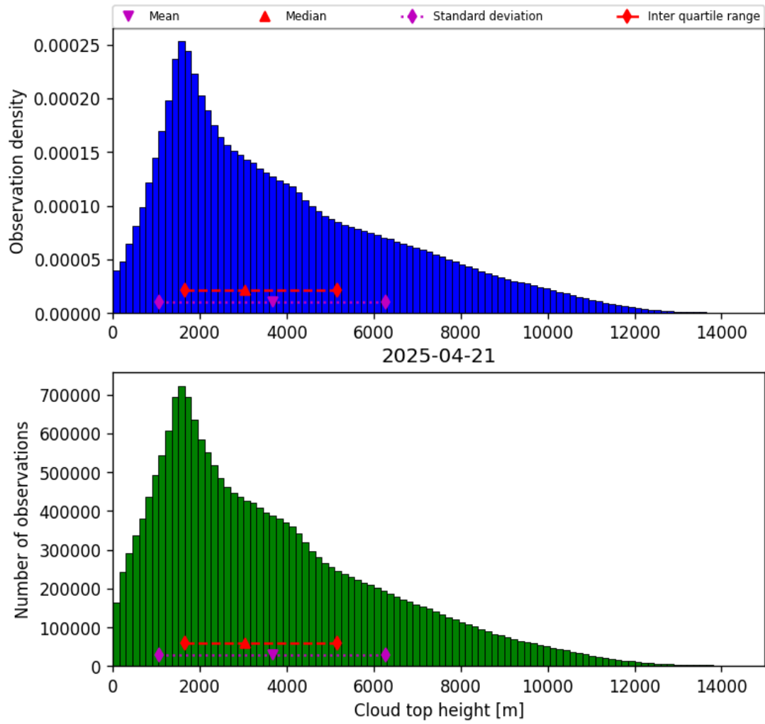
Figure 40: Histogram of “Cloud top height” for 2025-04-20 to 2025-04-22
