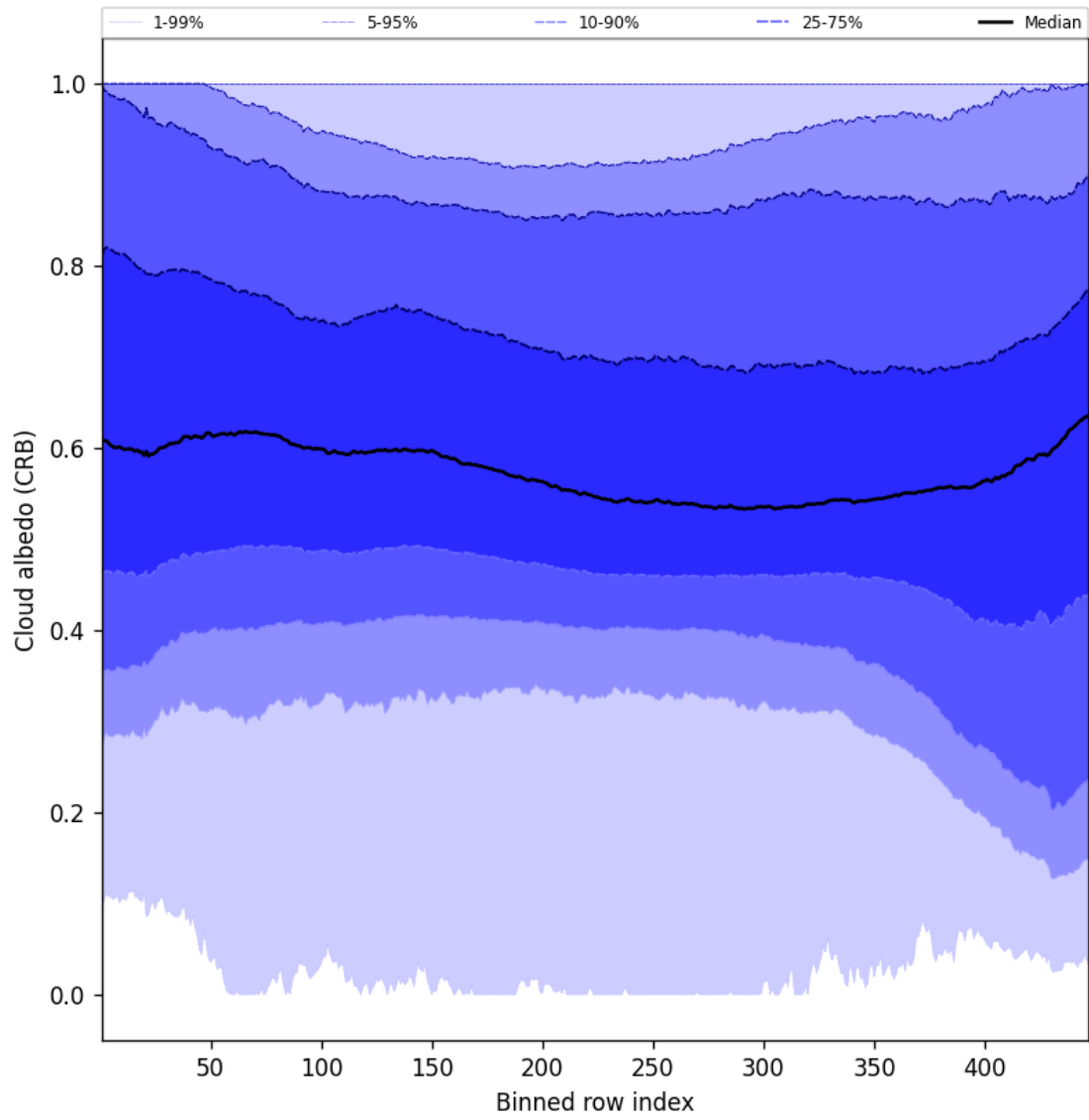
Figure 60: Along track statistics of “Cloud albedo (CRB)” for 2025-04-20 to 2025-04-22
