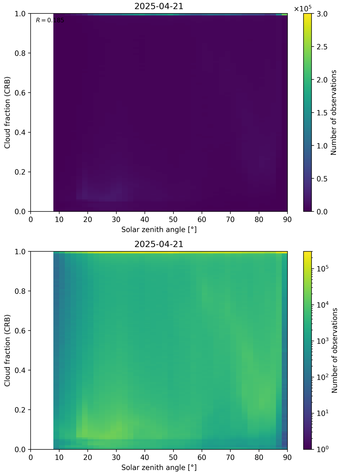
Figure 101: Scatter density plot of “Solar zenith angle” against “Cloud fraction (CRB)” for 2025-04-20 to 2025-04-22.
