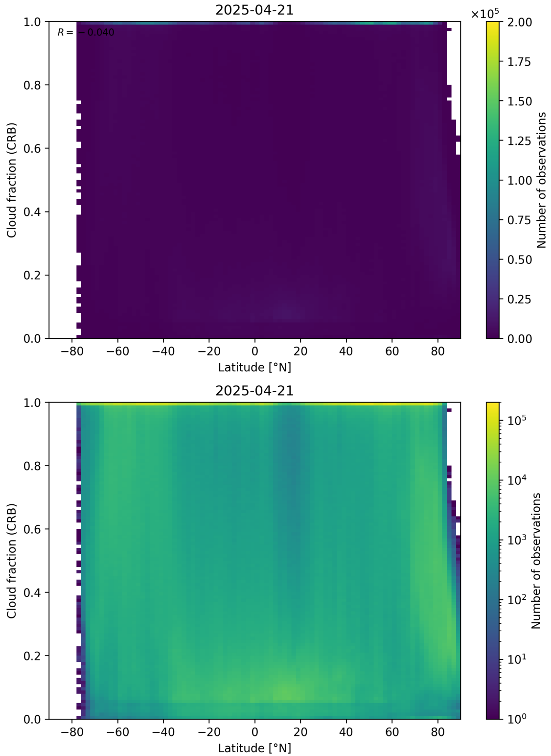
Figure 94: Scatter density plot of “Latitude” against “Cloud fraction (CRB)” for 2025-04-20 to 2025-04-22.
