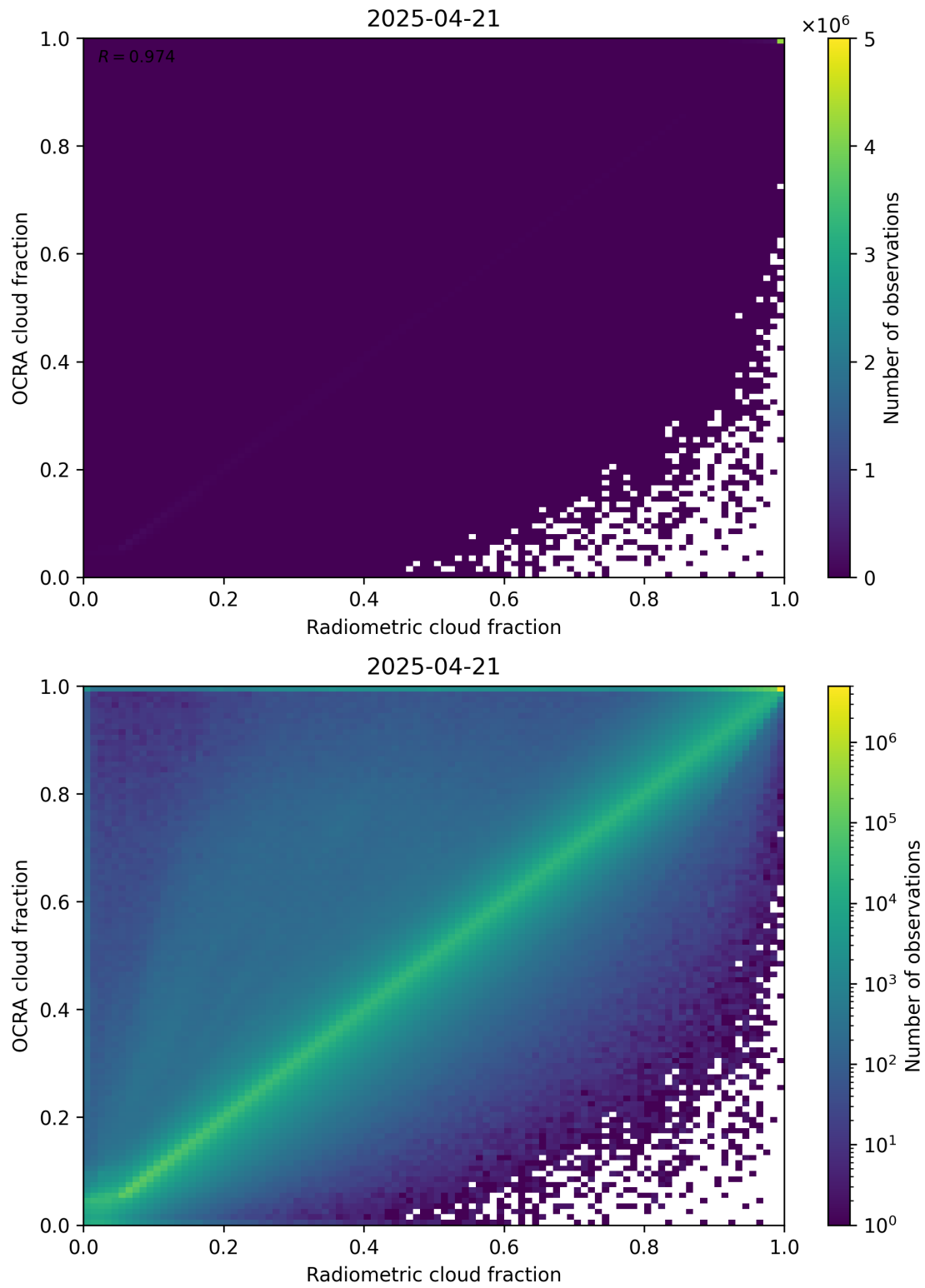
Figure 72: Scatter density plot of “Radiometric cloud fraction” against “OCRA cloud fraction” for 2025-04-20 to 2025-04-22.
