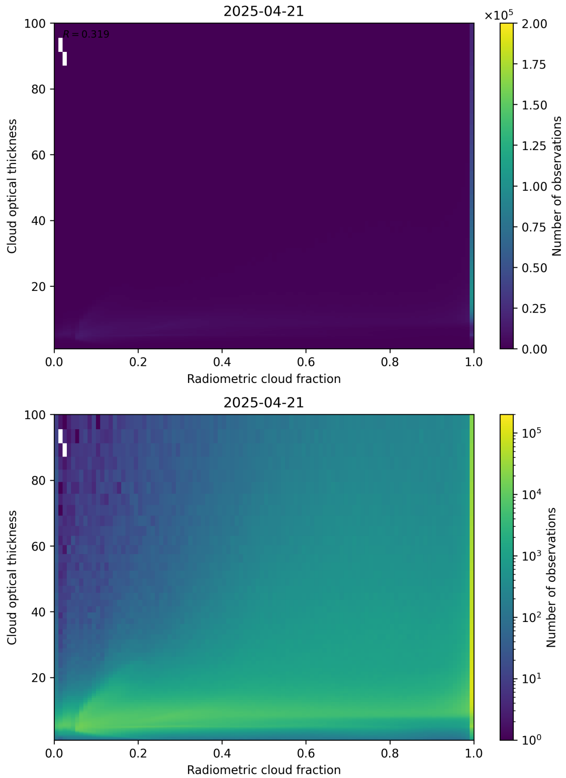
Figure 75: Scatter density plot of “Radiometric cloud fraction” against “Cloud optical thickness” for 2025-04-20 to 2025-04-22.
