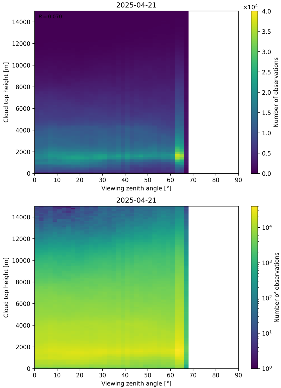
Figure 112: Scatter density plot of “Viewing zenith angle” against “Cloud top height” for 2025-04-20 to 2025-04-22.
