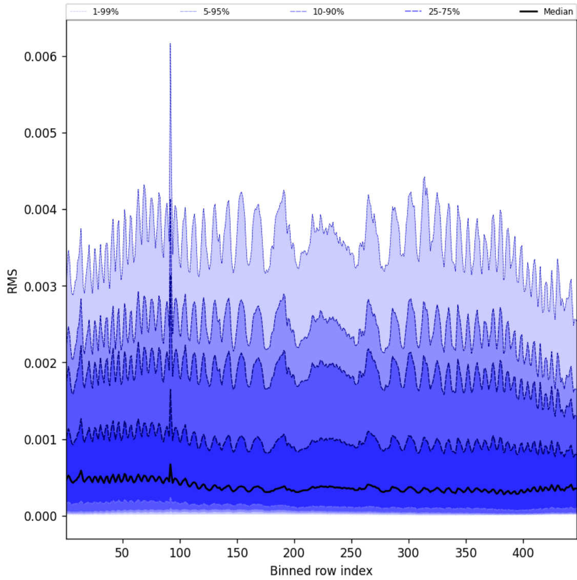
Figure 63: Along track statistics of “RMS” for 2025-04-20 to 2025-04-22
