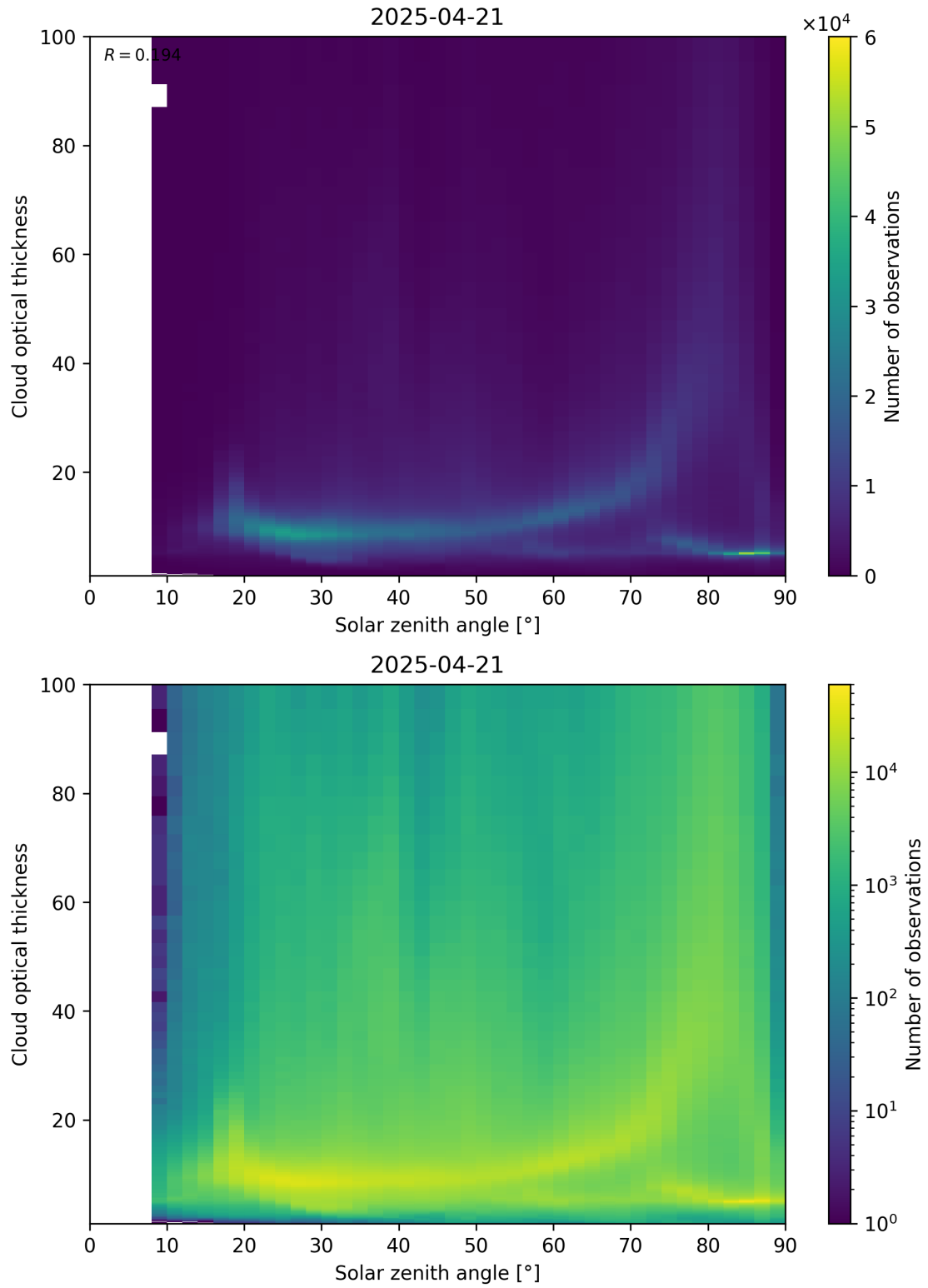
Figure 103: Scatter density plot of “Solar zenith angle” against “Cloud optical thickness” for 2025-04-20 to 2025-04-22.
