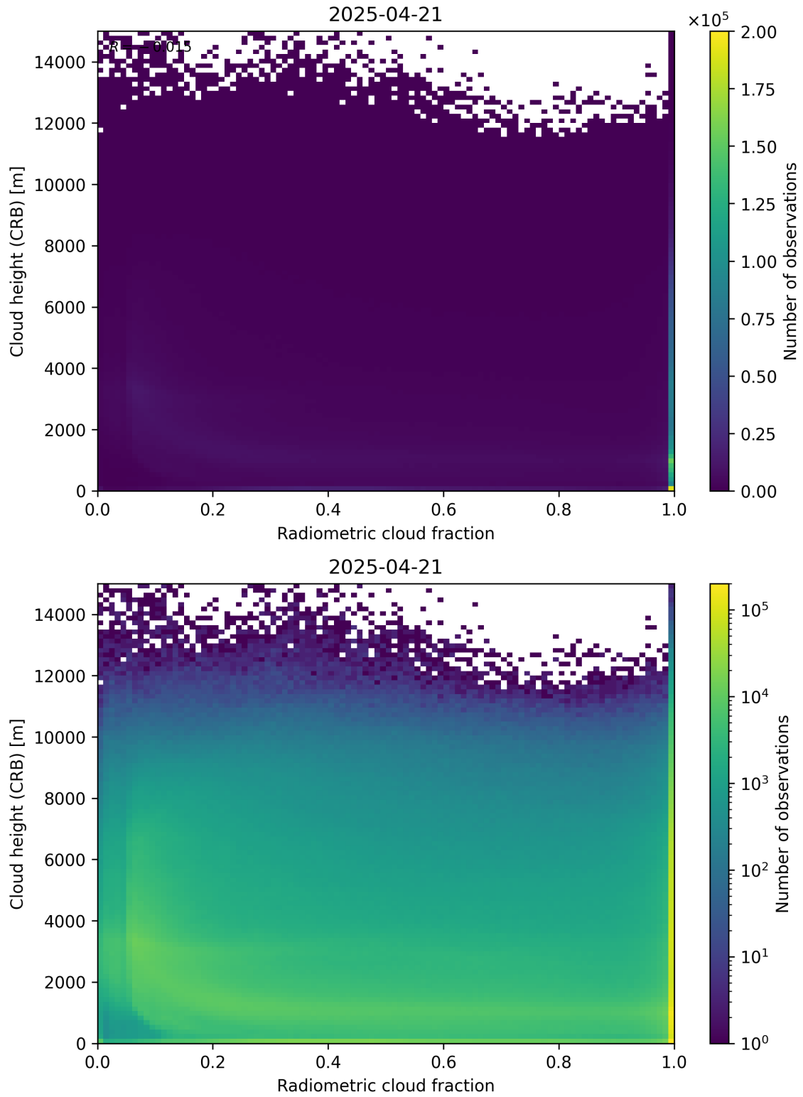
Figure 74: Scatter density plot of “Radiometric cloud fraction” against “Cloud height (CRB)” for 2025-04-20 to 2025-04-22.
