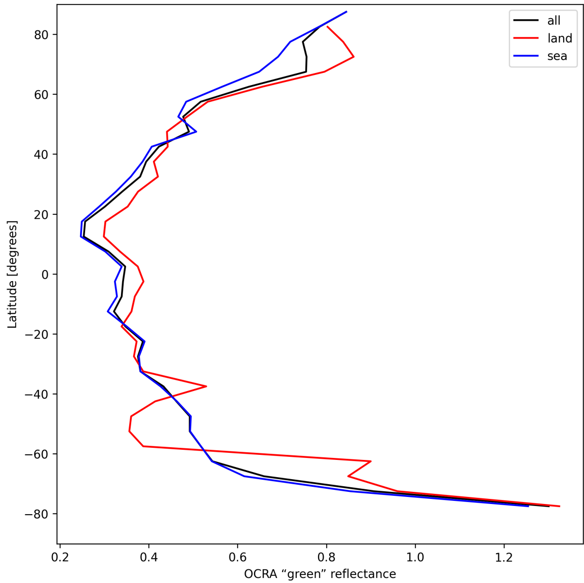
Figure 36: Zonal average of “OCRA “green” reflectance” for 2025-04-20 to 2025-04-22.
