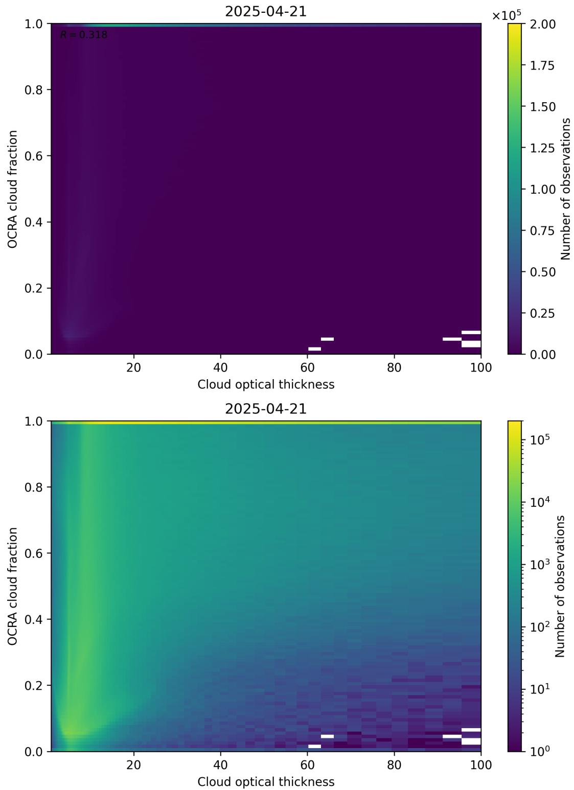
Figure 83: Scatter density plot of “Cloud optical thickness” against “OCRA cloud fraction” for 2025-04-20 to 2025-04-22.
