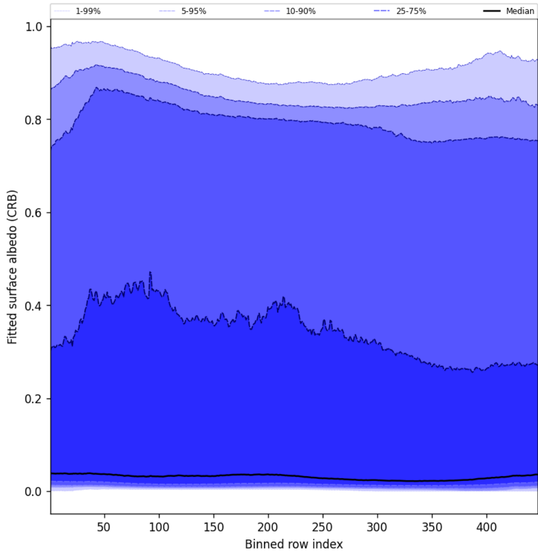
Figure 62: Along track statistics of “Fitted surface albedo (CRB)” for 2025-04-20 to 2025-04-22
