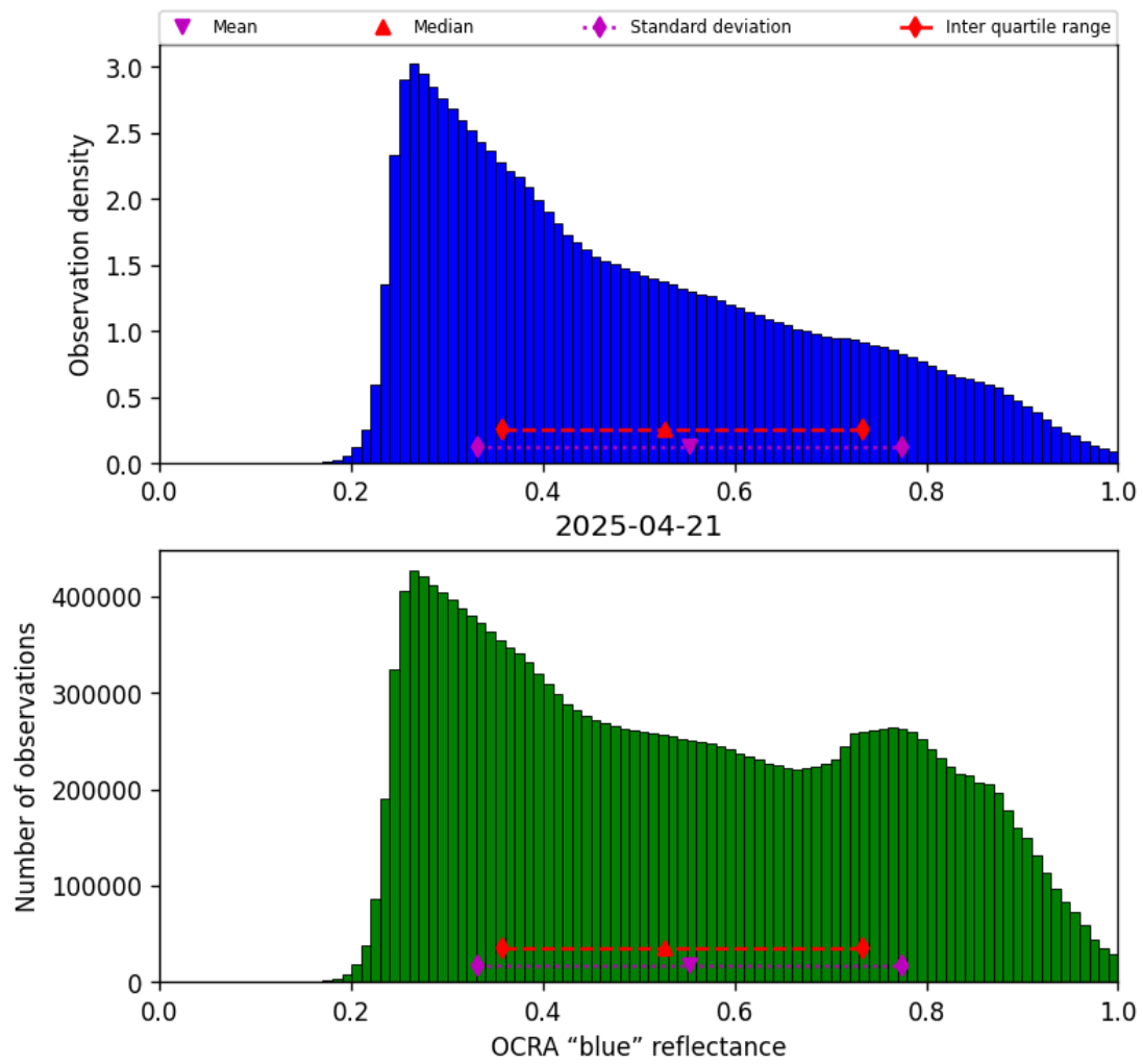
Figure 51: Histogram of “OCRA “blue” reflectance” for 2025-04-20 to 2025-04-22
