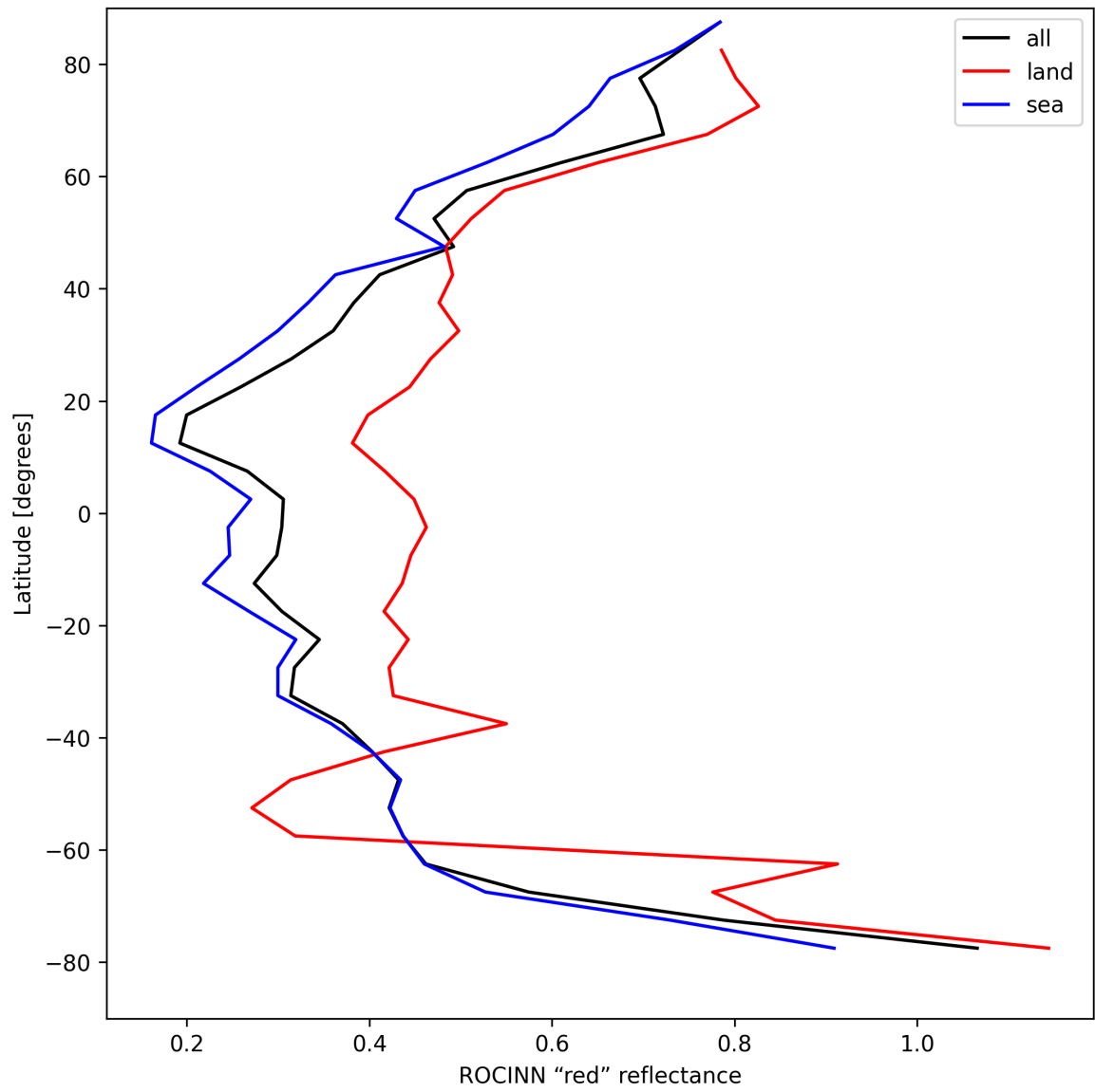
Figure 37: Zonal average of "ROCINN "red" reflectance" for 2025-04-20 to 2025-04-22.
