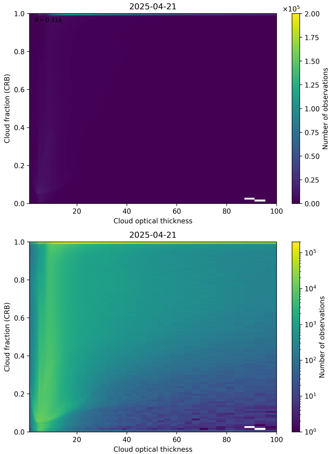
Figure 84: Scatter density plot of “Cloud optical thickness” against “Cloud fraction (CRB)” for 2025-04-20 to 2025-04-22.
