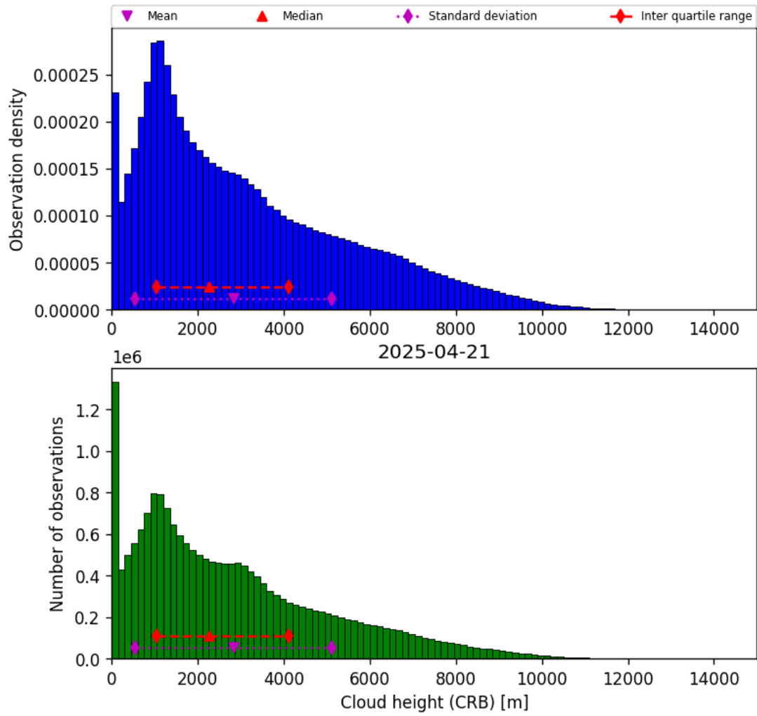
Figure 43: Histogram of “Cloud height (CRB)” for 2025-04-20 to 2025-04-22
