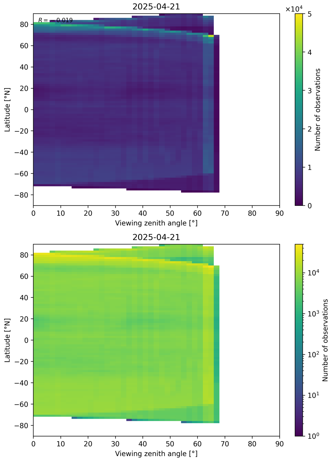
Figure 113: Scatter density plot of “Viewing zenith angle” against “Latitude” for 2025-04-20 to 2025-04-22.
