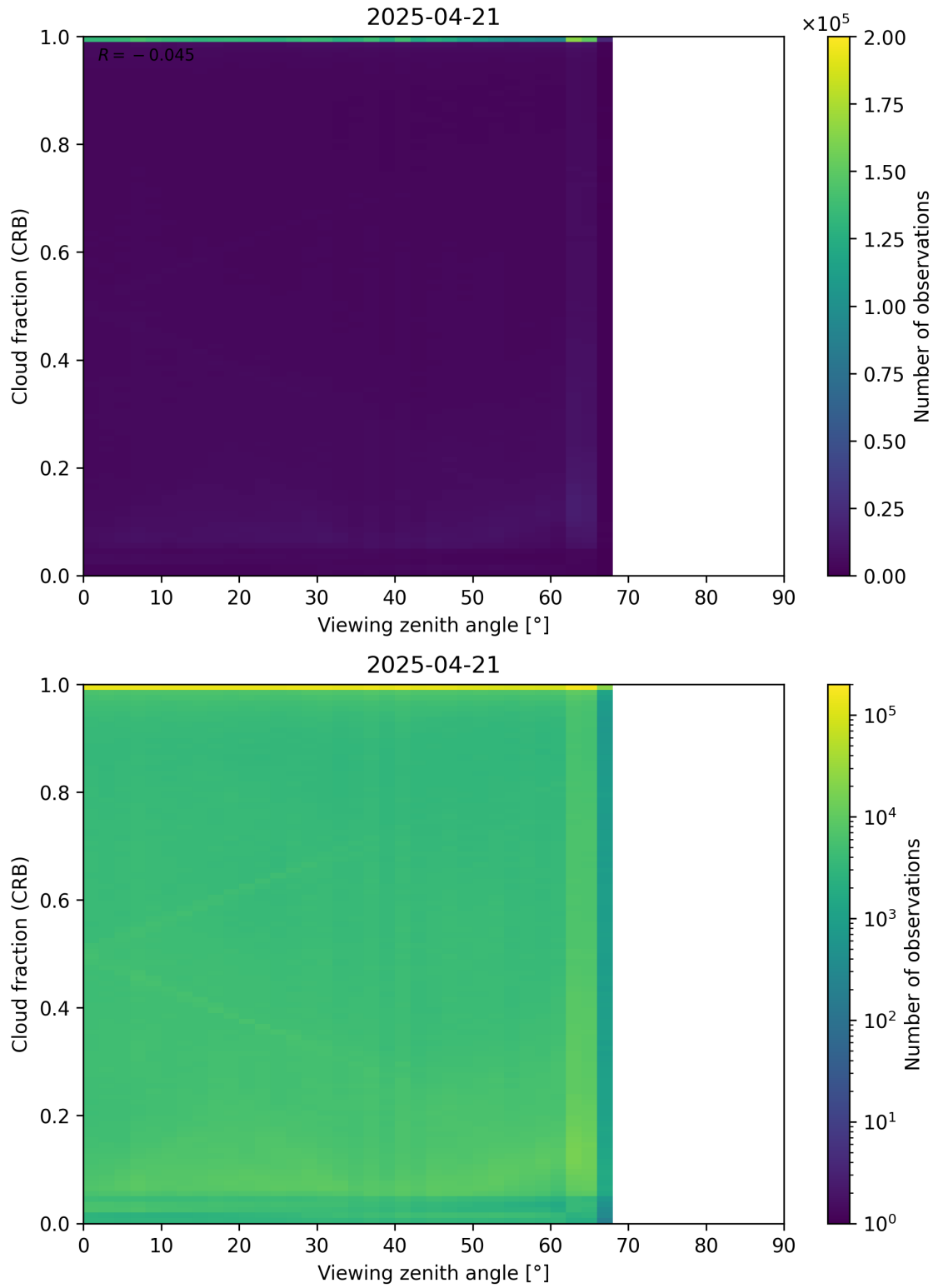
Figure 109: Scatter density plot of “Viewing zenith angle” against “Cloud fraction (CRB)” for 2025-04-20 to 2025-04-22.
