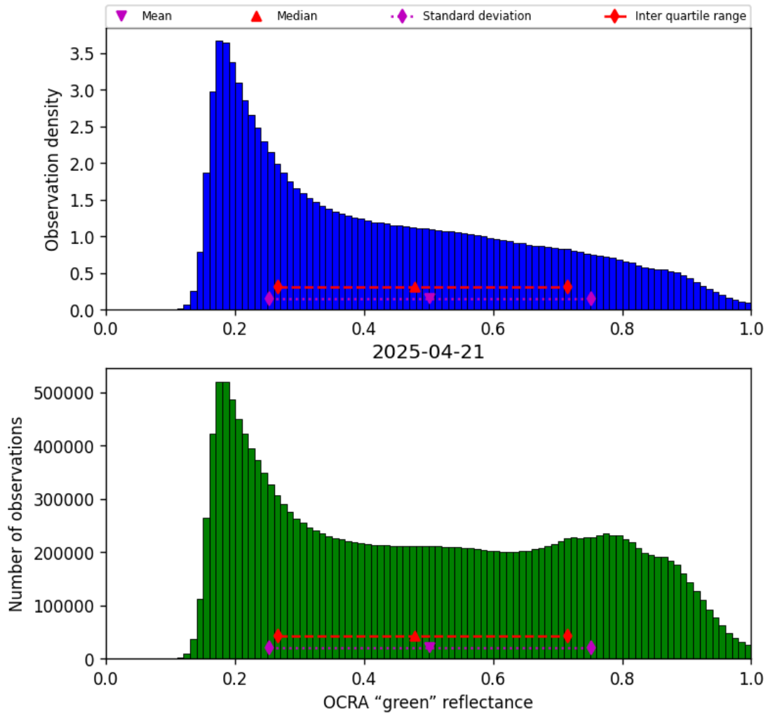
Figure 52: Histogram of “OCRA “green” reflectance” for 2025-04-20 to 2025-04-22
