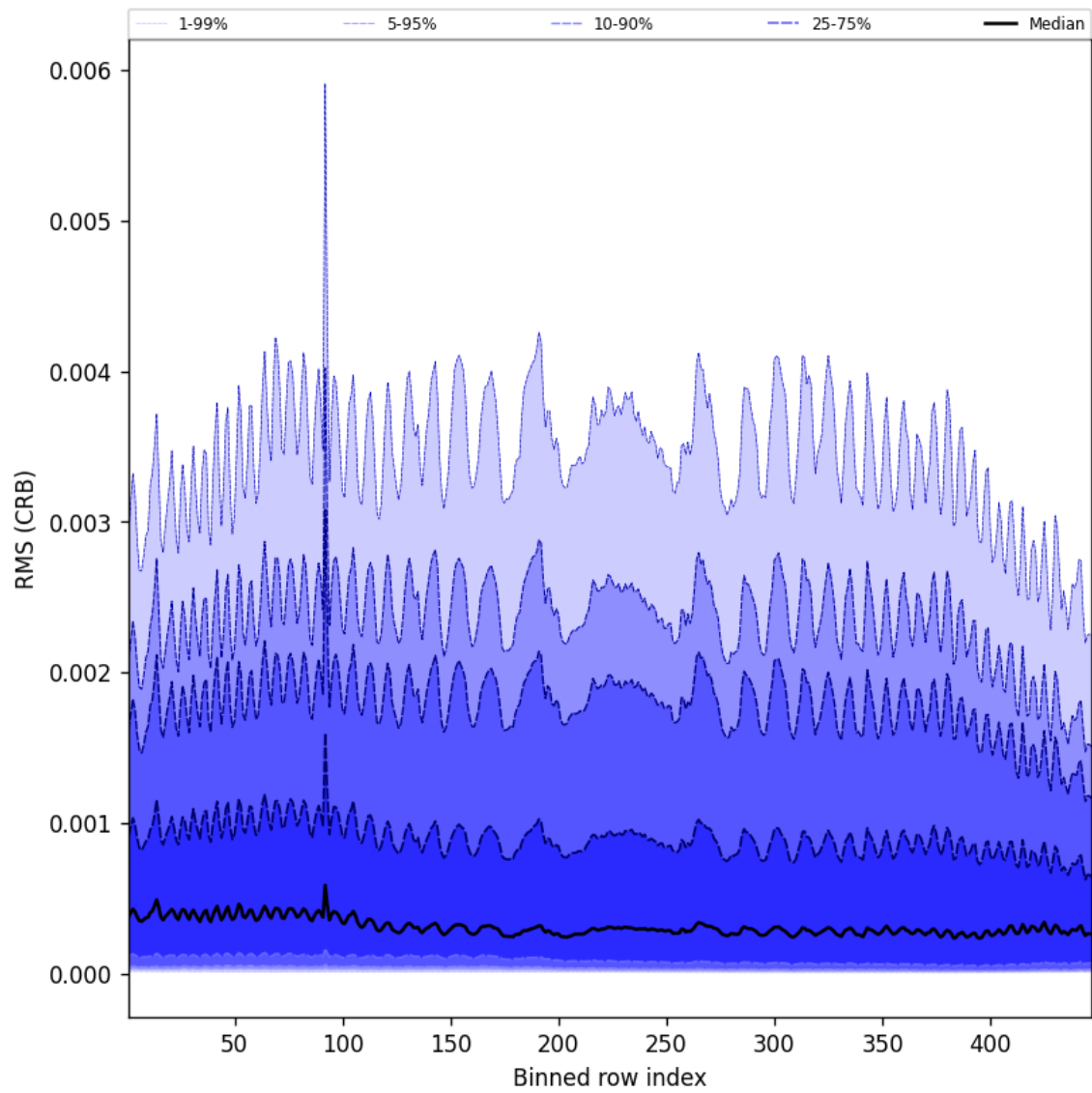
Figure 64: Along track statistics of “RMS (CRB)” for 2025-04-20 to 2025-04-22
