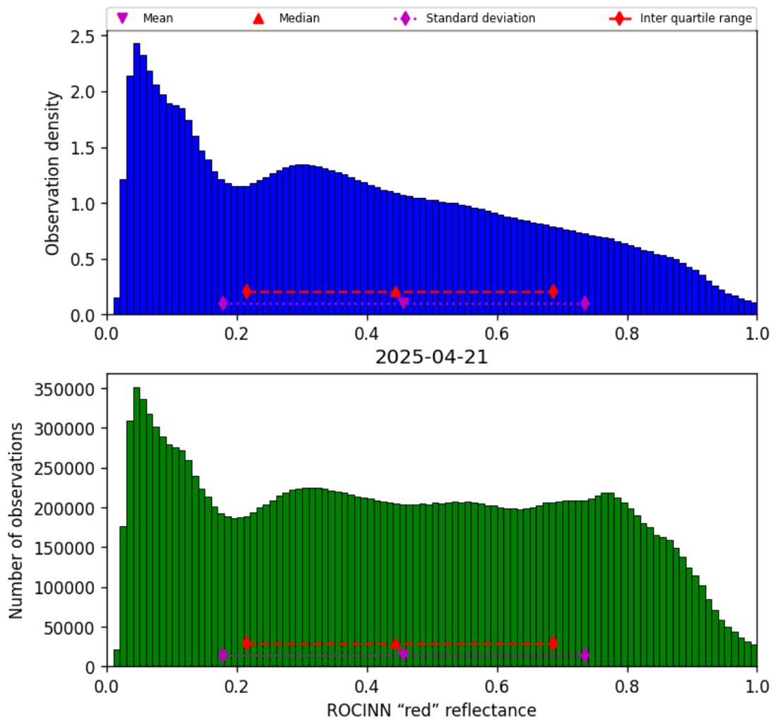
Figure 53: Histogram of “ROCINN “red” reflectance” for 2025-04-20 to 2025-04-22
