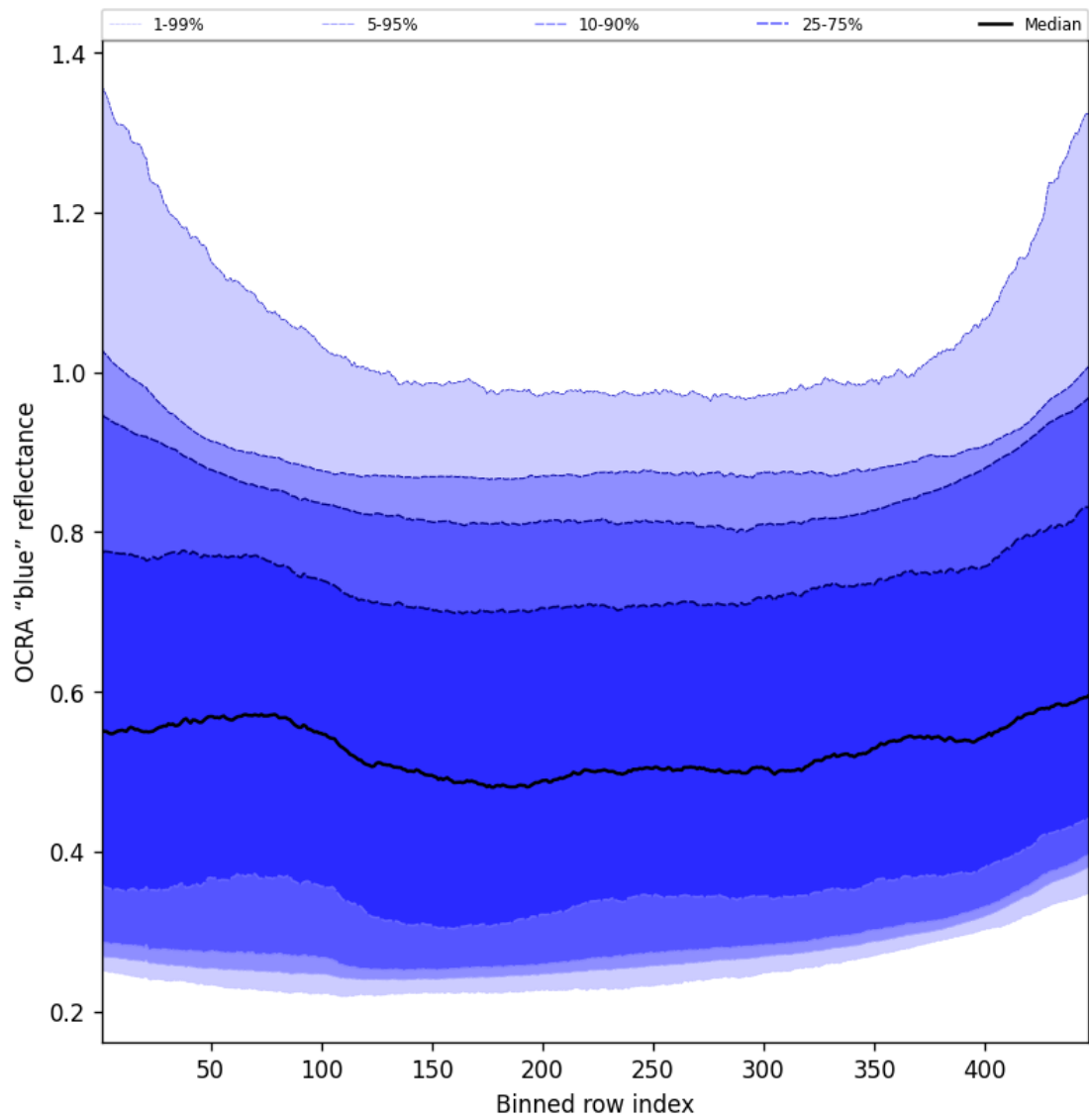
Figure 67: Along track statistics of “OCRA “blue” reflectance” for 2025-04-20 to 2025-04-22
