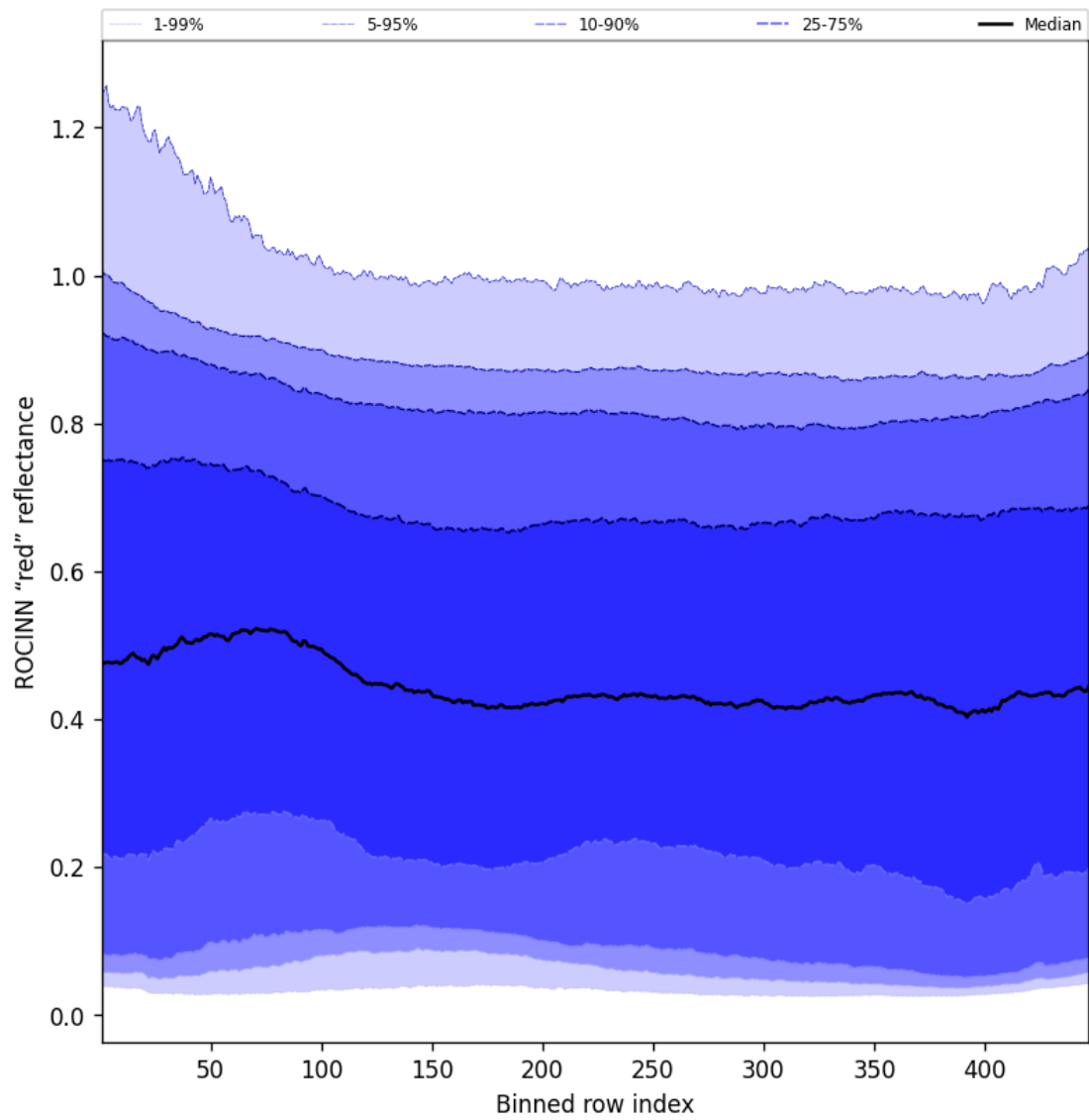
Figure 69: Along track statistics of “ROCINN “red” reflectance” for 2025-04-20 to 2025-04-22
