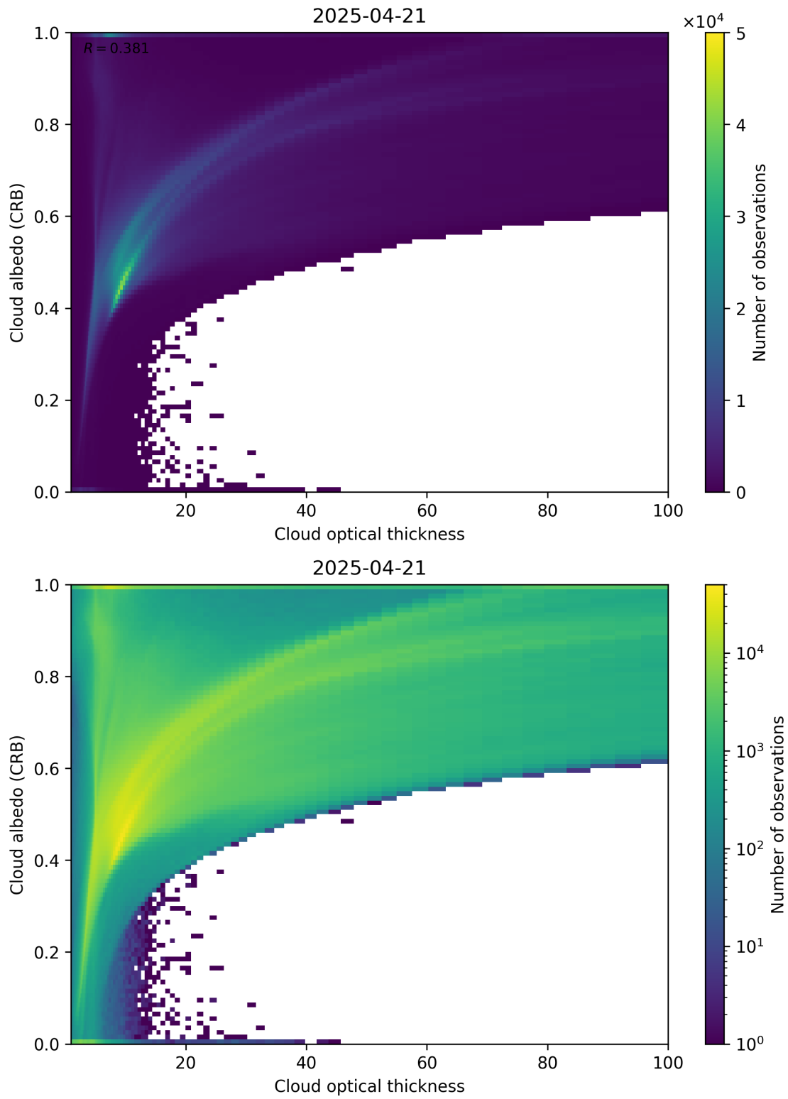
Figure 82: Scatter density plot of “Cloud optical thickness” against “Cloud albedo (CRB)” for 2025-04-20 to 2025-04-22.
