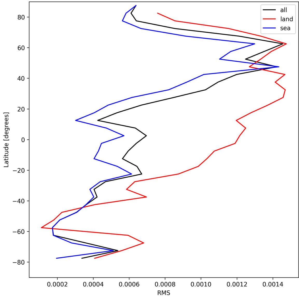
Figure 31: Zonal average of “RMS” for 2025-04-20 to 2025-04-22.
