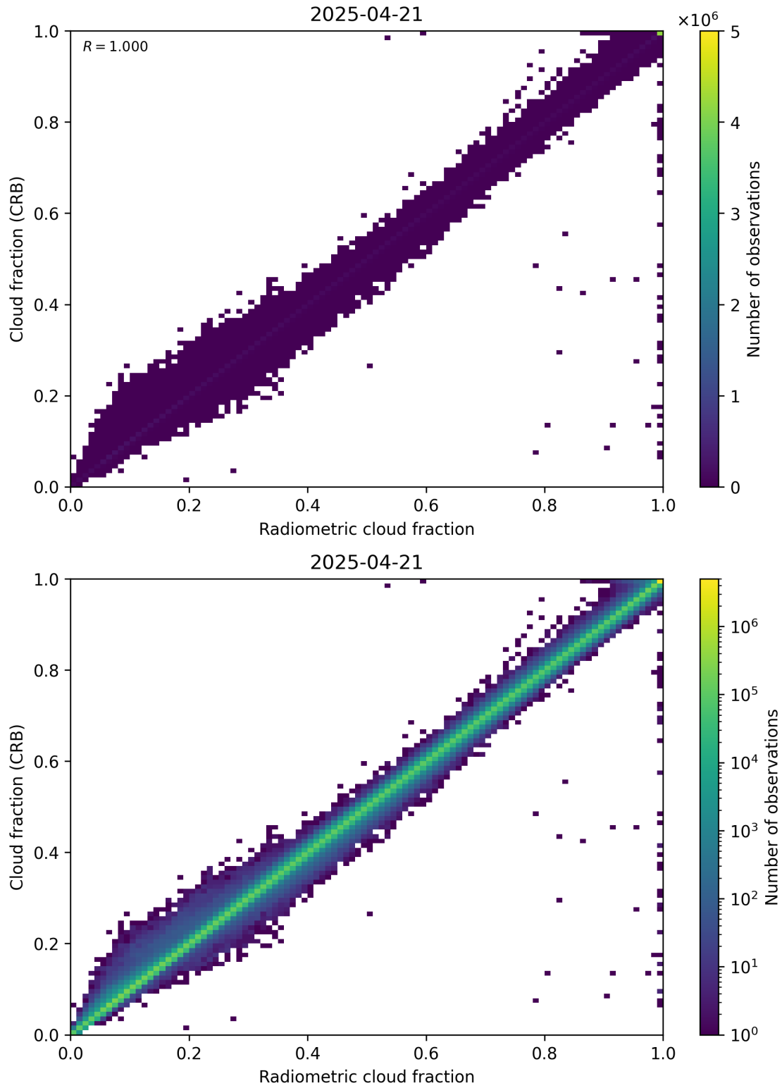
Figure 73: Scatter density plot of “Radiometric cloud fraction” against “Cloud fraction (CRB)” for 2025-04-20 to 2025-04-22.
