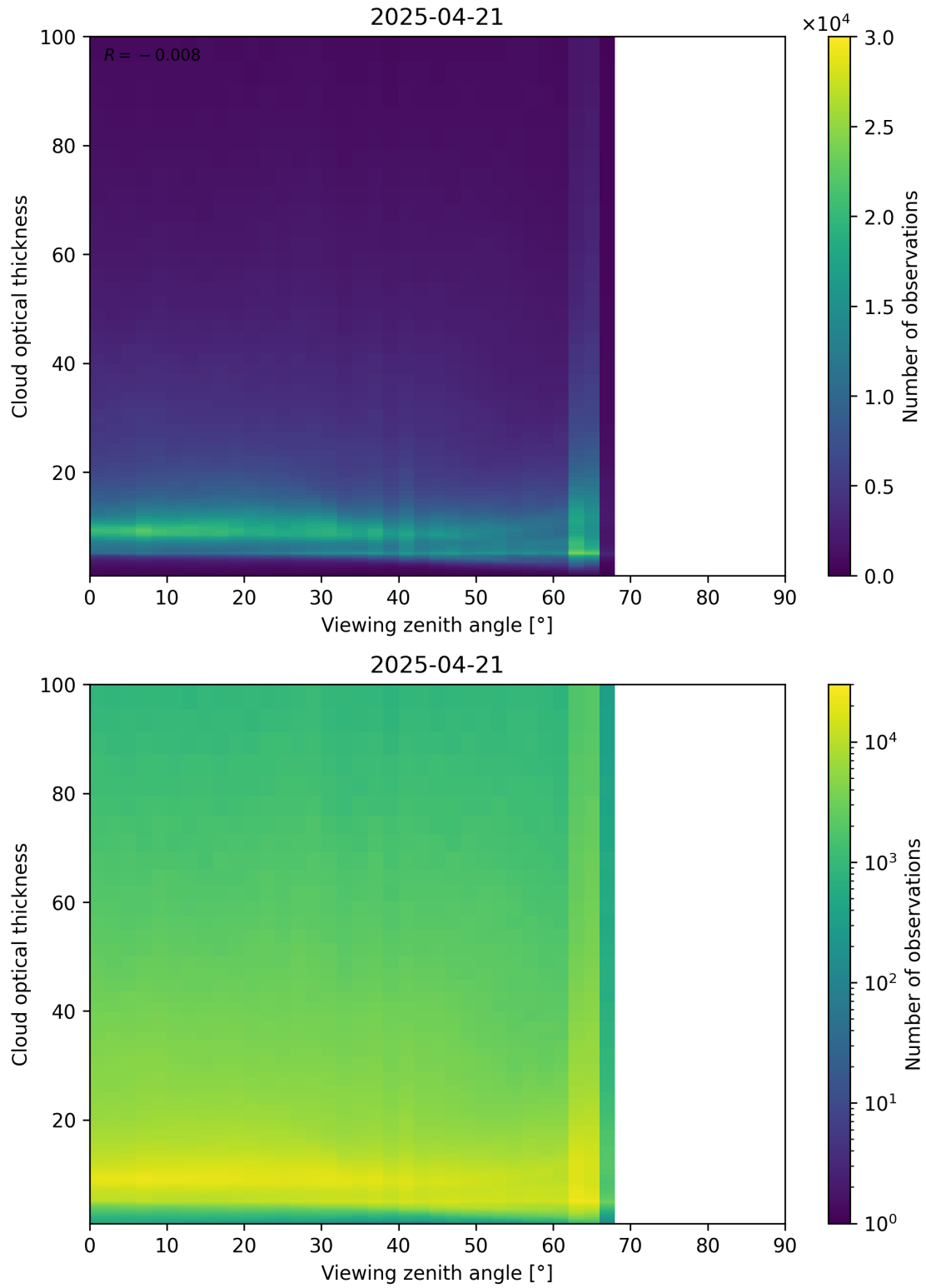
Figure 111: Scatter density plot of “Viewing zenith angle” against “Cloud optical thickness” for 2025-04-20 to 2025-04-22.
