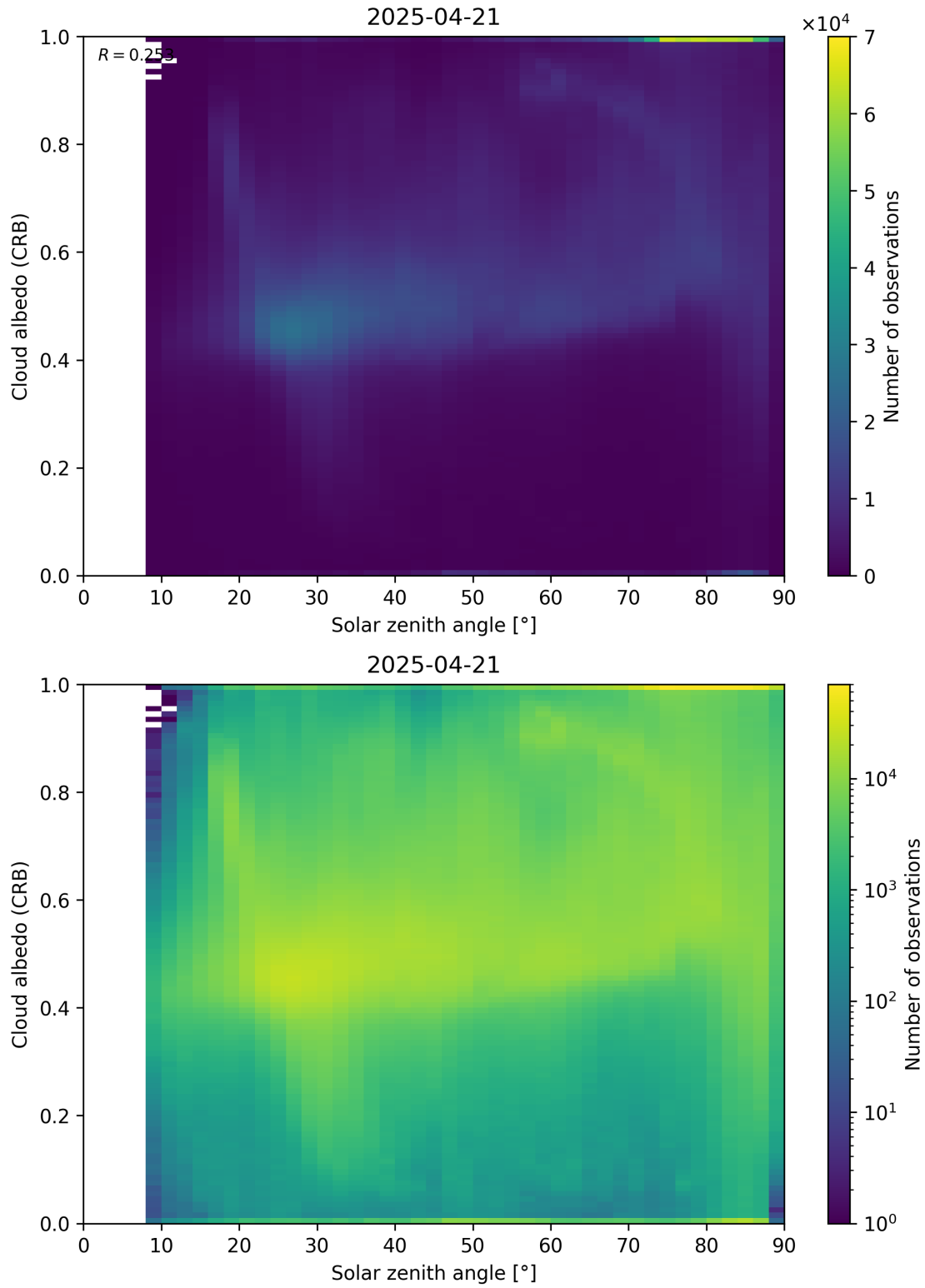
Figure 98: Scatter density plot of “Solar zenith angle” against “Cloud albedo (CRB)” for 2025-04-20 to 2025-04-22.
