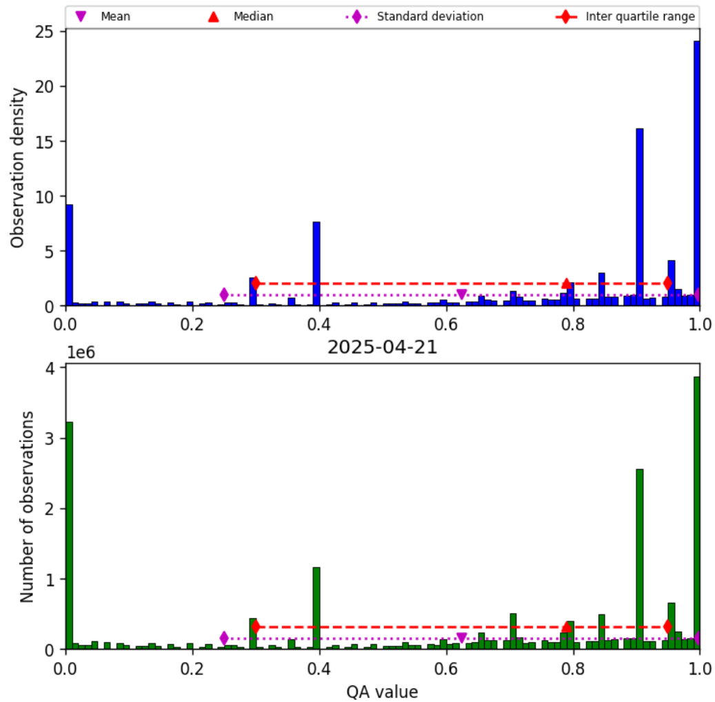
Figure 38: Histogram of “QA value” for 2025-04-20 to 2025-04-22
