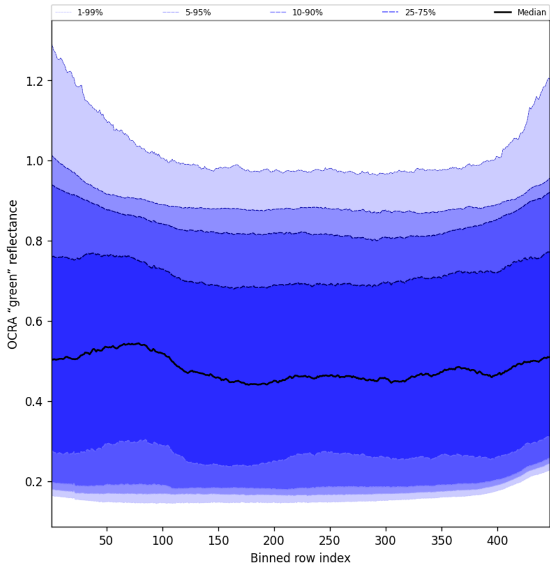
Figure 68: Along track statistics of "OCRA "green" reflectance" for 2025-04-20 to 2025-04-22
