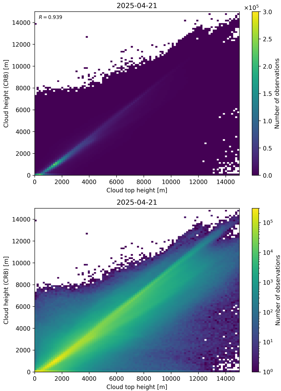
Figure 89: Scatter density plot of “Cloud top height” against “Cloud height (CRB)” for 2025-04-20 to 2025-04-22.
