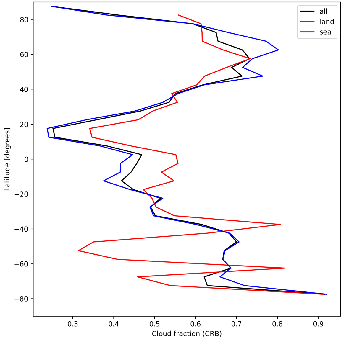
Figure 26: Zonal average of “Cloud fraction (CRB)” for 2025-04-20 to 2025-04-22.
