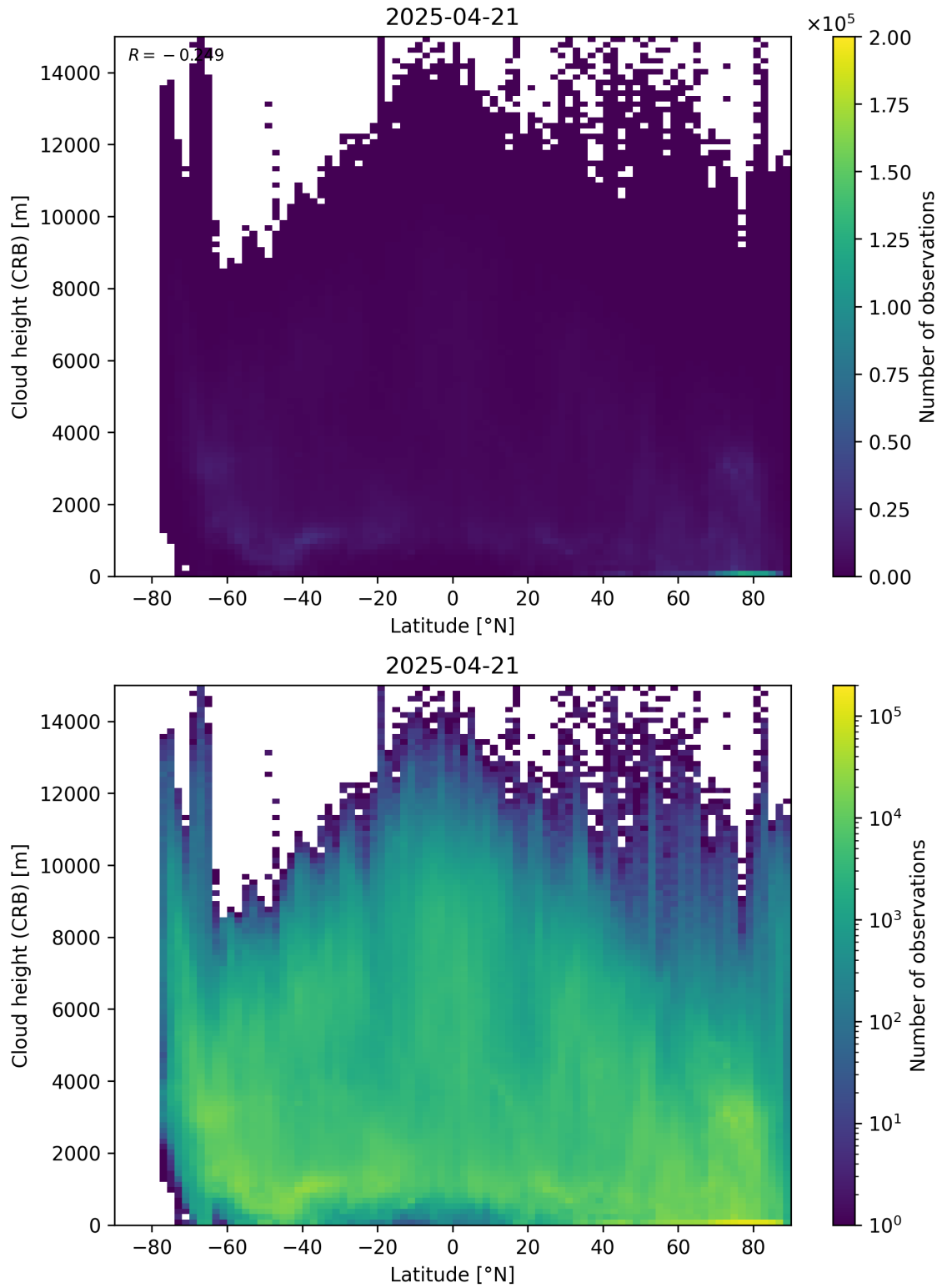
Figure 95: Scatter density plot of “Latitude” against “Cloud height (CRB)” for 2025-04-20 to 2025-04-22.
