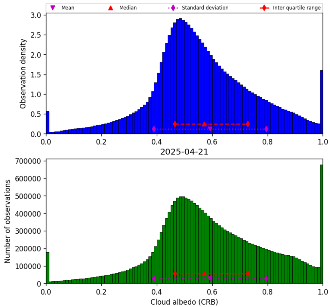
Figure 44: Histogram of “Cloud albedo (CRB)” for 2025-04-20 to 2025-04-22
