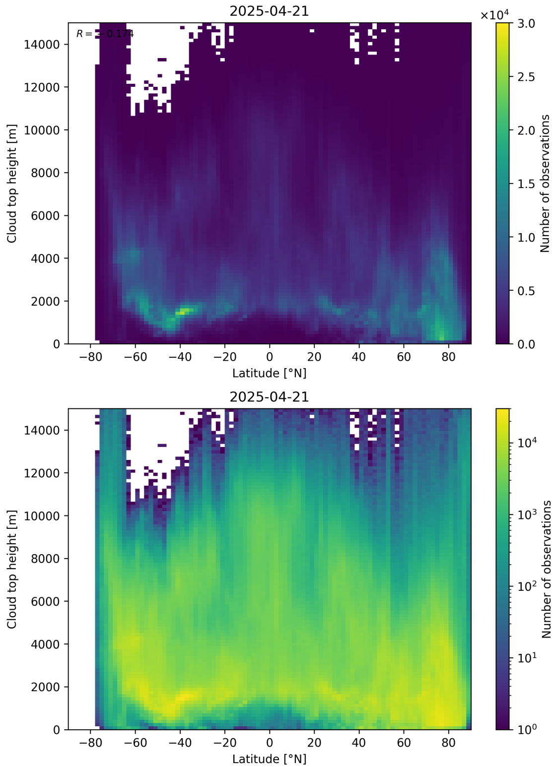
Figure 97: Scatter density plot of “Latitude” against “Cloud top height” for 2025-04-20 to 2025-04-22.
