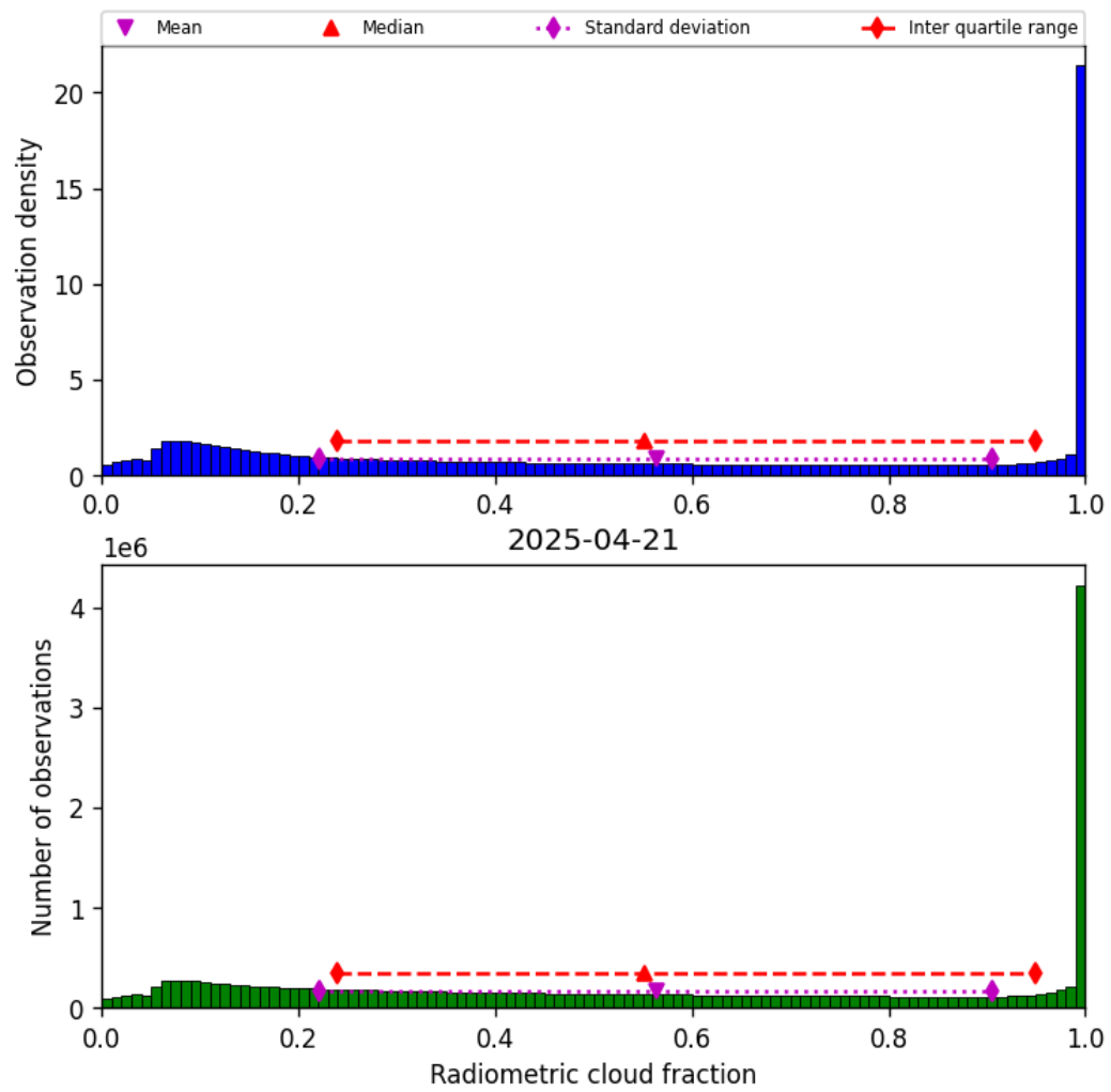
Figure 39: Histogram of “Radiometric cloud fraction” for 2025-04-20 to 2025-04-22
