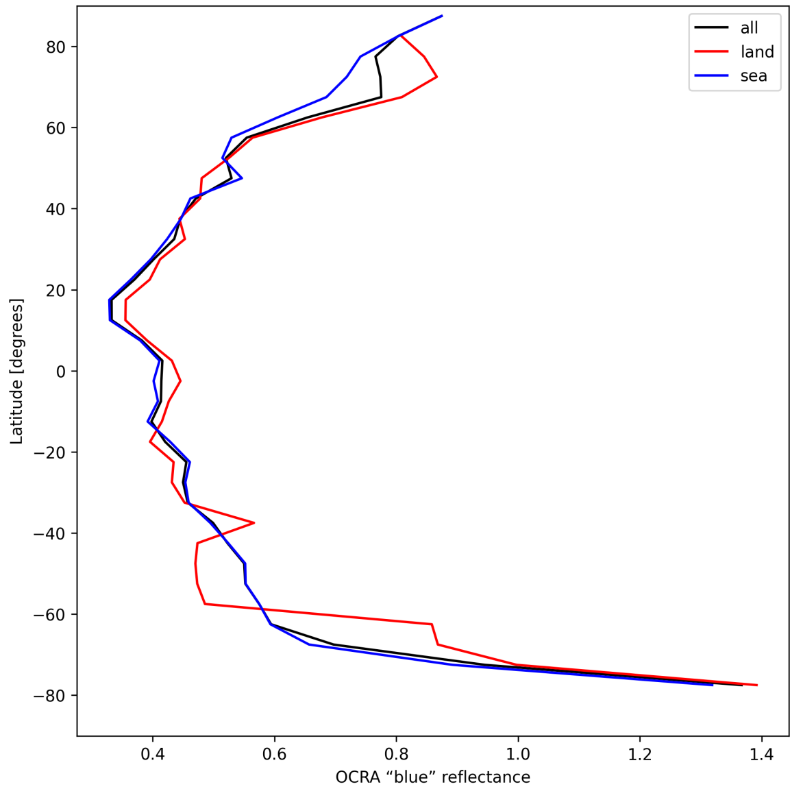
Figure 35: Zonal average of “OCRA “blue” reflectance” for 2025-04-20 to 2025-04-22.
