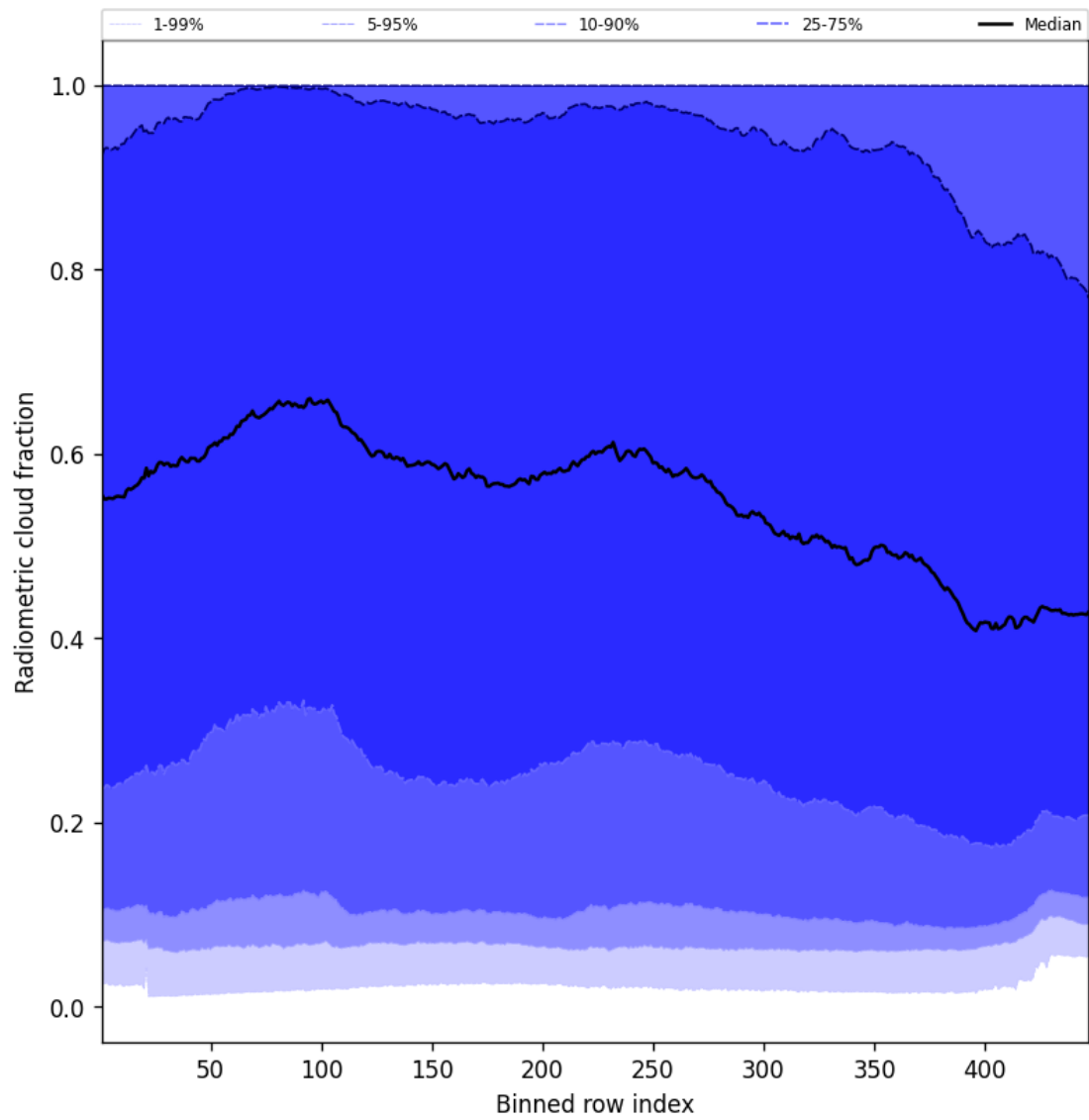
Figure 55: Along track statistics of “Radiometric cloud fraction” for 2025-04-20 to 2025-04-22
