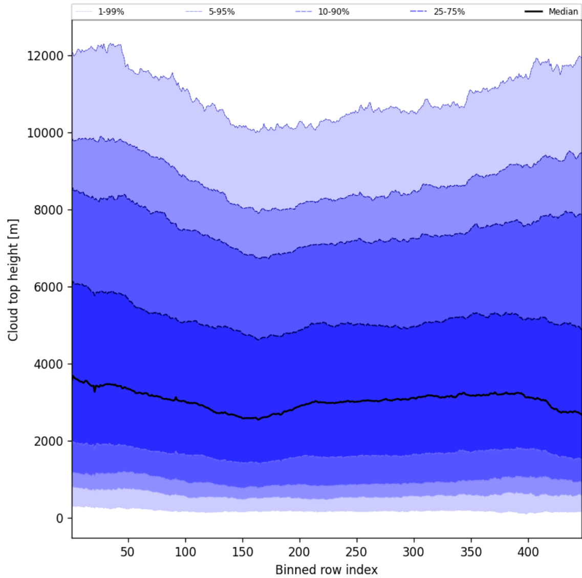
Figure 56: Along track statistics of “Cloud top height” for 2025-04-20 to 2025-04-22
