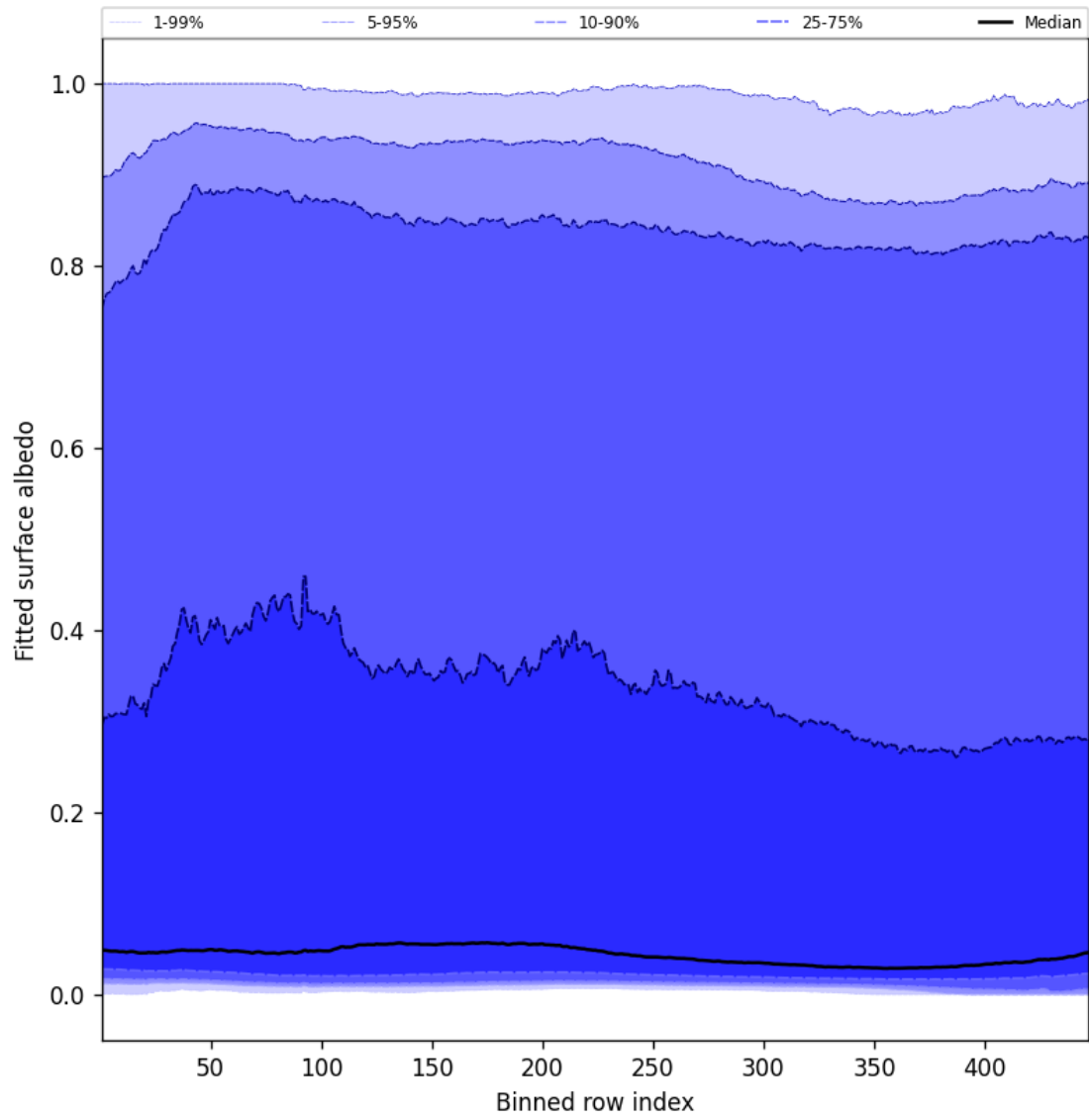
Figure 61: Along track statistics of “Fitted surface albedo” for 2025-04-20 to 2025-04-22
