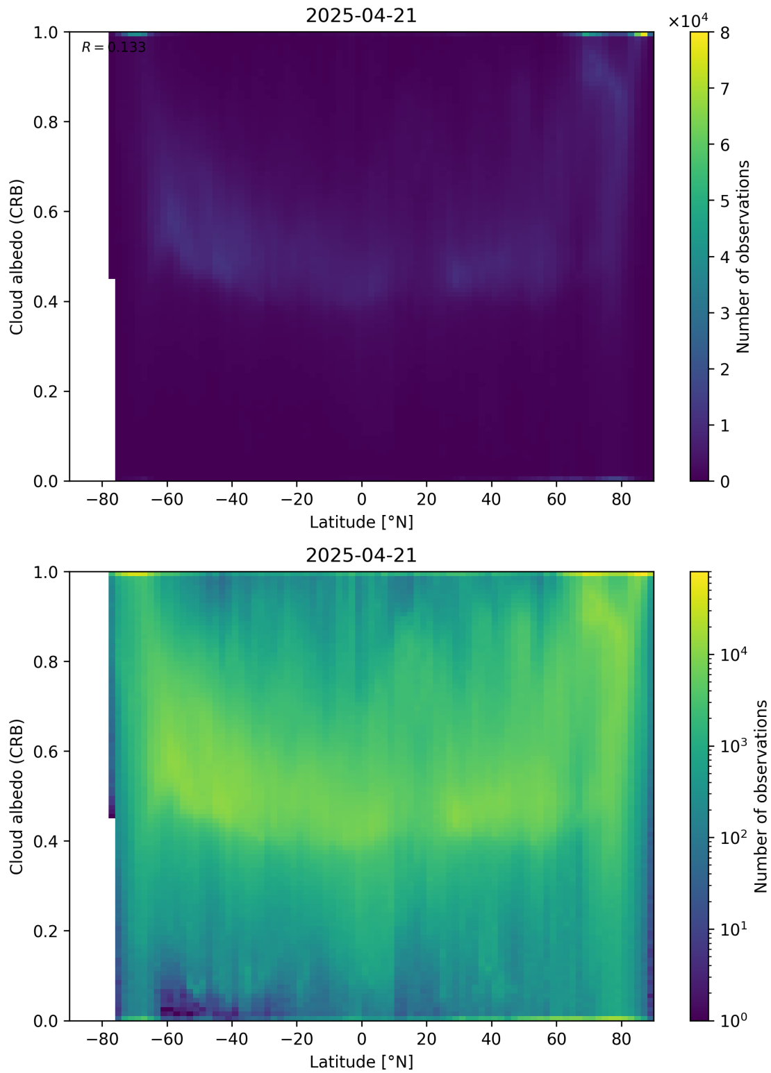
Figure 91: Scatter density plot of “Latitude” against “Cloud albedo (CRB)” for 2025-04-20 to 2025-04-22.
