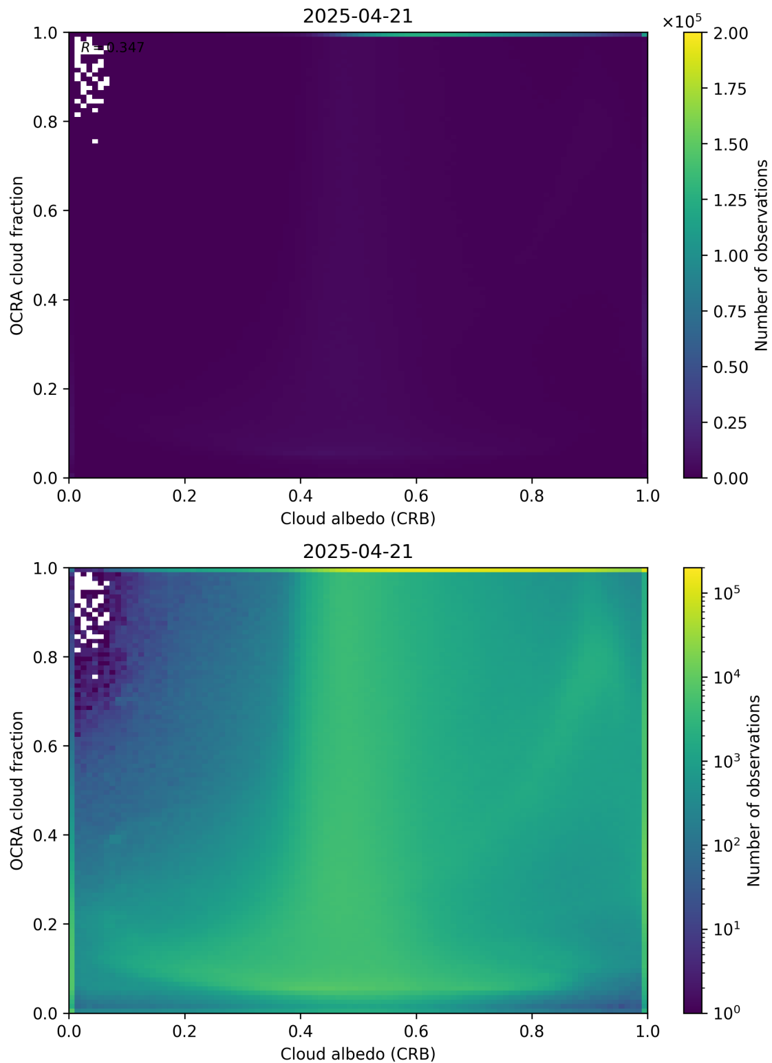
Figure 70: Scatter density plot of “Cloud albedo (CRB)” against “OCRA cloud fraction” for 2025-04-20 to 2025-04-22.
