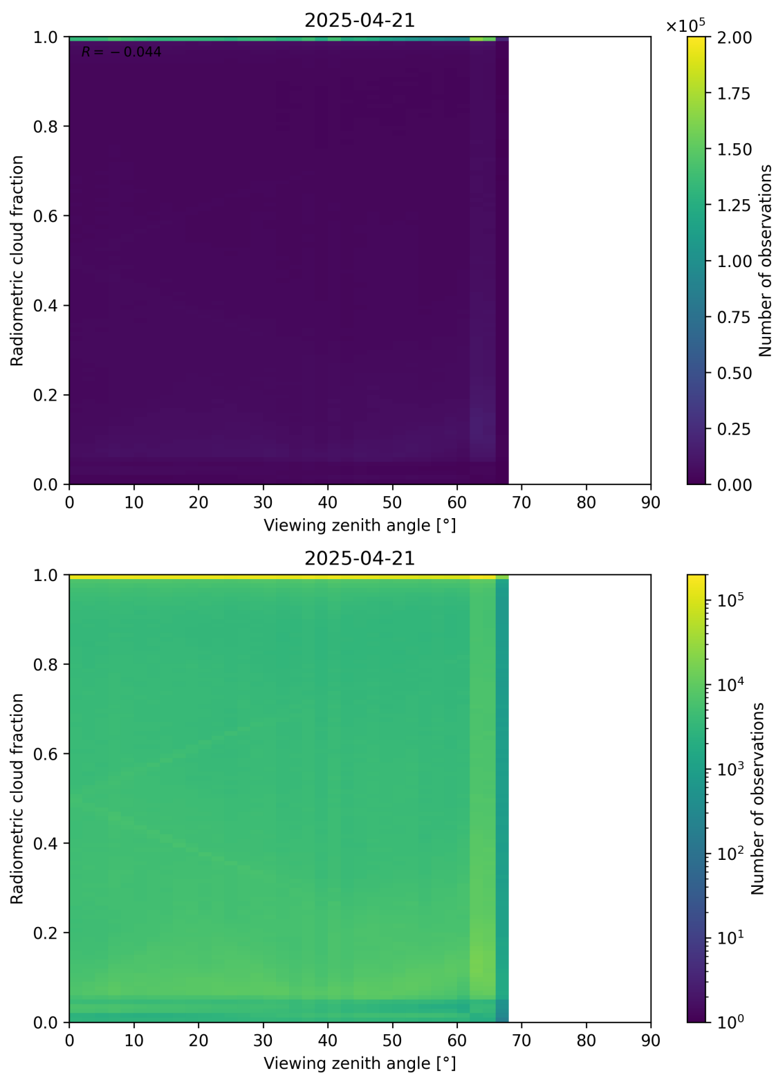
Figure 107: Scatter density plot of “Viewing zenith angle” against “Radiometric cloud fraction” for 2025-04-20 to 2025-04-22.
