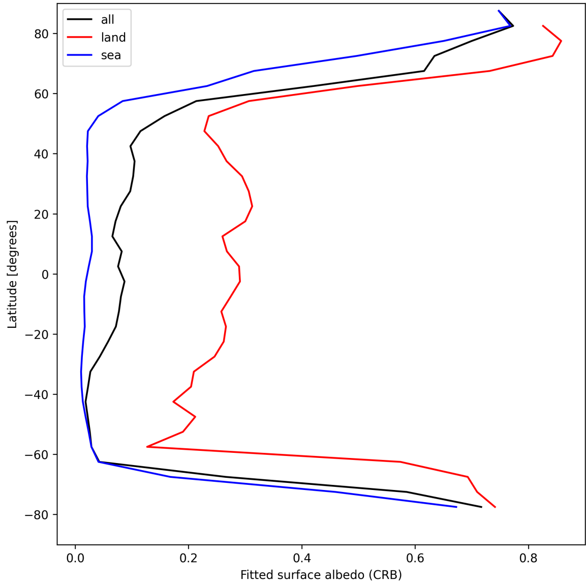
Figure 30: Zonal average of “Fitted surface albedo (CRB)” for 2025-04-21 to 2025-04-23.
