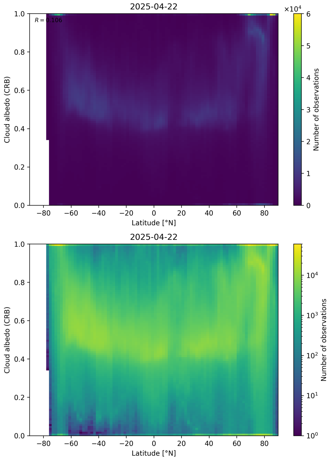
Figure 91: Scatter density plot of “Latitude” against “Cloud albedo (CRB)” for 2025-04-21 to 2025-04-23.
