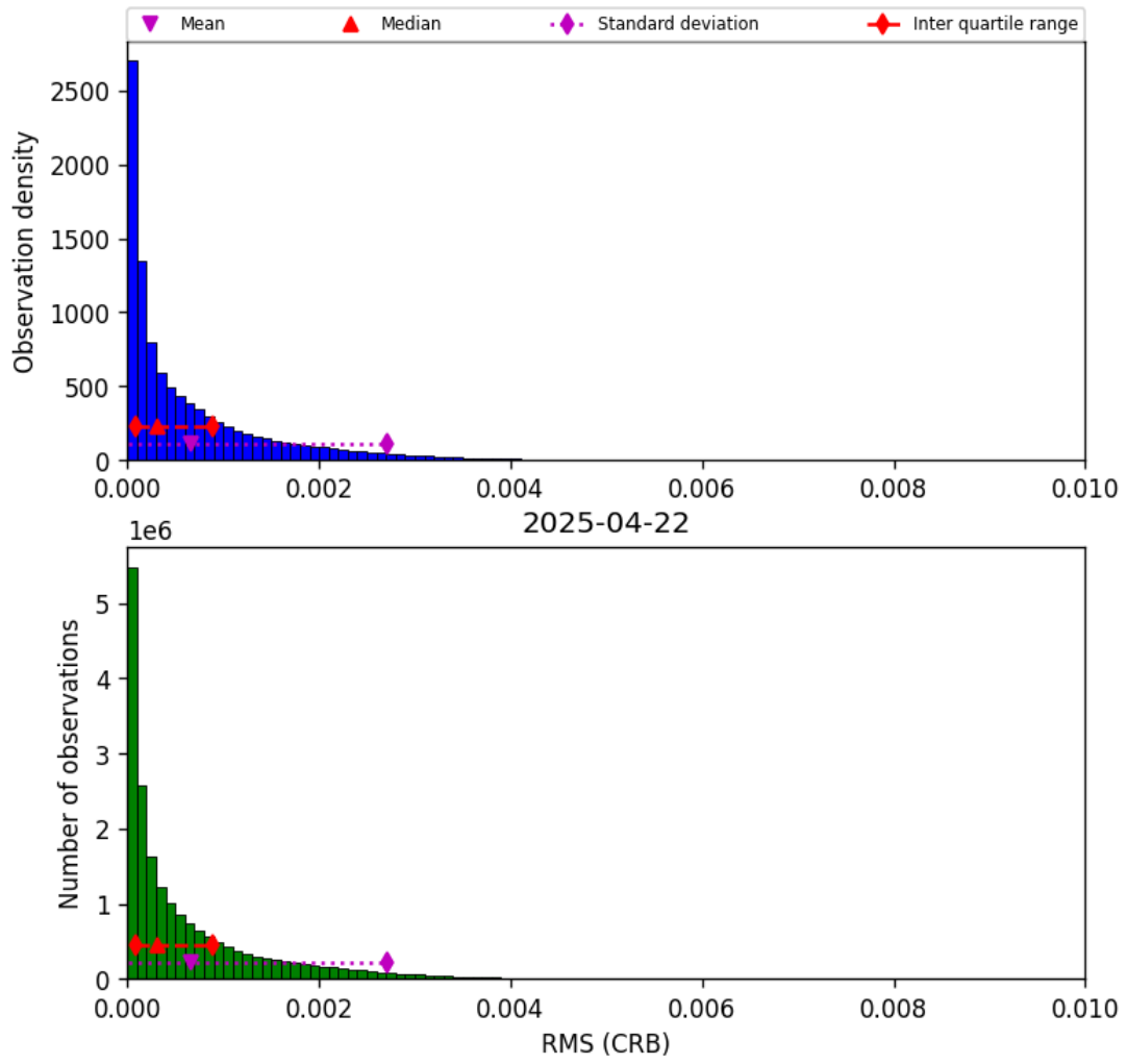
Figure 48: Histogram of “RMS (CRB)” for 2025-04-21 to 2025-04-23
