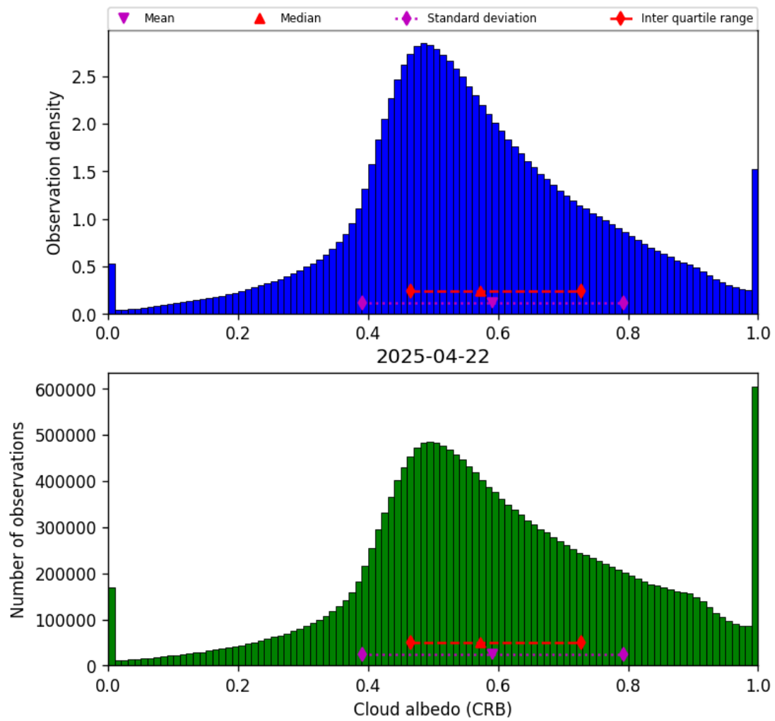
Figure 44: Histogram of “Cloud albedo (CRB)” for 2025-04-21 to 2025-04-23
