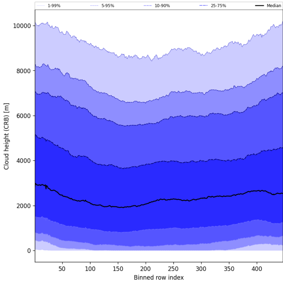
Figure 59: Along track statistics of “Cloud height (CRB)” for 2025-04-21 to 2025-04-23
