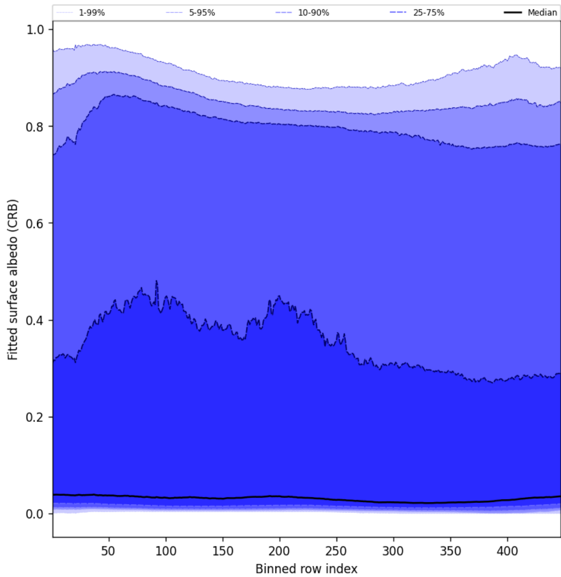
Figure 62: Along track statistics of “Fitted surface albedo (CRB)” for 2025-04-21 to 2025-04-23
