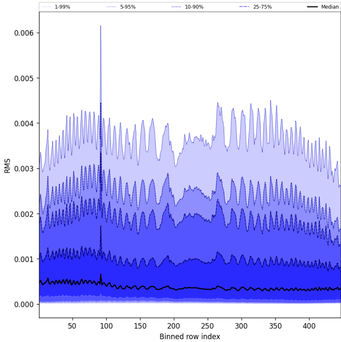
Figure 63: Along track statistics of “RMS” for 2025-04-21 to 2025-04-23
