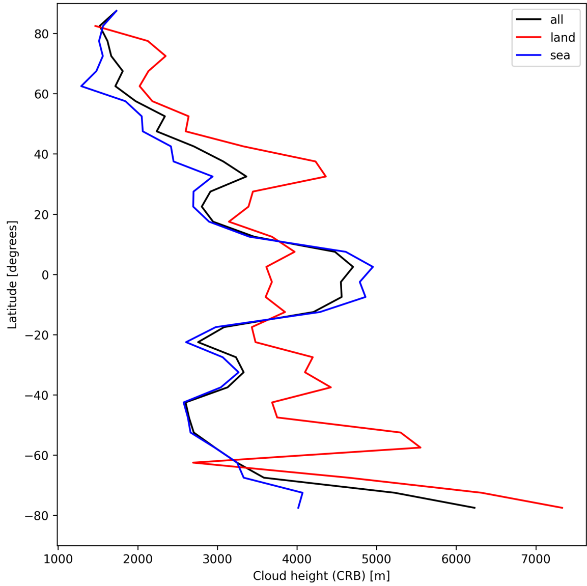
Figure 27: Zonal average of “Cloud height (CRB)” for 2025-04-21 to 2025-04-23.
