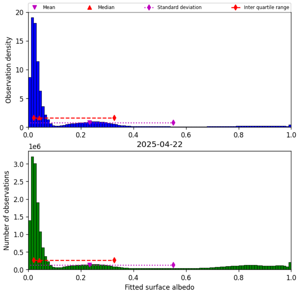
Figure 45: Histogram of “Fitted surface albedo” for 2025-04-21 to 2025-04-23
