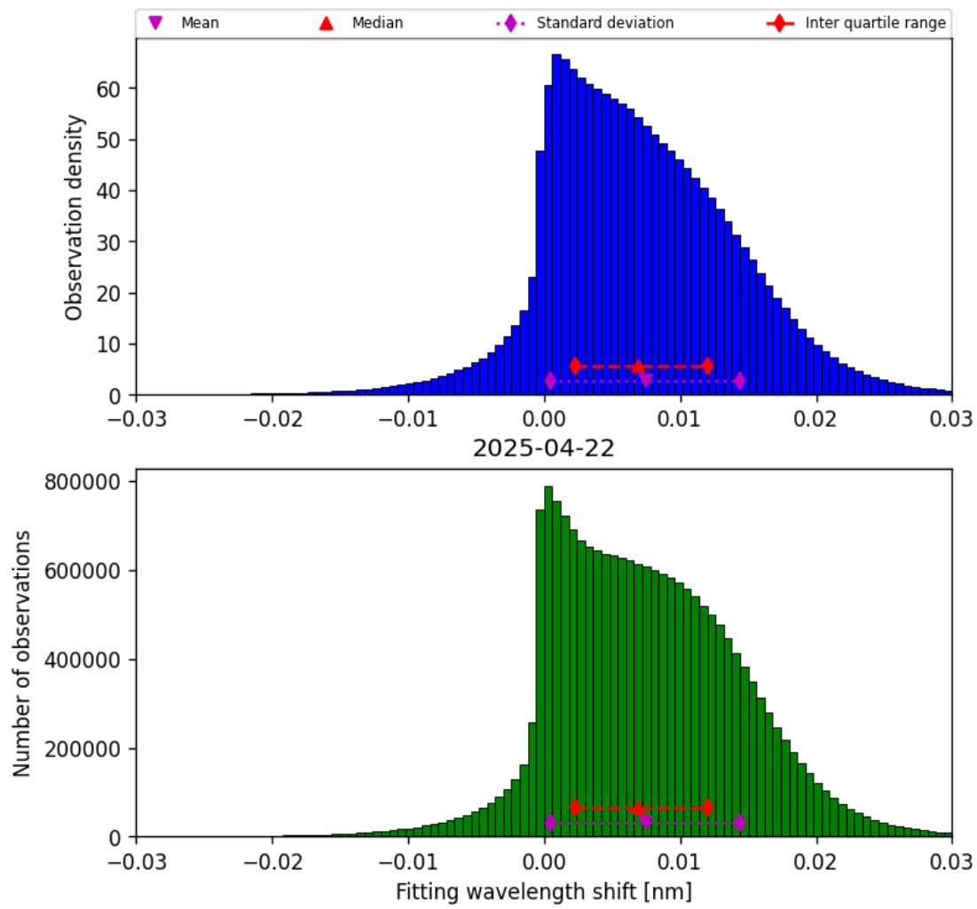
Figure 49: Histogram of “Fitting wavelength shift” for 2025-04-21 to 2025-04-23
