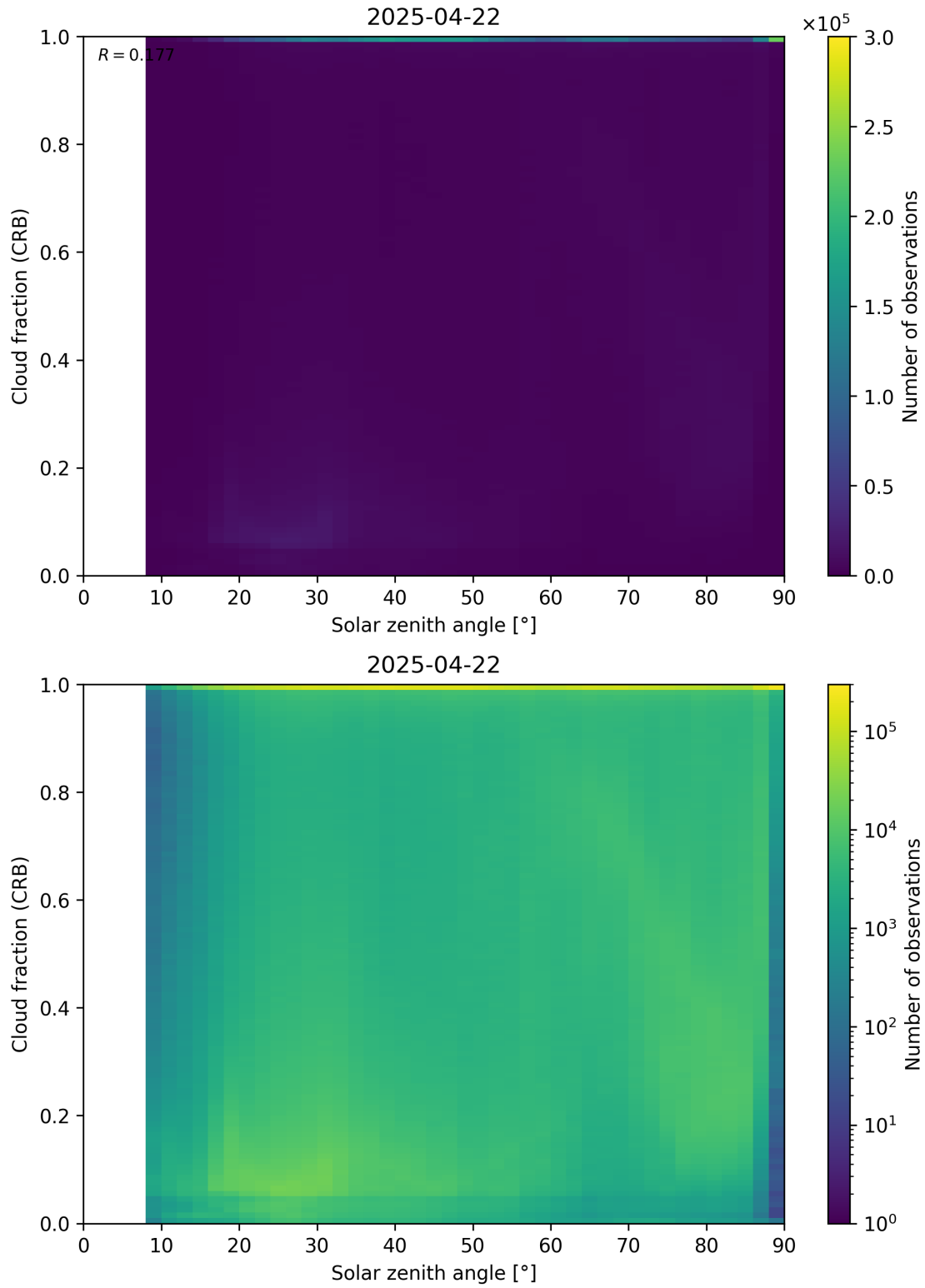
Figure 101: Scatter density plot of “Solar zenith angle” against “Cloud fraction (CRB)” for 2025-04-21 to 2025-04-23.
