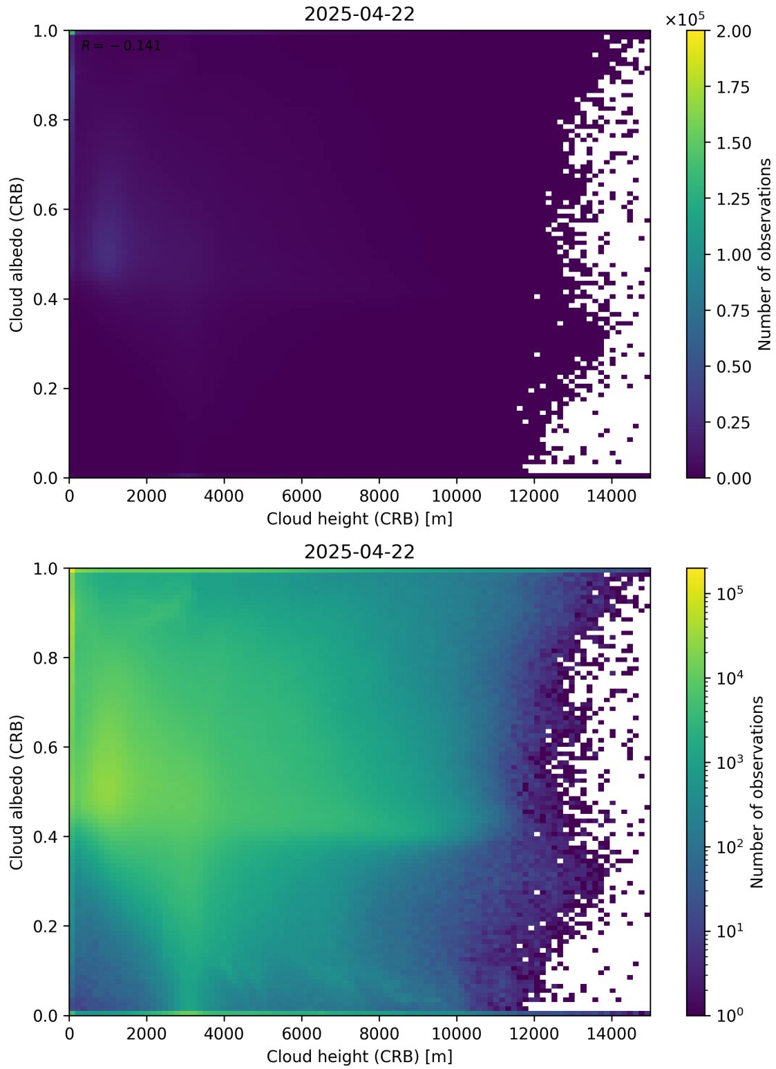
Figure 80: Scatter density plot of “Cloud height (CRB)” against “Cloud albedo (CRB)” for 2025-04-21 to 2025-04-23.
