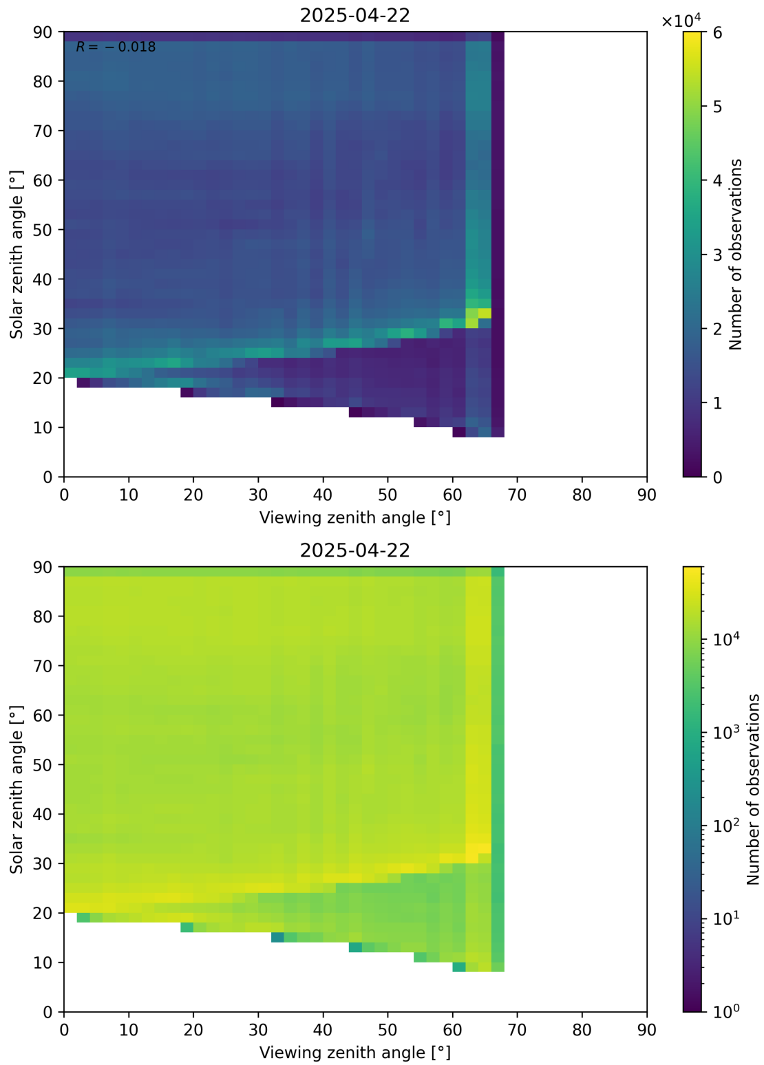
Figure 114: Scatter density plot of “Viewing zenith angle” against “Solar zenith angle” for 2025-04-21 to 2025-04-23.
