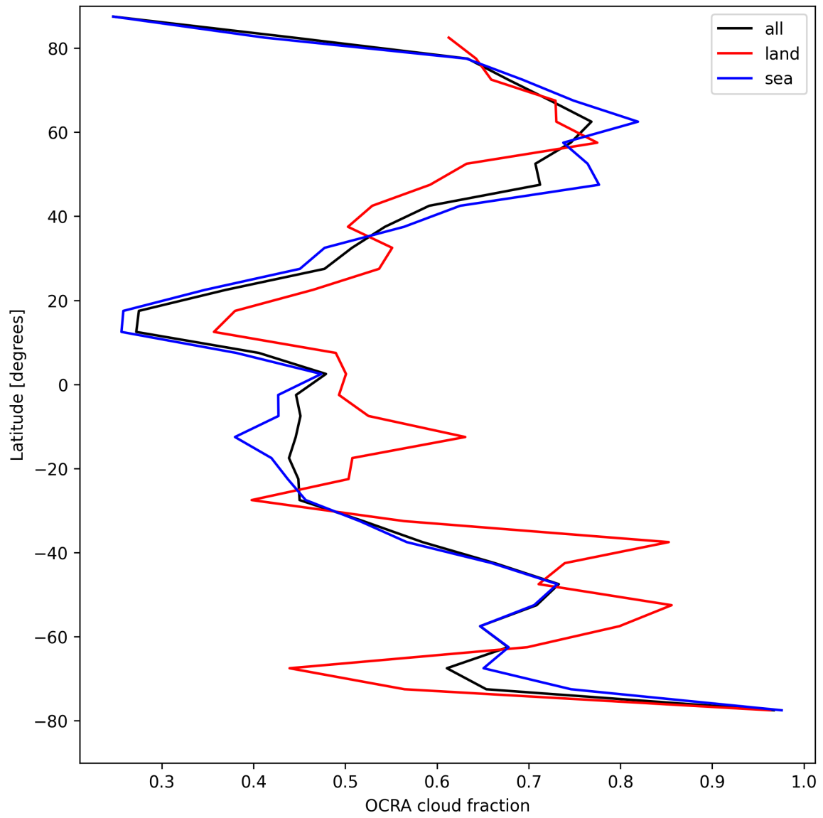
Figure 34: Zonal average of “OCRA cloud fraction” for 2025-04-21 to 2025-04-23.
