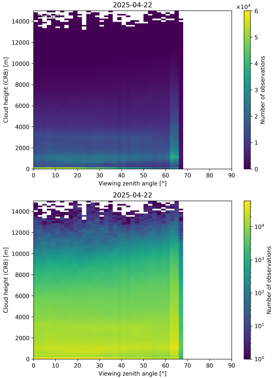
Figure 110: Scatter density plot of “Viewing zenith angle” against “Cloud height (CRB)” for 2025-04-21 to 2025-04-23.
