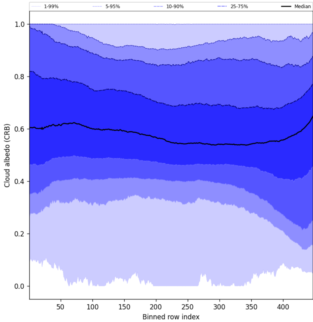
Figure 60: Along track statistics of “Cloud albedo (CRB)” for 2025-04-21 to 2025-04-23
