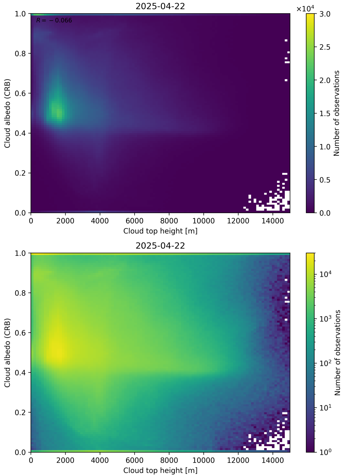
Figure 86: Scatter density plot of “Cloud top height” against “Cloud albedo (CRB)” for 2025-04-21 to 2025-04-23.
