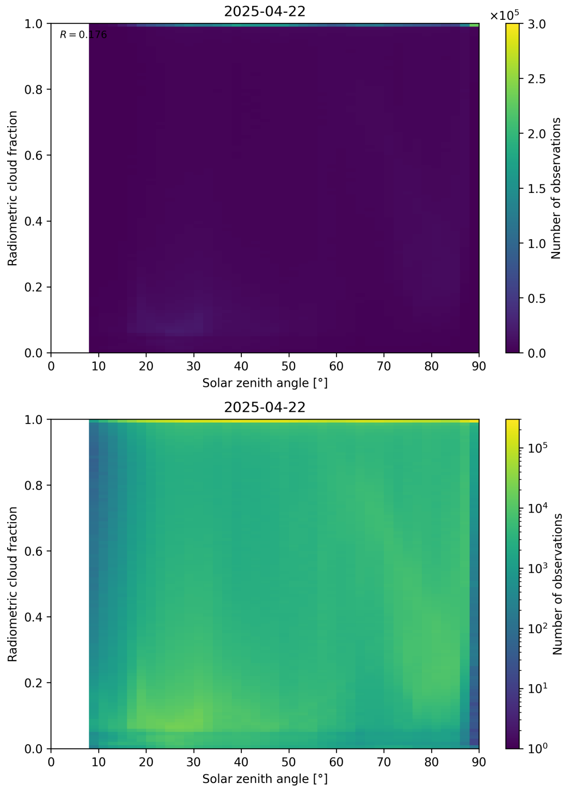
Figure 99: Scatter density plot of “Solar zenith angle” against “Radiometric cloud fraction” for 2025-04-21 to 2025-04-23.
