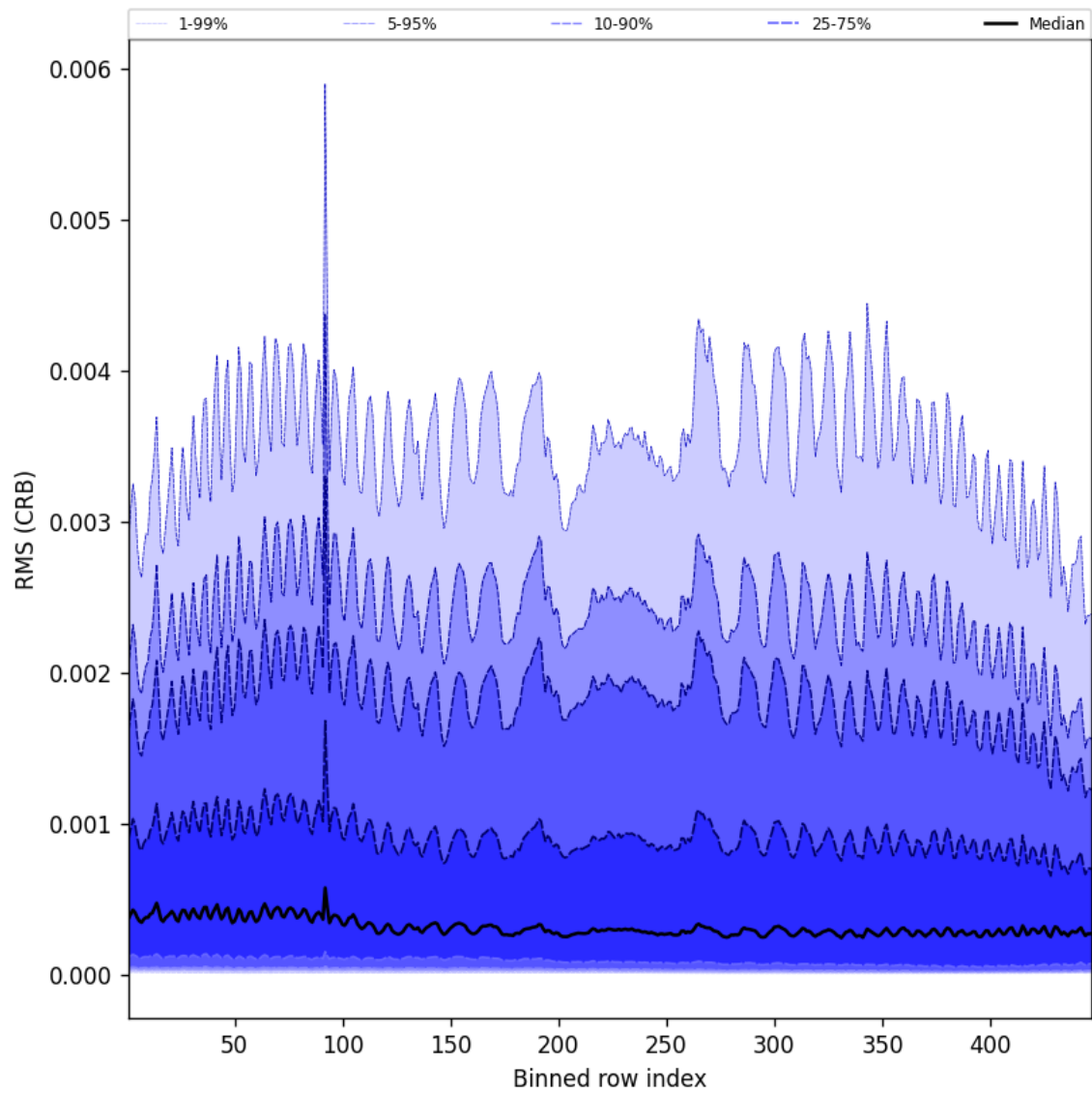
Figure 64: Along track statistics of “RMS (CRB)” for 2025-04-21 to 2025-04-23
