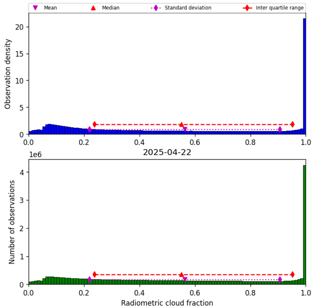
Figure 39: Histogram of “Radiometric cloud fraction” for 2025-04-21 to 2025-04-23
