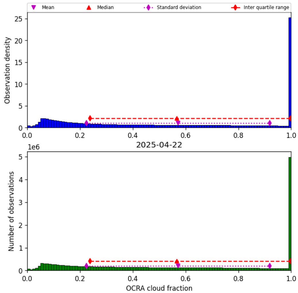
Figure 50: Histogram of “OCRA cloud fraction” for 2025-04-21 to 2025-04-23
