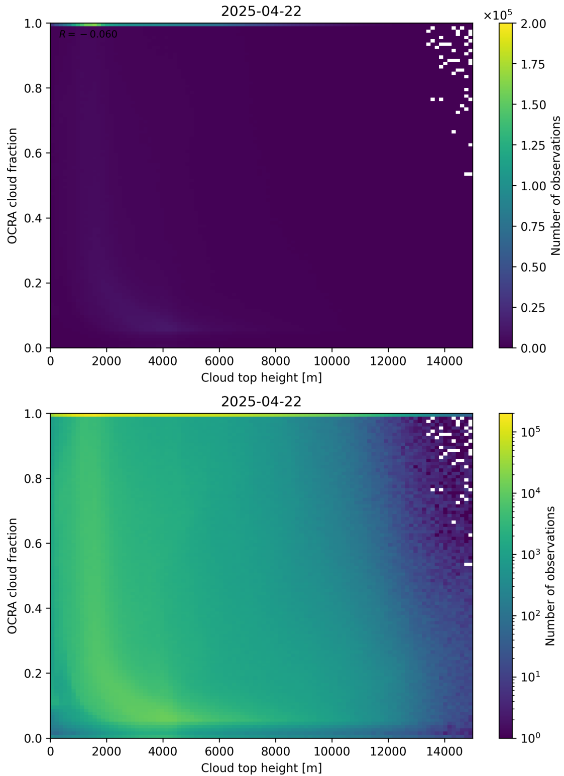
Figure 87: Scatter density plot of “Cloud top height” against “OCRA cloud fraction” for 2025-04-21 to 2025-04-23.
