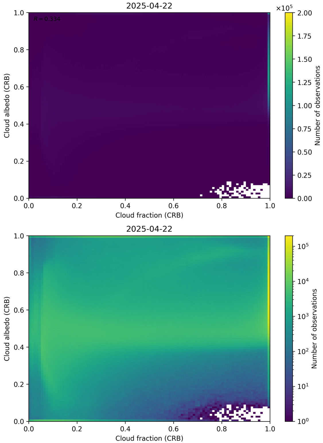
Figure 77: Scatter density plot of “Cloud fraction (CRB)” against “Cloud albedo (CRB)” for 2025-04-21 to 2025-04-23.
