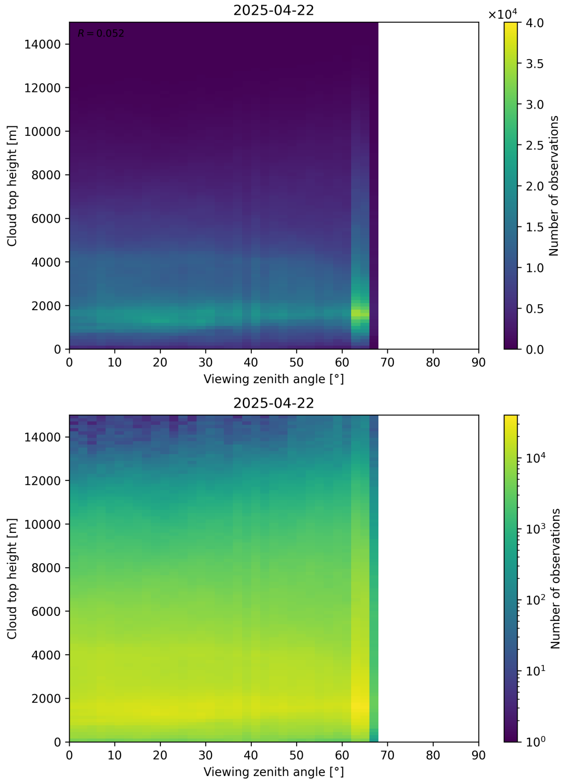
Figure 112: Scatter density plot of “Viewing zenith angle” against “Cloud top height” for 2025-04-21 to 2025-04-23.
