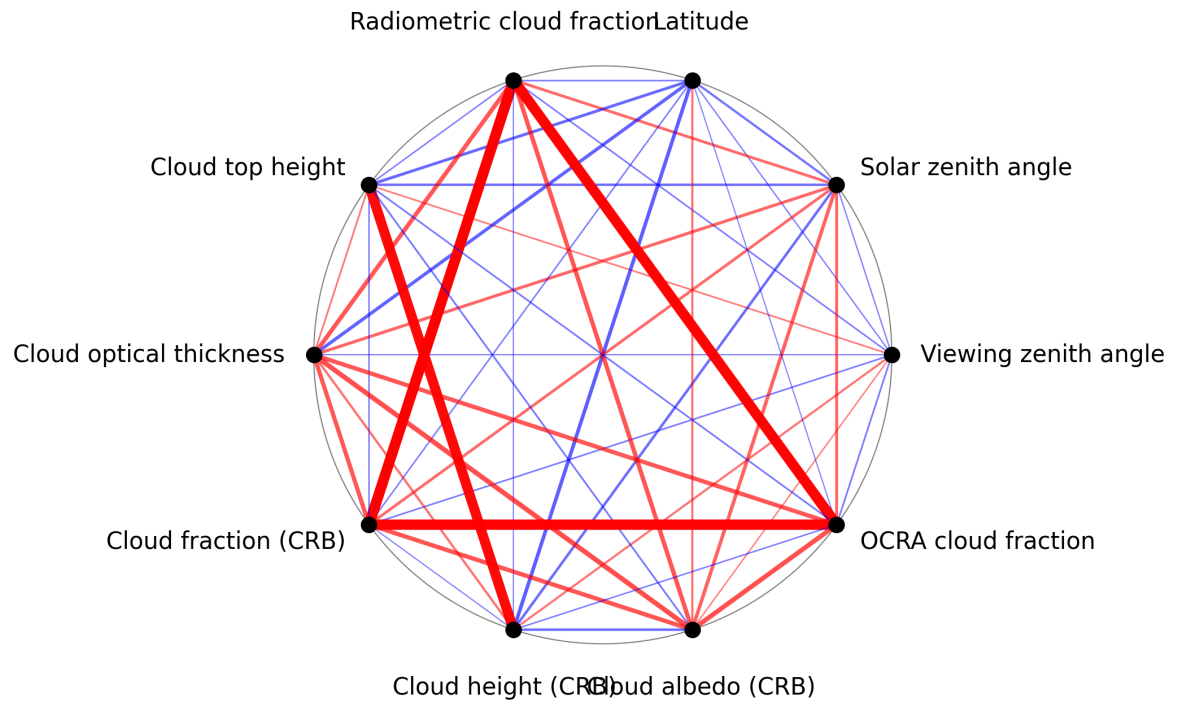
Figure 1: Map of correlation graph for 2025-04-21 to 2025-04-23.
