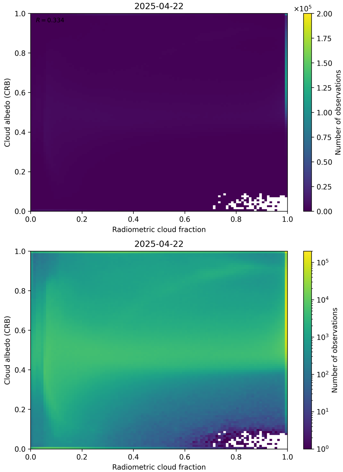
Figure 71: Scatter density plot of “Radiometric cloud fraction” against “Cloud albedo (CRB)” for 2025-04-21 to 2025-04-23.
