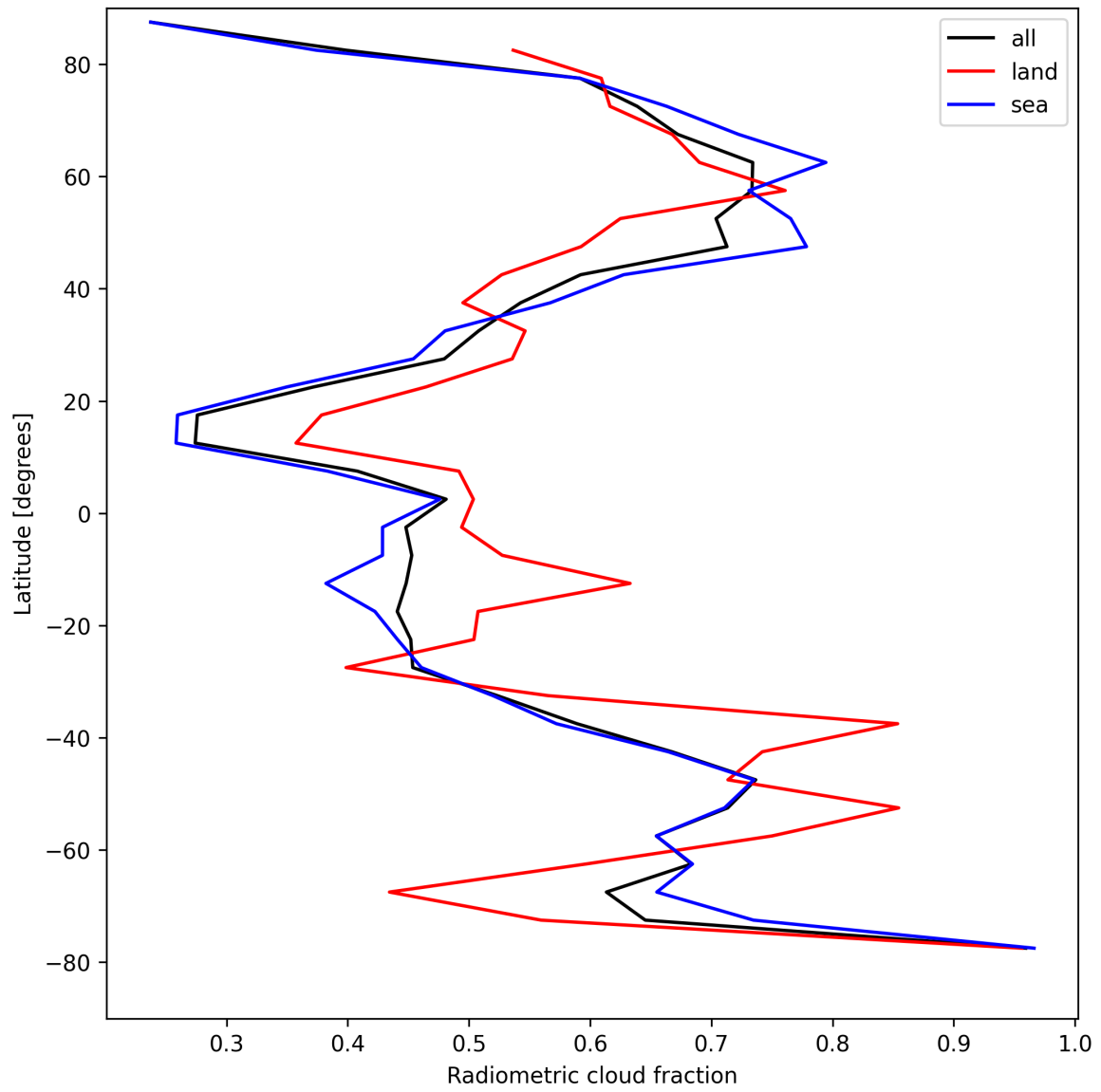
Figure 23: Zonal average of “Radiometric cloud fraction” for 2025-04-21 to 2025-04-23.
