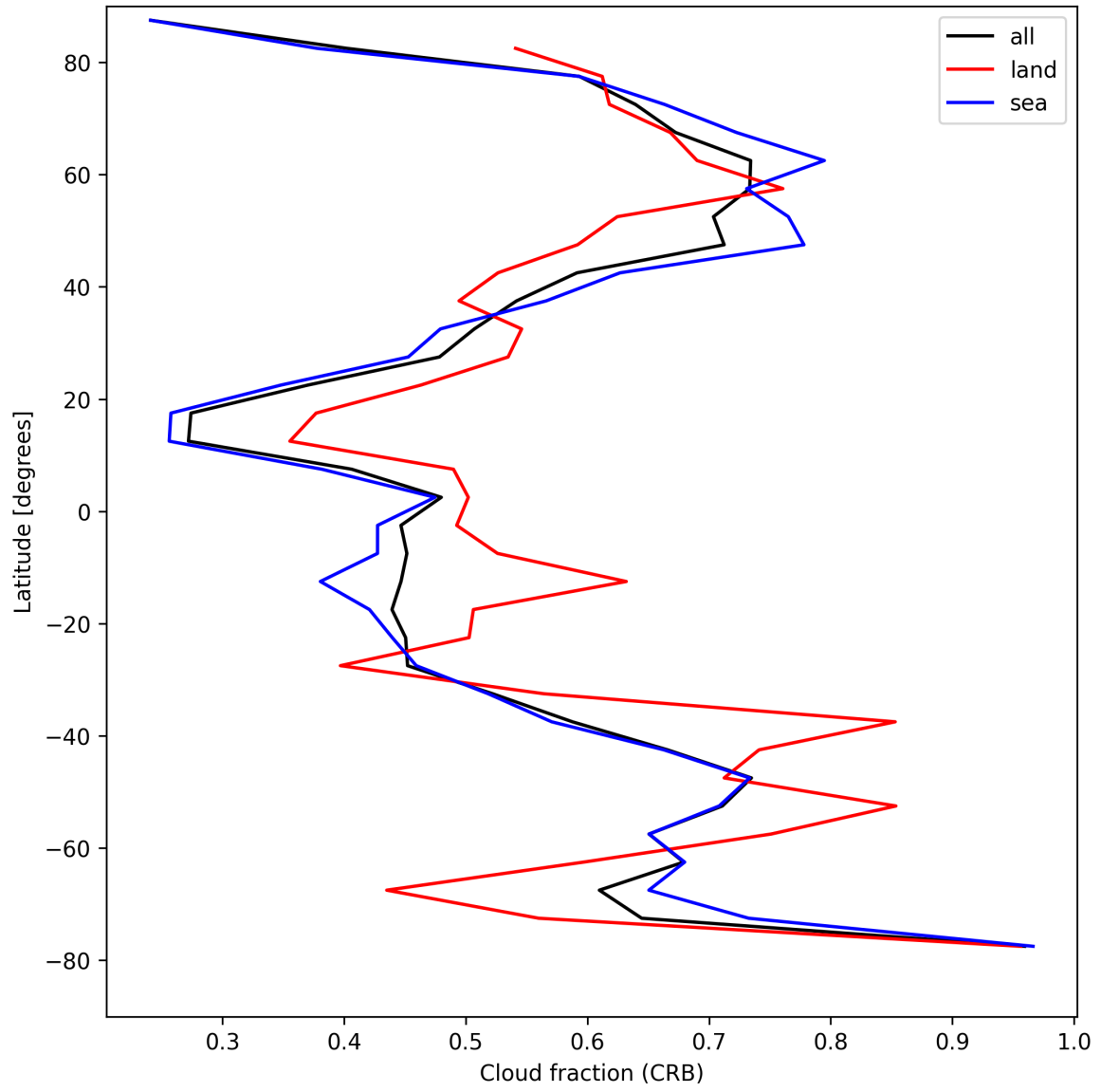
Figure 26: Zonal average of “Cloud fraction (CRB)” for 2025-04-21 to 2025-04-23.
