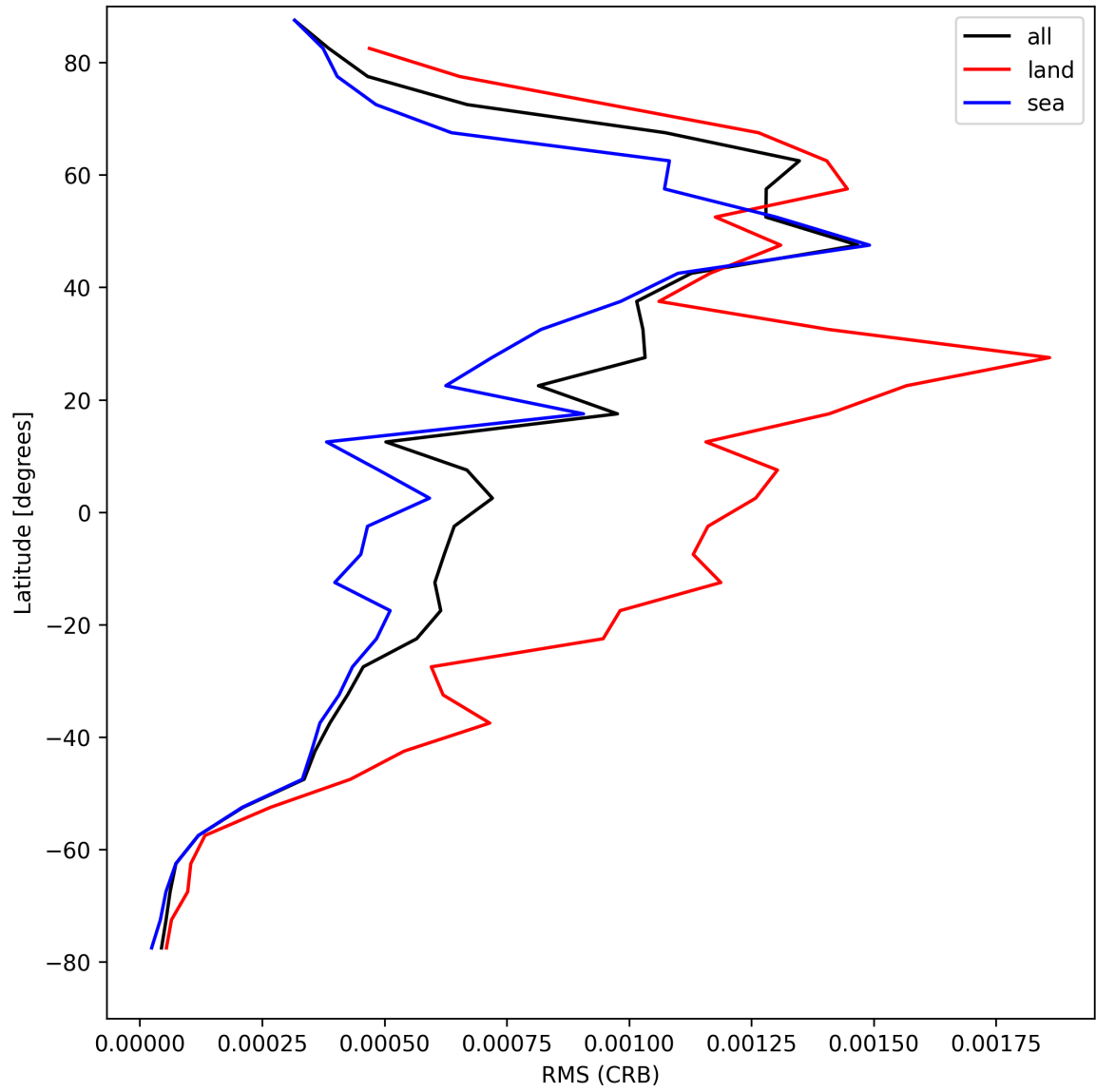
Figure 32: Zonal average of “RMS (CRB)” for 2025-04-21 to 2025-04-23.
