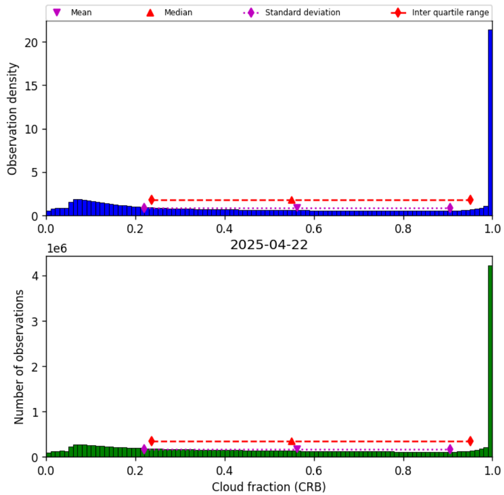
Figure 42: Histogram of “Cloud fraction (CRB)” for 2025-04-21 to 2025-04-23
