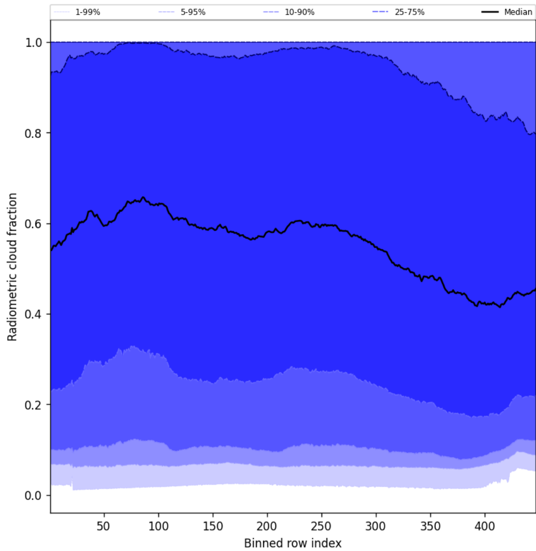
Figure 55: Along track statistics of “Radiometric cloud fraction” for 2025-04-21 to 2025-04-23
