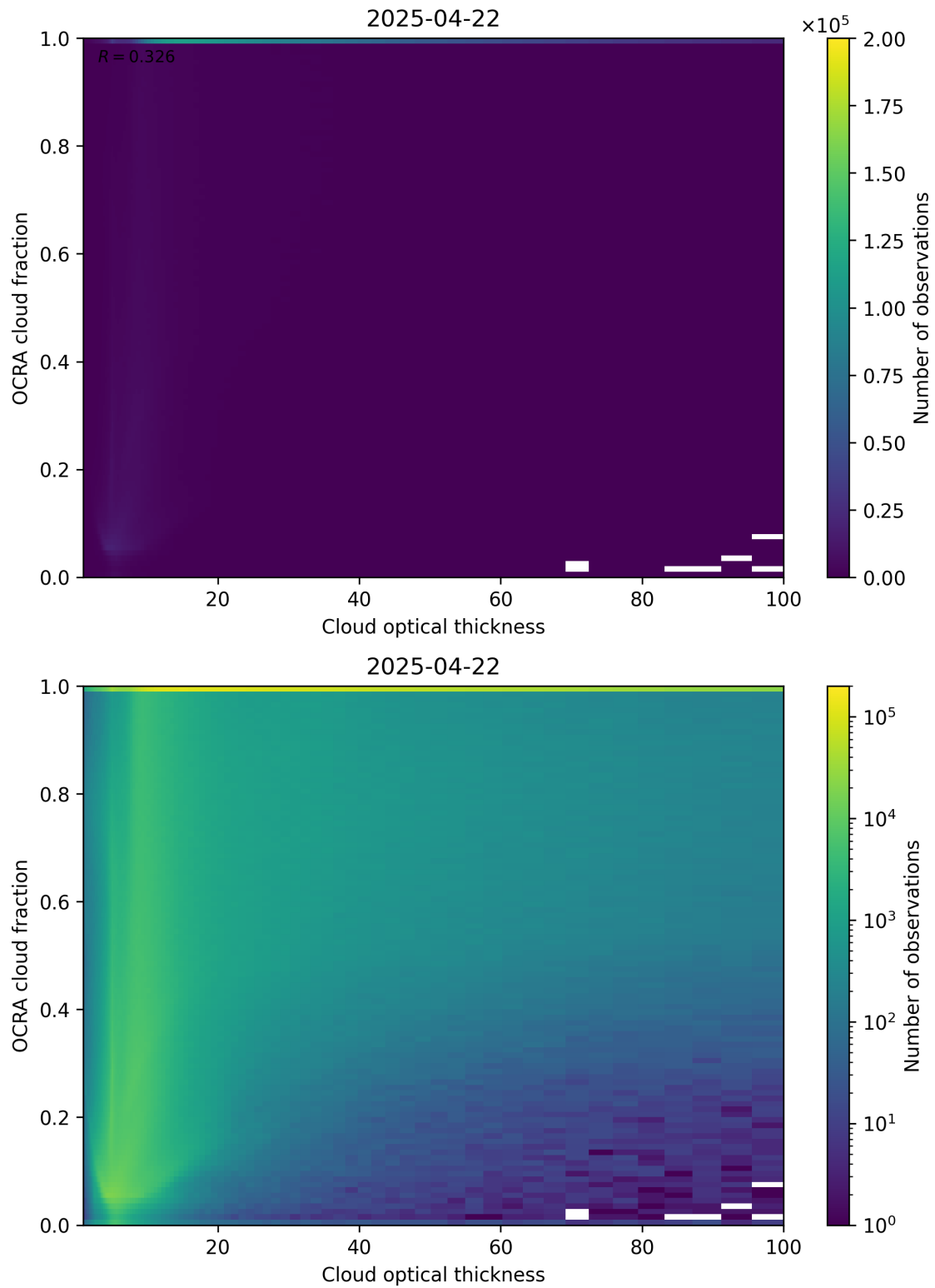
Figure 83: Scatter density plot of “Cloud optical thickness” against “OCRA cloud fraction” for 2025-04-21 to 2025-04-23.
