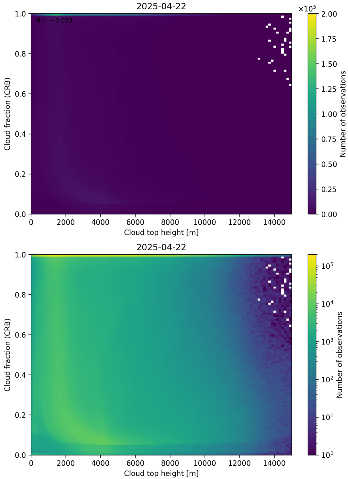
Figure 88: Scatter density plot of “Cloud top height” against “Cloud fraction (CRB)” for 2025-04-21 to 2025-04-23.
