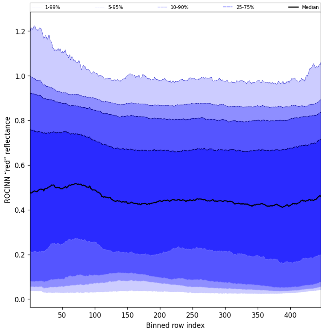
Figure 69: Along track statistics of “ROCINN “red” reflectance” for 2025-04-21 to 2025-04-23
