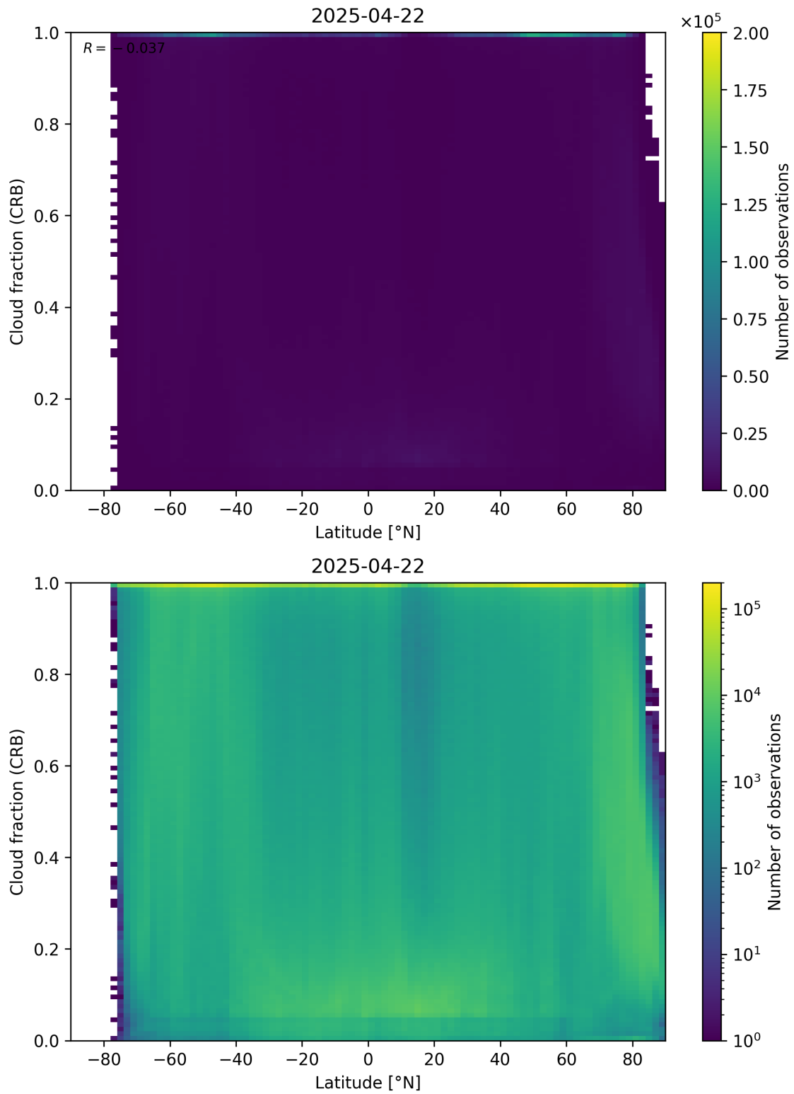
Figure 94: Scatter density plot of “Latitude” against “Cloud fraction (CRB)” for 2025-04-21 to 2025-04-23.
