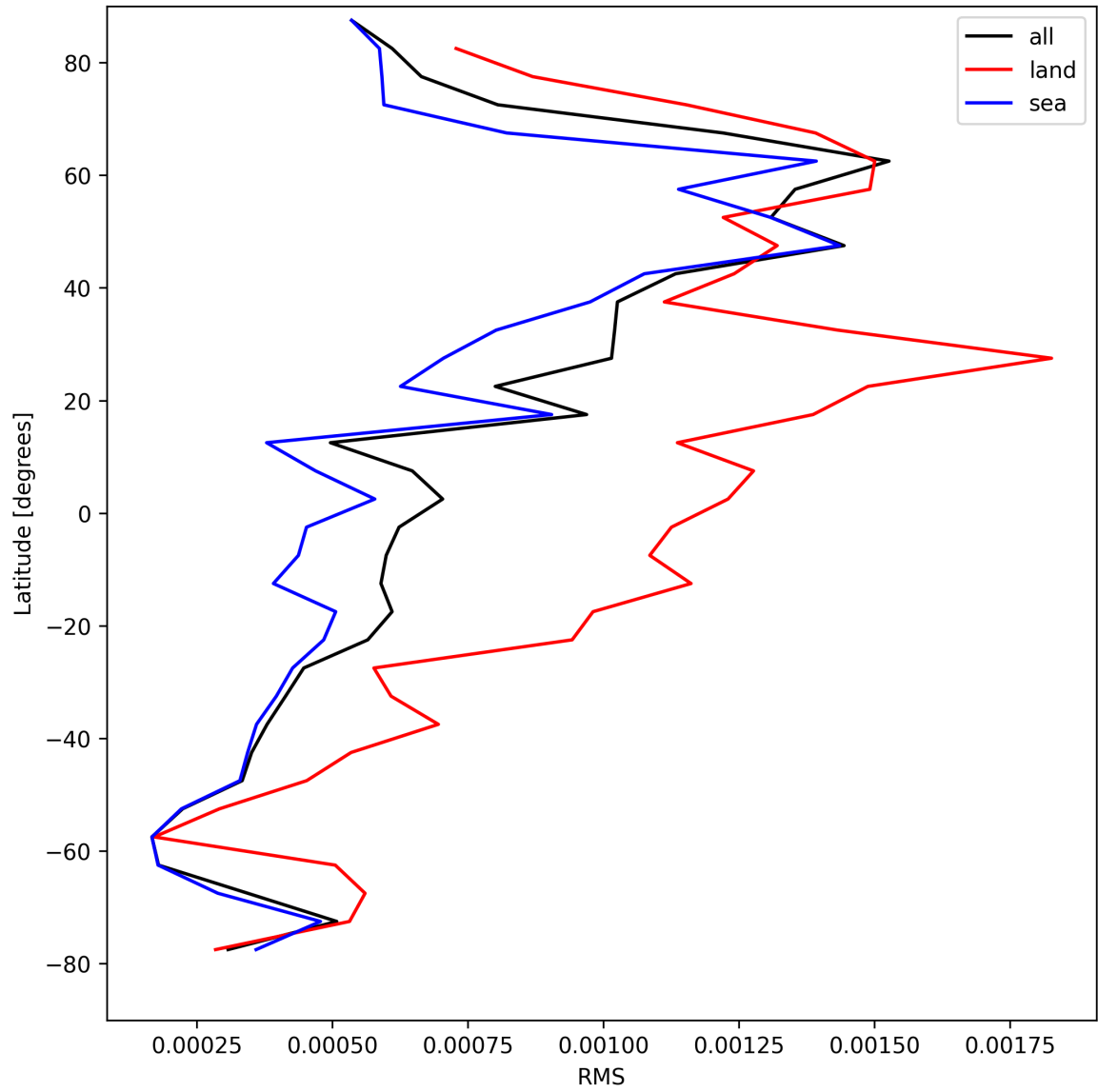
Figure 31: Zonal average of “RMS” for 2025-04-21 to 2025-04-23.
