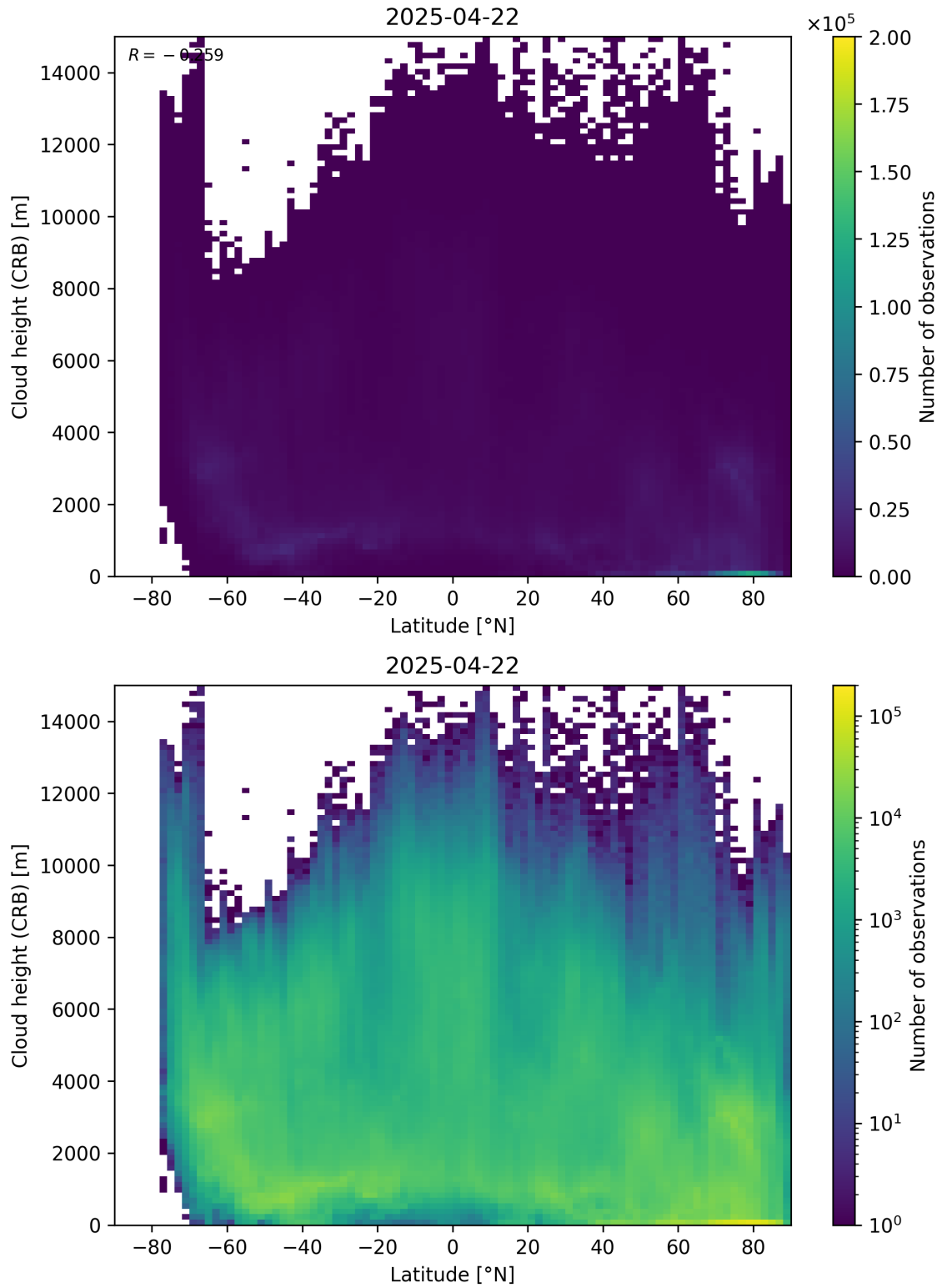
Figure 95: Scatter density plot of “Latitude” against “Cloud height (CRB)” for 2025-04-21 to 2025-04-23.
