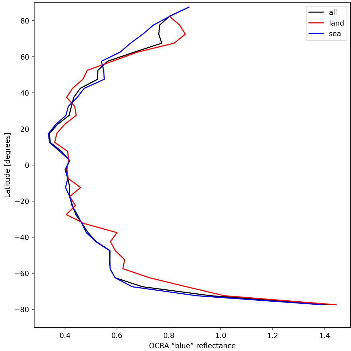
Figure 35: Zonal average of “OCRA “blue” reflectance” for 2025-04-21 to 2025-04-23.
