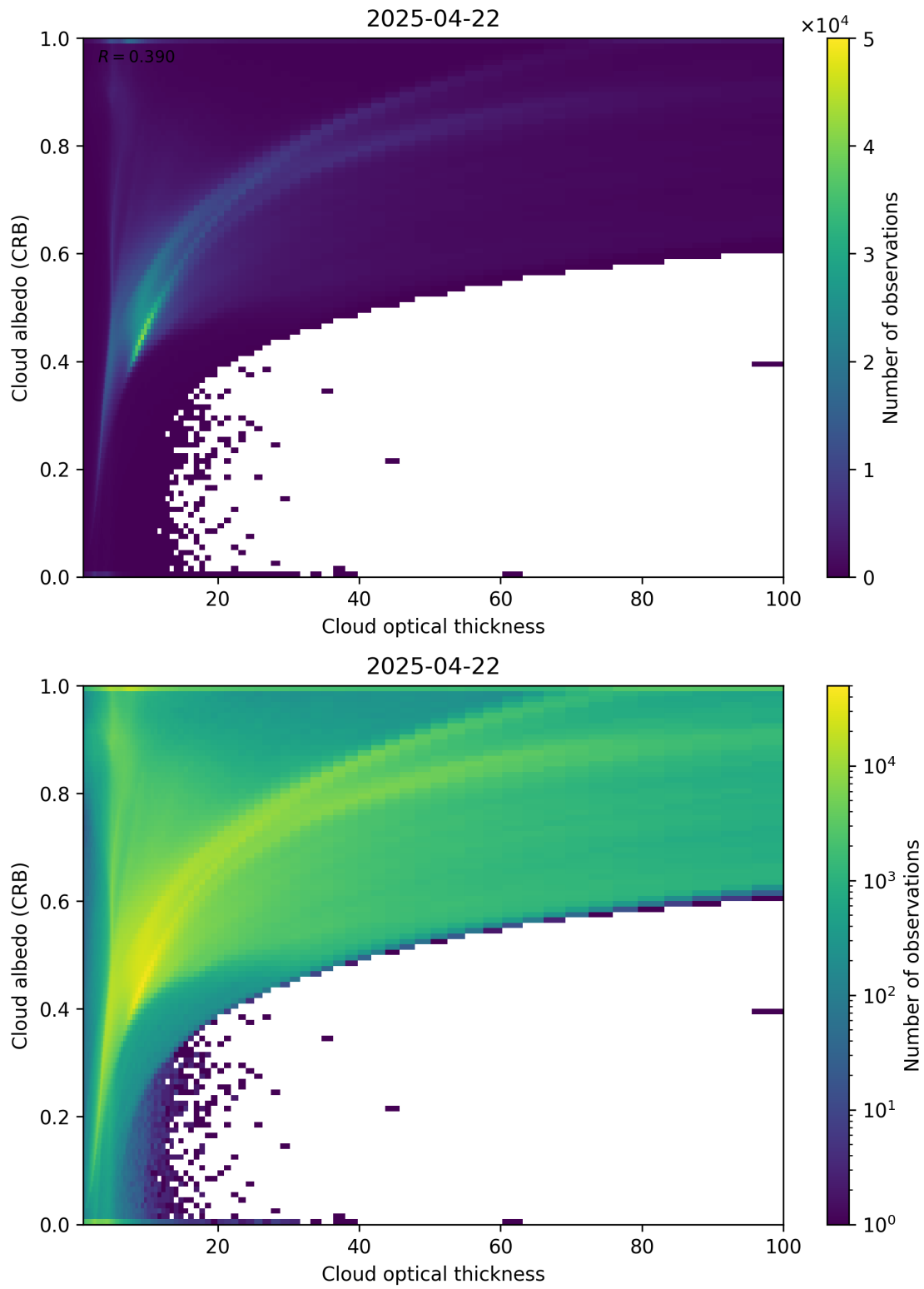
Figure 82: Scatter density plot of “Cloud optical thickness” against “Cloud albedo (CRB)” for 2025-04-21 to 2025-04-23.
