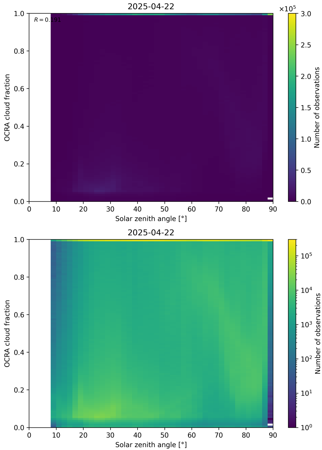
Figure 100: Scatter density plot of “Solar zenith angle” against “OCRA cloud fraction” for 2025-04-21 to 2025-04-23.
