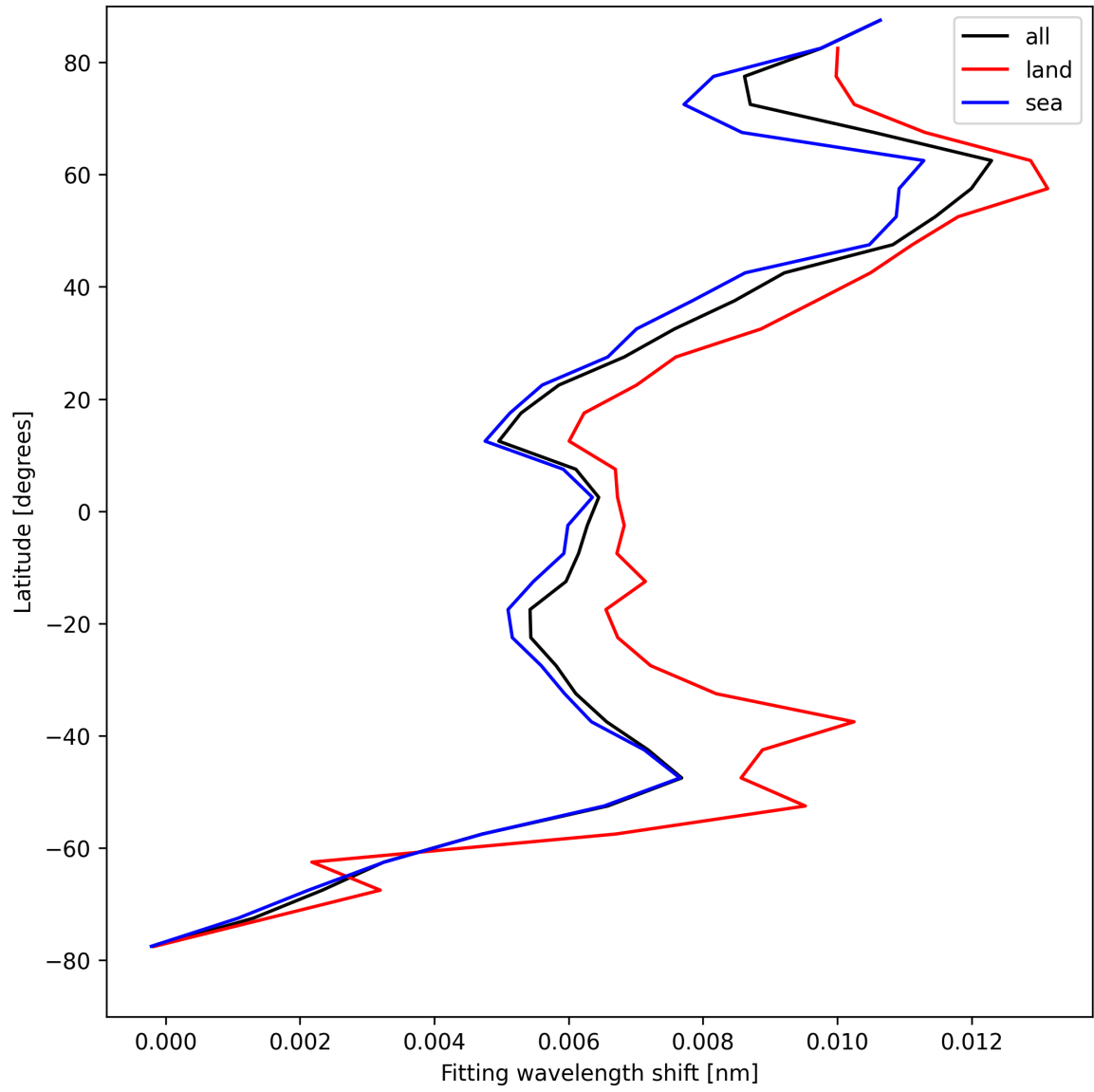
Figure 33: Zonal average of “Fitting wavelength shift” for 2025-04-21 to 2025-04-23.
