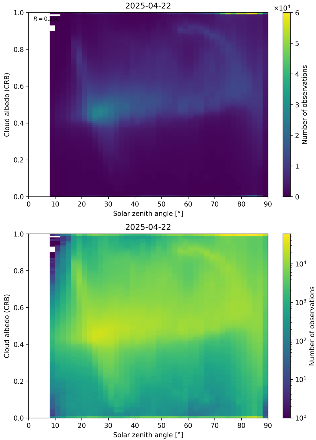
Figure 98: Scatter density plot of “Solar zenith angle” against “Cloud albedo (CRB)” for 2025-04-21 to 2025-04-23.
