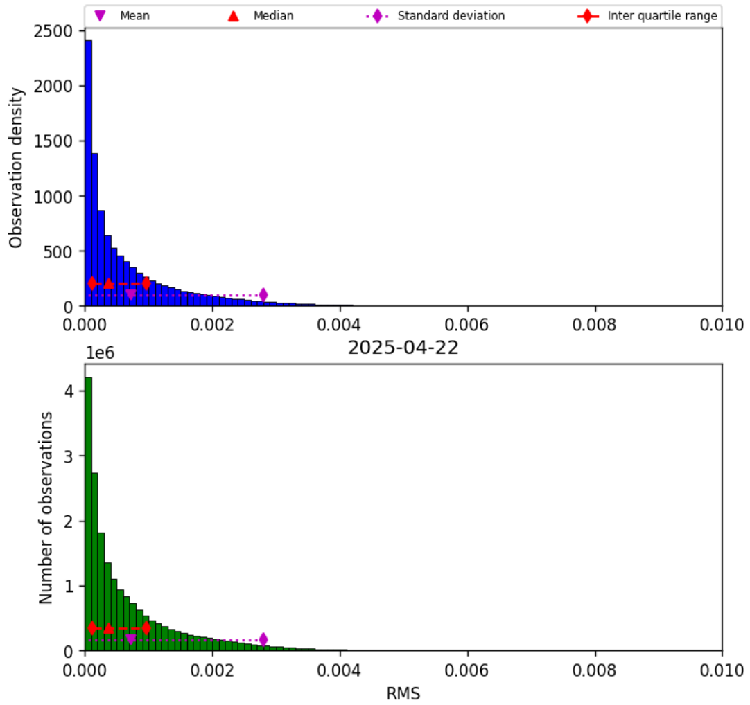
Figure 47: Histogram of “RMS” for 2025-04-21 to 2025-04-23
