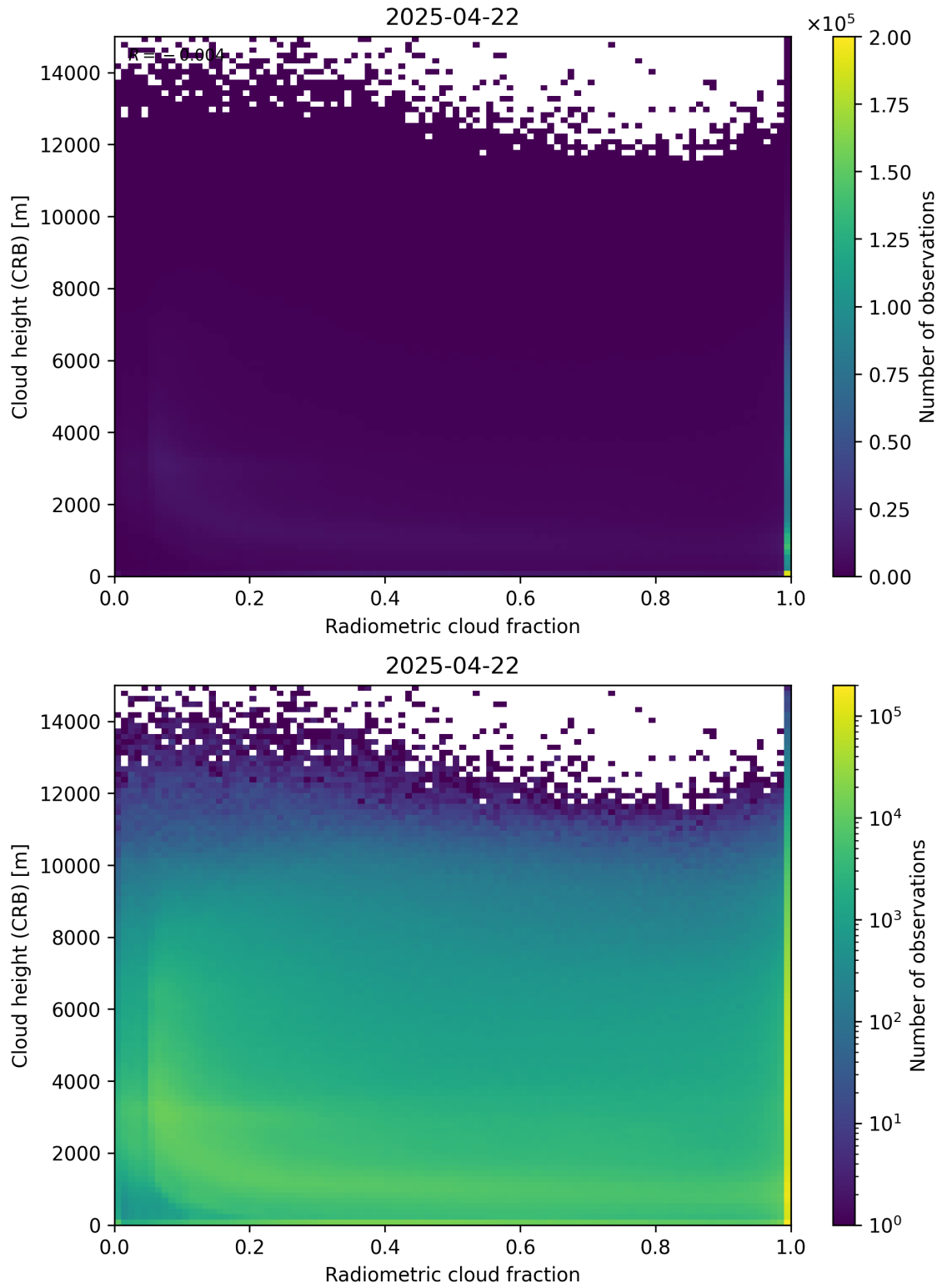
Figure 74: Scatter density plot of “Radiometric cloud fraction” against “Cloud height (CRB)” for 2025-04-21 to 2025-04-23.
