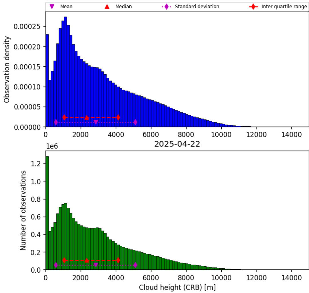
Figure 43: Histogram of “Cloud height (CRB)” for 2025-04-21 to 2025-04-23
