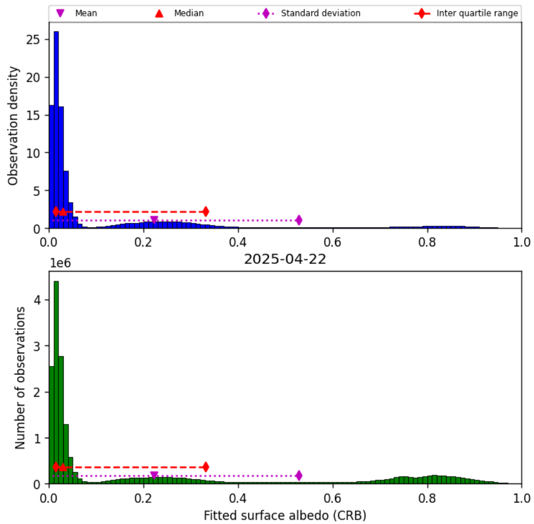
Figure 46: Histogram of “Fitted surface albedo (CRB)” for 2025-04-21 to 2025-04-23
