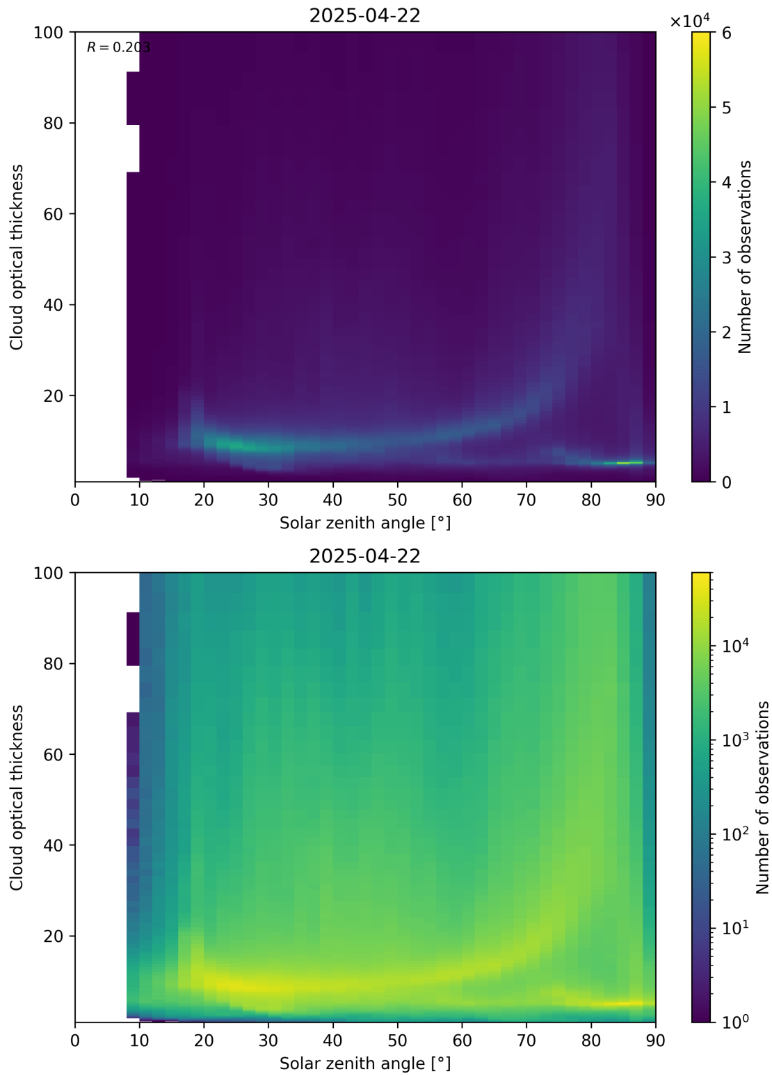
Figure 103: Scatter density plot of “Solar zenith angle” against “Cloud optical thickness” for 2025-04-21 to 2025-04-23.
