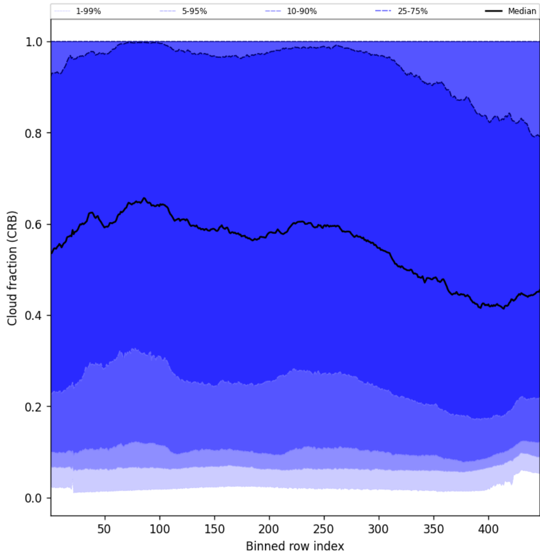
Figure 58: Along track statistics of “Cloud fraction (CRB)” for 2025-04-21 to 2025-04-23
