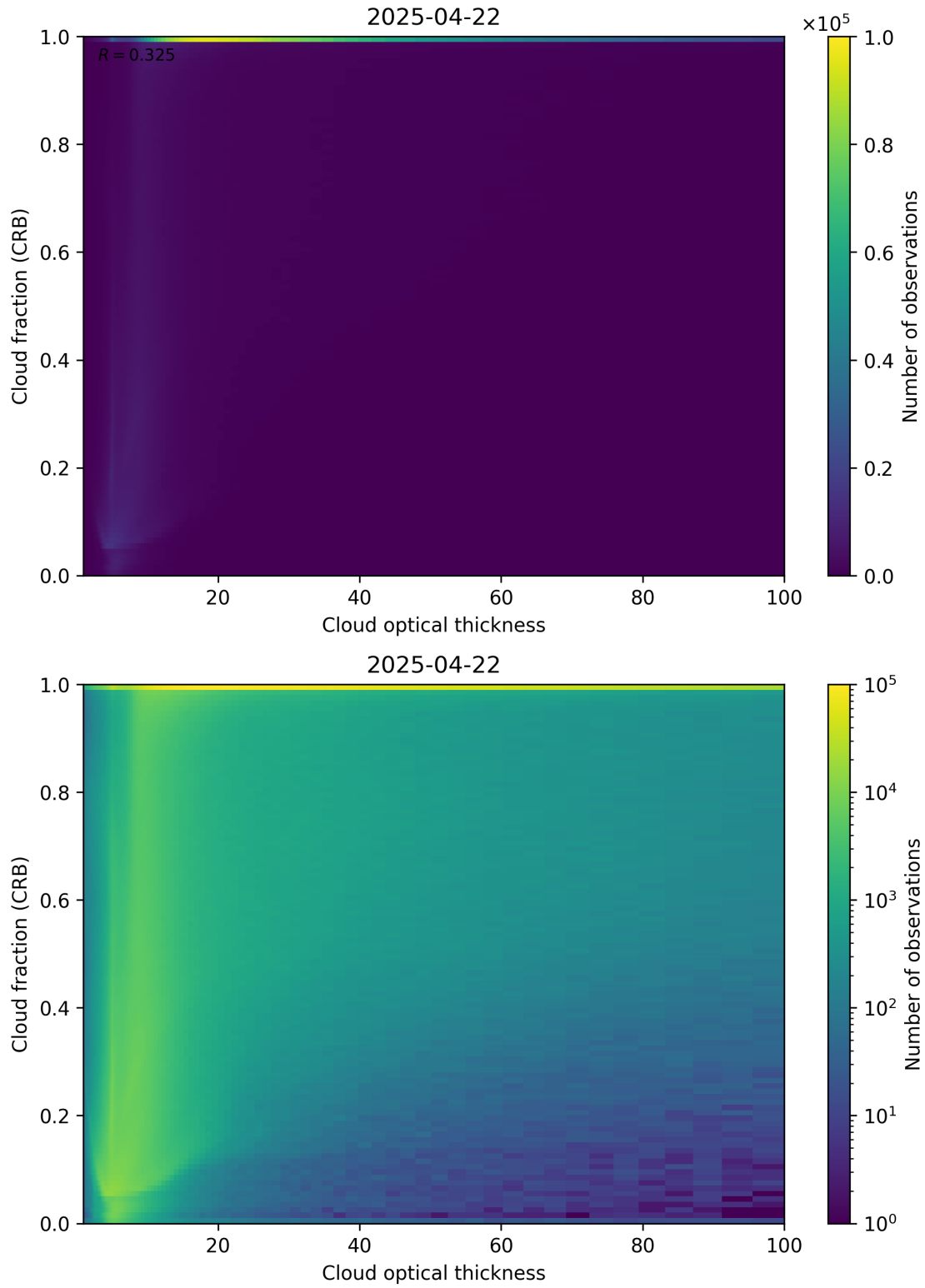
Figure 84: Scatter density plot of “Cloud optical thickness” against “Cloud fraction (CRB)” for 2025-04-21 to 2025-04-23.
