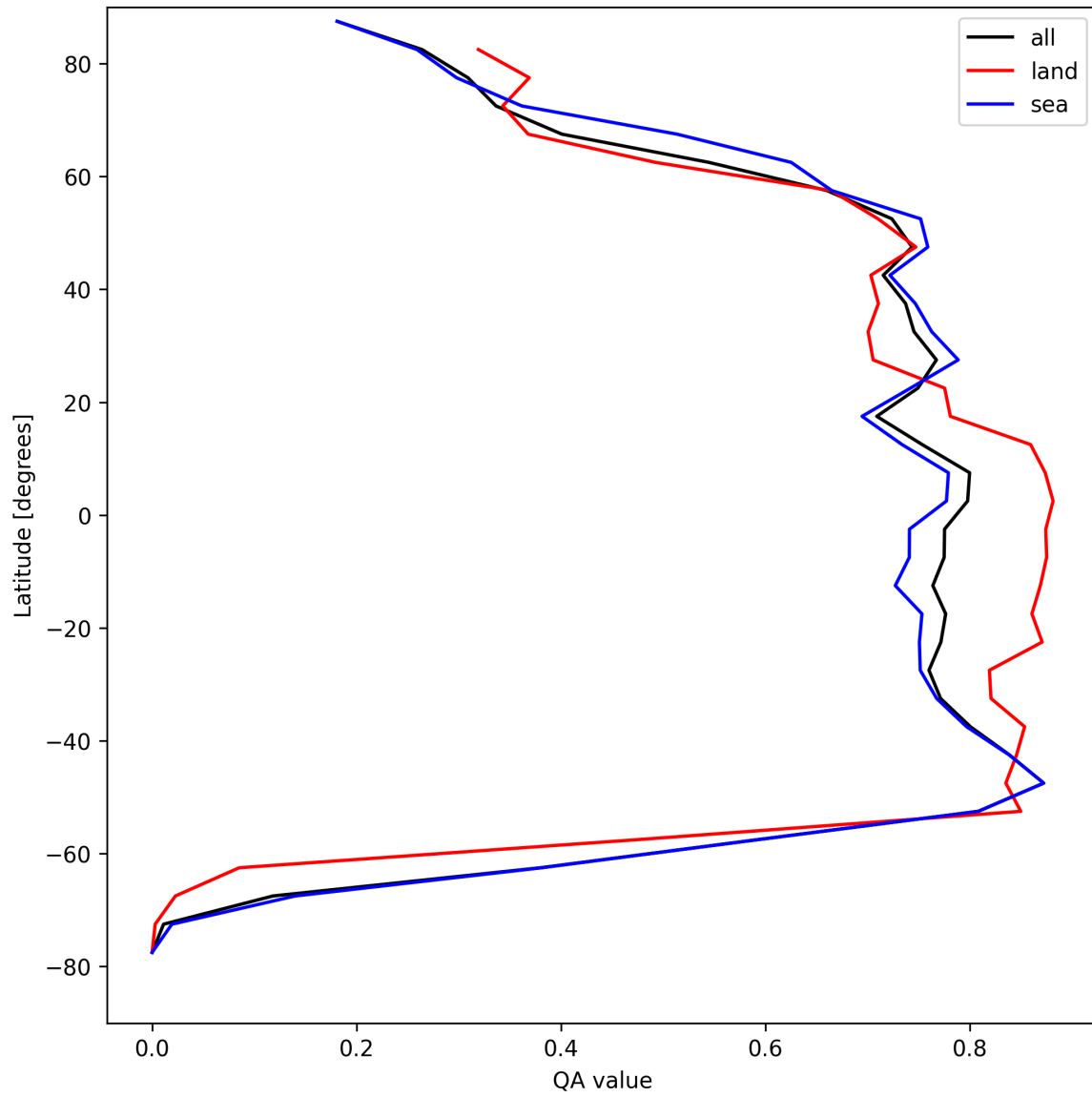
Figure 22: Zonal average of “QA value” for 2025-04-21 to 2025-04-23.
