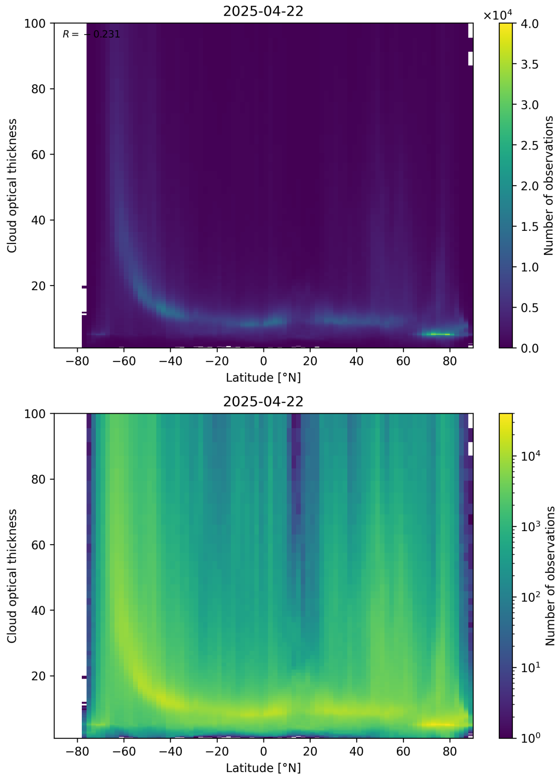
Figure 96: Scatter density plot of “Latitude” against “Cloud optical thickness” for 2025-04-21 to 2025-04-23.
