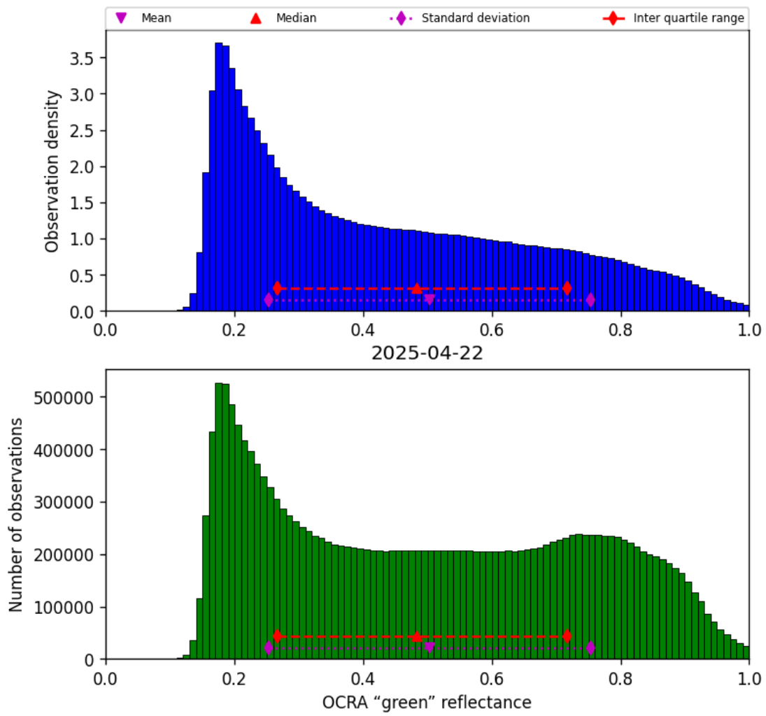
Figure 52: Histogram of “OCRA “green” reflectance” for 2025-04-21 to 2025-04-23
