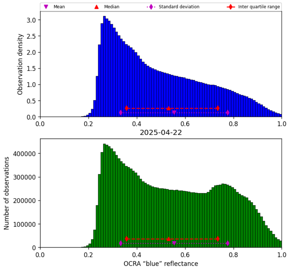
Figure 51: Histogram of “OCRA “blue” reflectance” for 2025-04-21 to 2025-04-23
