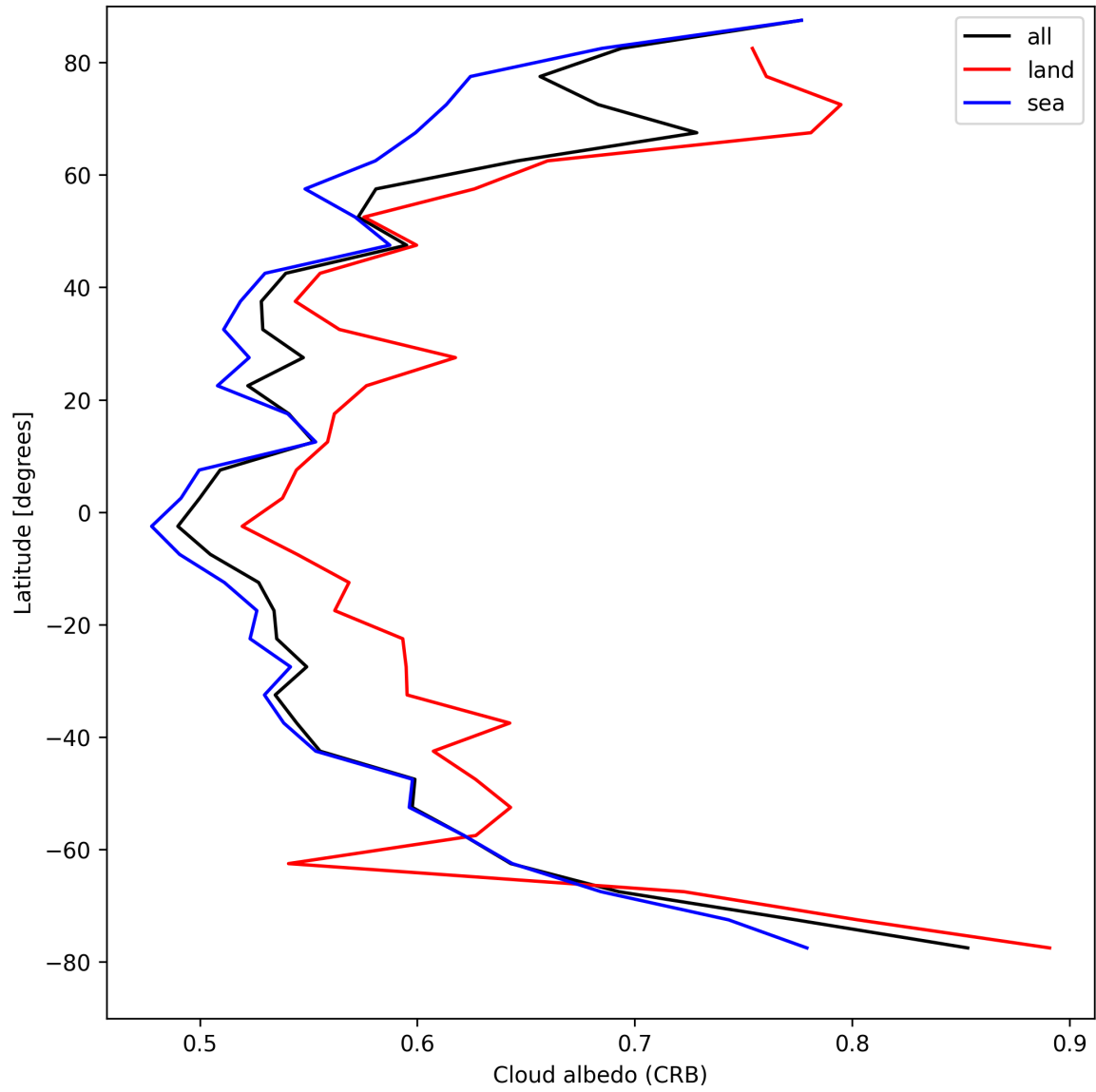
Figure 28: Zonal average of “Cloud albedo (CRB)” for 2025-04-21 to 2025-04-23.
