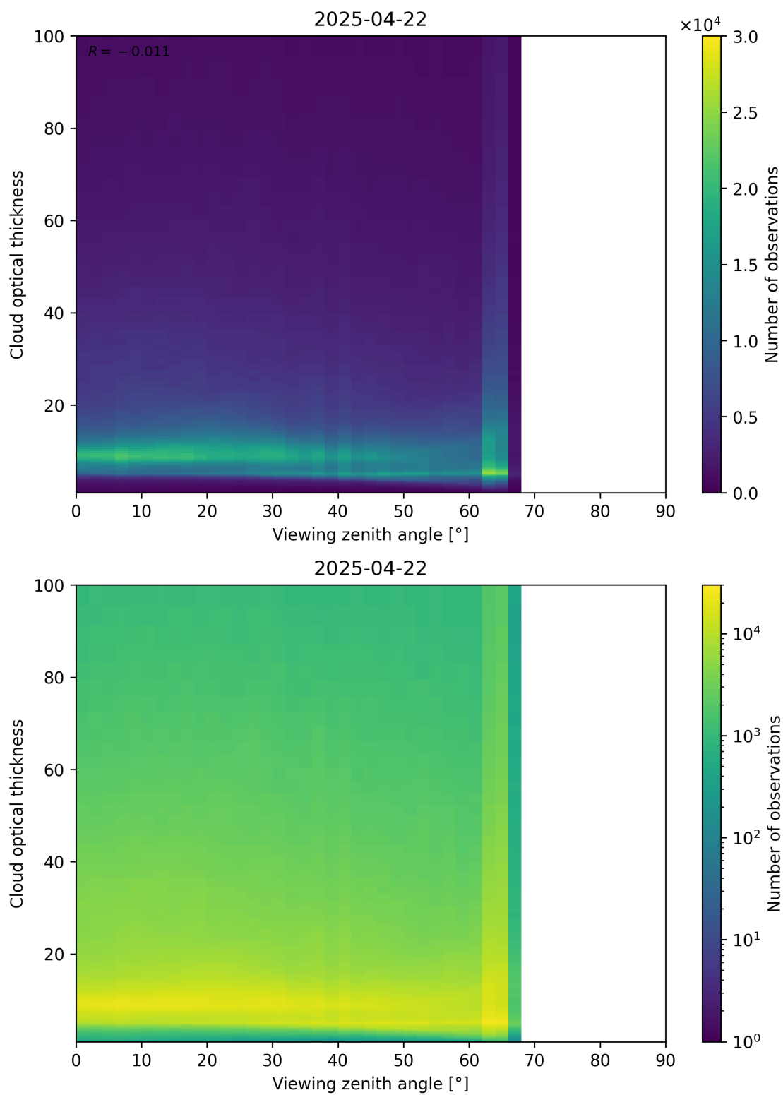
Figure 111: Scatter density plot of “Viewing zenith angle” against “Cloud optical thickness” for 2025-04-21 to 2025-04-23.
