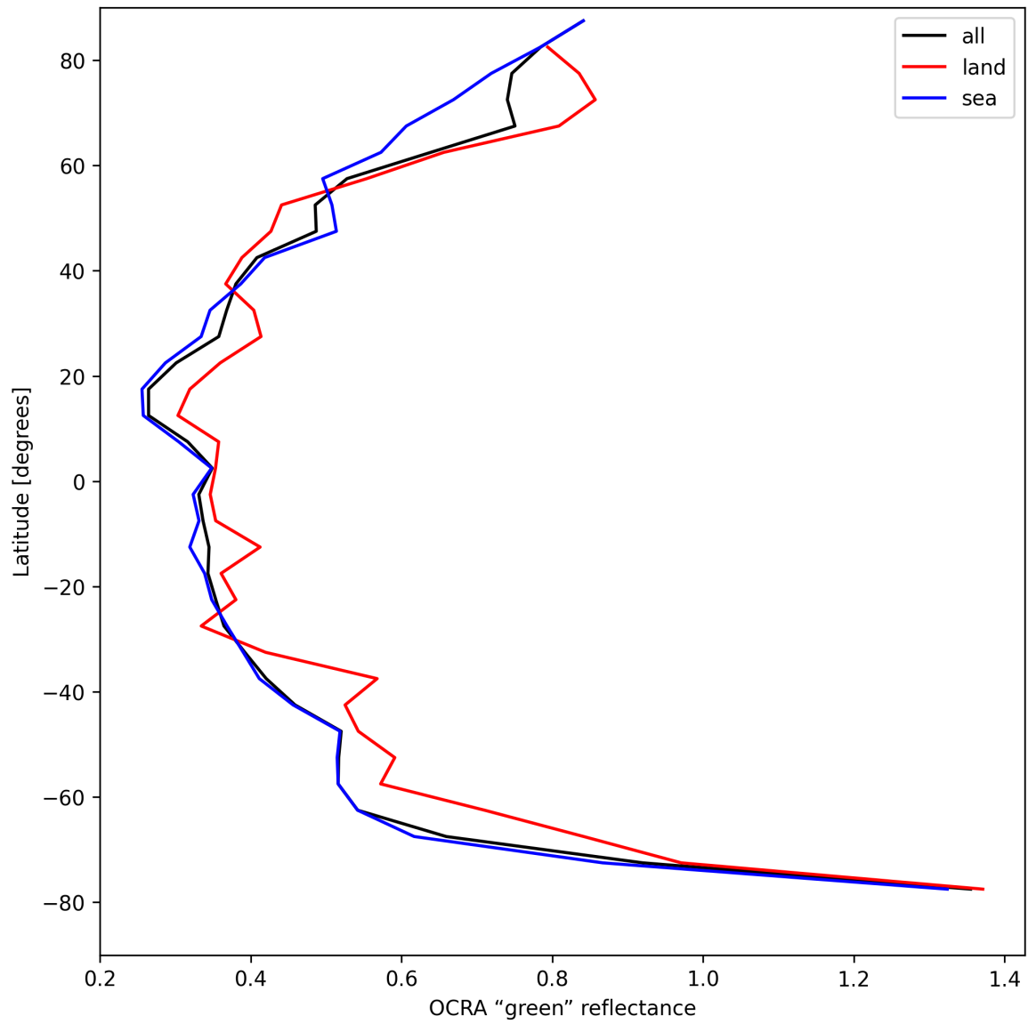
Figure 36: Zonal average of “OCRA “green” reflectance” for 2025-04-21 to 2025-04-23.
