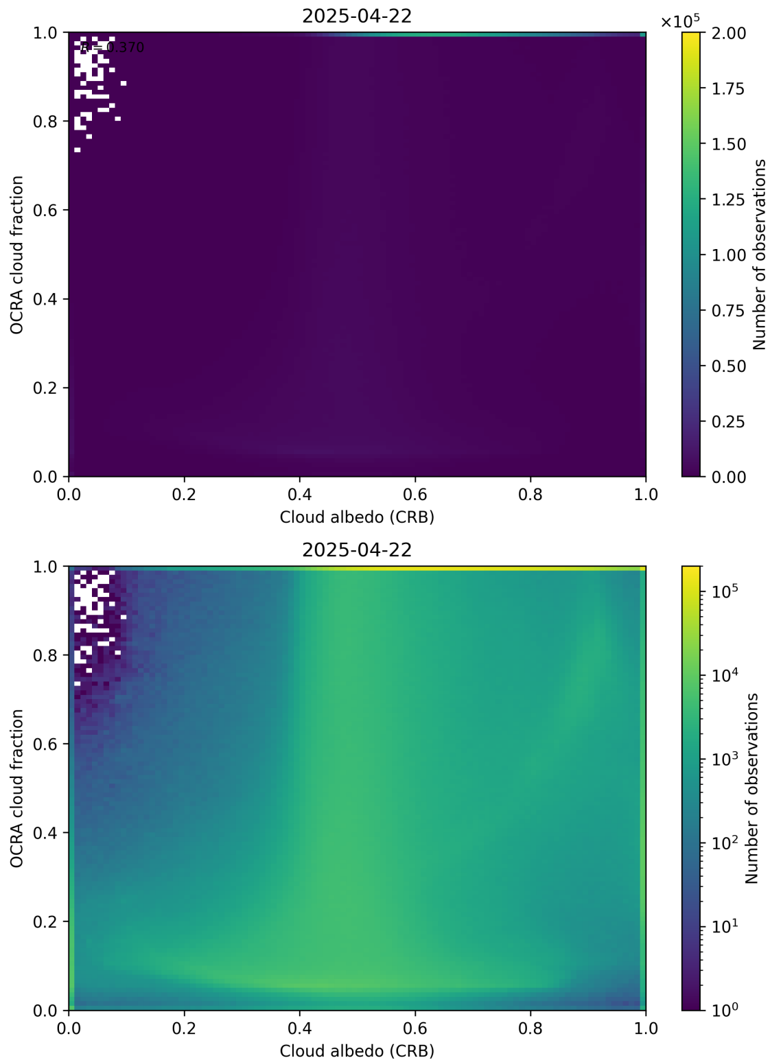
Figure 70: Scatter density plot of “Cloud albedo (CRB)” against “OCRA cloud fraction” for 2025-04-21 to 2025-04-23.
