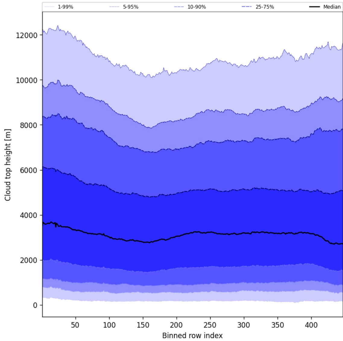
Figure 56: Along track statistics of “Cloud top height” for 2025-04-21 to 2025-04-23
