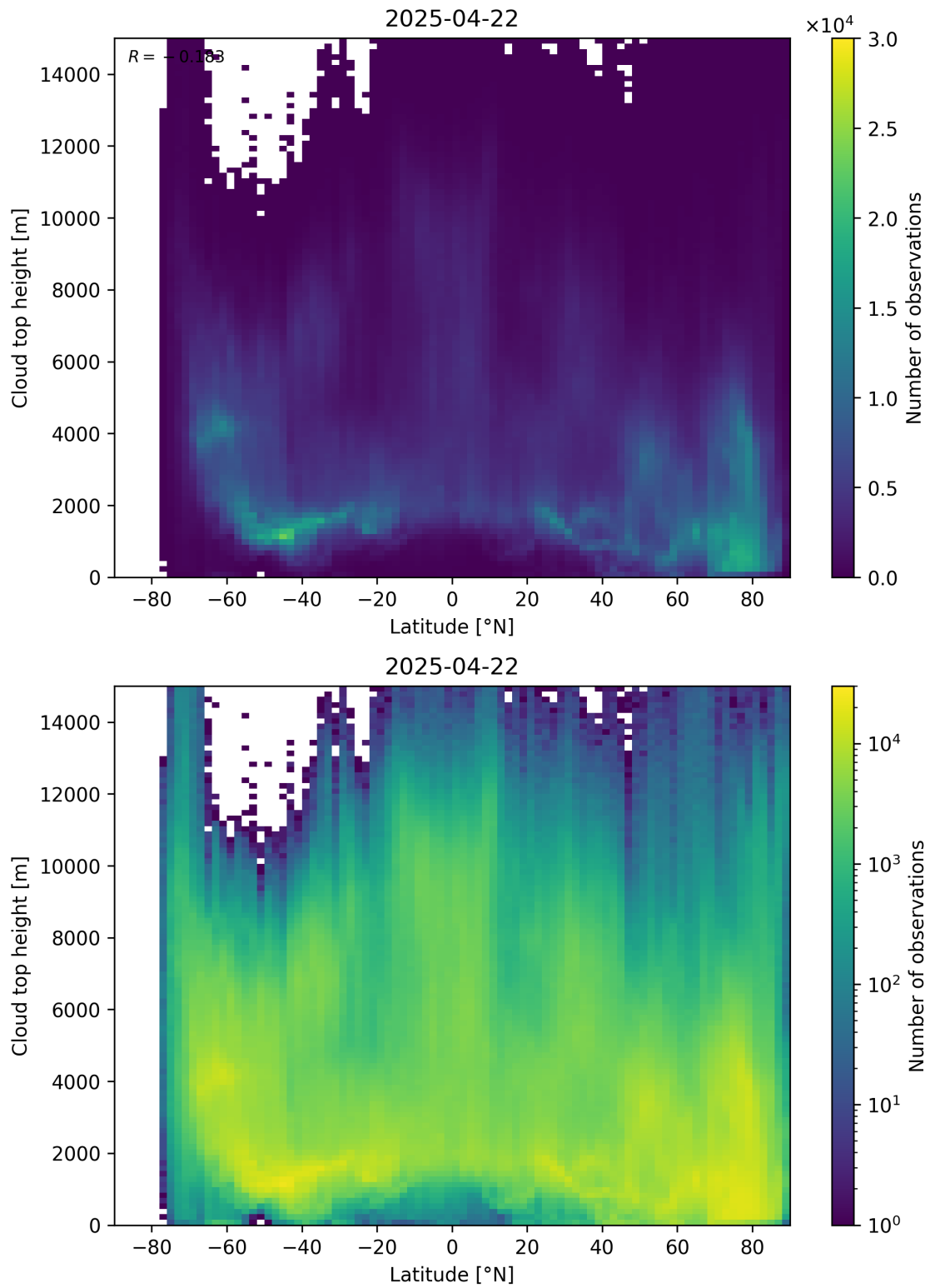
Figure 97: Scatter density plot of “Latitude” against “Cloud top height” for 2025-04-21 to 2025-04-23.
