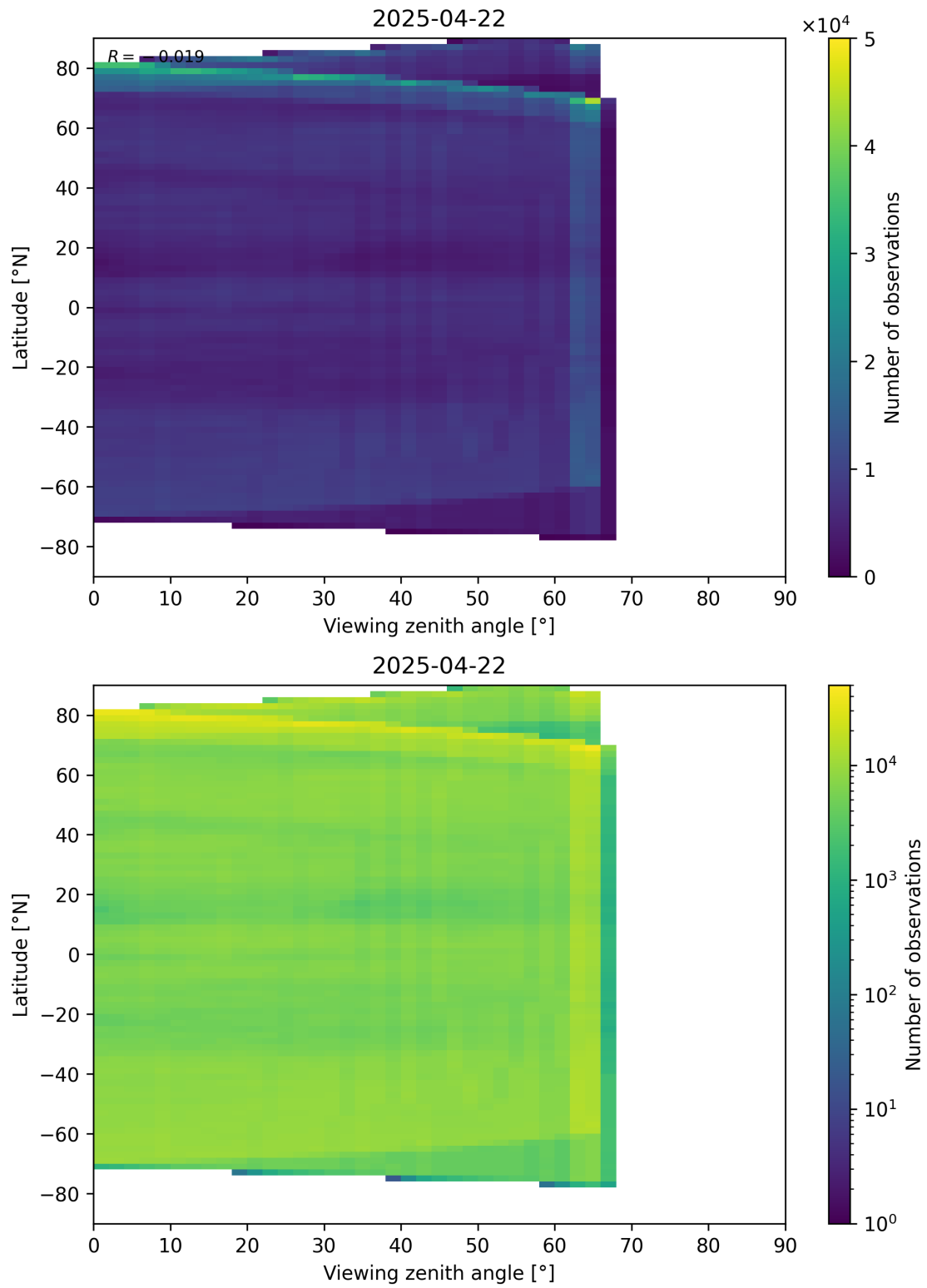
Figure 113: Scatter density plot of “Viewing zenith angle” against “Latitude” for 2025-04-21 to 2025-04-23.
