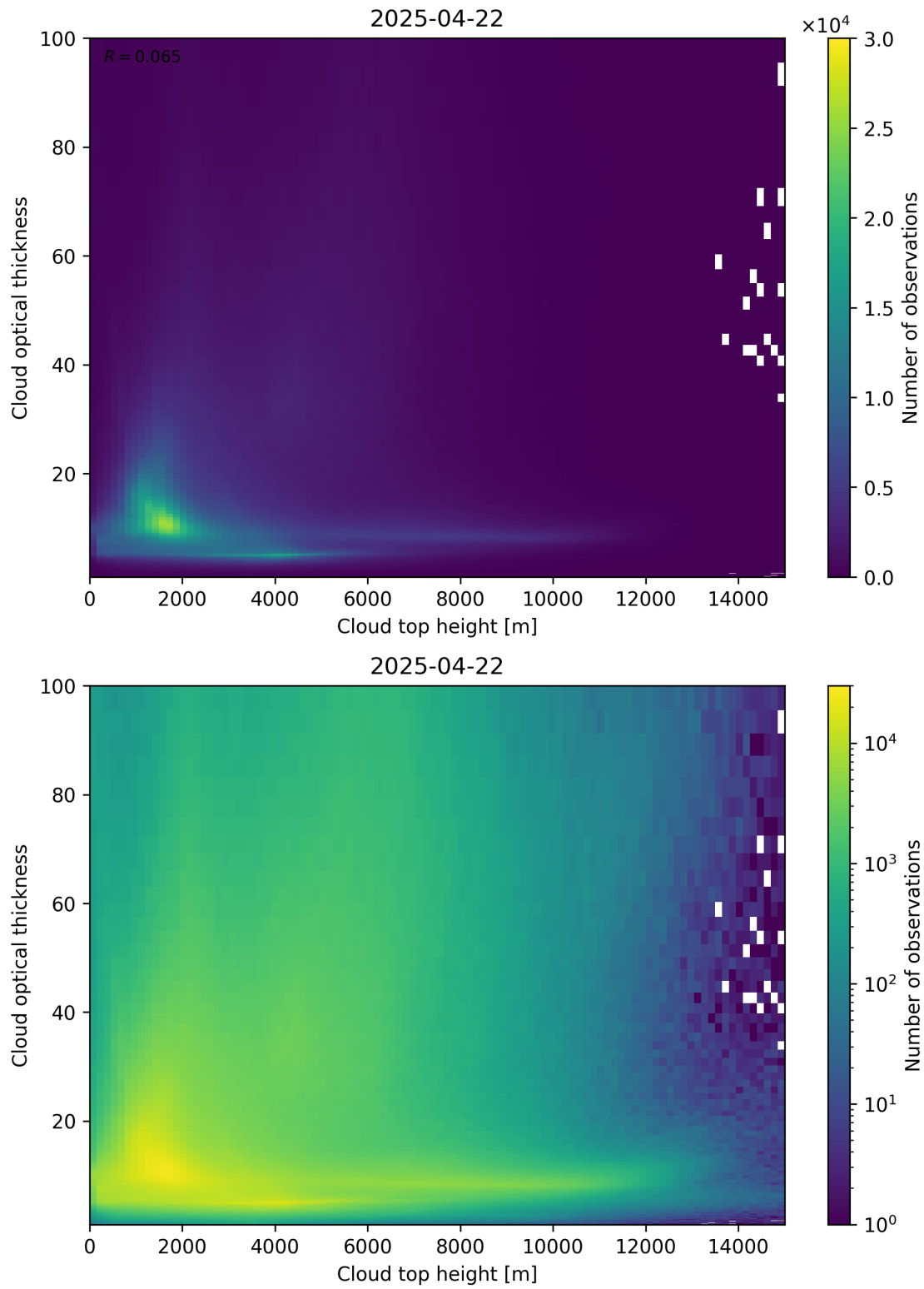
Figure 90: Scatter density plot of “Cloud top height” against “Cloud optical thickness” for 2025-04-21 to 2025-04-23.
