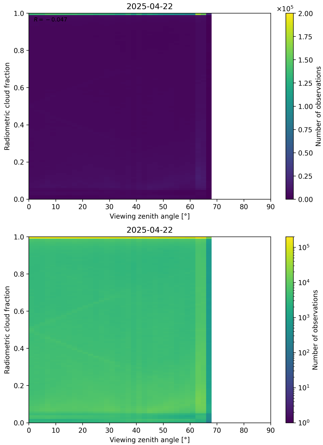
Figure 107: Scatter density plot of “Viewing zenith angle” against “Radiometric cloud fraction” for 2025-04-21 to 2025-04-23.
