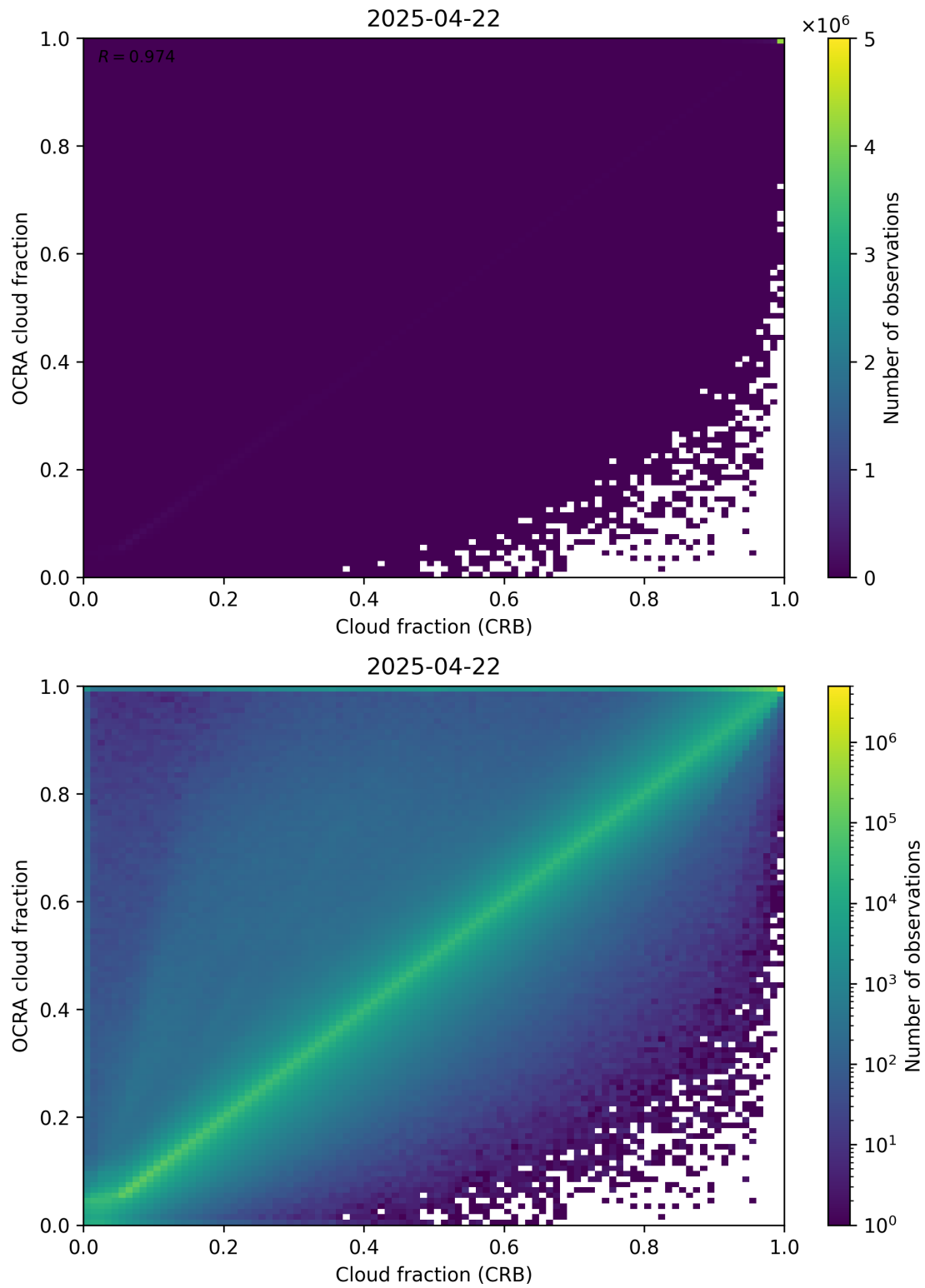
Figure 78: Scatter density plot of “Cloud fraction (CRB)” against “OCRA cloud fraction” for 2025-04-21 to 2025-04-23.
