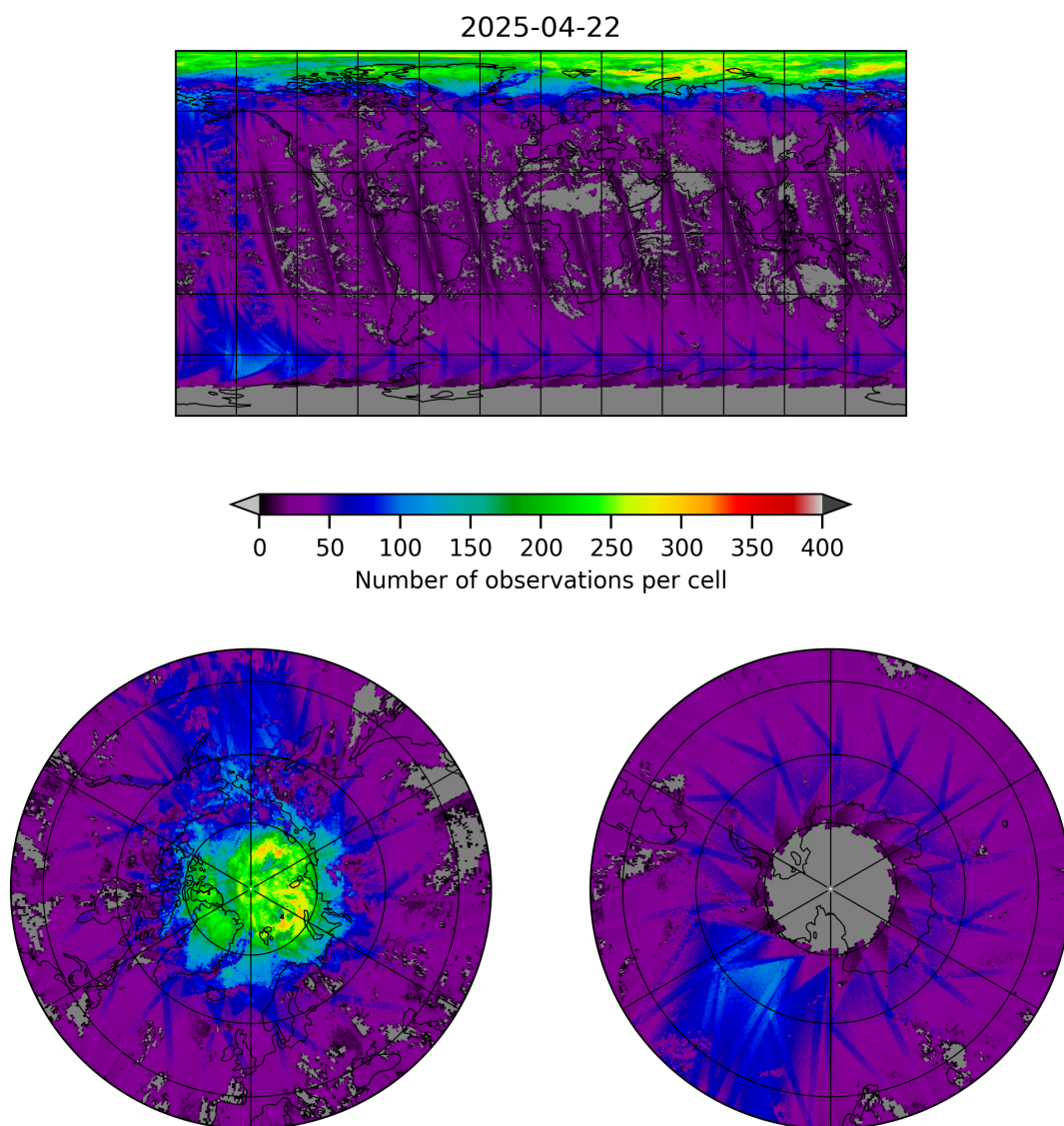
Figure 21: Map of the number of observations for 2025-04-21 to 2025-04-23
