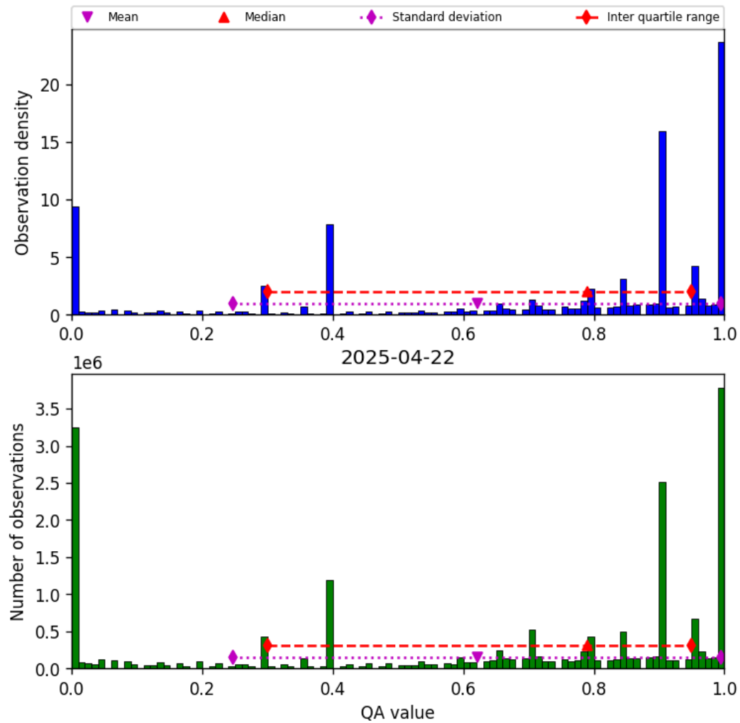
Figure 38: Histogram of “QA value” for 2025-04-21 to 2025-04-23
