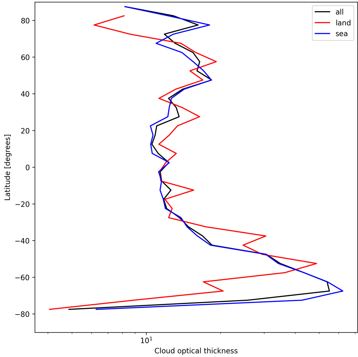
Figure 25: Zonal average of “Cloud optical thickness” for 2025-04-21 to 2025-04-23.
