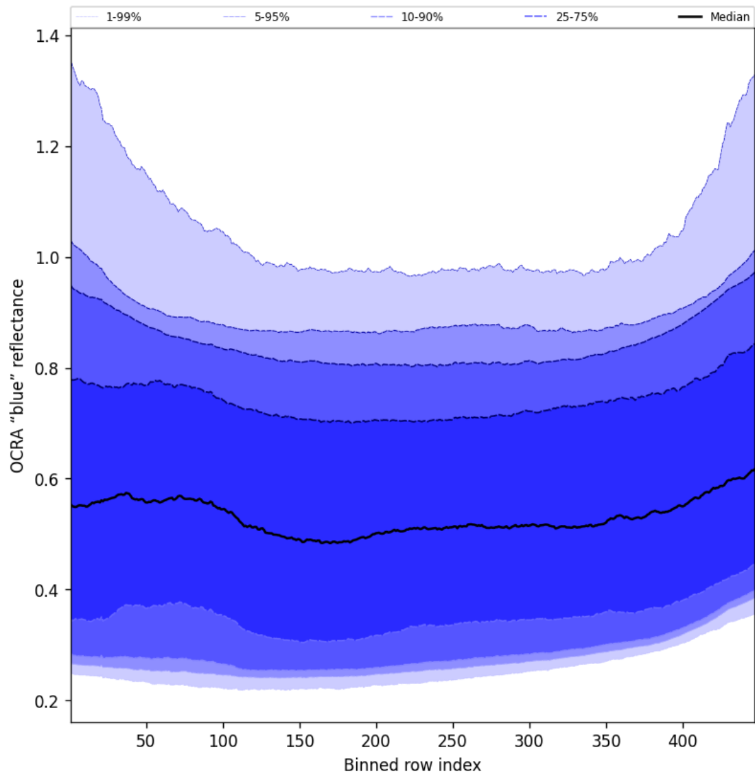
Figure 67: Along track statistics of “OCRA “blue” reflectance” for 2025-04-21 to 2025-04-23
