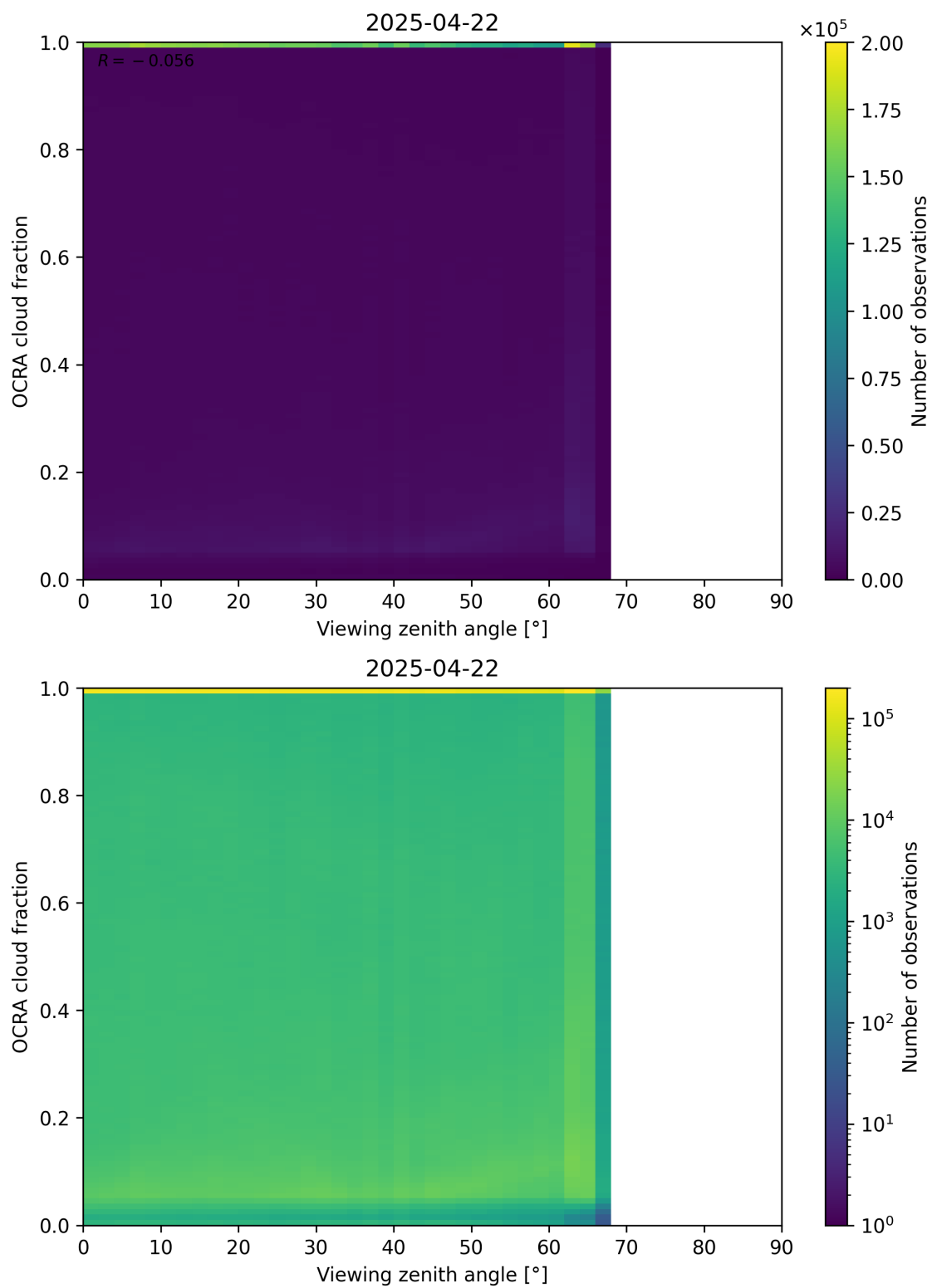
Figure 108: Scatter density plot of “Viewing zenith angle” against “OCRA cloud fraction” for 2025-04-21 to 2025-04-23.
