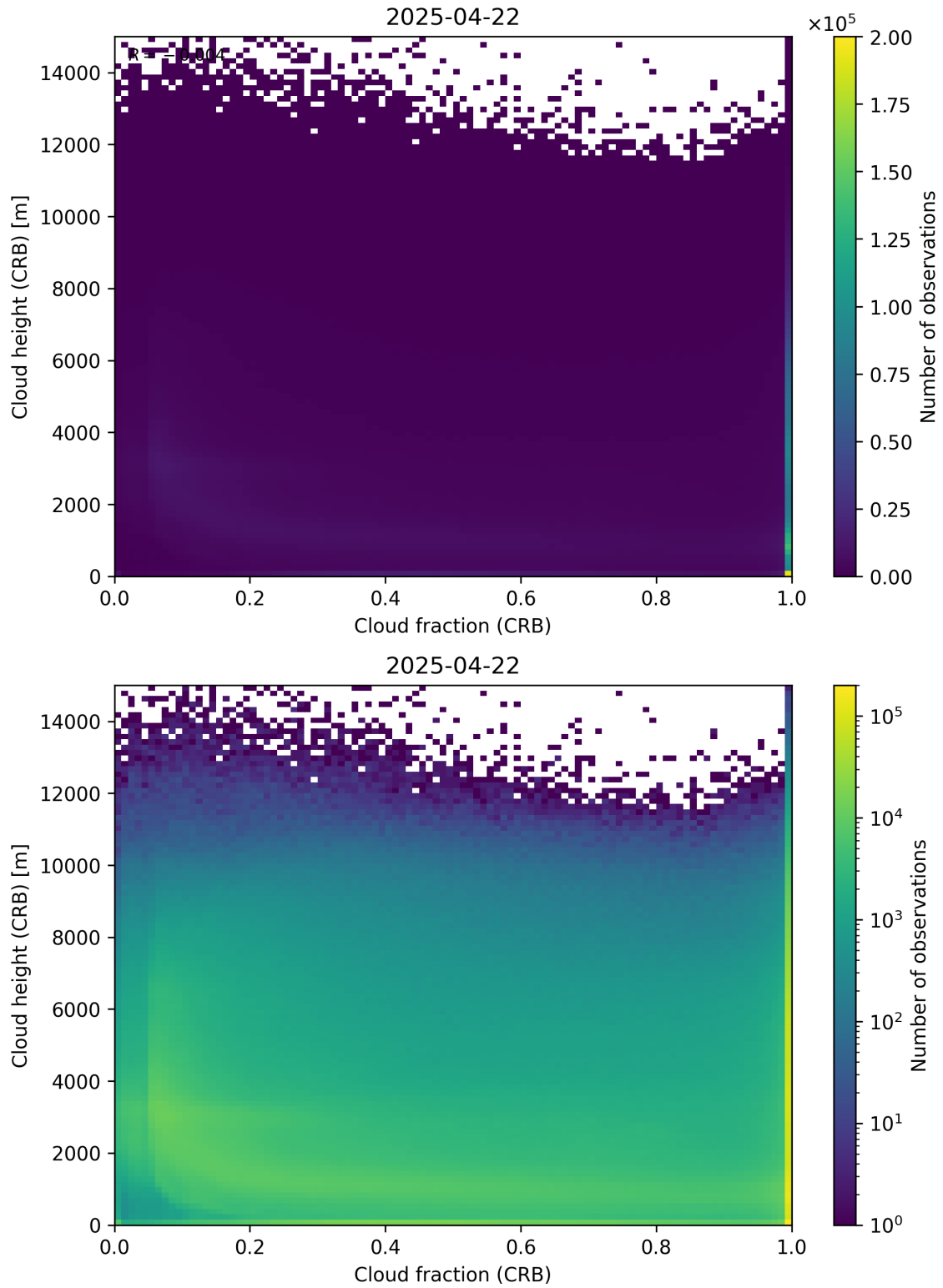
Figure 79: Scatter density plot of “Cloud fraction (CRB)” against “Cloud height (CRB)” for 2025-04-21 to 2025-04-23.
