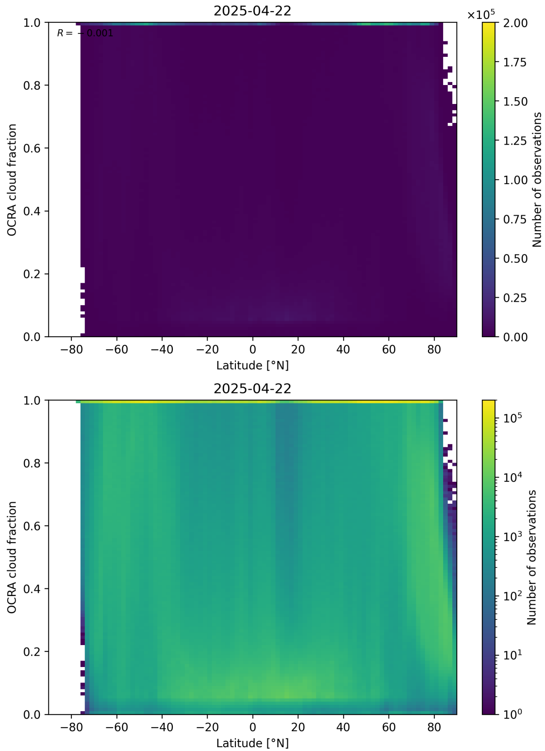
Figure 93: Scatter density plot of “Latitude” against “OCRA cloud fraction” for 2025-04-21 to 2025-04-23.
