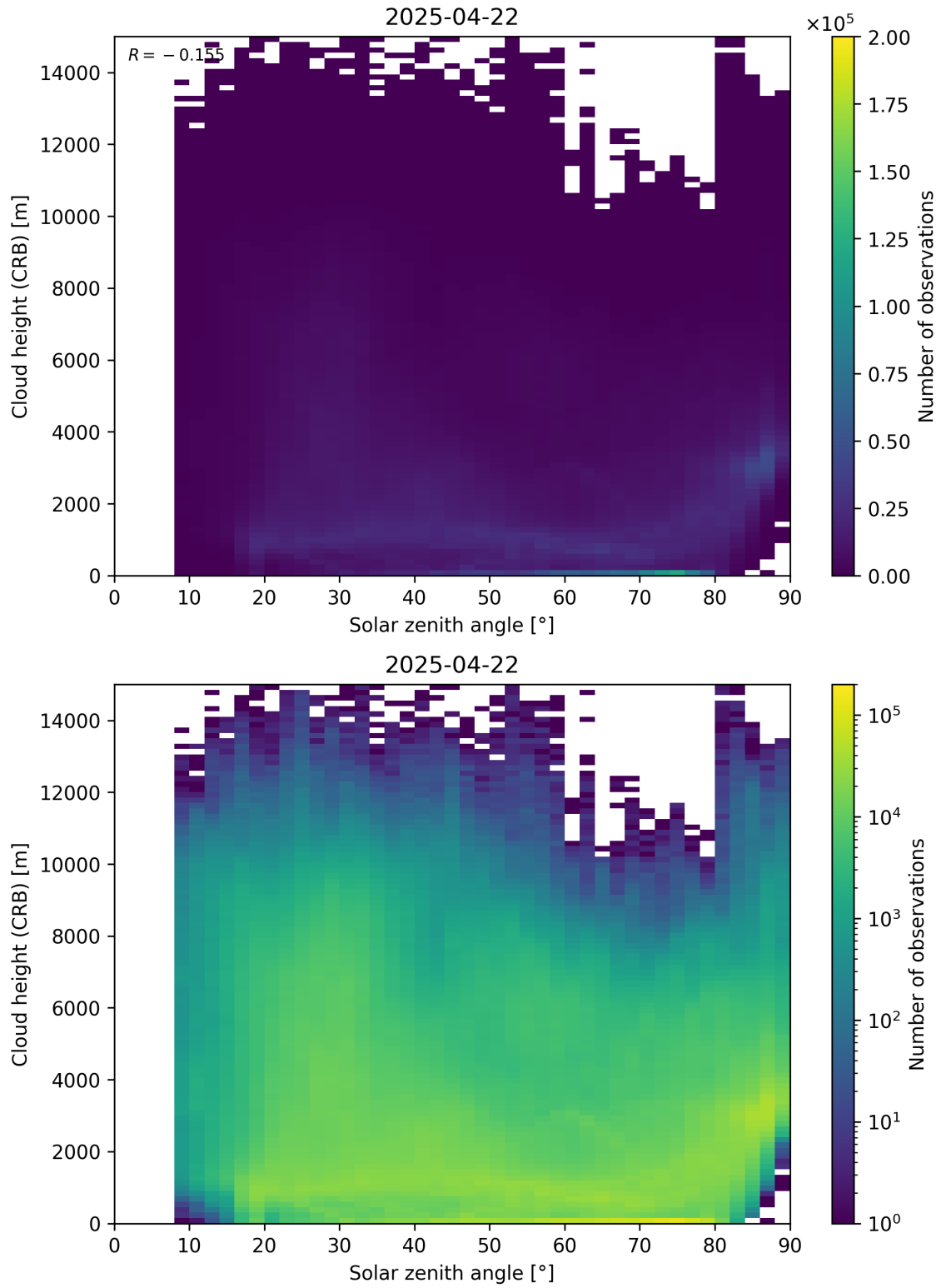
Figure 102: Scatter density plot of “Solar zenith angle” against “Cloud height (CRB)” for 2025-04-21 to 2025-04-23.
