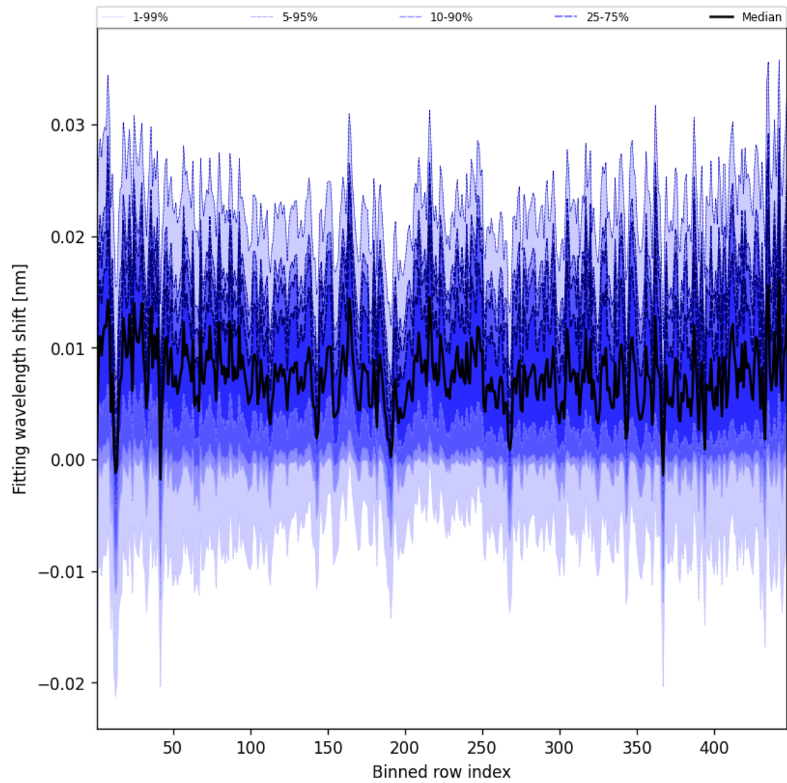
Figure 65: Along track statistics of “Fitting wavelength shift” for 2025-04-21 to 2025-04-23
