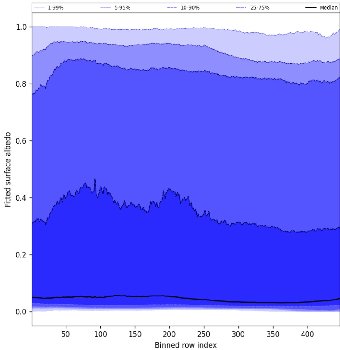
Figure 61: Along track statistics of “Fitted surface albedo” for 2025-04-21 to 2025-04-23
