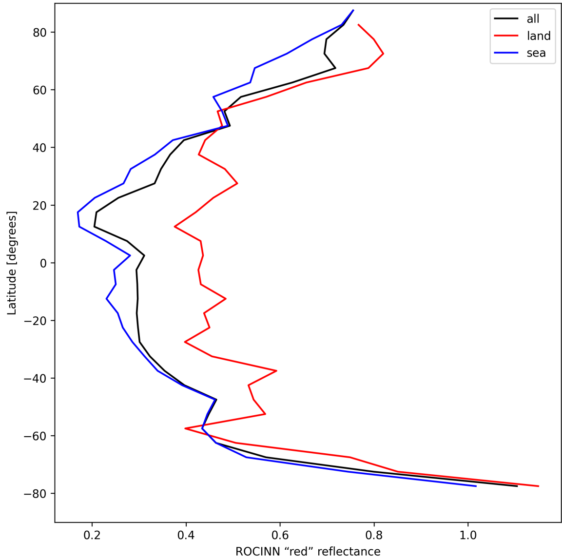
Figure 37: Zonal average of “ROCINN “red” reflectance” for 2025-04-21 to 2025-04-23.
