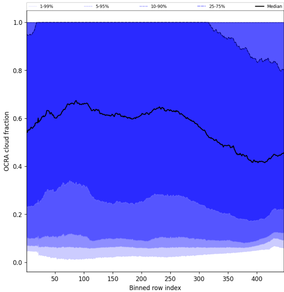
Figure 66: Along track statistics of “OCRA cloud fraction” for 2025-04-21 to 2025-04-23
