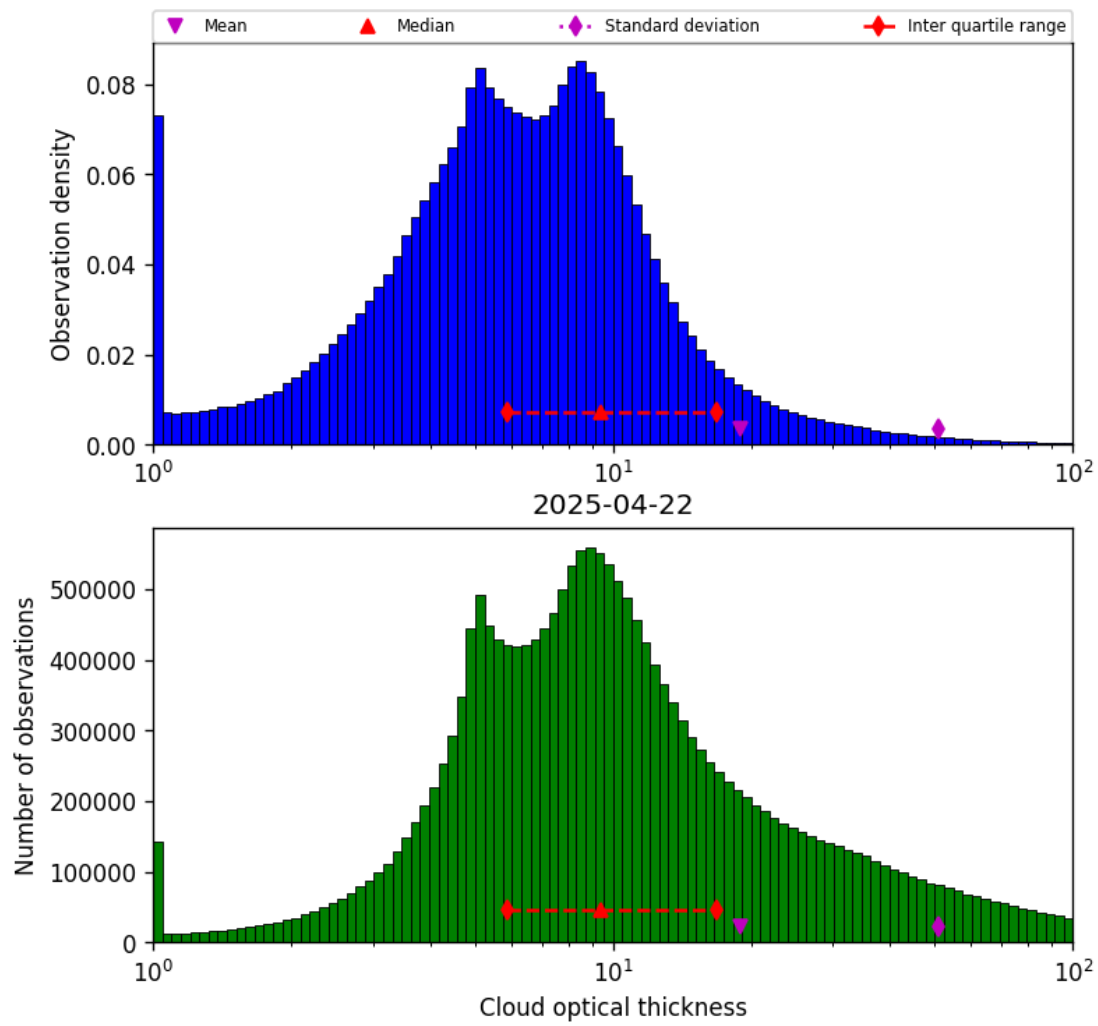
Figure 41: Histogram of “Cloud optical thickness” for 2025-04-21 to 2025-04-23
