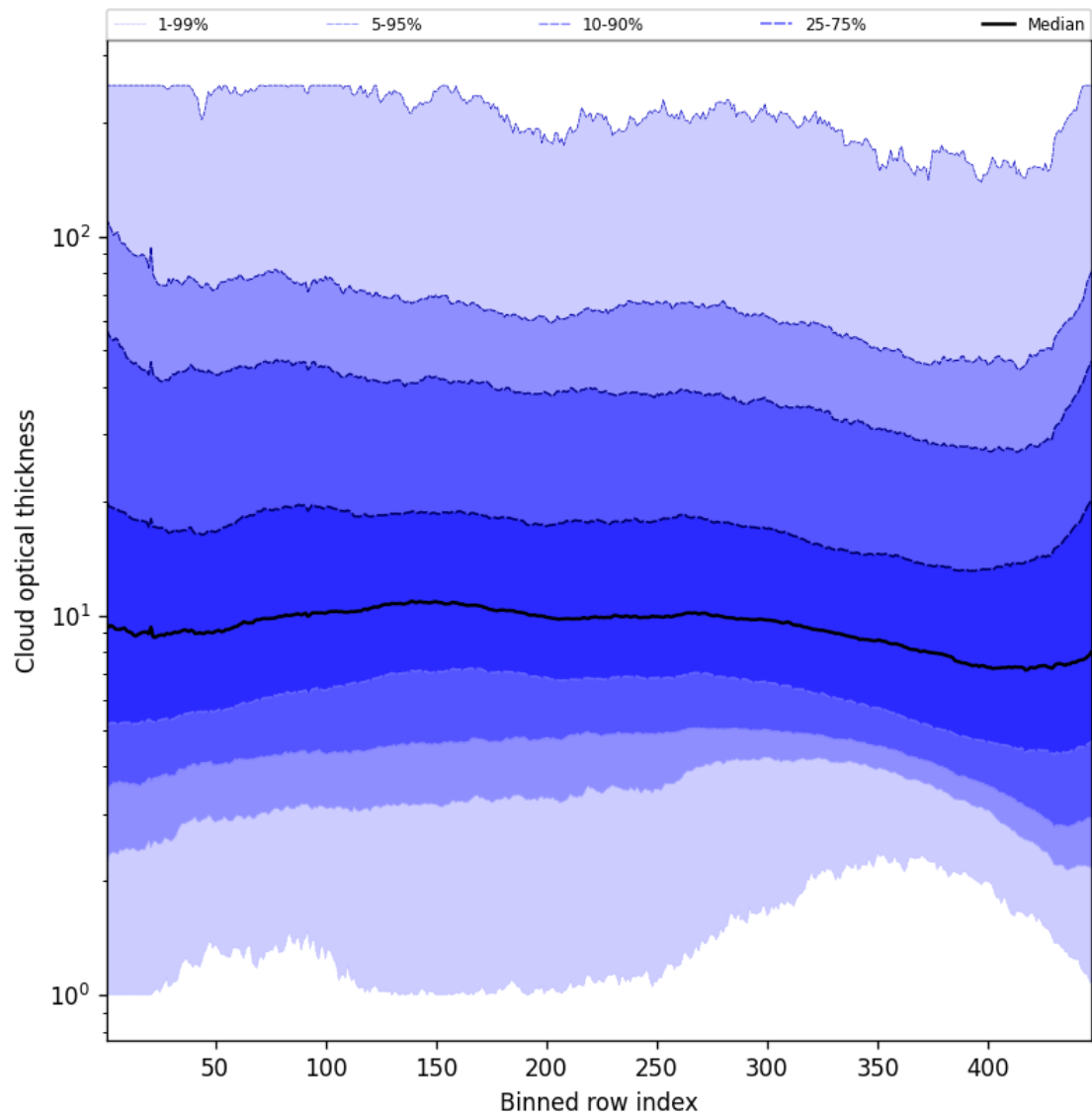
Figure 57: Along track statistics of “Cloud optical thickness” for 2025-04-21 to 2025-04-23
