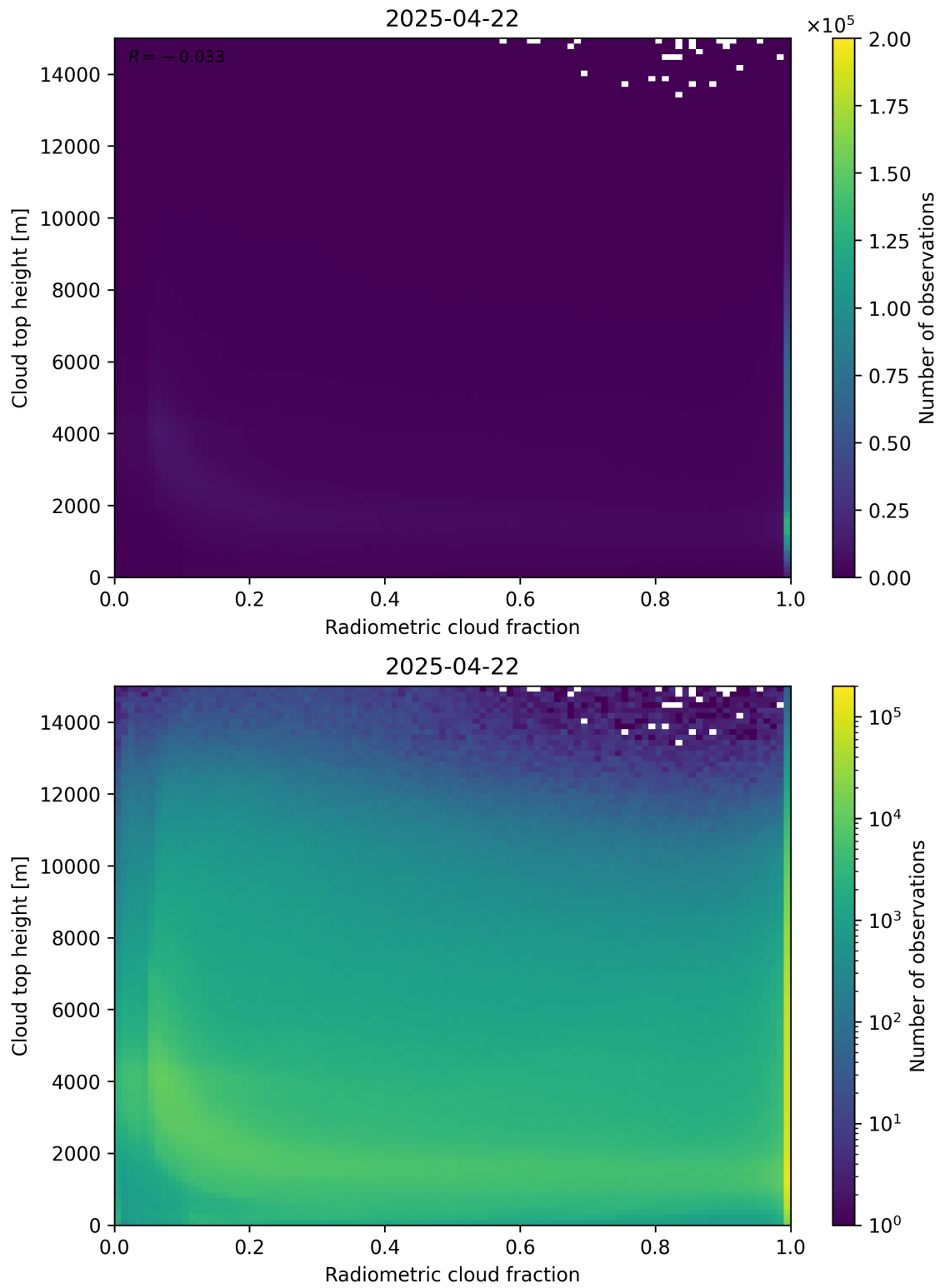
Figure 76: Scatter density plot of “Radiometric cloud fraction” against “Cloud top height” for 2025-04-21 to 2025-04-23.
