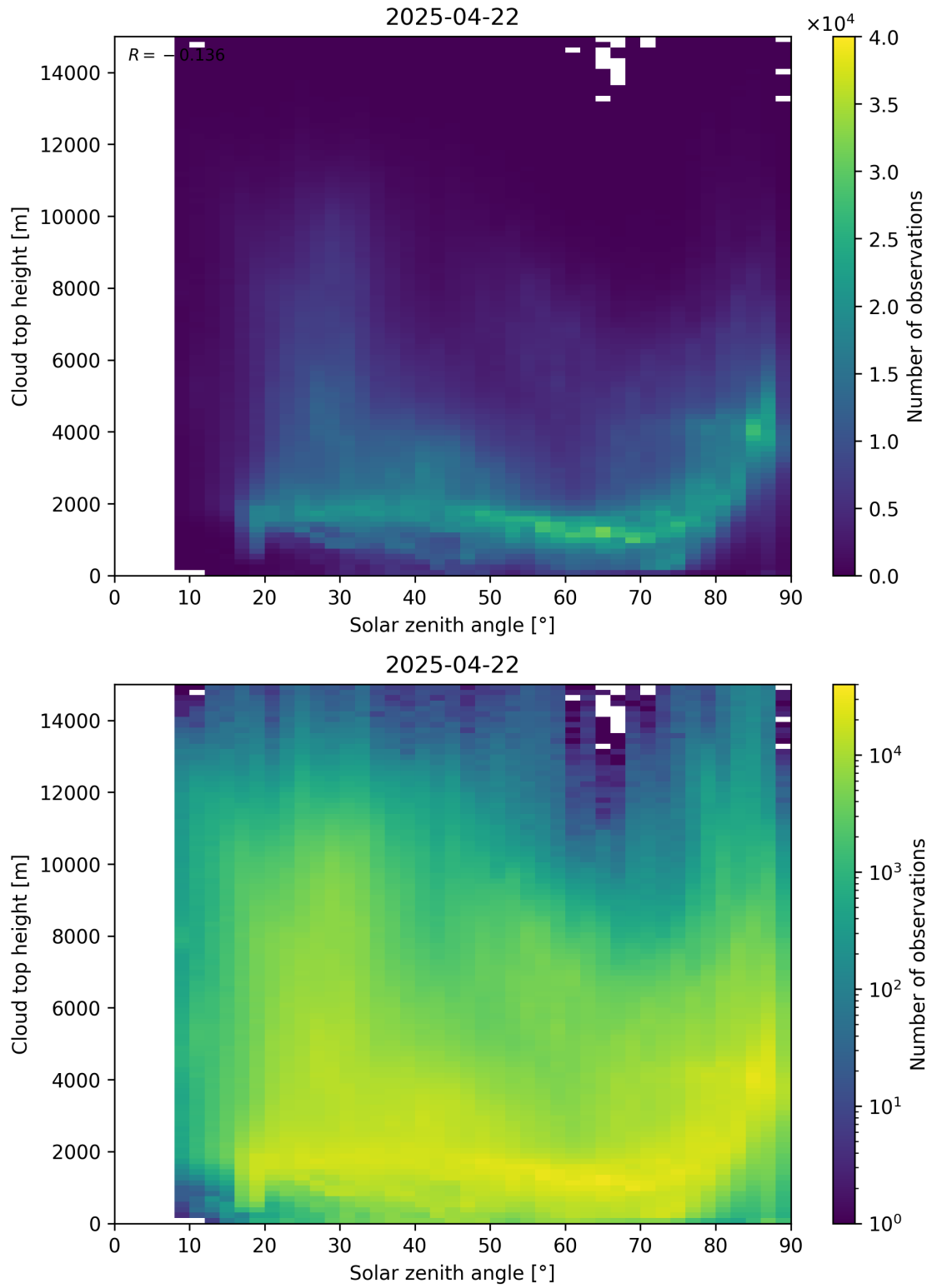
Figure 104: Scatter density plot of “Solar zenith angle” against “Cloud top height” for 2025-04-21 to 2025-04-23.
