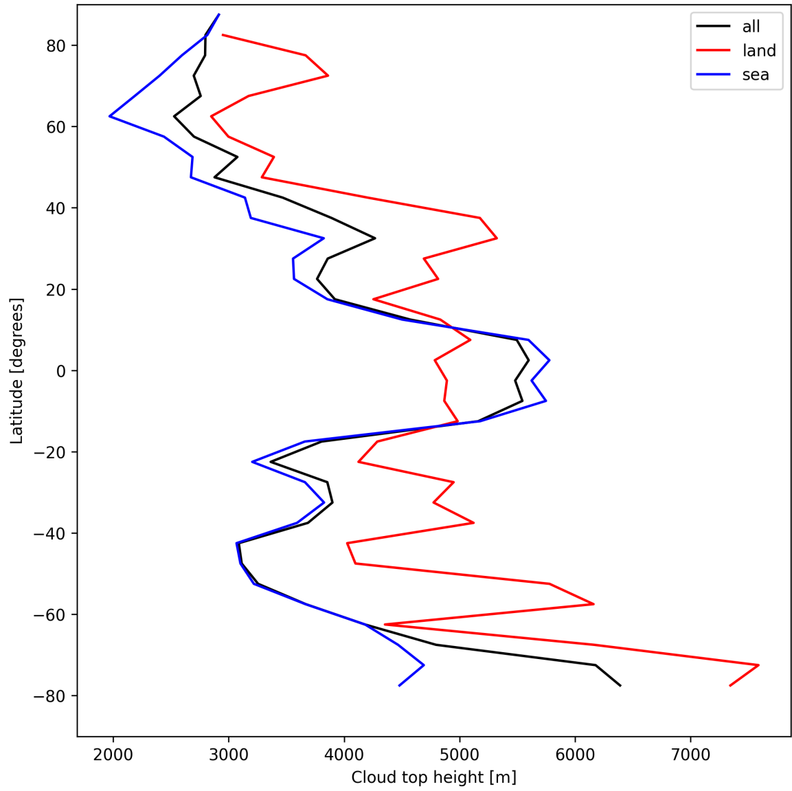
Figure 24: Zonal average of “Cloud top height” for 2025-04-21 to 2025-04-23.
