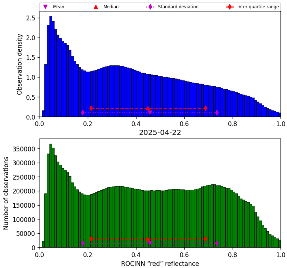
Figure 53: Histogram of “ROCINN “red” reflectance” for 2025-04-21 to 2025-04-23
