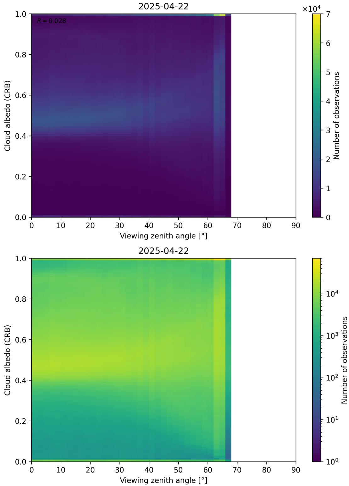
Figure 106: Scatter density plot of “Viewing zenith angle” against “Cloud albedo (CRB)” for 2025-04-21 to 2025-04-23.
