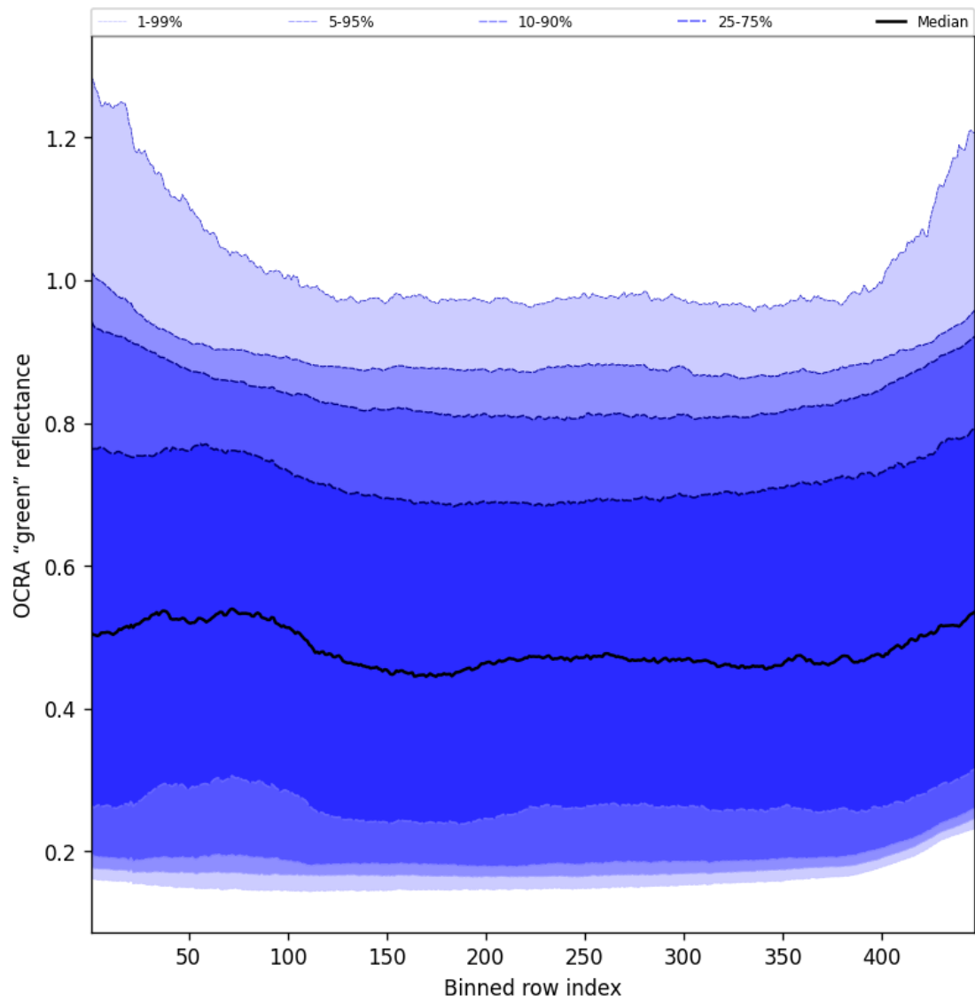
Figure 68: Along track statistics of “OCRA “green” reflectance” for 2025-04-21 to 2025-04-23
