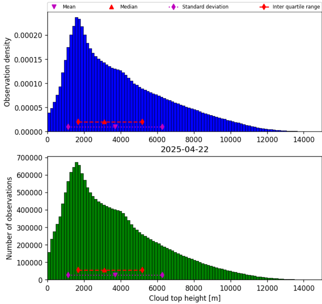
Figure 40: Histogram of “Cloud top height” for 2025-04-21 to 2025-04-23
