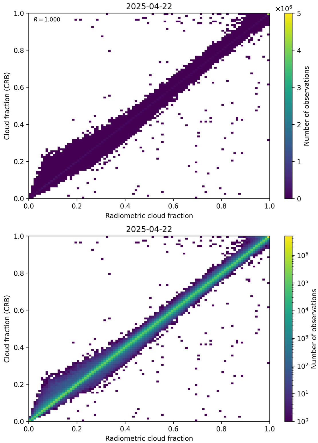
Figure 73: Scatter density plot of “Radiometric cloud fraction” against “Cloud fraction (CRB)” for 2025-04-21 to 2025-04-23.
