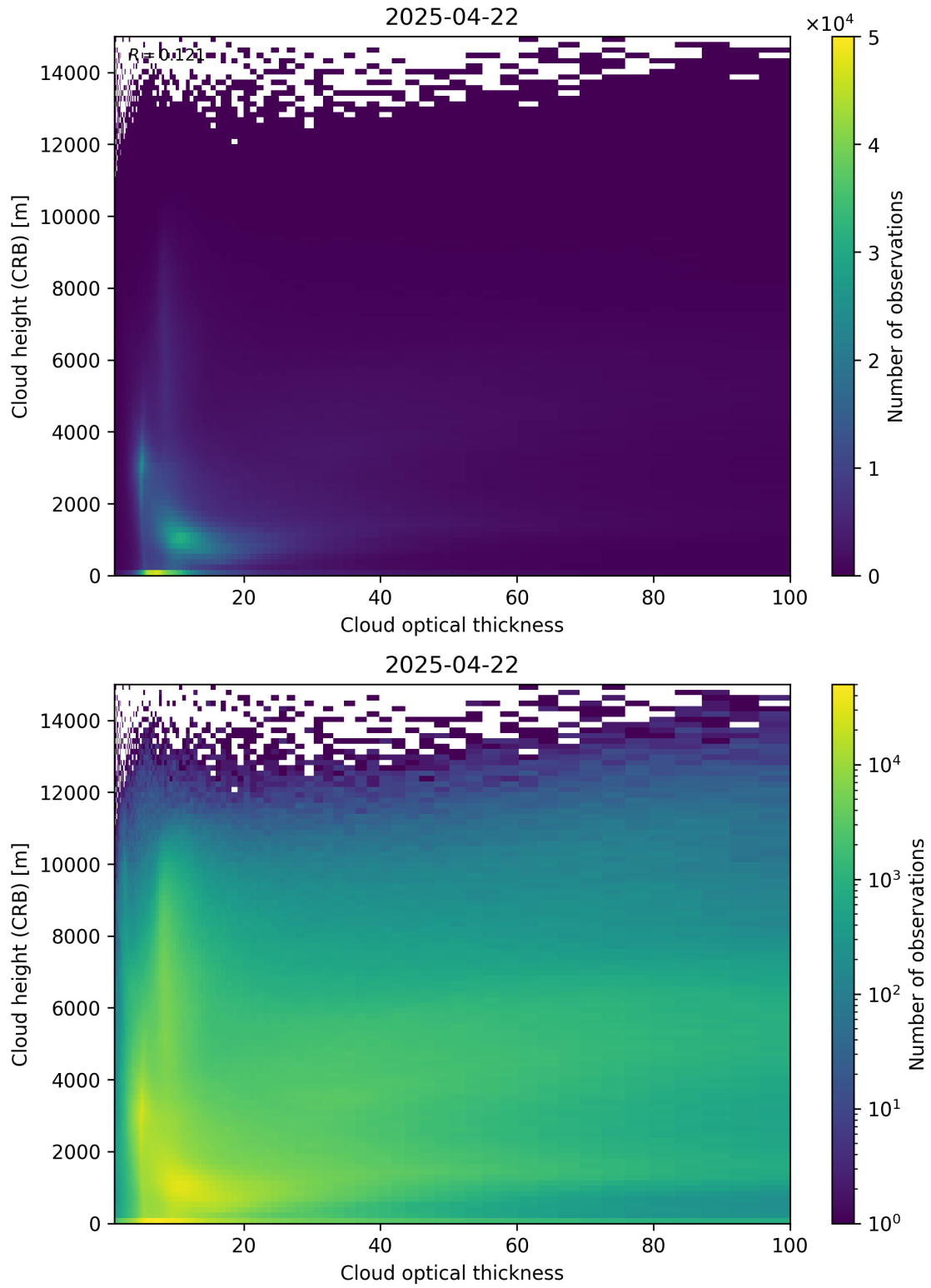
Figure 85: Scatter density plot of “Cloud optical thickness” against “Cloud height (CRB)” for 2025-04-21 to 2025-04-23.
