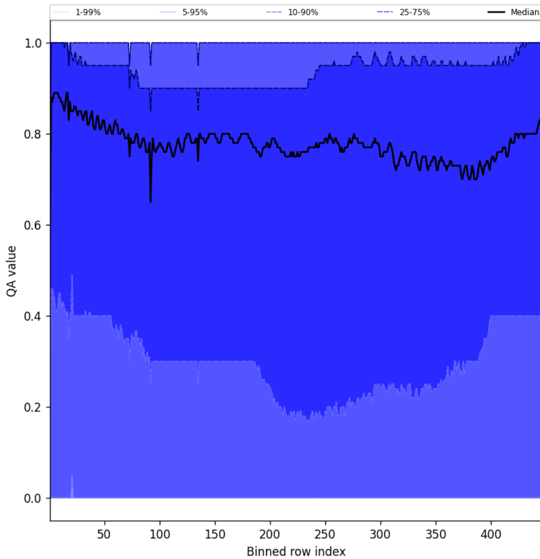
Figure 54: Along track statistics of “QA value” for 2025-04-21 to 2025-04-23
