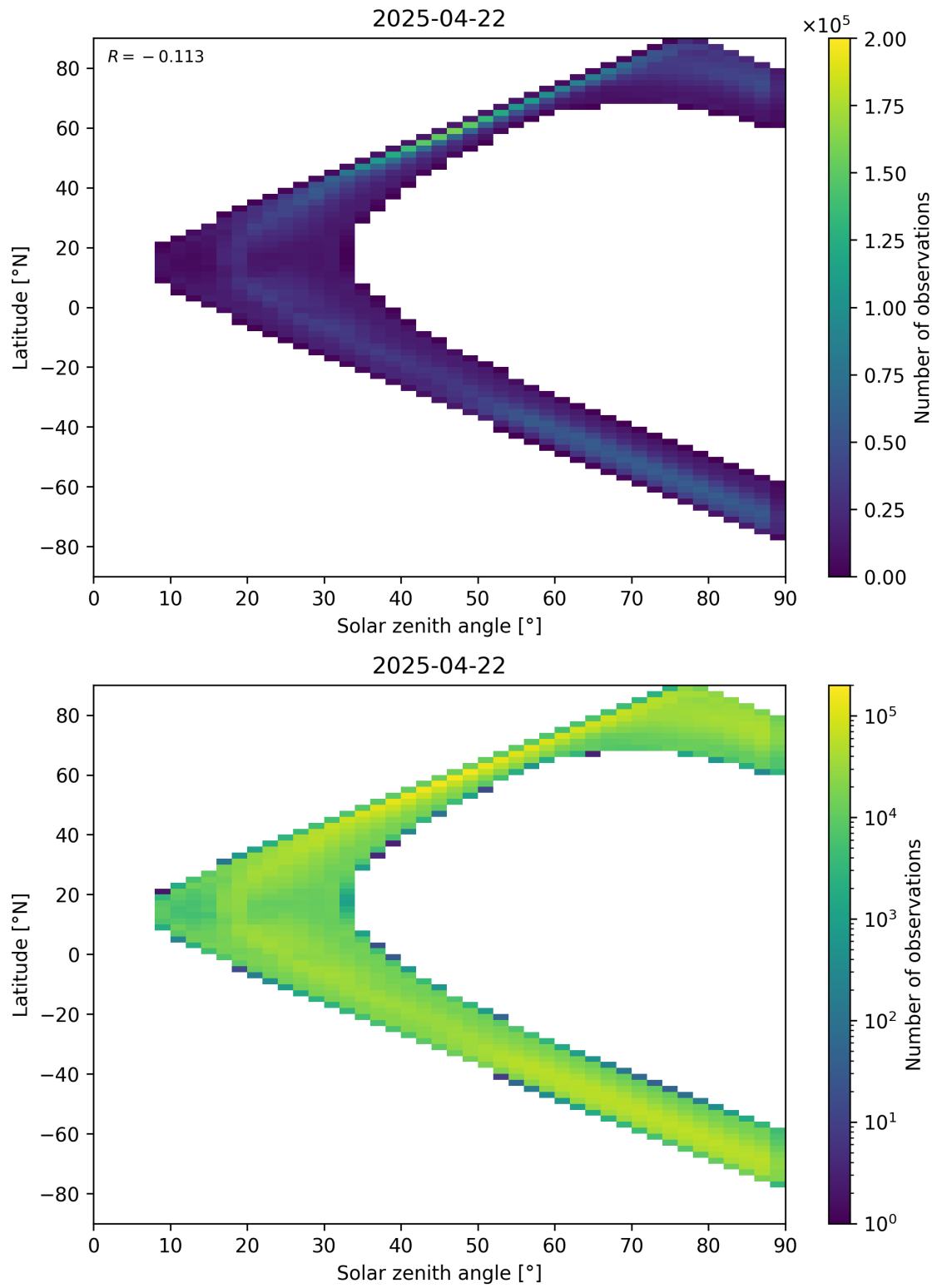
Figure 105: Scatter density plot of “Solar zenith angle” against “Latitude” for 2025-04-21 to 2025-04-23.
