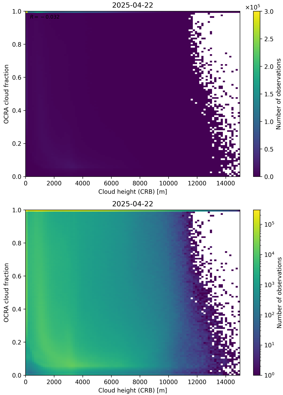
Figure 81: Scatter density plot of “Cloud height (CRB)” against “OCRA cloud fraction” for 2025-04-21 to 2025-04-23.
