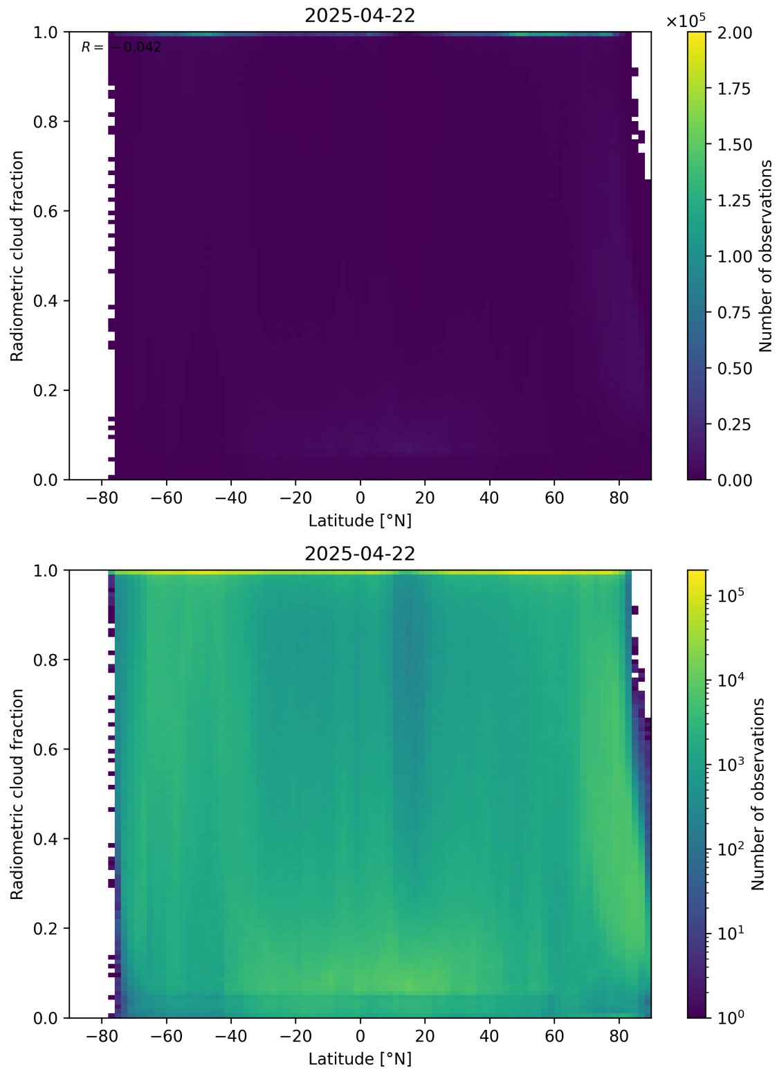
Figure 92: Scatter density plot of “Latitude” against “Radiometric cloud fraction” for 2025-04-21 to 2025-04-23.
