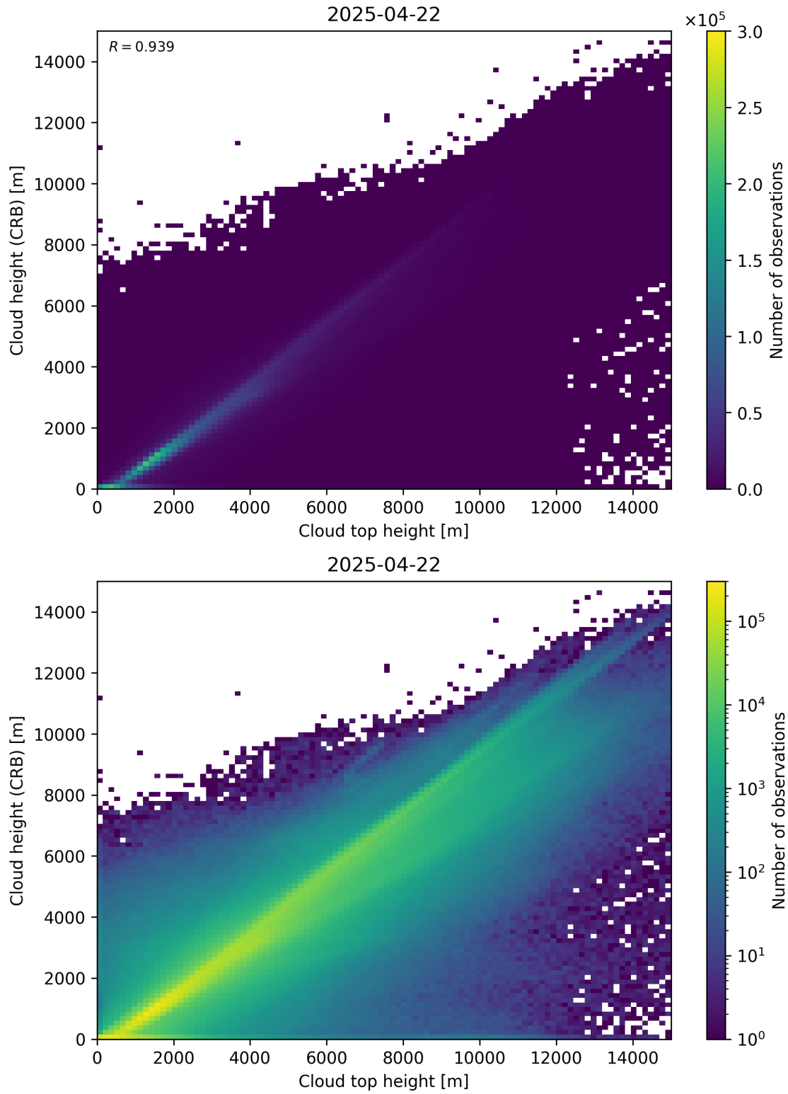
Figure 89: Scatter density plot of “Cloud top height” against “Cloud height (CRB)” for 2025-04-21 to 2025-04-23.
