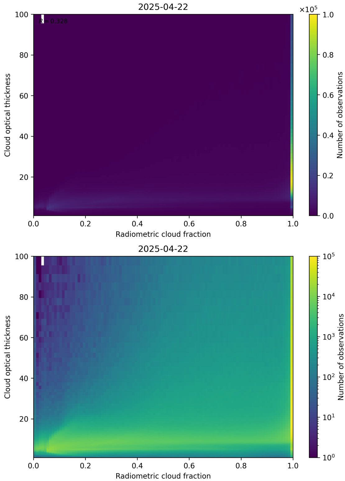
Figure 75: Scatter density plot of “Radiometric cloud fraction” against “Cloud optical thickness” for 2025-04-21 to 2025-04-23.
