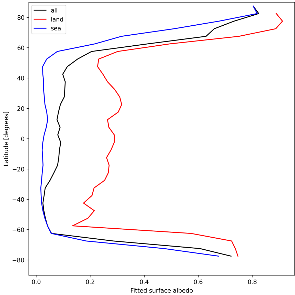
Figure 29: Zonal average of “Fitted surface albedo” for 2025-04-21 to 2025-04-23.
