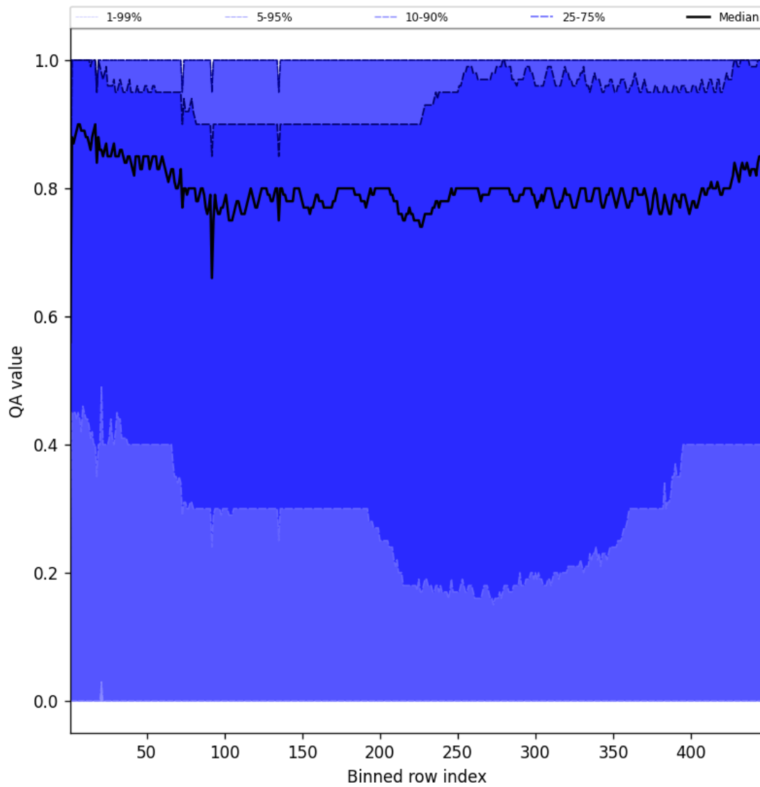
Figure 54: Along track statistics of “QA value” for 2025-04-22 to 2025-04-24
