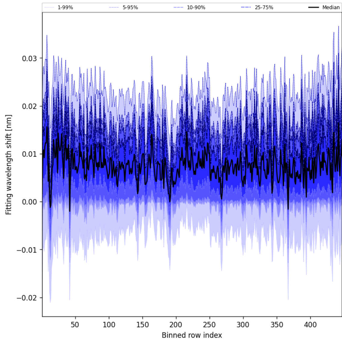
Figure 65: Along track statistics of “Fitting wavelength shift” for 2025-04-22 to 2025-04-24
