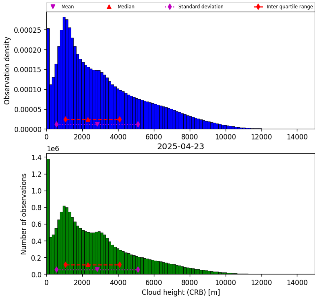
Figure 43: Histogram of “Cloud height (CRB)” for 2025-04-22 to 2025-04-24
