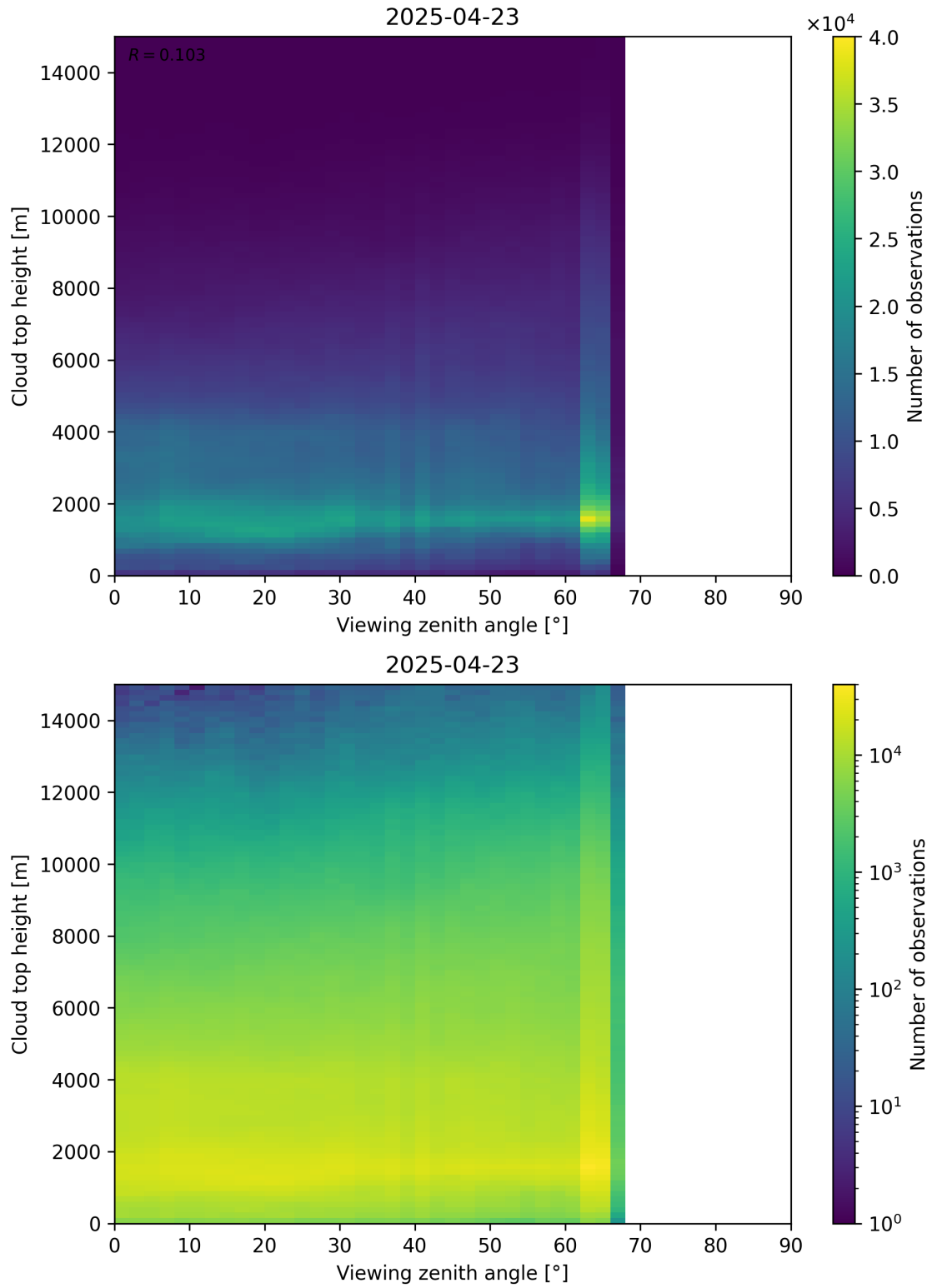
Figure 112: Scatter density plot of “Viewing zenith angle” against “Cloud top height” for 2025-04-22 to 2025-04-24.
