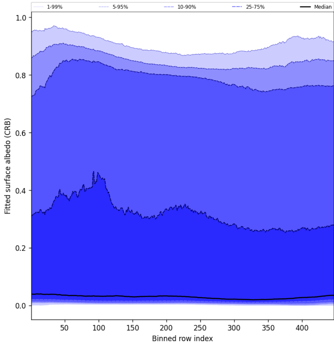
Figure 62: Along track statistics of “Fitted surface albedo (CRB)” for 2025-04-22 to 2025-04-24
