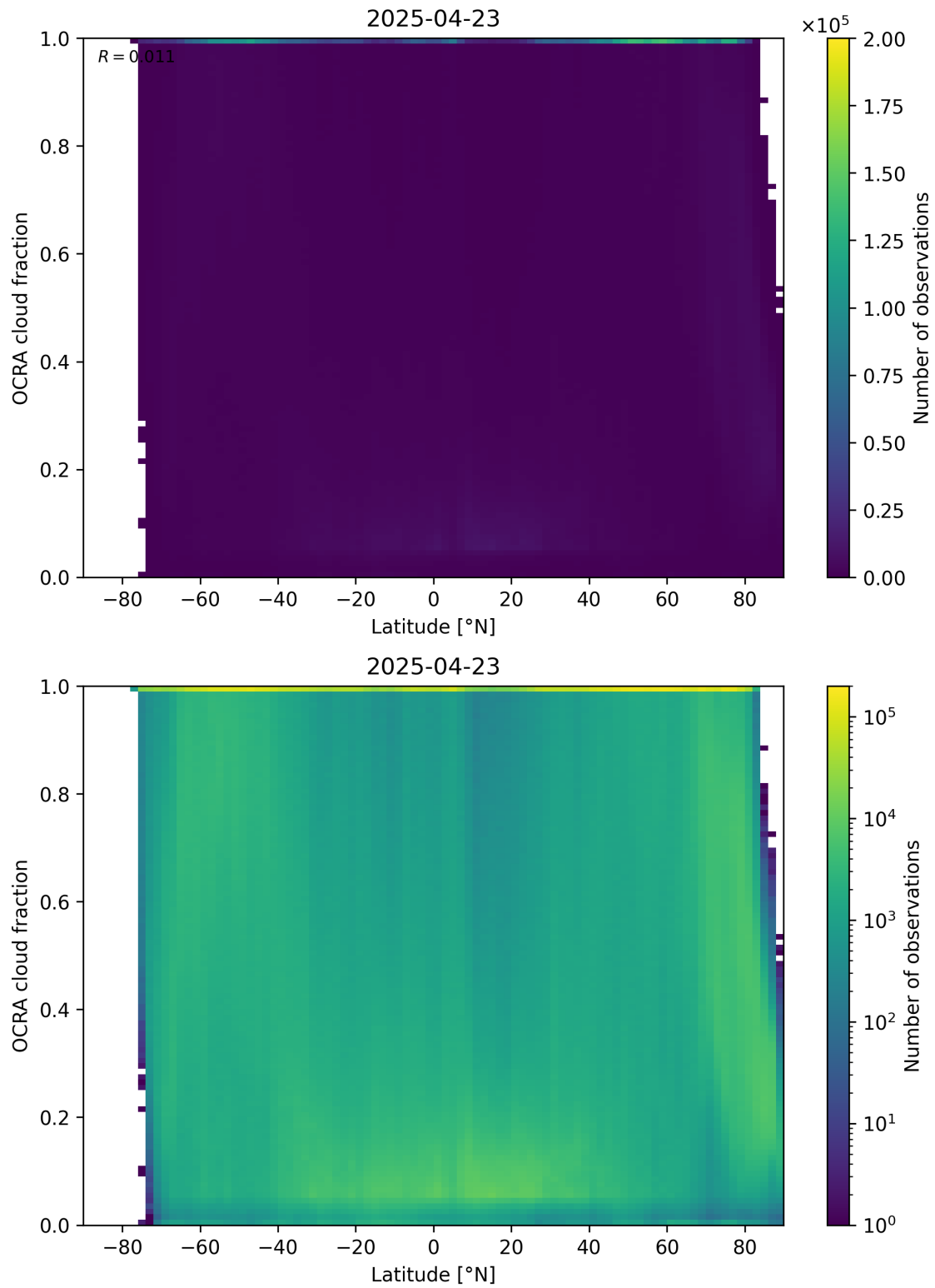
Figure 93: Scatter density plot of “Latitude” against “OCRA cloud fraction” for 2025-04-22 to 2025-04-24.
