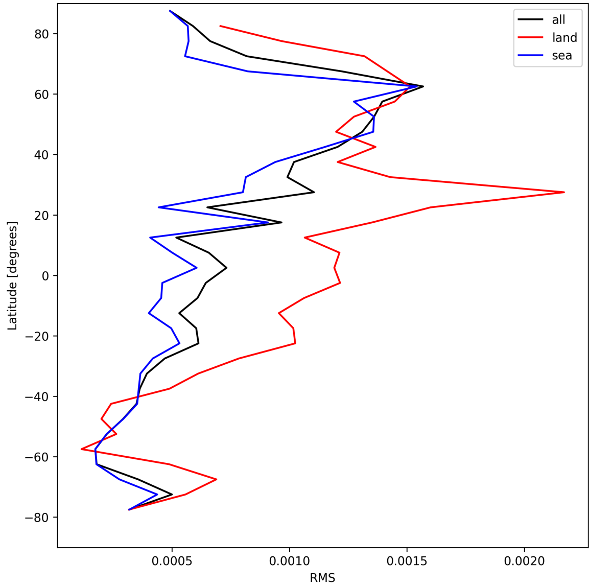
Figure 31: Zonal average of “RMS” for 2025-04-22 to 2025-04-24.
