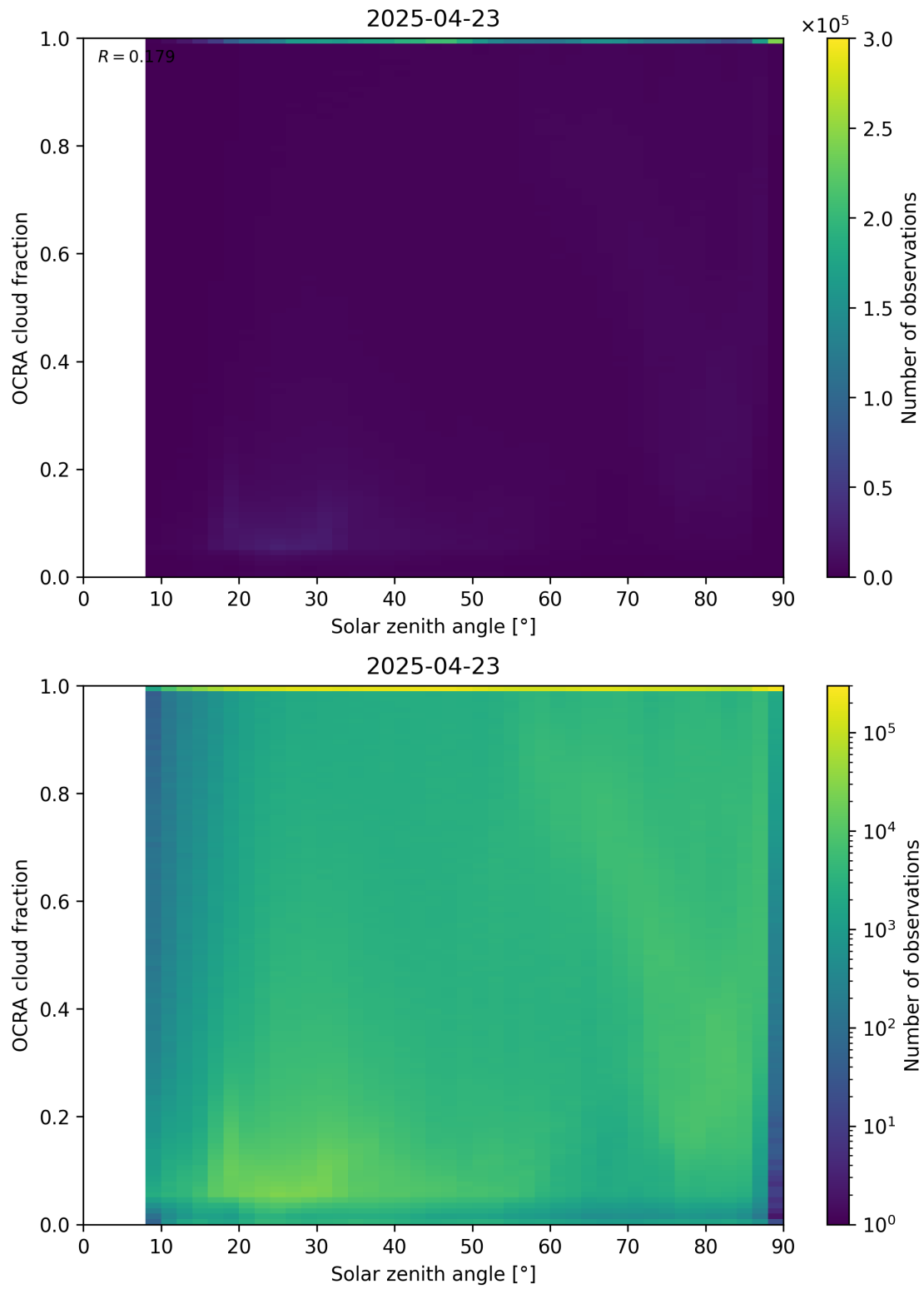
Figure 100: Scatter density plot of “Solar zenith angle” against “OCRA cloud fraction” for 2025-04-22 to 2025-04-24.
