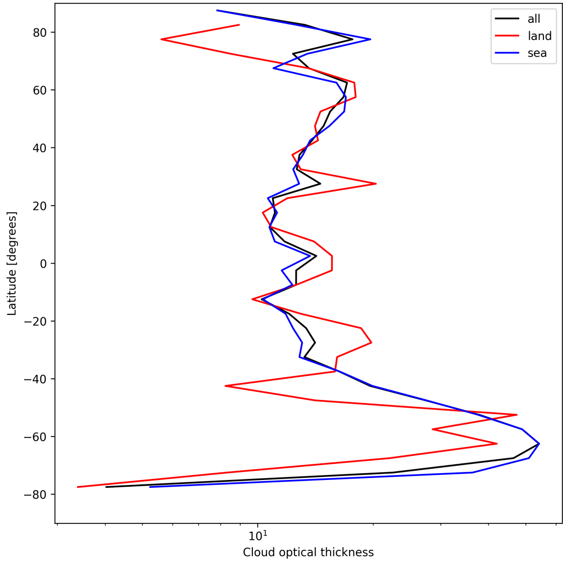
Figure 25: Zonal average of “Cloud optical thickness” for 2025-04-22 to 2025-04-24.
