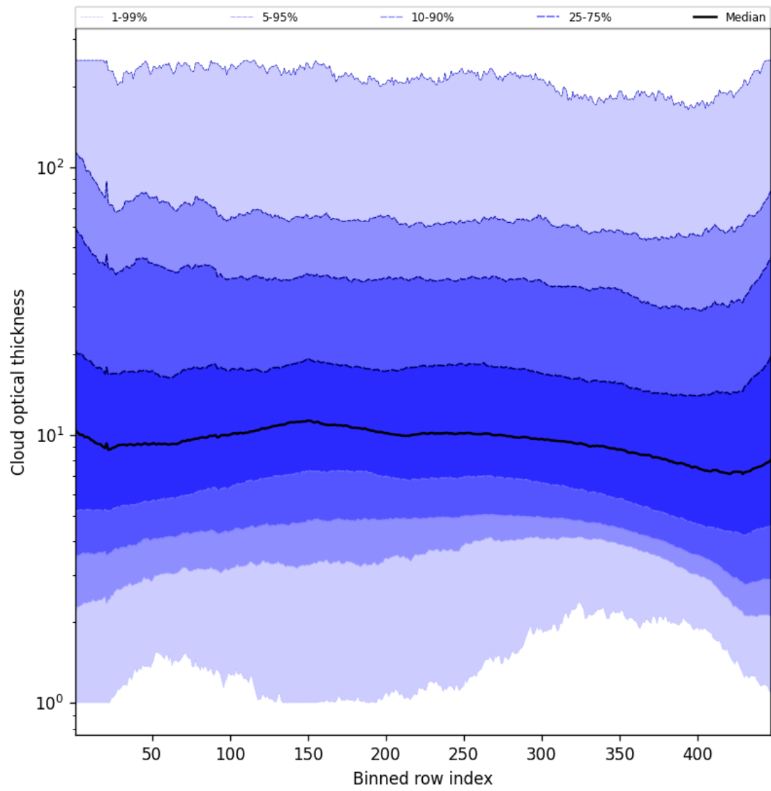
Figure 57: Along track statistics of “Cloud optical thickness” for 2025-04-22 to 2025-04-24
