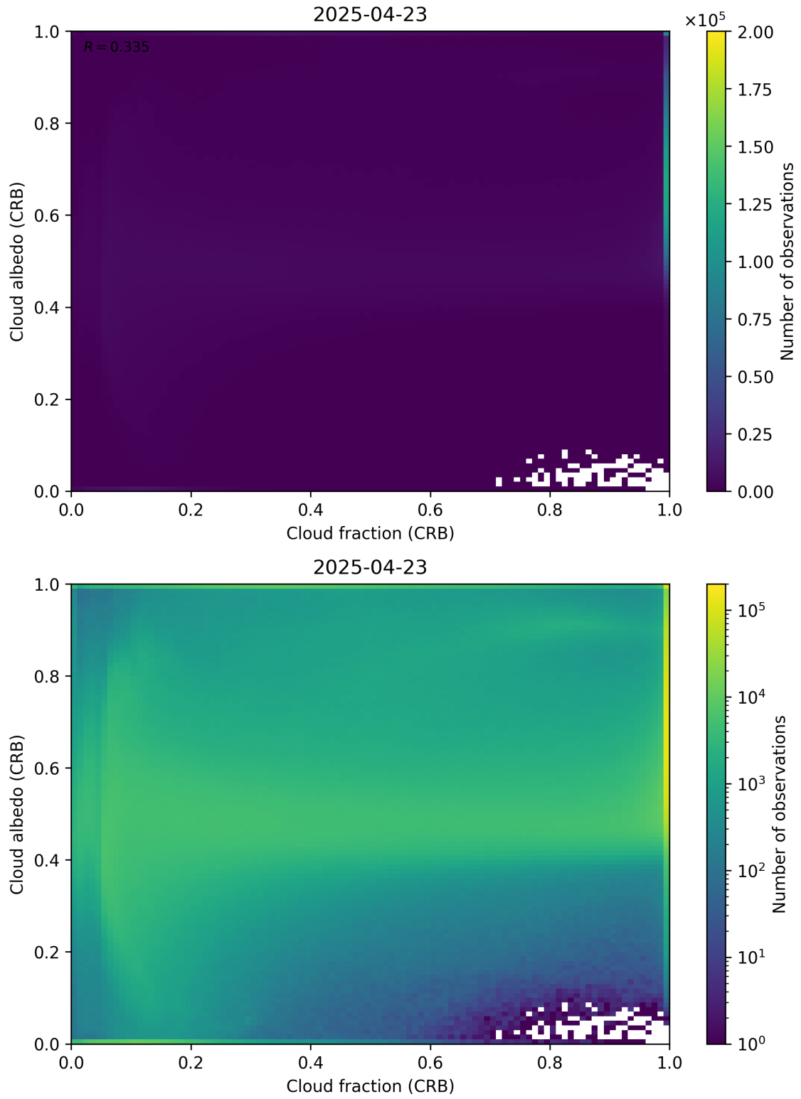
Figure 77: Scatter density plot of “Cloud fraction (CRB)” against “Cloud albedo (CRB)” for 2025-04-22 to 2025-04-24.
