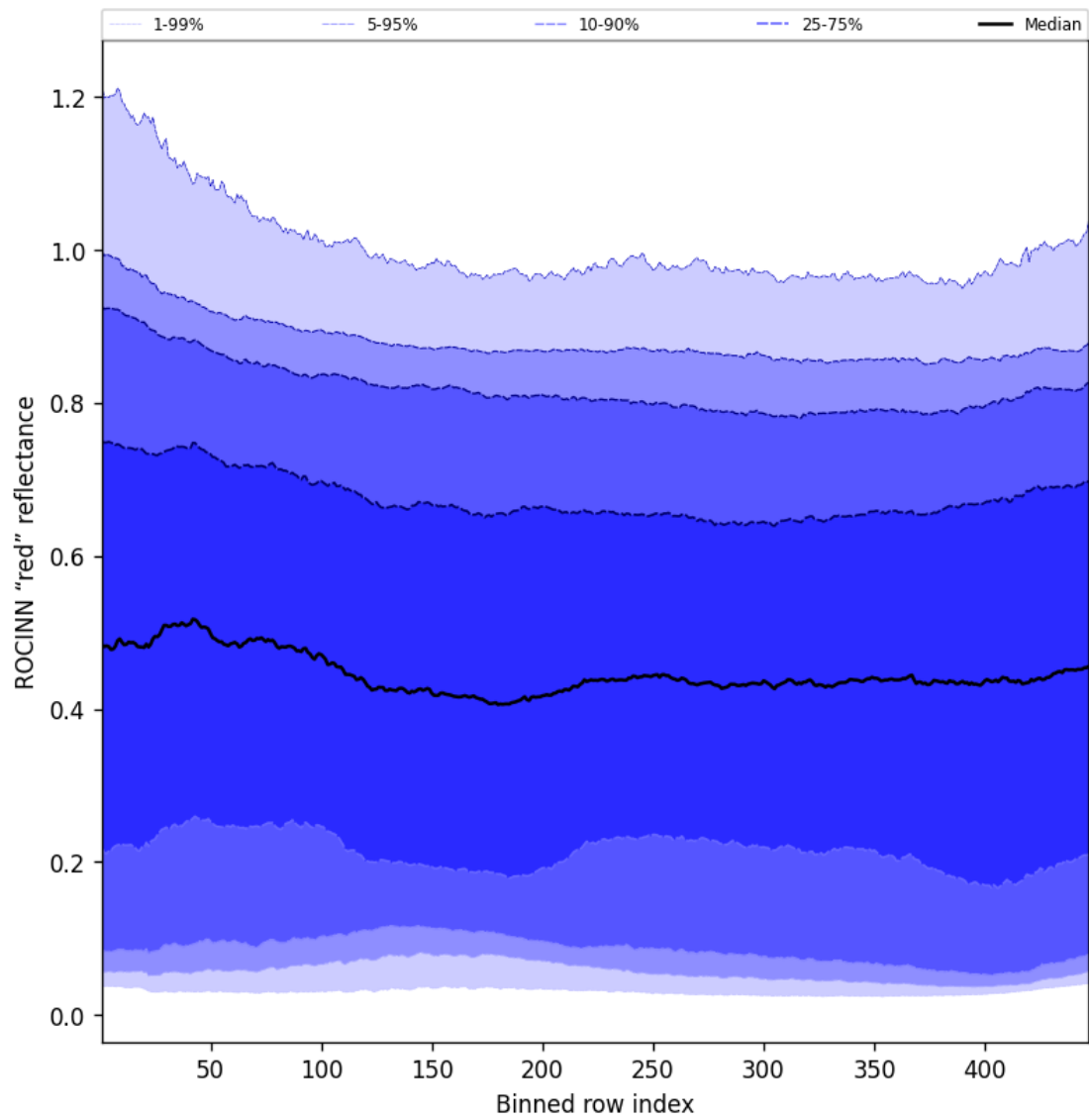
Figure 69: Along track statistics of “ROCINN “red” reflectance” for 2025-04-22 to 2025-04-24
