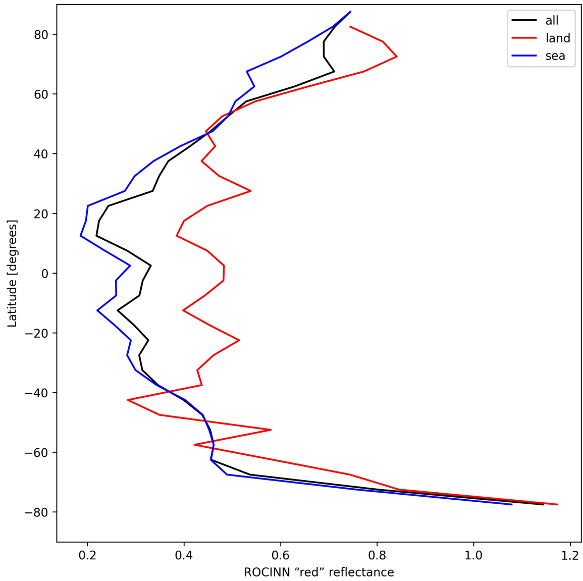
Figure 37: Zonal average of “ROCINN “red” reflectance” for 2025-04-22 to 2025-04-24.
