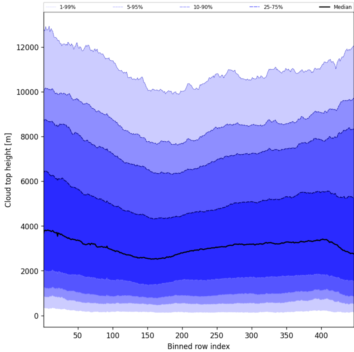
Figure 56: Along track statistics of “Cloud top height” for 2025-04-22 to 2025-04-24
