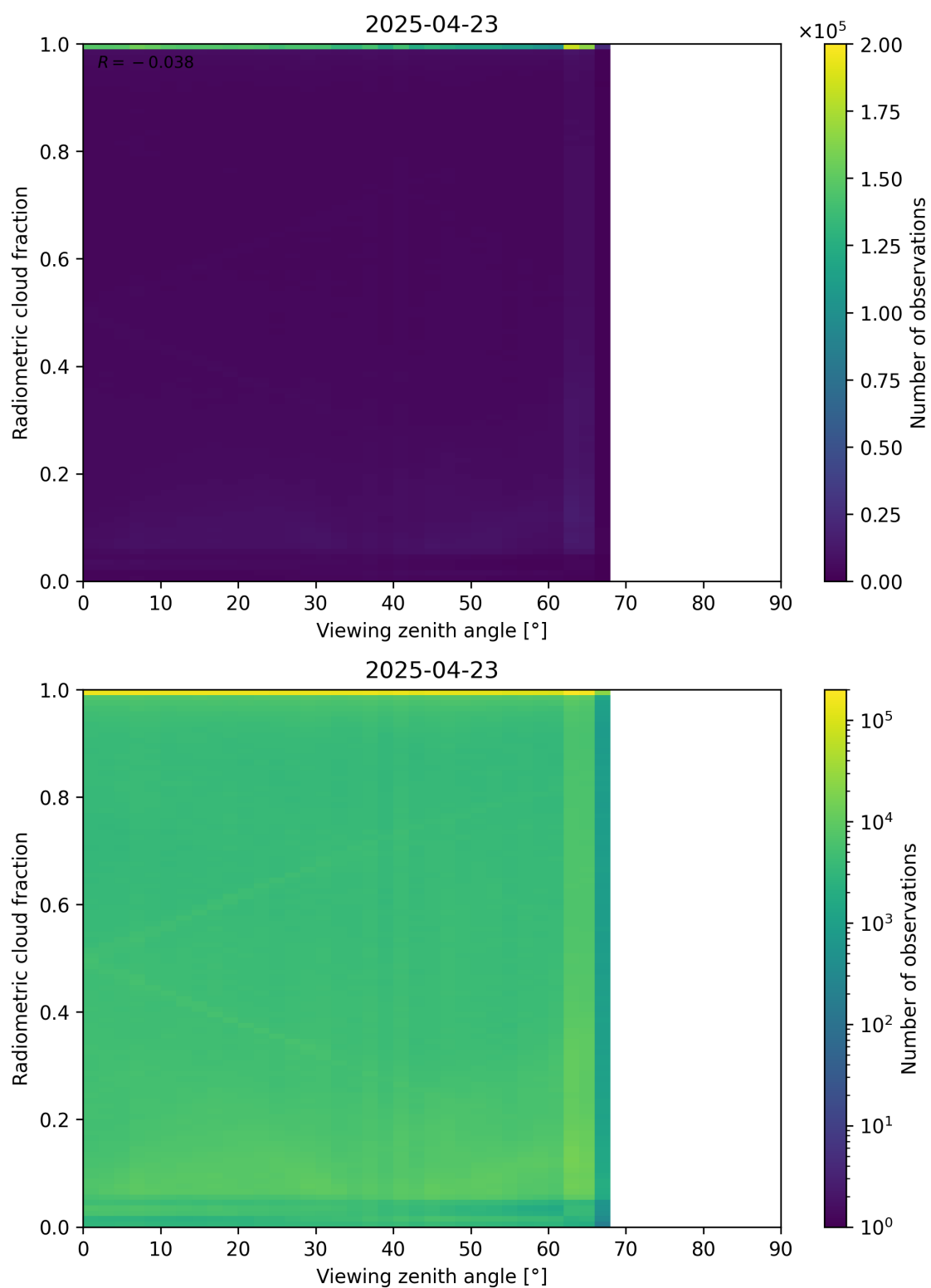
Figure 107: Scatter density plot of “Viewing zenith angle” against “Radiometric cloud fraction” for 2025-04-22 to 2025-04-24.
