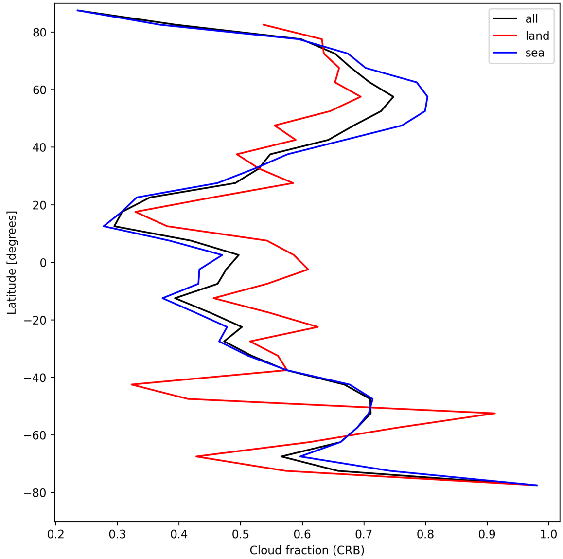
Figure 26: Zonal average of “Cloud fraction (CRB)” for 2025-04-22 to 2025-04-24.
