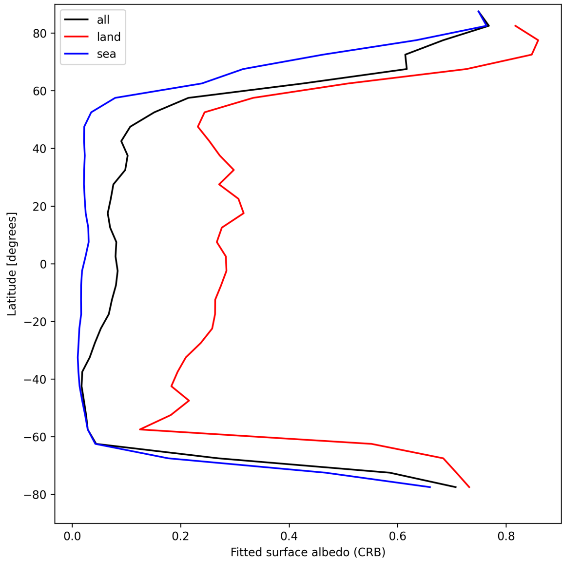
Figure 30: Zonal average of “Fitted surface albedo (CRB)” for 2025-04-22 to 2025-04-24.
