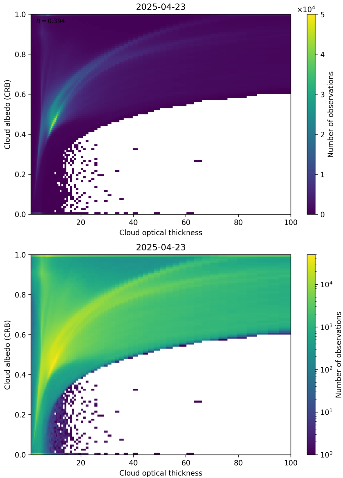
Figure 82: Scatter density plot of “Cloud optical thickness” against “Cloud albedo (CRB)” for 2025-04-22 to 2025-04-24.
