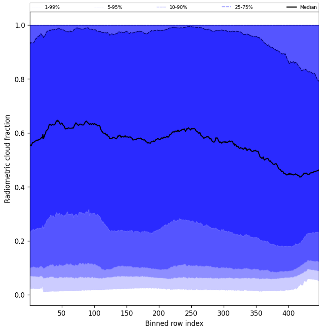
Figure 55: Along track statistics of “Radiometric cloud fraction” for 2025-04-22 to 2025-04-24
