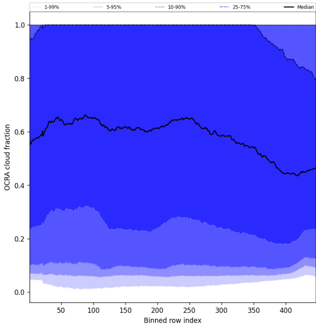
Figure 66: Along track statistics of “OCRA cloud fraction” for 2025-04-22 to 2025-04-24
