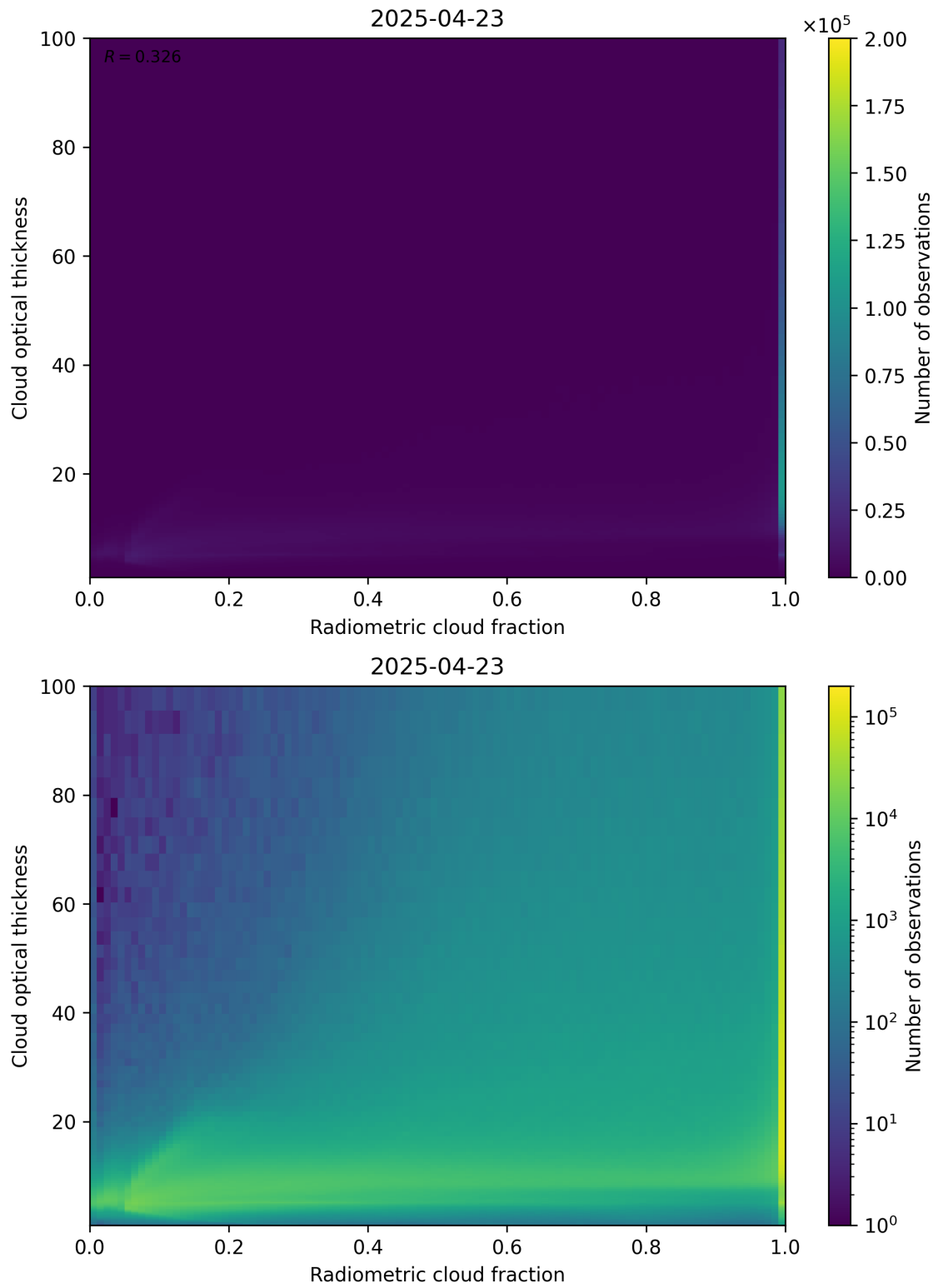
Figure 75: Scatter density plot of “Radiometric cloud fraction” against “Cloud optical thickness” for 2025-04-22 to 2025-04-24.
