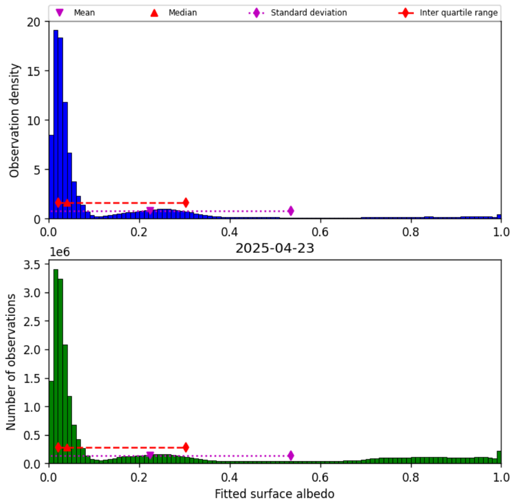
Figure 45: Histogram of “Fitted surface albedo” for 2025-04-22 to 2025-04-24
