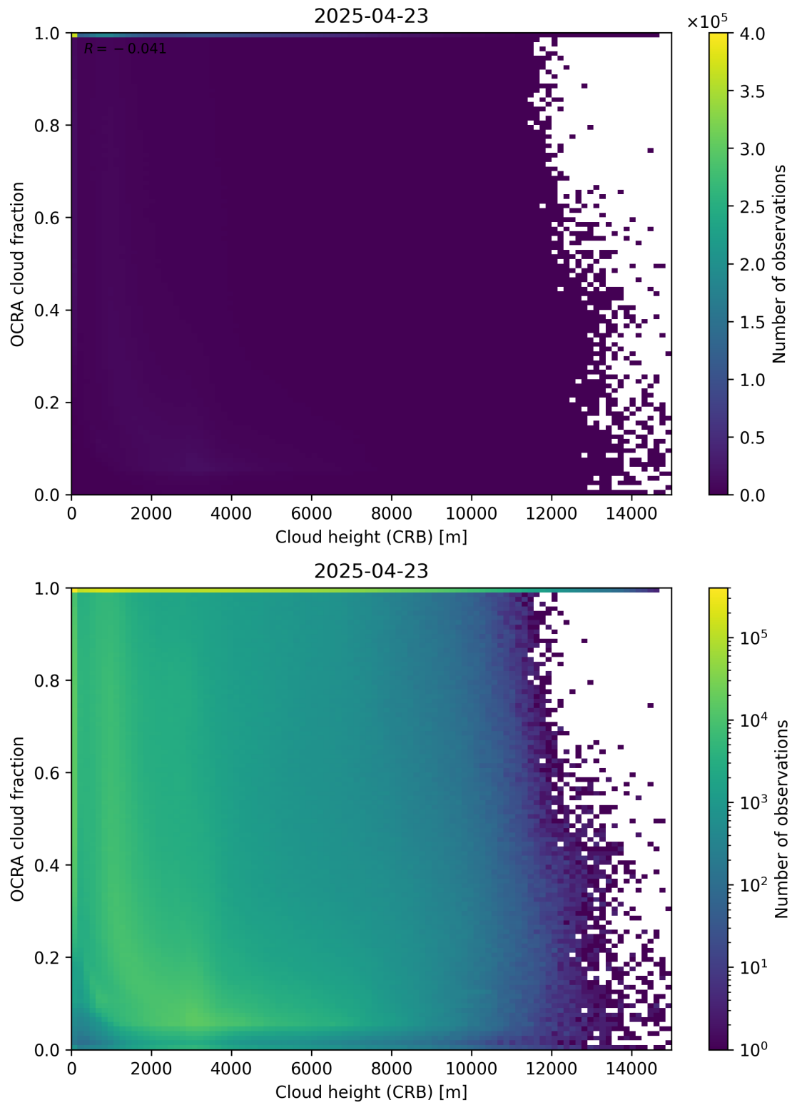
Figure 81: Scatter density plot of “Cloud height (CRB)” against “OCRA cloud fraction” for 2025-04-22 to 2025-04-24.
