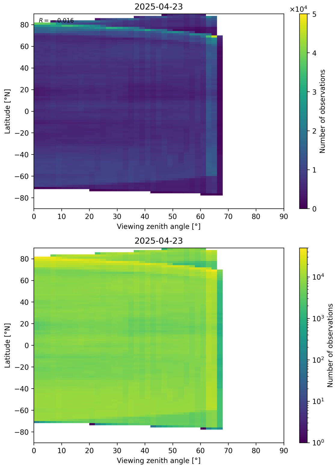
Figure 113: Scatter density plot of “Viewing zenith angle” against “Latitude” for 2025-04-22 to 2025-04-24.
