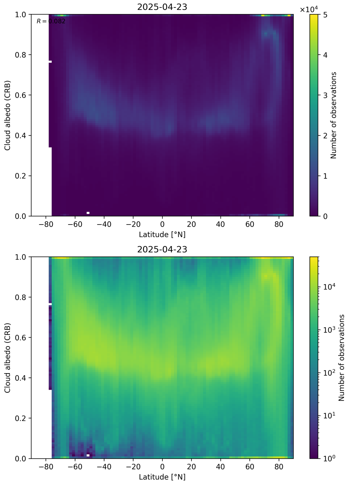
Figure 91: Scatter density plot of “Latitude” against “Cloud albedo (CRB)” for 2025-04-22 to 2025-04-24.
