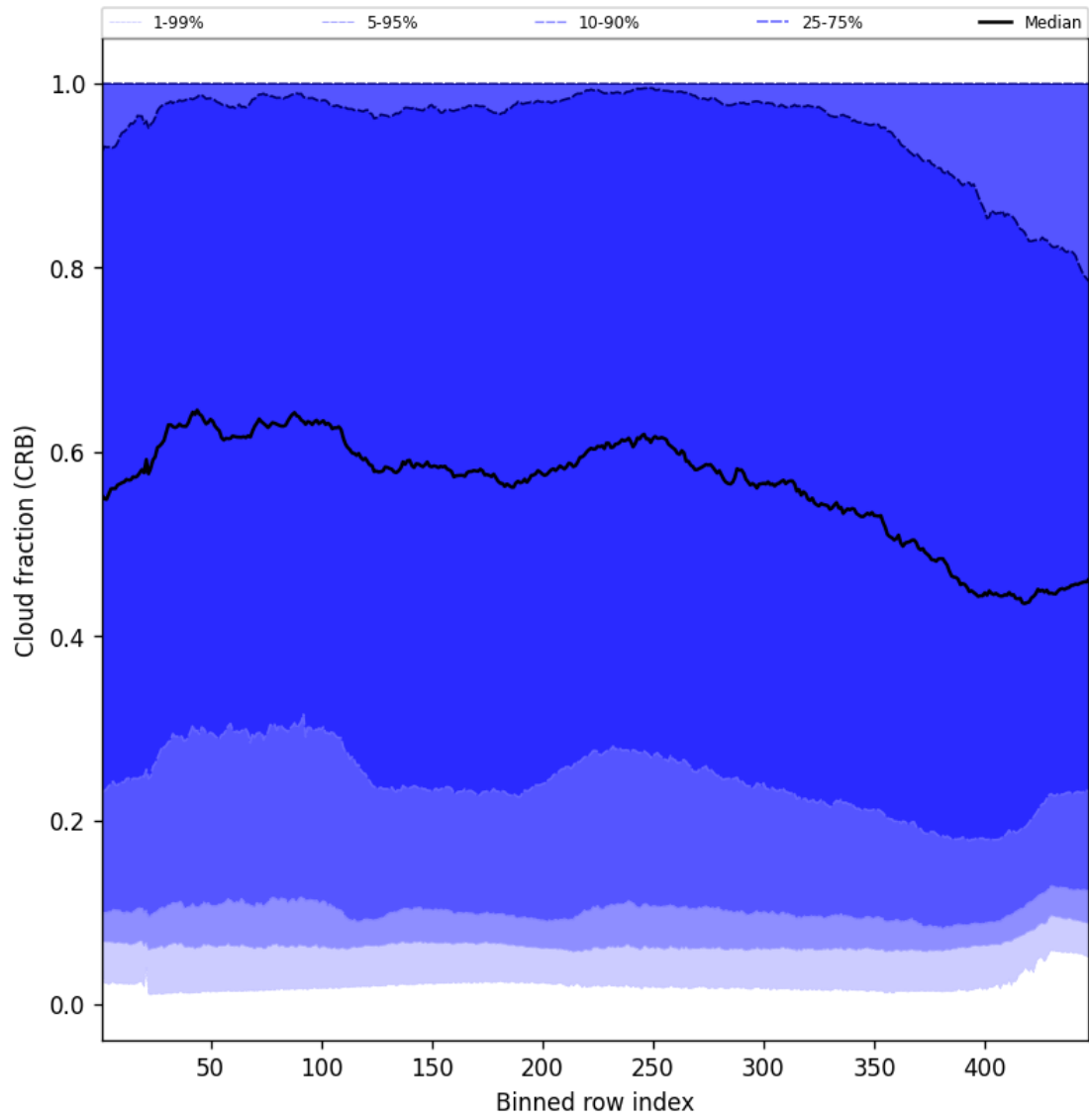
Figure 58: Along track statistics of “Cloud fraction (CRB)” for 2025-04-22 to 2025-04-24
