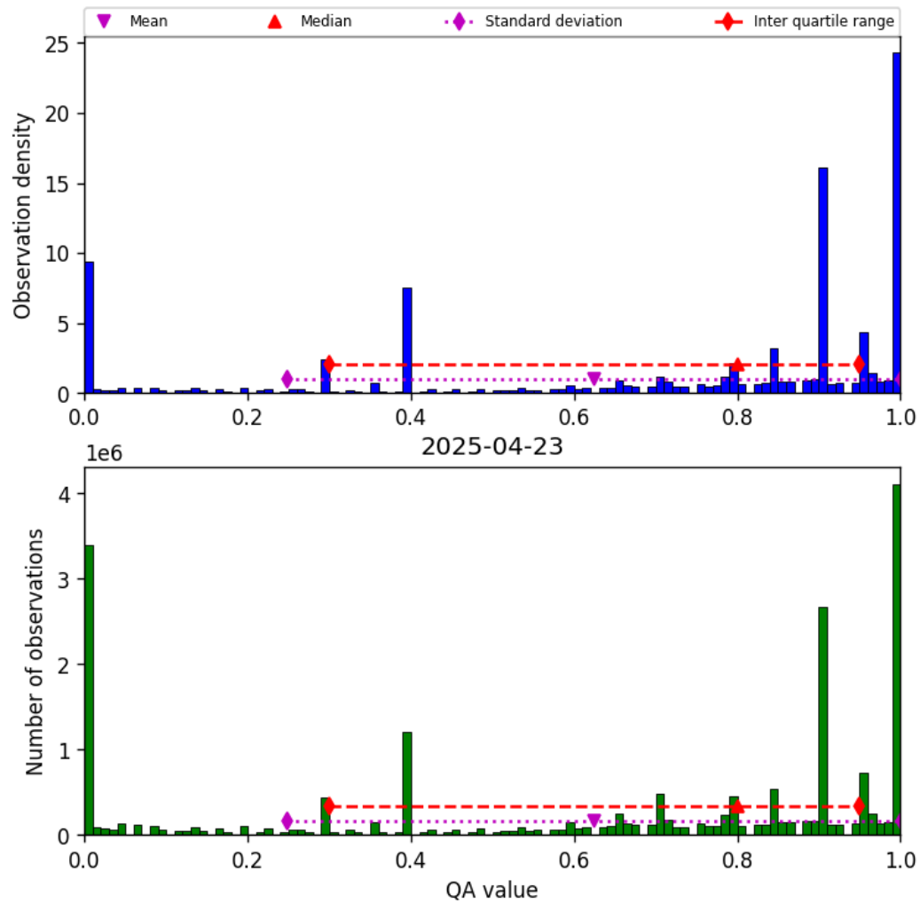
Figure 38: Histogram of “QA value” for 2025-04-22 to 2025-04-24
