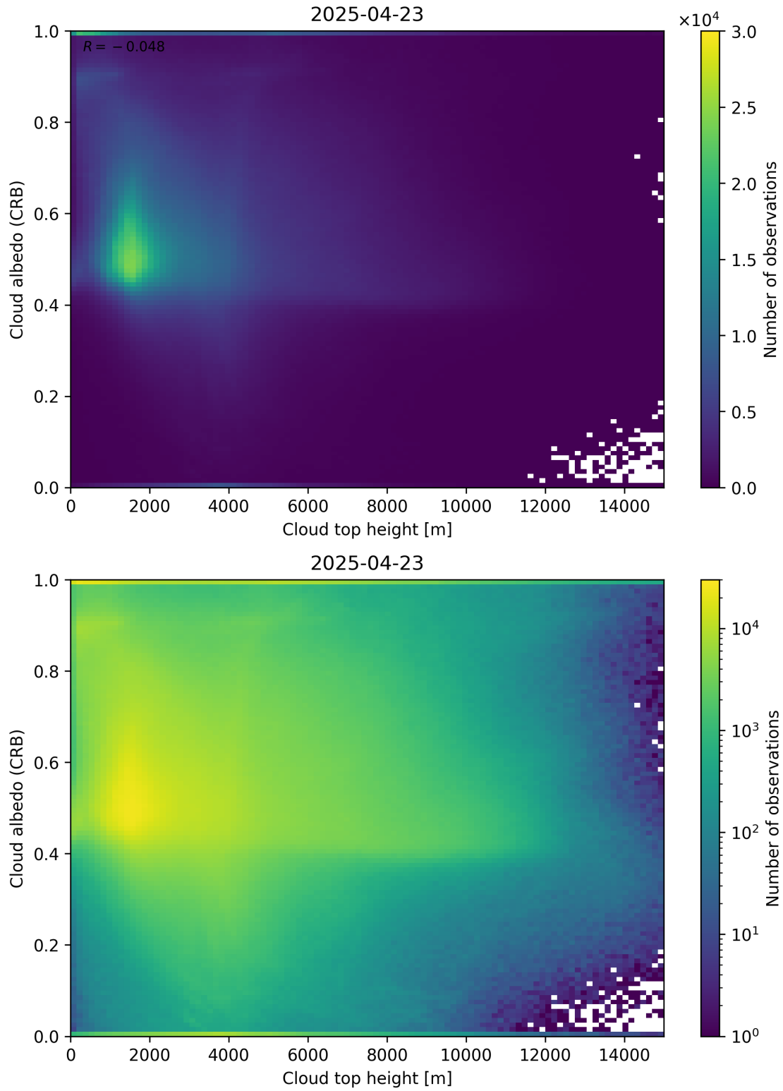
Figure 86: Scatter density plot of “Cloud top height” against “Cloud albedo (CRB)” for 2025-04-22 to 2025-04-24.
