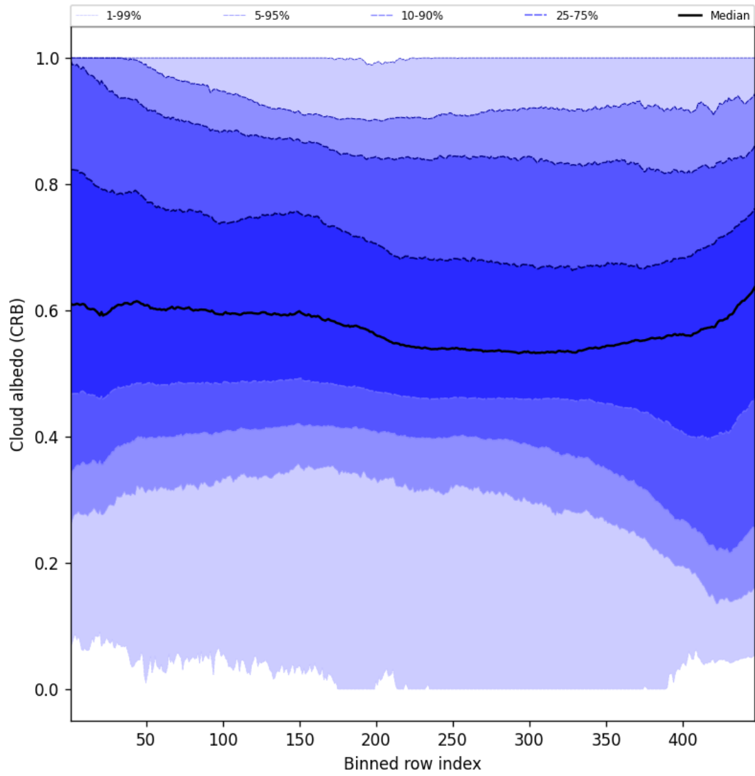
Figure 60: Along track statistics of “Cloud albedo (CRB)” for 2025-04-22 to 2025-04-24
