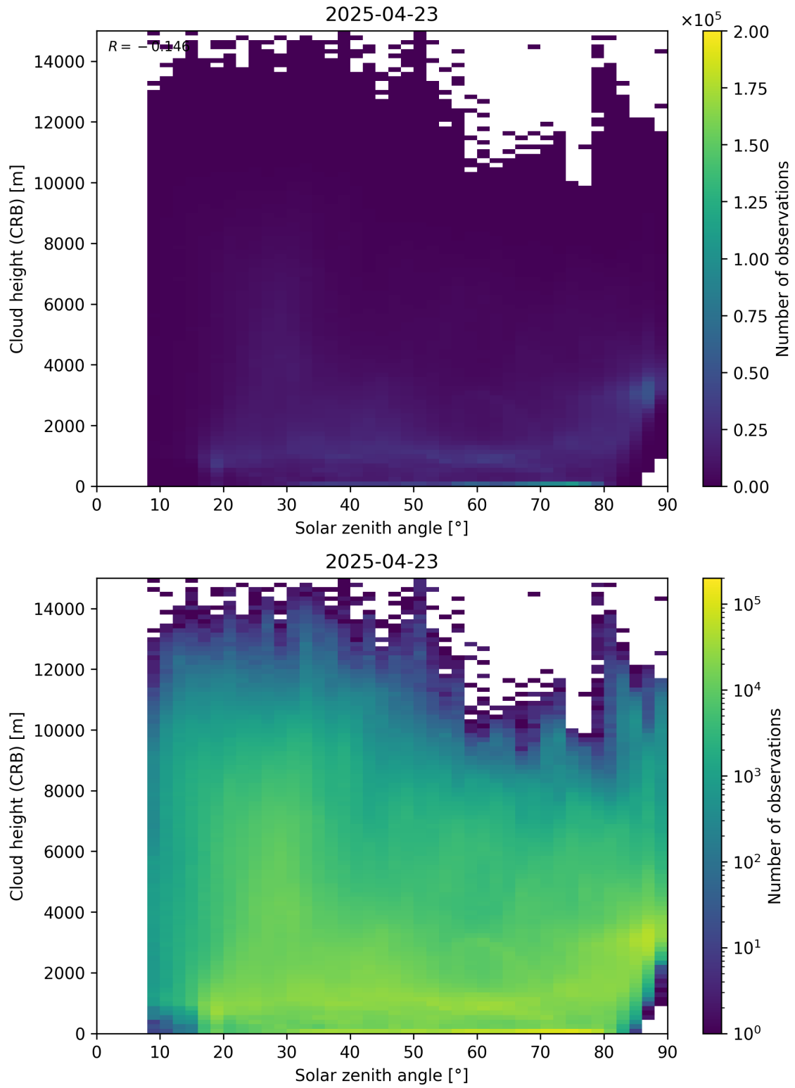
Figure 102: Scatter density plot of “Solar zenith angle” against “Cloud height (CRB)” for 2025-04-22 to 2025-04-24.
