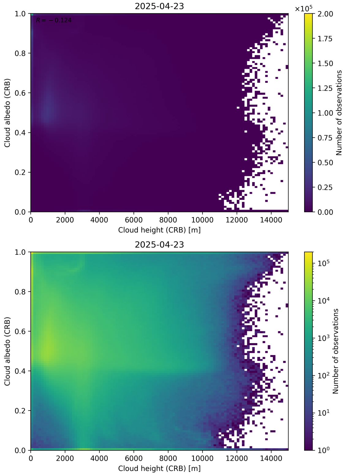
Figure 80: Scatter density plot of “Cloud height (CRB)” against “Cloud albedo (CRB)” for 2025-04-22 to 2025-04-24.
