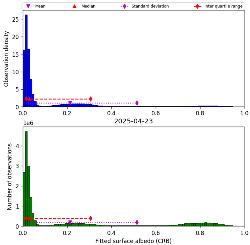
Figure 46: Histogram of “Fitted surface albedo (CRB)” for 2025-04-22 to 2025-04-24
