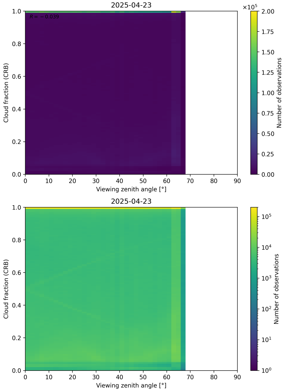
Figure 109: Scatter density plot of “Viewing zenith angle” against “Cloud fraction (CRB)” for 2025-04-22 to 2025-04-24.
