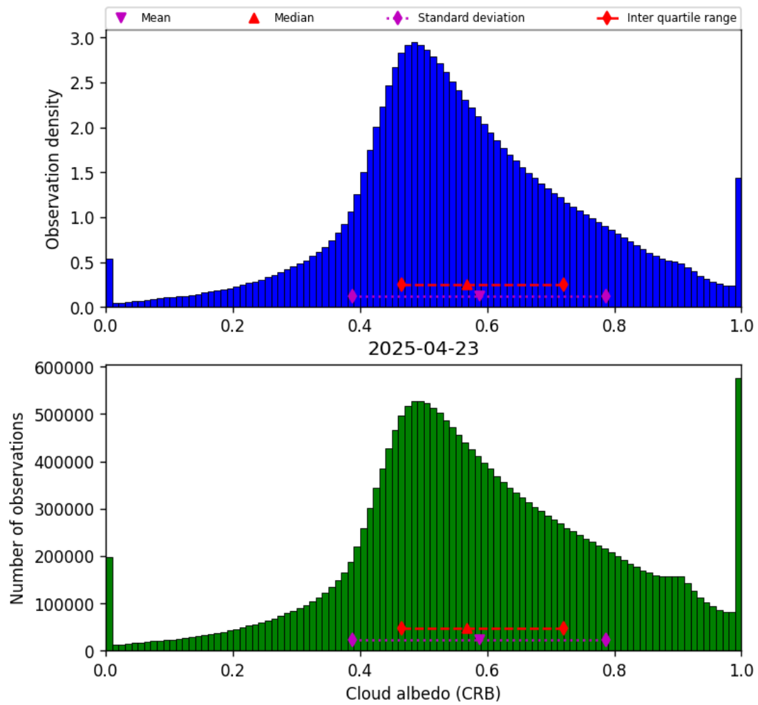
Figure 44: Histogram of “Cloud albedo (CRB)” for 2025-04-22 to 2025-04-24
