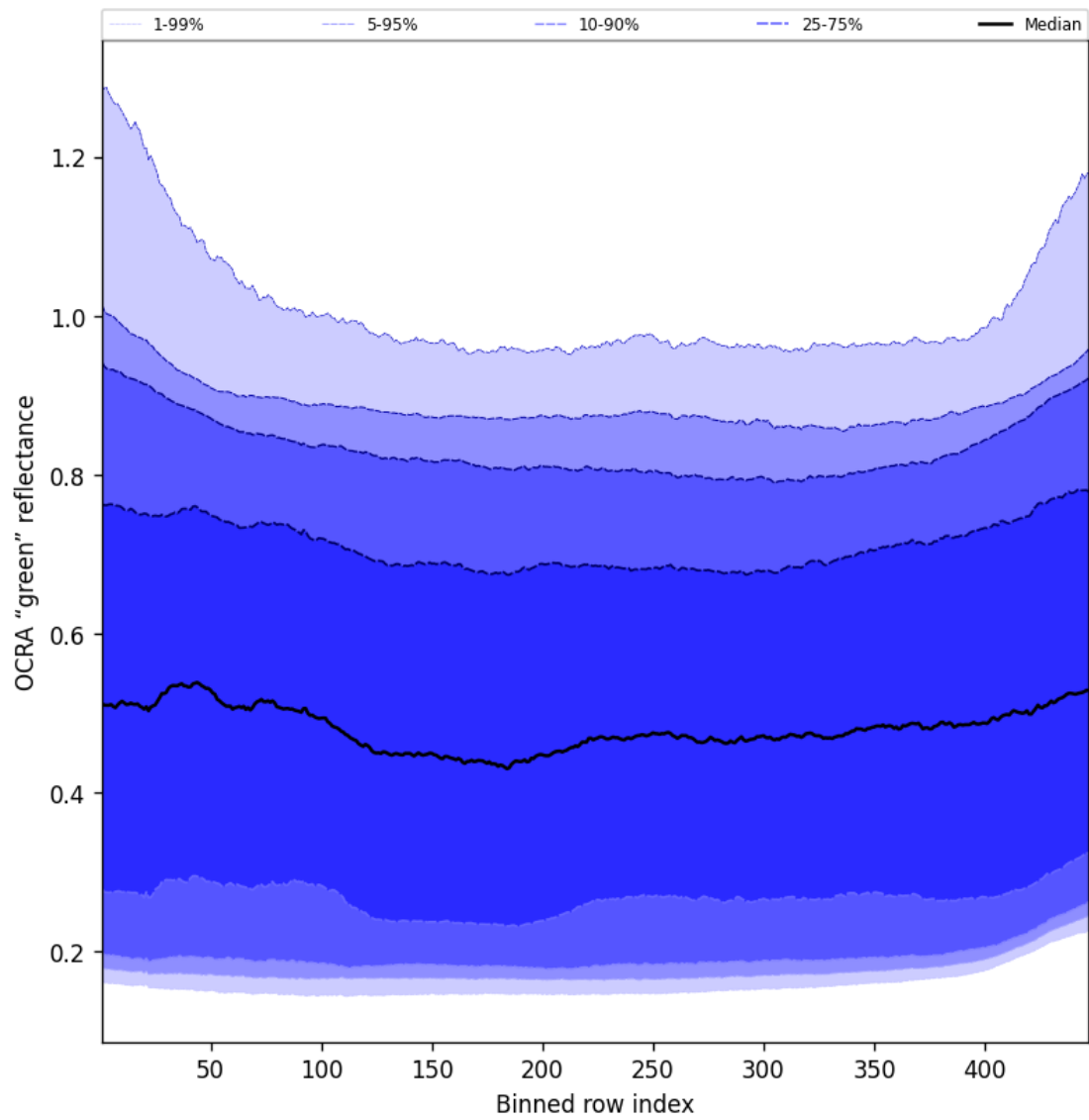
Figure 68: Along track statistics of “OCRA “green” reflectance” for 2025-04-22 to 2025-04-24
