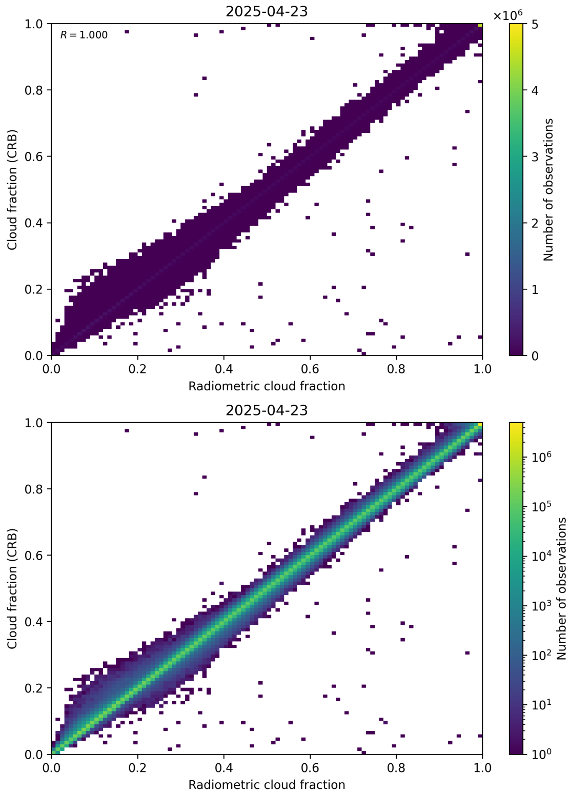
Figure 73: Scatter density plot of “Radiometric cloud fraction” against “Cloud fraction (CRB)” for 2025-04-22 to 2025-04-24.
