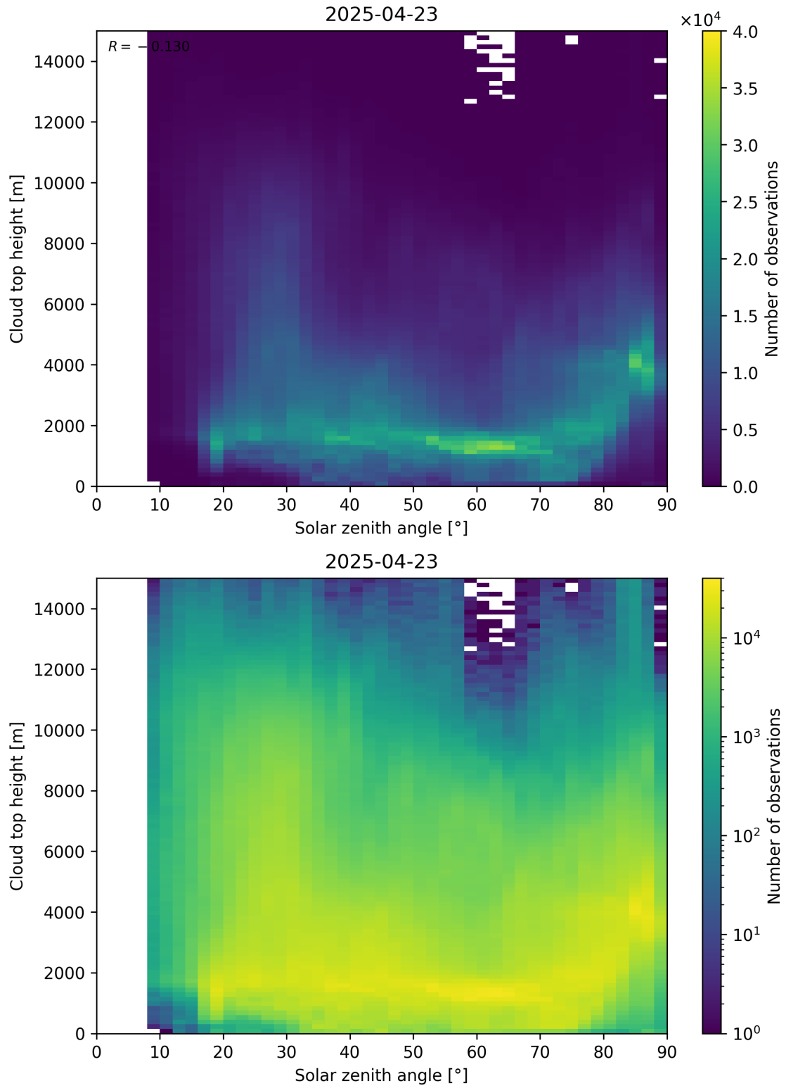
Figure 104: Scatter density plot of “Solar zenith angle” against “Cloud top height” for 2025-04-22 to 2025-04-24.
