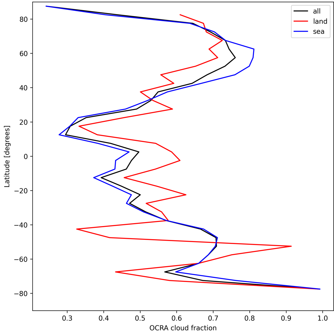
Figure 34: Zonal average of “OCRA cloud fraction” for 2025-04-22 to 2025-04-24.
