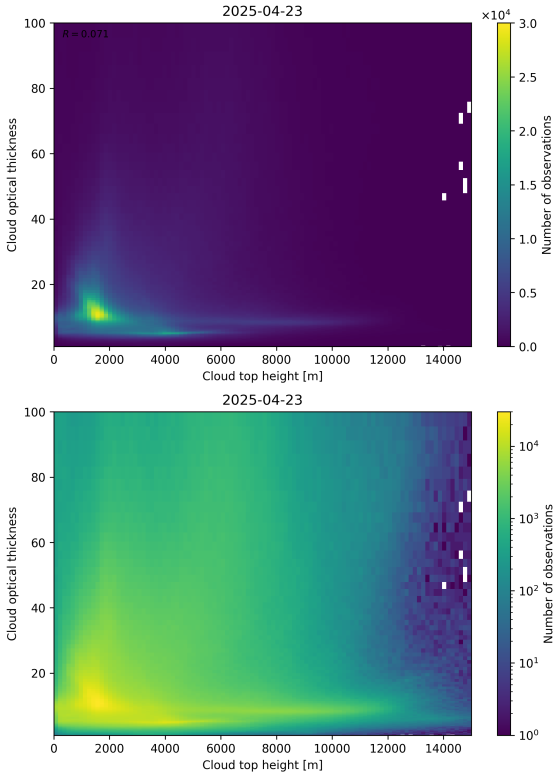
Figure 90: Scatter density plot of “Cloud top height” against “Cloud optical thickness” for 2025-04-22 to 2025-04-24.
