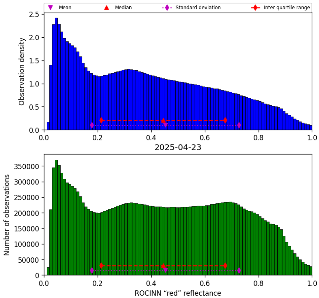
Figure 53: Histogram of “ROCINN “red” reflectance” for 2025-04-22 to 2025-04-24
