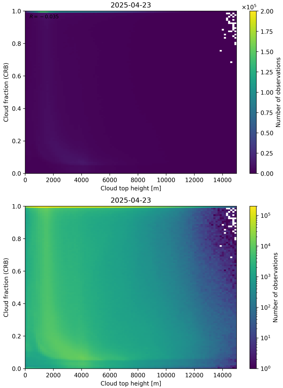
Figure 88: Scatter density plot of “Cloud top height” against “Cloud fraction (CRB)” for 2025-04-22 to 2025-04-24.
