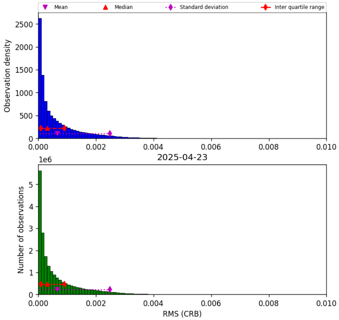
Figure 48: Histogram of “RMS (CRB)” for 2025-04-22 to 2025-04-24
