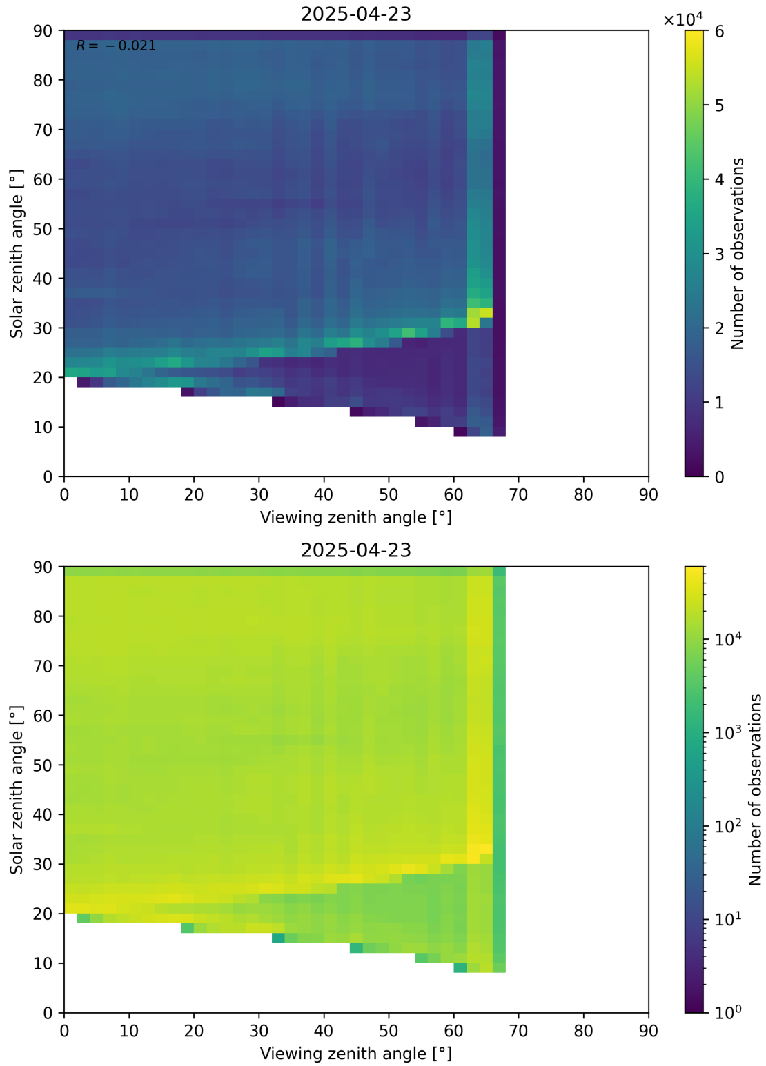
Figure 114: Scatter density plot of “Viewing zenith angle” against “Solar zenith angle” for 2025-04-22 to 2025-04-24.
