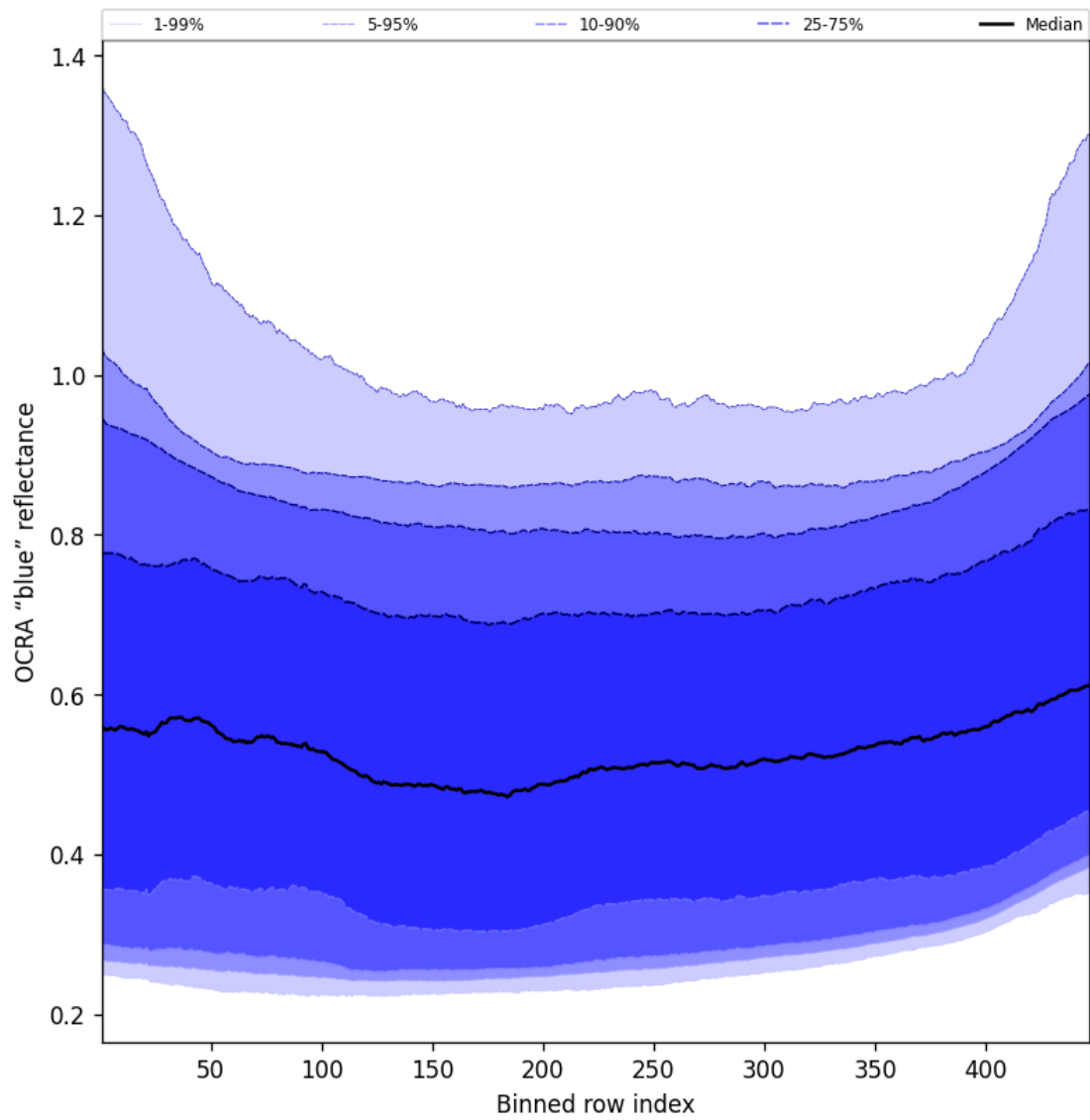
Figure 67: Along track statistics of “OCRA “blue” reflectance” for 2025-04-22 to 2025-04-24
