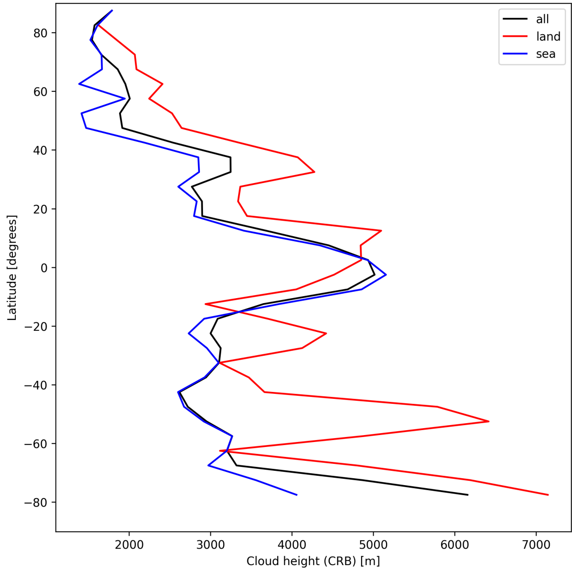
Figure 27: Zonal average of “Cloud height (CRB)” for 2025-04-22 to 2025-04-24.
