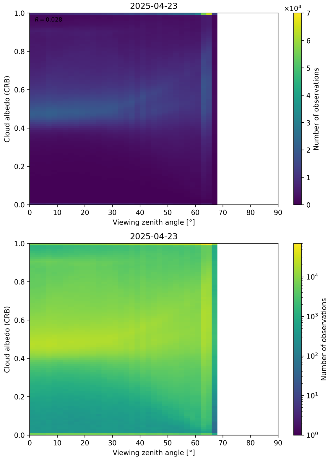
Figure 106: Scatter density plot of “Viewing zenith angle” against “Cloud albedo (CRB)” for 2025-04-22 to 2025-04-24.
