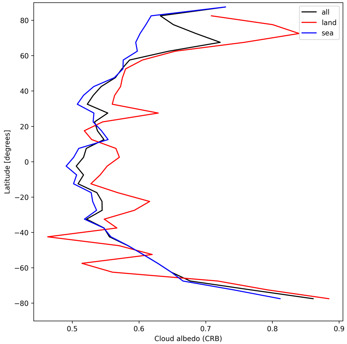
Figure 28: Zonal average of “Cloud albedo (CRB)” for 2025-04-22 to 2025-04-24.
