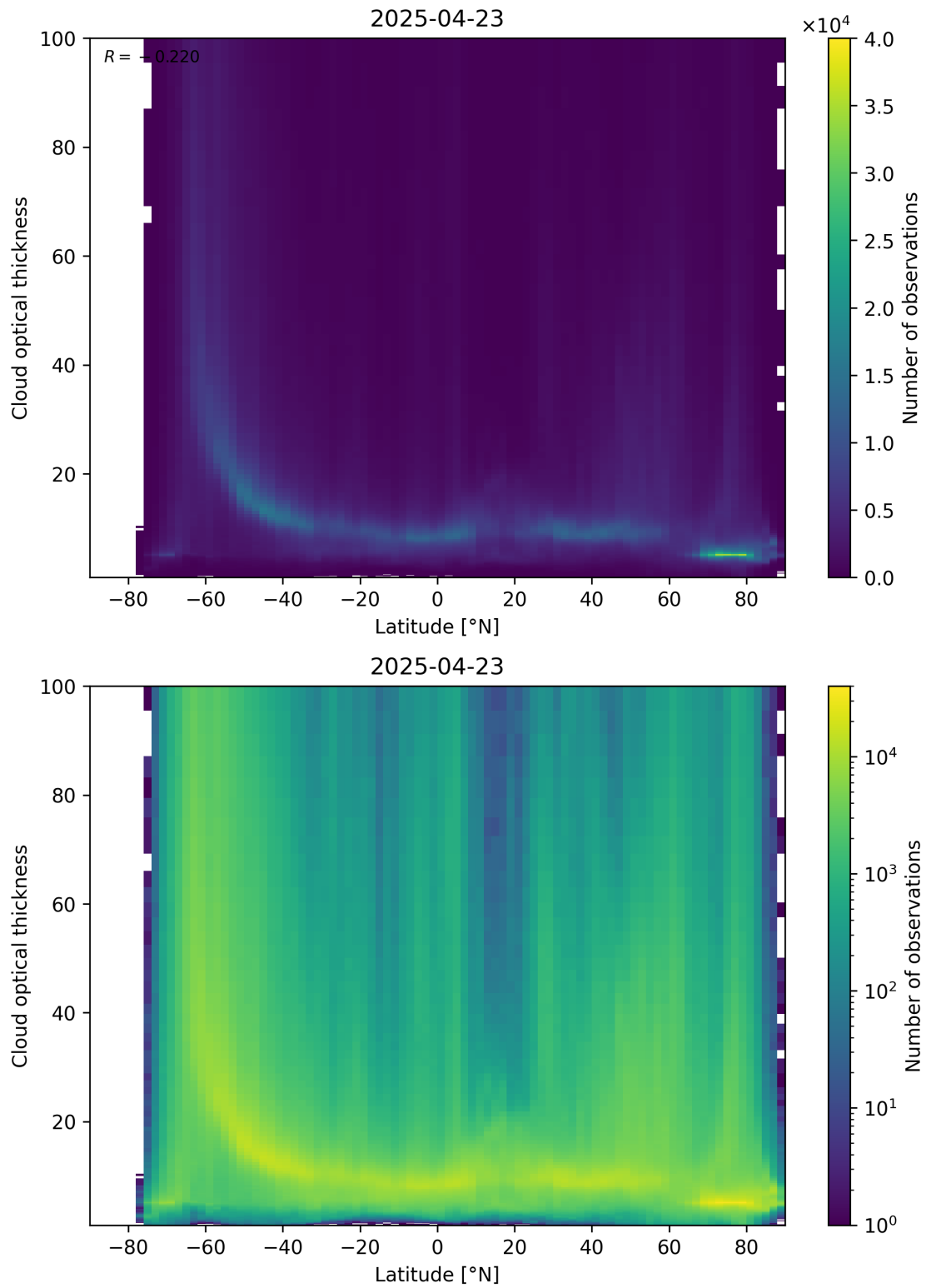
Figure 96: Scatter density plot of “Latitude” against “Cloud optical thickness” for 2025-04-22 to 2025-04-24.
