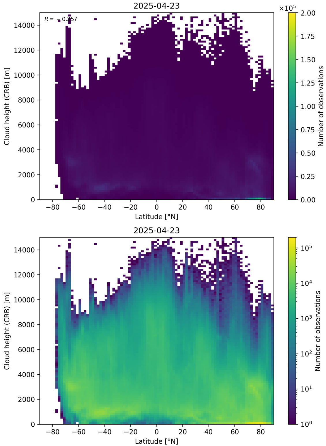
Figure 95: Scatter density plot of “Latitude” against “Cloud height (CRB)” for 2025-04-22 to 2025-04-24.
