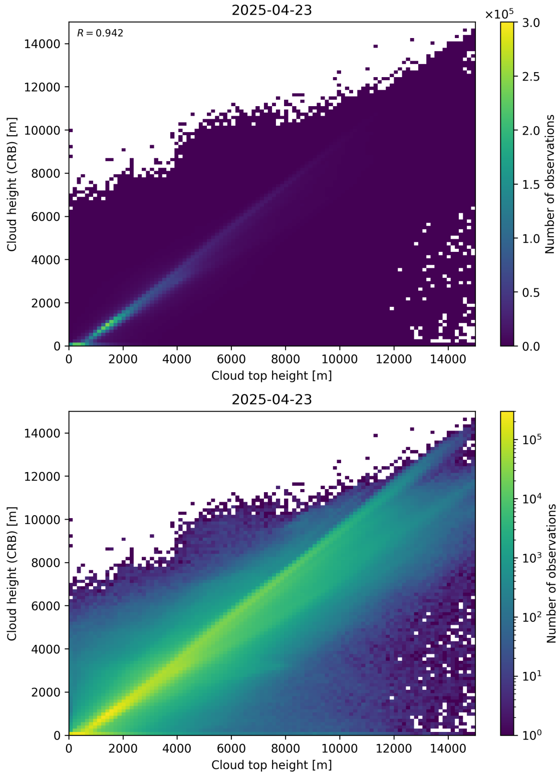
Figure 89: Scatter density plot of “Cloud top height” against “Cloud height (CRB)” for 2025-04-22 to 2025-04-24.
