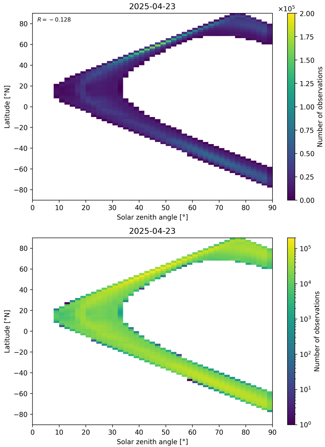
Figure 105: Scatter density plot of “Solar zenith angle” against “Latitude” for 2025-04-22 to 2025-04-24.
