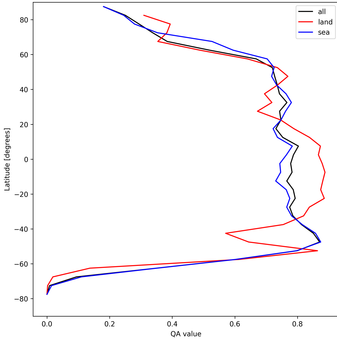
Figure 22: Zonal average of “QA value” for 2025-04-22 to 2025-04-24.
