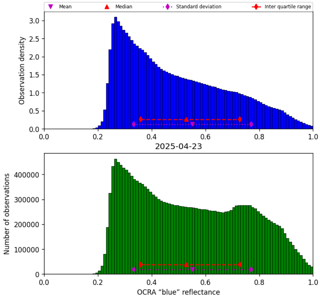
Figure 51: Histogram of “OCRA “blue” reflectance” for 2025-04-22 to 2025-04-24
