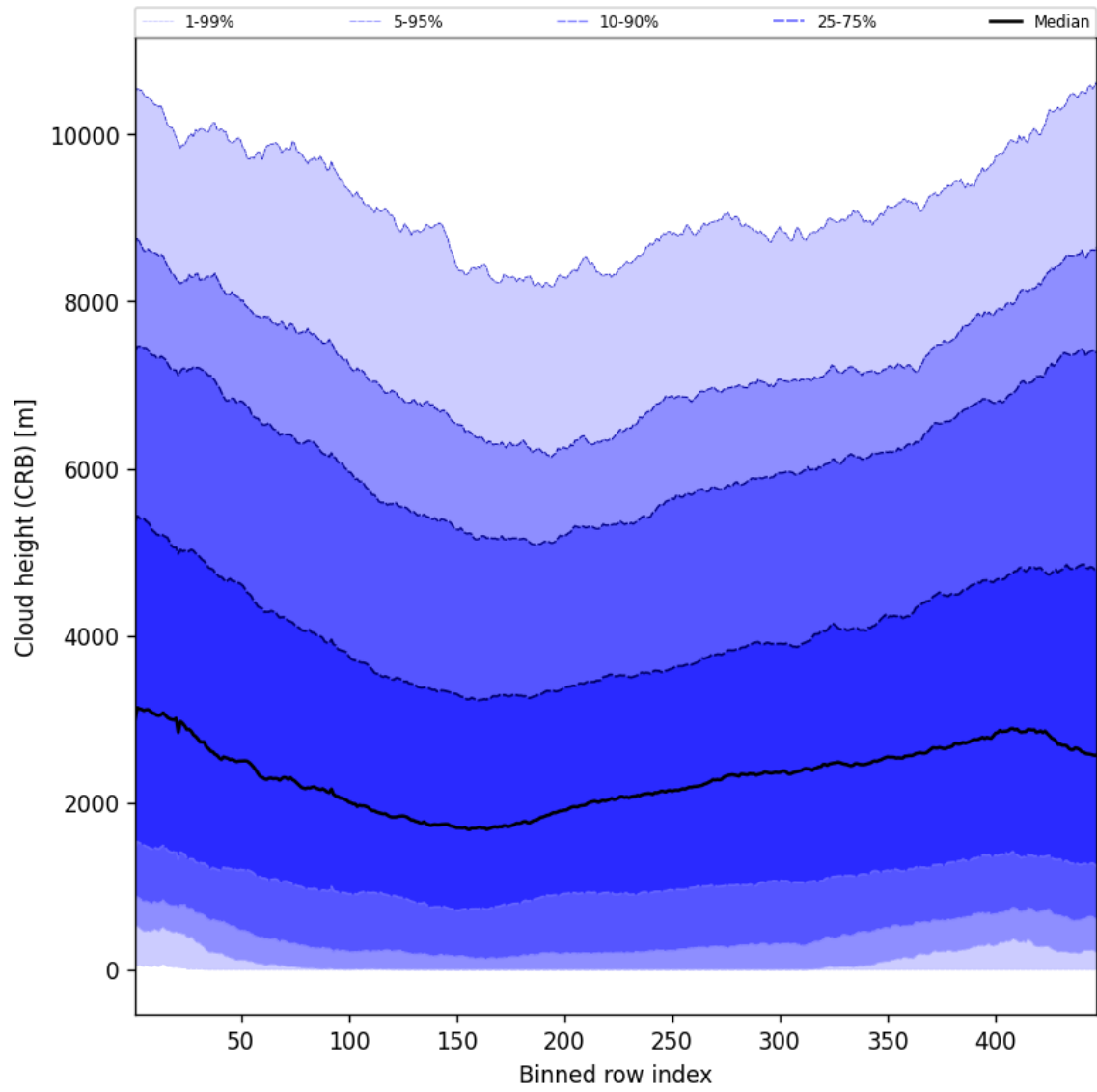
Figure 59: Along track statistics of “Cloud height (CRB)” for 2025-04-22 to 2025-04-24
