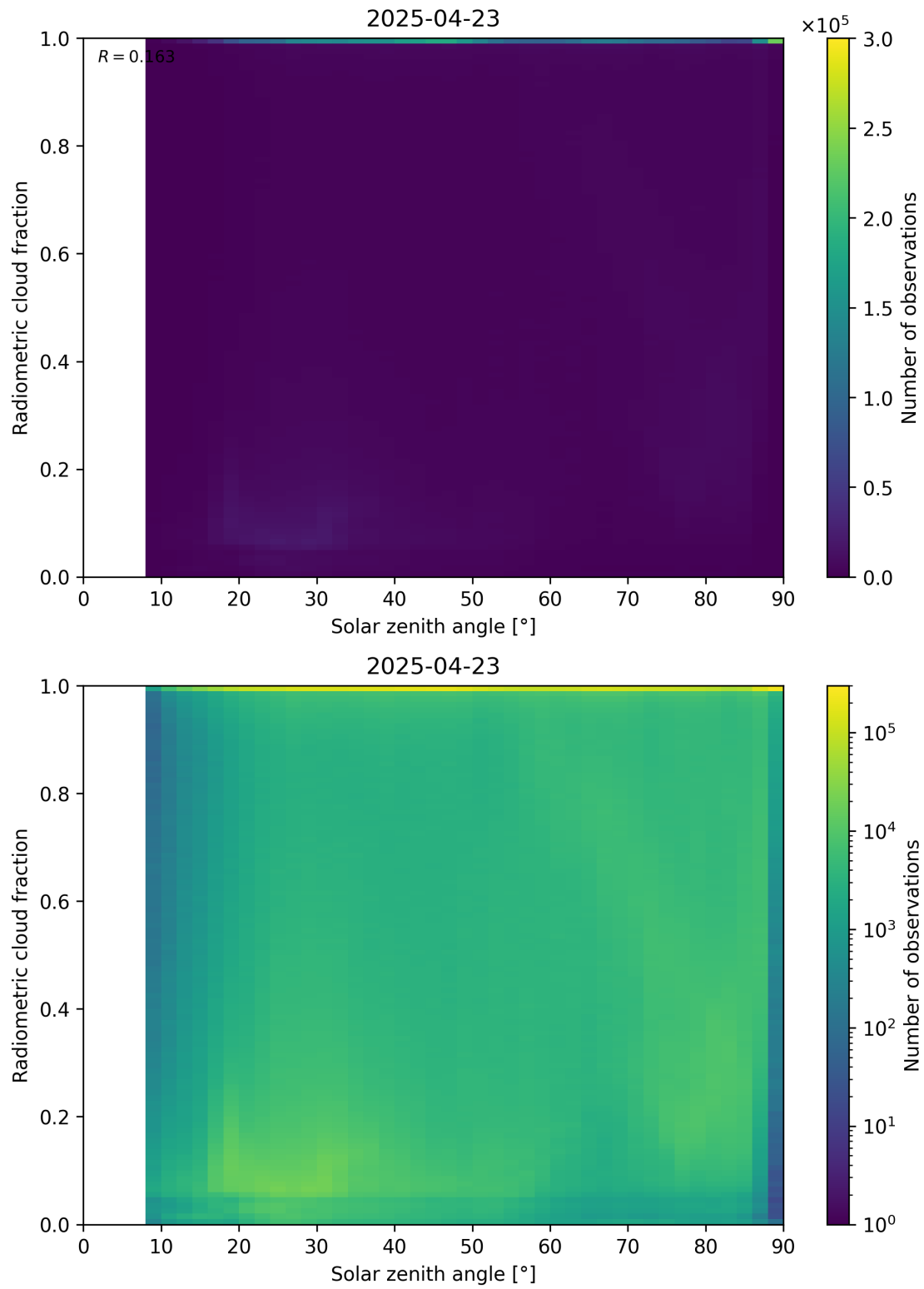
Figure 99: Scatter density plot of “Solar zenith angle” against “Radiometric cloud fraction” for 2025-04-22 to 2025-04-24.
