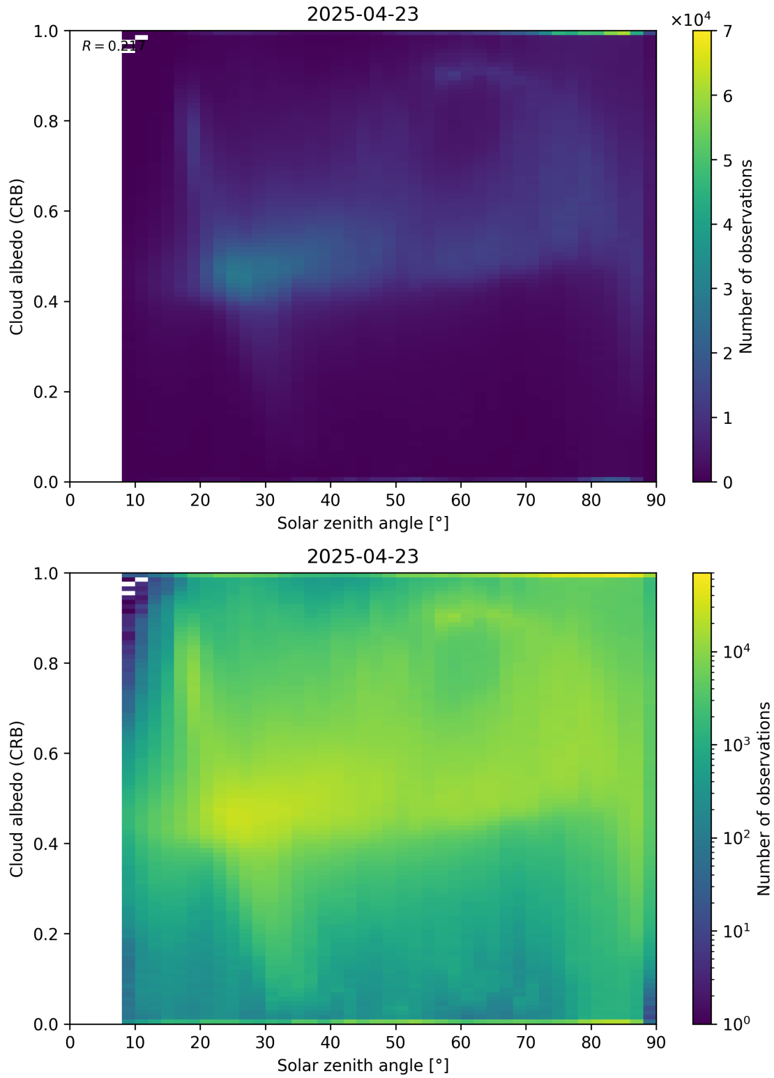
Figure 98: Scatter density plot of “Solar zenith angle” against “Cloud albedo (CRB)” for 2025-04-22 to 2025-04-24.
