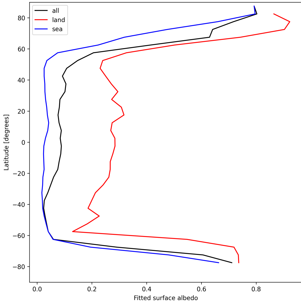
Figure 29: Zonal average of “Fitted surface albedo” for 2025-04-22 to 2025-04-24.
