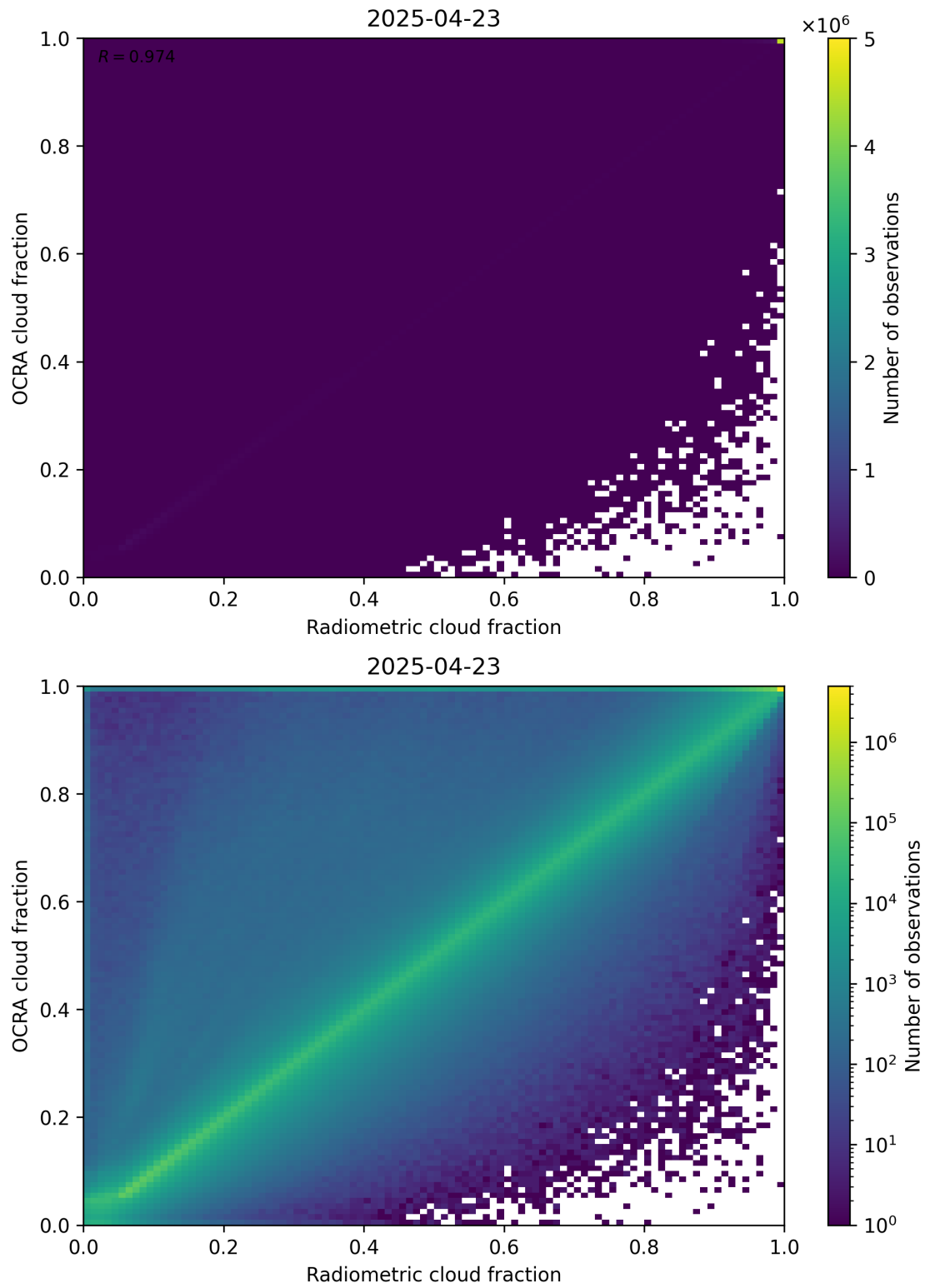
Figure 72: Scatter density plot of “Radiometric cloud fraction” against “OCRA cloud fraction” for 2025-04-22 to 2025-04-24.
