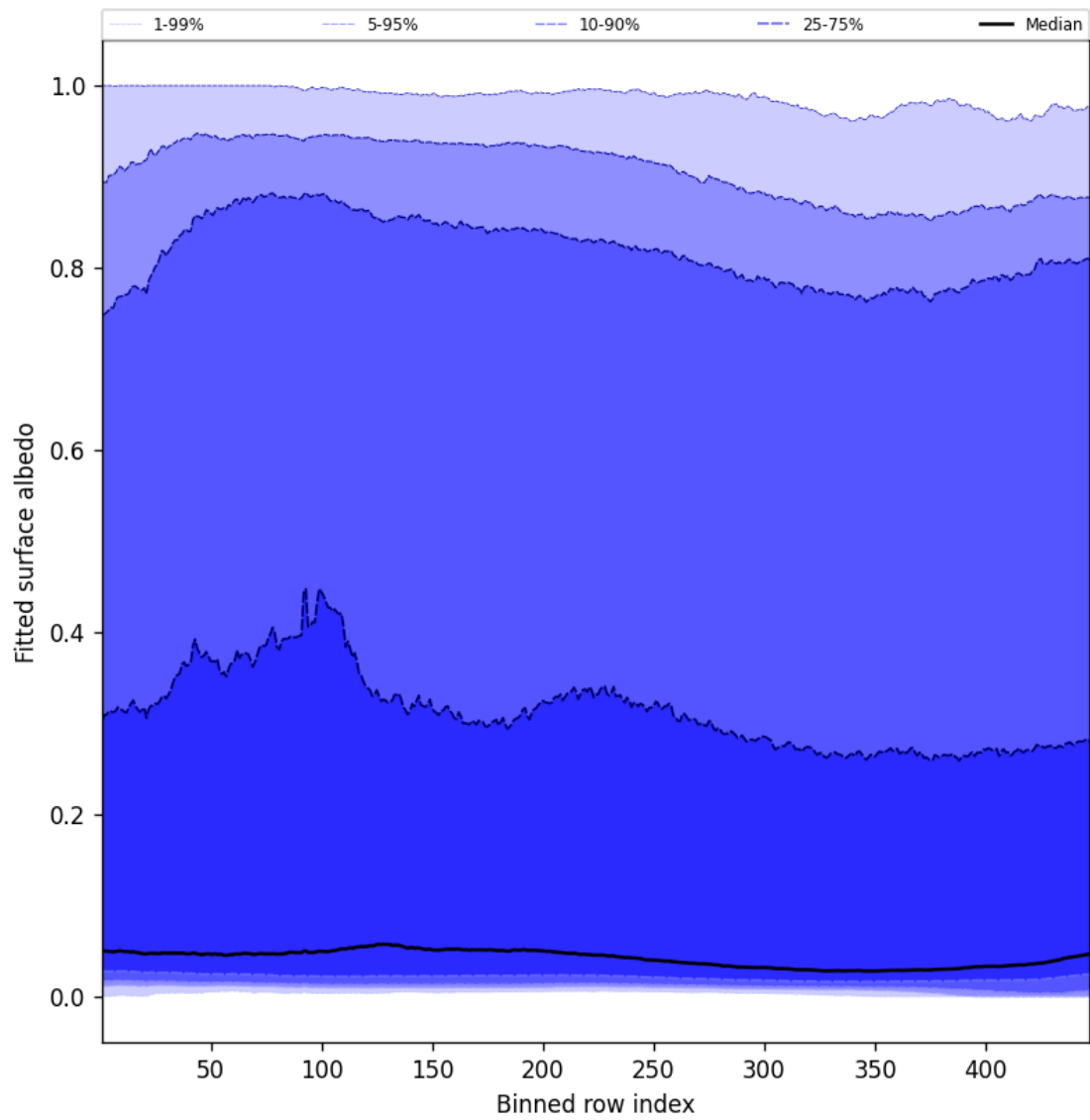
Figure 61: Along track statistics of “Fitted surface albedo” for 2025-04-22 to 2025-04-24
