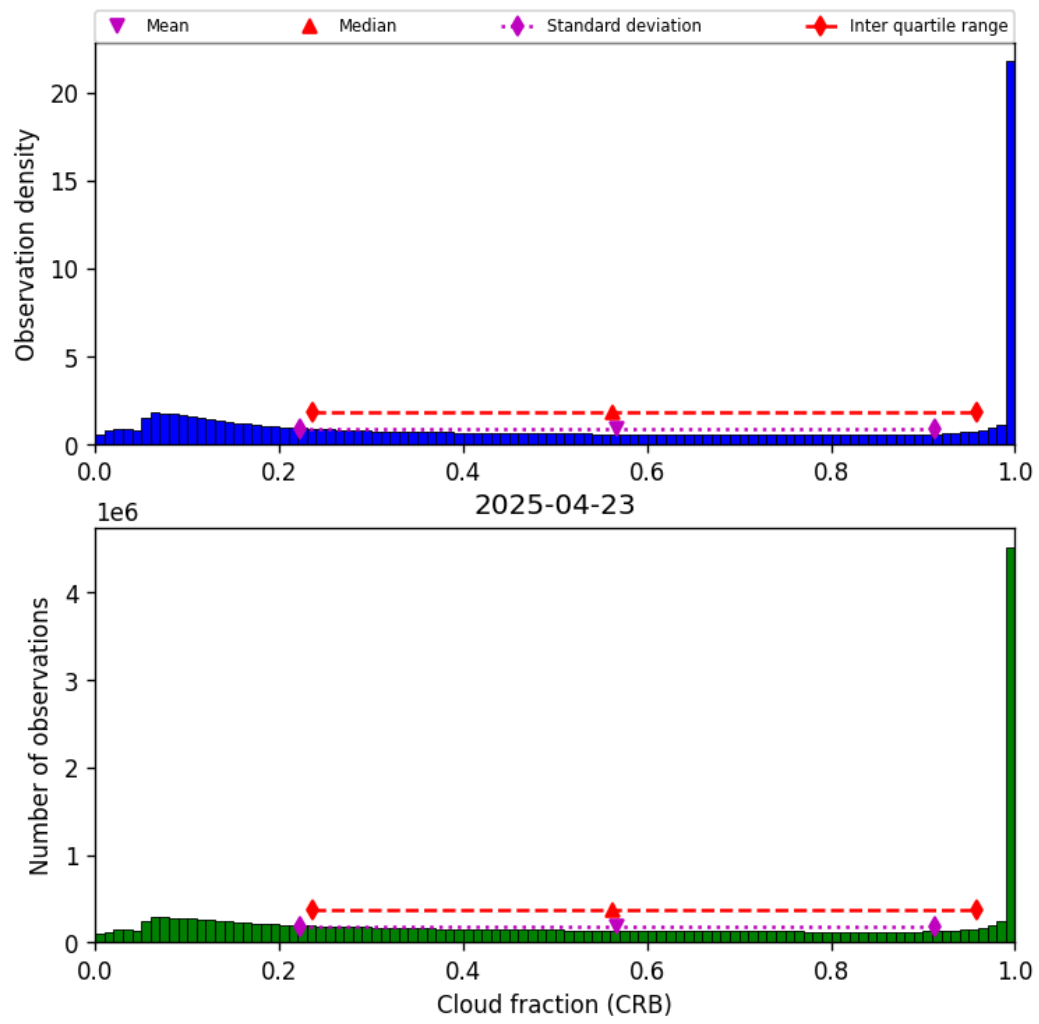
Figure 42: Histogram of “Cloud fraction (CRB)” for 2025-04-22 to 2025-04-24
