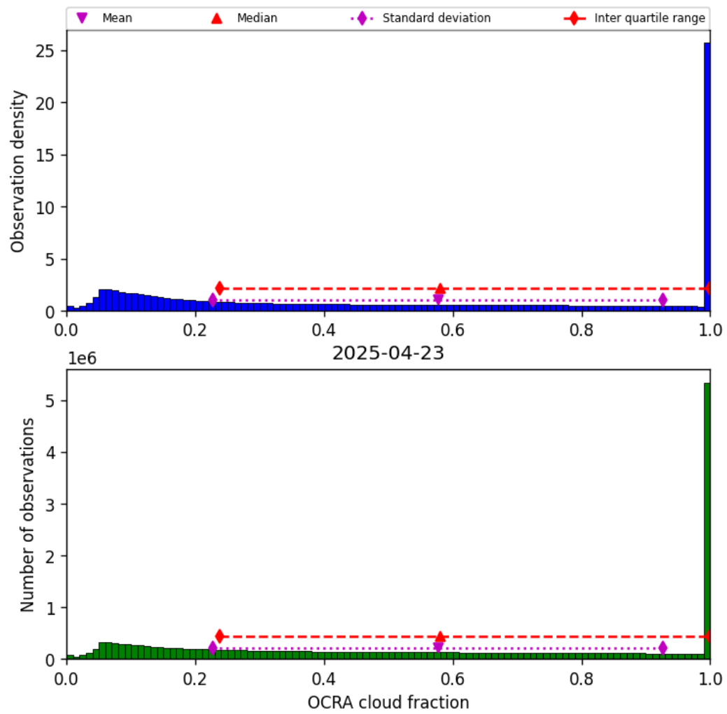
Figure 50: Histogram of “OCRA cloud fraction” for 2025-04-22 to 2025-04-24
