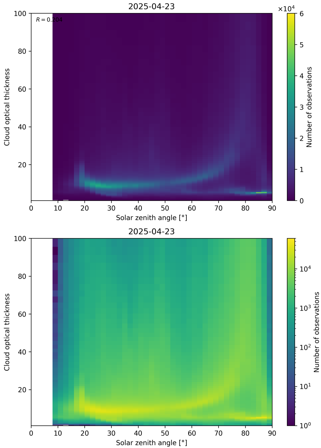
Figure 103: Scatter density plot of “Solar zenith angle” against “Cloud optical thickness” for 2025-04-22 to 2025-04-24.
