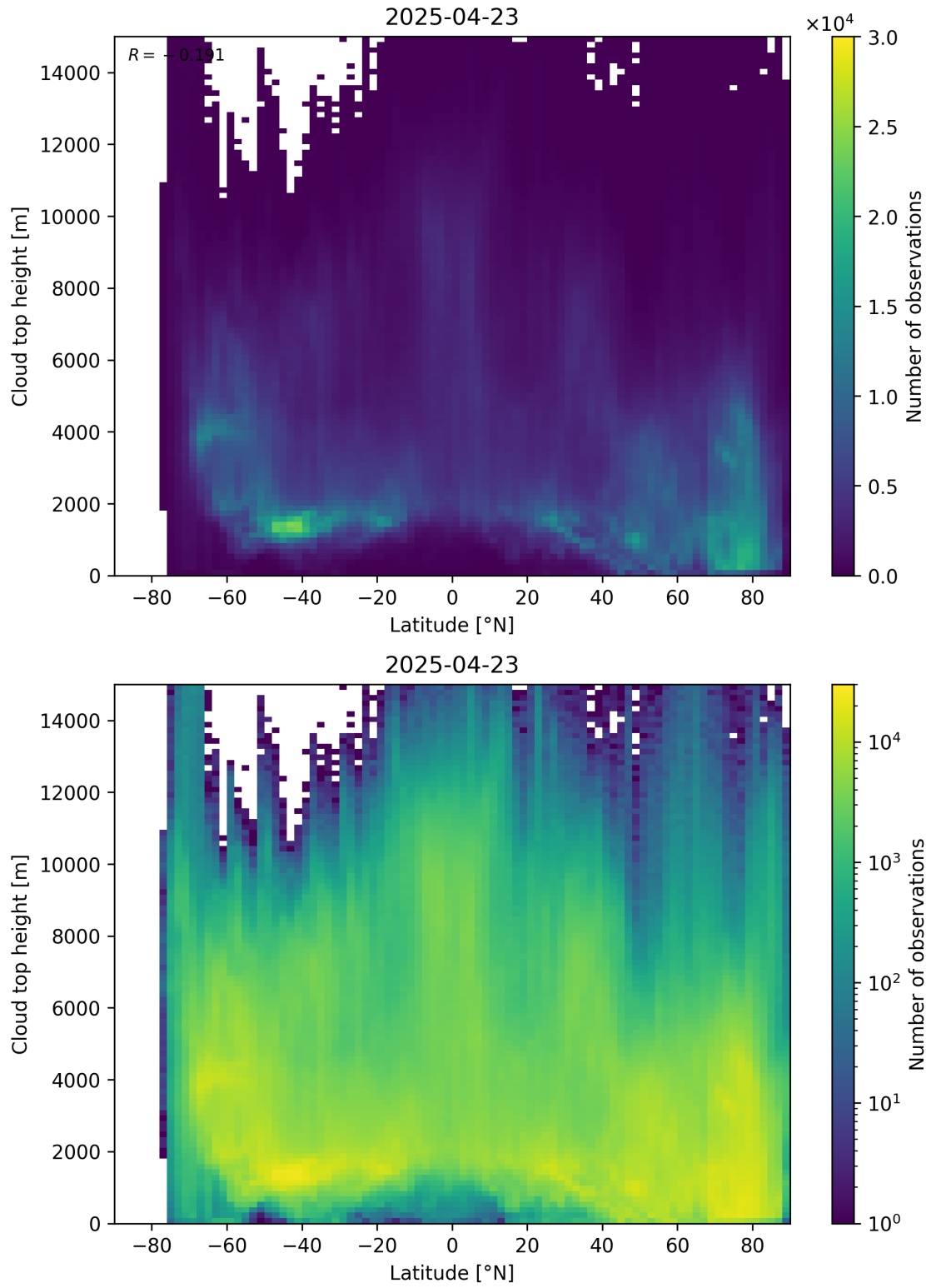
Figure 97: Scatter density plot of “Latitude” against “Cloud top height” for 2025-04-22 to 2025-04-24.
