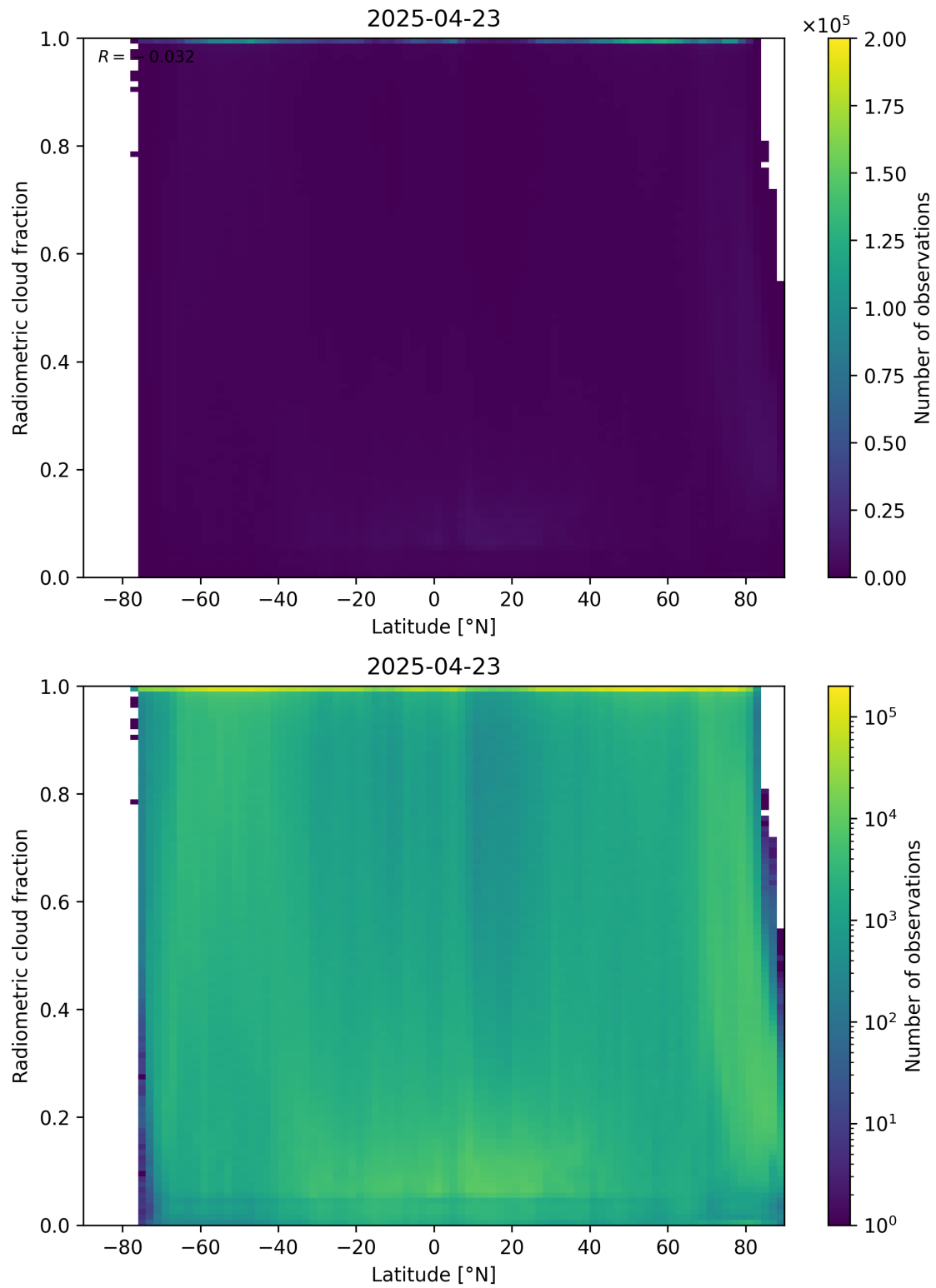
Figure 92: Scatter density plot of “Latitude” against “Radiometric cloud fraction” for 2025-04-22 to 2025-04-24.
