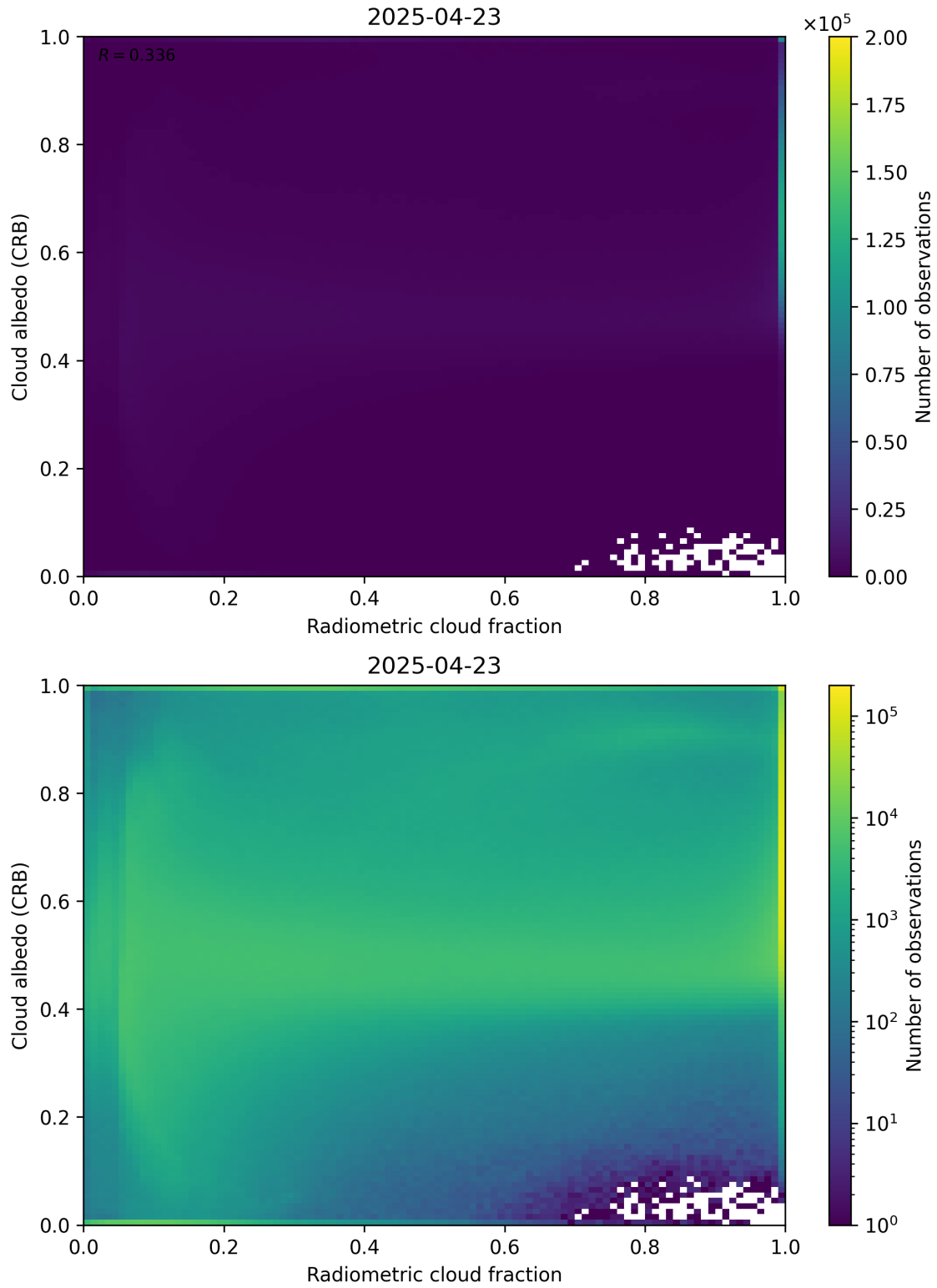
Figure 71: Scatter density plot of “Radiometric cloud fraction” against “Cloud albedo (CRB)” for 2025-04-22 to 2025-04-24.
