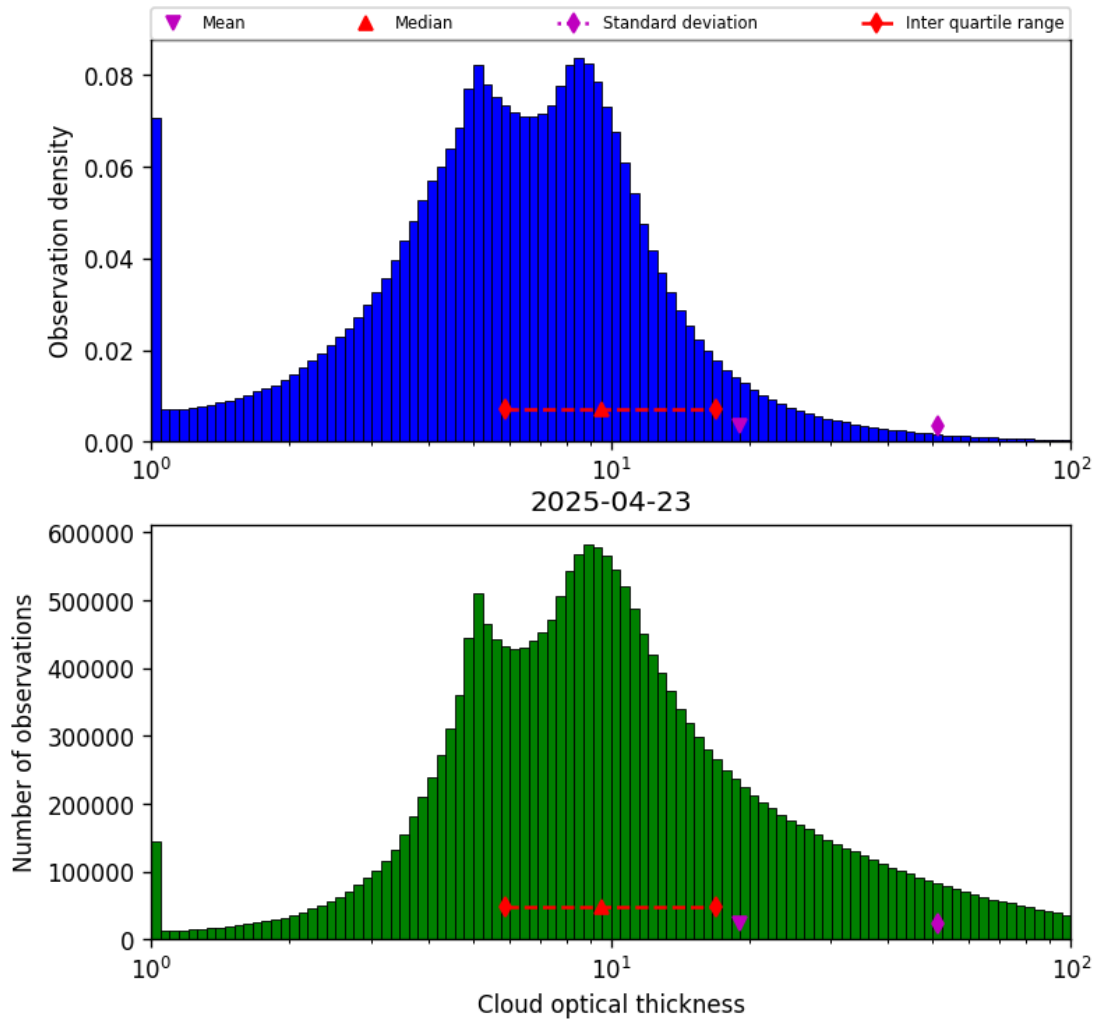
Figure 41: Histogram of “Cloud optical thickness” for 2025-04-22 to 2025-04-24
