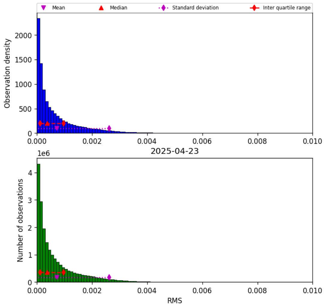
Figure 47: Histogram of “RMS” for 2025-04-22 to 2025-04-24
