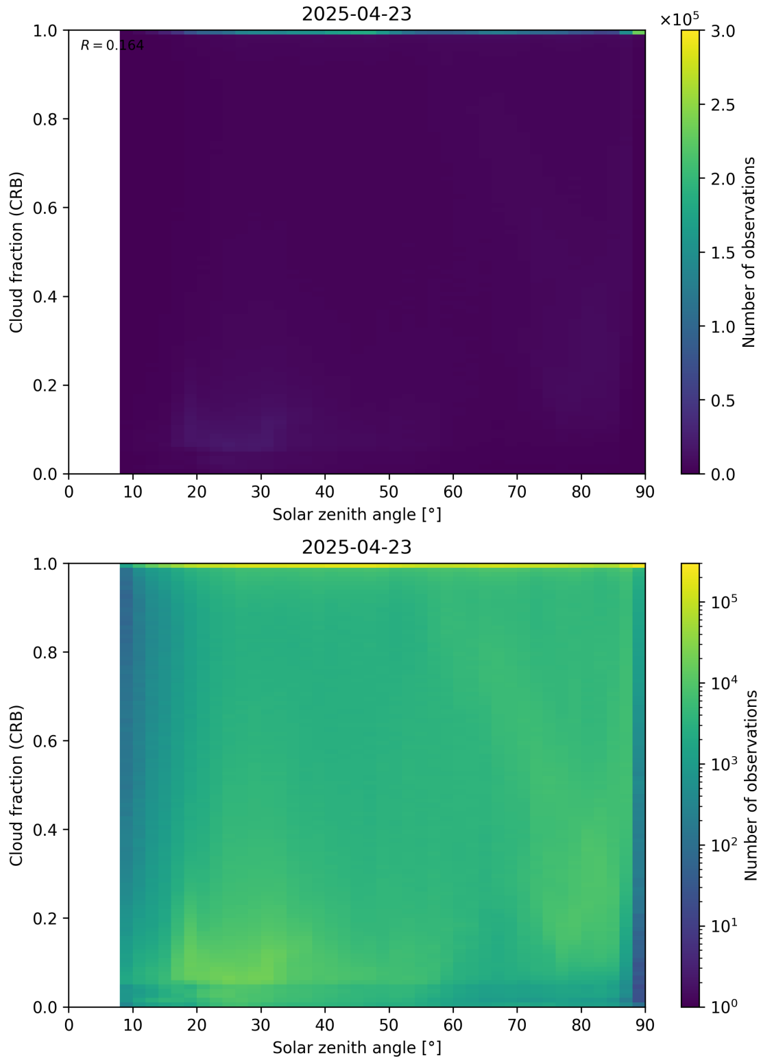
Figure 101: Scatter density plot of “Solar zenith angle” against “Cloud fraction (CRB)” for 2025-04-22 to 2025-04-24.
