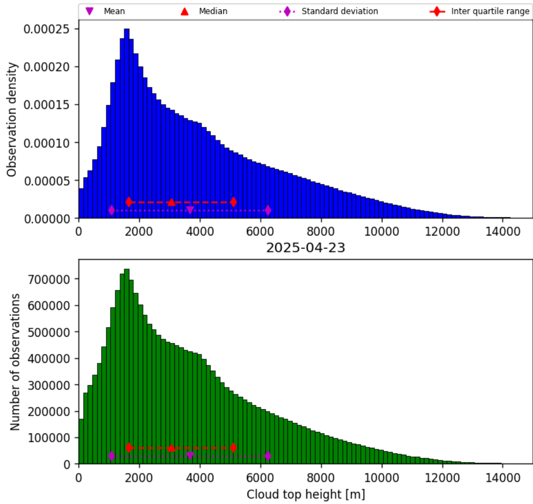
Figure 40: Histogram of “Cloud top height” for 2025-04-22 to 2025-04-24
