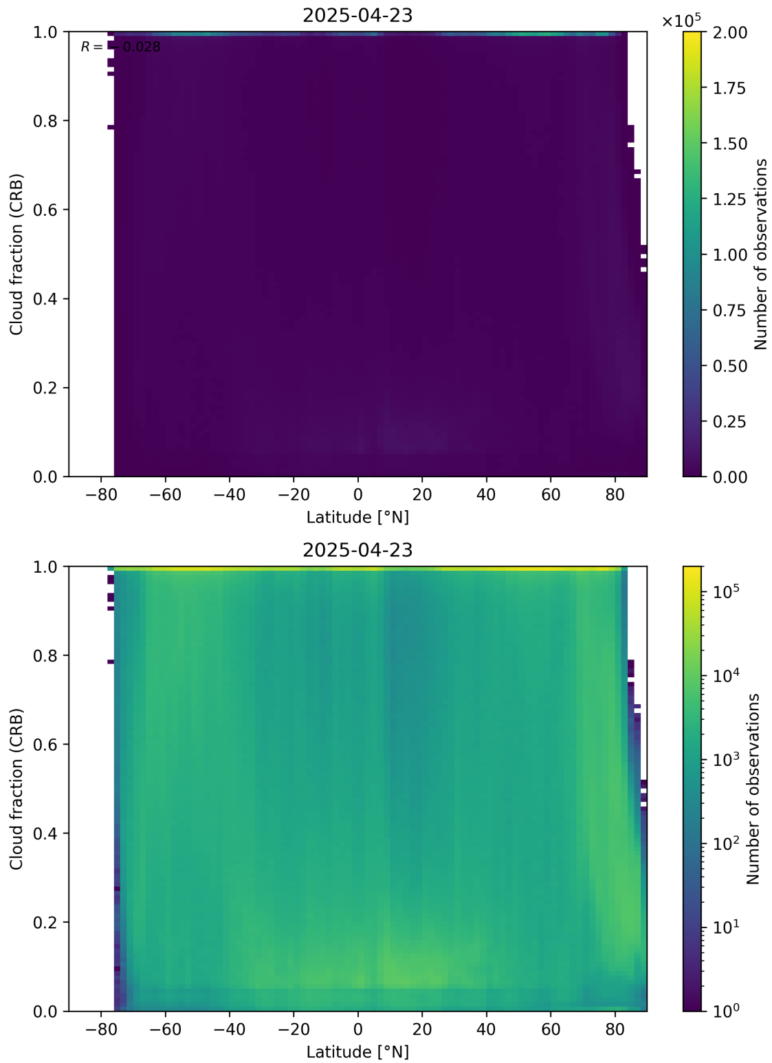
Figure 94: Scatter density plot of “Latitude” against “Cloud fraction (CRB)” for 2025-04-22 to 2025-04-24.
