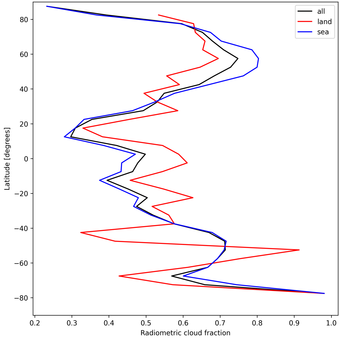
Figure 23: Zonal average of “Radiometric cloud fraction” for 2025-04-22 to 2025-04-24.
