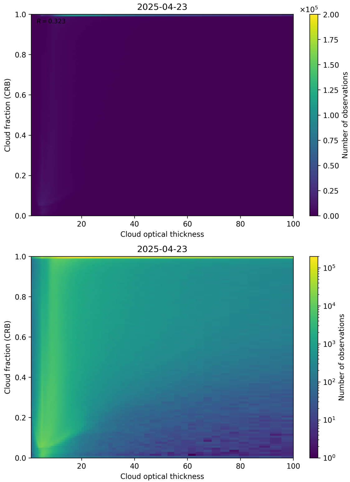
Figure 84: Scatter density plot of “Cloud optical thickness” against “Cloud fraction (CRB)” for 2025-04-22 to 2025-04-24.
