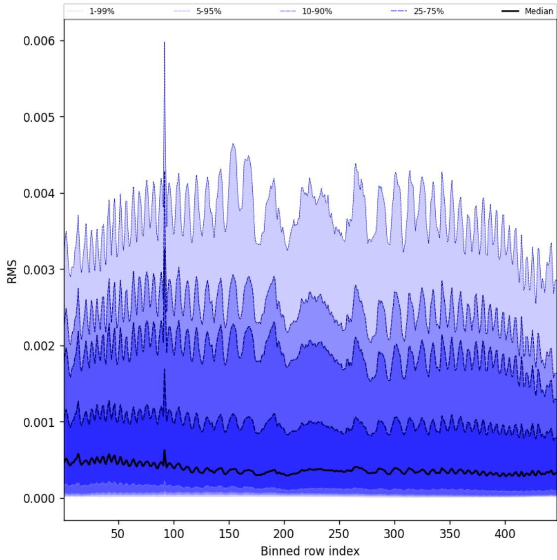
Figure 63: Along track statistics of “RMS” for 2025-04-22 to 2025-04-24
