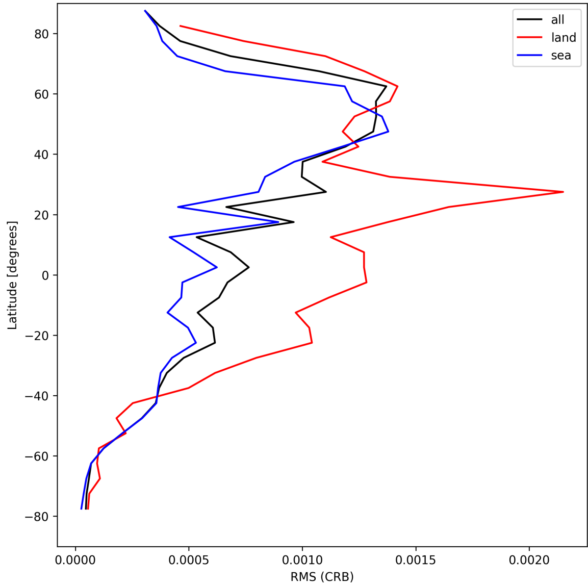
Figure 32: Zonal average of “RMS (CRB)” for 2025-04-22 to 2025-04-24.
