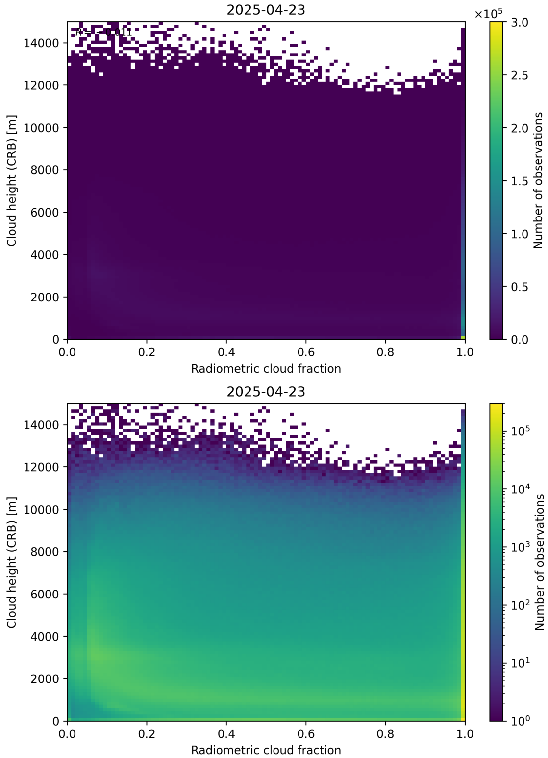
Figure 74: Scatter density plot of “Radiometric cloud fraction” against “Cloud height (CRB)” for 2025-04-22 to 2025-04-24.
