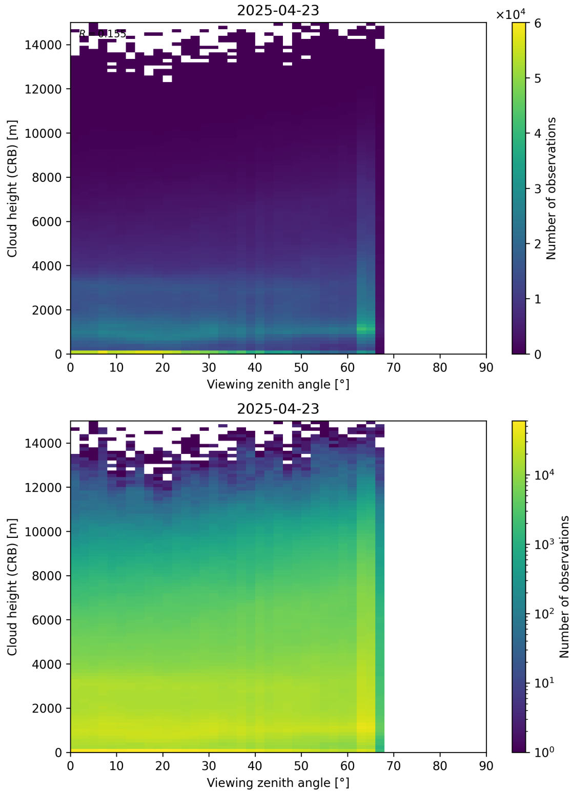
Figure 110: Scatter density plot of “Viewing zenith angle” against “Cloud height (CRB)” for 2025-04-22 to 2025-04-24.
