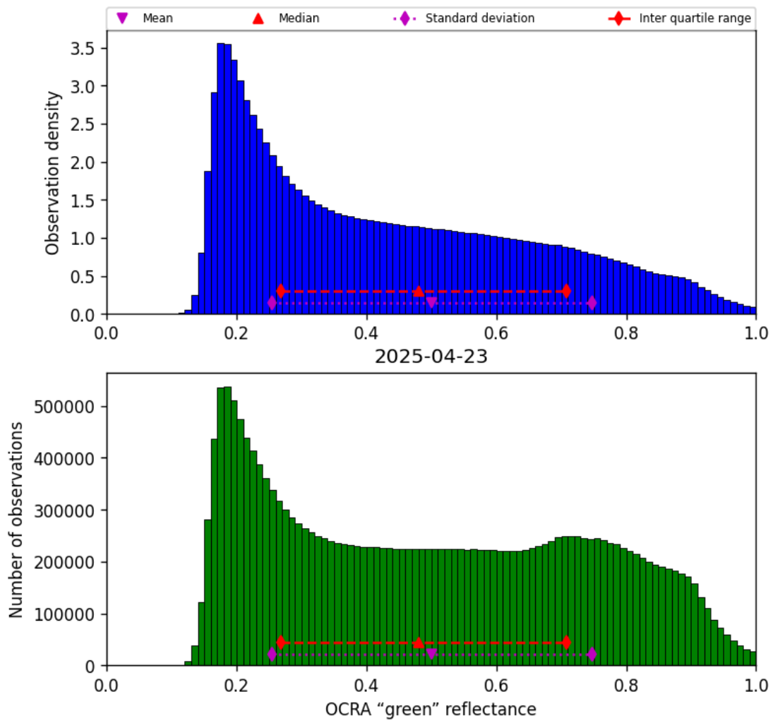
Figure 52: Histogram of “OCRA “green” reflectance” for 2025-04-22 to 2025-04-24
