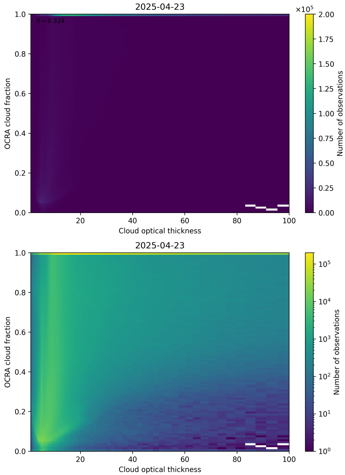
Figure 83: Scatter density plot of “Cloud optical thickness” against “OCRA cloud fraction” for 2025-04-22 to 2025-04-24.
