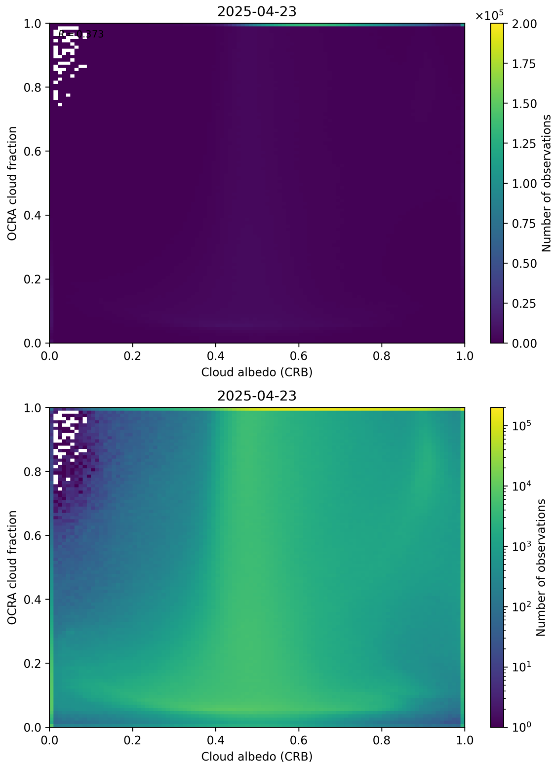
Figure 70: Scatter density plot of “Cloud albedo (CRB)” against “OCRA cloud fraction” for 2025-04-22 to 2025-04-24.
