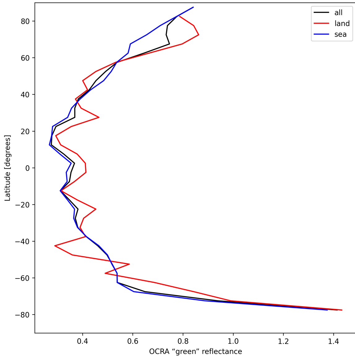
Figure 36: Zonal average of “OCRA “green” reflectance” for 2025-04-22 to 2025-04-24.
