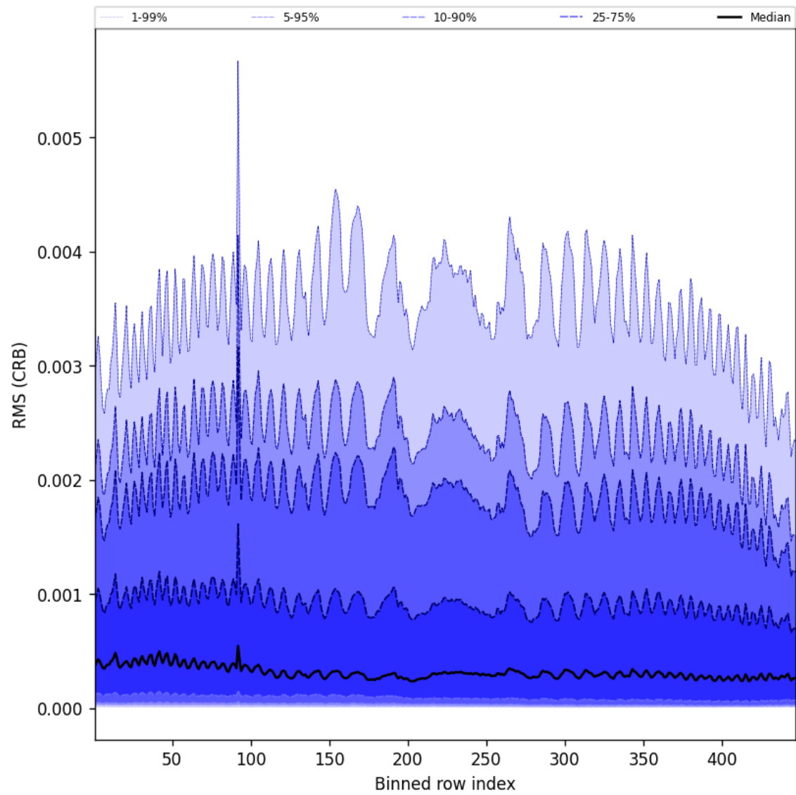
Figure 64: Along track statistics of “RMS (CRB)” for 2025-04-22 to 2025-04-24
