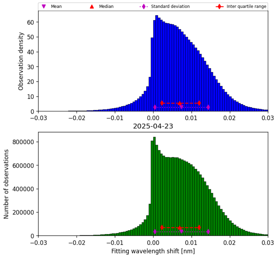
Figure 49: Histogram of “Fitting wavelength shift” for 2025-04-22 to 2025-04-24
