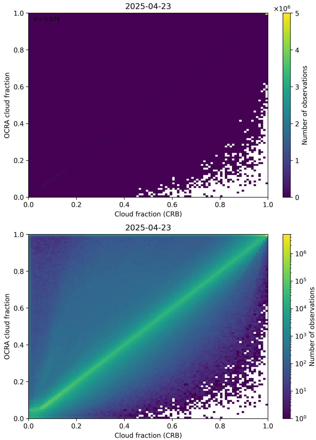
Figure 78: Scatter density plot of “Cloud fraction (CRB)” against “OCRA cloud fraction” for 2025-04-22 to 2025-04-24.
