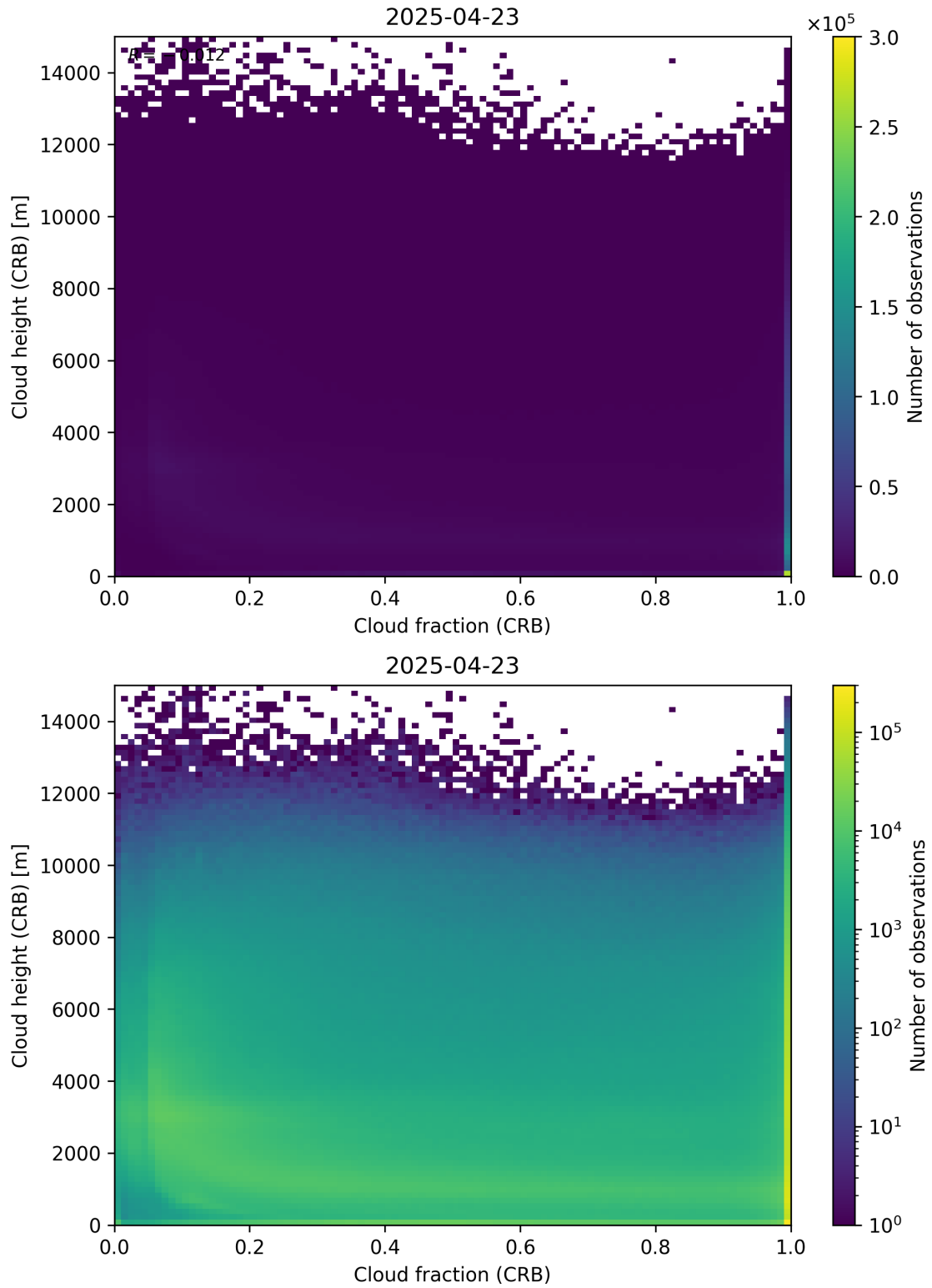
Figure 79: Scatter density plot of “Cloud fraction (CRB)” against “Cloud height (CRB)” for 2025-04-22 to 2025-04-24.
