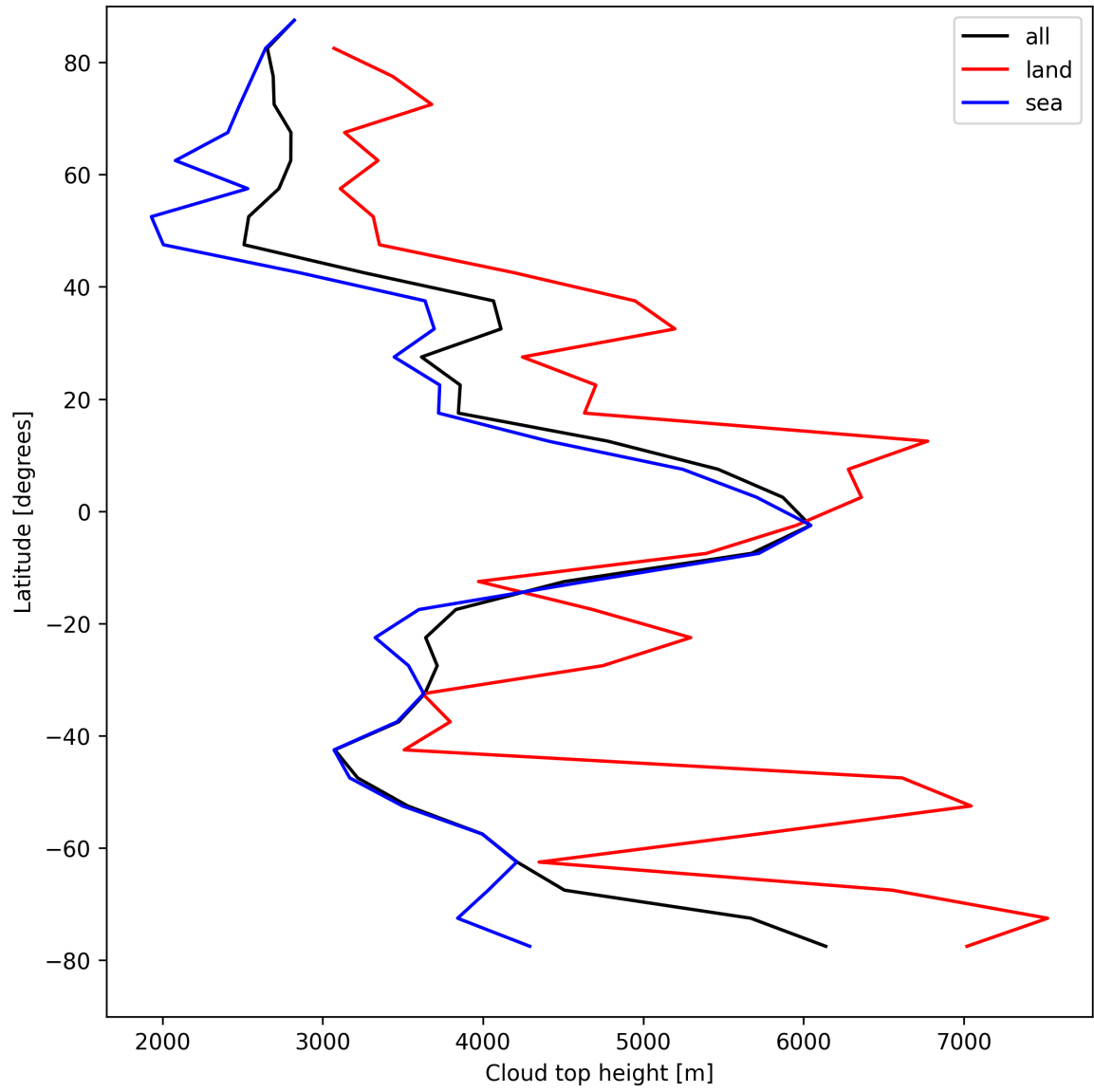
Figure 24: Zonal average of “Cloud top height” for 2025-04-22 to 2025-04-24.
