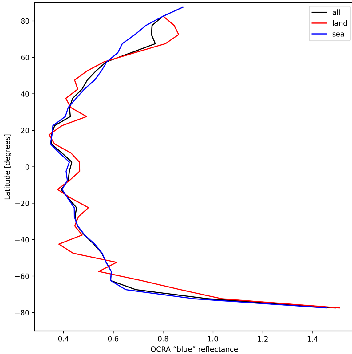
Figure 35: Zonal average of “OCRA “blue” reflectance” for 2025-04-22 to 2025-04-24.
