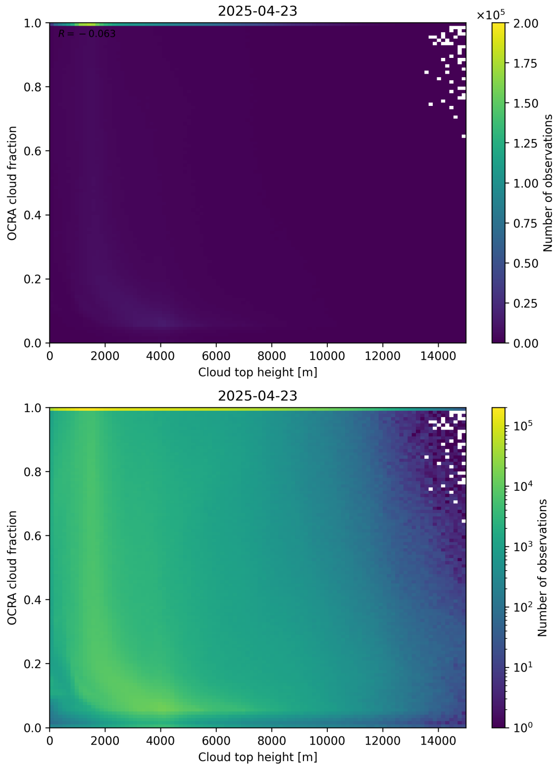
Figure 87: Scatter density plot of “Cloud top height” against “OCRA cloud fraction” for 2025-04-22 to 2025-04-24.
