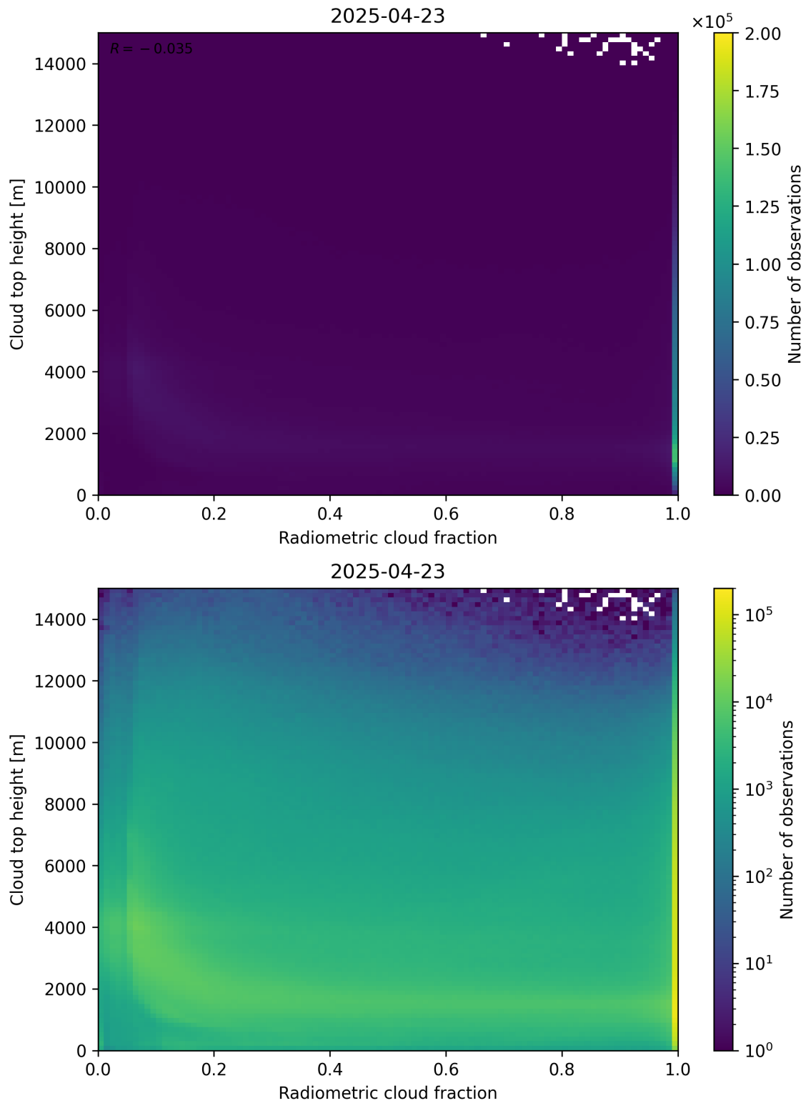
Figure 76: Scatter density plot of “Radiometric cloud fraction” against “Cloud top height” for 2025-04-22 to 2025-04-24.
