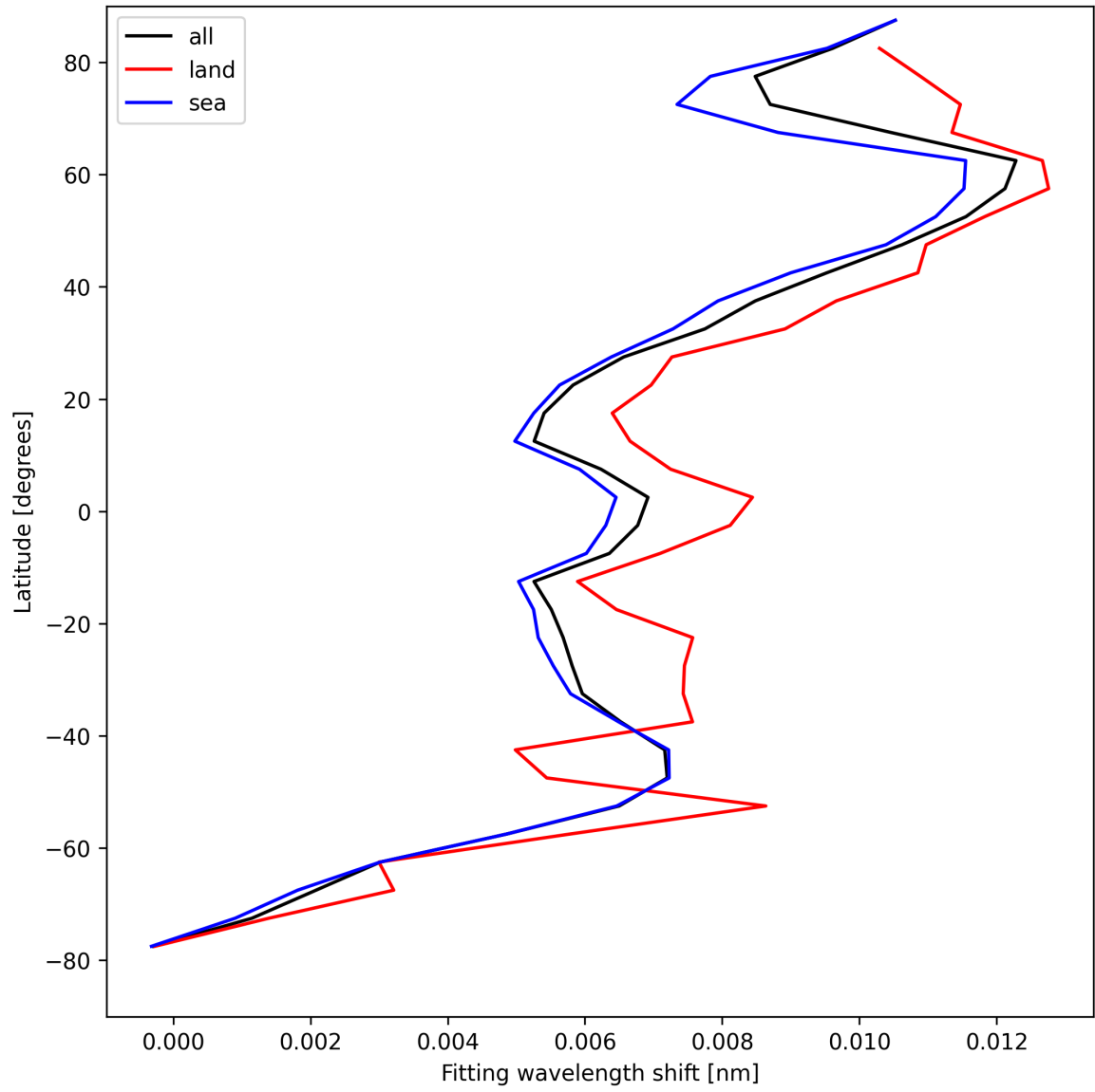
Figure 33: Zonal average of “Fitting wavelength shift” for 2025-04-22 to 2025-04-24.
