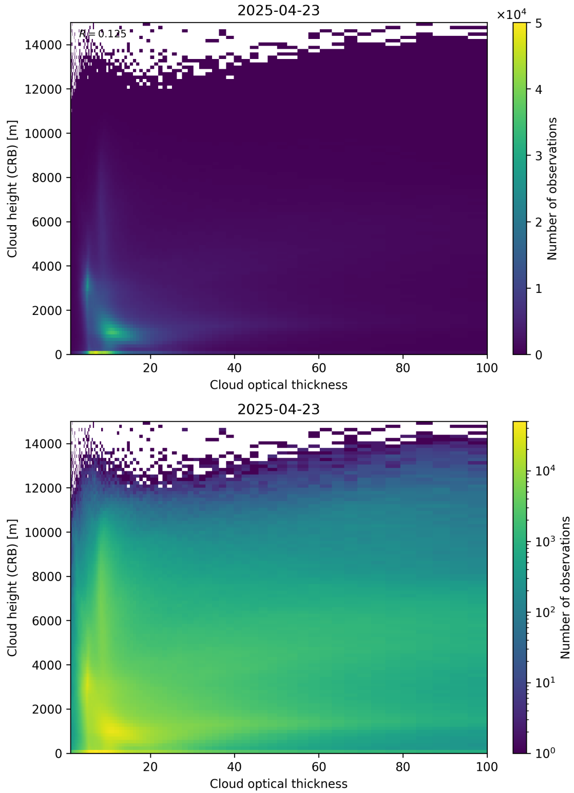
Figure 85: Scatter density plot of “Cloud optical thickness” against “Cloud height (CRB)” for 2025-04-22 to 2025-04-24.
