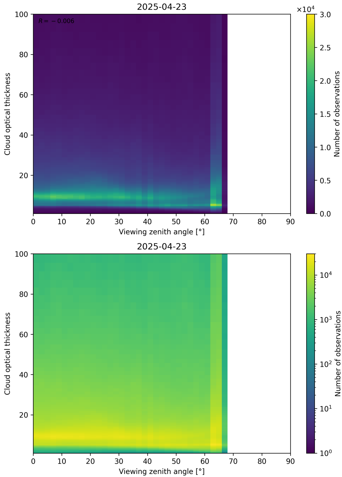
Figure 111: Scatter density plot of “Viewing zenith angle” against “Cloud optical thickness” for 2025-04-22 to 2025-04-24.
