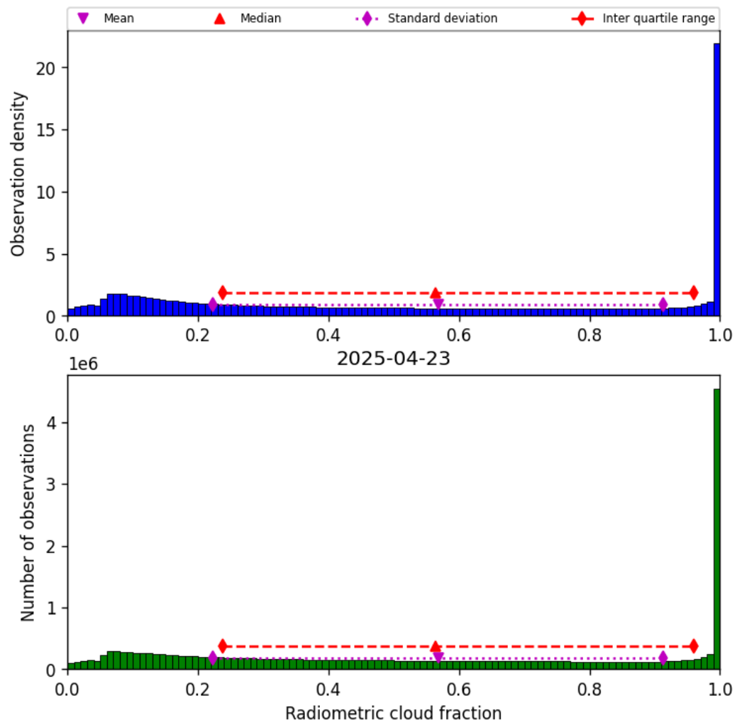
Figure 39: Histogram of “Radiometric cloud fraction” for 2025-04-22 to 2025-04-24
