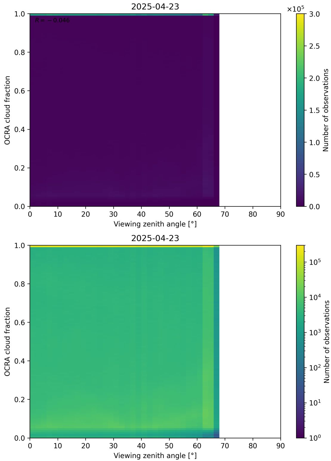
Figure 108: Scatter density plot of “Viewing zenith angle” against “OCRA cloud fraction” for 2025-04-22 to 2025-04-24.
