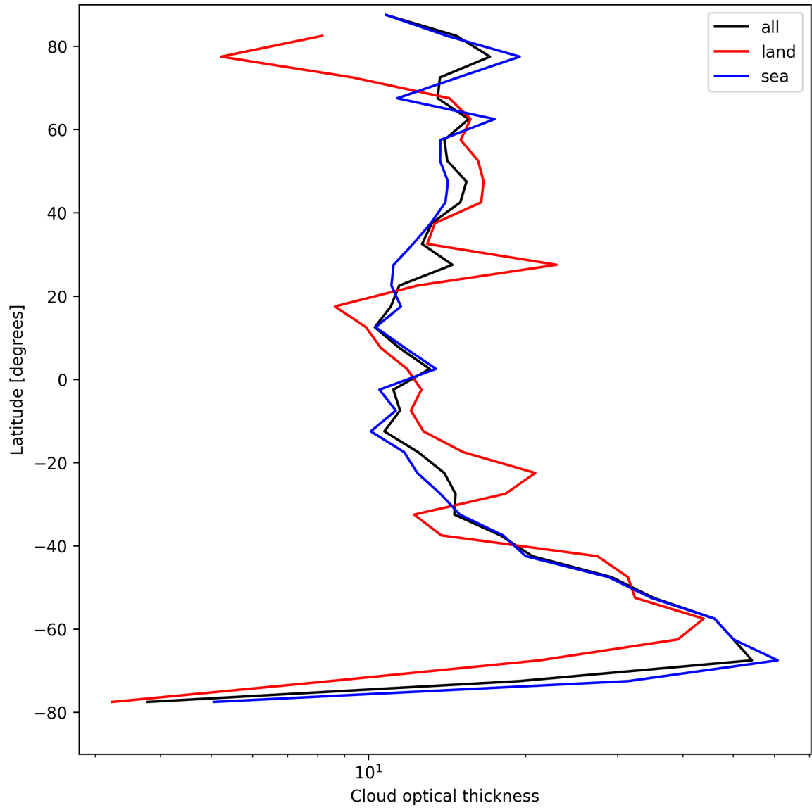
Figure 25: Zonal average of “Cloud optical thickness” for 2025-04-24 to 2025-04-25.
