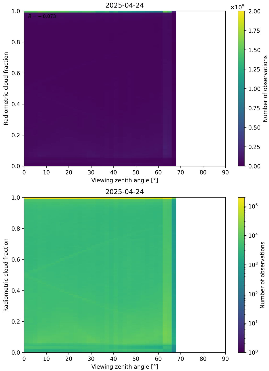
Figure 107: Scatter density plot of “Viewing zenith angle” against “Radiometric cloud fraction” for 2025-04-24 to 2025-04-25.
