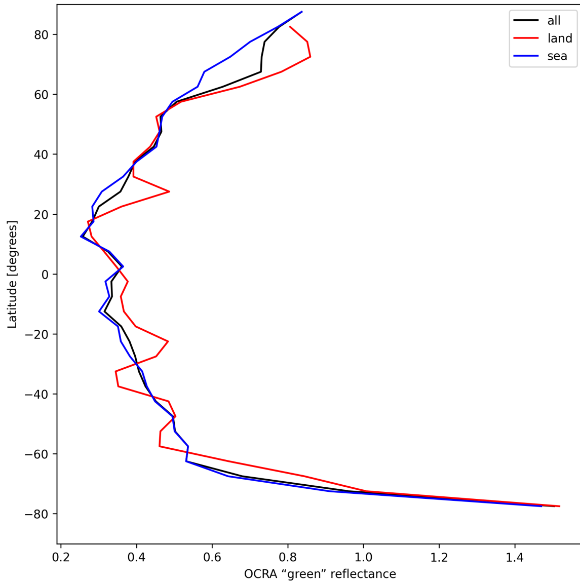
Figure 36: Zonal average of “OCRA “green” reflectance” for 2025-04-24 to 2025-04-25.
