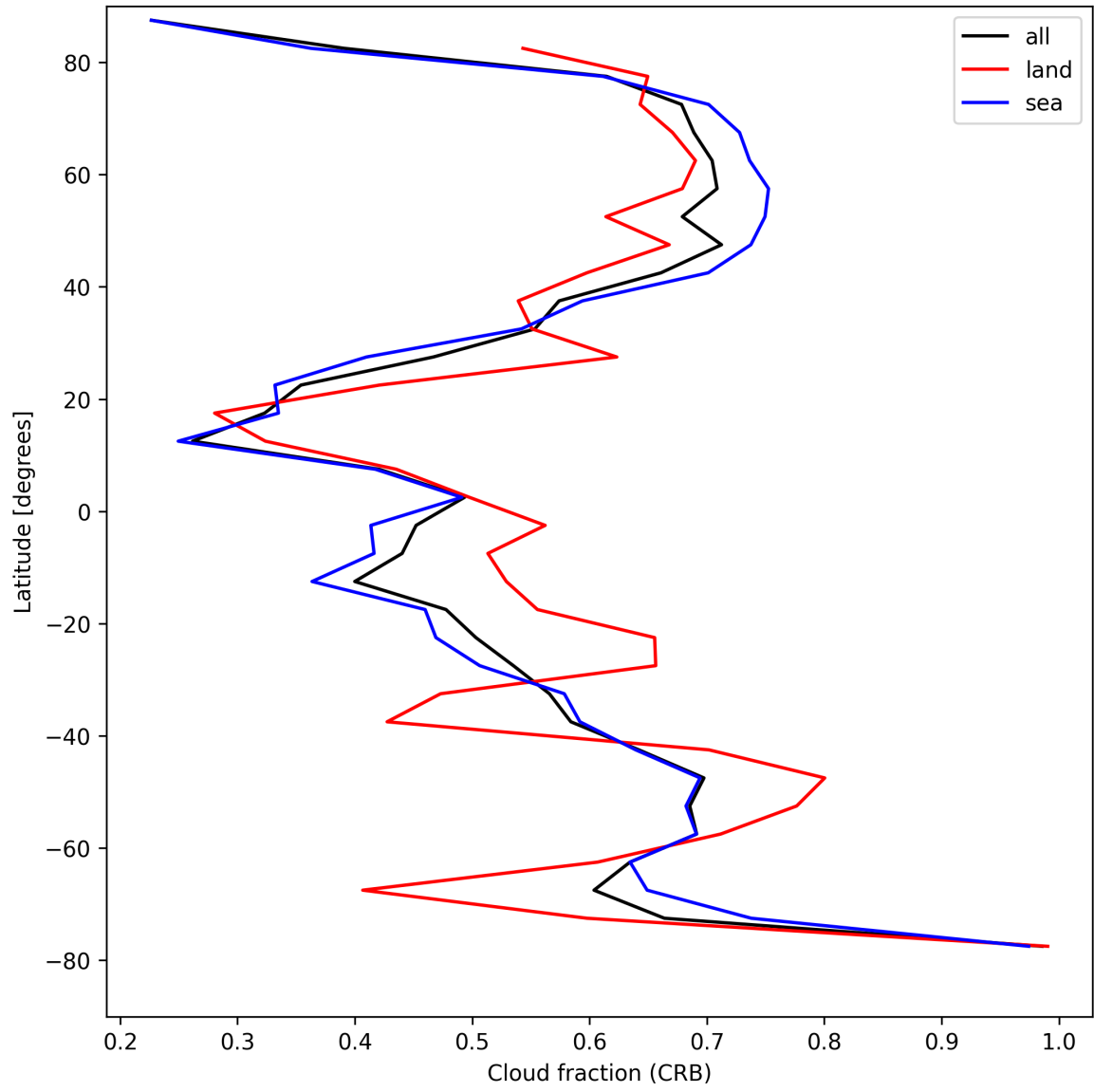
Figure 26: Zonal average of “Cloud fraction (CRB)” for 2025-04-24 to 2025-04-25.
