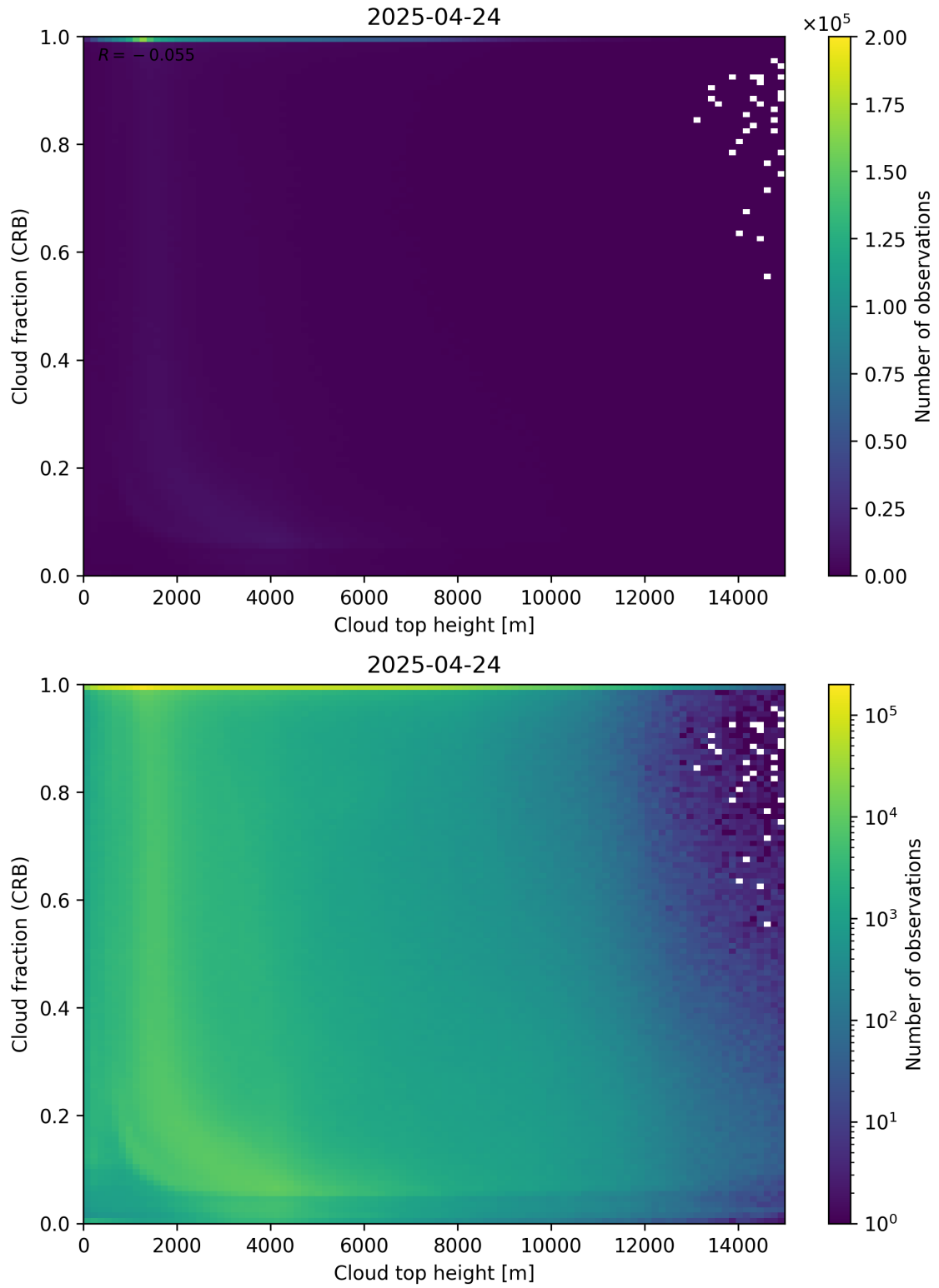
Figure 88: Scatter density plot of “Cloud top height” against “Cloud fraction (CRB)” for 2025-04-24 to 2025-04-25.
