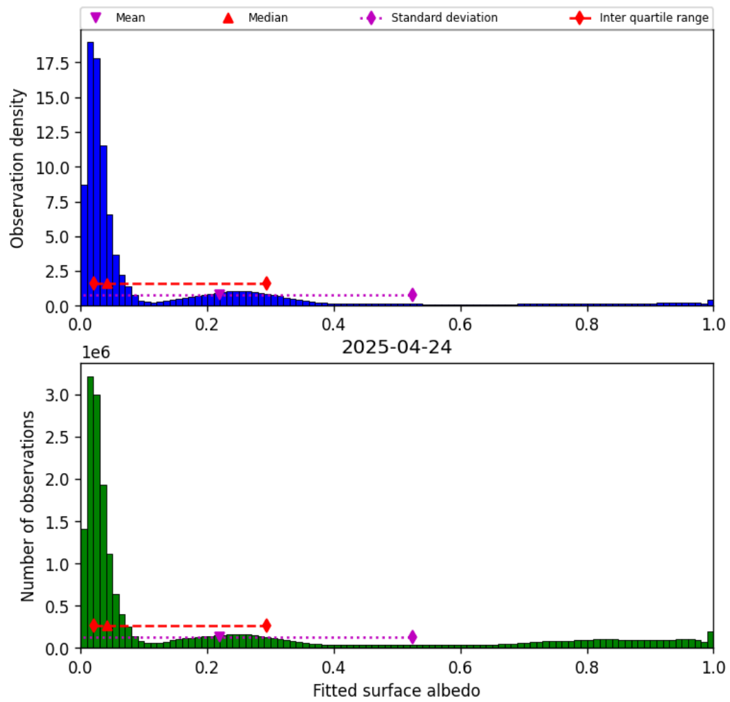
Figure 45: Histogram of “Fitted surface albedo” for 2025-04-24 to 2025-04-25
