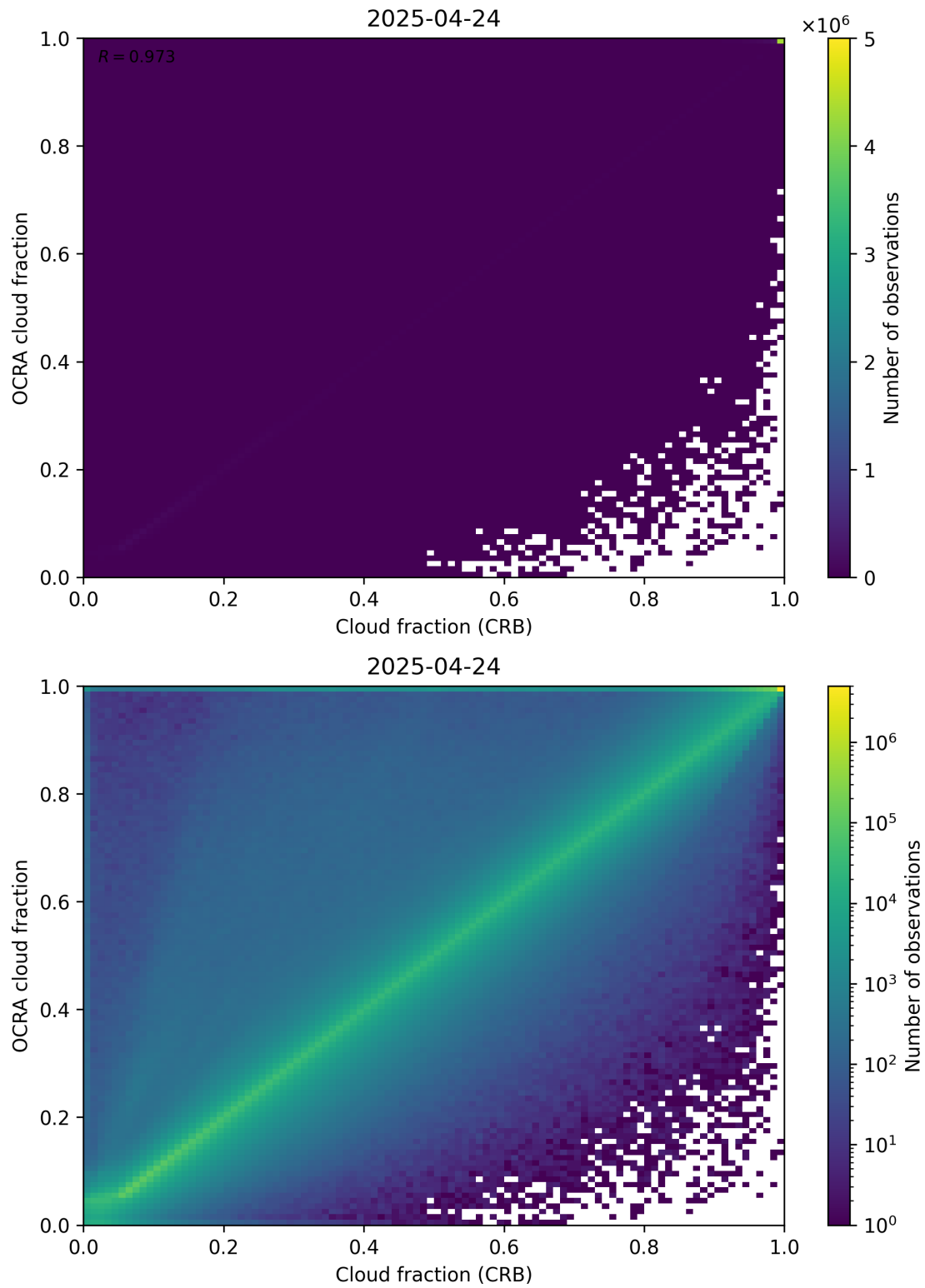
Figure 78: Scatter density plot of “Cloud fraction (CRB)” against “OCRA cloud fraction” for 2025-04-24 to 2025-04-25.
