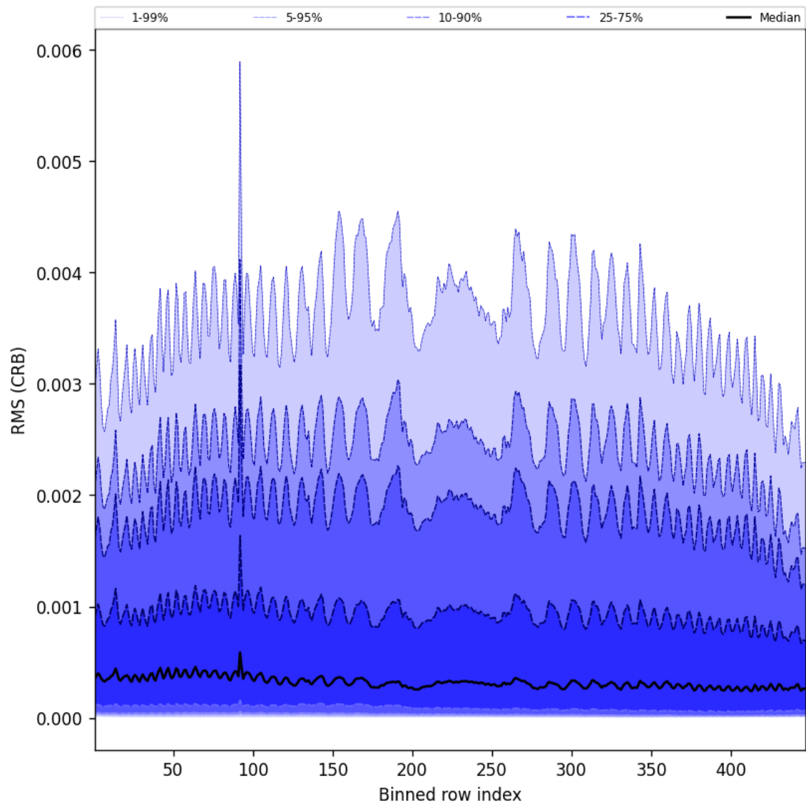
Figure 64: Along track statistics of “RMS (CRB)” for 2025-04-24 to 2025-04-25
