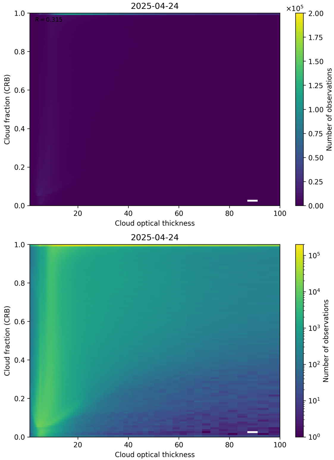
Figure 84: Scatter density plot of “Cloud optical thickness” against “Cloud fraction (CRB)” for 2025-04-24 to 2025-04-25.
