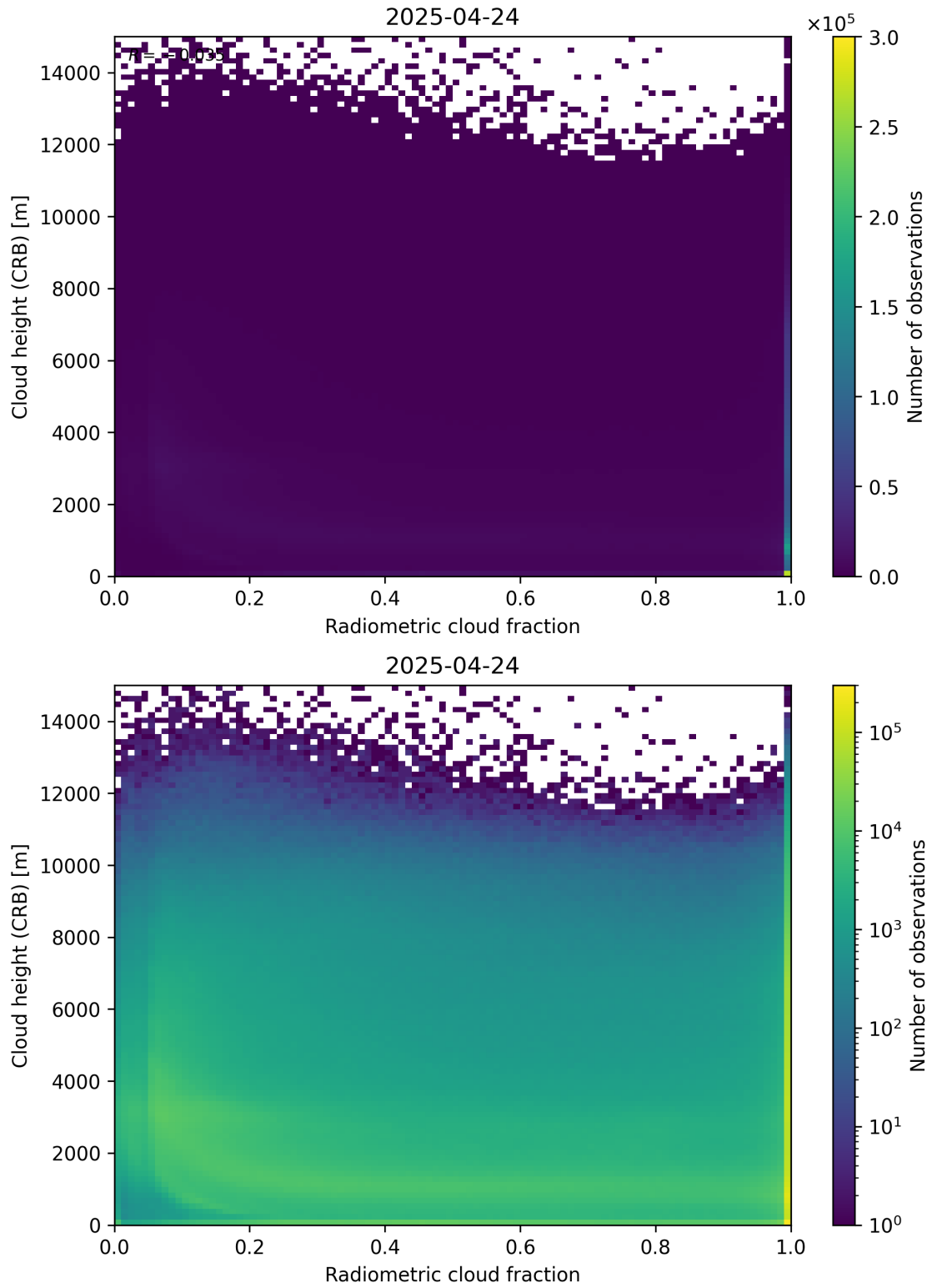
Figure 74: Scatter density plot of “Radiometric cloud fraction” against “Cloud height (CRB)” for 2025-04-24 to 2025-04-25.
