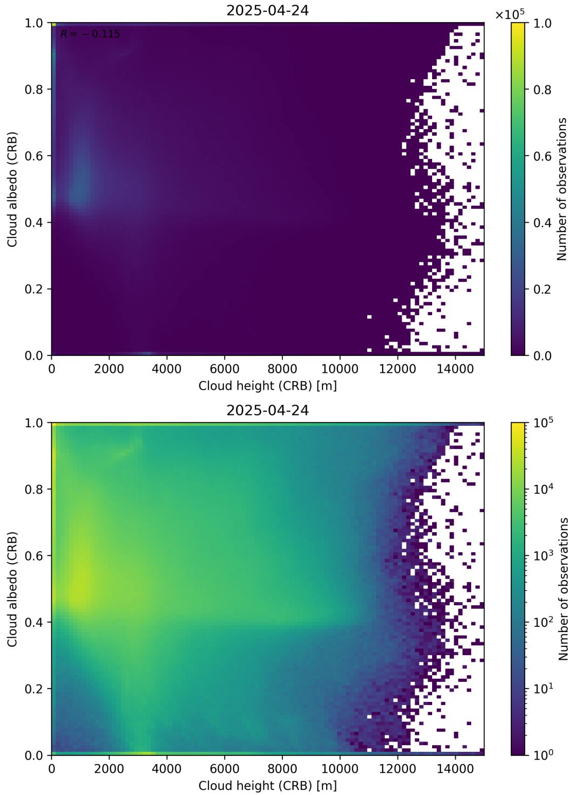
Figure 80: Scatter density plot of “Cloud height (CRB)” against “Cloud albedo (CRB)” for 2025-04-24 to 2025-04-25.
