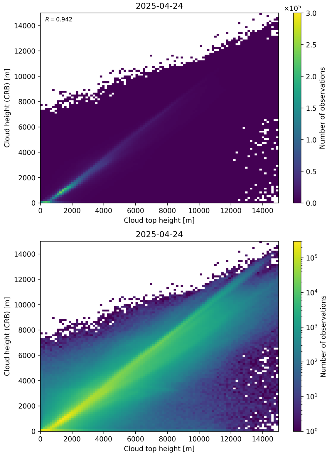
Figure 89: Scatter density plot of “Cloud top height” against “Cloud height (CRB)” for 2025-04-24 to 2025-04-25.
