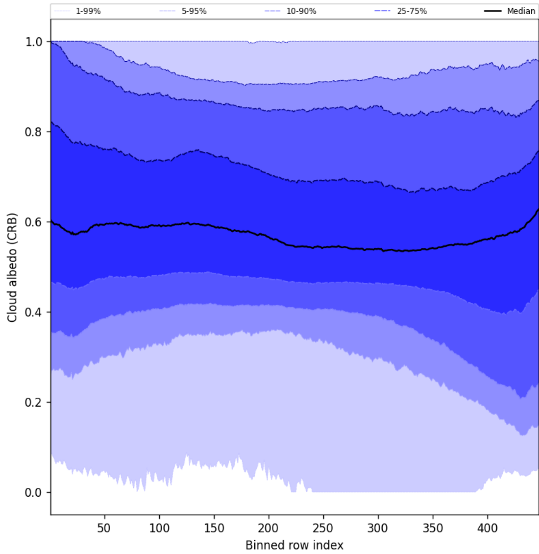
Figure 60: Along track statistics of “Cloud albedo (CRB)” for 2025-04-24 to 2025-04-25
