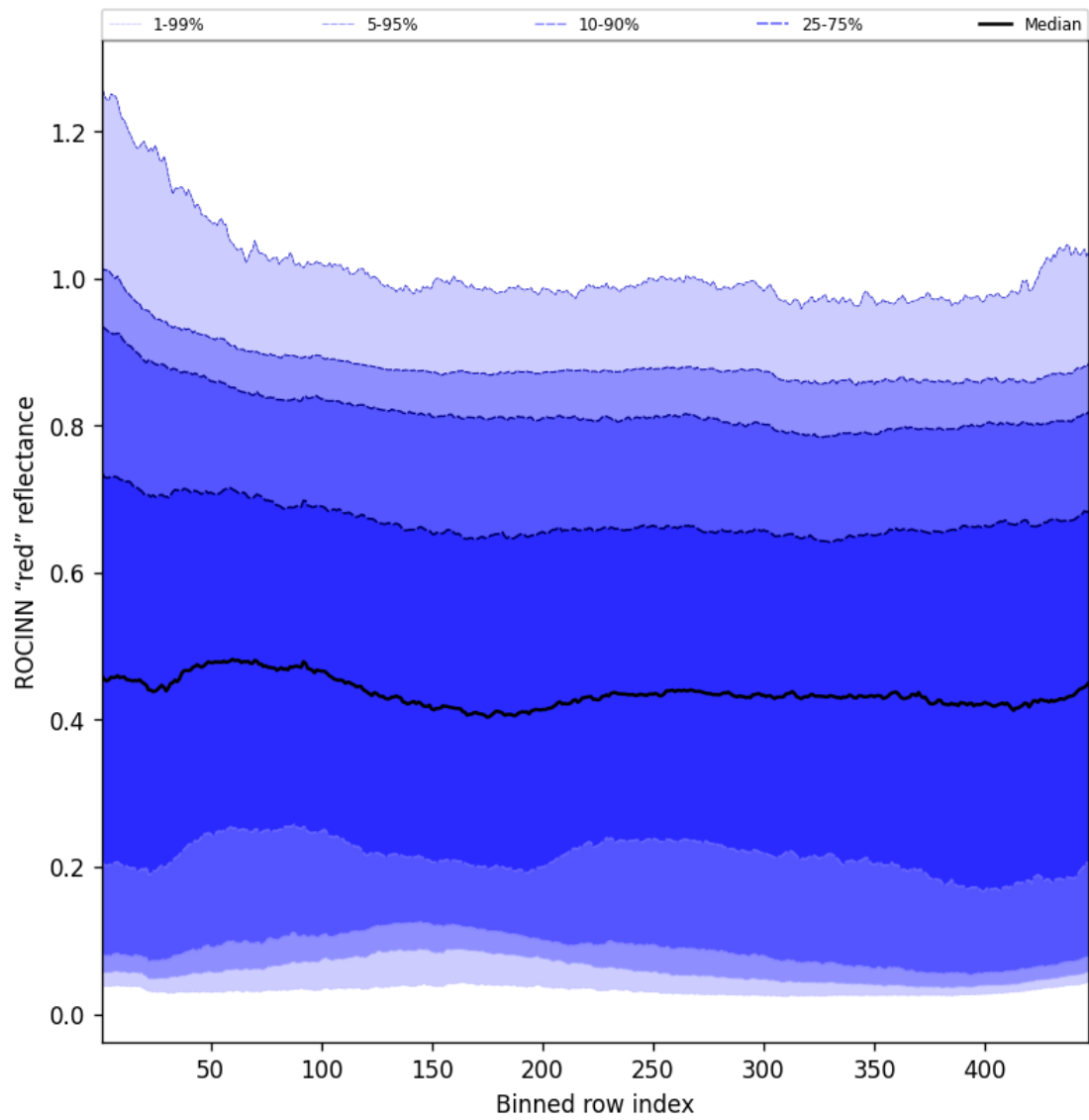
Figure 69: Along track statistics of "ROCINN "red" reflectance" for 2025-04-24 to 2025-04-25
