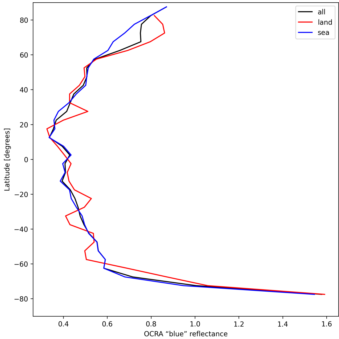
Figure 35: Zonal average of "OCRA "blue" reflectance" for 2025-04-24 to 2025-04-25.
