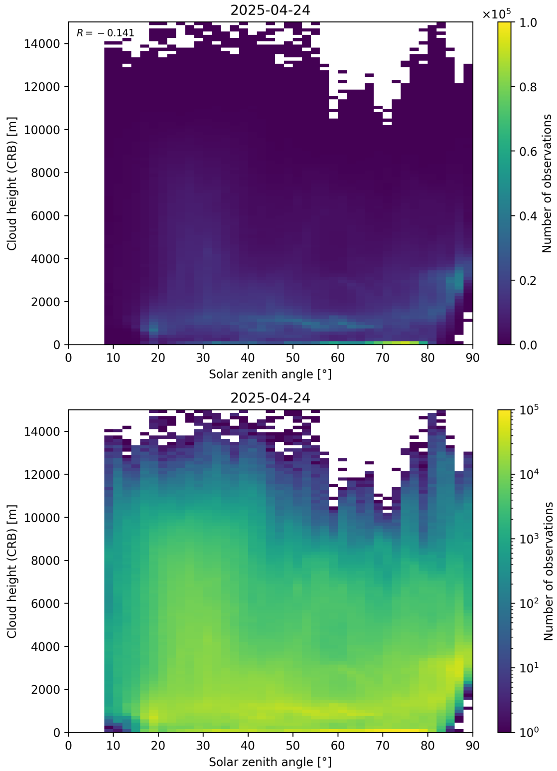
Figure 102: Scatter density plot of “Solar zenith angle” against “Cloud height (CRB)” for 2025-04-24 to 2025-04-25.
