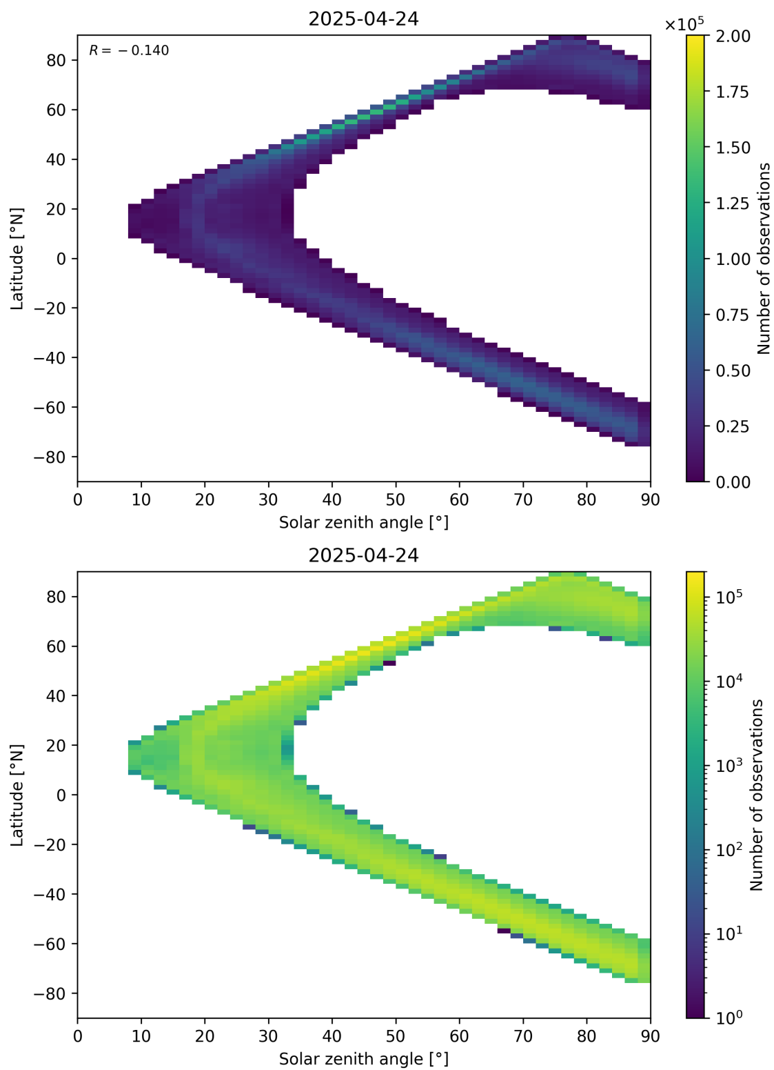
Figure 105: Scatter density plot of “Solar zenith angle” against “Latitude” for 2025-04-24 to 2025-04-25.
