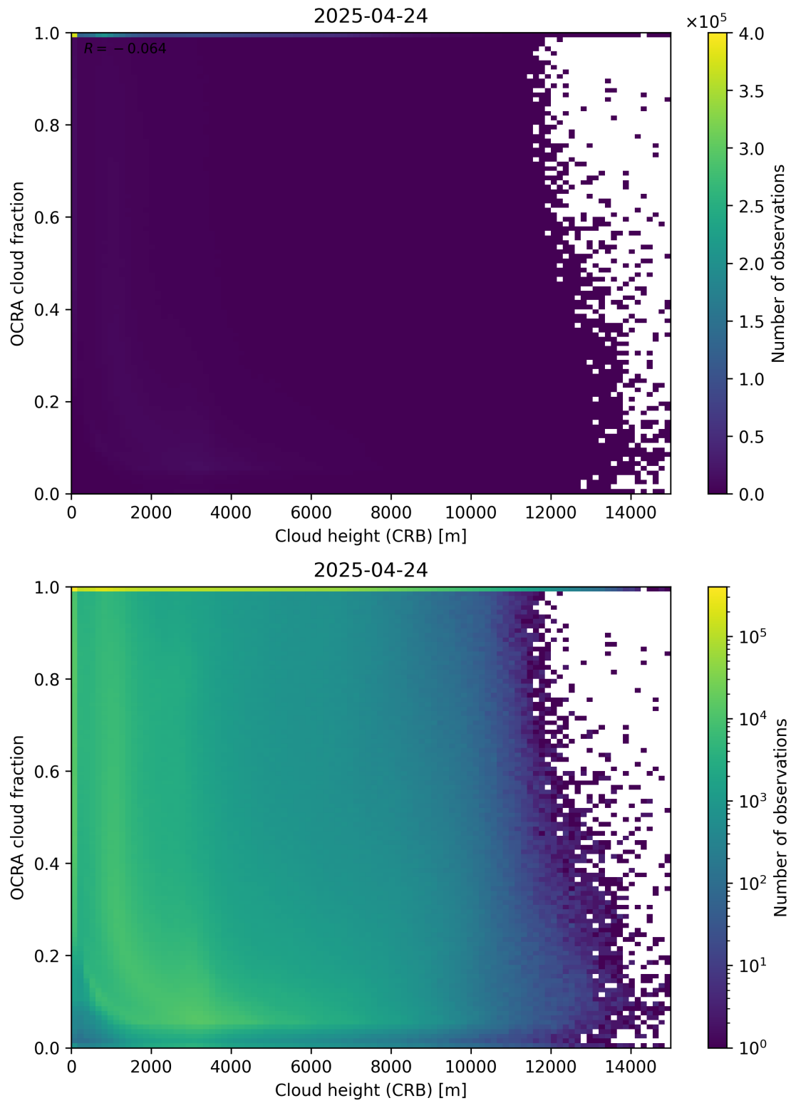
Figure 81: Scatter density plot of “Cloud height (CRB)” against “OCRA cloud fraction” for 2025-04-24 to 2025-04-25.
