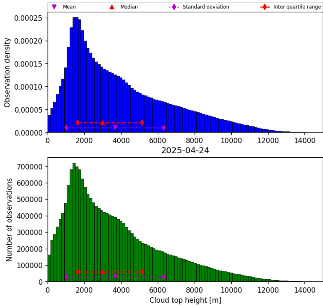
Figure 40: Histogram of “Cloud top height” for 2025-04-24 to 2025-04-25
