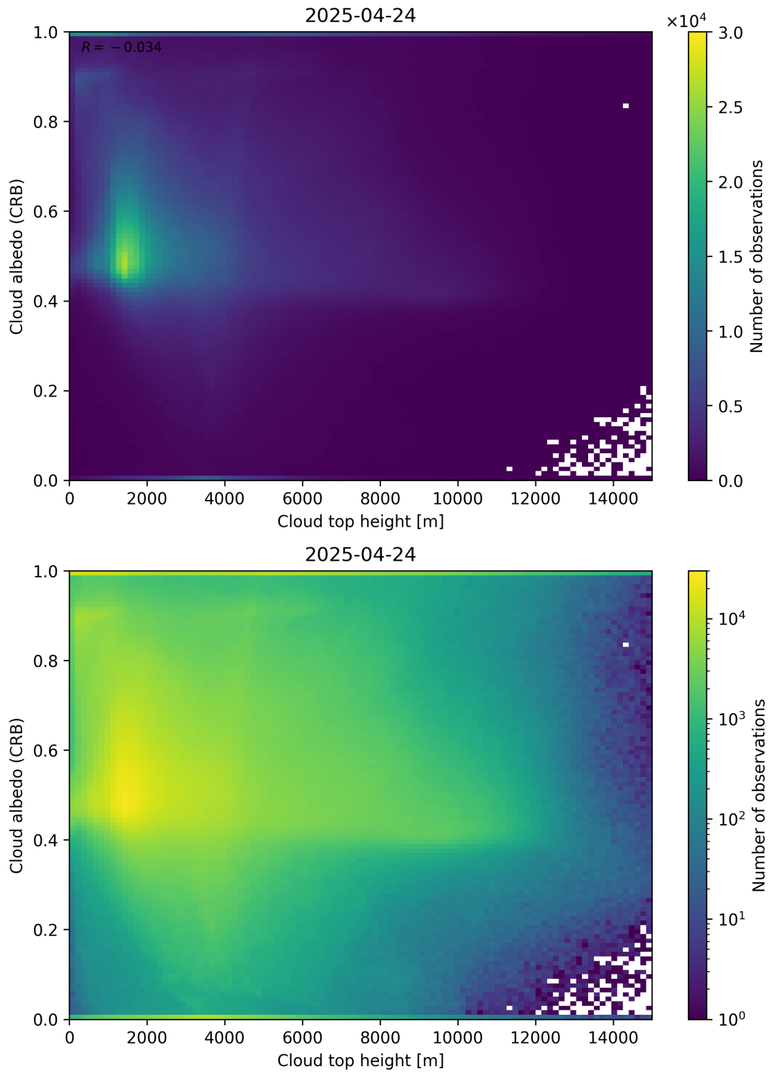
Figure 86: Scatter density plot of “Cloud top height” against “Cloud albedo (CRB)” for 2025-04-24 to 2025-04-25.
