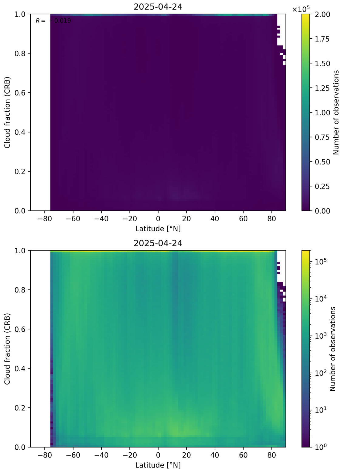
Figure 94: Scatter density plot of “Latitude” against “Cloud fraction (CRB)” for 2025-04-24 to 2025-04-25.
