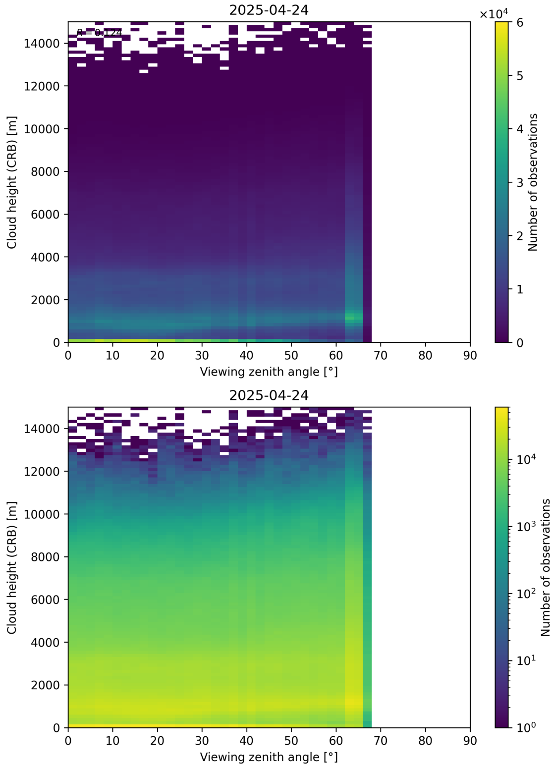
Figure 110: Scatter density plot of “Viewing zenith angle” against “Cloud height (CRB)” for 2025-04-24 to 2025-04-25.
