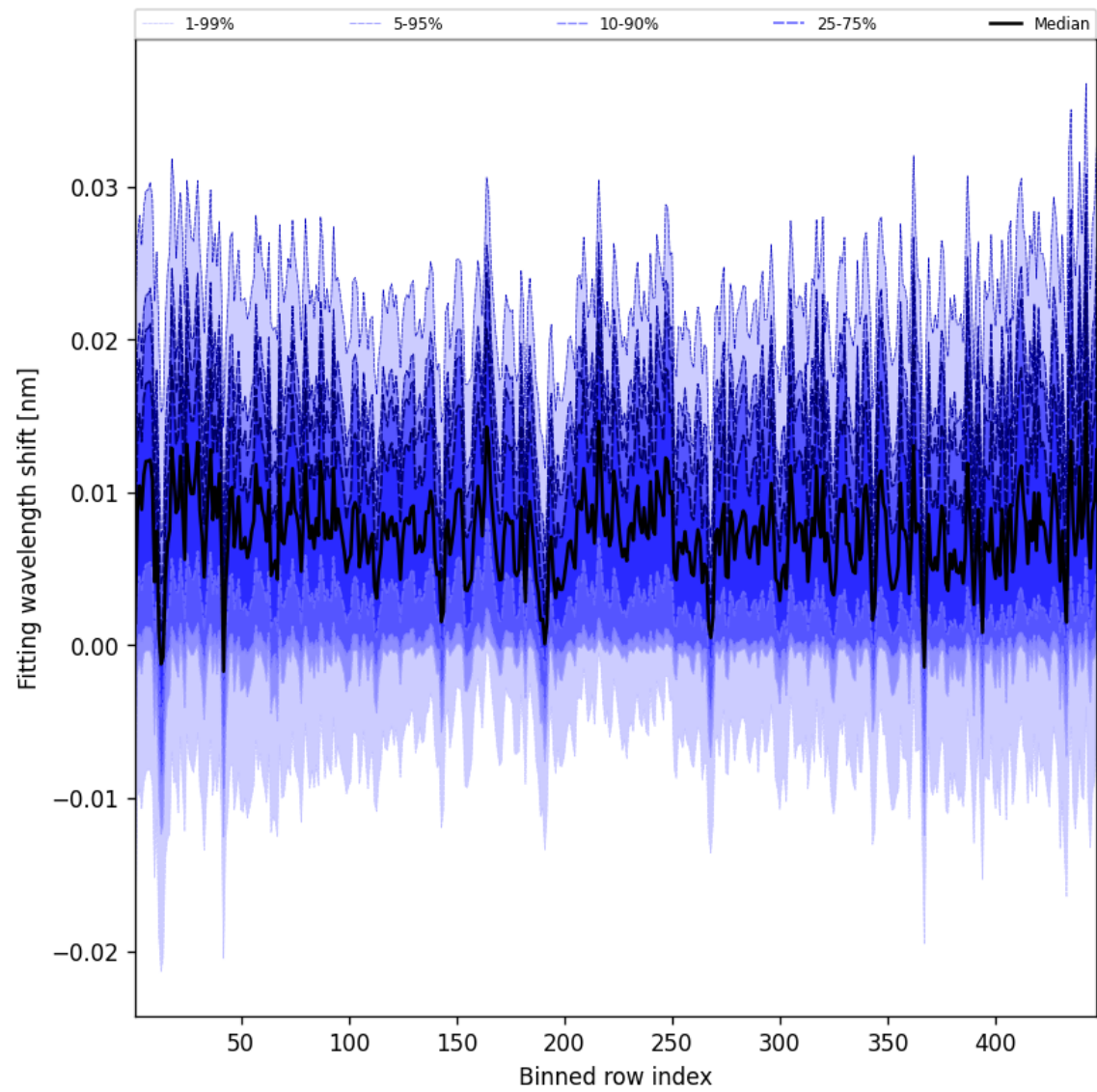
Figure 65: Along track statistics of “Fitting wavelength shift” for 2025-04-24 to 2025-04-25
