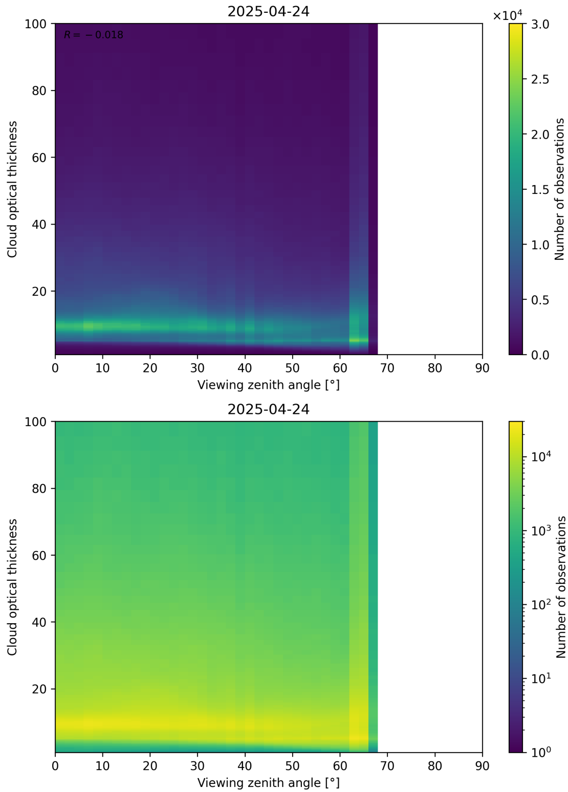
Figure 111: Scatter density plot of “Viewing zenith angle” against “Cloud optical thickness” for 2025-04-24 to 2025-04-25.
