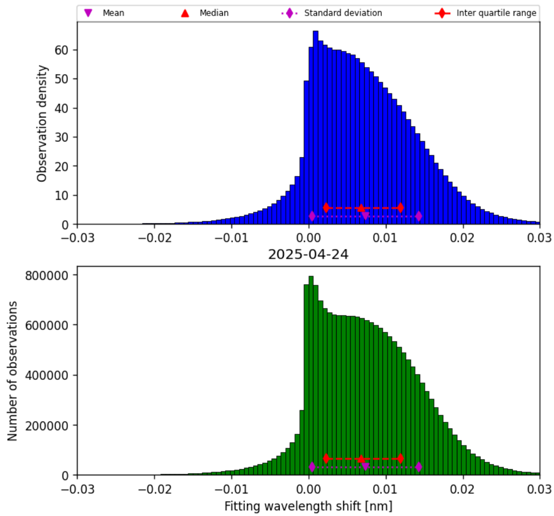
Figure 49: Histogram of “Fitting wavelength shift” for 2025-04-24 to 2025-04-25
