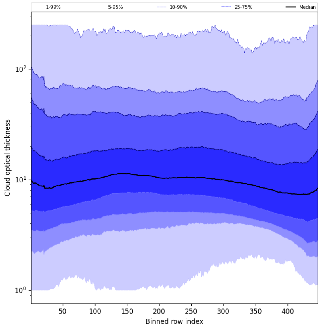
Figure 57: Along track statistics of “Cloud optical thickness” for 2025-04-24 to 2025-04-25
