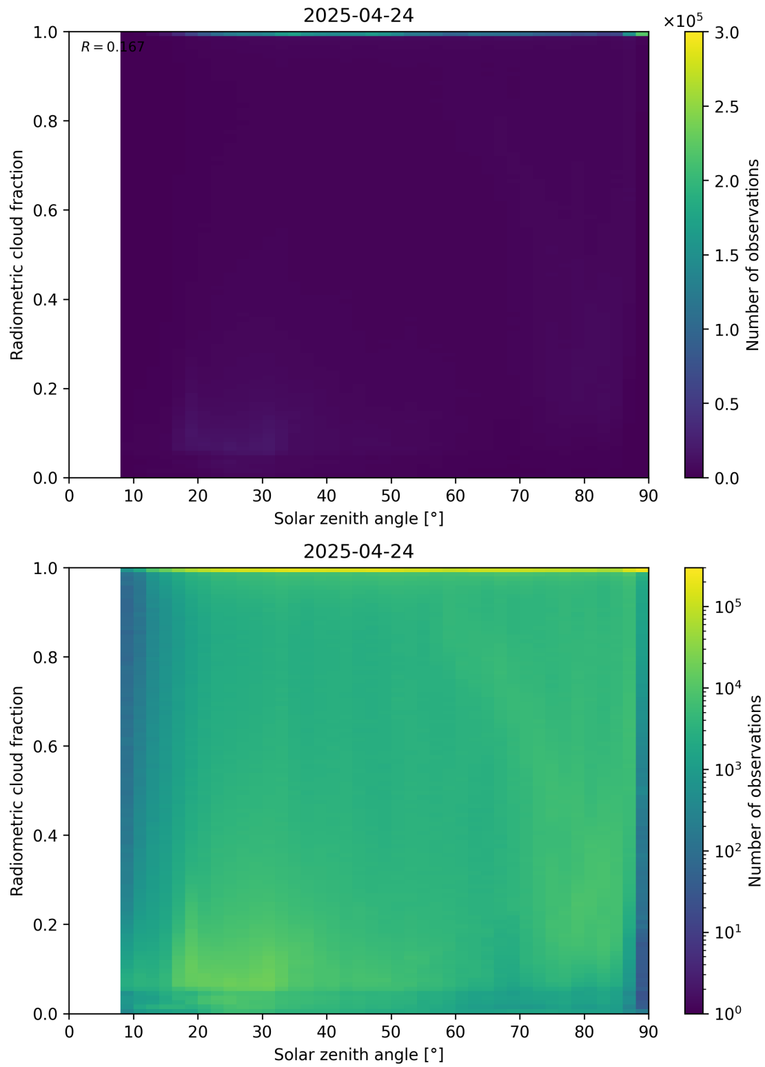
Figure 99: Scatter density plot of “Solar zenith angle” against “Radiometric cloud fraction” for 2025-04-24 to 2025-04-25.
