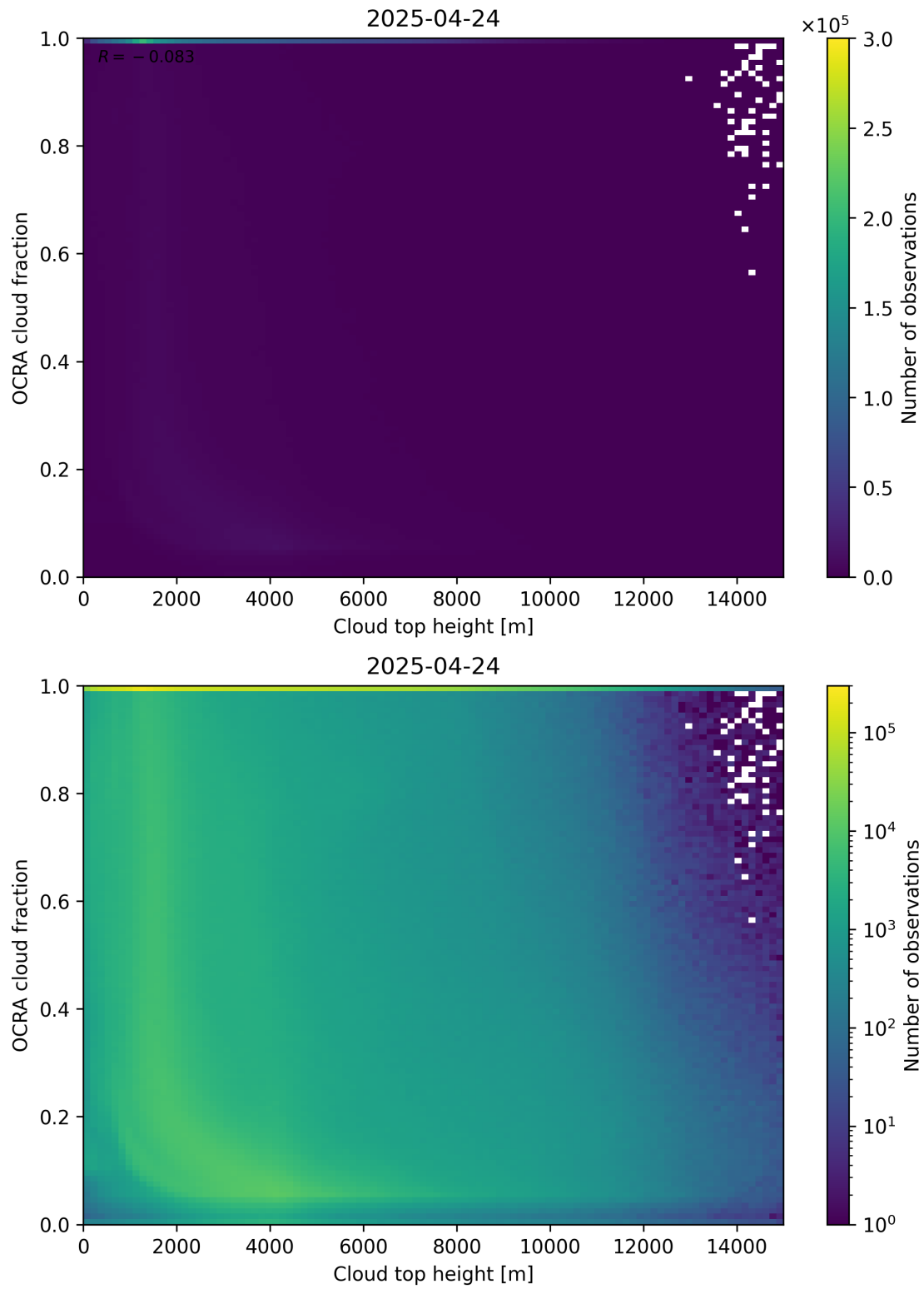
Figure 87: Scatter density plot of “Cloud top height” against “OCRA cloud fraction” for 2025-04-24 to 2025-04-25.
