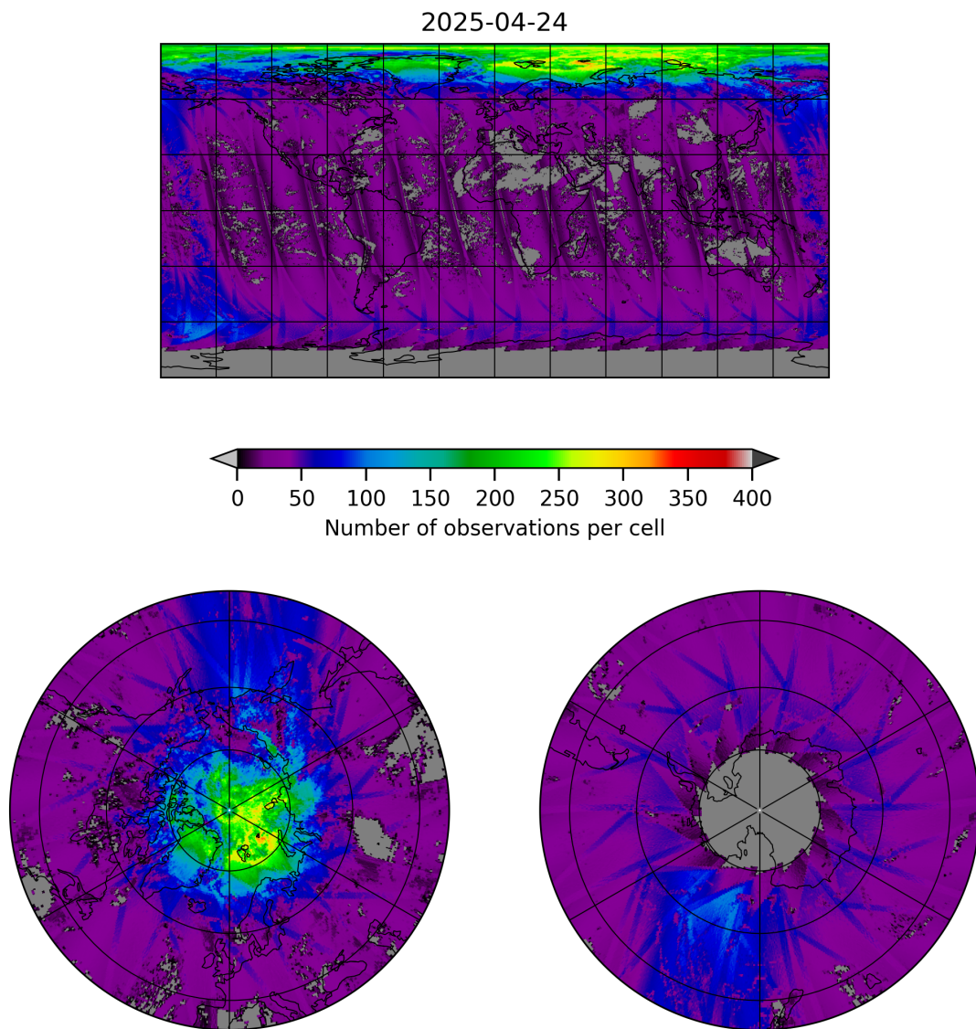
Figure 21: Map of the number of observations for 2025-04-24 to 2025-04-25
