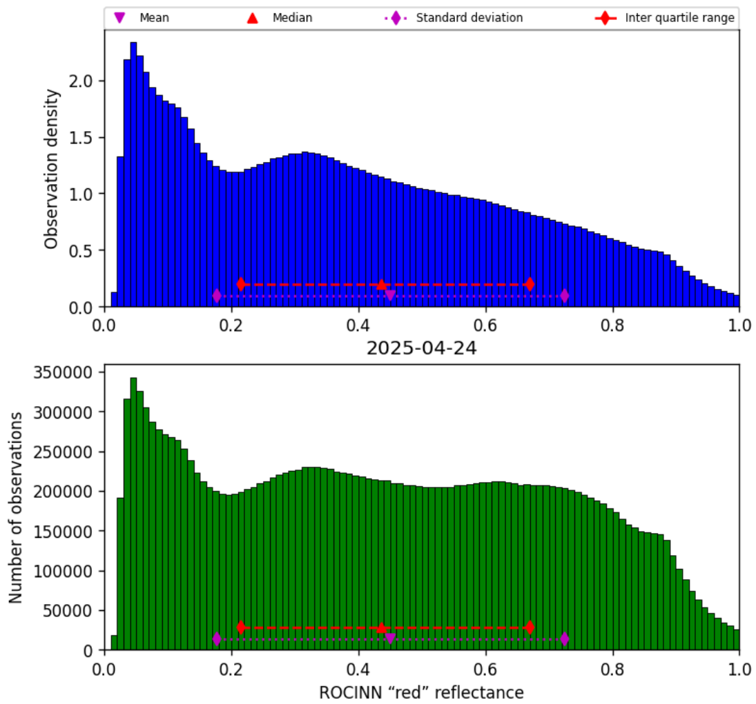
Figure 53: Histogram of “ROCINN “red” reflectance” for 2025-04-24 to 2025-04-25
