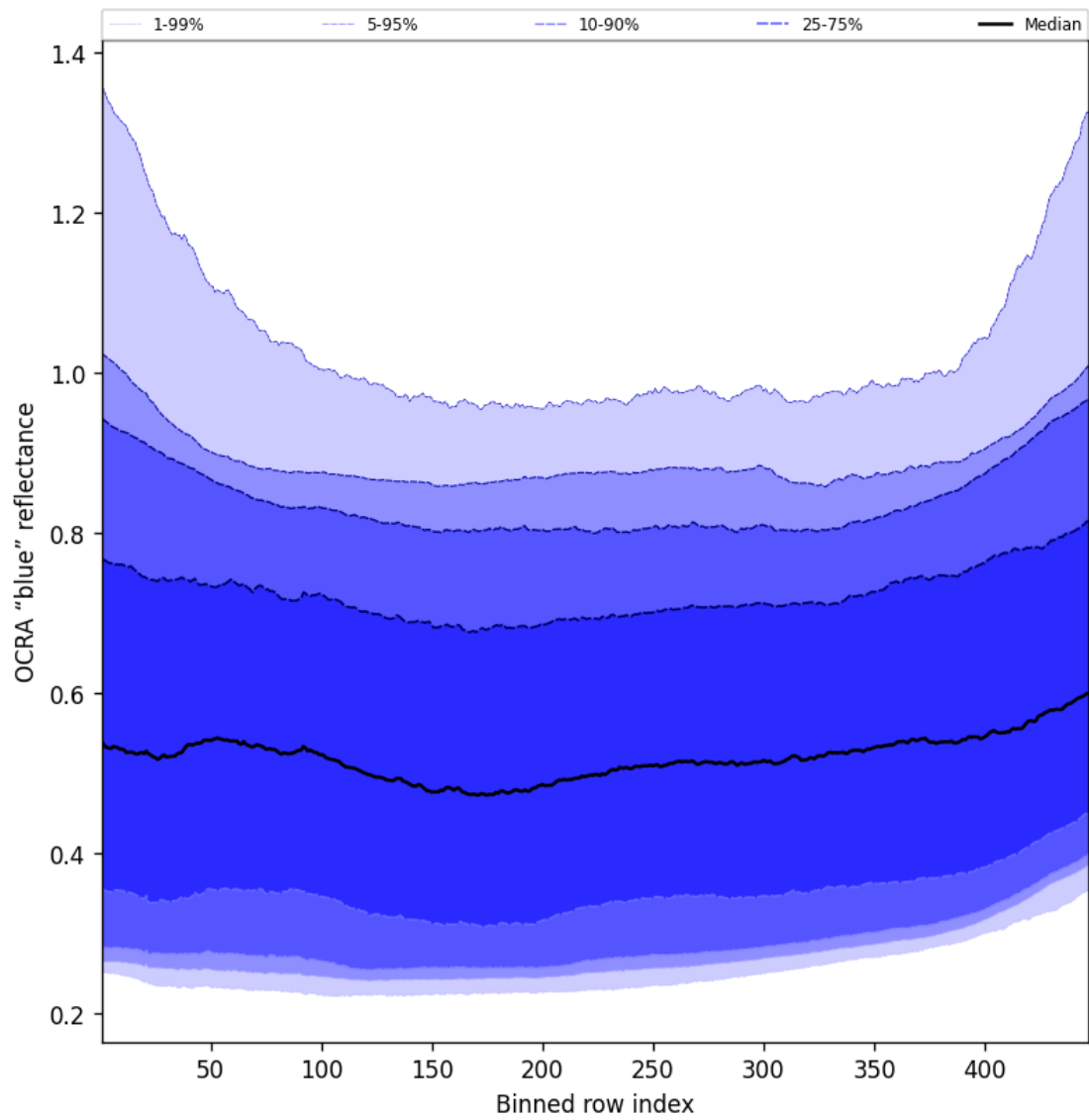
Figure 67: Along track statistics of "OCRA "blue" reflectance" for 2025-04-24 to 2025-04-25
