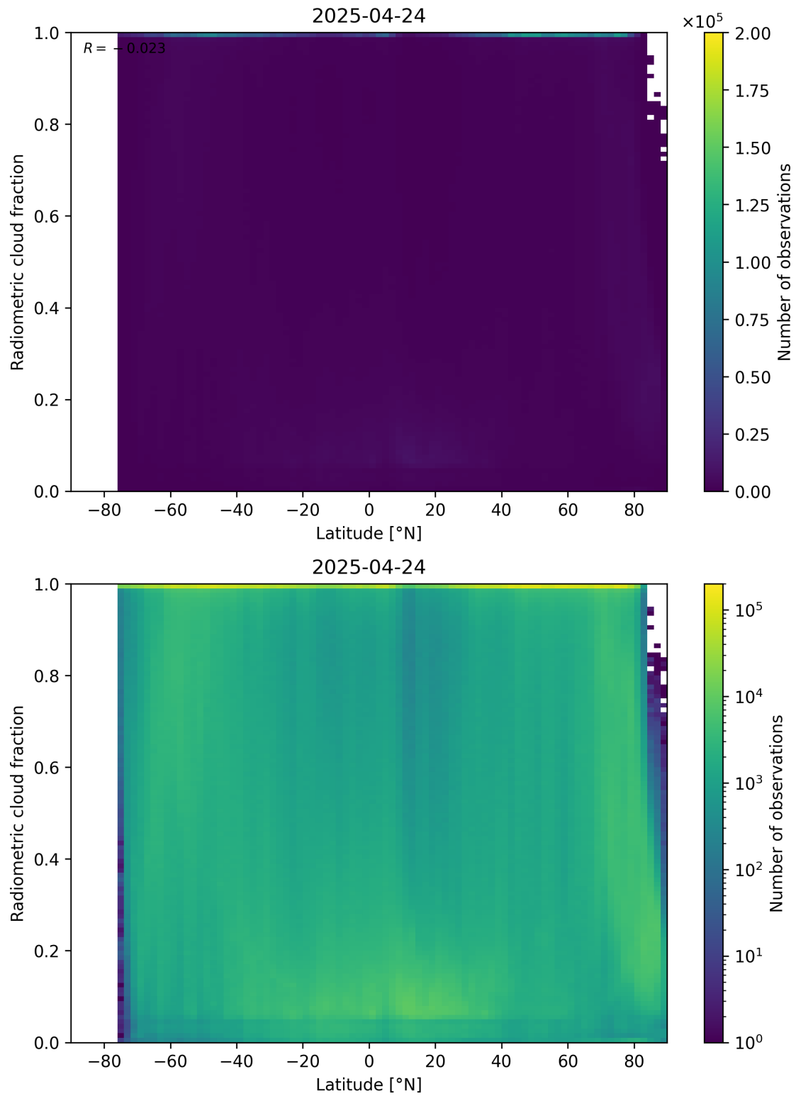
Figure 92: Scatter density plot of “Latitude” against “Radiometric cloud fraction” for 2025-04-24 to 2025-04-25.
