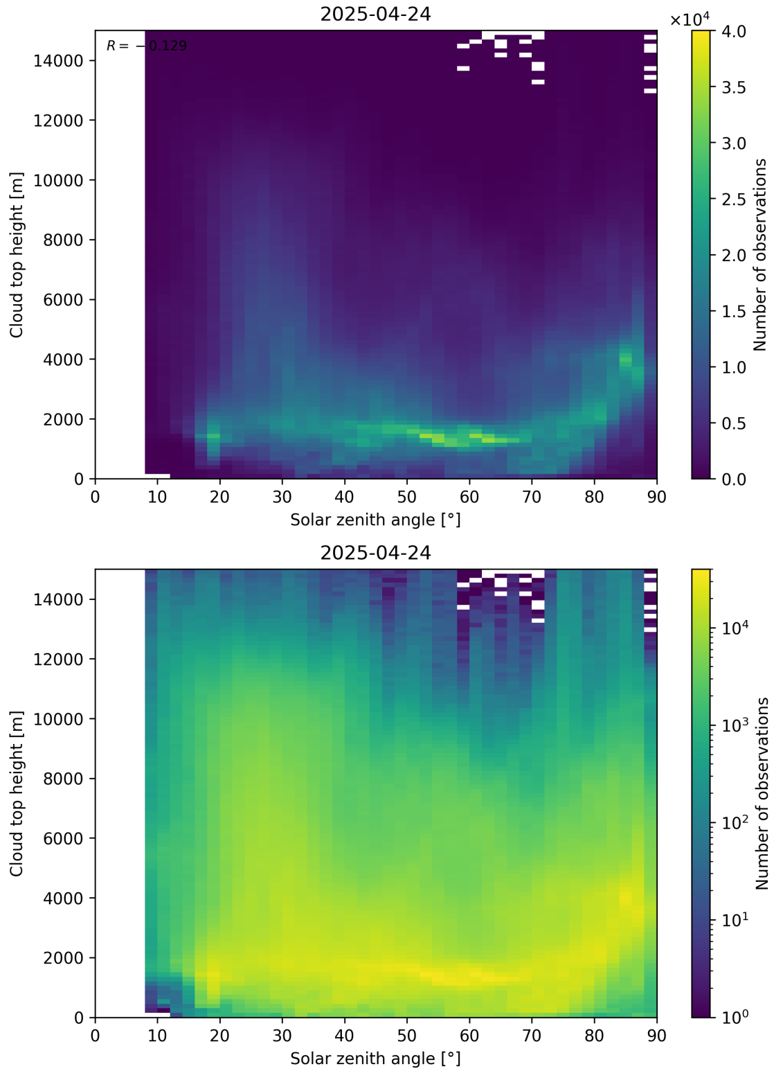
Figure 104: Scatter density plot of “Solar zenith angle” against “Cloud top height” for 2025-04-24 to 2025-04-25.
