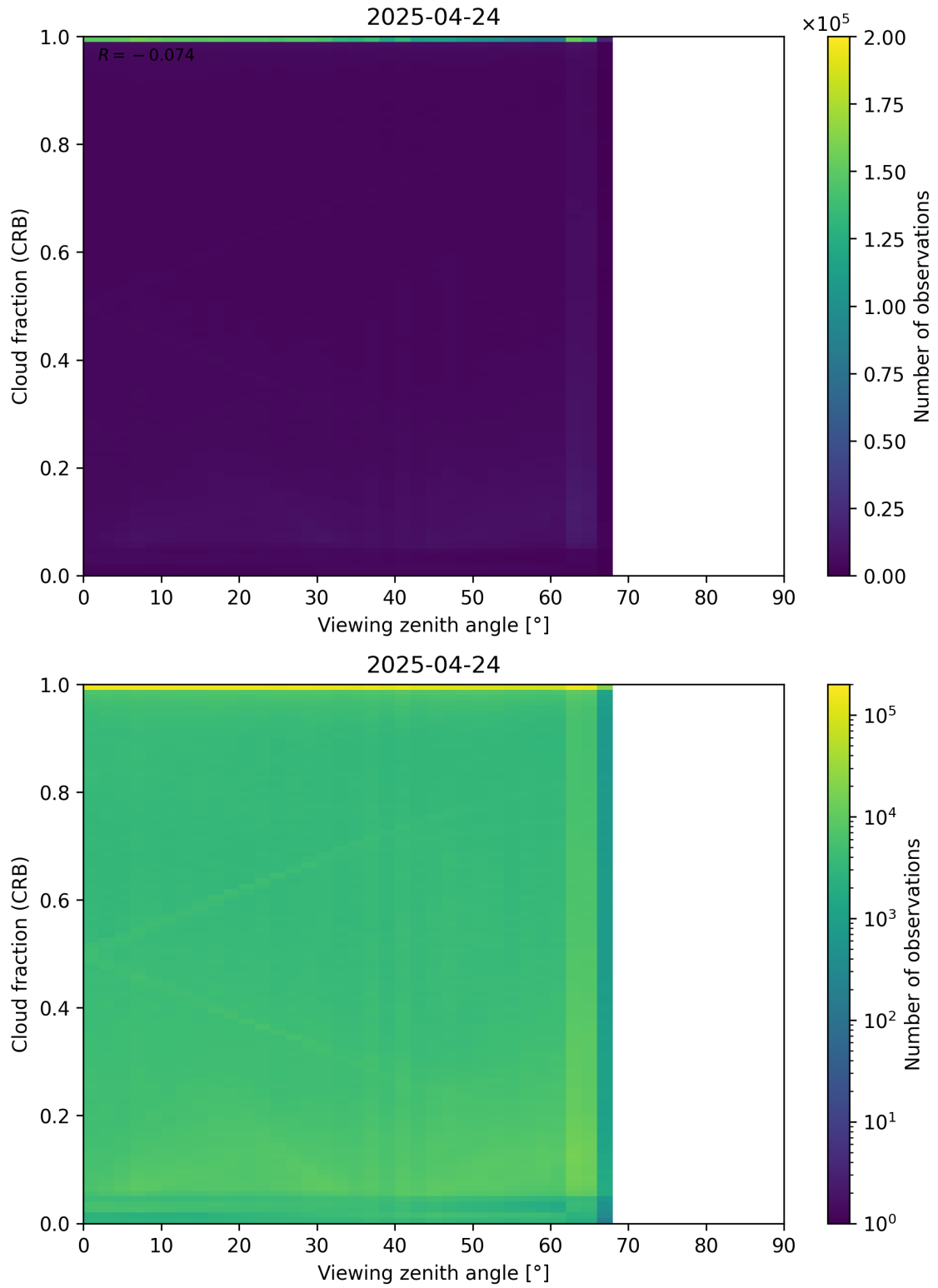
Figure 109: Scatter density plot of “Viewing zenith angle” against “Cloud fraction (CRB)” for 2025-04-24 to 2025-04-25.
