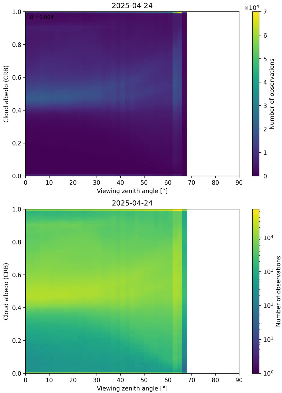
Figure 106: Scatter density plot of “Viewing zenith angle” against “Cloud albedo (CRB)” for 2025-04-24 to 2025-04-25.
