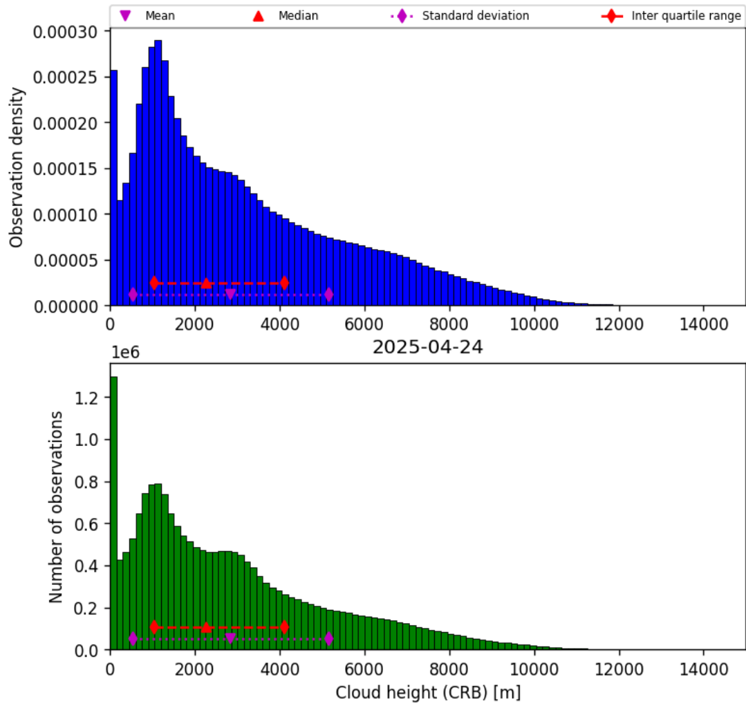
Figure 43: Histogram of “Cloud height (CRB)” for 2025-04-24 to 2025-04-25
