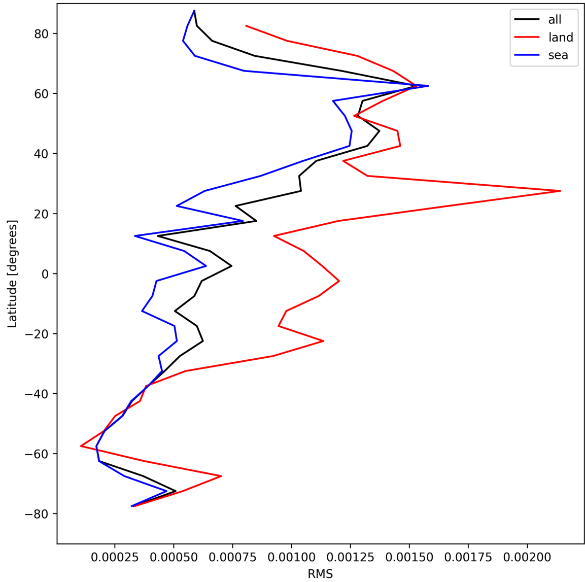
Figure 31: Zonal average of “RMS” for 2025-04-24 to 2025-04-25.
