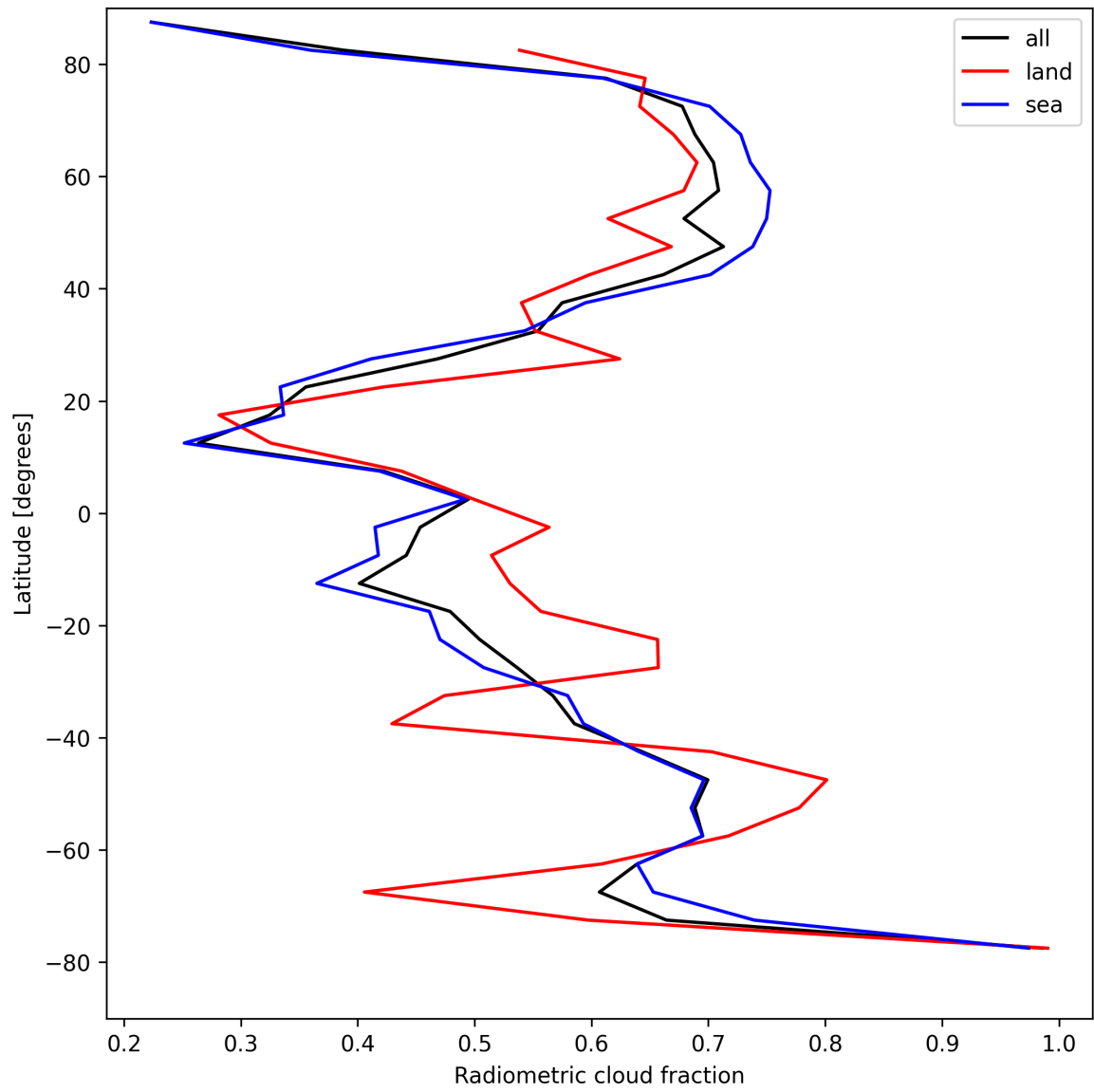
Figure 23: Zonal average of “Radiometric cloud fraction” for 2025-04-24 to 2025-04-25.
