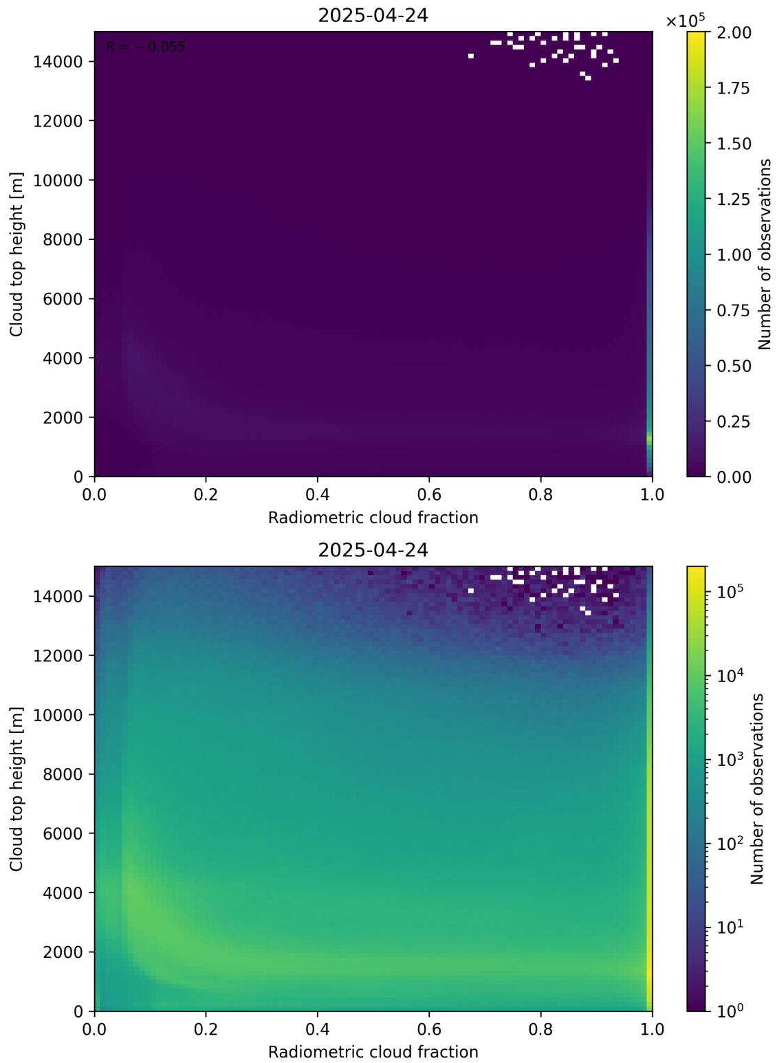
Figure 76: Scatter density plot of “Radiometric cloud fraction” against “Cloud top height” for 2025-04-24 to 2025-04-25.
