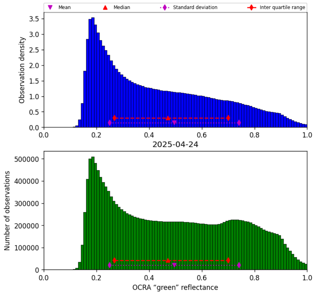
Figure 52: Histogram of “OCRA “green” reflectance” for 2025-04-24 to 2025-04-25
