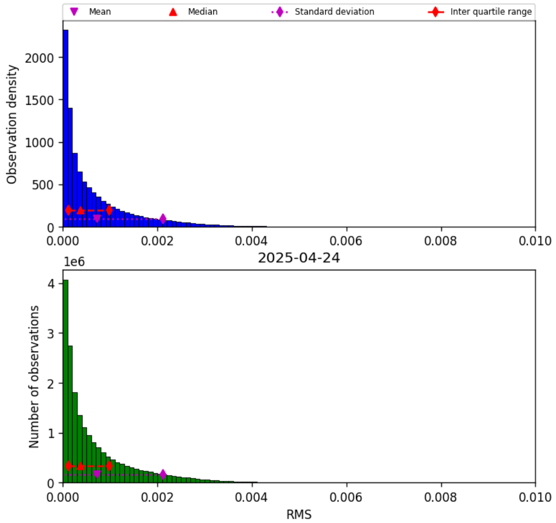
Figure 47: Histogram of “RMS” for 2025-04-24 to 2025-04-25
