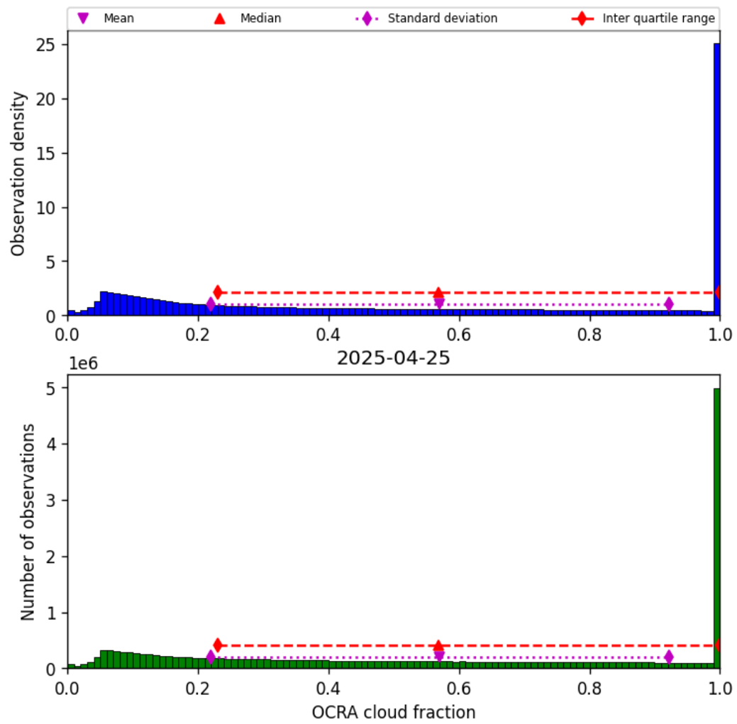
Figure 50: Histogram of “OCRA cloud fraction” for 2025-04-24 to 2025-04-26
