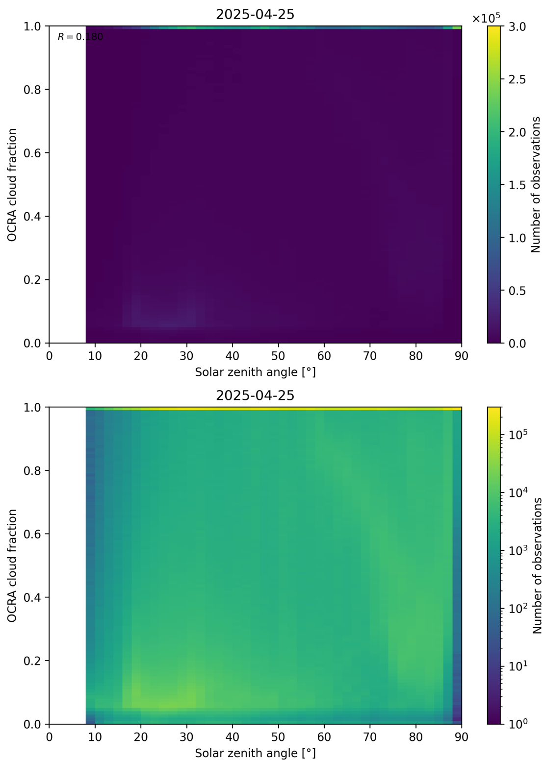
Figure 100: Scatter density plot of “Solar zenith angle” against “OCRA cloud fraction” for 2025-04-24 to 2025-04-26.
