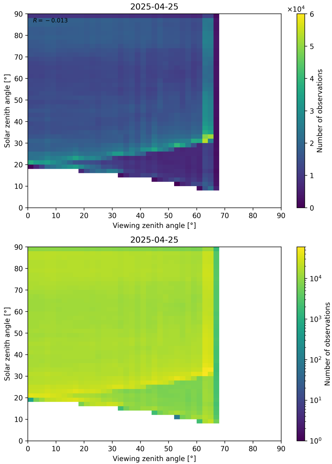
Figure 114: Scatter density plot of “Viewing zenith angle” against “Solar zenith angle” for 2025-04-24 to 2025-04-26.
