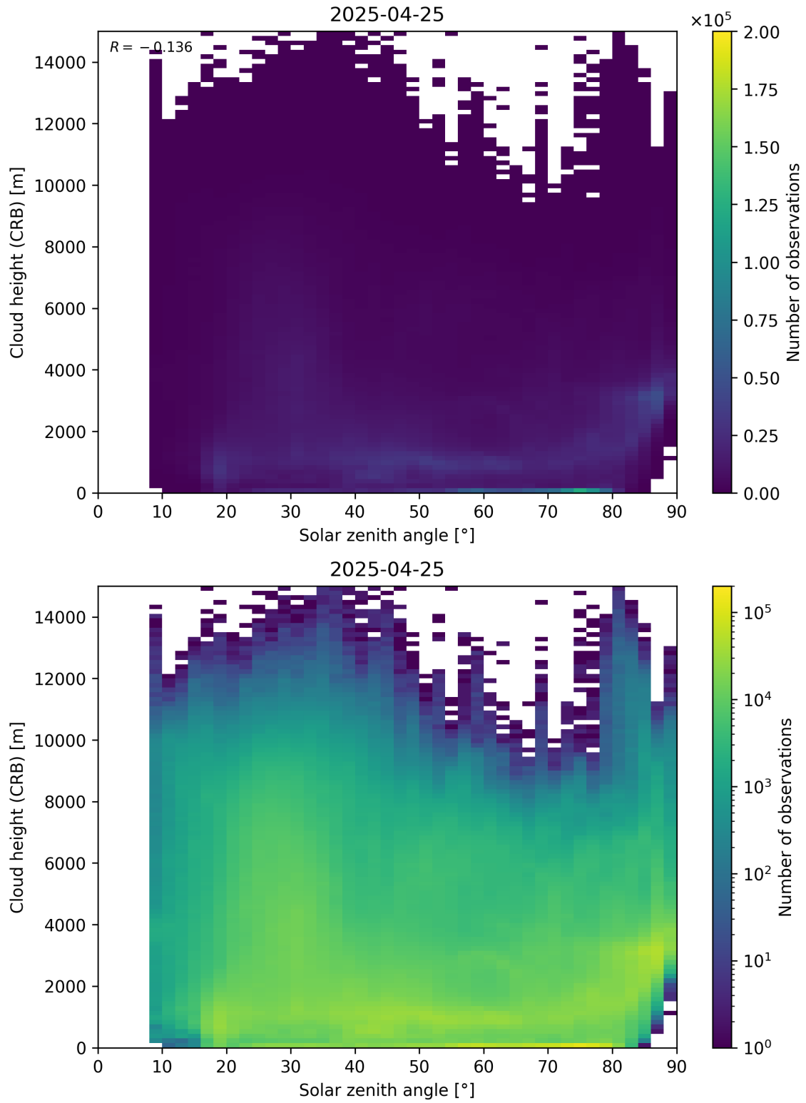
Figure 102: Scatter density plot of “Solar zenith angle” against “Cloud height (CRB)” for 2025-04-24 to 2025-04-26.
