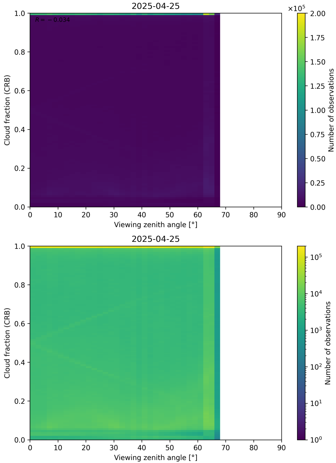
Figure 109: Scatter density plot of “Viewing zenith angle” against “Cloud fraction (CRB)” for 2025-04-24 to 2025-04-26.
