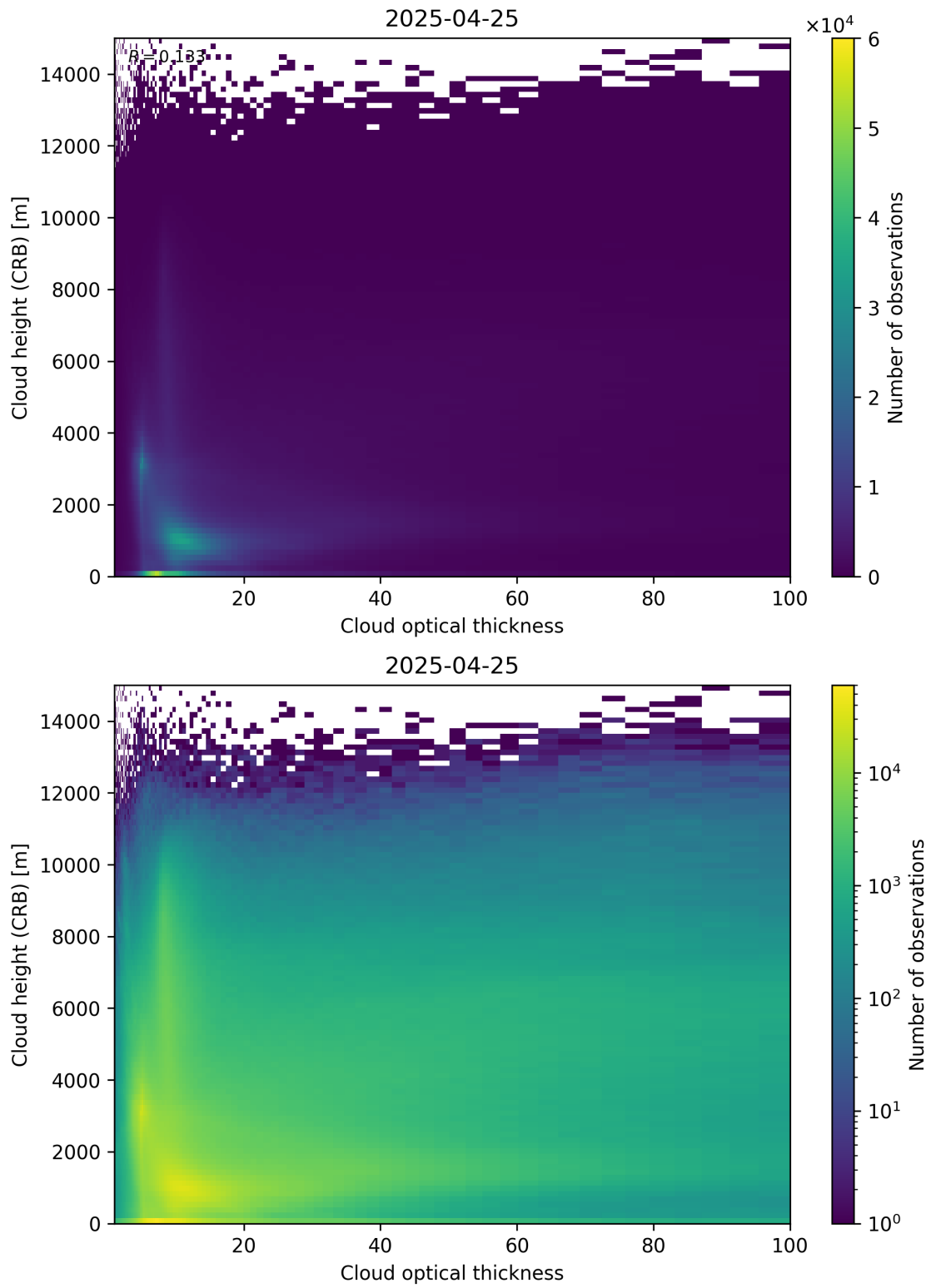
Figure 85: Scatter density plot of “Cloud optical thickness” against “Cloud height (CRB)” for 2025-04-24 to 2025-04-26.
