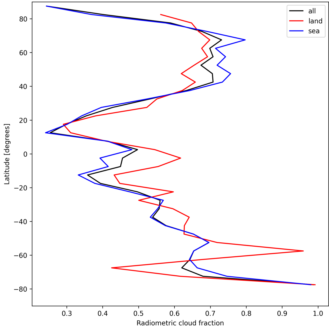
Figure 23: Zonal average of “Radiometric cloud fraction” for 2025-04-24 to 2025-04-26.
