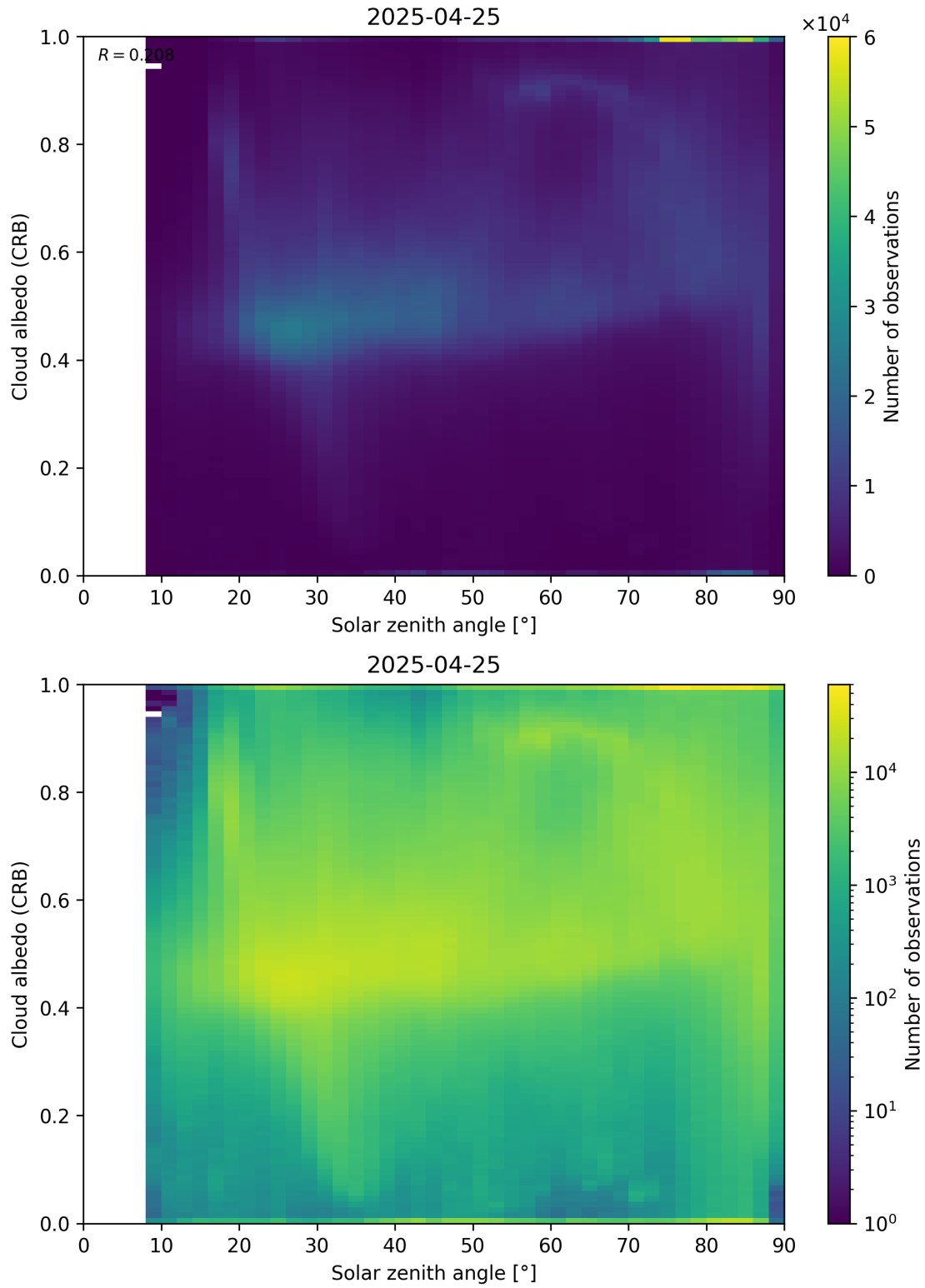
Figure 98: Scatter density plot of “Solar zenith angle” against “Cloud albedo (CRB)” for 2025-04-24 to 2025-04-26.
