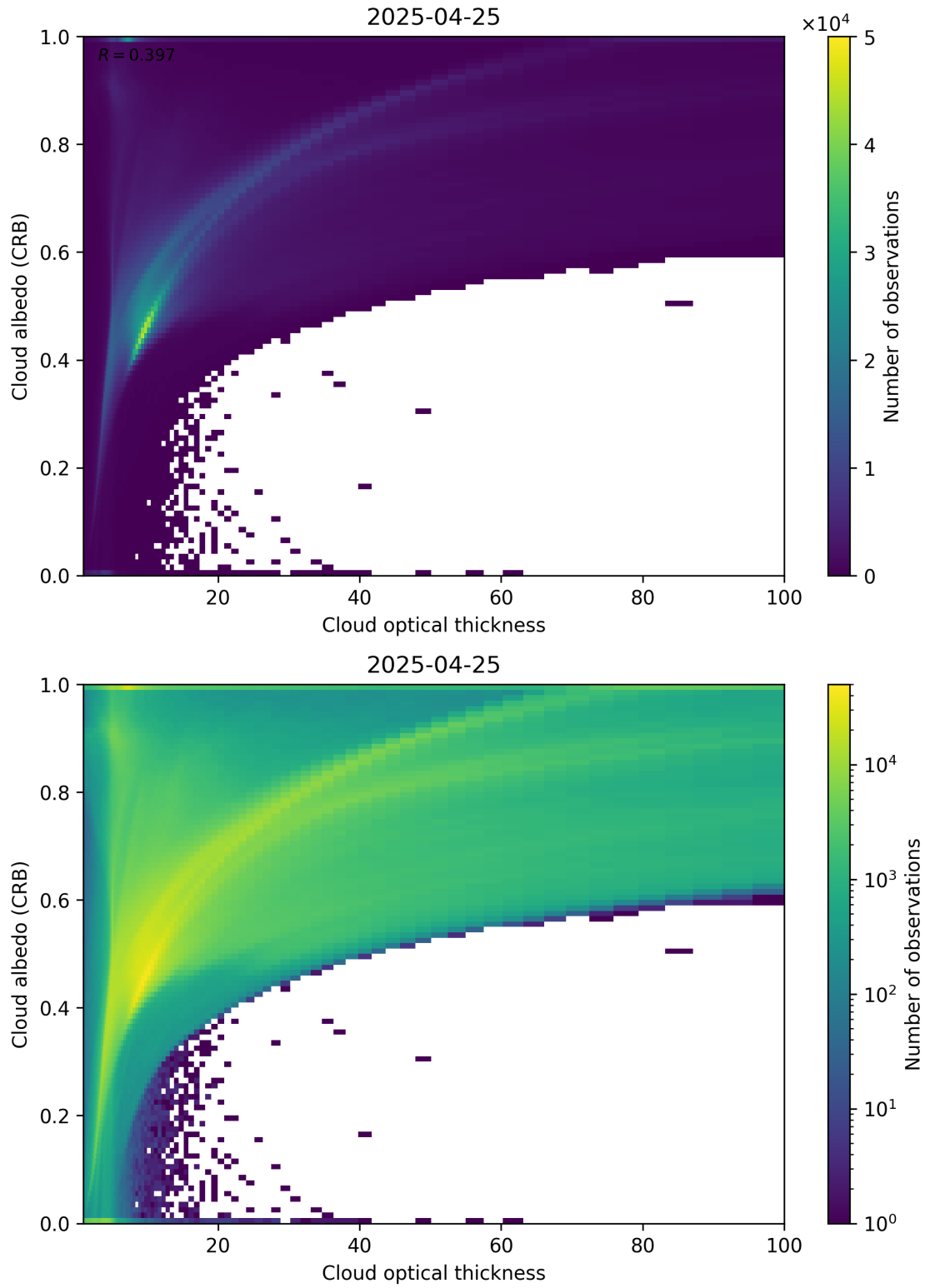
Figure 82: Scatter density plot of “Cloud optical thickness” against “Cloud albedo (CRB)” for 2025-04-24 to 2025-04-26.
