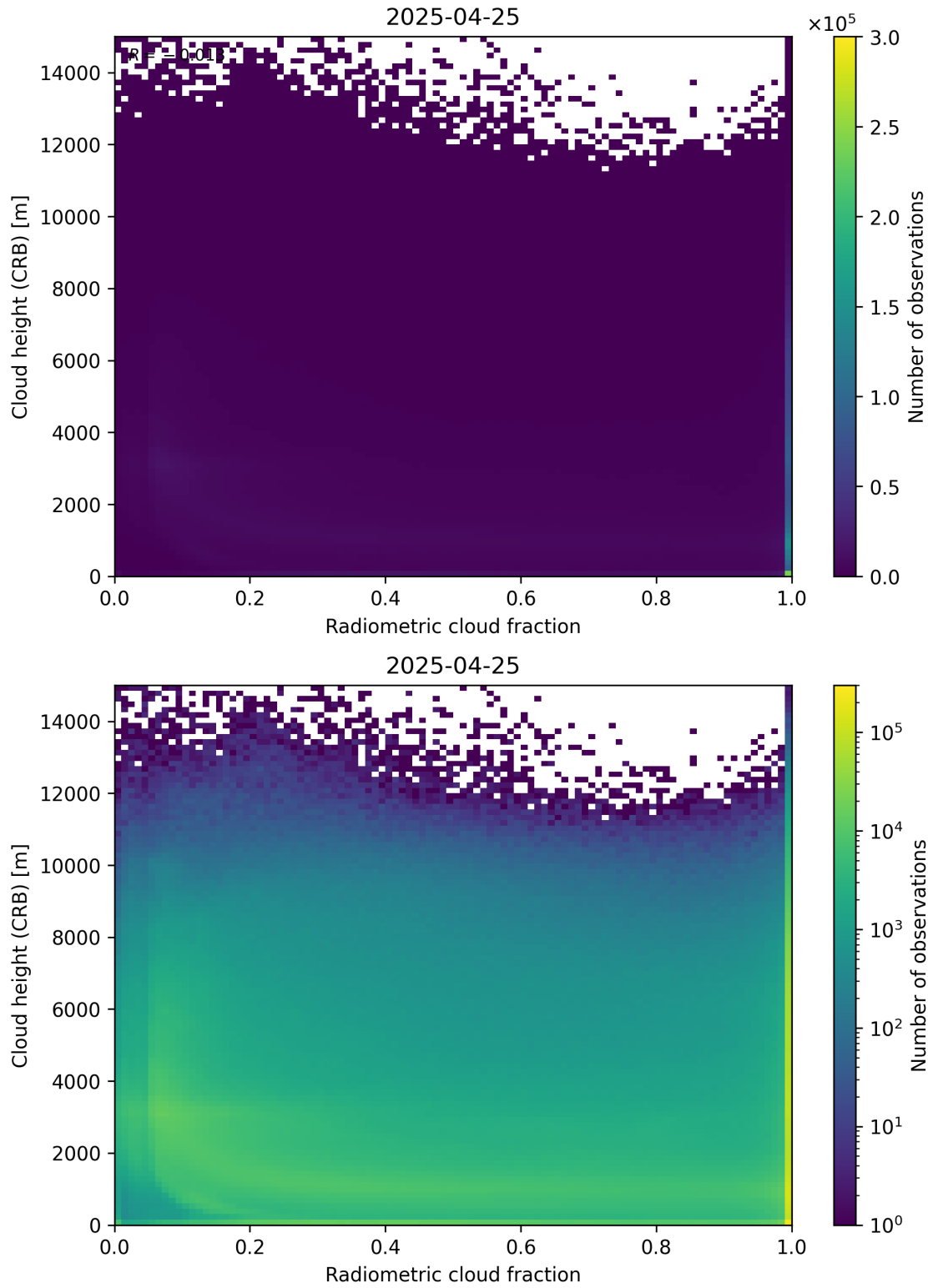
Figure 74: Scatter density plot of “Radiometric cloud fraction” against “Cloud height (CRB)” for 2025-04-24 to 2025-04-26.
