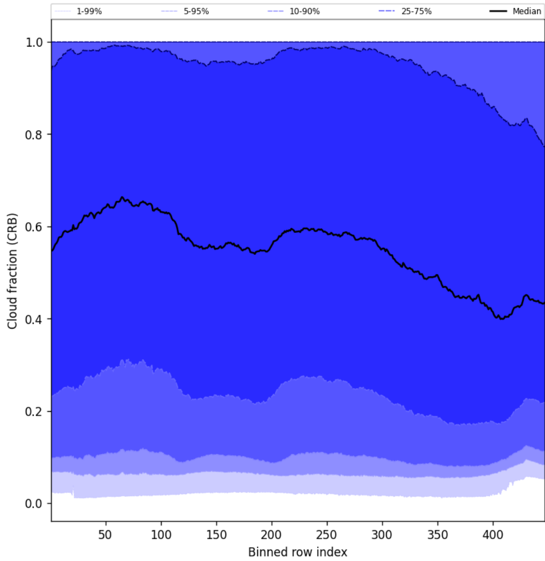
Figure 58: Along track statistics of “Cloud fraction (CRB)” for 2025-04-24 to 2025-04-26
