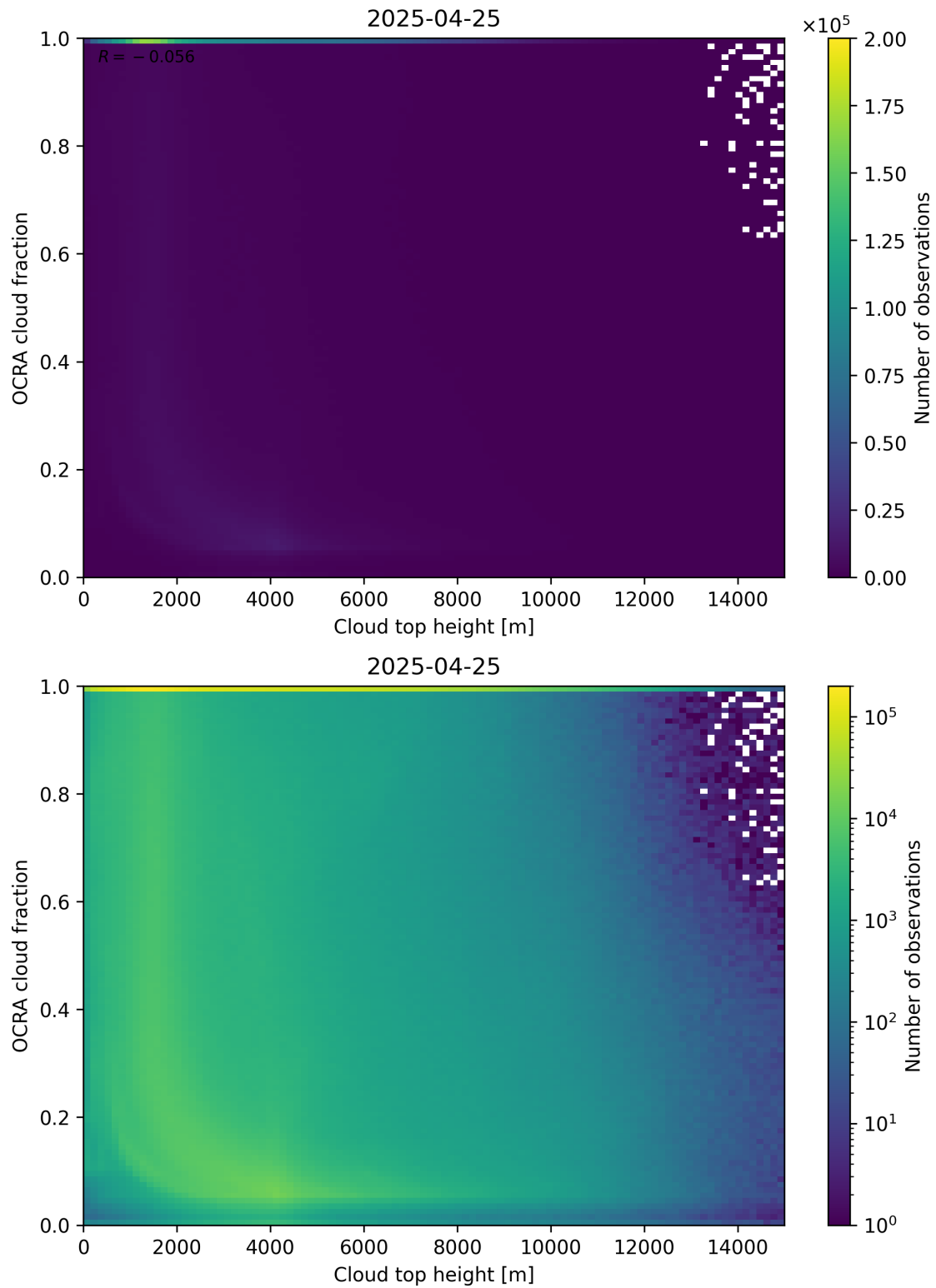
Figure 87: Scatter density plot of “Cloud top height” against “OCRA cloud fraction” for 2025-04-24 to 2025-04-26.
