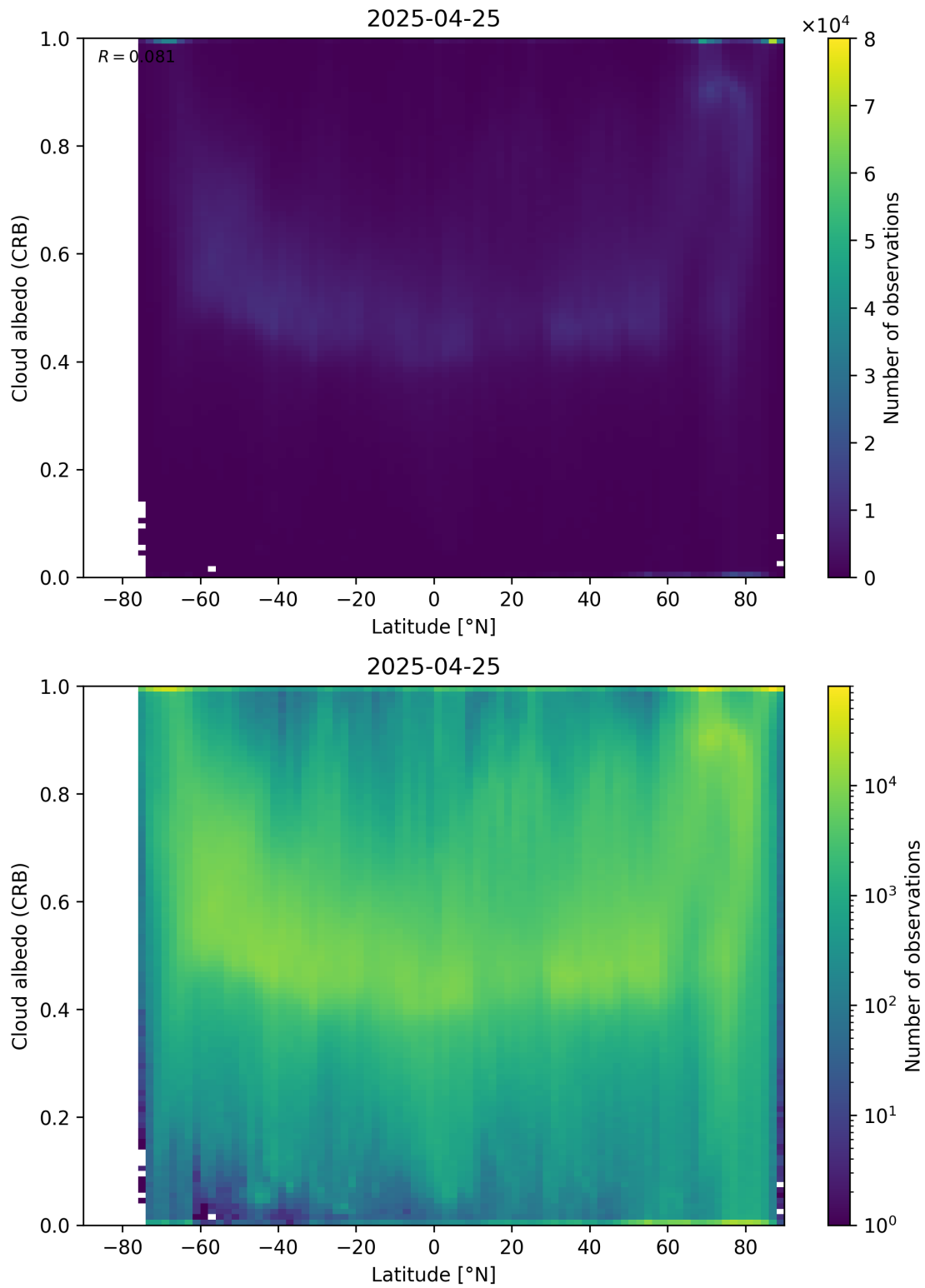
Figure 91: Scatter density plot of “Latitude” against “Cloud albedo (CRB)” for 2025-04-24 to 2025-04-26.
