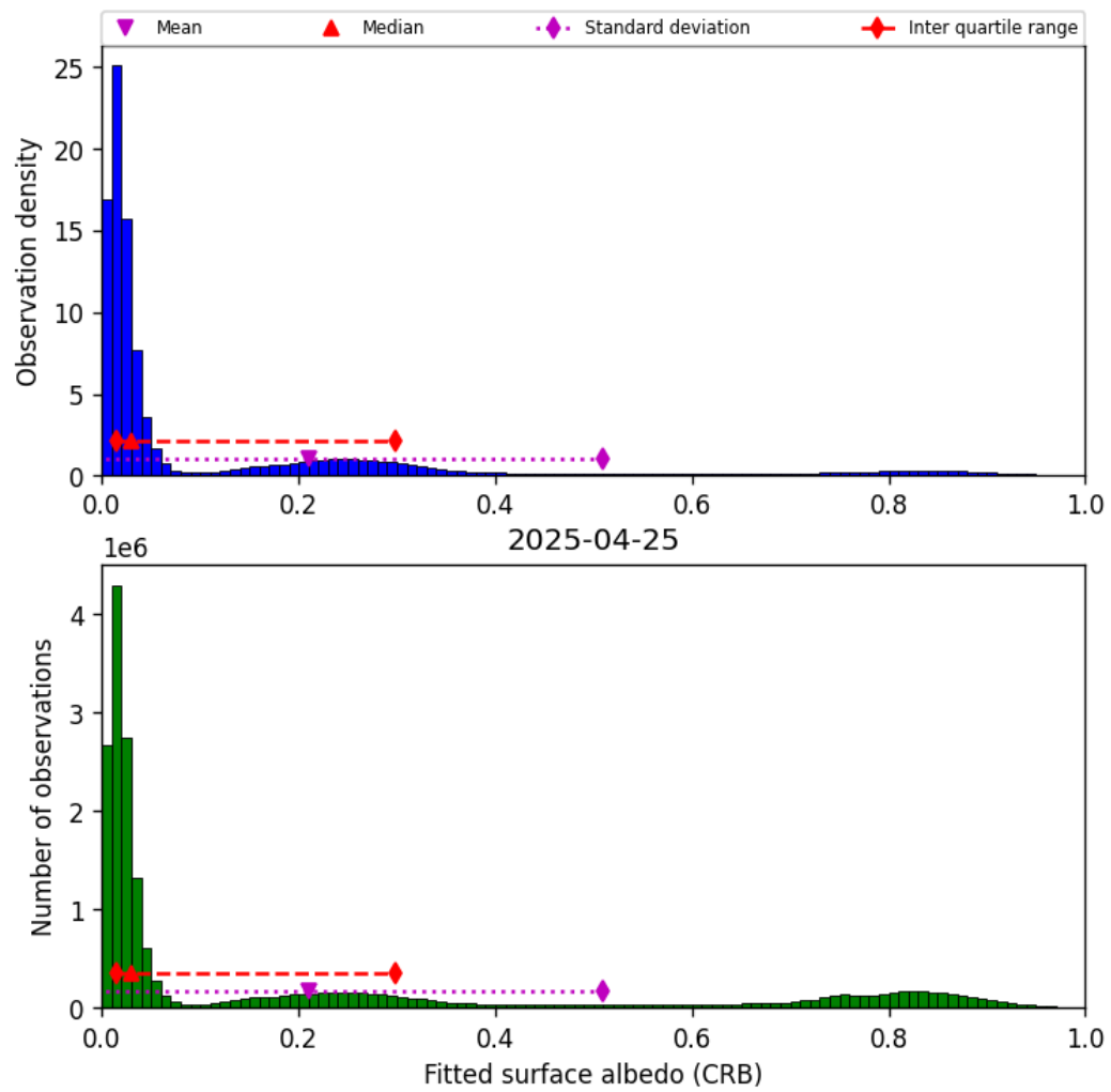
Figure 46: Histogram of “Fitted surface albedo (CRB)” for 2025-04-24 to 2025-04-26
