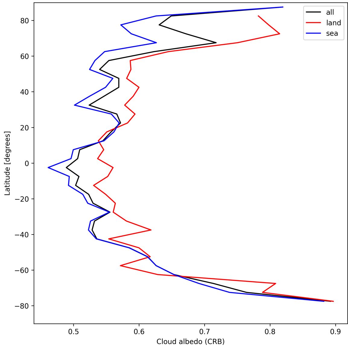
Figure 28: Zonal average of “Cloud albedo (CRB)” for 2025-04-24 to 2025-04-26.
