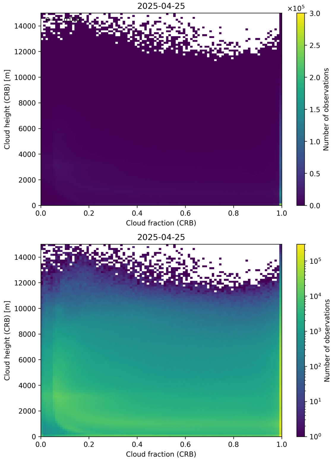
Figure 79: Scatter density plot of “Cloud fraction (CRB)” against “Cloud height (CRB)” for 2025-04-24 to 2025-04-26.
