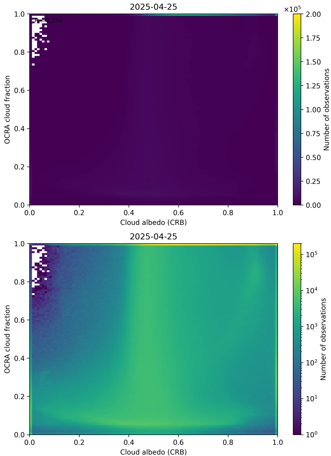
Figure 70: Scatter density plot of “Cloud albedo (CRB)” against “OCRA cloud fraction” for 2025-04-24 to 2025-04-26.
