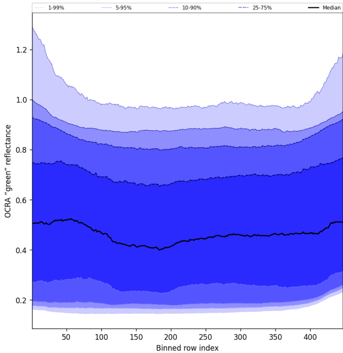
Figure 68: Along track statistics of "OCRA "green" reflectance" for 2025-04-24 to 2025-04-26
