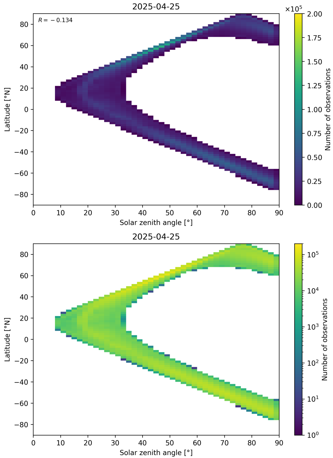
Figure 105: Scatter density plot of “Solar zenith angle” against “Latitude” for 2025-04-24 to 2025-04-26.
