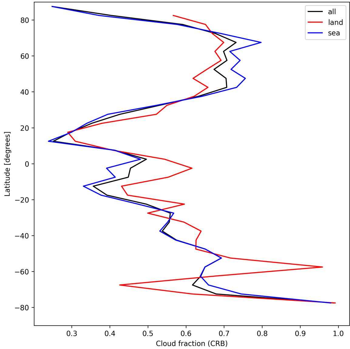
Figure 26: Zonal average of “Cloud fraction (CRB)” for 2025-04-24 to 2025-04-26.
