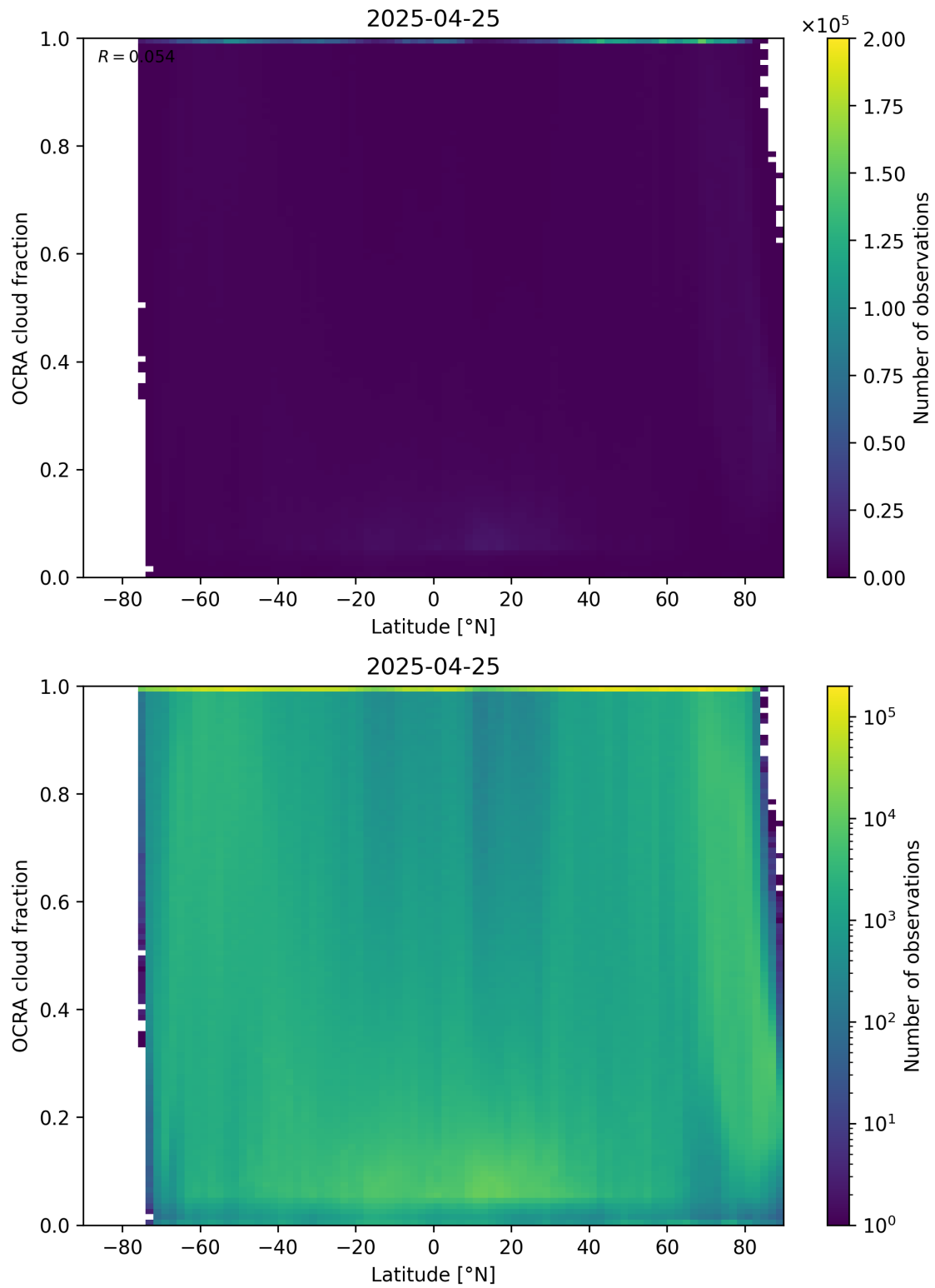
Figure 93: Scatter density plot of “Latitude” against “OCRA cloud fraction” for 2025-04-24 to 2025-04-26.
