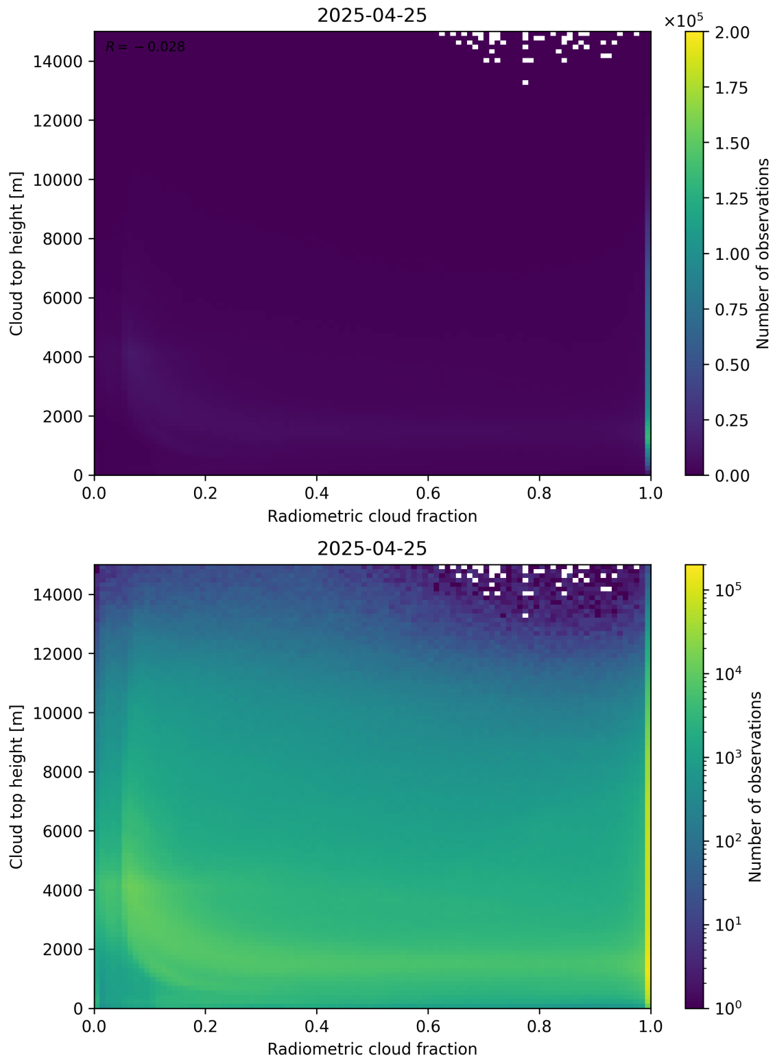
Figure 76: Scatter density plot of “Radiometric cloud fraction” against “Cloud top height” for 2025-04-24 to 2025-04-26.
