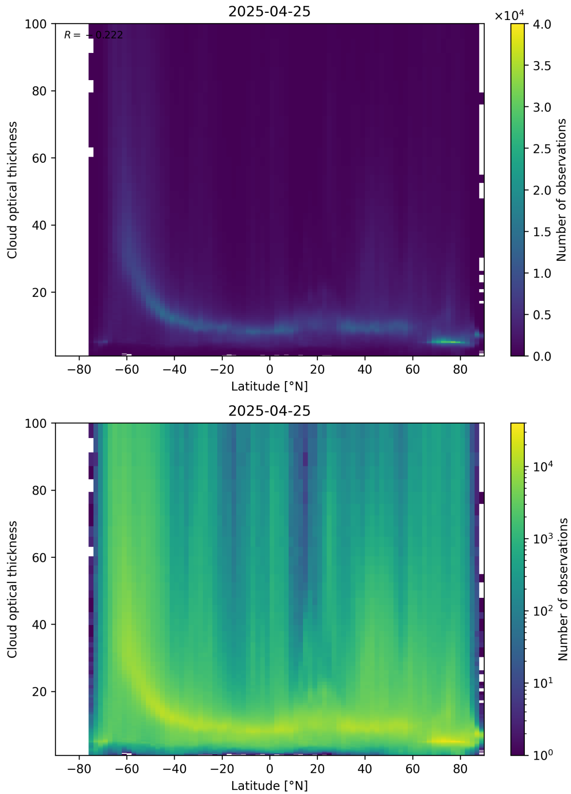
Figure 96: Scatter density plot of “Latitude” against “Cloud optical thickness” for 2025-04-24 to 2025-04-26.
