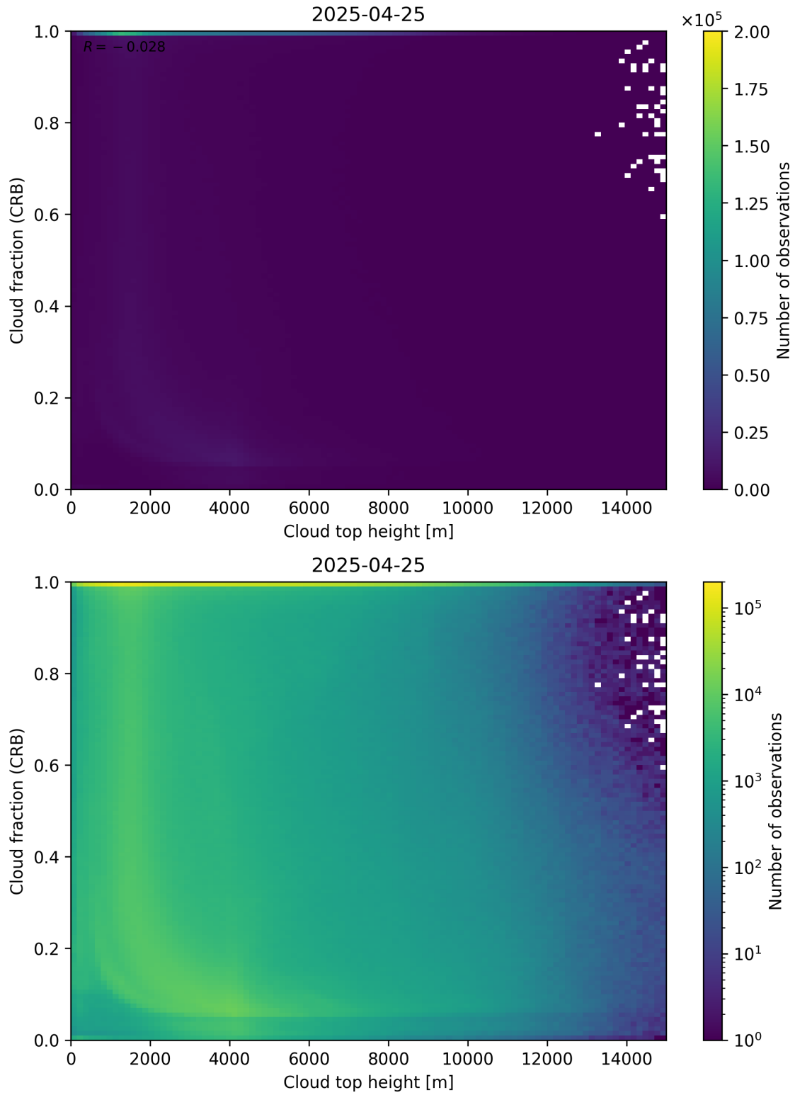
Figure 88: Scatter density plot of “Cloud top height” against “Cloud fraction (CRB)” for 2025-04-24 to 2025-04-26.
