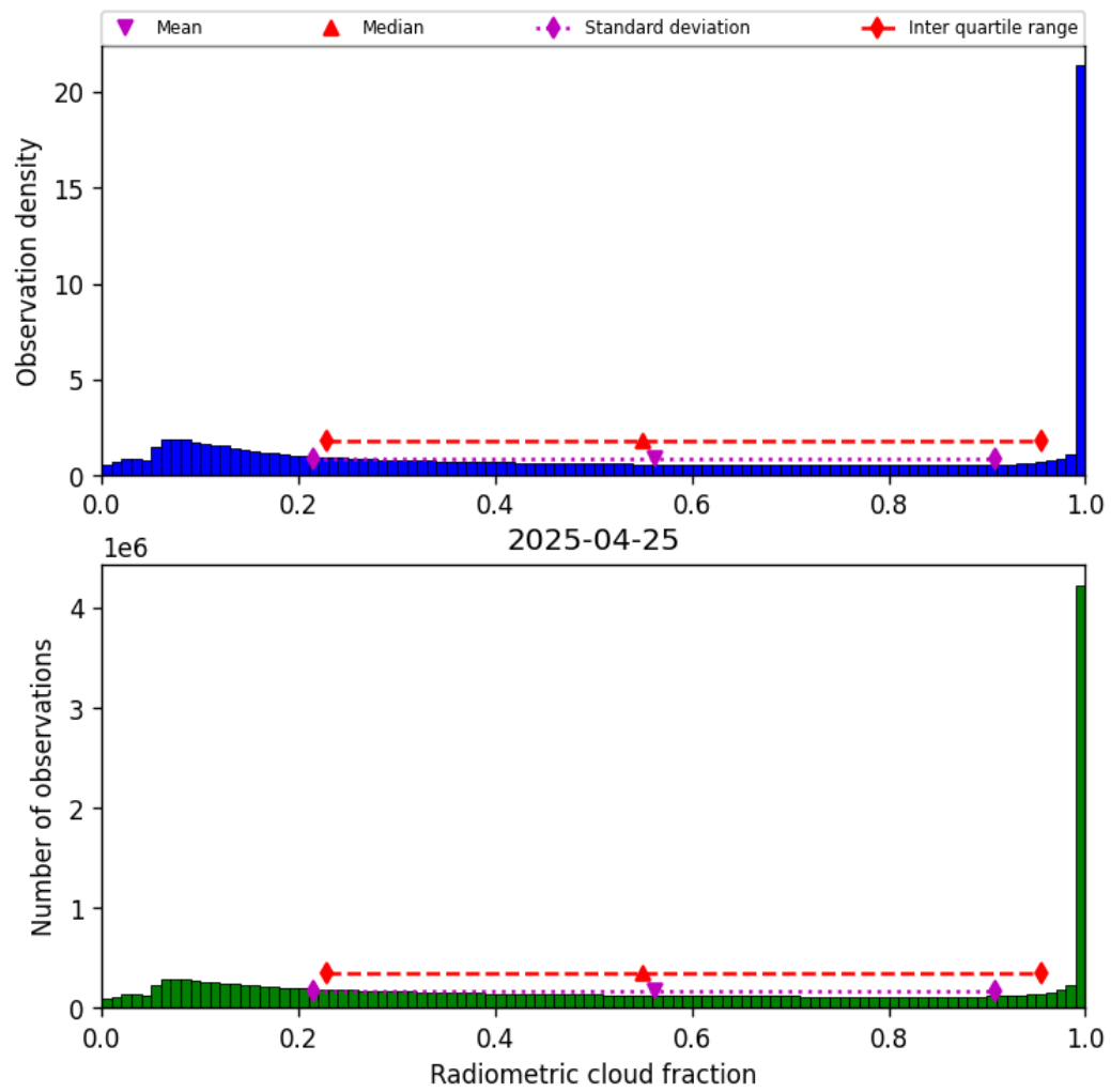
Figure 39: Histogram of “Radiometric cloud fraction” for 2025-04-24 to 2025-04-26
