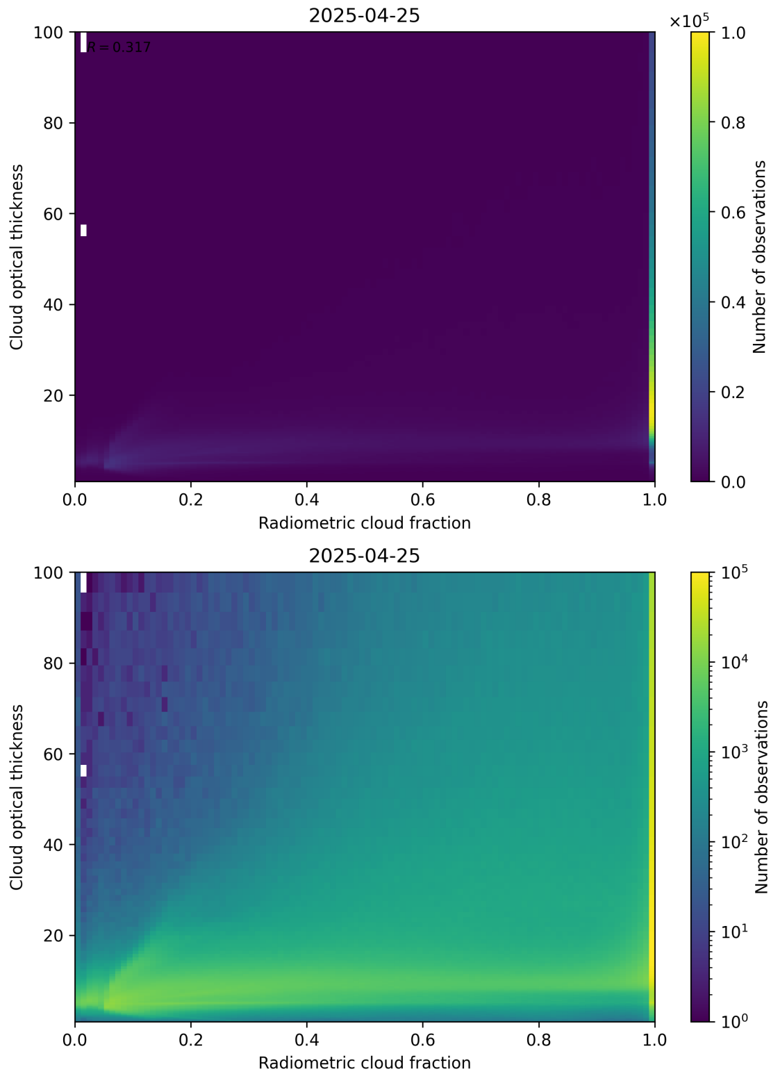
Figure 75: Scatter density plot of “Radiometric cloud fraction” against “Cloud optical thickness” for 2025-04-24 to 2025-04-26.
