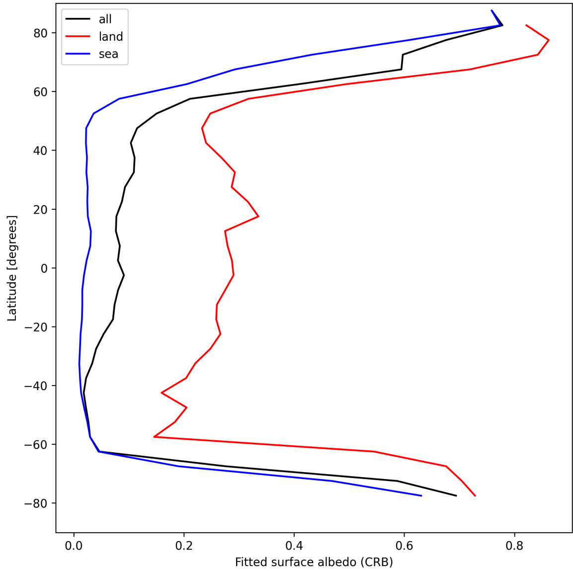
Figure 30: Zonal average of "Fitted surface albedo (CRB)" for 2025-04-24 to 2025-04-26.
