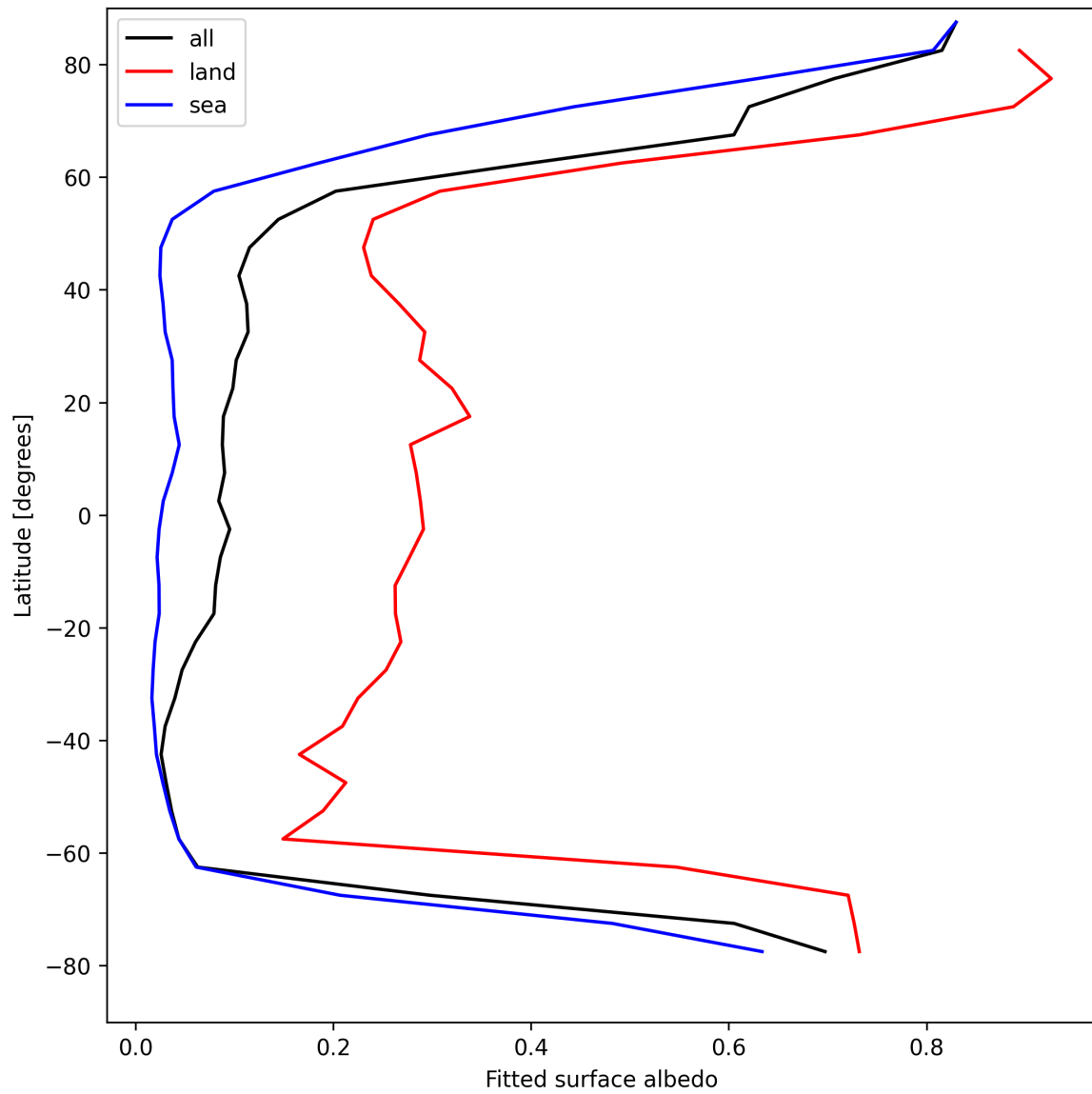
Figure 29: Zonal average of “Fitted surface albedo” for 2025-04-24 to 2025-04-26.
