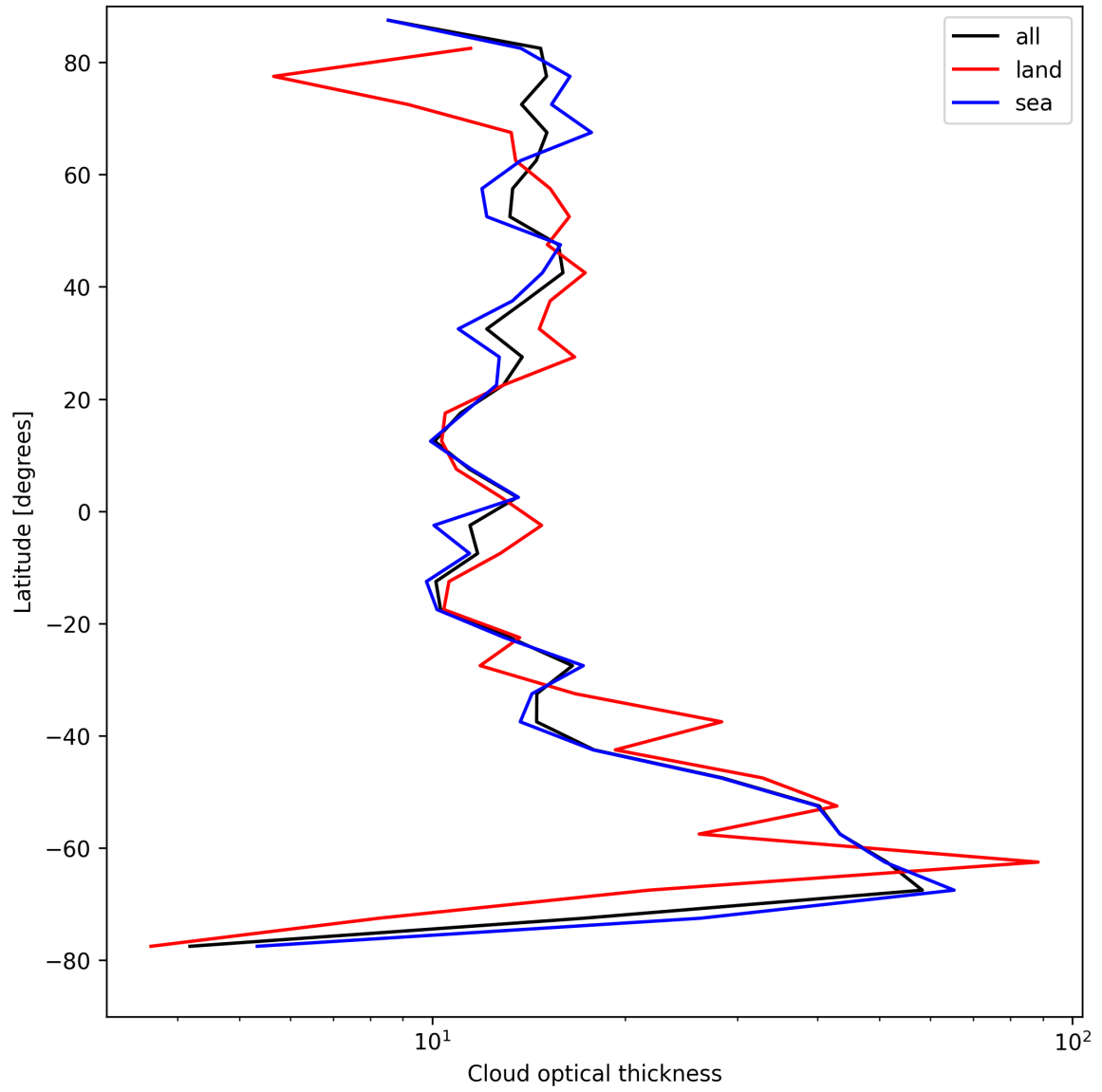
Figure 25: Zonal average of “Cloud optical thickness” for 2025-04-24 to 2025-04-26.
