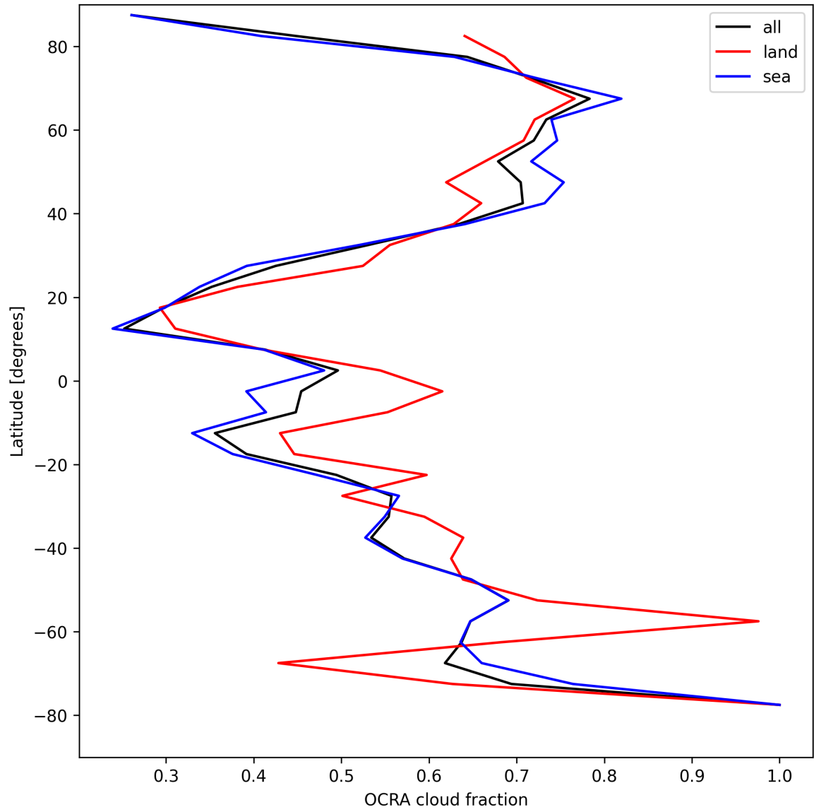
Figure 34: Zonal average of “OCRA cloud fraction” for 2025-04-24 to 2025-04-26.
