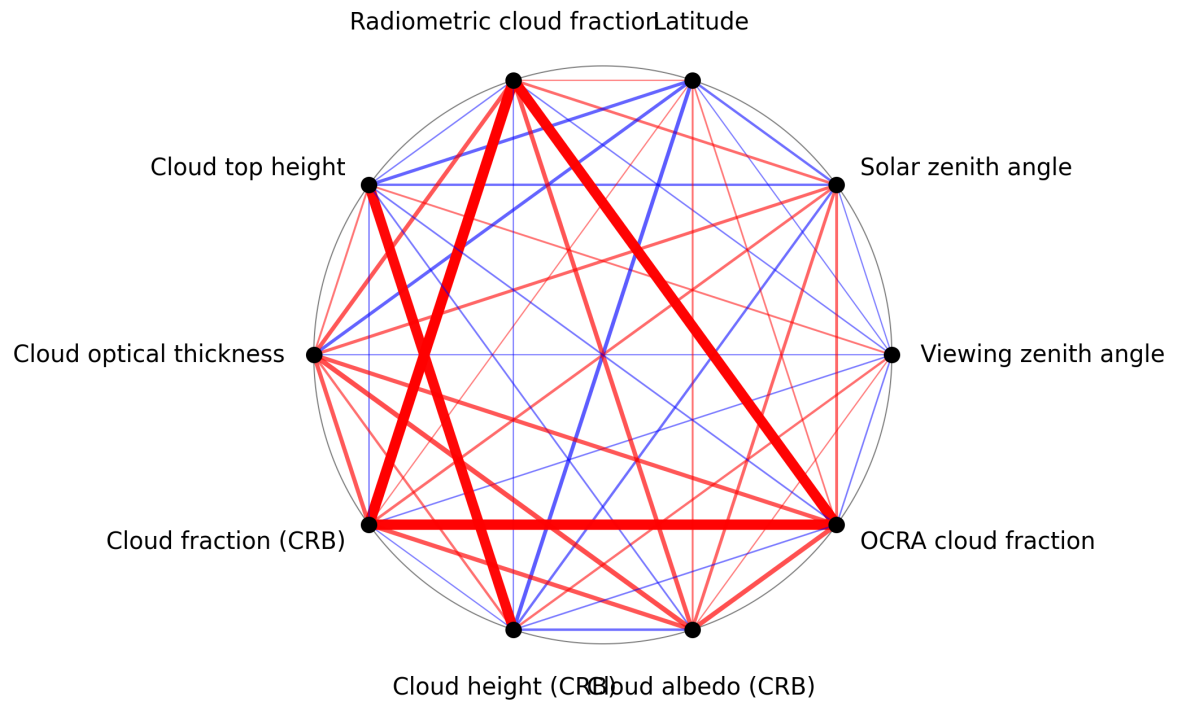
Figure 1: Map of correlation graph for 2025-04-24 to 2025-04-26.
