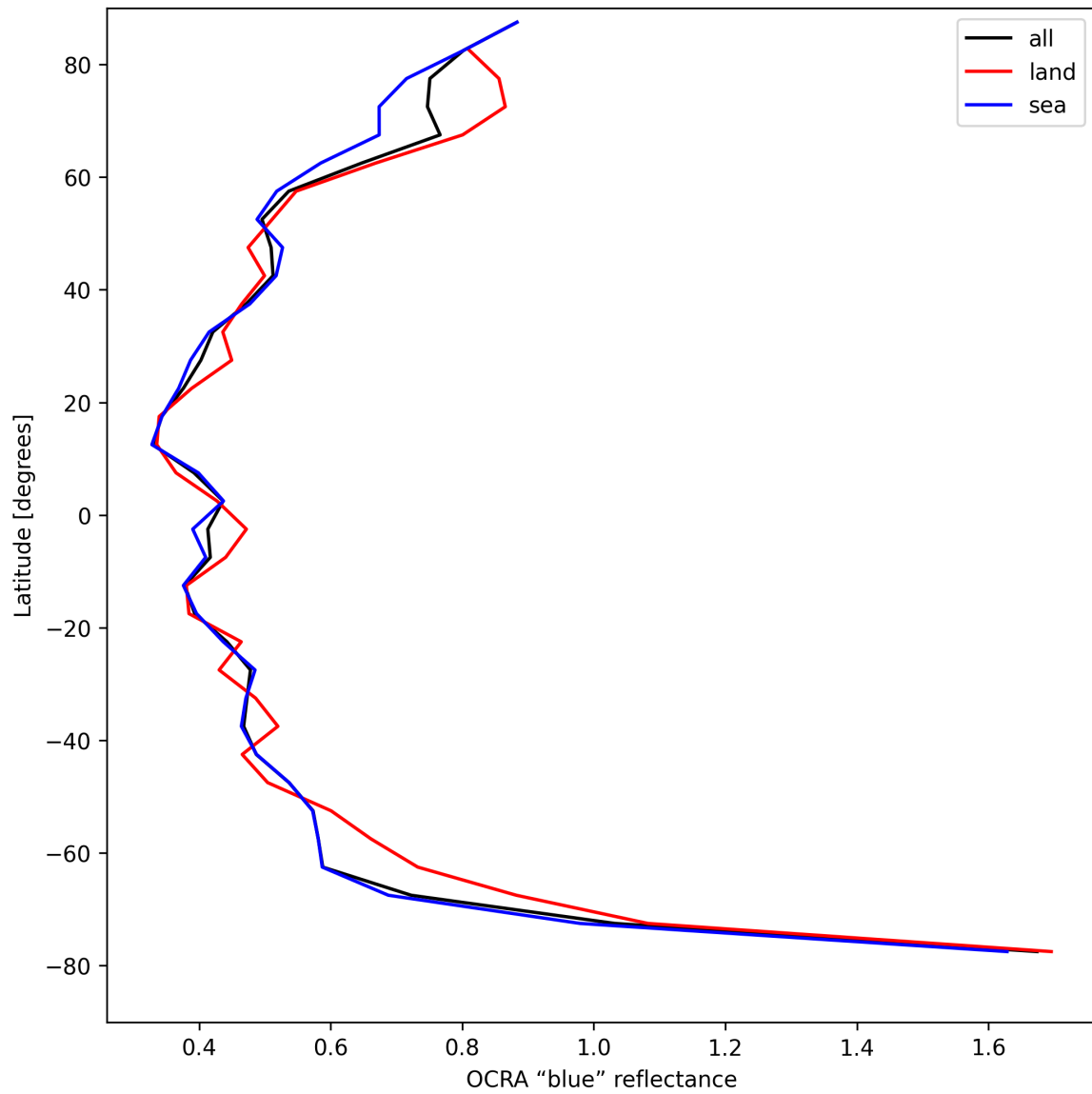
Figure 35: Zonal average of “OCRA “blue” reflectance” for 2025-04-24 to 2025-04-26.
