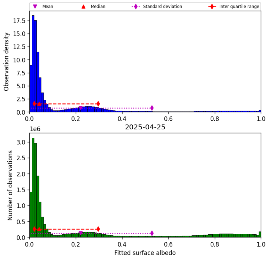
Figure 45: Histogram of “Fitted surface albedo” for 2025-04-24 to 2025-04-26
