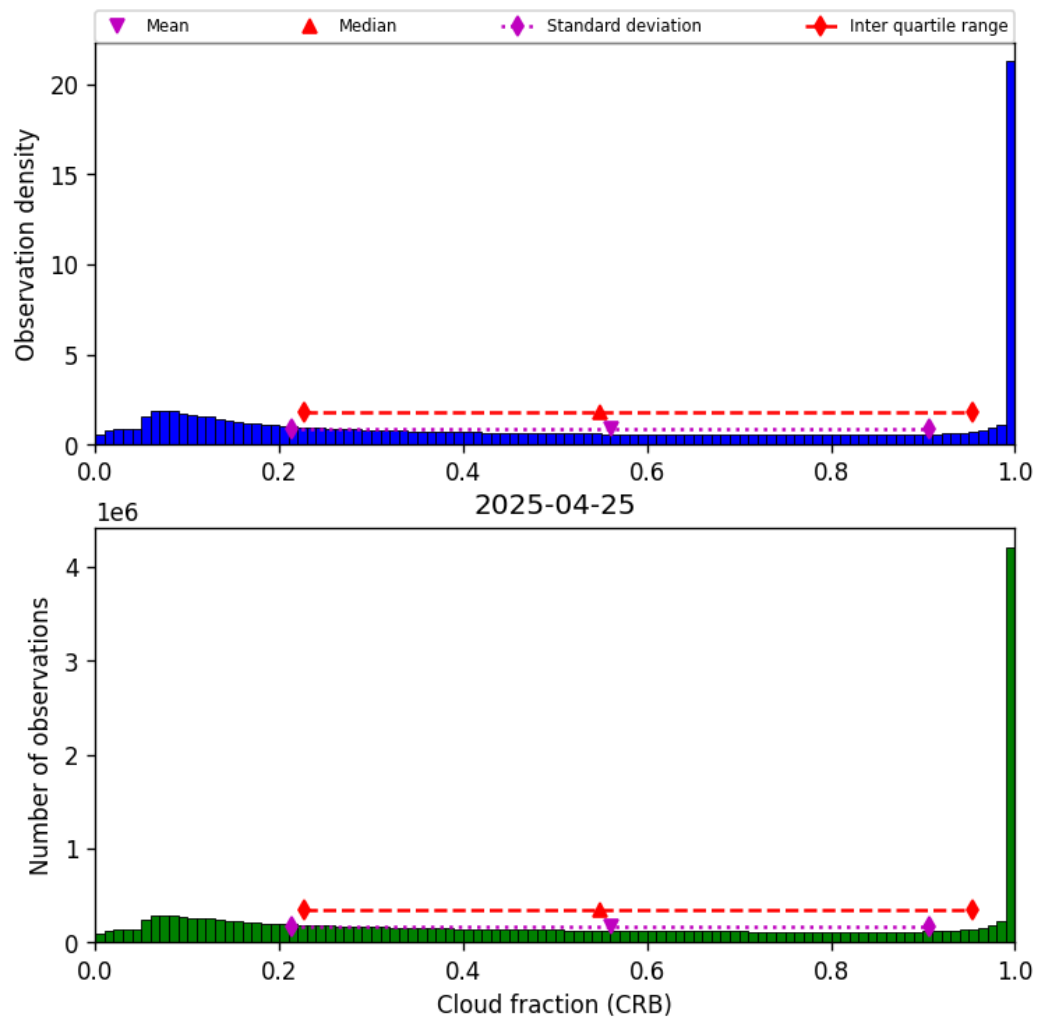
Figure 42: Histogram of “Cloud fraction (CRB)” for 2025-04-24 to 2025-04-26
