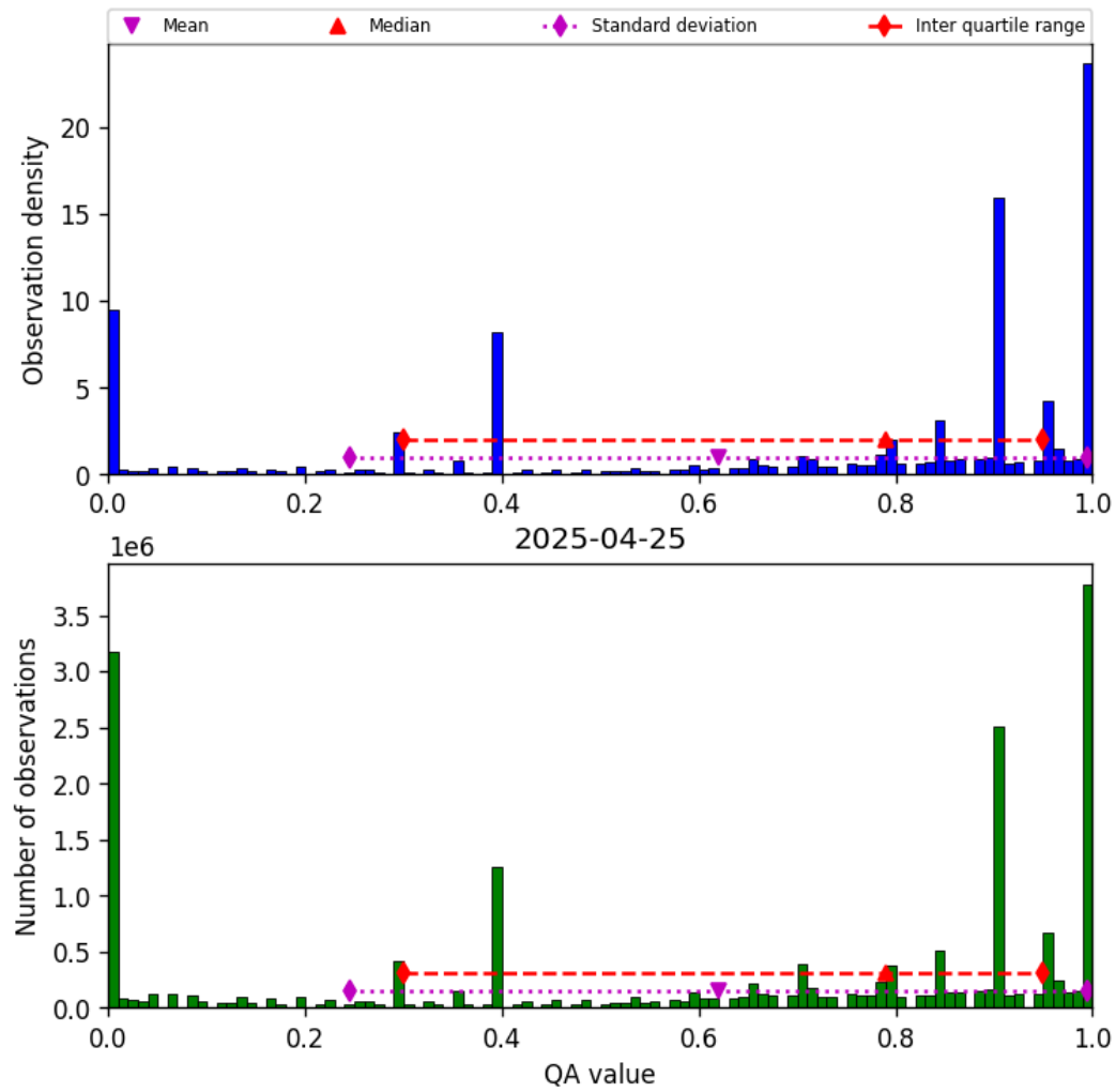
Figure 38: Histogram of “QA value” for 2025-04-24 to 2025-04-26
