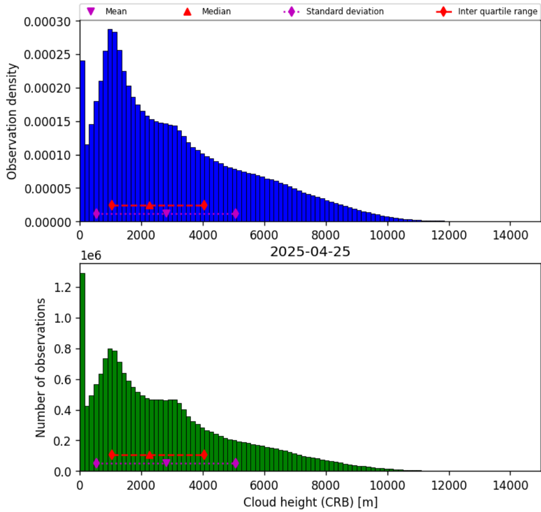
Figure 43: Histogram of “Cloud height (CRB)” for 2025-04-24 to 2025-04-26
