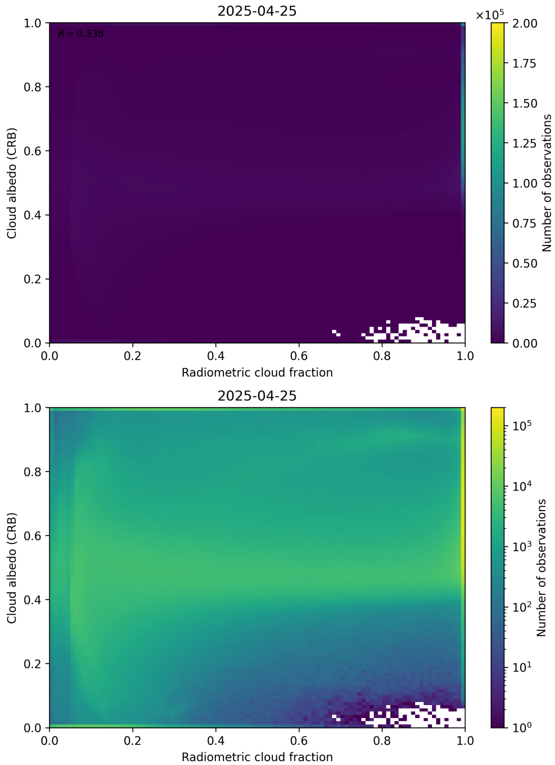
Figure 71: Scatter density plot of “Radiometric cloud fraction” against “Cloud albedo (CRB)” for 2025-04-24 to 2025-04-26.
