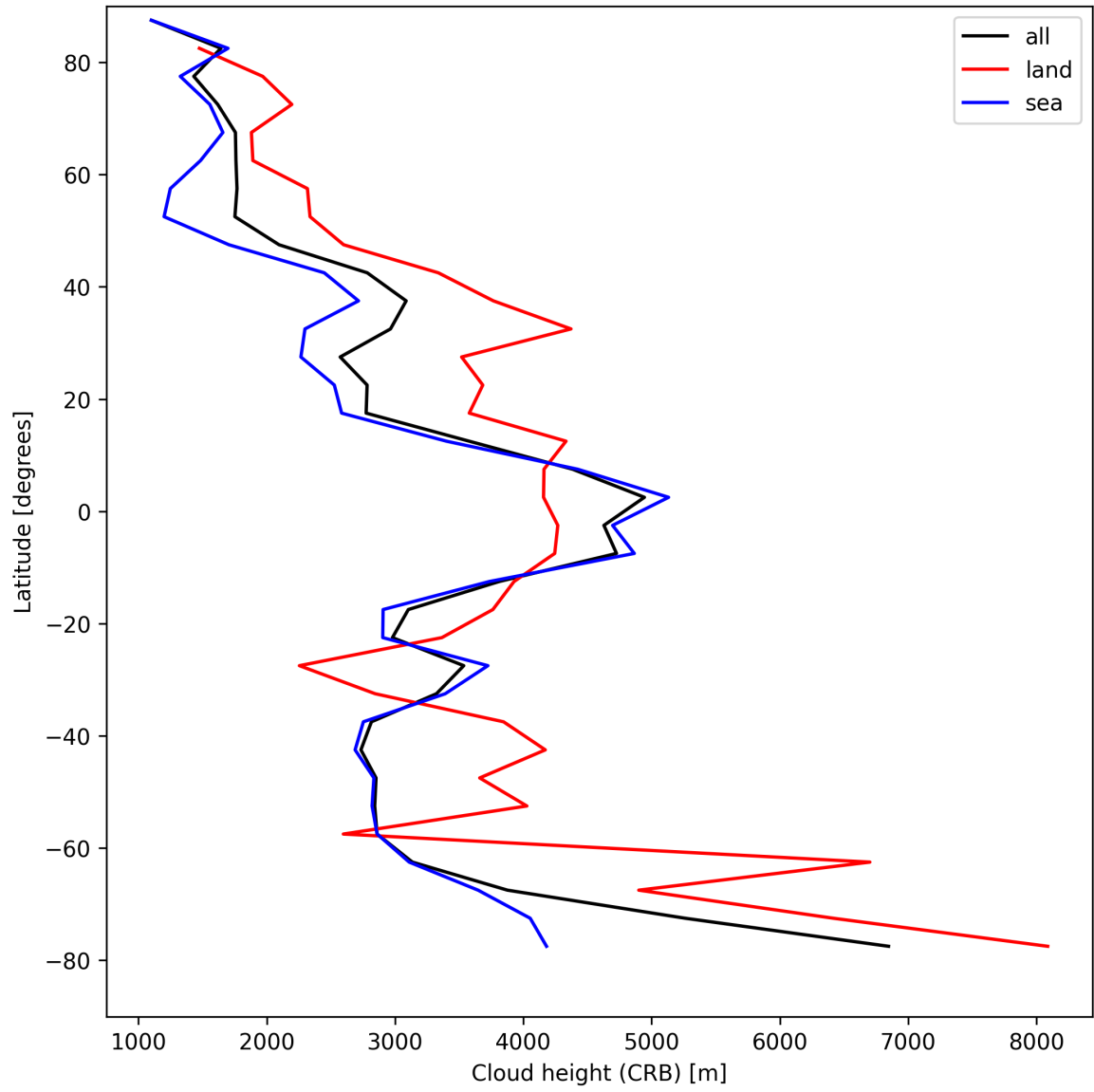
Figure 27: Zonal average of “Cloud height (CRB)” for 2025-04-24 to 2025-04-26.
