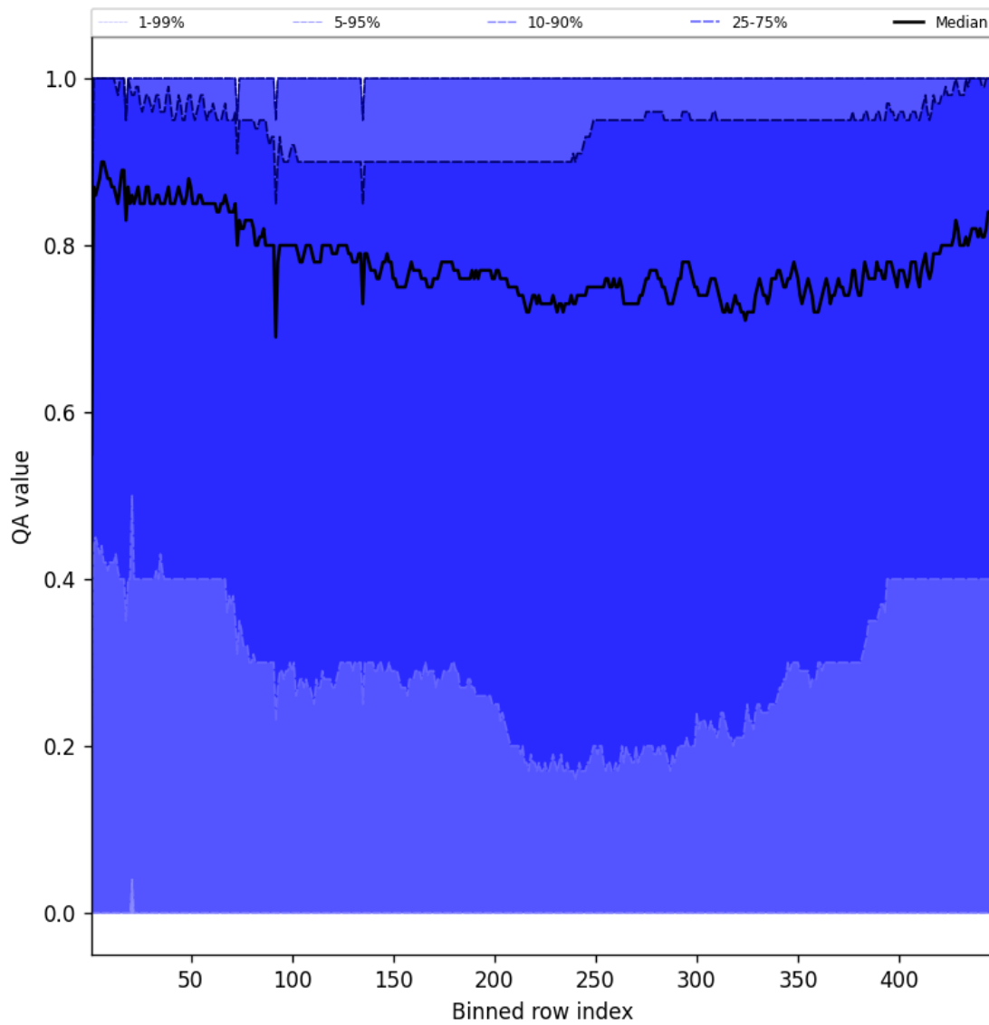
Figure 54: Along track statistics of "QA value" for 2025-04-24 to 2025-04-26
