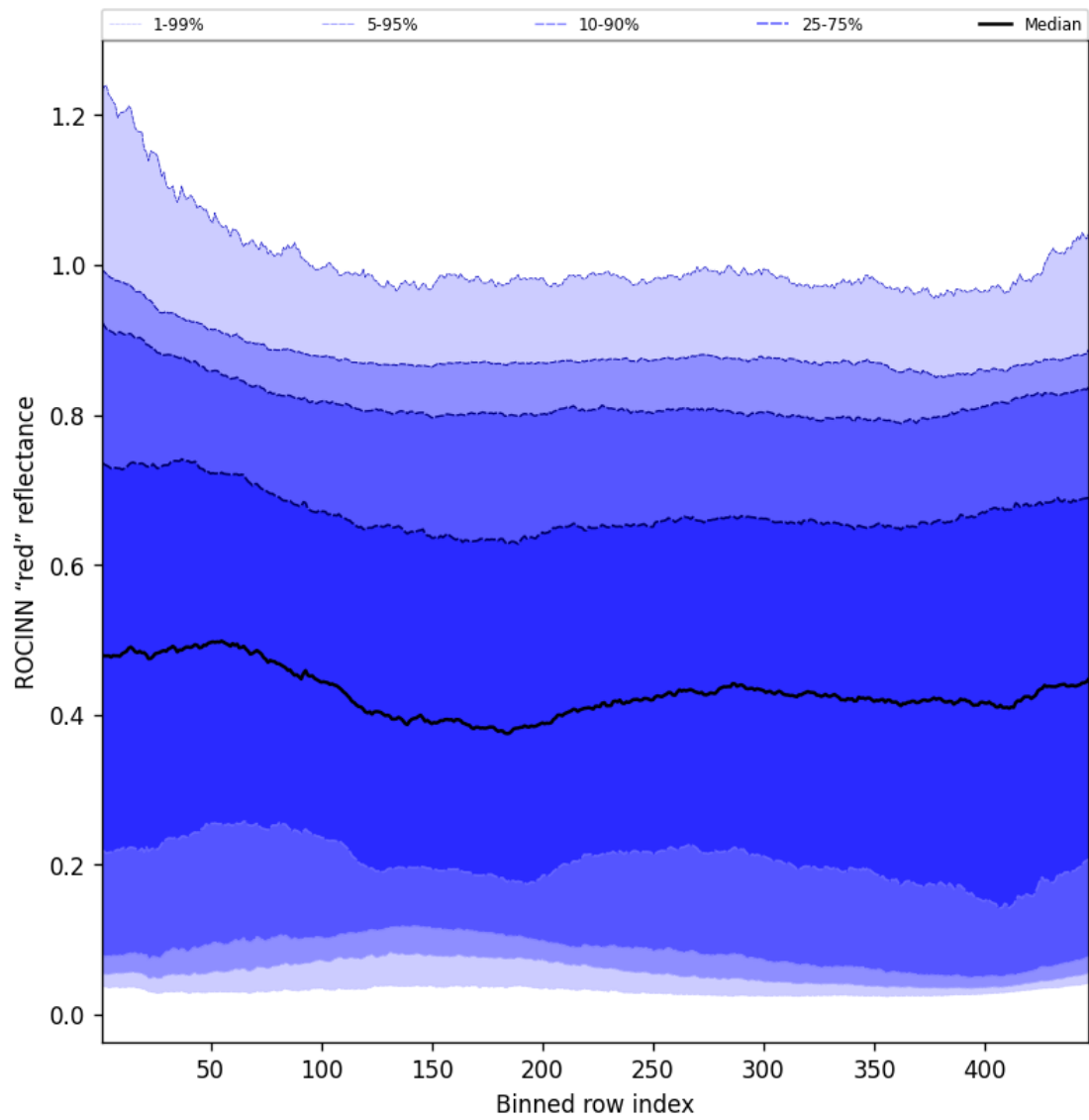
Figure 69: Along track statistics of "ROCINN "red" reflectance" for 2025-04-24 to 2025-04-26
