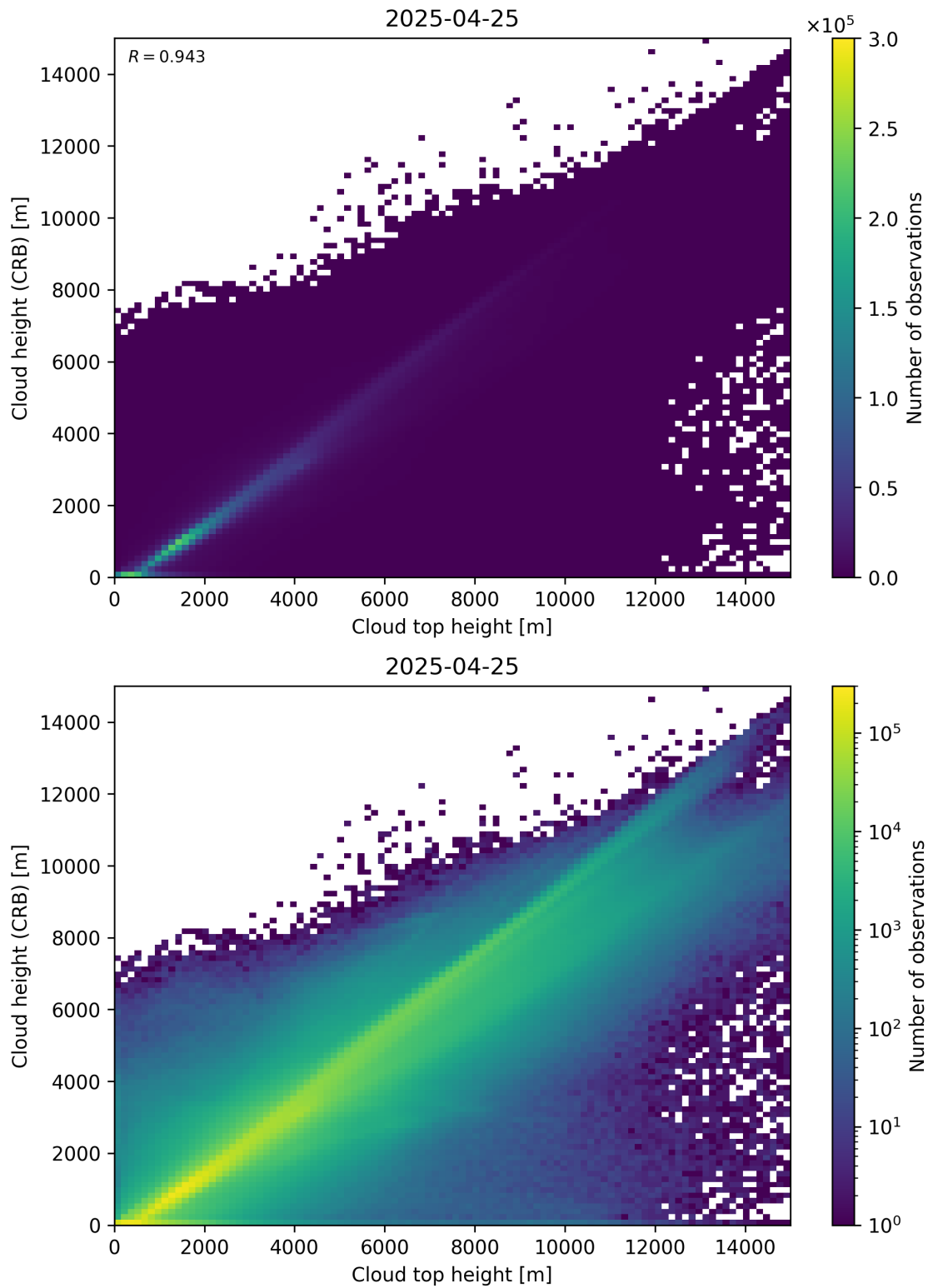
Figure 89: Scatter density plot of “Cloud top height” against “Cloud height (CRB)” for 2025-04-24 to 2025-04-26.
