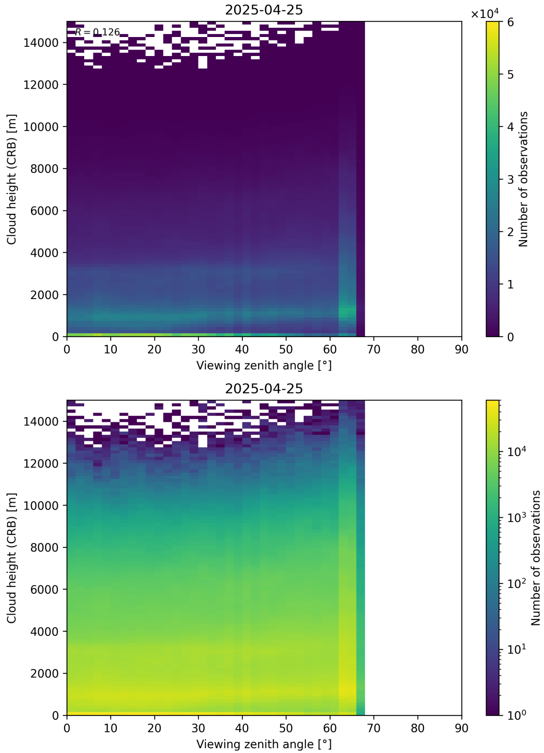
Figure 110: Scatter density plot of “Viewing zenith angle” against “Cloud height (CRB)” for 2025-04-24 to 2025-04-26.
