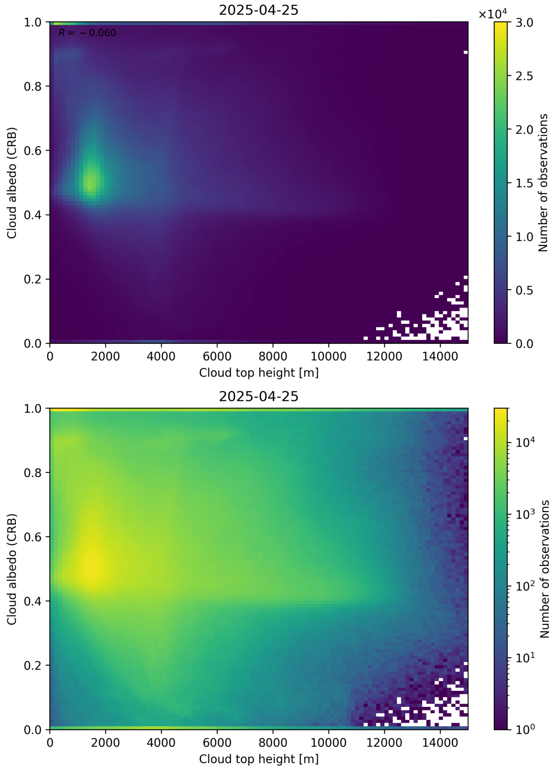
Figure 86: Scatter density plot of “Cloud top height” against “Cloud albedo (CRB)” for 2025-04-24 to 2025-04-26.
