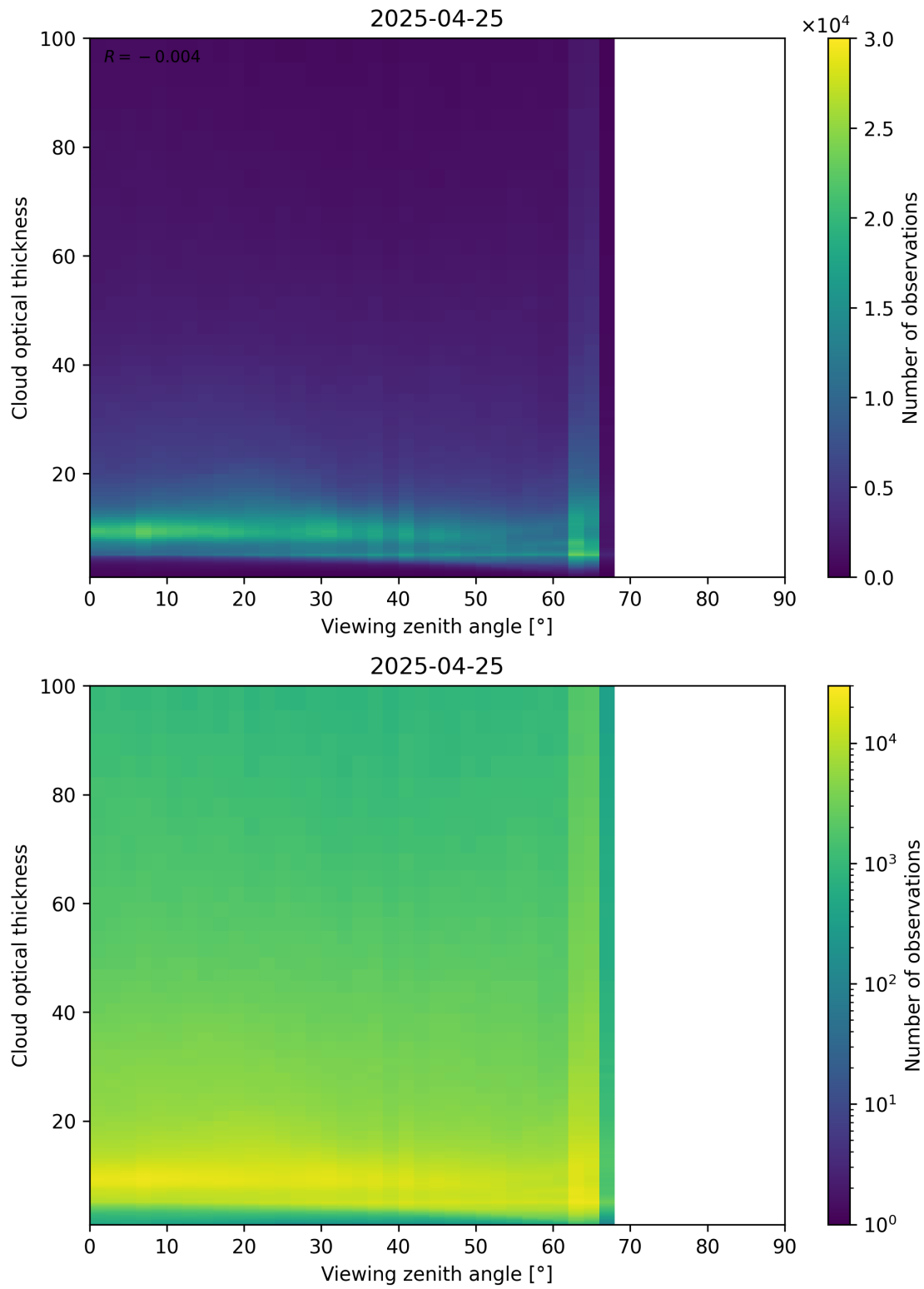
Figure 111: Scatter density plot of “Viewing zenith angle” against “Cloud optical thickness” for 2025-04-24 to 2025-04-26.
