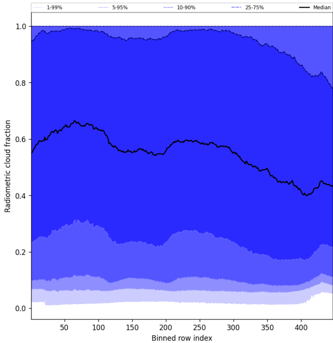
Figure 55: Along track statistics of “Radiometric cloud fraction” for 2025-04-24 to 2025-04-26
