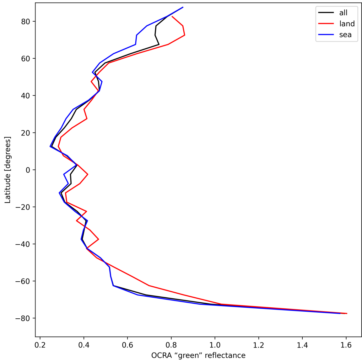
Figure 36: Zonal average of “OCRA “green” reflectance” for 2025-04-24 to 2025-04-26.
