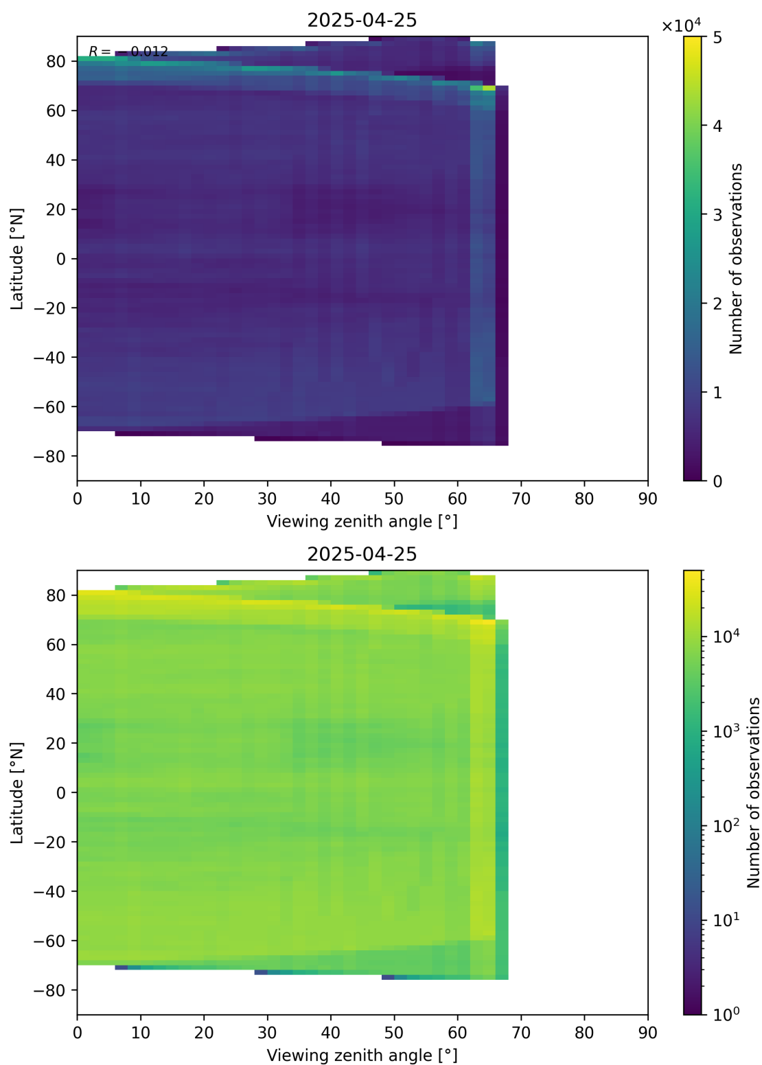
Figure 113: Scatter density plot of “Viewing zenith angle” against “Latitude” for 2025-04-24 to 2025-04-26.
