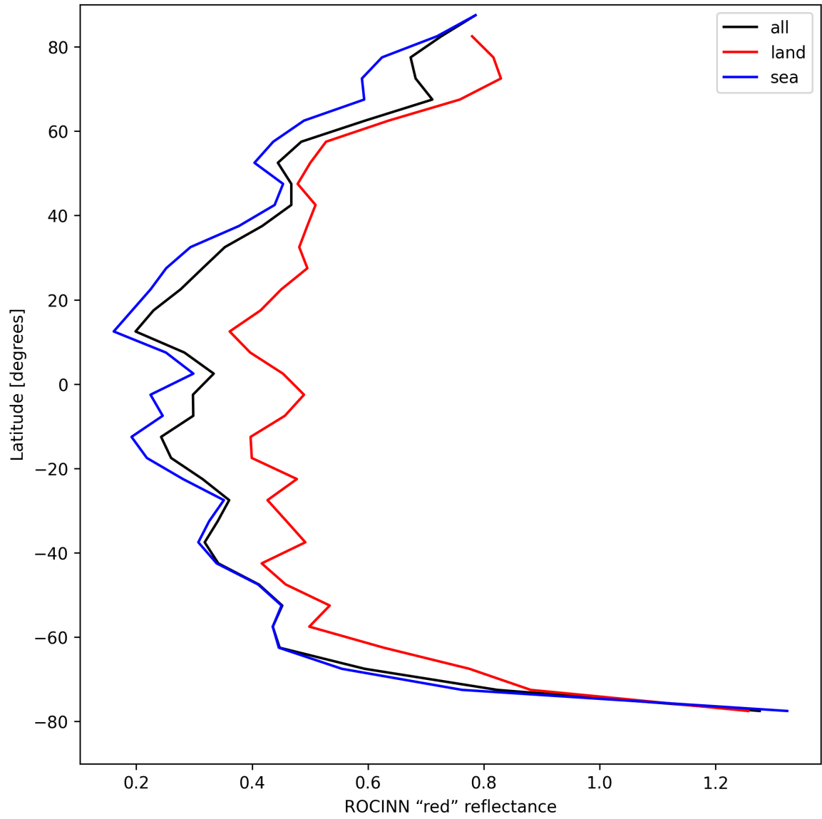
Figure 37: Zonal average of “ROCINN “red” reflectance” for 2025-04-24 to 2025-04-26.
