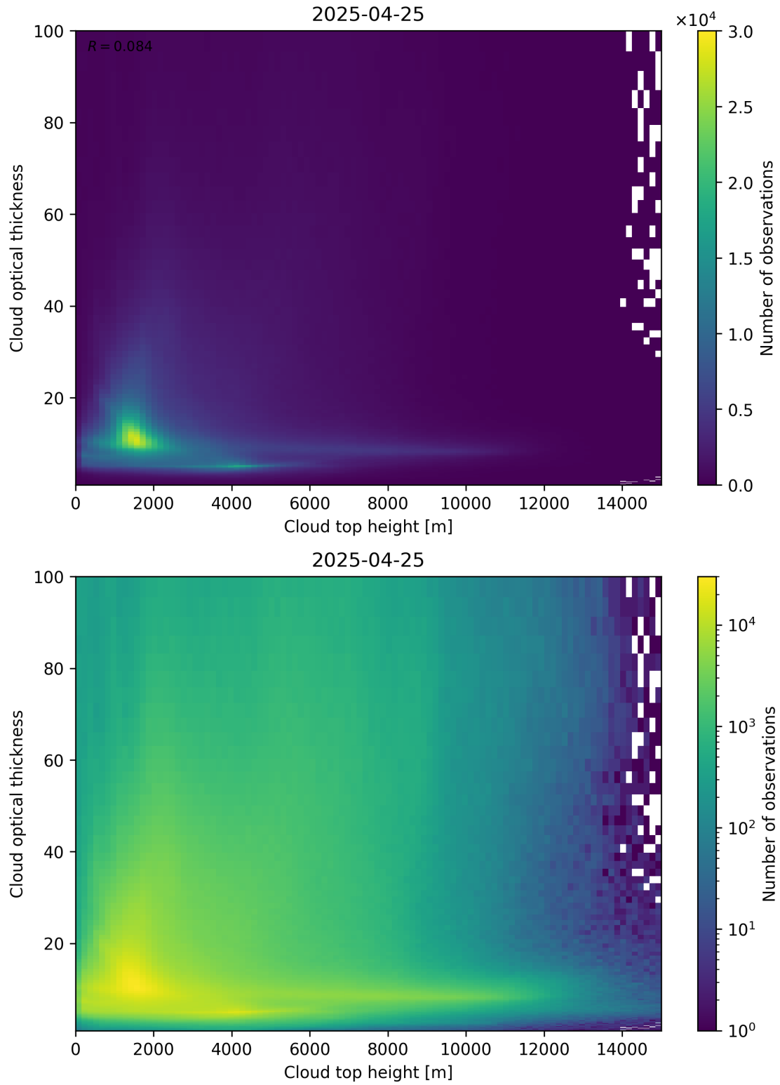
Figure 90: Scatter density plot of “Cloud top height” against “Cloud optical thickness” for 2025-04-24 to 2025-04-26.
