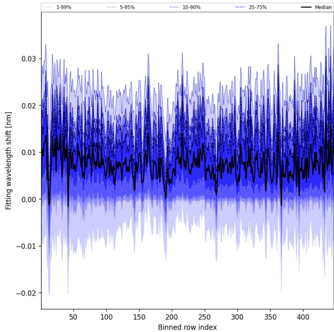
Figure 65: Along track statistics of “Fitting wavelength shift” for 2025-04-24 to 2025-04-26
