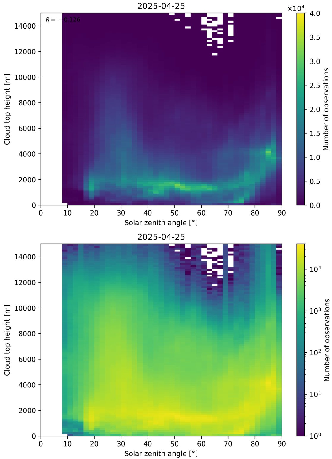
Figure 104: Scatter density plot of “Solar zenith angle” against “Cloud top height” for 2025-04-24 to 2025-04-26.
