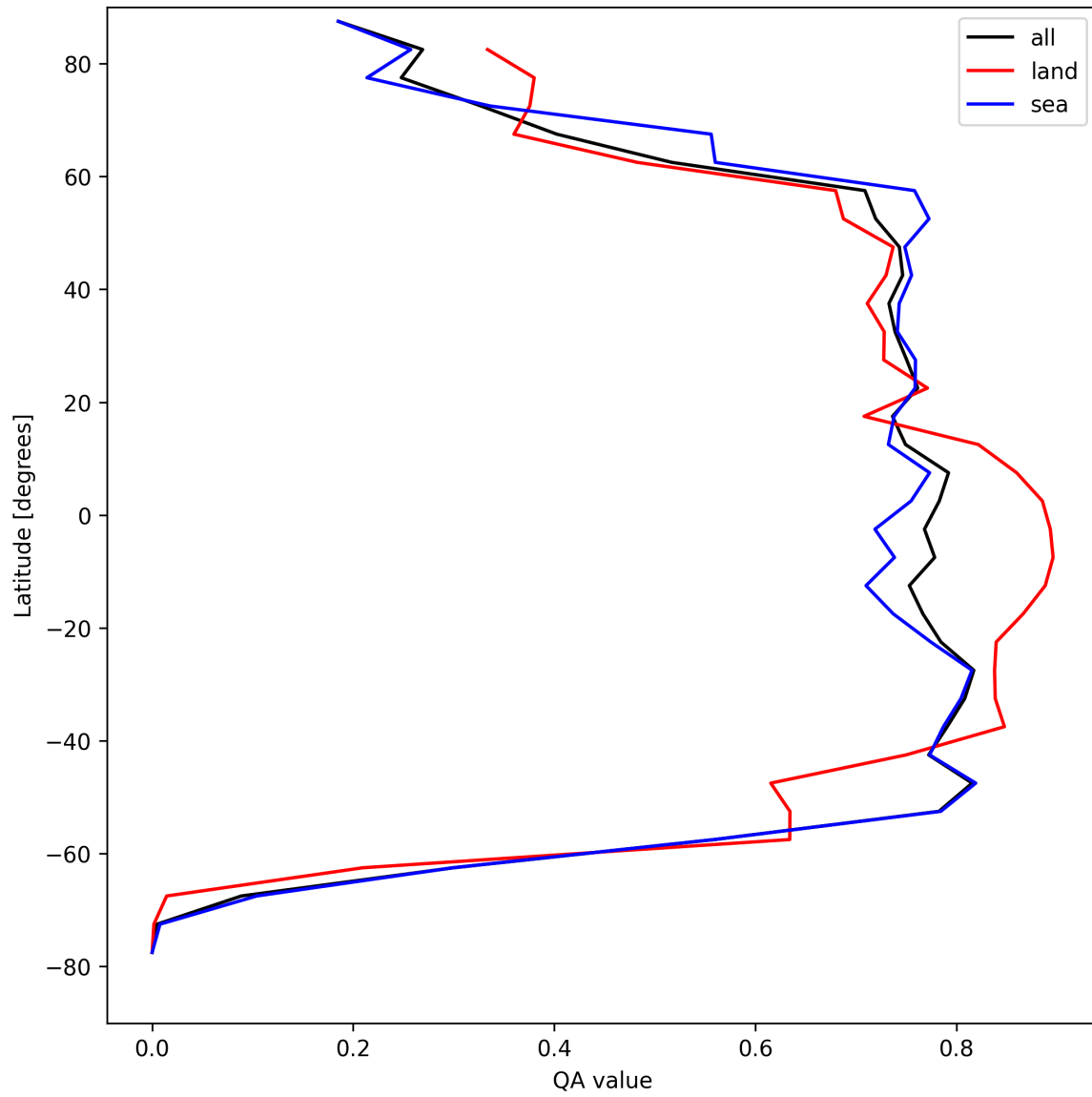
Figure 22: Zonal average of “QA value” for 2025-04-24 to 2025-04-26.
