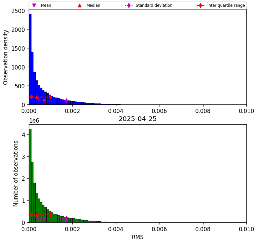
Figure 47: Histogram of “RMS” for 2025-04-24 to 2025-04-26
