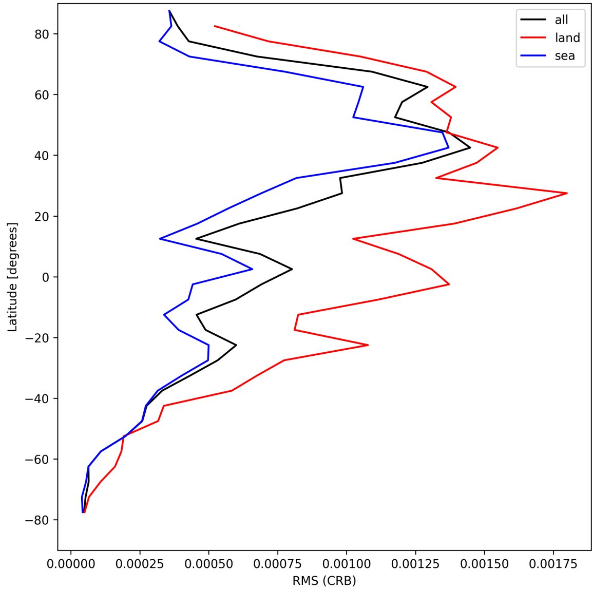
Figure 32: Zonal average of “RMS (CRB)” for 2025-04-24 to 2025-04-26.
