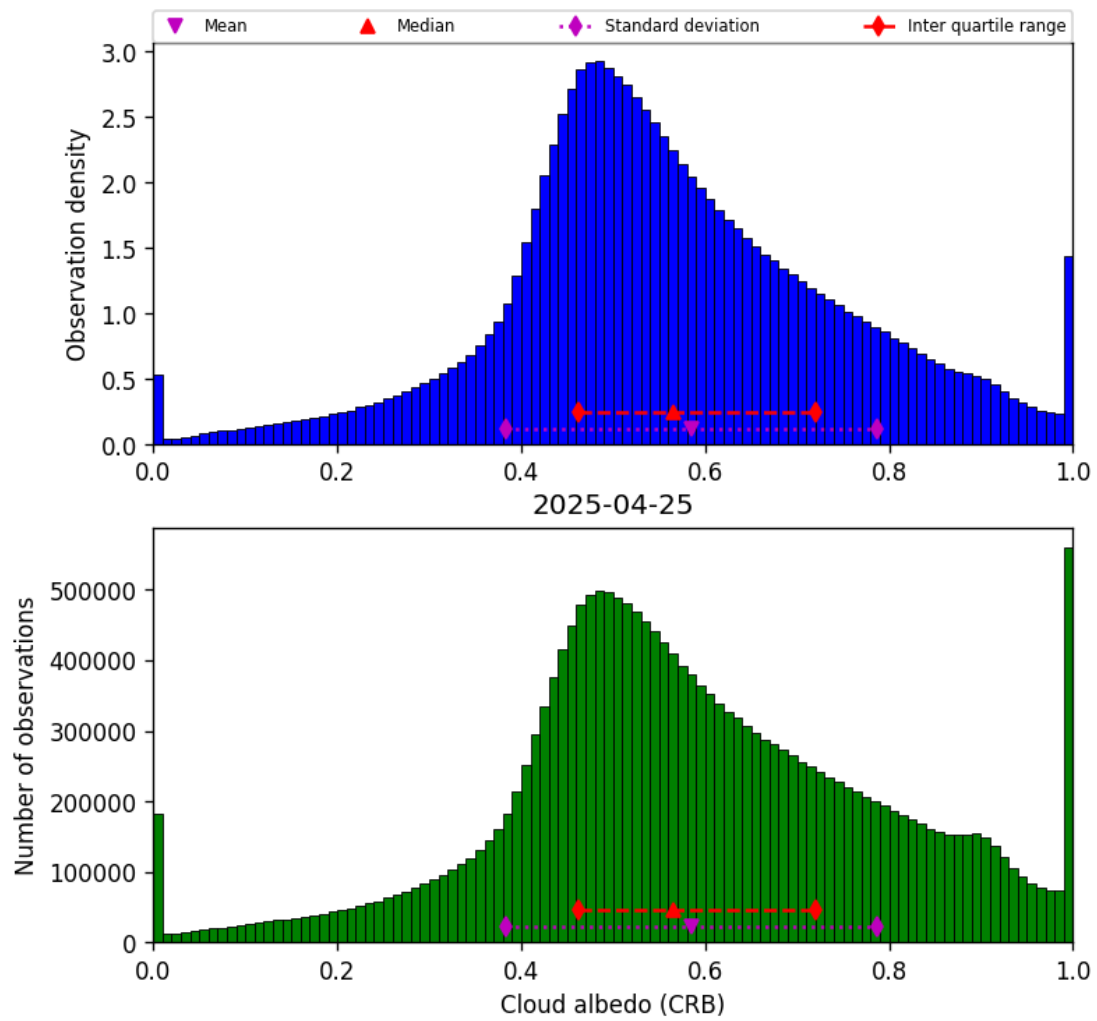
Figure 44: Histogram of “Cloud albedo (CRB)” for 2025-04-24 to 2025-04-26
