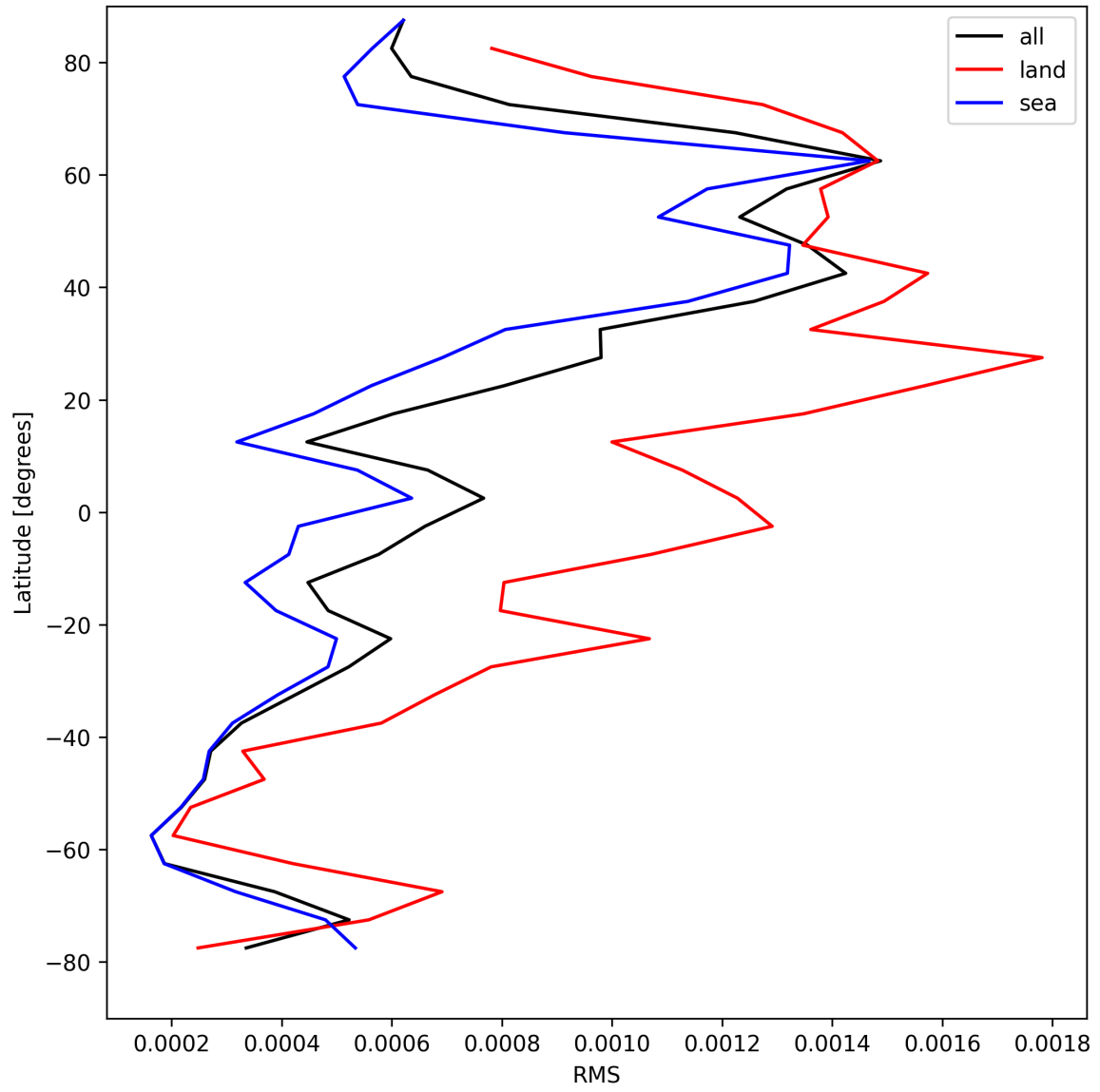
Figure 31: Zonal average of “RMS” for 2025-04-24 to 2025-04-26.
