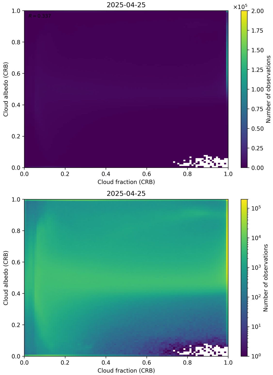
Figure 77: Scatter density plot of “Cloud fraction (CRB)” against “Cloud albedo (CRB)” for 2025-04-24 to 2025-04-26.
