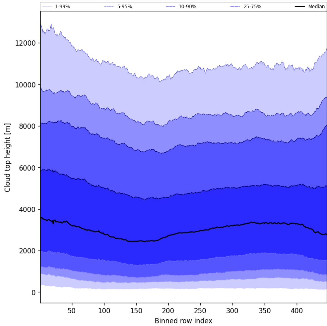
Figure 56: Along track statistics of “Cloud top height” for 2025-04-24 to 2025-04-26
