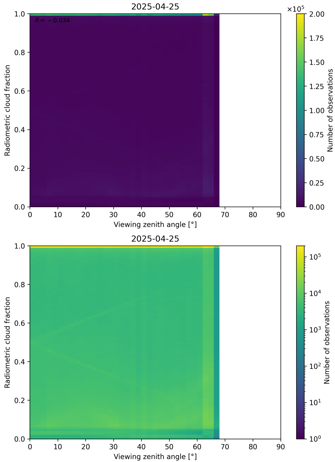
Figure 107: Scatter density plot of “Viewing zenith angle” against “Radiometric cloud fraction” for 2025-04-24 to 2025-04-26.
