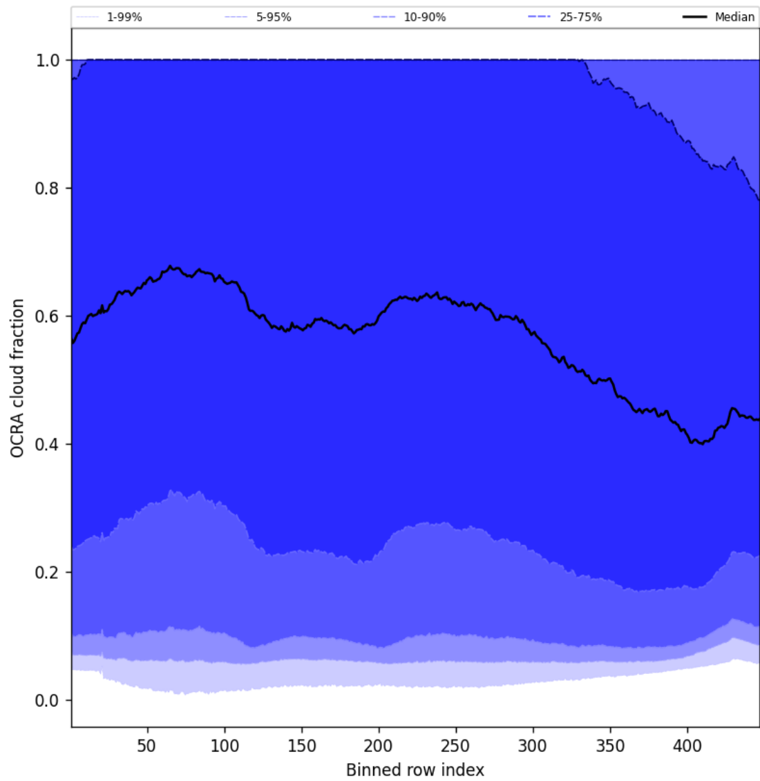
Figure 66: Along track statistics of “OCRA cloud fraction” for 2025-04-24 to 2025-04-26
