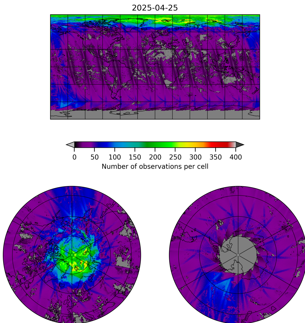
Figure 21: Map of the number of observations for 2025-04-24 to 2025-04-26
