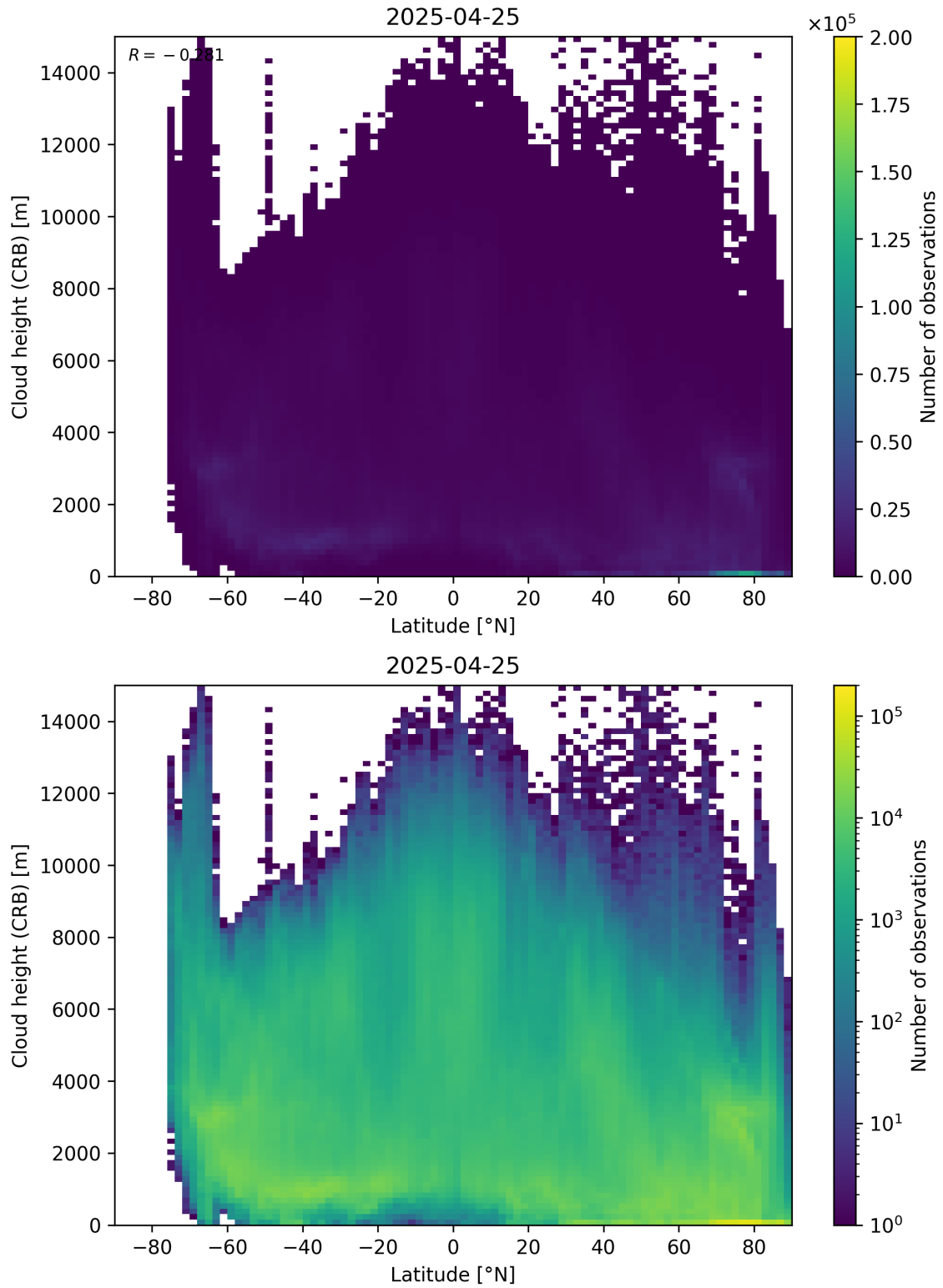
Figure 95: Scatter density plot of “Latitude” against “Cloud height (CRB)” for 2025-04-24 to 2025-04-26.
