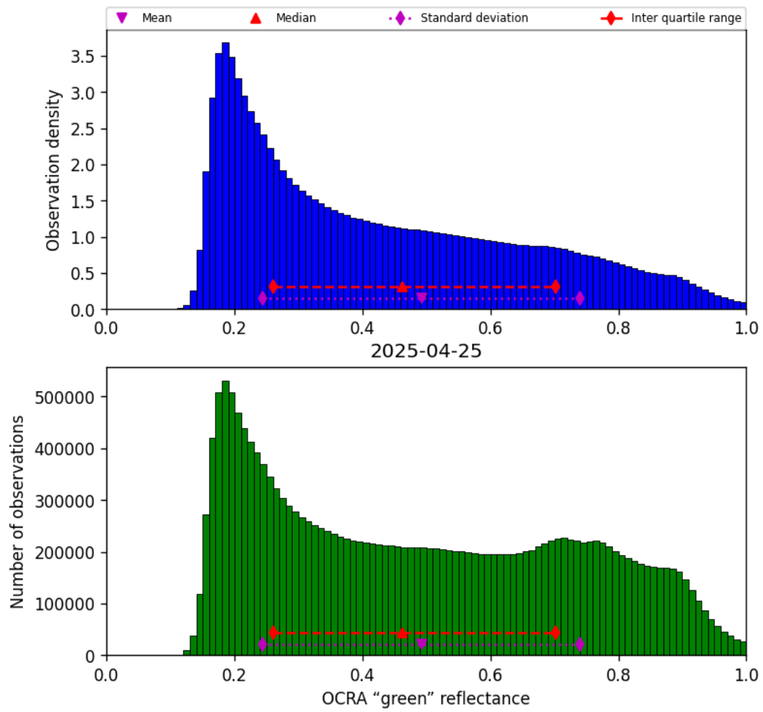
Figure 52: Histogram of “OCRA “green” reflectance” for 2025-04-24 to 2025-04-26
