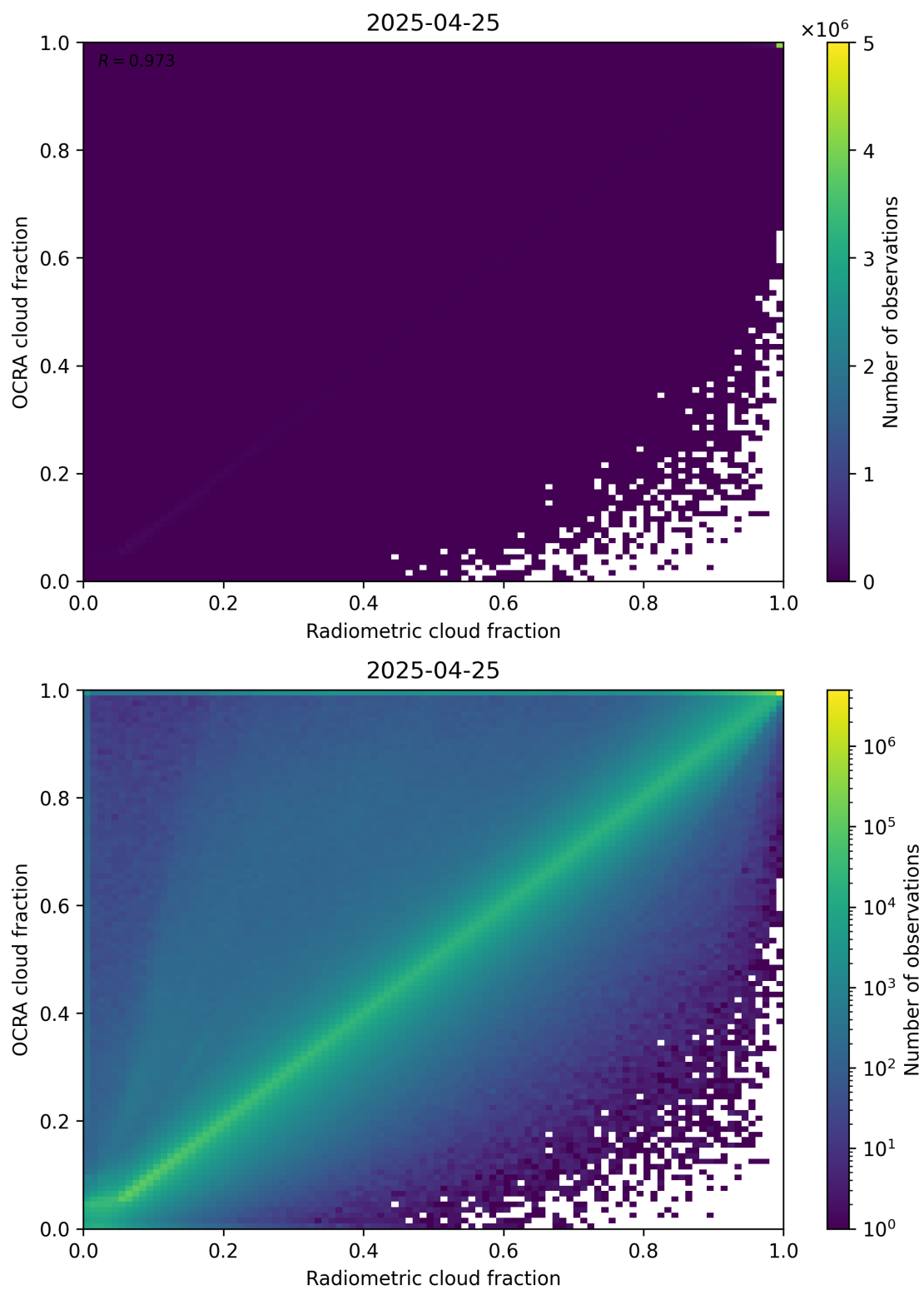
Figure 72: Scatter density plot of “Radiometric cloud fraction” against “OCRA cloud fraction” for 2025-04-24 to 2025-04-26.
