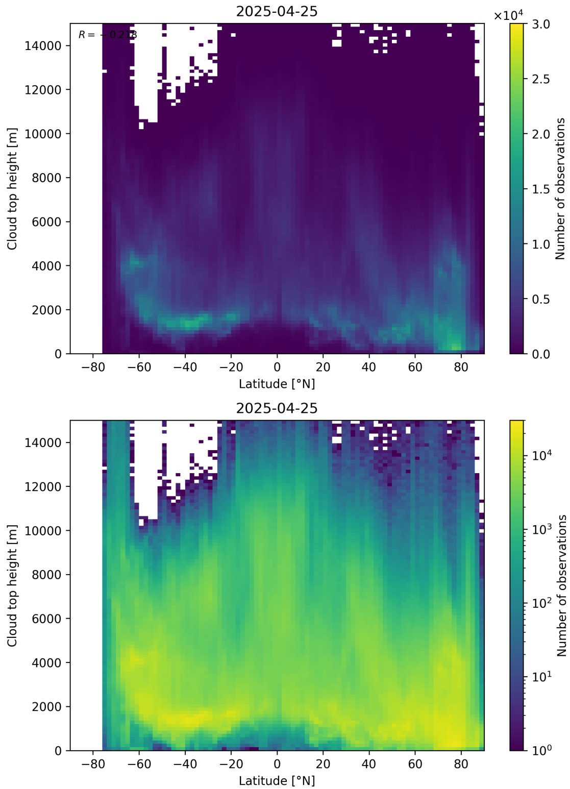
Figure 97: Scatter density plot of “Latitude” against “Cloud top height” for 2025-04-24 to 2025-04-26.
