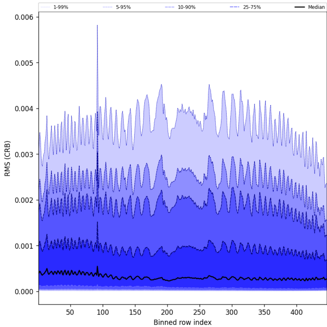
Figure 64: Along track statistics of "RMS (CRB)" for 2025-04-24 to 2025-04-26
