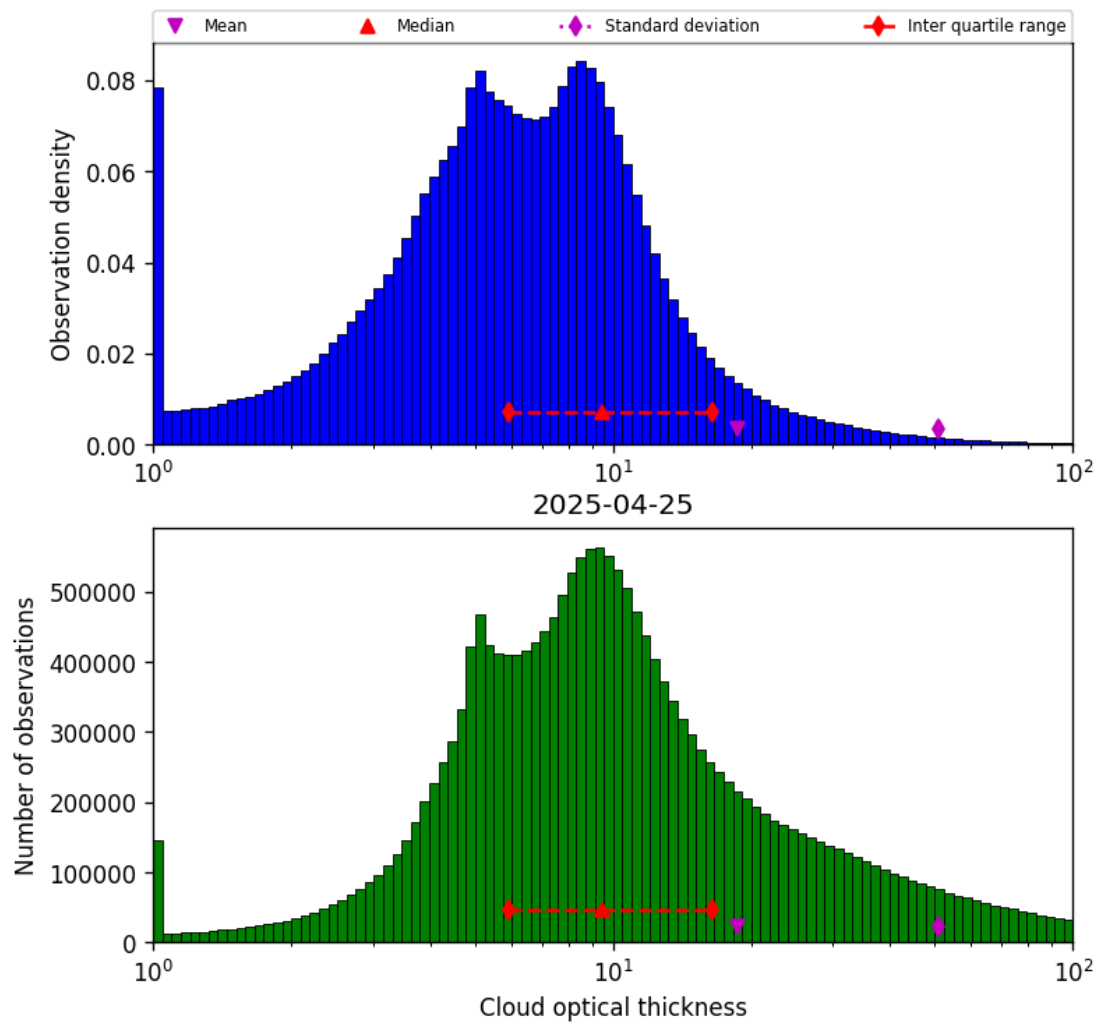
Figure 41: Histogram of “Cloud optical thickness” for 2025-04-24 to 2025-04-26
