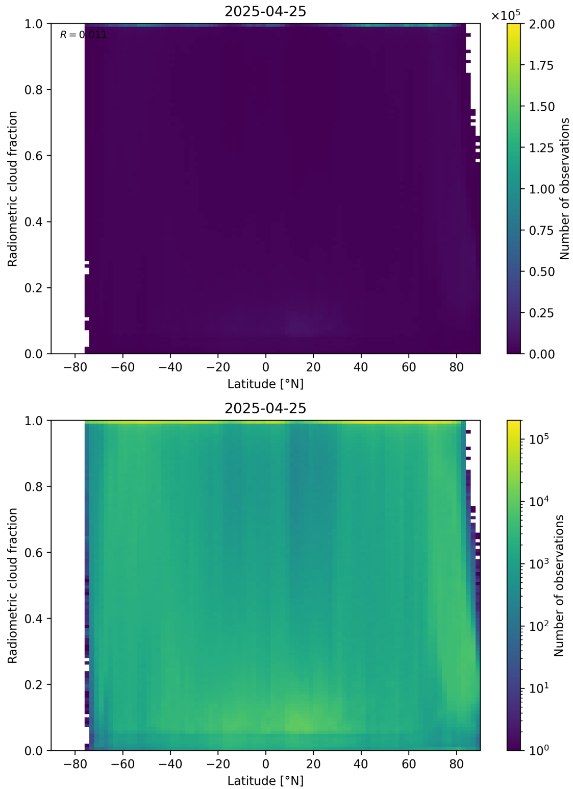
Figure 92: Scatter density plot of “Latitude” against “Radiometric cloud fraction” for 2025-04-24 to 2025-04-26.
