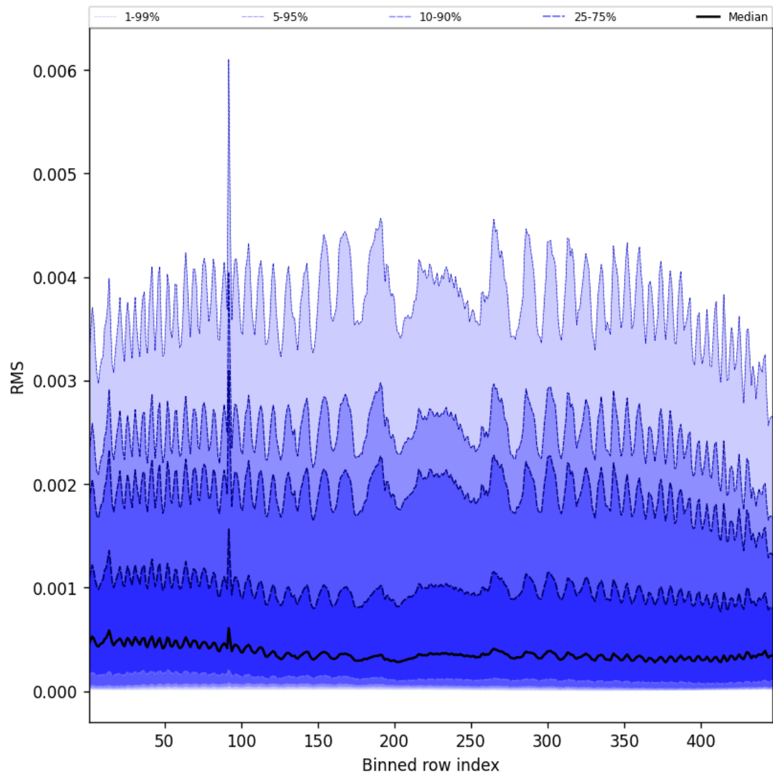
Figure 63: Along track statistics of “RMS” for 2025-04-24 to 2025-04-26
