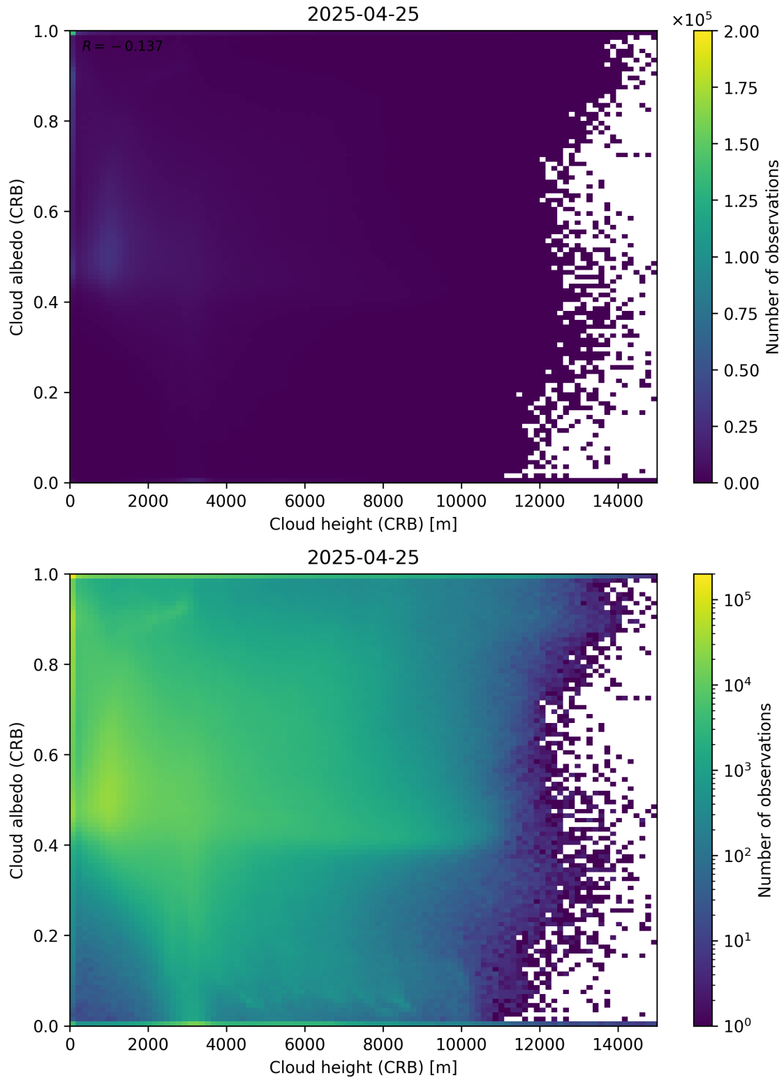
Figure 80: Scatter density plot of “Cloud height (CRB)” against “Cloud albedo (CRB)” for 2025-04-24 to 2025-04-26.
