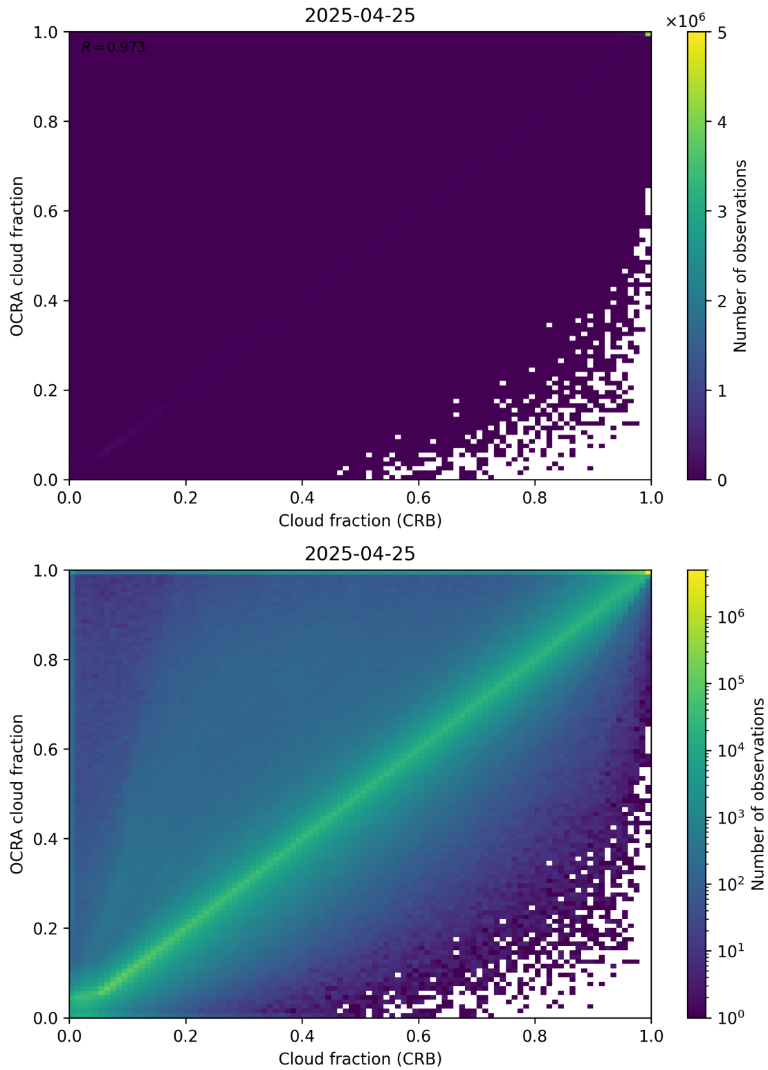
Figure 78: Scatter density plot of “Cloud fraction (CRB)” against “OCRA cloud fraction” for 2025-04-24 to 2025-04-26.
