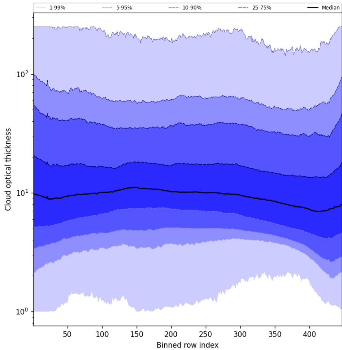
Figure 57: Along track statistics of “Cloud optical thickness” for 2025-04-24 to 2025-04-26
