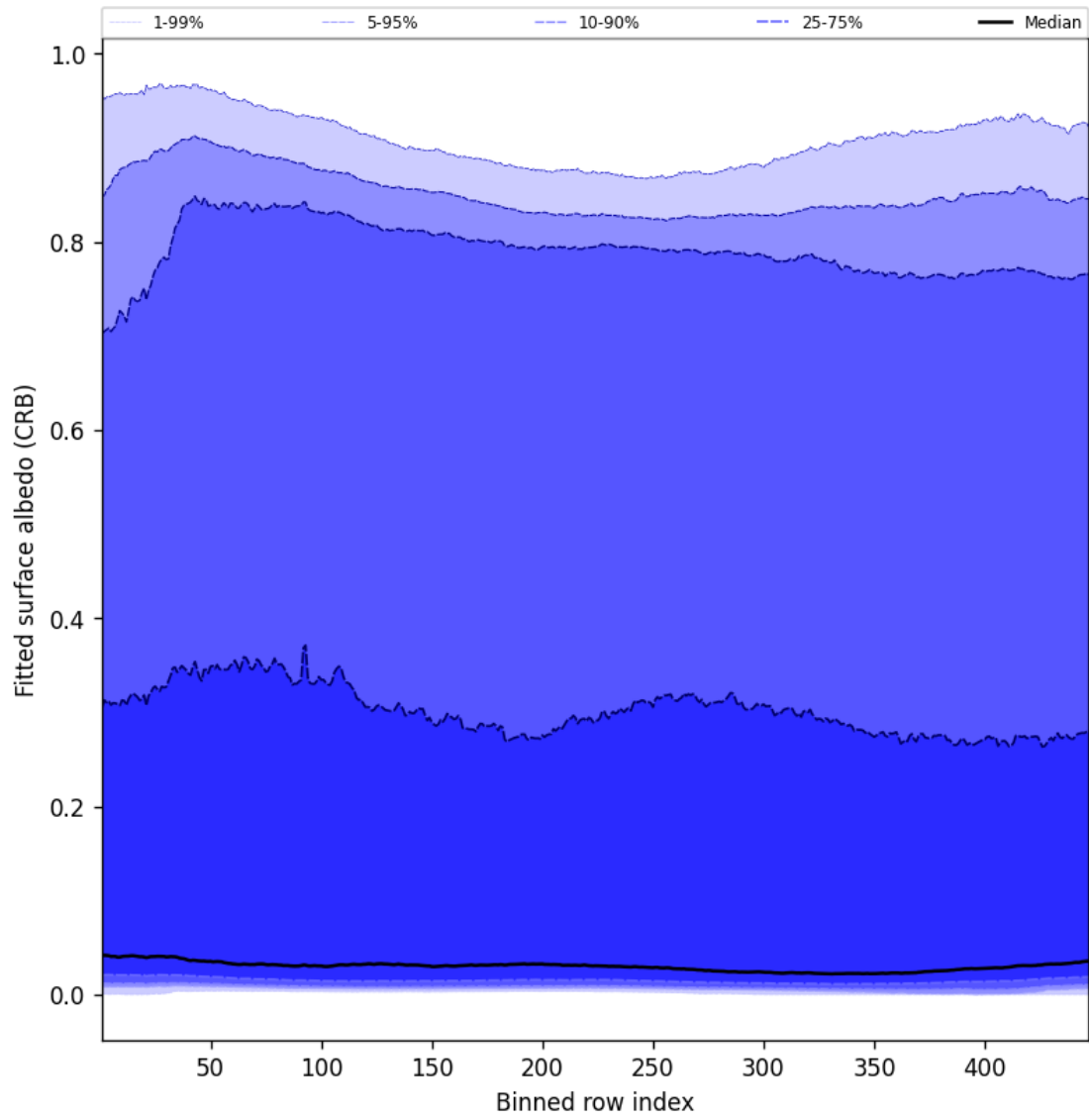
Figure 62: Along track statistics of “Fitted surface albedo (CRB)” for 2025-04-24 to 2025-04-26
