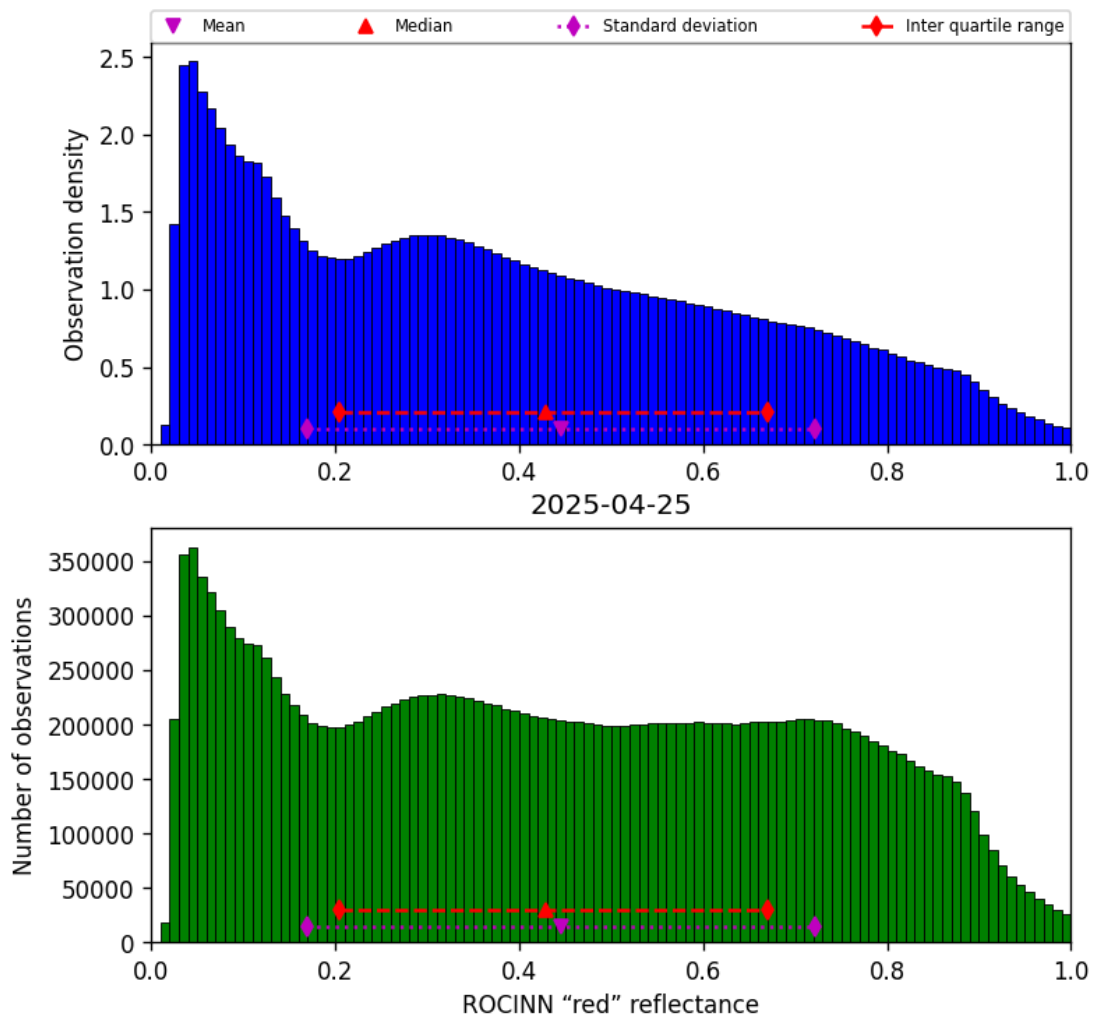
Figure 53: Histogram of “ROCINN “red” reflectance” for 2025-04-24 to 2025-04-26
