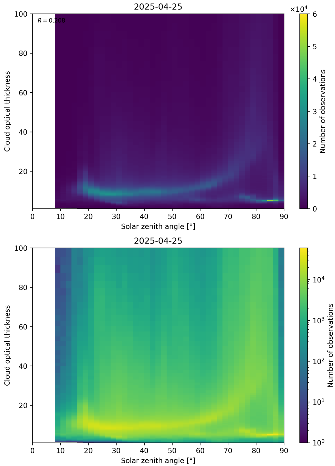
Figure 103: Scatter density plot of “Solar zenith angle” against “Cloud optical thickness” for 2025-04-24 to 2025-04-26.
