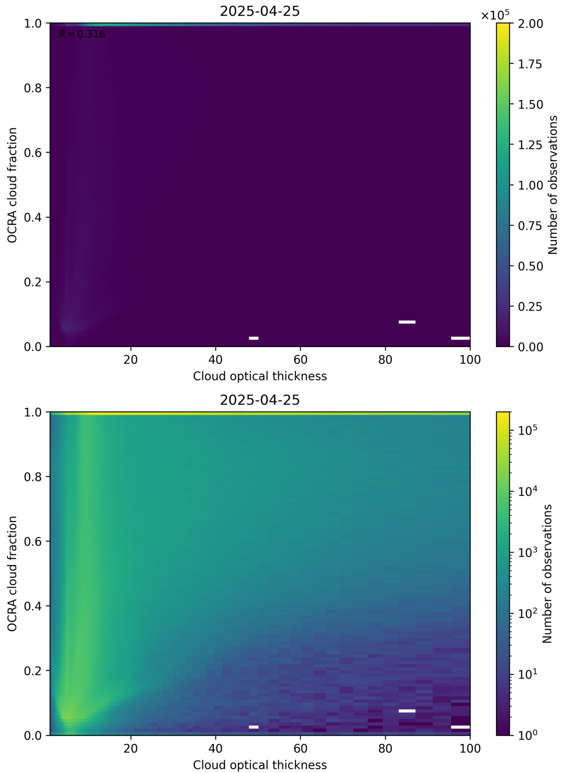
Figure 83: Scatter density plot of “Cloud optical thickness” against “OCRA cloud fraction” for 2025-04-24 to 2025-04-26.
