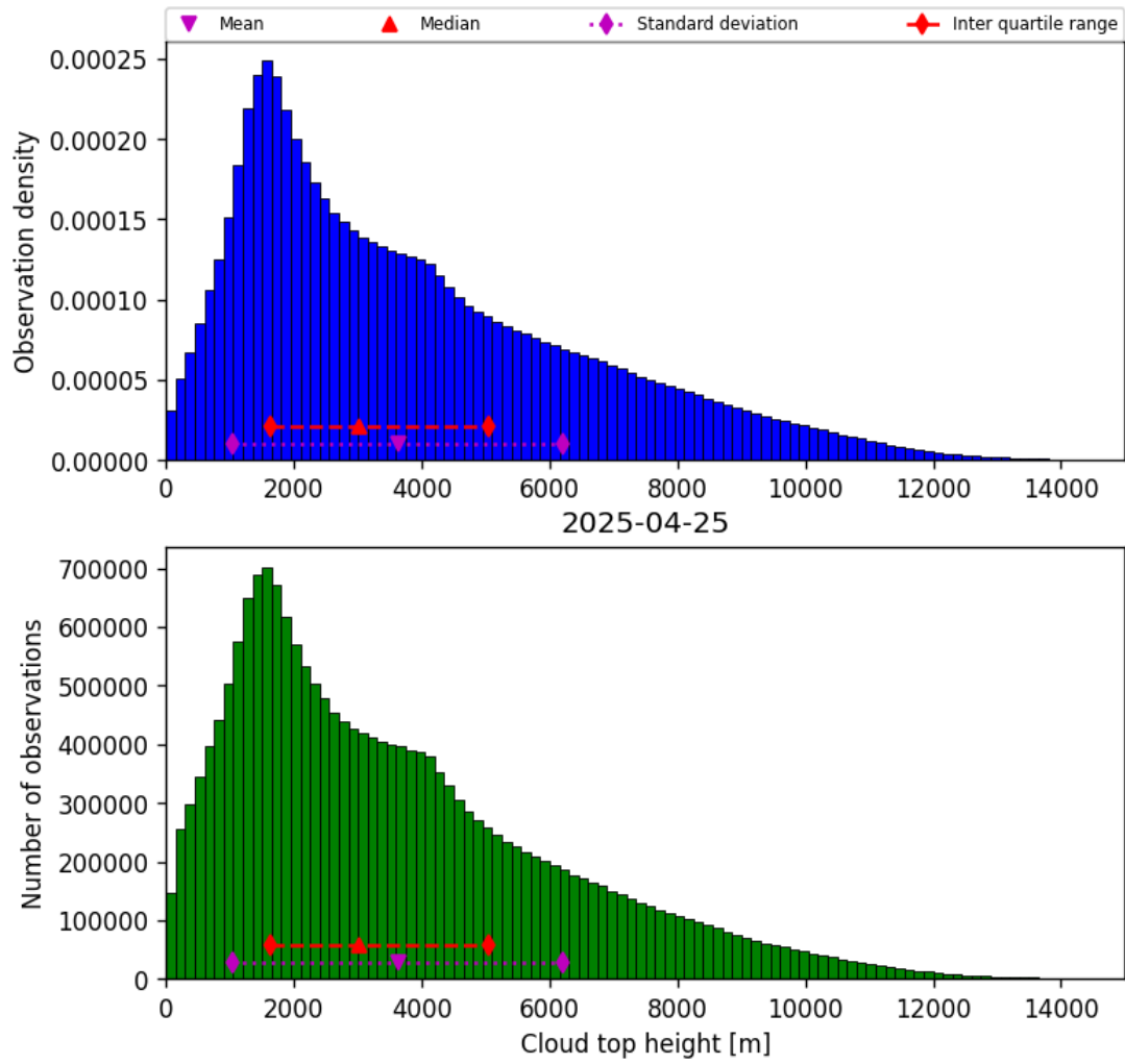
Figure 40: Histogram of “Cloud top height” for 2025-04-24 to 2025-04-26
