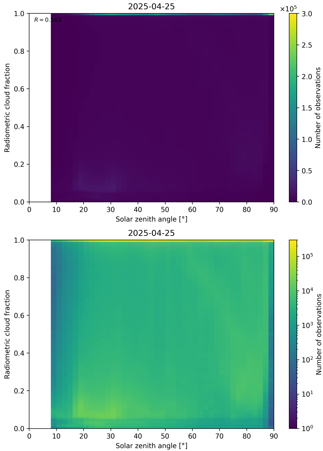
Figure 99: Scatter density plot of “Solar zenith angle” against “Radiometric cloud fraction” for 2025-04-24 to 2025-04-26.
