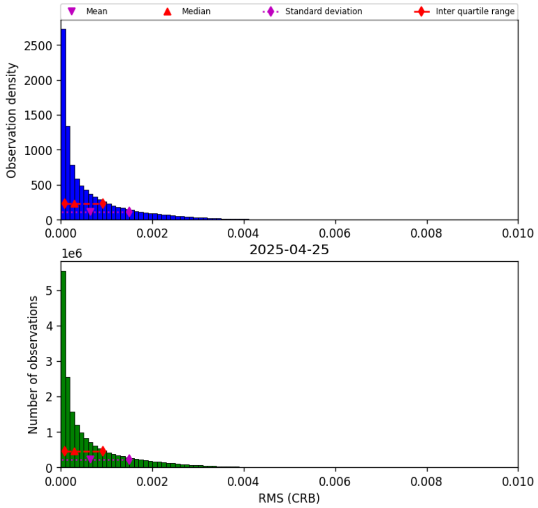
Figure 48: Histogram of “RMS (CRB)” for 2025-04-24 to 2025-04-26
