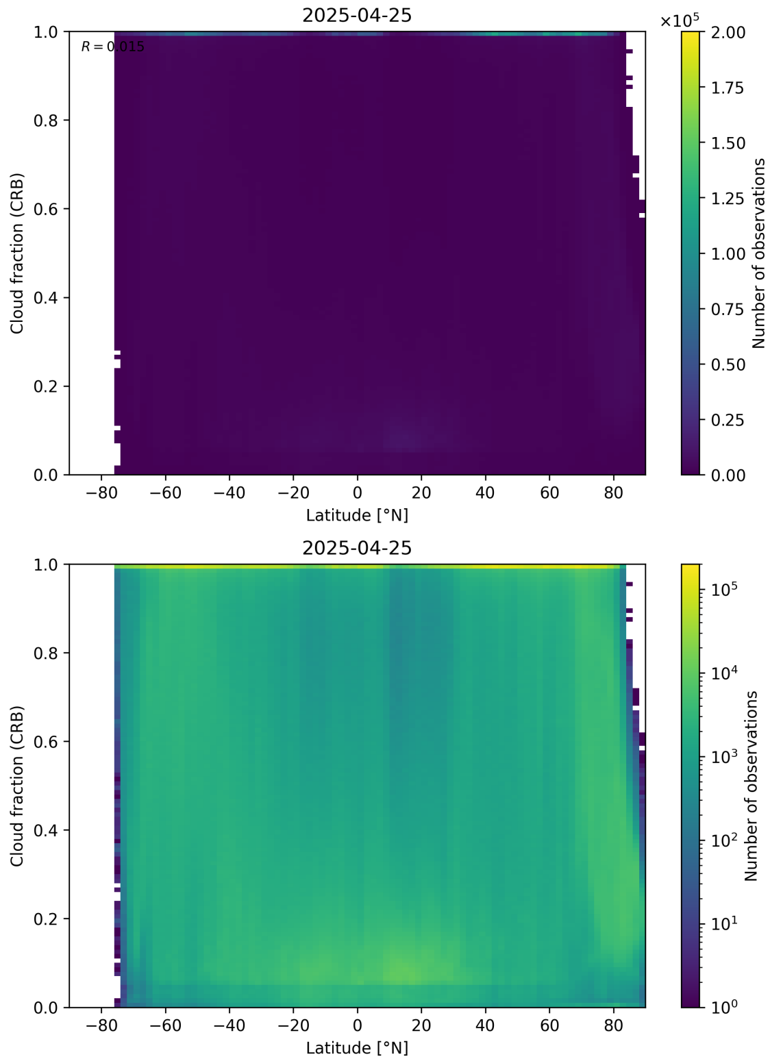
Figure 94: Scatter density plot of “Latitude” against “Cloud fraction (CRB)” for 2025-04-24 to 2025-04-26.
