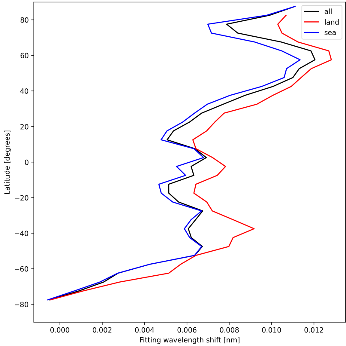
Figure 33: Zonal average of “Fitting wavelength shift” for 2025-04-24 to 2025-04-26.
