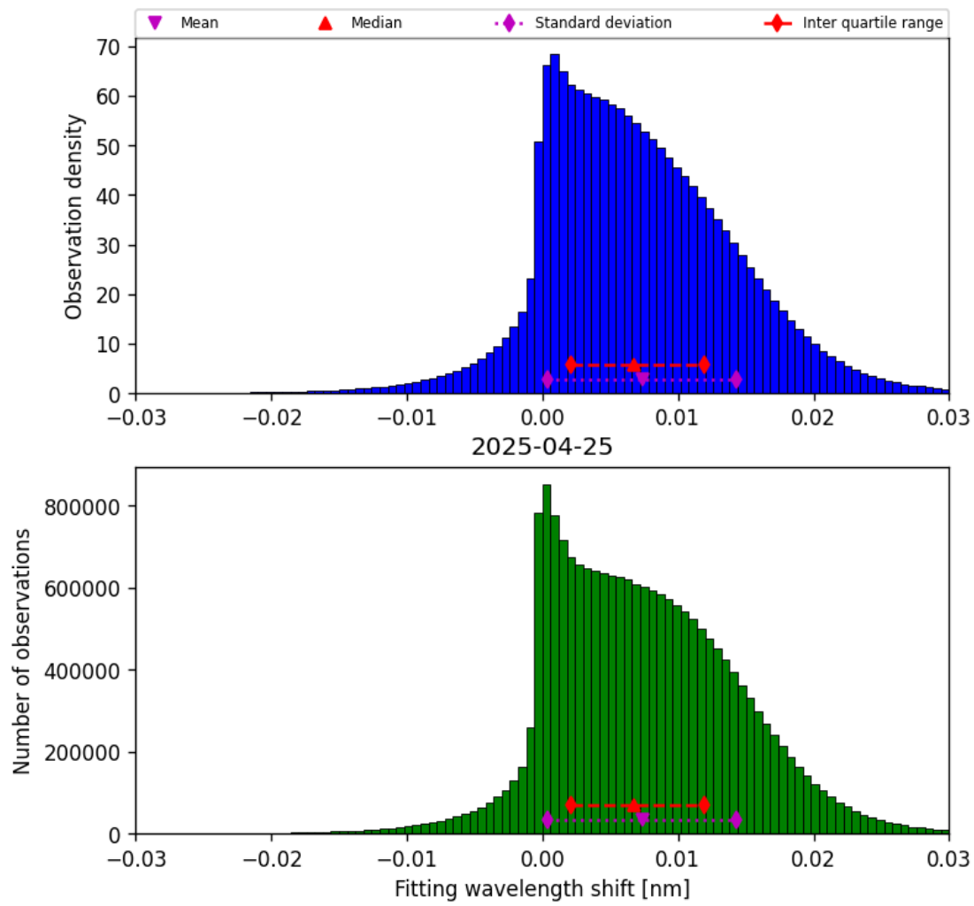
Figure 49: Histogram of “Fitting wavelength shift” for 2025-04-24 to 2025-04-26
