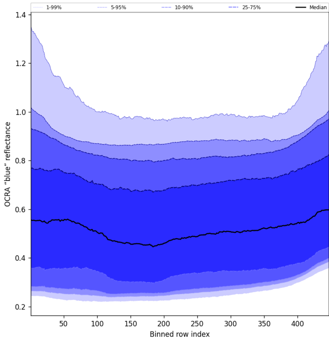
Figure 67: Along track statistics of “OCRA “blue” reflectance” for 2025-04-24 to 2025-04-26
