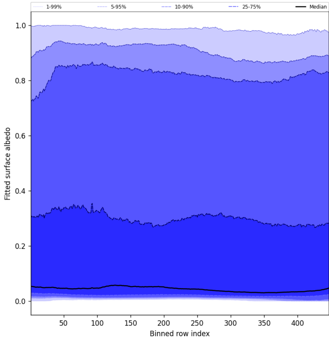
Figure 61: Along track statistics of “Fitted surface albedo” for 2025-04-24 to 2025-04-26
