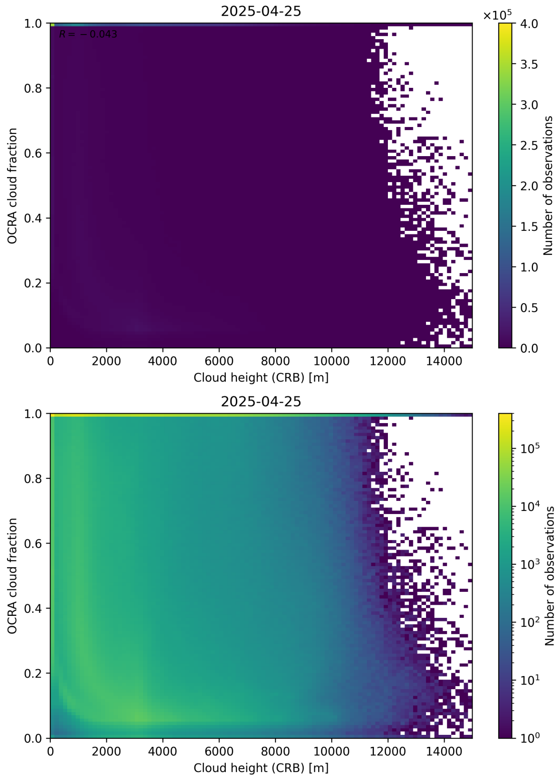
Figure 81: Scatter density plot of “Cloud height (CRB)” against “OCRA cloud fraction” for 2025-04-24 to 2025-04-26.
