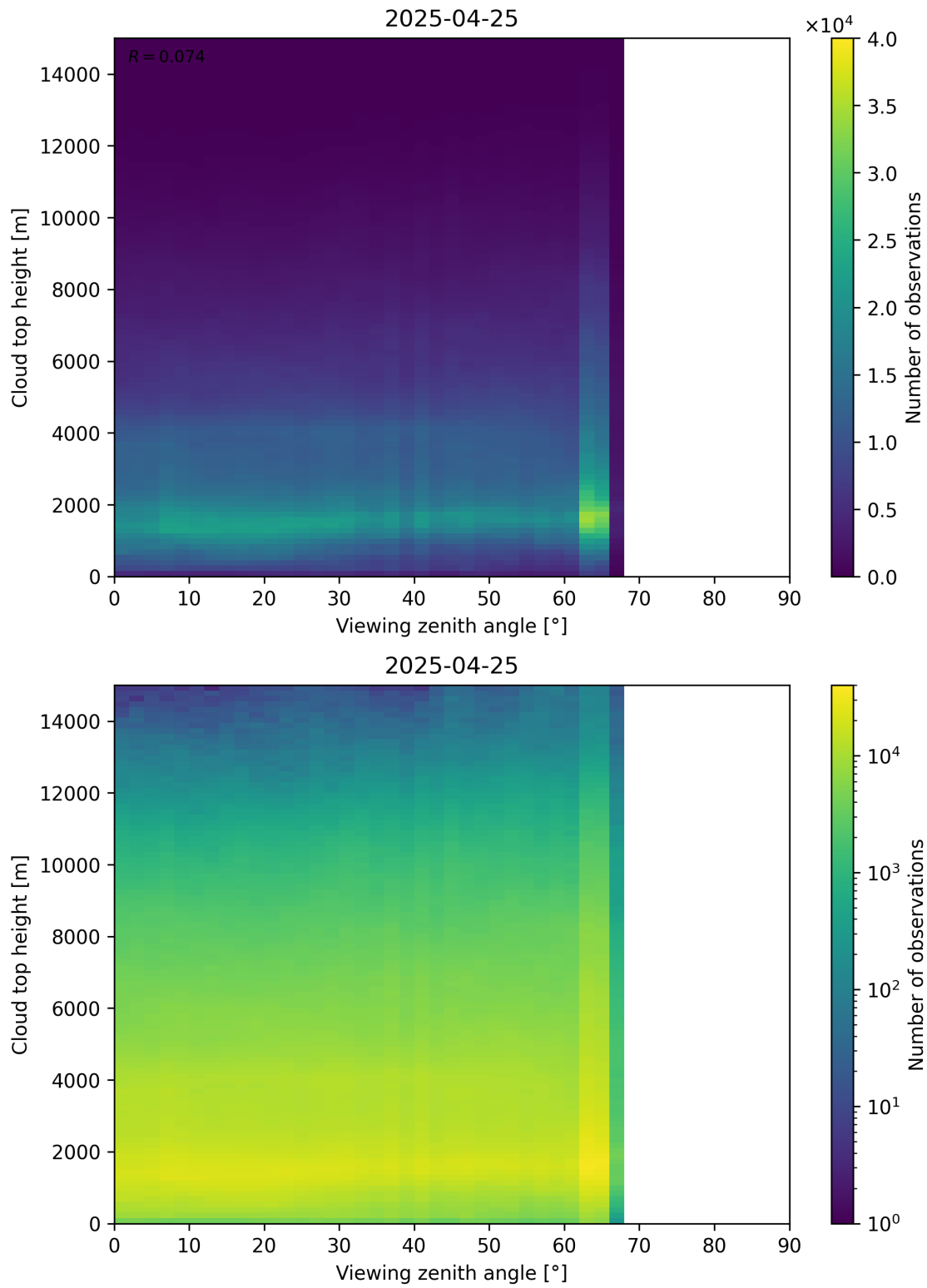
Figure 112: Scatter density plot of “Viewing zenith angle” against “Cloud top height” for 2025-04-24 to 2025-04-26.
