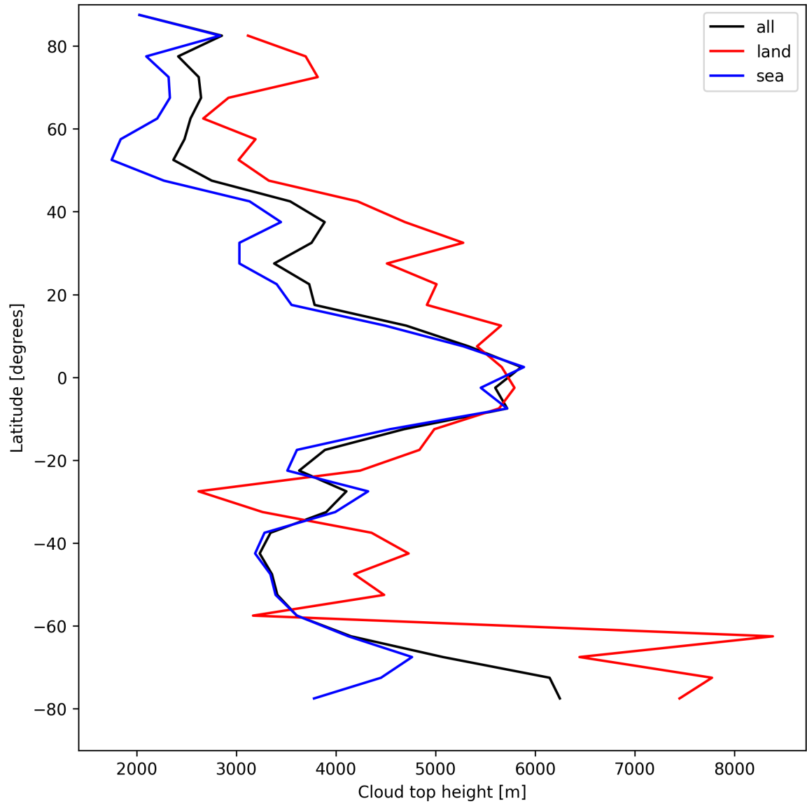
Figure 24: Zonal average of “Cloud top height” for 2025-04-24 to 2025-04-26.
