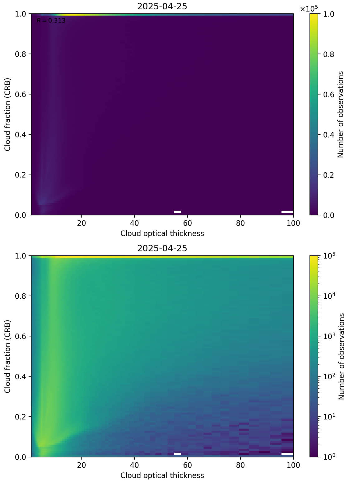
Figure 84: Scatter density plot of “Cloud optical thickness” against “Cloud fraction (CRB)” for 2025-04-24 to 2025-04-26.
