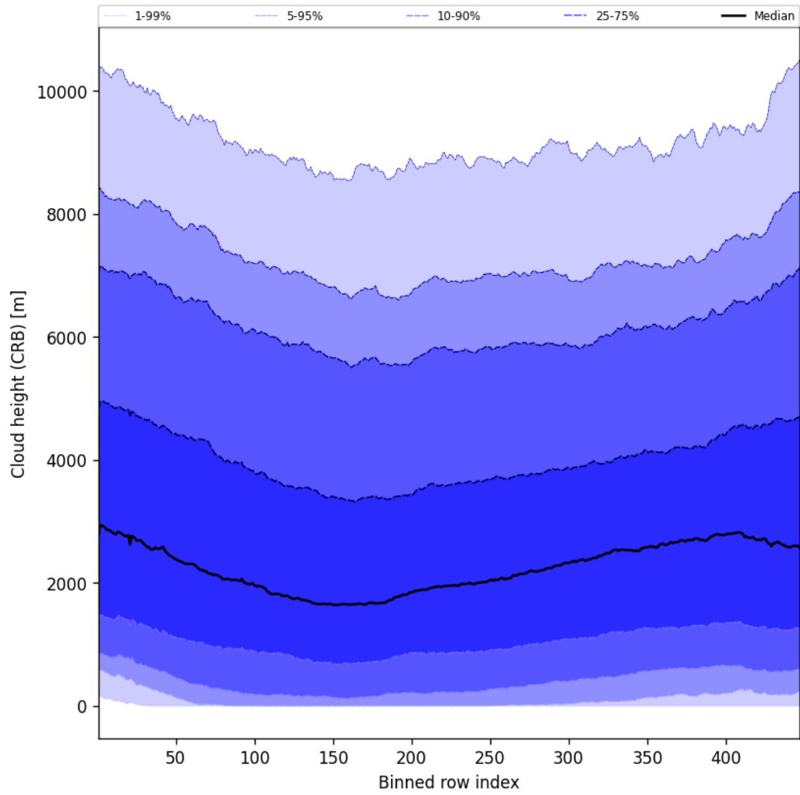
Figure 59: Along track statistics of “Cloud height (CRB)” for 2025-04-24 to 2025-04-26
