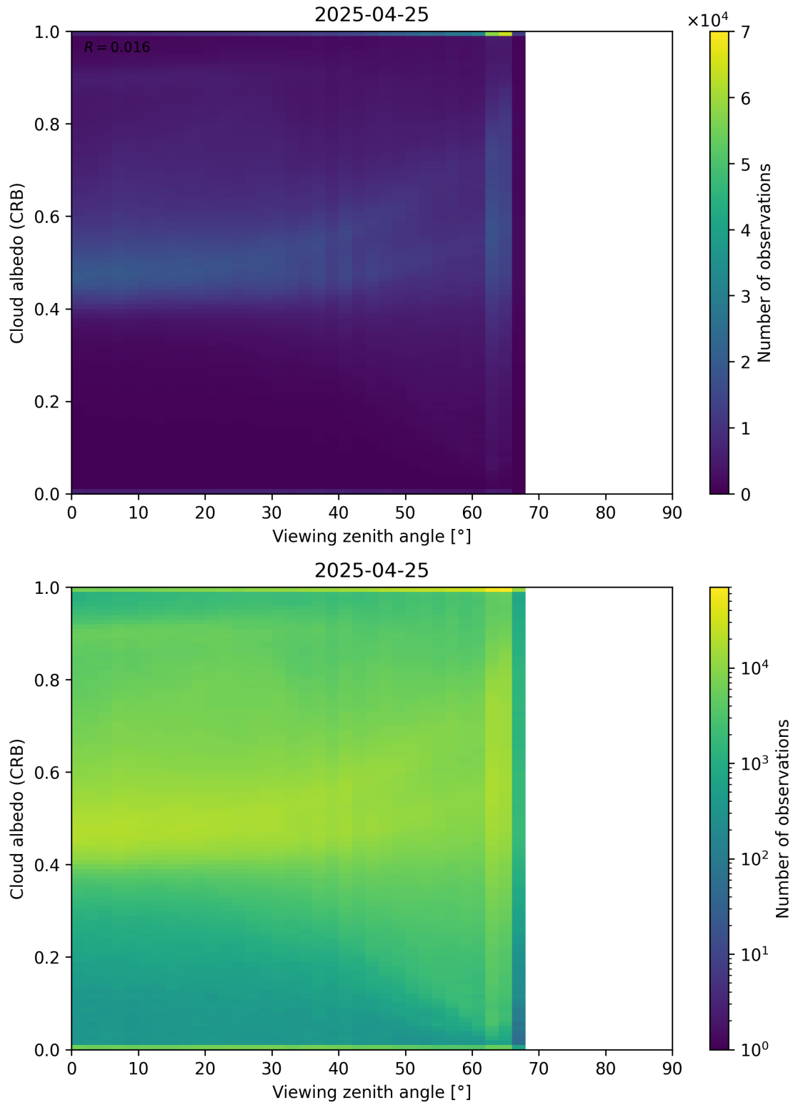
Figure 106: Scatter density plot of “Viewing zenith angle” against “Cloud albedo (CRB)” for 2025-04-24 to 2025-04-26.
