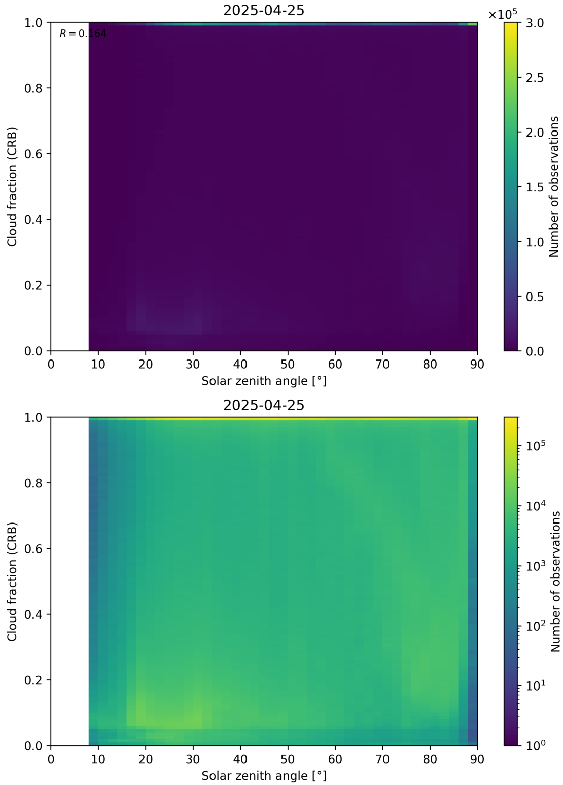
Figure 101: Scatter density plot of “Solar zenith angle” against “Cloud fraction (CRB)” for 2025-04-24 to 2025-04-26.
