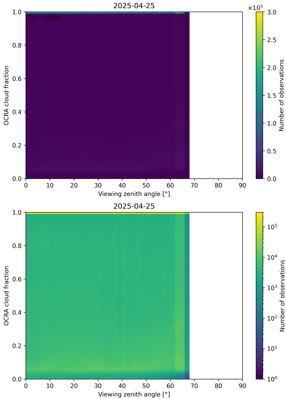
Figure 108: Scatter density plot of “Viewing zenith angle” against “OCRA cloud fraction” for 2025-04-24 to 2025-04-26.
