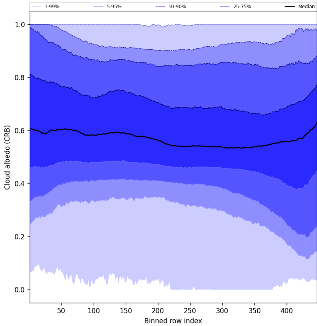
Figure 60: Along track statistics of “Cloud albedo (CRB)” for 2025-04-24 to 2025-04-26
