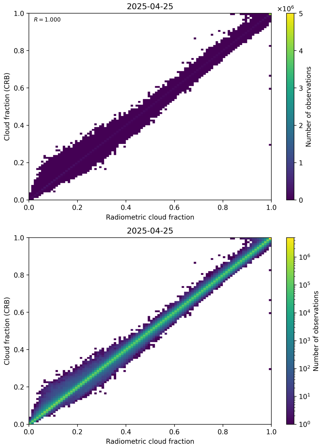
Figure 73: Scatter density plot of “Radiometric cloud fraction” against “Cloud fraction (CRB)” for 2025-04-24 to 2025-04-26.
