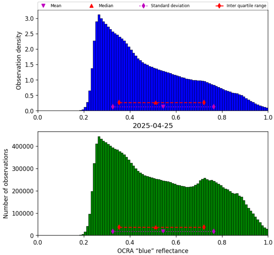
Figure 51: Histogram of “OCRA “blue” reflectance” for 2025-04-24 to 2025-04-26
