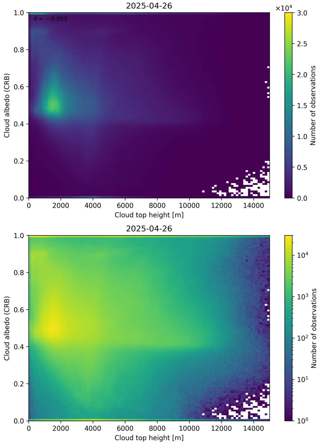
Figure 86: Scatter density plot of “Cloud top height” against “Cloud albedo (CRB)” for 2025-04-25 to 2025-04-27.
