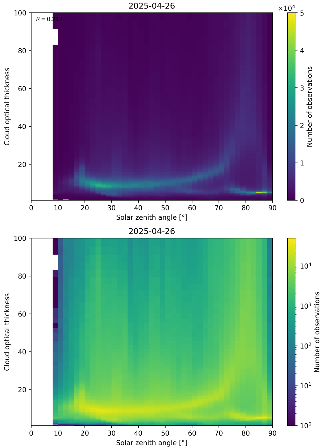
Figure 103: Scatter density plot of “Solar zenith angle” against “Cloud optical thickness” for 2025-04-25 to 2025-04-27.
