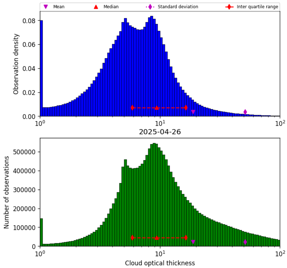
Figure 41: Histogram of “Cloud optical thickness” for 2025-04-25 to 2025-04-27
