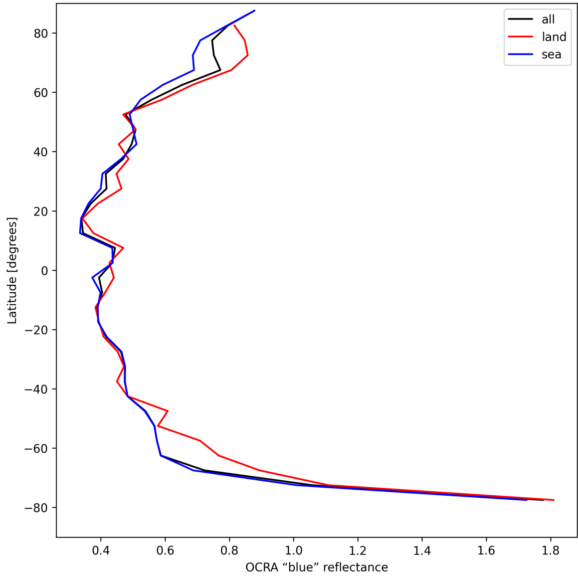
Figure 35: Zonal average of “OCRA “blue” reflectance” for 2025-04-25 to 2025-04-27.
