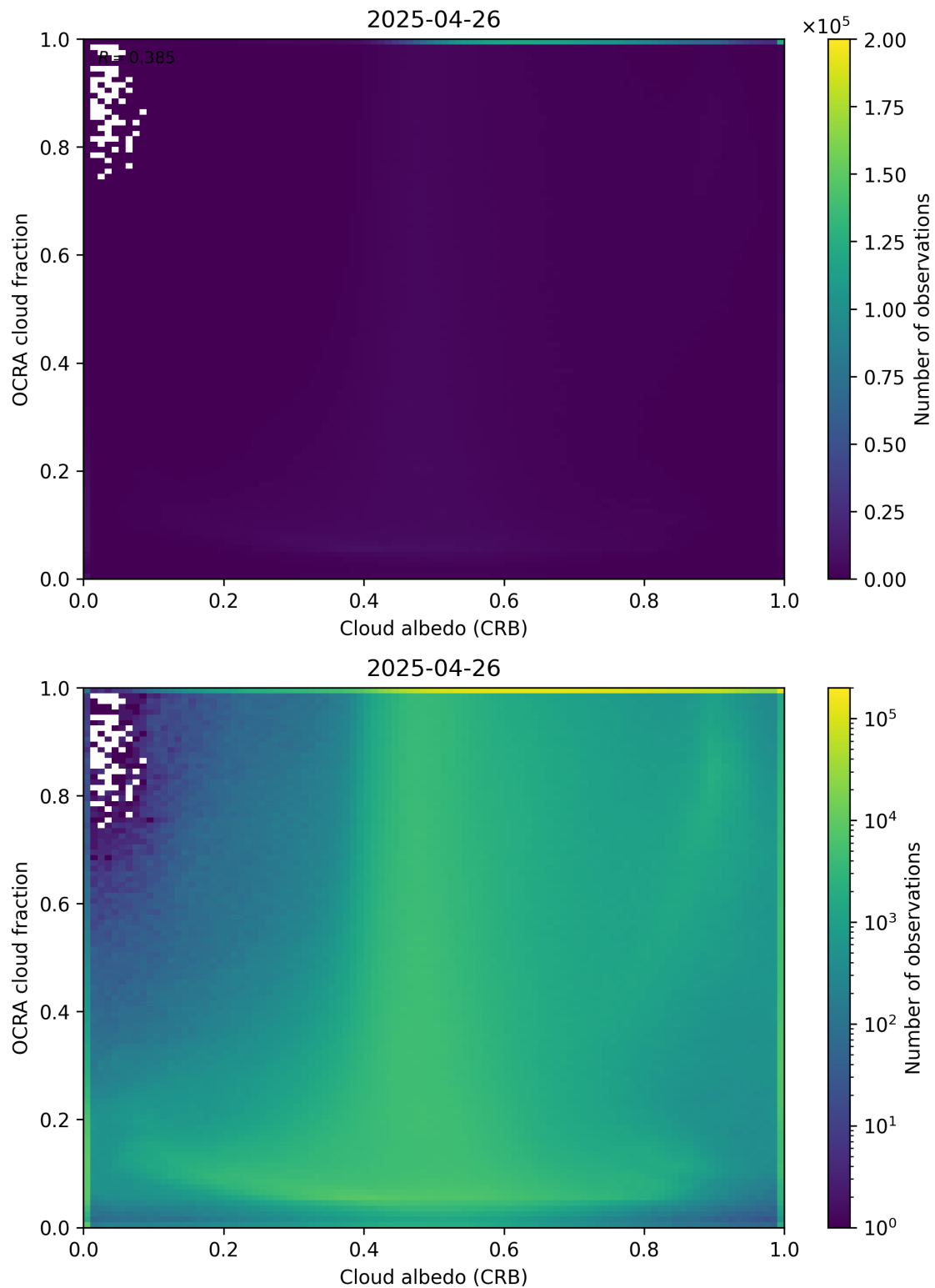
Figure 70: Scatter density plot of “Cloud albedo (CRB)” against “OCRA cloud fraction” for 2025-04-25 to 2025-04-27.
