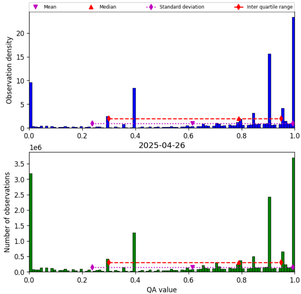
Figure 38: Histogram of “QA value” for 2025-04-25 to 2025-04-27
