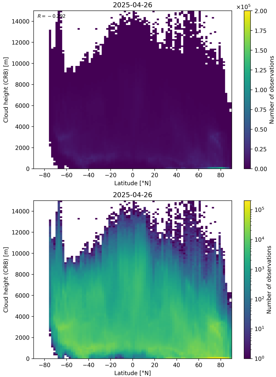
Figure 95: Scatter density plot of “Latitude” against “Cloud height (CRB)” for 2025-04-25 to 2025-04-27.
