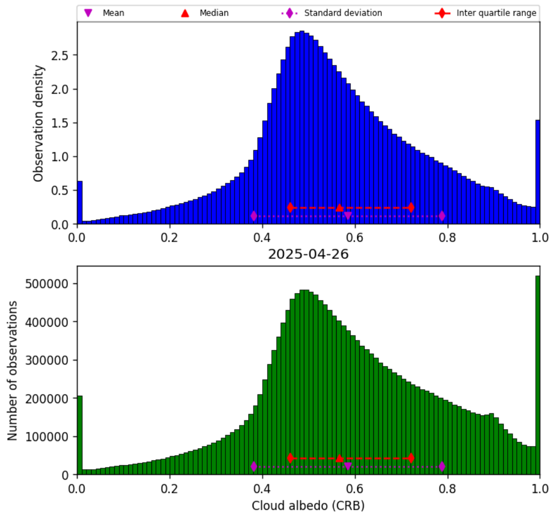
Figure 44: Histogram of “Cloud albedo (CRB)” for 2025-04-25 to 2025-04-27
