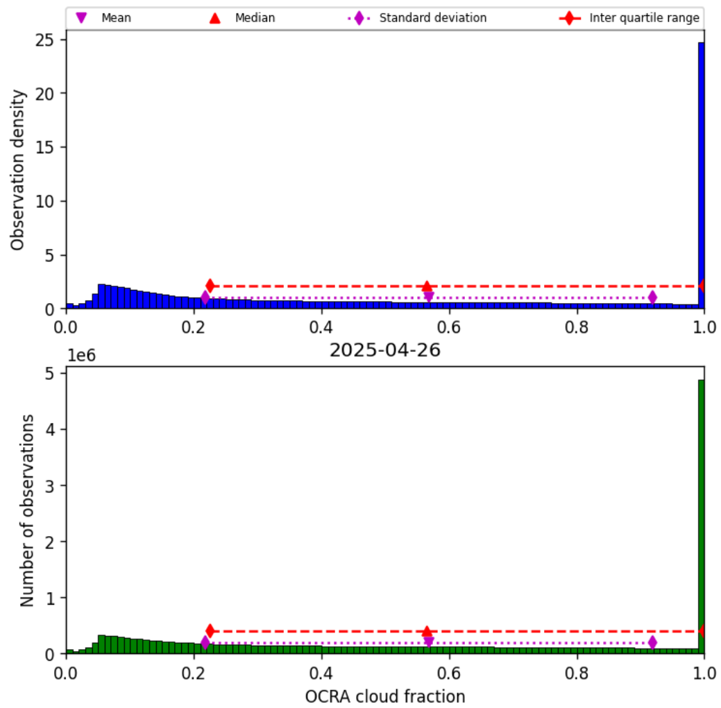
Figure 50: Histogram of “OCRA cloud fraction” for 2025-04-25 to 2025-04-27
