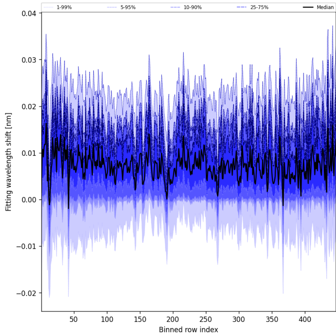
Figure 65: Along track statistics of “Fitting wavelength shift” for 2025-04-25 to 2025-04-27
