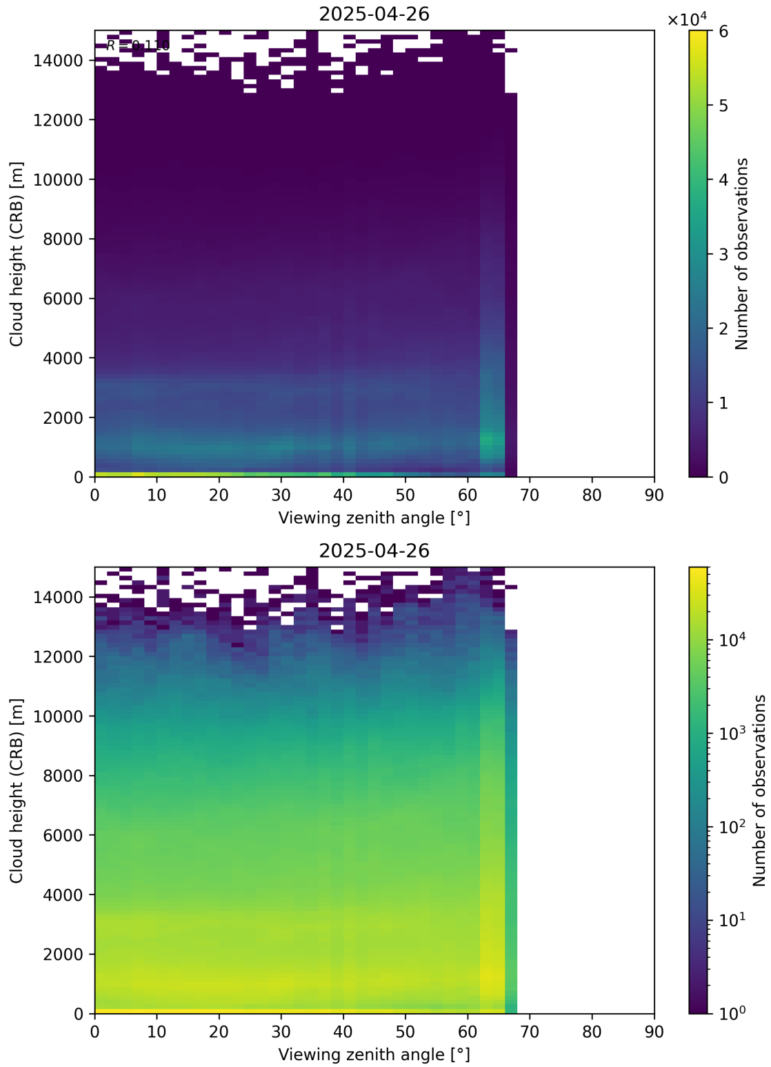
Figure 110: Scatter density plot of “Viewing zenith angle” against “Cloud height (CRB)” for 2025-04-25 to 2025-04-27.
