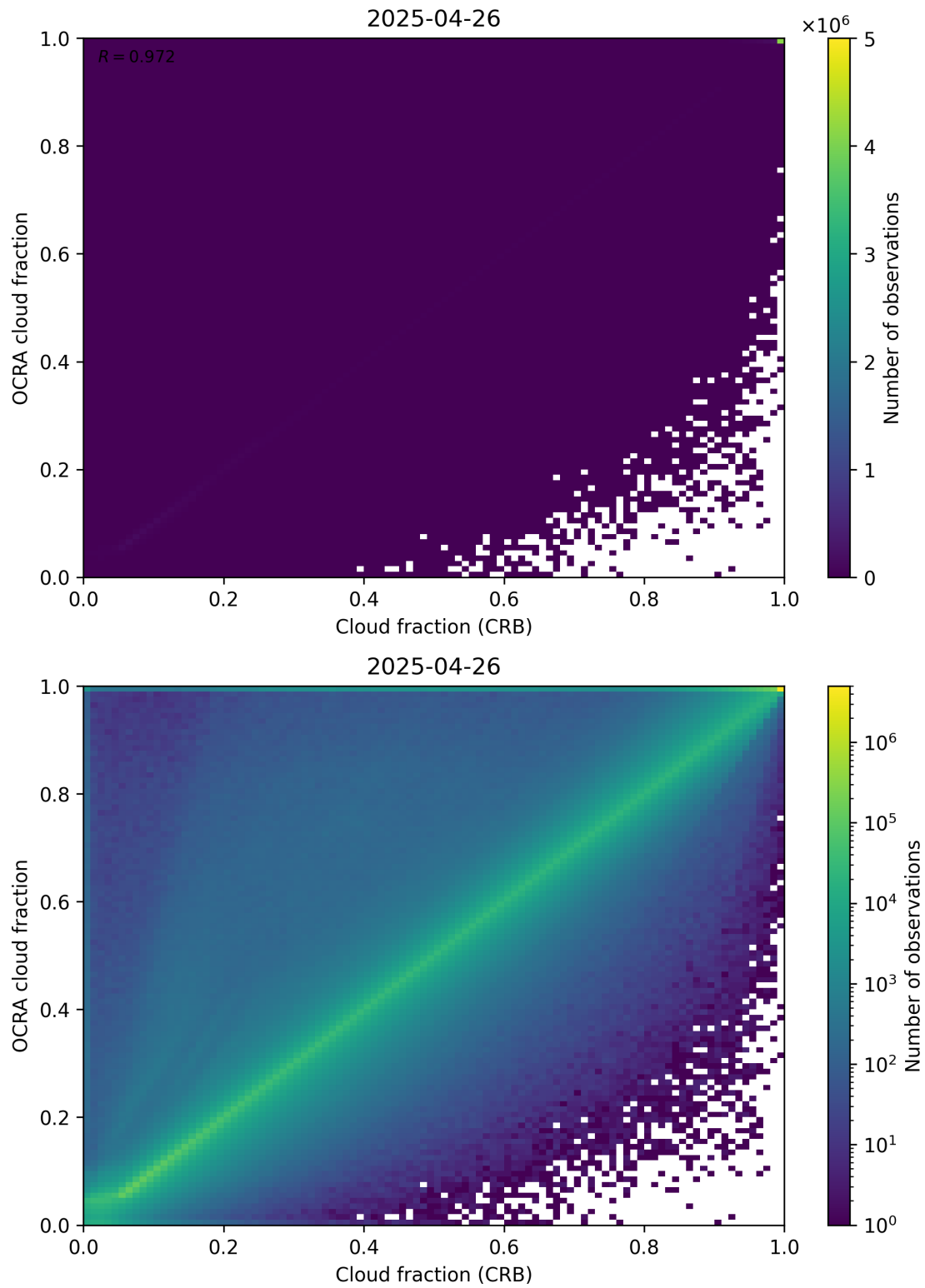
Figure 78: Scatter density plot of “Cloud fraction (CRB)” against “OCRA cloud fraction” for 2025-04-25 to 2025-04-27.
