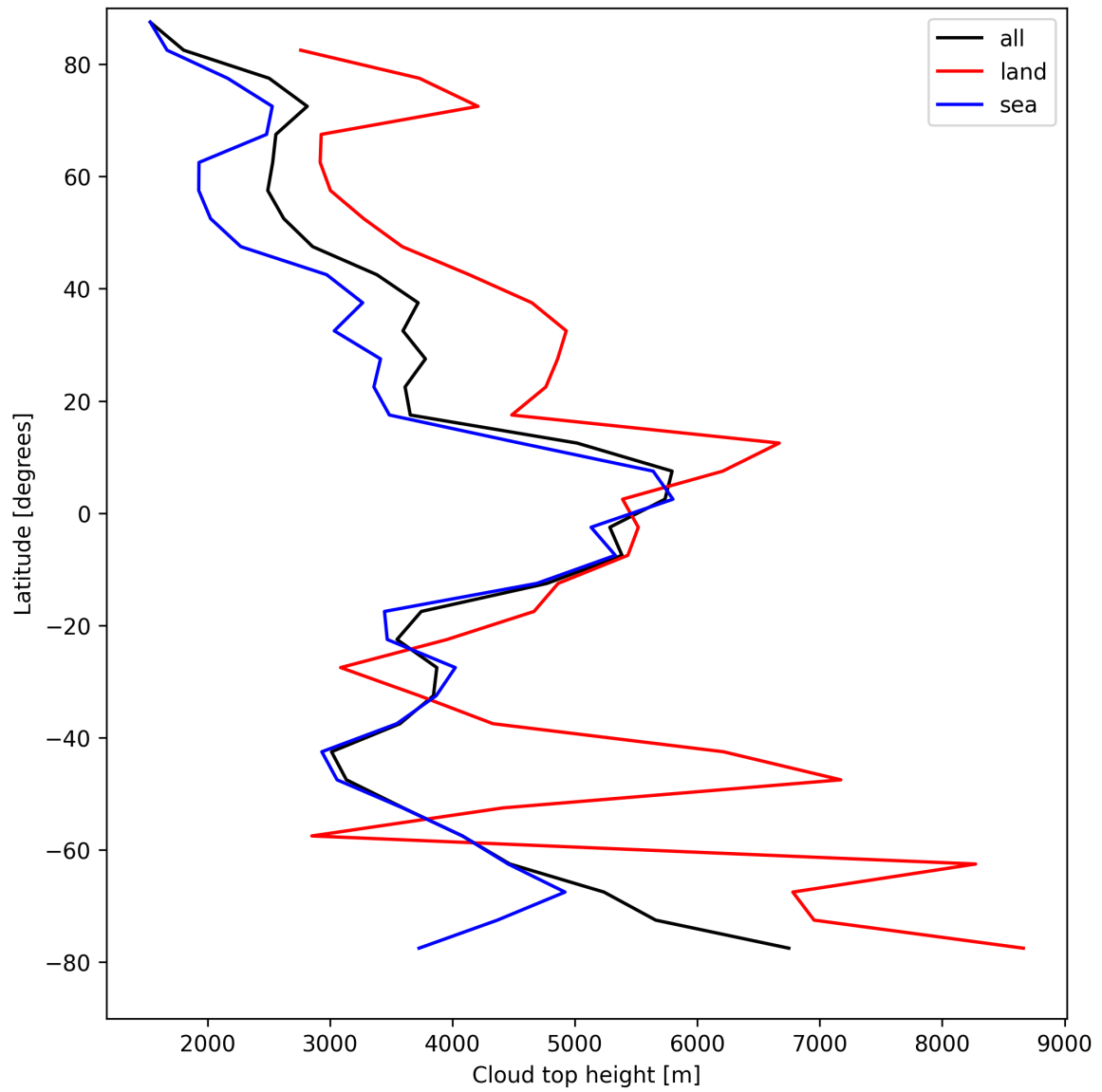
Figure 24: Zonal average of “Cloud top height” for 2025-04-25 to 2025-04-27.
