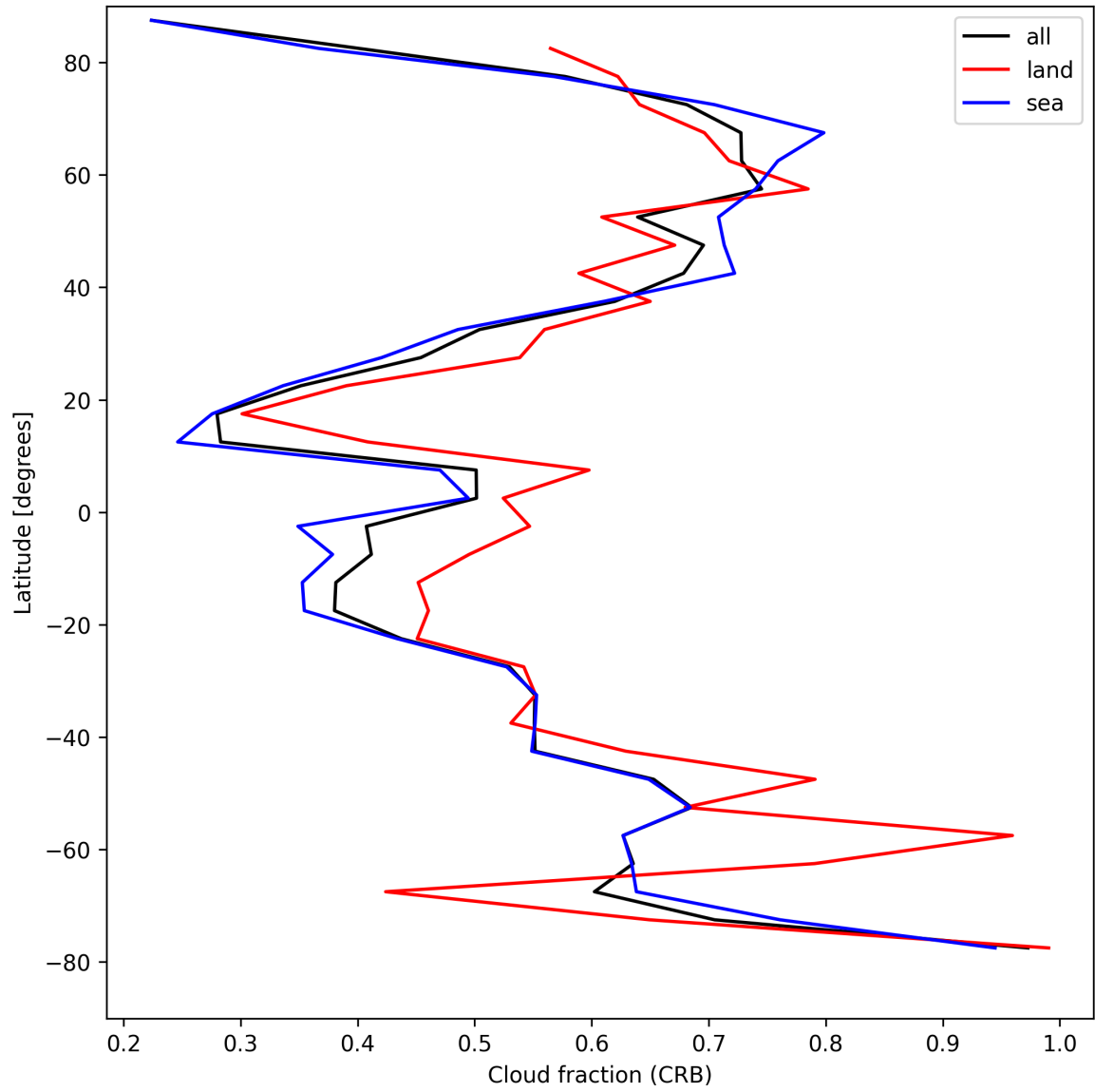
Figure 26: Zonal average of “Cloud fraction (CRB)” for 2025-04-25 to 2025-04-27.
