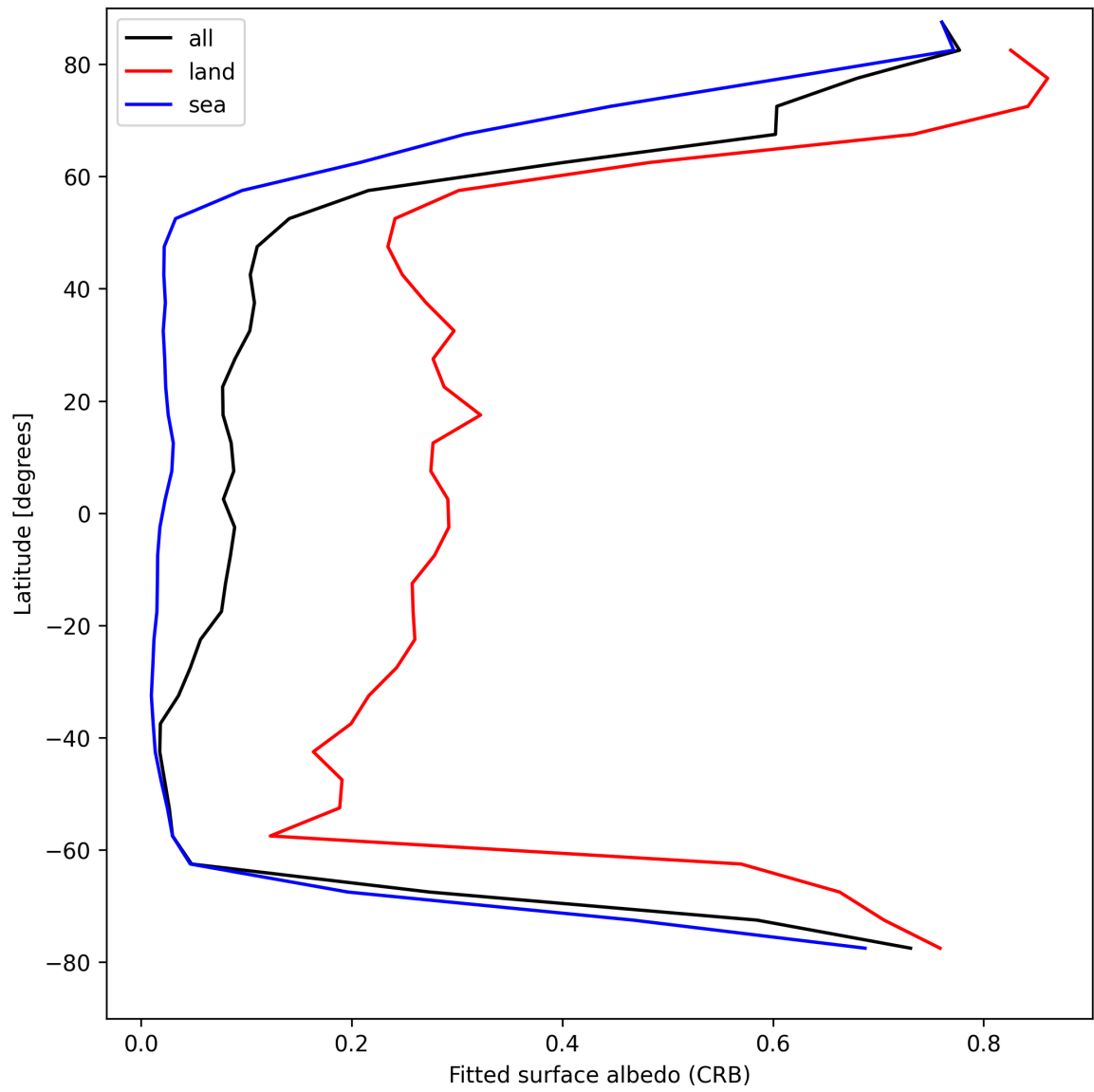
Figure 30: Zonal average of “Fitted surface albedo (CRB)” for 2025-04-25 to 2025-04-27.
