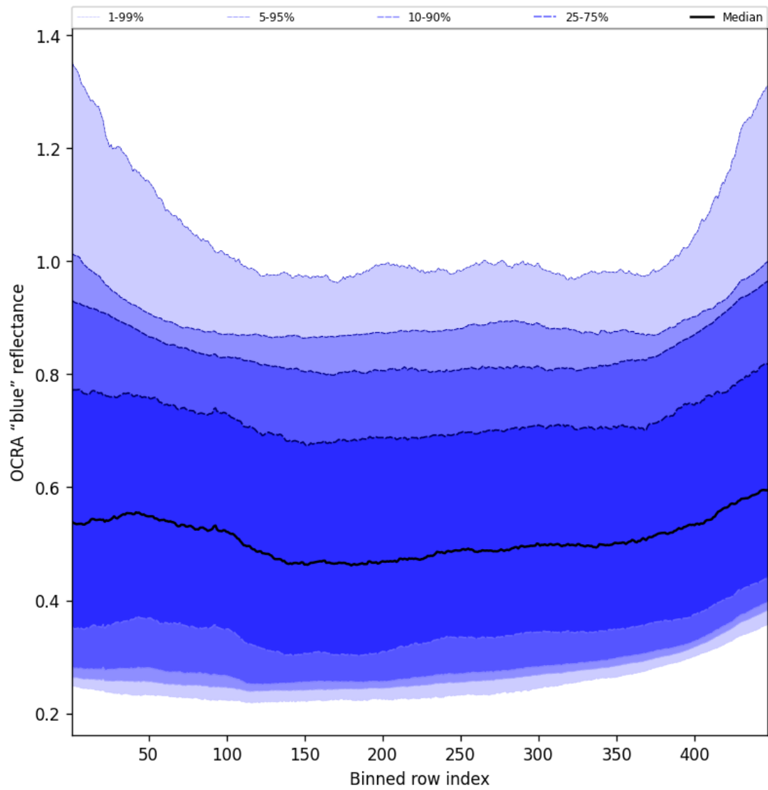
Figure 67: Along track statistics of “OCRA “blue” reflectance” for 2025-04-25 to 2025-04-27
