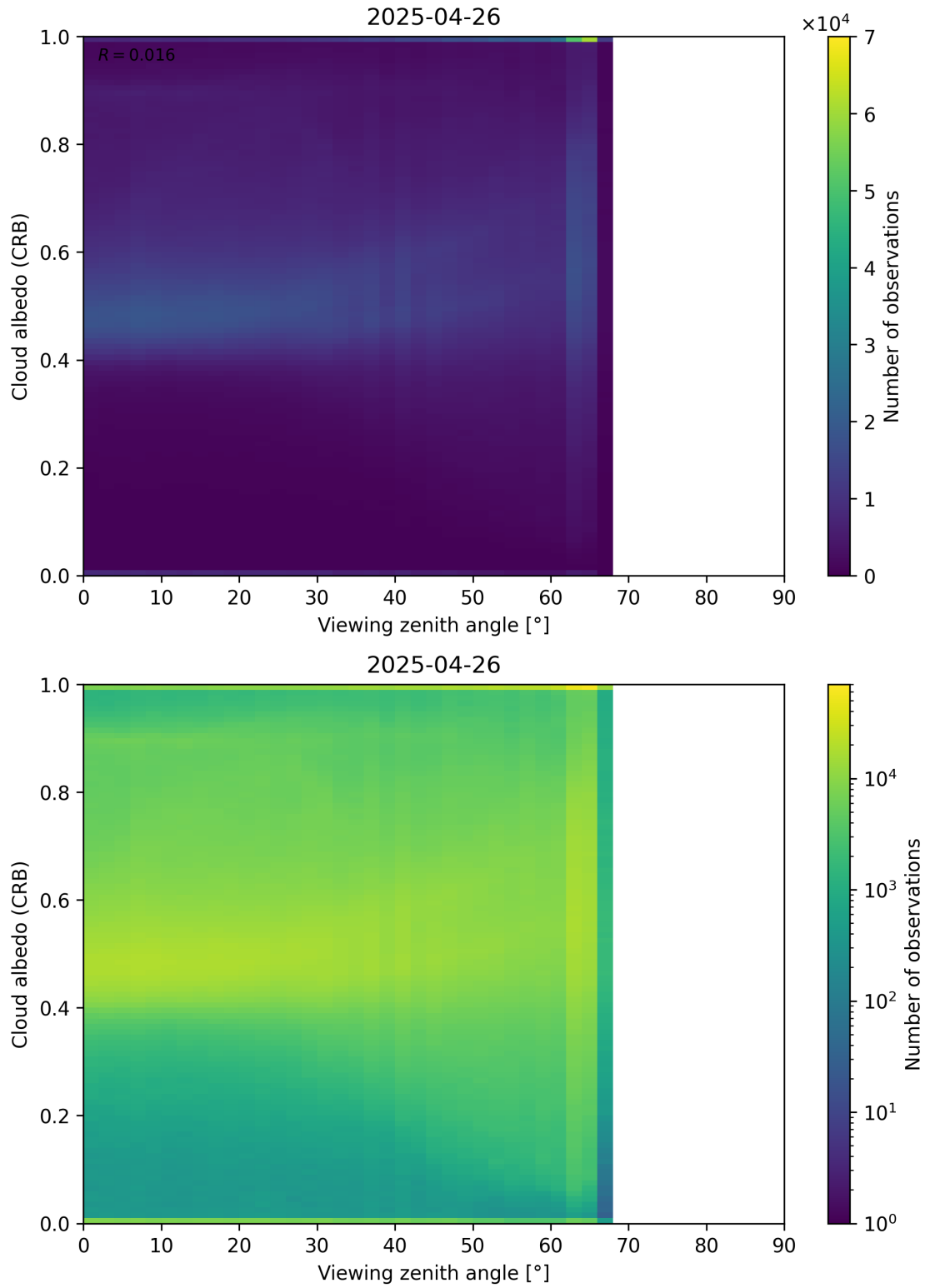
Figure 106: Scatter density plot of “Viewing zenith angle” against “Cloud albedo (CRB)” for 2025-04-25 to 2025-04-27.
