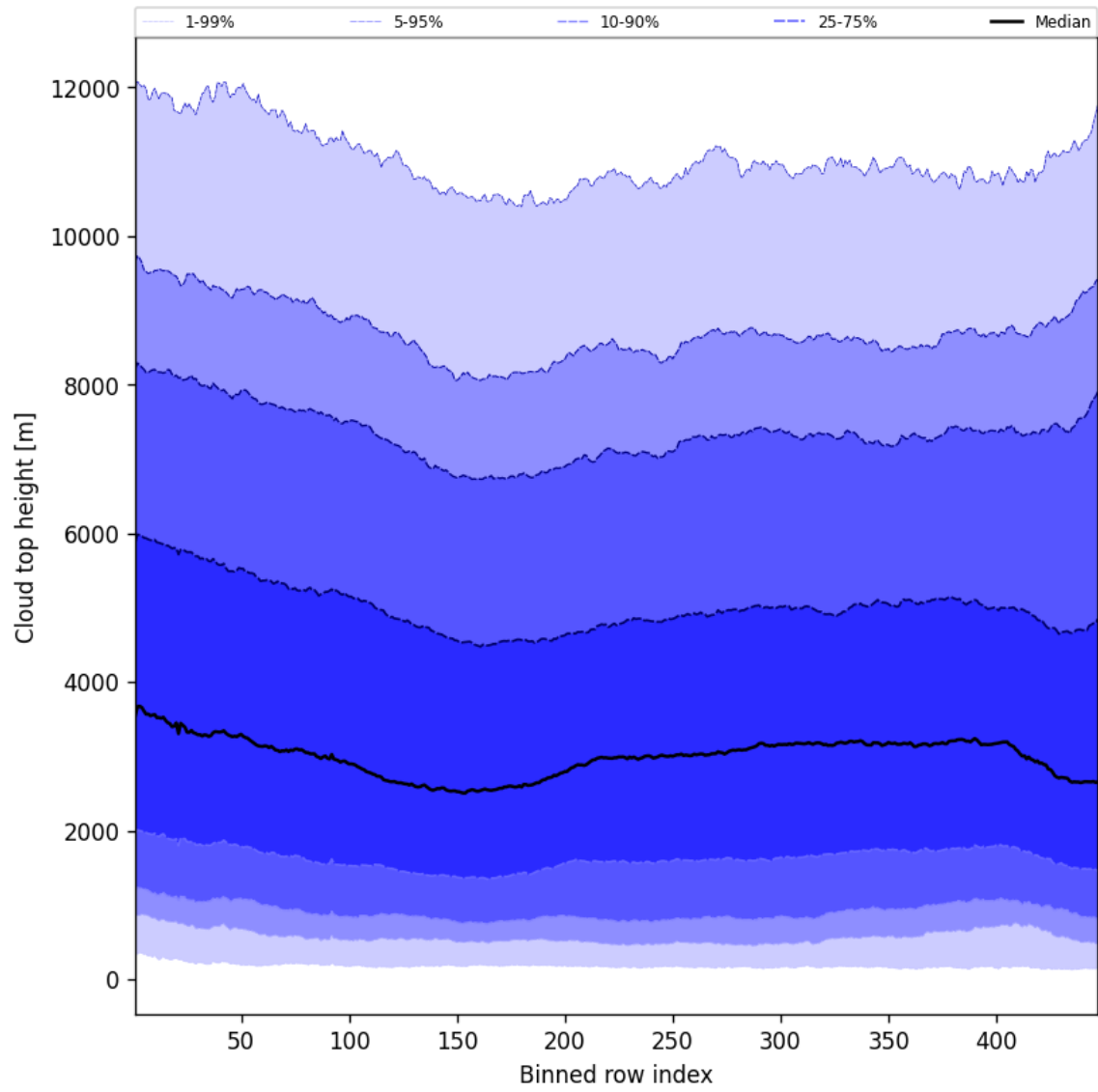
Figure 56: Along track statistics of “Cloud top height” for 2025-04-25 to 2025-04-27
