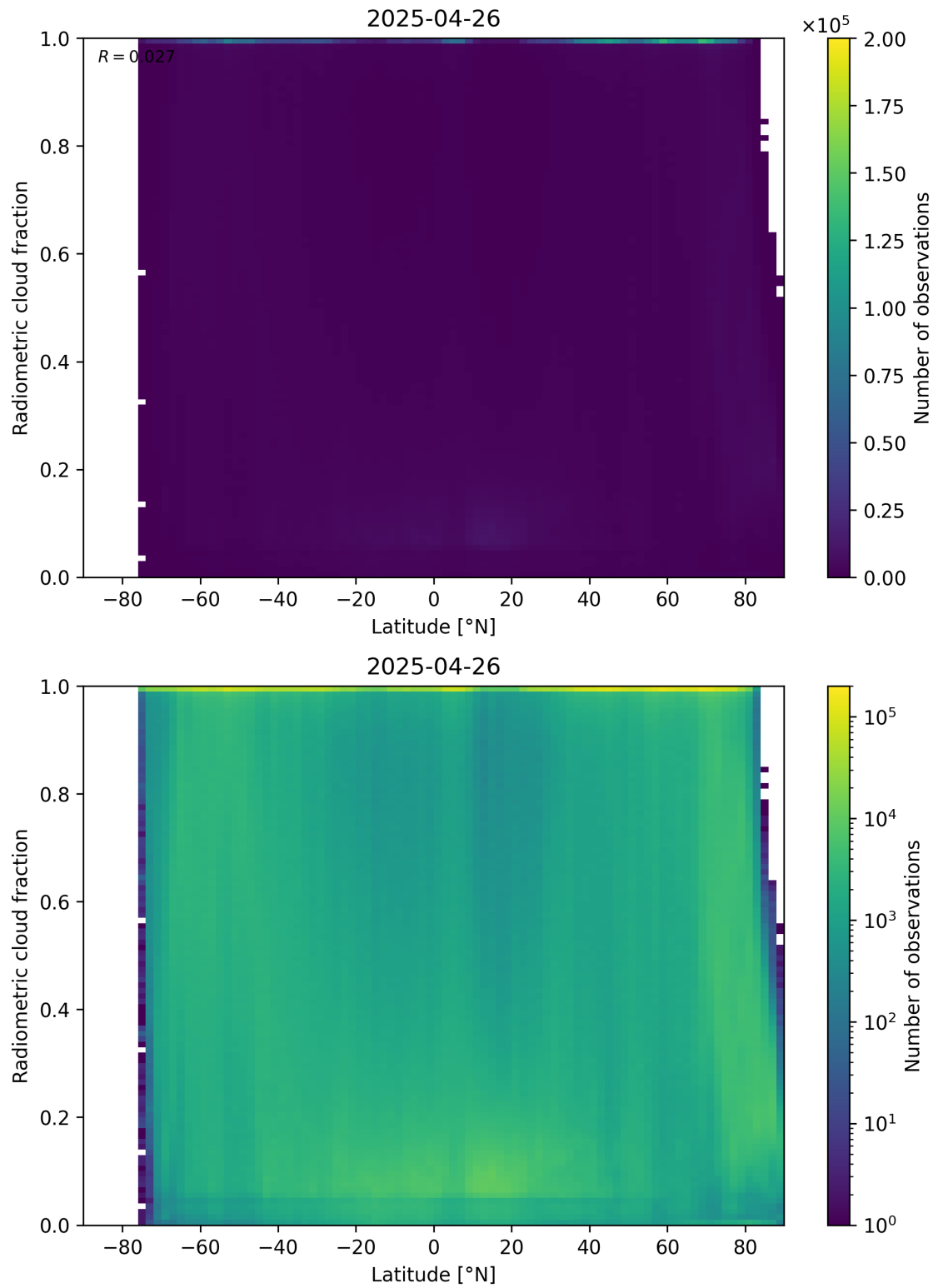
Figure 92: Scatter density plot of “Latitude” against “Radiometric cloud fraction” for 2025-04-25 to 2025-04-27.
