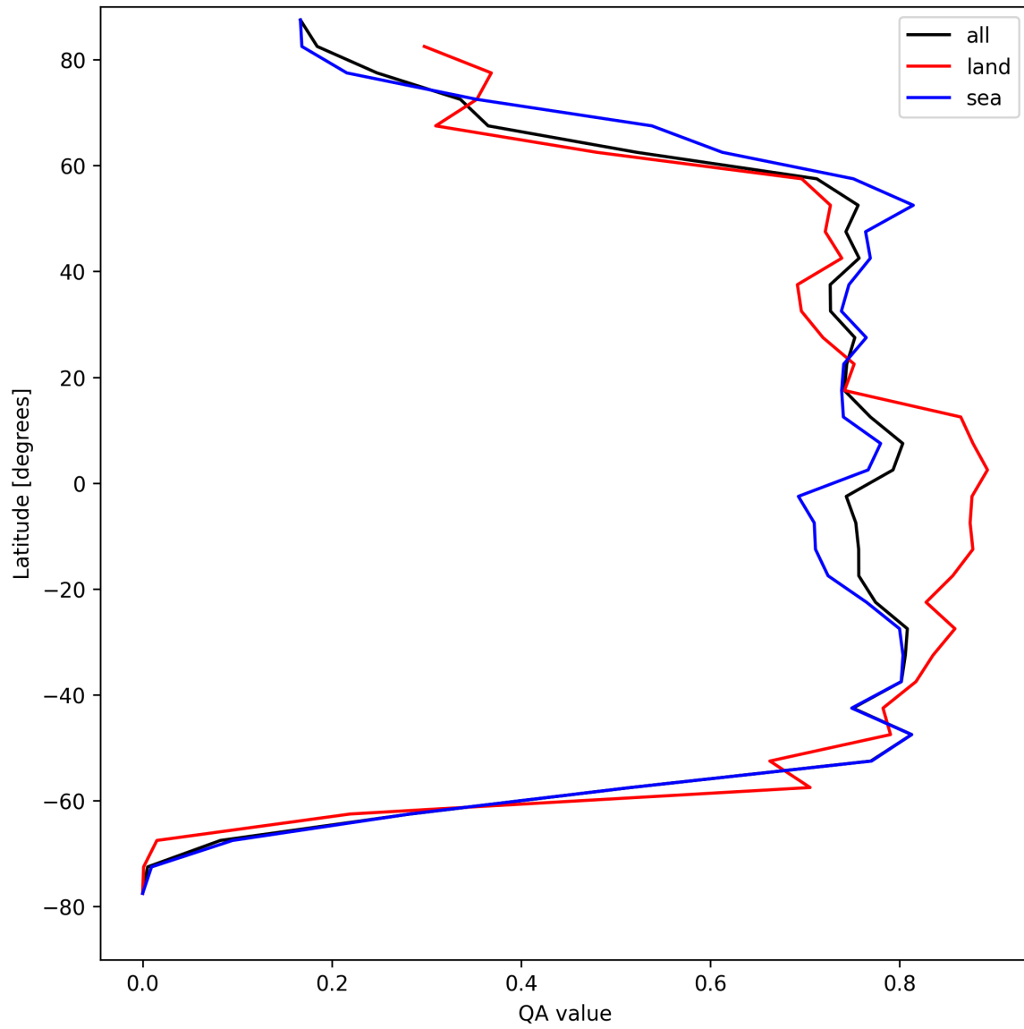
Figure 22: Zonal average of “QA value” for 2025-04-25 to 2025-04-27.
