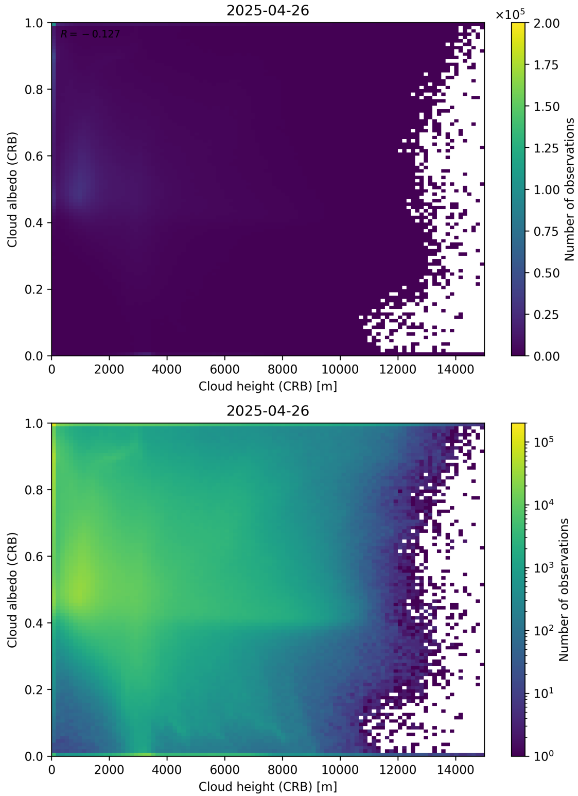
Figure 80: Scatter density plot of “Cloud height (CRB)” against “Cloud albedo (CRB)” for 2025-04-25 to 2025-04-27.
