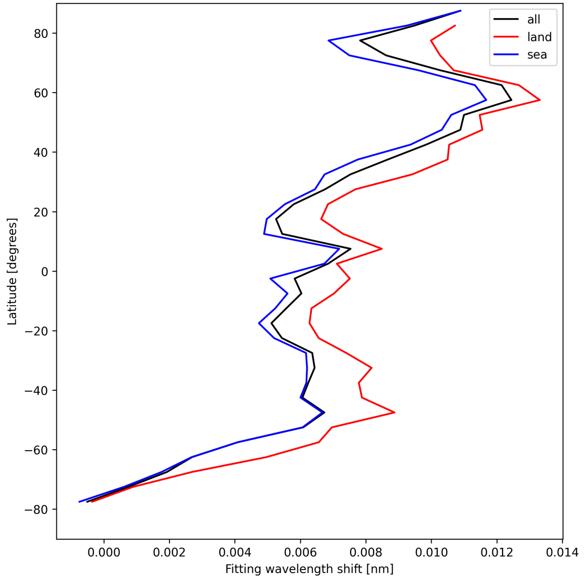
Figure 33: Zonal average of “Fitting wavelength shift” for 2025-04-25 to 2025-04-27.
