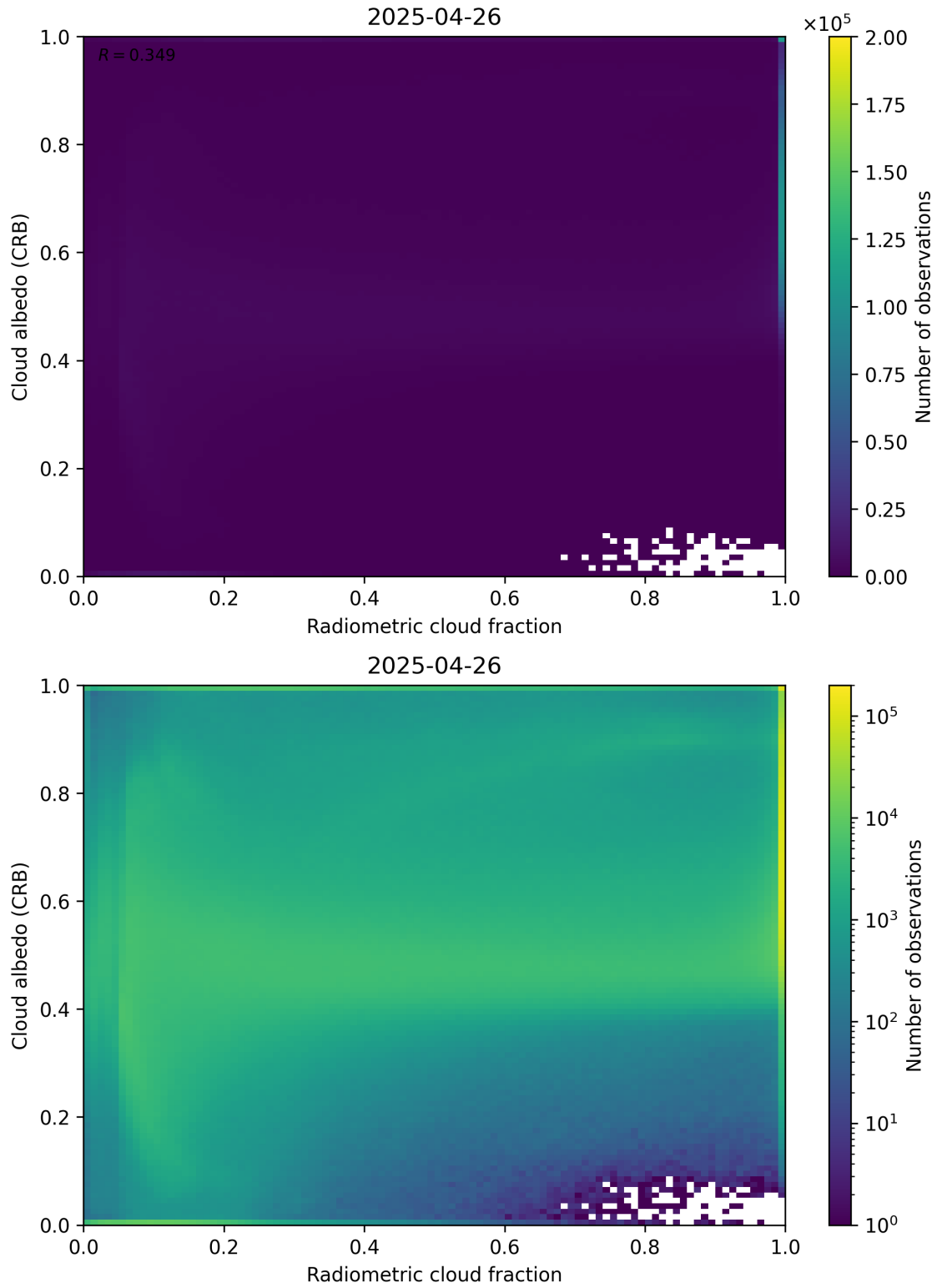
Figure 71: Scatter density plot of “Radiometric cloud fraction” against “Cloud albedo (CRB)” for 2025-04-25 to 2025-04-27.
