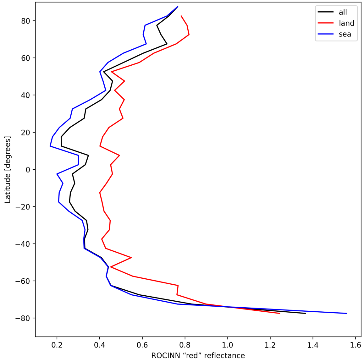
Figure 37: Zonal average of “ROCINN “red” reflectance” for 2025-04-25 to 2025-04-27.
