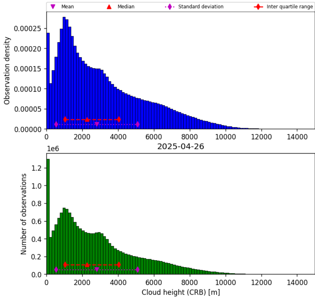
Figure 43: Histogram of “Cloud height (CRB)” for 2025-04-25 to 2025-04-27
