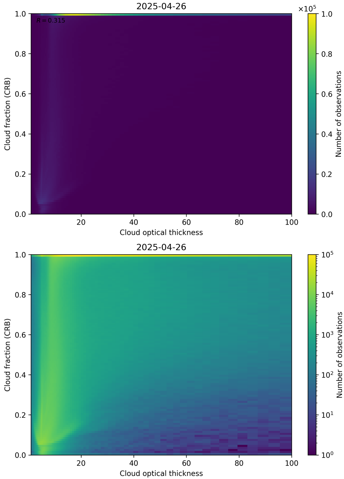
Figure 84: Scatter density plot of “Cloud optical thickness” against “Cloud fraction (CRB)” for 2025-04-25 to 2025-04-27.
