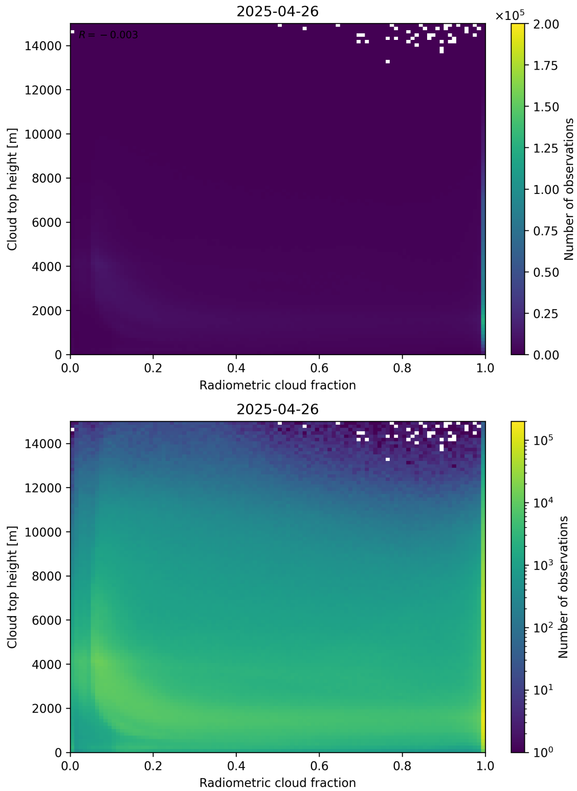
Figure 76: Scatter density plot of “Radiometric cloud fraction” against “Cloud top height” for 2025-04-25 to 2025-04-27.
