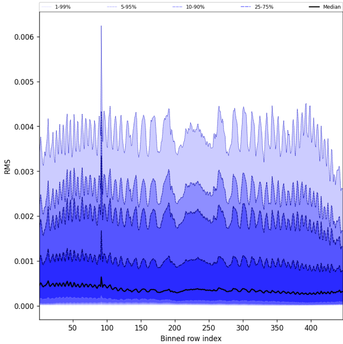
Figure 63: Along track statistics of “RMS” for 2025-04-25 to 2025-04-27
