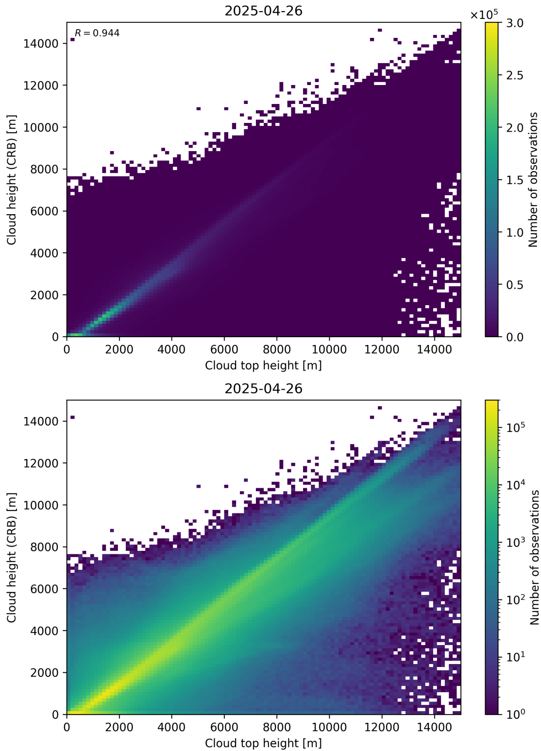
Figure 89: Scatter density plot of “Cloud top height” against “Cloud height (CRB)” for 2025-04-25 to 2025-04-27.
