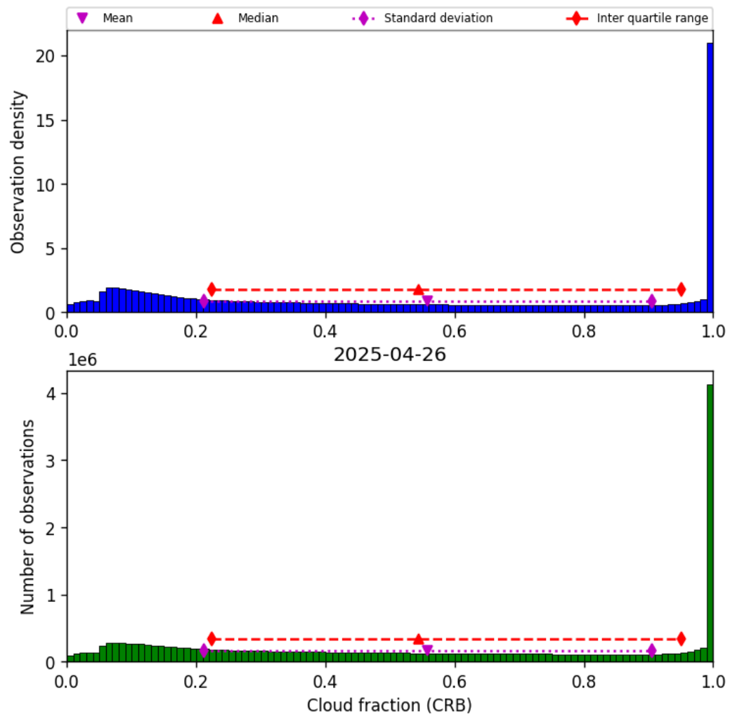
Figure 42: Histogram of “Cloud fraction (CRB)” for 2025-04-25 to 2025-04-27
