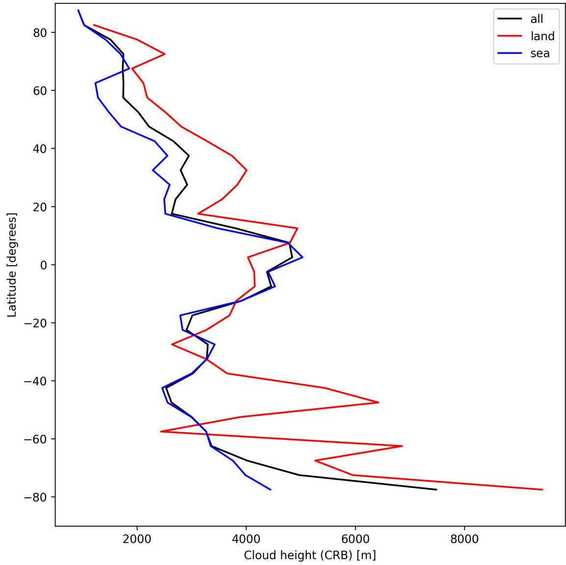
Figure 27: Zonal average of “Cloud height (CRB)” for 2025-04-25 to 2025-04-27.
