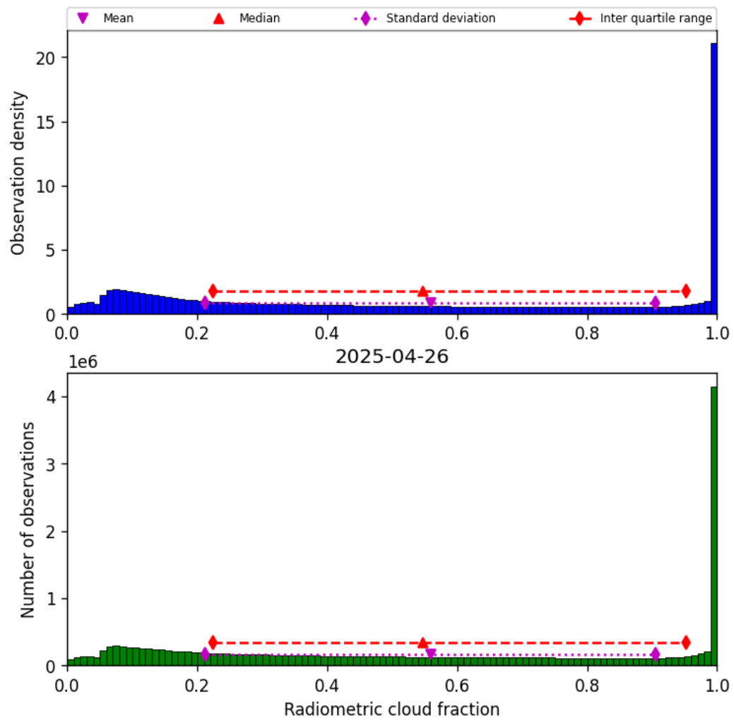
Figure 39: Histogram of “Radiometric cloud fraction” for 2025-04-25 to 2025-04-27
