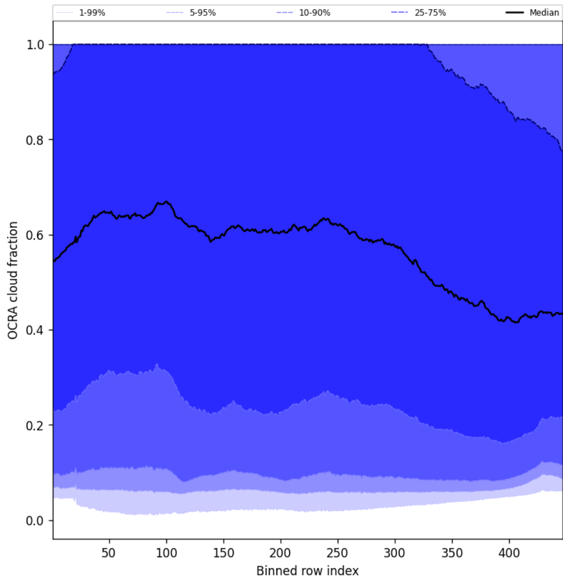
Figure 66: Along track statistics of “OCRA cloud fraction” for 2025-04-25 to 2025-04-27
