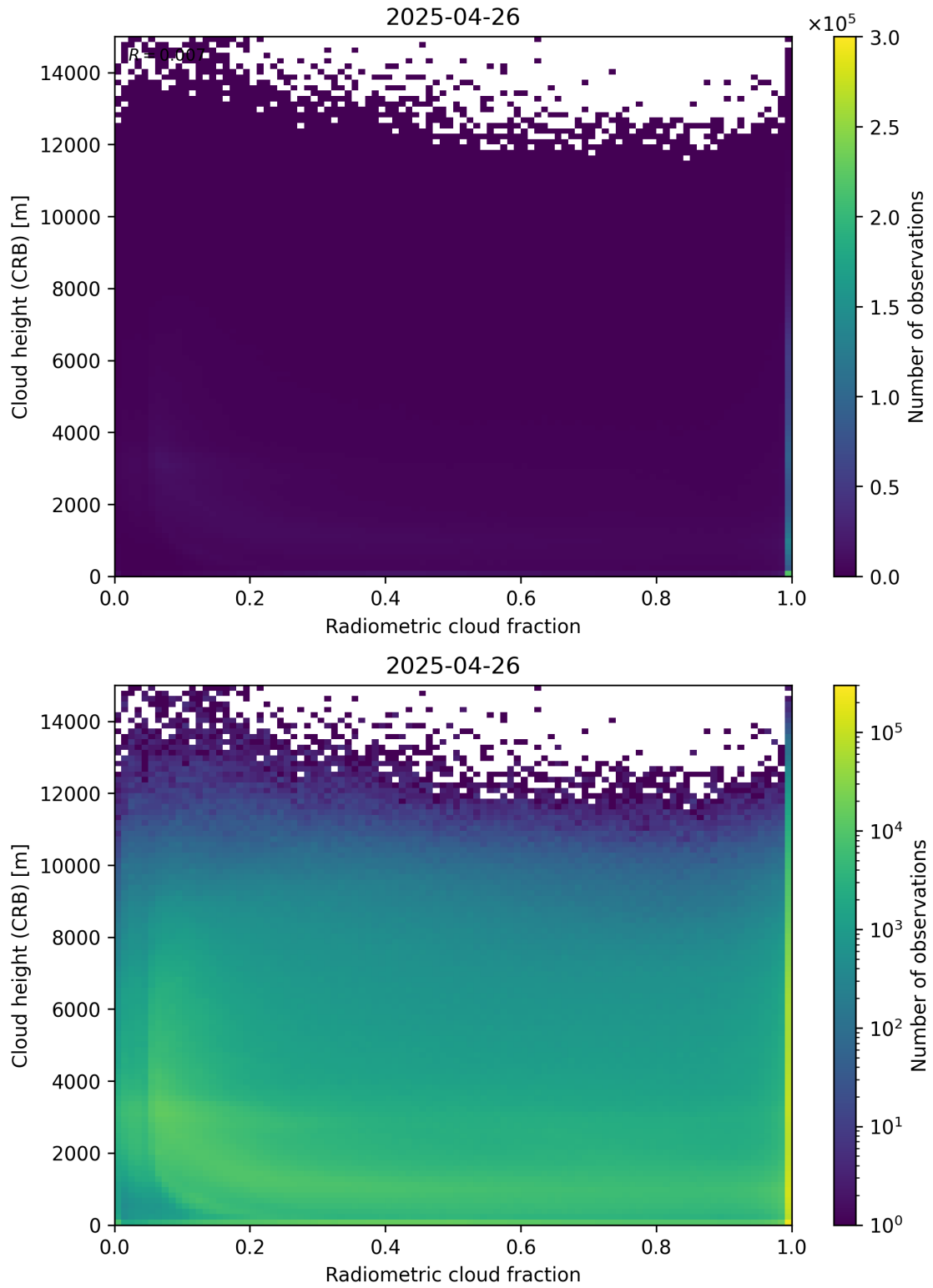
Figure 74: Scatter density plot of “Radiometric cloud fraction” against “Cloud height (CRB)” for 2025-04-25 to 2025-04-27.
