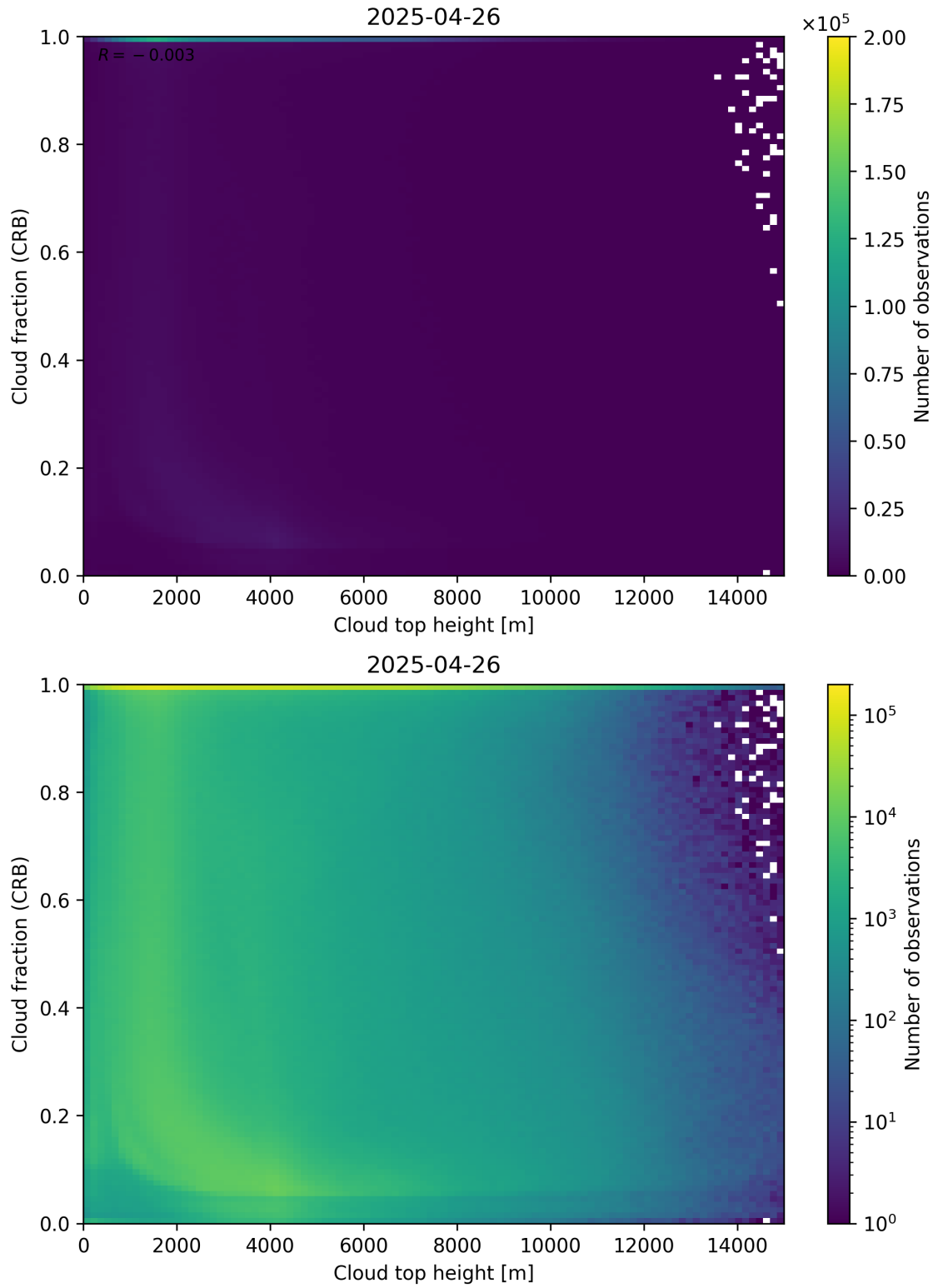
Figure 88: Scatter density plot of “Cloud top height” against “Cloud fraction (CRB)” for 2025-04-25 to 2025-04-27.
