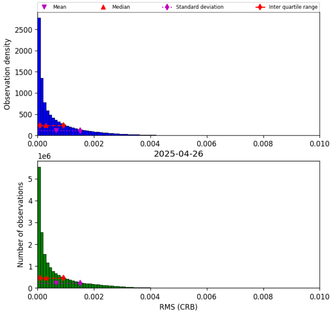
Figure 48: Histogram of “RMS (CRB)” for 2025-04-25 to 2025-04-27
