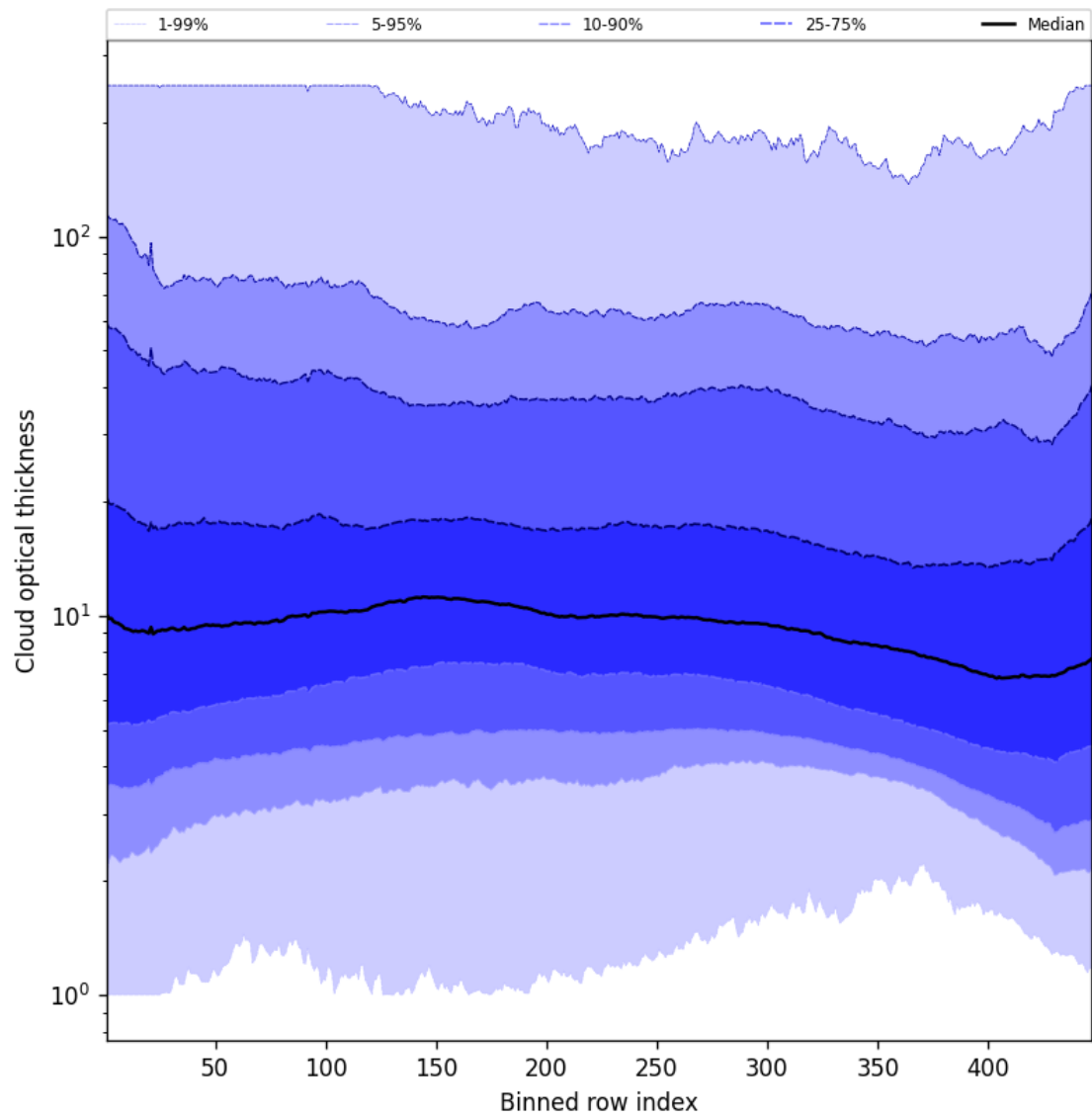
Figure 57: Along track statistics of “Cloud optical thickness” for 2025-04-25 to 2025-04-27
