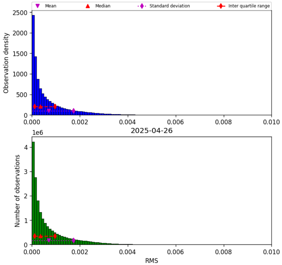
Figure 47: Histogram of “RMS” for 2025-04-25 to 2025-04-27
