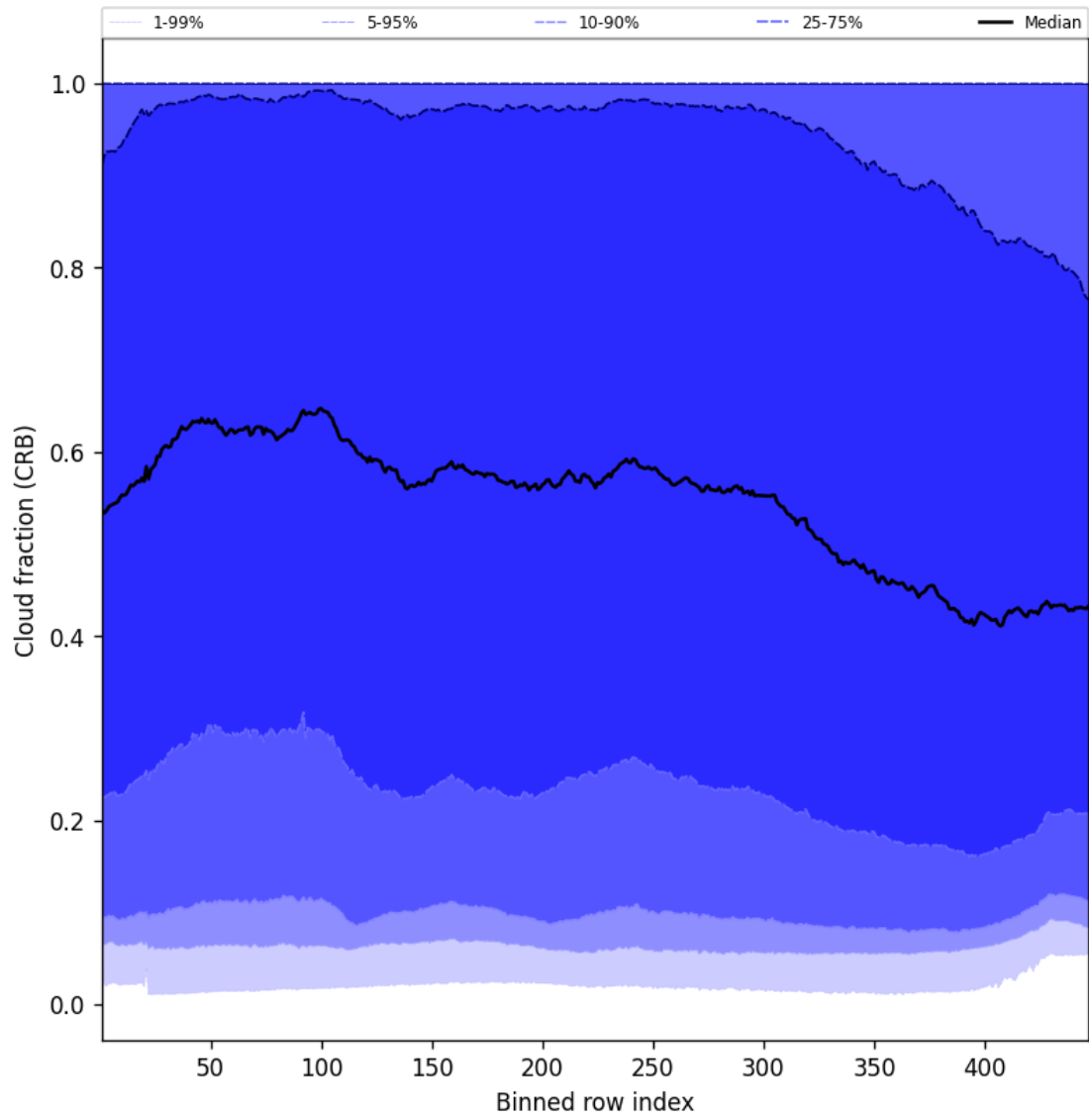
Figure 58: Along track statistics of “Cloud fraction (CRB)” for 2025-04-25 to 2025-04-27
