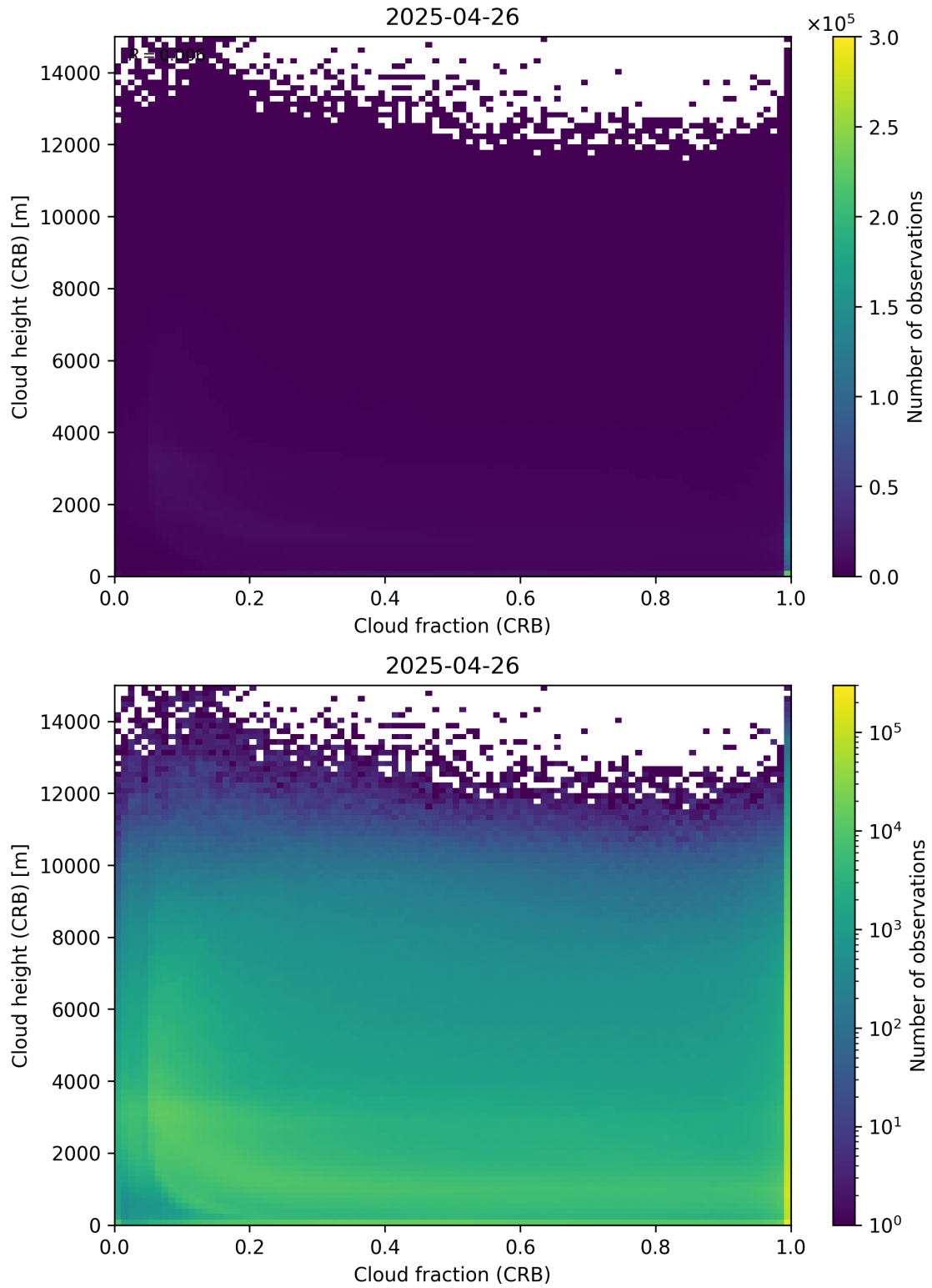
Figure 79: Scatter density plot of “Cloud fraction (CRB)” against “Cloud height (CRB)” for 2025-04-25 to 2025-04-27.
