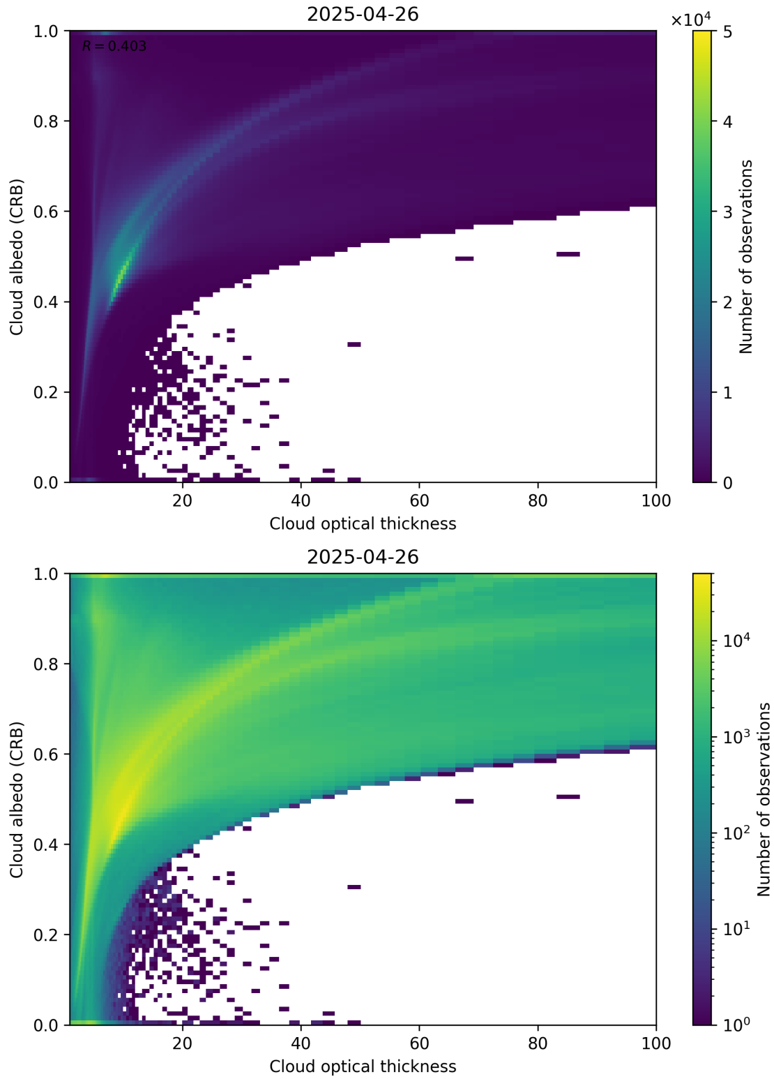
Figure 82: Scatter density plot of “Cloud optical thickness” against “Cloud albedo (CRB)” for 2025-04-25 to 2025-04-27.
