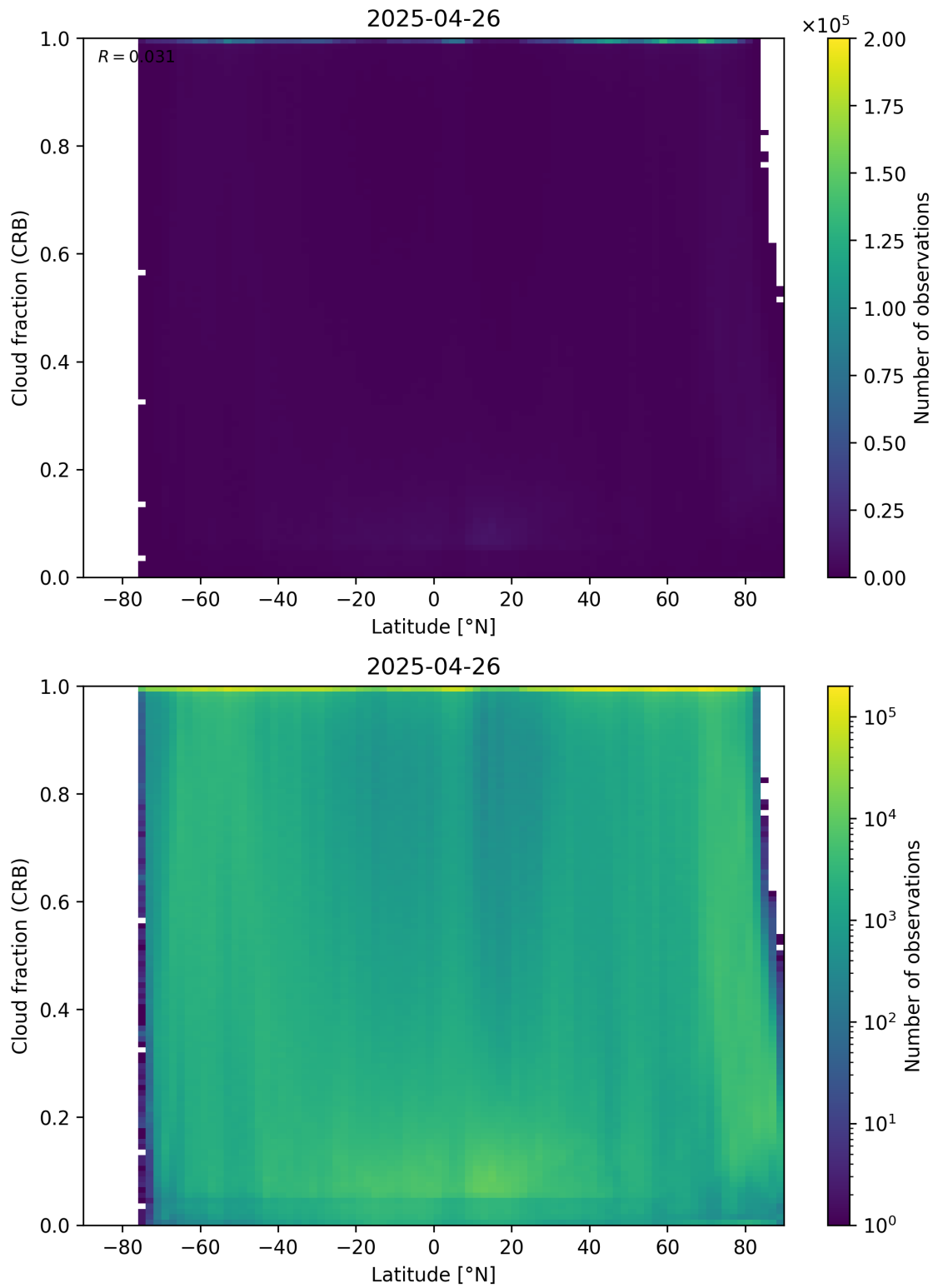
Figure 94: Scatter density plot of “Latitude” against “Cloud fraction (CRB)” for 2025-04-25 to 2025-04-27.
