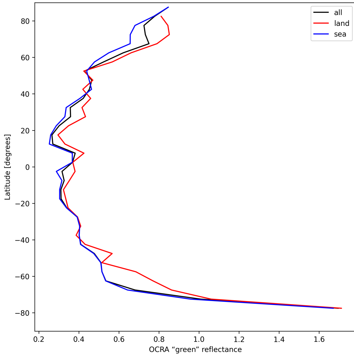
Figure 36: Zonal average of “OCRA “green” reflectance” for 2025-04-25 to 2025-04-27.
