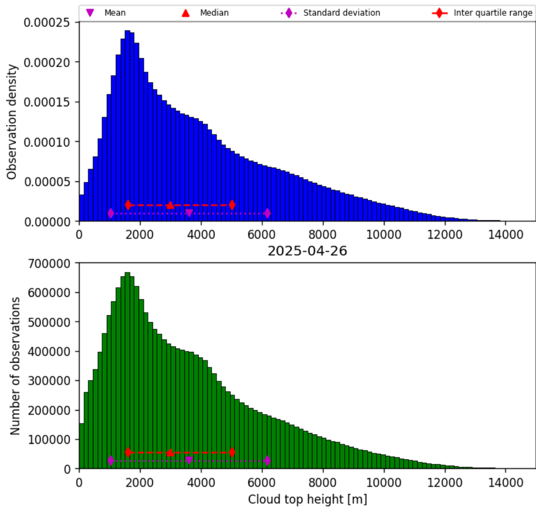
Figure 40: Histogram of “Cloud top height” for 2025-04-25 to 2025-04-27
