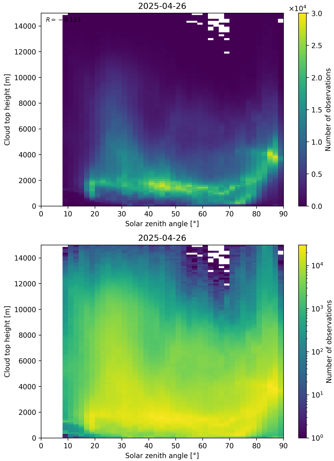
Figure 104: Scatter density plot of “Solar zenith angle” against “Cloud top height” for 2025-04-25 to 2025-04-27.
