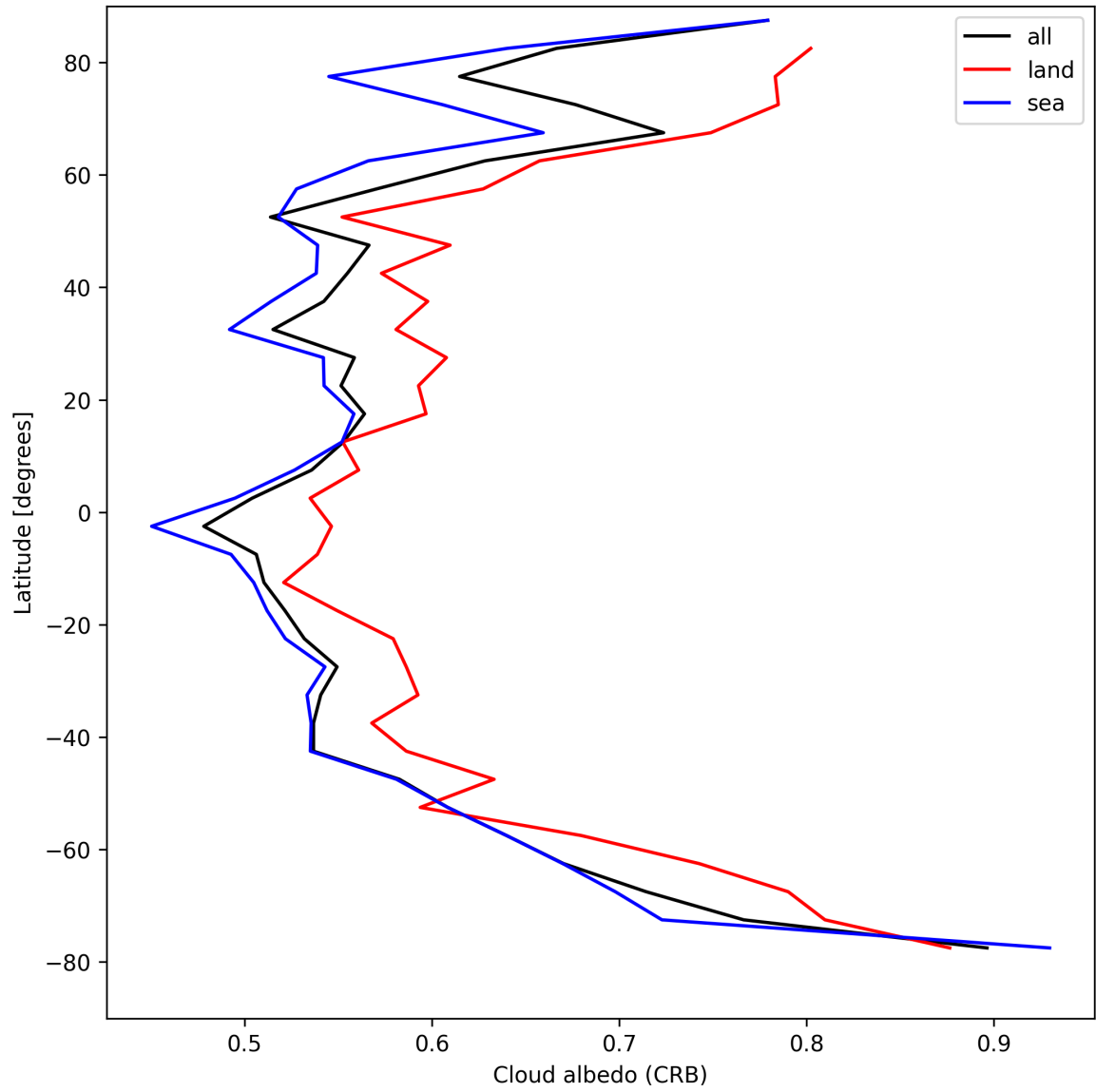
Figure 28: Zonal average of “Cloud albedo (CRB)” for 2025-04-25 to 2025-04-27.
