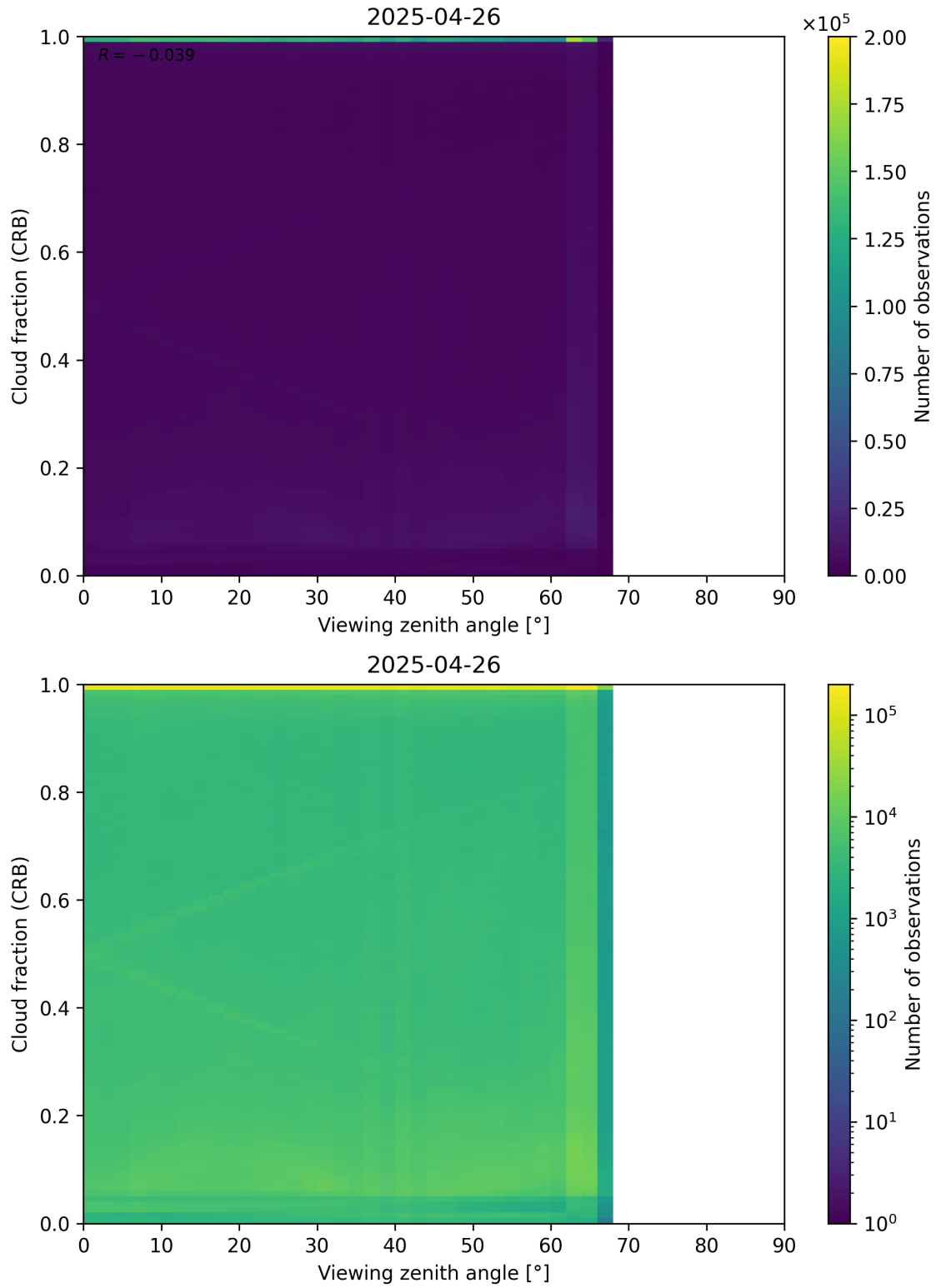
Figure 109: Scatter density plot of “Viewing zenith angle” against “Cloud fraction (CRB)” for 2025-04-25 to 2025-04-27.
