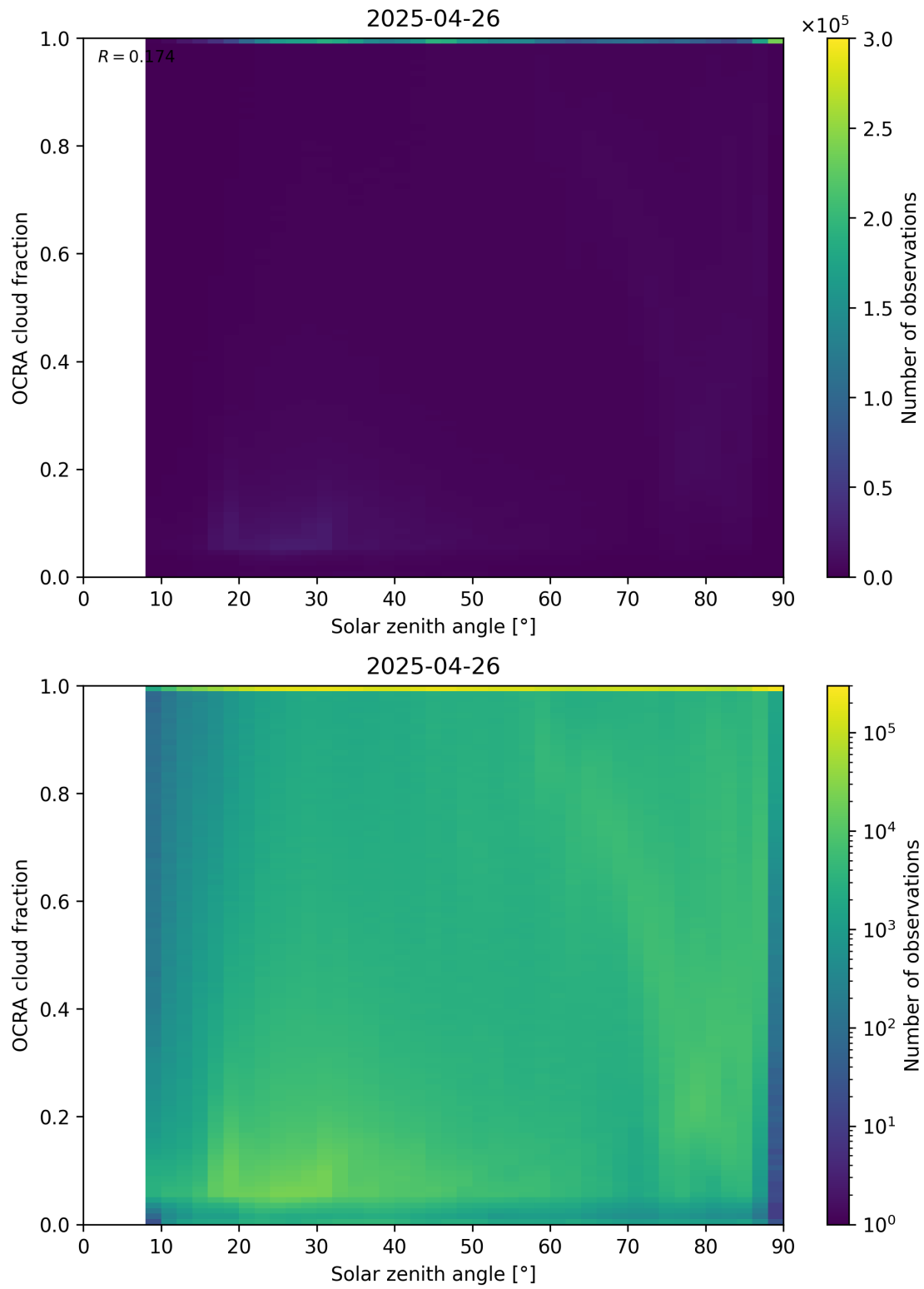
Figure 100: Scatter density plot of “Solar zenith angle” against “OCRA cloud fraction” for 2025-04-25 to 2025-04-27.
