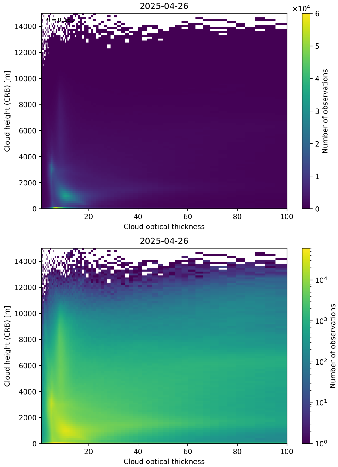
Figure 85: Scatter density plot of “Cloud optical thickness” against “Cloud height (CRB)” for 2025-04-25 to 2025-04-27.
