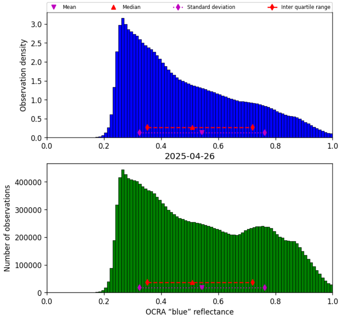
Figure 51: Histogram of “OCRA “blue” reflectance” for 2025-04-25 to 2025-04-27
