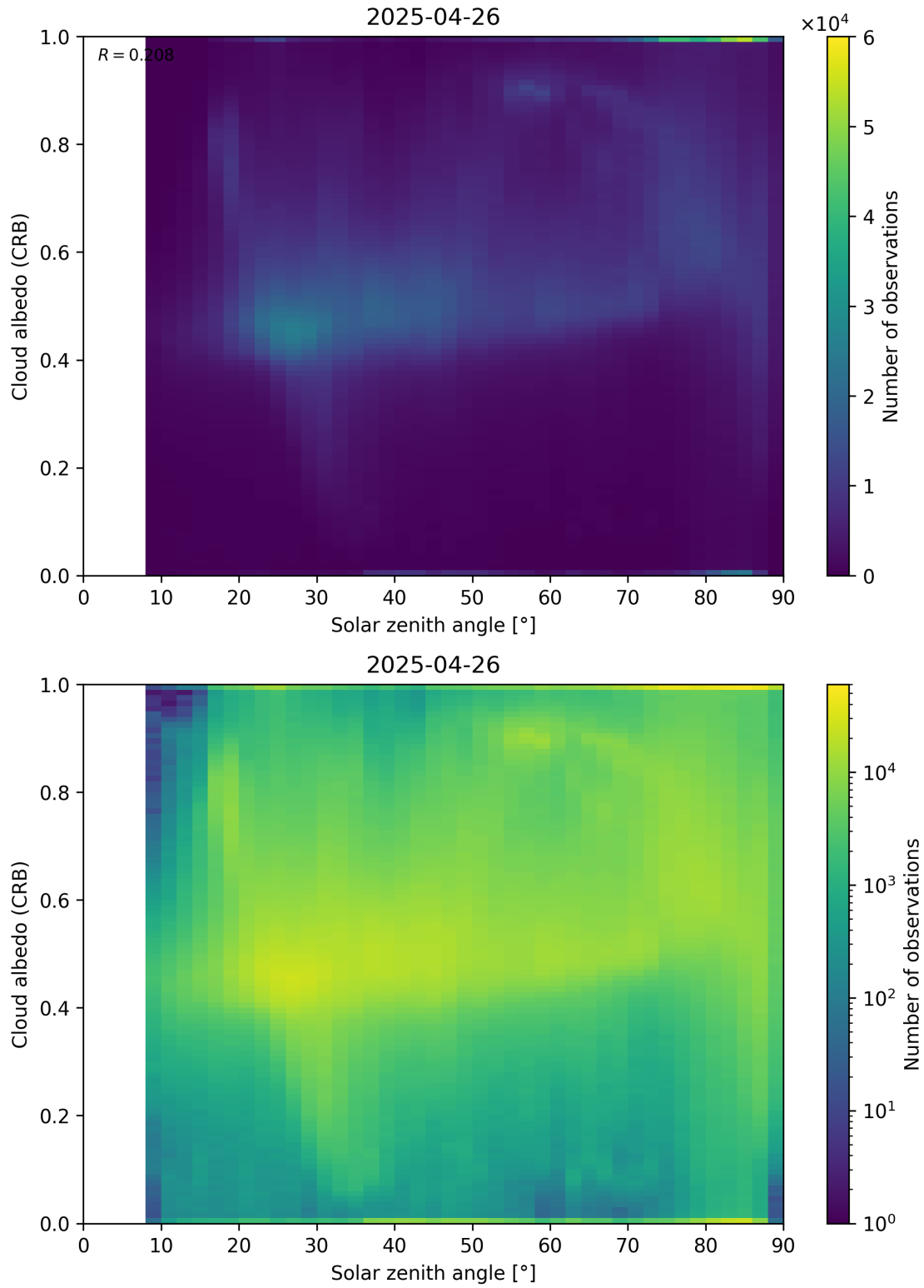
Figure 98: Scatter density plot of “Solar zenith angle” against “Cloud albedo (CRB)” for 2025-04-25 to 2025-04-27.
