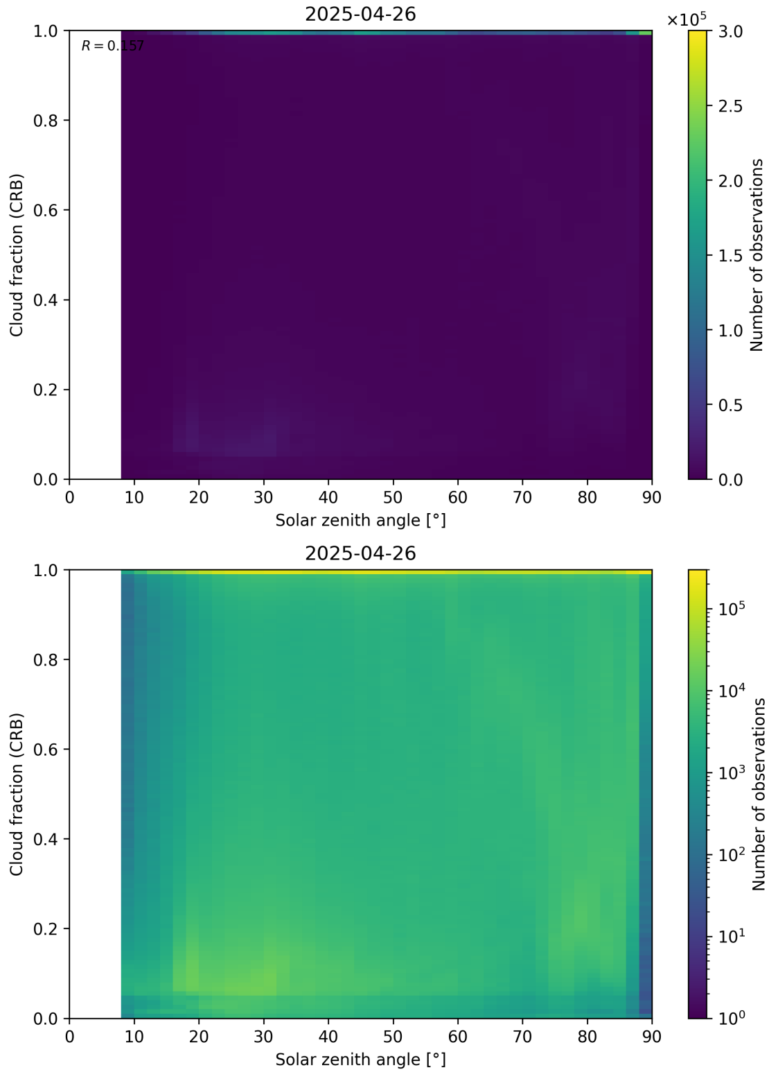
Figure 101: Scatter density plot of “Solar zenith angle” against “Cloud fraction (CRB)” for 2025-04-25 to 2025-04-27.
