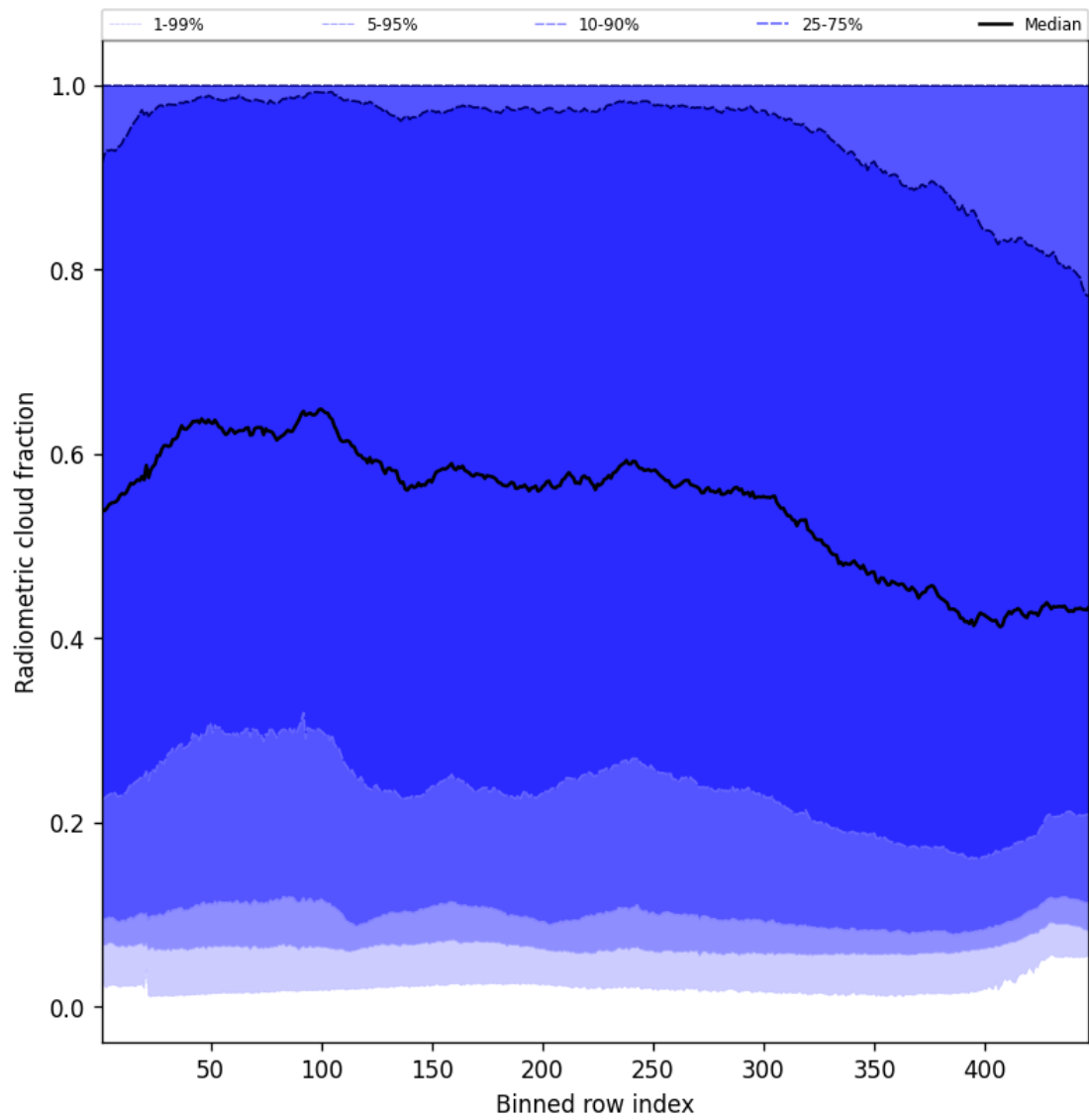
Figure 55: Along track statistics of “Radiometric cloud fraction” for 2025-04-25 to 2025-04-27
