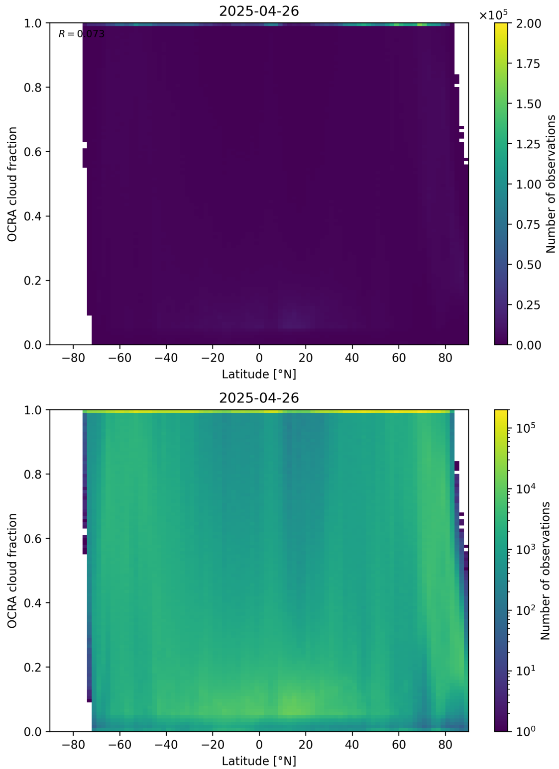
Figure 93: Scatter density plot of “Latitude” against “OCRA cloud fraction” for 2025-04-25 to 2025-04-27.
