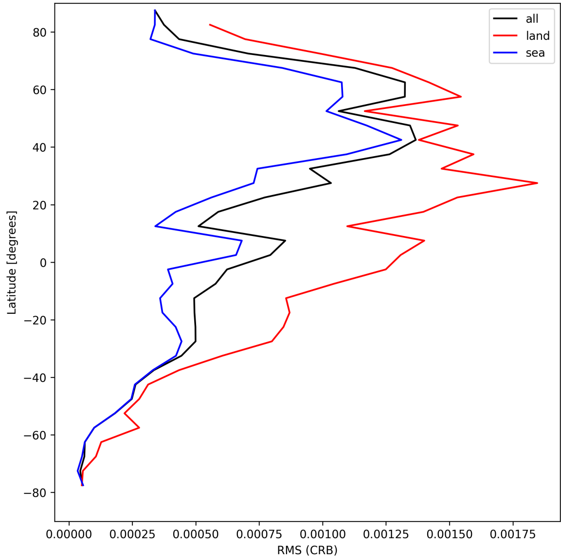
Figure 32: Zonal average of “RMS (CRB)” for 2025-04-25 to 2025-04-27.
