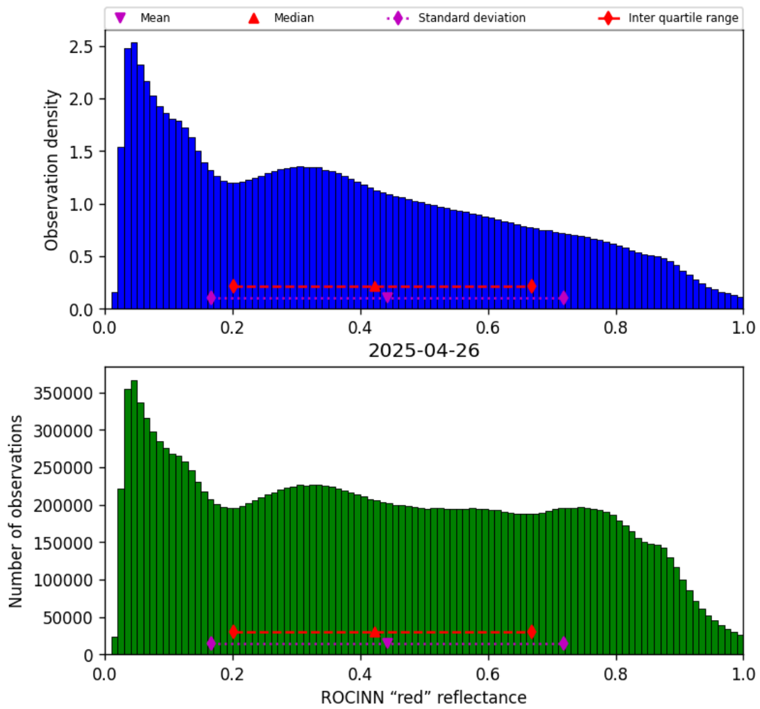
Figure 53: Histogram of “ROCINN “red” reflectance” for 2025-04-25 to 2025-04-27
