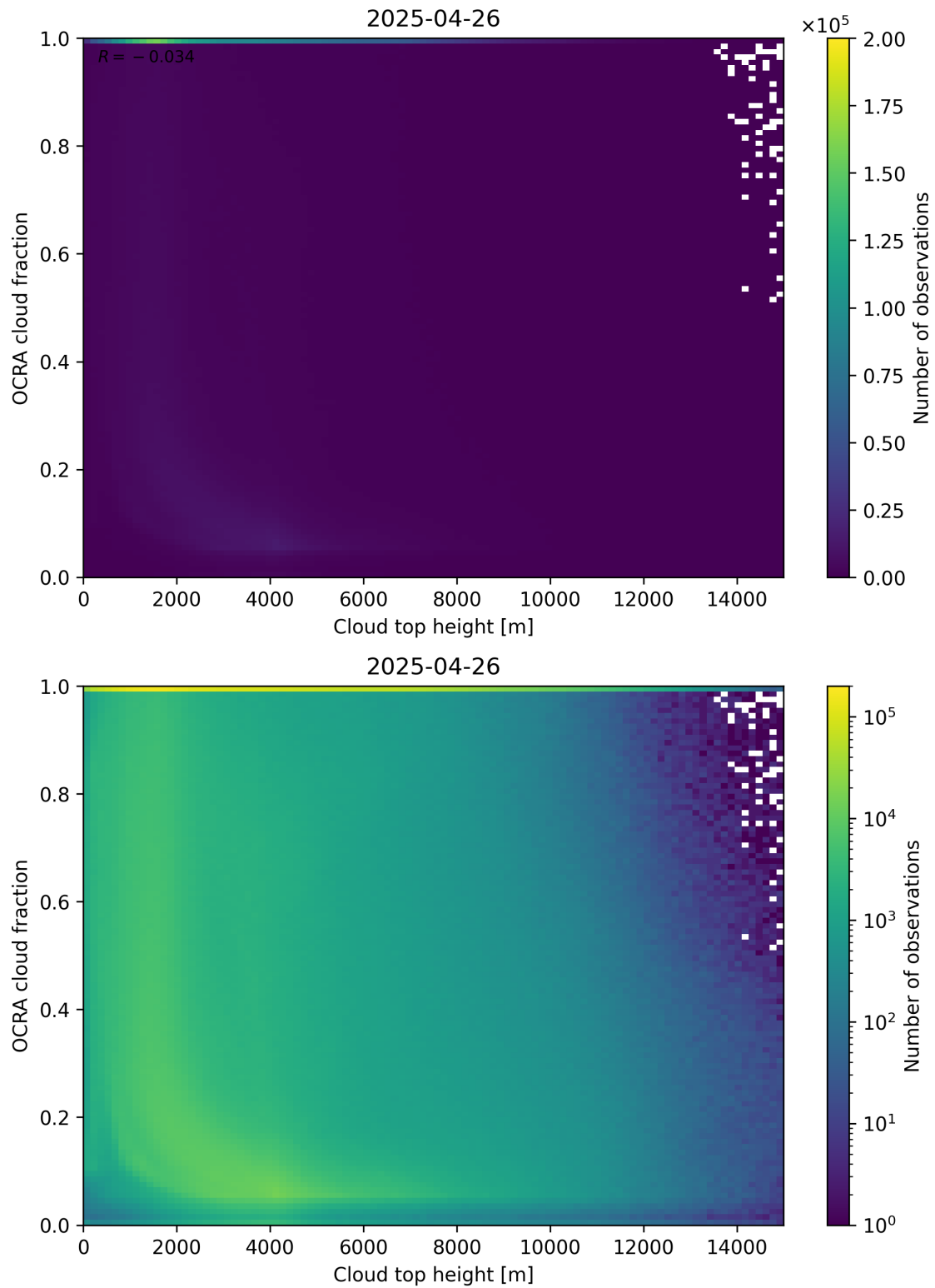
Figure 87: Scatter density plot of “Cloud top height” against “OCRA cloud fraction” for 2025-04-25 to 2025-04-27.
