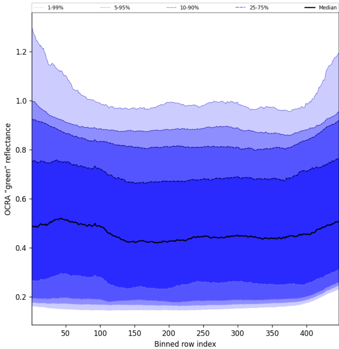
Figure 68: Along track statistics of "OCRA "green" reflectance" for 2025-04-25 to 2025-04-27
