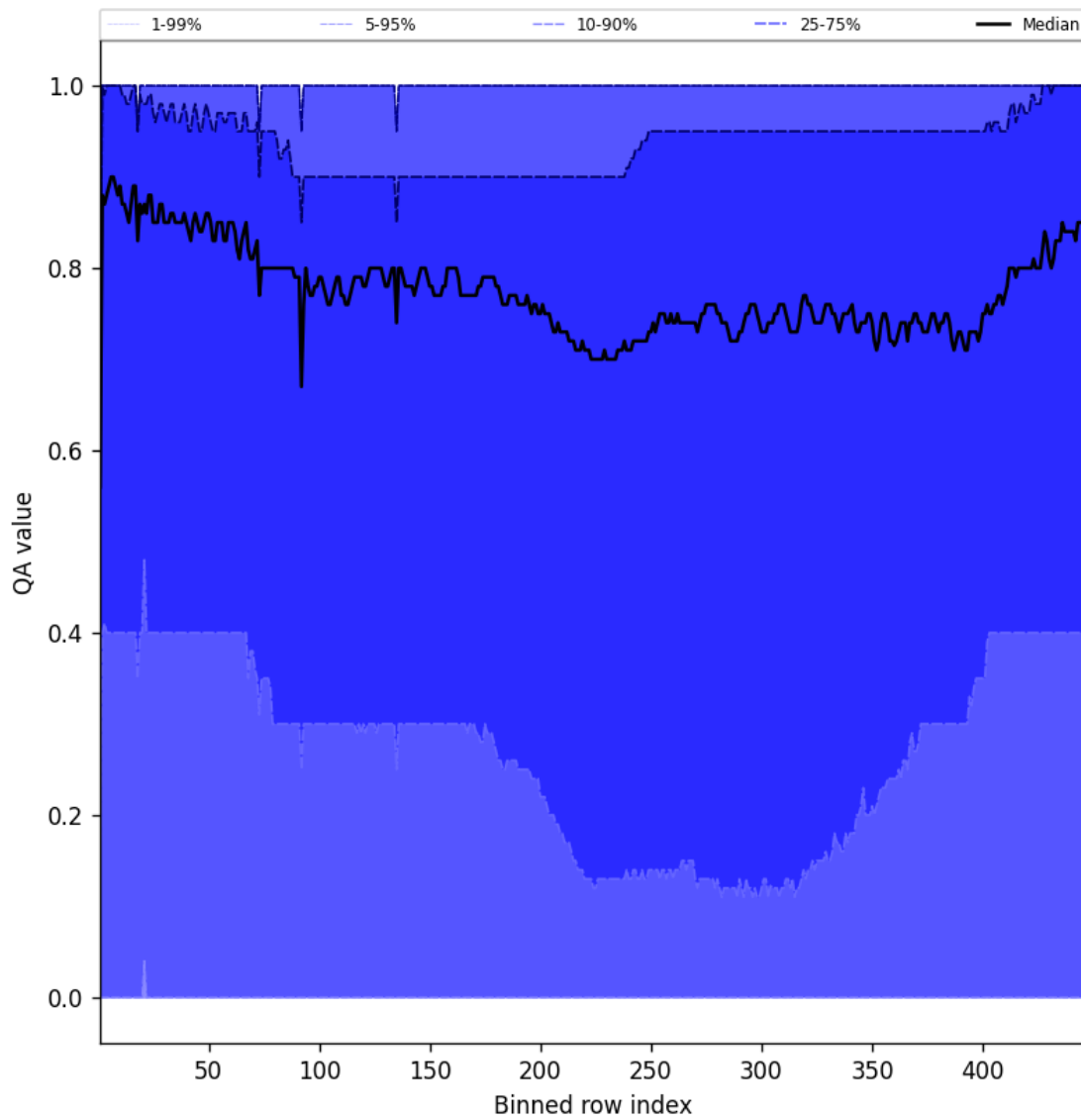
Figure 54: Along track statistics of “QA value” for 2025-04-25 to 2025-04-27
