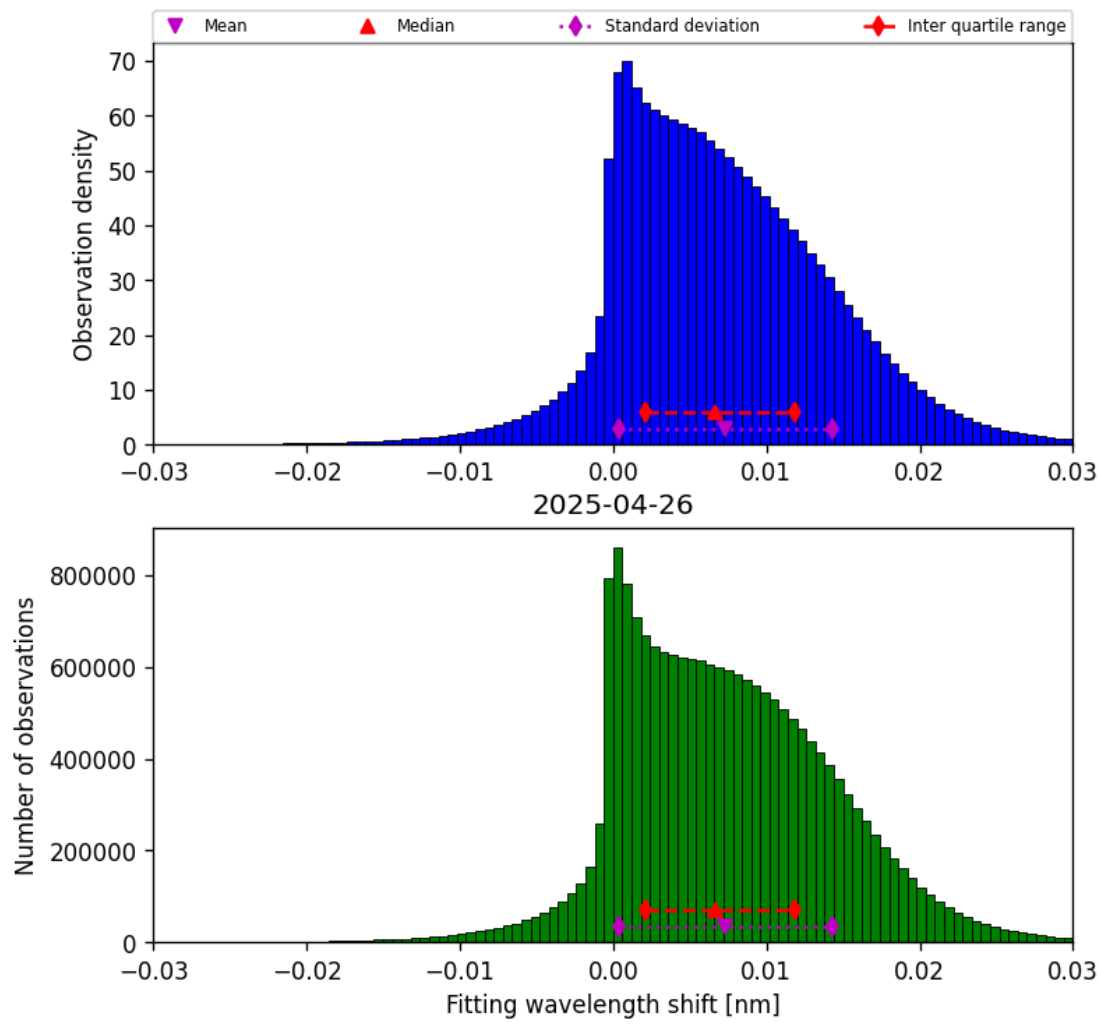
Figure 49: Histogram of “Fitting wavelength shift” for 2025-04-25 to 2025-04-27
