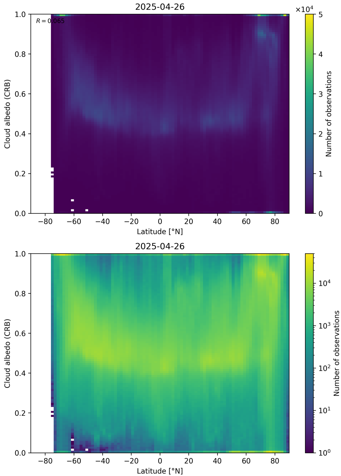
Figure 91: Scatter density plot of “Latitude” against “Cloud albedo (CRB)” for 2025-04-25 to 2025-04-27.
