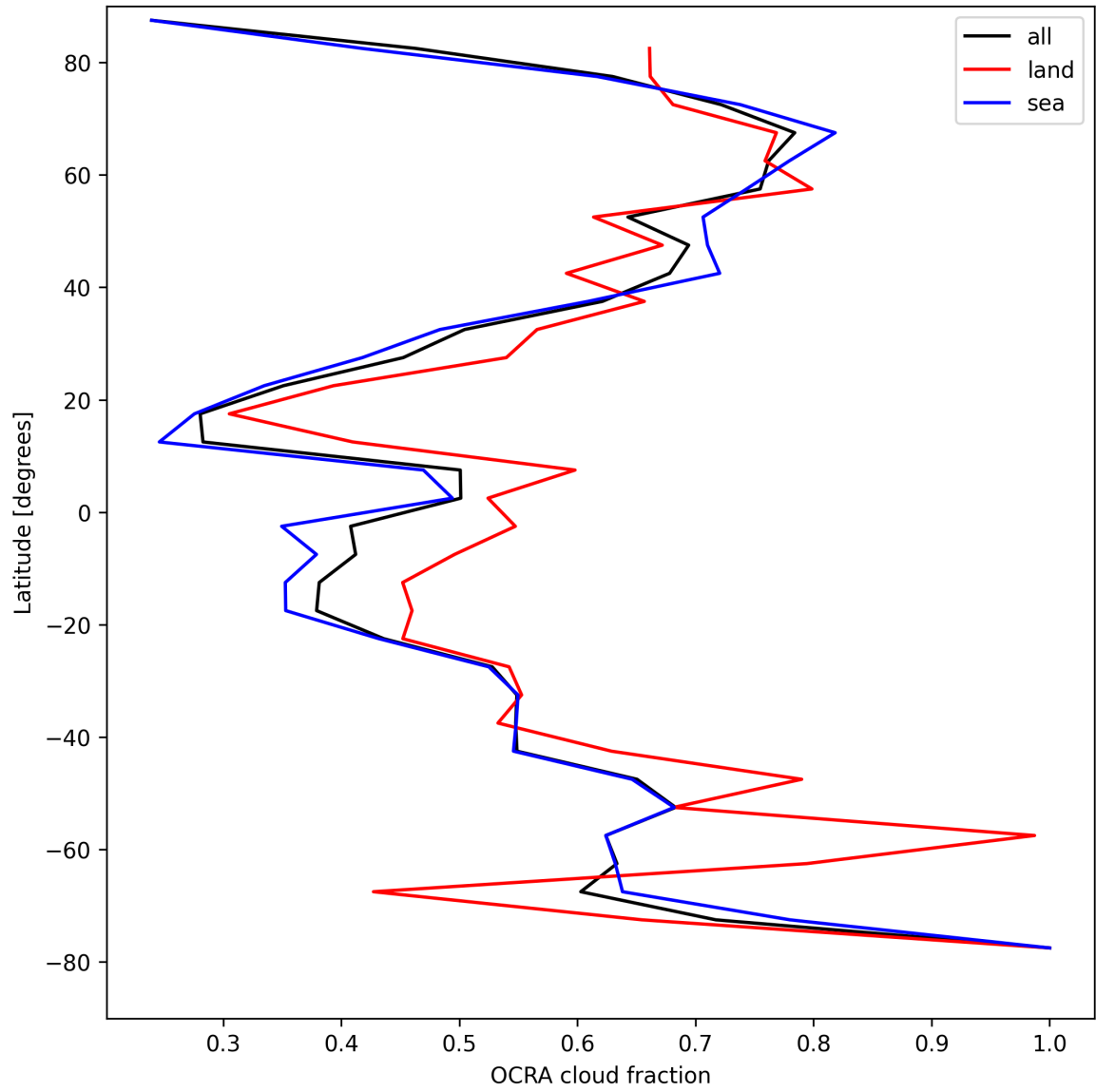
Figure 34: Zonal average of “OCRA cloud fraction” for 2025-04-25 to 2025-04-27.
