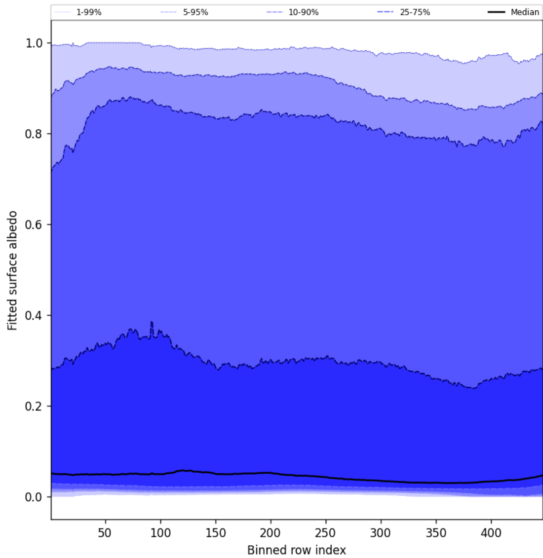
Figure 61: Along track statistics of “Fitted surface albedo” for 2025-04-25 to 2025-04-27
