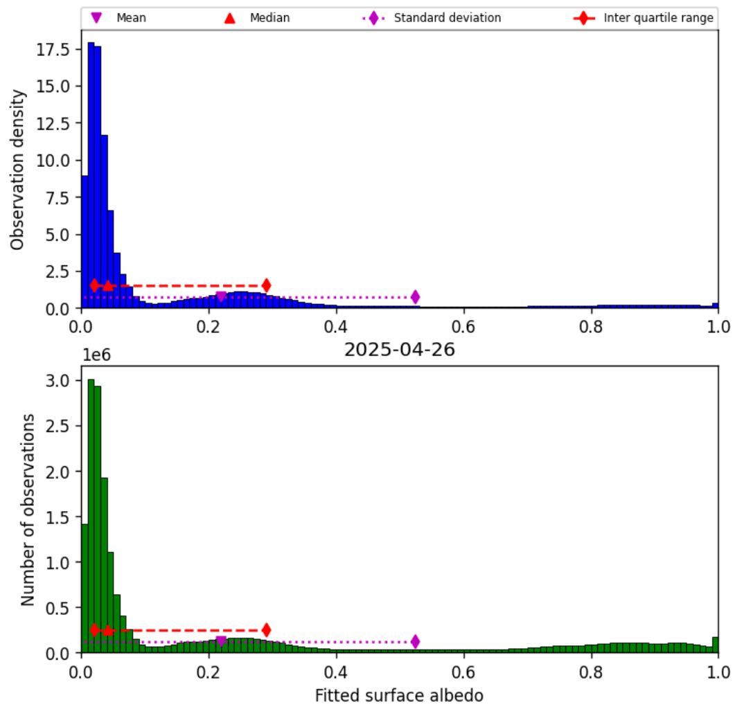
Figure 45: Histogram of “Fitted surface albedo” for 2025-04-25 to 2025-04-27
