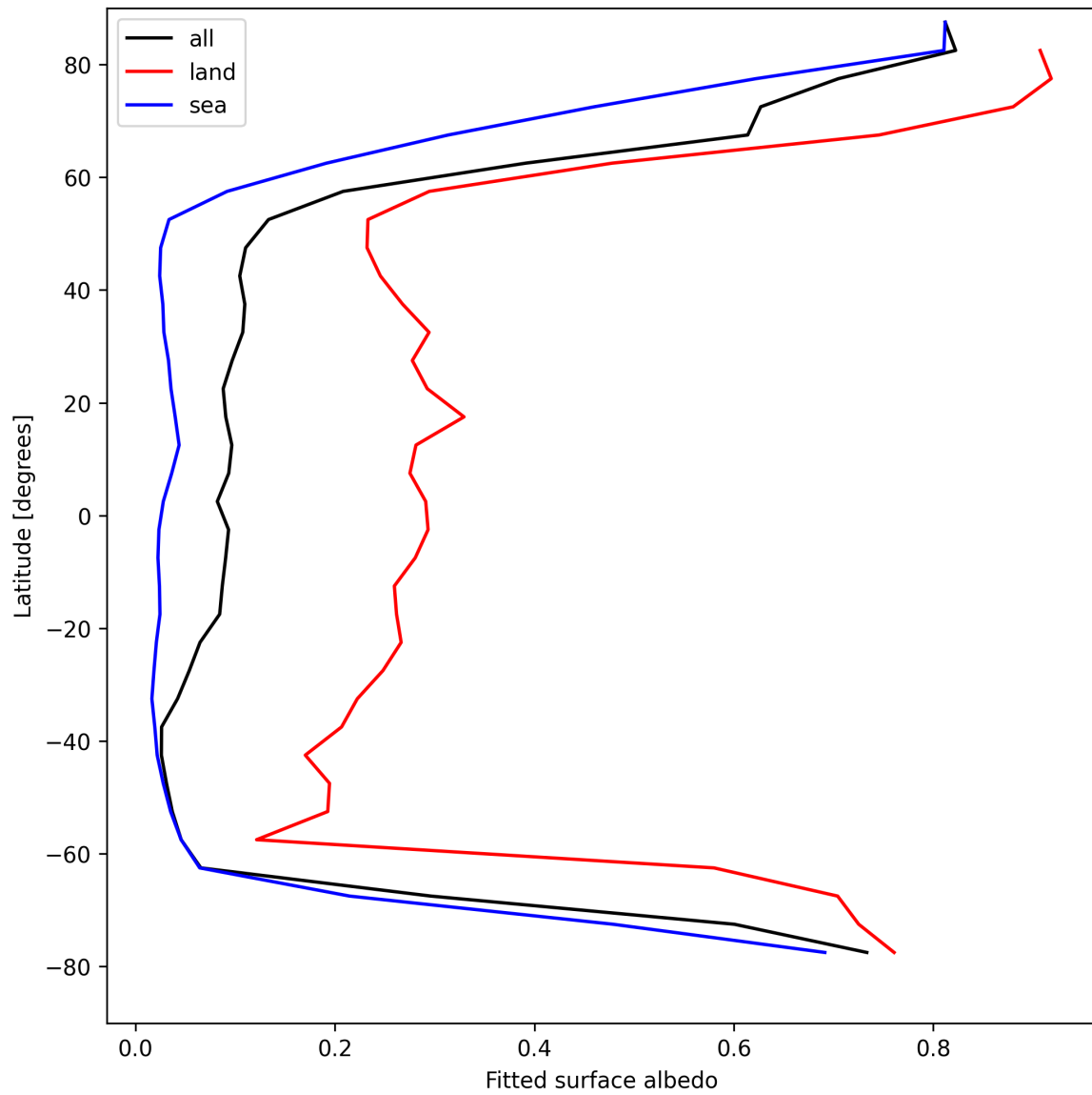
Figure 29: Zonal average of “Fitted surface albedo” for 2025-04-25 to 2025-04-27.
