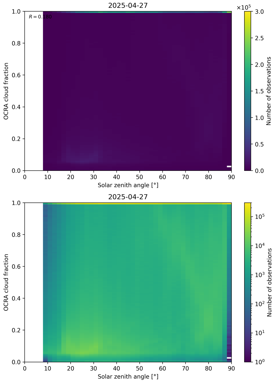
Figure 100: Scatter density plot of “Solar zenith angle” against “OCRA cloud fraction” for 2025-04-26 to 2025-04-28.
