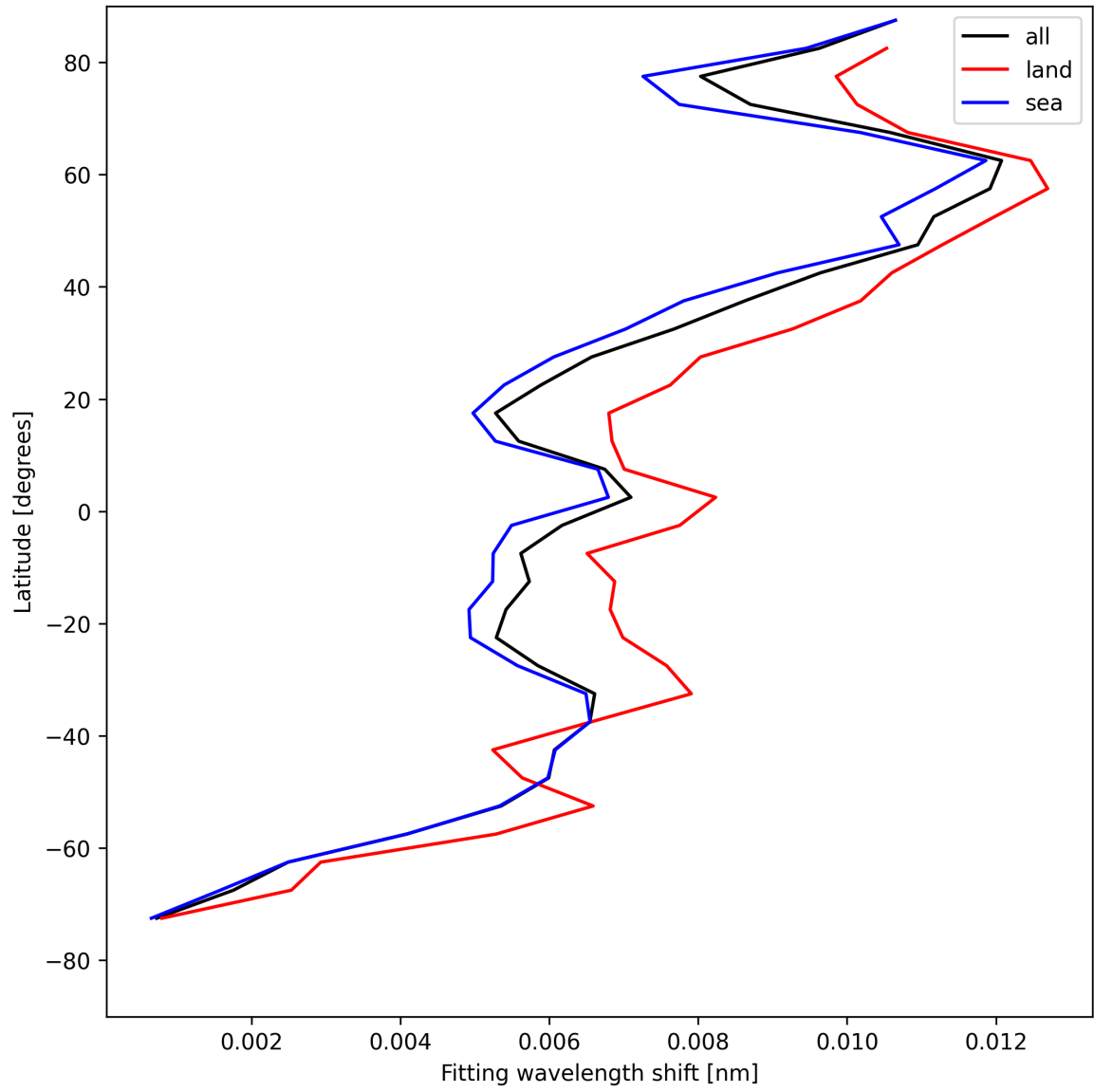
Figure 33: Zonal average of “Fitting wavelength shift” for 2025-04-26 to 2025-04-28.
