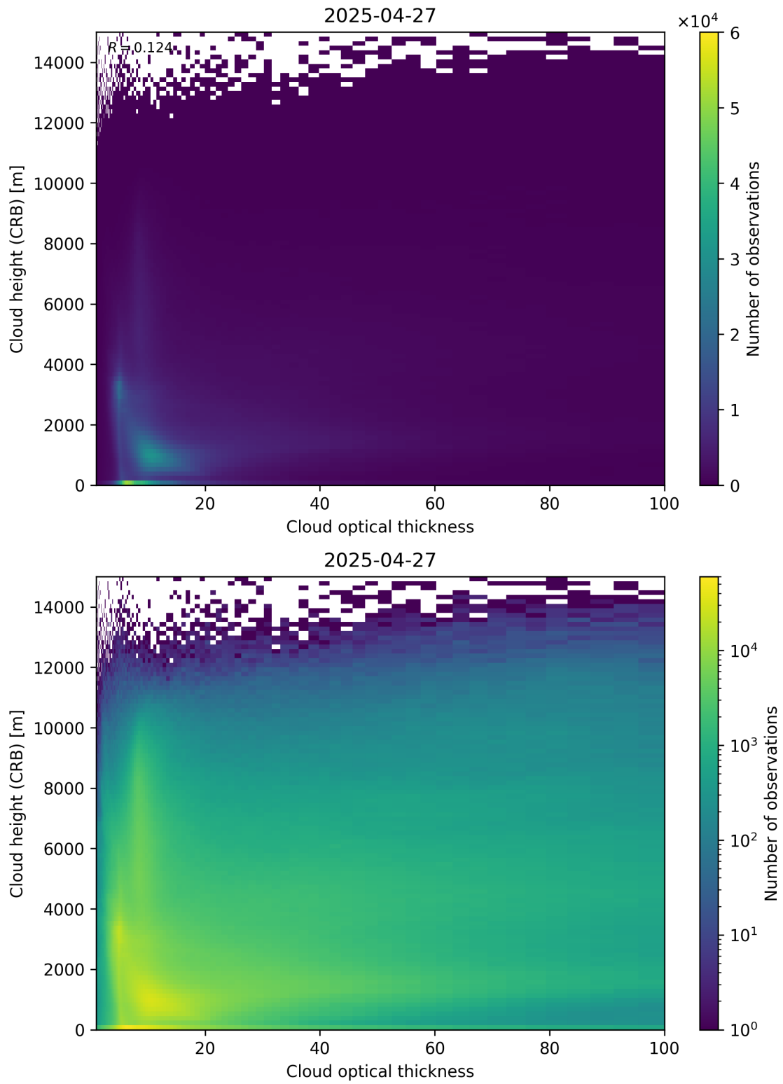
Figure 85: Scatter density plot of “Cloud optical thickness” against “Cloud height (CRB)” for 2025-04-26 to 2025-04-28.
