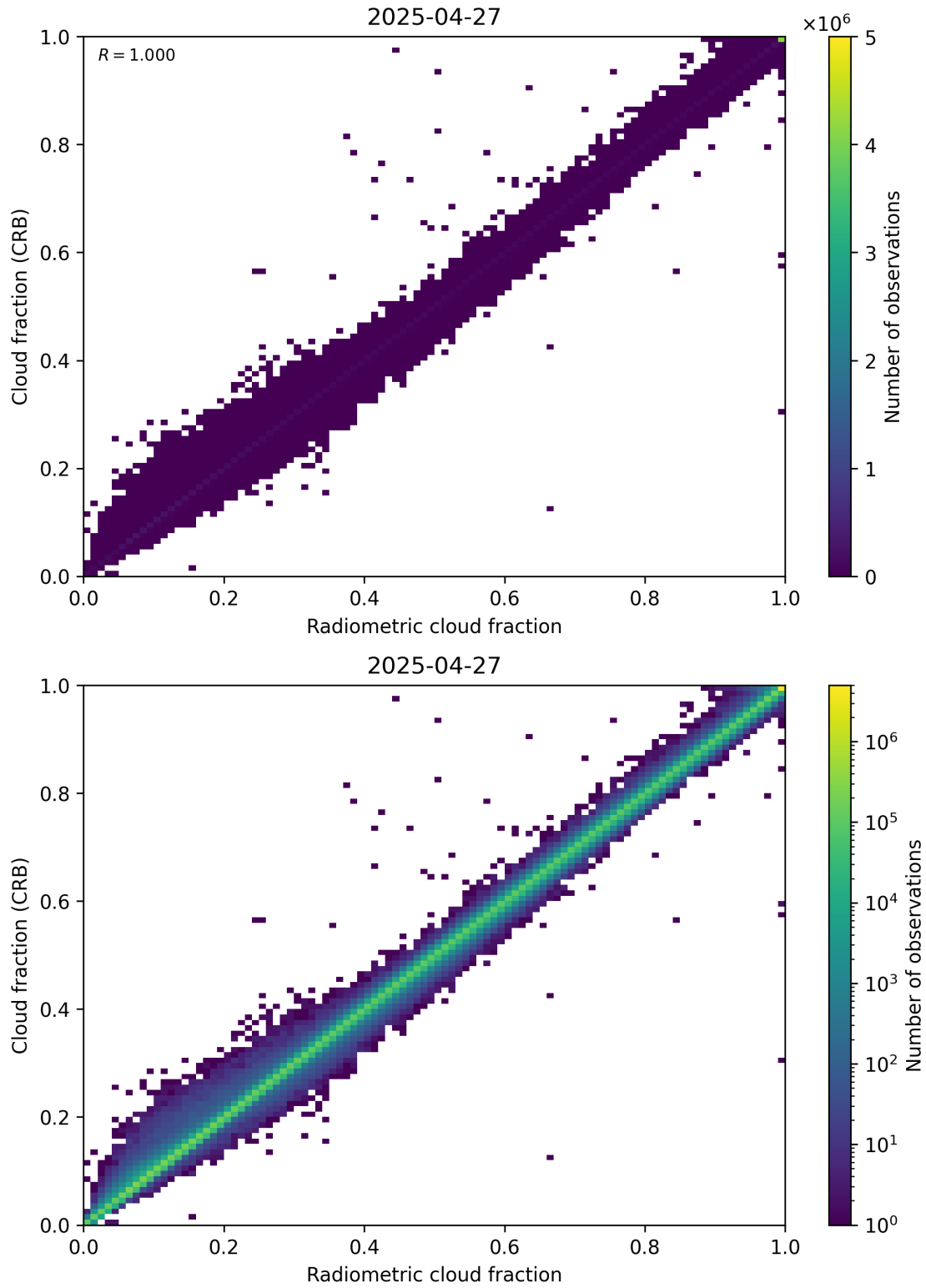
Figure 73: Scatter density plot of “Radiometric cloud fraction” against “Cloud fraction (CRB)” for 2025-04-26 to 2025-04-28.
