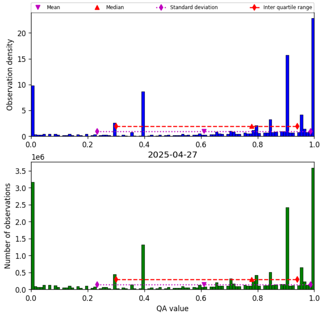
Figure 38: Histogram of “QA value” for 2025-04-26 to 2025-04-28
