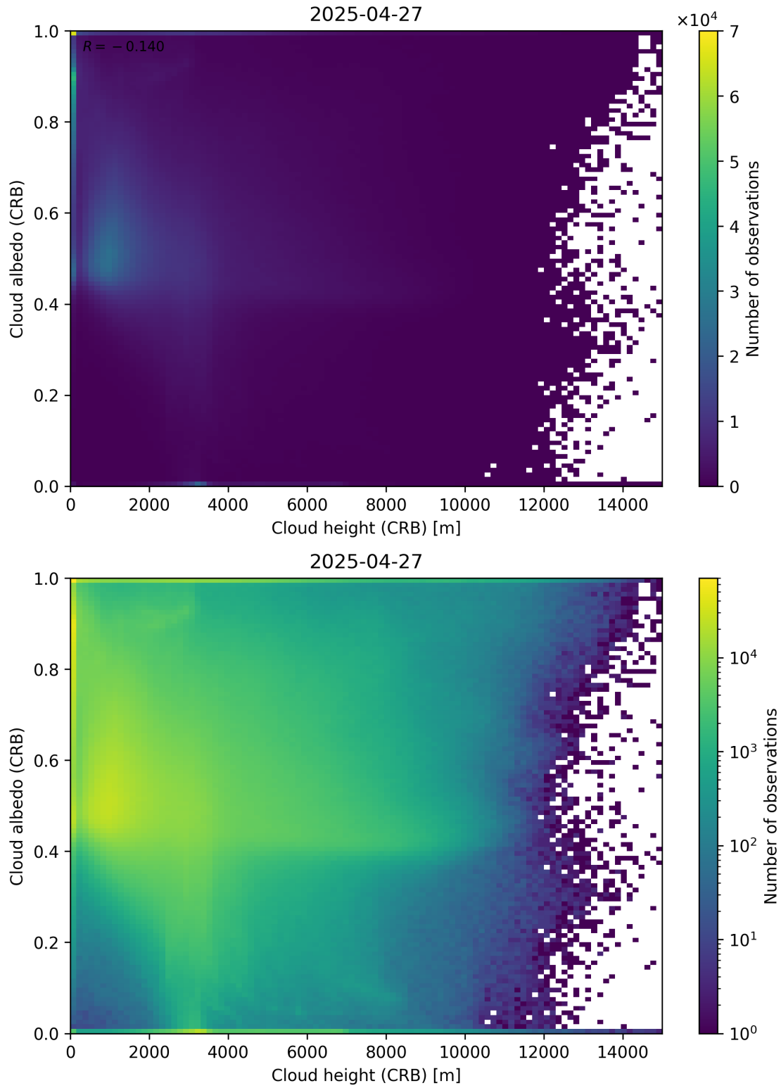
Figure 80: Scatter density plot of “Cloud height (CRB)” against “Cloud albedo (CRB)” for 2025-04-26 to 2025-04-28.
