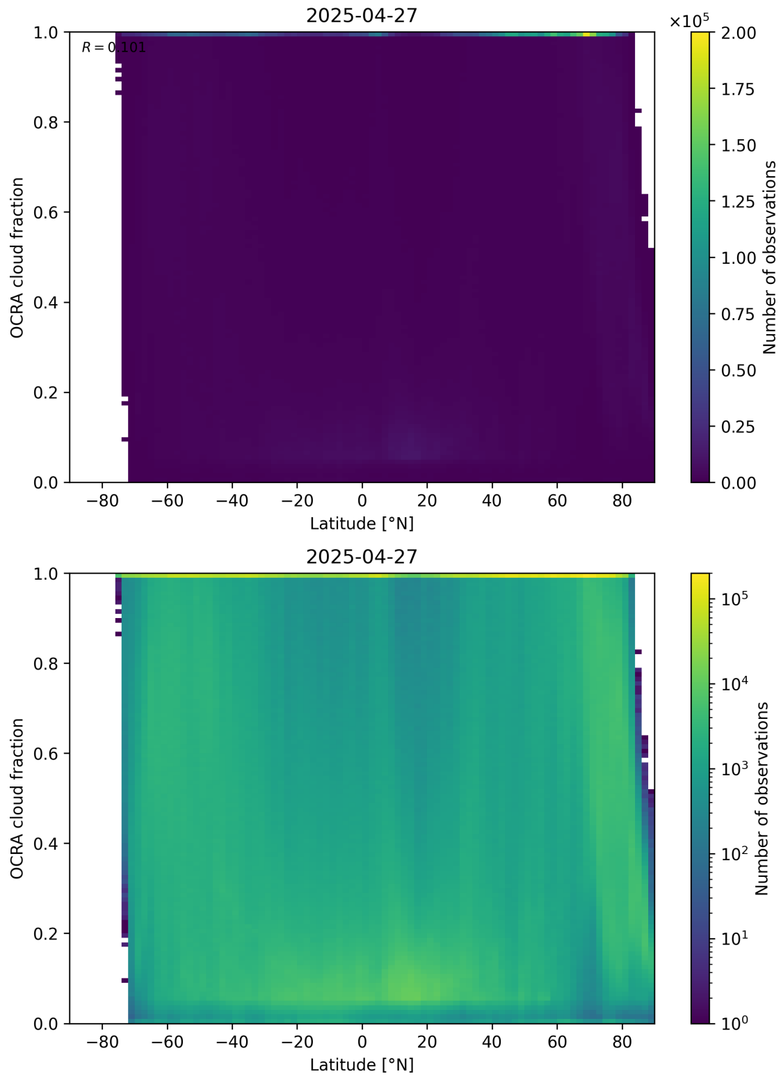
Figure 93: Scatter density plot of “Latitude” against “OCRA cloud fraction” for 2025-04-26 to 2025-04-28.
