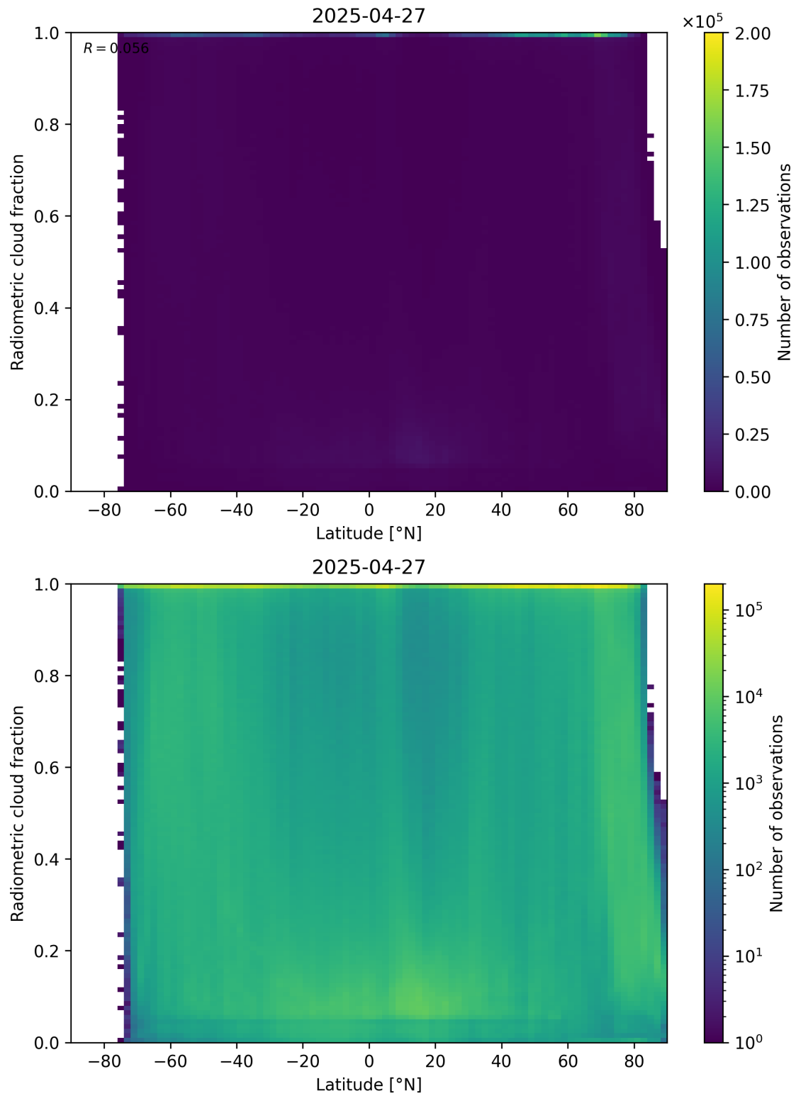
Figure 92: Scatter density plot of “Latitude” against “Radiometric cloud fraction” for 2025-04-26 to 2025-04-28.
