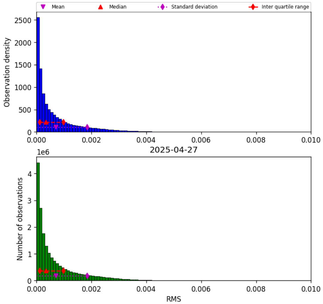
Figure 47: Histogram of “RMS” for 2025-04-26 to 2025-04-28
