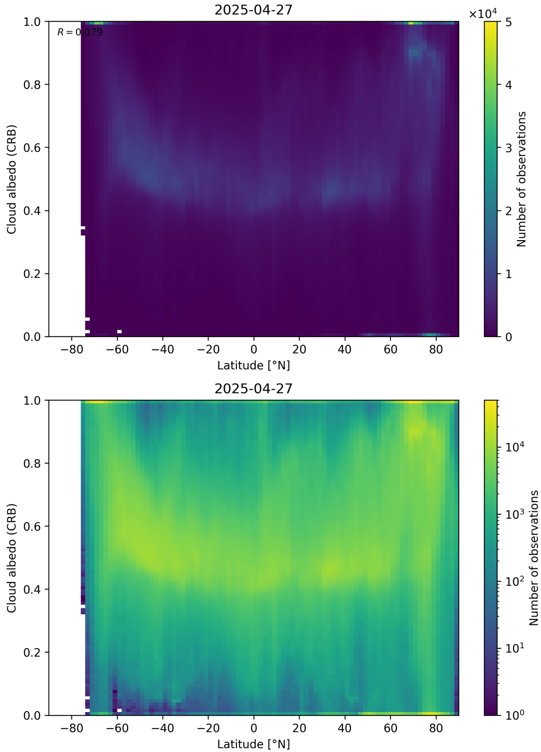
Figure 91: Scatter density plot of “Latitude” against “Cloud albedo (CRB)” for 2025-04-26 to 2025-04-28.
