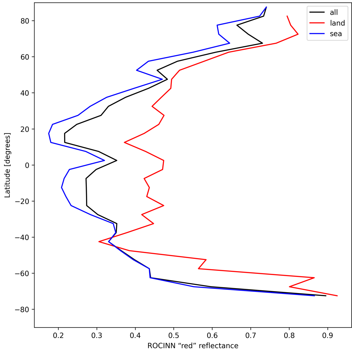
Figure 37: Zonal average of “ROCINN “red” reflectance” for 2025-04-26 to 2025-04-28.
