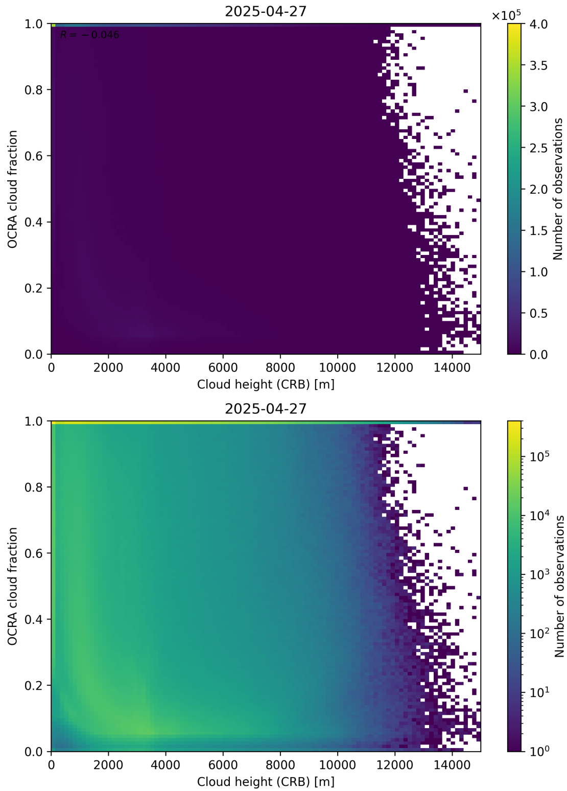
Figure 81: Scatter density plot of “Cloud height (CRB)” against “OCRA cloud fraction” for 2025-04-26 to 2025-04-28.
