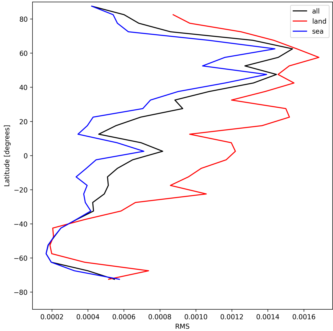
Figure 31: Zonal average of “RMS” for 2025-04-26 to 2025-04-28.
