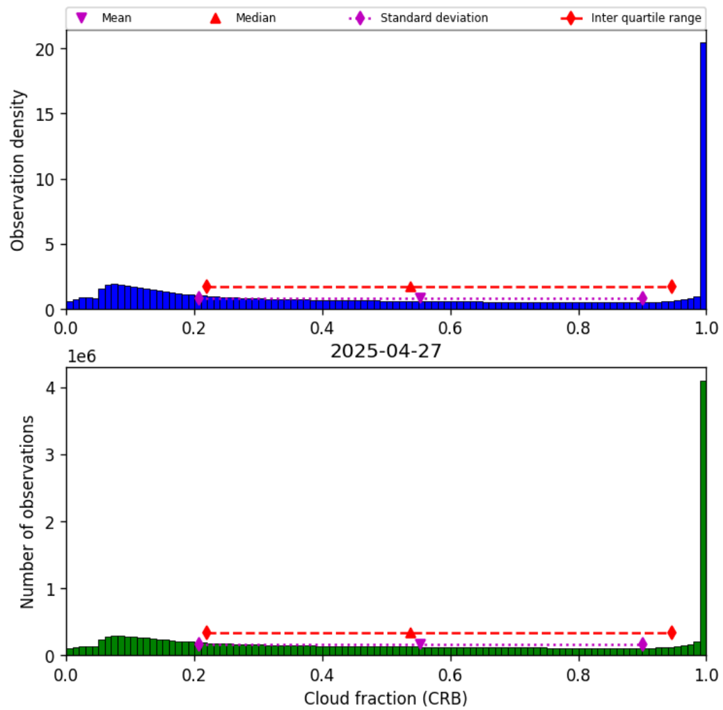
Figure 42: Histogram of “Cloud fraction (CRB)” for 2025-04-26 to 2025-04-28
