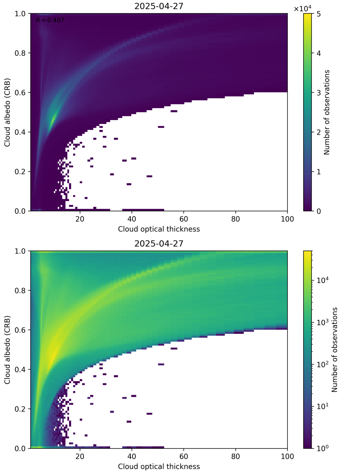
Figure 82: Scatter density plot of “Cloud optical thickness” against “Cloud albedo (CRB)” for 2025-04-26 to 2025-04-28.
