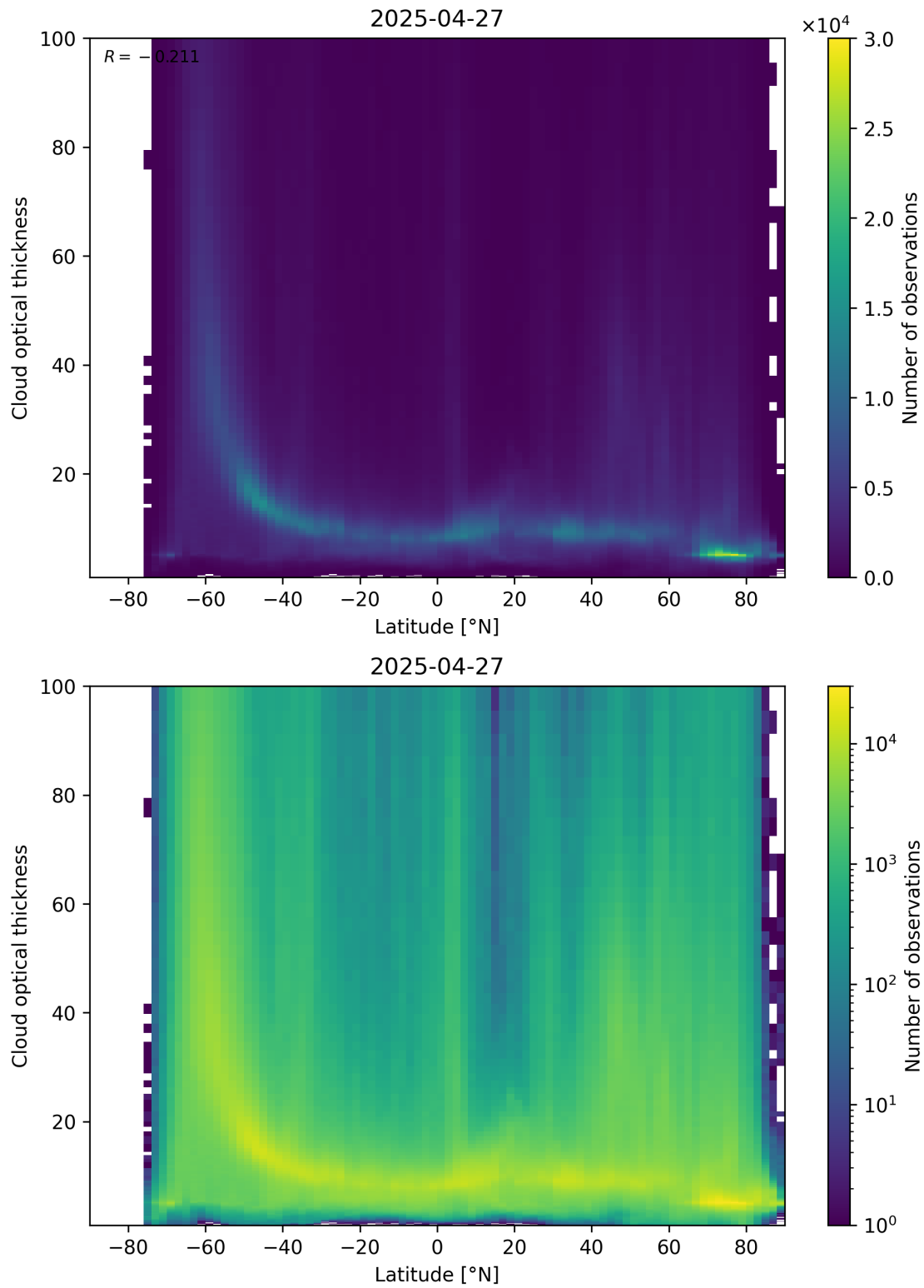
Figure 96: Scatter density plot of “Latitude” against “Cloud optical thickness” for 2025-04-26 to 2025-04-28.
