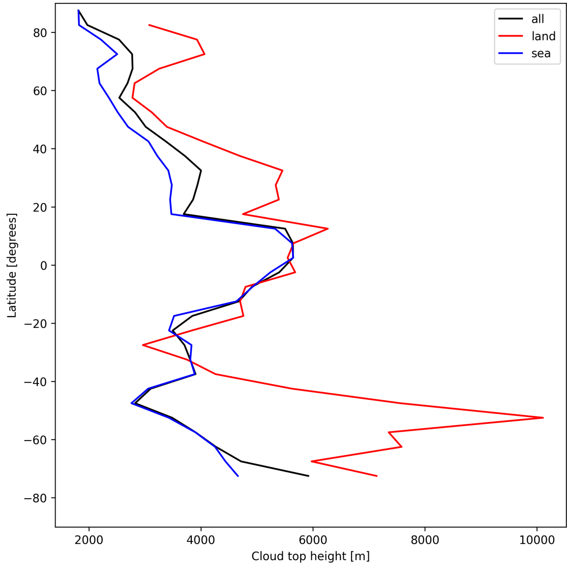
Figure 24: Zonal average of “Cloud top height” for 2025-04-26 to 2025-04-28.
