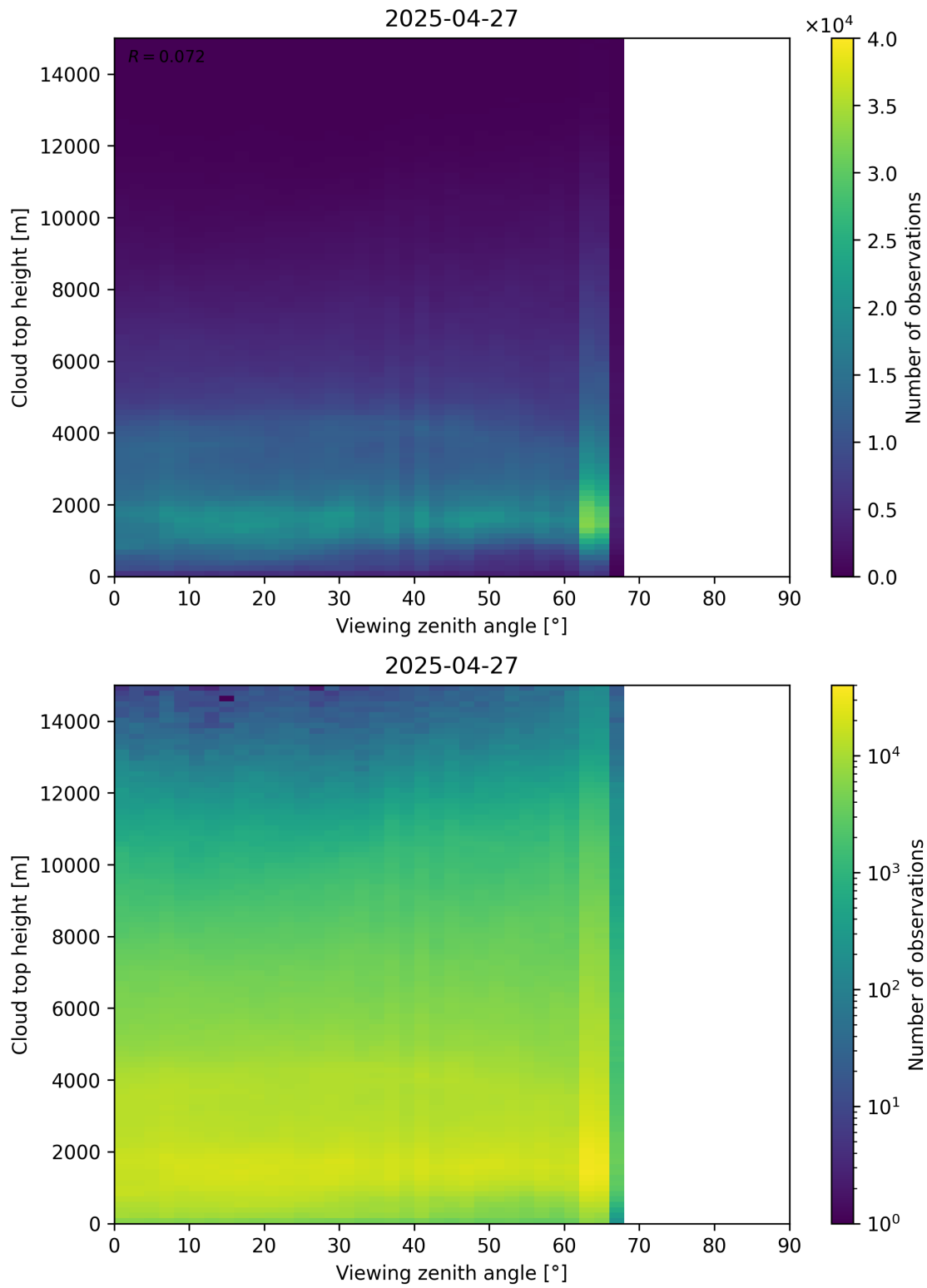
Figure 112: Scatter density plot of “Viewing zenith angle” against “Cloud top height” for 2025-04-26 to 2025-04-28.
