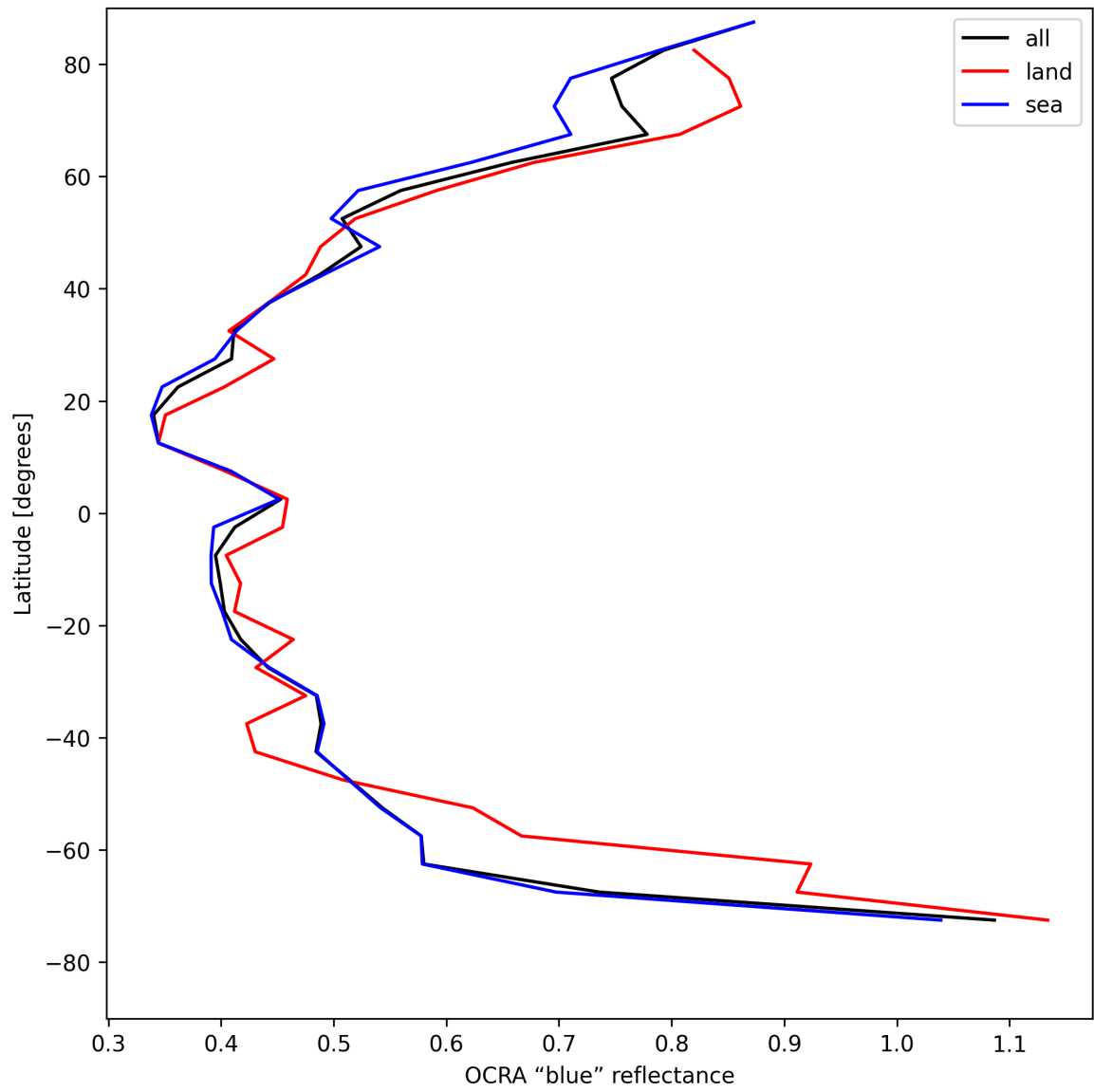
Figure 35: Zonal average of “OCRA “blue” reflectance” for 2025-04-26 to 2025-04-28.
