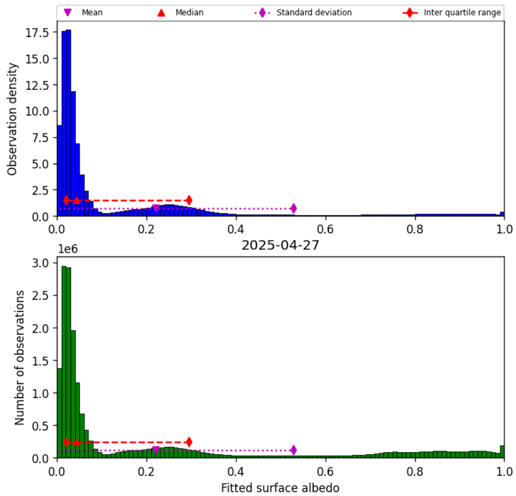
Figure 45: Histogram of “Fitted surface albedo” for 2025-04-26 to 2025-04-28
