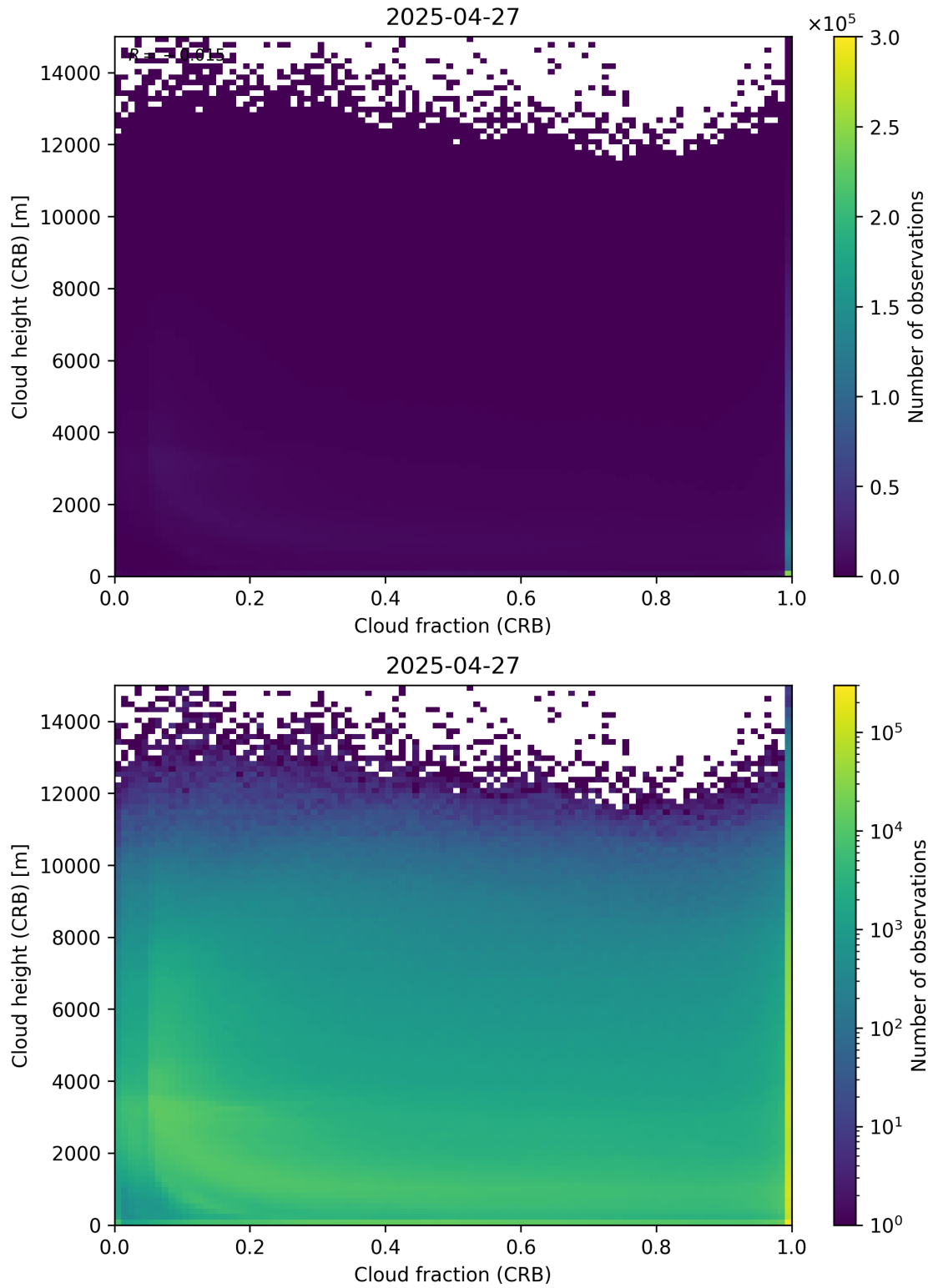
Figure 79: Scatter density plot of “Cloud fraction (CRB)” against “Cloud height (CRB)” for 2025-04-26 to 2025-04-28.
