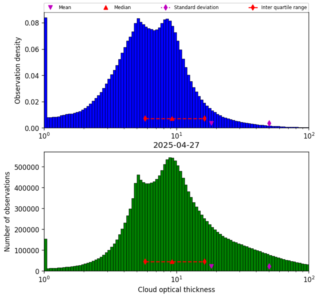
Figure 41: Histogram of “Cloud optical thickness” for 2025-04-26 to 2025-04-28
