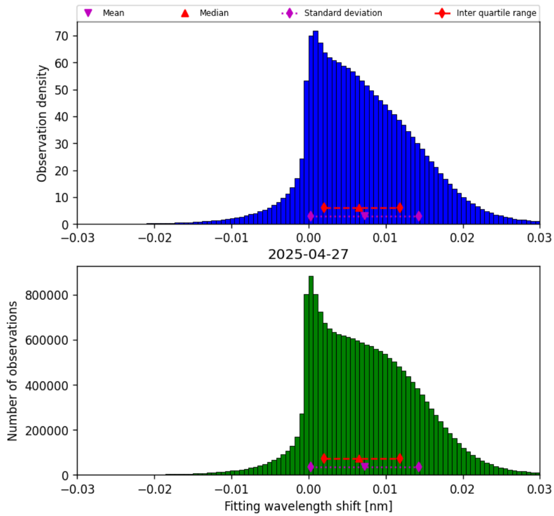
Figure 49: Histogram of “Fitting wavelength shift” for 2025-04-26 to 2025-04-28
