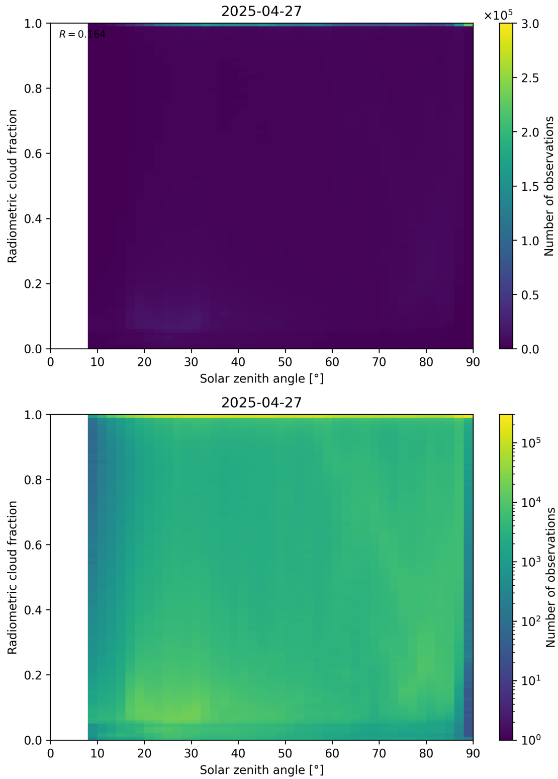
Figure 99: Scatter density plot of “Solar zenith angle” against “Radiometric cloud fraction” for 2025-04-26 to 2025-04-28.
