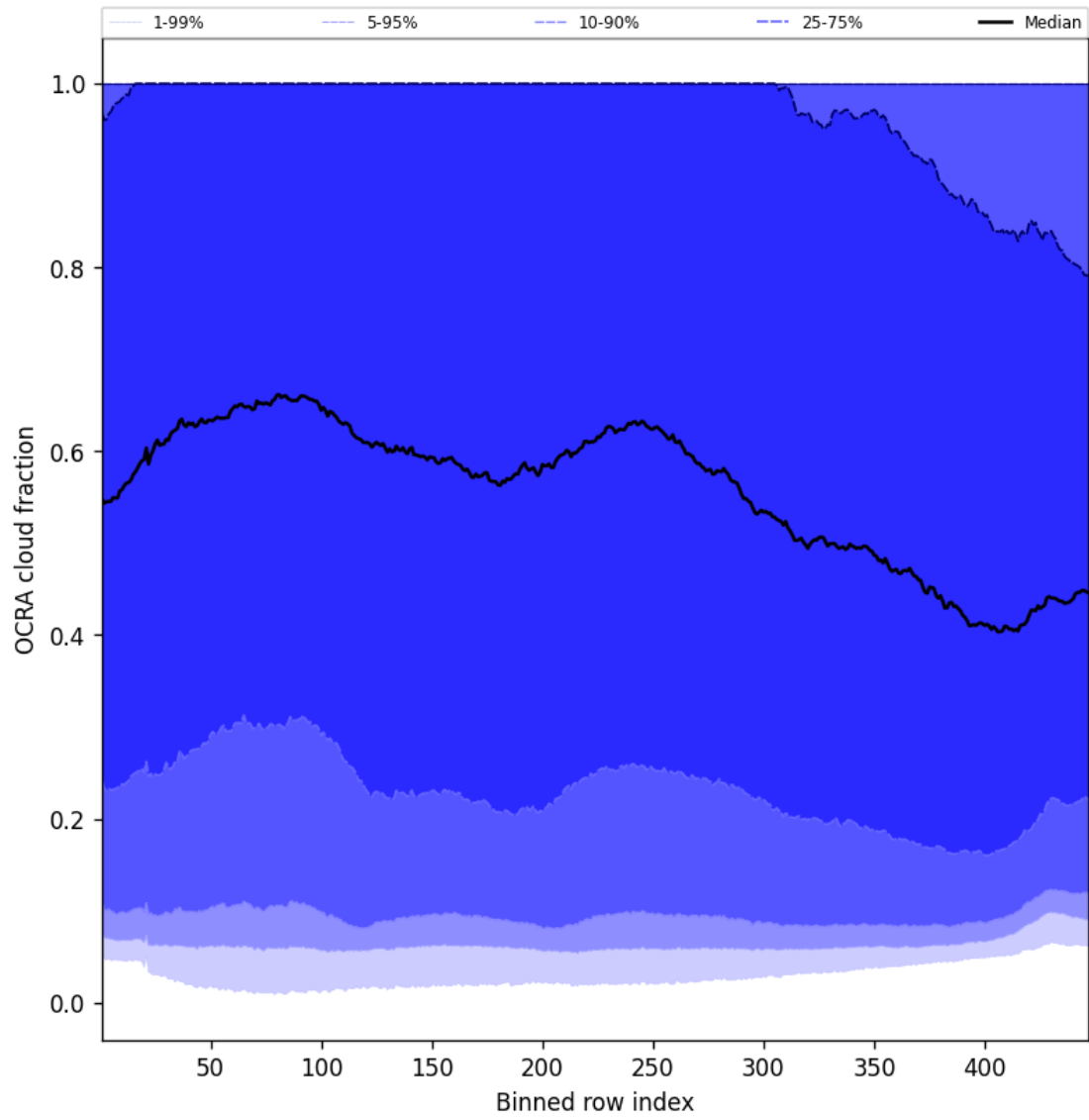
Figure 66: Along track statistics of “OCRA cloud fraction” for 2025-04-26 to 2025-04-28
