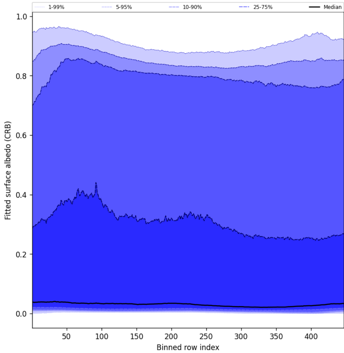
Figure 62: Along track statistics of “Fitted surface albedo (CRB)” for 2025-04-26 to 2025-04-28
