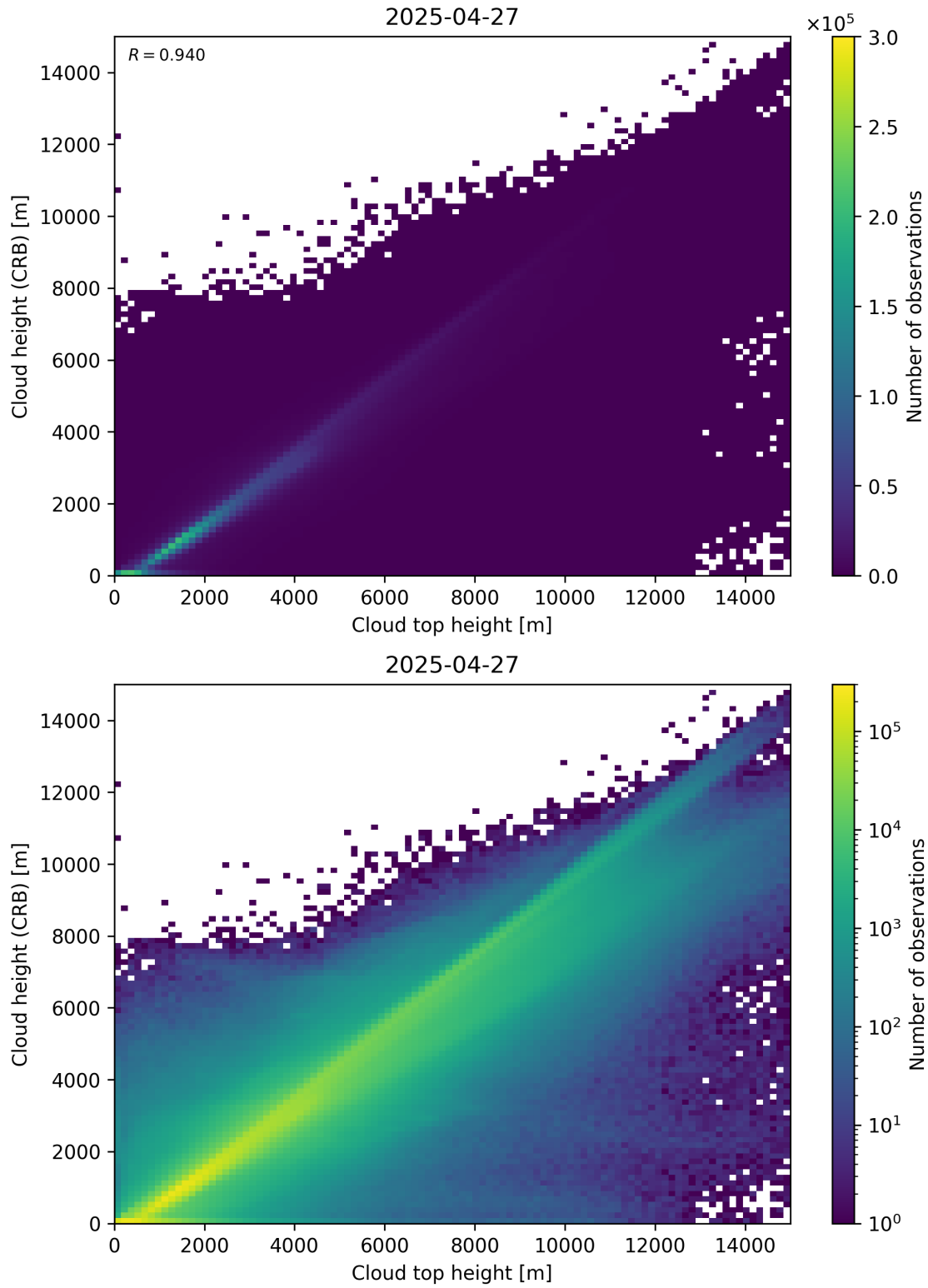
Figure 89: Scatter density plot of “Cloud top height” against “Cloud height (CRB)” for 2025-04-26 to 2025-04-28.
