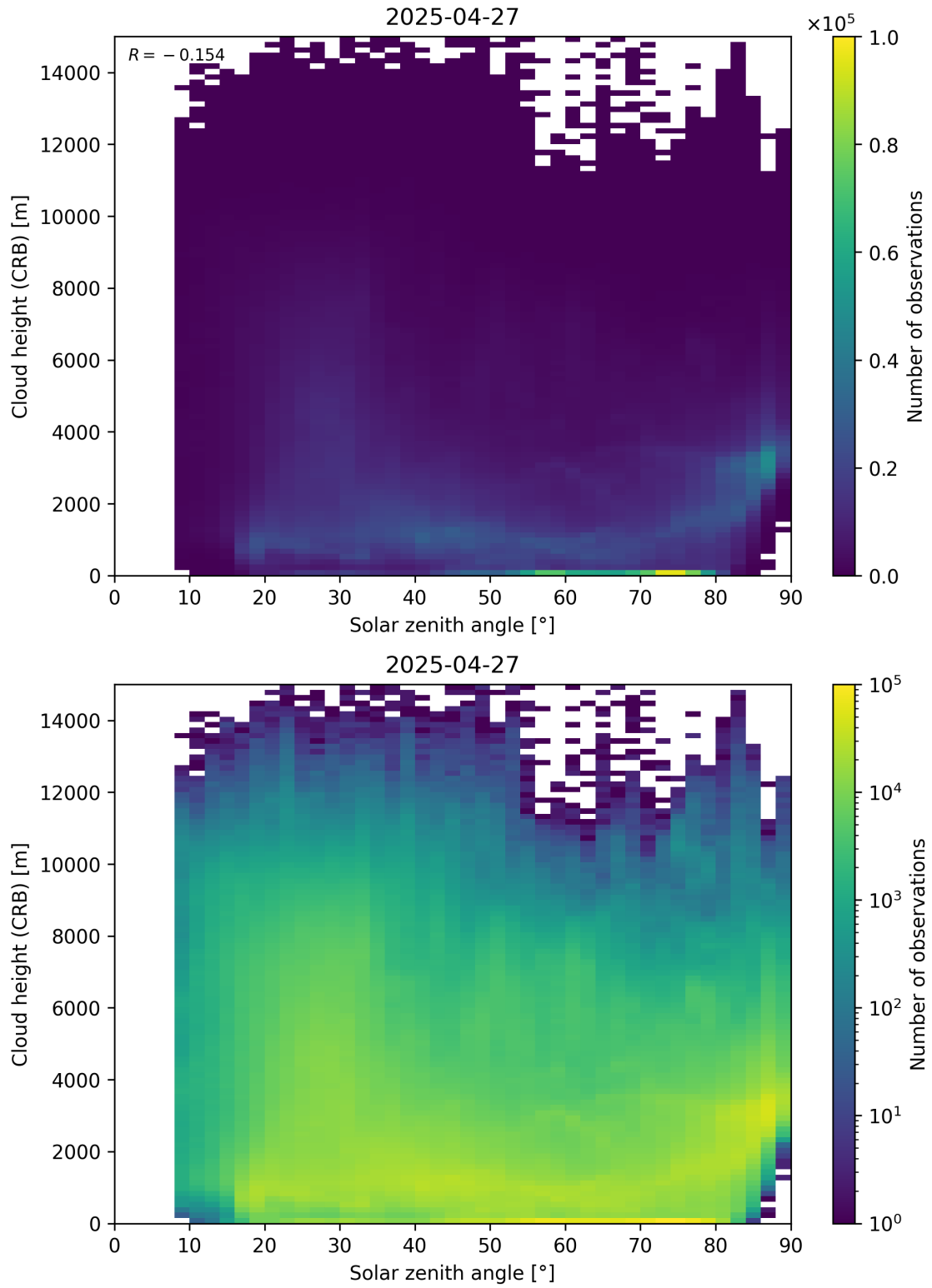
Figure 102: Scatter density plot of “Solar zenith angle” against “Cloud height (CRB)” for 2025-04-26 to 2025-04-28.
