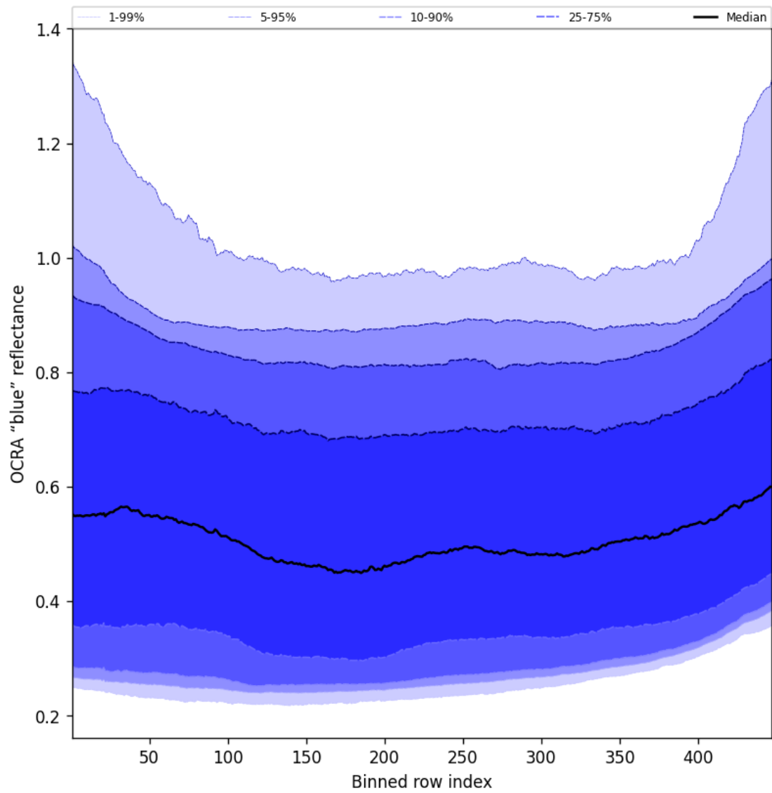
Figure 67: Along track statistics of “OCRA “blue” reflectance” for 2025-04-26 to 2025-04-28
