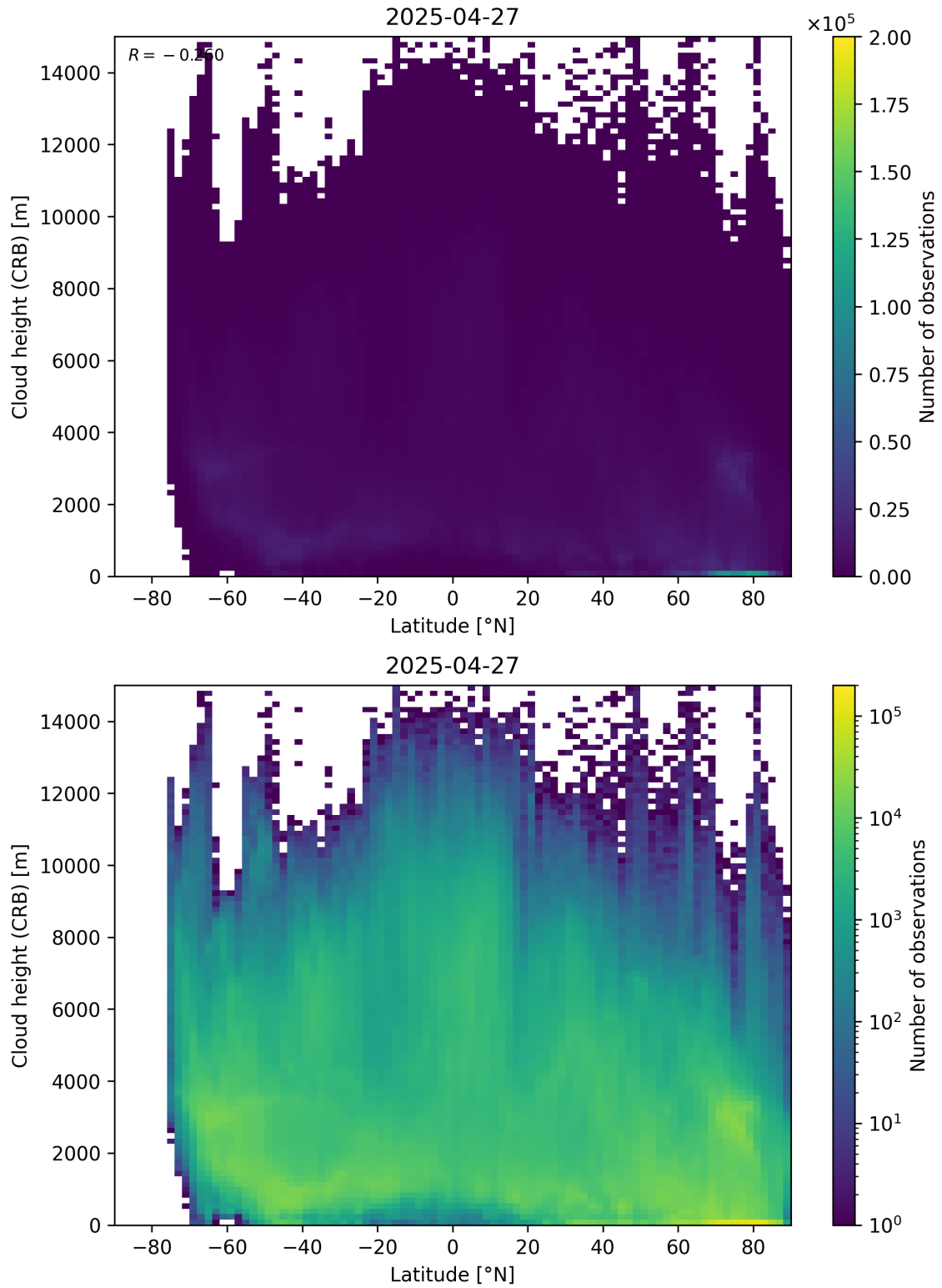
Figure 95: Scatter density plot of “Latitude” against “Cloud height (CRB)” for 2025-04-26 to 2025-04-28.
