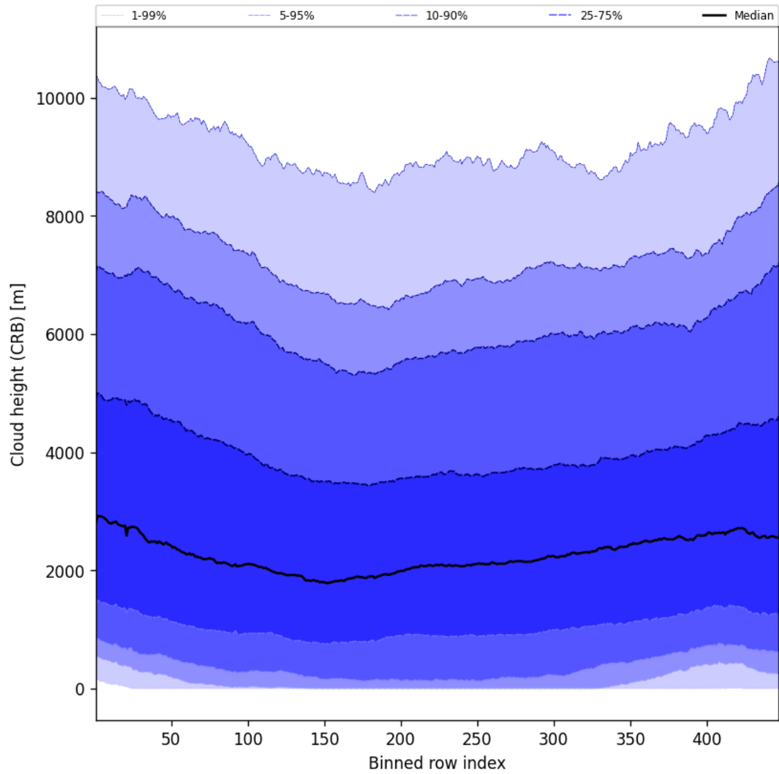
Figure 59: Along track statistics of “Cloud height (CRB)” for 2025-04-26 to 2025-04-28
