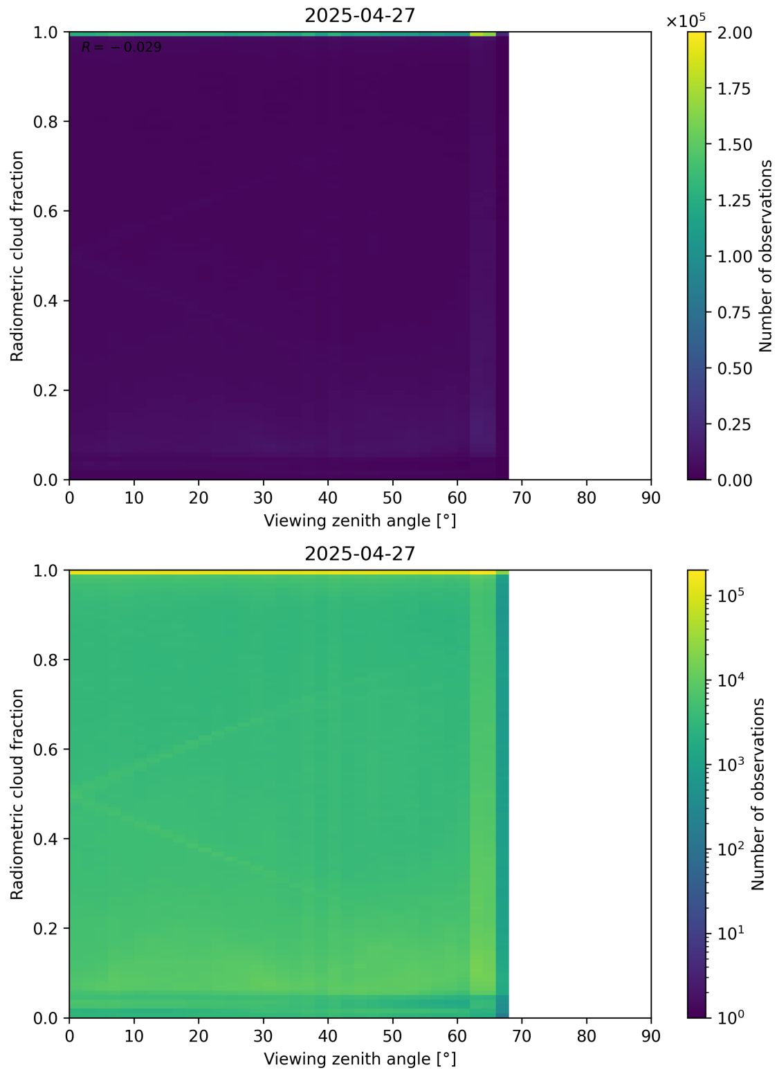
Figure 107: Scatter density plot of “Viewing zenith angle” against “Radiometric cloud fraction” for 2025-04-26 to 2025-04-28.
