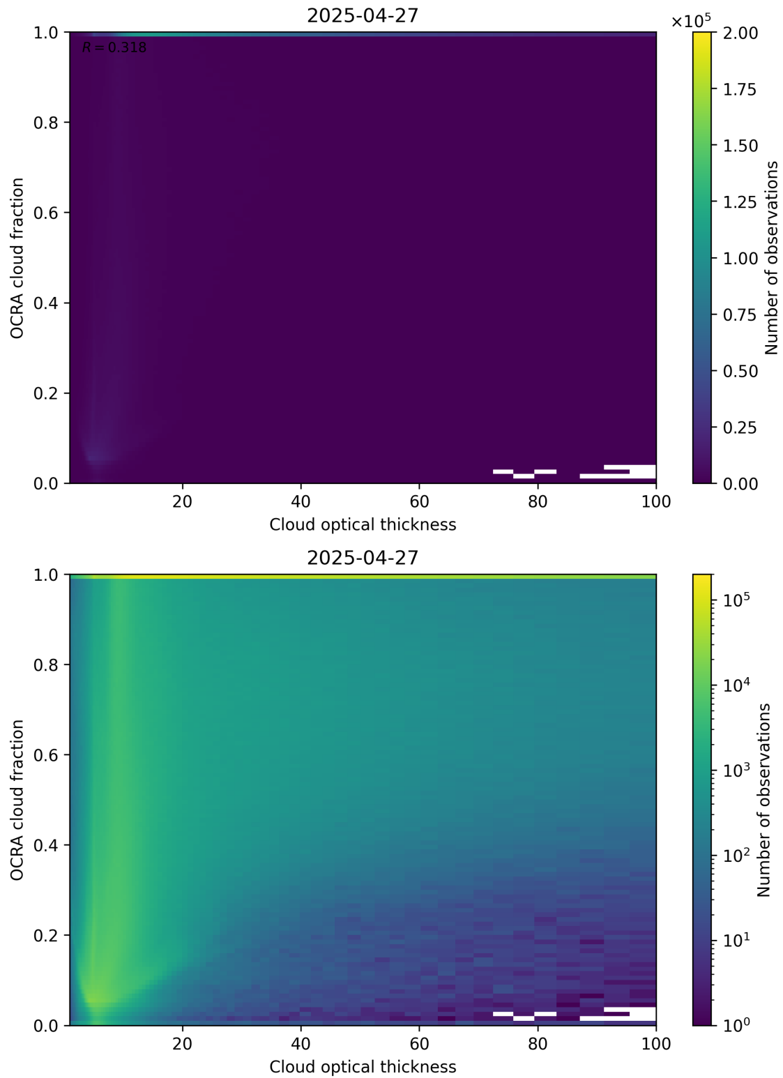
Figure 83: Scatter density plot of “Cloud optical thickness” against “OCRA cloud fraction” for 2025-04-26 to 2025-04-28.
