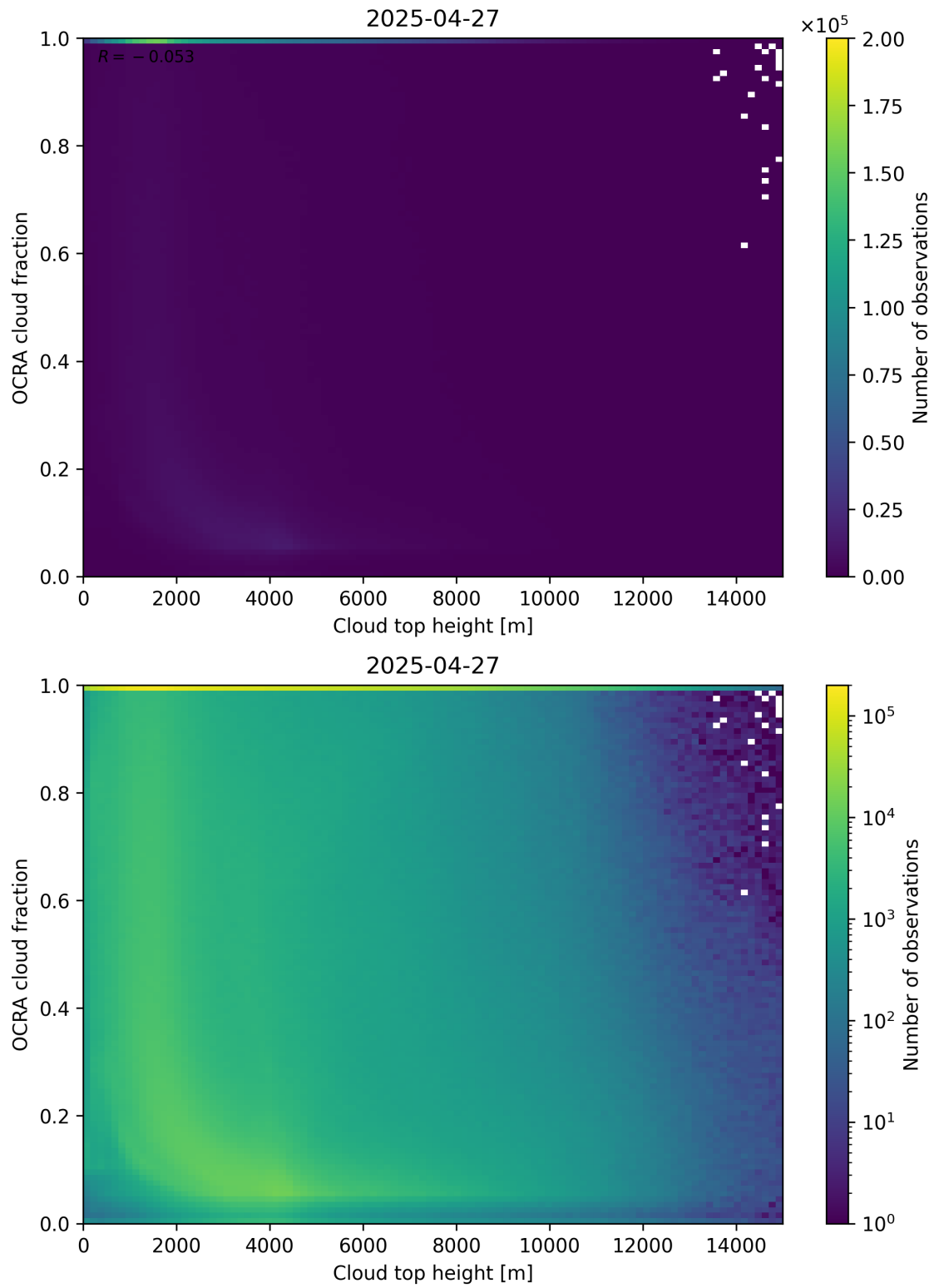
Figure 87: Scatter density plot of “Cloud top height” against “OCRA cloud fraction” for 2025-04-26 to 2025-04-28.
