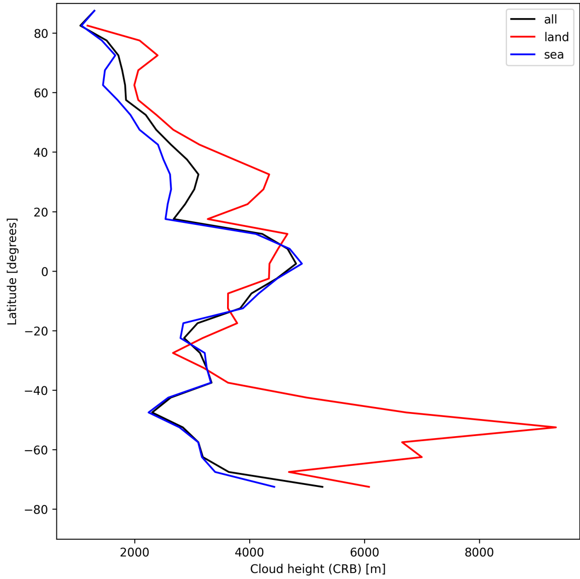
Figure 27: Zonal average of “Cloud height (CRB)” for 2025-04-26 to 2025-04-28.
