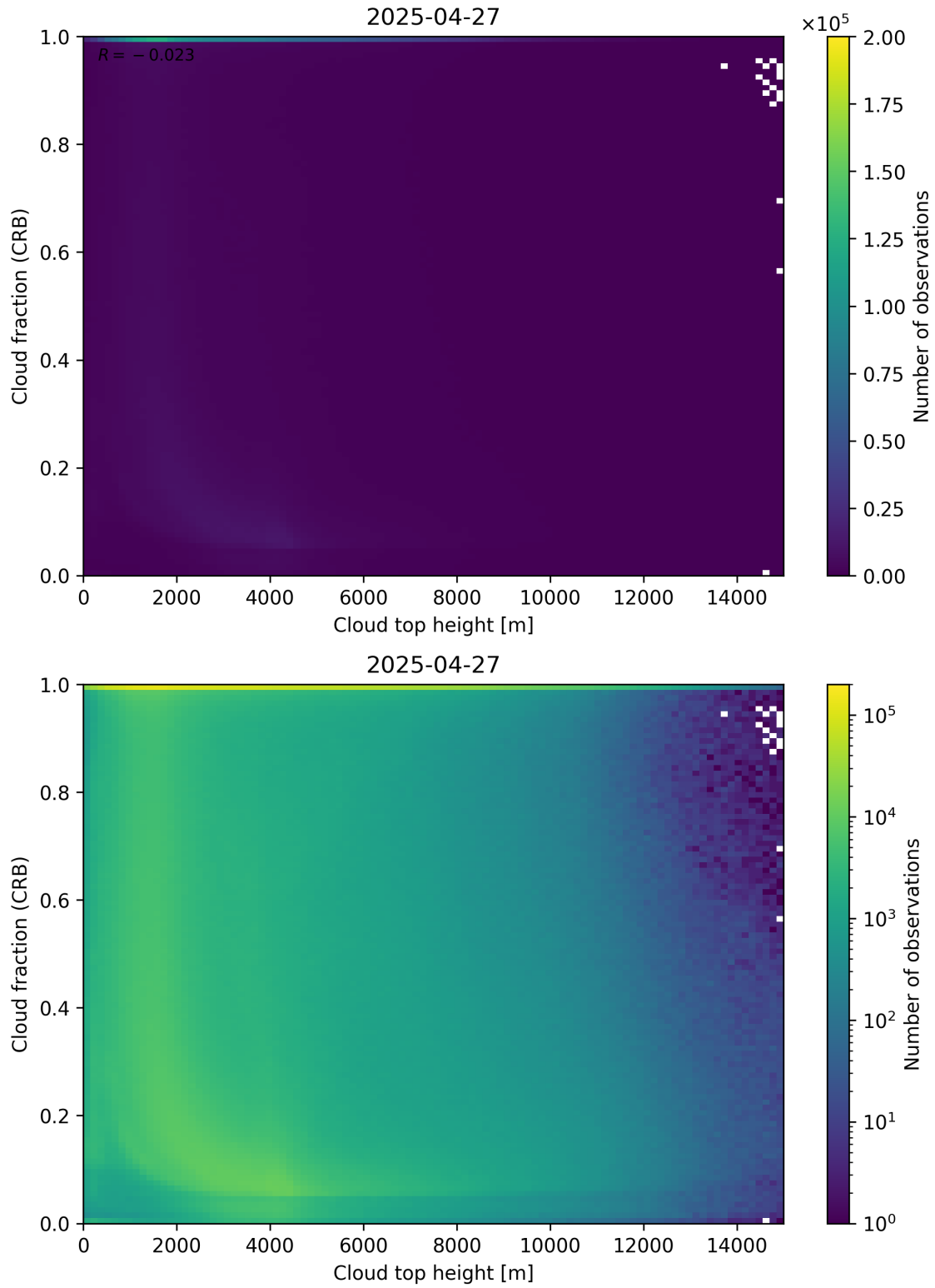
Figure 88: Scatter density plot of “Cloud top height” against “Cloud fraction (CRB)” for 2025-04-26 to 2025-04-28.
