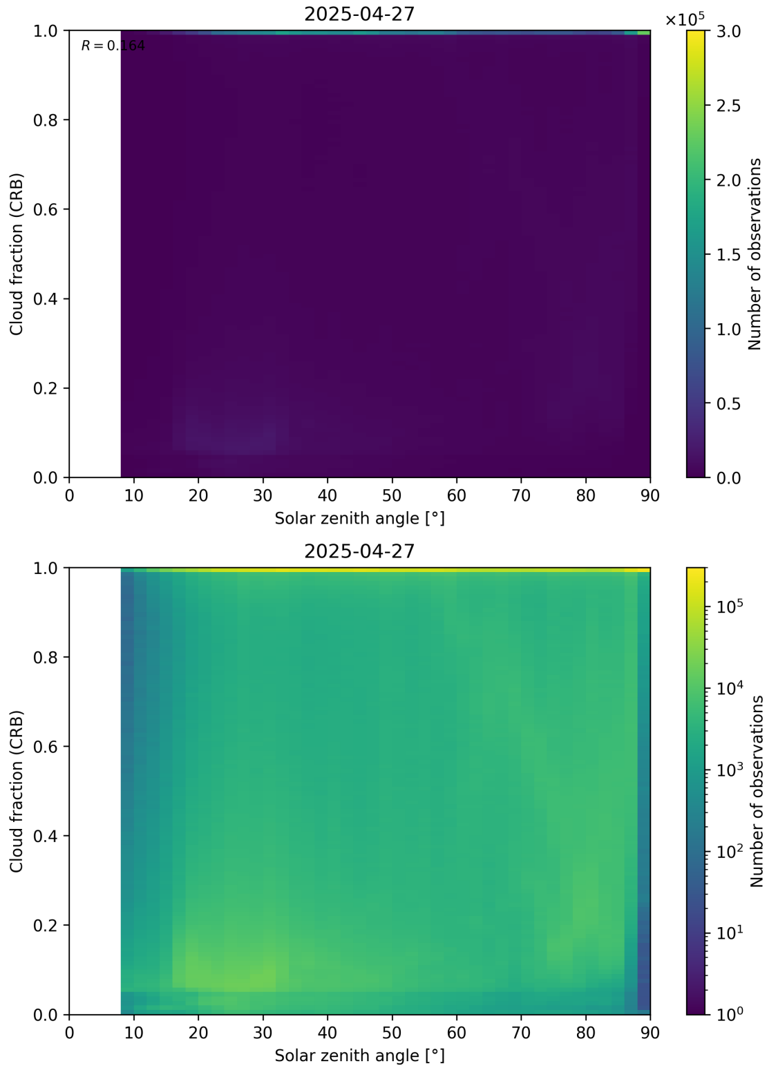
Figure 101: Scatter density plot of “Solar zenith angle” against “Cloud fraction (CRB)” for 2025-04-26 to 2025-04-28.
