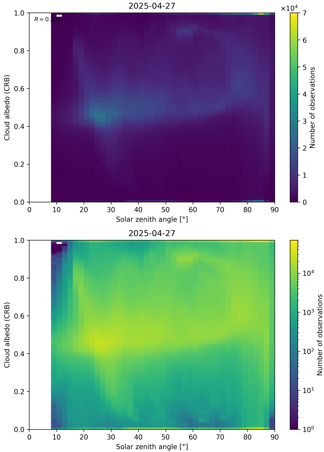
Figure 98: Scatter density plot of “Solar zenith angle” against “Cloud albedo (CRB)” for 2025-04-26 to 2025-04-28.
