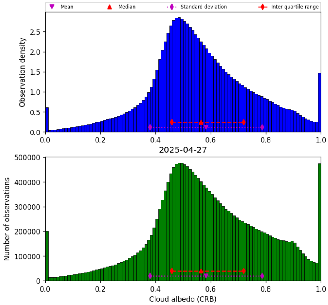
Figure 44: Histogram of “Cloud albedo (CRB)” for 2025-04-26 to 2025-04-28
