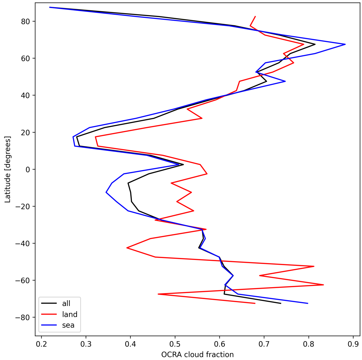
Figure 34: Zonal average of “OCRA cloud fraction” for 2025-04-26 to 2025-04-28.
