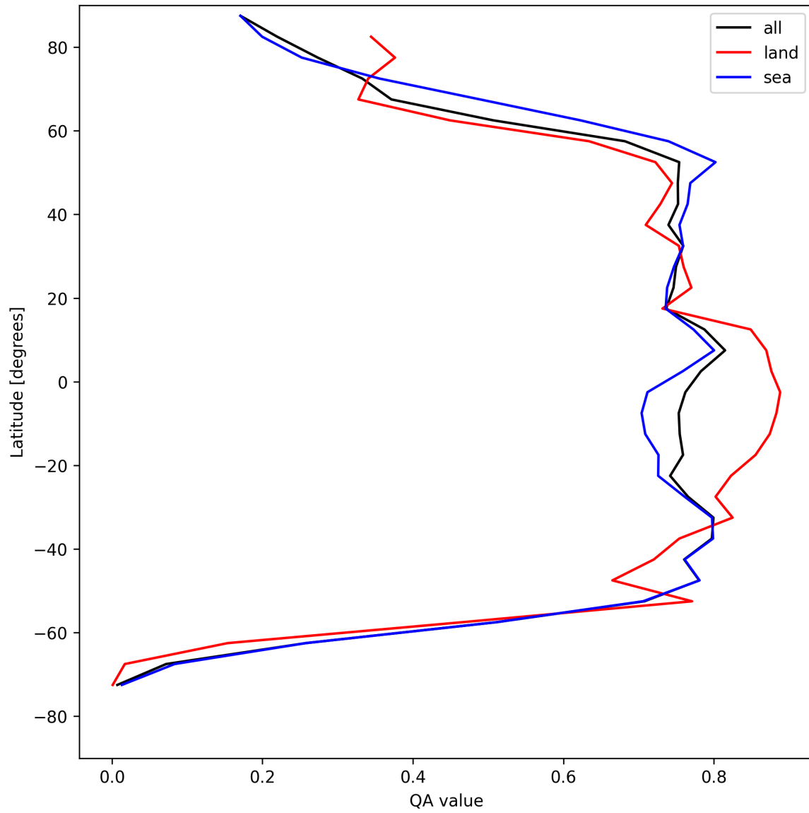
Figure 22: Zonal average of “QA value” for 2025-04-26 to 2025-04-28.
