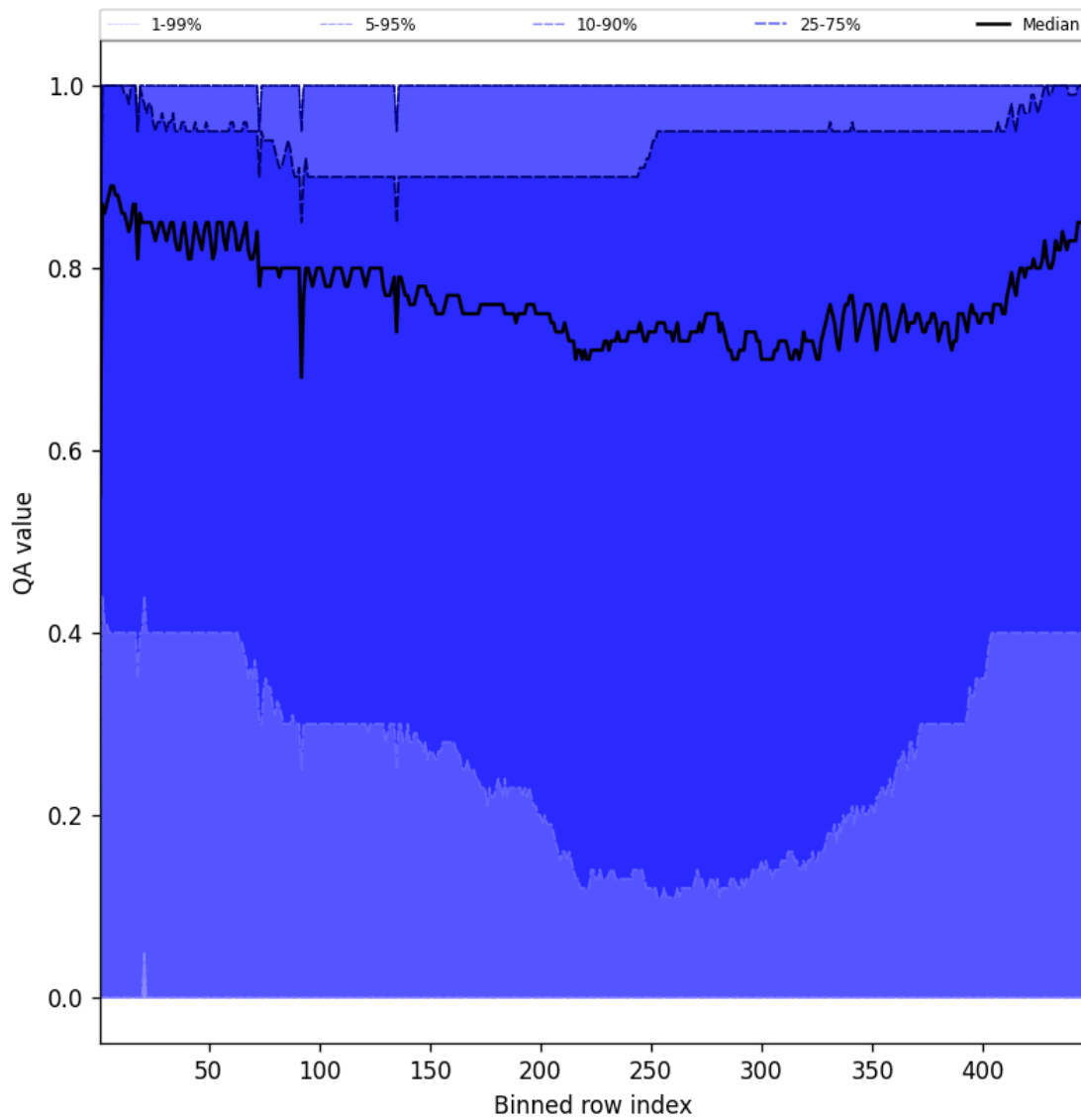
Figure 54: Along track statistics of “QA value” for 2025-04-26 to 2025-04-28
