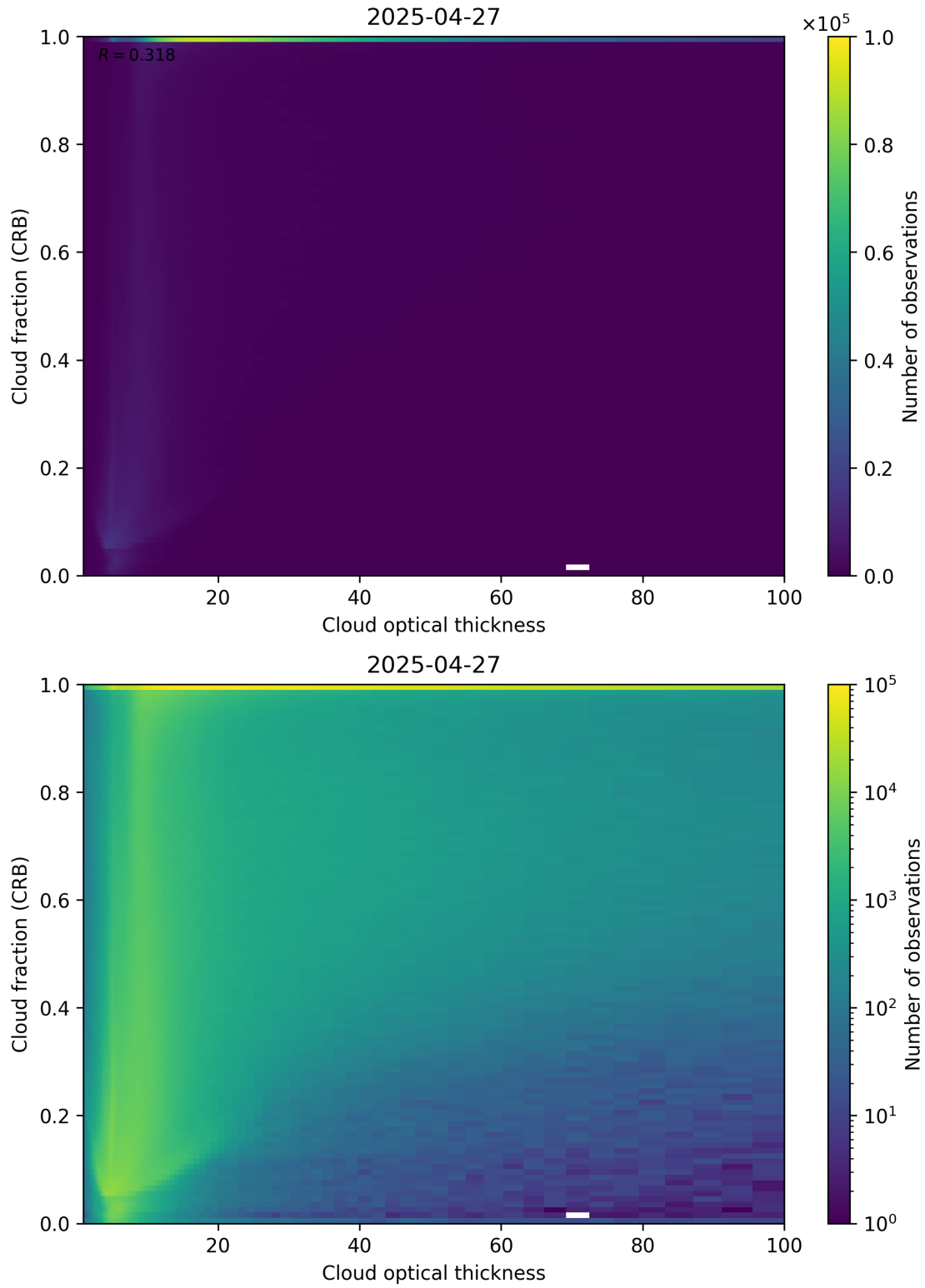
Figure 84: Scatter density plot of “Cloud optical thickness” against “Cloud fraction (CRB)” for 2025-04-26 to 2025-04-28.
