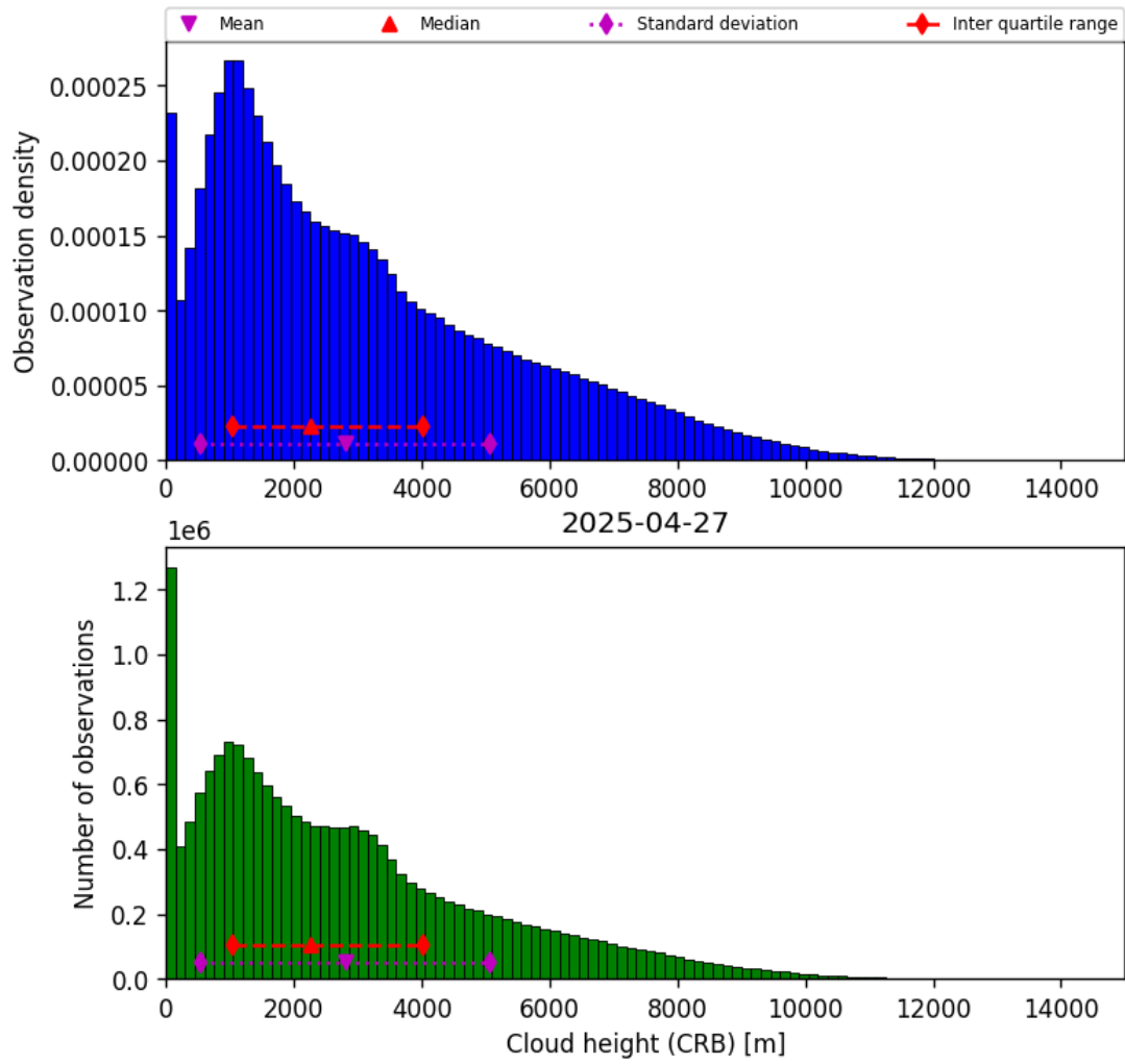
Figure 43: Histogram of “Cloud height (CRB)” for 2025-04-26 to 2025-04-28
