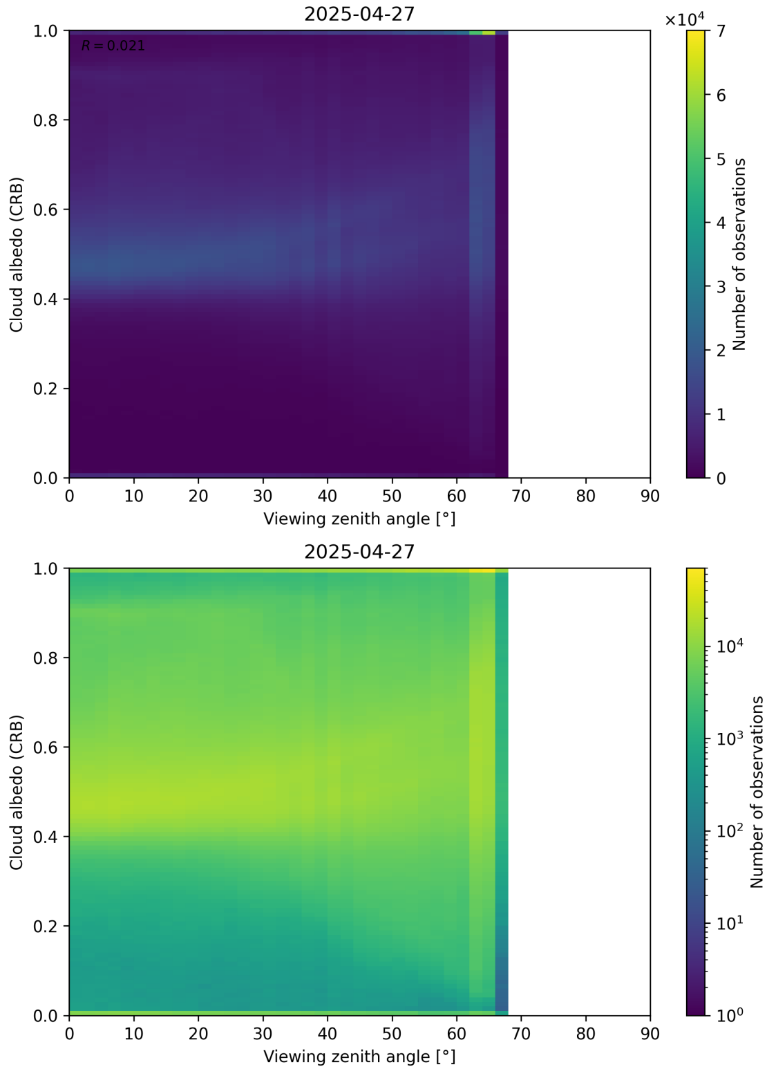
Figure 106: Scatter density plot of “Viewing zenith angle” against “Cloud albedo (CRB)” for 2025-04-26 to 2025-04-28.
