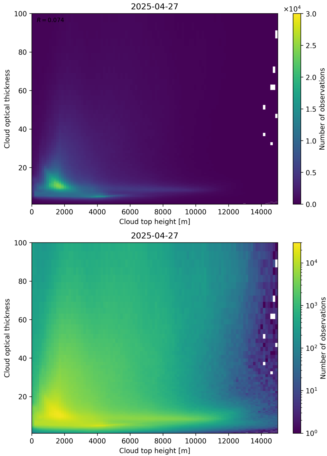
Figure 90: Scatter density plot of “Cloud top height” against “Cloud optical thickness” for 2025-04-26 to 2025-04-28.
