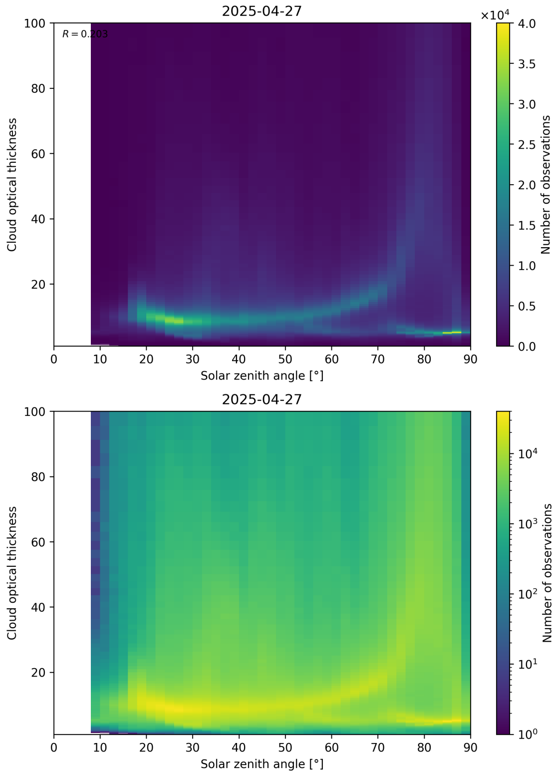
Figure 103: Scatter density plot of “Solar zenith angle” against “Cloud optical thickness” for 2025-04-26 to 2025-04-28.
