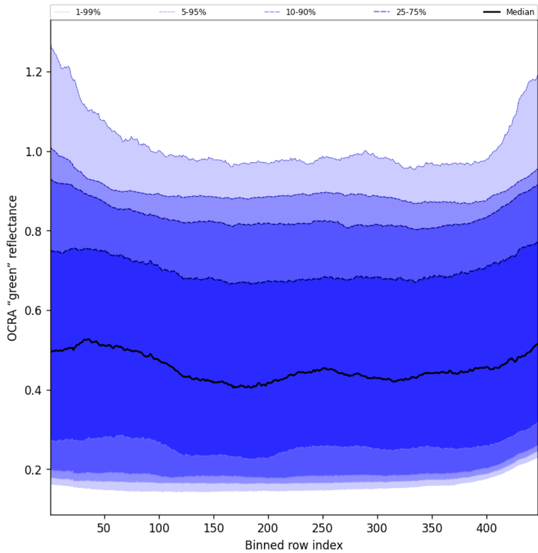
Figure 68: Along track statistics of "OCRA "green" reflectance" for 2025-04-26 to 2025-04-28
