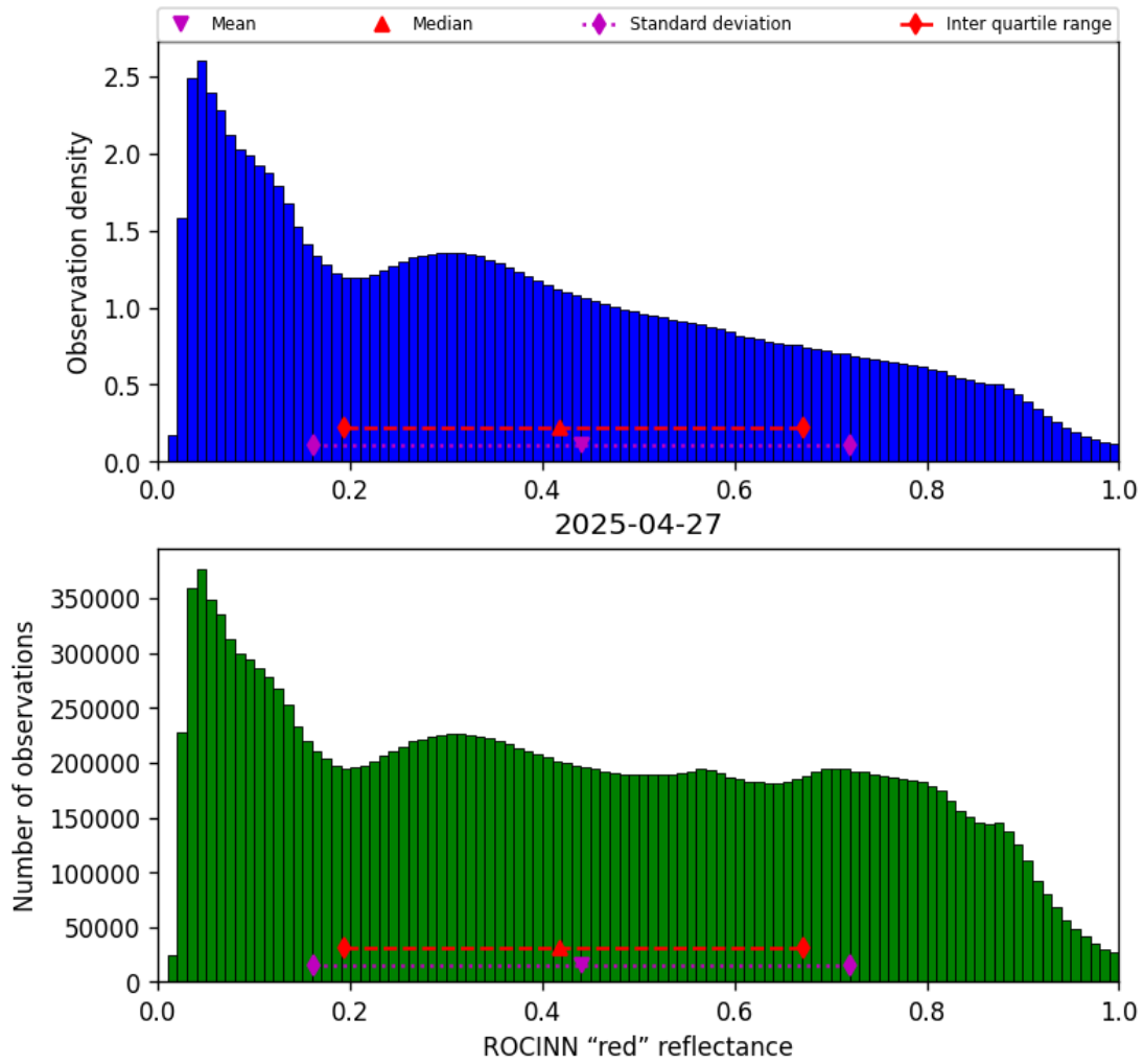
Figure 53: Histogram of “ROCINN “red” reflectance” for 2025-04-26 to 2025-04-28
