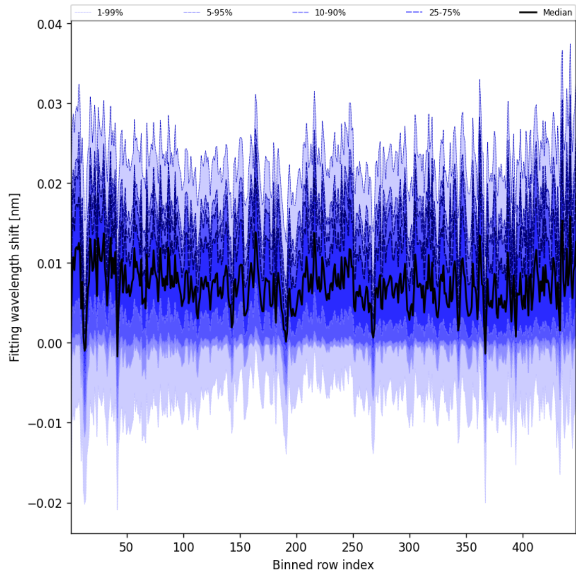
Figure 65: Along track statistics of “Fitting wavelength shift” for 2025-04-26 to 2025-04-28
