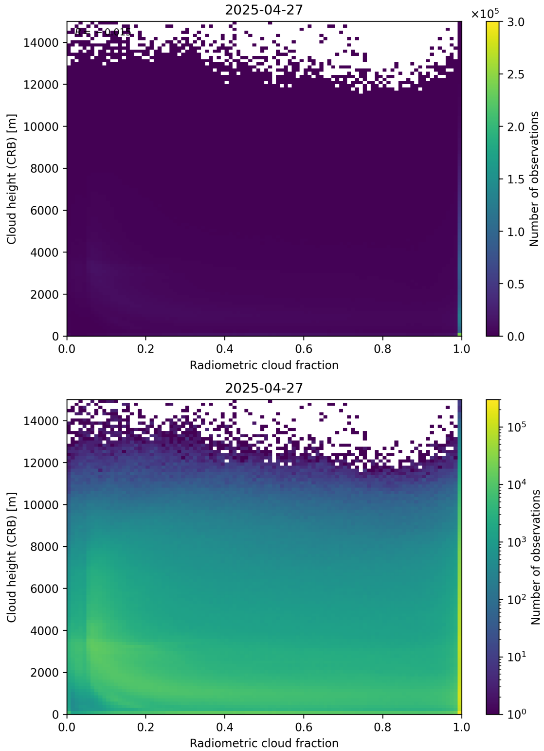
Figure 74: Scatter density plot of “Radiometric cloud fraction” against “Cloud height (CRB)” for 2025-04-26 to 2025-04-28.
