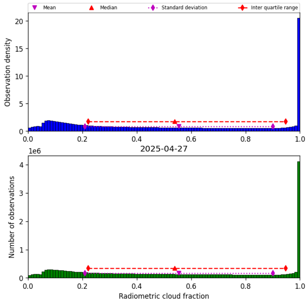
Figure 39: Histogram of “Radiometric cloud fraction” for 2025-04-26 to 2025-04-28
