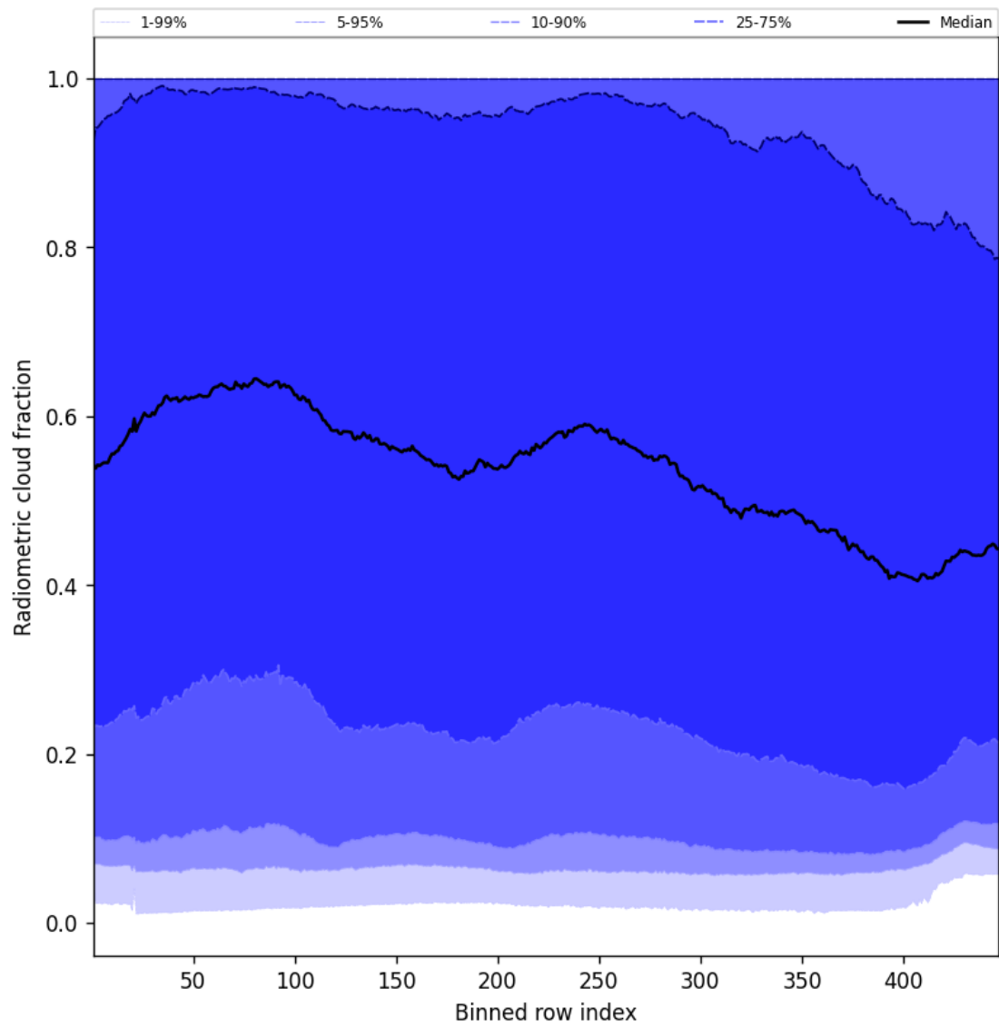
Figure 55: Along track statistics of “Radiometric cloud fraction” for 2025-04-26 to 2025-04-28
