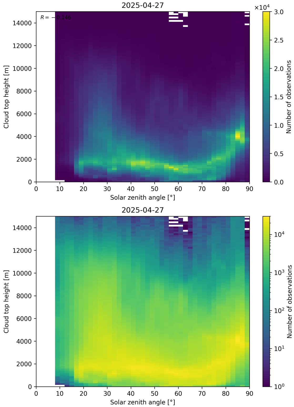
Figure 104: Scatter density plot of “Solar zenith angle” against “Cloud top height” for 2025-04-26 to 2025-04-28.
