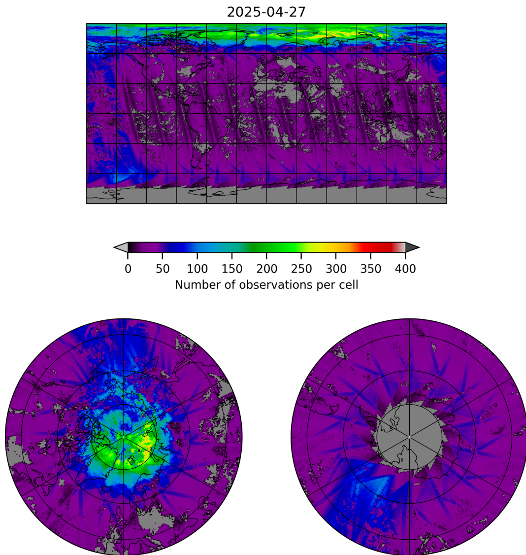
Figure 21: Map of the number of observations for 2025-04-26 to 2025-04-28
