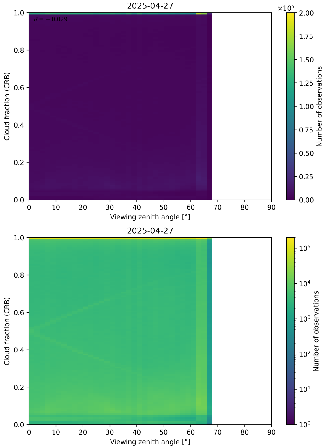
Figure 109: Scatter density plot of “Viewing zenith angle” against “Cloud fraction (CRB)” for 2025-04-26 to 2025-04-28.
