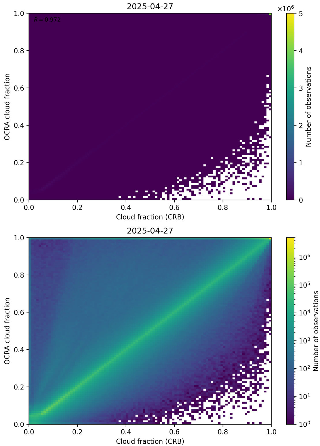
Figure 78: Scatter density plot of “Cloud fraction (CRB)” against “OCRA cloud fraction” for 2025-04-26 to 2025-04-28.
