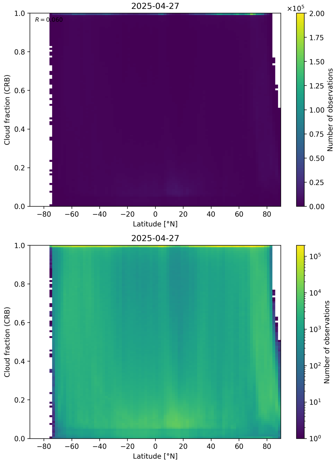
Figure 94: Scatter density plot of “Latitude” against “Cloud fraction (CRB)” for 2025-04-26 to 2025-04-28.
