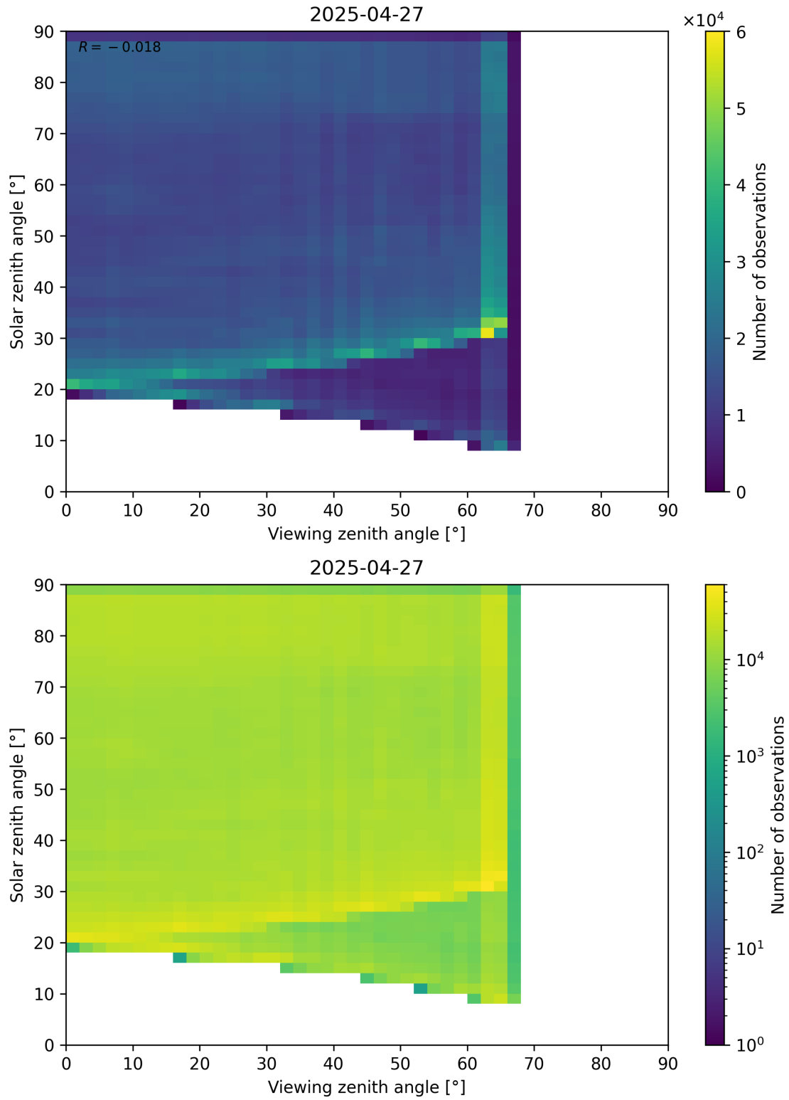
Figure 114: Scatter density plot of “Viewing zenith angle” against “Solar zenith angle” for 2025-04-26 to 2025-04-28.
