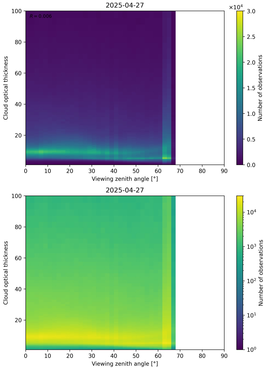
Figure 111: Scatter density plot of “Viewing zenith angle” against “Cloud optical thickness” for 2025-04-26 to 2025-04-28.
