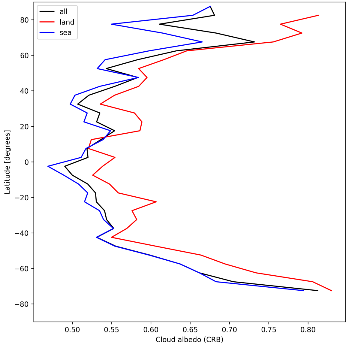
Figure 28: Zonal average of “Cloud albedo (CRB)” for 2025-04-26 to 2025-04-28.
