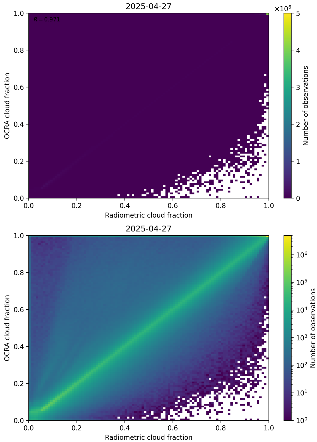
Figure 72: Scatter density plot of “Radiometric cloud fraction” against “OCRA cloud fraction” for 2025-04-26 to 2025-04-28.
