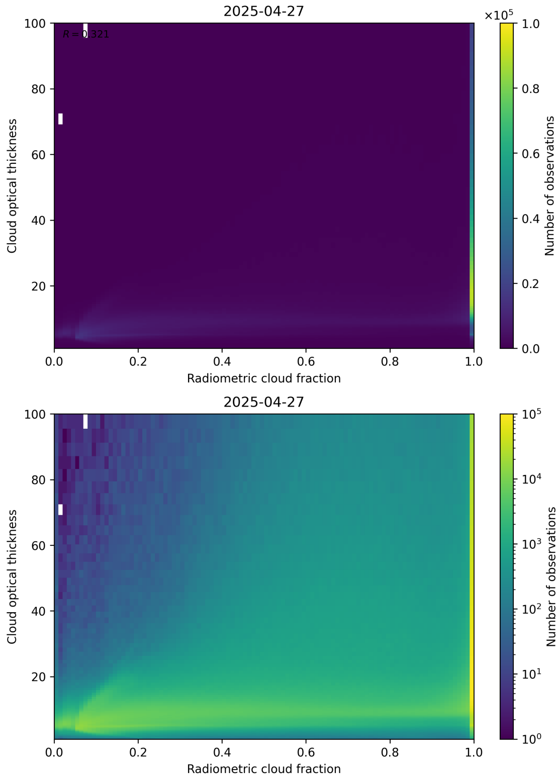
Figure 75: Scatter density plot of “Radiometric cloud fraction” against “Cloud optical thickness” for 2025-04-26 to 2025-04-28.
