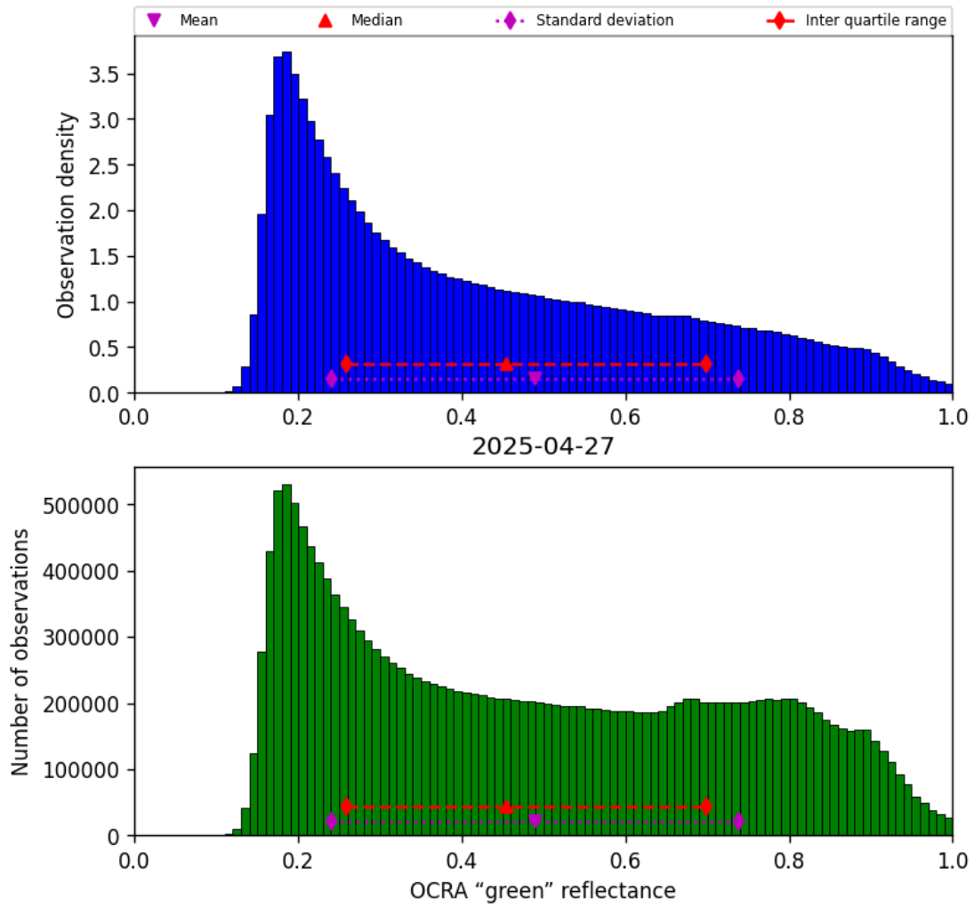
Figure 52: Histogram of “OCRA “green” reflectance” for 2025-04-26 to 2025-04-28
