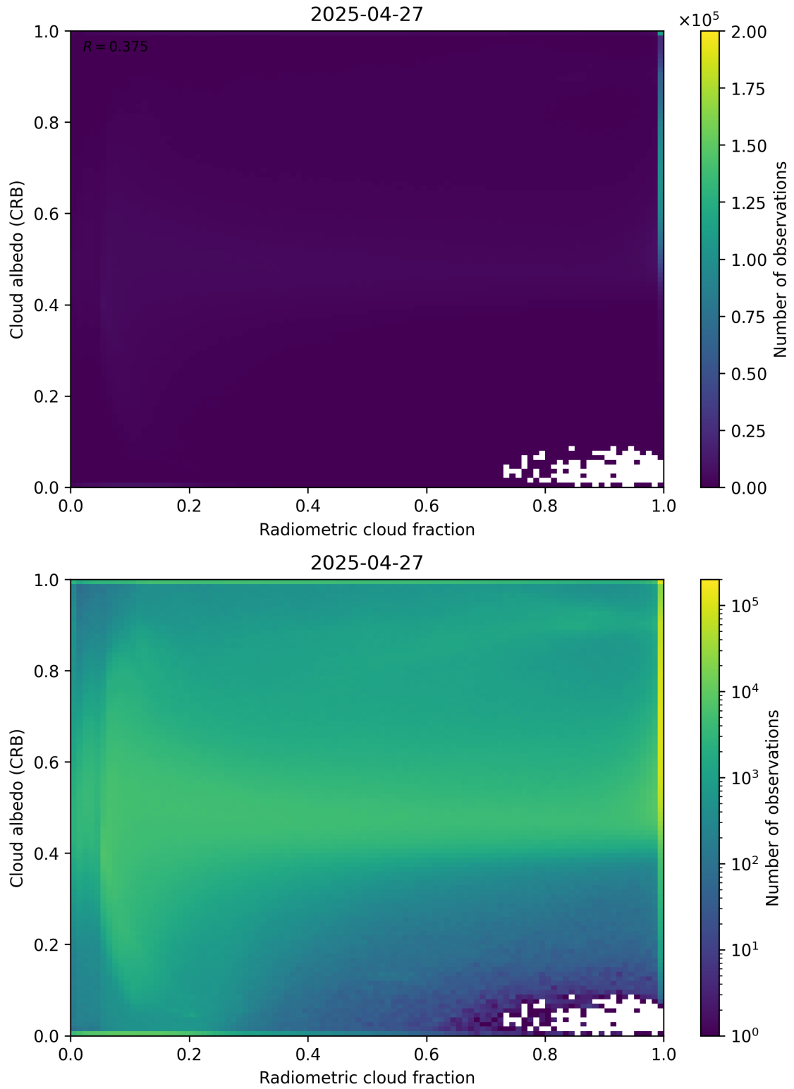
Figure 71: Scatter density plot of “Radiometric cloud fraction” against “Cloud albedo (CRB)” for 2025-04-26 to 2025-04-28.
