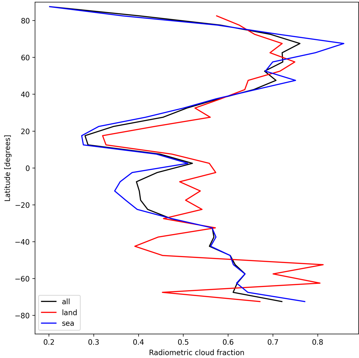
Figure 23: Zonal average of “Radiometric cloud fraction” for 2025-04-26 to 2025-04-28.
