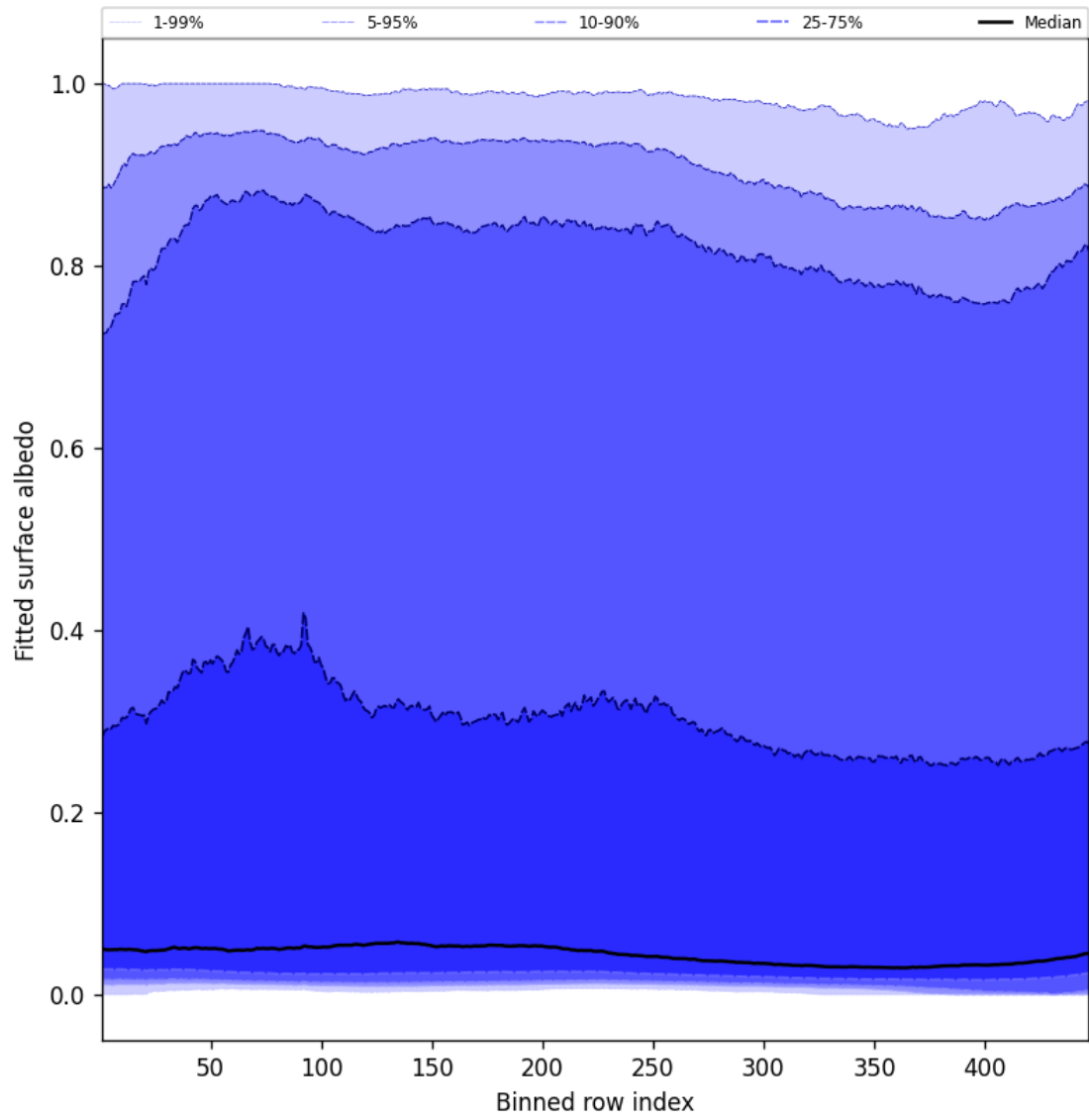
Figure 61: Along track statistics of “Fitted surface albedo” for 2025-04-26 to 2025-04-28
