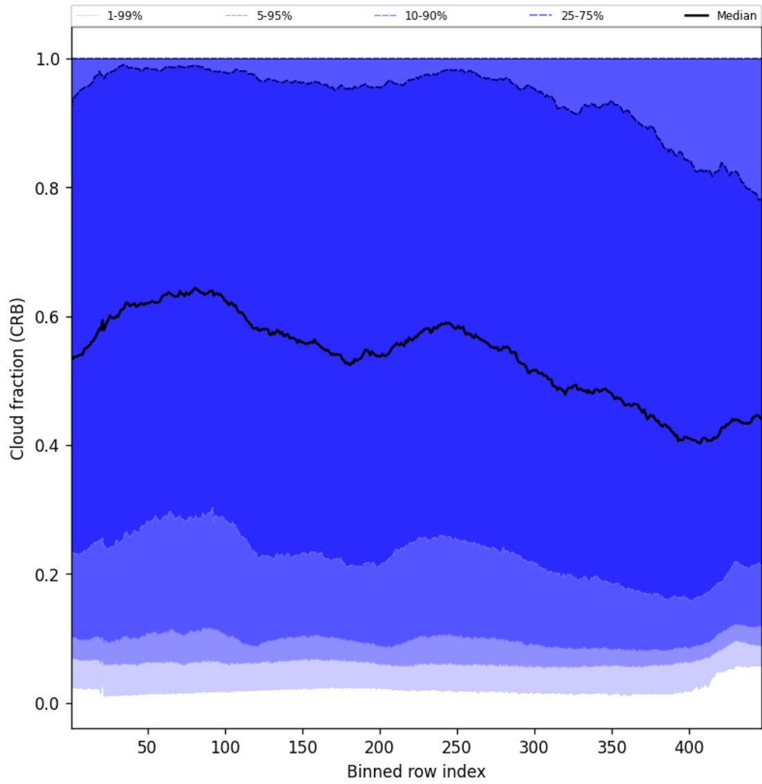
Figure 58: Along track statistics of “Cloud fraction (CRB)” for 2025-04-26 to 2025-04-28
