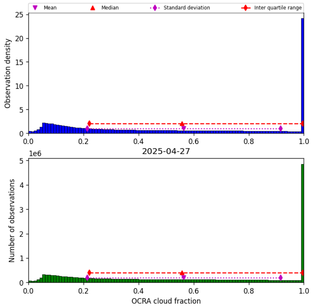
Figure 50: Histogram of “OCRA cloud fraction” for 2025-04-26 to 2025-04-28
