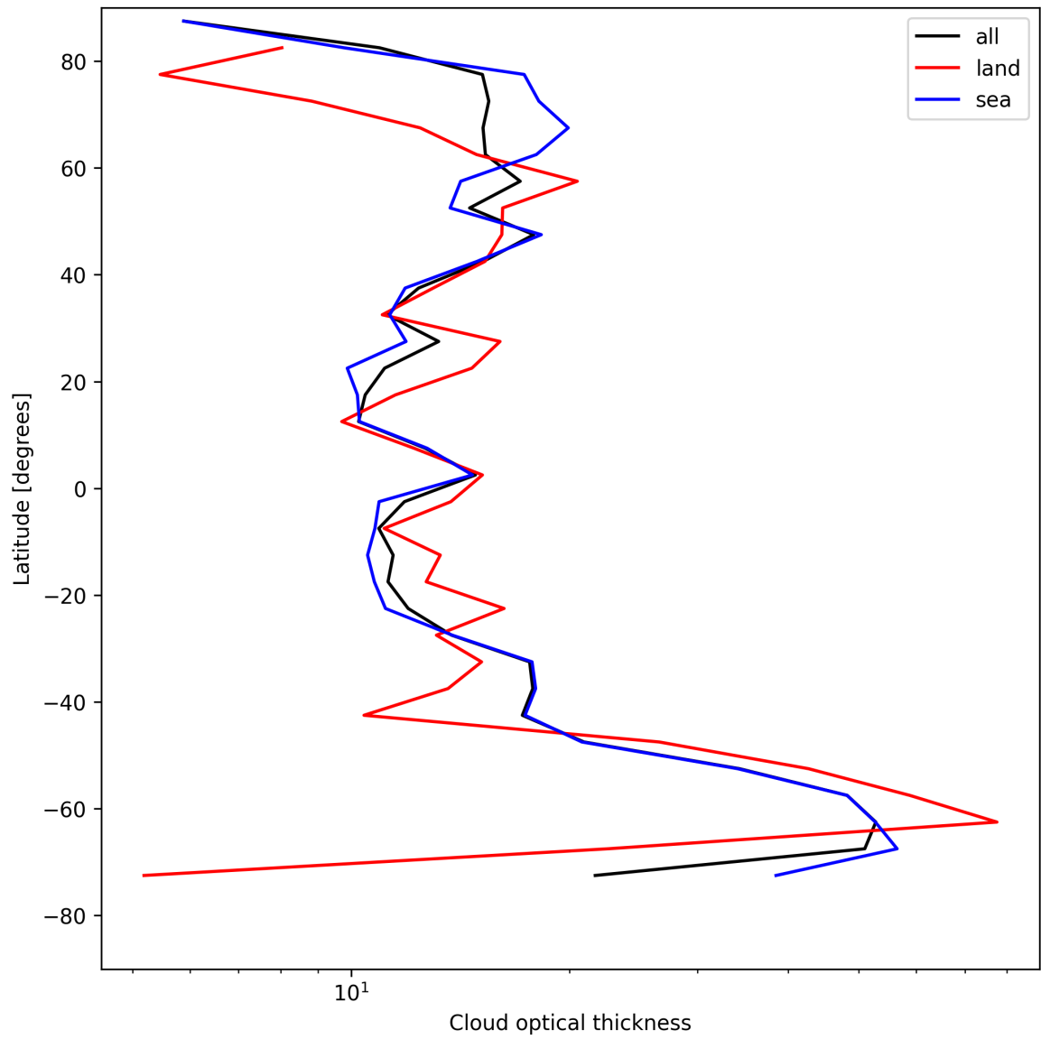
Figure 25: Zonal average of “Cloud optical thickness” for 2025-04-26 to 2025-04-28.
