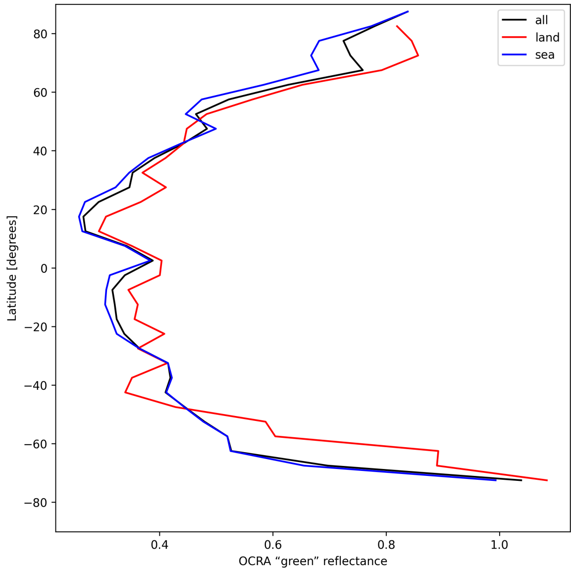
Figure 36: Zonal average of “OCRA “green” reflectance” for 2025-04-26 to 2025-04-28.
