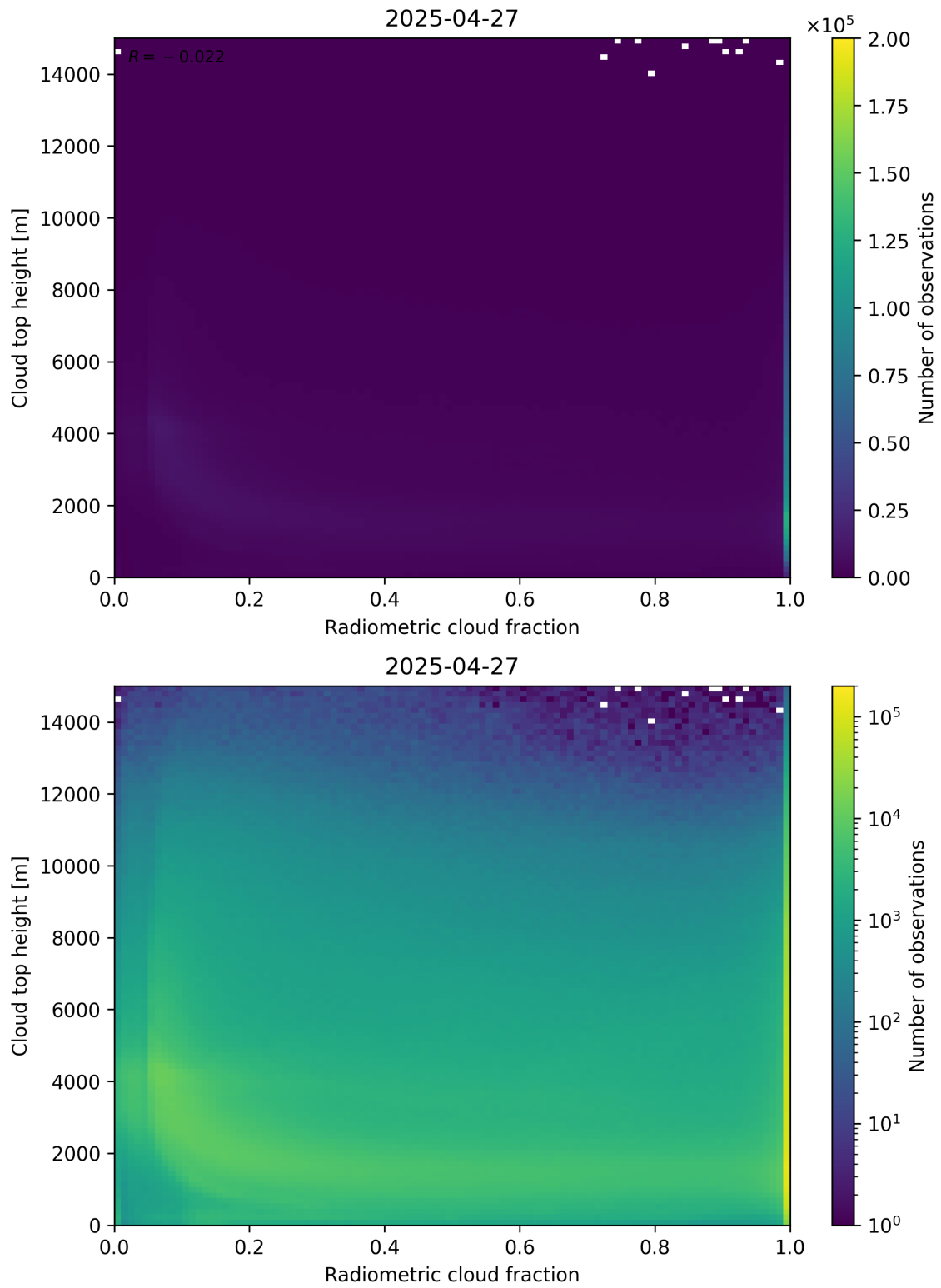
Figure 76: Scatter density plot of “Radiometric cloud fraction” against “Cloud top height” for 2025-04-26 to 2025-04-28.
