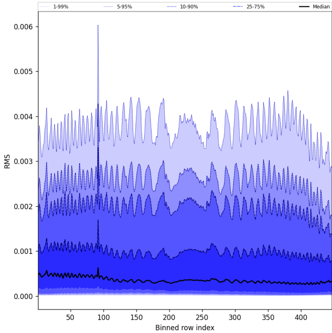
Figure 63: Along track statistics of “RMS” for 2025-04-26 to 2025-04-28
