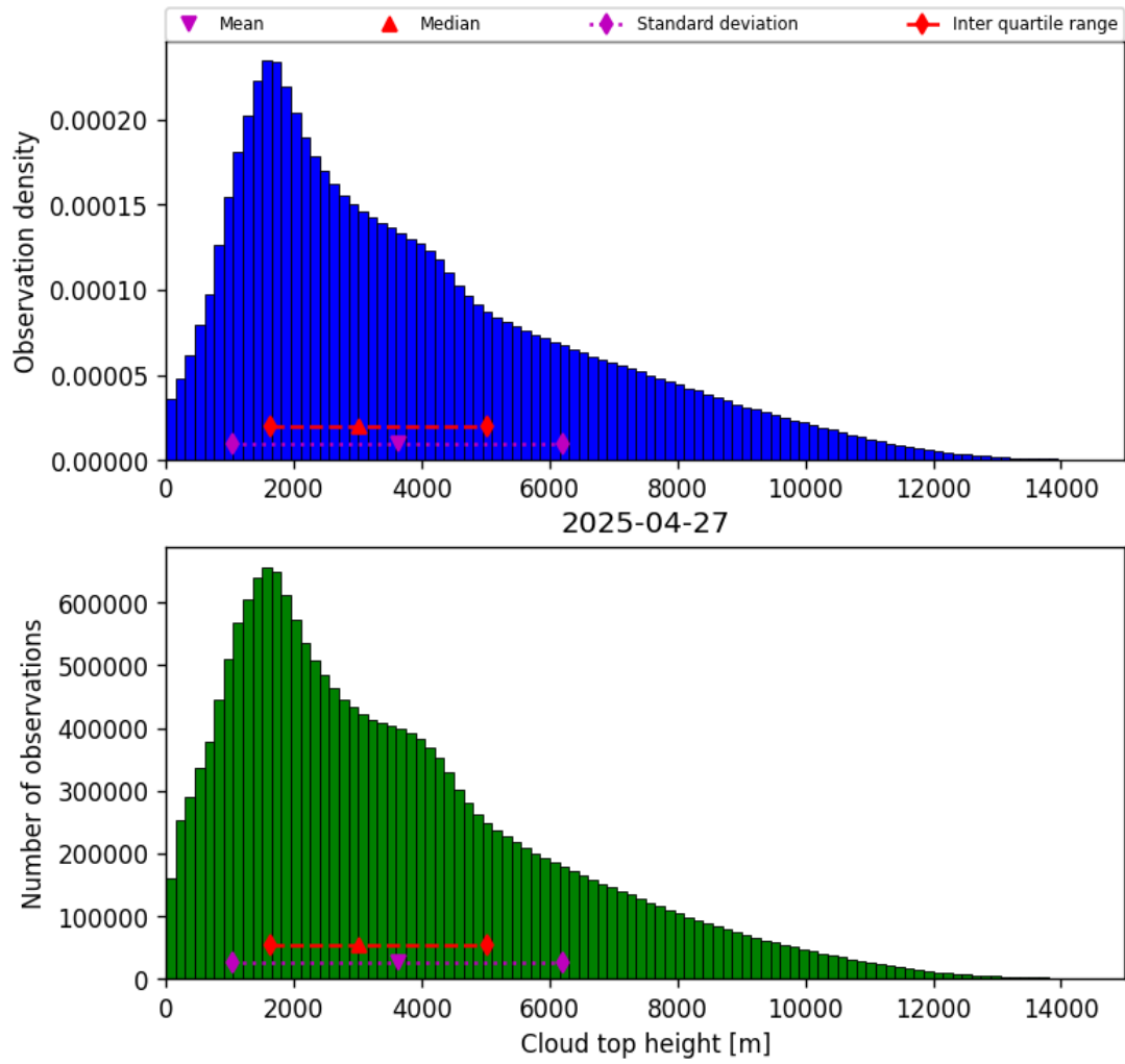
Figure 40: Histogram of “Cloud top height” for 2025-04-26 to 2025-04-28
