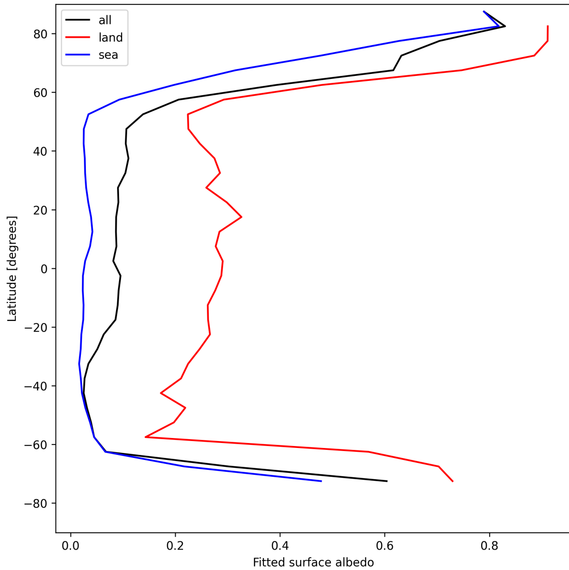
Figure 29: Zonal average of “Fitted surface albedo” for 2025-04-26 to 2025-04-28.
