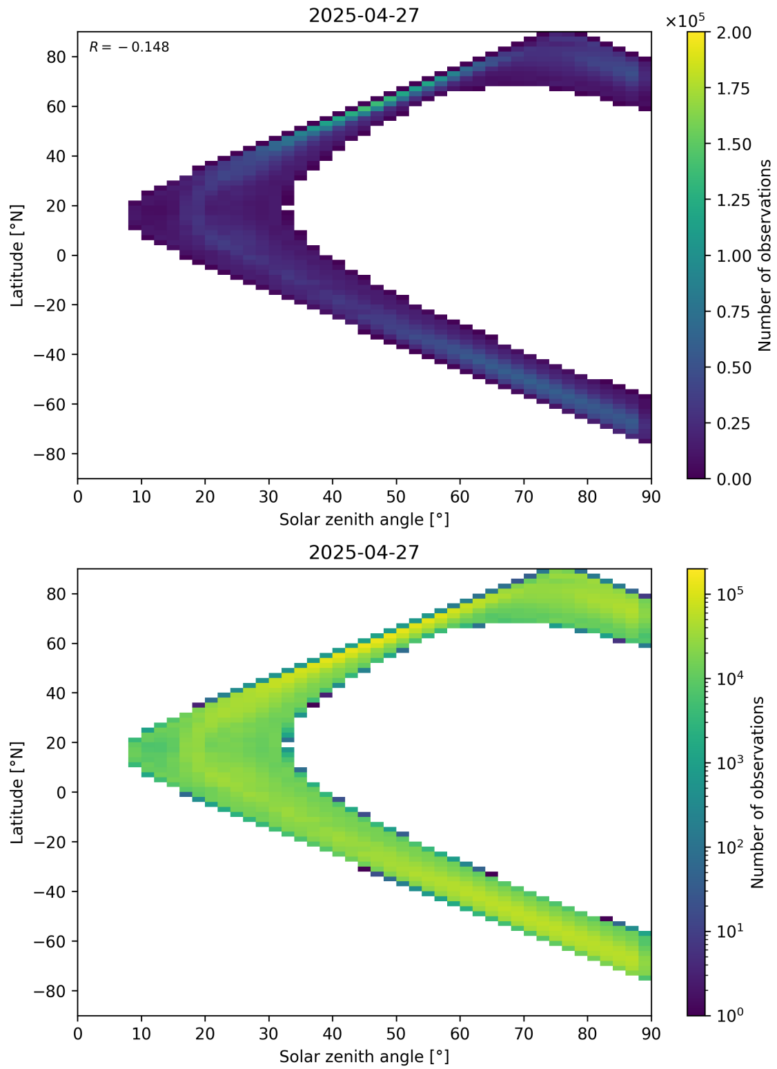
Figure 105: Scatter density plot of “Solar zenith angle” against “Latitude” for 2025-04-26 to 2025-04-28.
