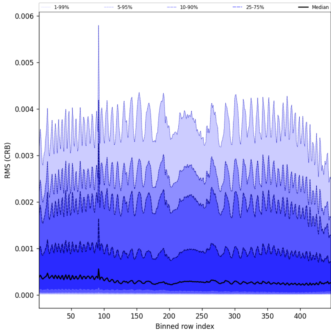
Figure 64: Along track statistics of “RMS (CRB)” for 2025-04-26 to 2025-04-28
