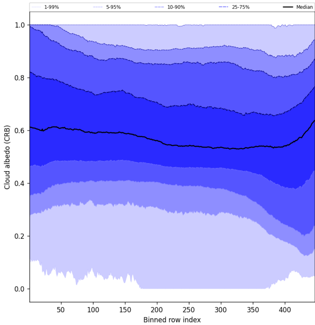
Figure 60: Along track statistics of “Cloud albedo (CRB)” for 2025-04-26 to 2025-04-28
