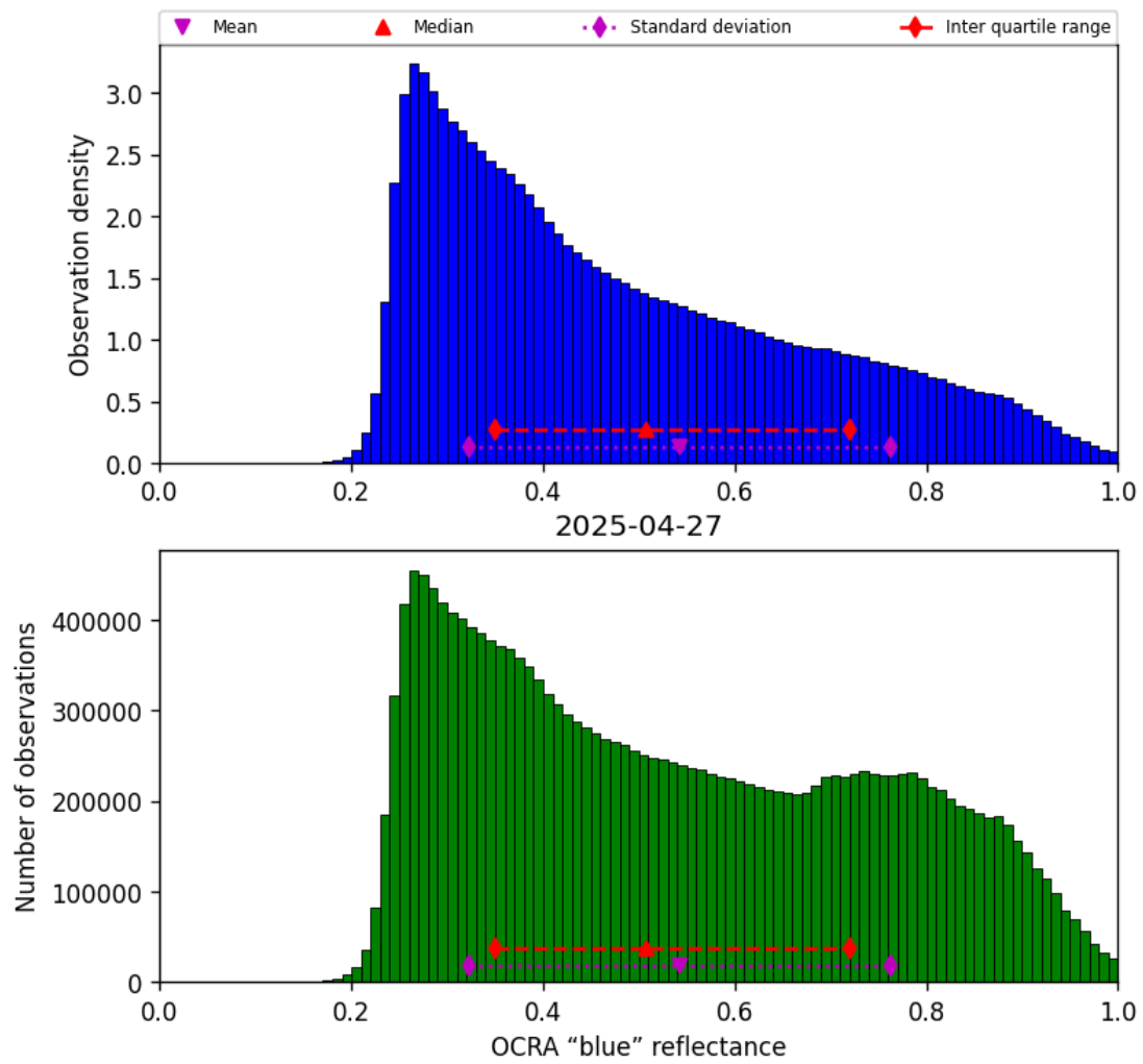
Figure 51: Histogram of “OCRA “blue” reflectance” for 2025-04-26 to 2025-04-28
