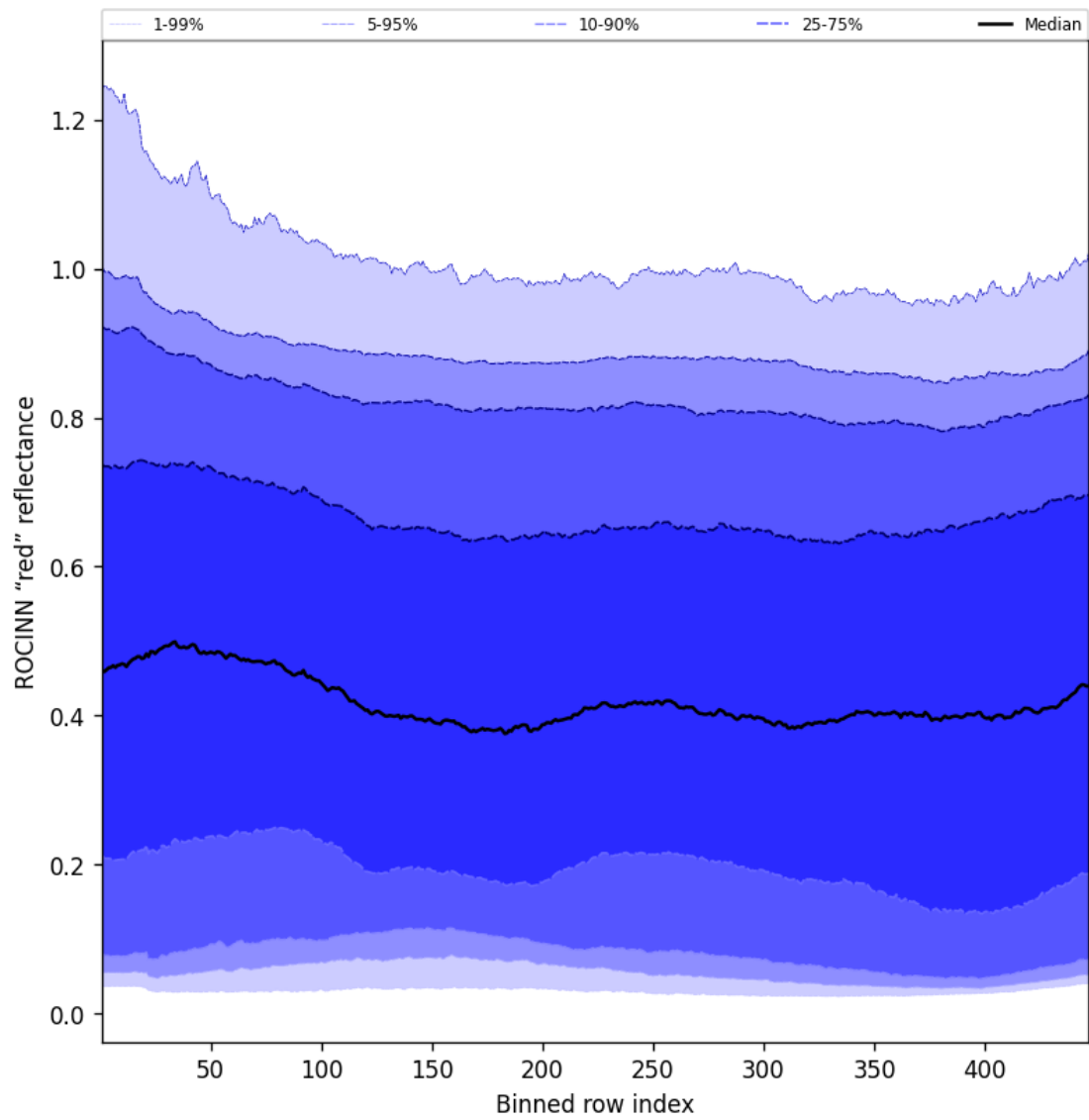
Figure 69: Along track statistics of "ROCINN "red" reflectance" for 2025-04-26 to 2025-04-28
