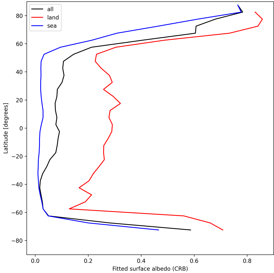
Figure 30: Zonal average of “Fitted surface albedo (CRB)” for 2025-04-26 to 2025-04-28.
