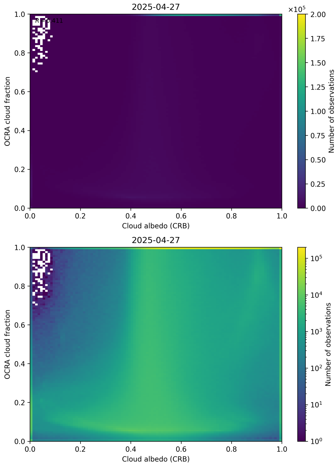
Figure 70: Scatter density plot of “Cloud albedo (CRB)” against “OCRA cloud fraction” for 2025-04-26 to 2025-04-28.
