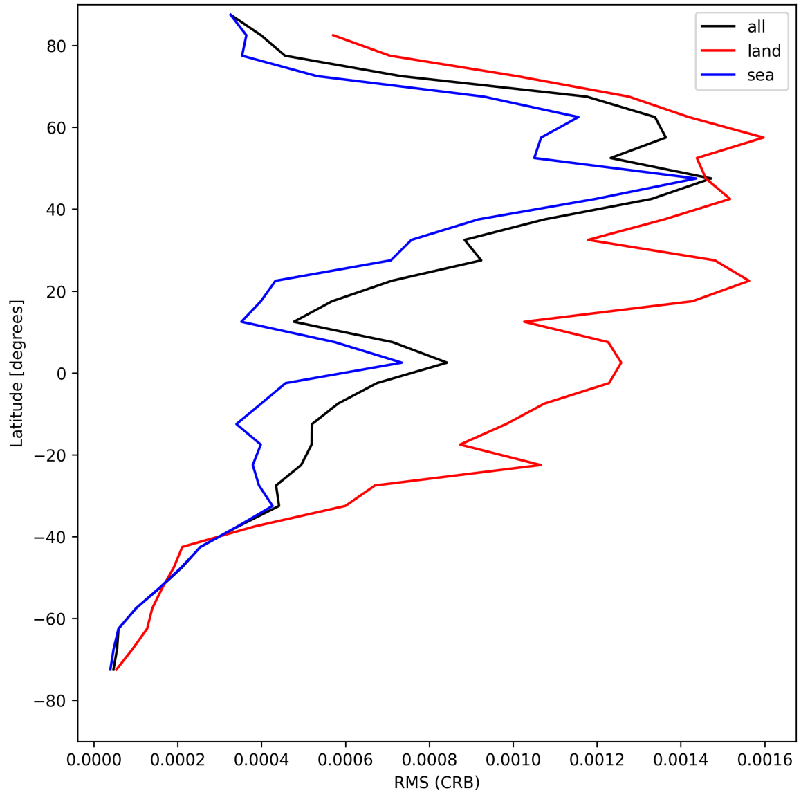
Figure 32: Zonal average of “RMS (CRB)” for 2025-04-26 to 2025-04-28.
