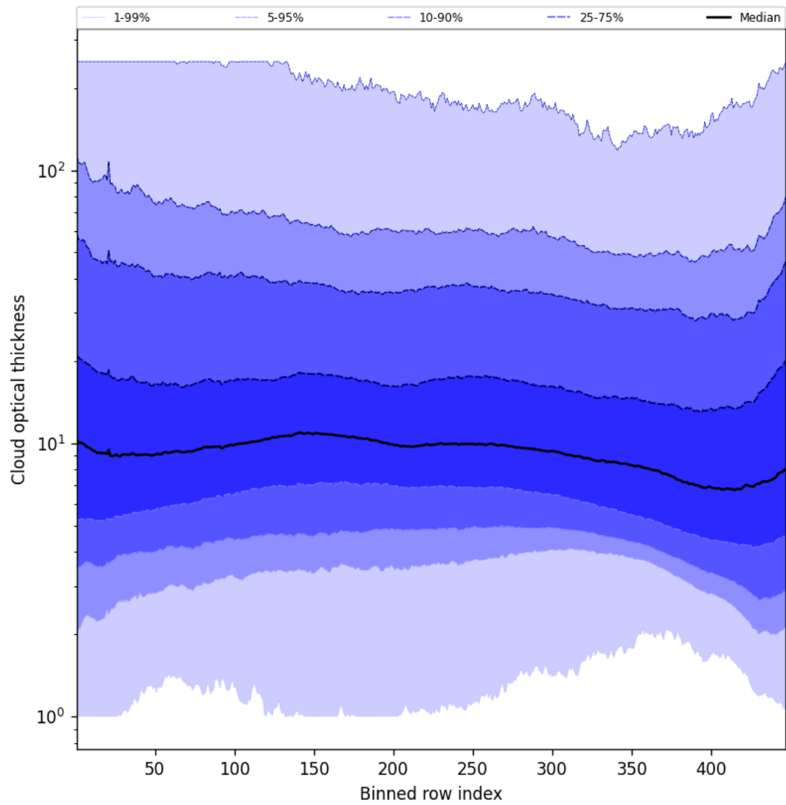
Figure 57: Along track statistics of “Cloud optical thickness” for 2025-04-26 to 2025-04-28
