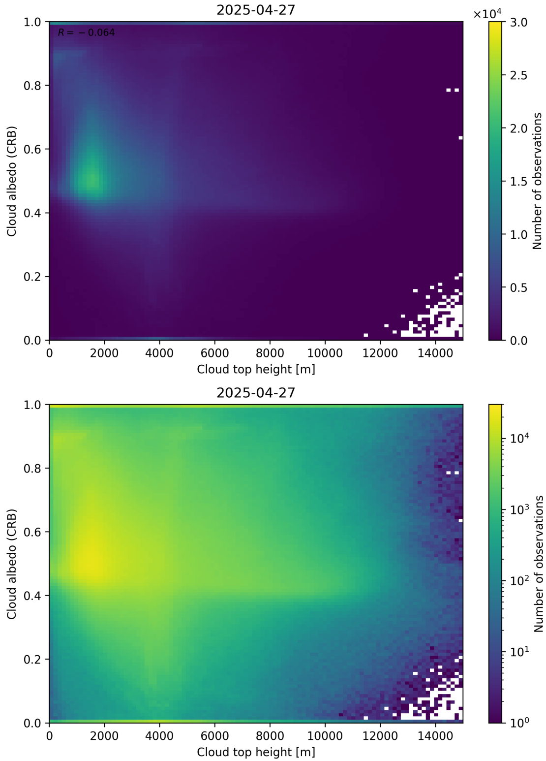
Figure 86: Scatter density plot of “Cloud top height” against “Cloud albedo (CRB)” for 2025-04-26 to 2025-04-28.
