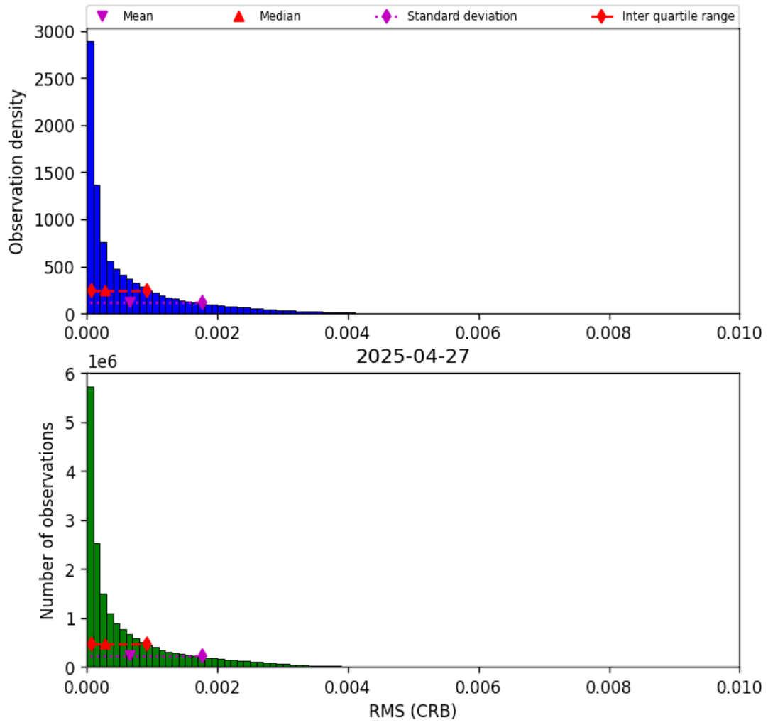
Figure 48: Histogram of “RMS (CRB)” for 2025-04-26 to 2025-04-28
