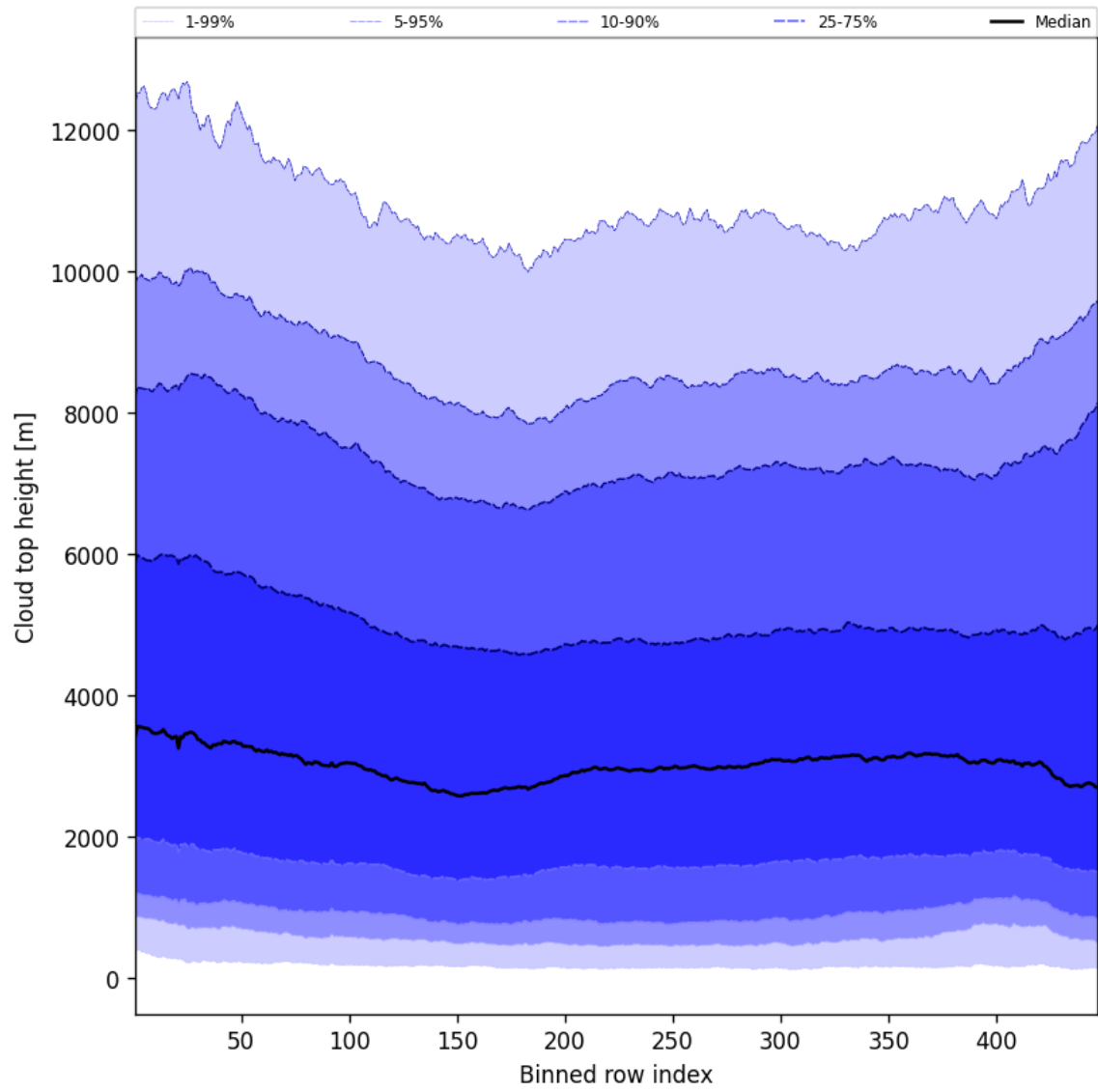
Figure 56: Along track statistics of “Cloud top height” for 2025-04-26 to 2025-04-28
