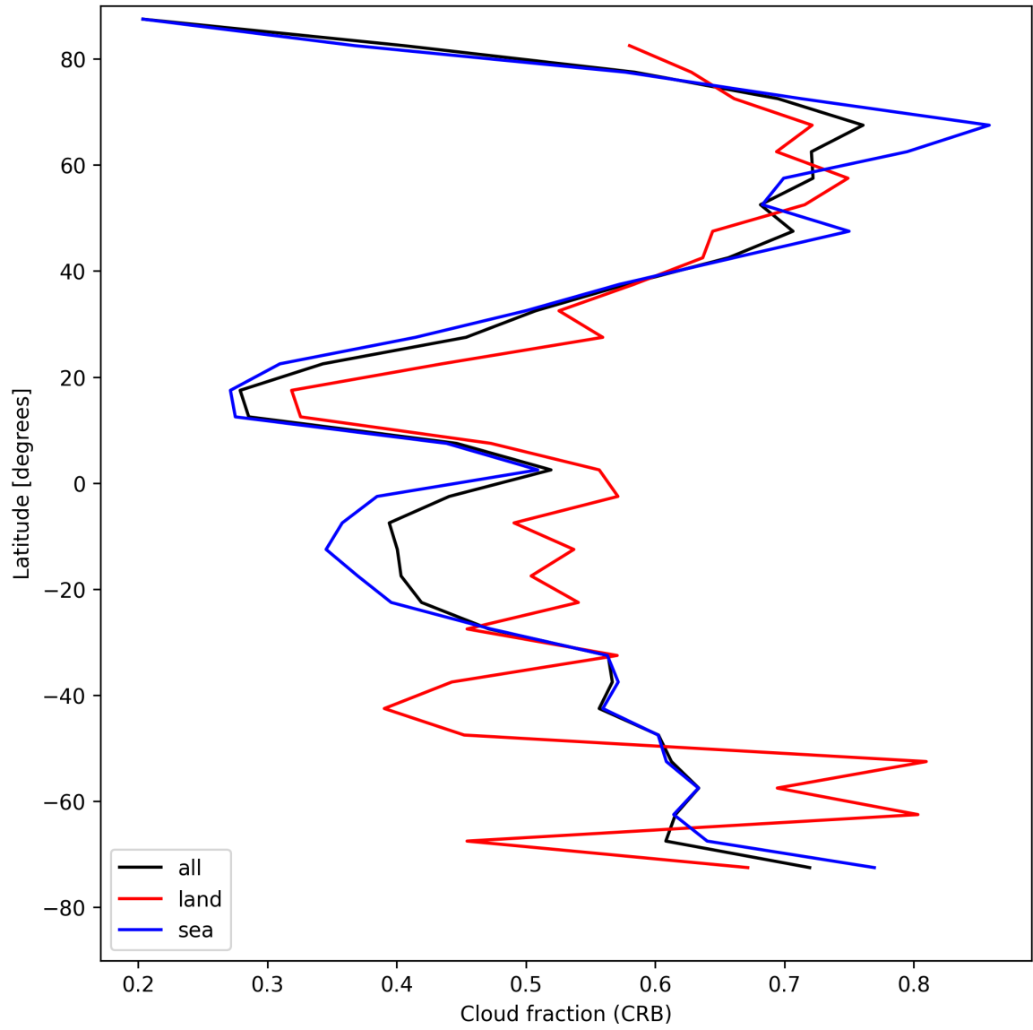
Figure 26: Zonal average of “Cloud fraction (CRB)” for 2025-04-26 to 2025-04-28.
