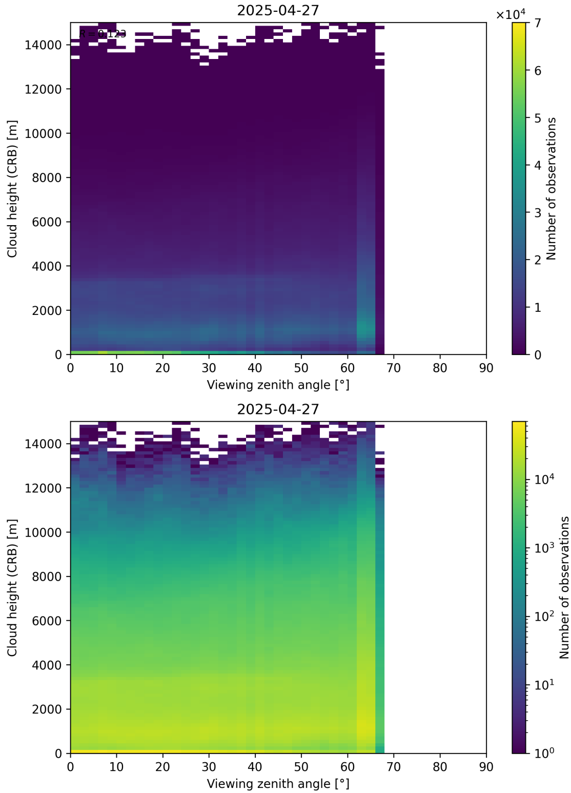
Figure 110: Scatter density plot of “Viewing zenith angle” against “Cloud height (CRB)” for 2025-04-26 to 2025-04-28.
