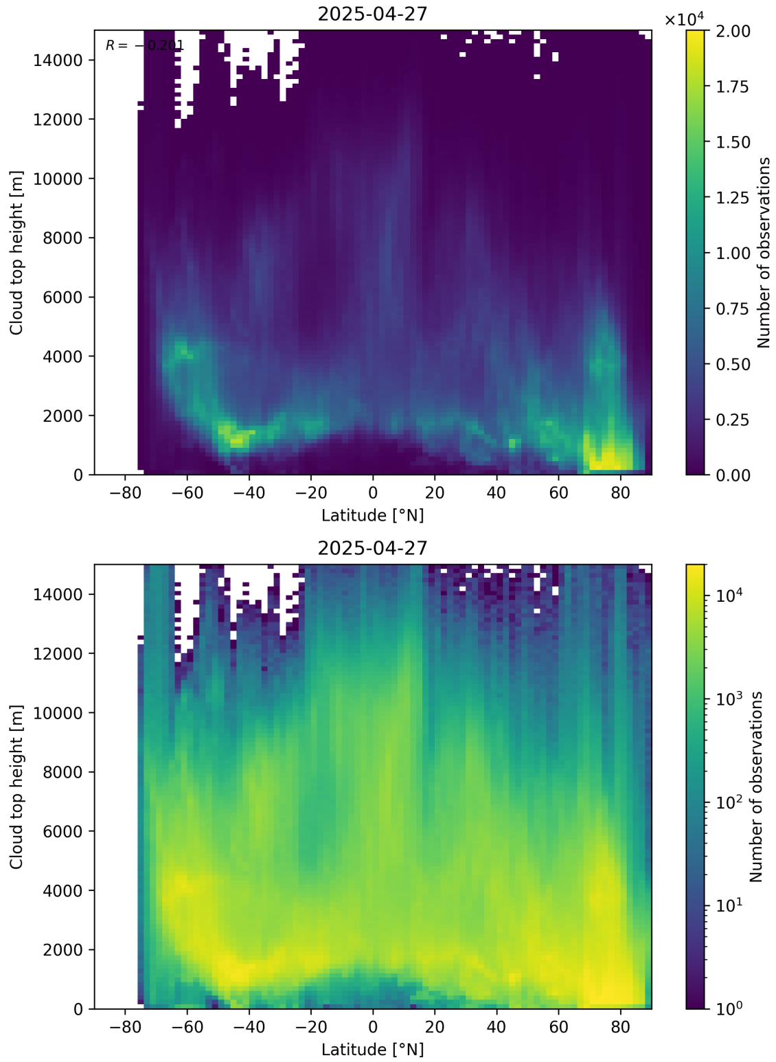
Figure 97: Scatter density plot of “Latitude” against “Cloud top height” for 2025-04-26 to 2025-04-28.
