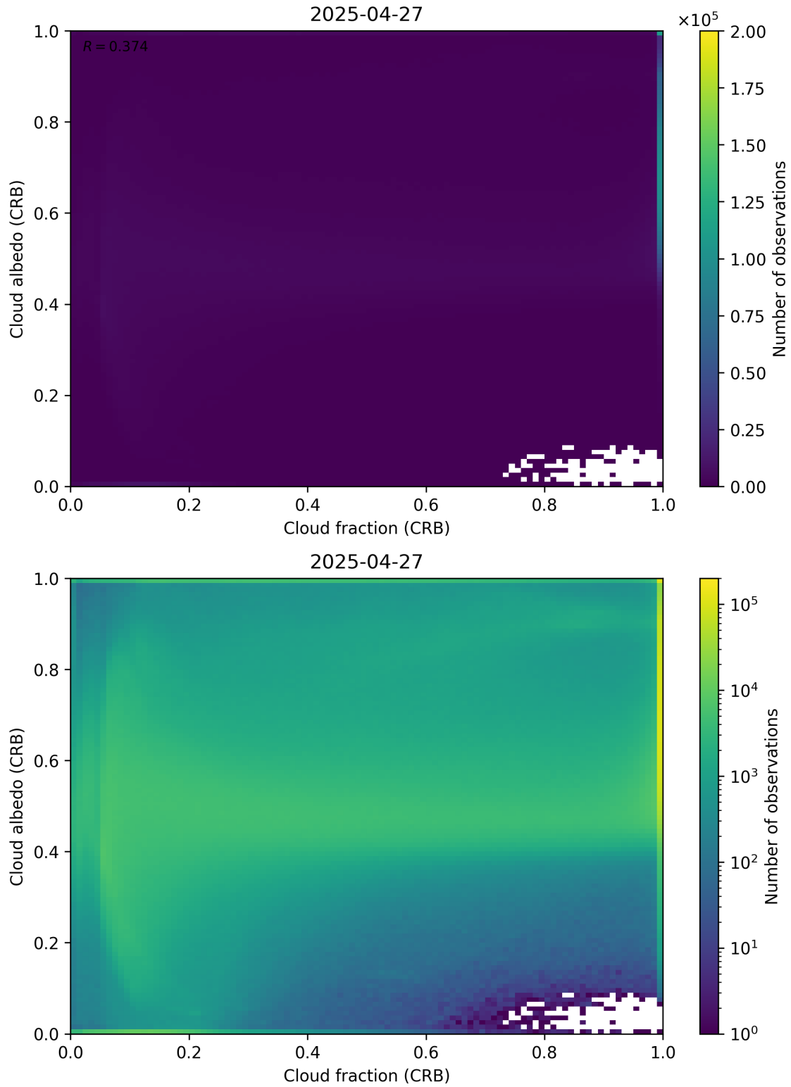
Figure 77: Scatter density plot of “Cloud fraction (CRB)” against “Cloud albedo (CRB)” for 2025-04-26 to 2025-04-28.
