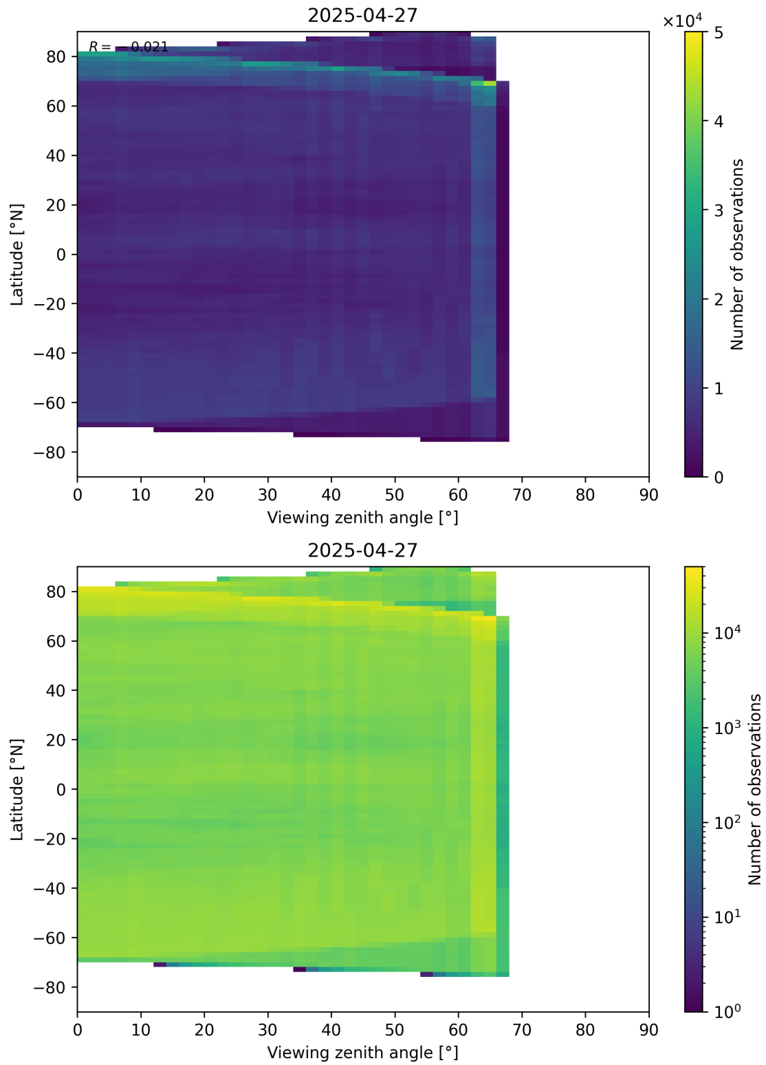
Figure 113: Scatter density plot of “Viewing zenith angle” against “Latitude” for 2025-04-26 to 2025-04-28.
