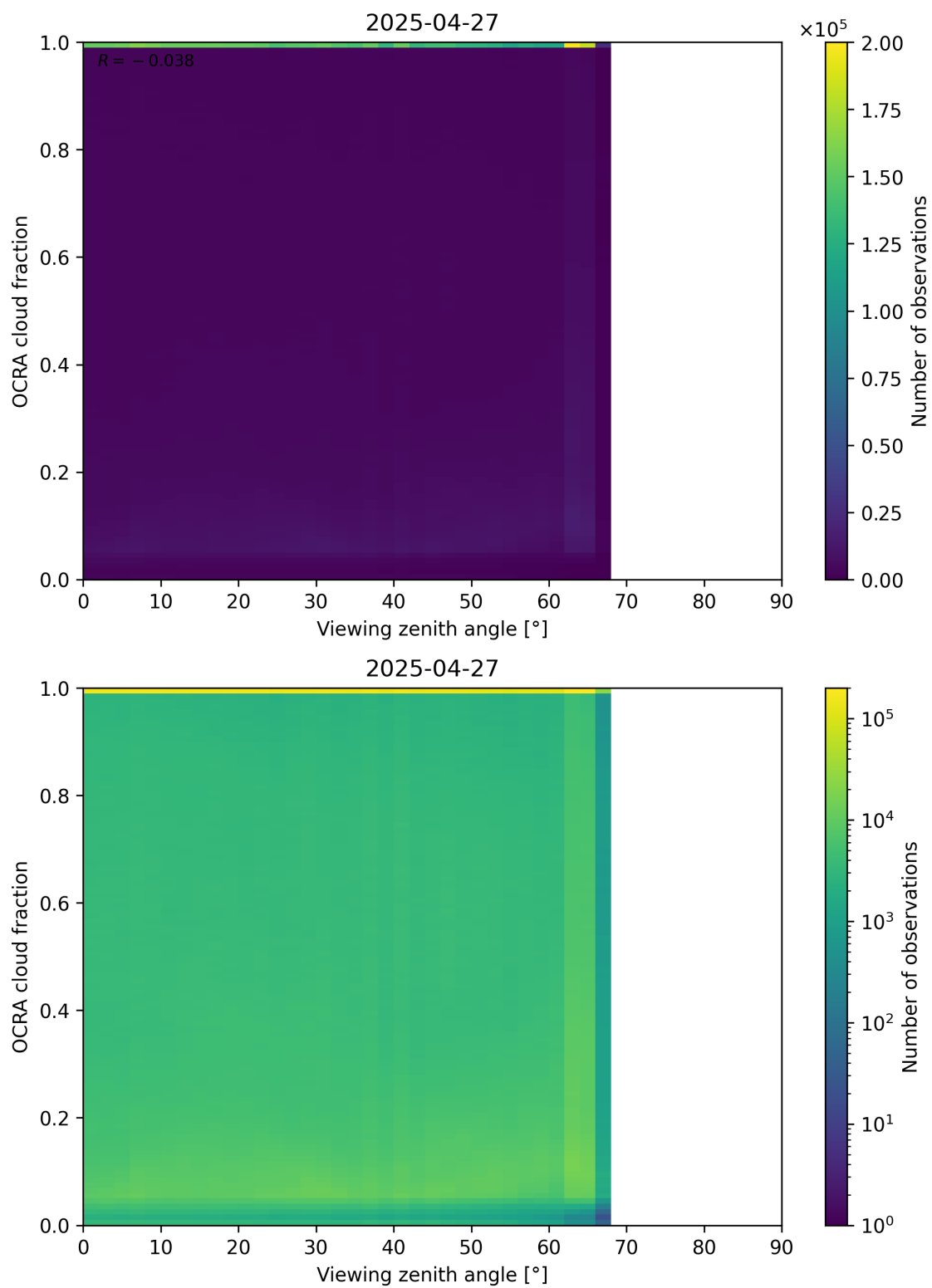
Figure 108: Scatter density plot of “Viewing zenith angle” against “OCRA cloud fraction” for 2025-04-26 to 2025-04-28.
