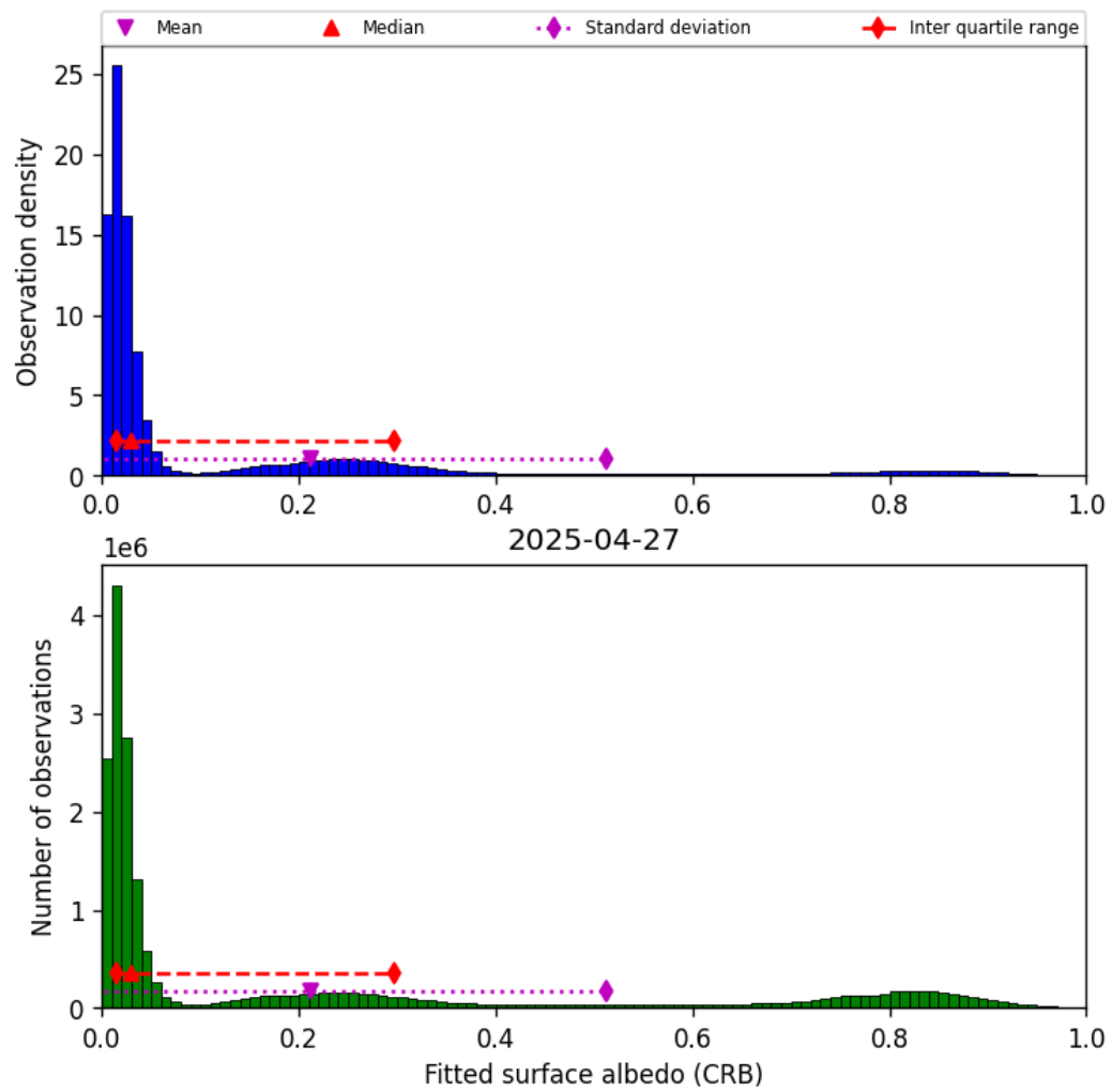
Figure 46: Histogram of “Fitted surface albedo (CRB)” for 2025-04-26 to 2025-04-28
