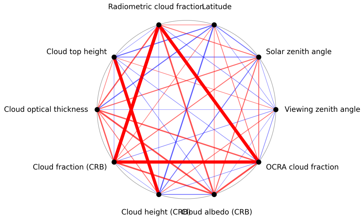
Figure 1: Map of correlation graph for 2025-04-27 to 2025-04-29.
