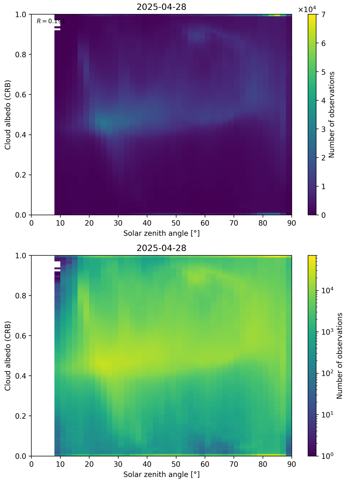
Figure 98: Scatter density plot of “Solar zenith angle” against “Cloud albedo (CRB)” for 2025-04-27 to 2025-04-29.
