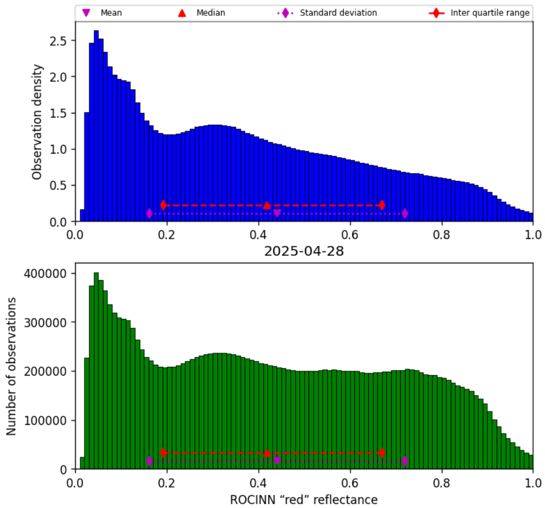
Figure 53: Histogram of "ROCINN "red" reflectance" for 2025-04-27 to 2025-04-29
