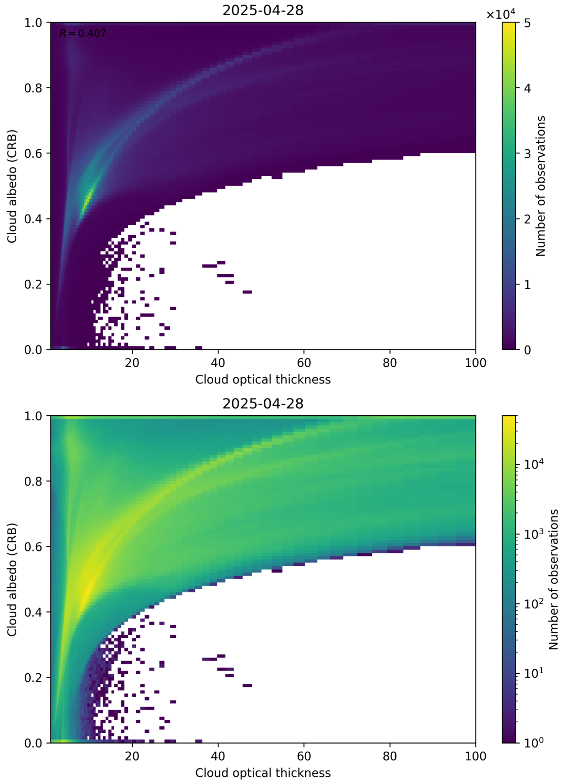
Figure 82: Scatter density plot of “Cloud optical thickness” against “Cloud albedo (CRB)” for 2025-04-27 to 2025-04-29.
