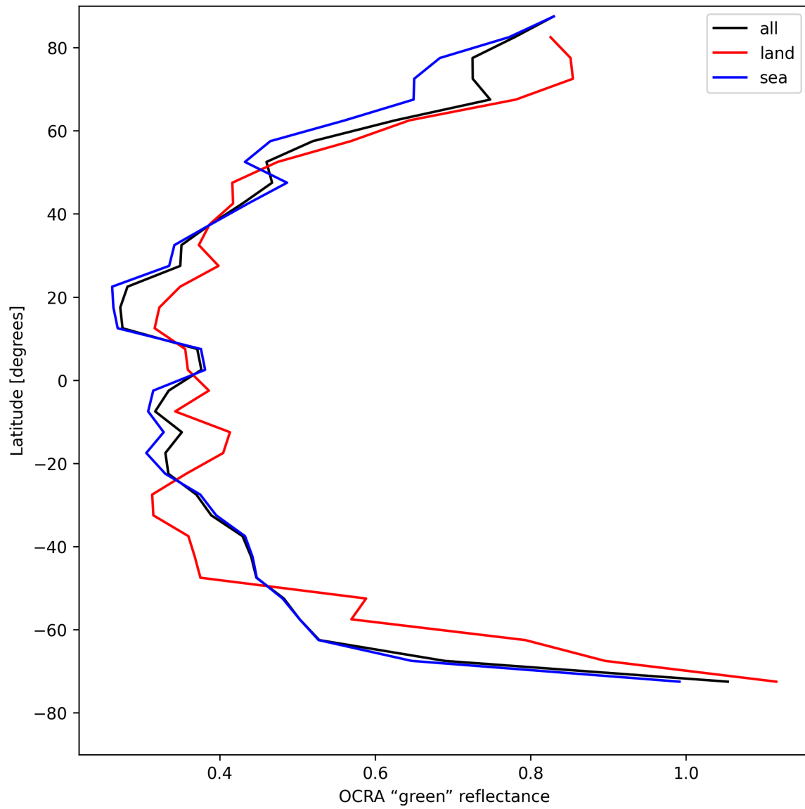
Figure 36: Zonal average of “OCRA “green” reflectance” for 2025-04-27 to 2025-04-29.
