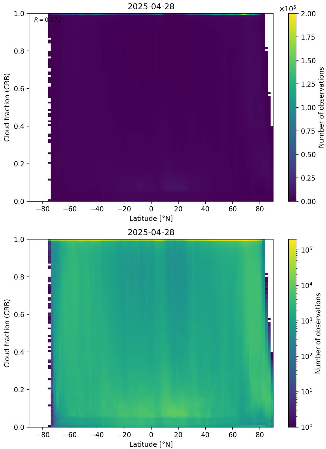
Figure 94: Scatter density plot of “Latitude” against “Cloud fraction (CRB)” for 2025-04-27 to 2025-04-29.
