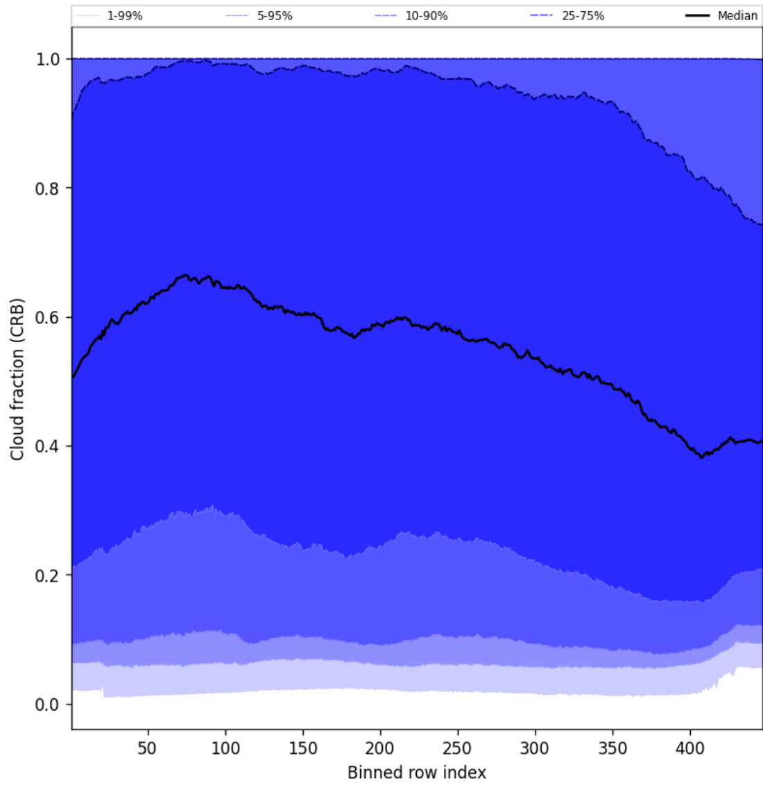
Figure 58: Along track statistics of “Cloud fraction (CRB)” for 2025-04-27 to 2025-04-29
