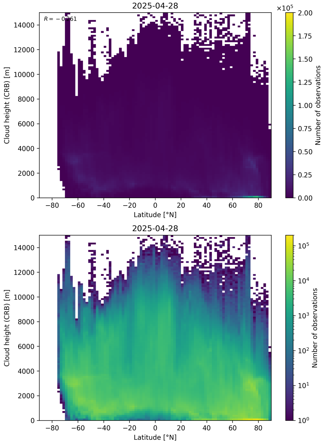
Figure 95: Scatter density plot of “Latitude” against “Cloud height (CRB)” for 2025-04-27 to 2025-04-29.
