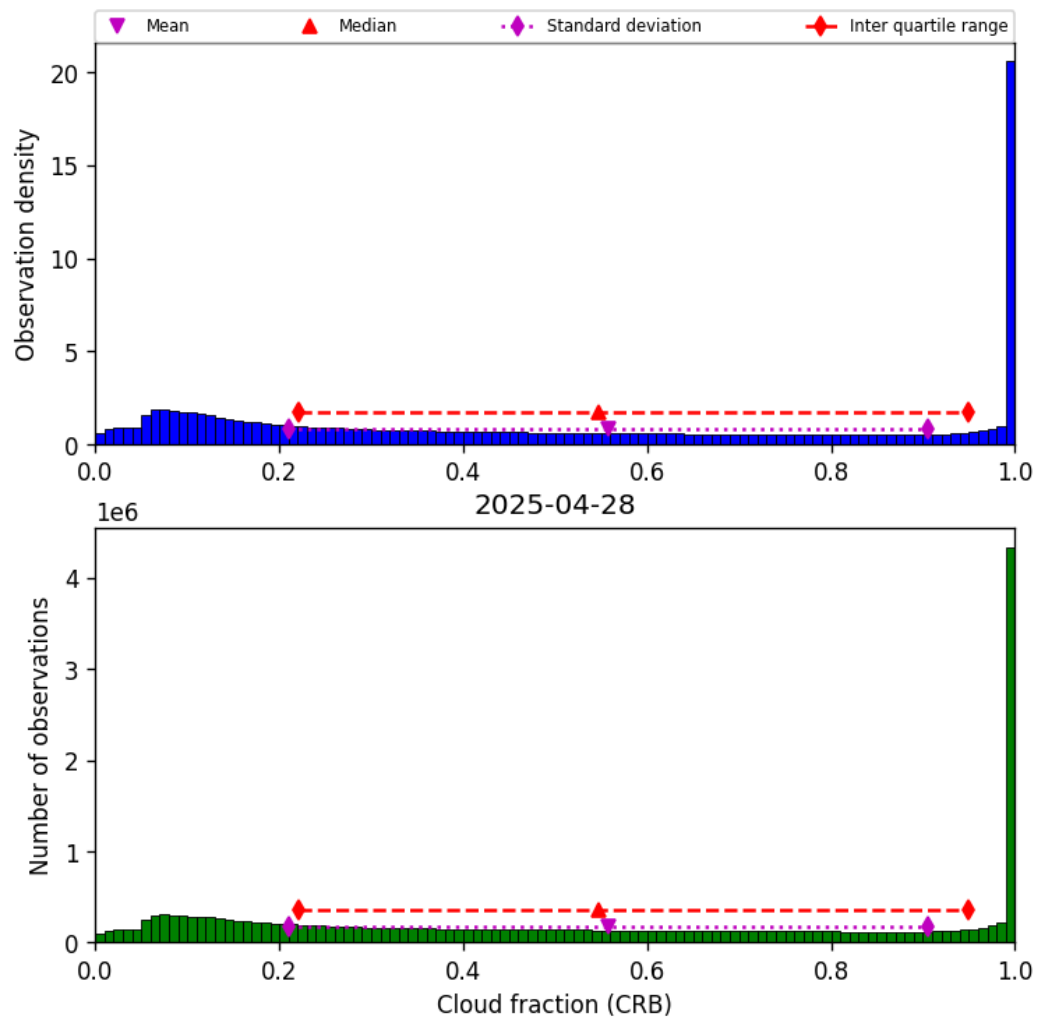
Figure 42: Histogram of “Cloud fraction (CRB)” for 2025-04-27 to 2025-04-29
