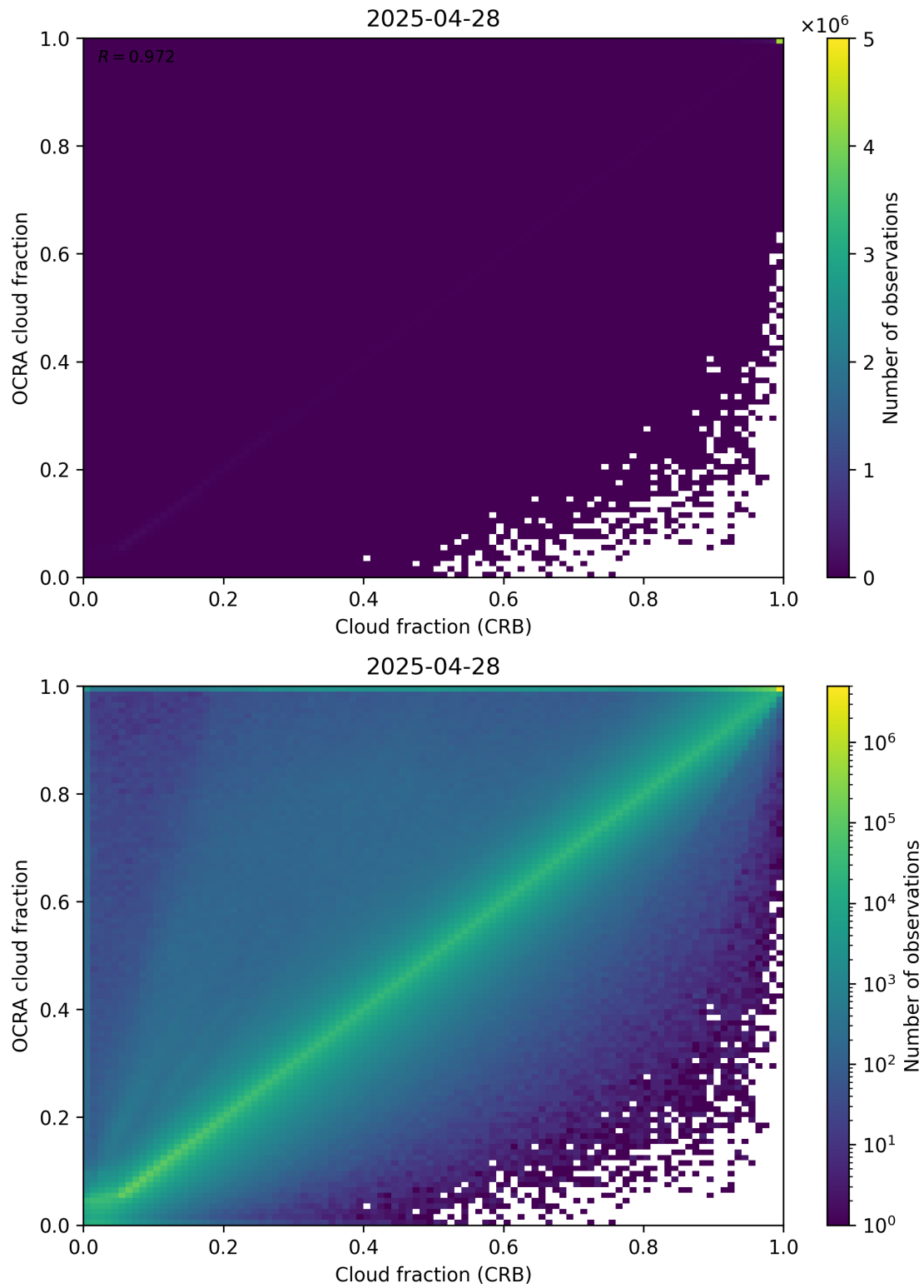
Figure 78: Scatter density plot of “Cloud fraction (CRB)” against “OCRA cloud fraction” for 2025-04-27 to 2025-04-29.
