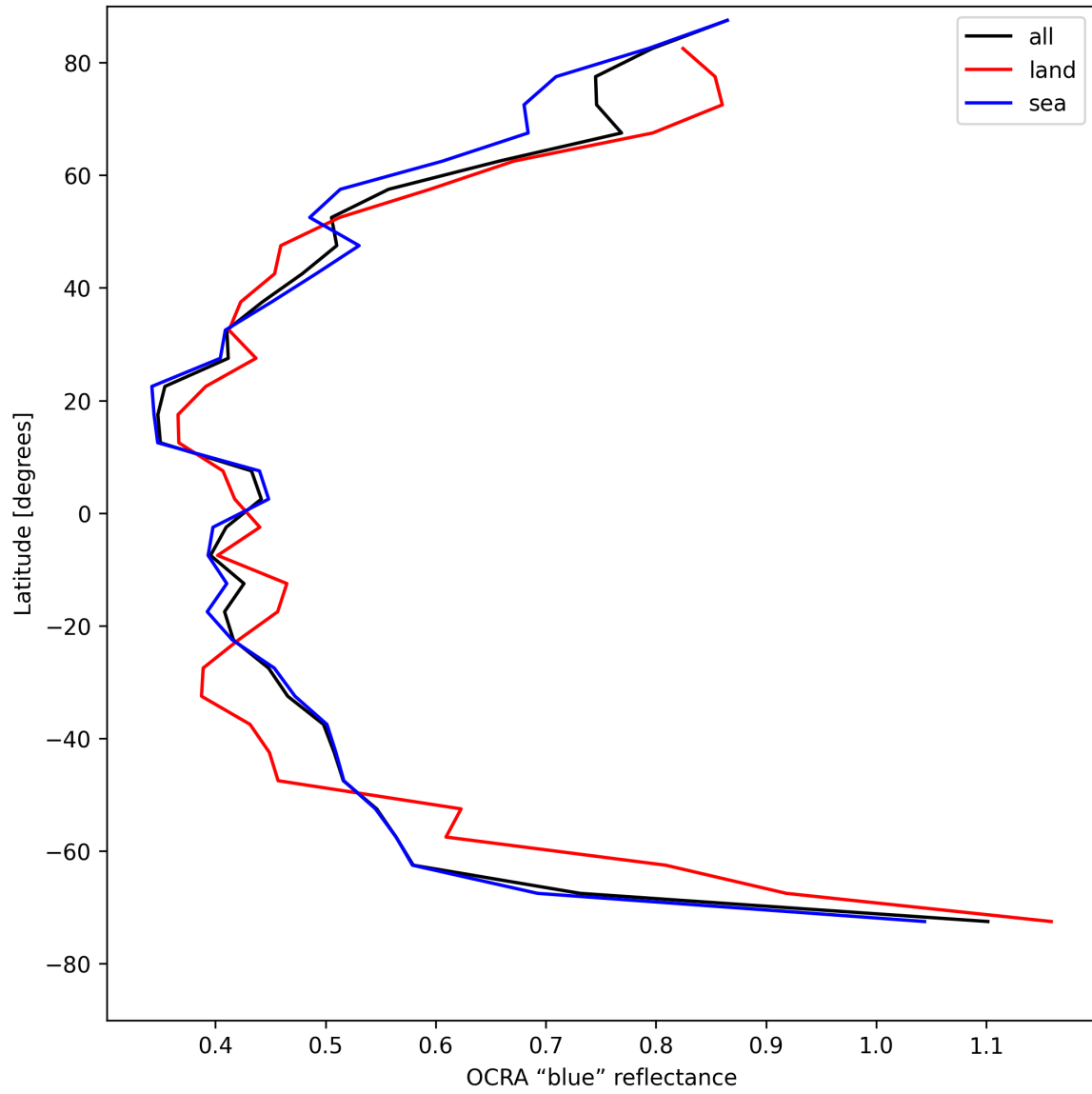
Figure 35: Zonal average of “OCRA “blue” reflectance” for 2025-04-27 to 2025-04-29.
