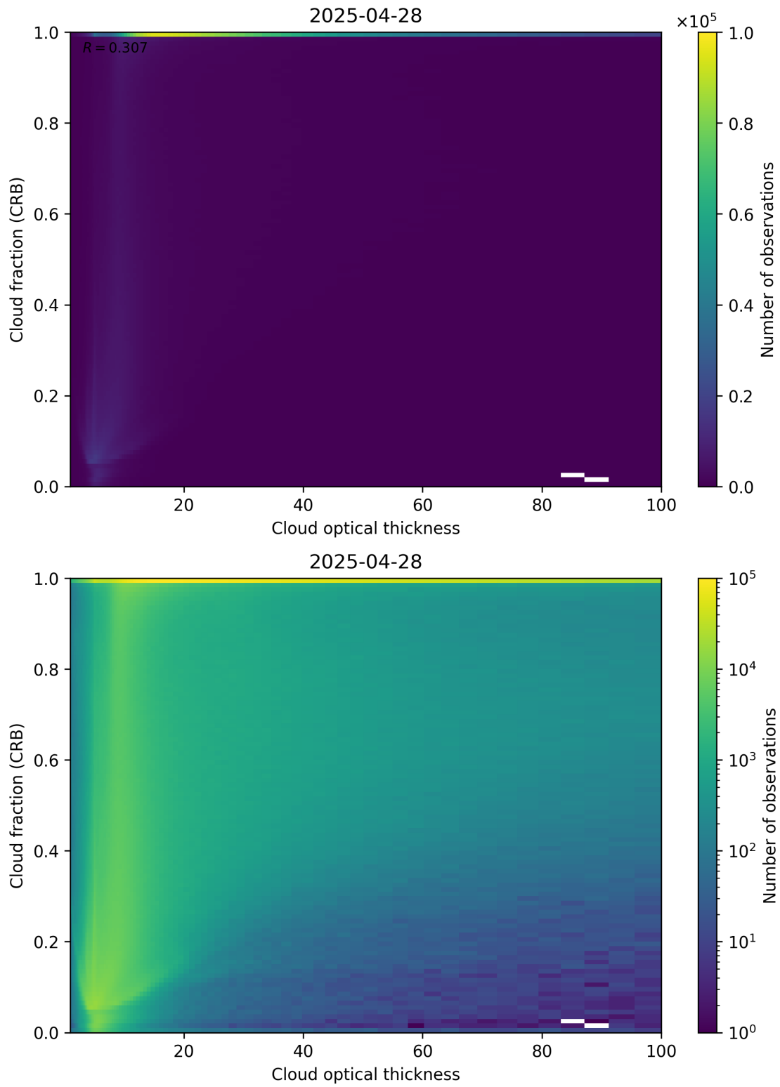
Figure 84: Scatter density plot of “Cloud optical thickness” against “Cloud fraction (CRB)” for 2025-04-27 to 2025-04-29.
