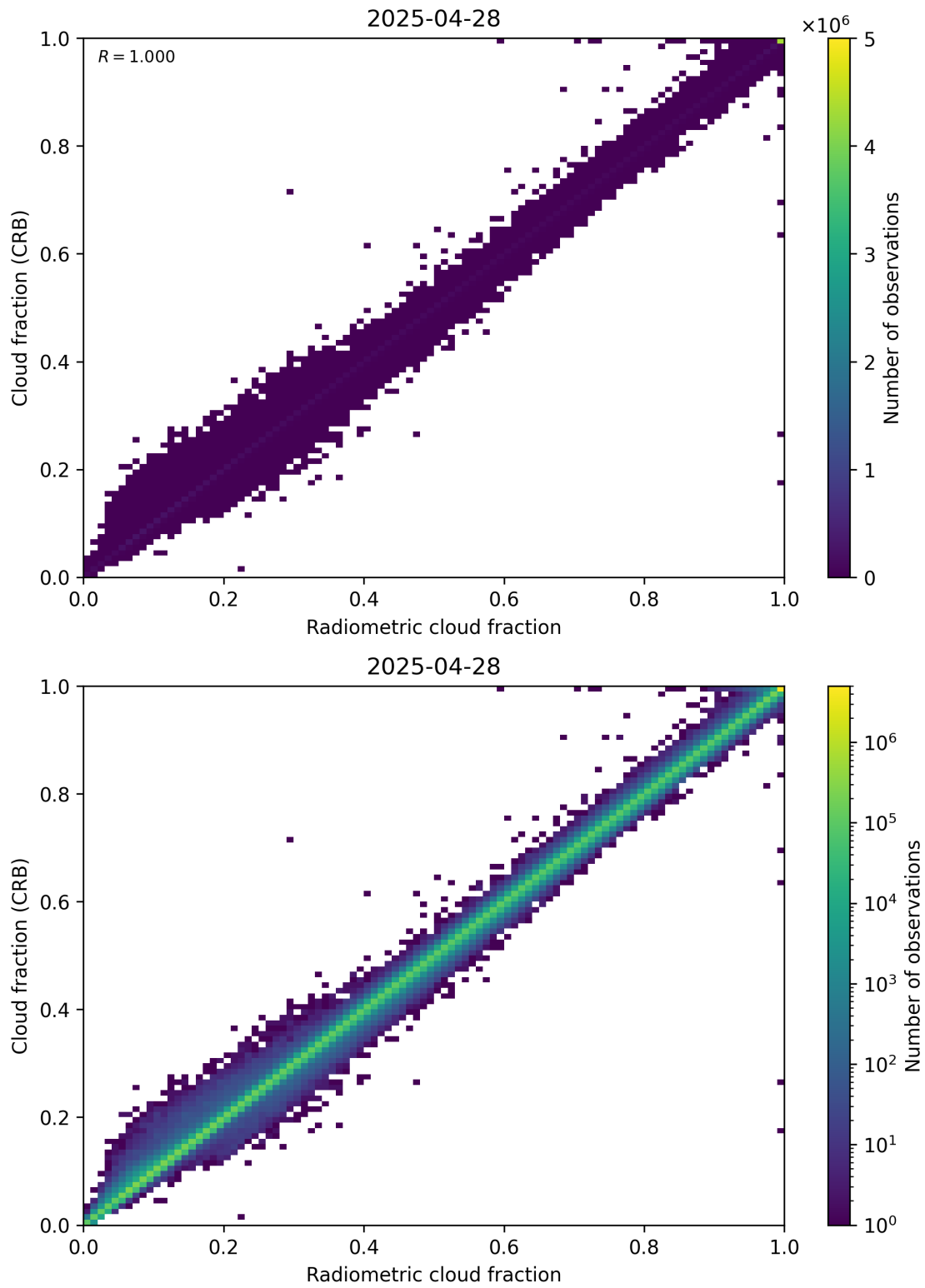
Figure 73: Scatter density plot of “Radiometric cloud fraction” against “Cloud fraction (CRB)” for 2025-04-27 to 2025-04-29.
