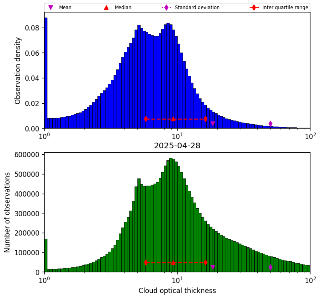
Figure 41: Histogram of “Cloud optical thickness” for 2025-04-27 to 2025-04-29
