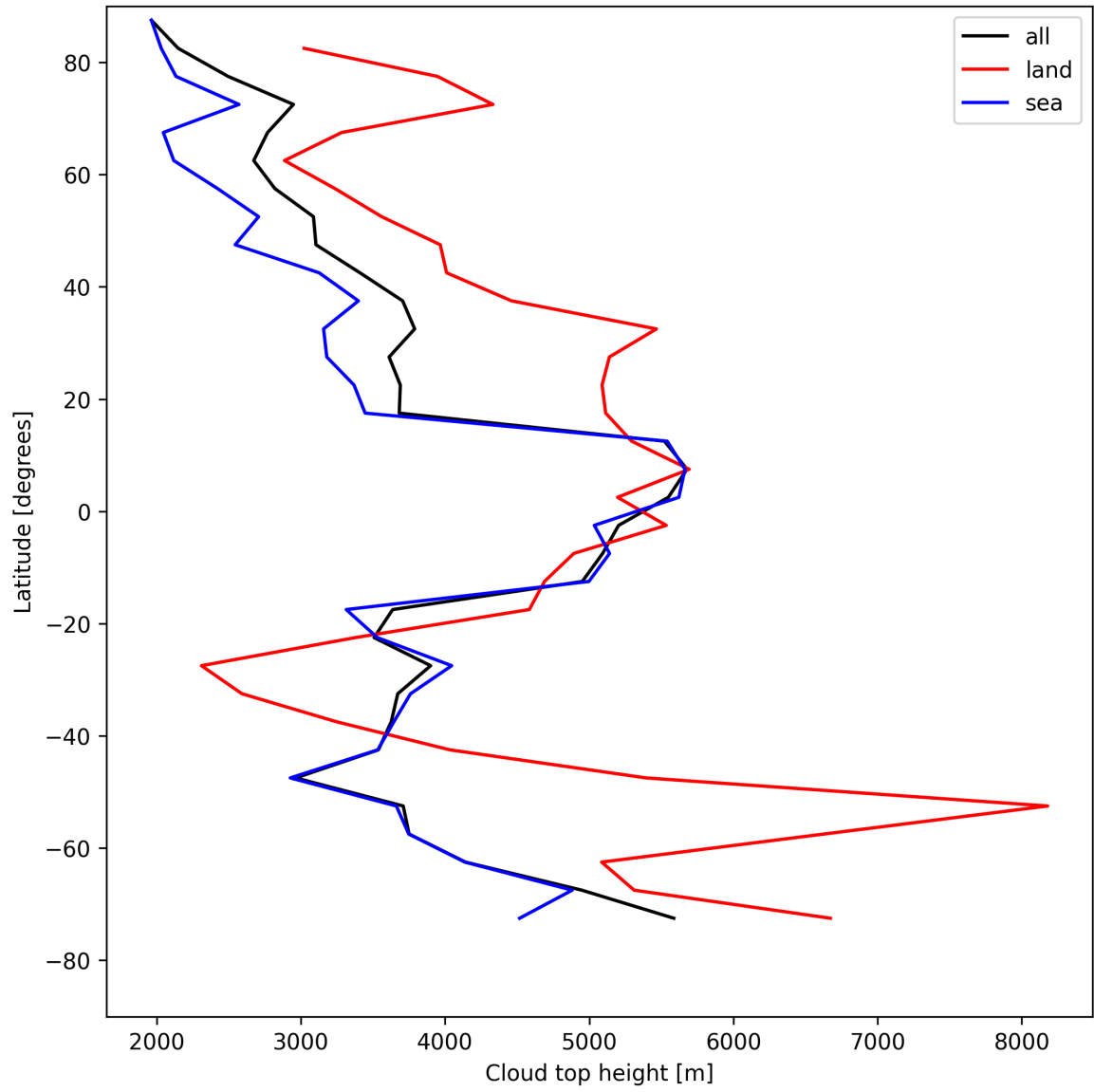
Figure 24: Zonal average of “Cloud top height” for 2025-04-27 to 2025-04-29.
