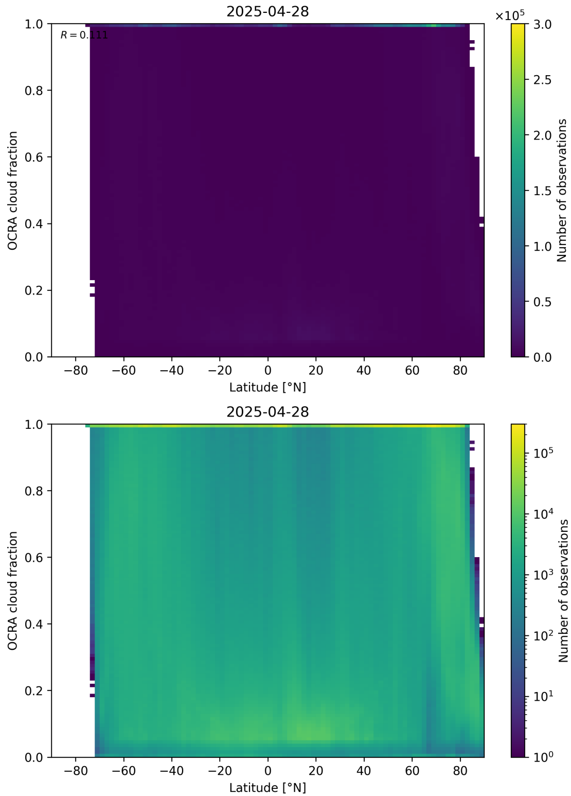
Figure 93: Scatter density plot of “Latitude” against “OCRA cloud fraction” for 2025-04-27 to 2025-04-29.
