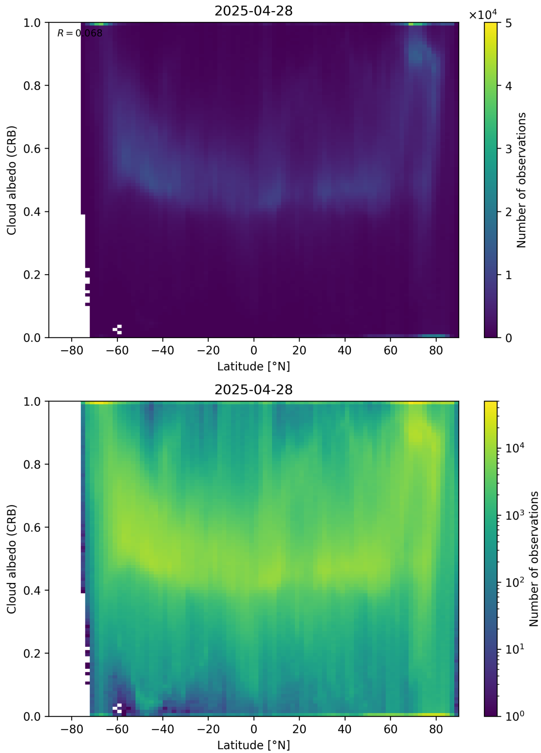
Figure 91: Scatter density plot of “Latitude” against “Cloud albedo (CRB)” for 2025-04-27 to 2025-04-29.
