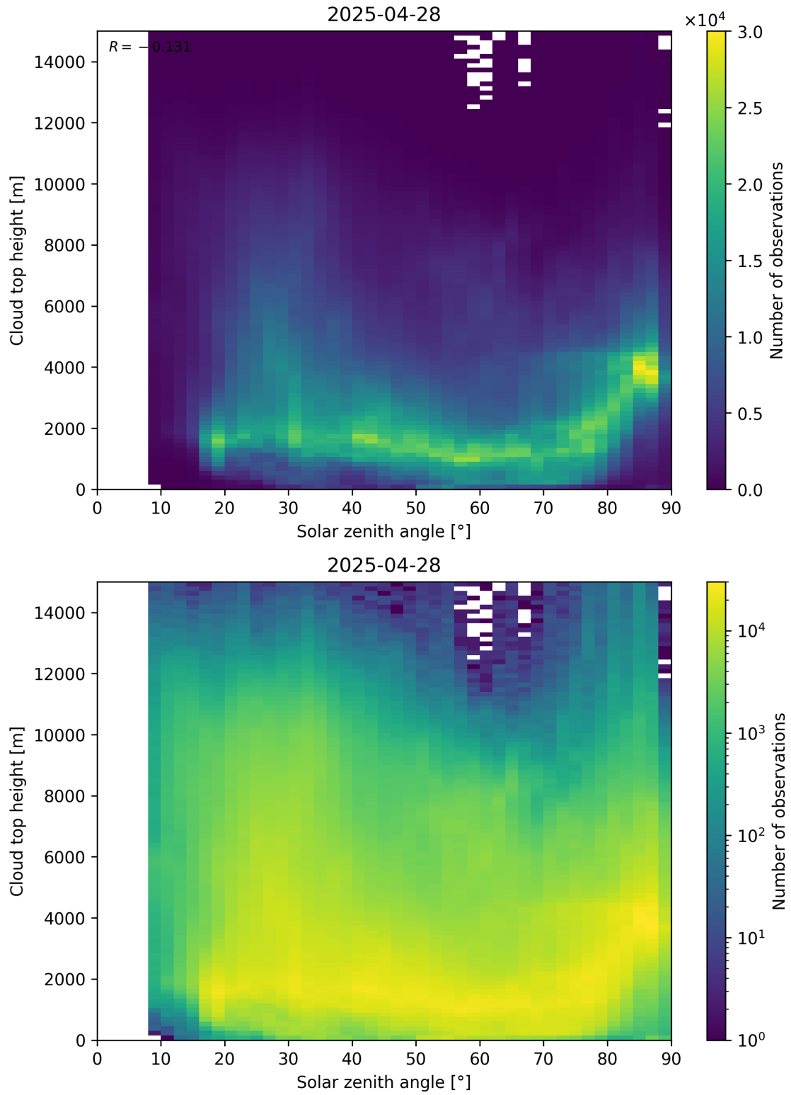
Figure 104: Scatter density plot of “Solar zenith angle” against “Cloud top height” for 2025-04-27 to 2025-04-29.
