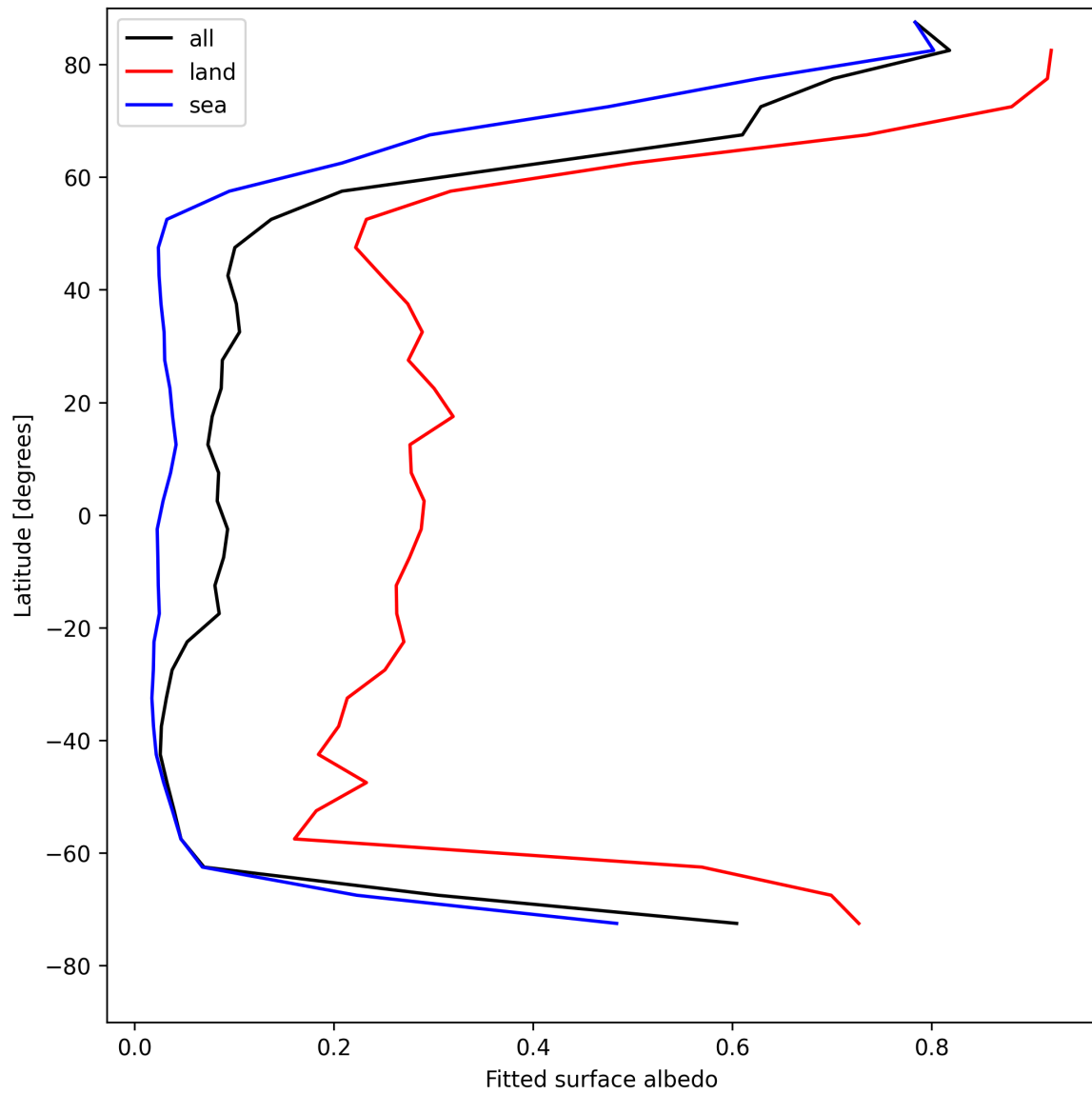
Figure 29: Zonal average of “Fitted surface albedo” for 2025-04-27 to 2025-04-29.
