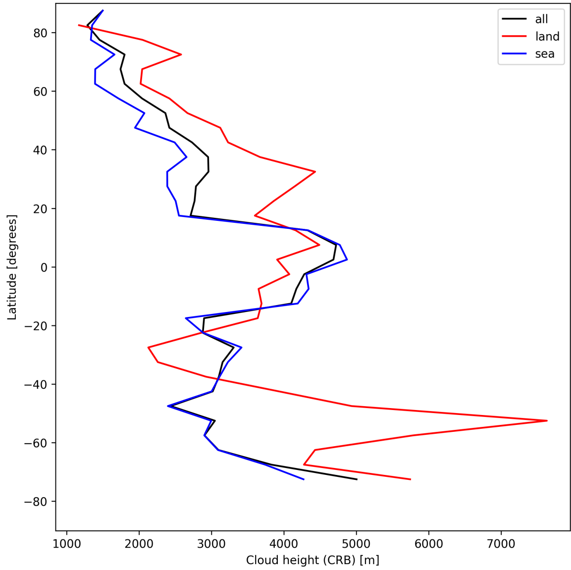
Figure 27: Zonal average of “Cloud height (CRB)” for 2025-04-27 to 2025-04-29.
