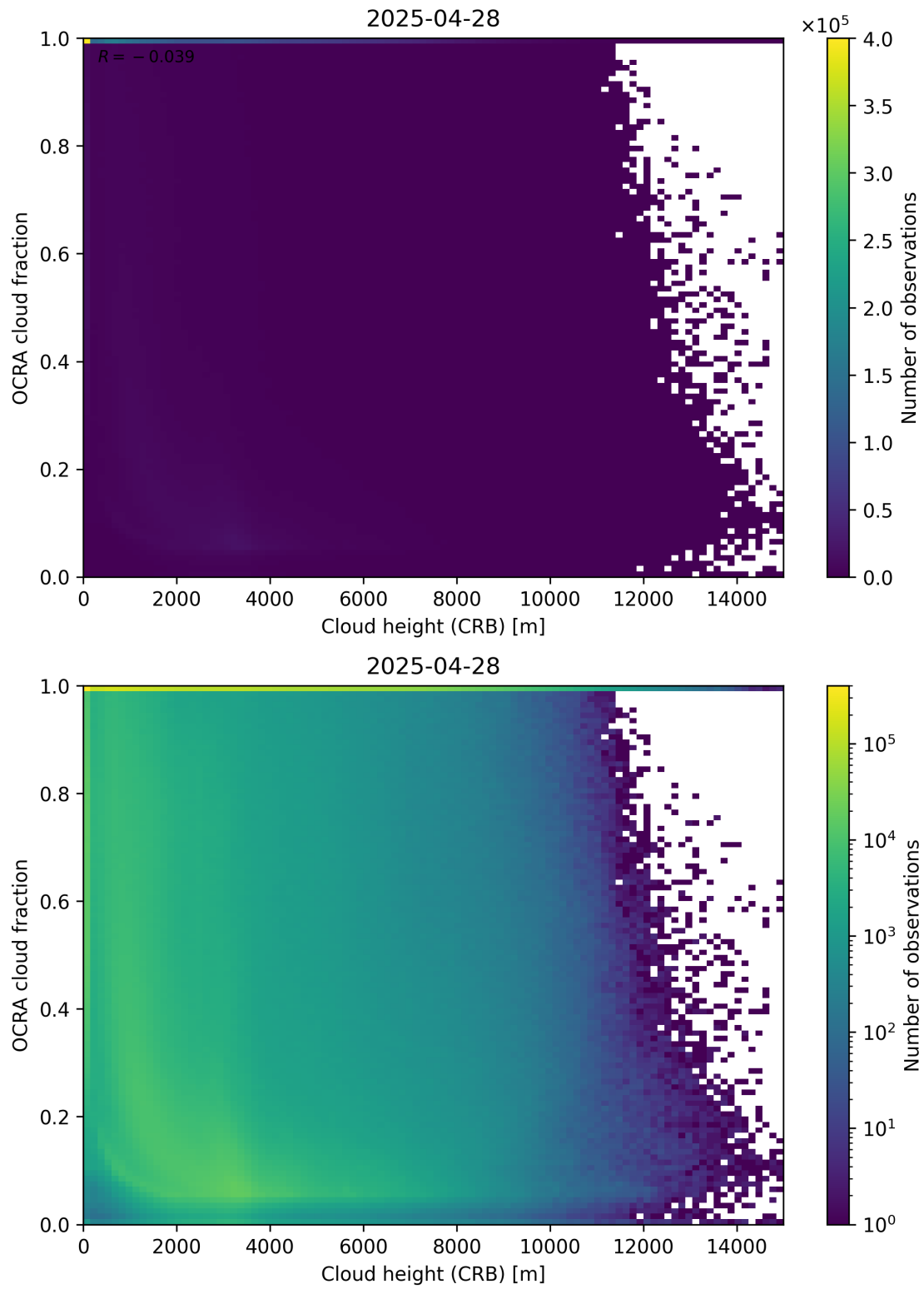
Figure 81: Scatter density plot of “Cloud height (CRB)” against “OCRA cloud fraction” for 2025-04-27 to 2025-04-29.
