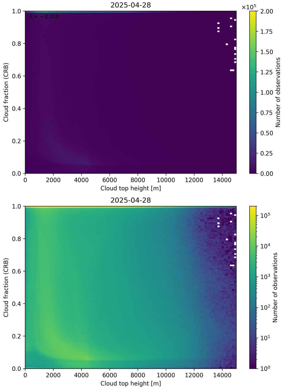
Figure 88: Scatter density plot of “Cloud top height” against “Cloud fraction (CRB)” for 2025-04-27 to 2025-04-29.
