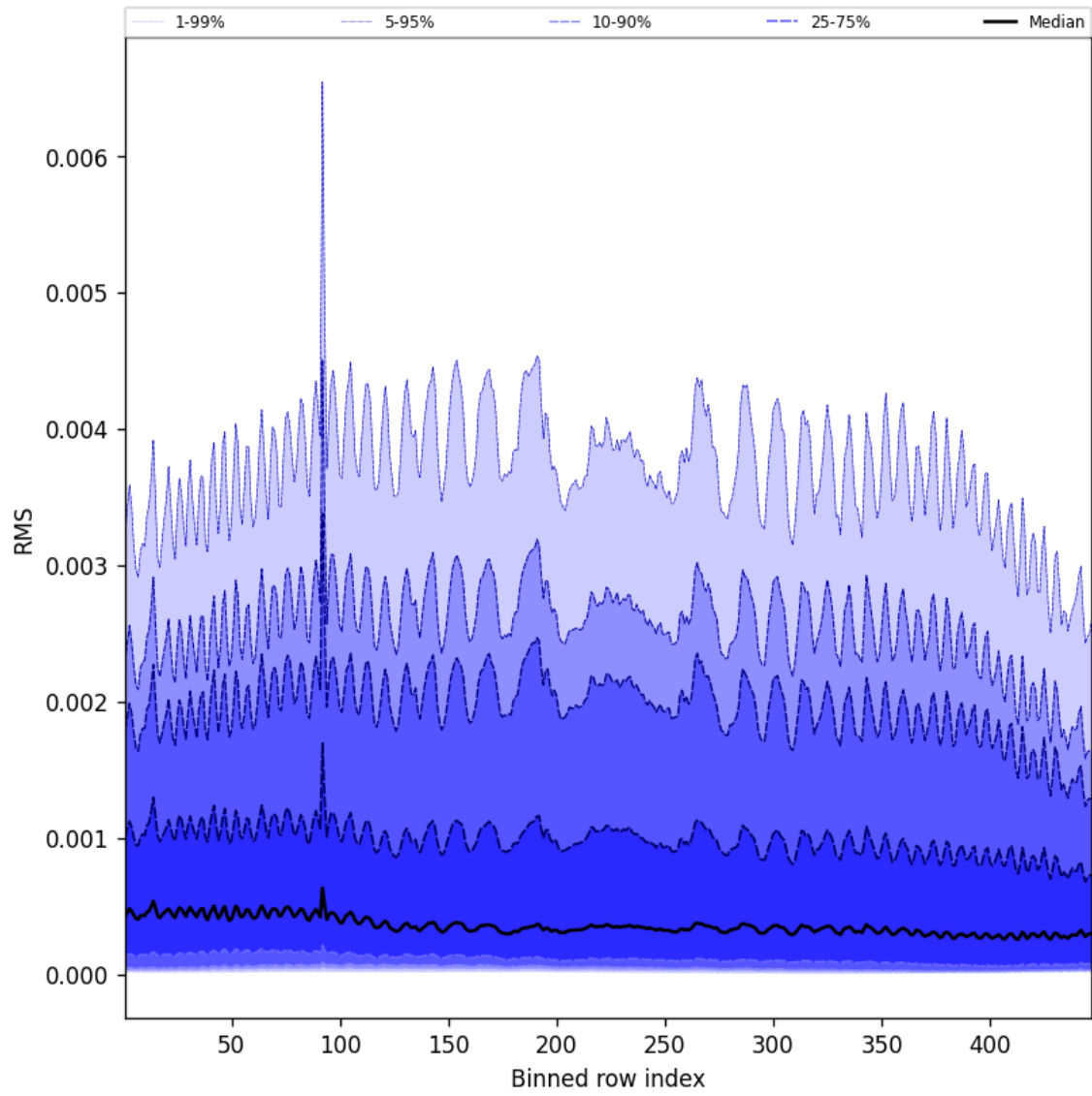
Figure 63: Along track statistics of “RMS” for 2025-04-27 to 2025-04-29
