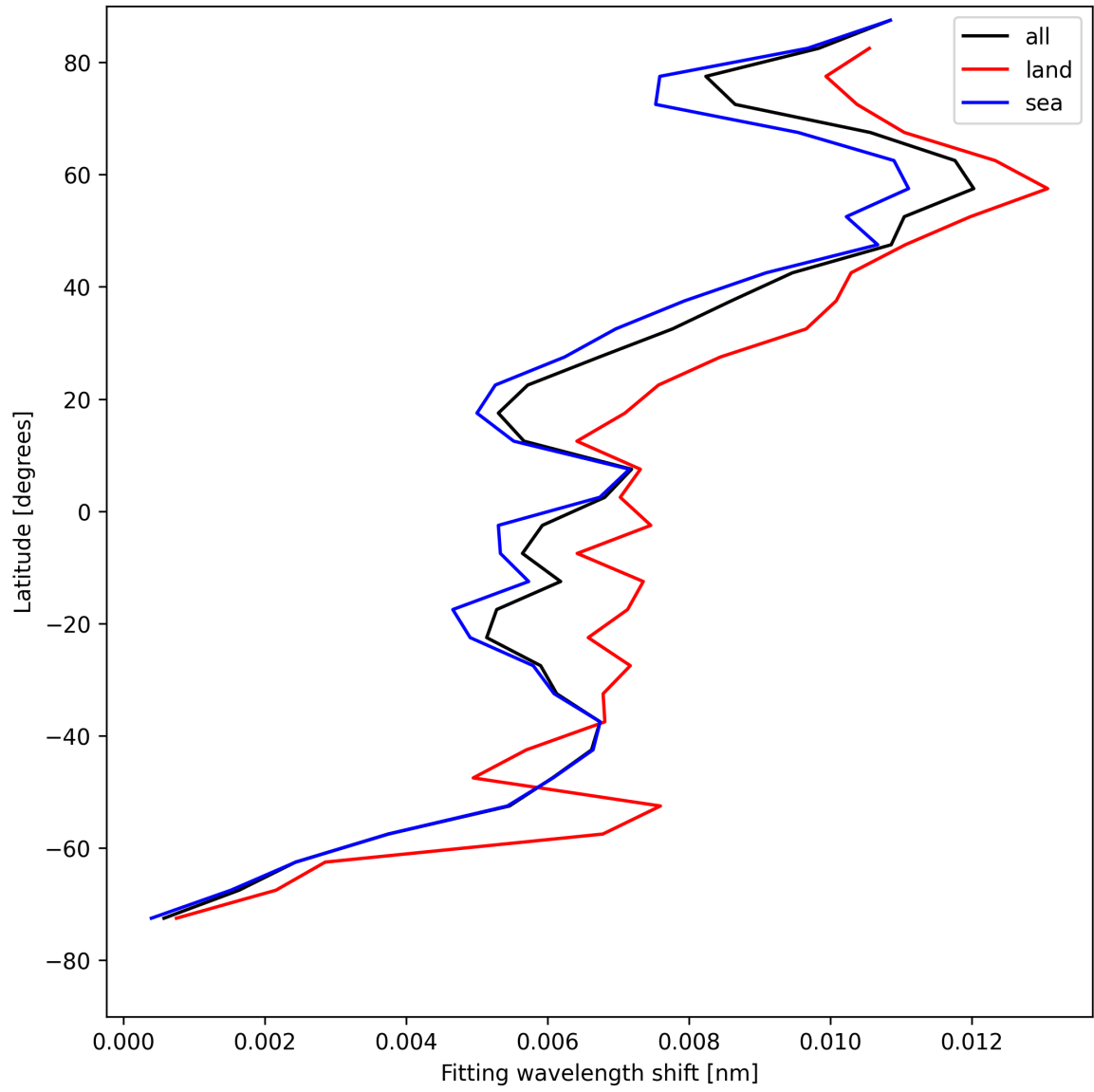
Figure 33: Zonal average of “Fitting wavelength shift” for 2025-04-27 to 2025-04-29.
