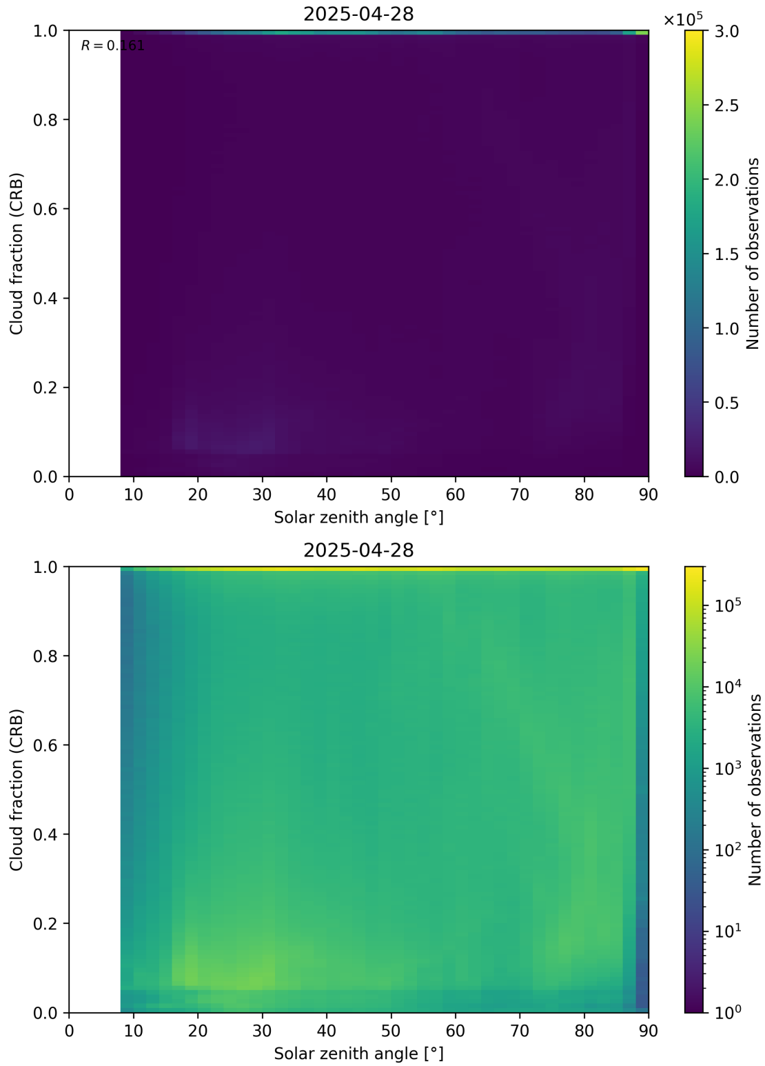
Figure 101: Scatter density plot of “Solar zenith angle” against “Cloud fraction (CRB)” for 2025-04-27 to 2025-04-29.
