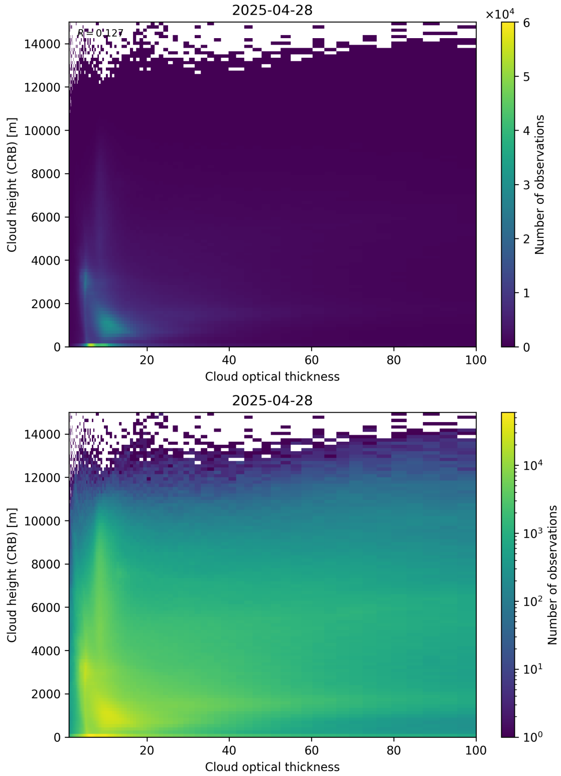
Figure 85: Scatter density plot of “Cloud optical thickness” against “Cloud height (CRB)” for 2025-04-27 to 2025-04-29.
