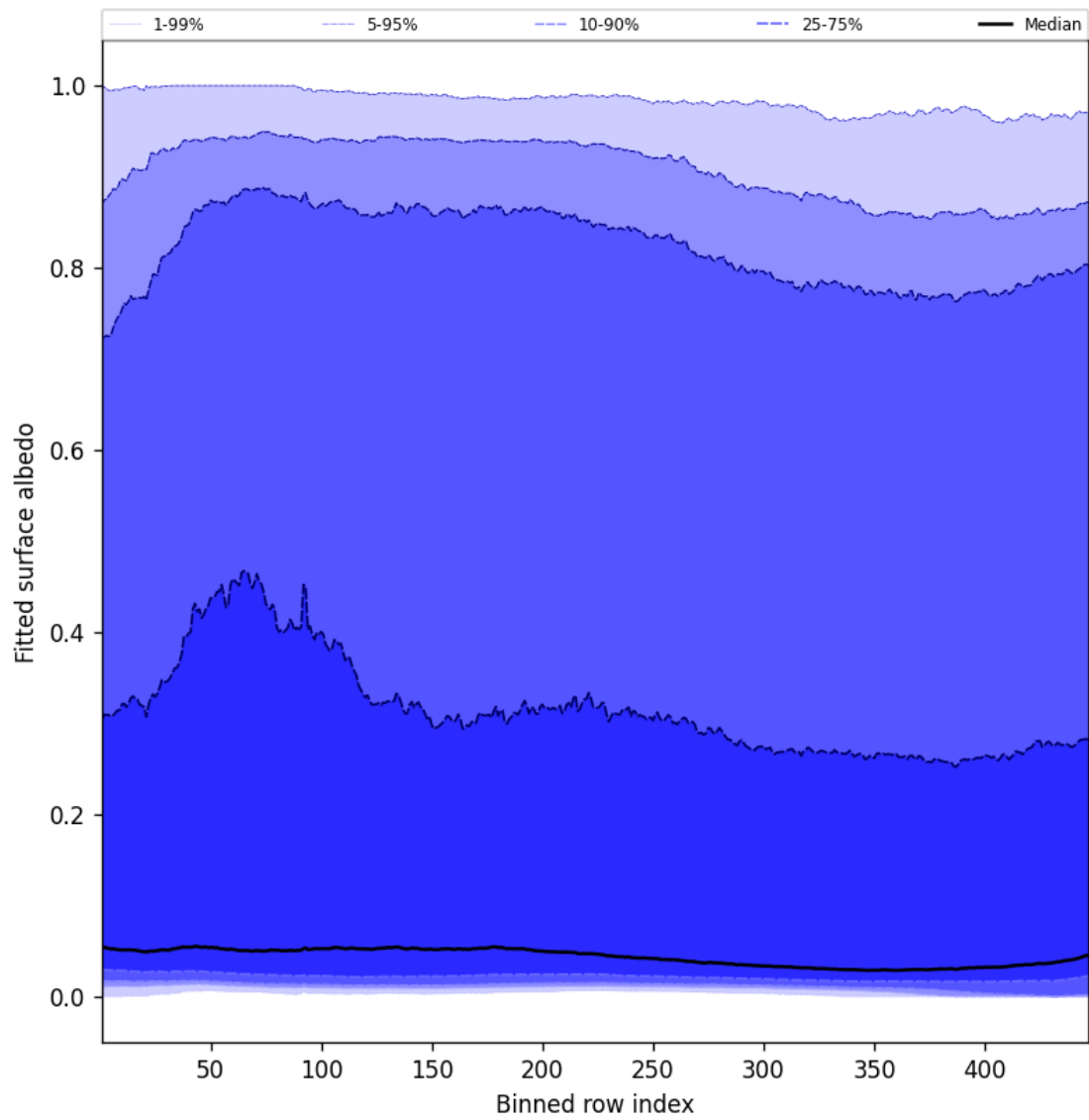
Figure 61: Along track statistics of “Fitted surface albedo” for 2025-04-27 to 2025-04-29
