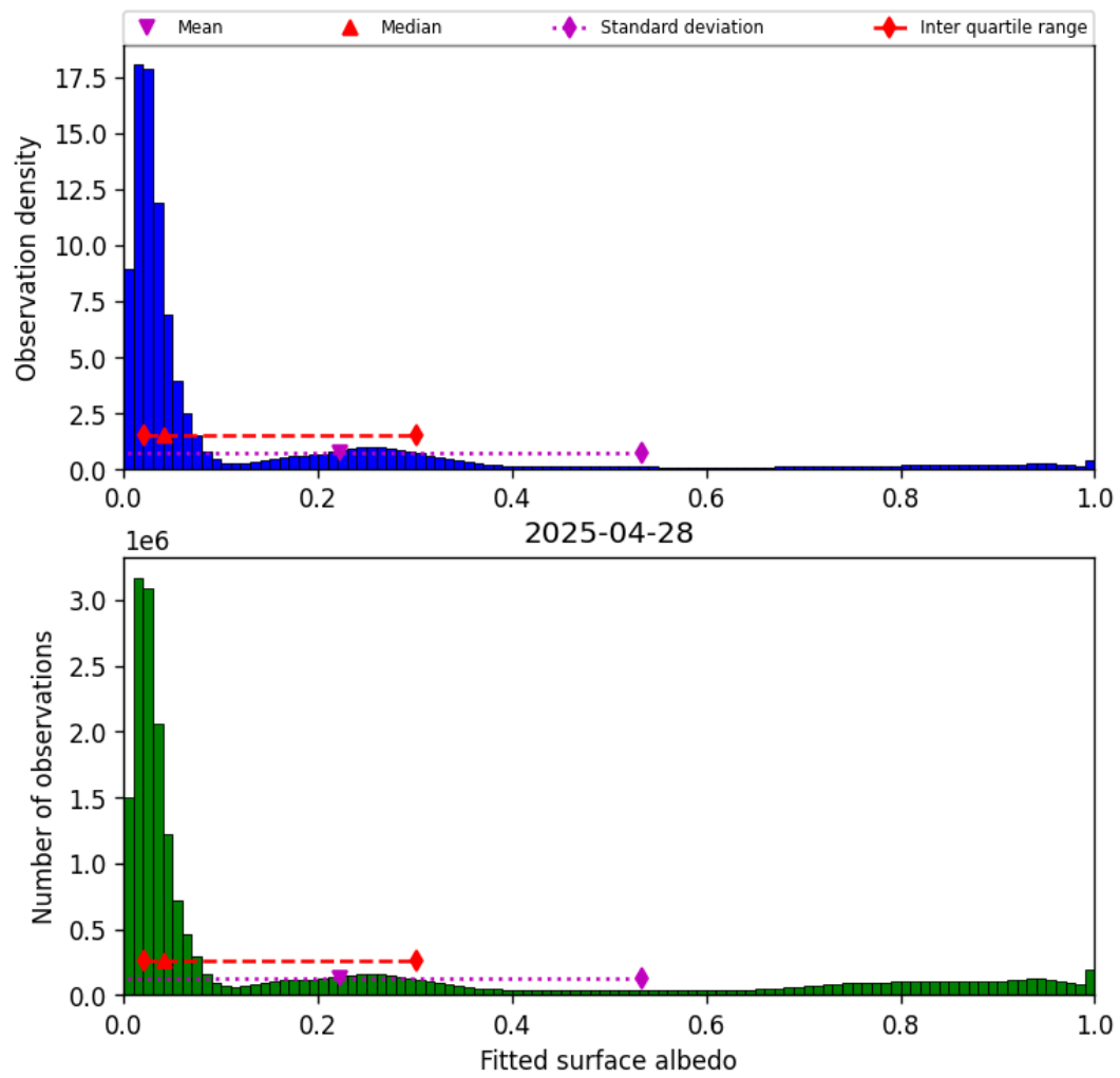
Figure 45: Histogram of “Fitted surface albedo” for 2025-04-27 to 2025-04-29
