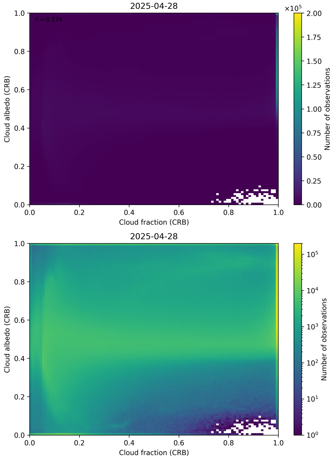
Figure 77: Scatter density plot of “Cloud fraction (CRB)” against “Cloud albedo (CRB)” for 2025-04-27 to 2025-04-29.
