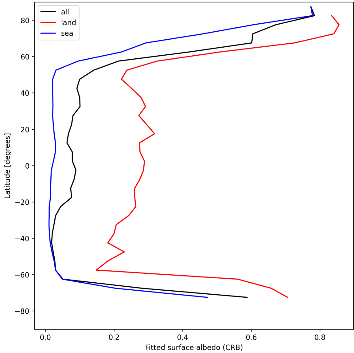
Figure 30: Zonal average of “Fitted surface albedo (CRB)” for 2025-04-27 to 2025-04-29.
