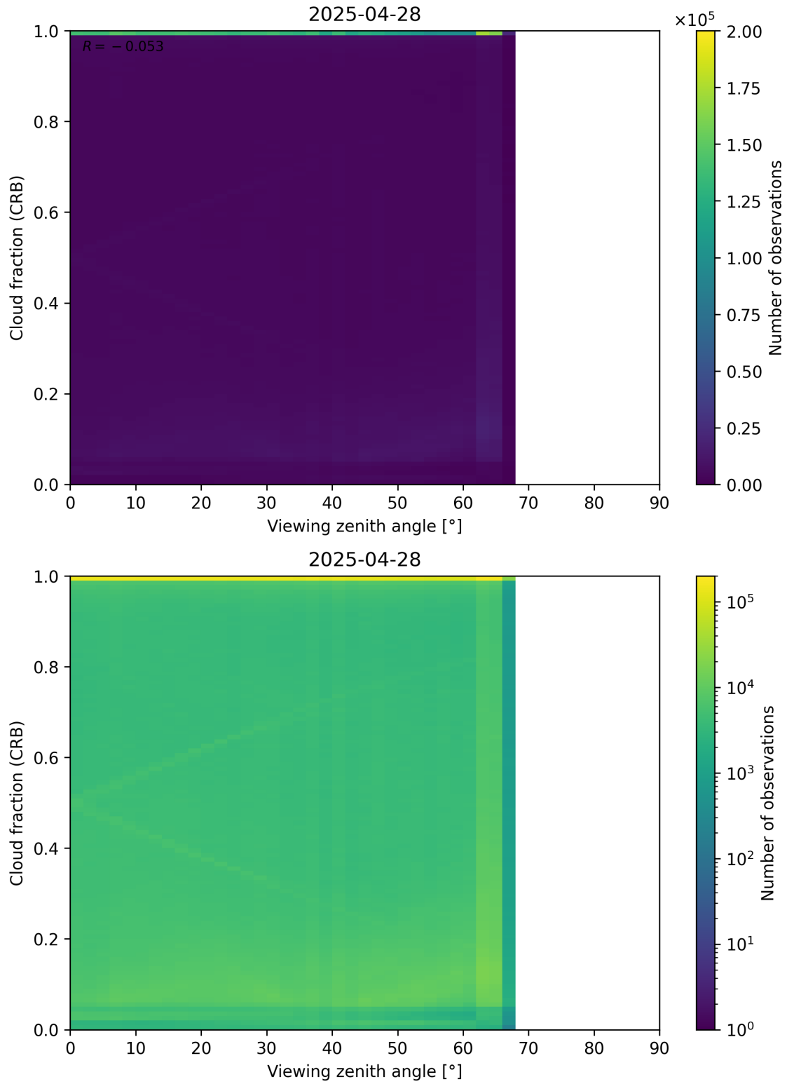
Figure 109: Scatter density plot of “Viewing zenith angle” against “Cloud fraction (CRB)” for 2025-04-27 to 2025-04-29.
