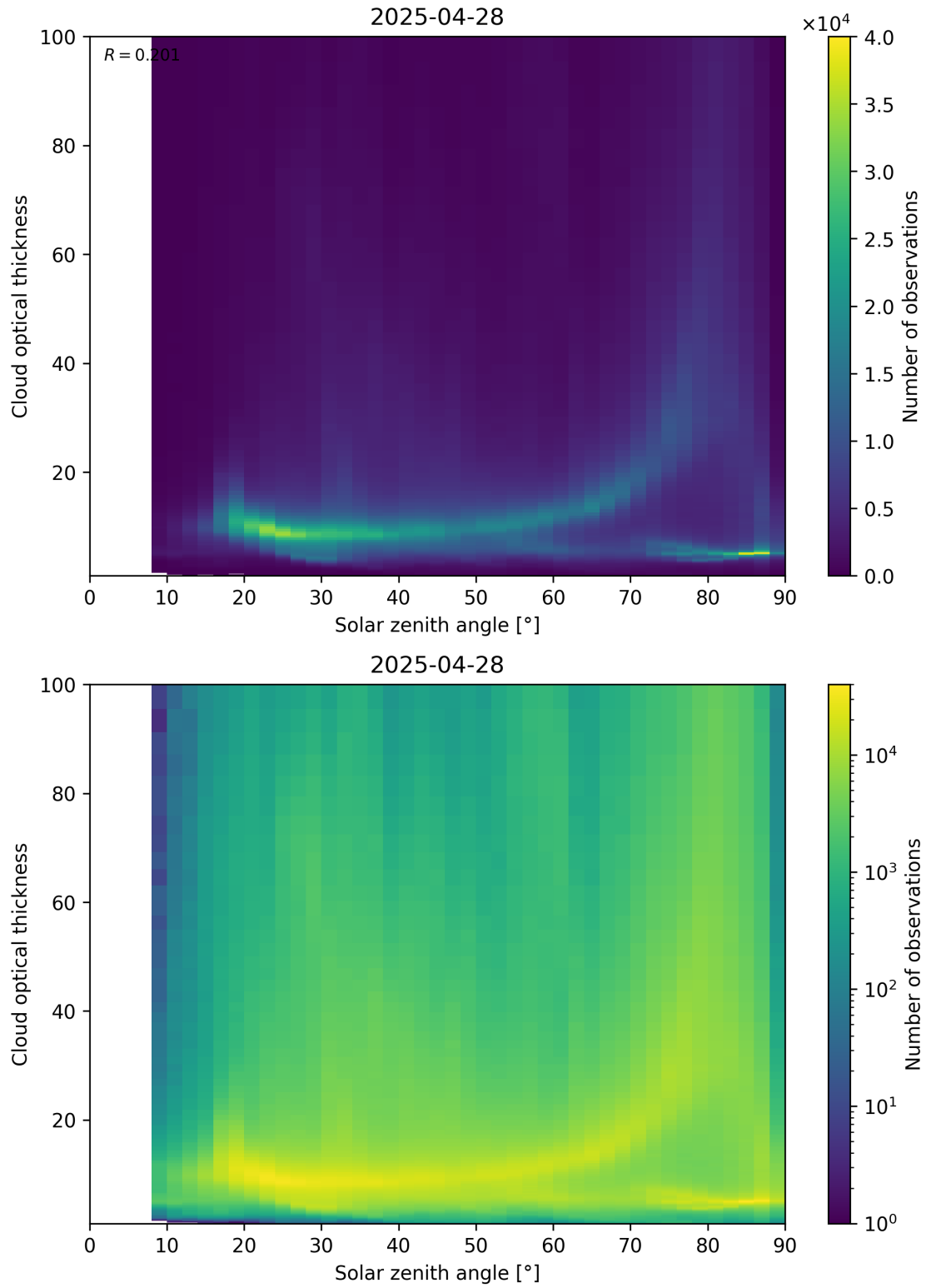
Figure 103: Scatter density plot of “Solar zenith angle” against “Cloud optical thickness” for 2025-04-27 to 2025-04-29.
