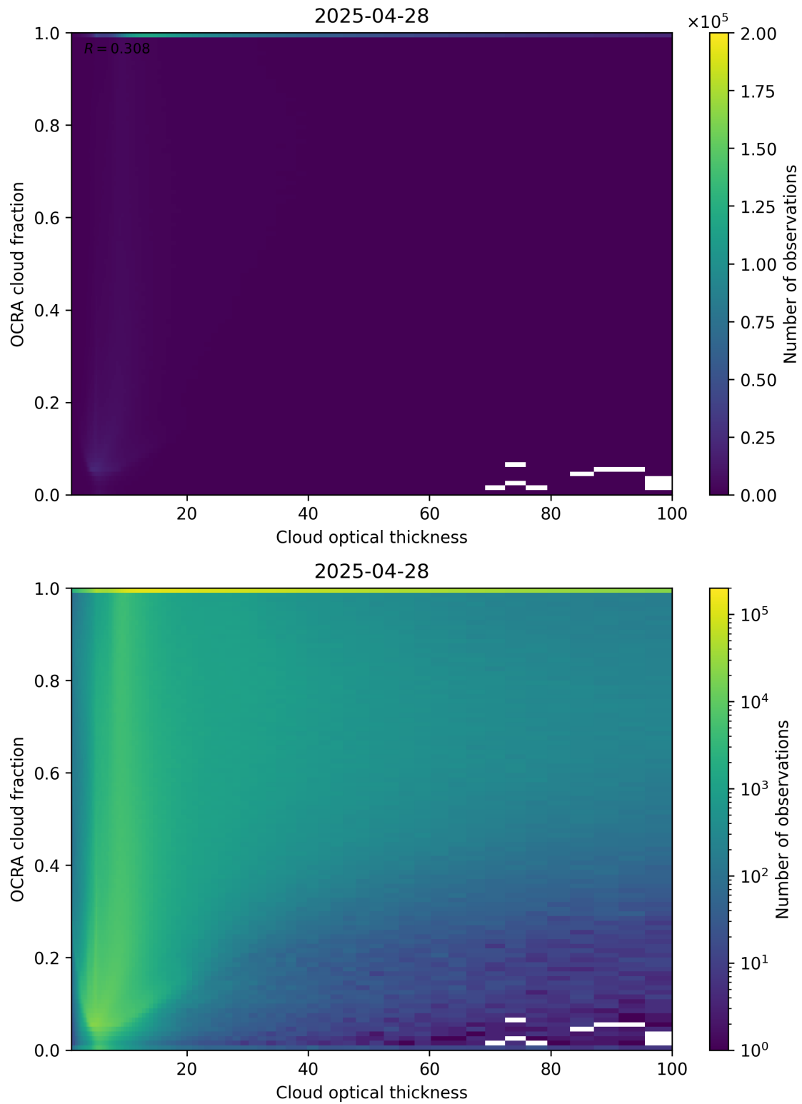
Figure 83: Scatter density plot of “Cloud optical thickness” against “OCRA cloud fraction” for 2025-04-27 to 2025-04-29.
