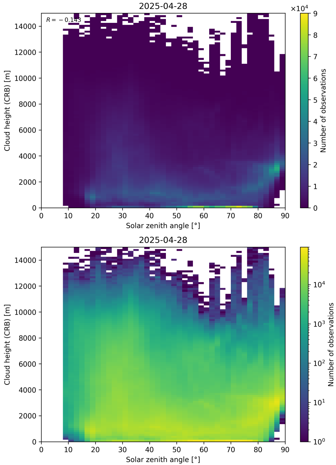
Figure 102: Scatter density plot of “Solar zenith angle” against “Cloud height (CRB)” for 2025-04-27 to 2025-04-29.
