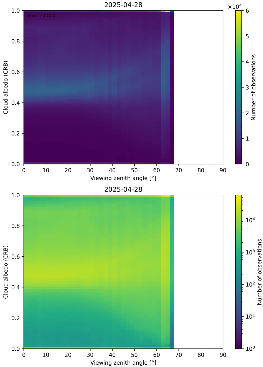
Figure 106: Scatter density plot of “Viewing zenith angle” against “Cloud albedo (CRB)” for 2025-04-27 to 2025-04-29.
