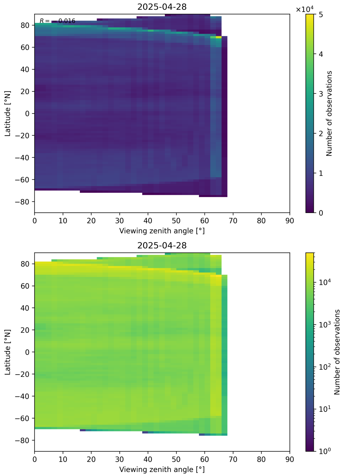
Figure 113: Scatter density plot of “Viewing zenith angle” against “Latitude” for 2025-04-27 to 2025-04-29.
