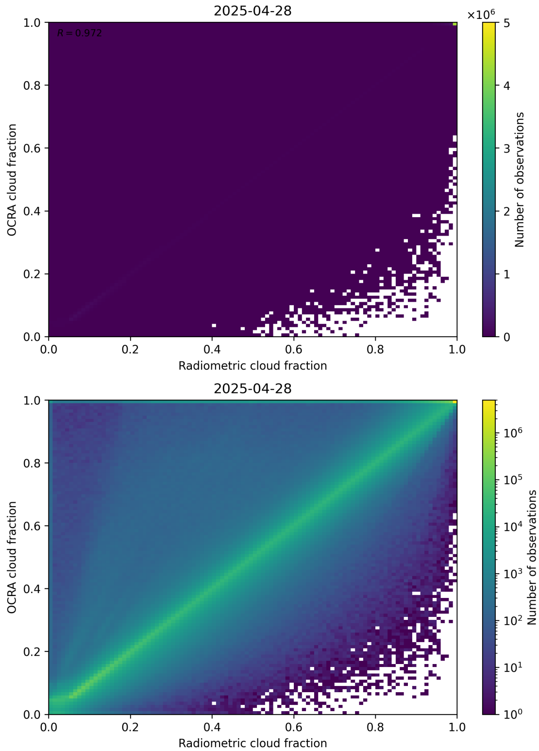
Figure 72: Scatter density plot of “Radiometric cloud fraction” against “OCRA cloud fraction” for 2025-04-27 to 2025-04-29.
