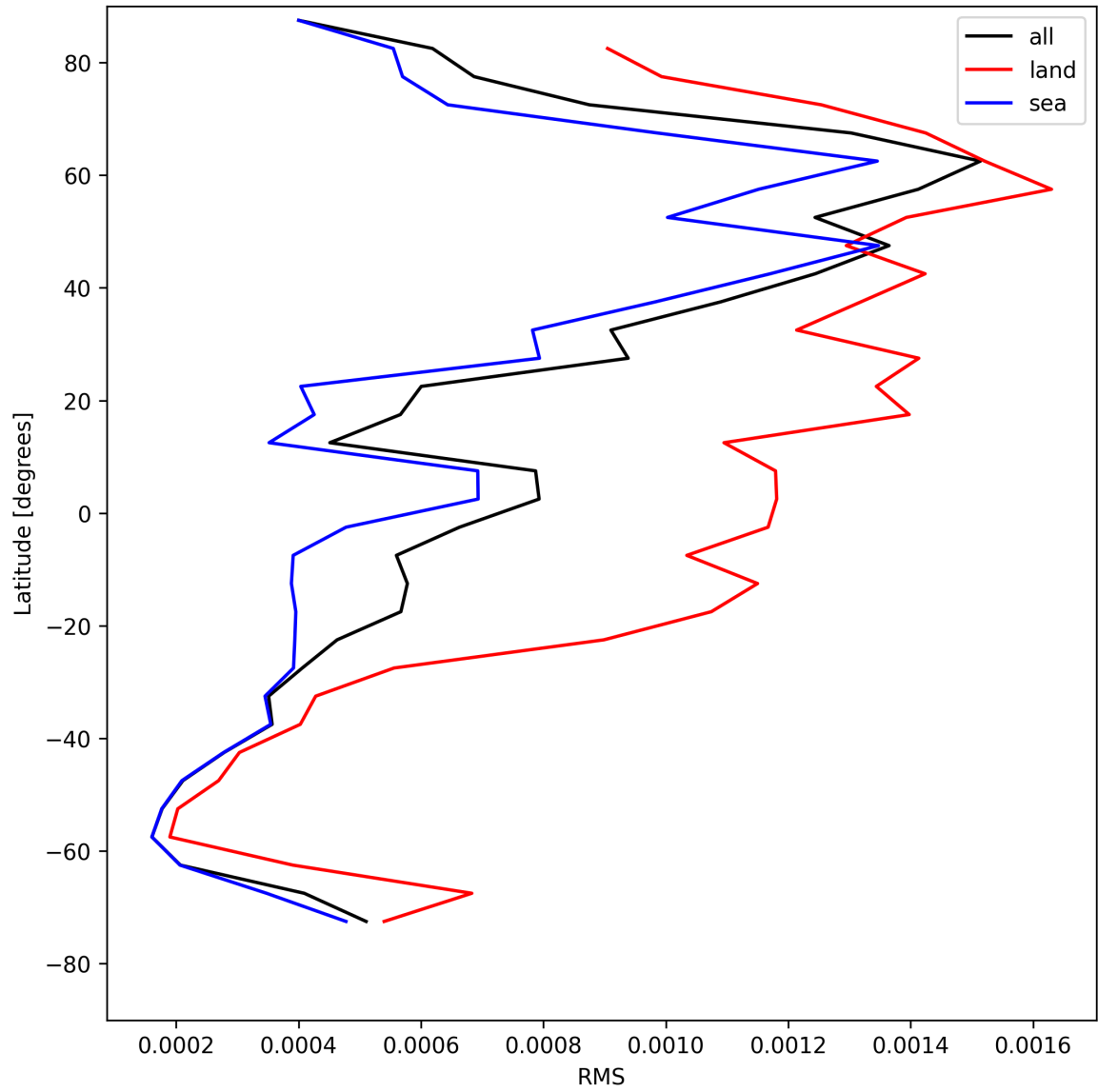
Figure 31: Zonal average of “RMS” for 2025-04-27 to 2025-04-29.
