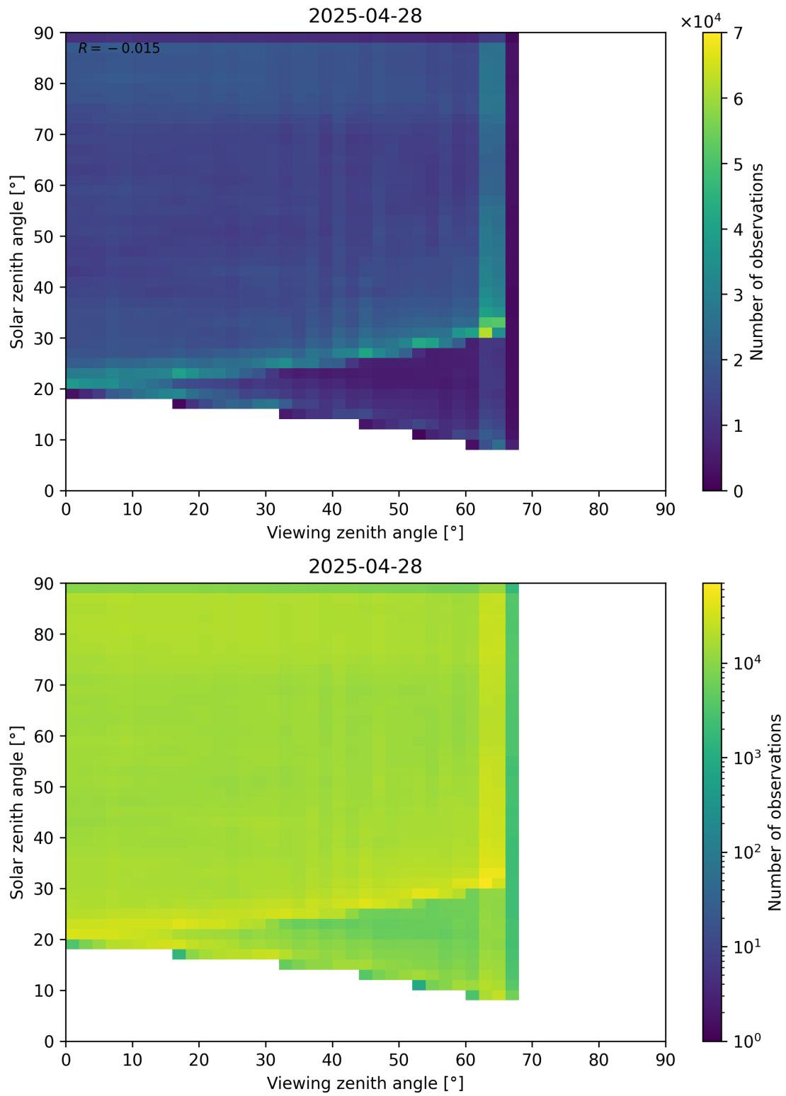
Figure 114: Scatter density plot of “Viewing zenith angle” against “Solar zenith angle” for 2025-04-27 to 2025-04-29.
