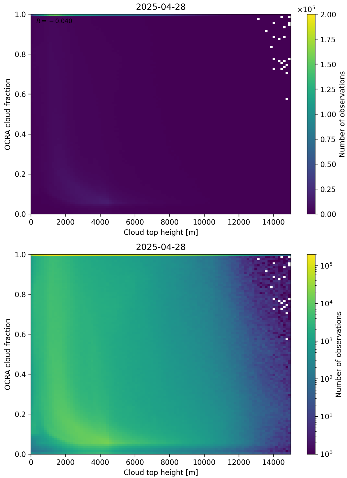
Figure 87: Scatter density plot of “Cloud top height” against “OCRA cloud fraction” for 2025-04-27 to 2025-04-29.
