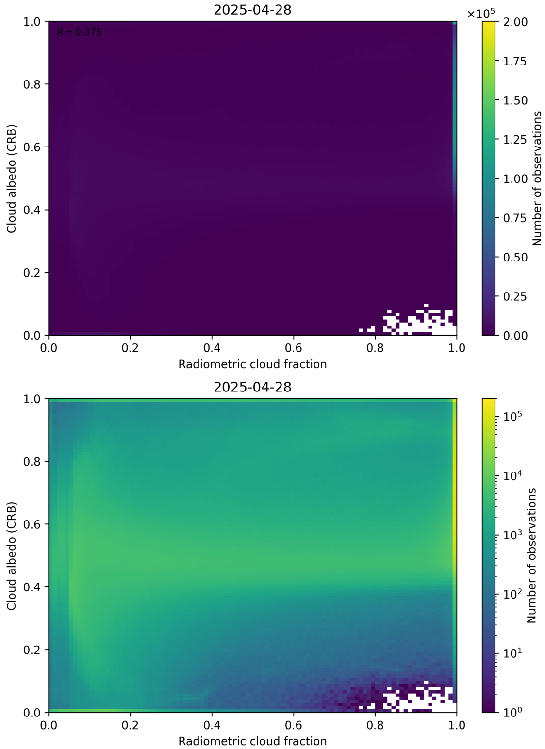
Figure 71: Scatter density plot of “Radiometric cloud fraction” against “Cloud albedo (CRB)” for 2025-04-27 to 2025-04-29.
