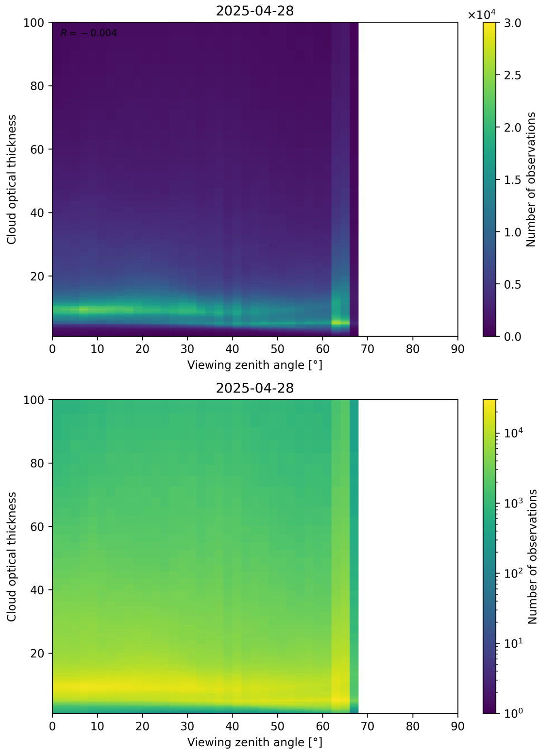
Figure 111: Scatter density plot of “Viewing zenith angle” against “Cloud optical thickness” for 2025-04-27 to 2025-04-29.
