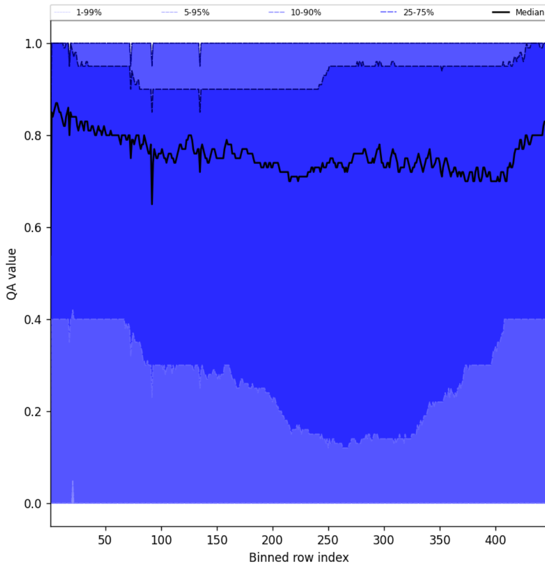
Figure 54: Along track statistics of “QA value” for 2025-04-27 to 2025-04-29
