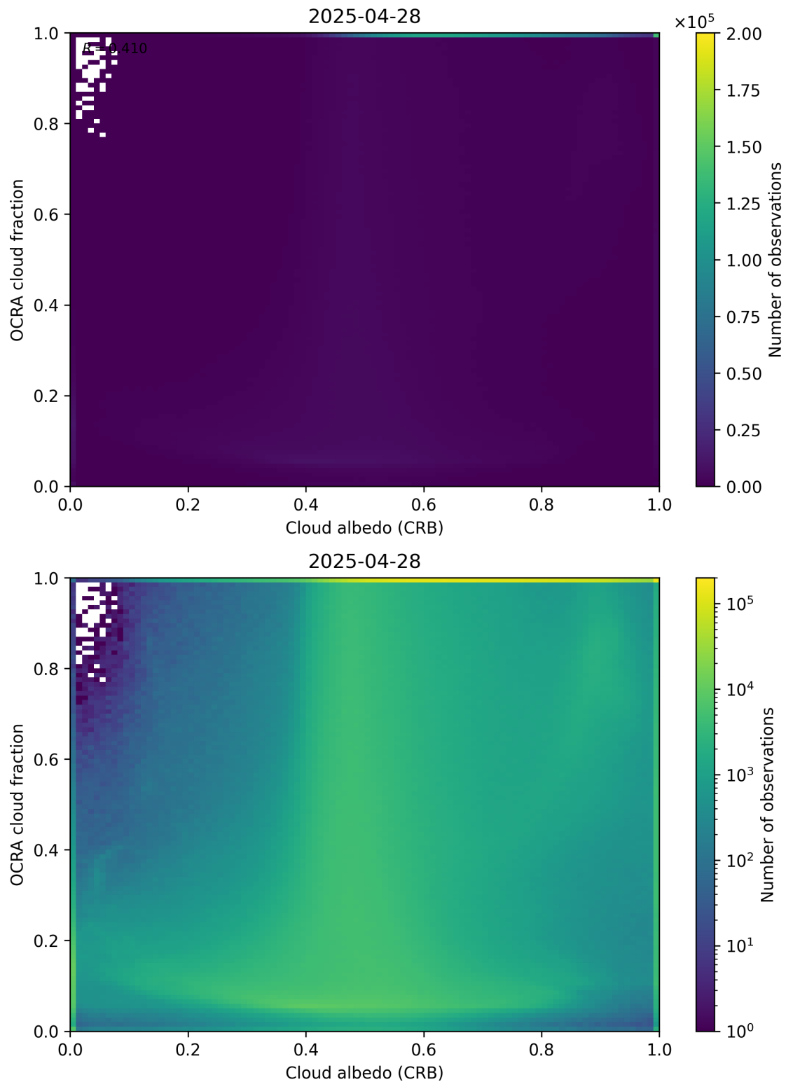
Figure 70: Scatter density plot of “Cloud albedo (CRB)” against “OCRA cloud fraction” for 2025-04-27 to 2025-04-29.
