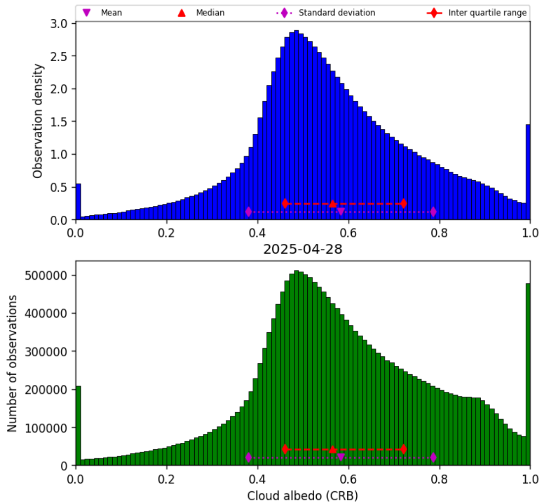
Figure 44: Histogram of “Cloud albedo (CRB)” for 2025-04-27 to 2025-04-29
