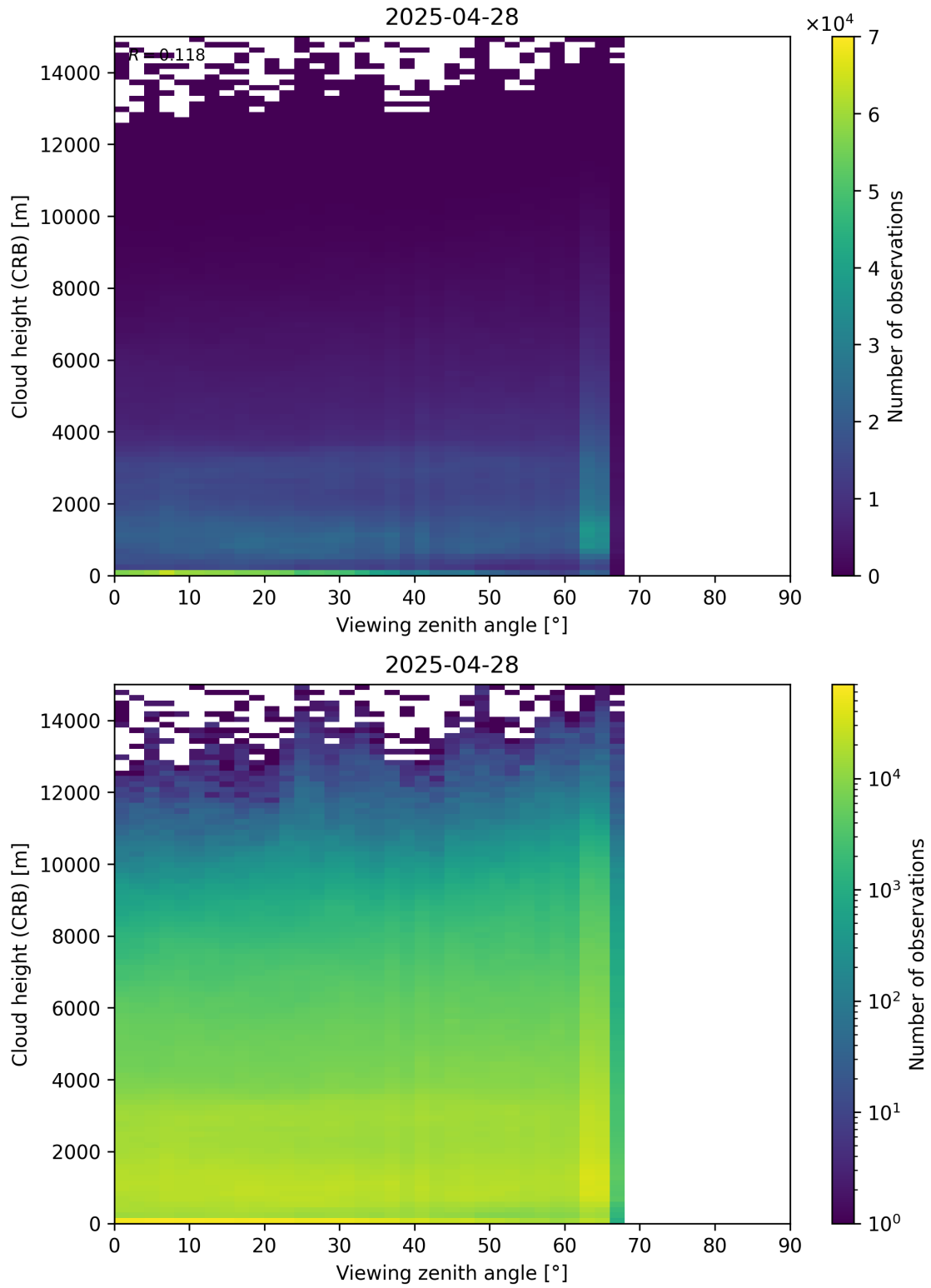
Figure 110: Scatter density plot of “Viewing zenith angle” against “Cloud height (CRB)” for 2025-04-27 to 2025-04-29.
