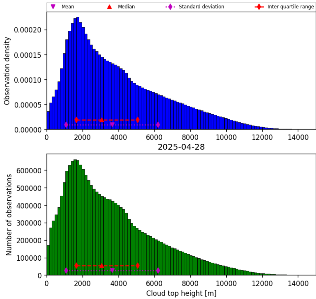
Figure 40: Histogram of “Cloud top height” for 2025-04-27 to 2025-04-29
