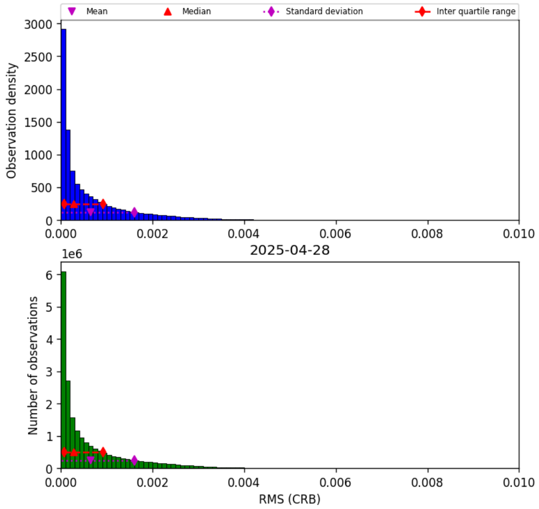
Figure 48: Histogram of “RMS (CRB)” for 2025-04-27 to 2025-04-29
