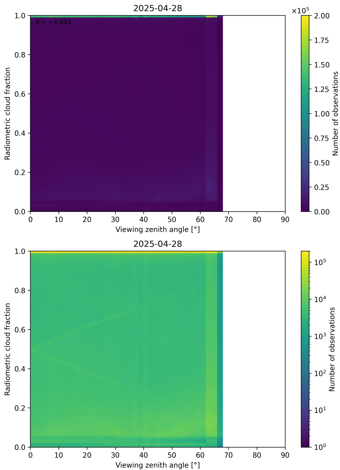
Figure 107: Scatter density plot of “Viewing zenith angle” against “Radiometric cloud fraction” for 2025-04-27 to 2025-04-29.
