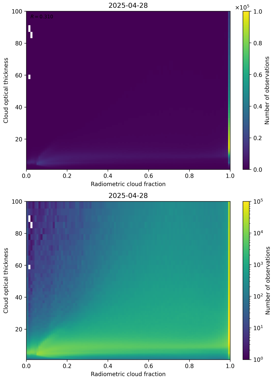
Figure 75: Scatter density plot of “Radiometric cloud fraction” against “Cloud optical thickness” for 2025-04-27 to 2025-04-29.
