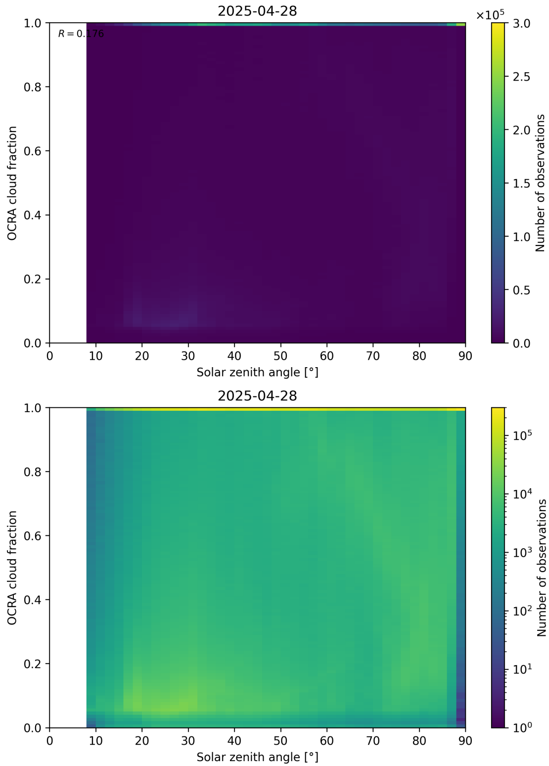
Figure 100: Scatter density plot of “Solar zenith angle” against “OCRA cloud fraction” for 2025-04-27 to 2025-04-29.
