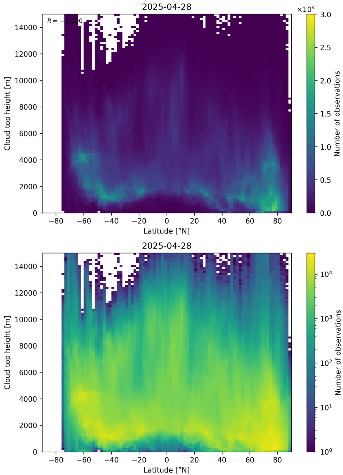
Figure 97: Scatter density plot of “Latitude” against “Cloud top height” for 2025-04-27 to 2025-04-29.
