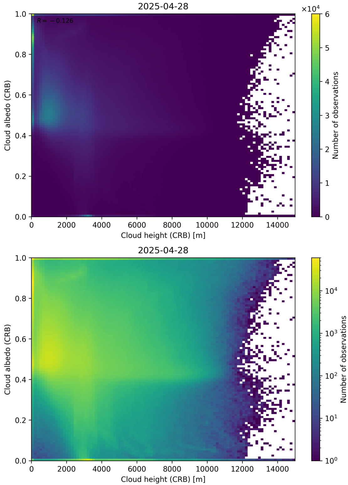
Figure 80: Scatter density plot of “Cloud height (CRB)” against “Cloud albedo (CRB)” for 2025-04-27 to 2025-04-29.
