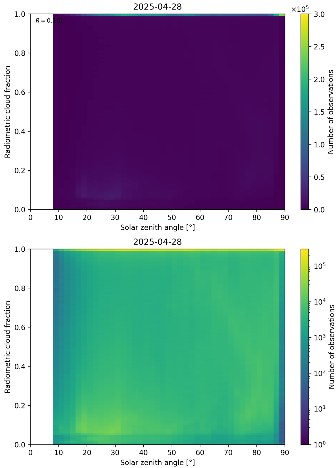
Figure 99: Scatter density plot of “Solar zenith angle” against “Radiometric cloud fraction” for 2025-04-27 to 2025-04-29.
