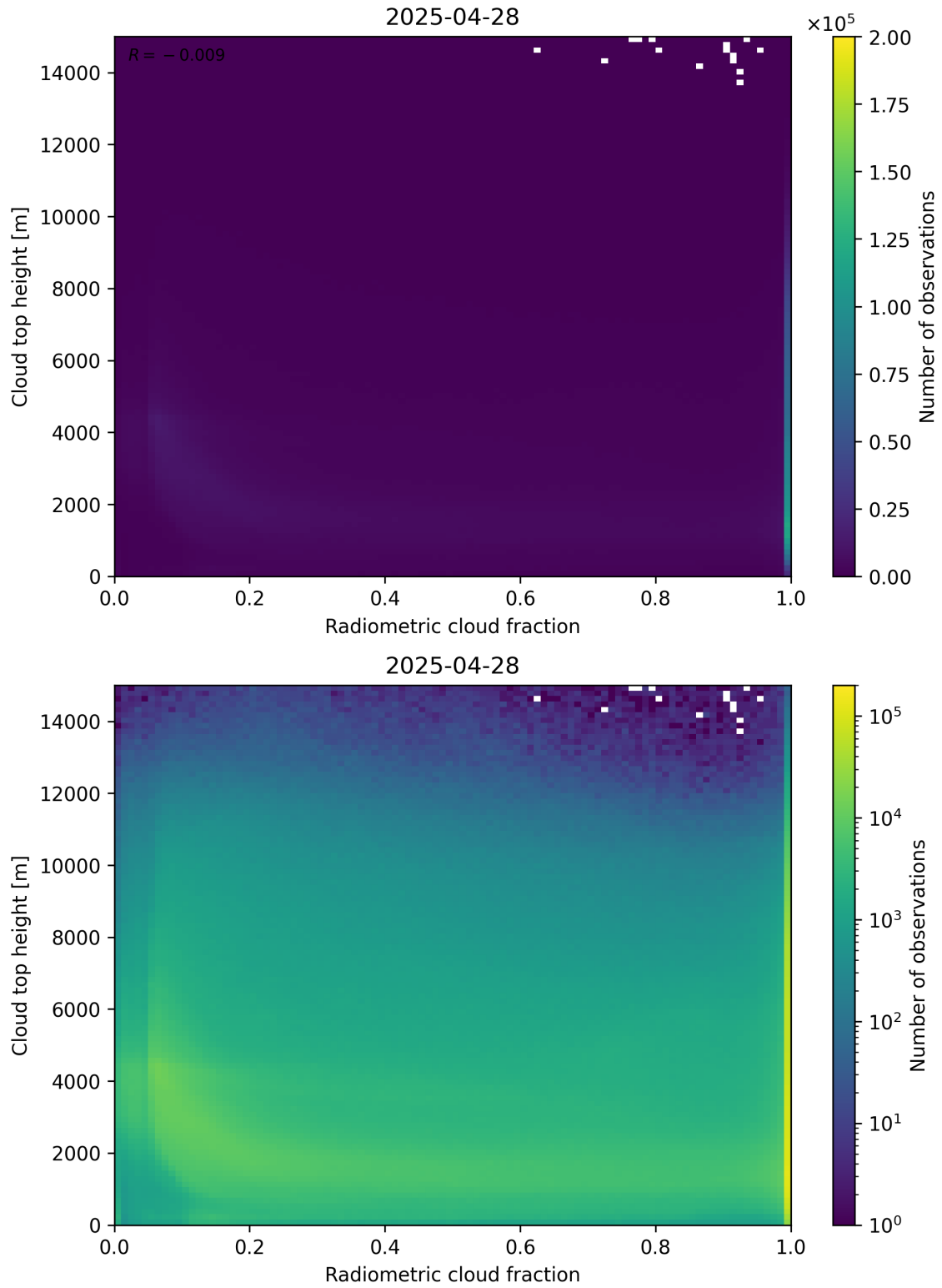
Figure 76: Scatter density plot of “Radiometric cloud fraction” against “Cloud top height” for 2025-04-27 to 2025-04-29.
