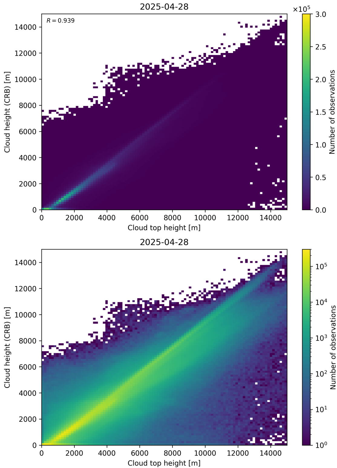
Figure 89: Scatter density plot of “Cloud top height” against “Cloud height (CRB)” for 2025-04-27 to 2025-04-29.
