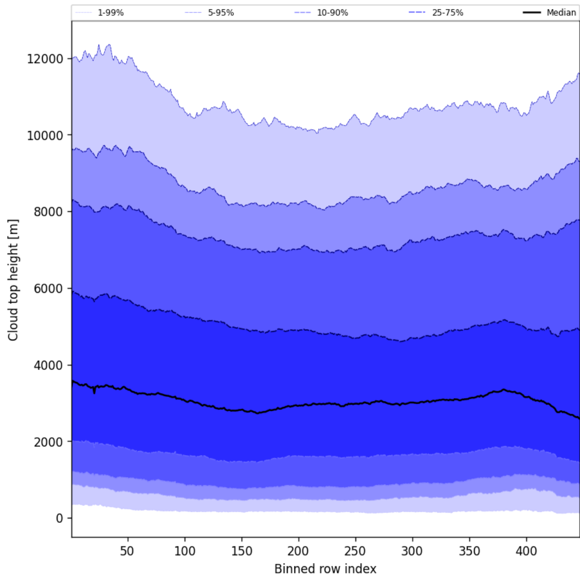
Figure 56: Along track statistics of “Cloud top height” for 2025-04-27 to 2025-04-29
