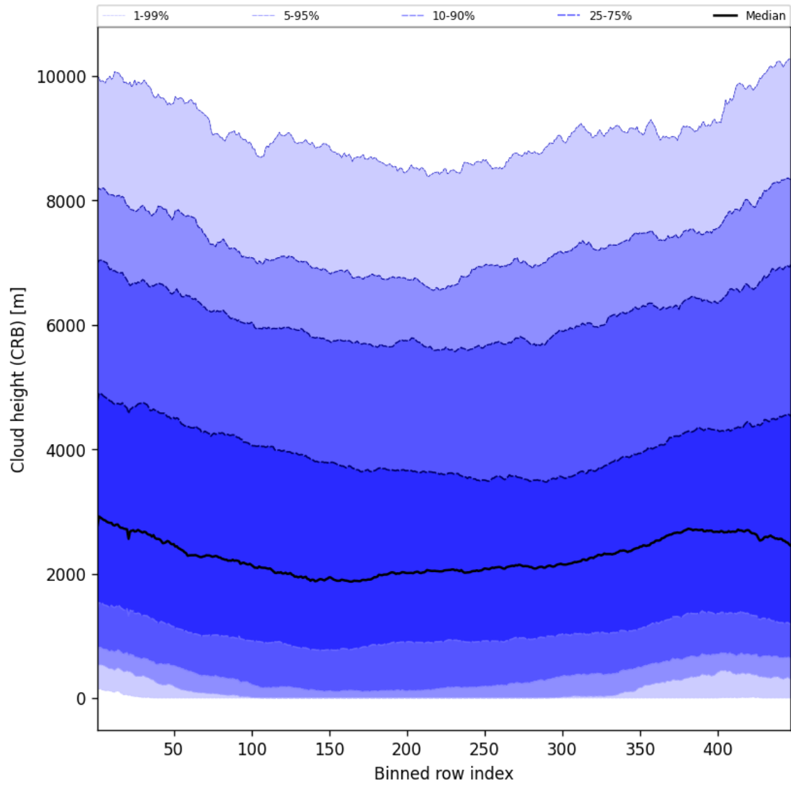
Figure 59: Along track statistics of “Cloud height (CRB)” for 2025-04-27 to 2025-04-29
