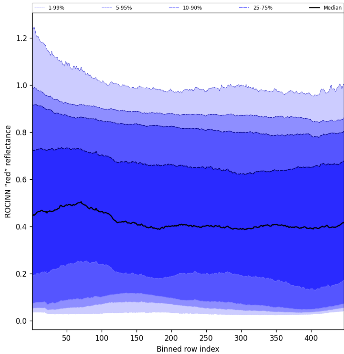
Figure 69: Along track statistics of "ROCINN "red" reflectance" for 2025-04-27 to 2025-04-29
