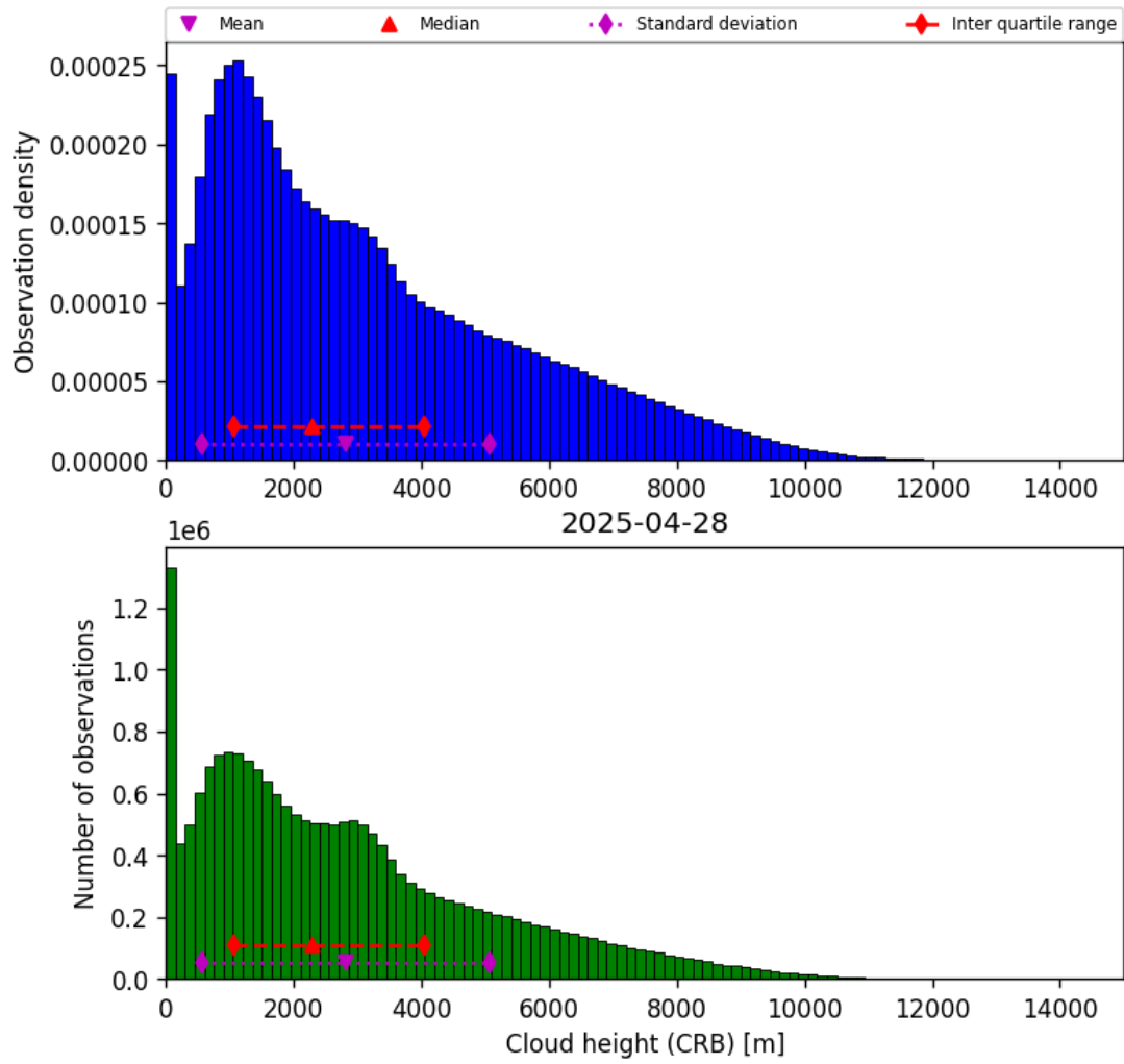
Figure 43: Histogram of “Cloud height (CRB)” for 2025-04-27 to 2025-04-29
