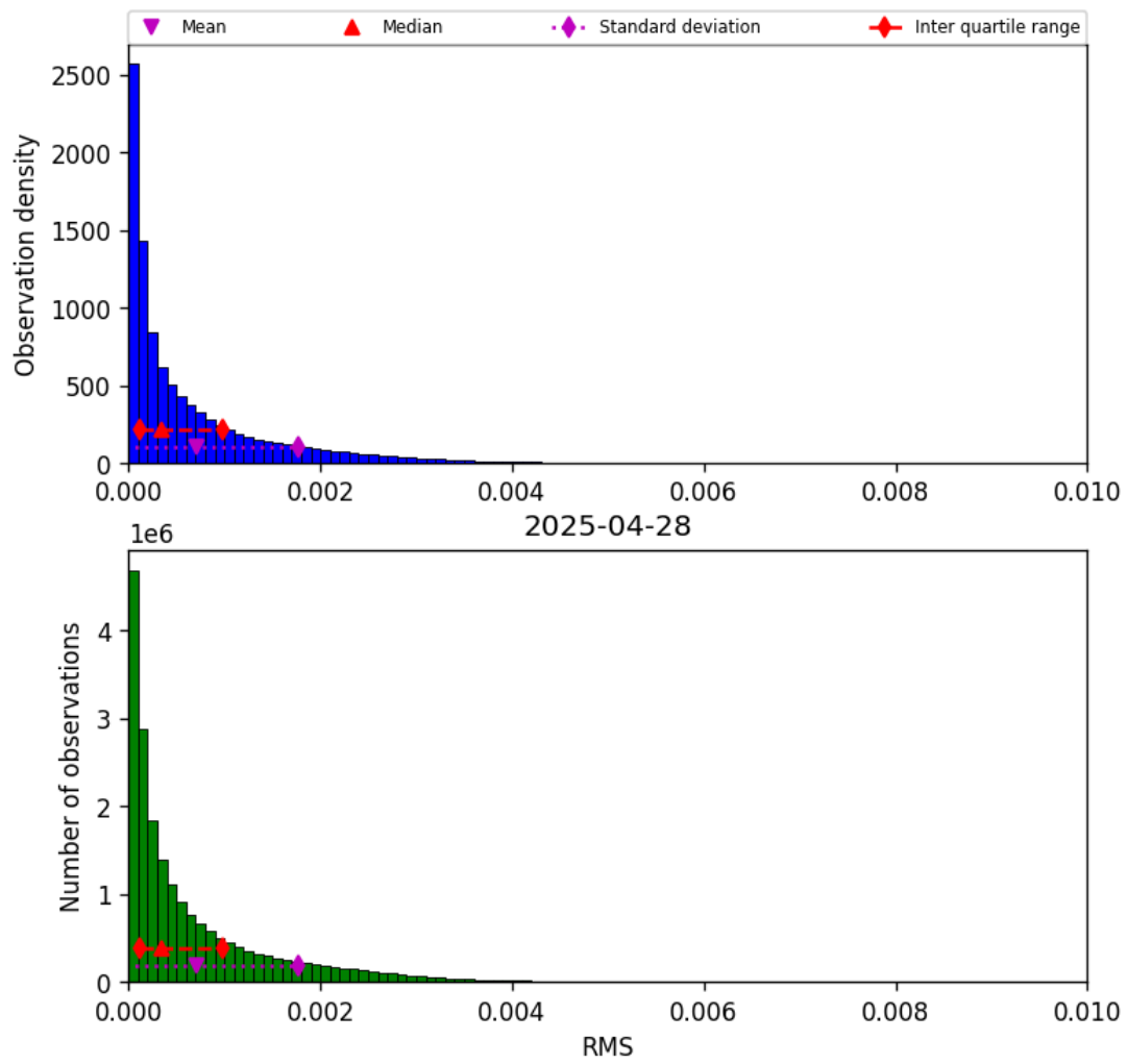
Figure 47: Histogram of “RMS” for 2025-04-27 to 2025-04-29
