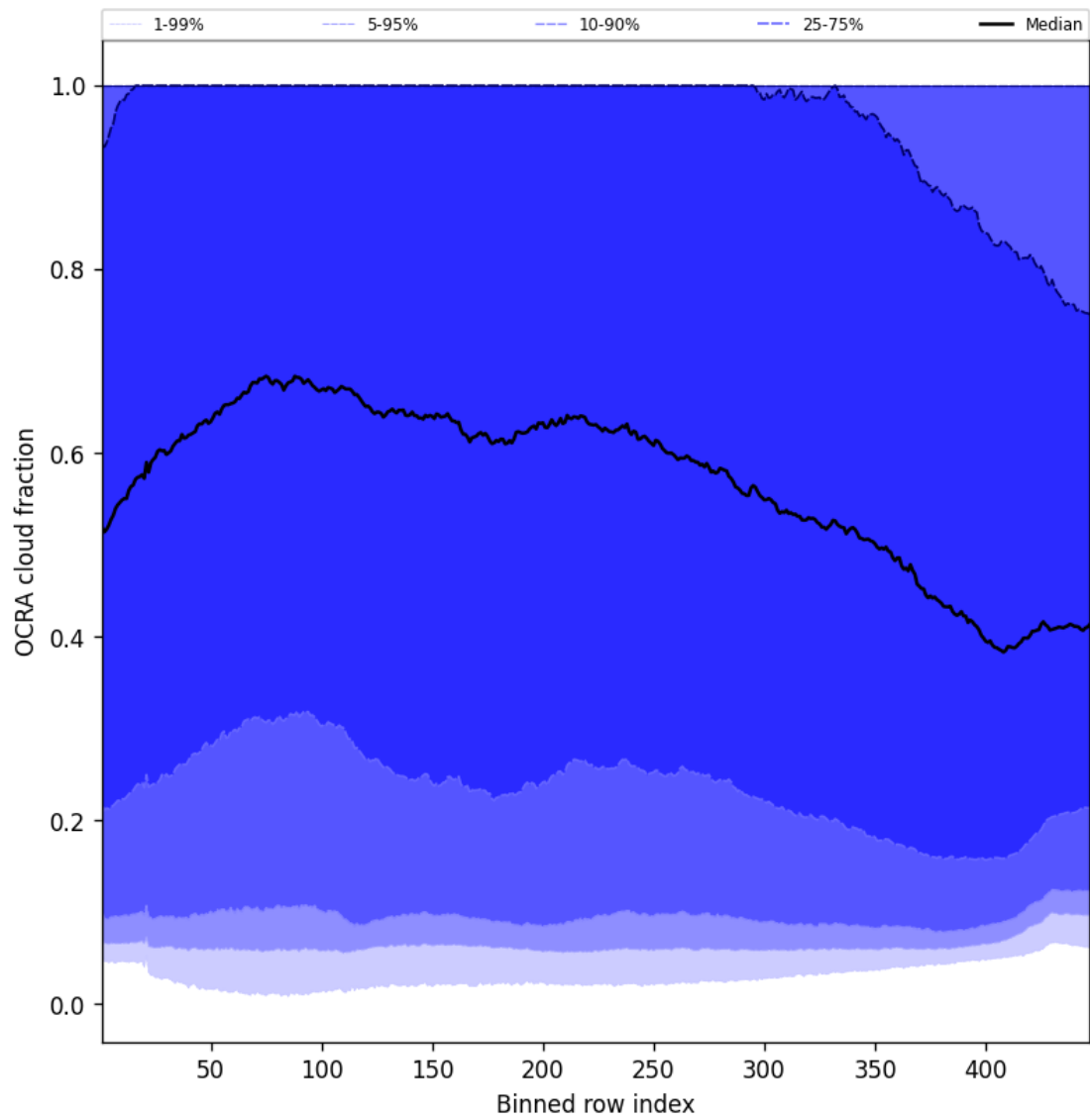
Figure 66: Along track statistics of “OCRA cloud fraction” for 2025-04-27 to 2025-04-29
