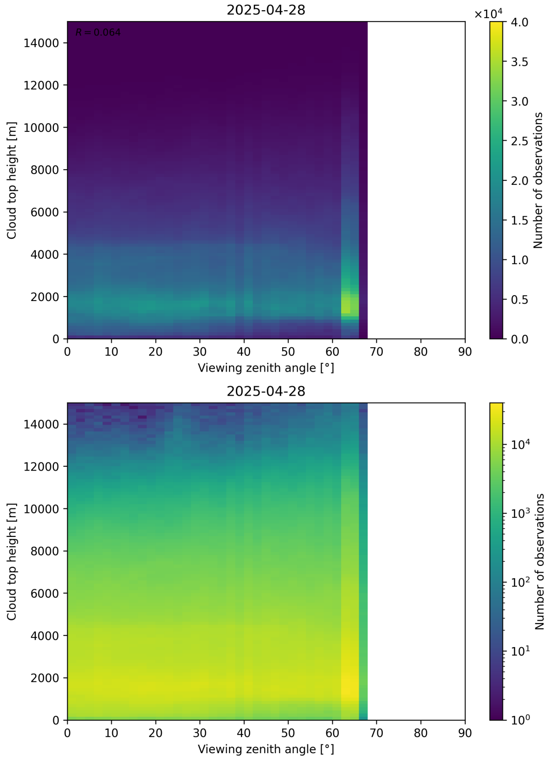
Figure 112: Scatter density plot of “Viewing zenith angle” against “Cloud top height” for 2025-04-27 to 2025-04-29.
