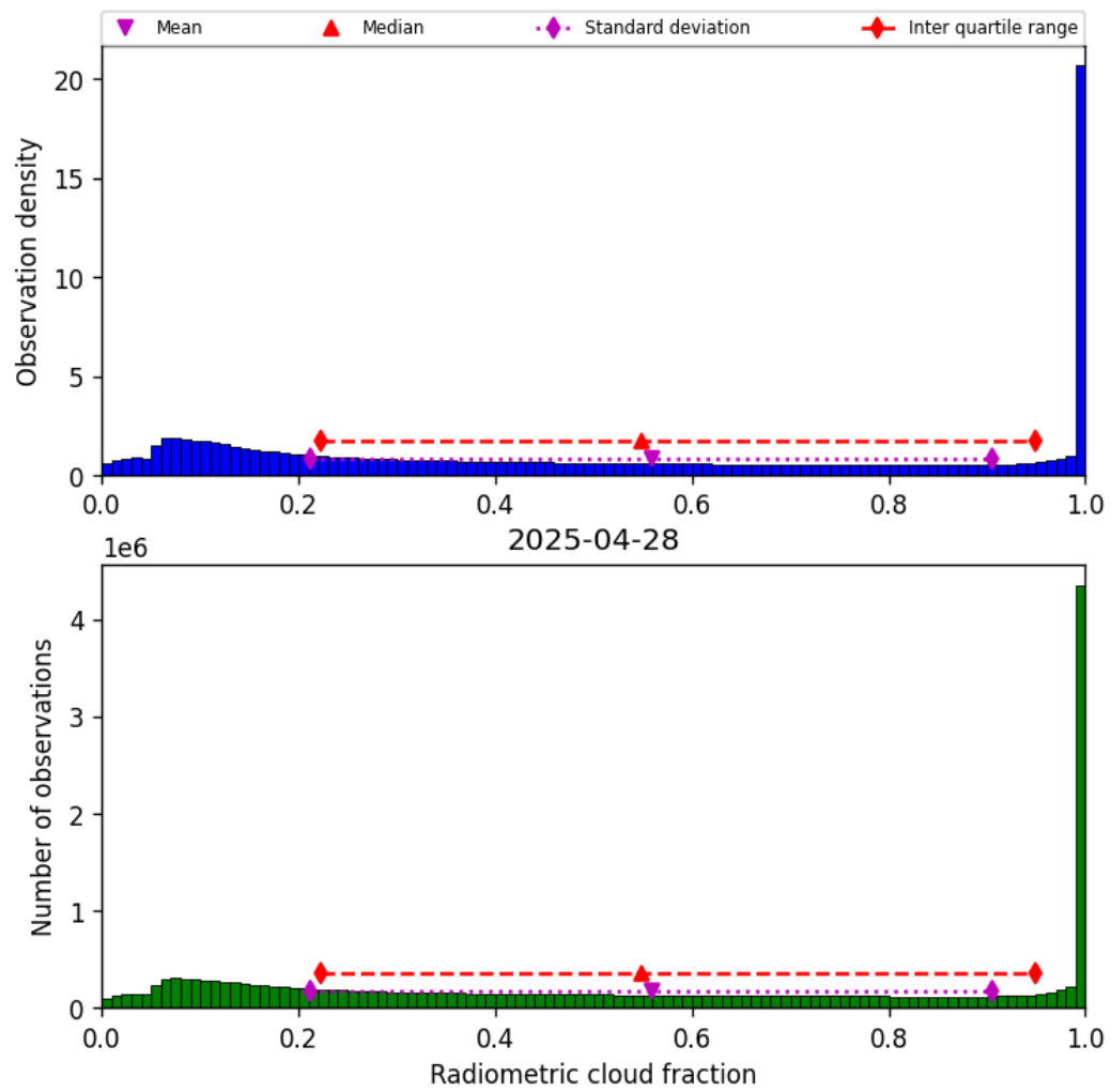
Figure 39: Histogram of “Radiometric cloud fraction” for 2025-04-27 to 2025-04-29
