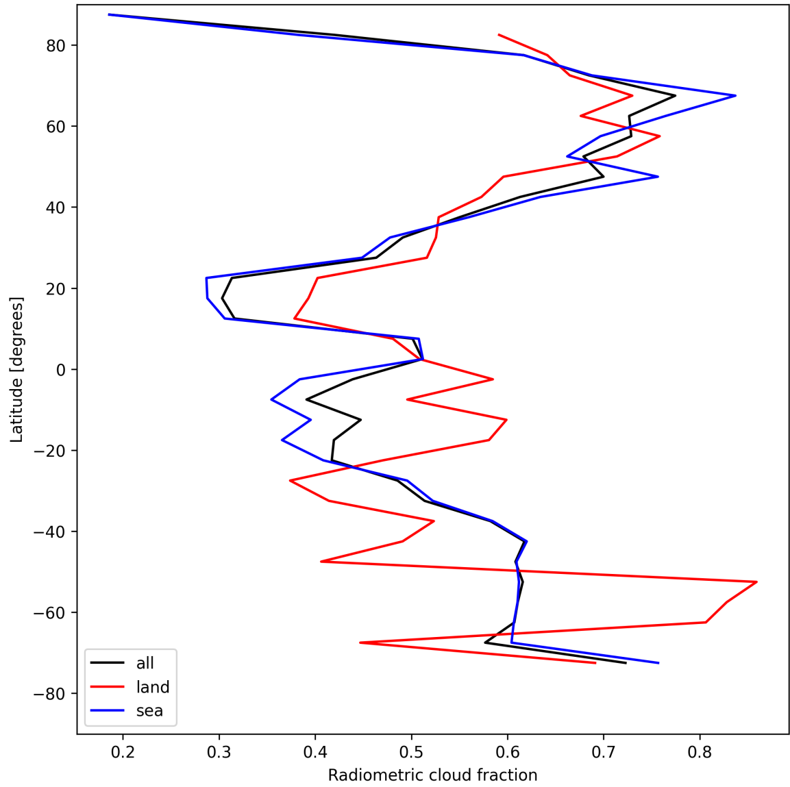
Figure 23: Zonal average of “Radiometric cloud fraction” for 2025-04-27 to 2025-04-29.
