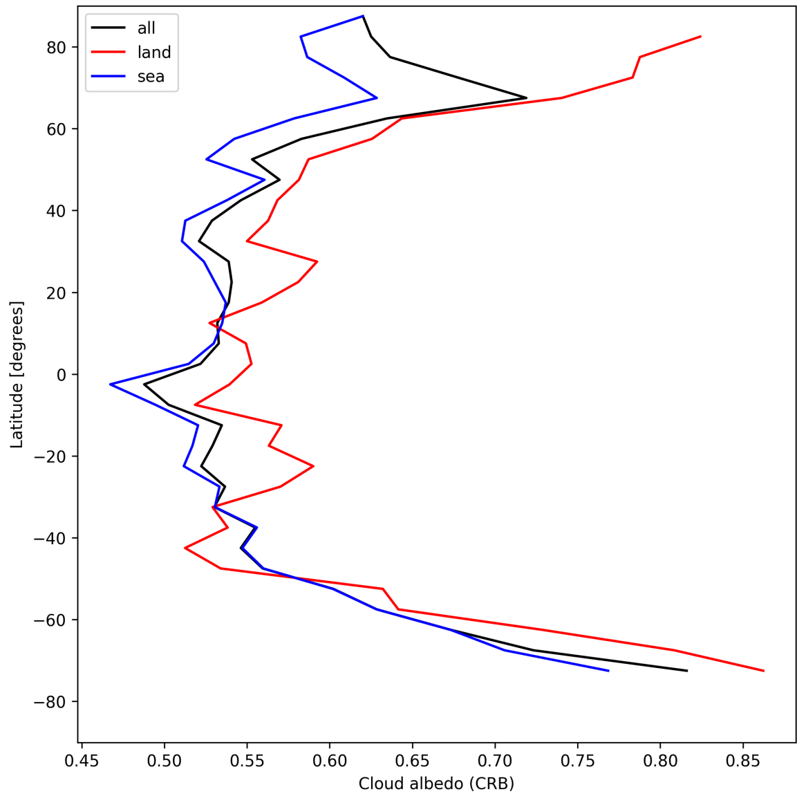
Figure 28: Zonal average of “Cloud albedo (CRB)” for 2025-04-27 to 2025-04-29.
