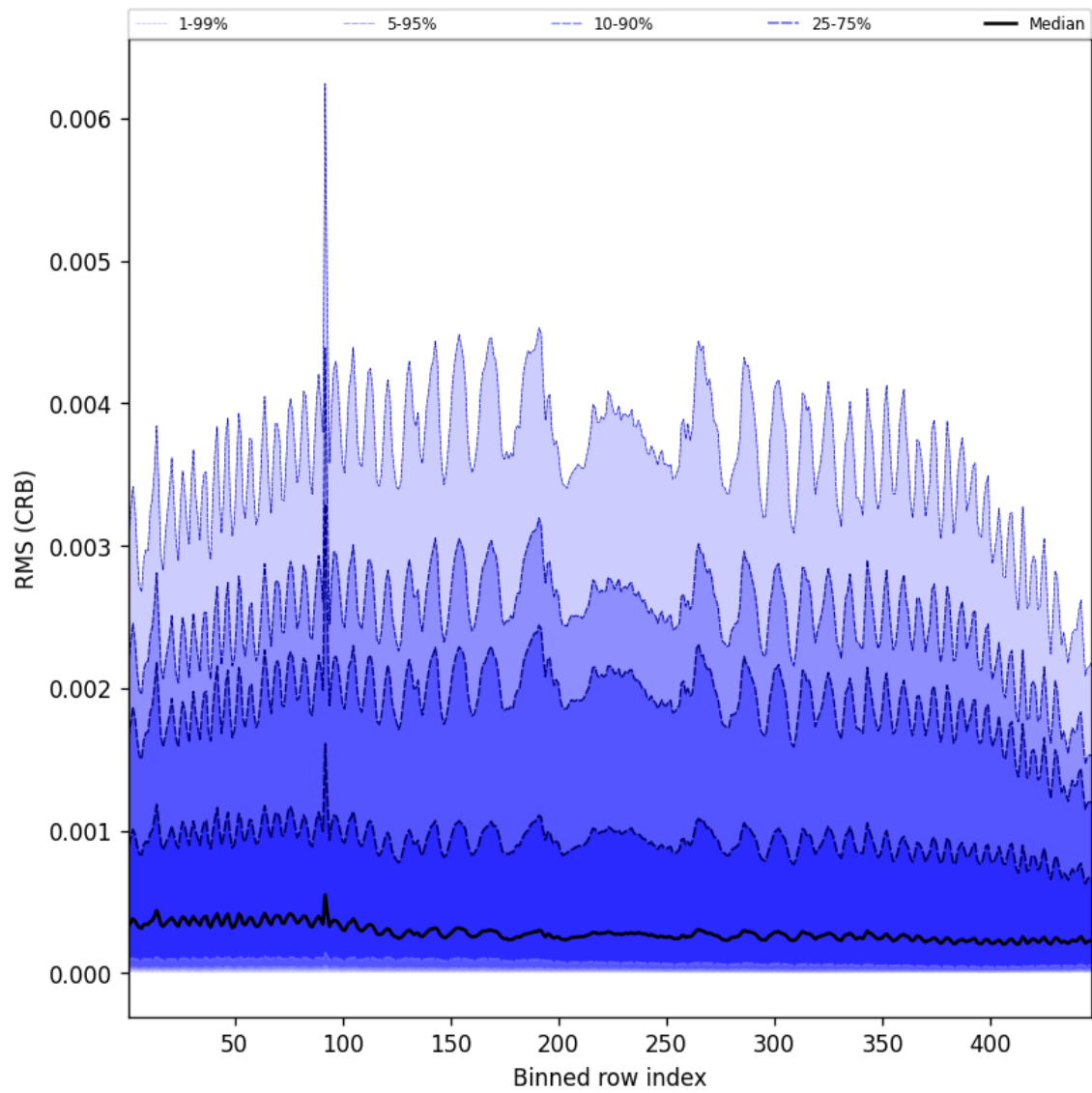
Figure 64: Along track statistics of “RMS (CRB)” for 2025-04-27 to 2025-04-29
