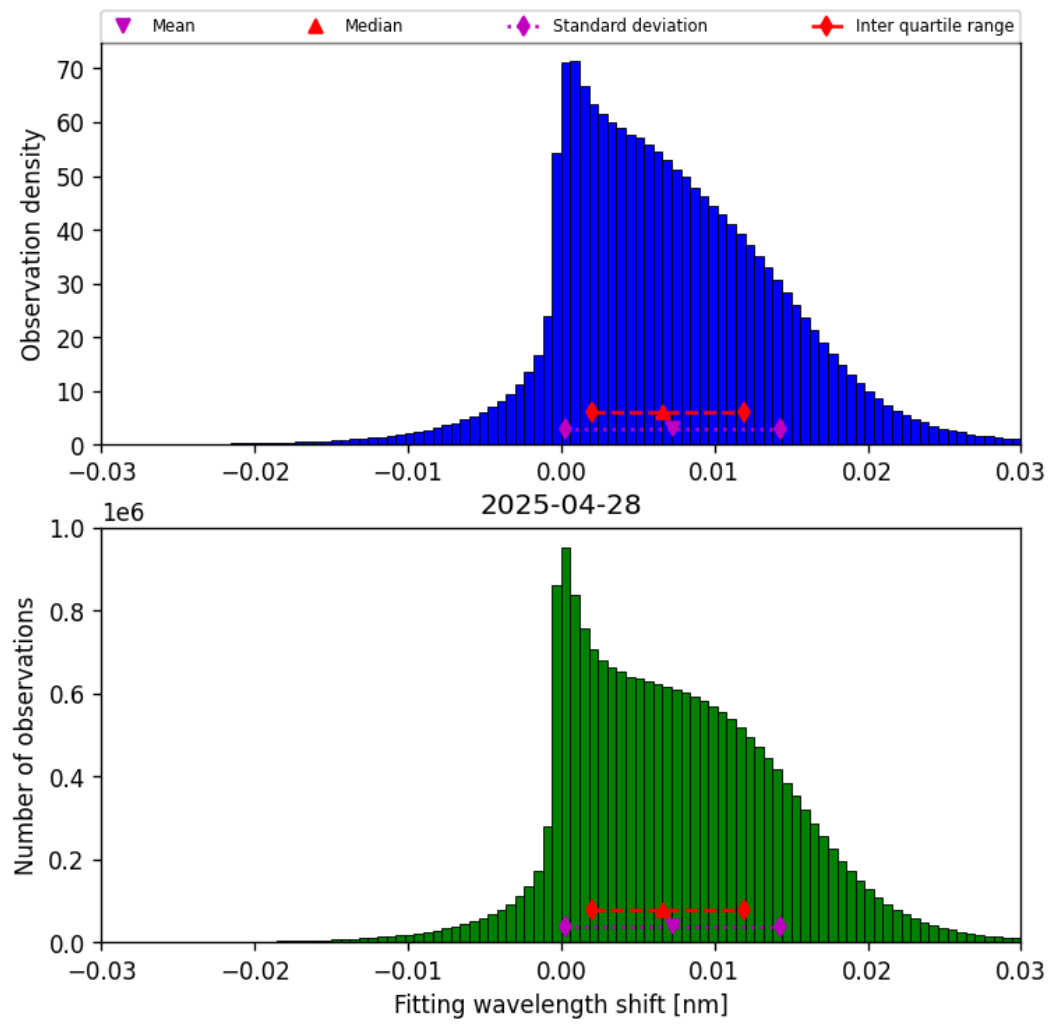
Figure 49: Histogram of “Fitting wavelength shift” for 2025-04-27 to 2025-04-29
