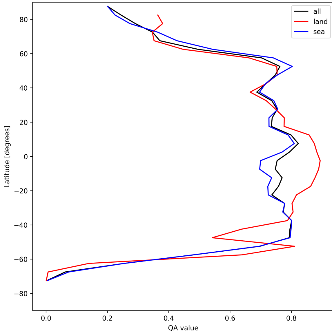
Figure 22: Zonal average of “QA value” for 2025-04-27 to 2025-04-29.
