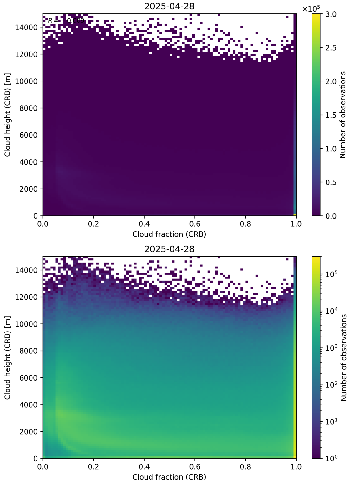
Figure 79: Scatter density plot of “Cloud fraction (CRB)” against “Cloud height (CRB)” for 2025-04-27 to 2025-04-29.
