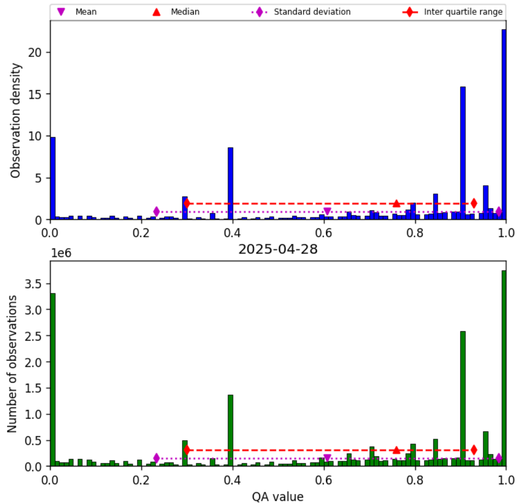
Figure 38: Histogram of “QA value” for 2025-04-27 to 2025-04-29
