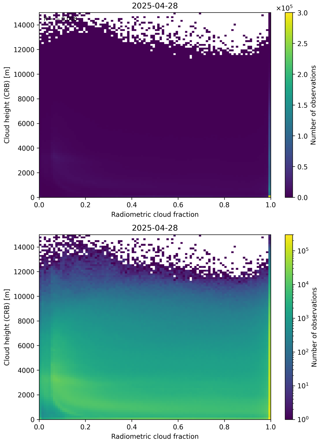
Figure 74: Scatter density plot of “Radiometric cloud fraction” against “Cloud height (CRB)” for 2025-04-27 to 2025-04-29.
