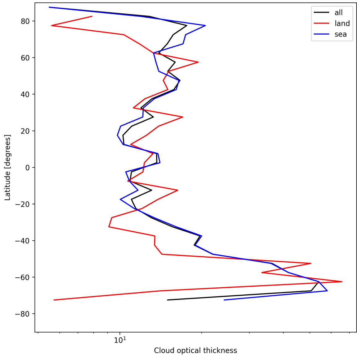
Figure 25: Zonal average of “Cloud optical thickness” for 2025-04-27 to 2025-04-29.
