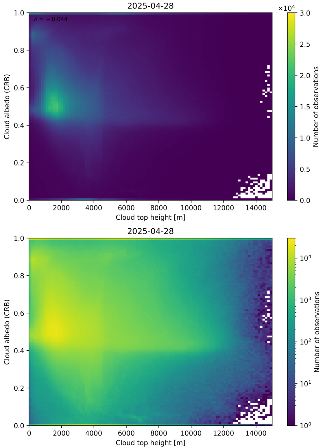
Figure 86: Scatter density plot of “Cloud top height” against “Cloud albedo (CRB)” for 2025-04-27 to 2025-04-29.
