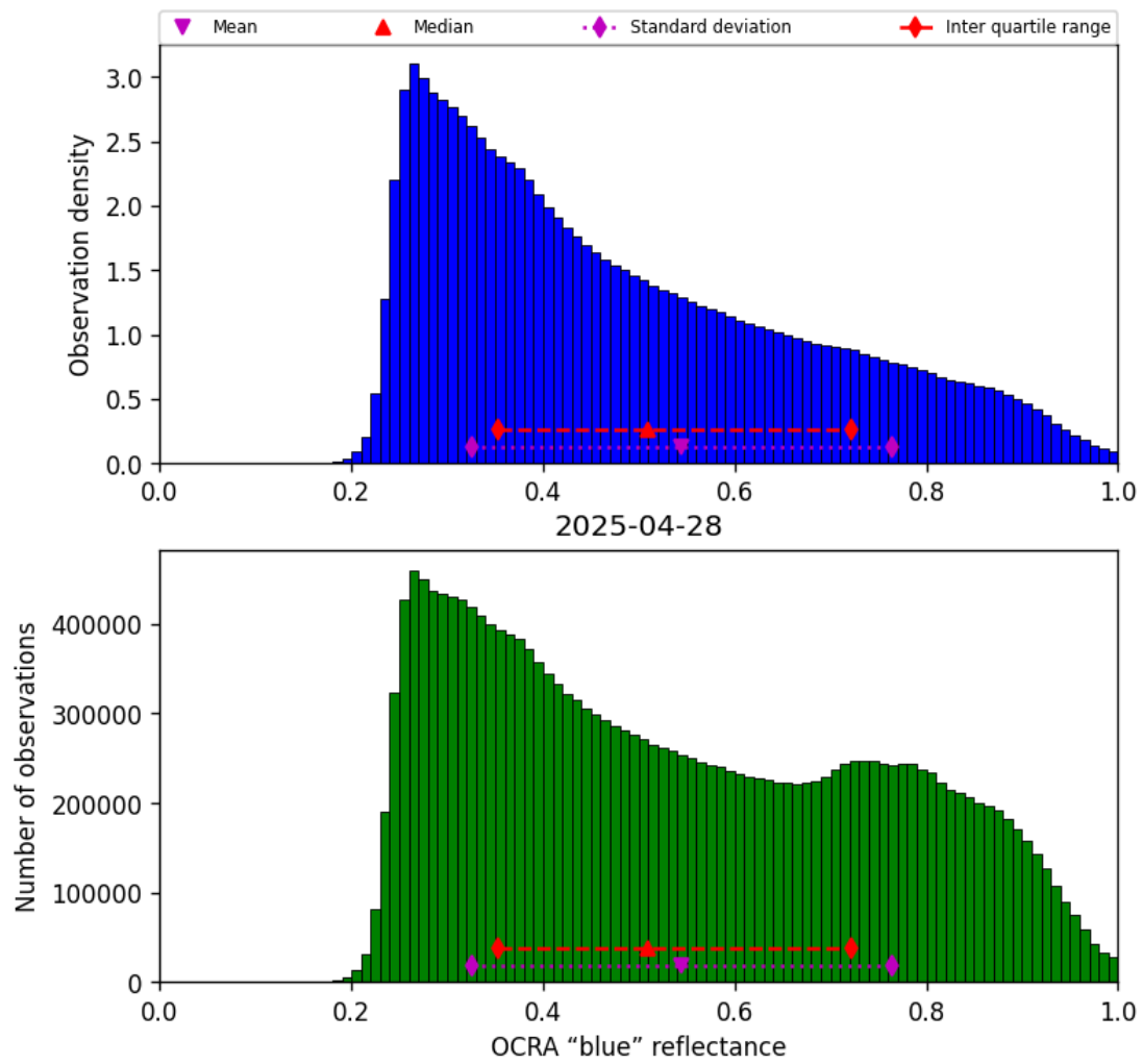
Figure 51: Histogram of “OCRA “blue” reflectance” for 2025-04-27 to 2025-04-29
