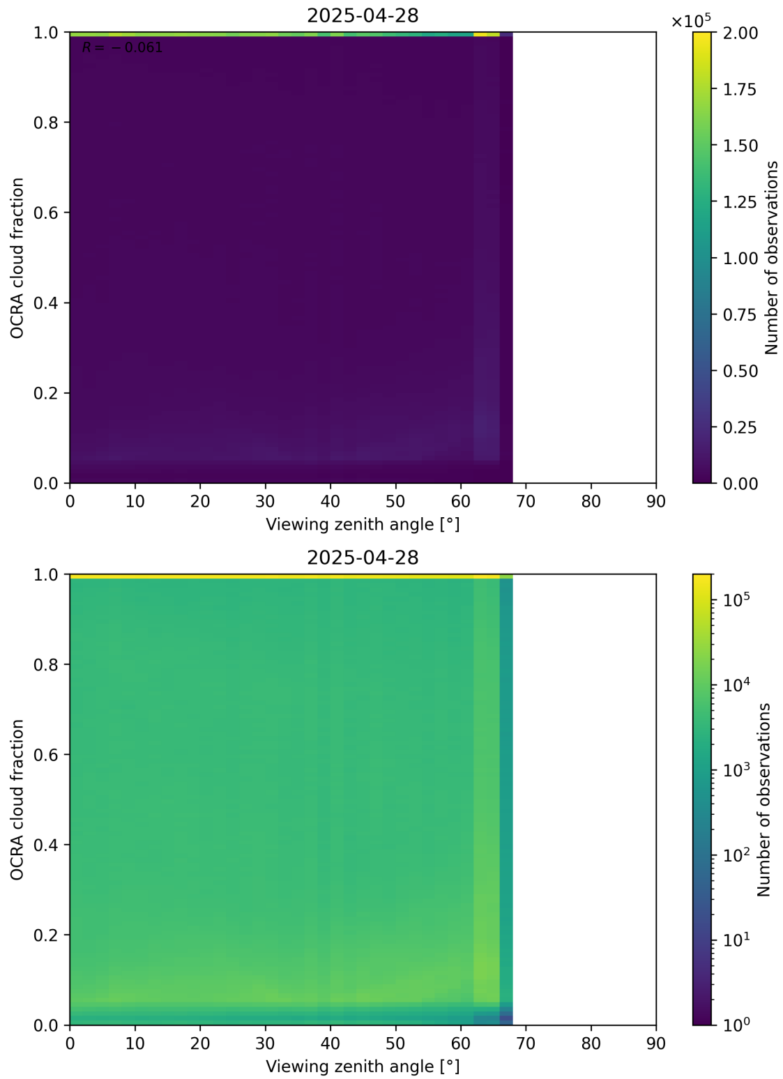
Figure 108: Scatter density plot of “Viewing zenith angle” against “OCRA cloud fraction” for 2025-04-27 to 2025-04-29.
