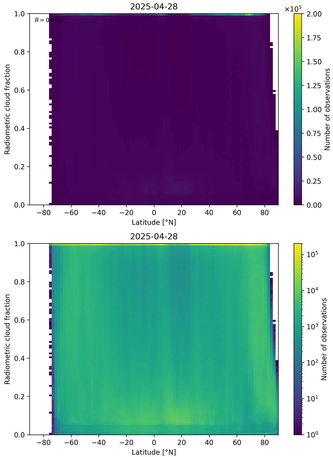
Figure 92: Scatter density plot of “Latitude” against “Radiometric cloud fraction” for 2025-04-27 to 2025-04-29.
