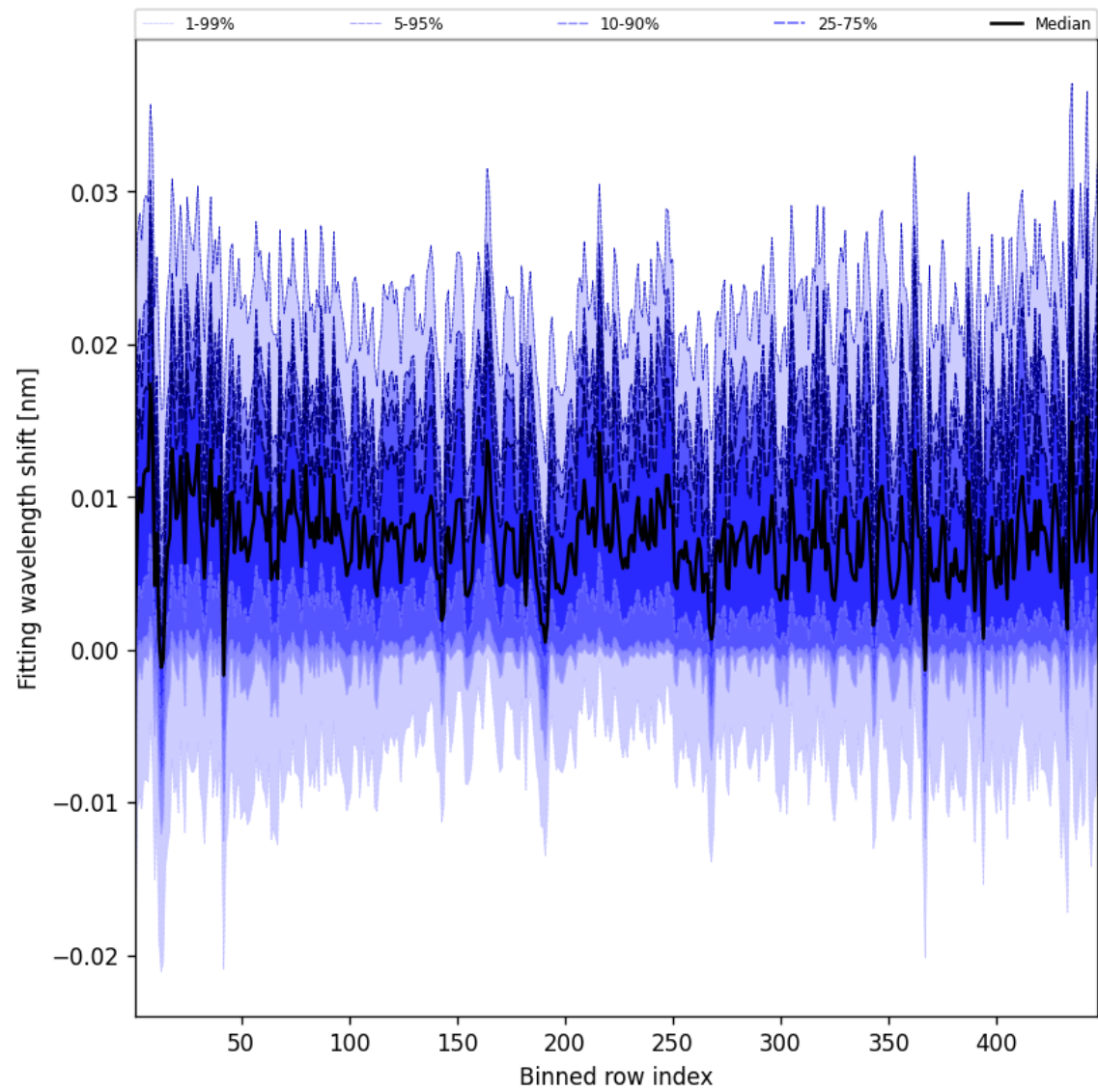
Figure 65: Along track statistics of “Fitting wavelength shift” for 2025-04-27 to 2025-04-29
