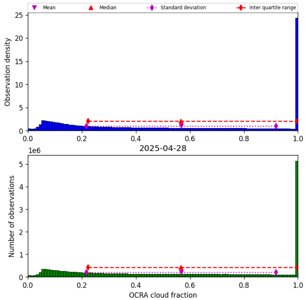
Figure 50: Histogram of “OCRA cloud fraction” for 2025-04-27 to 2025-04-29
