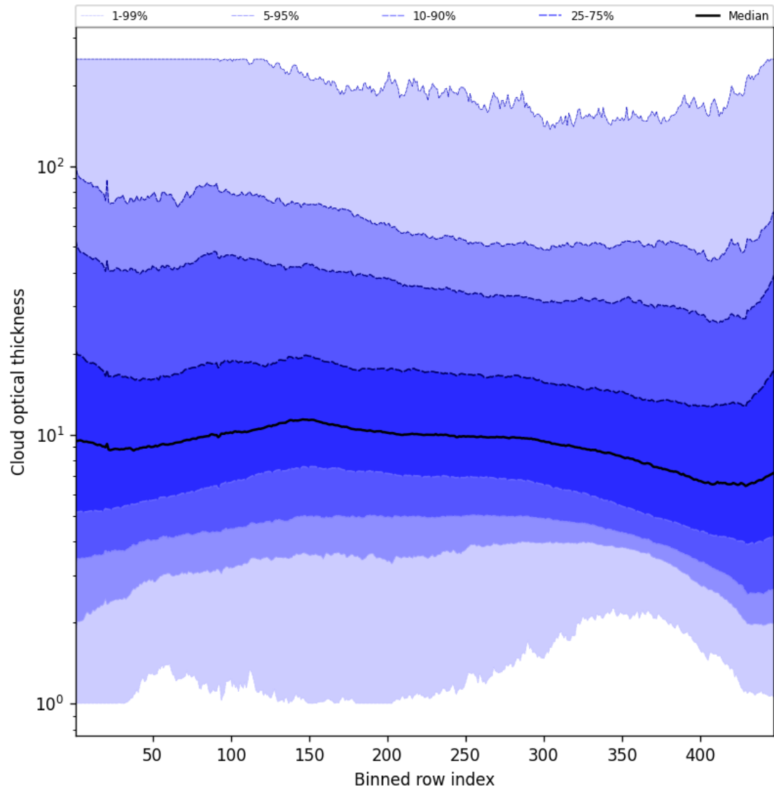
Figure 57: Along track statistics of “Cloud optical thickness” for 2025-04-27 to 2025-04-29
