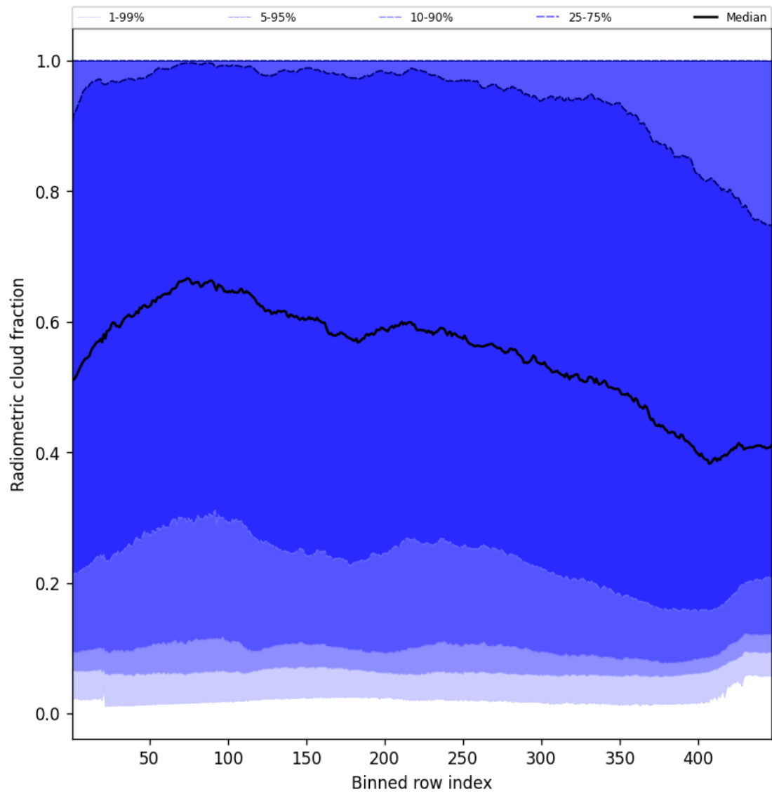
Figure 55: Along track statistics of “Radiometric cloud fraction” for 2025-04-27 to 2025-04-29
