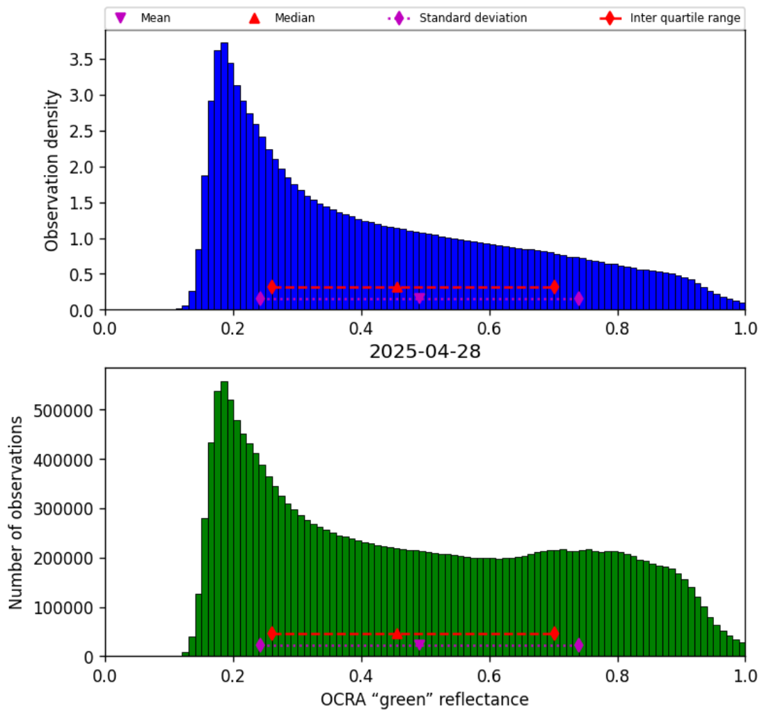
Figure 52: Histogram of “OCRA “green” reflectance” for 2025-04-27 to 2025-04-29
