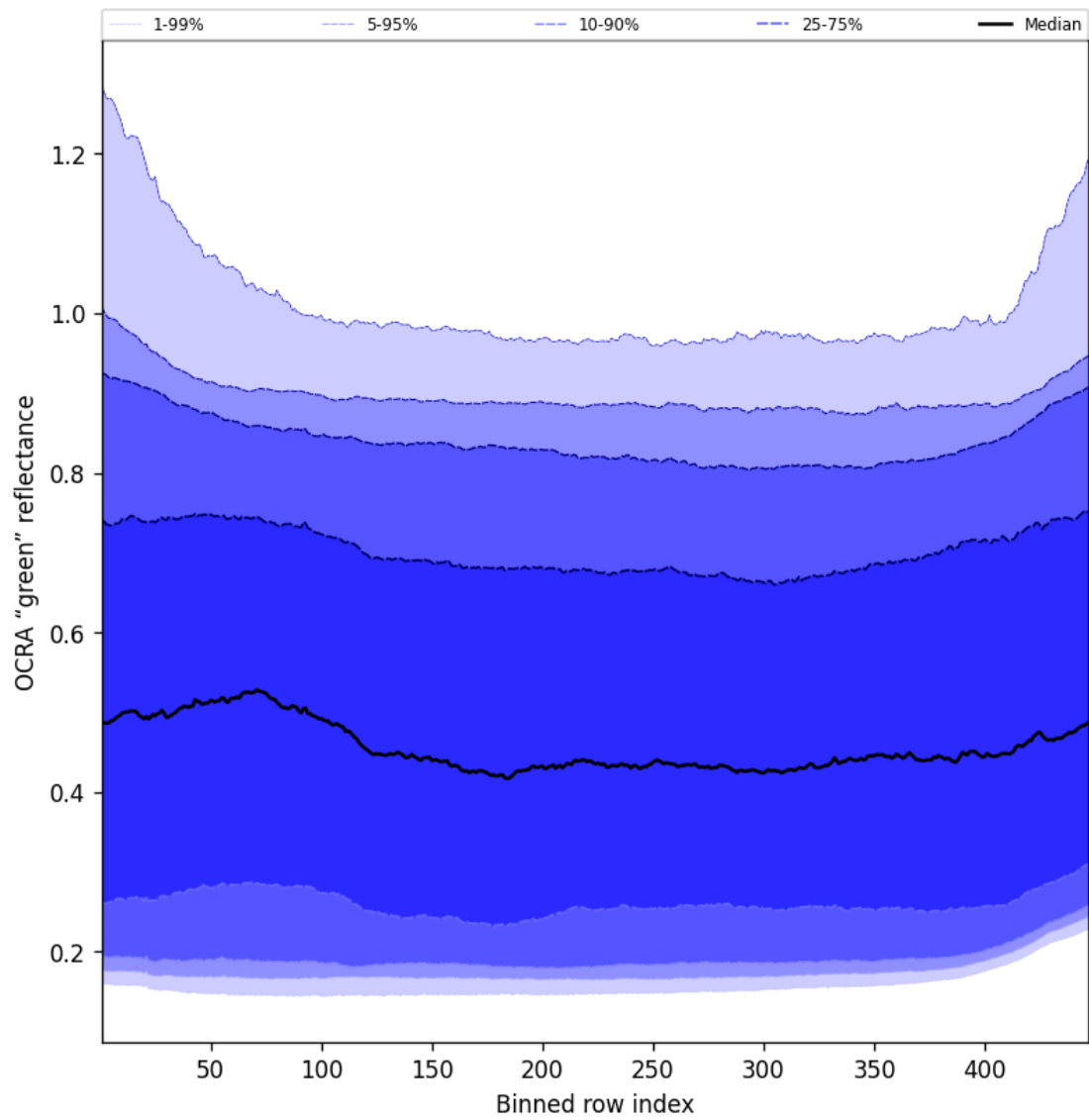
Figure 68: Along track statistics of "OCRA "green" reflectance" for 2025-04-27 to 2025-04-29
