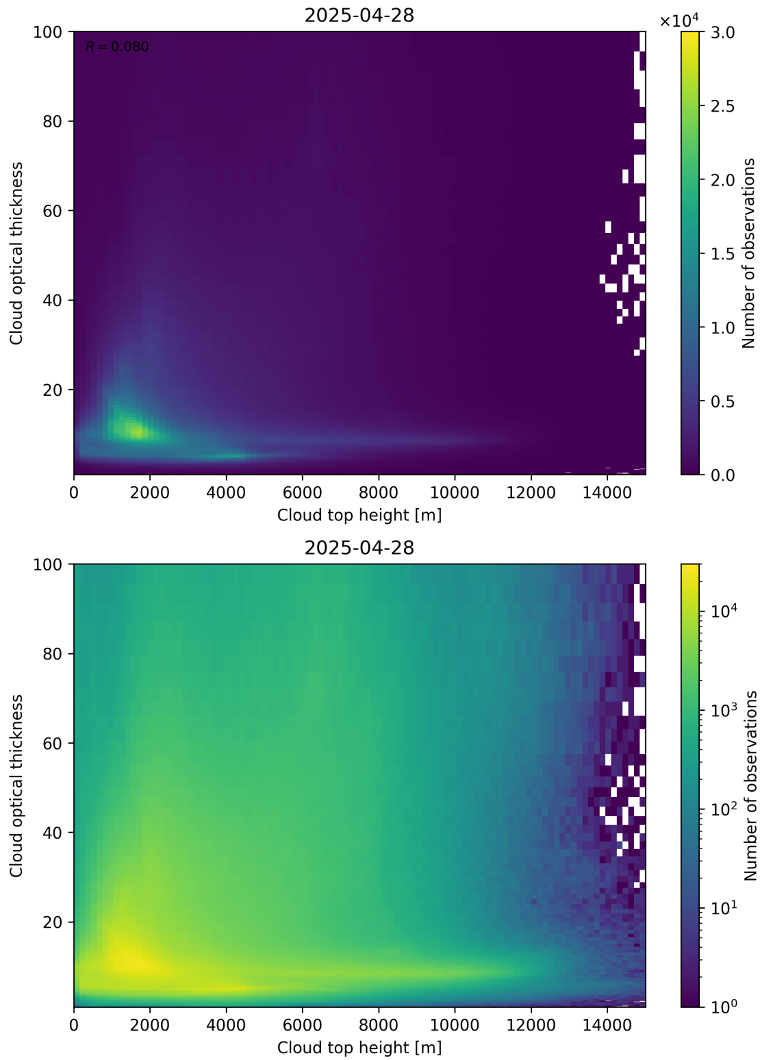
Figure 90: Scatter density plot of “Cloud top height” against “Cloud optical thickness” for 2025-04-27 to 2025-04-29.
