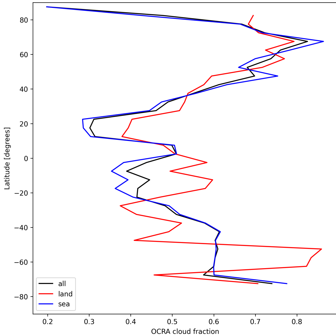
Figure 34: Zonal average of “OCRA cloud fraction” for 2025-04-27 to 2025-04-29.
