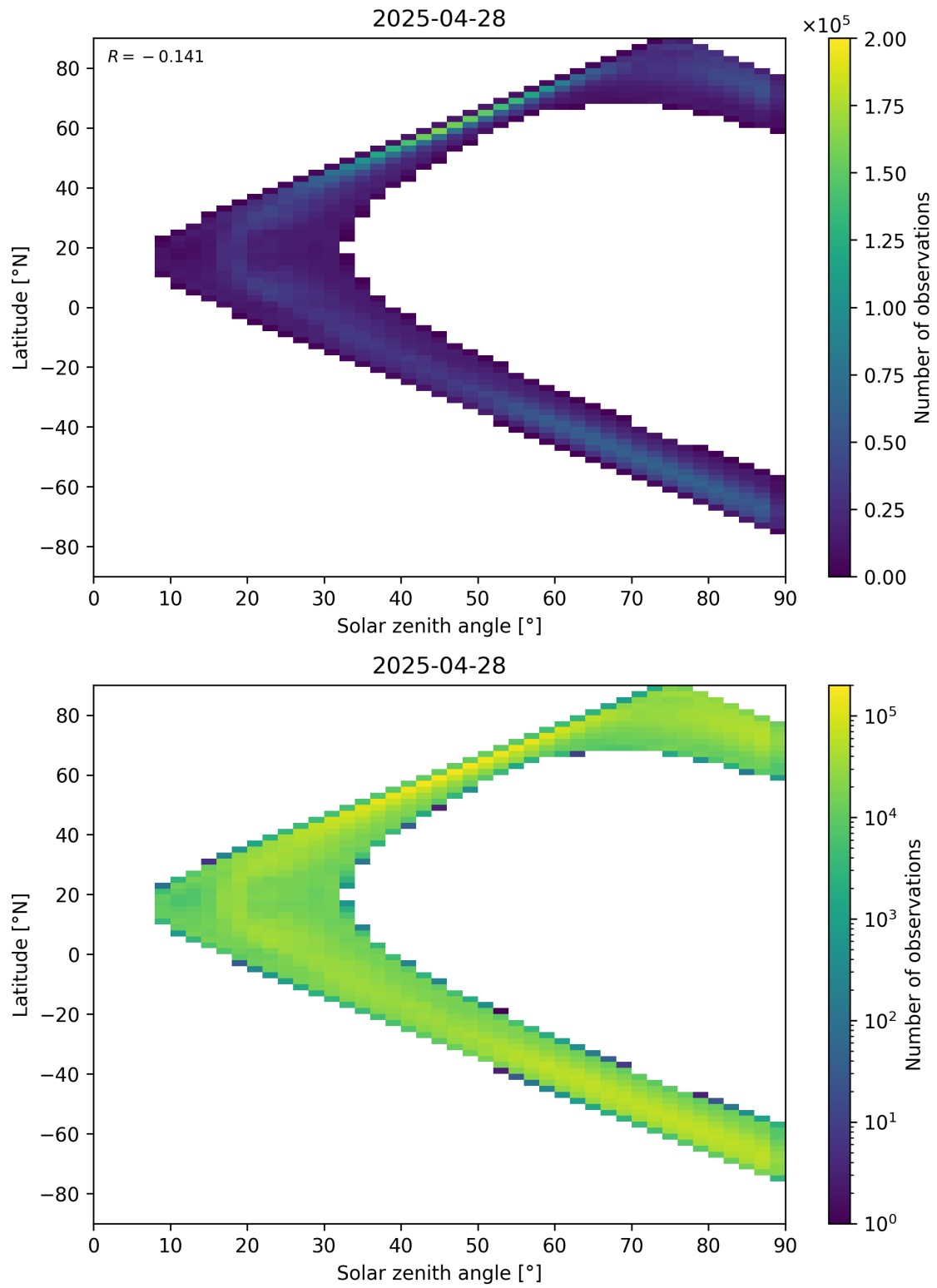
Figure 105: Scatter density plot of “Solar zenith angle” against “Latitude” for 2025-04-27 to 2025-04-29.
