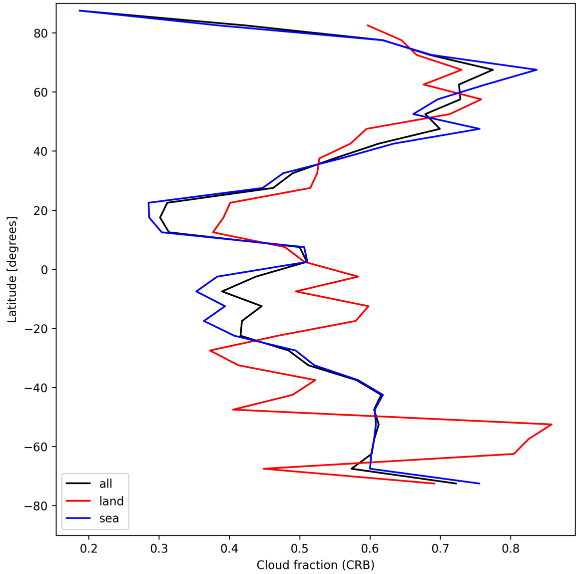
Figure 26: Zonal average of “Cloud fraction (CRB)” for 2025-04-27 to 2025-04-29.
