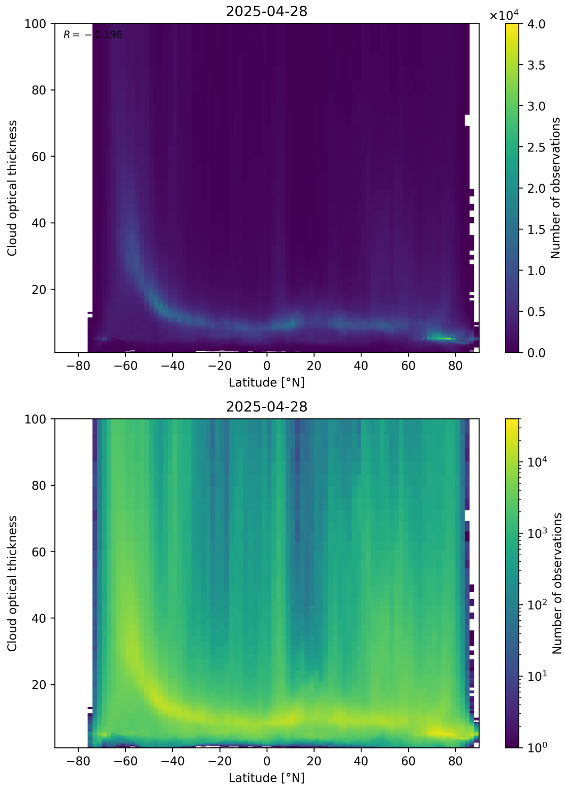
Figure 96: Scatter density plot of “Latitude” against “Cloud optical thickness” for 2025-04-27 to 2025-04-29.
