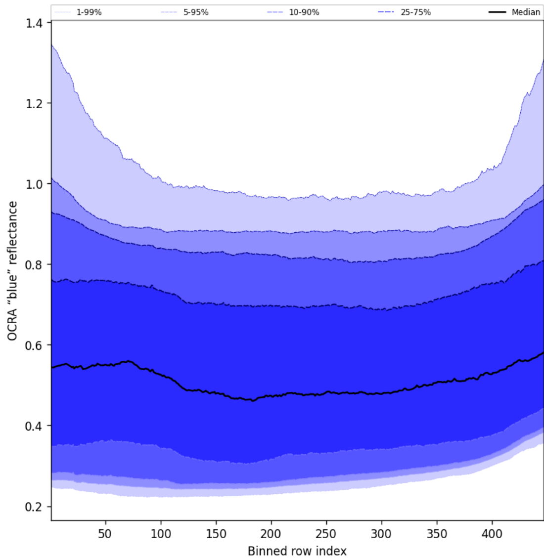
Figure 67: Along track statistics of “OCRA “blue” reflectance” for 2025-04-27 to 2025-04-29
