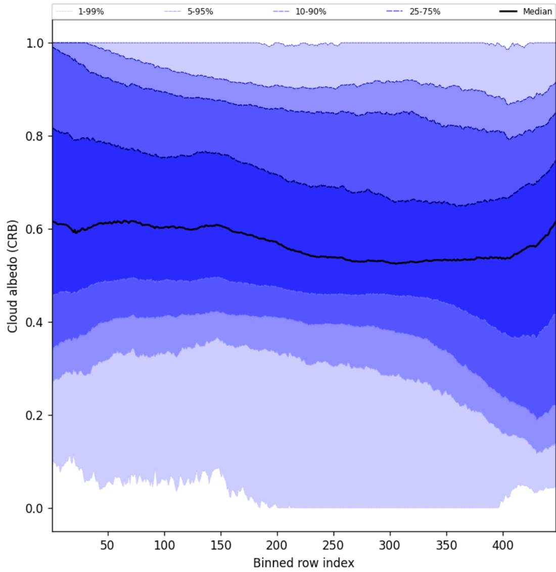
Figure 60: Along track statistics of “Cloud albedo (CRB)” for 2025-04-27 to 2025-04-29
