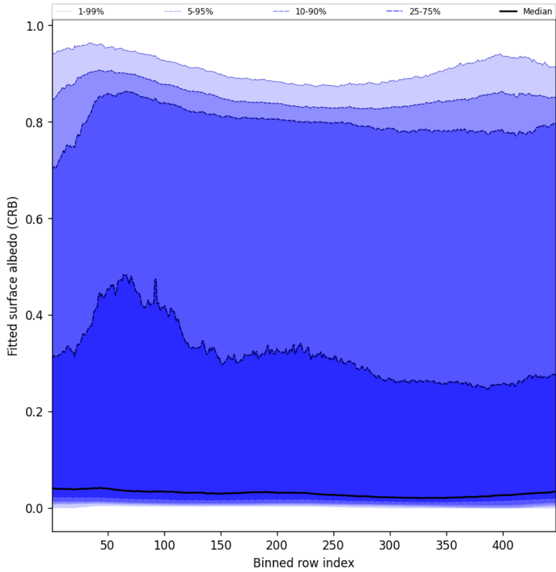
Figure 62: Along track statistics of “Fitted surface albedo (CRB)” for 2025-04-27 to 2025-04-29
