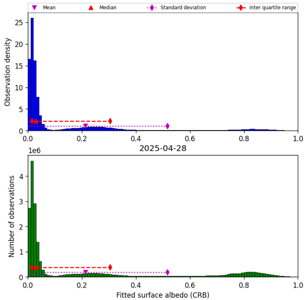
Figure 46: Histogram of “Fitted surface albedo (CRB)” for 2025-04-27 to 2025-04-29
