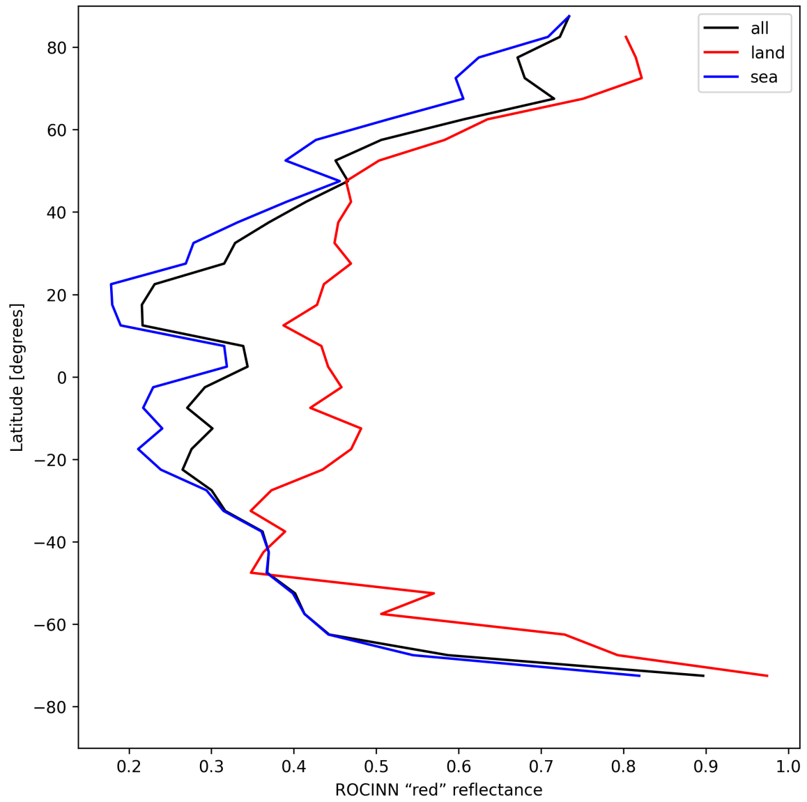
Figure 37: Zonal average of “ROCINN “red” reflectance” for 2025-04-27 to 2025-04-29.
