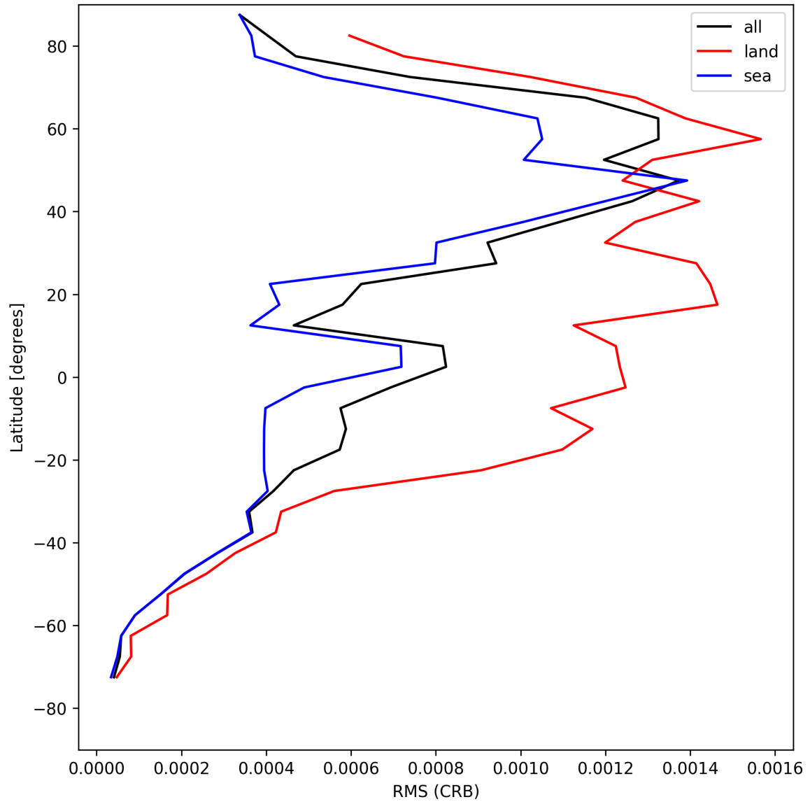
Figure 32: Zonal average of “RMS (CRB)” for 2025-04-27 to 2025-04-29.
