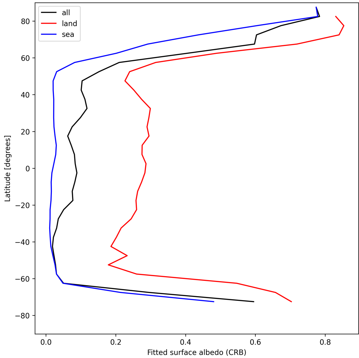
Figure 30: Zonal average of “Fitted surface albedo (CRB)” for 2025-04-29 to 2025-04-30.
