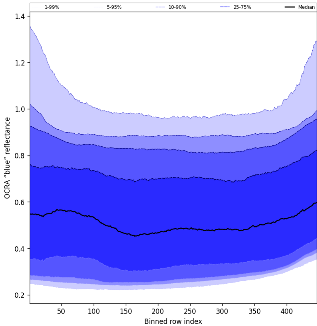
Figure 67: Along track statistics of “OCRA “blue” reflectance” for 2025-04-29 to 2025-04-30
