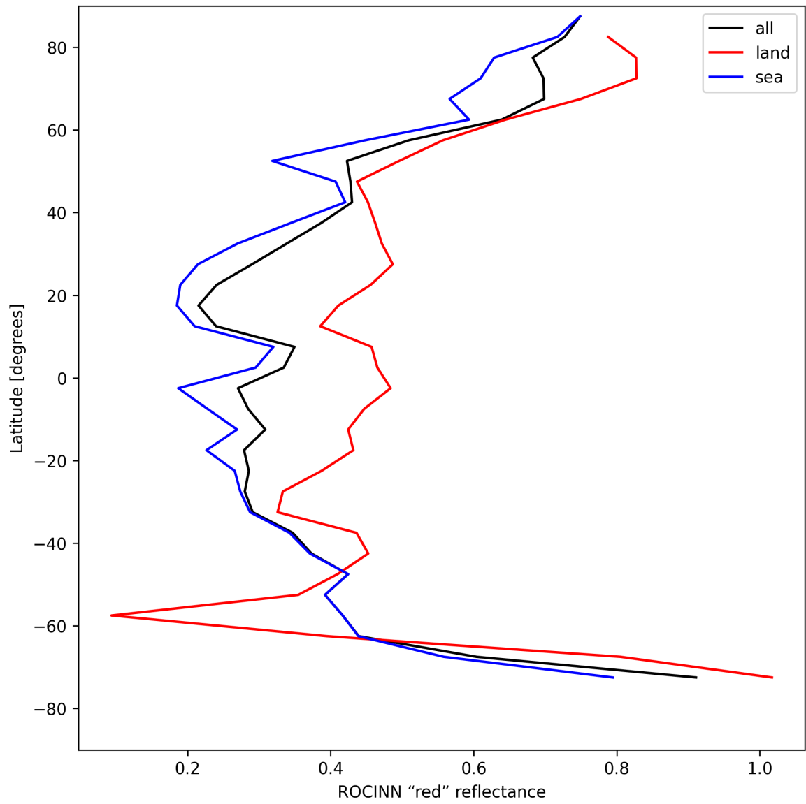
Figure 37: Zonal average of "ROCINN "red" reflectance" for 2025-04-29 to 2025-04-30.
