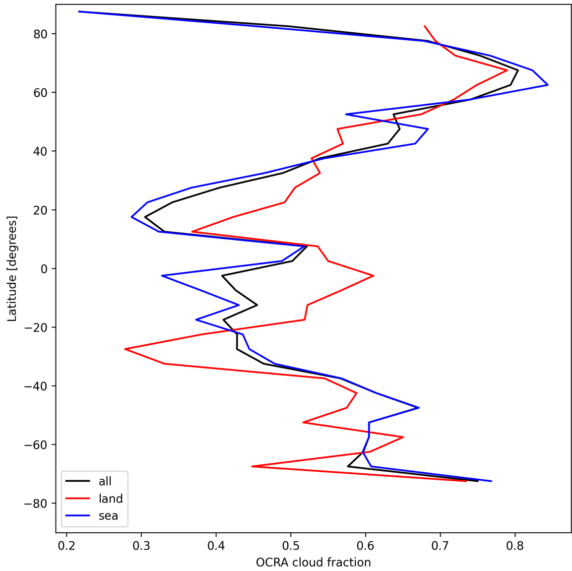
Figure 34: Zonal average of “OCRA cloud fraction” for 2025-04-29 to 2025-04-30.
