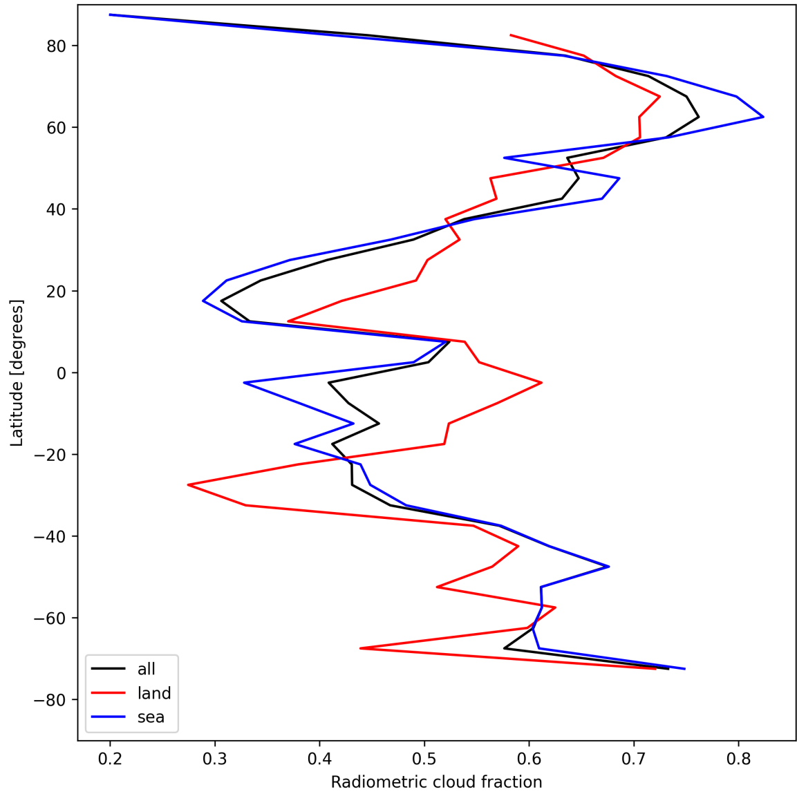
Figure 23: Zonal average of “Radiometric cloud fraction” for 2025-04-29 to 2025-04-30.
