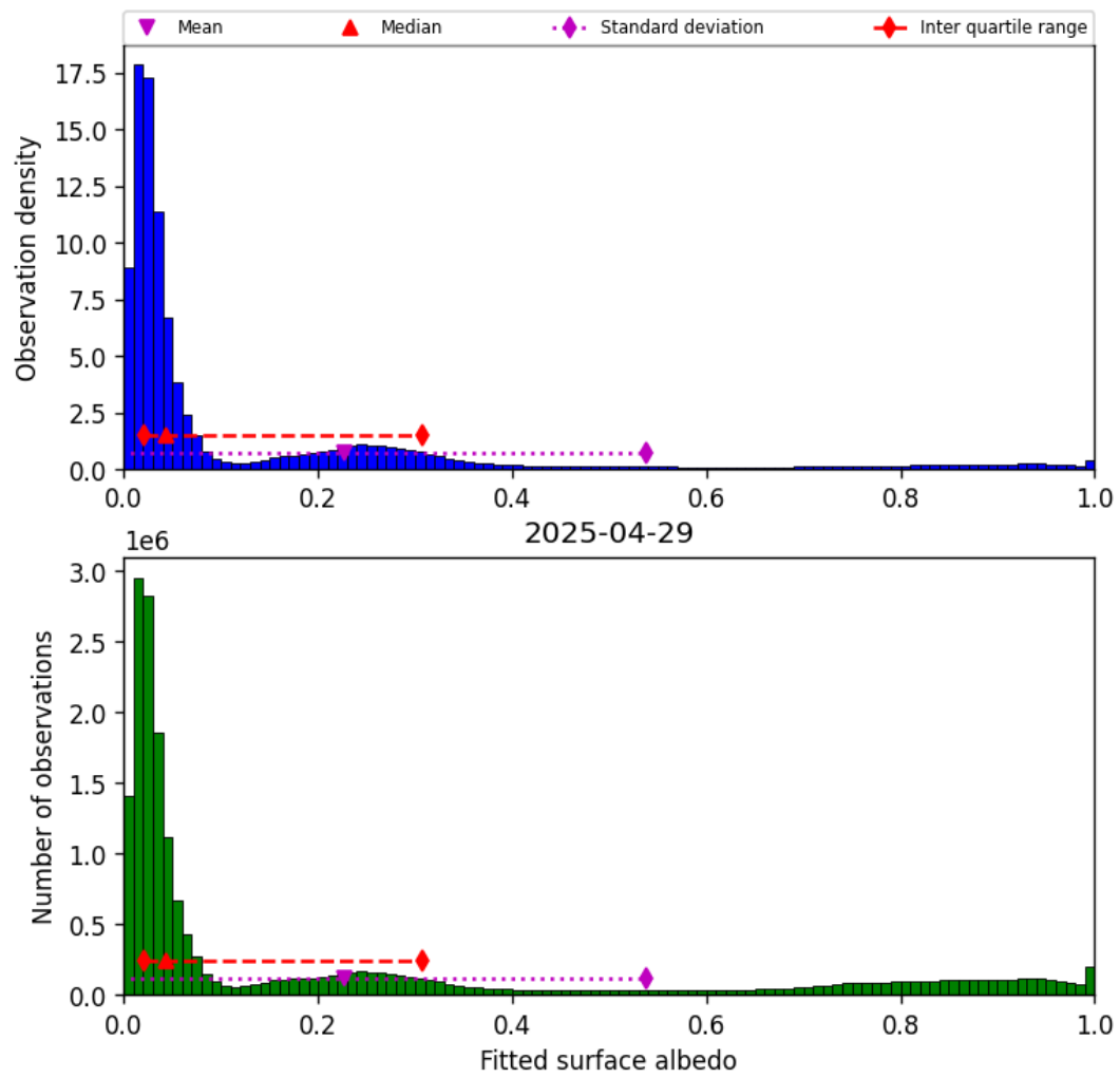
Figure 45: Histogram of “Fitted surface albedo” for 2025-04-29 to 2025-04-30
