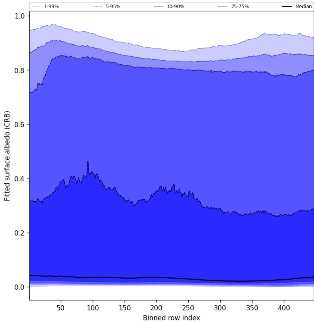
Figure 62: Along track statistics of “Fitted surface albedo (CRB)” for 2025-04-29 to 2025-04-30
