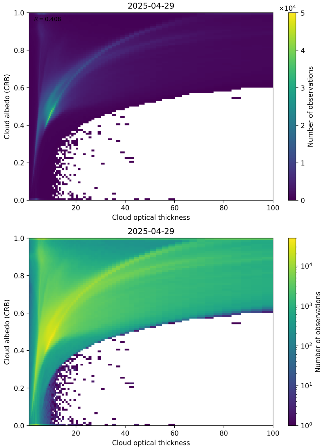
Figure 82: Scatter density plot of “Cloud optical thickness” against “Cloud albedo (CRB)” for 2025-04-29 to 2025-04-30.
