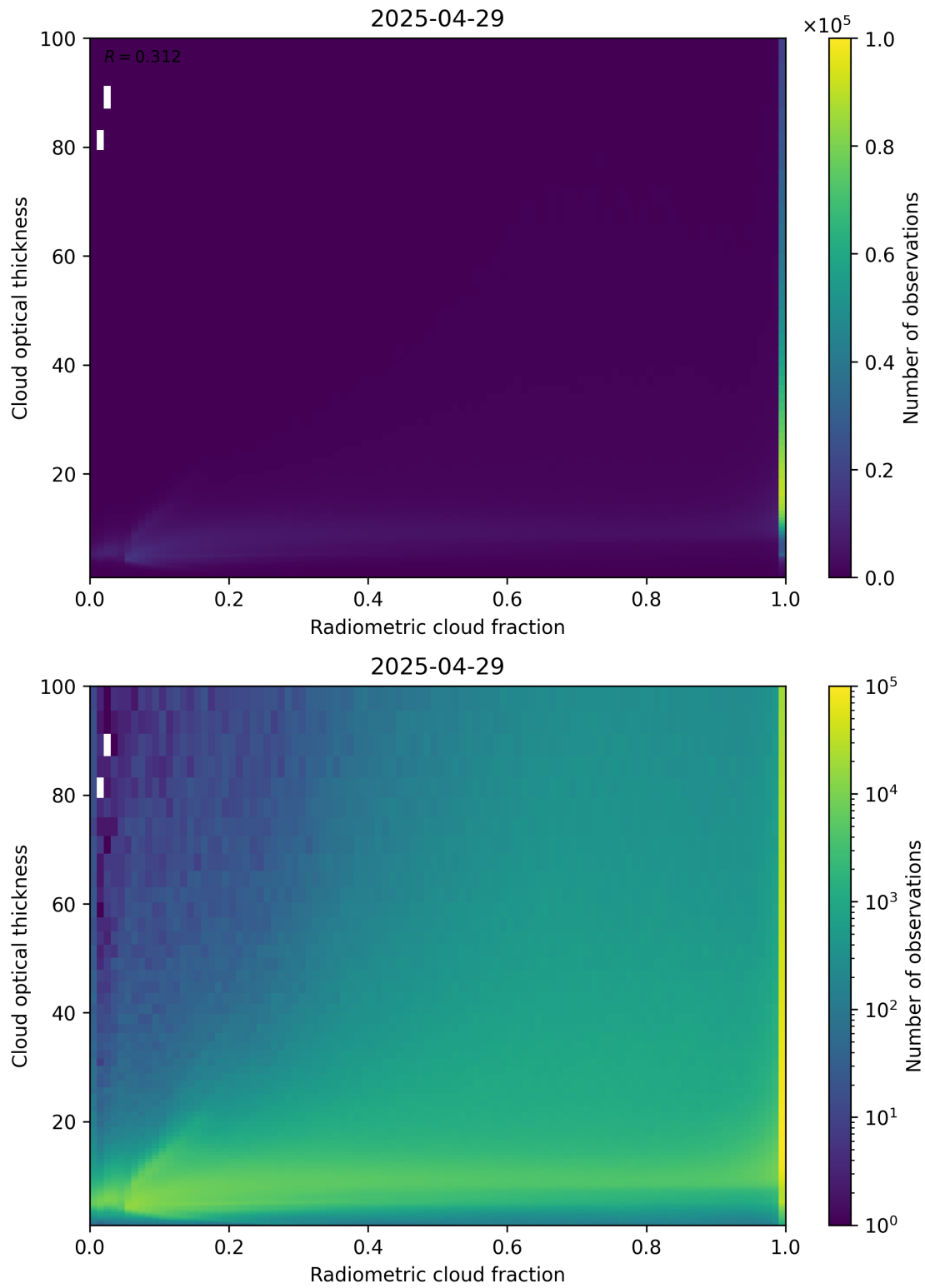
Figure 75: Scatter density plot of “Radiometric cloud fraction” against “Cloud optical thickness” for 2025-04-29 to 2025-04-30.
