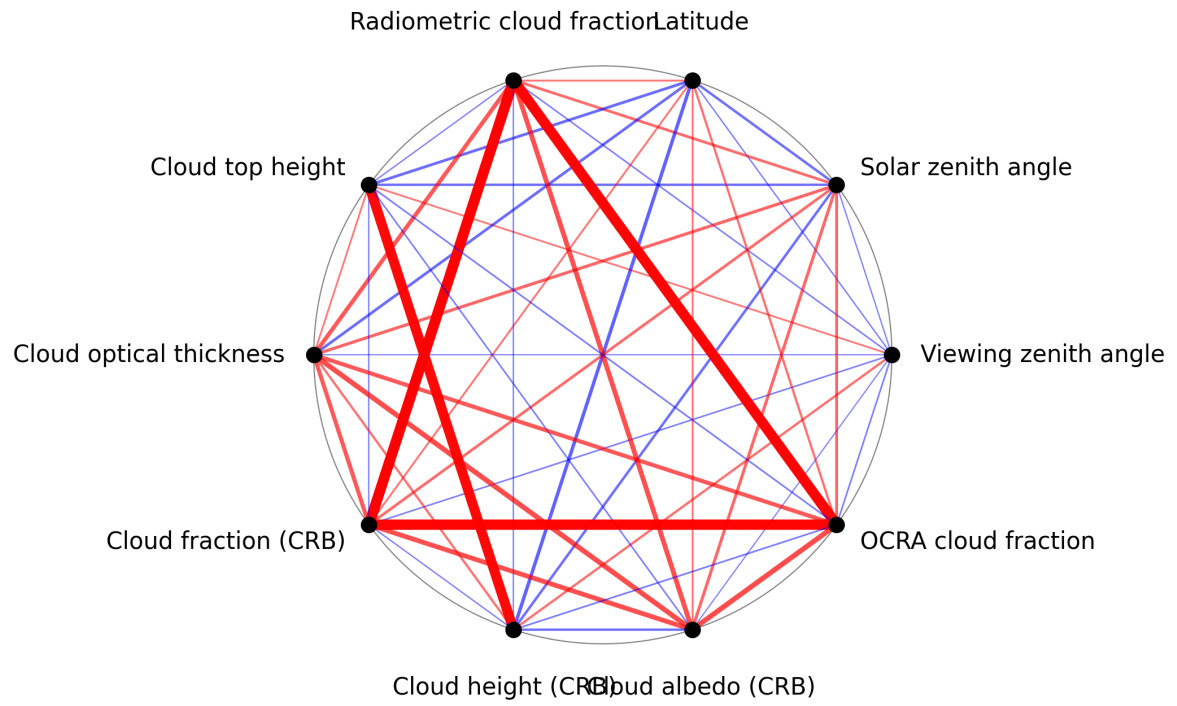
Figure 1: Map of correlation graph for 2025-04-29 to 2025-04-30.
