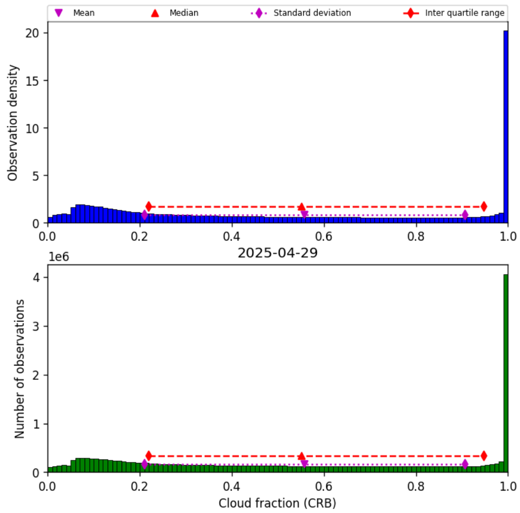
Figure 42: Histogram of “Cloud fraction (CRB)” for 2025-04-29 to 2025-04-30
