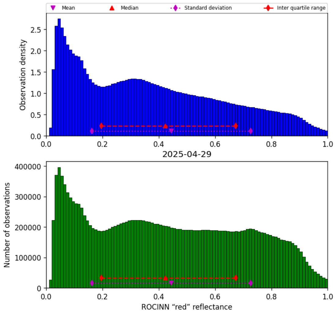
Figure 53: Histogram of “ROCINN “red” reflectance” for 2025-04-29 to 2025-04-30
