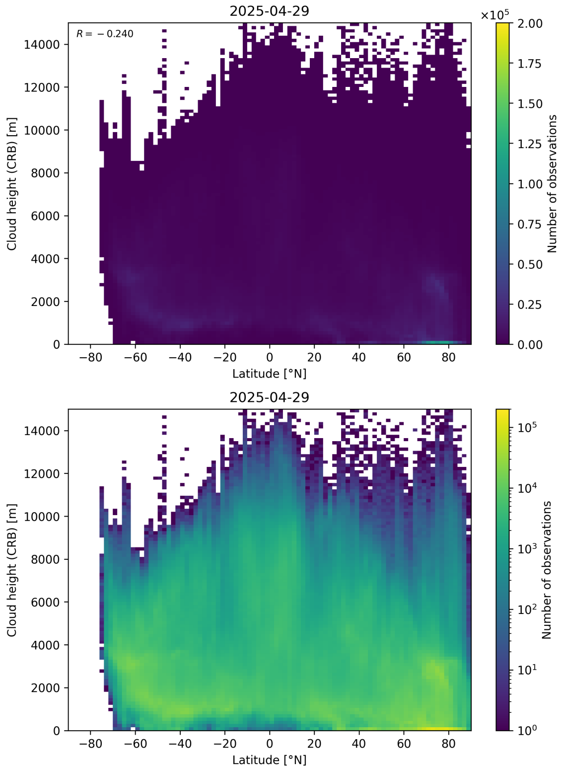
Figure 95: Scatter density plot of “Latitude” against “Cloud height (CRB)” for 2025-04-29 to 2025-04-30.
