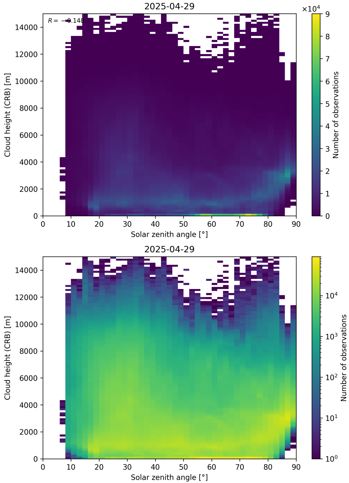
Figure 102: Scatter density plot of “Solar zenith angle” against “Cloud height (CRB)” for 2025-04-29 to 2025-04-30.
