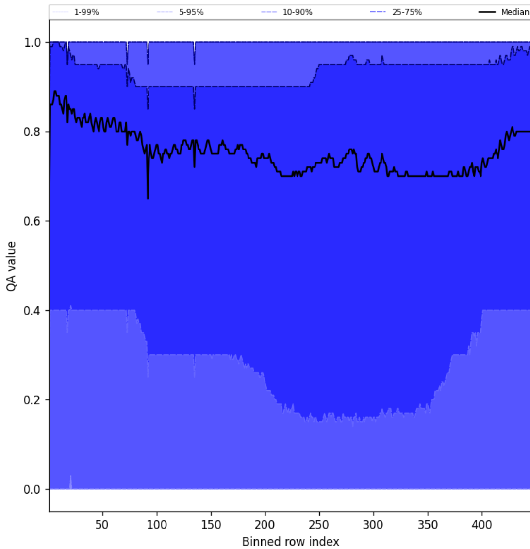
Figure 54: Along track statistics of “QA value” for 2025-04-29 to 2025-04-30
