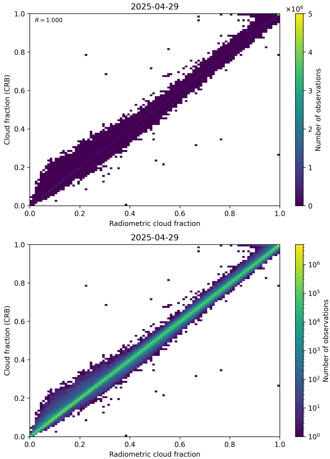
Figure 73: Scatter density plot of “Radiometric cloud fraction” against “Cloud fraction (CRB)” for 2025-04-29 to 2025-04-30.
