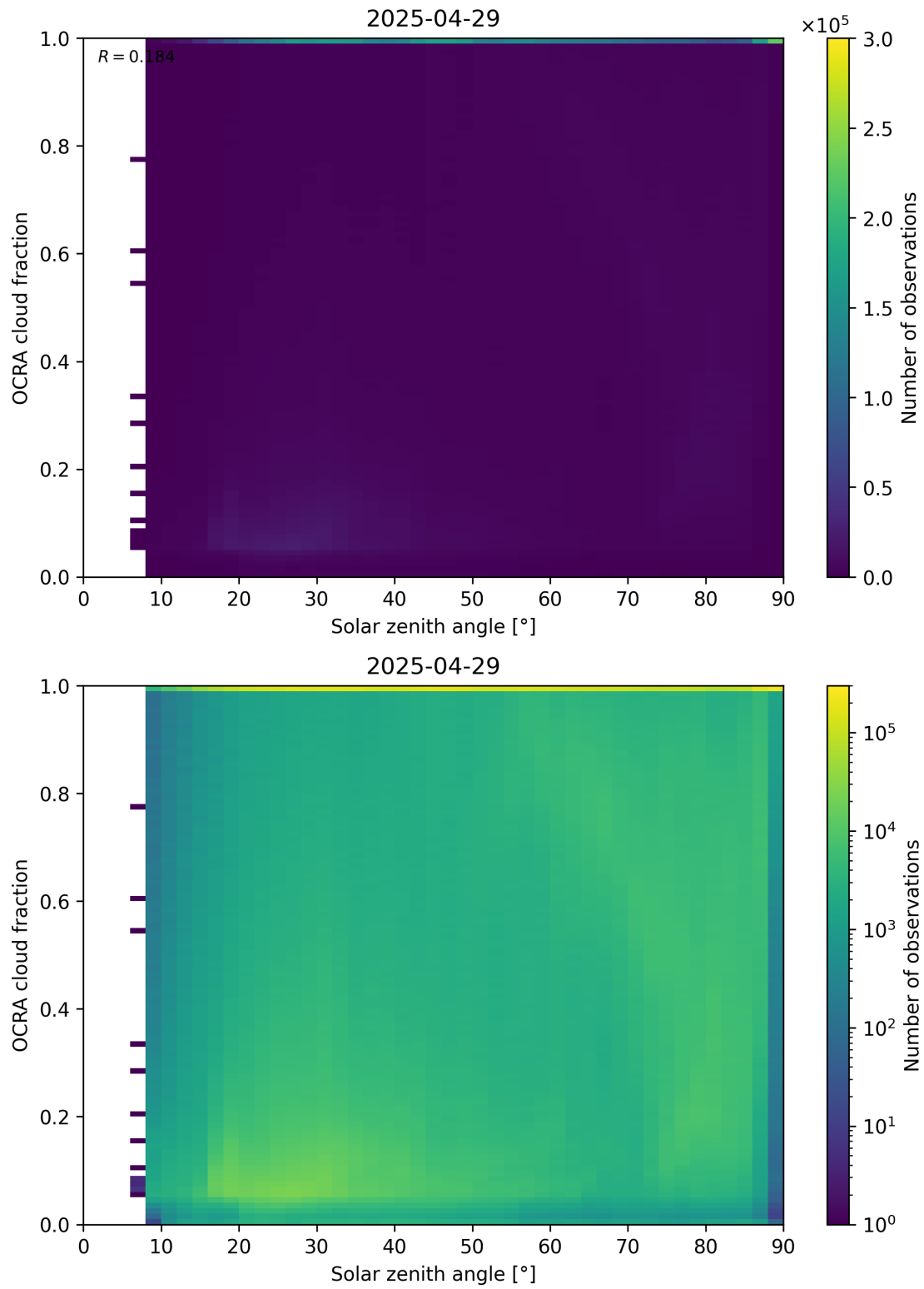
Figure 100: Scatter density plot of “Solar zenith angle” against “OCRA cloud fraction” for 2025-04-29 to 2025-04-30.
