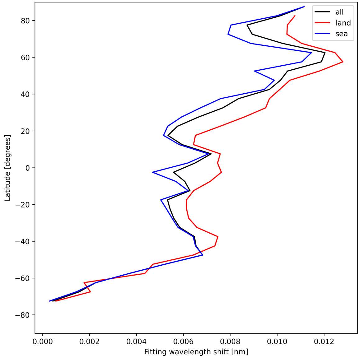
Figure 33: Zonal average of “Fitting wavelength shift” for 2025-04-29 to 2025-04-30.
