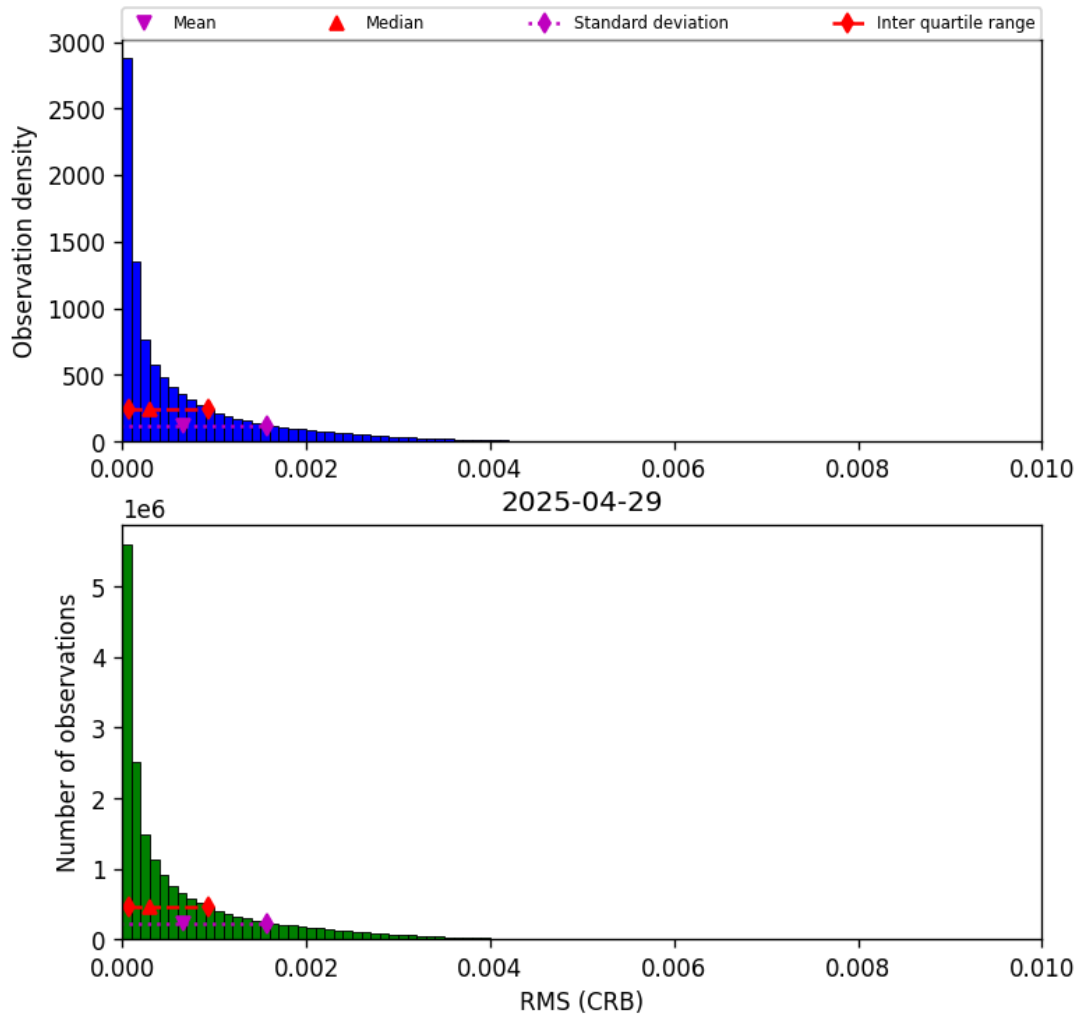
Figure 48: Histogram of “RMS (CRB)” for 2025-04-29 to 2025-04-30
