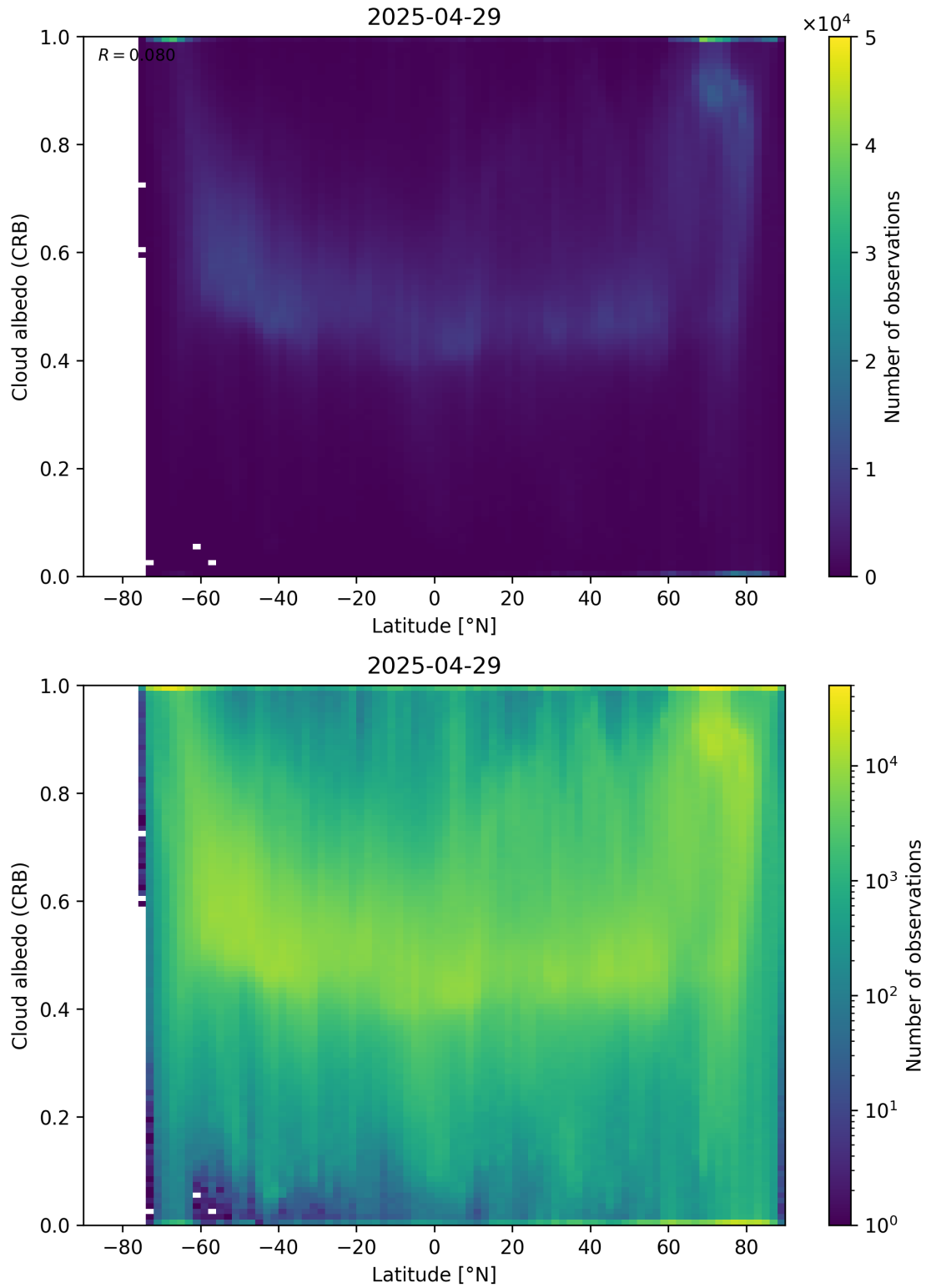
Figure 91: Scatter density plot of “Latitude” against “Cloud albedo (CRB)” for 2025-04-29 to 2025-04-30.
