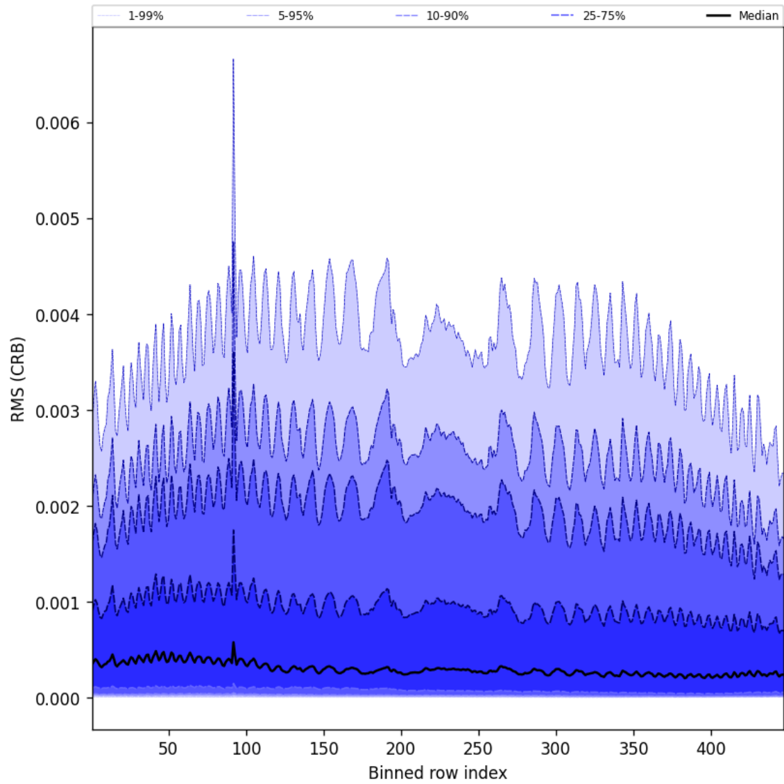
Figure 64: Along track statistics of “RMS (CRB)” for 2025-04-29 to 2025-04-30
