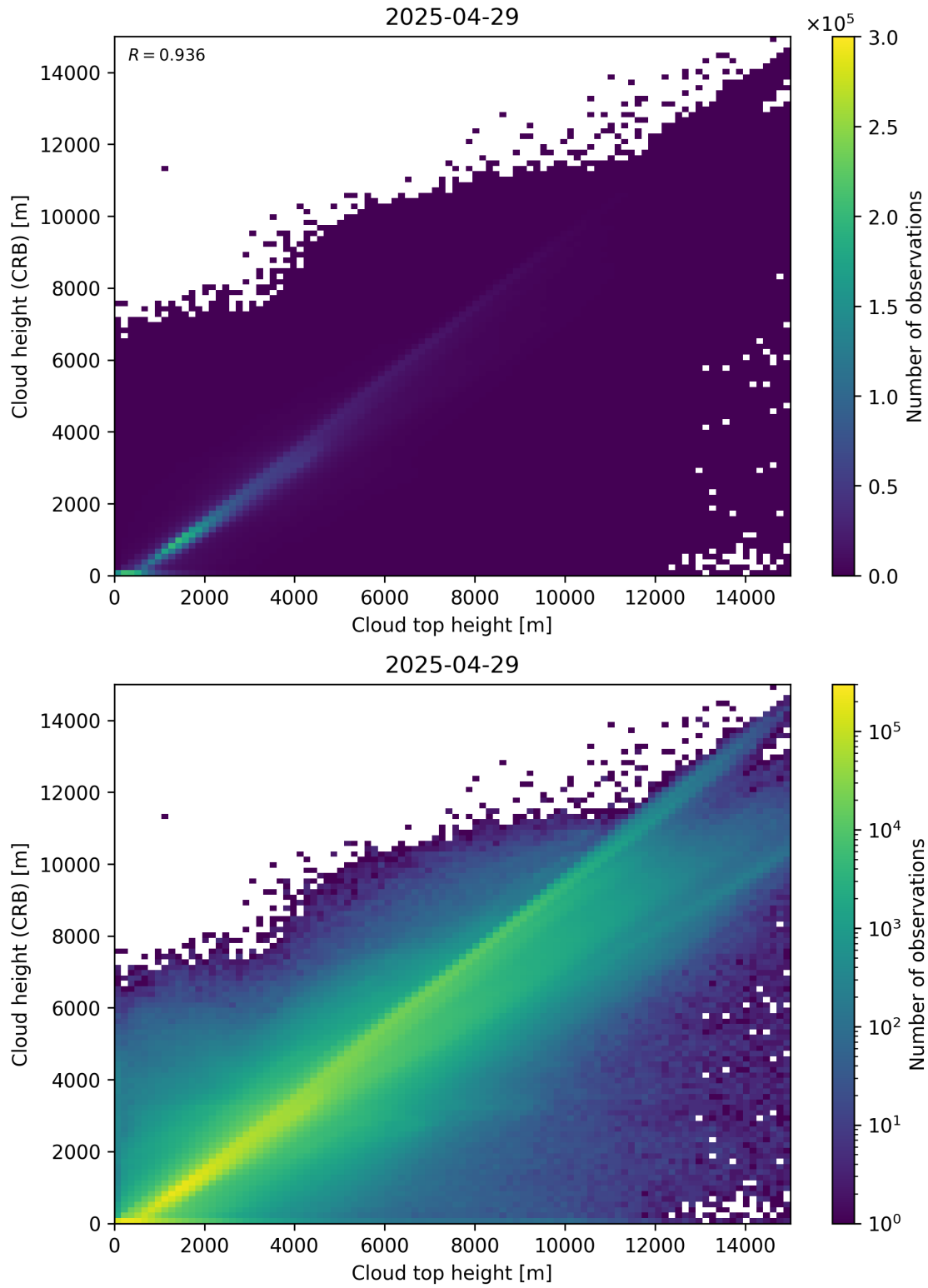
Figure 89: Scatter density plot of “Cloud top height” against “Cloud height (CRB)” for 2025-04-29 to 2025-04-30.
