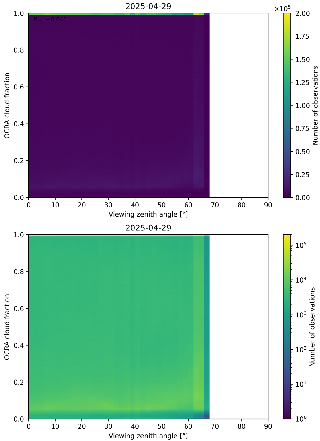
Figure 108: Scatter density plot of “Viewing zenith angle” against “OCRA cloud fraction” for 2025-04-29 to 2025-04-30.
