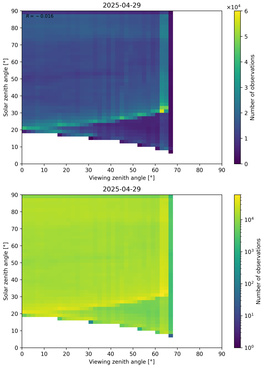
Figure 114: Scatter density plot of “Viewing zenith angle” against “Solar zenith angle” for 2025-04-29 to 2025-04-30.
