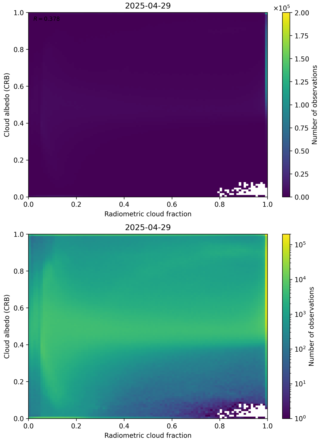
Figure 71: Scatter density plot of “Radiometric cloud fraction” against “Cloud albedo (CRB)” for 2025-04-29 to 2025-04-30.
