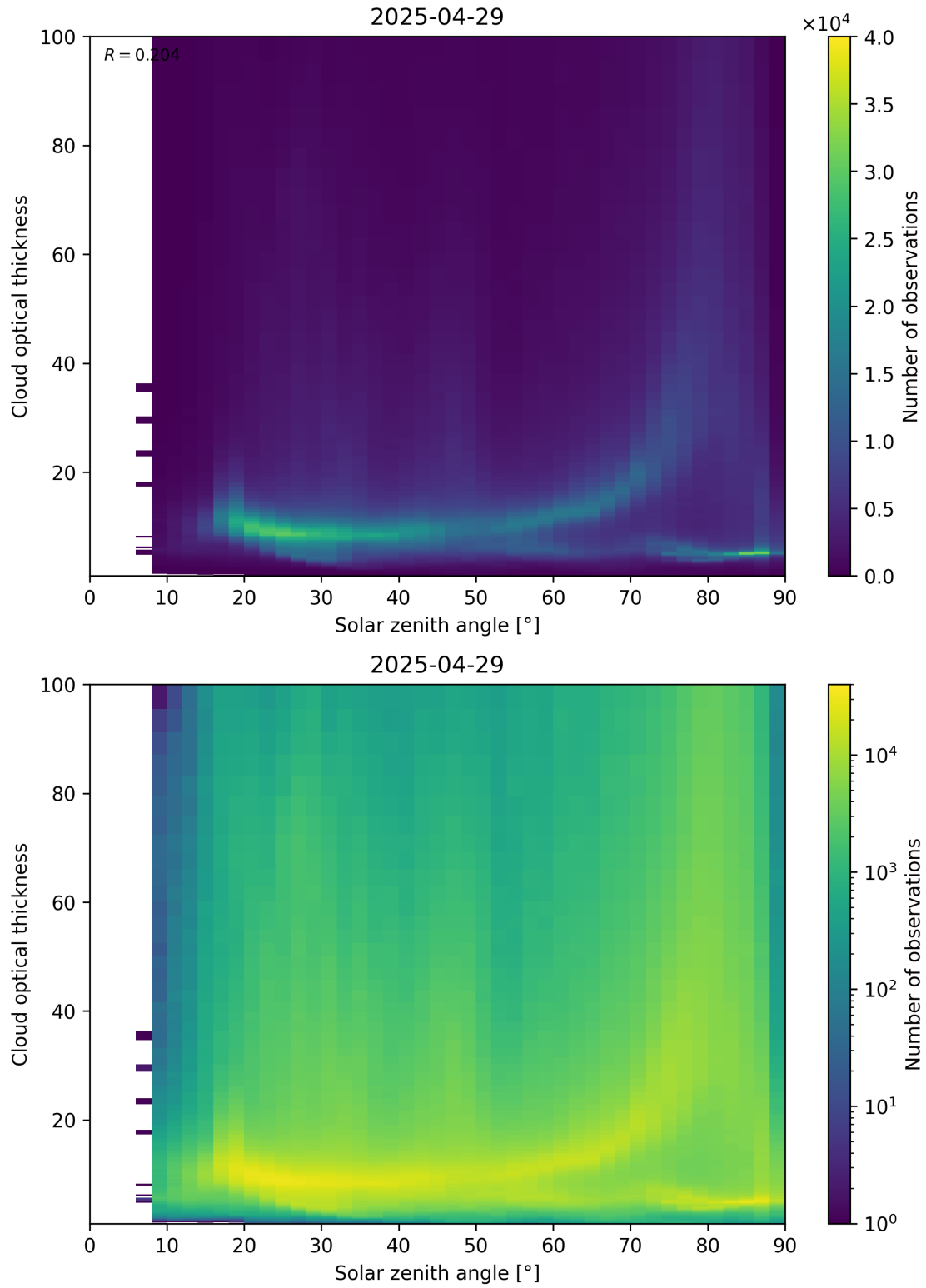
Figure 103: Scatter density plot of “Solar zenith angle” against “Cloud optical thickness” for 2025-04-29 to 2025-04-30.
