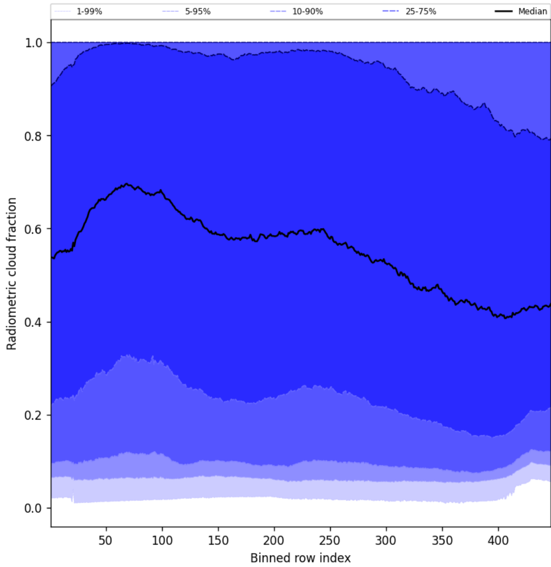
Figure 55: Along track statistics of “Radiometric cloud fraction” for 2025-04-29 to 2025-04-30
