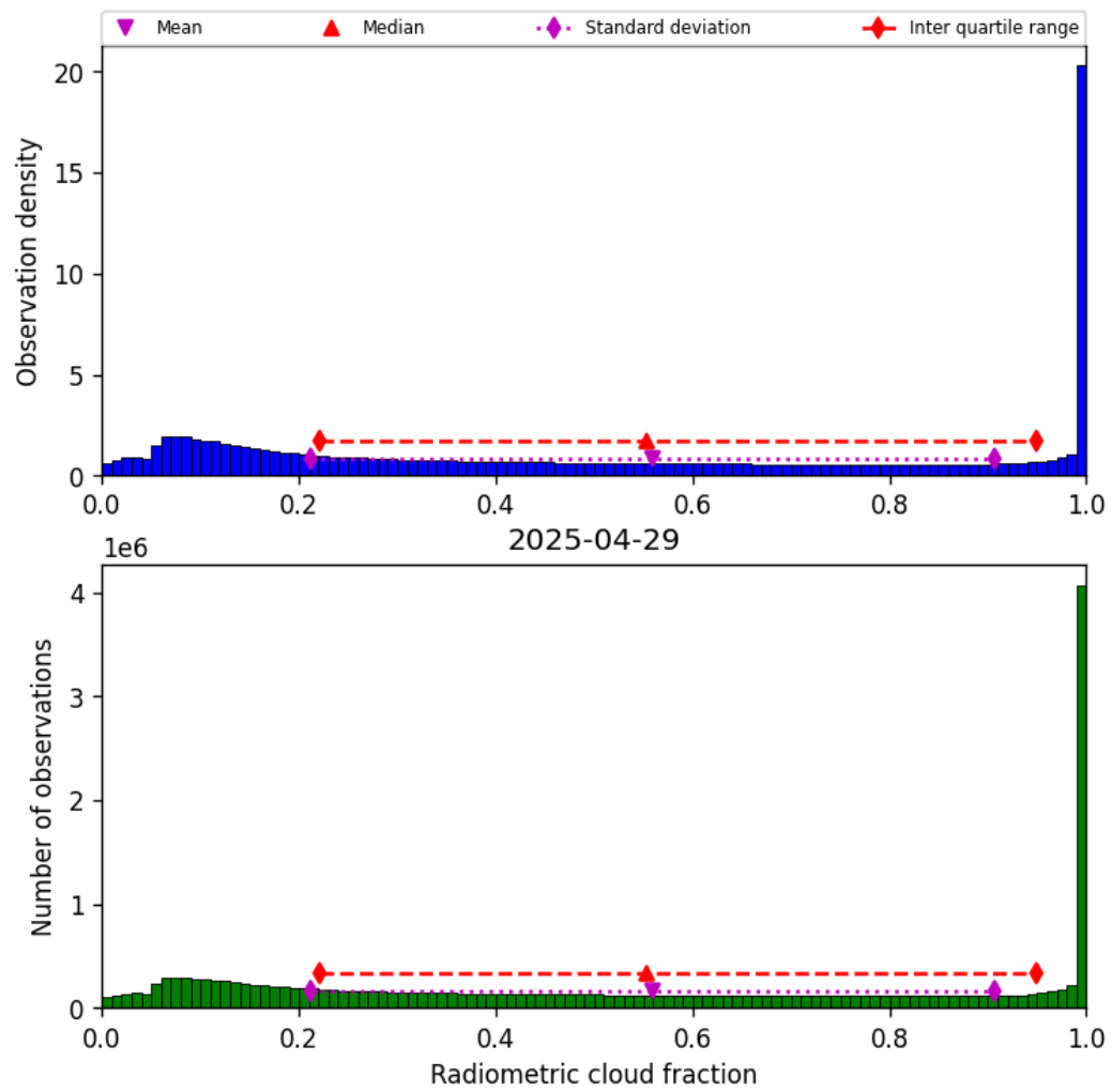
Figure 39: Histogram of “Radiometric cloud fraction” for 2025-04-29 to 2025-04-30
