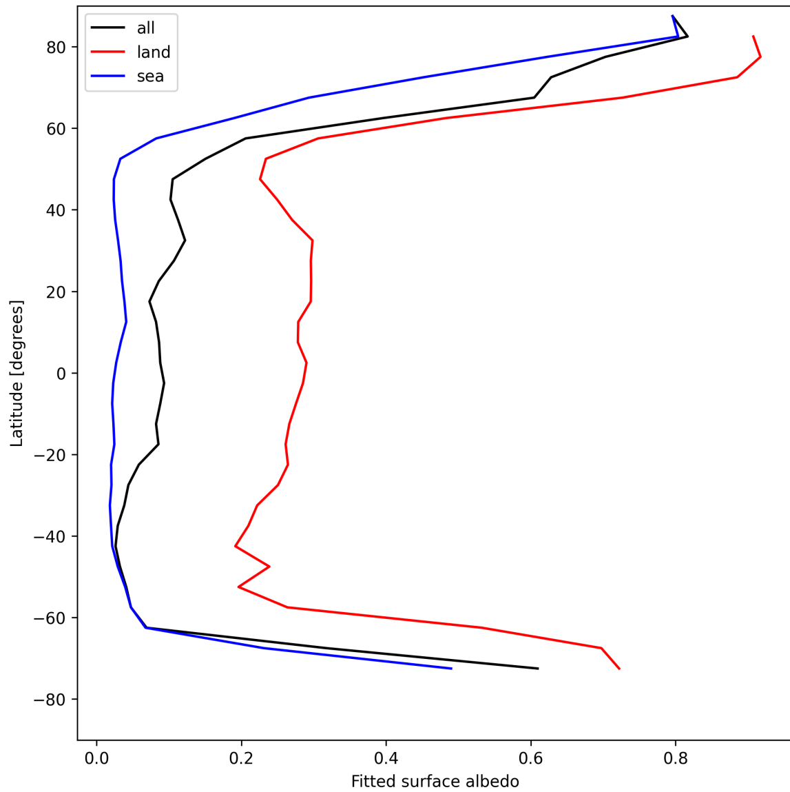
Figure 29: Zonal average of “Fitted surface albedo” for 2025-04-29 to 2025-04-30.
