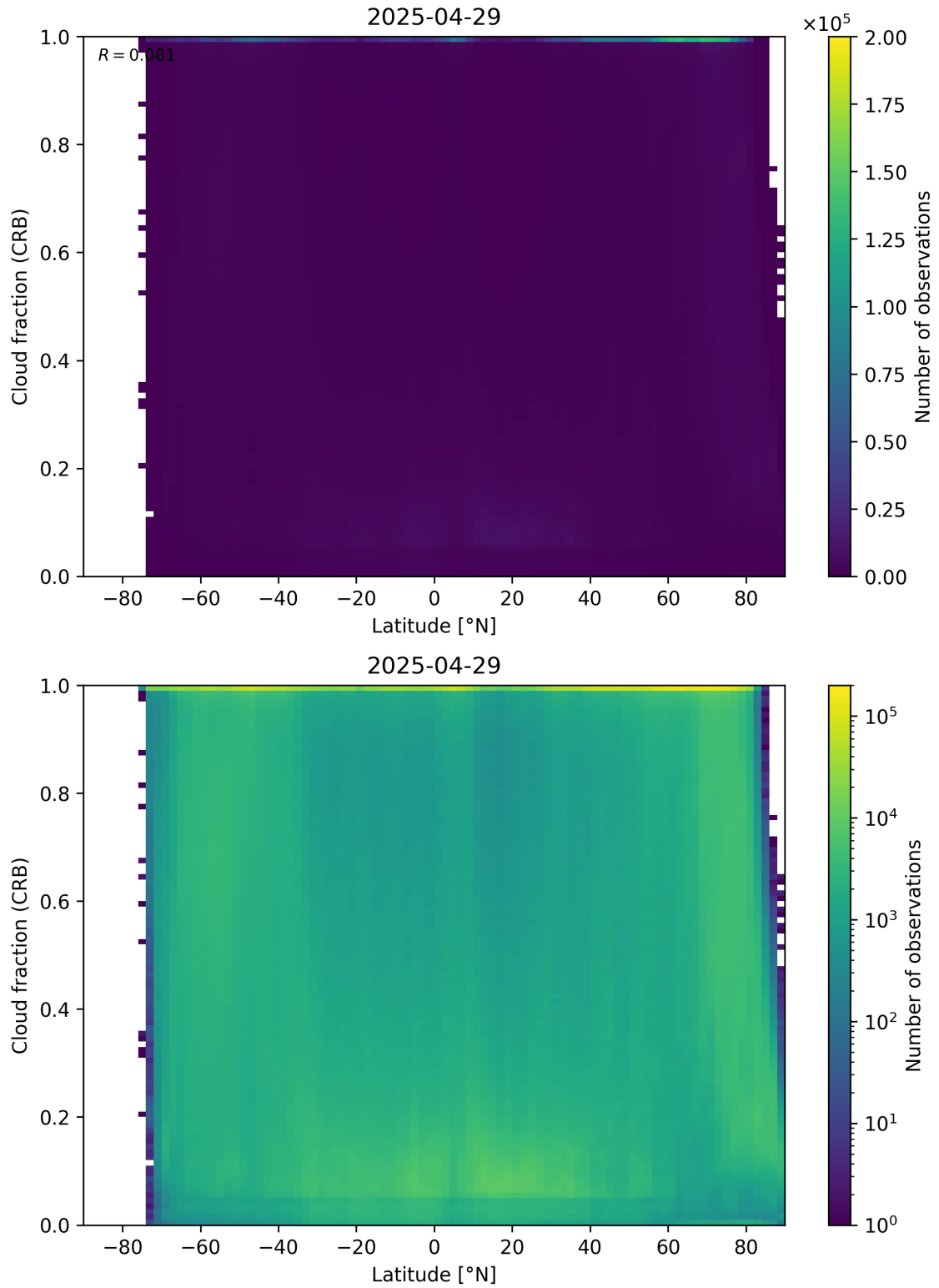
Figure 94: Scatter density plot of “Latitude” against “Cloud fraction (CRB)” for 2025-04-29 to 2025-04-30.
