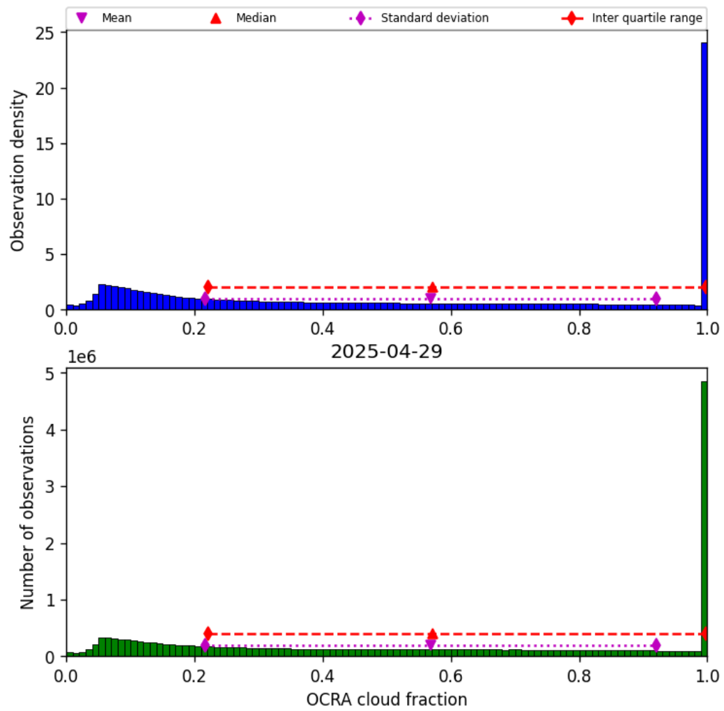
Figure 50: Histogram of “OCRA cloud fraction” for 2025-04-29 to 2025-04-30
