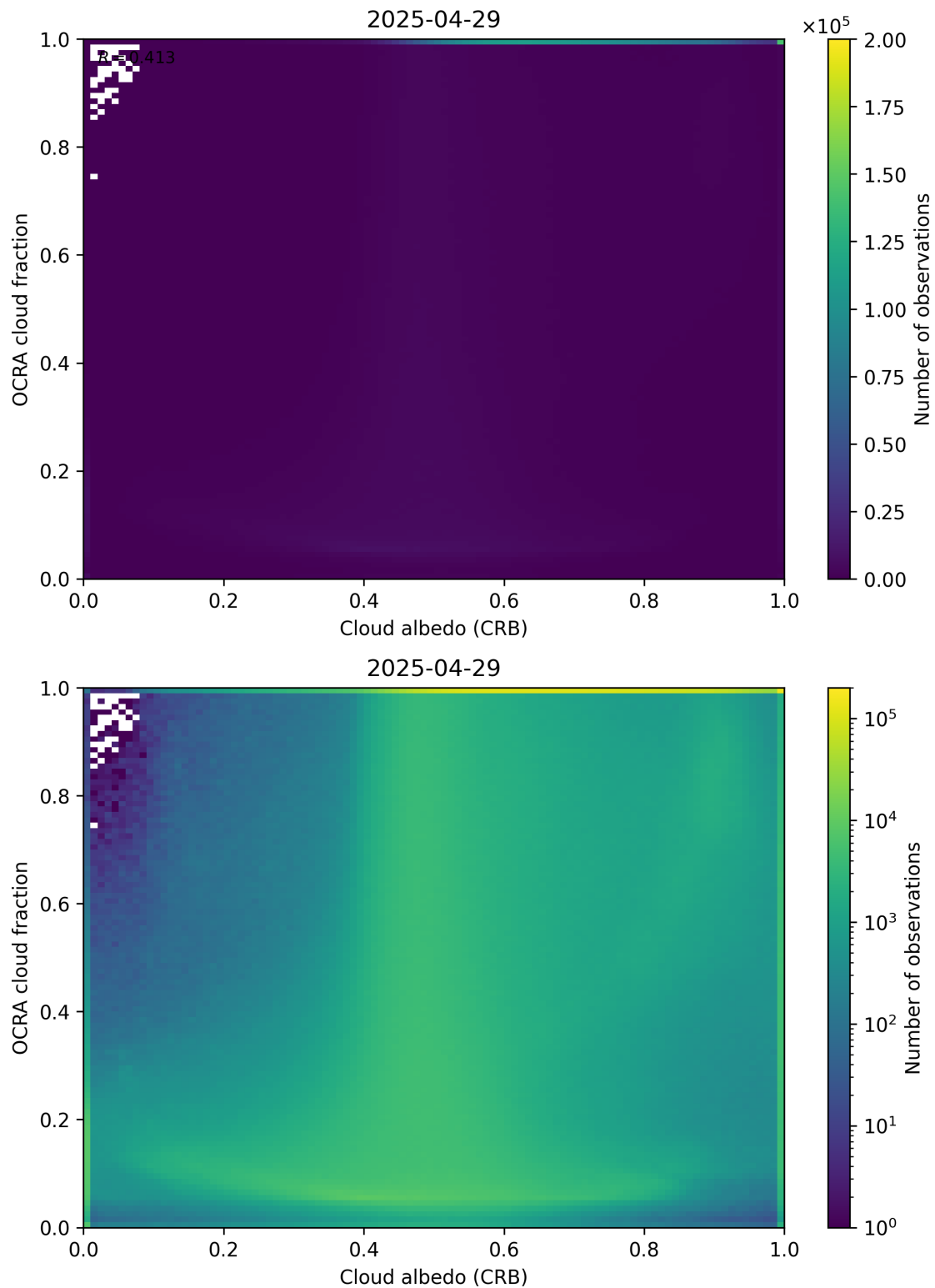
Figure 70: Scatter density plot of “Cloud albedo (CRB)” against “OCRA cloud fraction” for 2025-04-29 to 2025-04-30.
