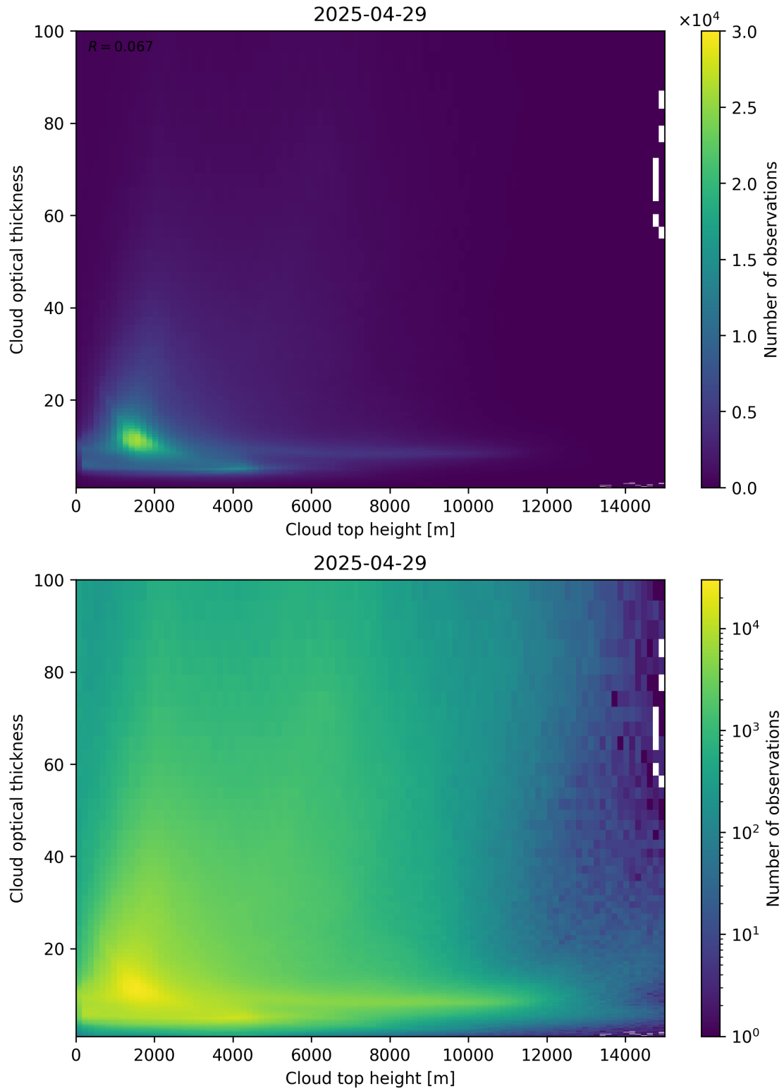
Figure 90: Scatter density plot of “Cloud top height” against “Cloud optical thickness” for 2025-04-29 to 2025-04-30.
