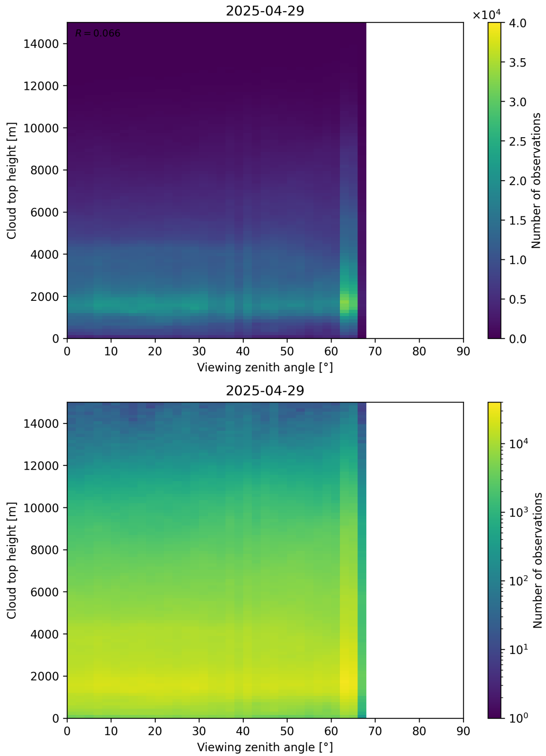
Figure 112: Scatter density plot of “Viewing zenith angle” against “Cloud top height” for 2025-04-29 to 2025-04-30.
