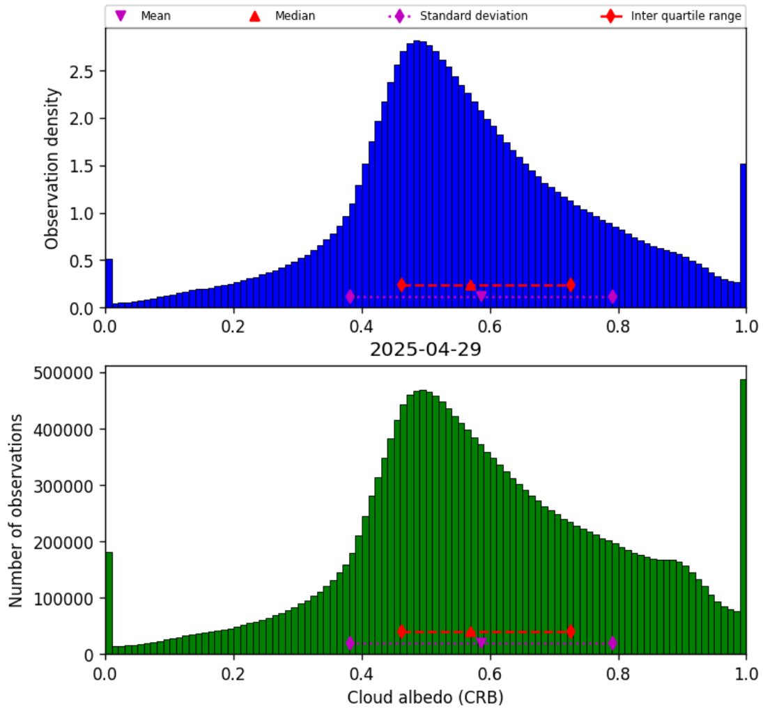
Figure 44: Histogram of “Cloud albedo (CRB)” for 2025-04-29 to 2025-04-30
