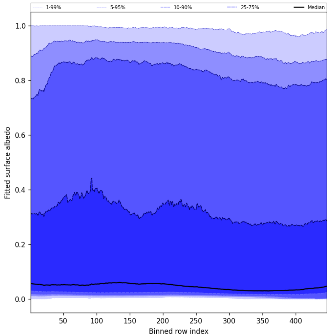
Figure 61: Along track statistics of “Fitted surface albedo” for 2025-04-29 to 2025-04-30
