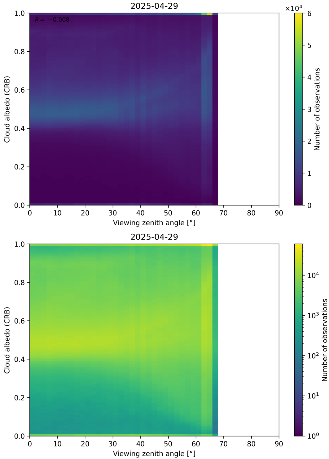
Figure 106: Scatter density plot of “Viewing zenith angle” against “Cloud albedo (CRB)” for 2025-04-29 to 2025-04-30.
