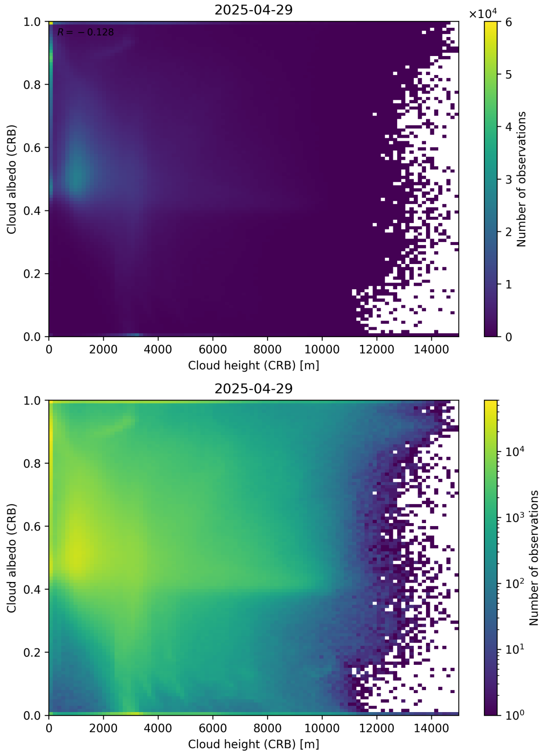
Figure 80: Scatter density plot of “Cloud height (CRB)” against “Cloud albedo (CRB)” for 2025-04-29 to 2025-04-30.
