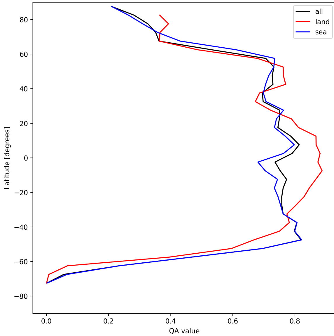
Figure 22: Zonal average of “QA value” for 2025-04-29 to 2025-04-30.
