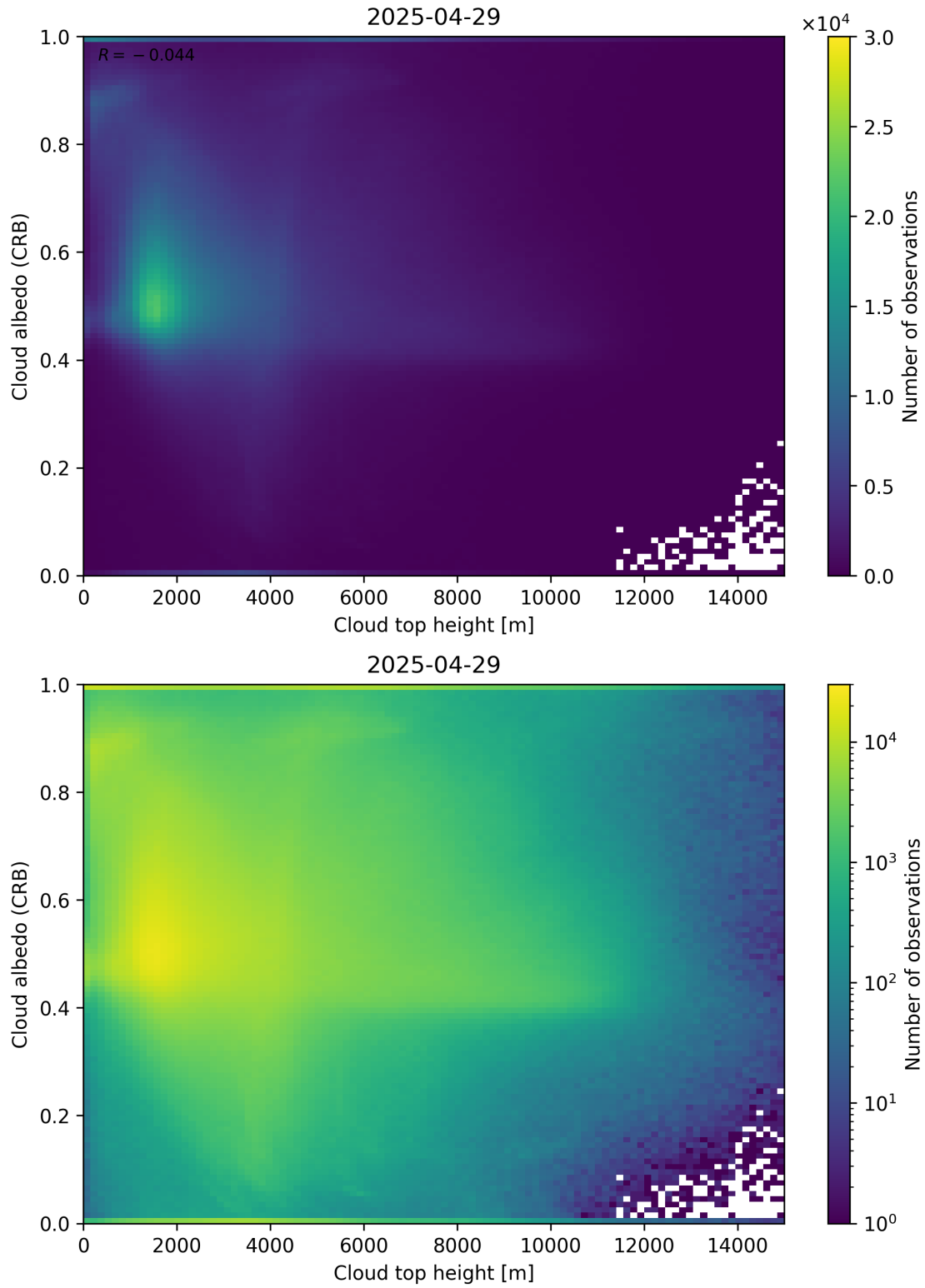
Figure 86: Scatter density plot of “Cloud top height” against “Cloud albedo (CRB)” for 2025-04-29 to 2025-04-30.
