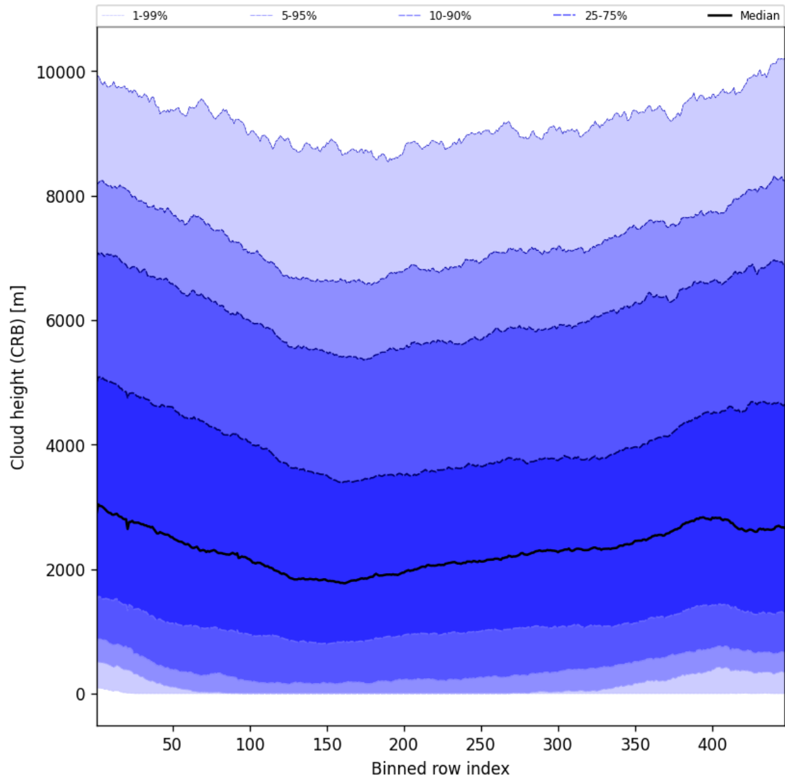
Figure 59: Along track statistics of “Cloud height (CRB)” for 2025-04-29 to 2025-04-30
