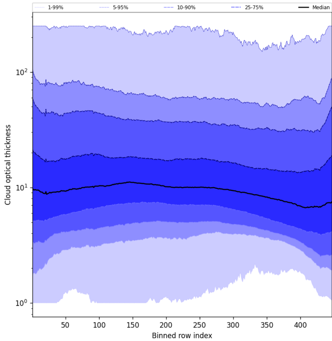
Figure 57: Along track statistics of “Cloud optical thickness” for 2025-04-29 to 2025-04-30
