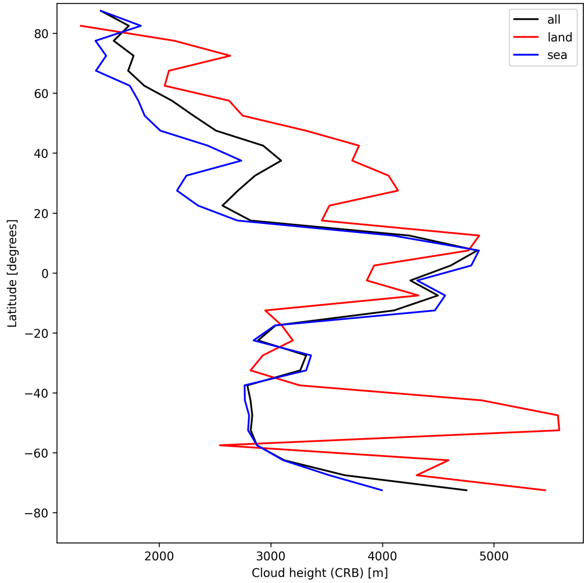
Figure 27: Zonal average of “Cloud height (CRB)” for 2025-04-29 to 2025-04-30.
