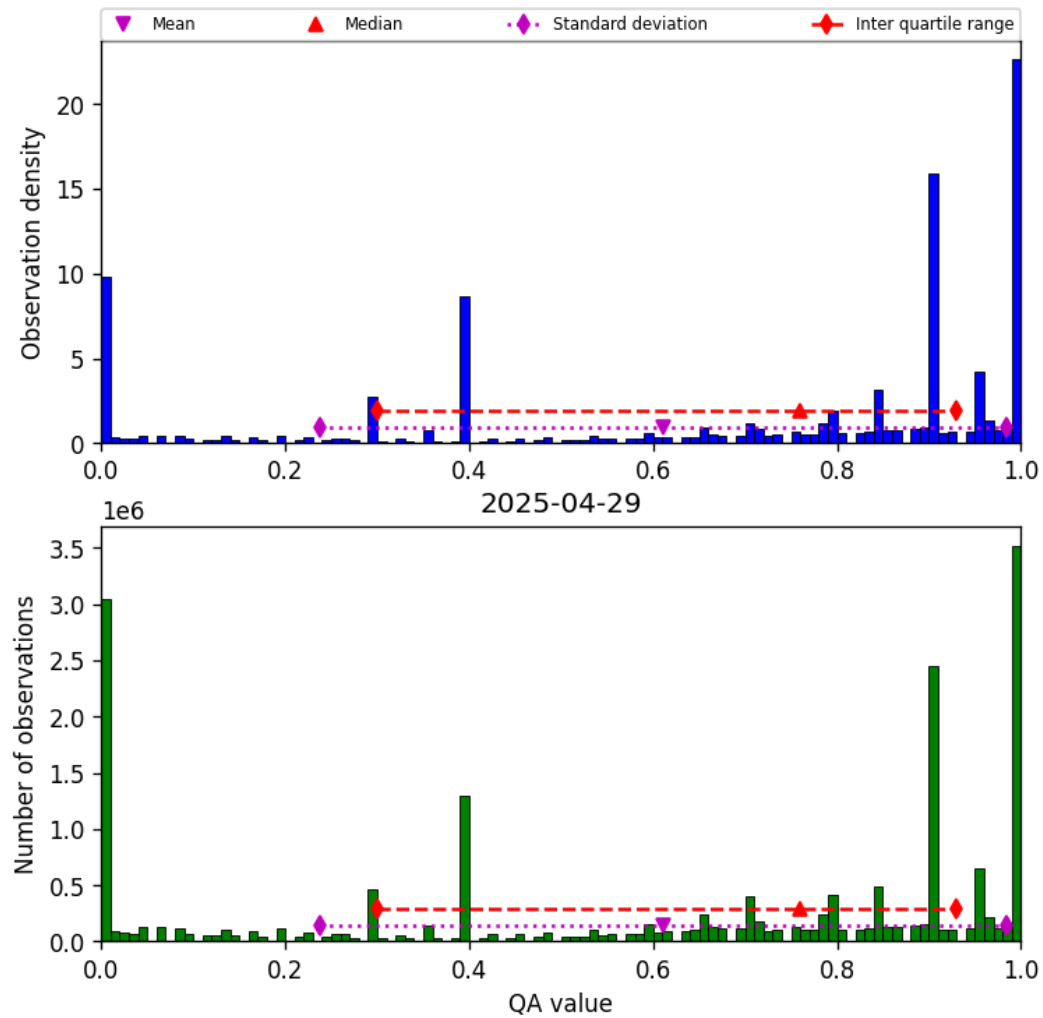
Figure 38: Histogram of “QA value” for 2025-04-29 to 2025-04-30
