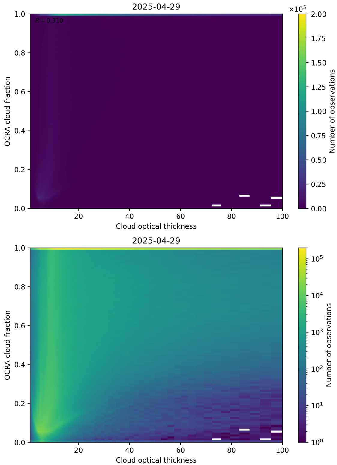
Figure 83: Scatter density plot of “Cloud optical thickness” against “OCRA cloud fraction” for 2025-04-29 to 2025-04-30.
