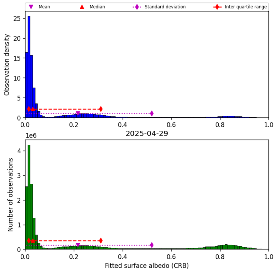
Figure 46: Histogram of “Fitted surface albedo (CRB)” for 2025-04-29 to 2025-04-30
