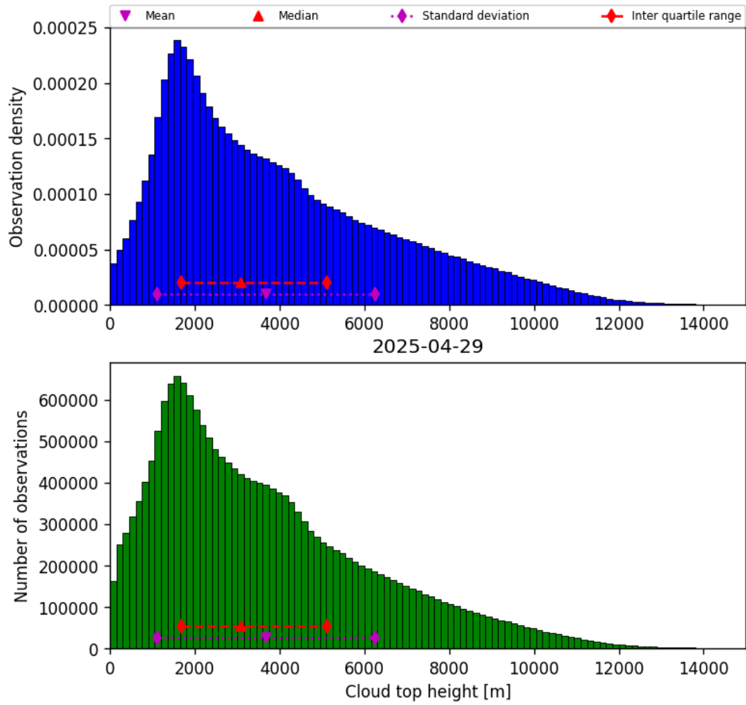
Figure 40: Histogram of “Cloud top height” for 2025-04-29 to 2025-04-30
