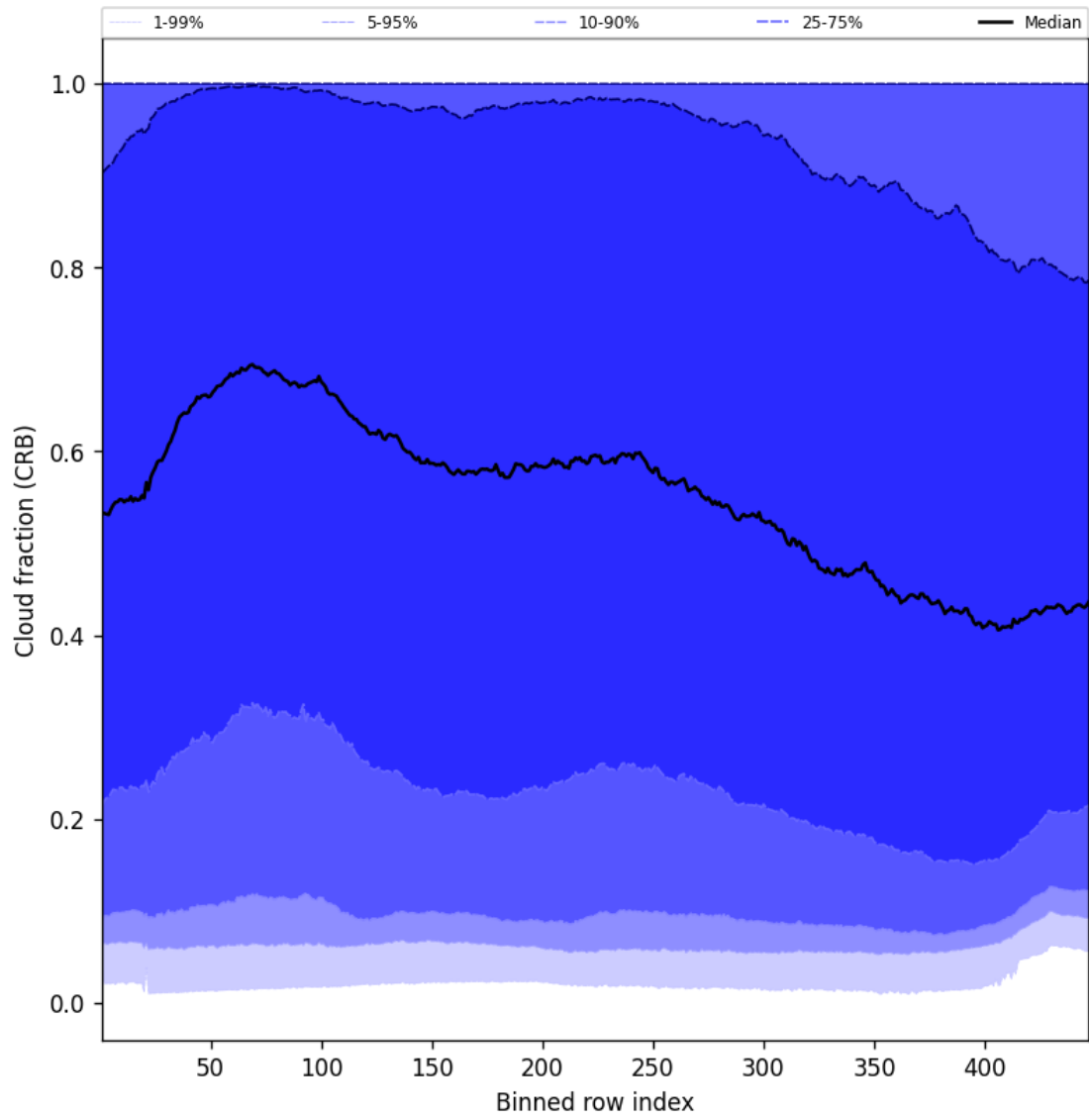
Figure 58: Along track statistics of “Cloud fraction (CRB)” for 2025-04-29 to 2025-04-30
