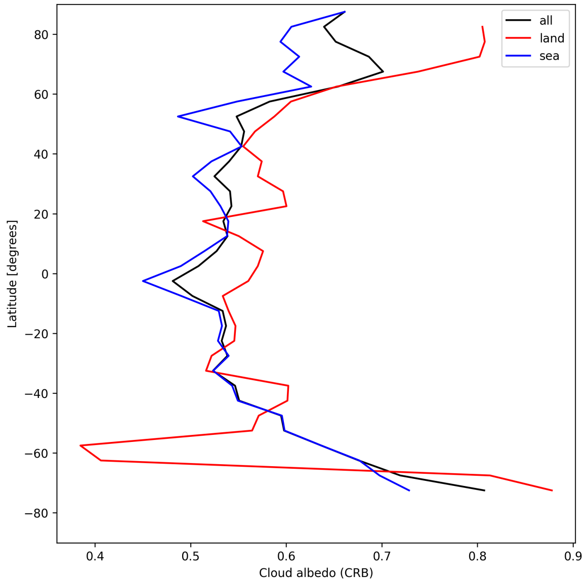
Figure 28: Zonal average of “Cloud albedo (CRB)” for 2025-04-29 to 2025-04-30.
