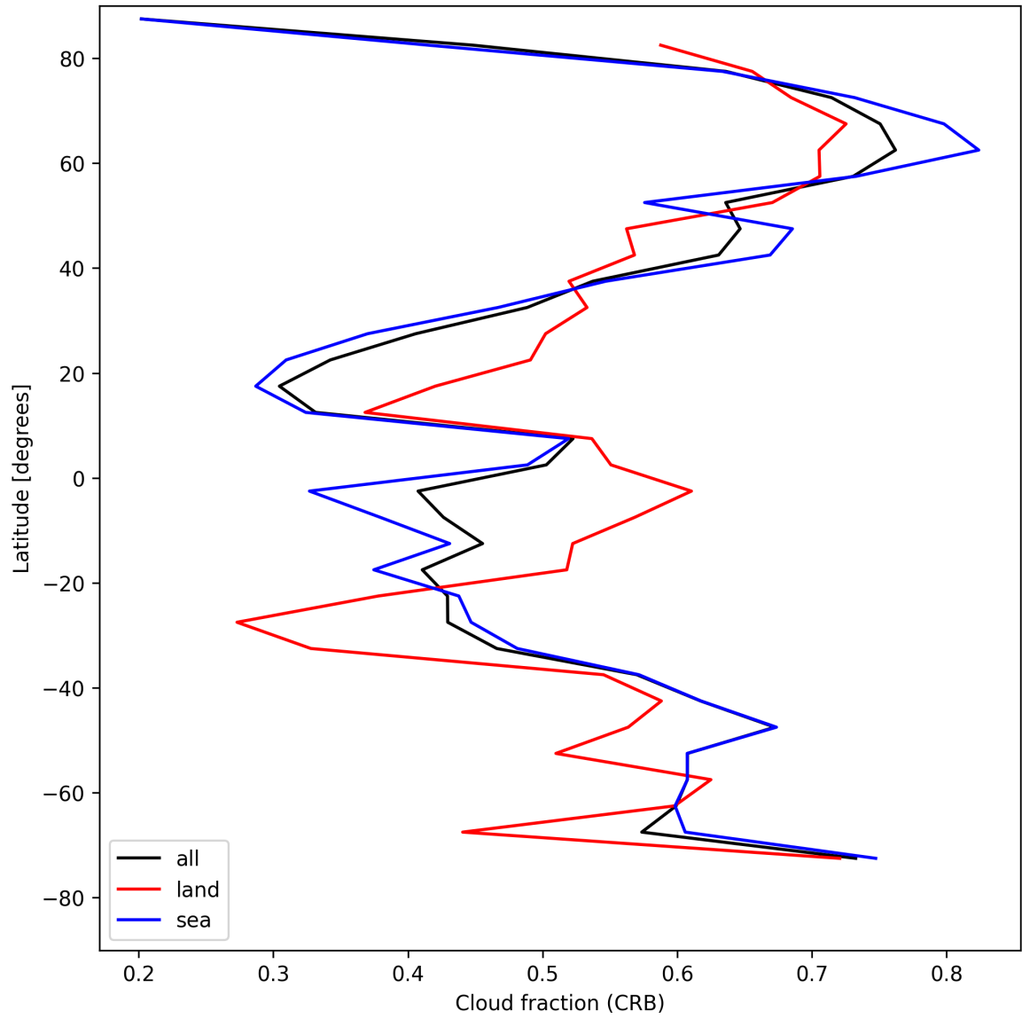
Figure 26: Zonal average of “Cloud fraction (CRB)” for 2025-04-29 to 2025-04-30.
