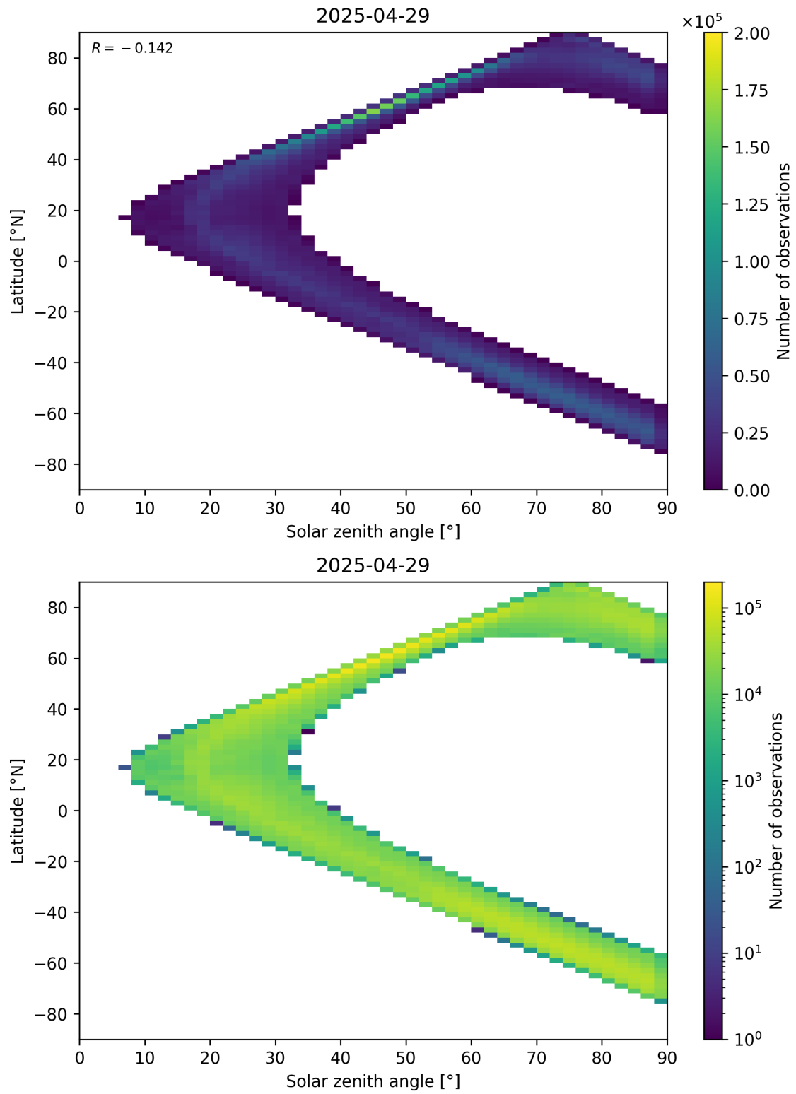
Figure 105: Scatter density plot of “Solar zenith angle” against “Latitude” for 2025-04-29 to 2025-04-30.
