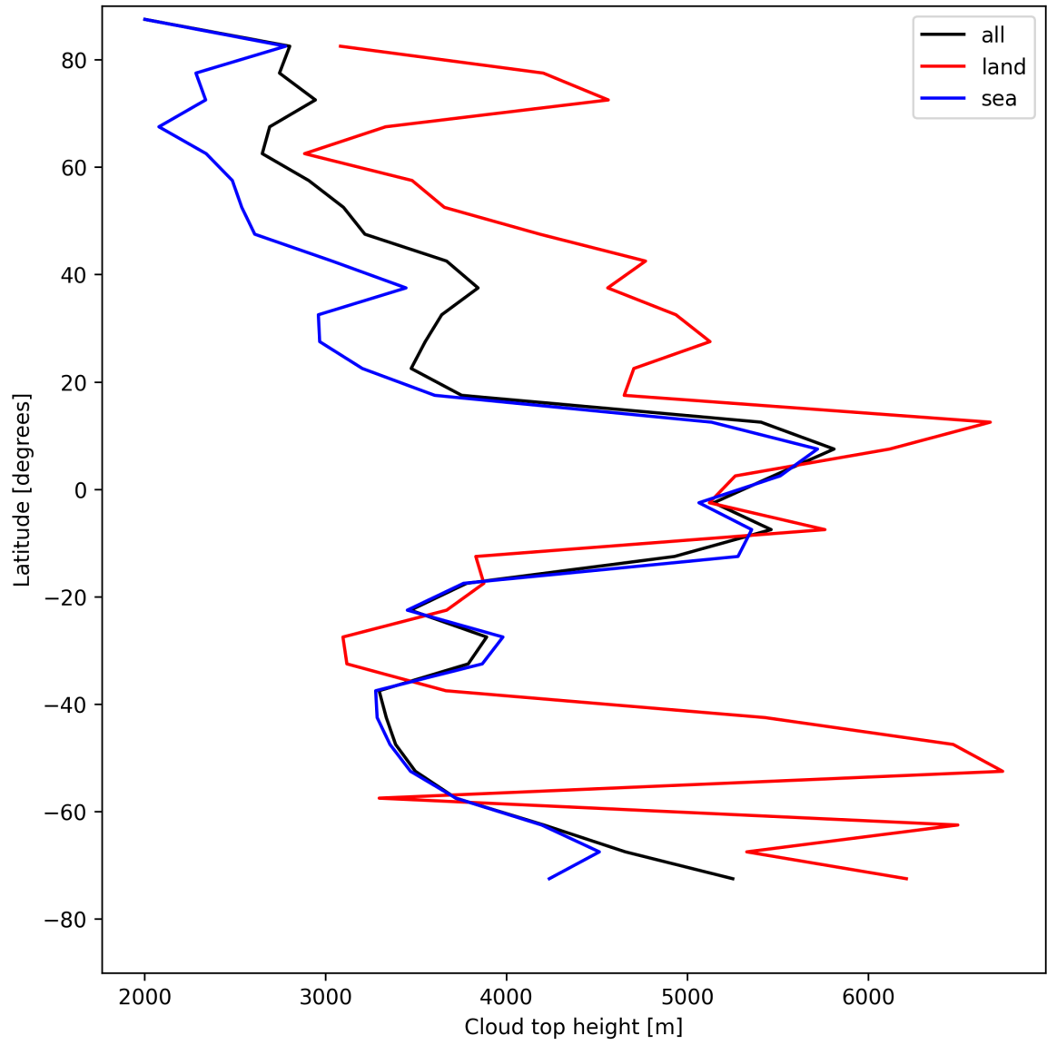
Figure 24: Zonal average of “Cloud top height” for 2025-04-29 to 2025-04-30.
