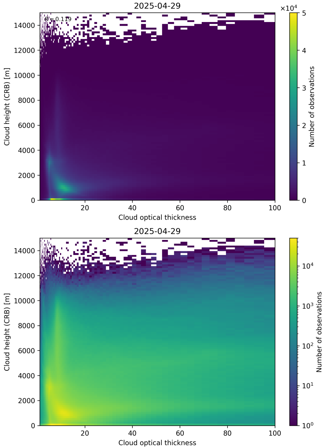
Figure 85: Scatter density plot of “Cloud optical thickness” against “Cloud height (CRB)” for 2025-04-29 to 2025-04-30.
