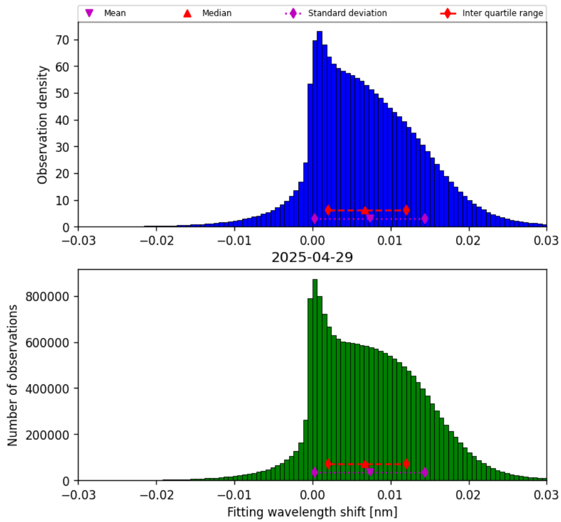
Figure 49: Histogram of “Fitting wavelength shift” for 2025-04-29 to 2025-04-30
