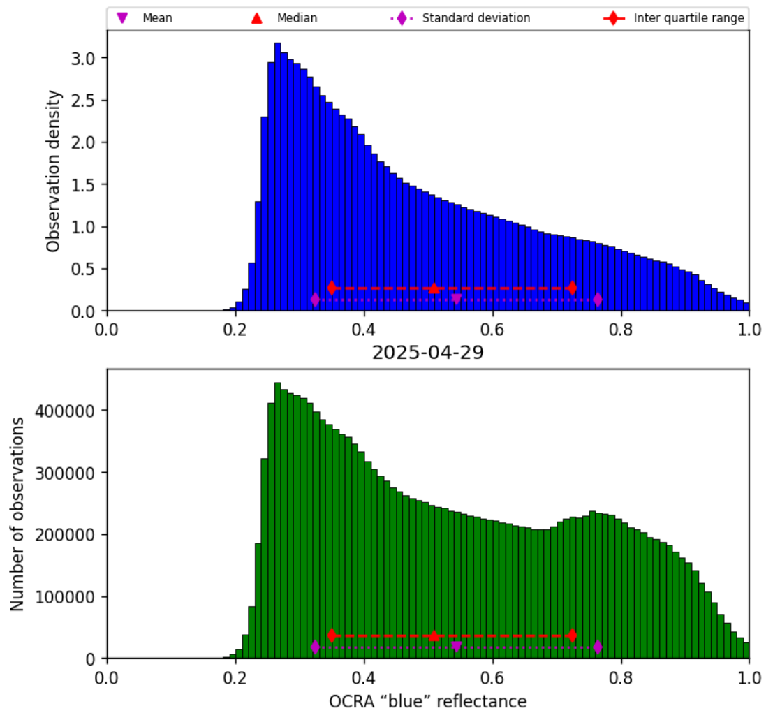
Figure 51: Histogram of “OCRA “blue” reflectance” for 2025-04-29 to 2025-04-30
