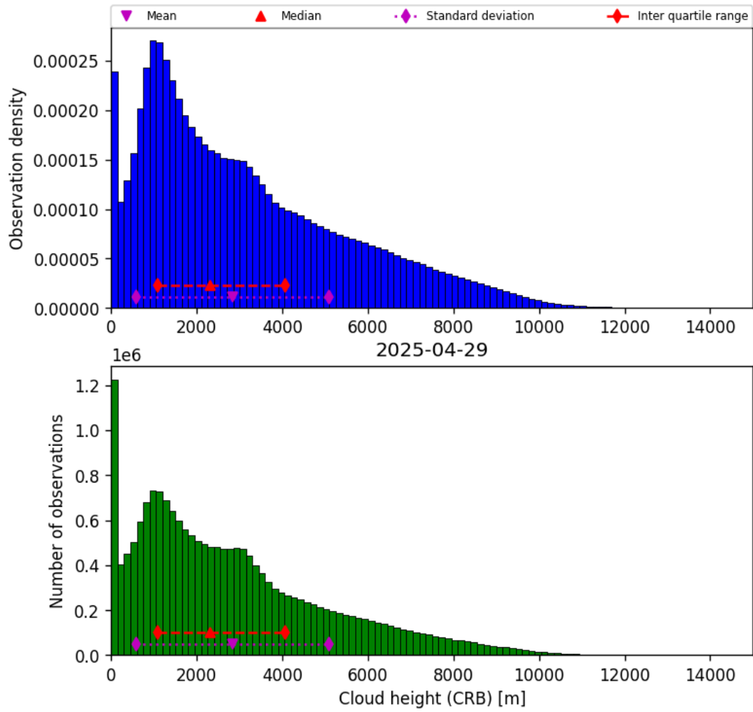
Figure 43: Histogram of “Cloud height (CRB)” for 2025-04-29 to 2025-04-30
