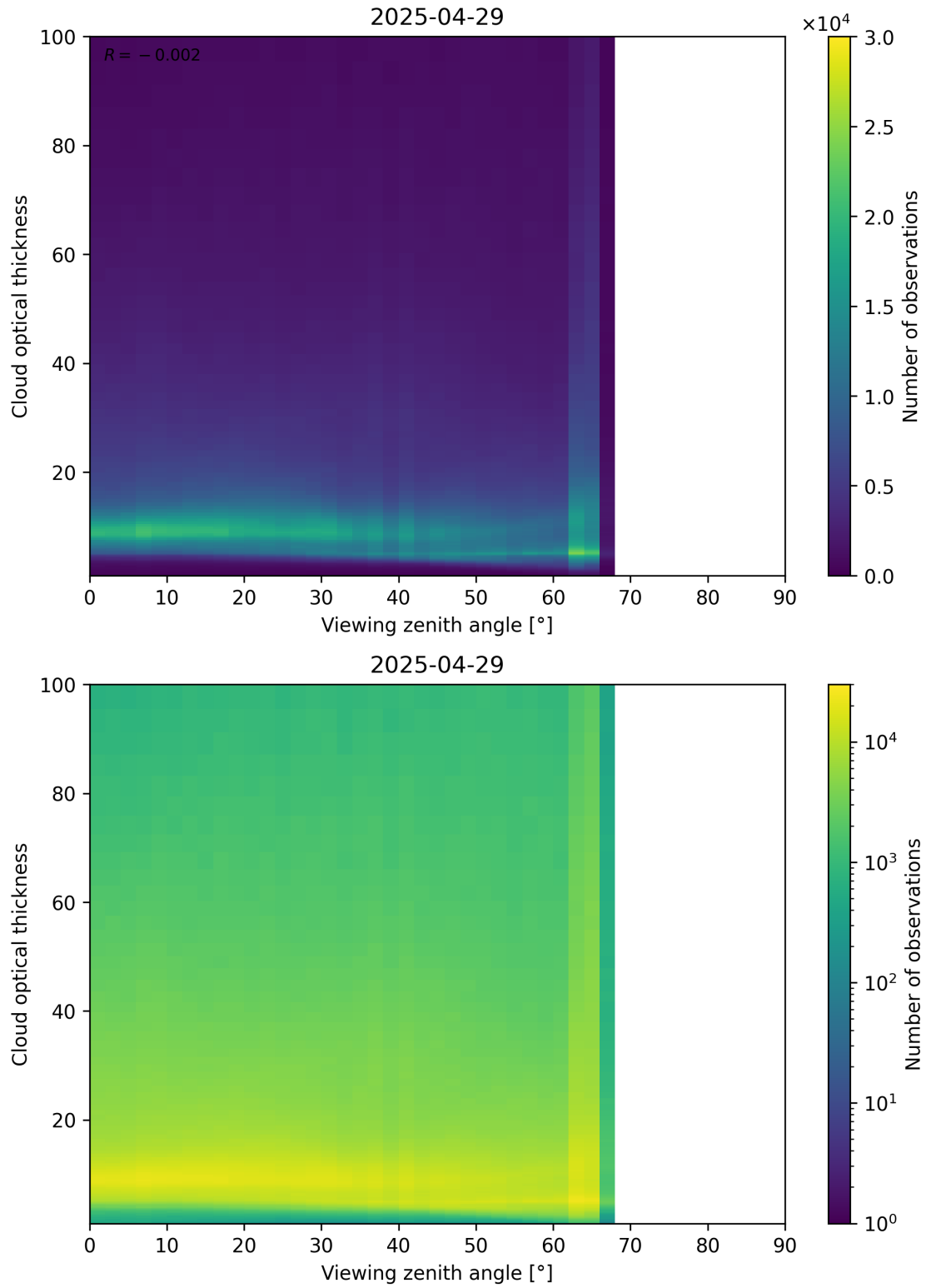
Figure 111: Scatter density plot of “Viewing zenith angle” against “Cloud optical thickness” for 2025-04-29 to 2025-04-30.
