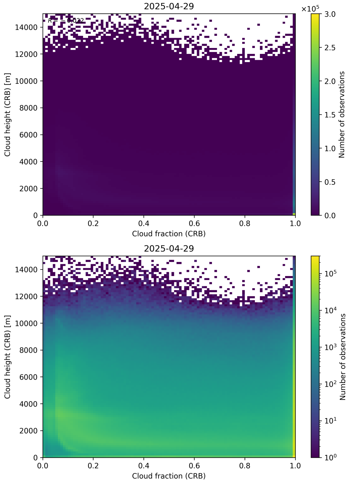
Figure 79: Scatter density plot of “Cloud fraction (CRB)” against “Cloud height (CRB)” for 2025-04-29 to 2025-04-30.
