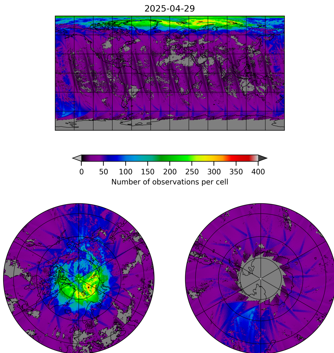
Figure 21: Map of the number of observations for 2025-04-29 to 2025-04-30
