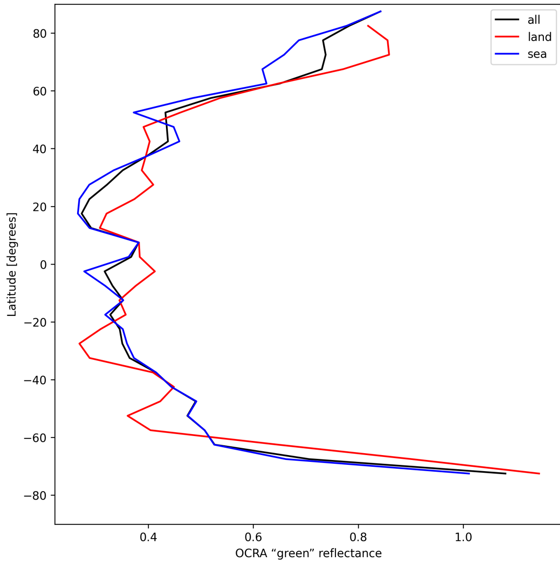
Figure 36: Zonal average of “OCRA “green” reflectance” for 2025-04-29 to 2025-04-30.
