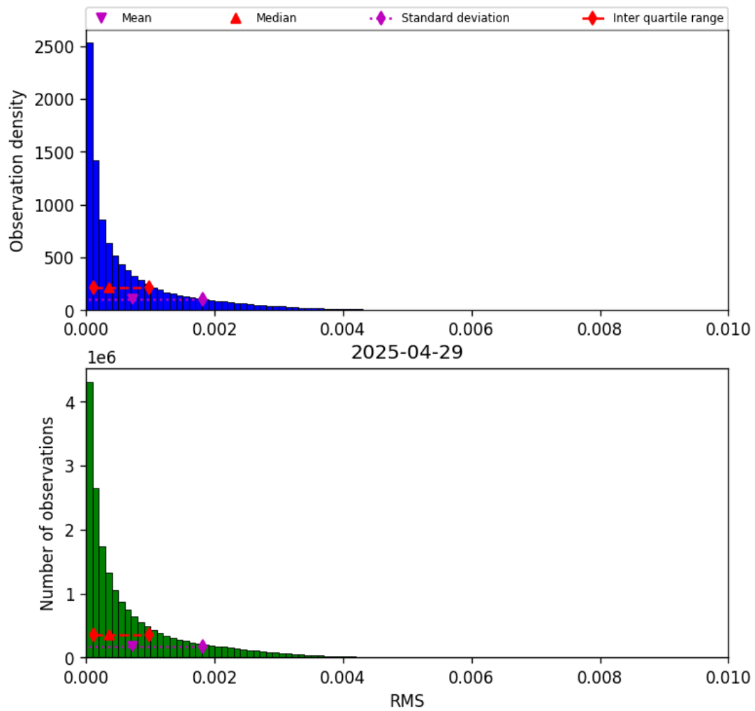
Figure 47: Histogram of “RMS” for 2025-04-29 to 2025-04-30
