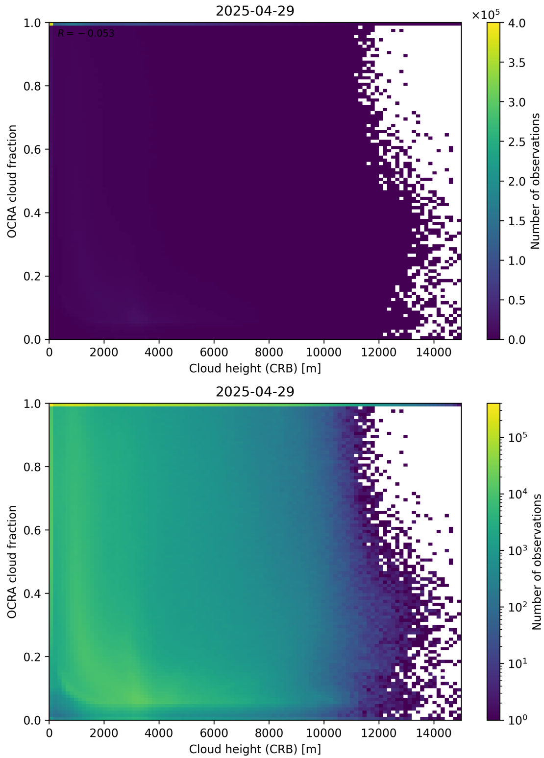
Figure 81: Scatter density plot of “Cloud height (CRB)” against “OCRA cloud fraction” for 2025-04-29 to 2025-04-30.
