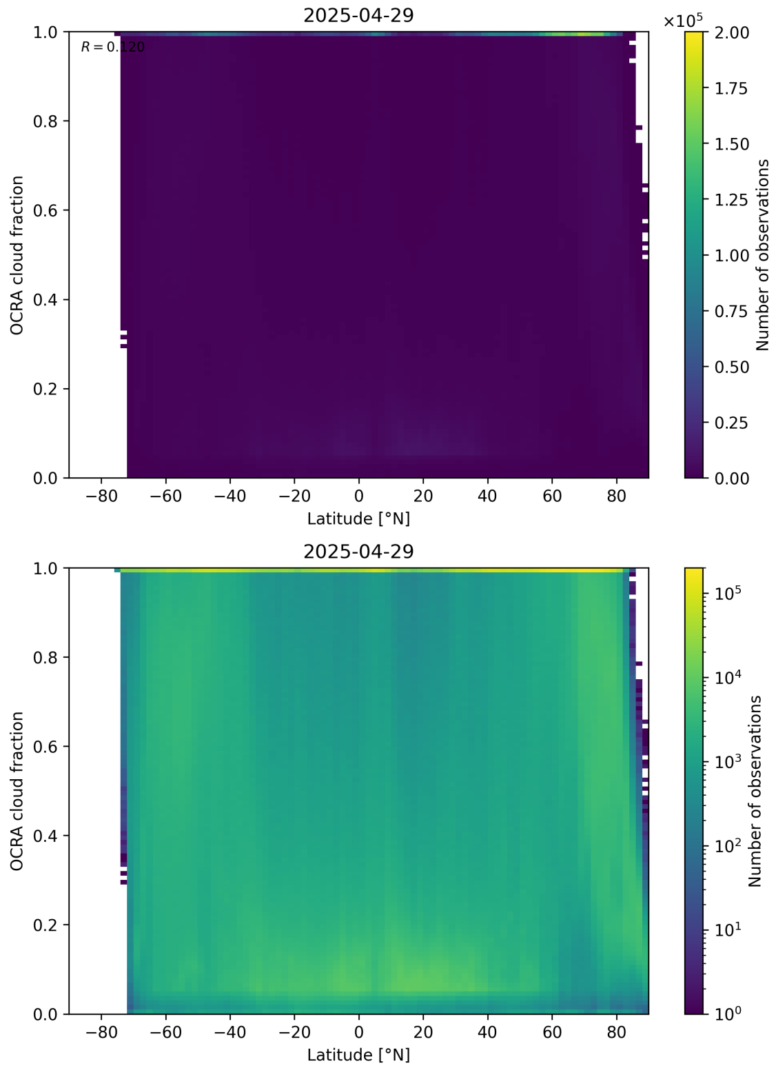
Figure 93: Scatter density plot of “Latitude” against “OCRA cloud fraction” for 2025-04-29 to 2025-04-30.
