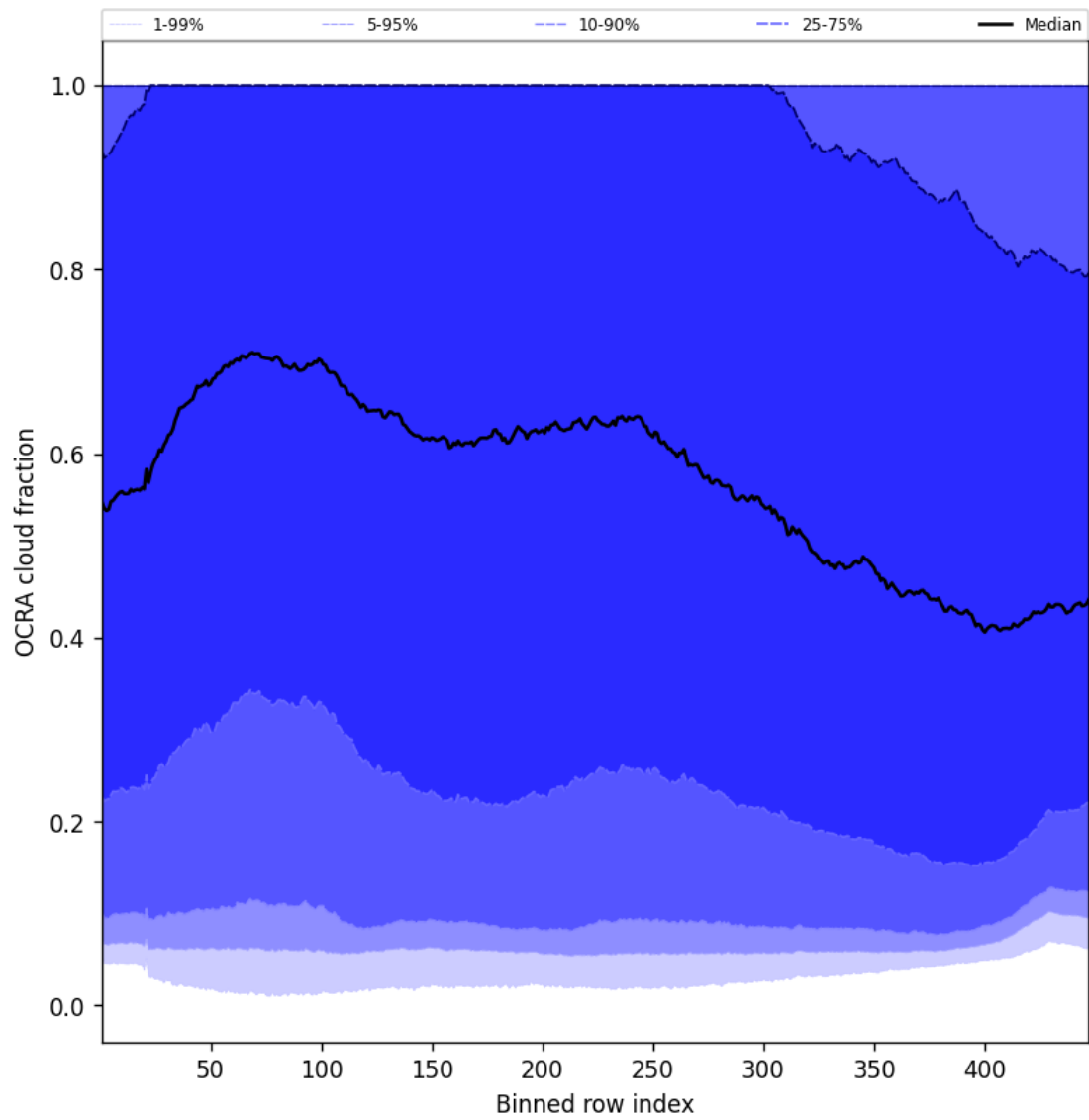
Figure 66: Along track statistics of “OCRA cloud fraction” for 2025-04-29 to 2025-04-30
