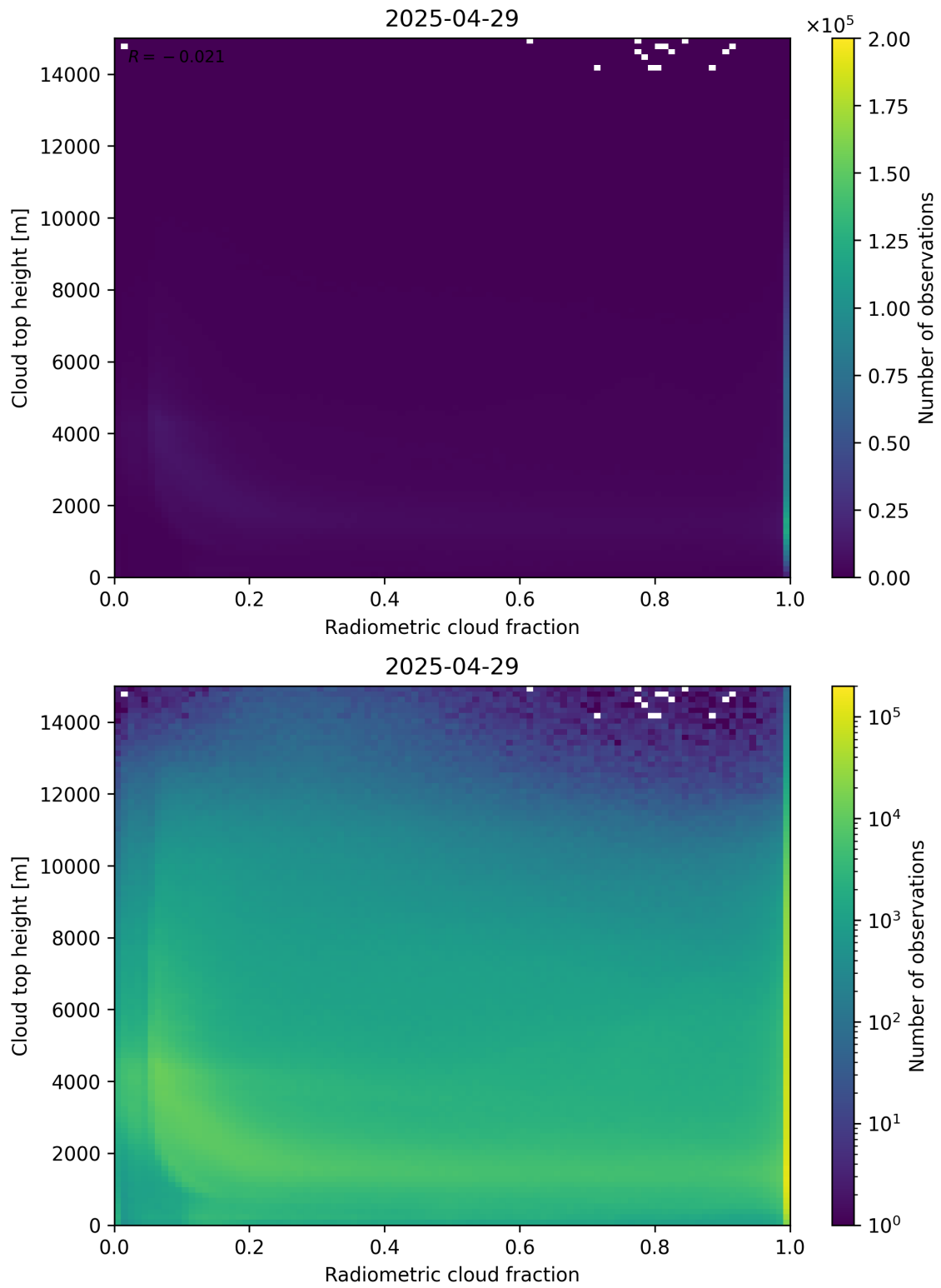
Figure 76: Scatter density plot of “Radiometric cloud fraction” against “Cloud top height” for 2025-04-29 to 2025-04-30.
