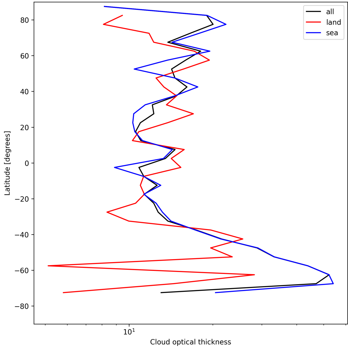
Figure 25: Zonal average of “Cloud optical thickness” for 2025-04-29 to 2025-04-30.
