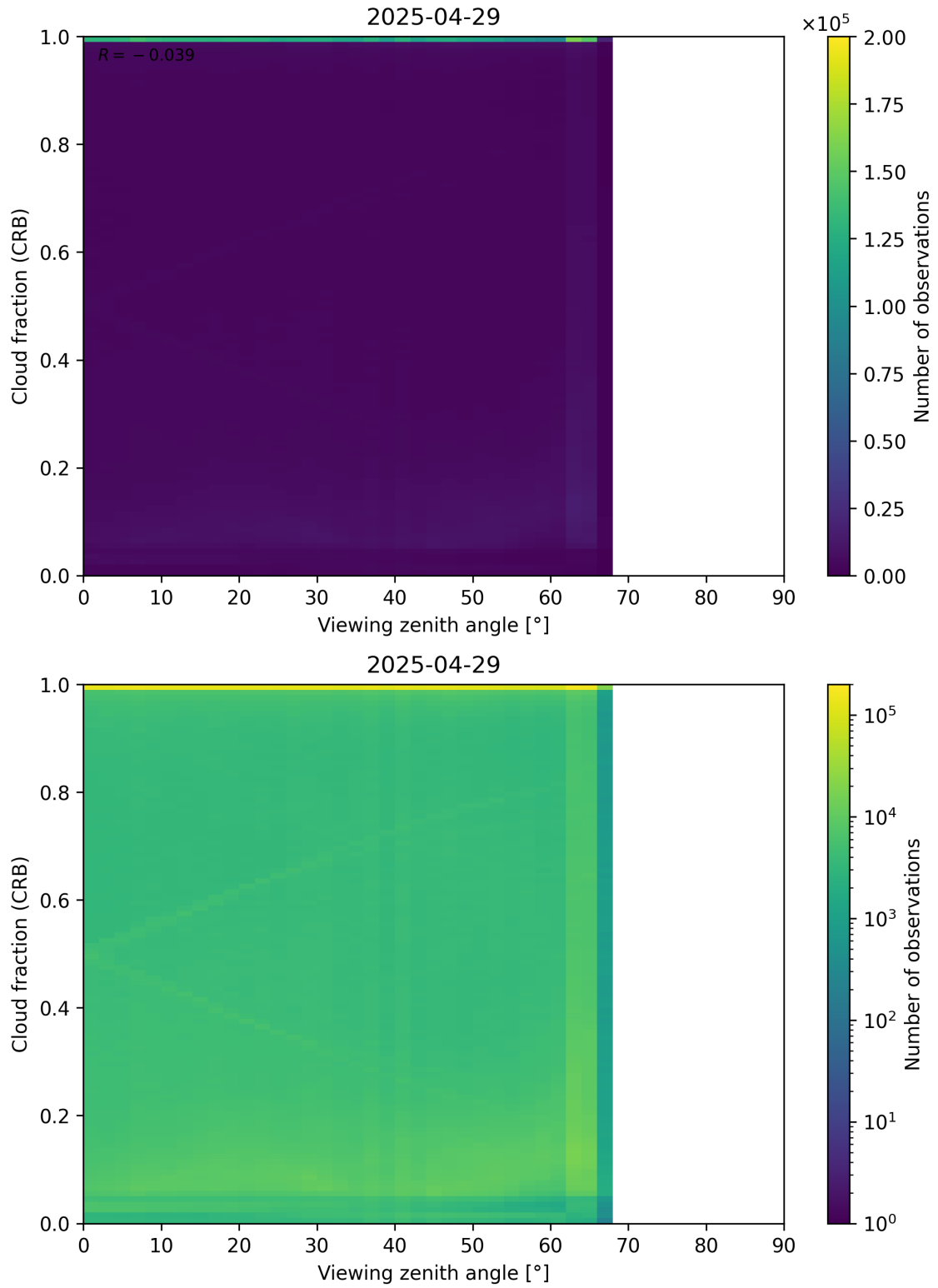
Figure 109: Scatter density plot of “Viewing zenith angle” against “Cloud fraction (CRB)” for 2025-04-29 to 2025-04-30.
