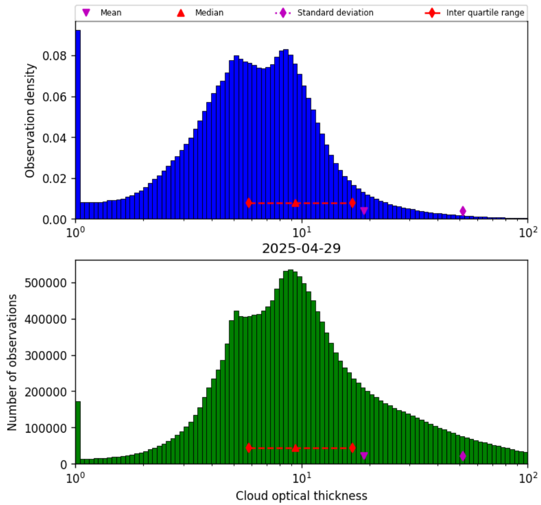
Figure 41: Histogram of “Cloud optical thickness” for 2025-04-29 to 2025-04-30
