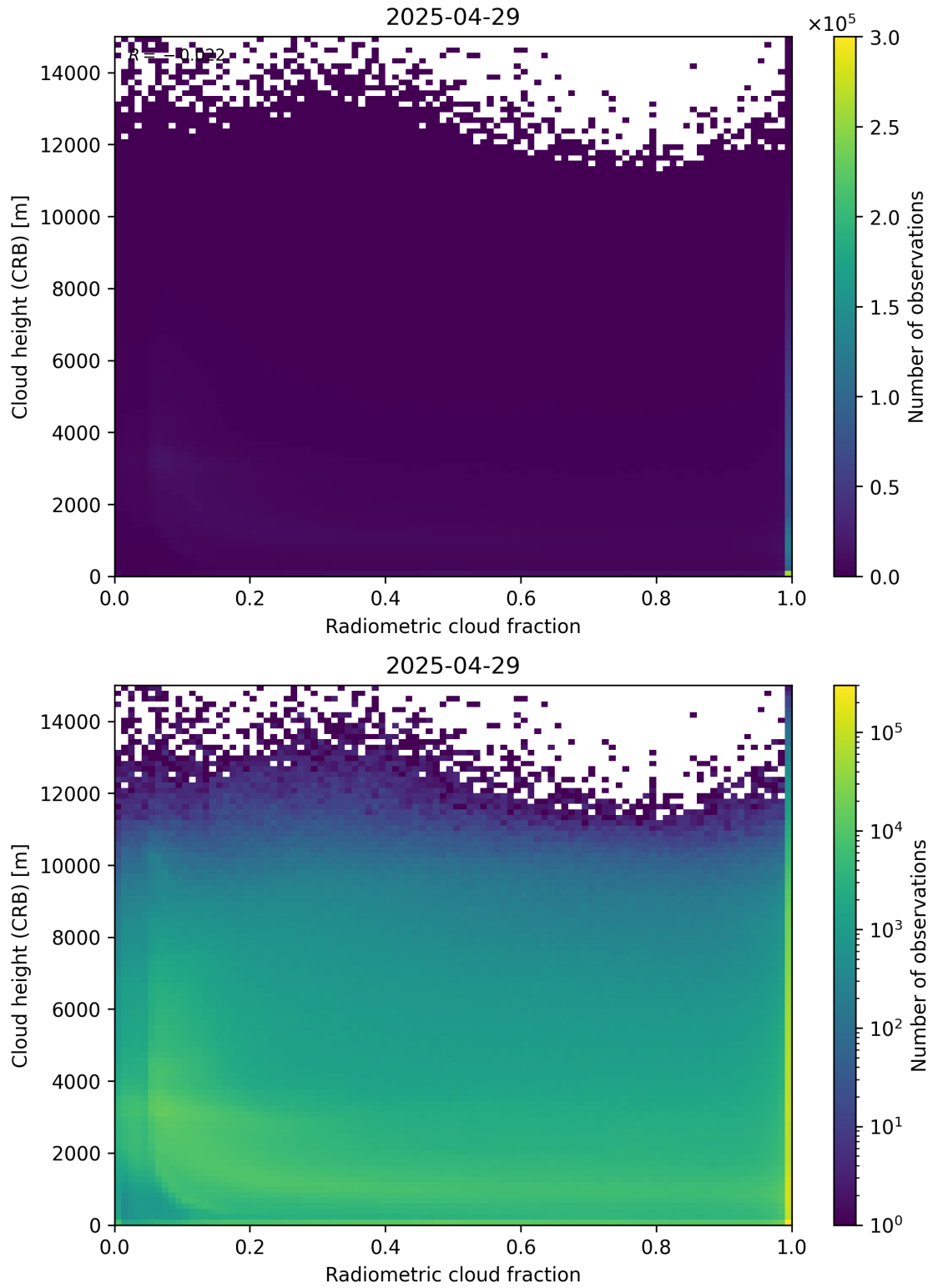
Figure 74: Scatter density plot of “Radiometric cloud fraction” against “Cloud height (CRB)” for 2025-04-29 to 2025-04-30.
