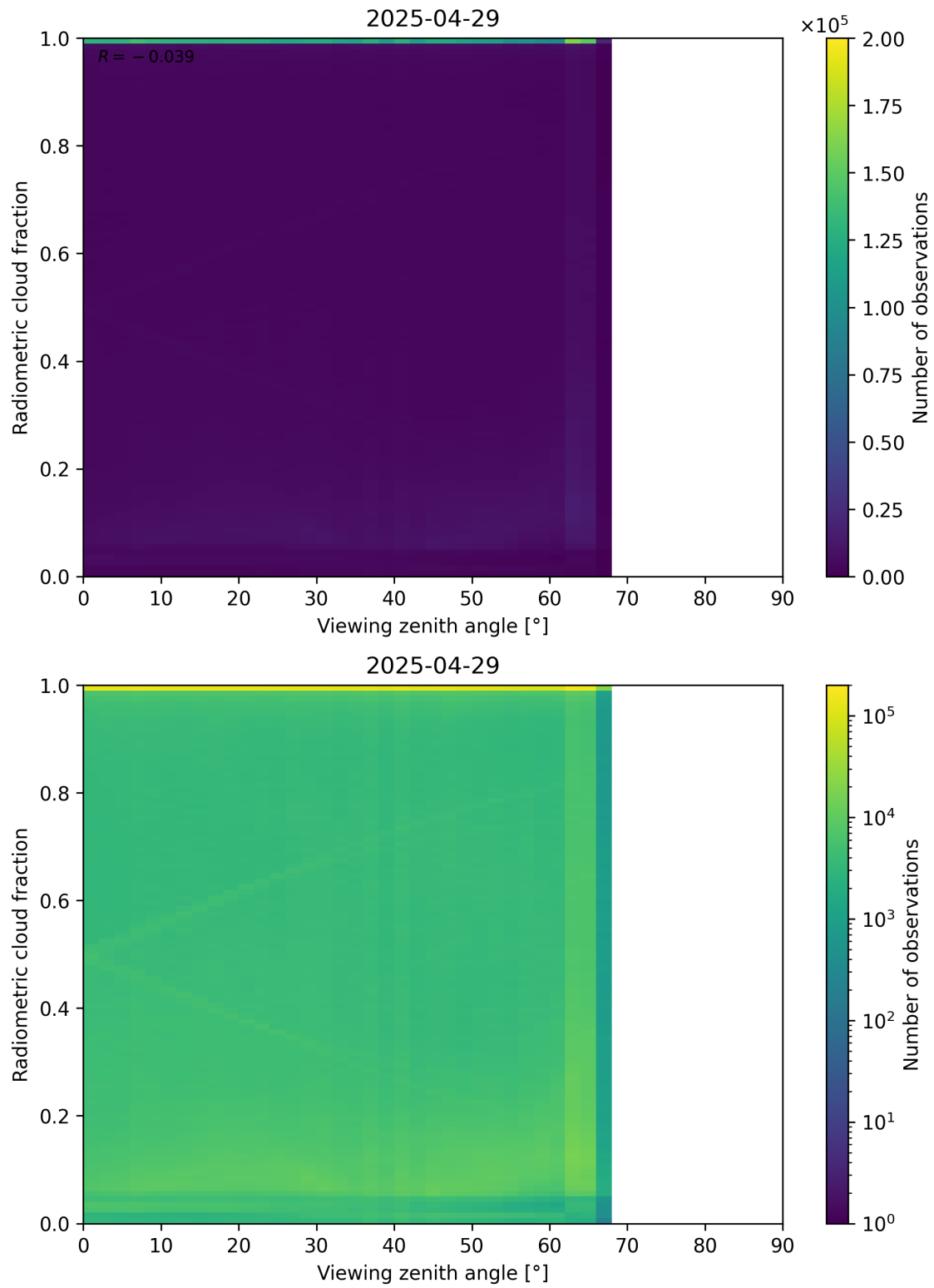
Figure 107: Scatter density plot of “Viewing zenith angle” against “Radiometric cloud fraction” for 2025-04-29 to 2025-04-30.
