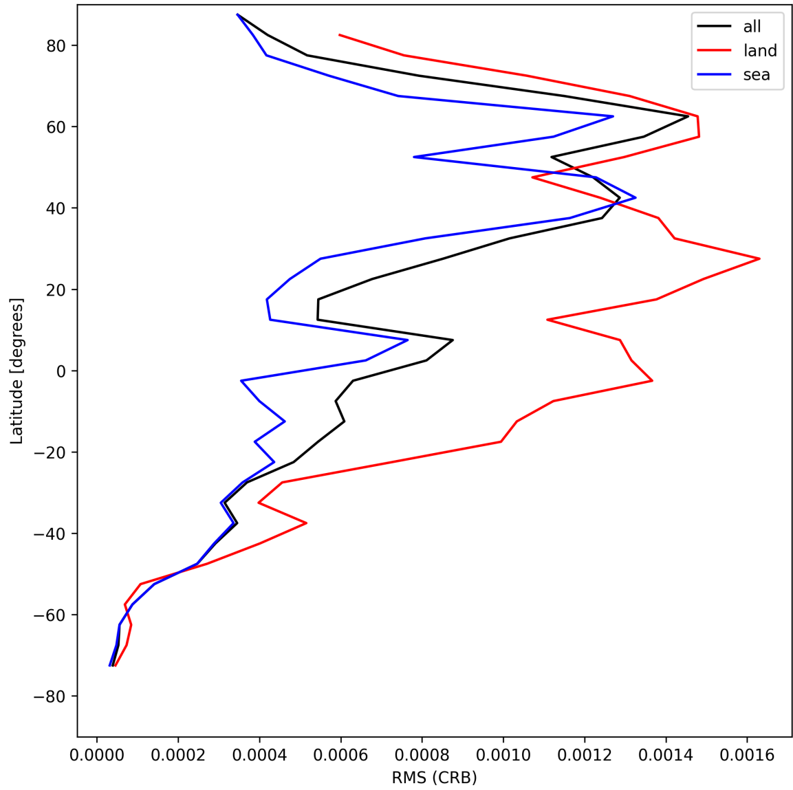
Figure 32: Zonal average of “RMS (CRB)” for 2025-04-29 to 2025-04-30.
