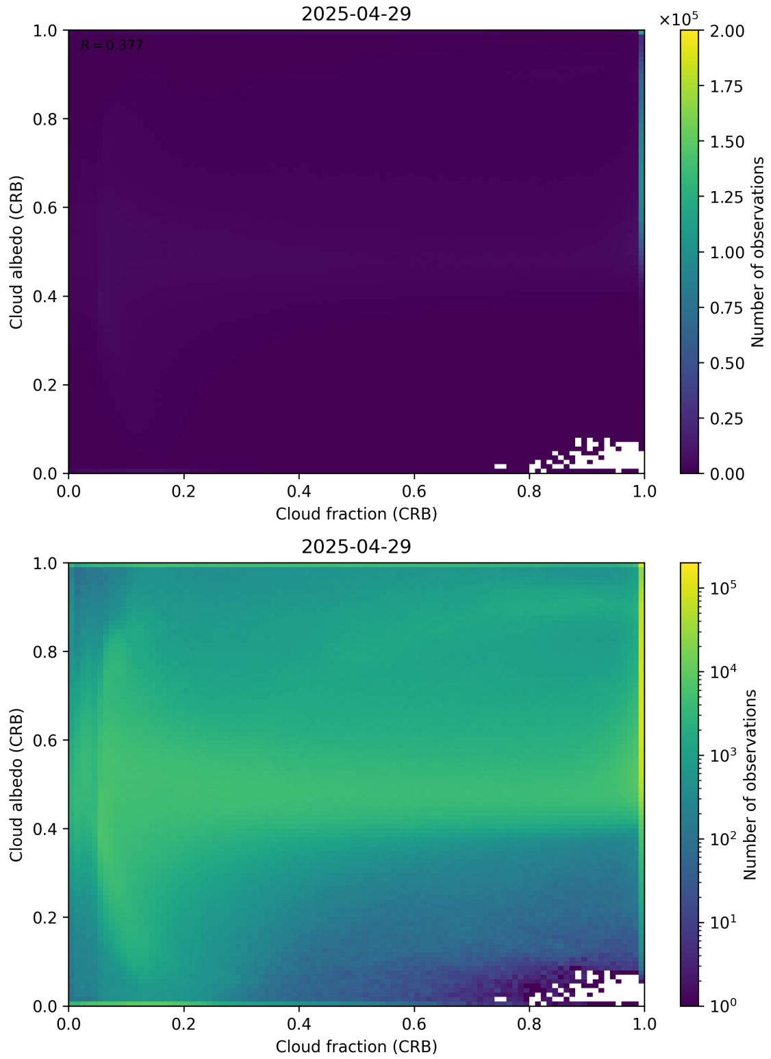
Figure 77: Scatter density plot of “Cloud fraction (CRB)” against “Cloud albedo (CRB)” for 2025-04-29 to 2025-04-30.
