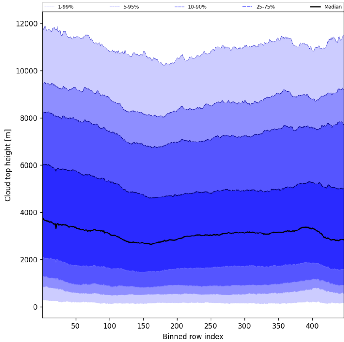
Figure 56: Along track statistics of “Cloud top height” for 2025-04-29 to 2025-04-30
