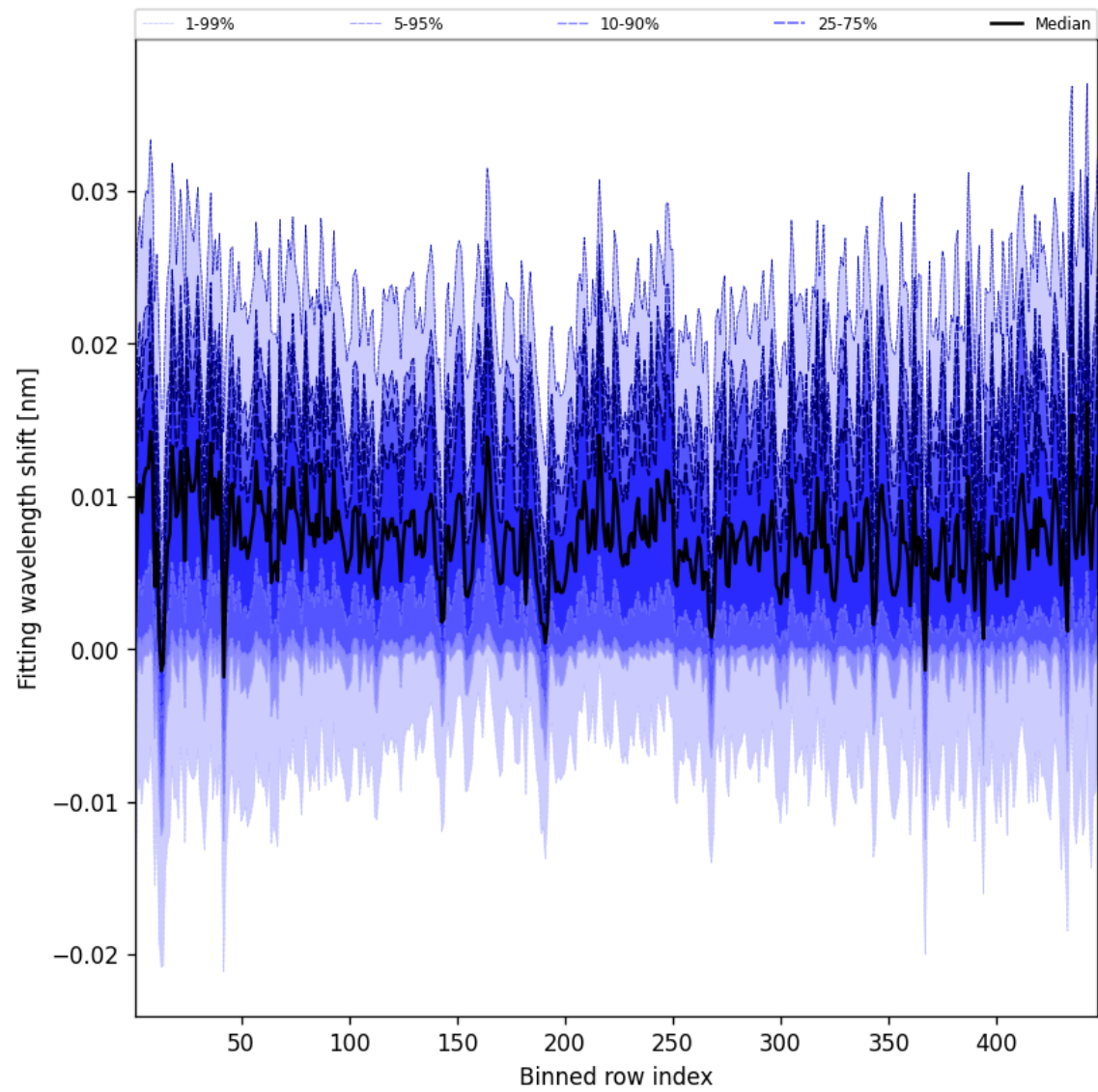
Figure 65: Along track statistics of “Fitting wavelength shift” for 2025-04-29 to 2025-04-30
