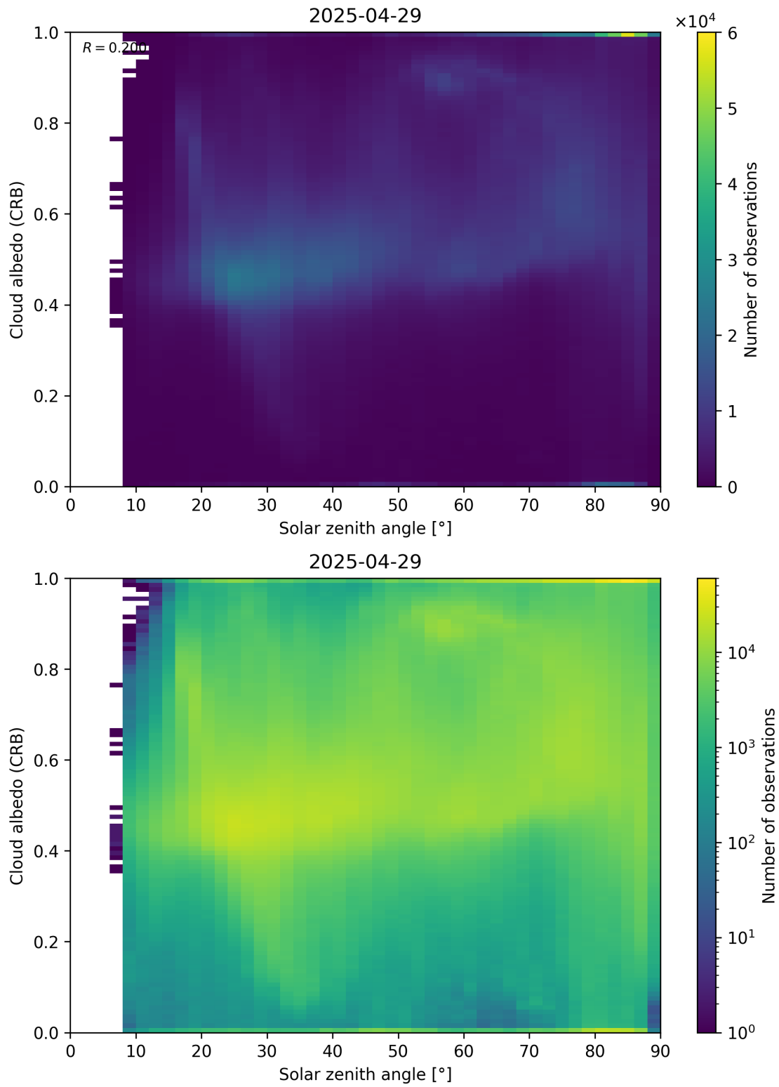
Figure 98: Scatter density plot of “Solar zenith angle” against “Cloud albedo (CRB)” for 2025-04-29 to 2025-04-30.
