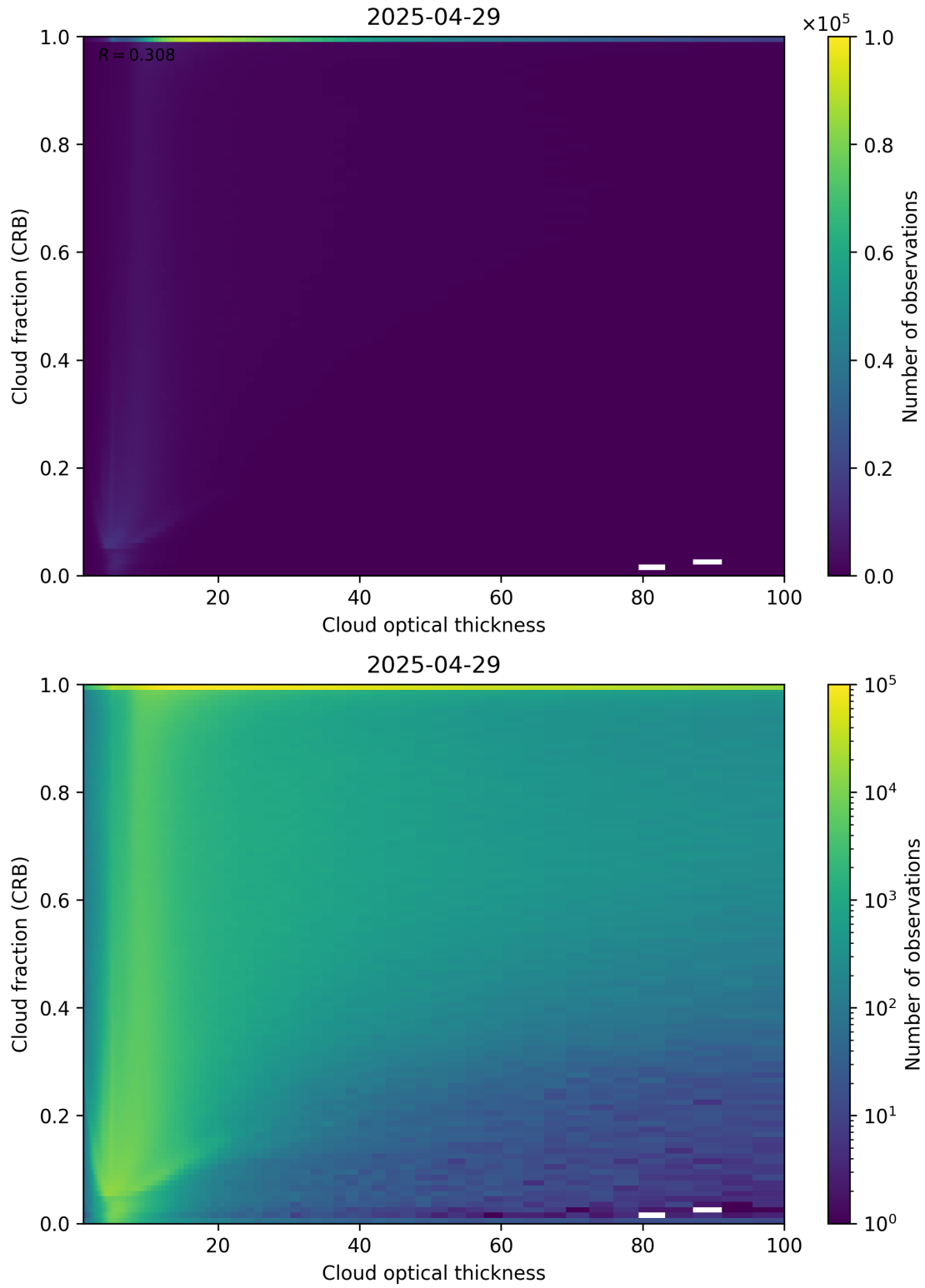
Figure 84: Scatter density plot of “Cloud optical thickness” against “Cloud fraction (CRB)” for 2025-04-29 to 2025-04-30.
