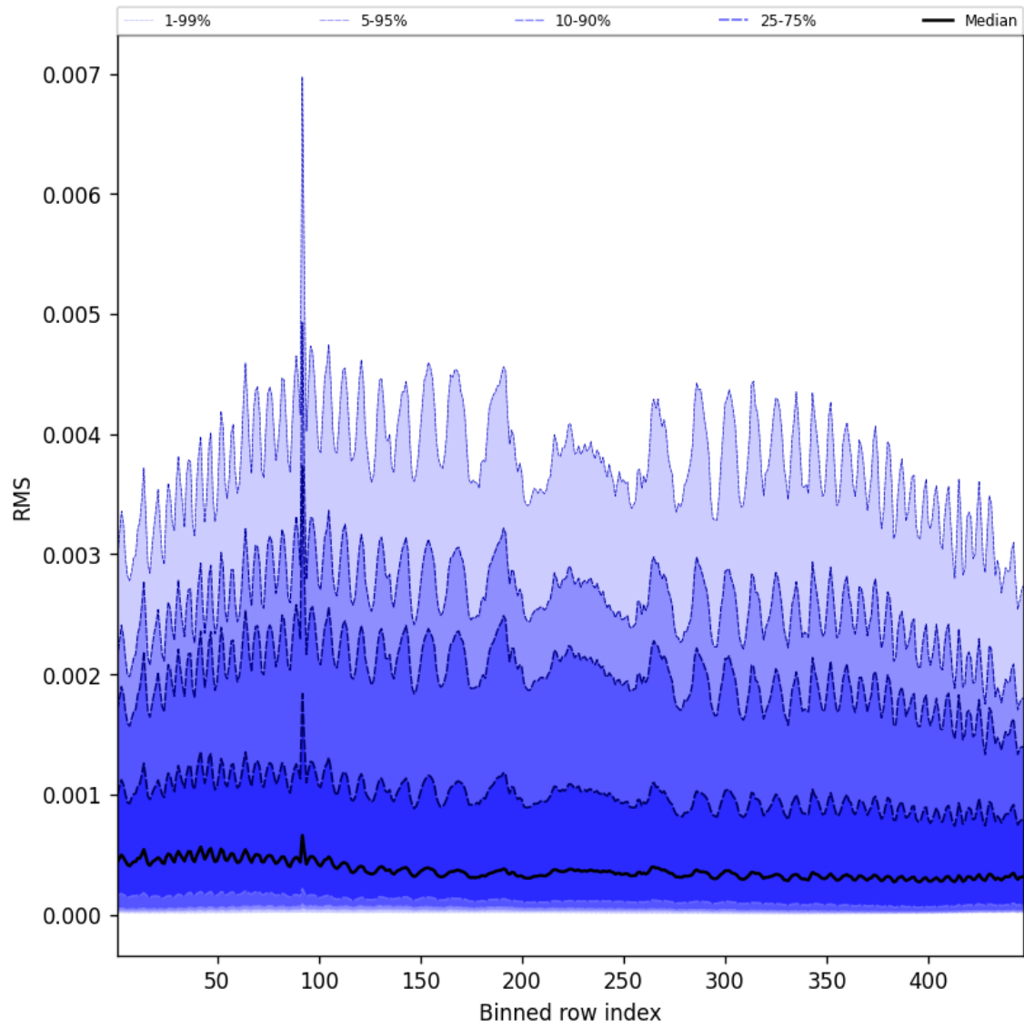
Figure 63: Along track statistics of “RMS” for 2025-04-29 to 2025-04-30
