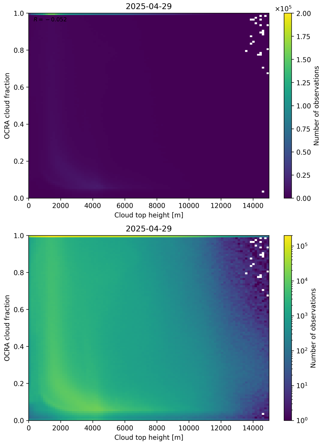
Figure 87: Scatter density plot of “Cloud top height” against “OCRA cloud fraction” for 2025-04-29 to 2025-04-30.
