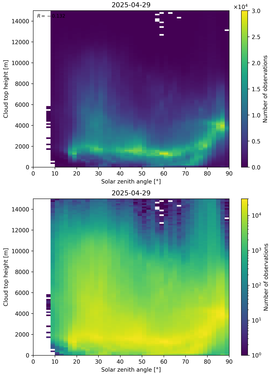
Figure 104: Scatter density plot of “Solar zenith angle” against “Cloud top height” for 2025-04-29 to 2025-04-30.
