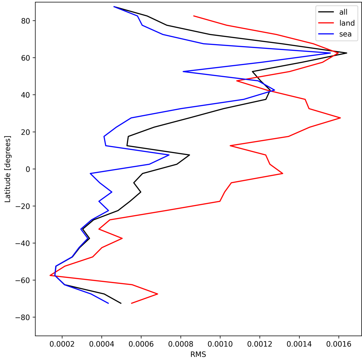
Figure 31: Zonal average of “RMS” for 2025-04-29 to 2025-04-30.
