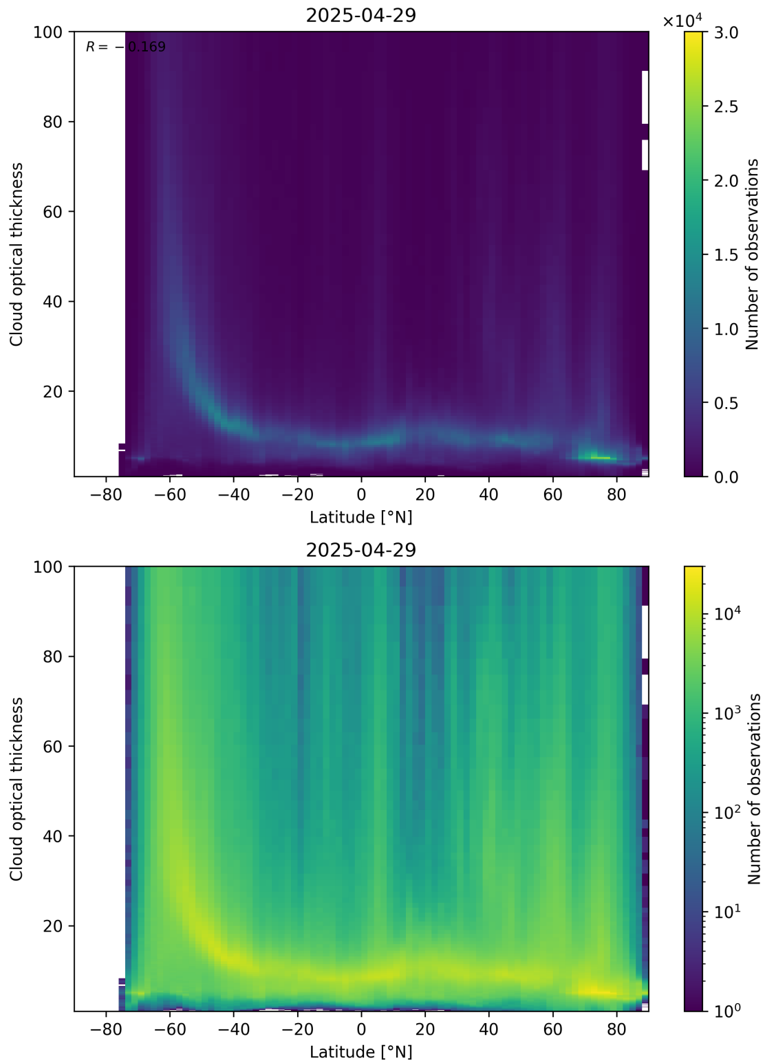
Figure 96: Scatter density plot of “Latitude” against “Cloud optical thickness” for 2025-04-29 to 2025-04-30.
