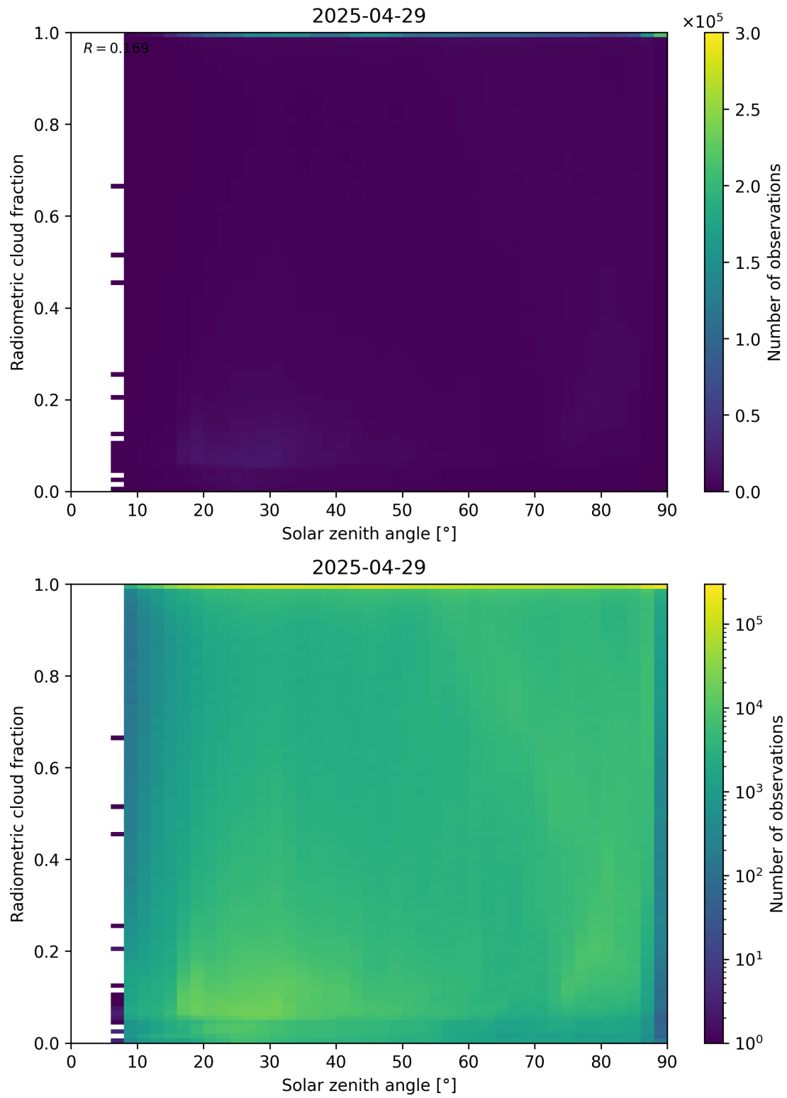
Figure 99: Scatter density plot of “Solar zenith angle” against “Radiometric cloud fraction” for 2025-04-29 to 2025-04-30.
