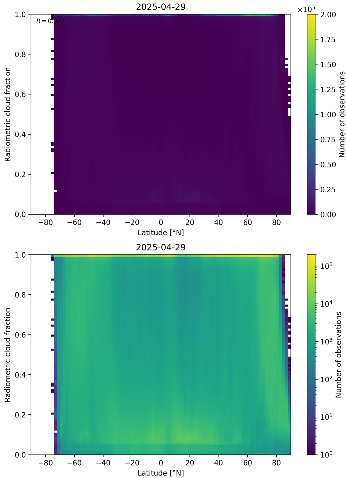
Figure 92: Scatter density plot of “Latitude” against “Radiometric cloud fraction” for 2025-04-29 to 2025-04-30.
