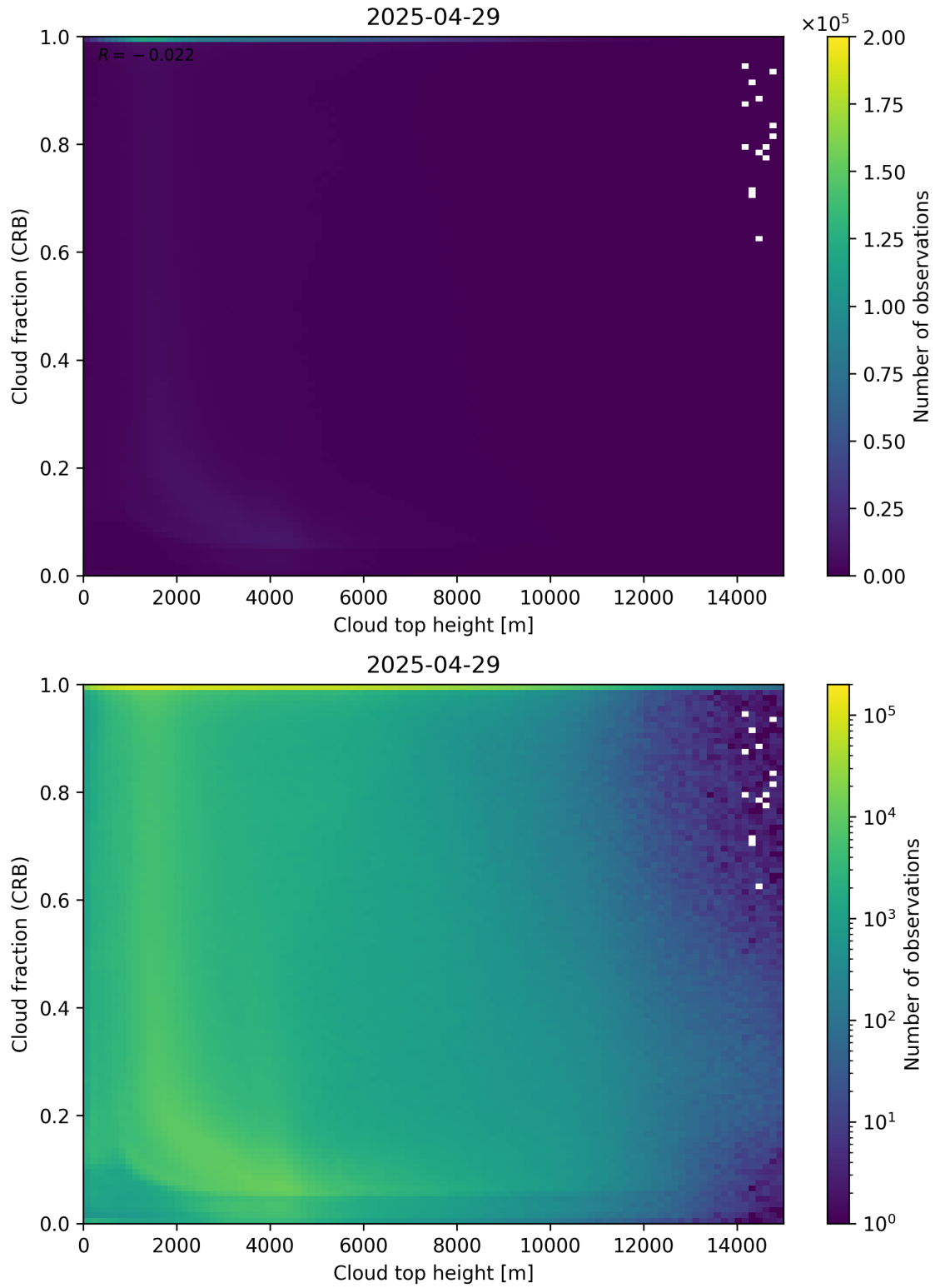
Figure 88: Scatter density plot of “Cloud top height” against “Cloud fraction (CRB)” for 2025-04-29 to 2025-04-30.
