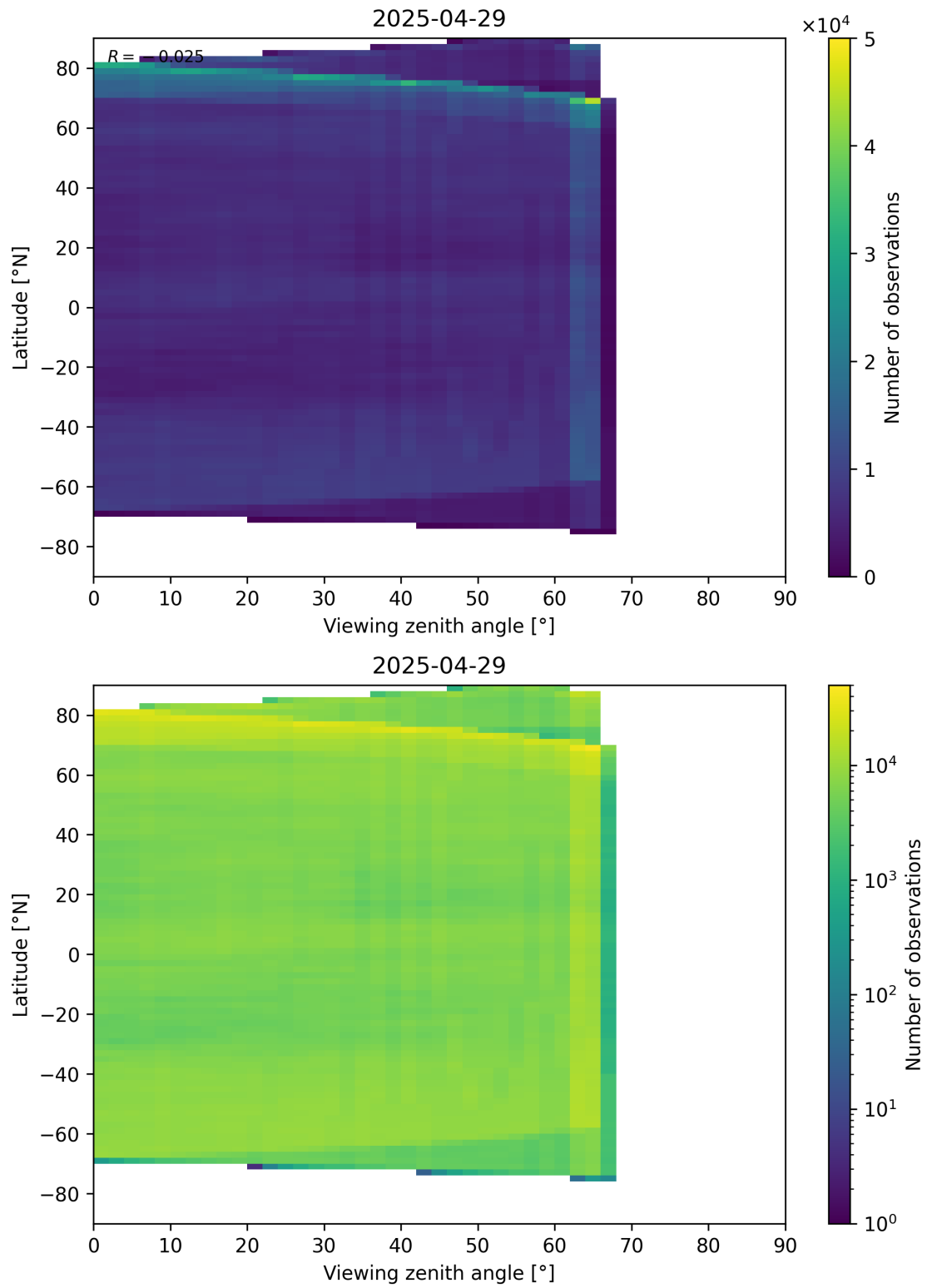
Figure 113: Scatter density plot of “Viewing zenith angle” against “Latitude” for 2025-04-29 to 2025-04-30.
