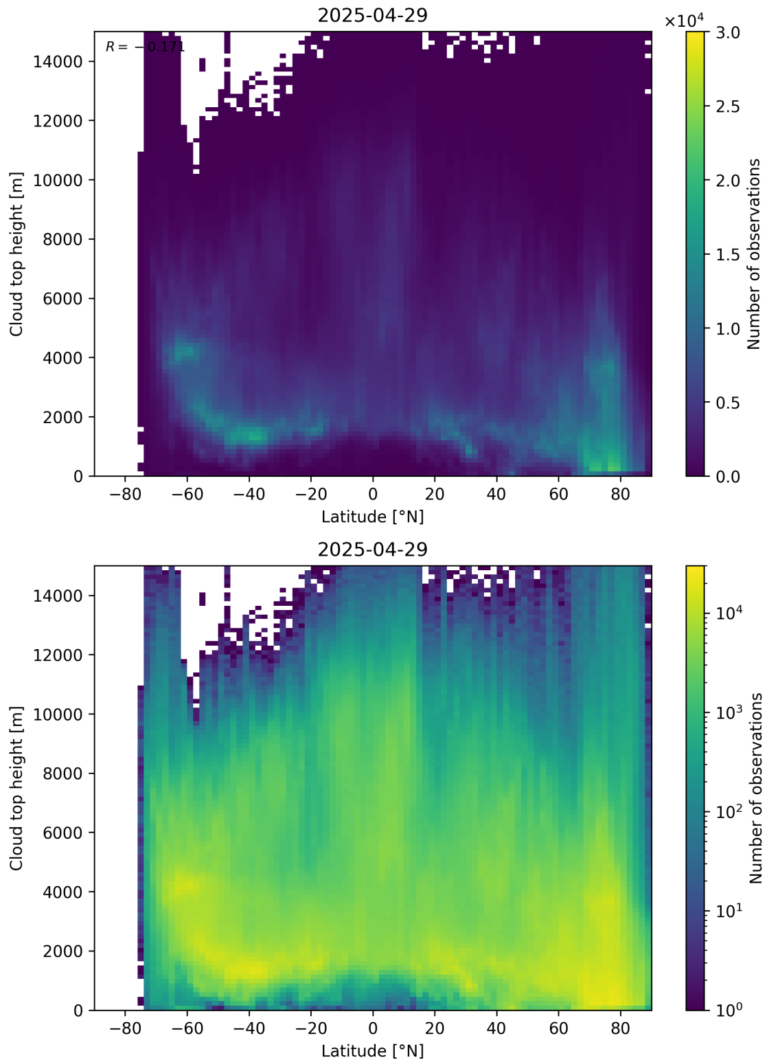
Figure 97: Scatter density plot of “Latitude” against “Cloud top height” for 2025-04-29 to 2025-04-30.
