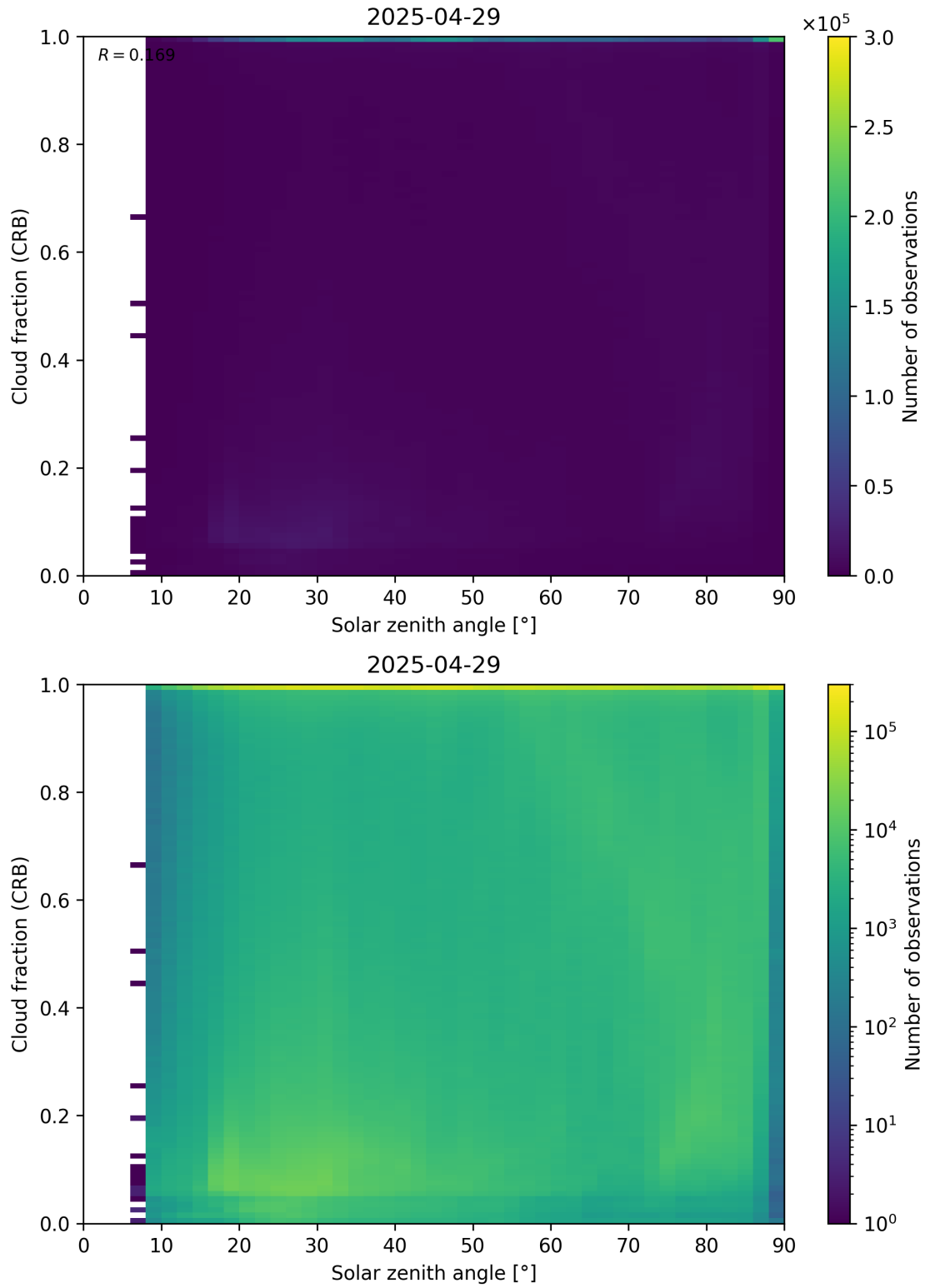
Figure 101: Scatter density plot of “Solar zenith angle” against “Cloud fraction (CRB)” for 2025-04-29 to 2025-04-30.
