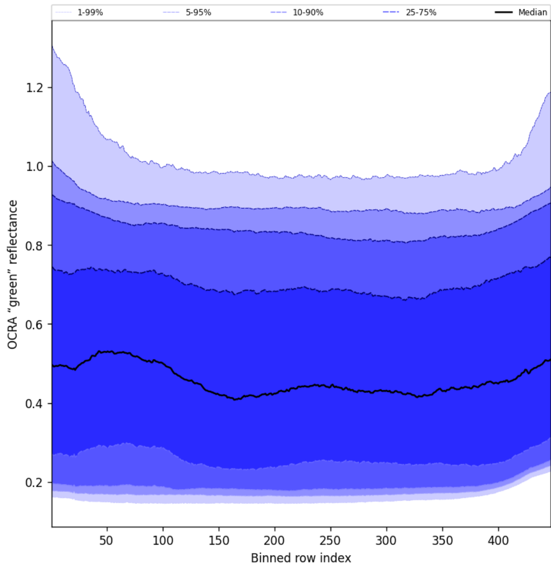
Figure 68: Along track statistics of “OCRA “green” reflectance” for 2025-04-29 to 2025-04-30
