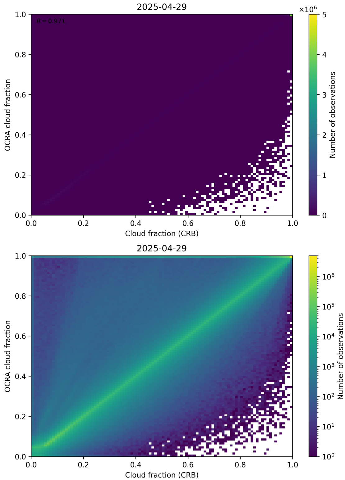
Figure 78: Scatter density plot of “Cloud fraction (CRB)” against “OCRA cloud fraction” for 2025-04-29 to 2025-04-30.
