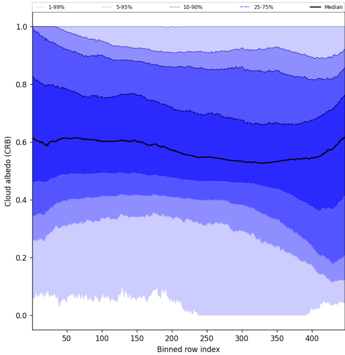
Figure 60: Along track statistics of “Cloud albedo (CRB)” for 2025-04-29 to 2025-04-30
