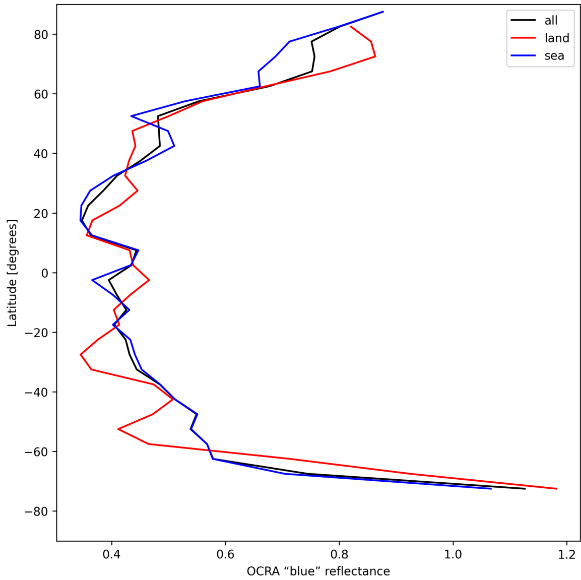
Figure 35: Zonal average of "OCRA "blue" reflectance" for 2025-04-29 to 2025-04-30.
