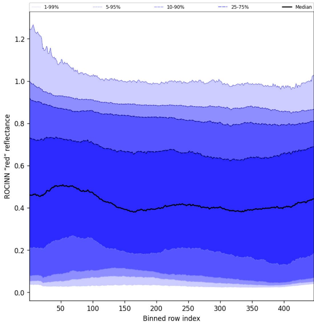
Figure 69: Along track statistics of “ROCINN “red” reflectance” for 2025-04-29 to 2025-04-30
