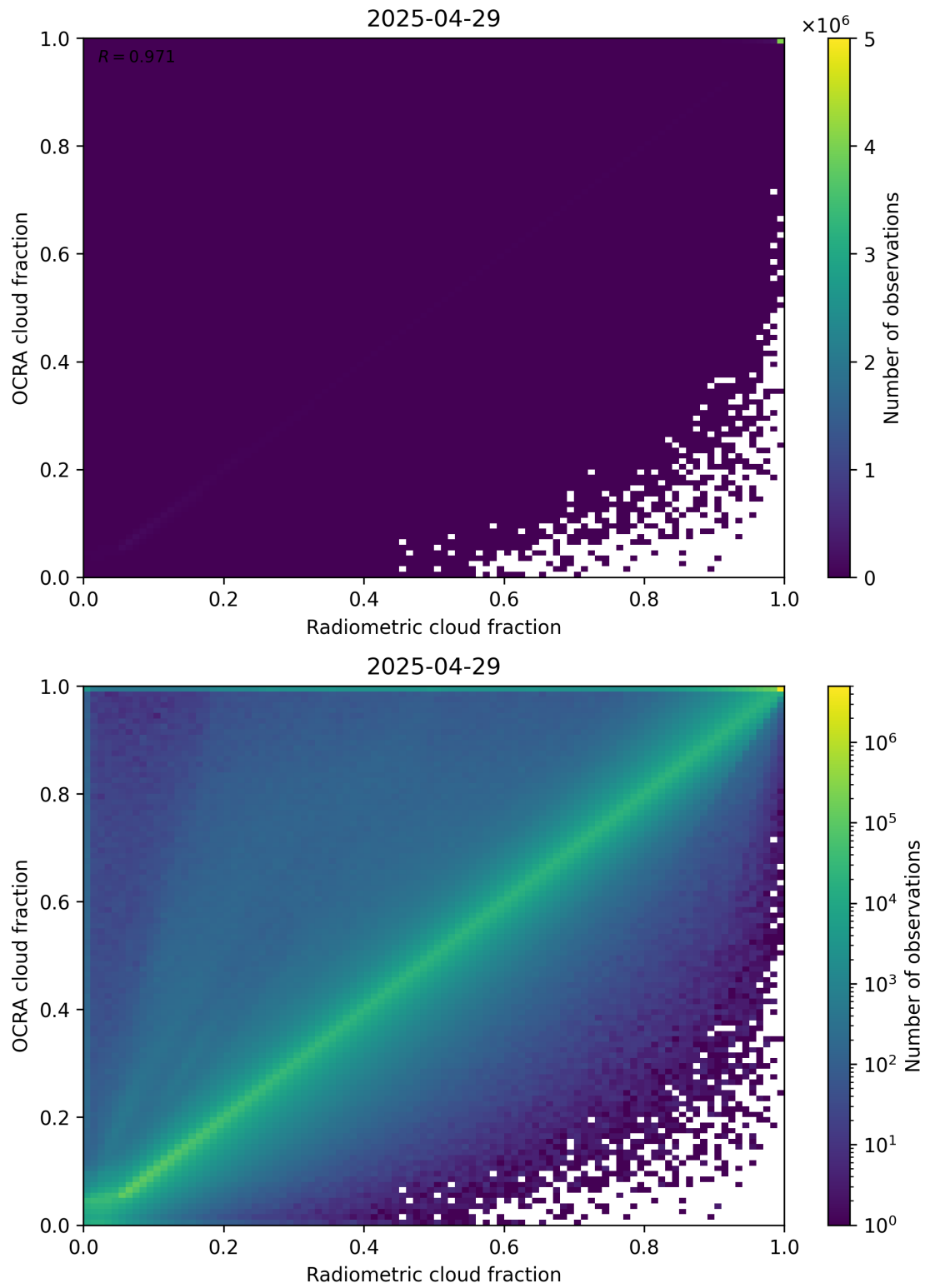
Figure 72: Scatter density plot of “Radiometric cloud fraction” against “OCRA cloud fraction” for 2025-04-29 to 2025-04-30.
