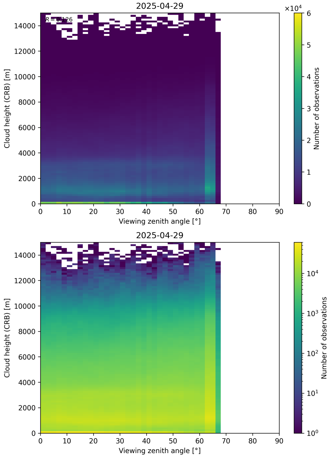
Figure 110: Scatter density plot of “Viewing zenith angle” against “Cloud height (CRB)” for 2025-04-29 to 2025-04-30.
