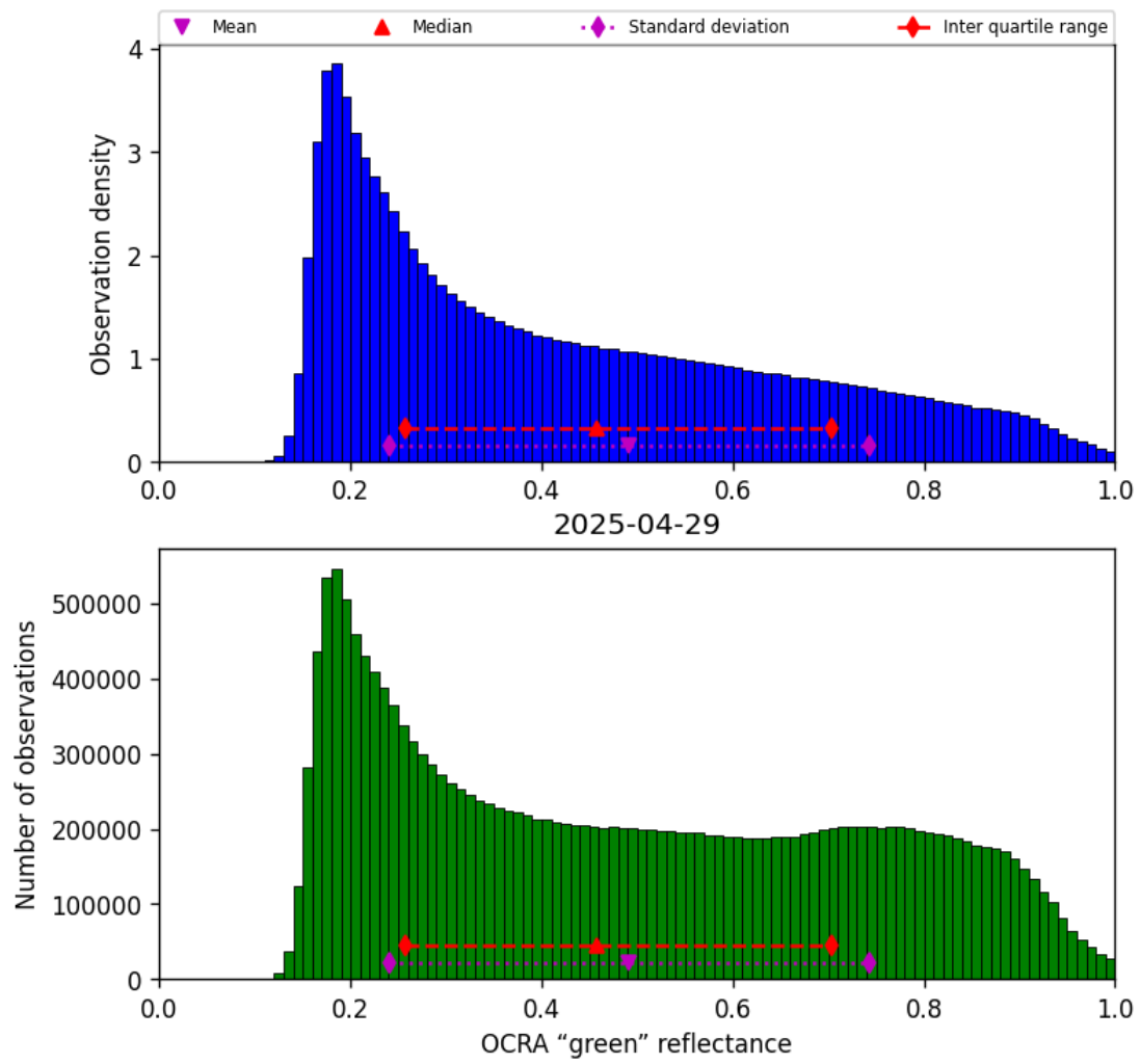
Figure 52: Histogram of “OCRA “green” reflectance” for 2025-04-29 to 2025-04-30
