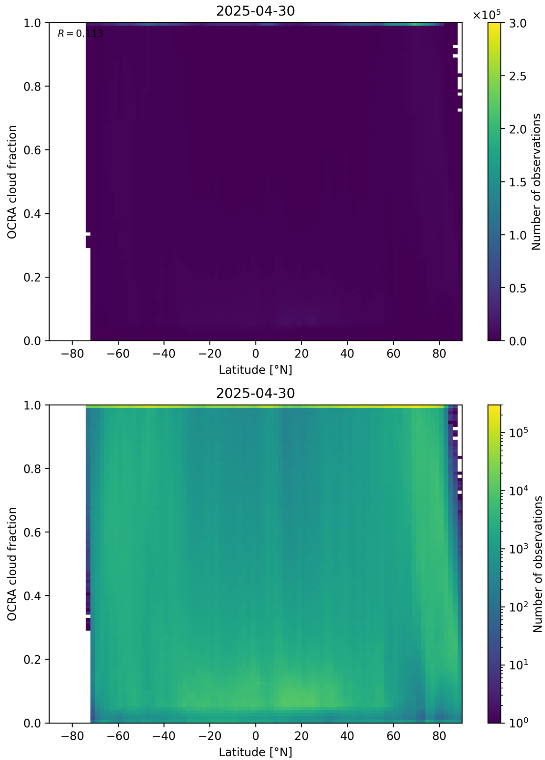
Figure 93: Scatter density plot of “Latitude” against “OCRA cloud fraction” for 2025-04-29 to 2025-05-01.
