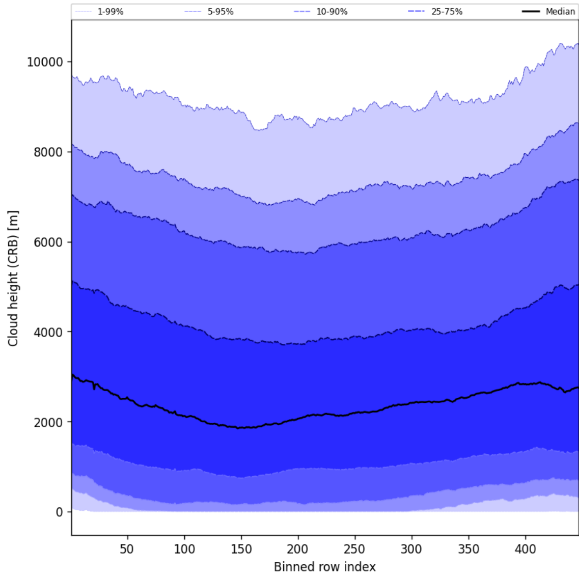
Figure 59: Along track statistics of “Cloud height (CRB)” for 2025-04-29 to 2025-05-01
