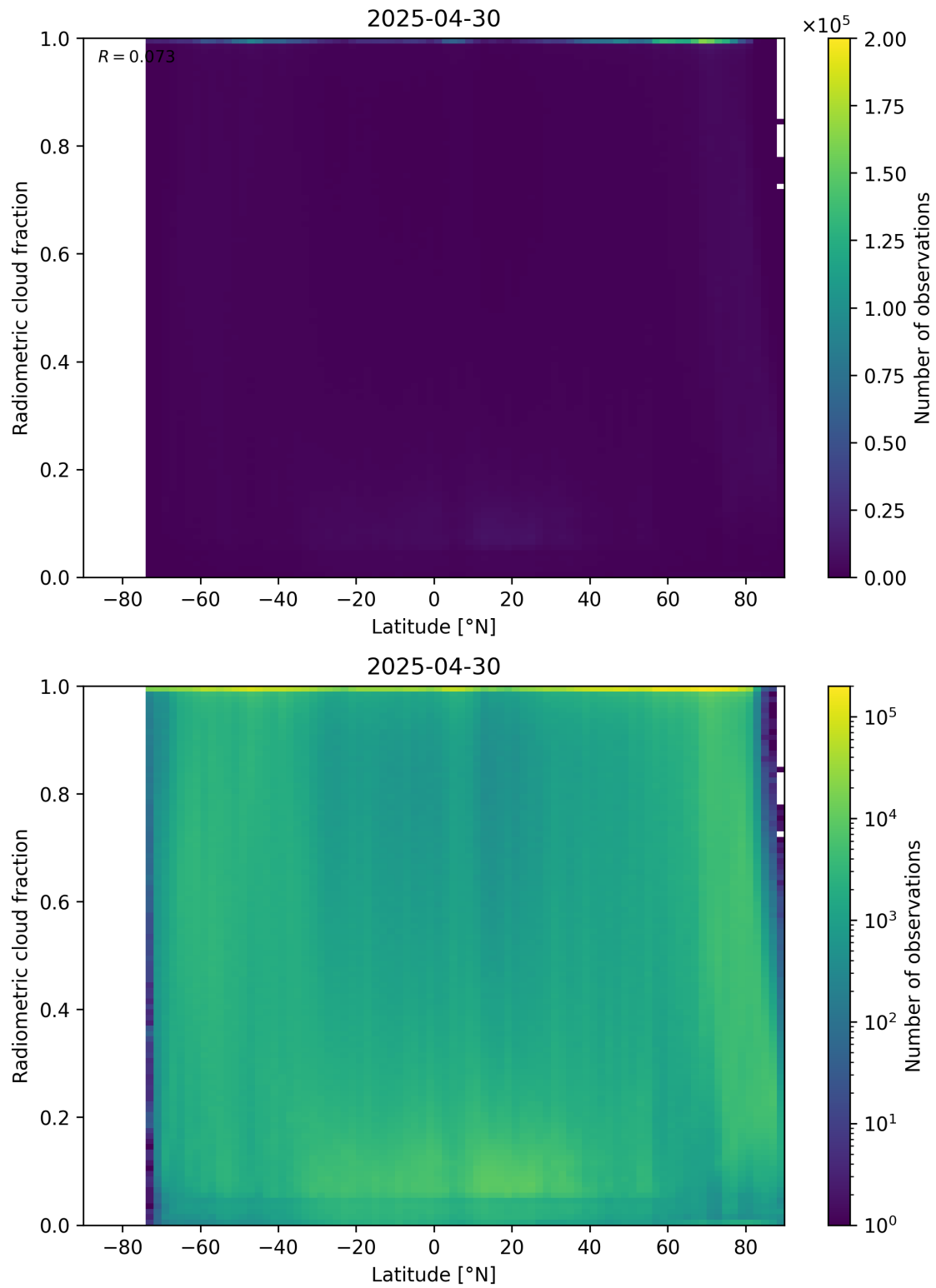
Figure 92: Scatter density plot of “Latitude” against “Radiometric cloud fraction” for 2025-04-29 to 2025-05-01.
