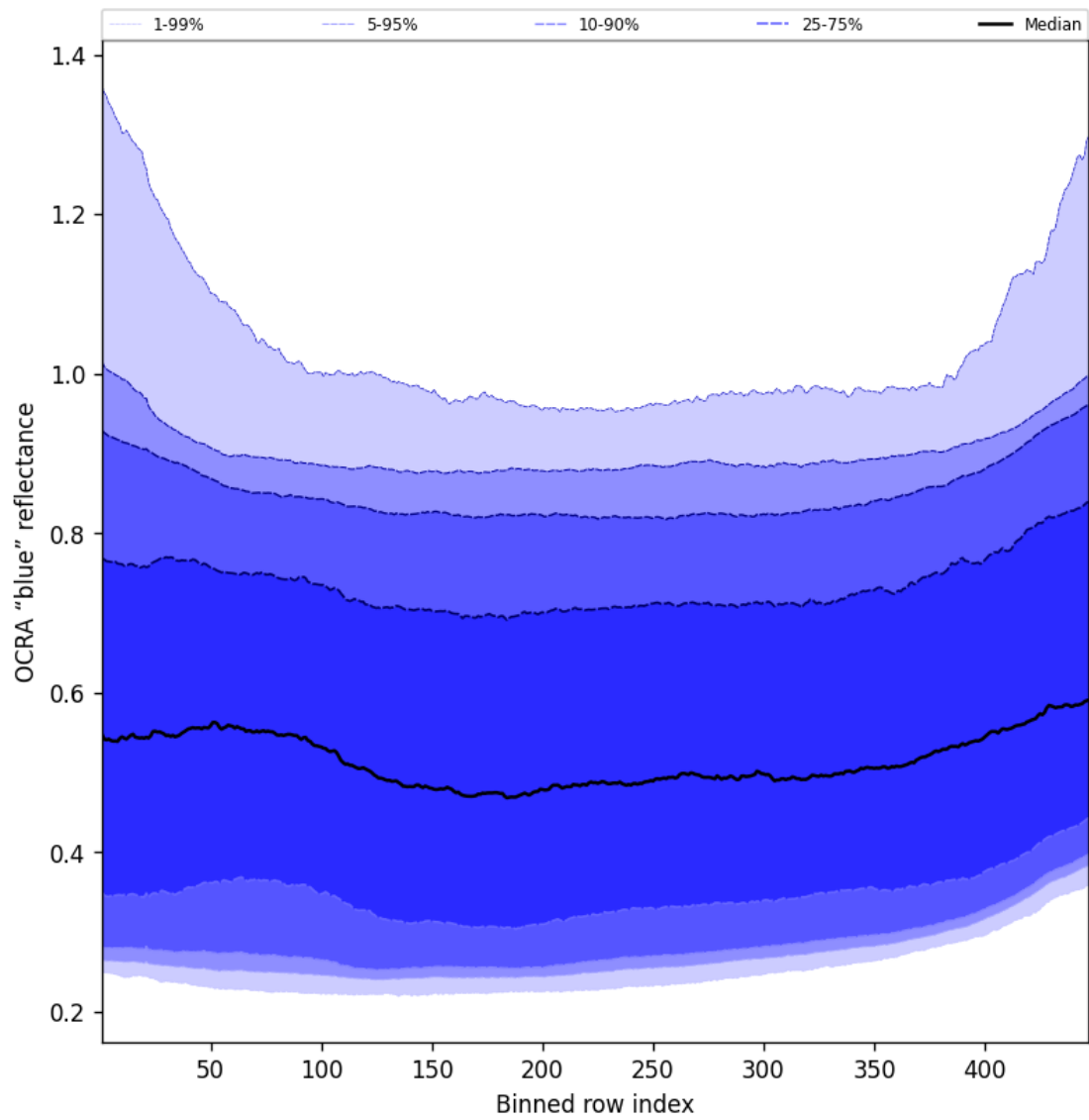
Figure 67: Along track statistics of “OCRA “blue” reflectance” for 2025-04-29 to 2025-05-01
