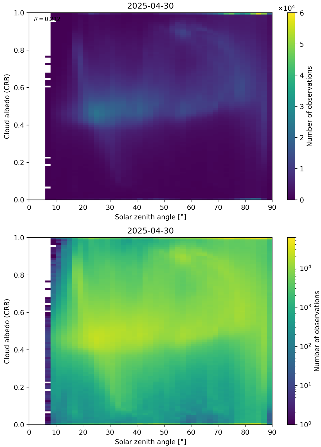
Figure 98: Scatter density plot of “Solar zenith angle” against “Cloud albedo (CRB)” for 2025-04-29 to 2025-05-01.
