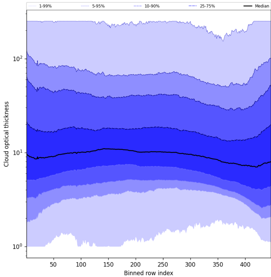
Figure 57: Along track statistics of “Cloud optical thickness” for 2025-04-29 to 2025-05-01
