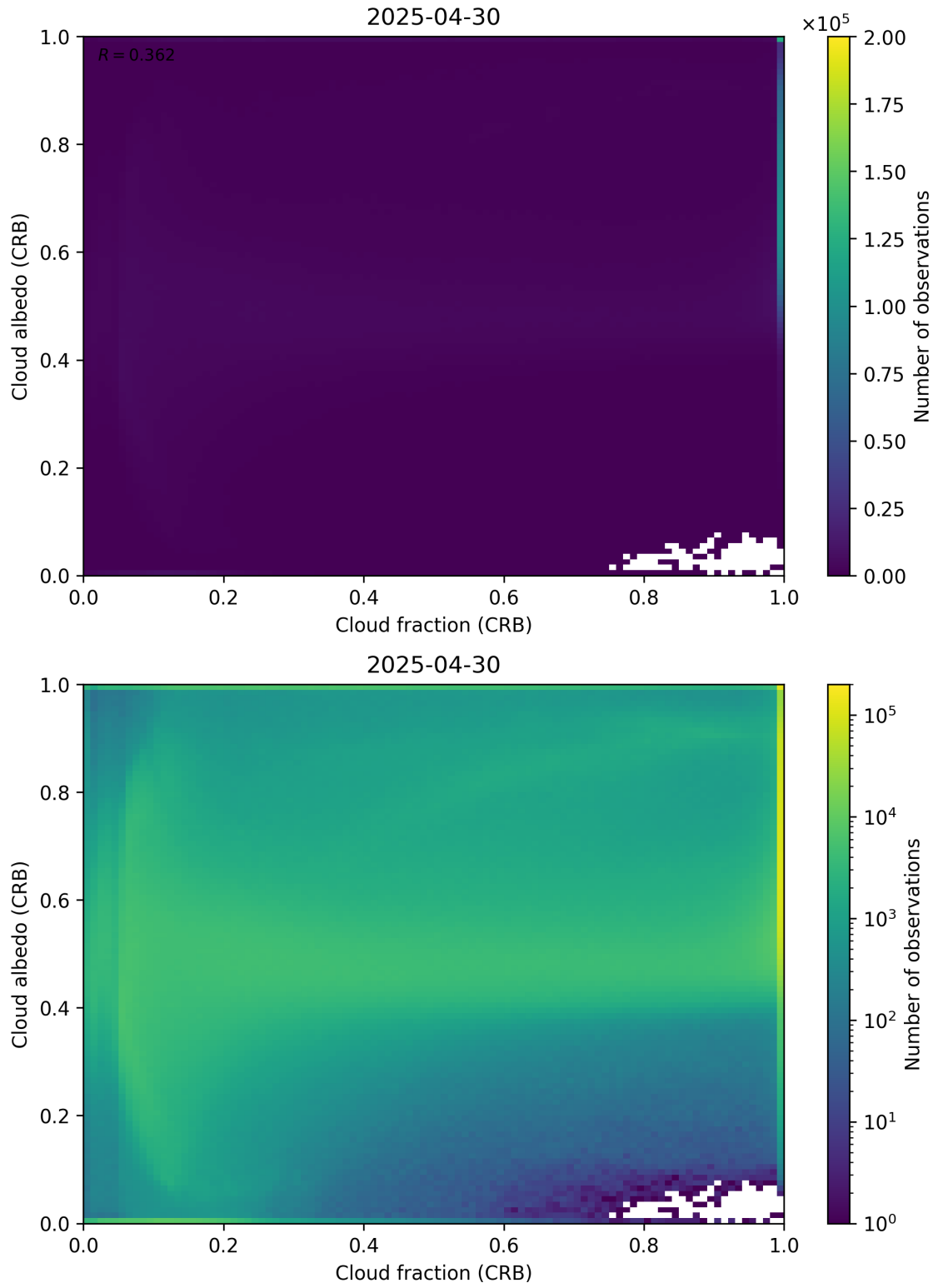
Figure 77: Scatter density plot of “Cloud fraction (CRB)” against “Cloud albedo (CRB)” for 2025-04-29 to 2025-05-01.
