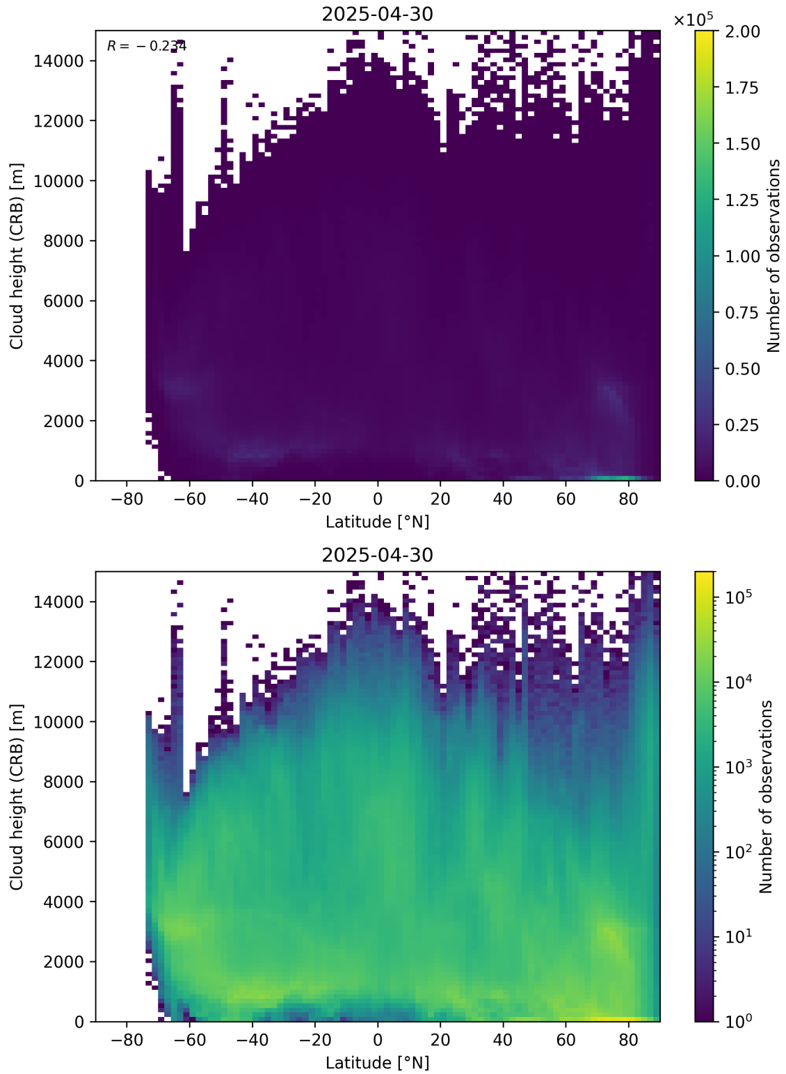
Figure 95: Scatter density plot of “Latitude” against “Cloud height (CRB)” for 2025-04-29 to 2025-05-01.
