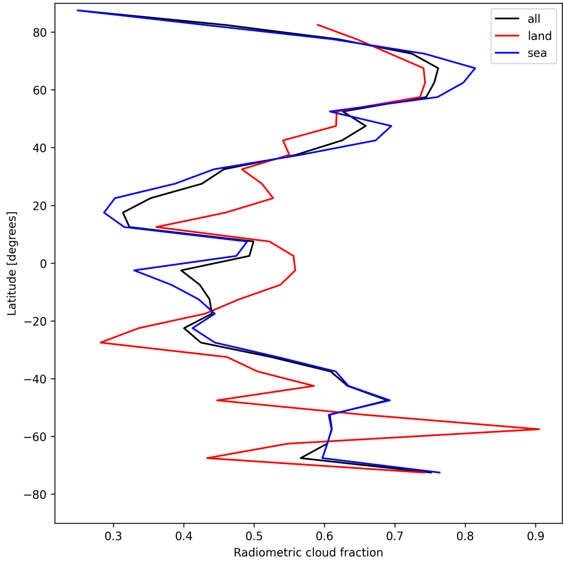
Figure 23: Zonal average of “Radiometric cloud fraction” for 2025-04-29 to 2025-05-01.
