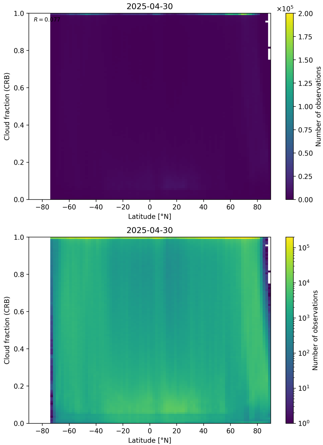
Figure 94: Scatter density plot of “Latitude” against “Cloud fraction (CRB)” for 2025-04-29 to 2025-05-01.
