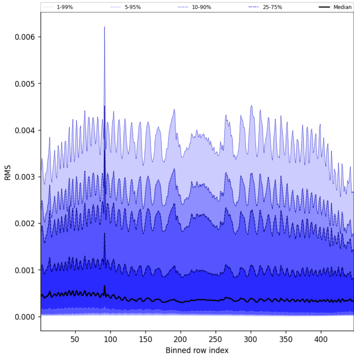
Figure 63: Along track statistics of “RMS” for 2025-04-29 to 2025-05-01
