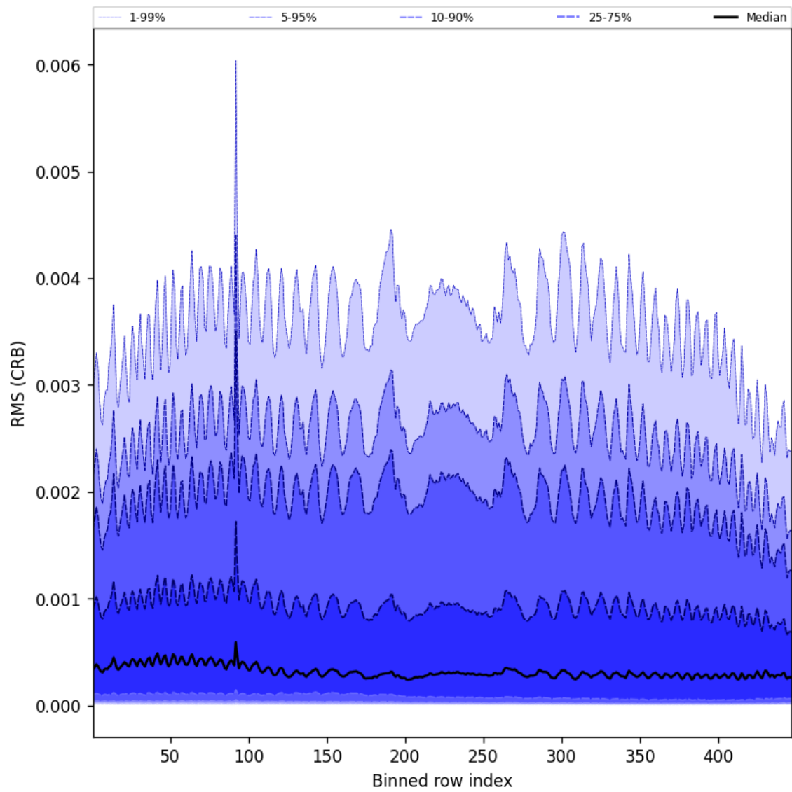
Figure 64: Along track statistics of “RMS (CRB)” for 2025-04-29 to 2025-05-01
