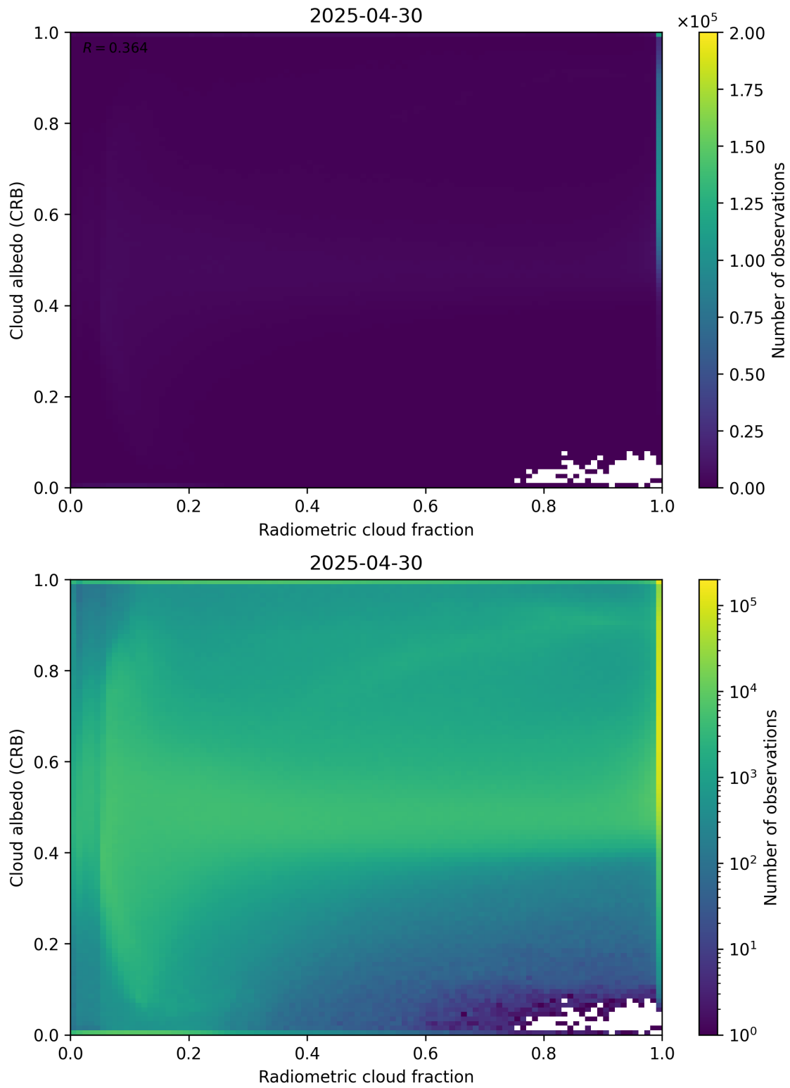
Figure 71: Scatter density plot of “Radiometric cloud fraction” against “Cloud albedo (CRB)” for 2025-04-29 to 2025-05-01.
