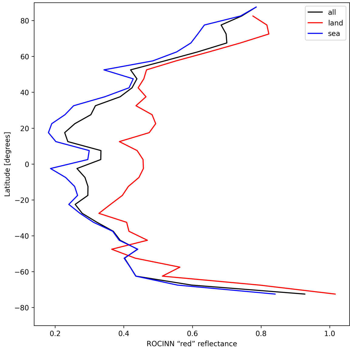
Figure 37: Zonal average of “ROCINN “red” reflectance” for 2025-04-29 to 2025-05-01.
