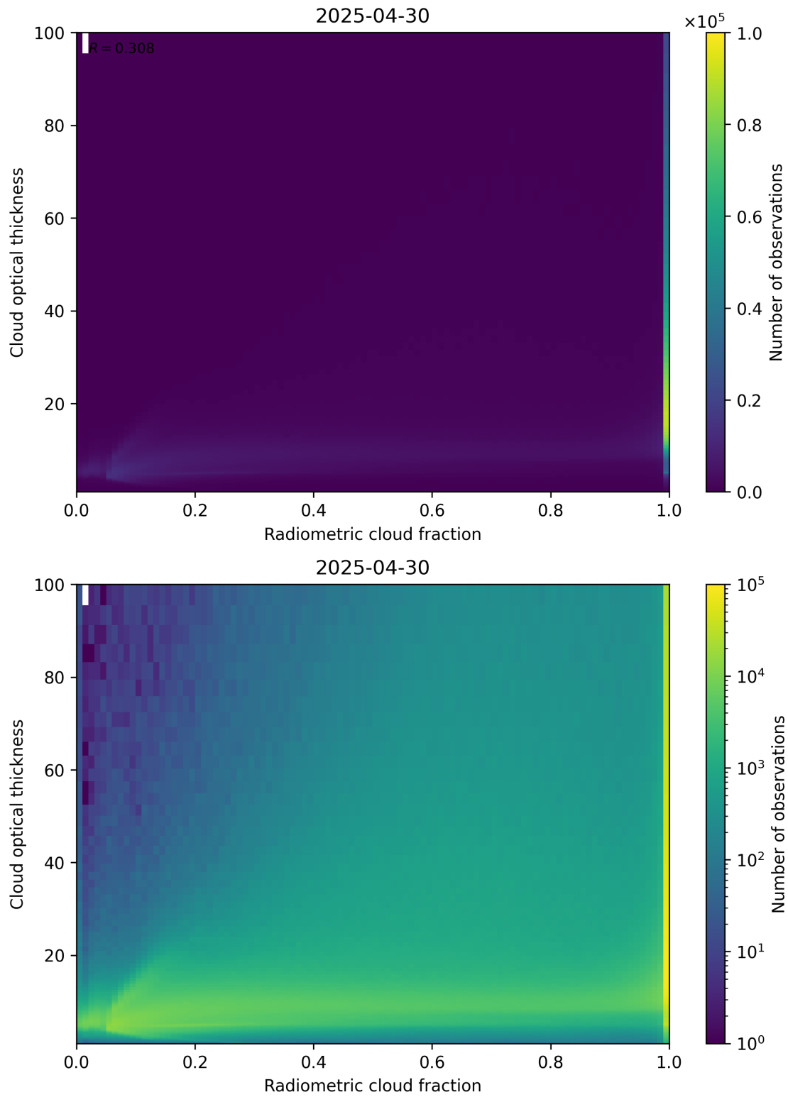
Figure 75: Scatter density plot of “Radiometric cloud fraction” against “Cloud optical thickness” for 2025-04-29 to 2025-05-01.
