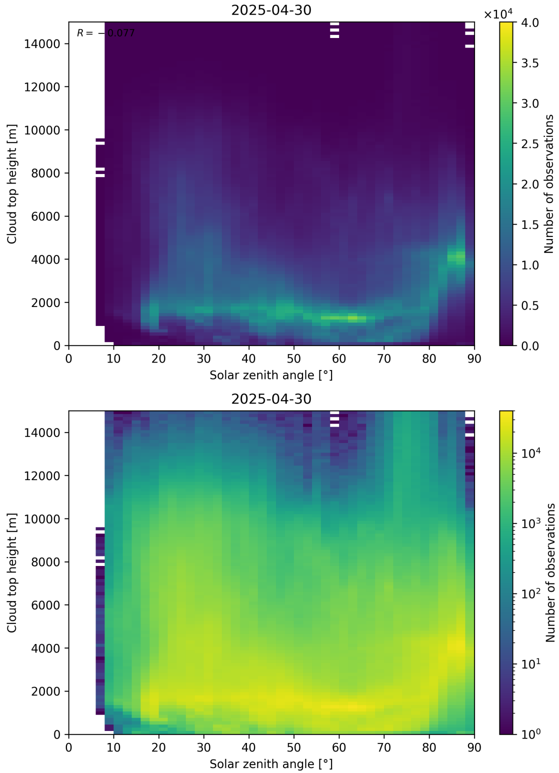
Figure 104: Scatter density plot of “Solar zenith angle” against “Cloud top height” for 2025-04-29 to 2025-05-01.
