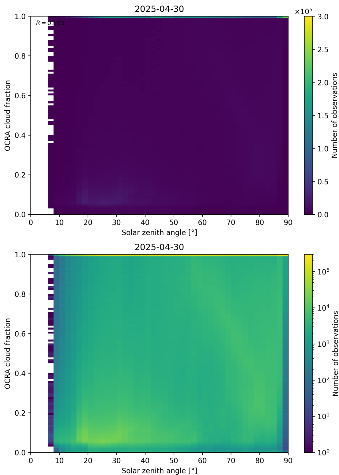
Figure 100: Scatter density plot of “Solar zenith angle” against “OCRA cloud fraction” for 2025-04-29 to 2025-05-01.
