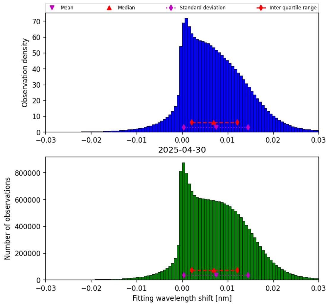
Figure 49: Histogram of “Fitting wavelength shift” for 2025-04-29 to 2025-05-01
