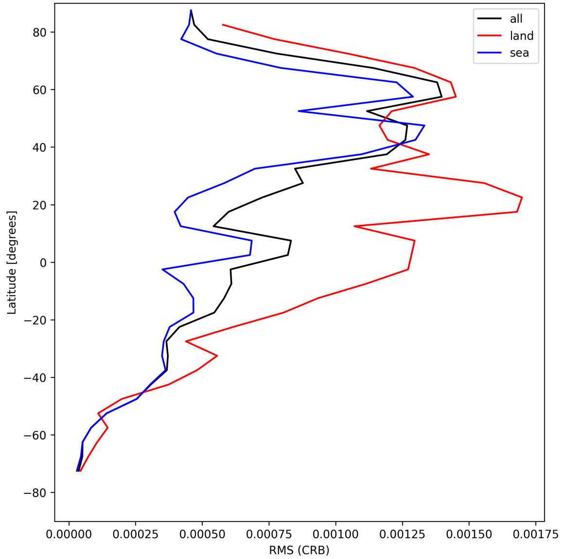
Figure 32: Zonal average of “RMS (CRB)” for 2025-04-29 to 2025-05-01.
