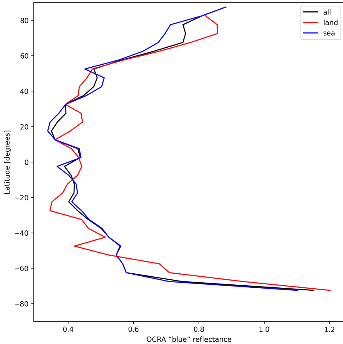
Figure 35: Zonal average of “OCRA “blue” reflectance” for 2025-04-29 to 2025-05-01.
