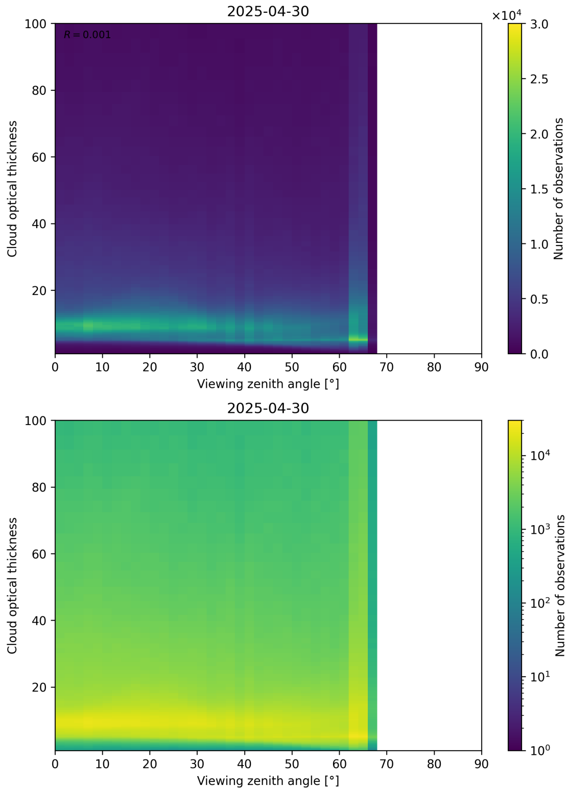
Figure 111: Scatter density plot of “Viewing zenith angle” against “Cloud optical thickness” for 2025-04-29 to 2025-05-01.
