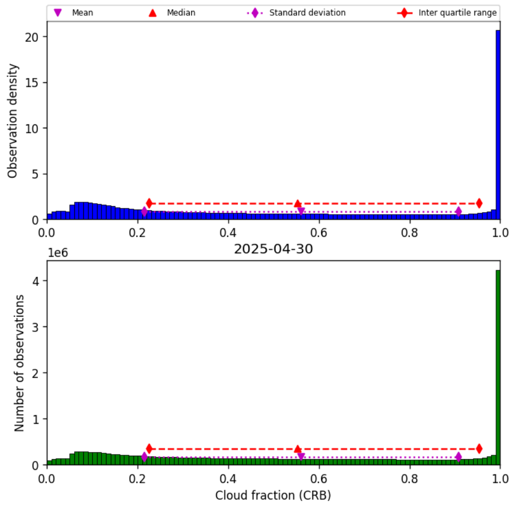
Figure 42: Histogram of “Cloud fraction (CRB)” for 2025-04-29 to 2025-05-01
