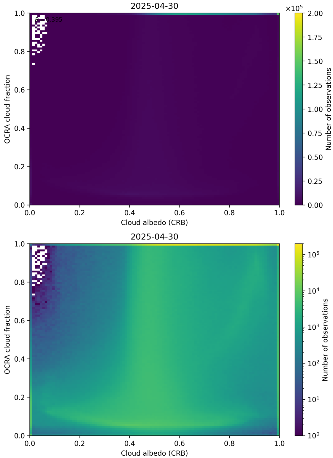
Figure 70: Scatter density plot of “Cloud albedo (CRB)” against “OCRA cloud fraction” for 2025-04-29 to 2025-05-01.
