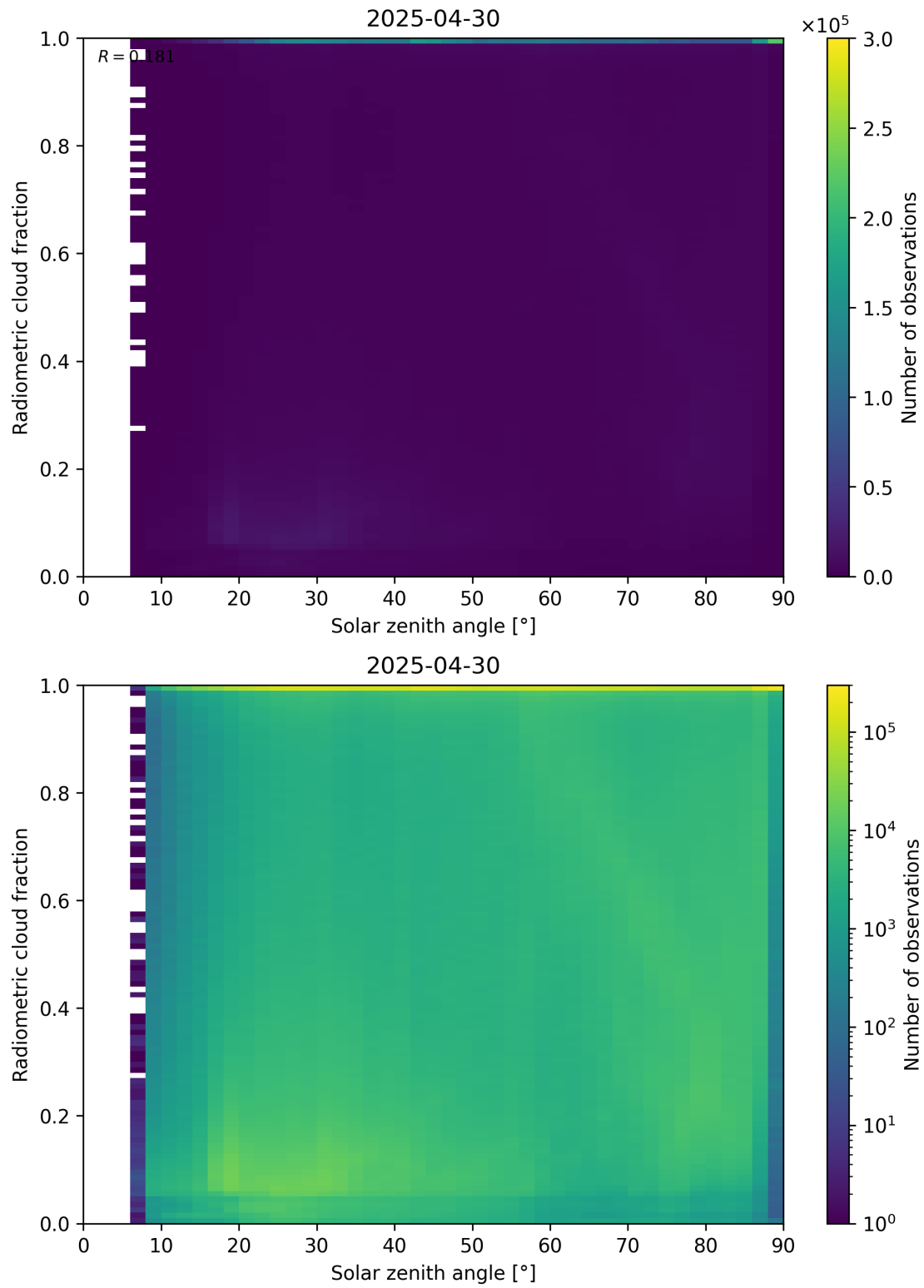
Figure 99: Scatter density plot of “Solar zenith angle” against “Radiometric cloud fraction” for 2025-04-29 to 2025-05-01.
