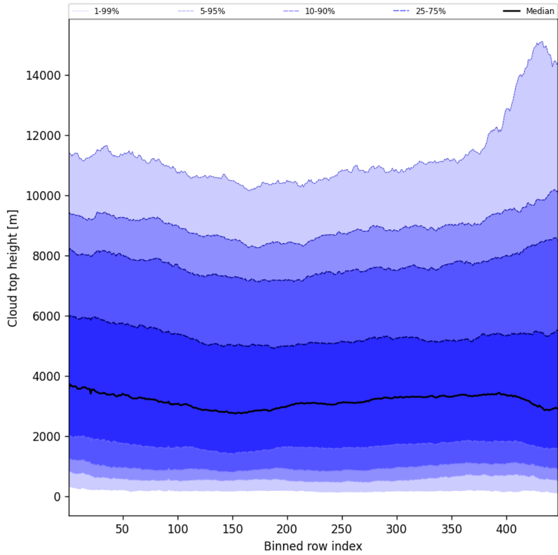
Figure 56: Along track statistics of “Cloud top height” for 2025-04-29 to 2025-05-01
