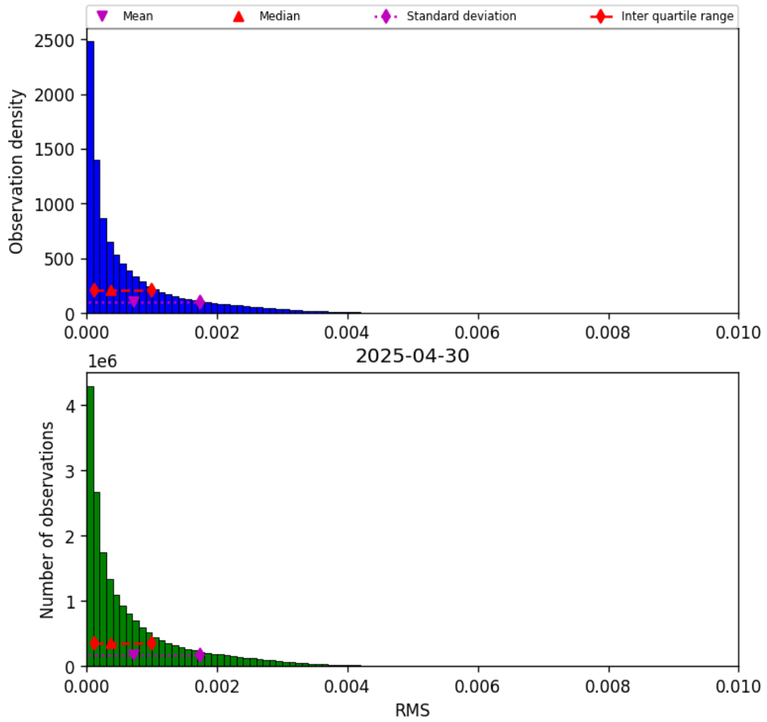
Figure 47: Histogram of “RMS” for 2025-04-29 to 2025-05-01
