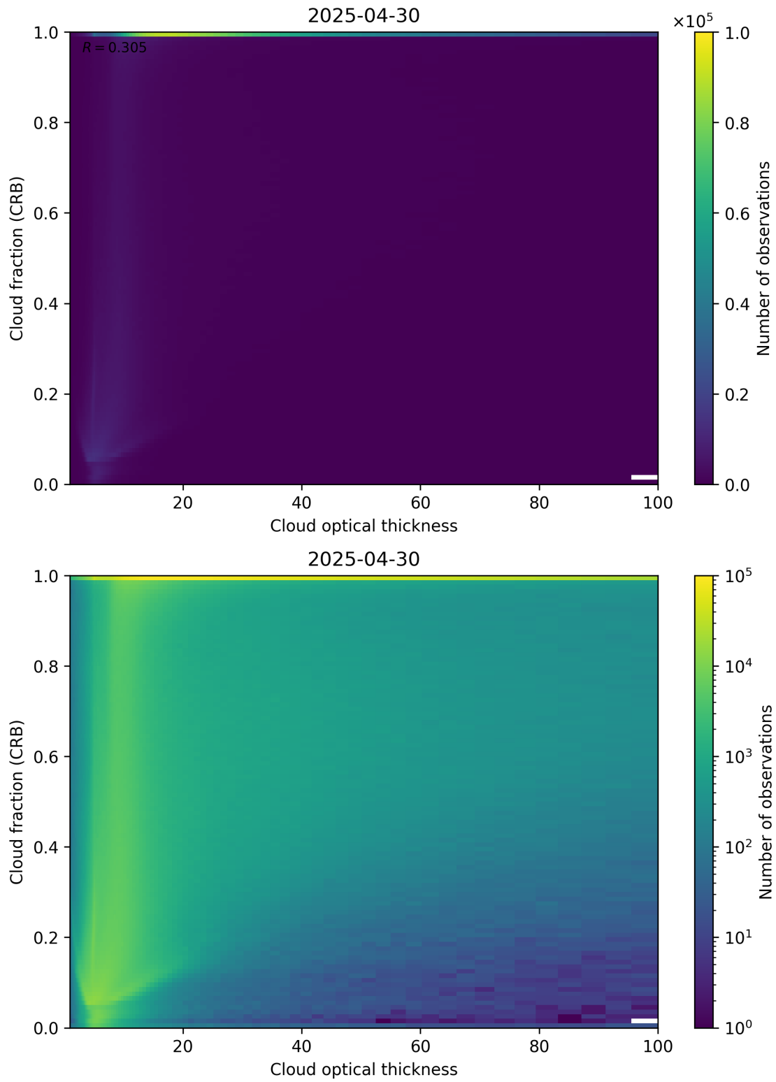
Figure 84: Scatter density plot of “Cloud optical thickness” against “Cloud fraction (CRB)” for 2025-04-29 to 2025-05-01.
