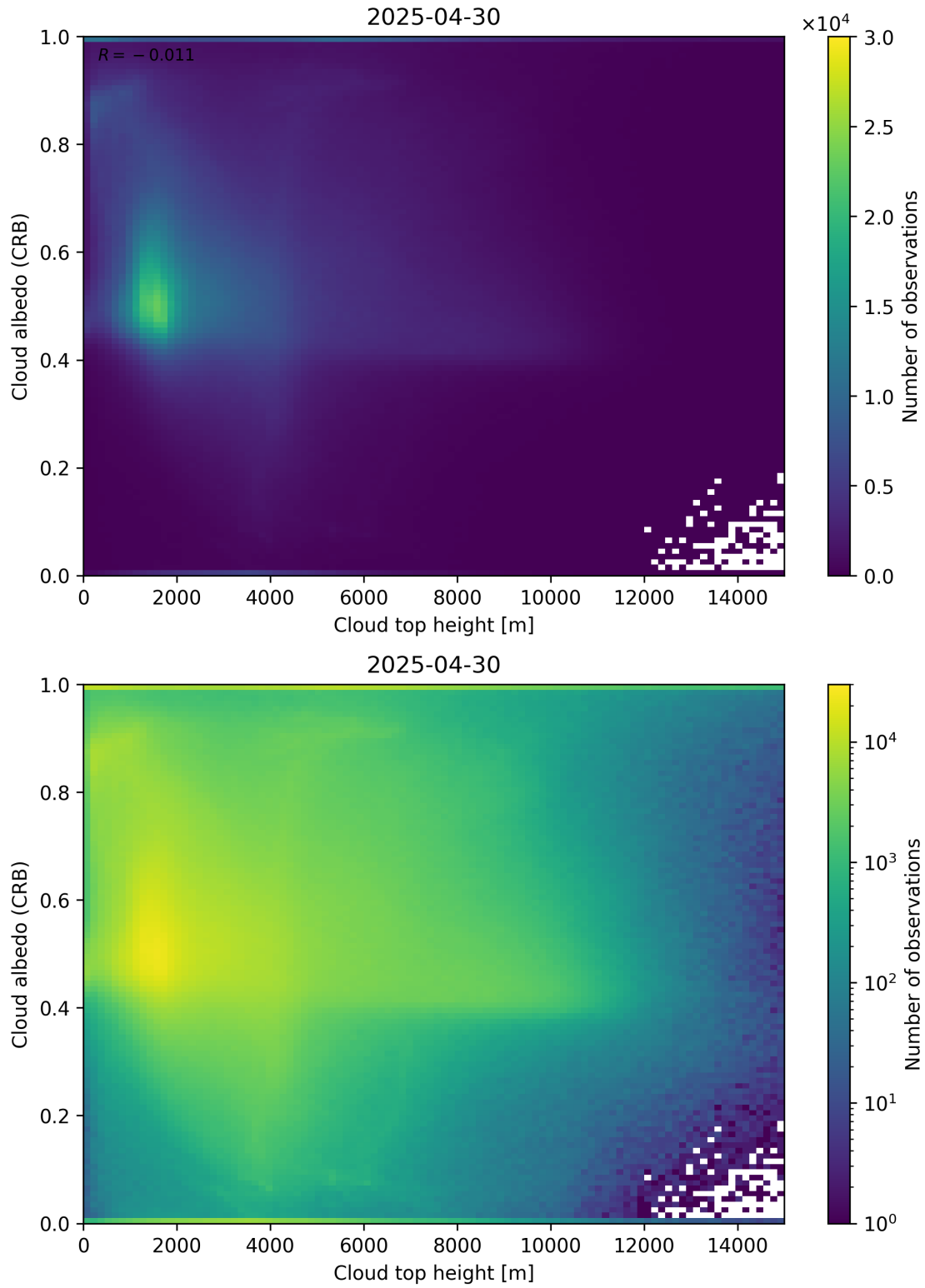
Figure 86: Scatter density plot of “Cloud top height” against “Cloud albedo (CRB)” for 2025-04-29 to 2025-05-01.
