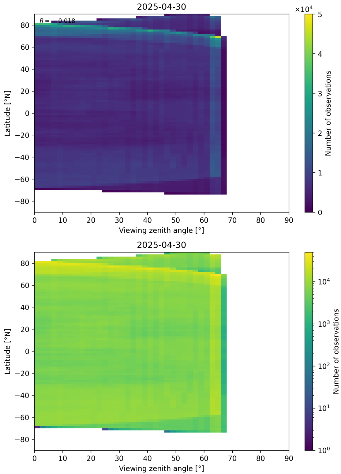
Figure 113: Scatter density plot of “Viewing zenith angle” against “Latitude” for 2025-04-29 to 2025-05-01.
