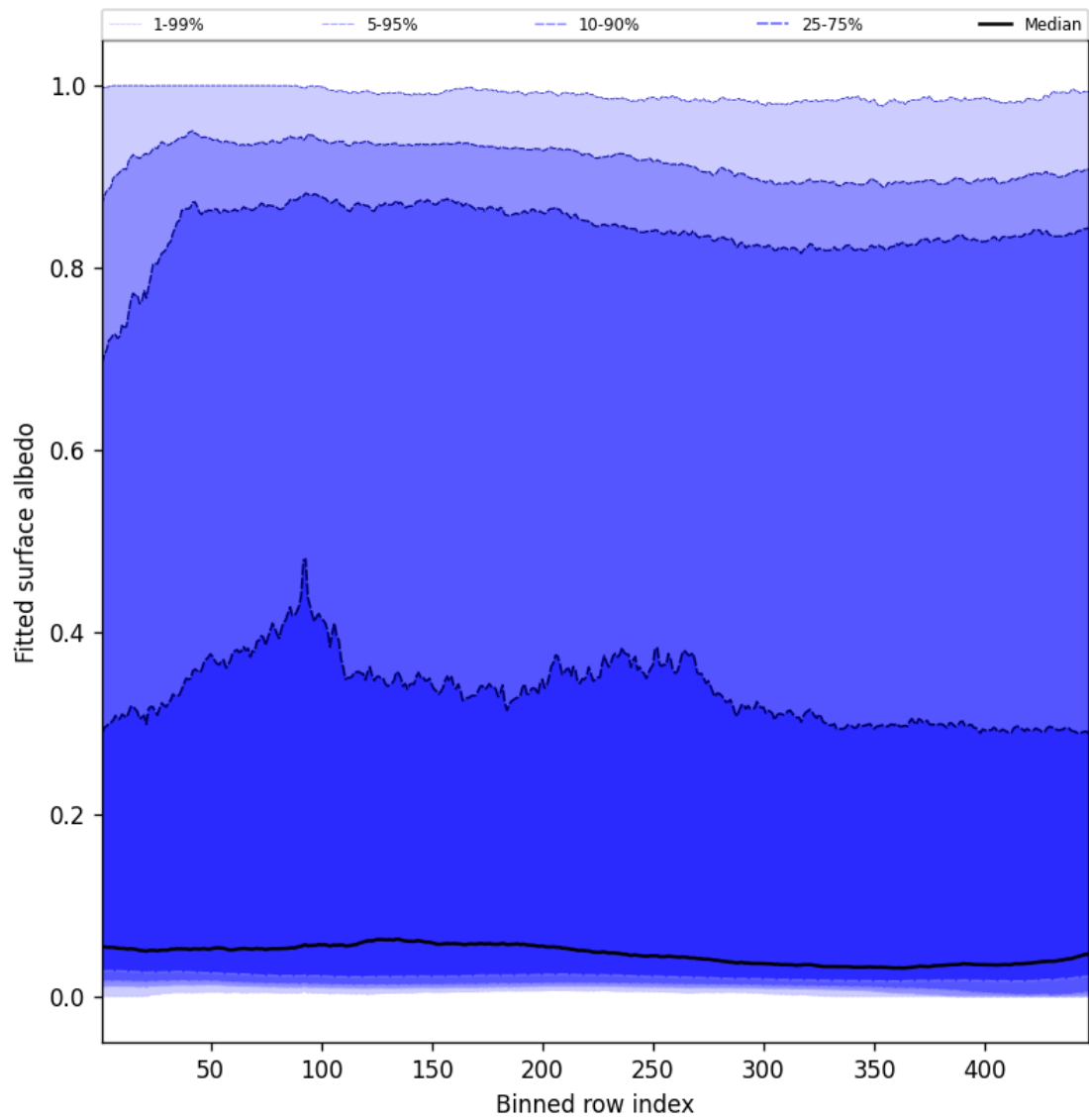
Figure 61: Along track statistics of “Fitted surface albedo” for 2025-04-29 to 2025-05-01
