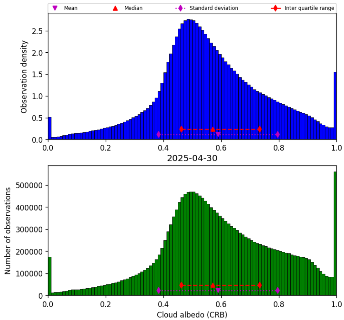
Figure 44: Histogram of “Cloud albedo (CRB)” for 2025-04-29 to 2025-05-01
