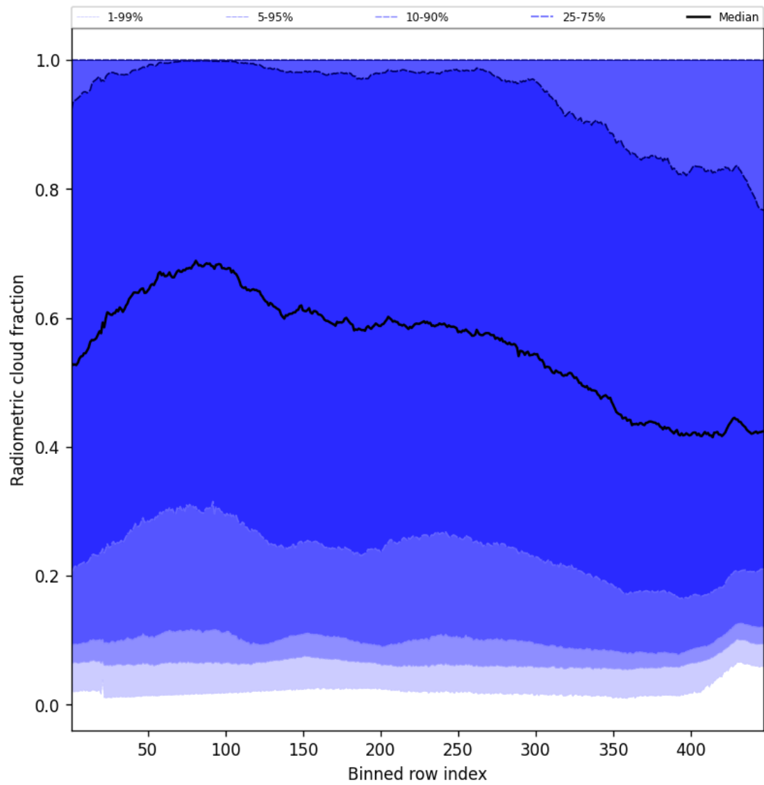
Figure 55: Along track statistics of “Radiometric cloud fraction” for 2025-04-29 to 2025-05-01
