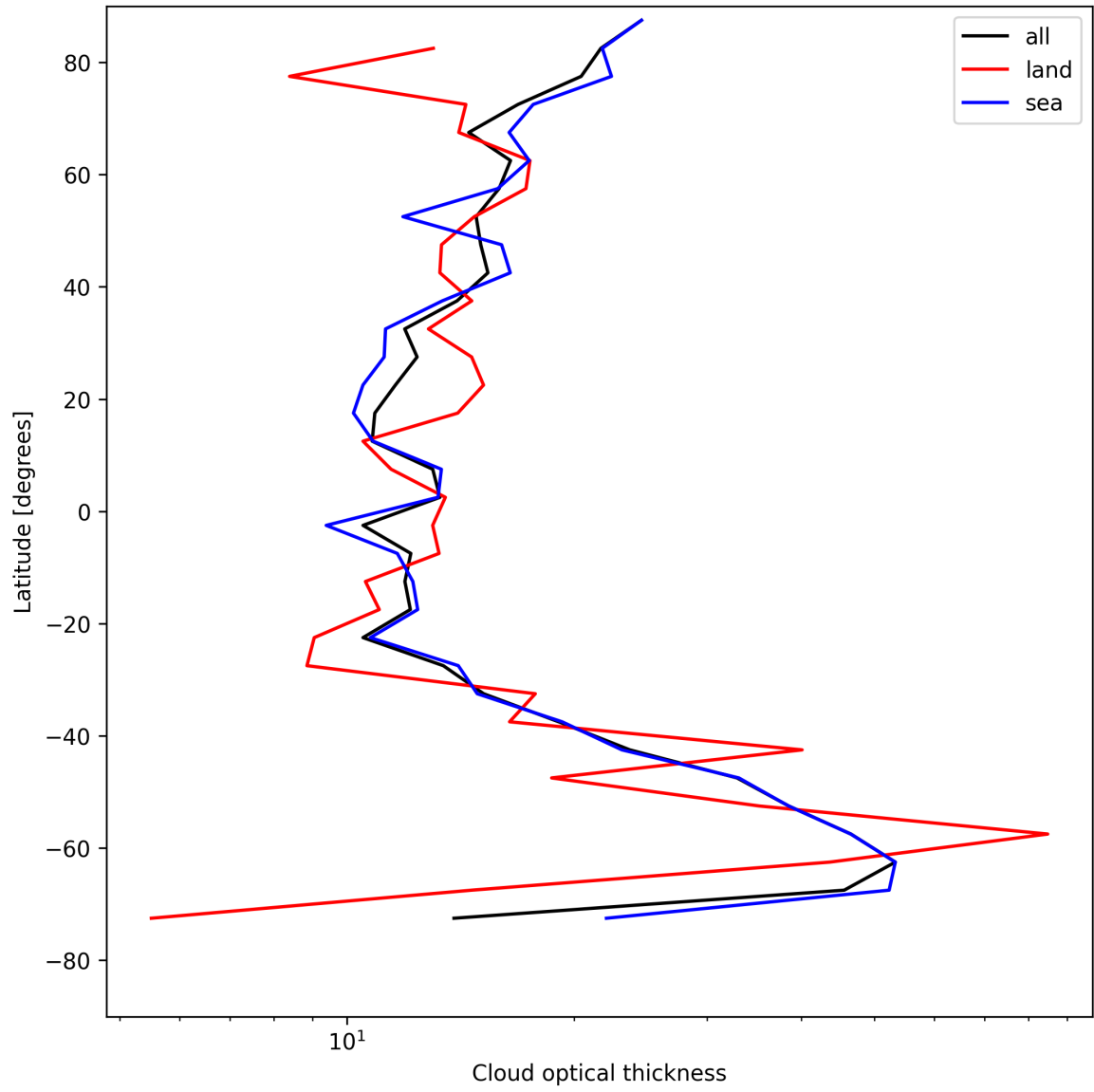
Figure 25: Zonal average of “Cloud optical thickness” for 2025-04-29 to 2025-05-01.
