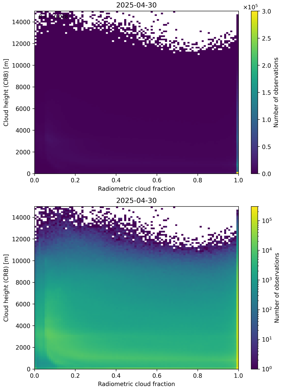
Figure 74: Scatter density plot of “Radiometric cloud fraction” against “Cloud height (CRB)” for 2025-04-29 to 2025-05-01.
