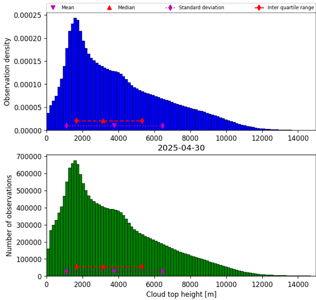
Figure 40: Histogram of “Cloud top height” for 2025-04-29 to 2025-05-01
