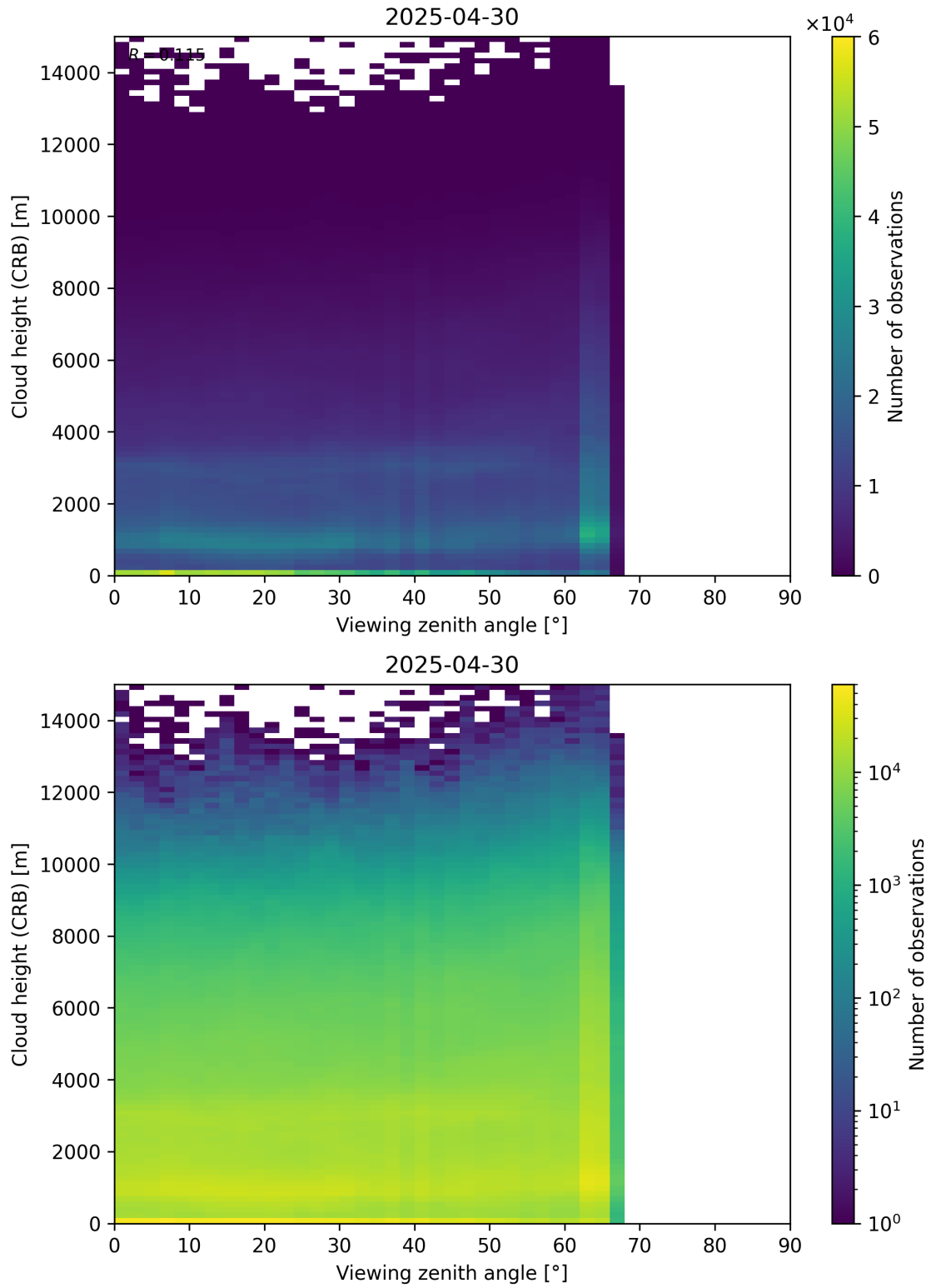
Figure 110: Scatter density plot of “Viewing zenith angle” against “Cloud height (CRB)” for 2025-04-29 to 2025-05-01.
