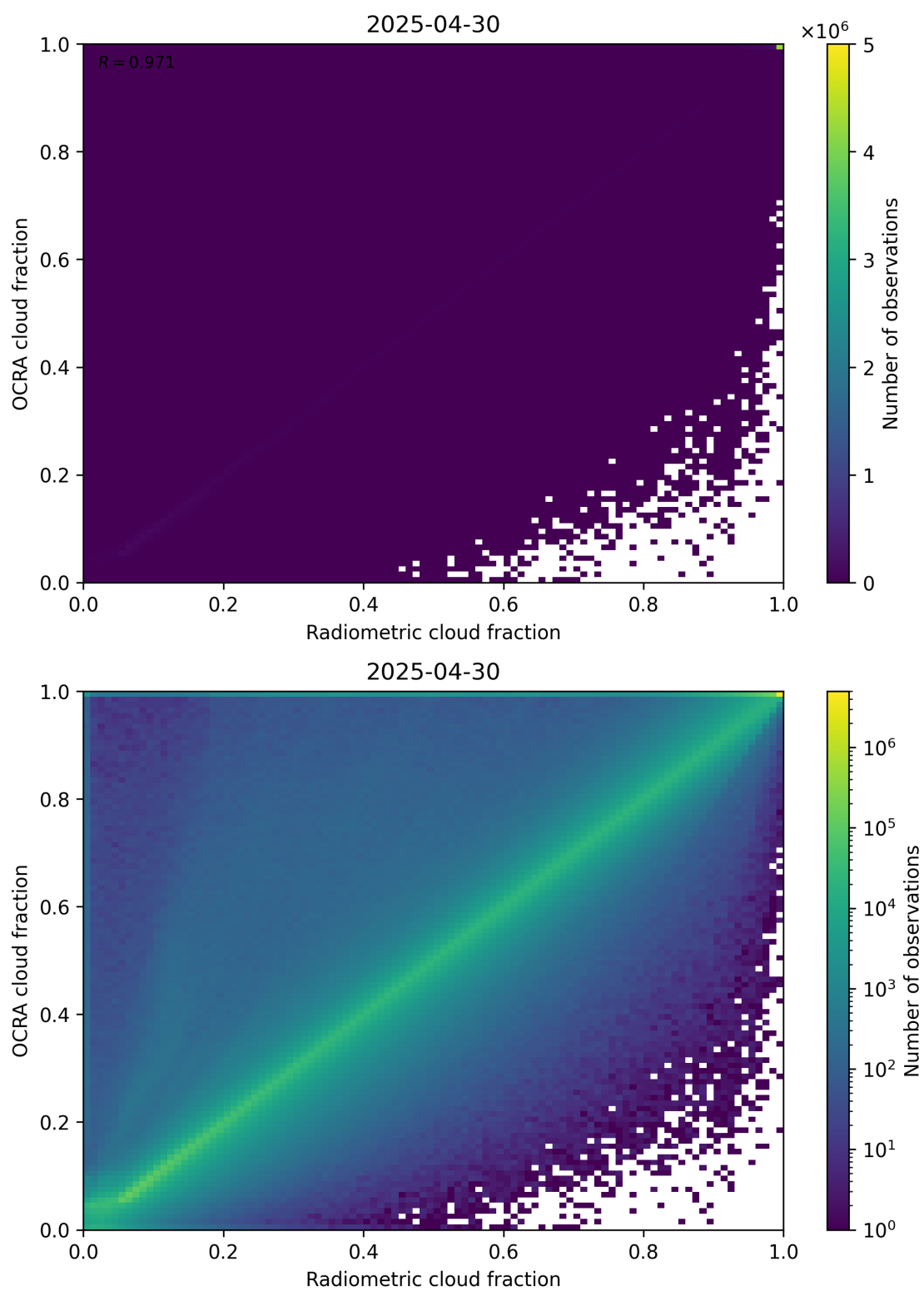
Figure 72: Scatter density plot of “Radiometric cloud fraction” against “OCRA cloud fraction” for 2025-04-29 to 2025-05-01.
