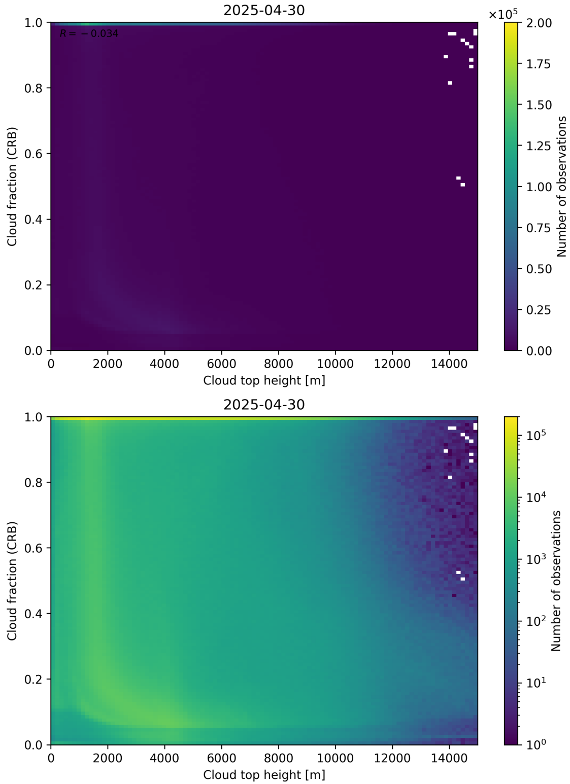
Figure 88: Scatter density plot of “Cloud top height” against “Cloud fraction (CRB)” for 2025-04-29 to 2025-05-01.
