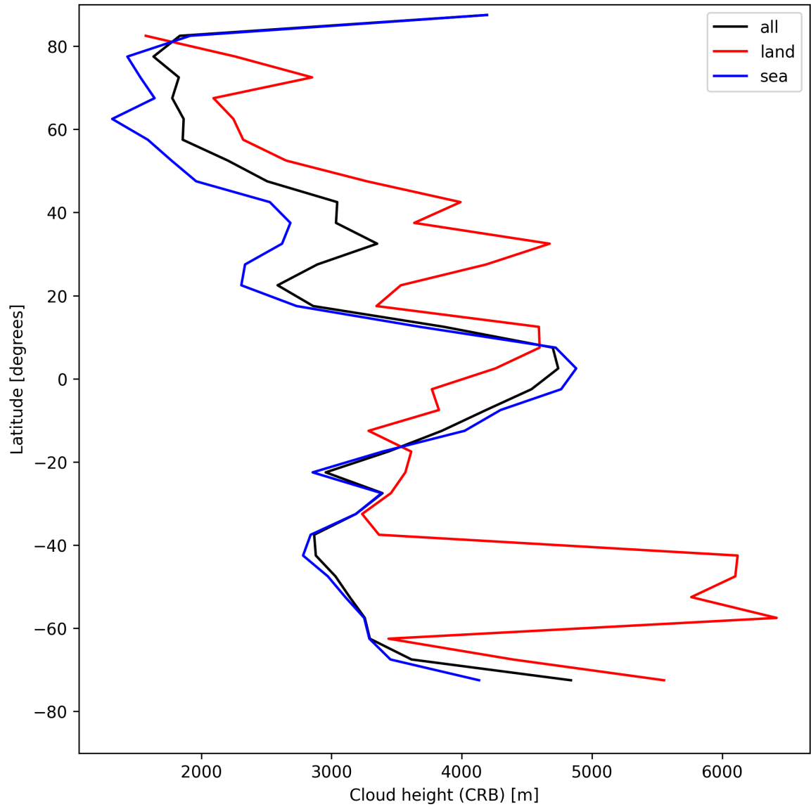
Figure 27: Zonal average of “Cloud height (CRB)” for 2025-04-29 to 2025-05-01.
