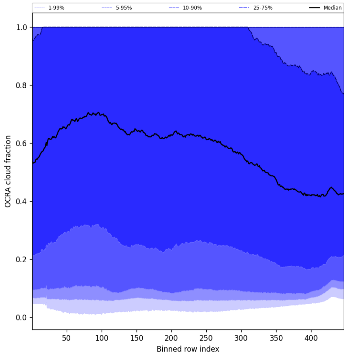
Figure 66: Along track statistics of “OCRA cloud fraction” for 2025-04-29 to 2025-05-01
