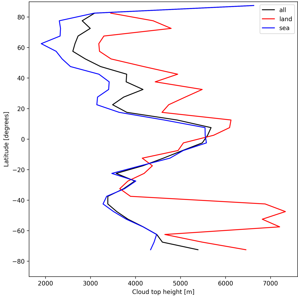
Figure 24: Zonal average of “Cloud top height” for 2025-04-29 to 2025-05-01.
