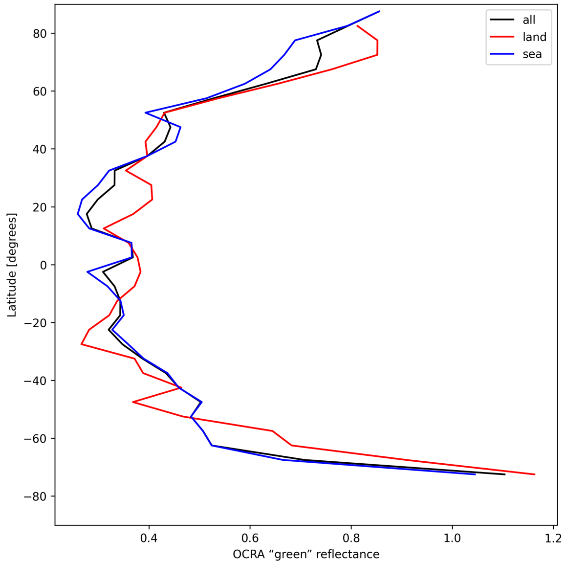
Figure 36: Zonal average of “OCRA “green” reflectance” for 2025-04-29 to 2025-05-01.
