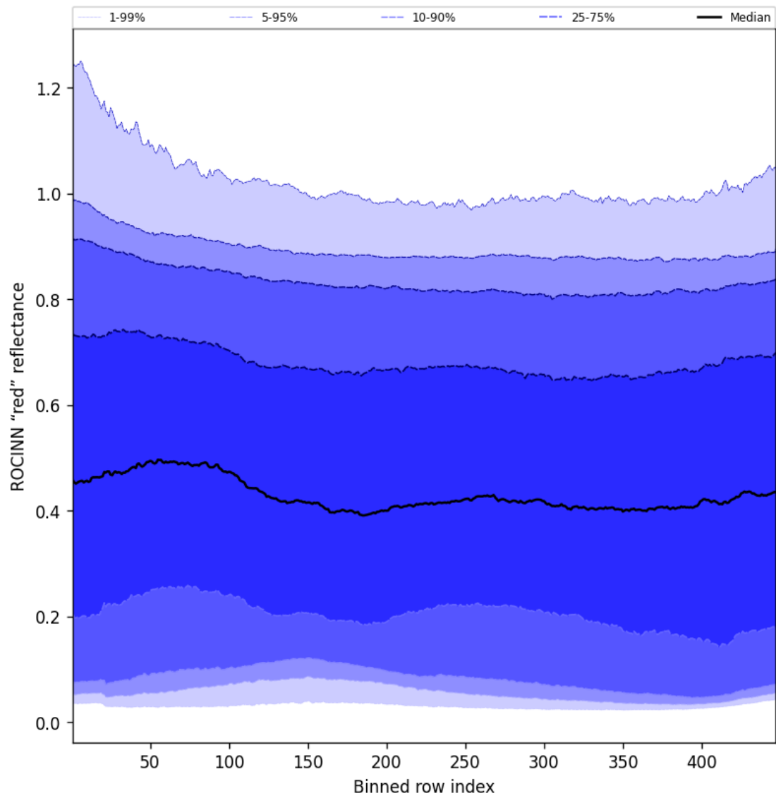
Figure 69: Along track statistics of “ROCINN “red” reflectance” for 2025-04-29 to 2025-05-01
