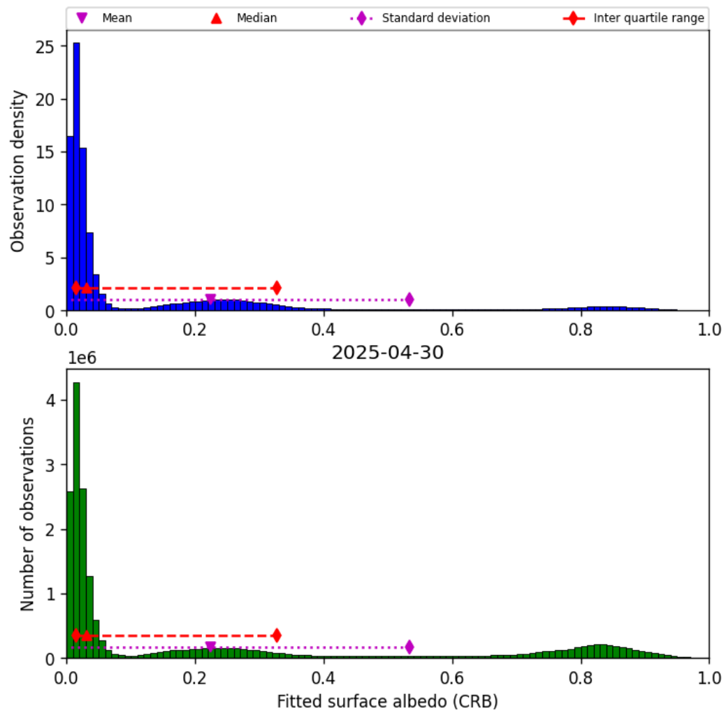
Figure 46: Histogram of “Fitted surface albedo (CRB)” for 2025-04-29 to 2025-05-01
