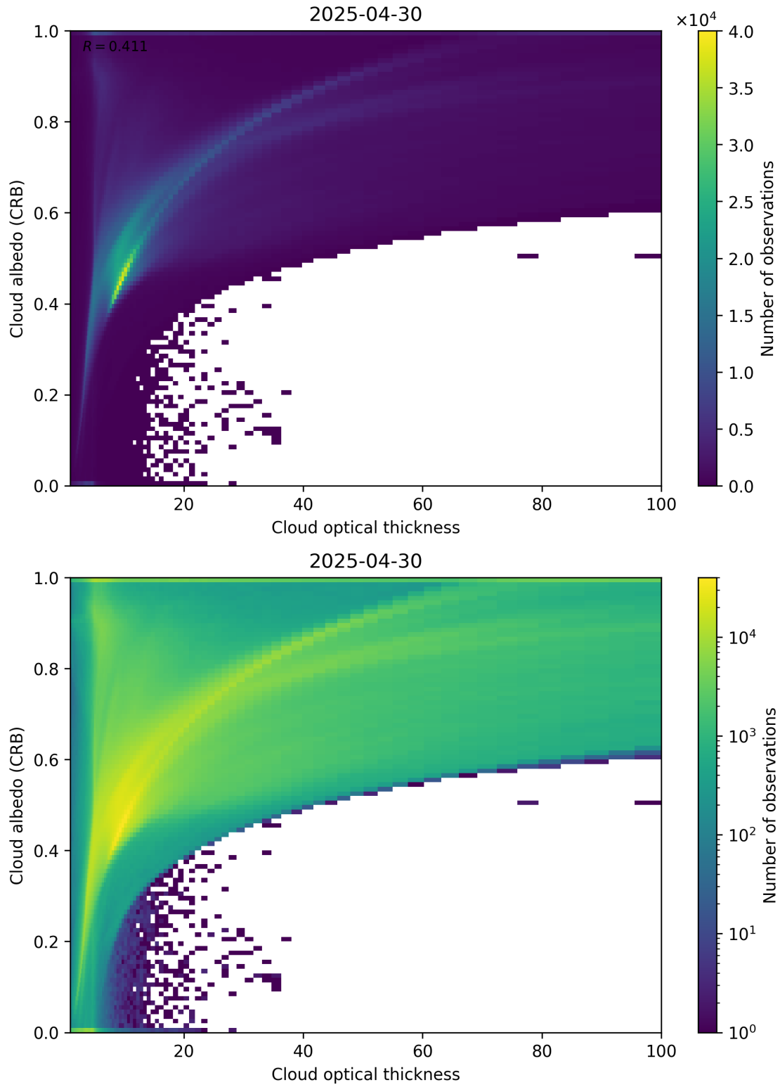
Figure 82: Scatter density plot of “Cloud optical thickness” against “Cloud albedo (CRB)” for 2025-04-29 to 2025-05-01.
