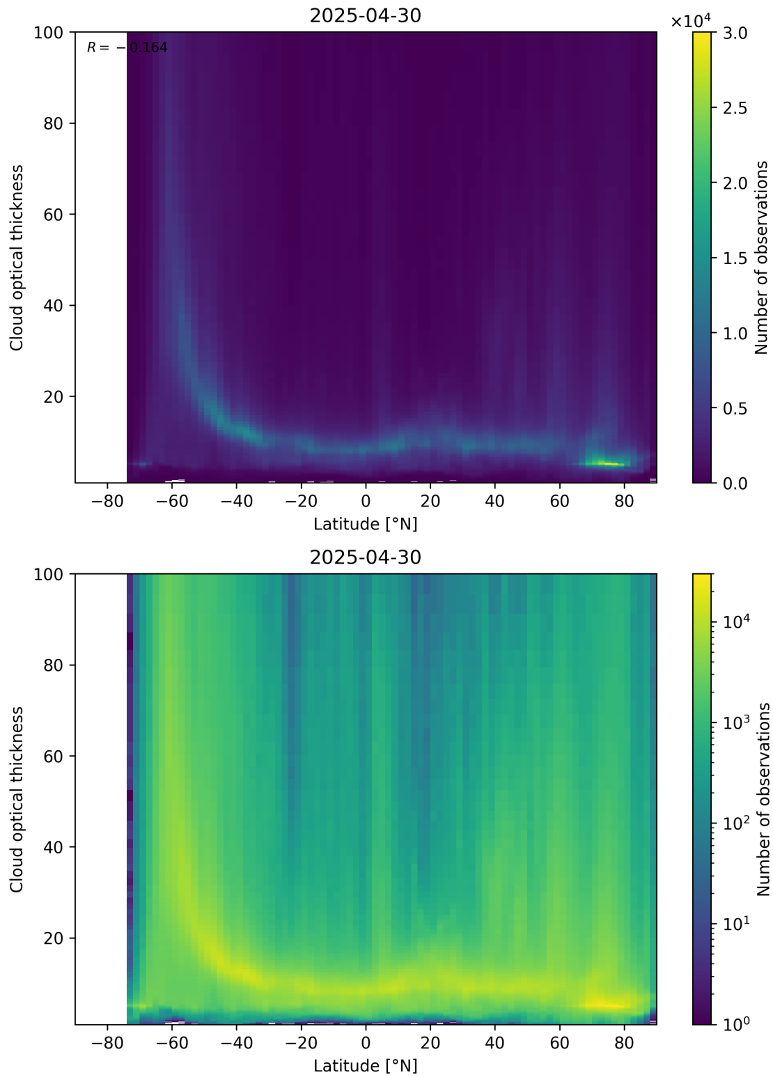
Figure 96: Scatter density plot of “Latitude” against “Cloud optical thickness” for 2025-04-29 to 2025-05-01.
