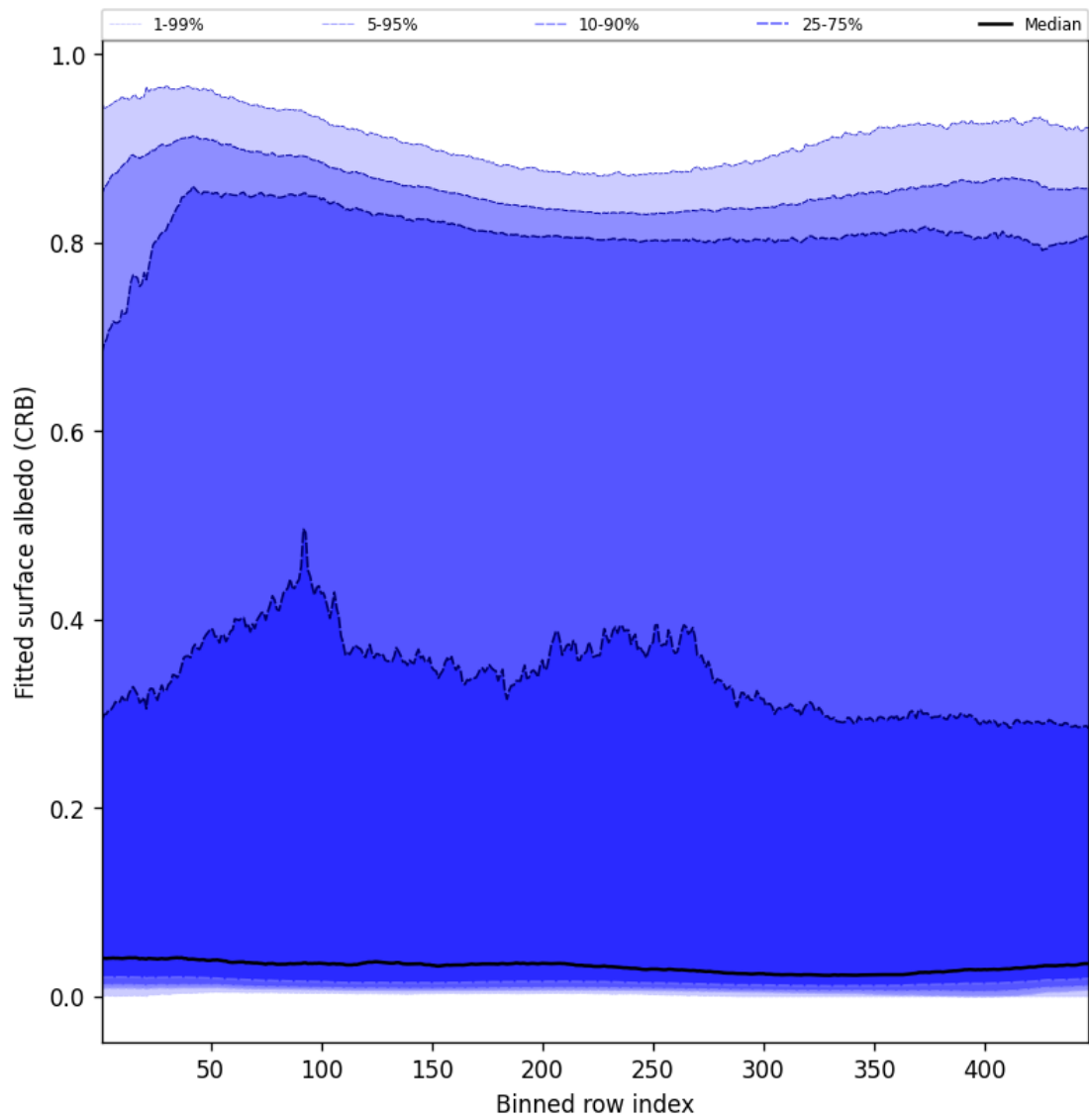
Figure 62: Along track statistics of “Fitted surface albedo (CRB)” for 2025-04-29 to 2025-05-01
