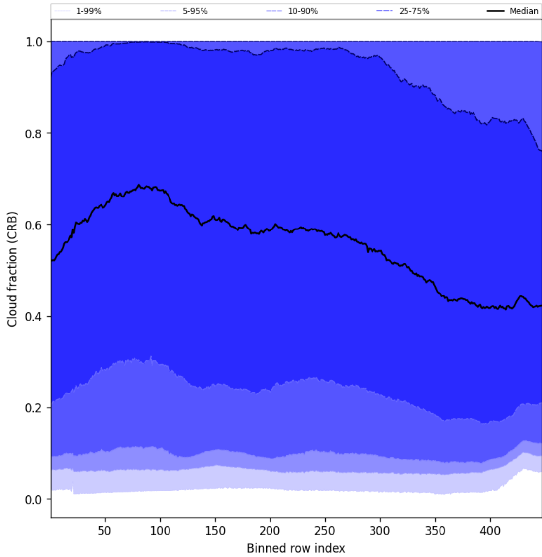
Figure 58: Along track statistics of “Cloud fraction (CRB)” for 2025-04-29 to 2025-05-01
