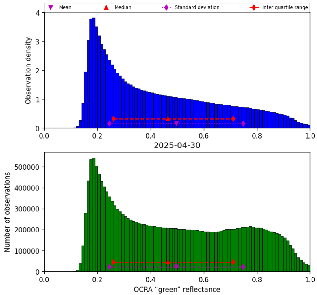
Figure 52: Histogram of “OCRA “green” reflectance” for 2025-04-29 to 2025-05-01
