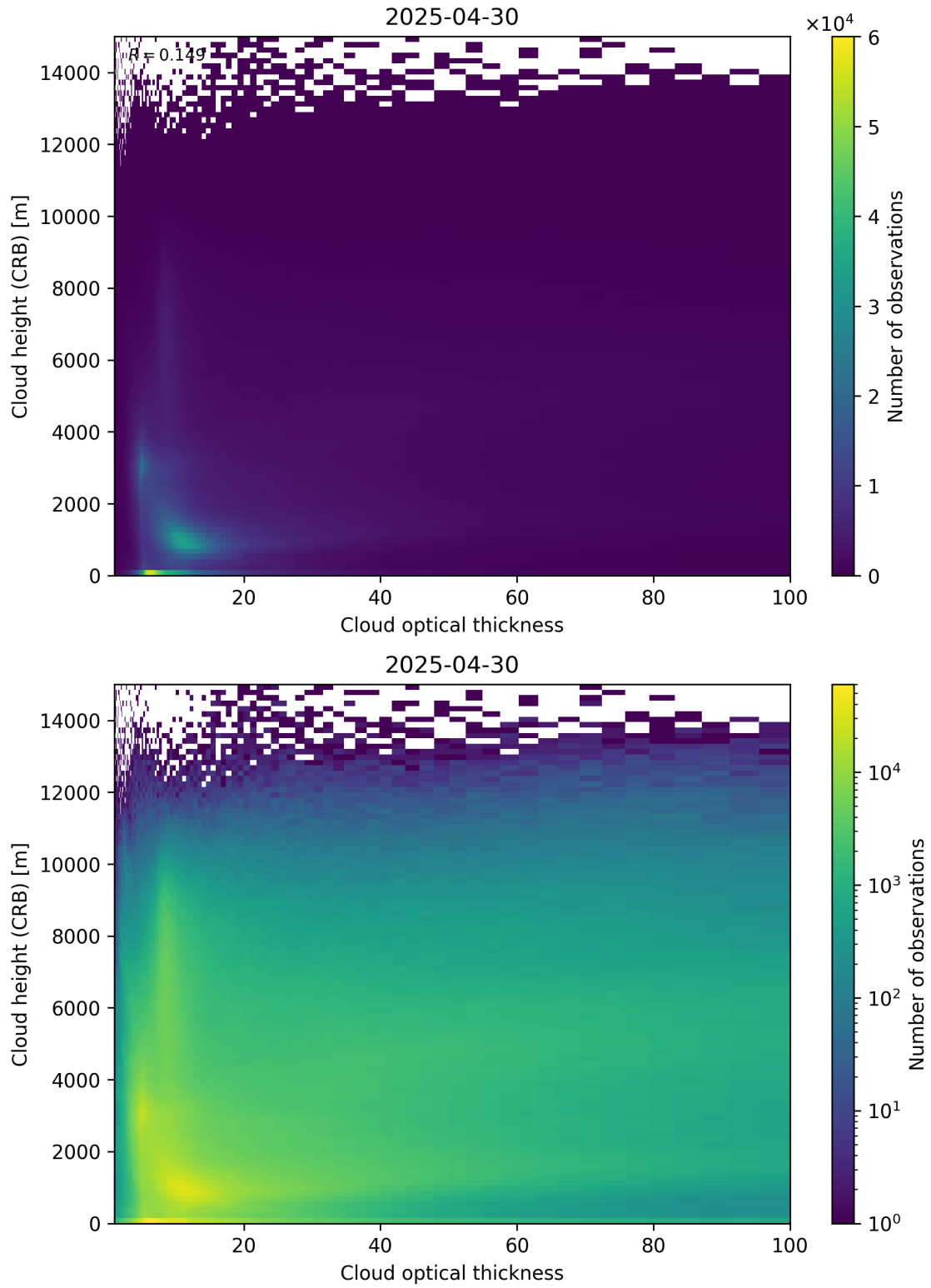
Figure 85: Scatter density plot of “Cloud optical thickness” against “Cloud height (CRB)” for 2025-04-29 to 2025-05-01.
