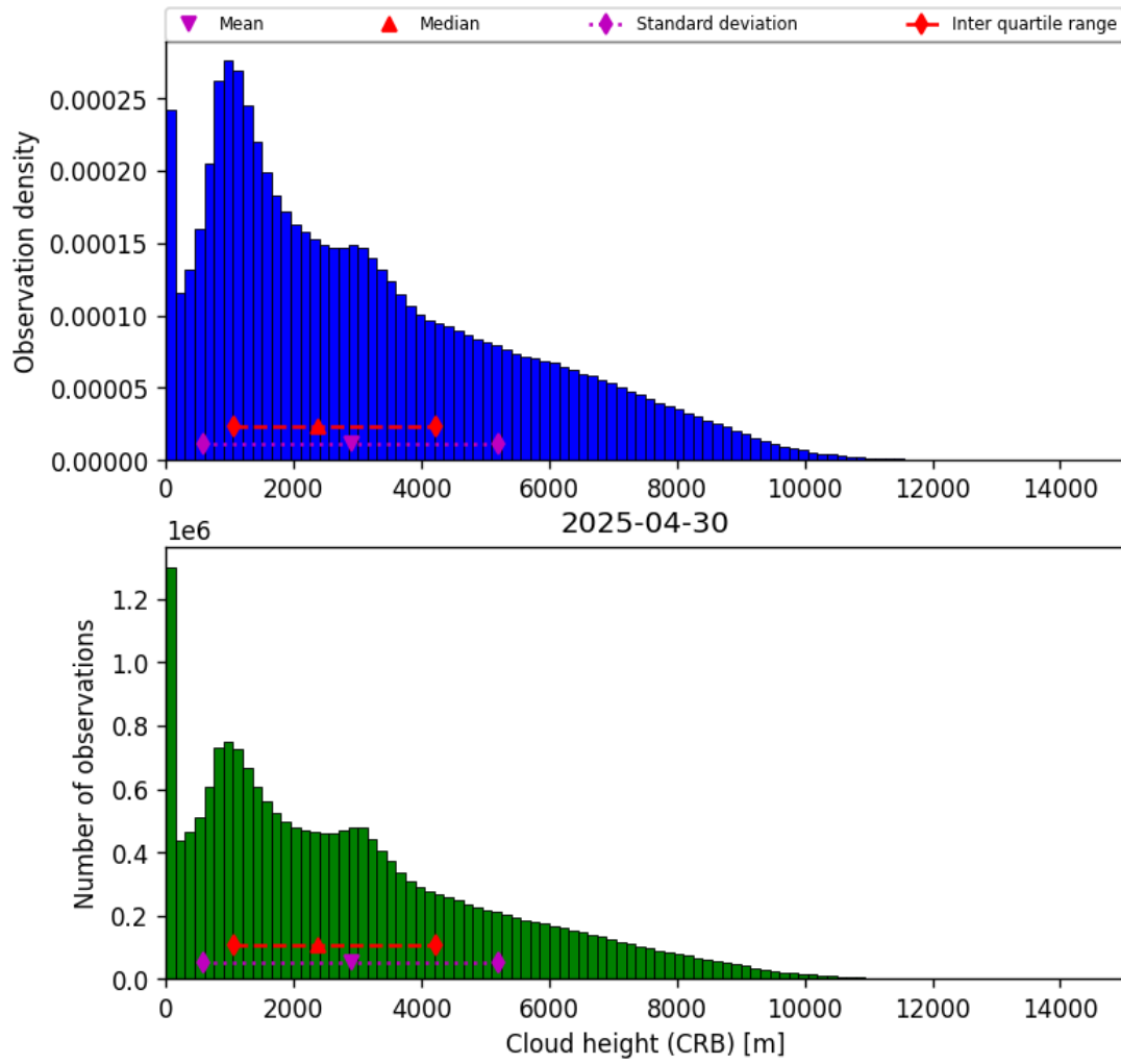
Figure 43: Histogram of “Cloud height (CRB)” for 2025-04-29 to 2025-05-01
