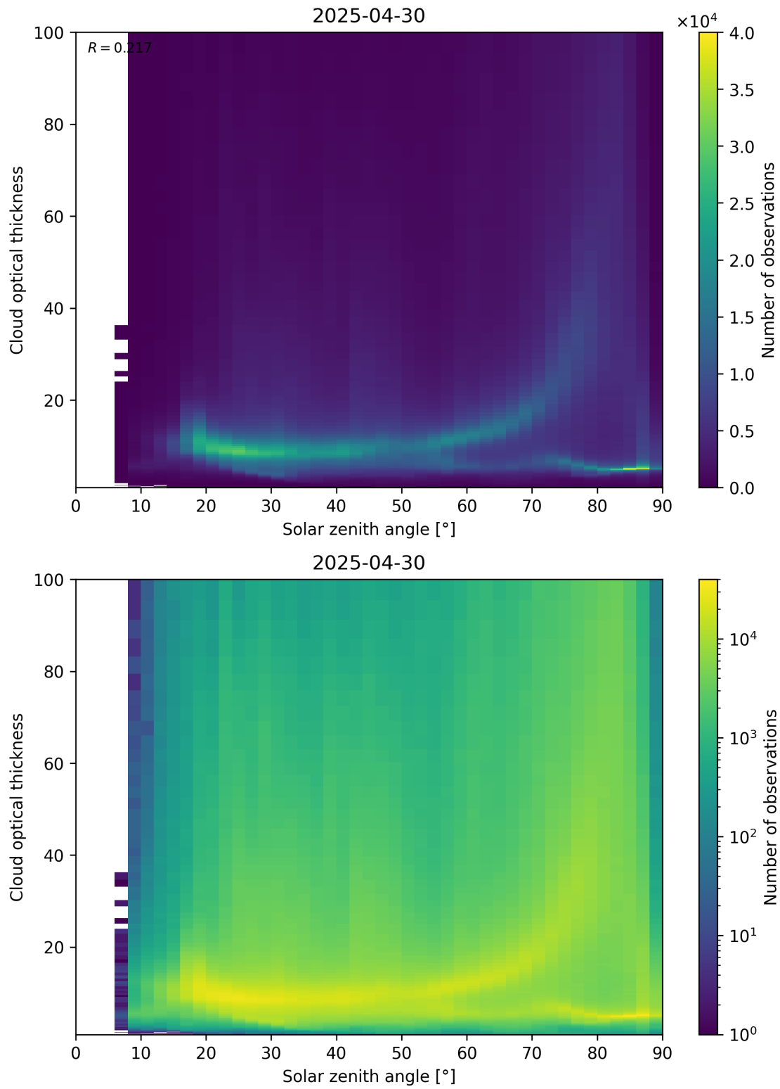
Figure 103: Scatter density plot of “Solar zenith angle” against “Cloud optical thickness” for 2025-04-29 to 2025-05-01.
