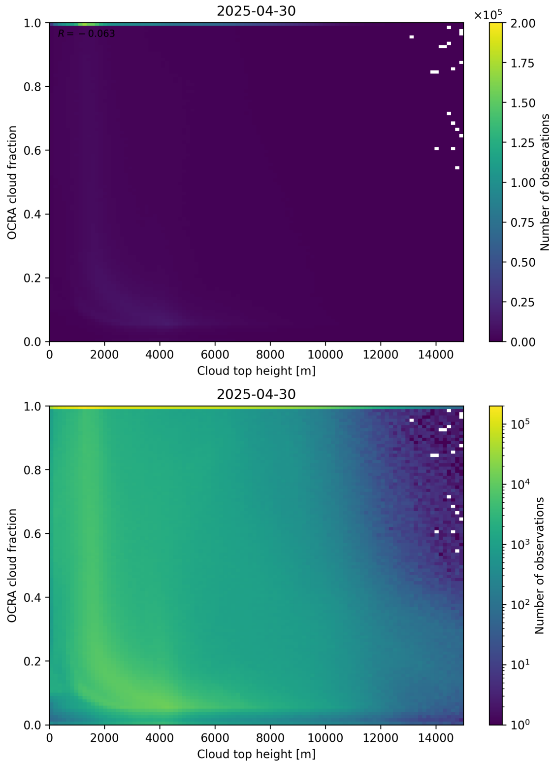
Figure 87: Scatter density plot of “Cloud top height” against “OCRA cloud fraction” for 2025-04-29 to 2025-05-01.
