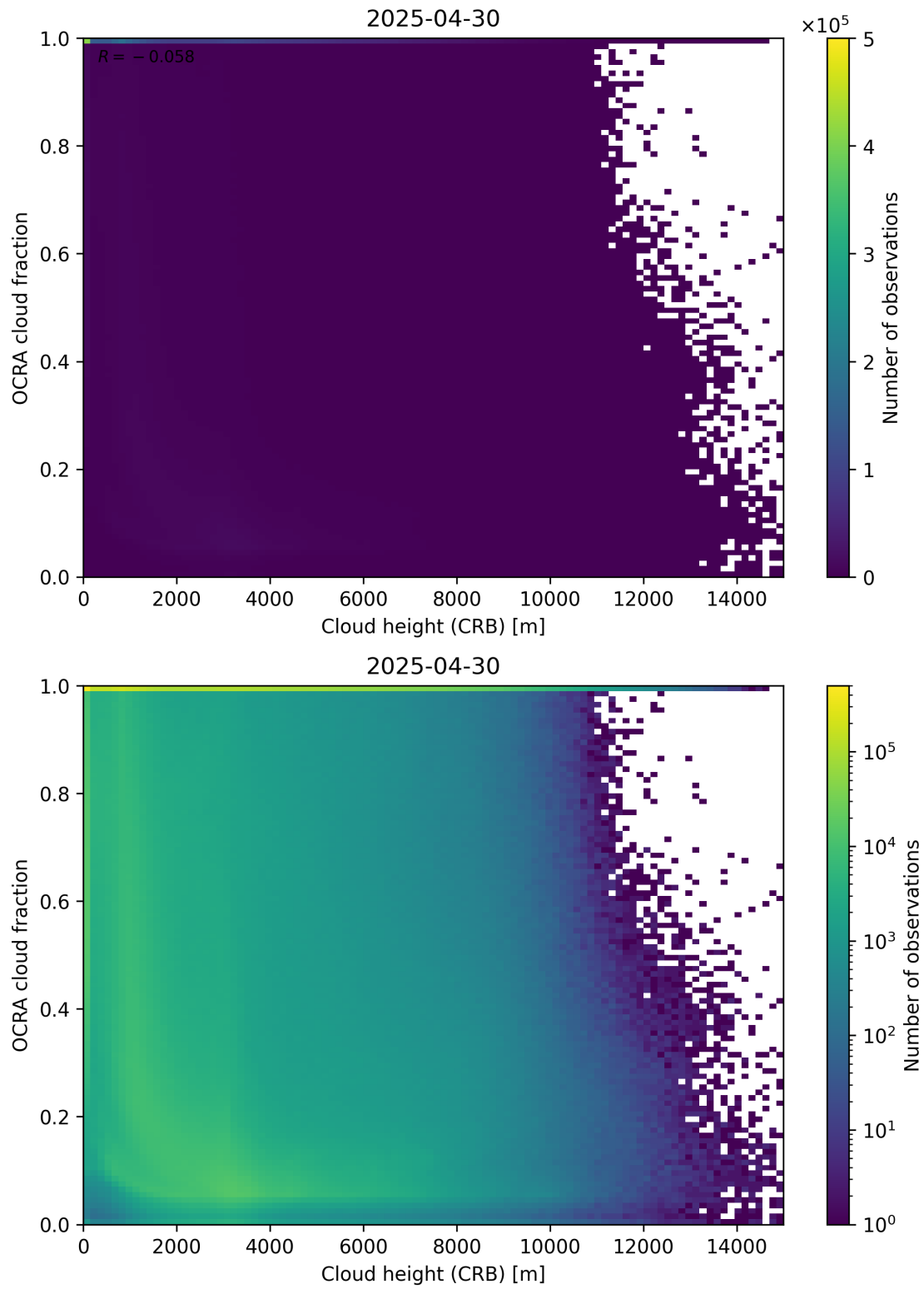
Figure 81: Scatter density plot of “Cloud height (CRB)” against “OCRA cloud fraction” for 2025-04-29 to 2025-05-01.
