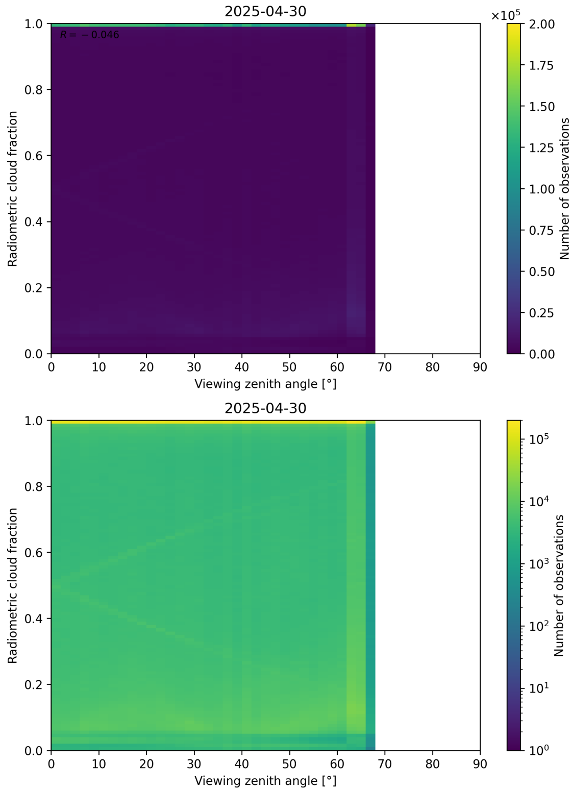
Figure 107: Scatter density plot of “Viewing zenith angle” against “Radiometric cloud fraction” for 2025-04-29 to 2025-05-01.
