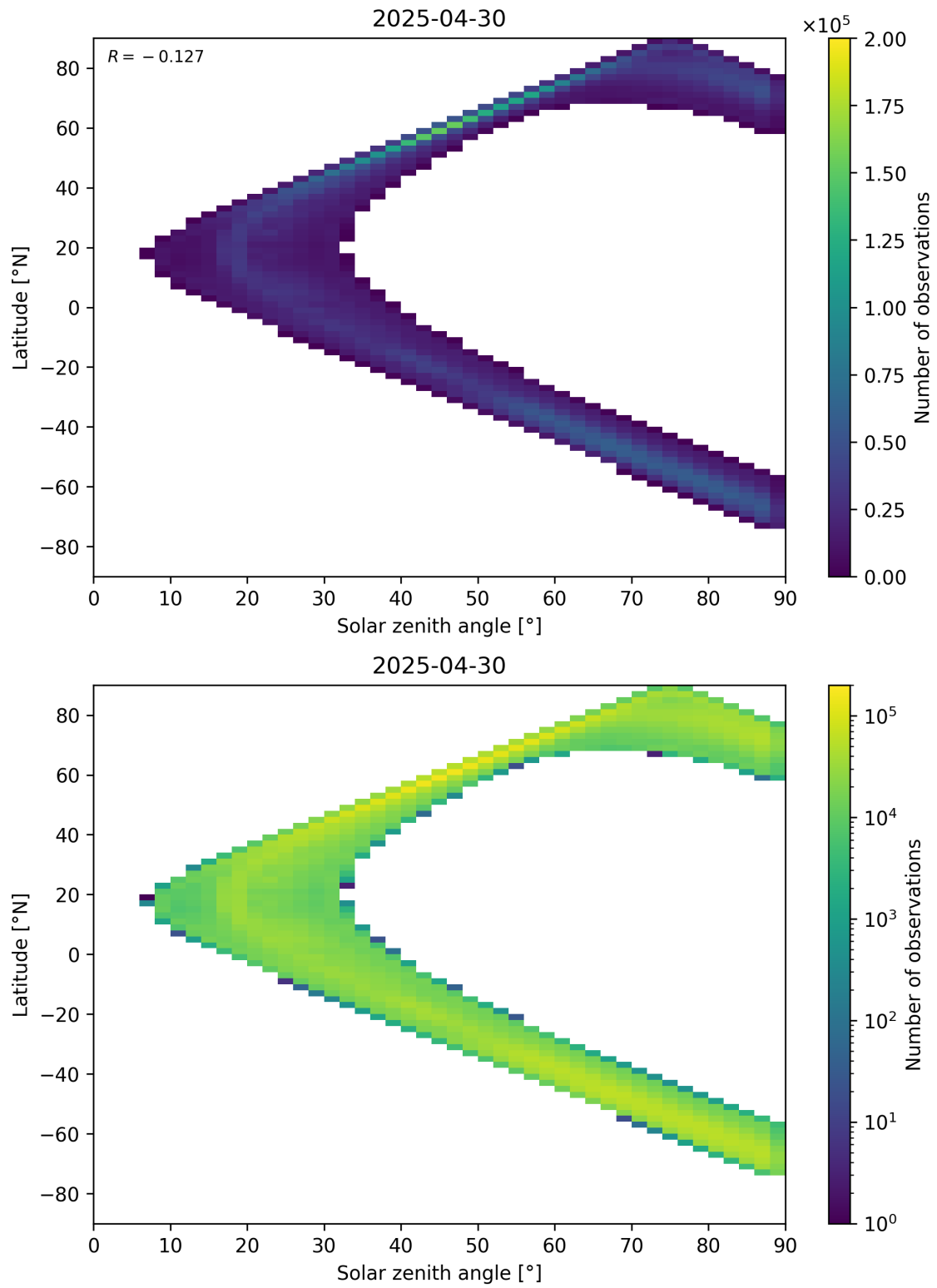
Figure 105: Scatter density plot of “Solar zenith angle” against “Latitude” for 2025-04-29 to 2025-05-01.
