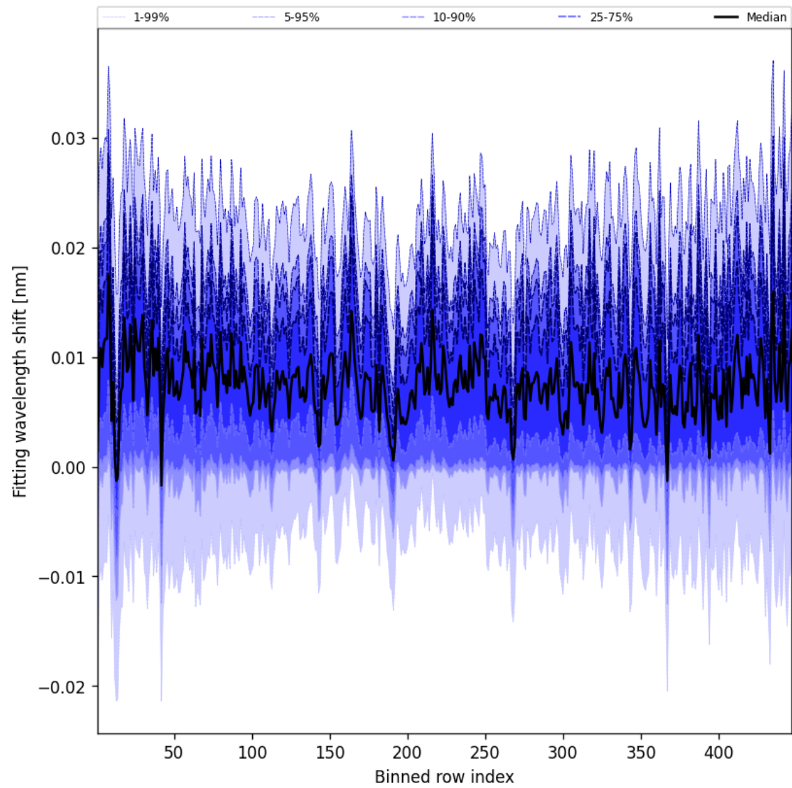
Figure 65: Along track statistics of “Fitting wavelength shift” for 2025-04-29 to 2025-05-01
