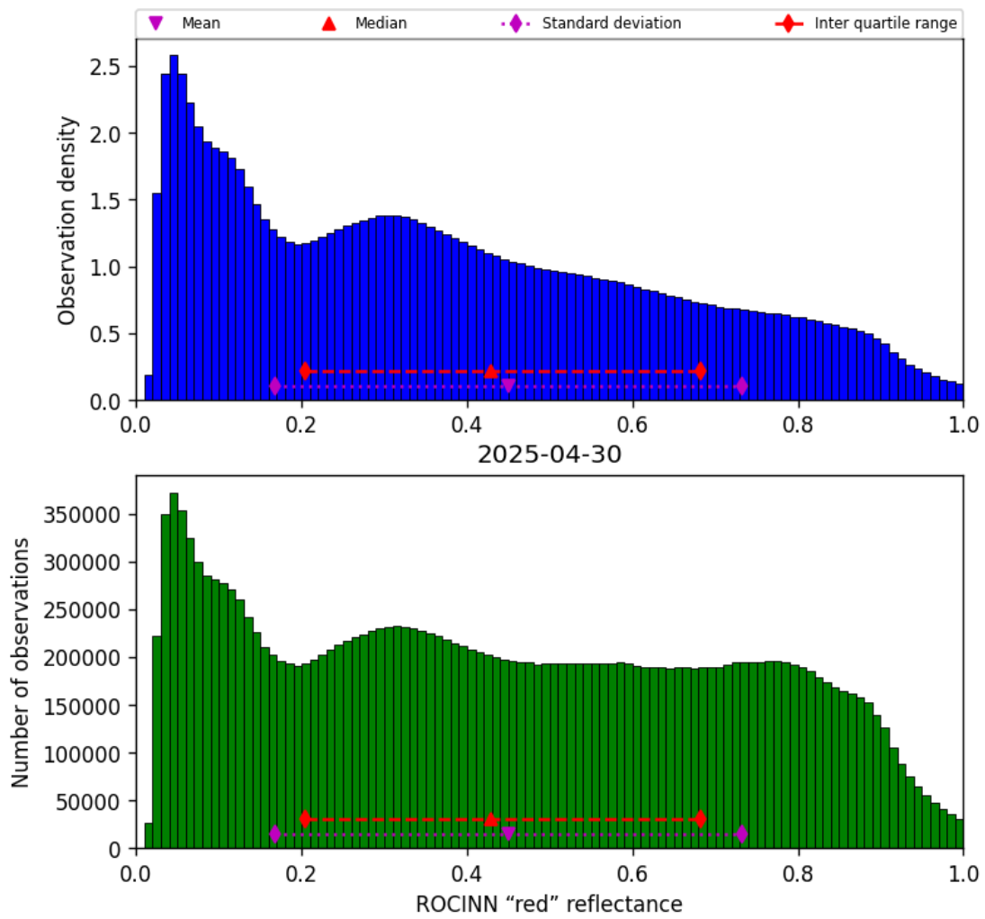
Figure 53: Histogram of “ROCINN “red” reflectance” for 2025-04-29 to 2025-05-01
