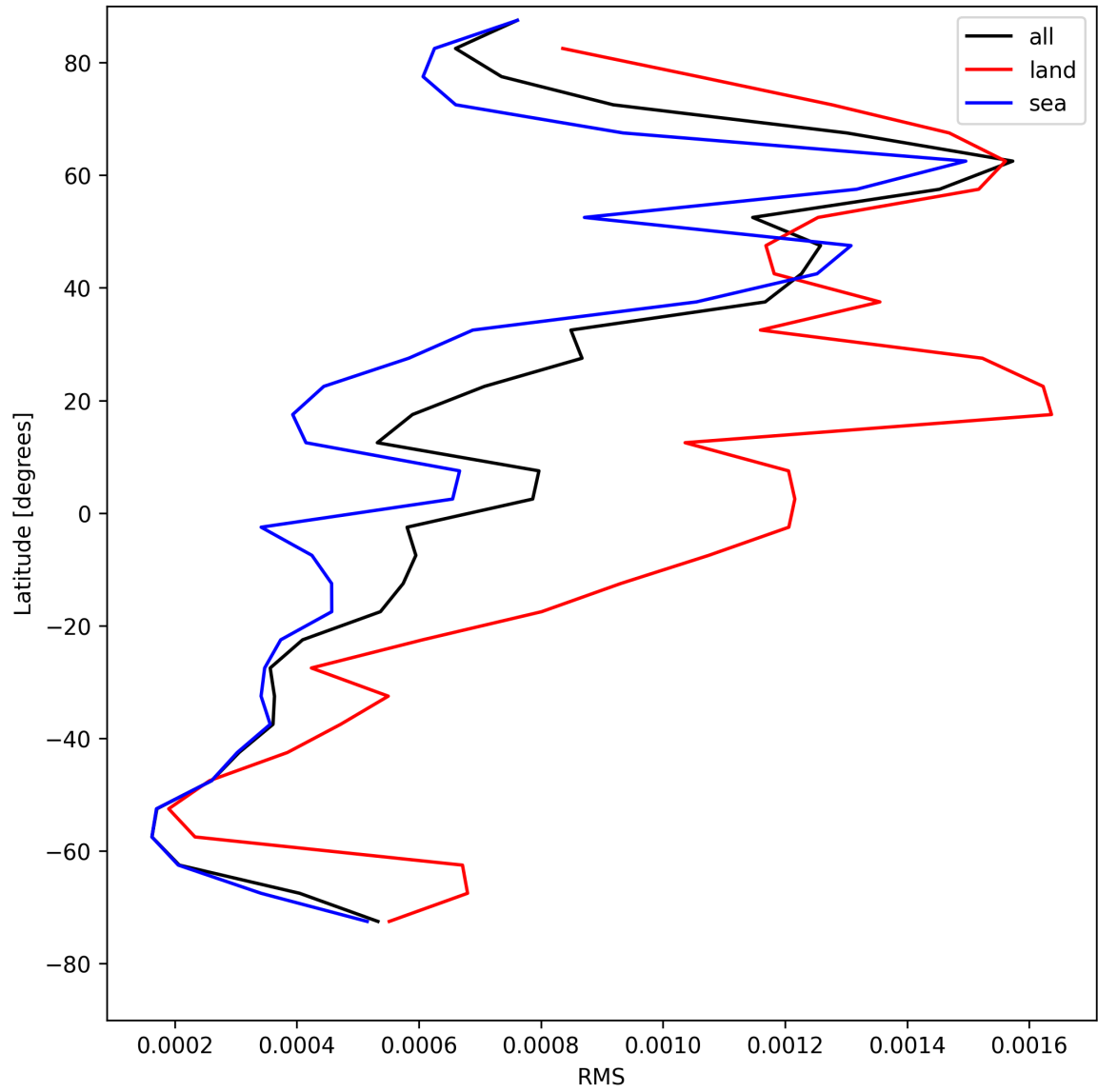
Figure 31: Zonal average of “RMS” for 2025-04-29 to 2025-05-01.
