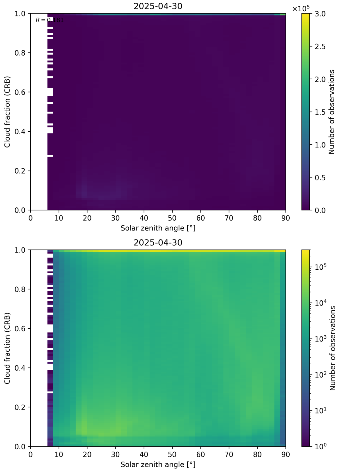
Figure 101: Scatter density plot of “Solar zenith angle” against “Cloud fraction (CRB)” for 2025-04-29 to 2025-05-01.
