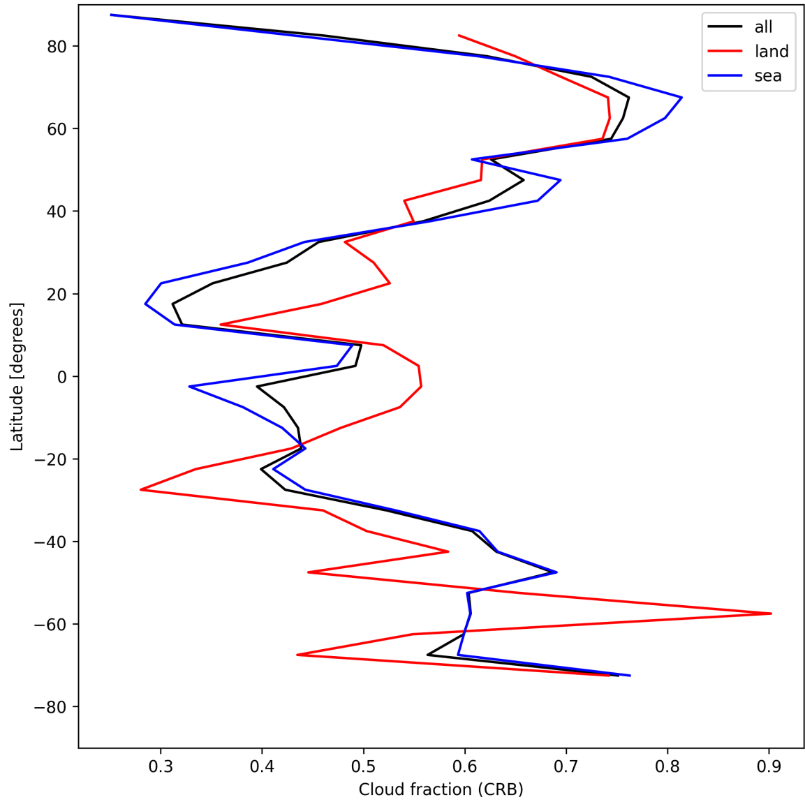
Figure 26: Zonal average of “Cloud fraction (CRB)” for 2025-04-29 to 2025-05-01.
