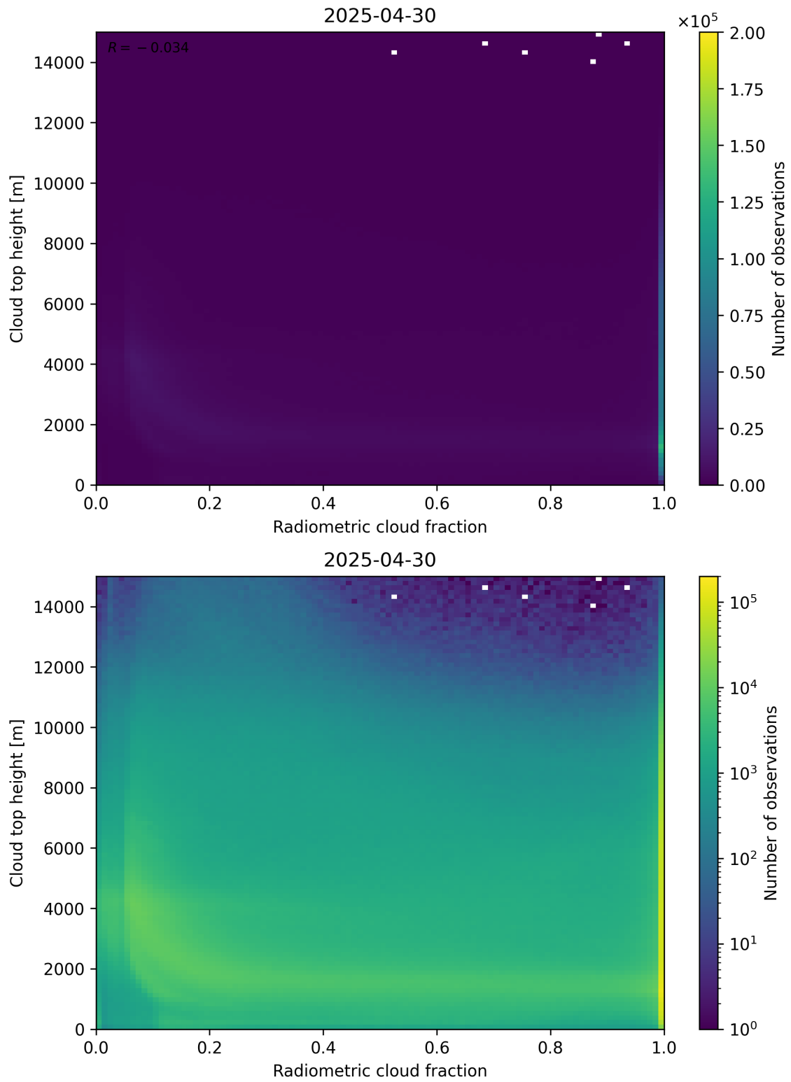
Figure 76: Scatter density plot of “Radiometric cloud fraction” against “Cloud top height” for 2025-04-29 to 2025-05-01.
