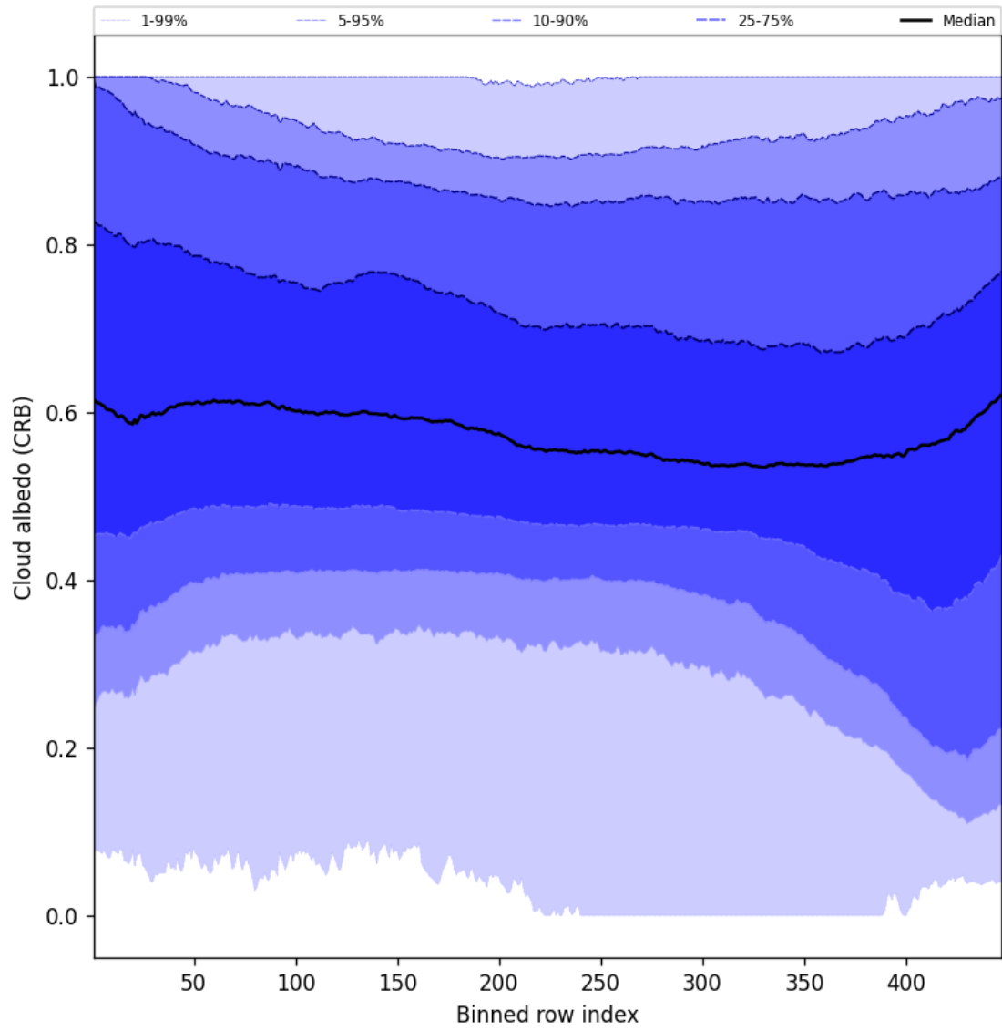
Figure 60: Along track statistics of “Cloud albedo (CRB)” for 2025-04-29 to 2025-05-01
