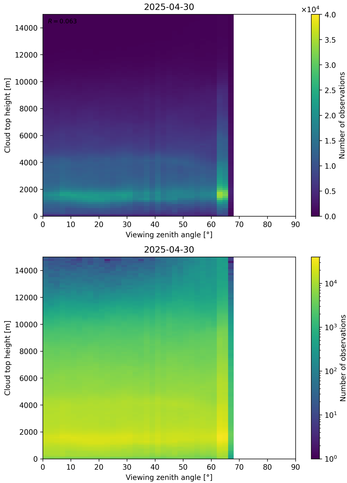
Figure 112: Scatter density plot of “Viewing zenith angle” against “Cloud top height” for 2025-04-29 to 2025-05-01.
