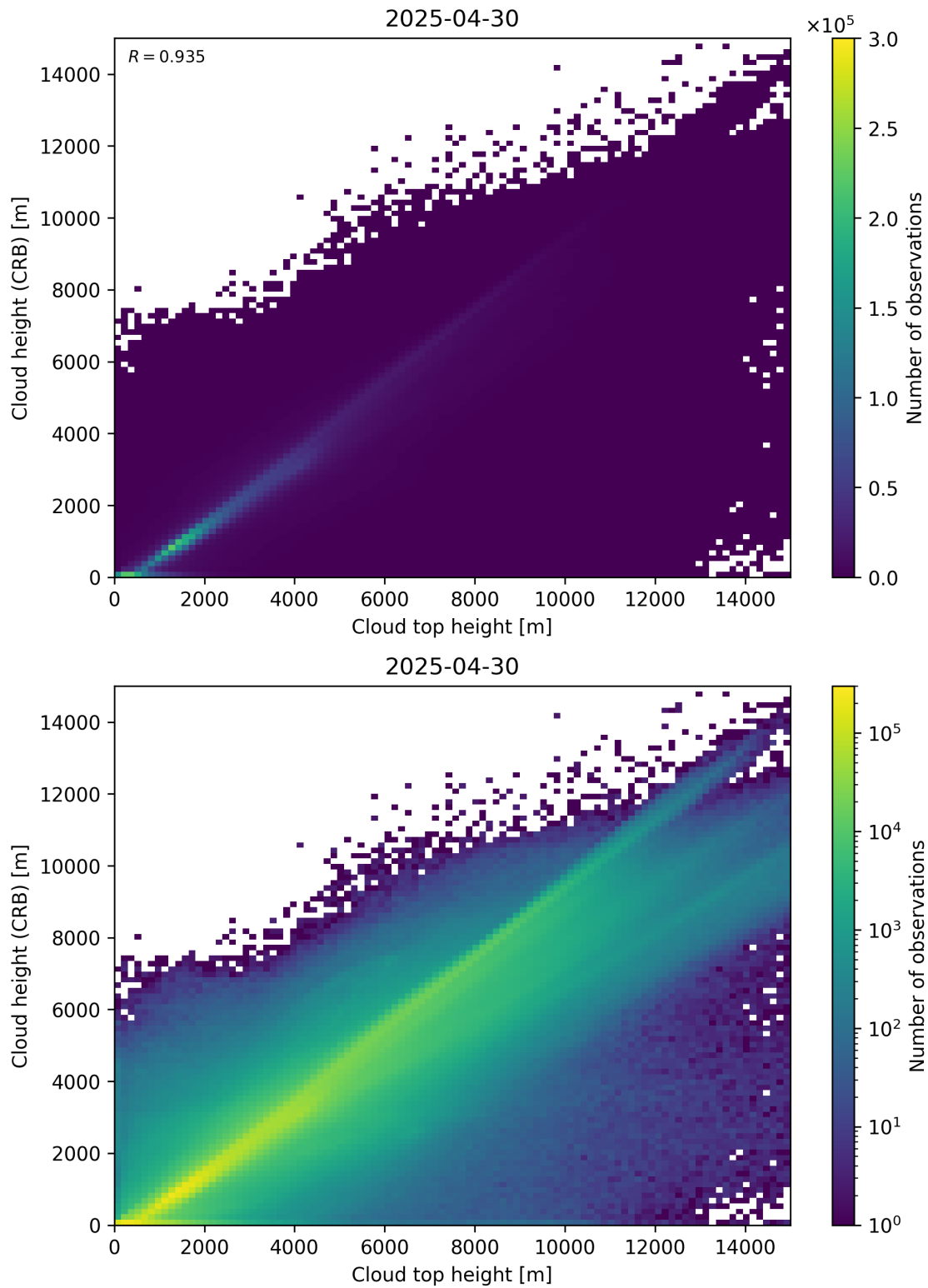
Figure 89: Scatter density plot of “Cloud top height” against “Cloud height (CRB)” for 2025-04-29 to 2025-05-01.
