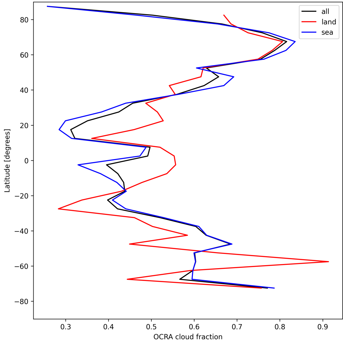
Figure 34: Zonal average of “OCRA cloud fraction” for 2025-04-29 to 2025-05-01.
