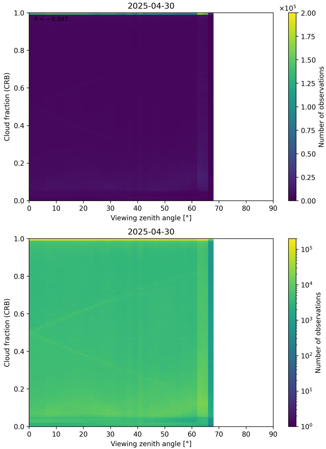
Figure 109: Scatter density plot of “Viewing zenith angle” against “Cloud fraction (CRB)” for 2025-04-29 to 2025-05-01.
