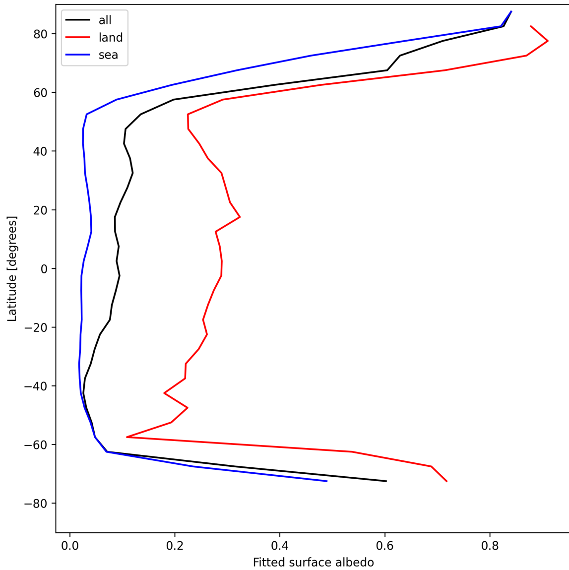
Figure 29: Zonal average of “Fitted surface albedo” for 2025-04-29 to 2025-05-01.
