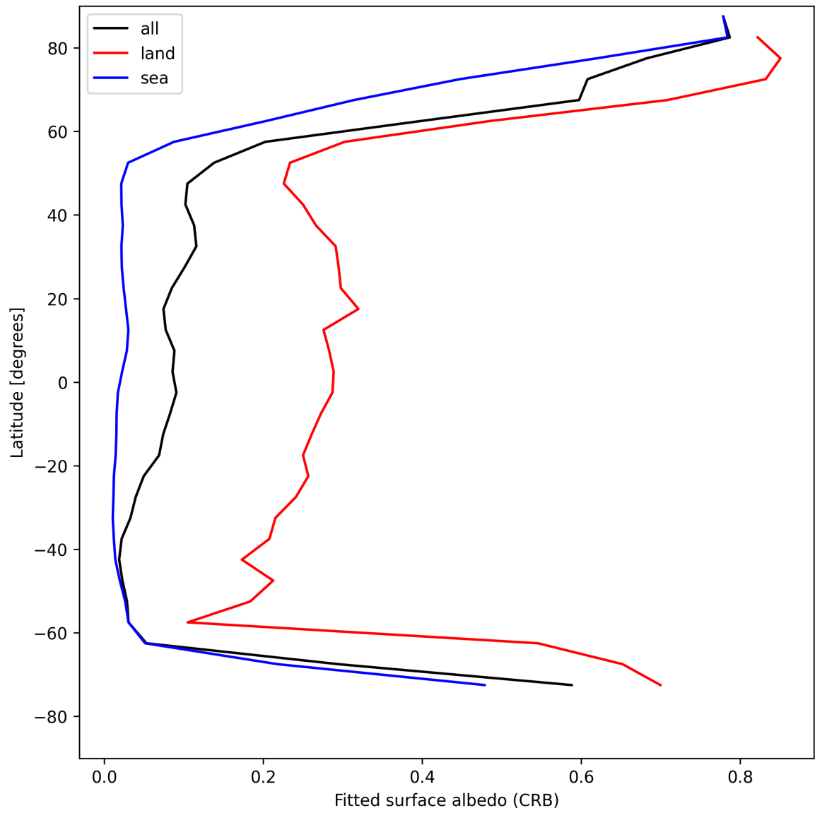
Figure 30: Zonal average of “Fitted surface albedo (CRB)” for 2025-04-29 to 2025-05-01.
