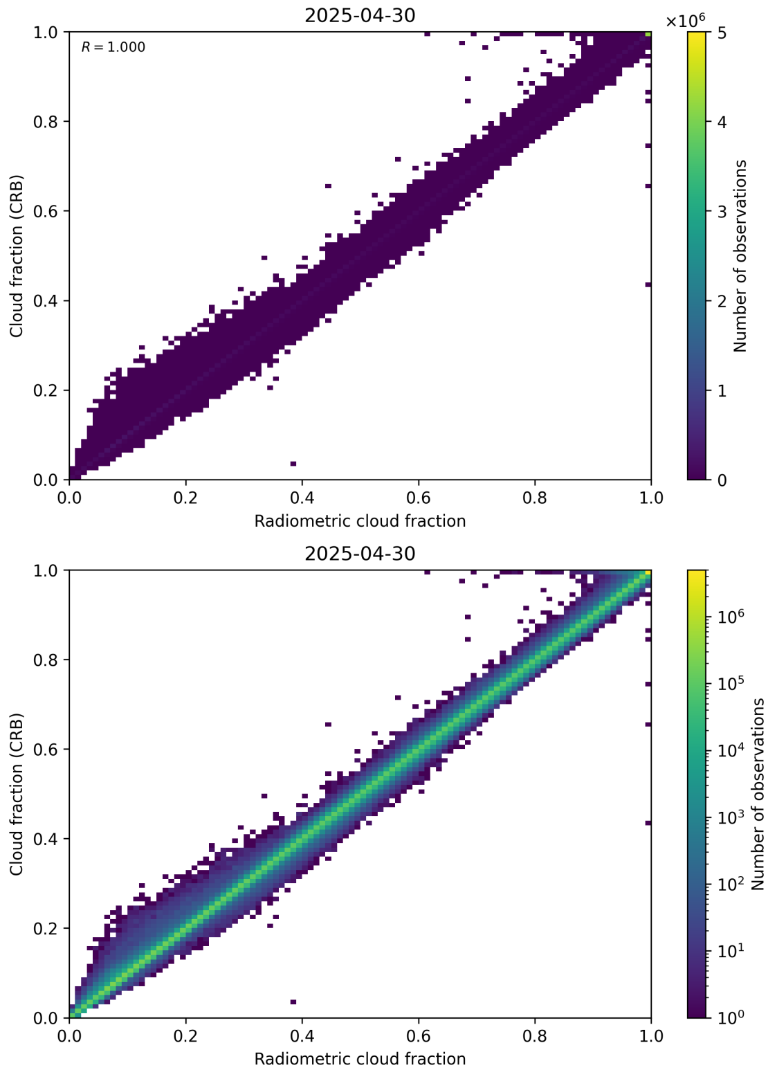
Figure 73: Scatter density plot of “Radiometric cloud fraction” against “Cloud fraction (CRB)” for 2025-04-29 to 2025-05-01.
