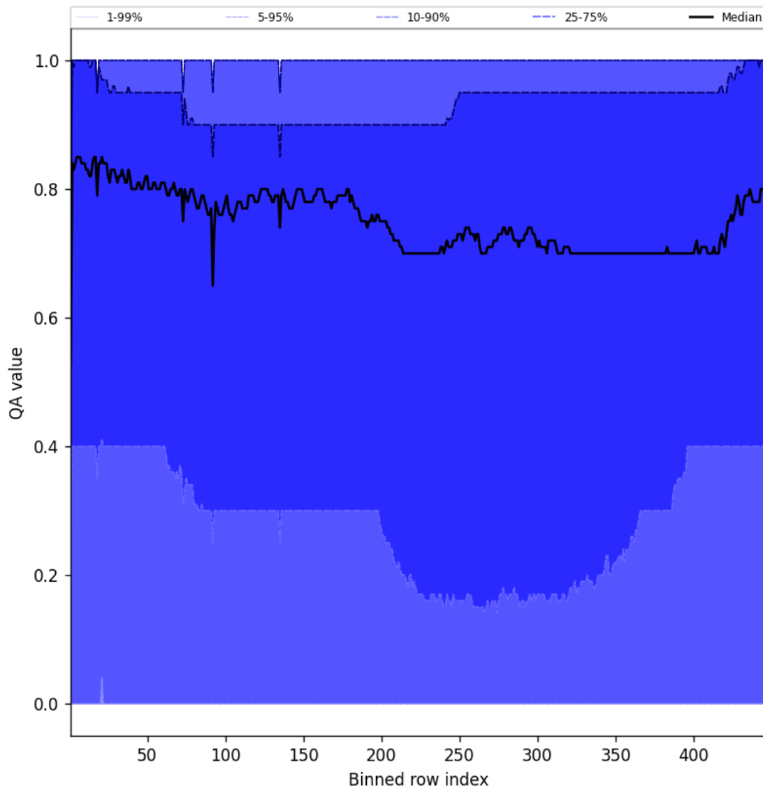
Figure 54: Along track statistics of “QA value” for 2025-04-29 to 2025-05-01
