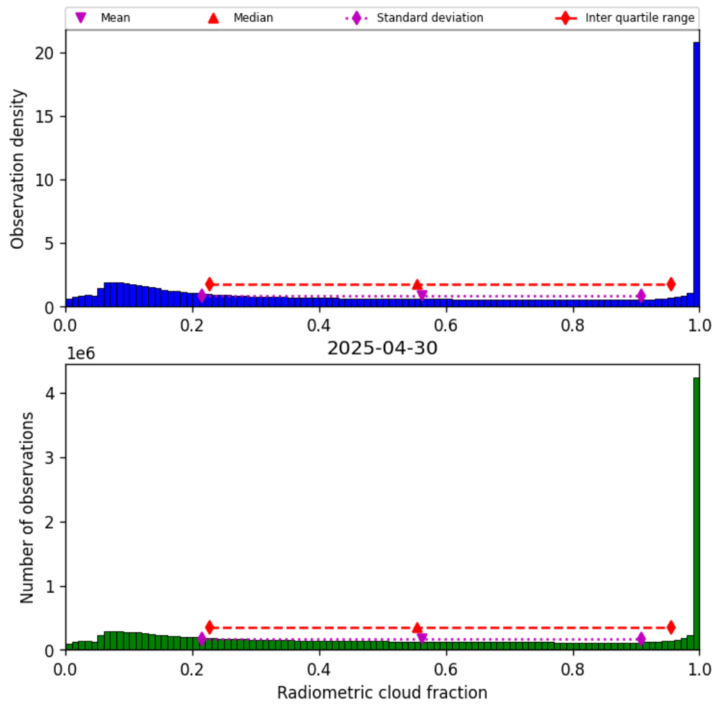
Figure 39: Histogram of “Radiometric cloud fraction” for 2025-04-29 to 2025-05-01
