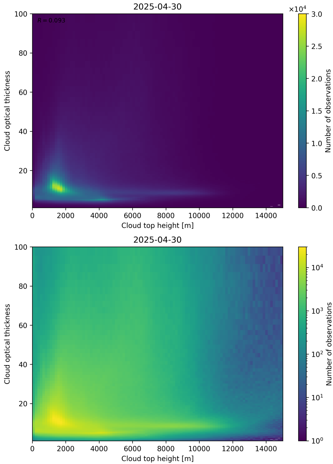
Figure 90: Scatter density plot of “Cloud top height” against “Cloud optical thickness” for 2025-04-29 to 2025-05-01.
