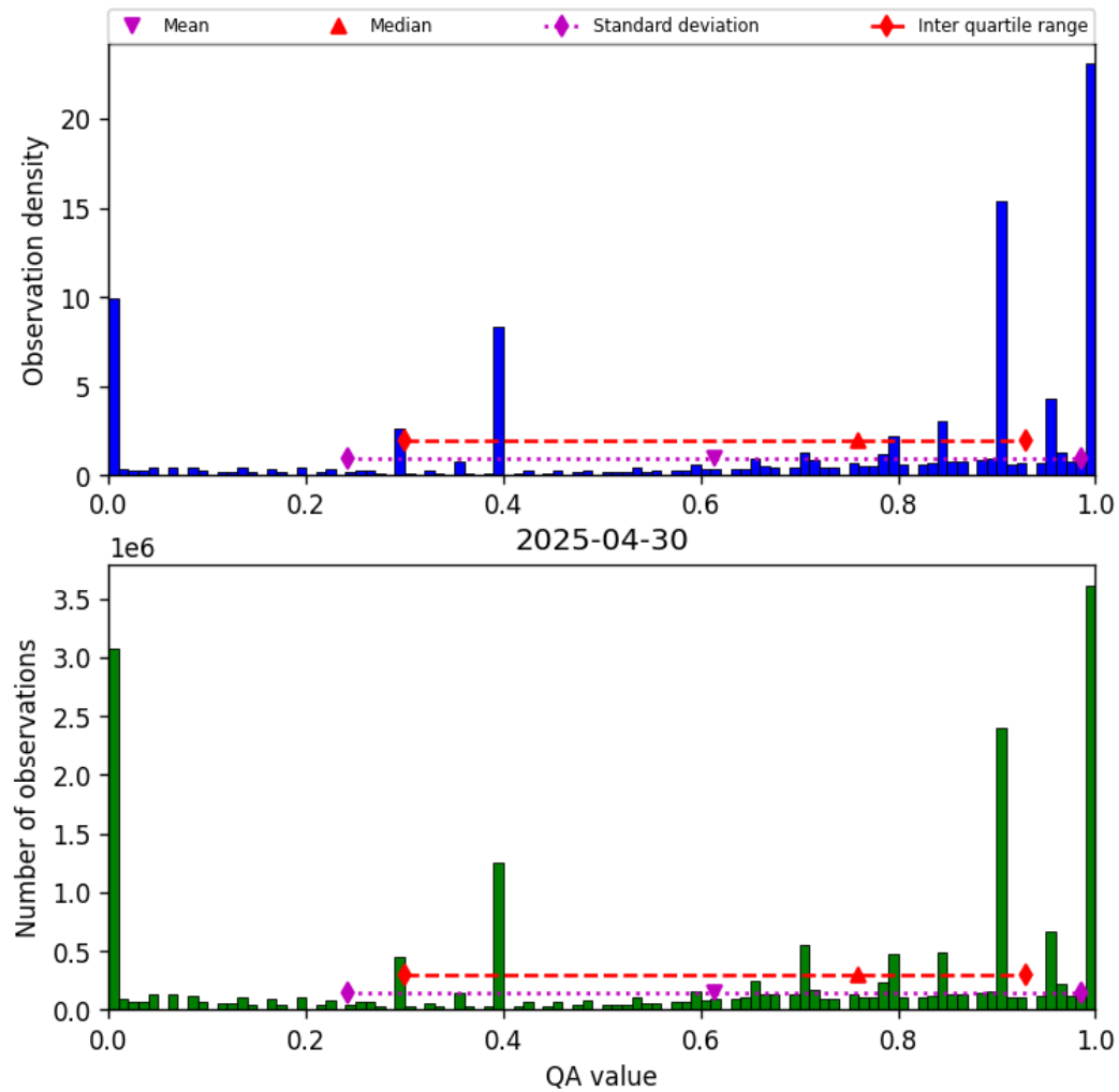
Figure 38: Histogram of “QA value” for 2025-04-29 to 2025-05-01
