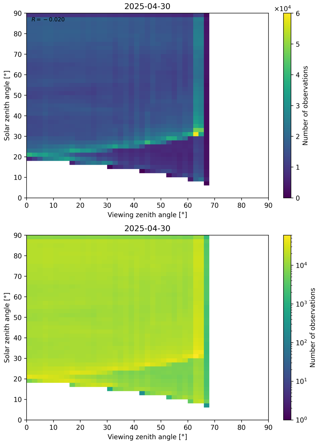
Figure 114: Scatter density plot of “Viewing zenith angle” against “Solar zenith angle” for 2025-04-29 to 2025-05-01.
