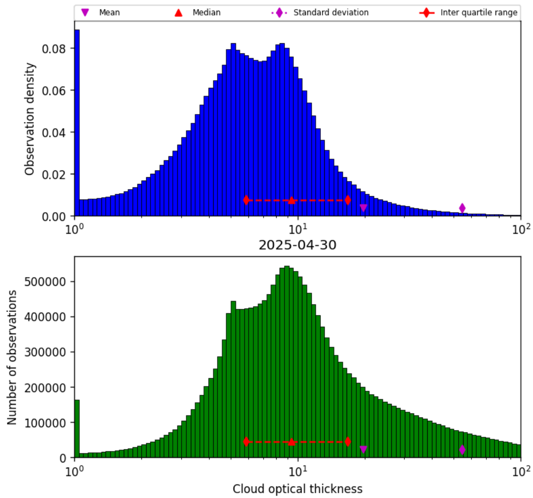
Figure 41: Histogram of “Cloud optical thickness” for 2025-04-29 to 2025-05-01
