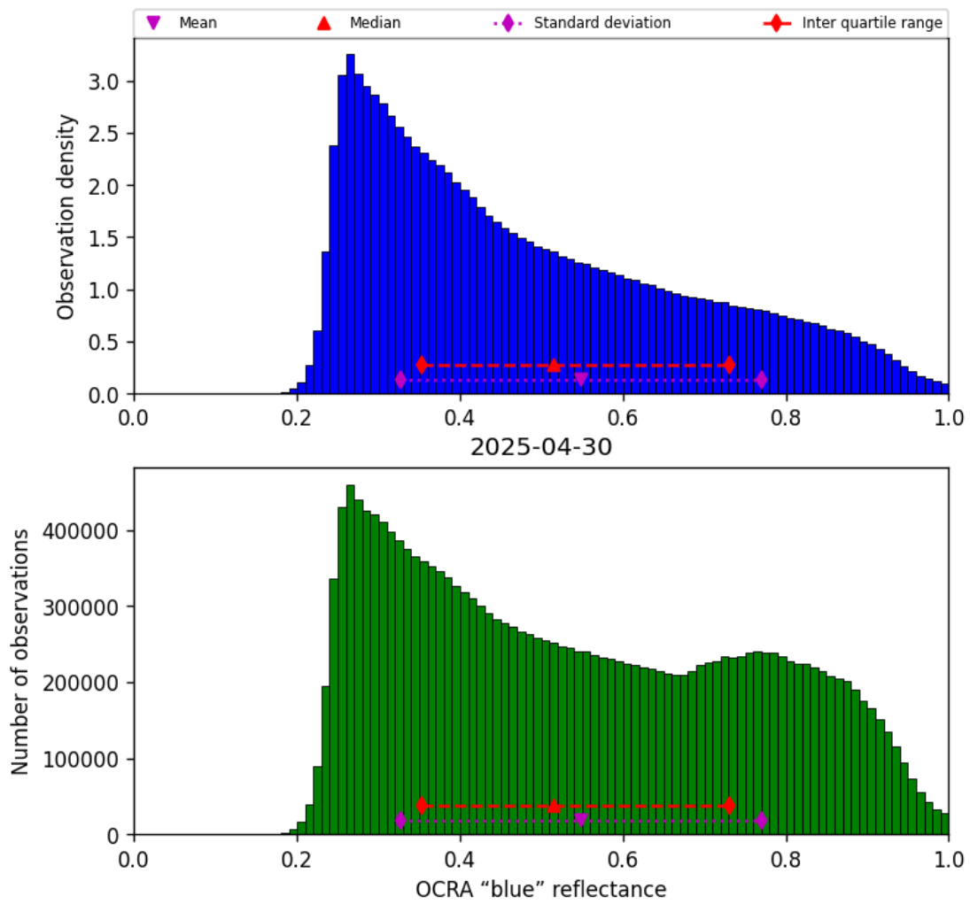
Figure 51: Histogram of “OCRA “blue” reflectance” for 2025-04-29 to 2025-05-01
