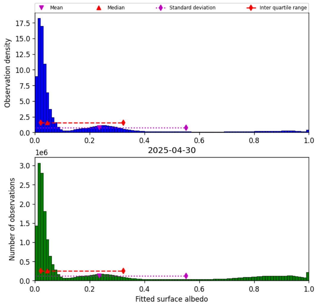
Figure 45: Histogram of “Fitted surface albedo” for 2025-04-29 to 2025-05-01
