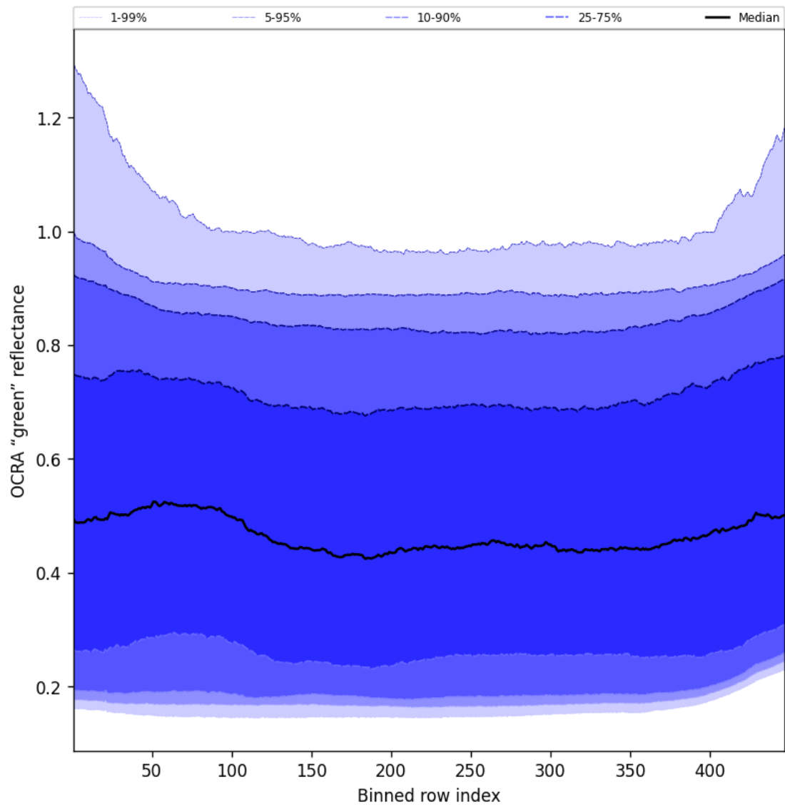
Figure 68: Along track statistics of “OCRA “green” reflectance” for 2025-04-29 to 2025-05-01
