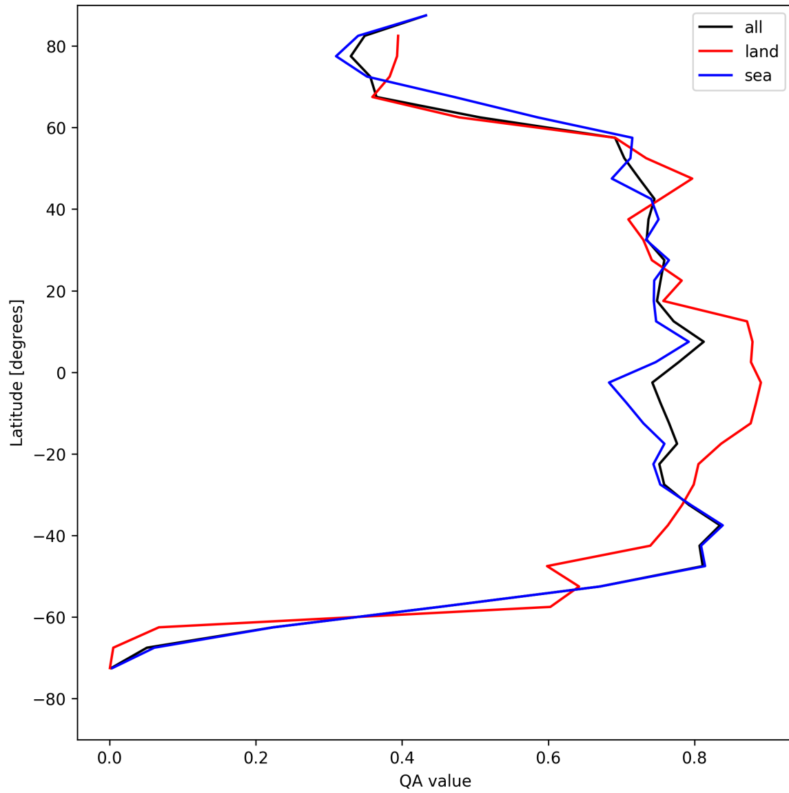
Figure 22: Zonal average of “QA value” for 2025-04-29 to 2025-05-01.
