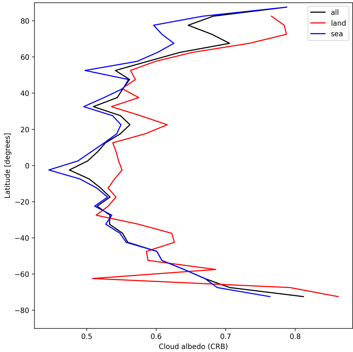
Figure 28: Zonal average of “Cloud albedo (CRB)” for 2025-04-29 to 2025-05-01.
