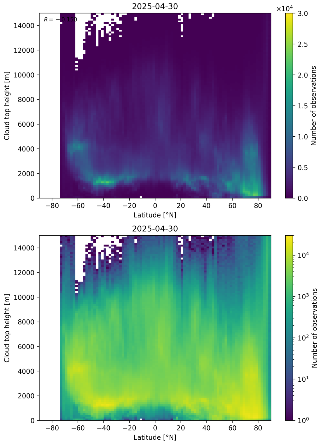
Figure 97: Scatter density plot of “Latitude” against “Cloud top height” for 2025-04-29 to 2025-05-01.
