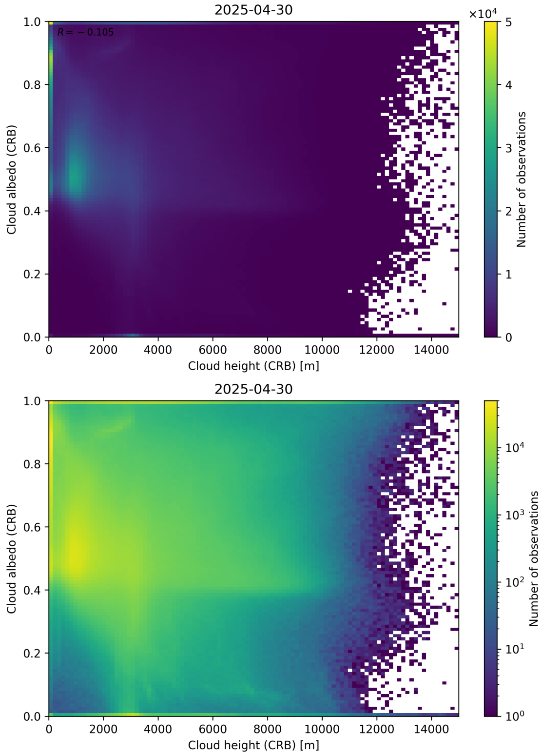
Figure 80: Scatter density plot of “Cloud height (CRB)” against “Cloud albedo (CRB)” for 2025-04-29 to 2025-05-01.
