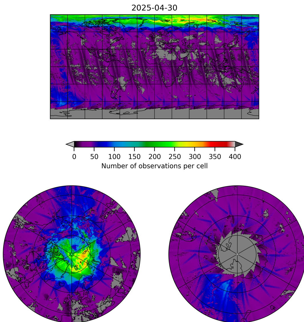
Figure 21: Map of the number of observations for 2025-04-29 to 2025-05-01
