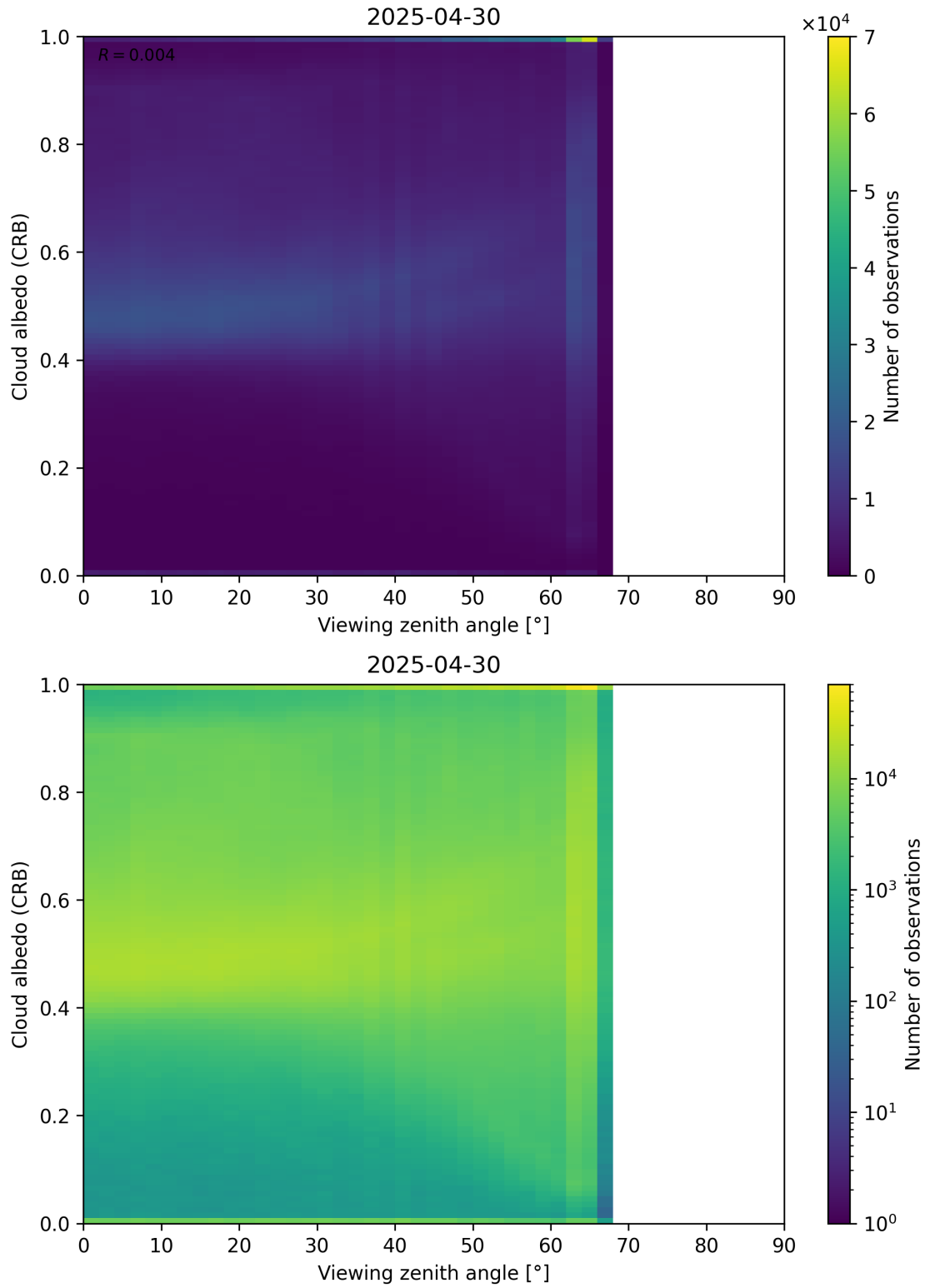
Figure 106: Scatter density plot of “Viewing zenith angle” against “Cloud albedo (CRB)” for 2025-04-29 to 2025-05-01.
