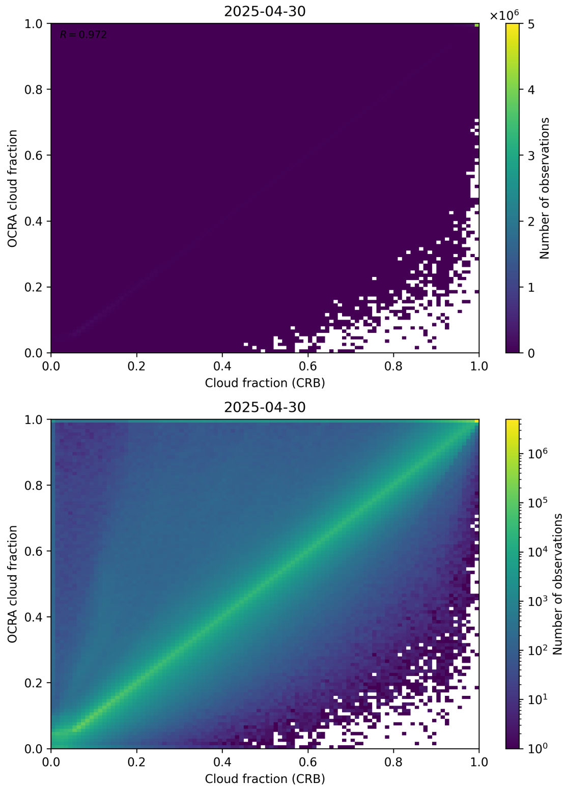
Figure 78: Scatter density plot of “Cloud fraction (CRB)” against “OCRA cloud fraction” for 2025-04-29 to 2025-05-01.
