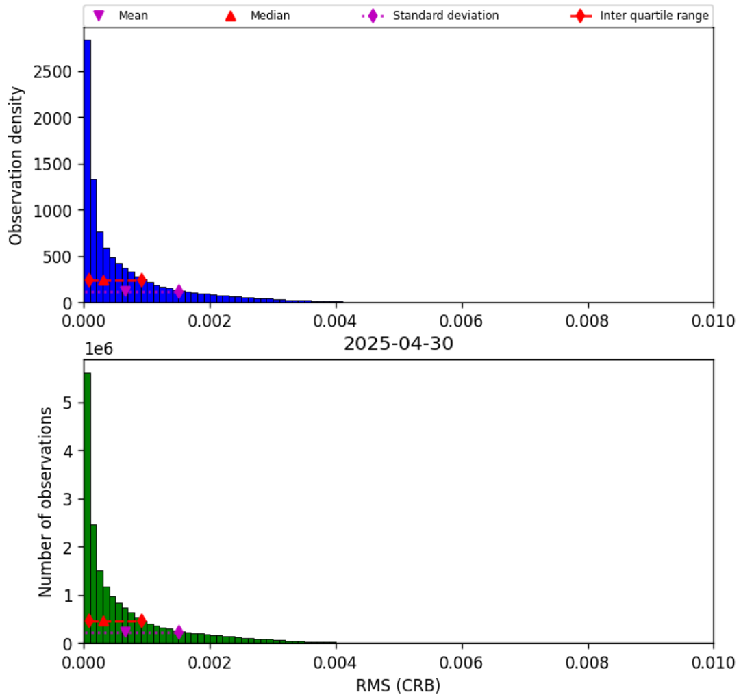
Figure 48: Histogram of “RMS (CRB)” for 2025-04-29 to 2025-05-01
