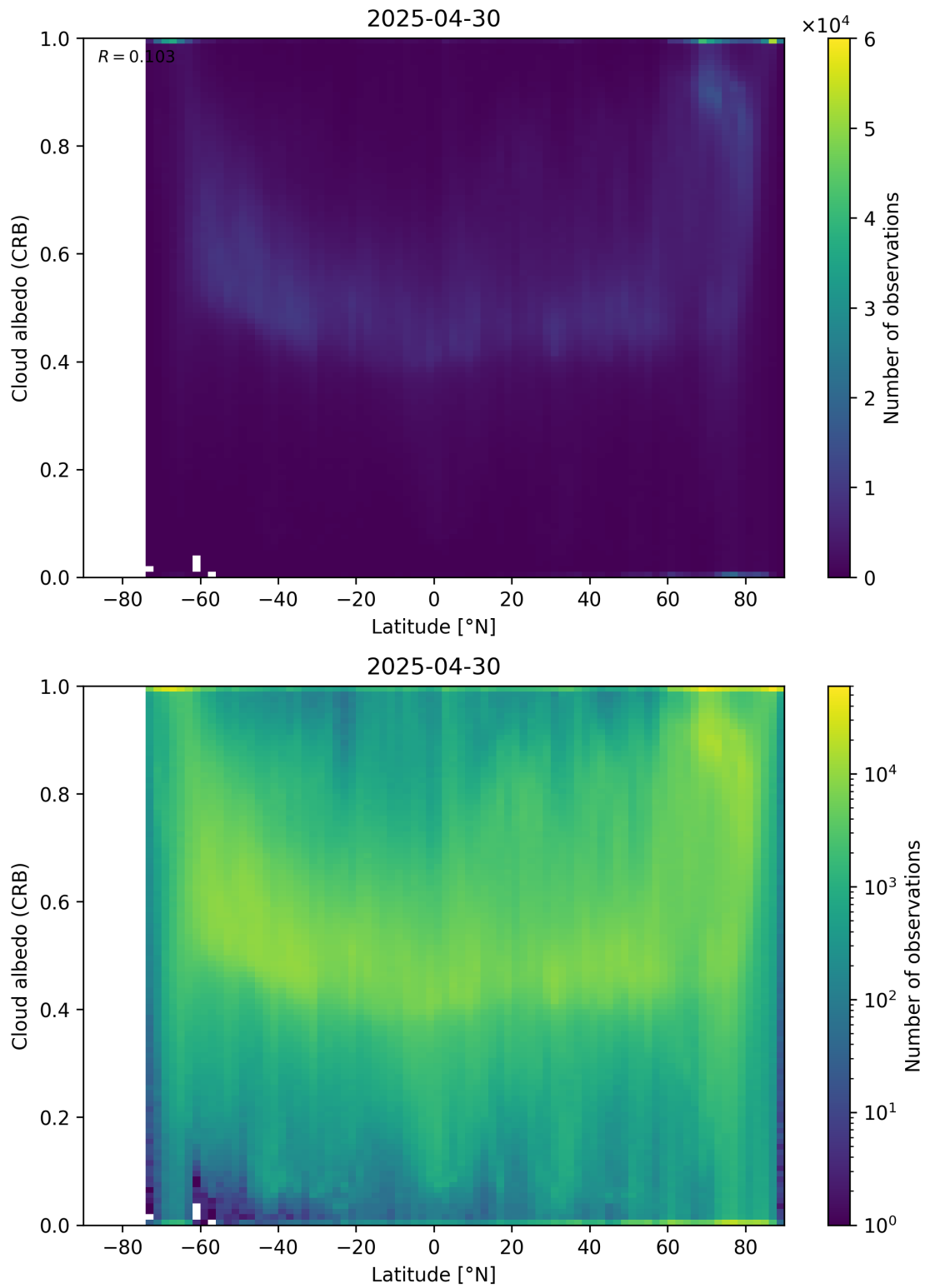
Figure 91: Scatter density plot of “Latitude” against “Cloud albedo (CRB)” for 2025-04-29 to 2025-05-01.
