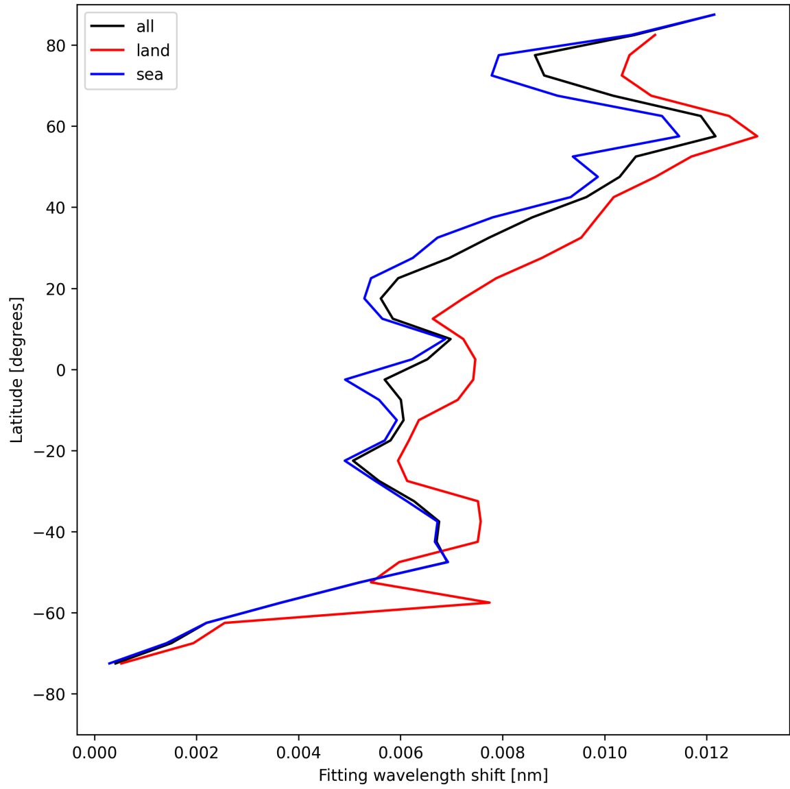
Figure 33: Zonal average of “Fitting wavelength shift” for 2025-04-29 to 2025-05-01.
