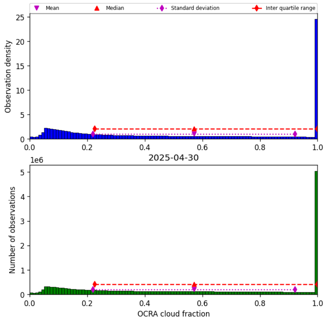
Figure 50: Histogram of “OCRA cloud fraction” for 2025-04-29 to 2025-05-01
