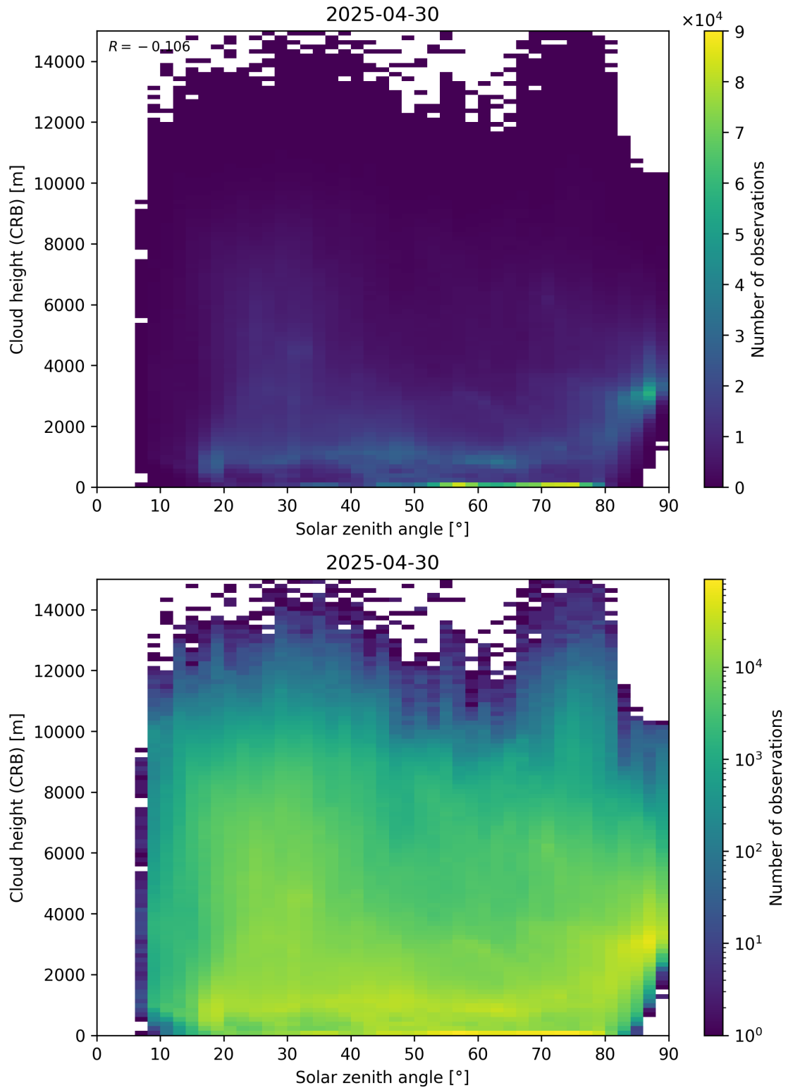
Figure 102: Scatter density plot of “Solar zenith angle” against “Cloud height (CRB)” for 2025-04-29 to 2025-05-01.
