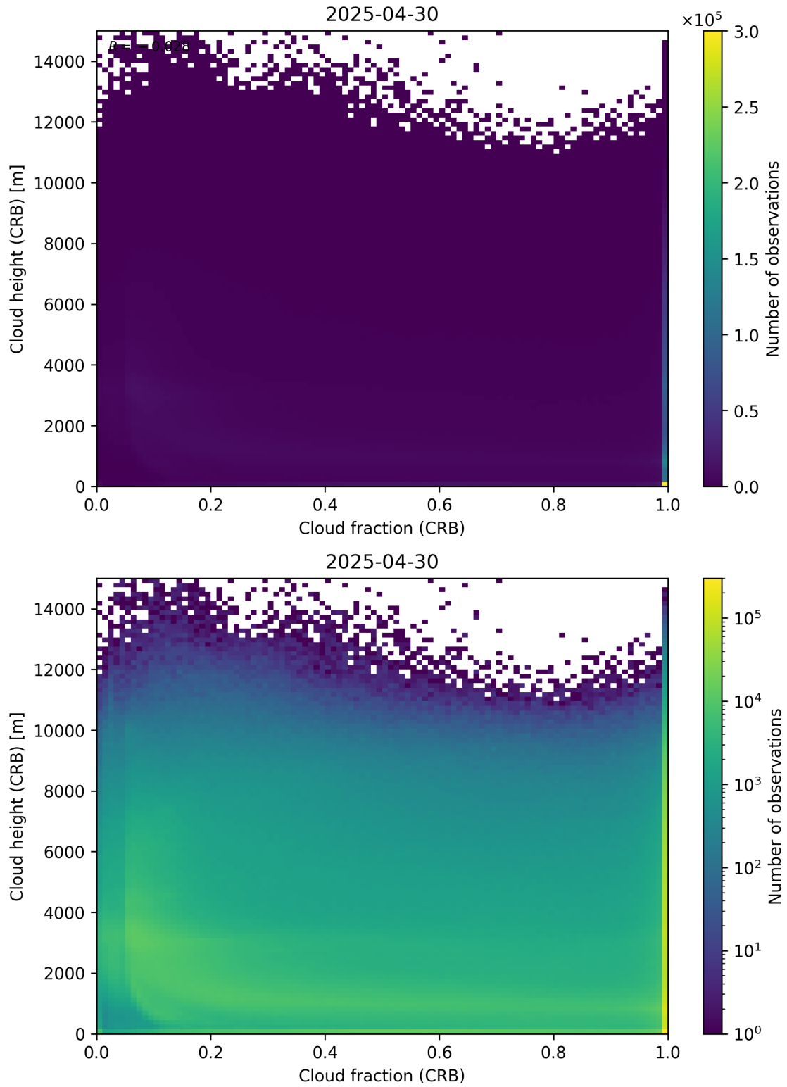
Figure 79: Scatter density plot of “Cloud fraction (CRB)” against “Cloud height (CRB)” for 2025-04-29 to 2025-05-01.
