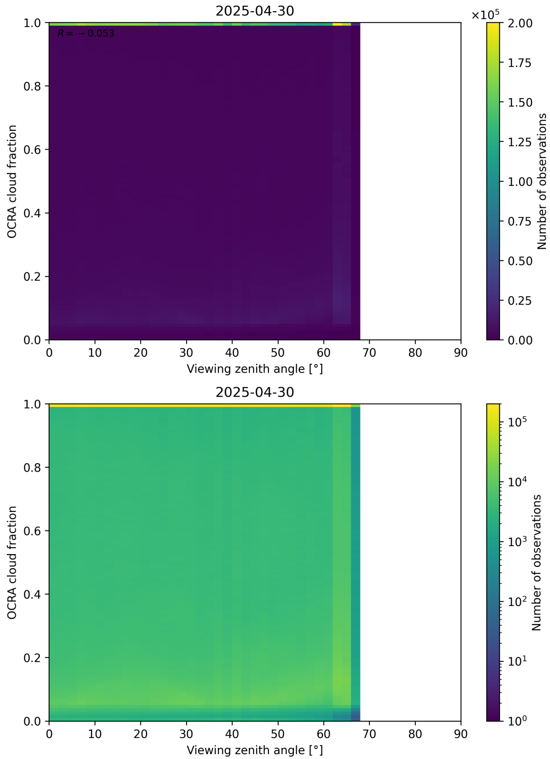
Figure 108: Scatter density plot of “Viewing zenith angle” against “OCRA cloud fraction” for 2025-04-29 to 2025-05-01.
