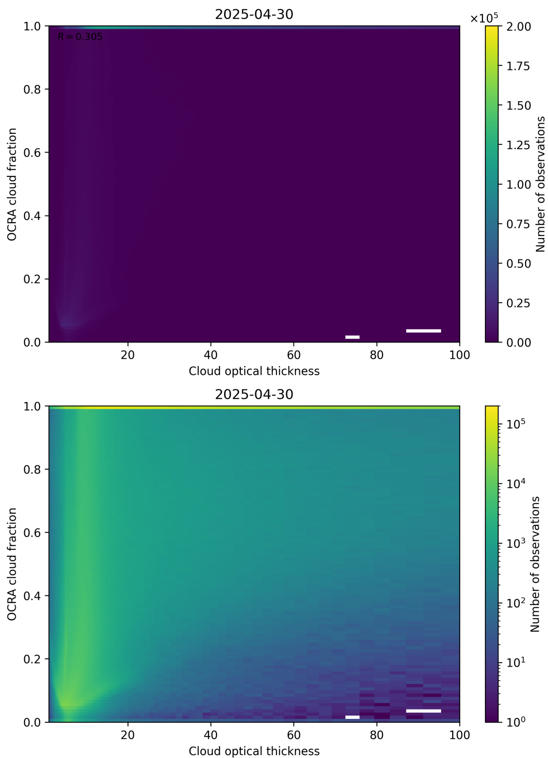
Figure 83: Scatter density plot of “Cloud optical thickness” against “OCRA cloud fraction” for 2025-04-29 to 2025-05-01.
