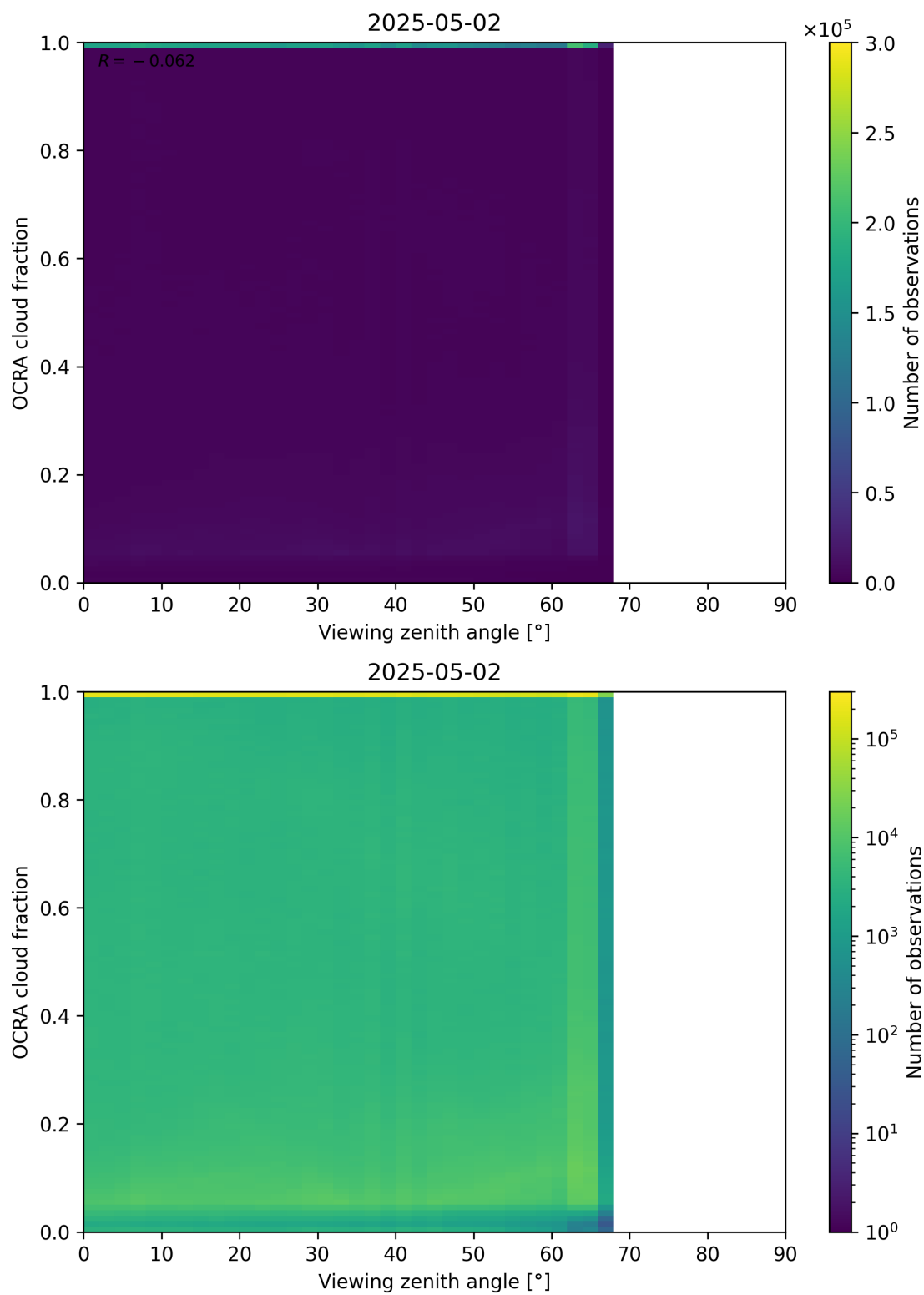
Figure 108: Scatter density plot of “Viewing zenith angle” against “OCRA cloud fraction” for 2025-05-01 to 2025-05-03.
