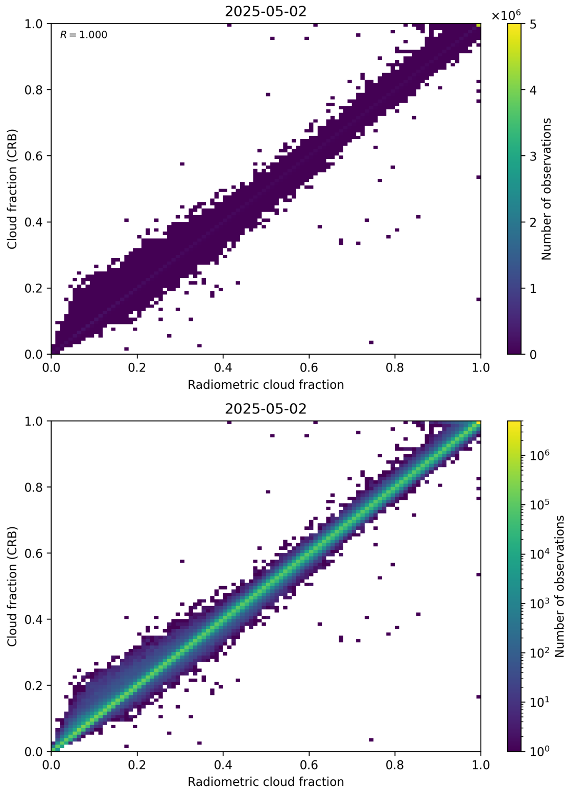
Figure 73: Scatter density plot of “Radiometric cloud fraction” against “Cloud fraction (CRB)” for 2025-05-01 to 2025-05-03.
