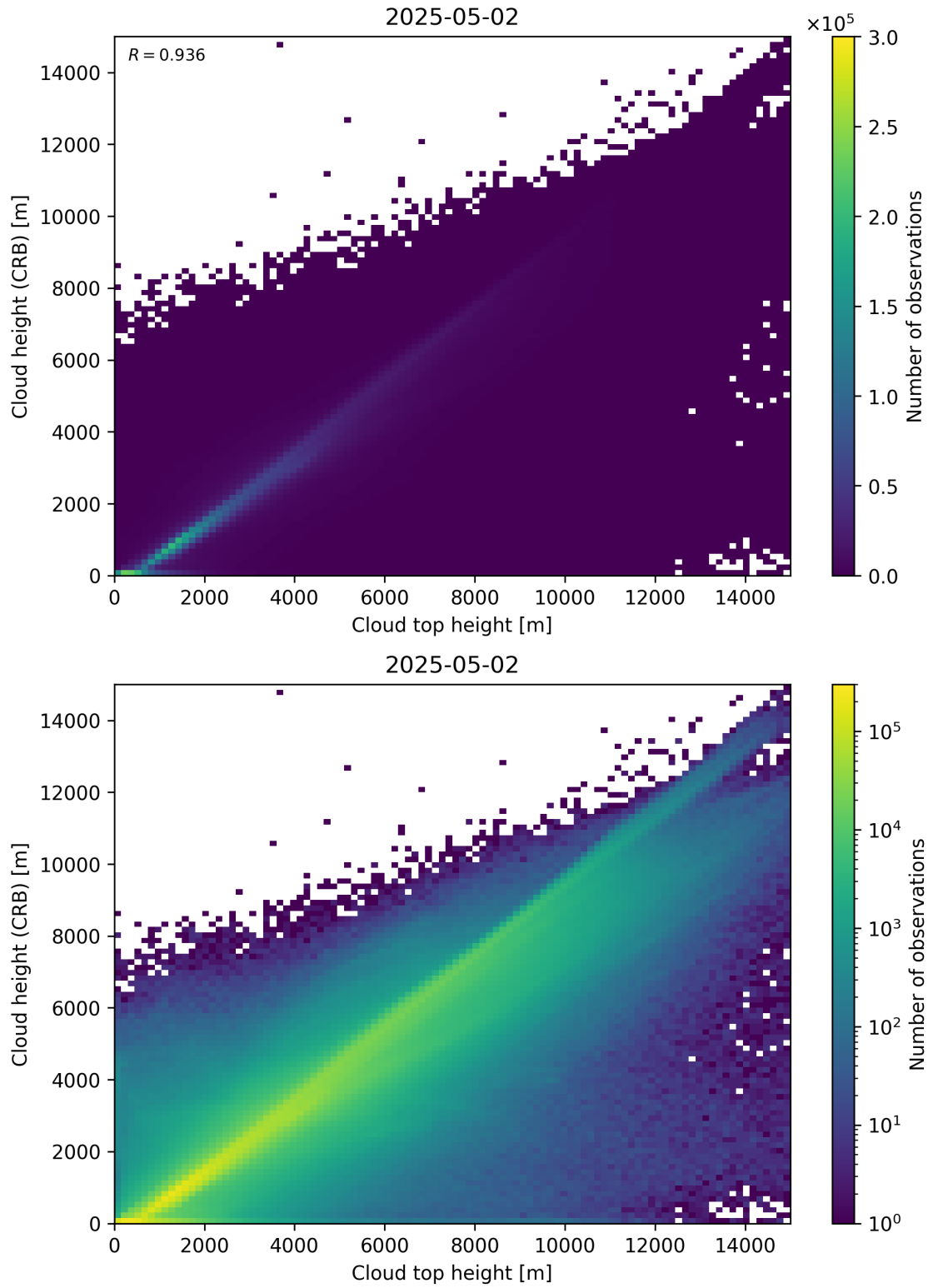
Figure 89: Scatter density plot of “Cloud top height” against “Cloud height (CRB)” for 2025-05-01 to 2025-05-03.
