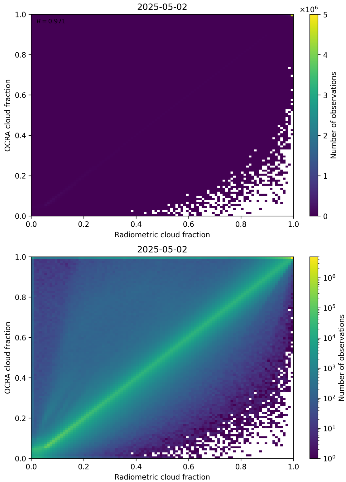
Figure 72: Scatter density plot of “Radiometric cloud fraction” against “OCRA cloud fraction” for 2025-05-01 to 2025-05-03.
