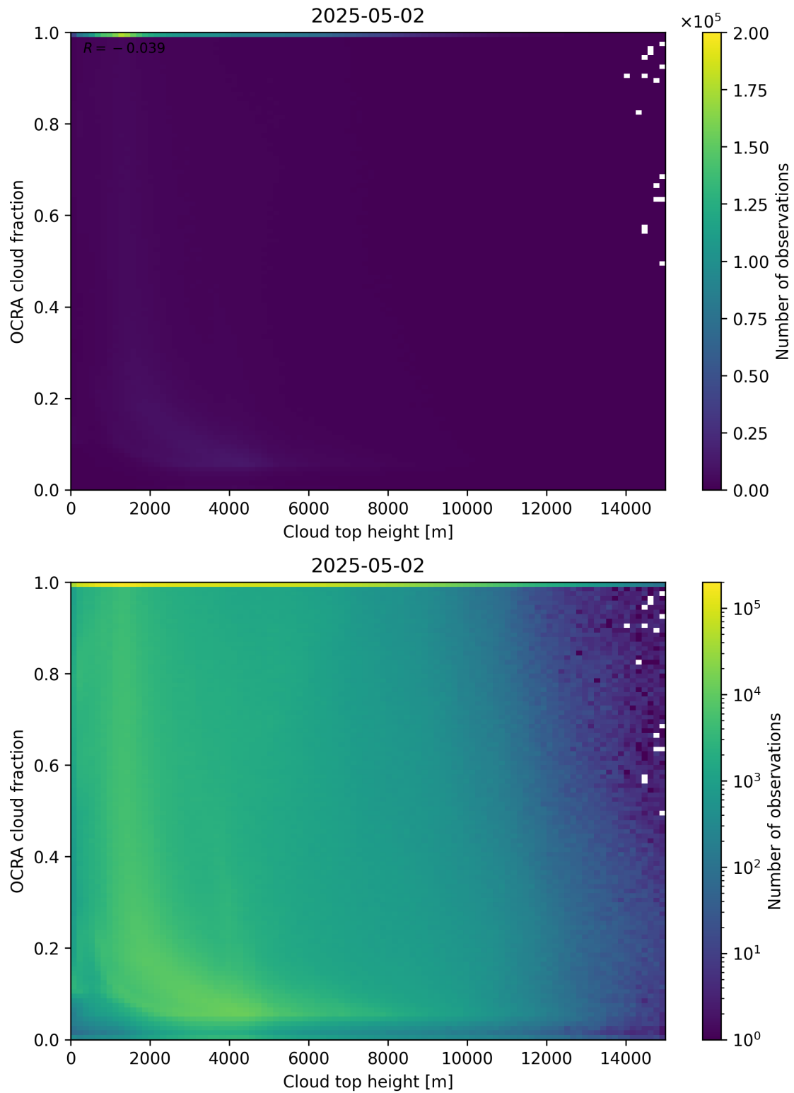
Figure 87: Scatter density plot of “Cloud top height” against “OCRA cloud fraction” for 2025-05-01 to 2025-05-03.
