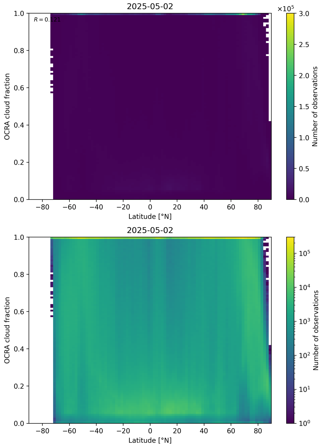
Figure 93: Scatter density plot of “Latitude” against “OCRA cloud fraction” for 2025-05-01 to 2025-05-03.
