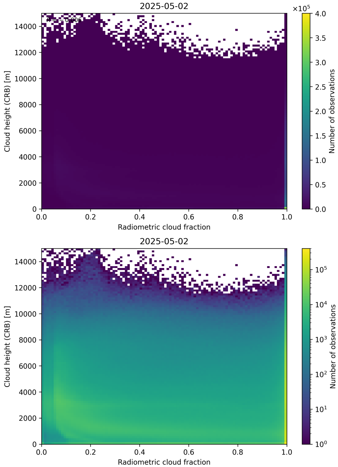
Figure 74: Scatter density plot of “Radiometric cloud fraction” against “Cloud height (CRB)” for 2025-05-01 to 2025-05-03.
