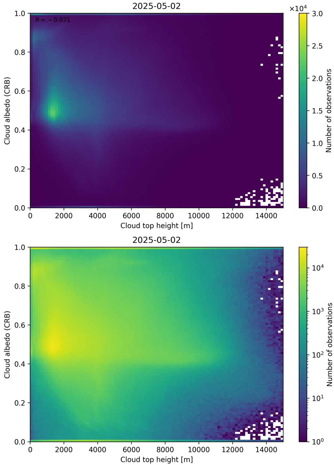
Figure 86: Scatter density plot of “Cloud top height” against “Cloud albedo (CRB)” for 2025-05-01 to 2025-05-03.
