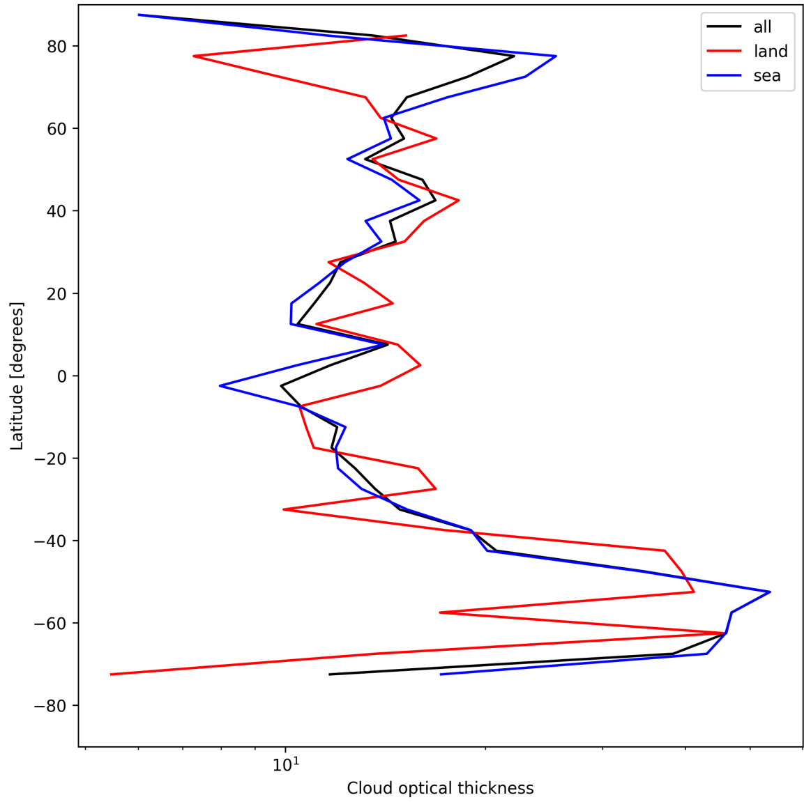
Figure 25: Zonal average of “Cloud optical thickness” for 2025-05-01 to 2025-05-03.
