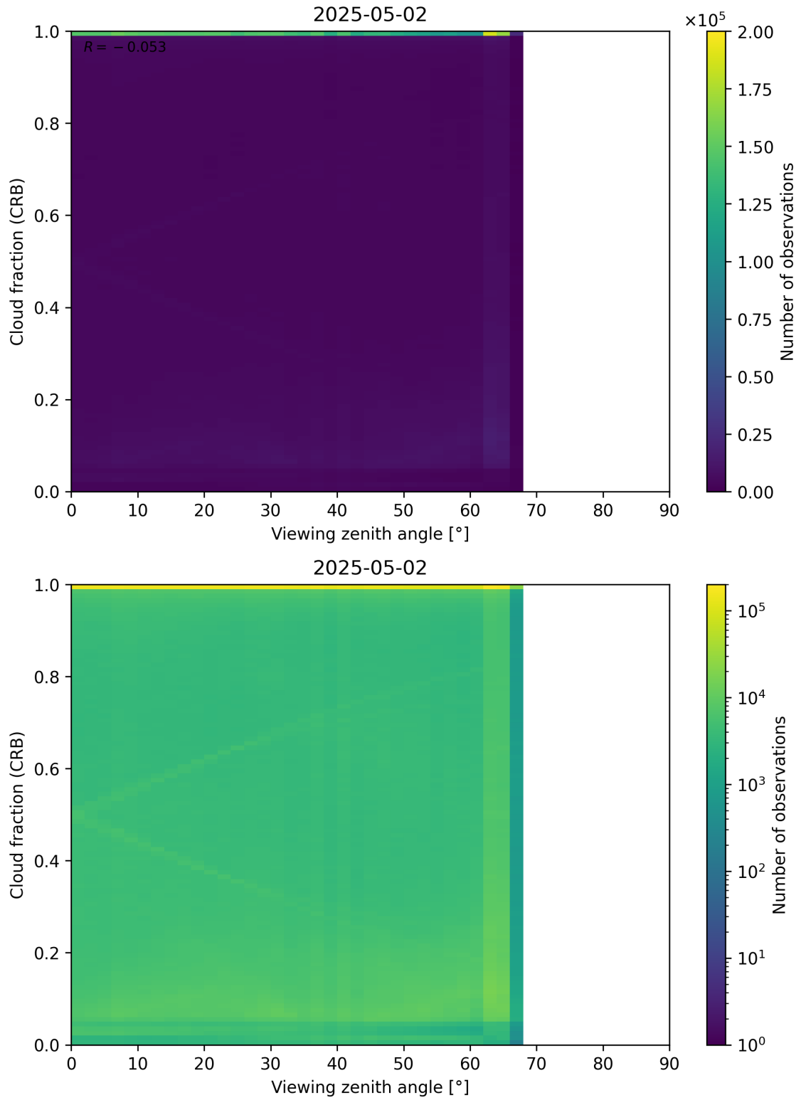
Figure 109: Scatter density plot of “Viewing zenith angle” against “Cloud fraction (CRB)” for 2025-05-01 to 2025-05-03.
