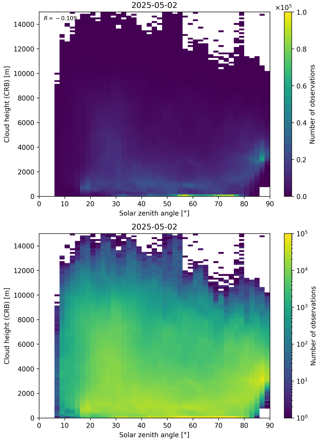
Figure 102: Scatter density plot of “Solar zenith angle” against “Cloud height (CRB)” for 2025-05-01 to 2025-05-03.
