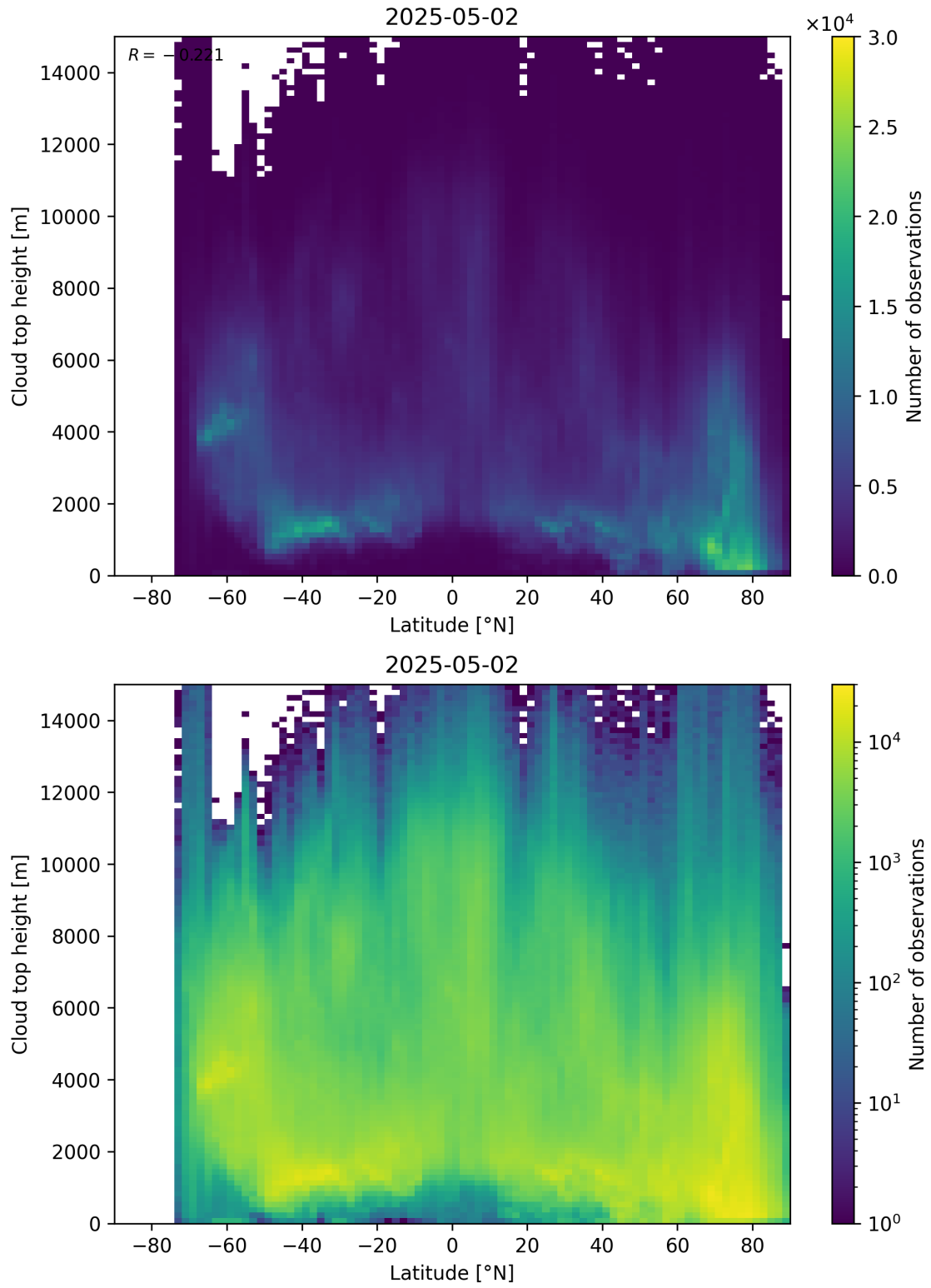
Figure 97: Scatter density plot of “Latitude” against “Cloud top height” for 2025-05-01 to 2025-05-03.
