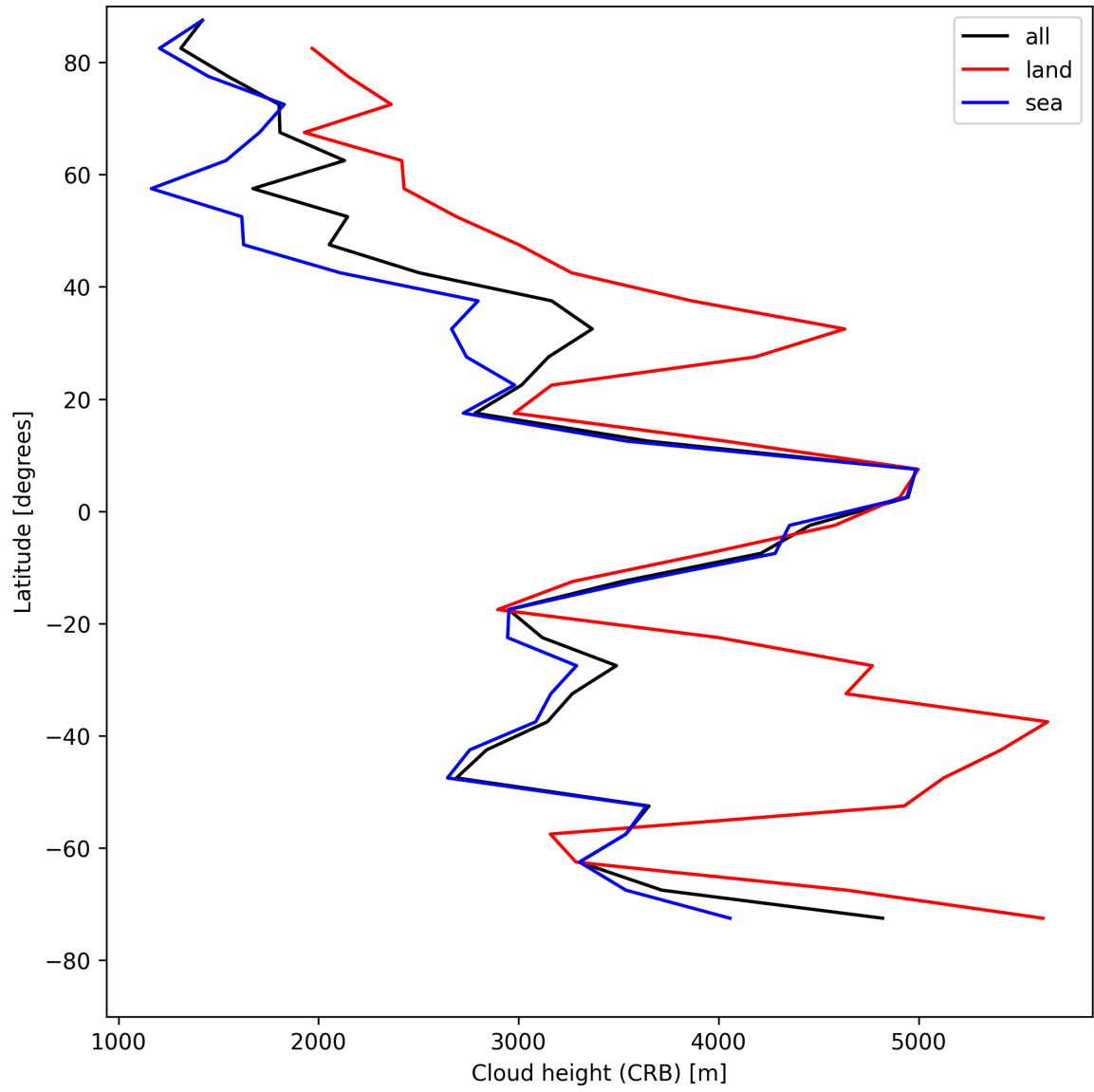
Figure 27: Zonal average of “Cloud height (CRB)” for 2025-05-01 to 2025-05-03.
