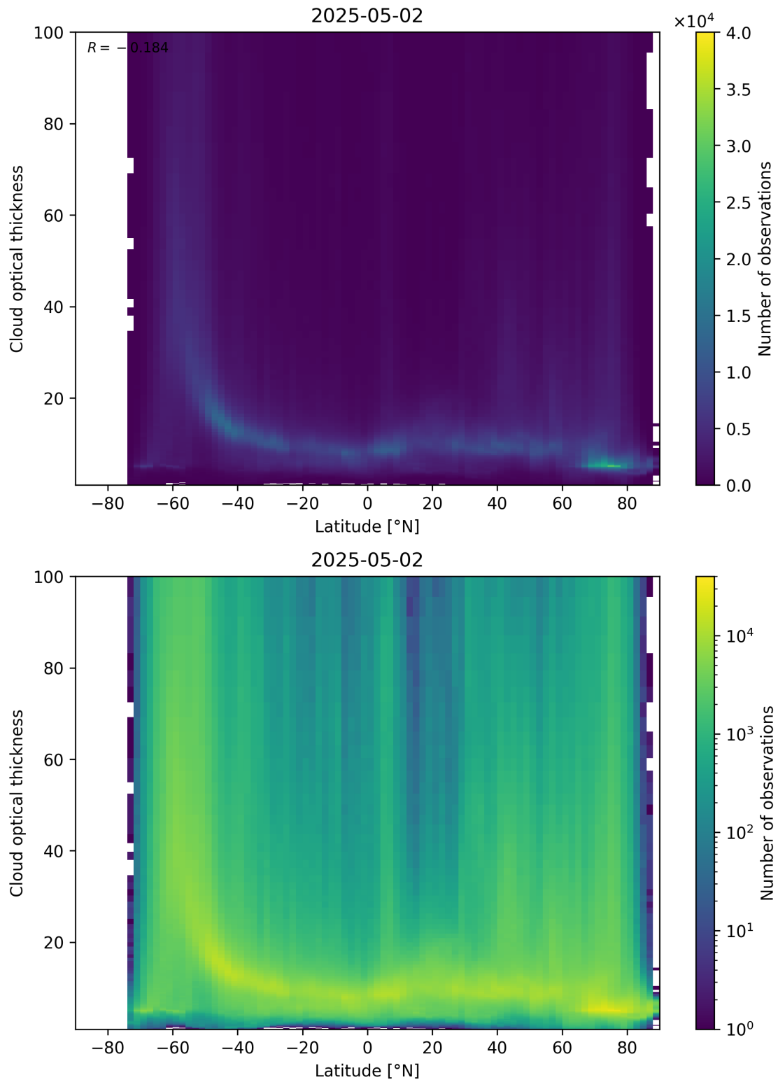
Figure 96: Scatter density plot of “Latitude” against “Cloud optical thickness” for 2025-05-01 to 2025-05-03.
