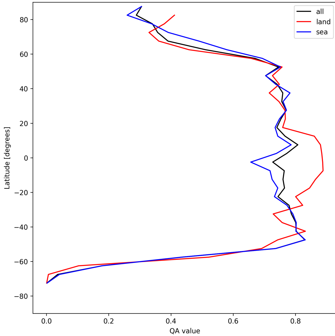
Figure 22: Zonal average of “QA value” for 2025-05-01 to 2025-05-03.
