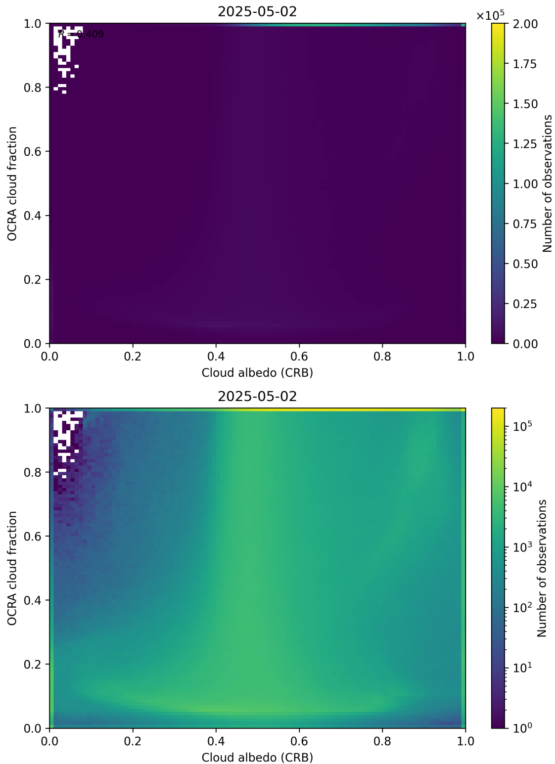
Figure 70: Scatter density plot of “Cloud albedo (CRB)” against “OCRA cloud fraction” for 2025-05-01 to 2025-05-03.
