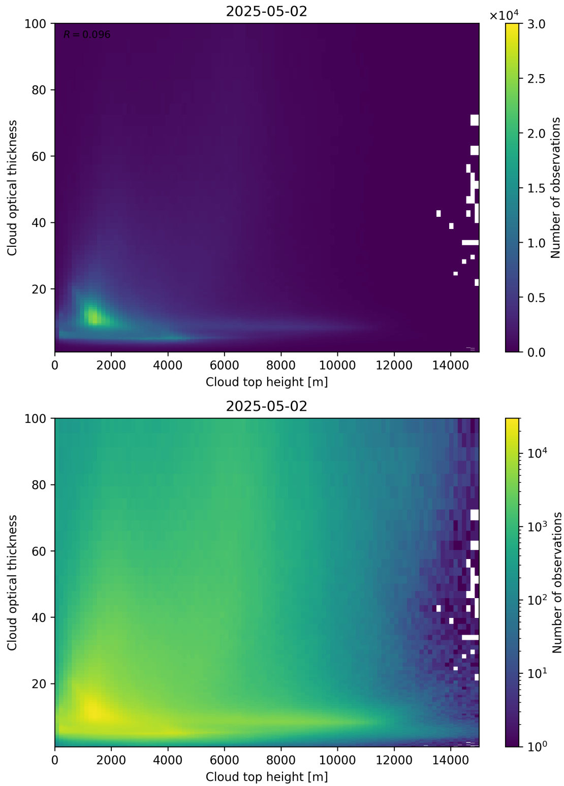
Figure 90: Scatter density plot of “Cloud top height” against “Cloud optical thickness” for 2025-05-01 to 2025-05-03.
