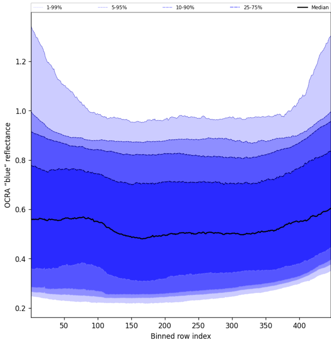
Figure 67: Along track statistics of “OCRA “blue” reflectance” for 2025-05-01 to 2025-05-03
