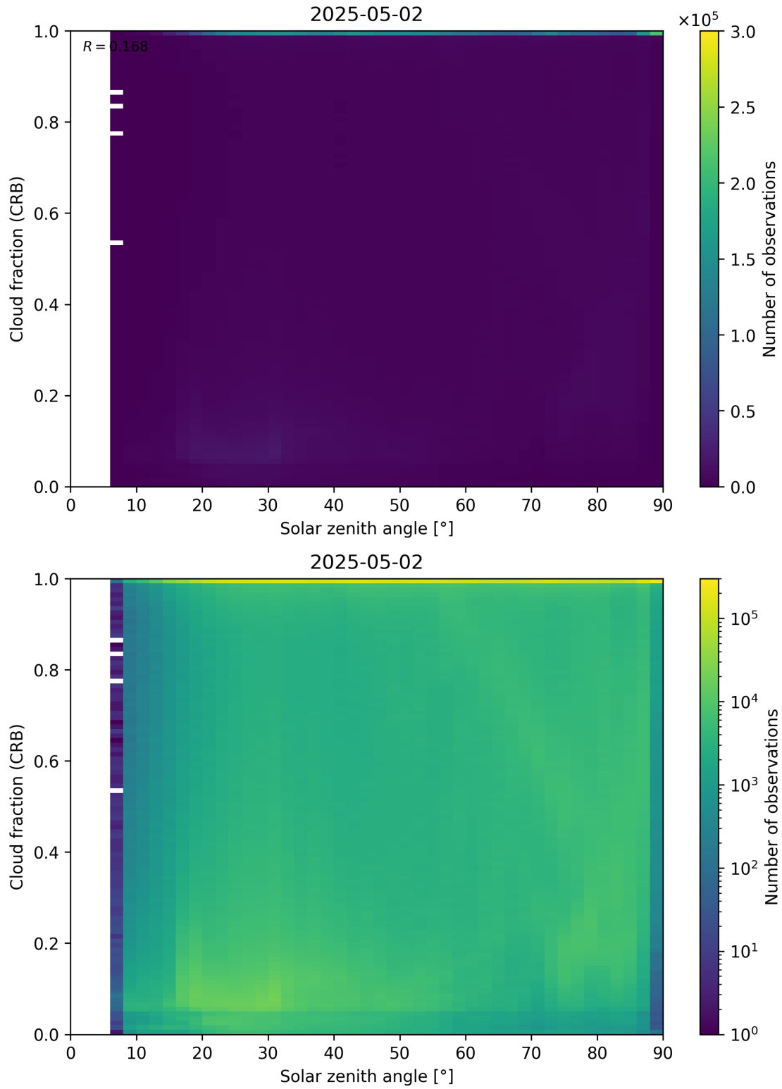
Figure 101: Scatter density plot of “Solar zenith angle” against “Cloud fraction (CRB)” for 2025-05-01 to 2025-05-03.
