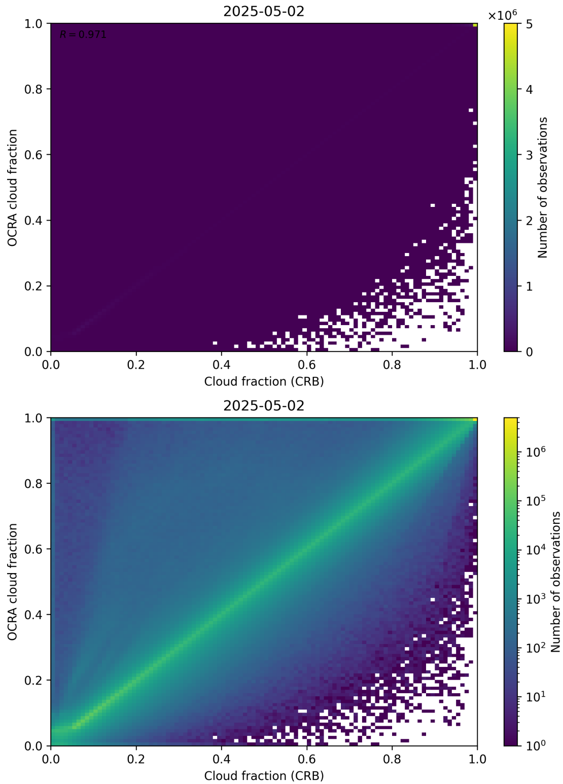
Figure 78: Scatter density plot of “Cloud fraction (CRB)” against “OCRA cloud fraction” for 2025-05-01 to 2025-05-03.
