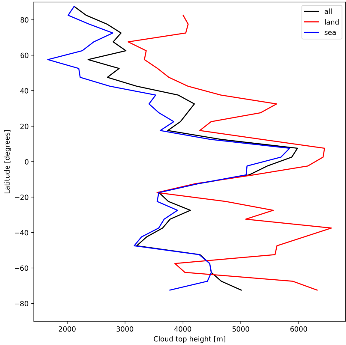
Figure 24: Zonal average of “Cloud top height” for 2025-05-01 to 2025-05-03.
