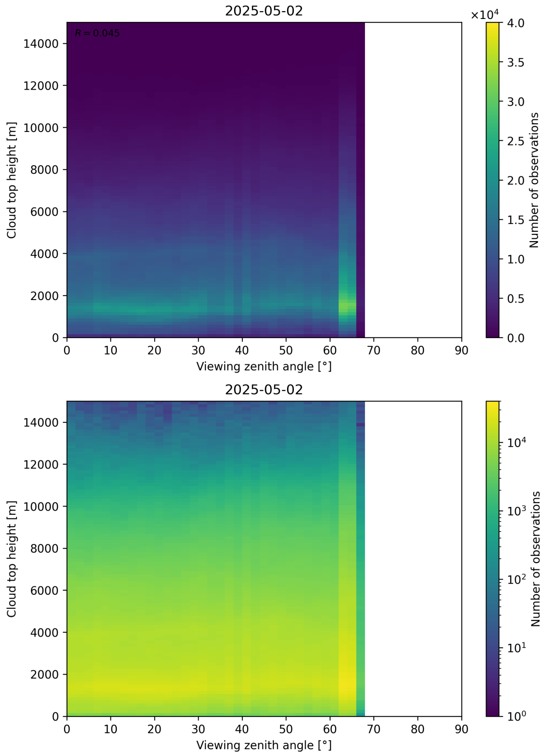
Figure 112: Scatter density plot of “Viewing zenith angle” against “Cloud top height” for 2025-05-01 to 2025-05-03.
