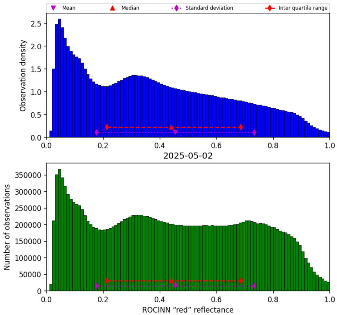
Figure 53: Histogram of “ROCINN “red” reflectance” for 2025-05-01 to 2025-05-03
