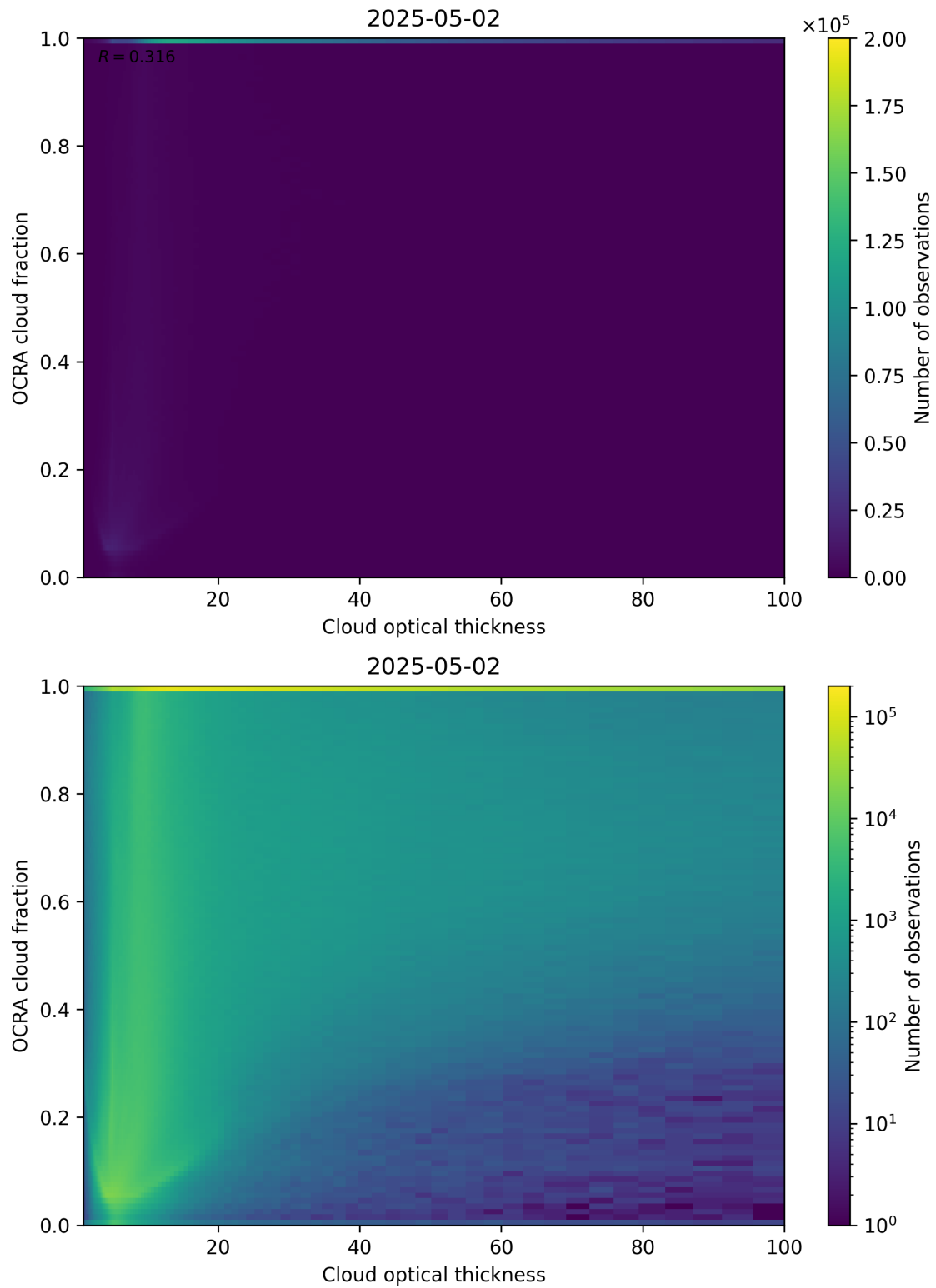
Figure 83: Scatter density plot of “Cloud optical thickness” against “OCRA cloud fraction” for 2025-05-01 to 2025-05-03.
