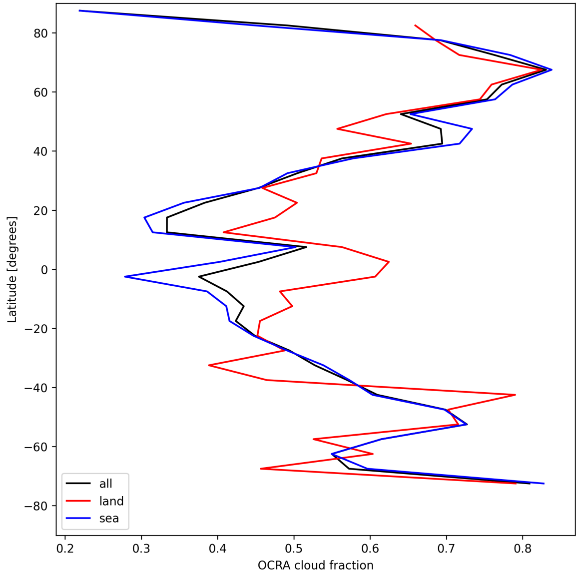
Figure 34: Zonal average of “OCRA cloud fraction” for 2025-05-01 to 2025-05-03.
