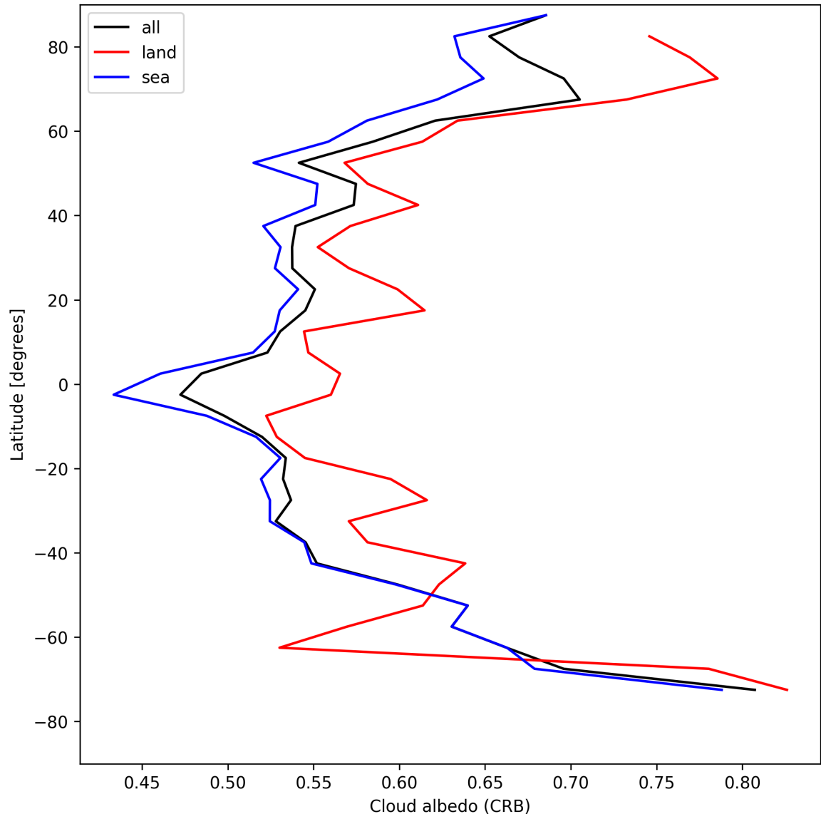
Figure 28: Zonal average of “Cloud albedo (CRB)” for 2025-05-01 to 2025-05-03.
