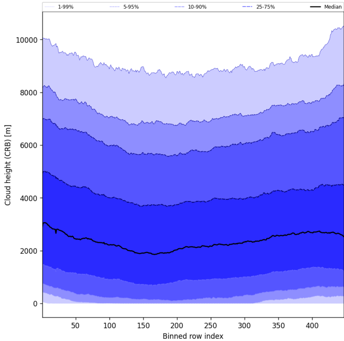
Figure 59: Along track statistics of “Cloud height (CRB)” for 2025-05-01 to 2025-05-03
