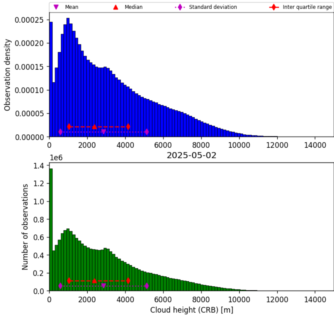
Figure 43: Histogram of “Cloud height (CRB)” for 2025-05-01 to 2025-05-03
