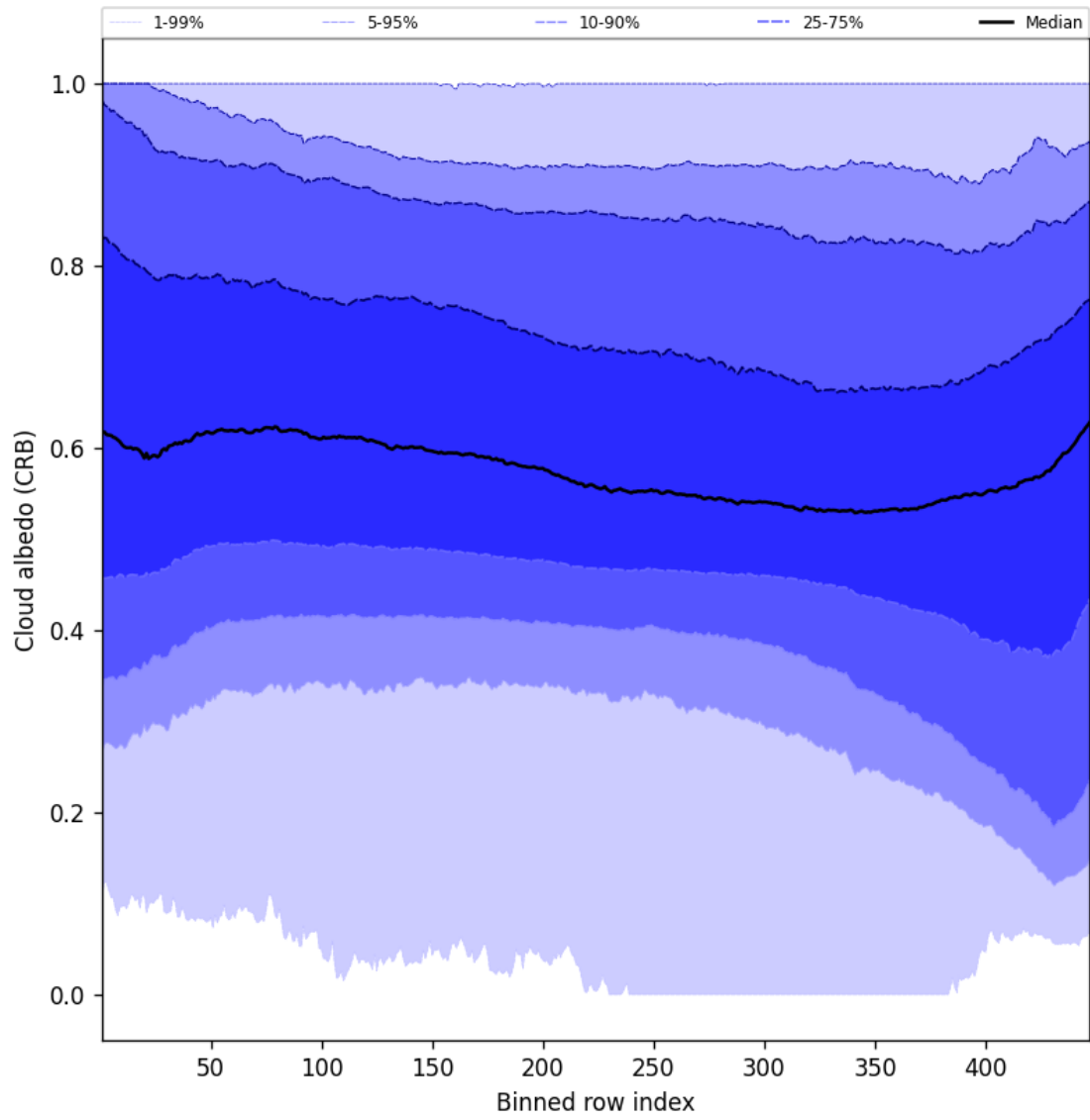
Figure 60: Along track statistics of “Cloud albedo (CRB)” for 2025-05-01 to 2025-05-03
