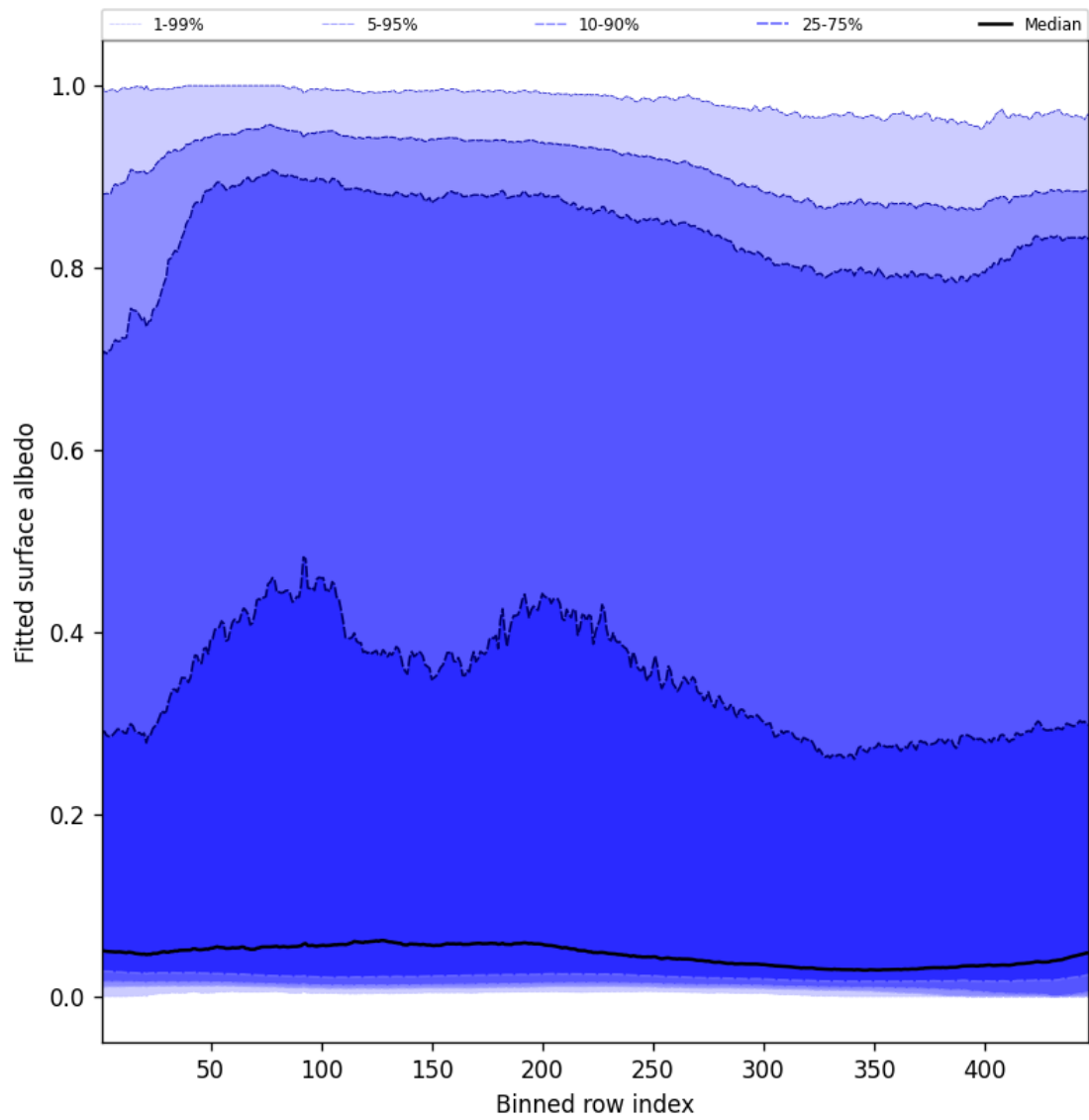
Figure 61: Along track statistics of “Fitted surface albedo” for 2025-05-01 to 2025-05-03
