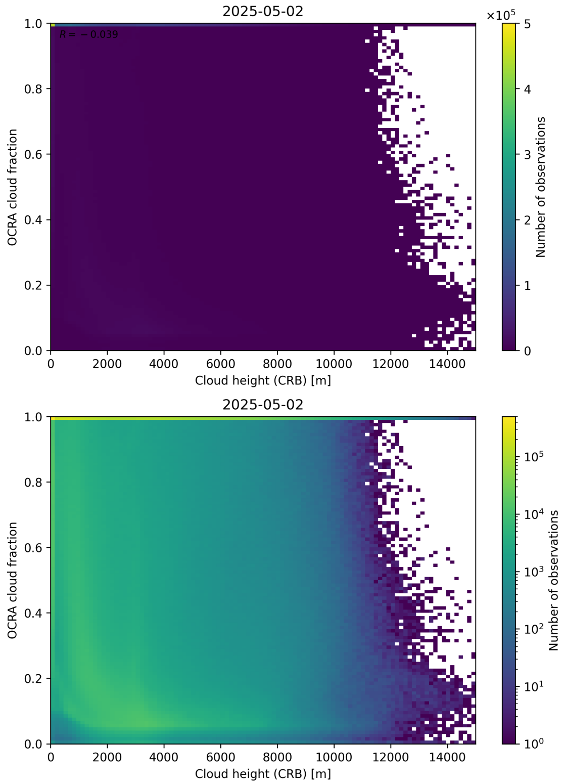
Figure 81: Scatter density plot of “Cloud height (CRB)” against “OCRA cloud fraction” for 2025-05-01 to 2025-05-03.
