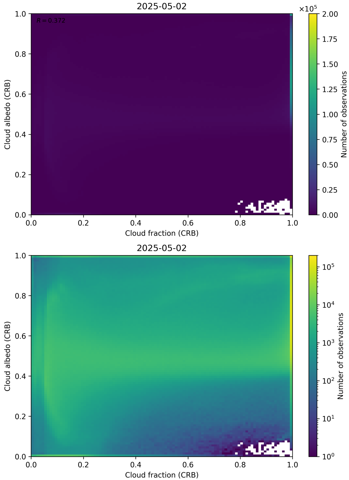
Figure 77: Scatter density plot of “Cloud fraction (CRB)” against “Cloud albedo (CRB)” for 2025-05-01 to 2025-05-03.
