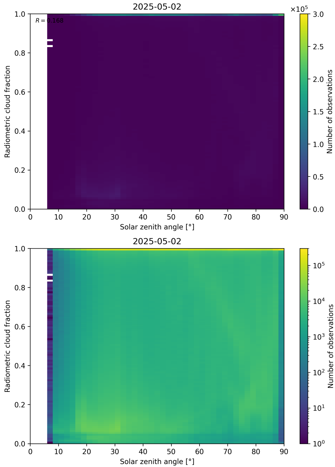
Figure 99: Scatter density plot of “Solar zenith angle” against “Radiometric cloud fraction” for 2025-05-01 to 2025-05-03.
