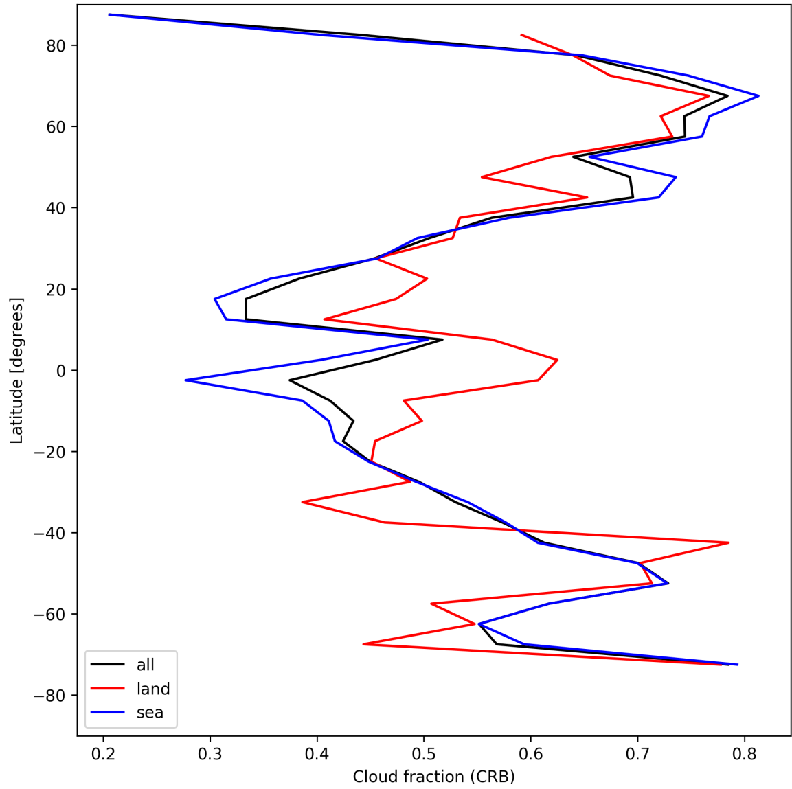
Figure 26: Zonal average of “Cloud fraction (CRB)” for 2025-05-01 to 2025-05-03.
