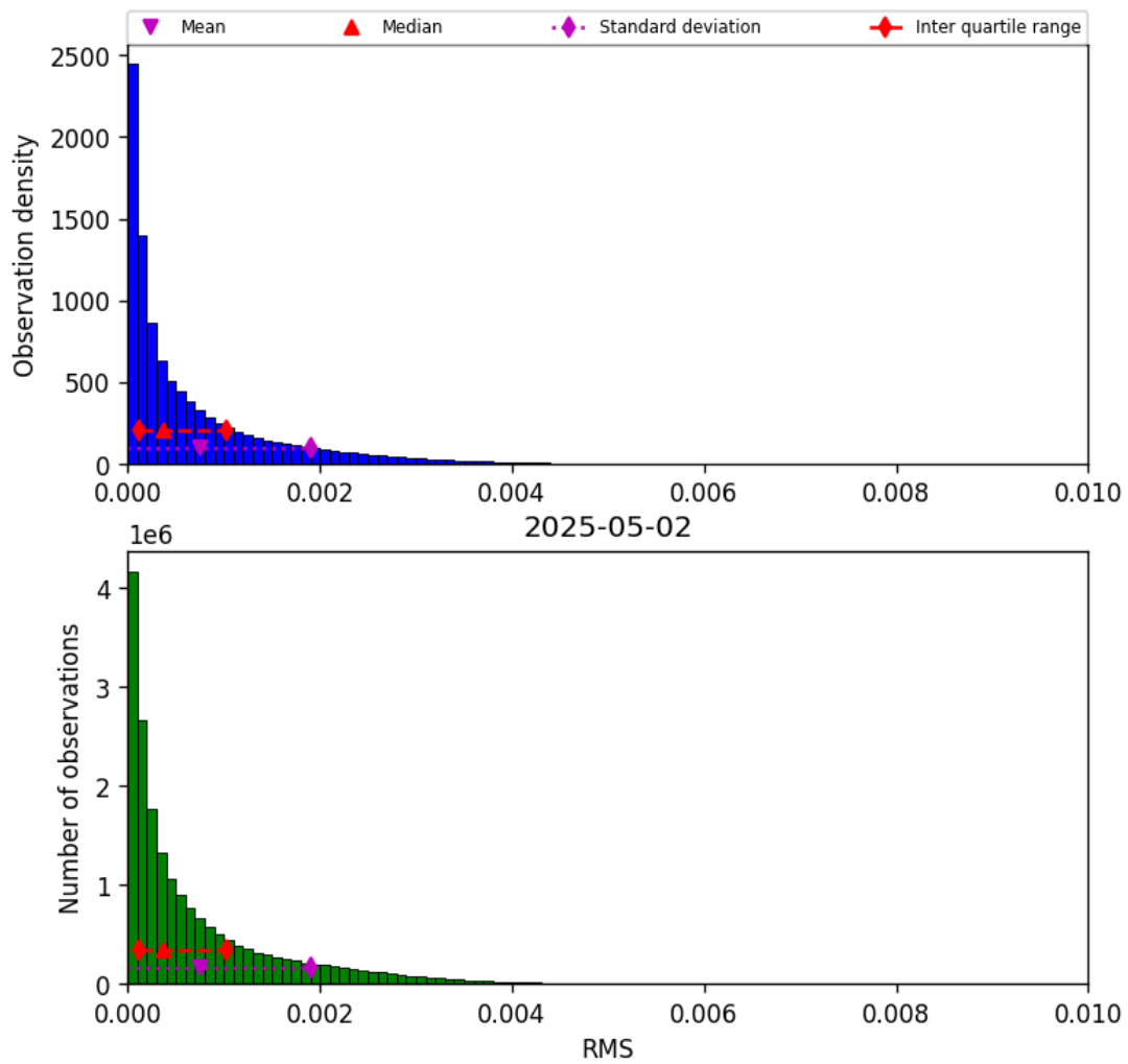
Figure 47: Histogram of “RMS” for 2025-05-01 to 2025-05-03
