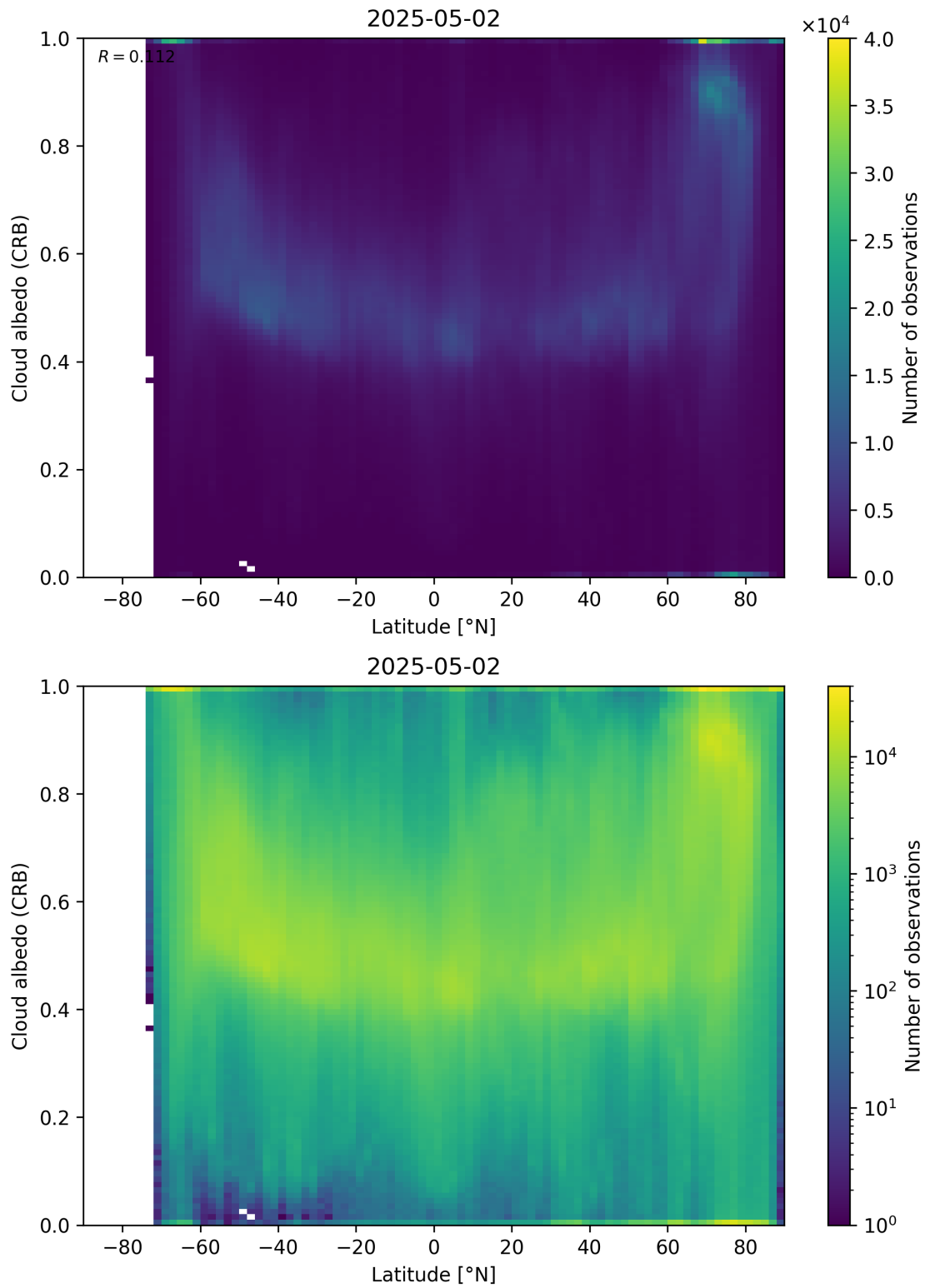
Figure 91: Scatter density plot of “Latitude” against “Cloud albedo (CRB)” for 2025-05-01 to 2025-05-03.
