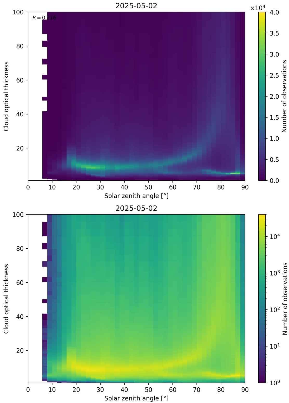
Figure 103: Scatter density plot of “Solar zenith angle” against “Cloud optical thickness” for 2025-05-01 to 2025-05-03.
