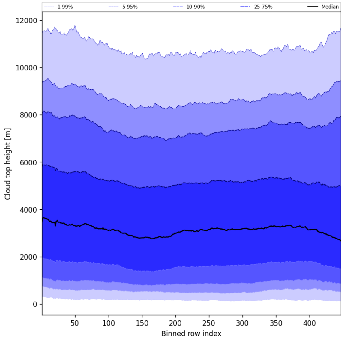
Figure 56: Along track statistics of “Cloud top height” for 2025-05-01 to 2025-05-03
