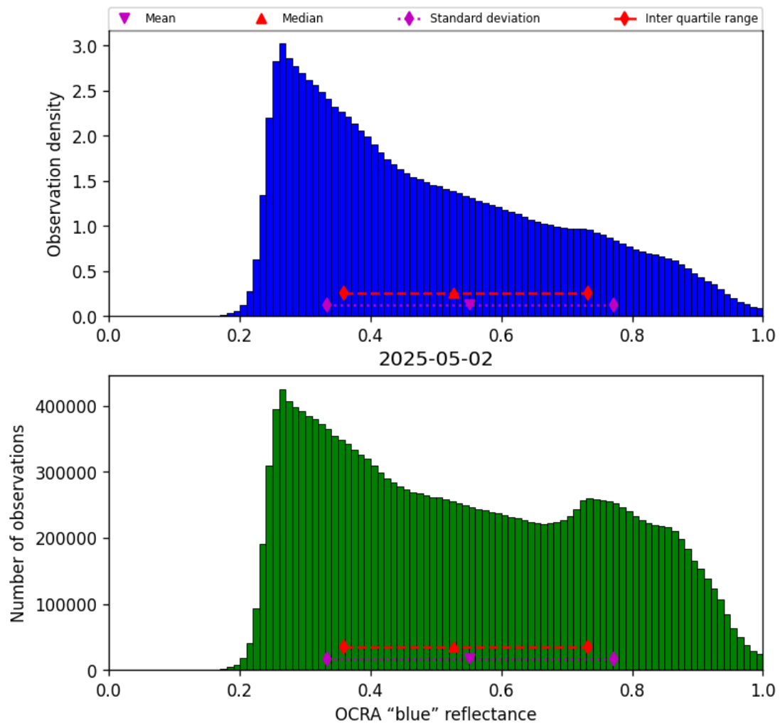
Figure 51: Histogram of “OCRA “blue” reflectance” for 2025-05-01 to 2025-05-03
