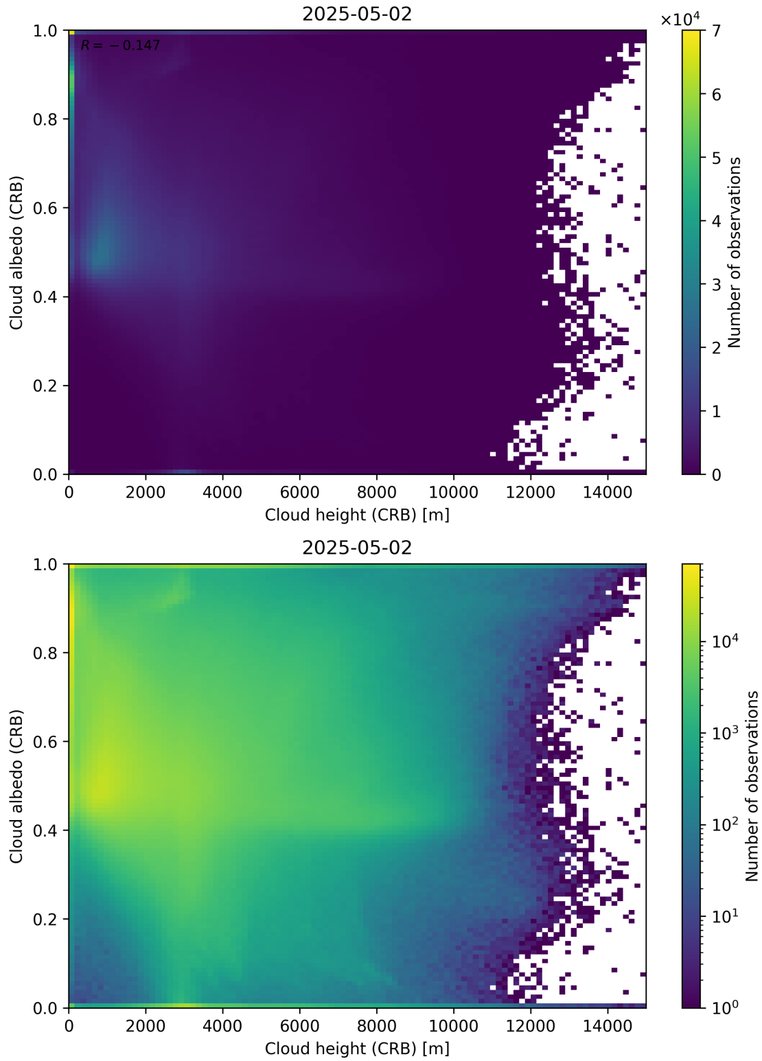
Figure 80: Scatter density plot of “Cloud height (CRB)” against “Cloud albedo (CRB)” for 2025-05-01 to 2025-05-03.
