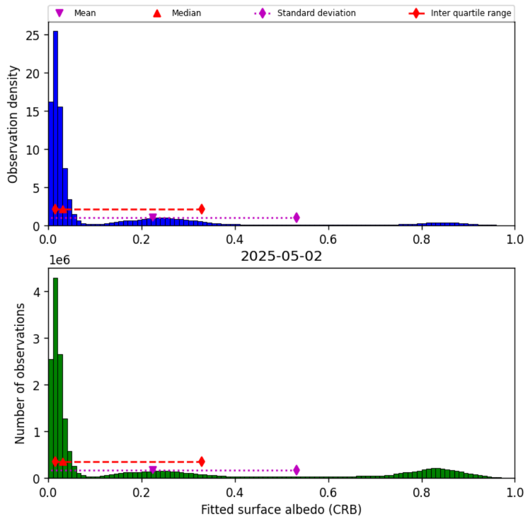
Figure 46: Histogram of “Fitted surface albedo (CRB)” for 2025-05-01 to 2025-05-03
