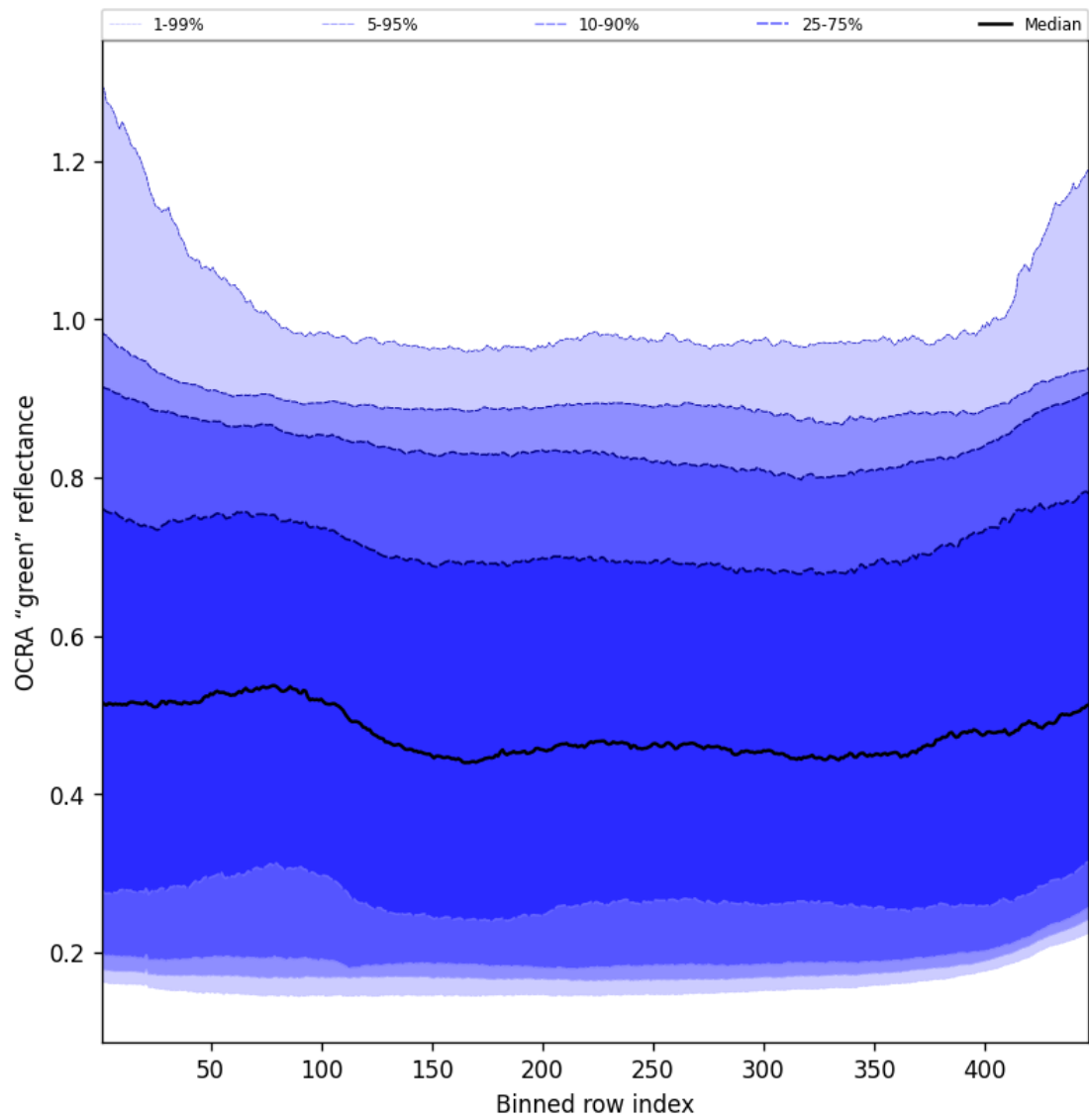
Figure 68: Along track statistics of “OCRA “green” reflectance” for 2025-05-01 to 2025-05-03
