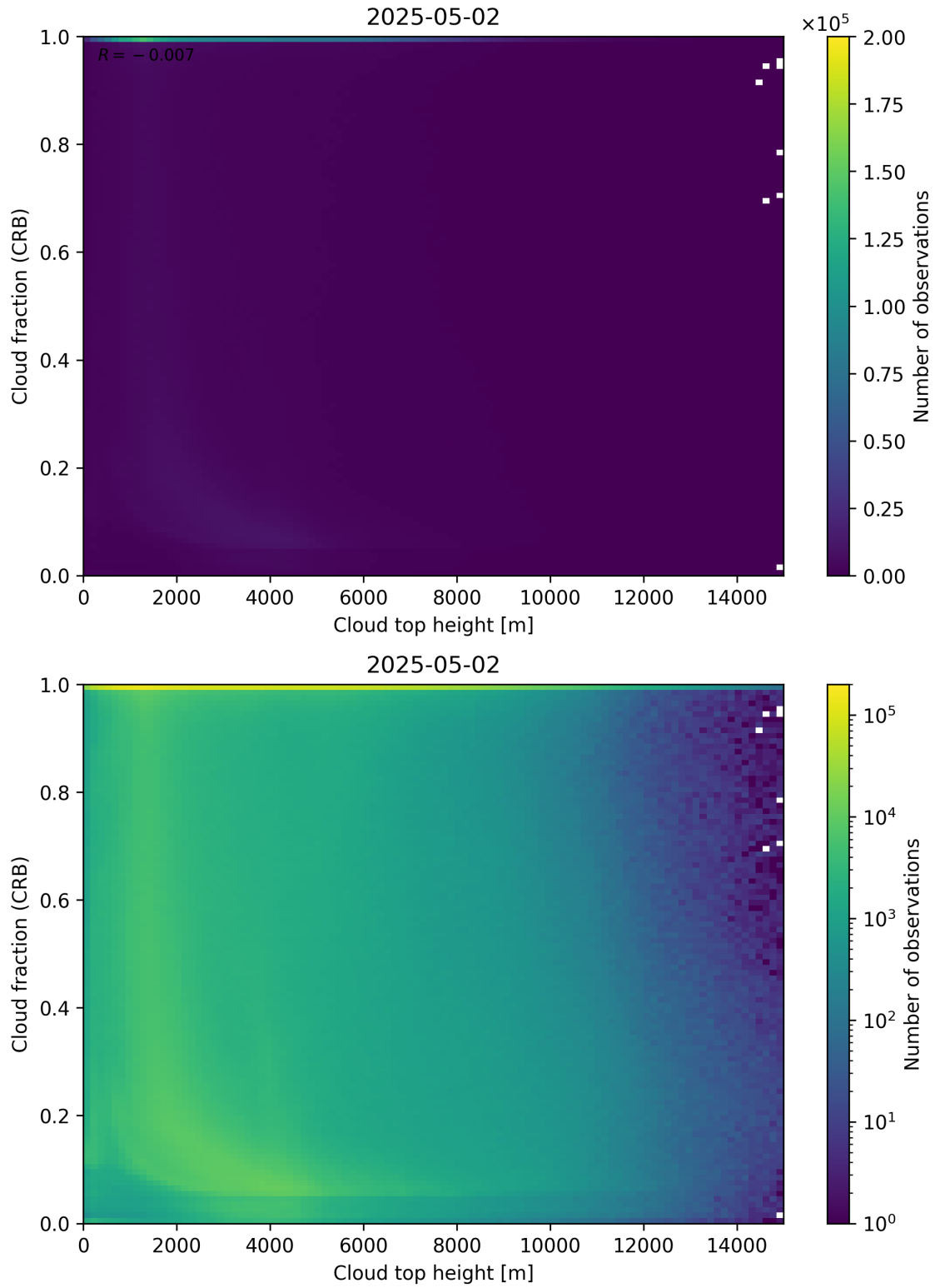
Figure 88: Scatter density plot of “Cloud top height” against “Cloud fraction (CRB)” for 2025-05-01 to 2025-05-03.
