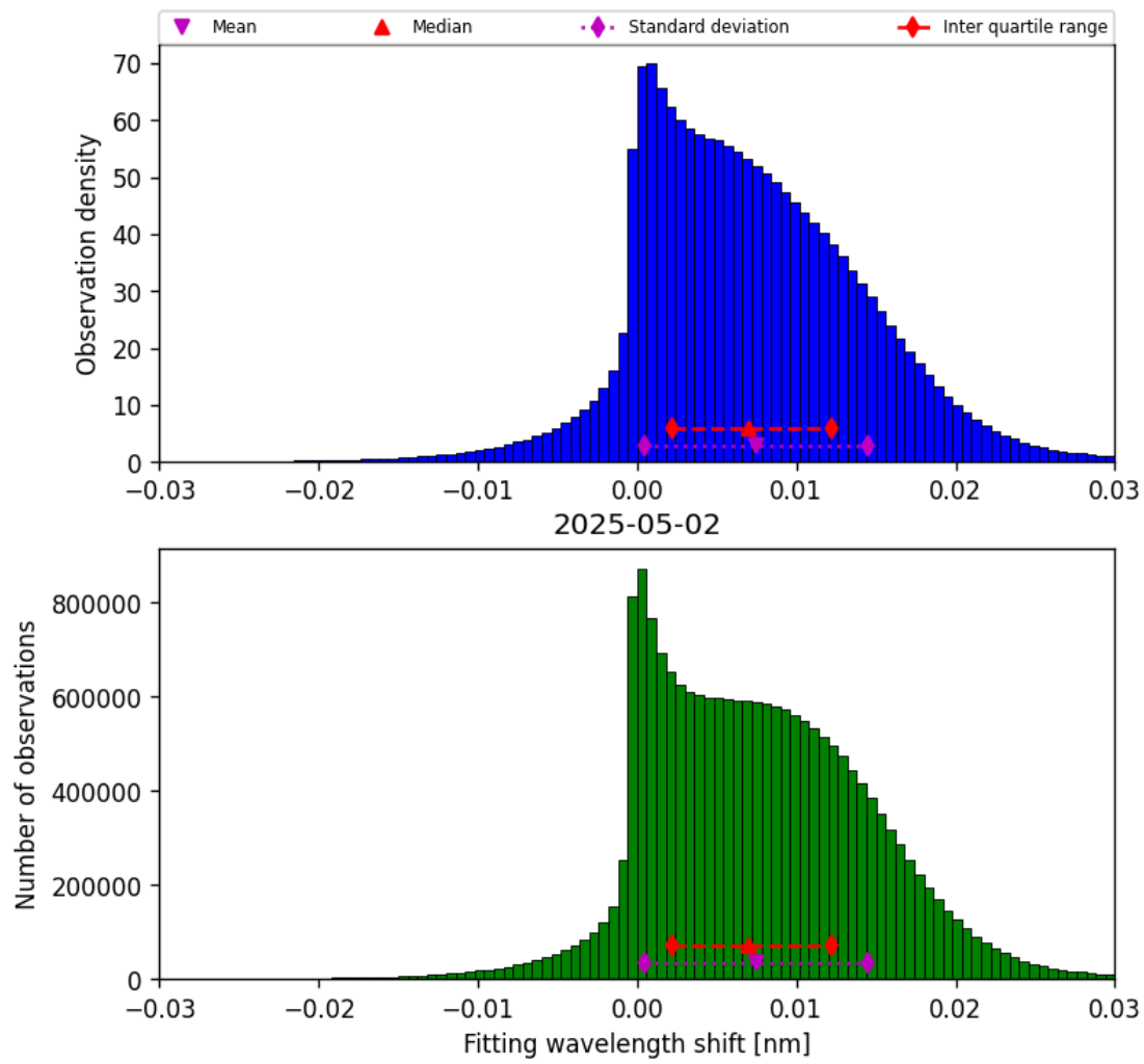
Figure 49: Histogram of “Fitting wavelength shift” for 2025-05-01 to 2025-05-03
