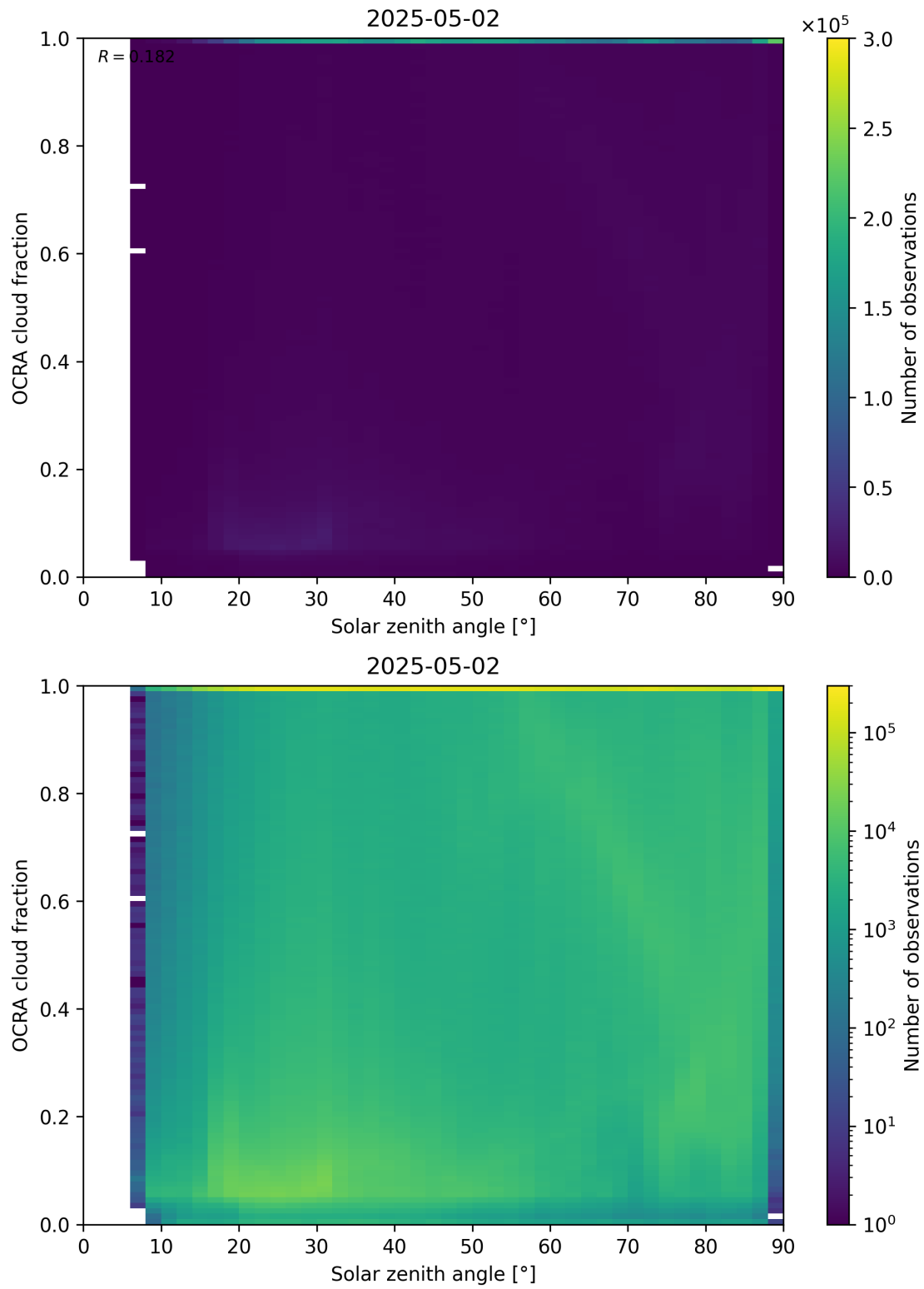
Figure 100: Scatter density plot of “Solar zenith angle” against “OCRA cloud fraction” for 2025-05-01 to 2025-05-03.
