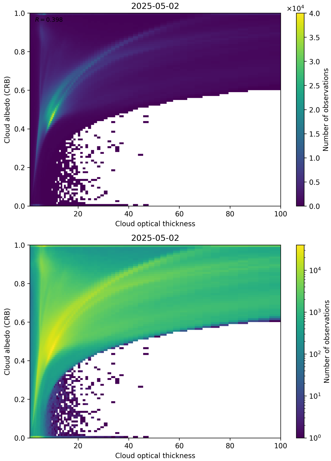
Figure 82: Scatter density plot of “Cloud optical thickness” against “Cloud albedo (CRB)” for 2025-05-01 to 2025-05-03.
