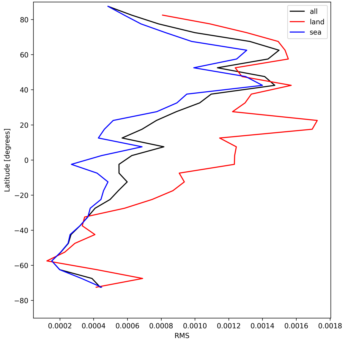
Figure 31: Zonal average of “RMS” for 2025-05-01 to 2025-05-03.
