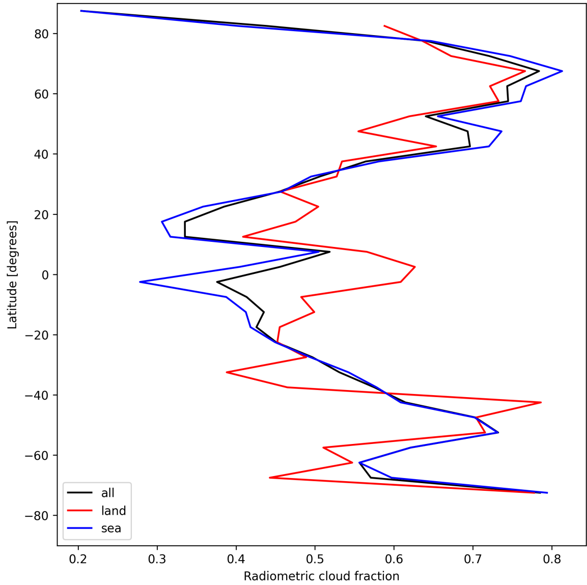
Figure 23: Zonal average of “Radiometric cloud fraction” for 2025-05-01 to 2025-05-03.
