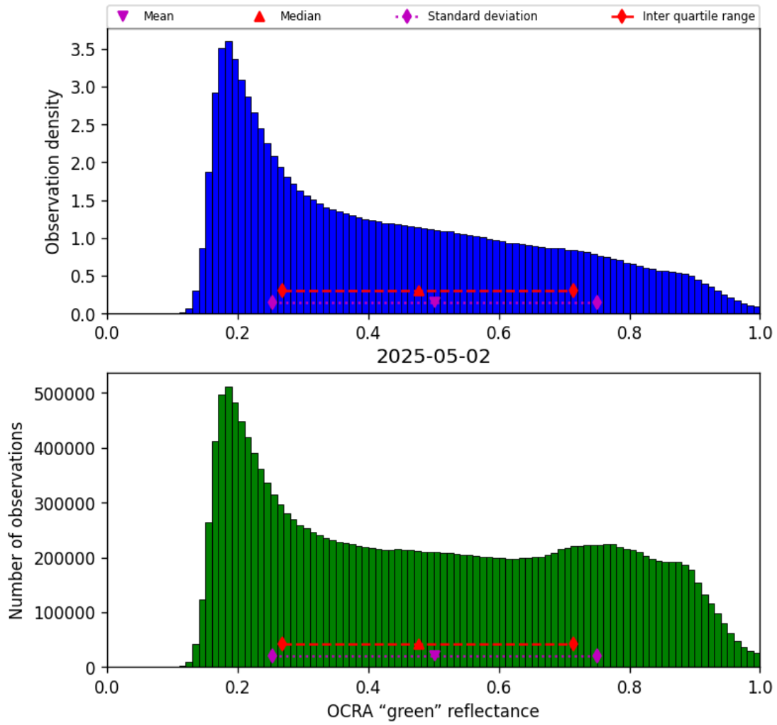
Figure 52: Histogram of “OCRA “green” reflectance” for 2025-05-01 to 2025-05-03
