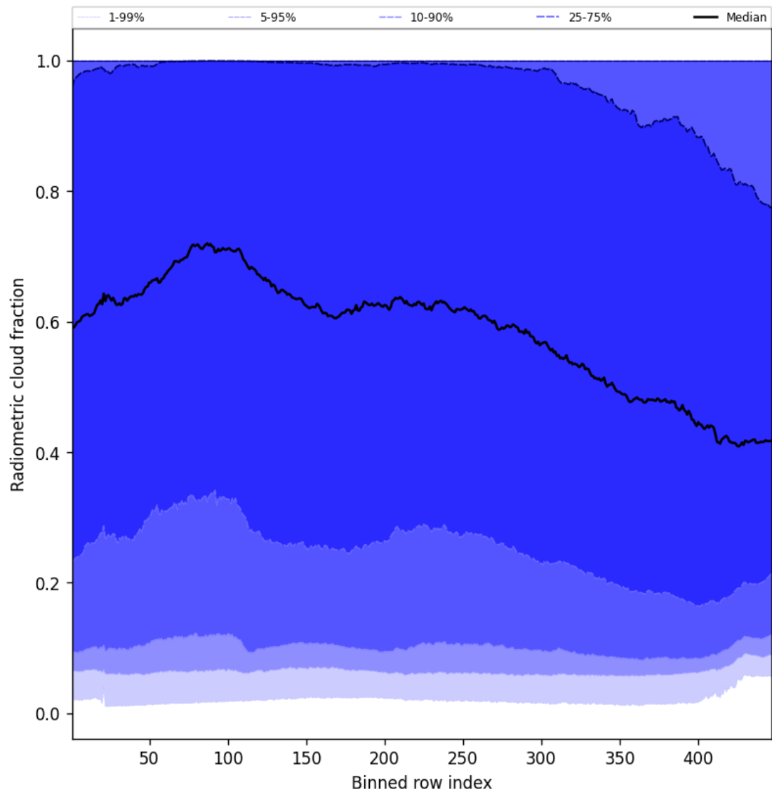
Figure 55: Along track statistics of “Radiometric cloud fraction” for 2025-05-01 to 2025-05-03
