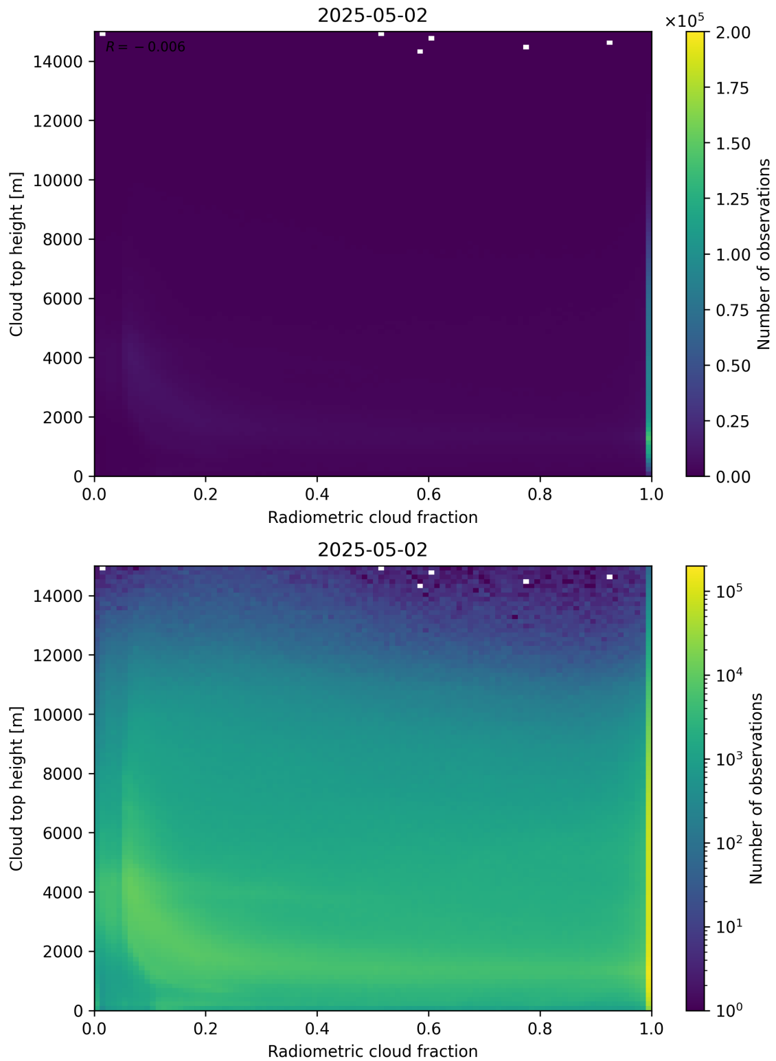
Figure 76: Scatter density plot of “Radiometric cloud fraction” against “Cloud top height” for 2025-05-01 to 2025-05-03.
