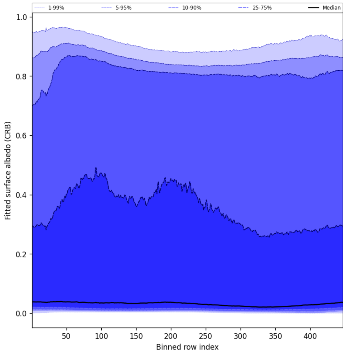
Figure 62: Along track statistics of “Fitted surface albedo (CRB)” for 2025-05-01 to 2025-05-03
