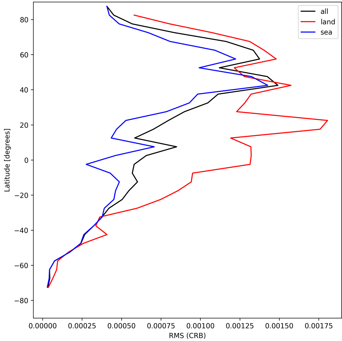
Figure 32: Zonal average of “RMS (CRB)” for 2025-05-01 to 2025-05-03.
