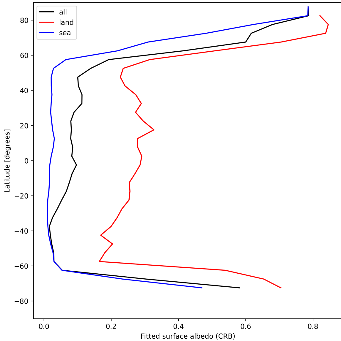
Figure 30: Zonal average of “Fitted surface albedo (CRB)” for 2025-05-01 to 2025-05-03.
