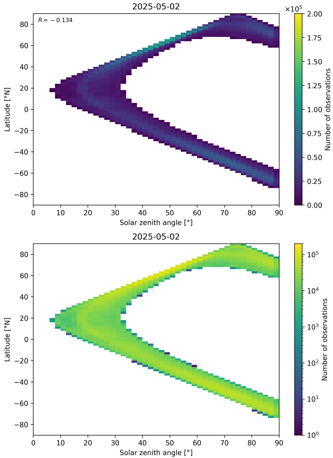
Figure 105: Scatter density plot of “Solar zenith angle” against “Latitude” for 2025-05-01 to 2025-05-03.
