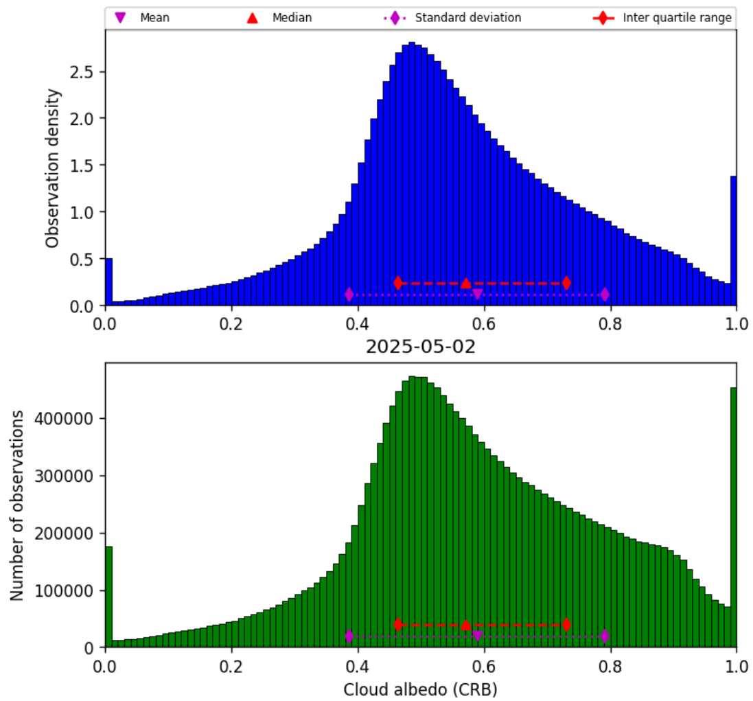
Figure 44: Histogram of “Cloud albedo (CRB)” for 2025-05-01 to 2025-05-03
