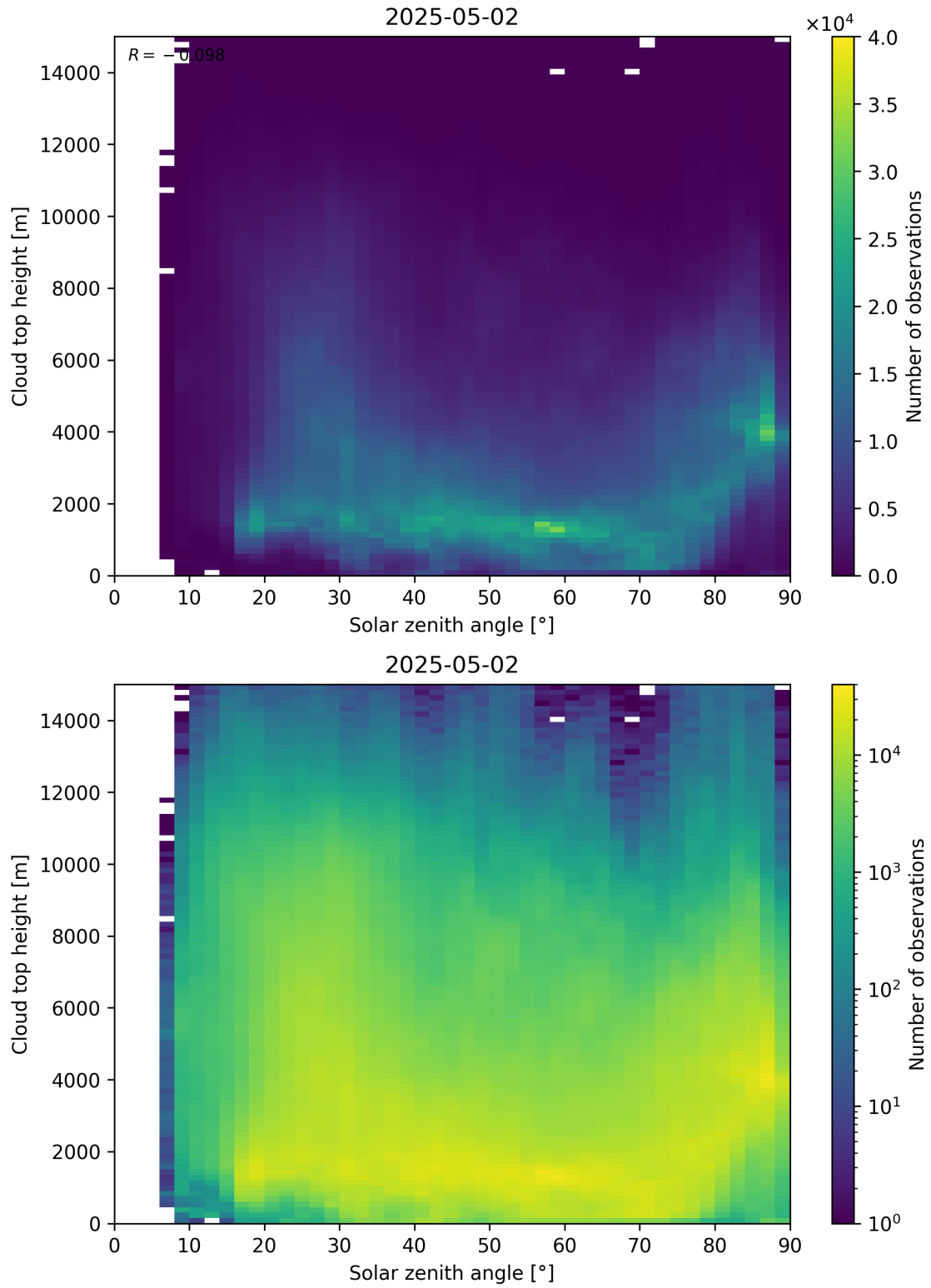
Figure 104: Scatter density plot of “Solar zenith angle” against “Cloud top height” for 2025-05-01 to 2025-05-03.
