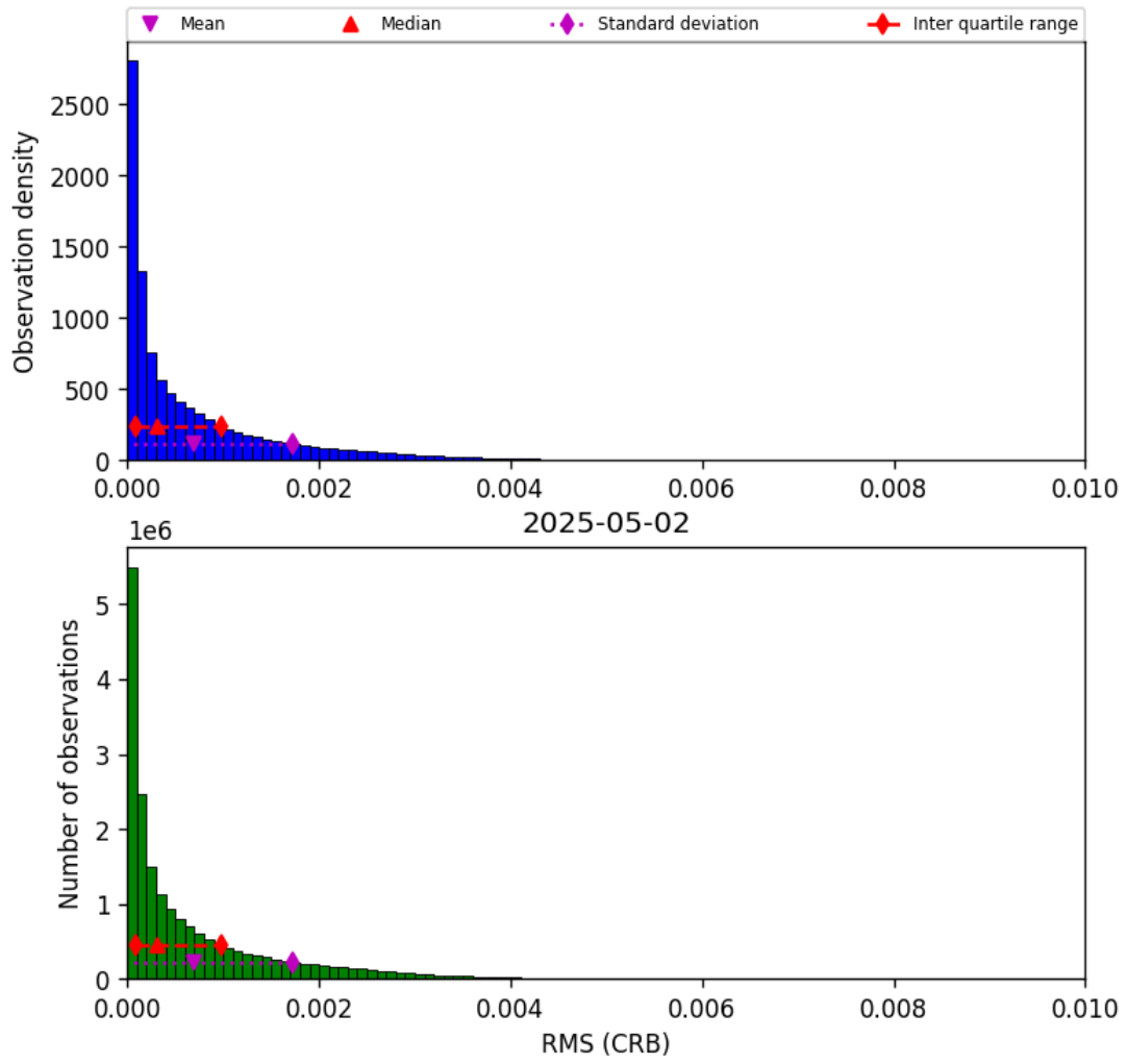
Figure 48: Histogram of “RMS (CRB)” for 2025-05-01 to 2025-05-03
