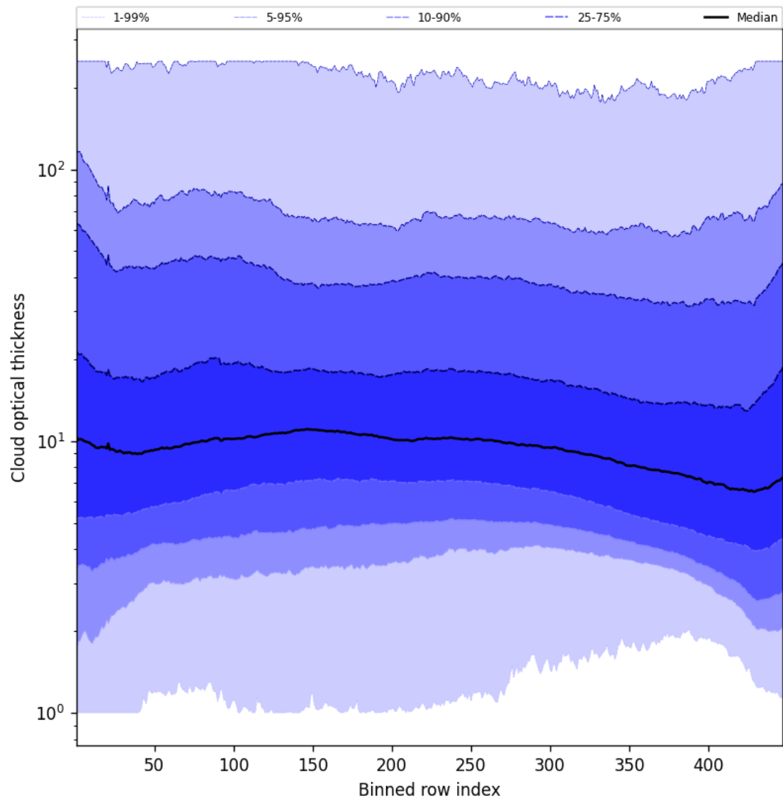
Figure 57: Along track statistics of “Cloud optical thickness” for 2025-05-01 to 2025-05-03
