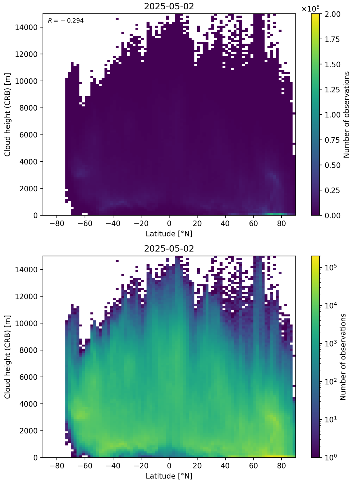
Figure 95: Scatter density plot of “Latitude” against “Cloud height (CRB)” for 2025-05-01 to 2025-05-03.
