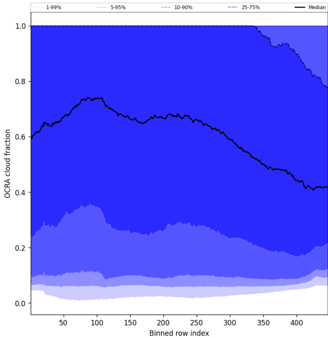
Figure 66: Along track statistics of “OCRA cloud fraction” for 2025-05-01 to 2025-05-03
