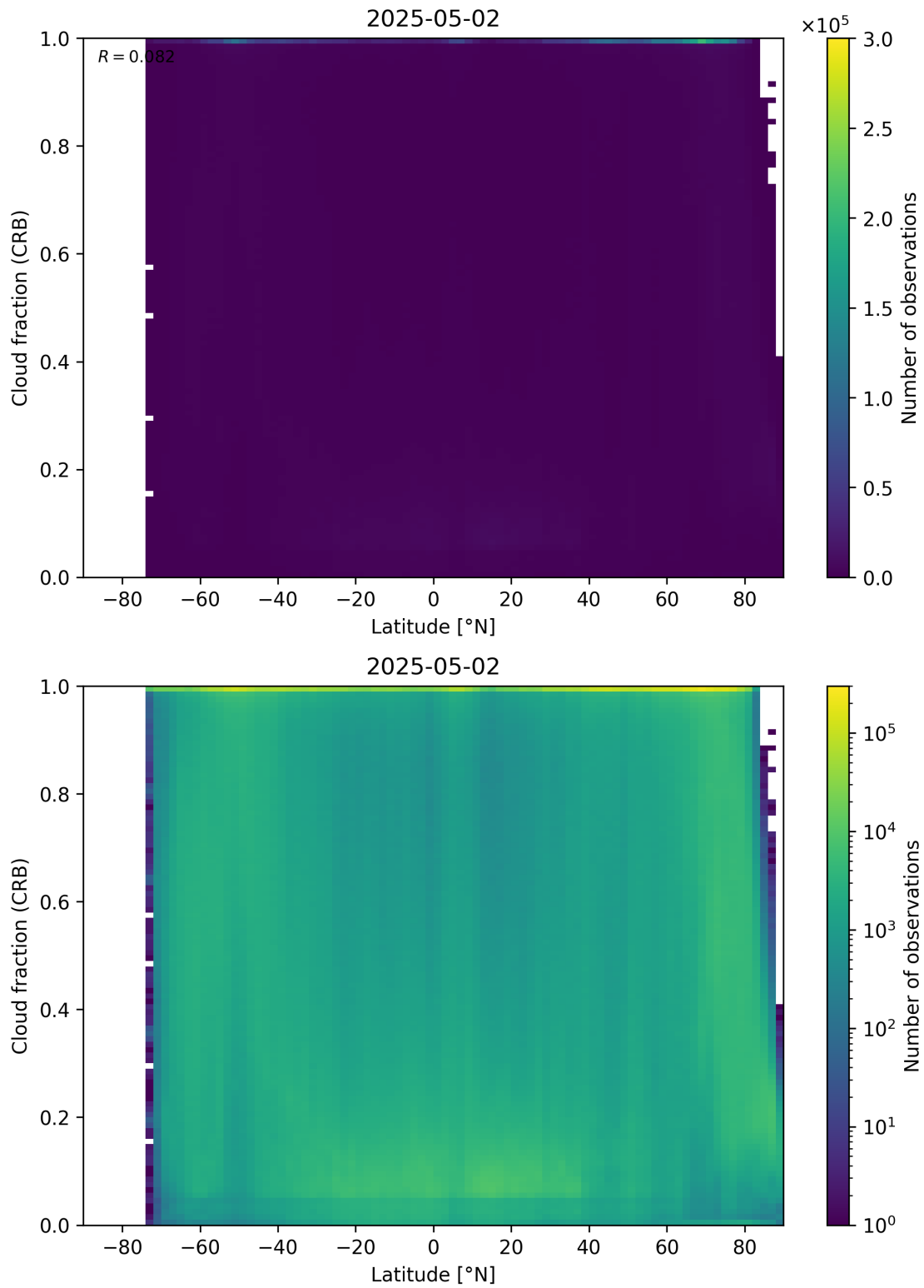
Figure 94: Scatter density plot of “Latitude” against “Cloud fraction (CRB)” for 2025-05-01 to 2025-05-03.
