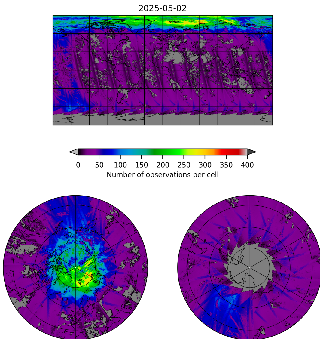
Figure 21: Map of the number of observations for 2025-05-01 to 2025-05-03
