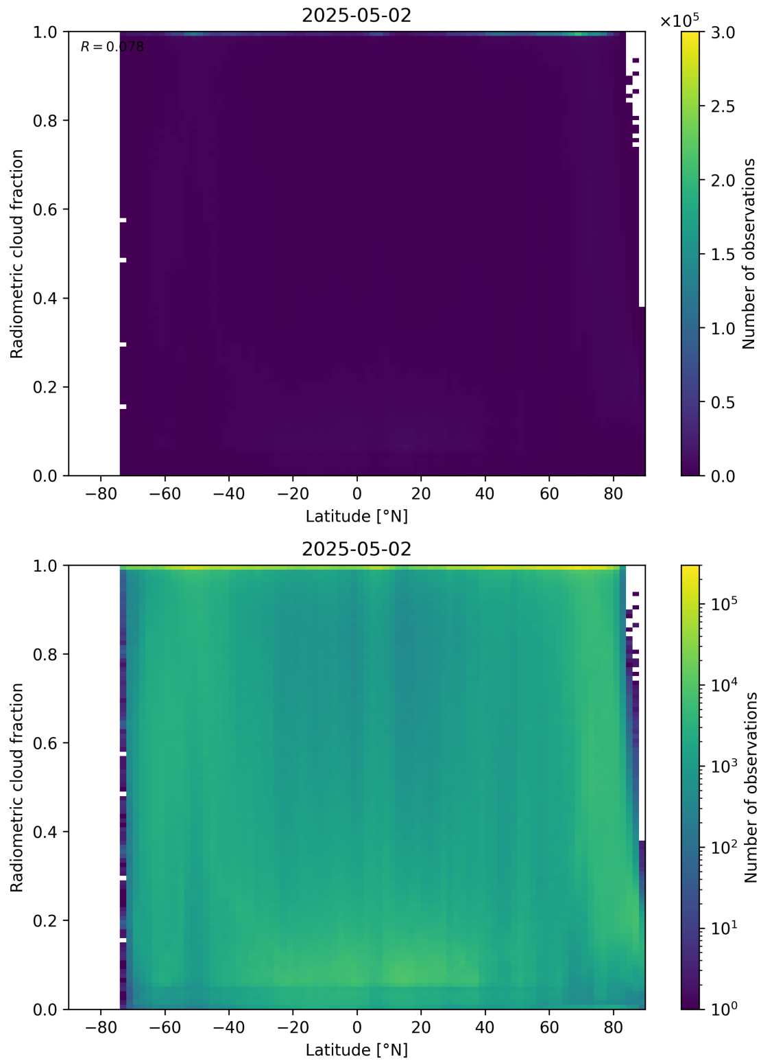
Figure 92: Scatter density plot of “Latitude” against “Radiometric cloud fraction” for 2025-05-01 to 2025-05-03.
