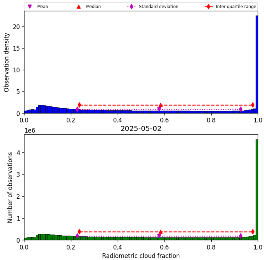
Figure 39: Histogram of “Radiometric cloud fraction” for 2025-05-01 to 2025-05-03
