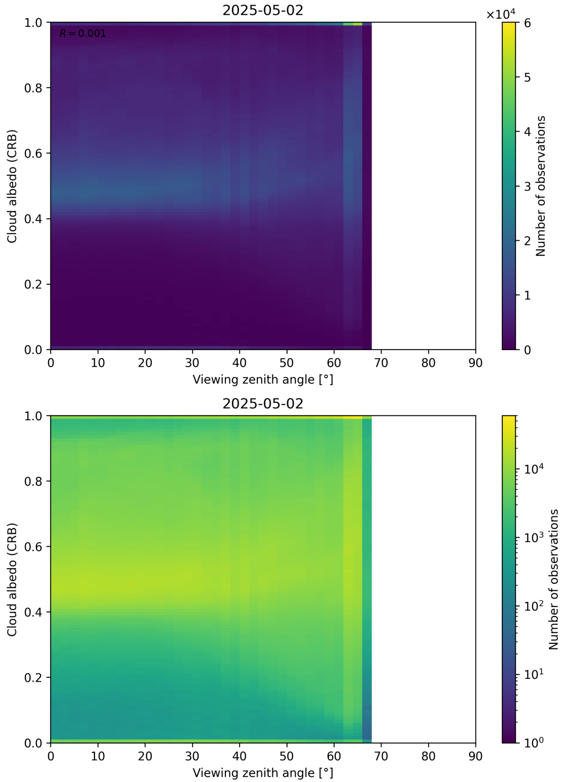
Figure 106: Scatter density plot of “Viewing zenith angle” against “Cloud albedo (CRB)” for 2025-05-01 to 2025-05-03.
