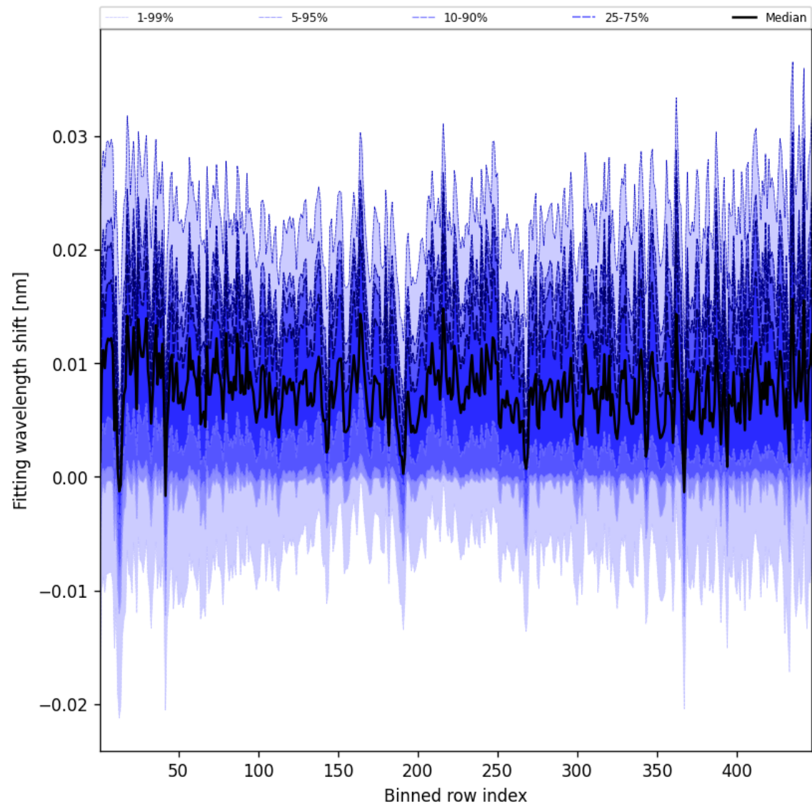
Figure 65: Along track statistics of “Fitting wavelength shift” for 2025-05-01 to 2025-05-03
