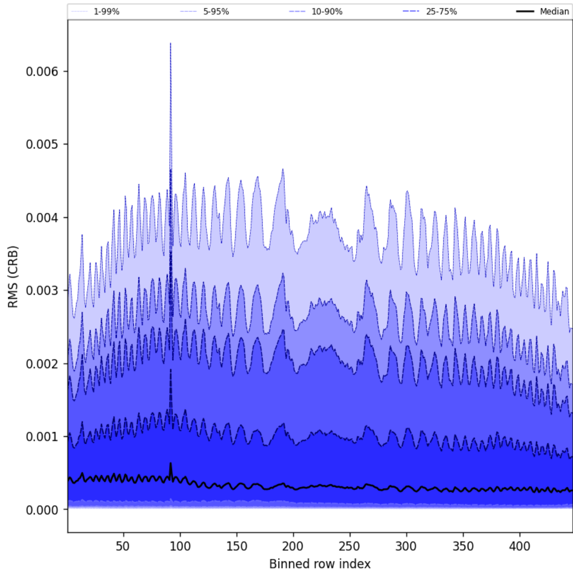
Figure 64: Along track statistics of “RMS (CRB)” for 2025-05-01 to 2025-05-03
