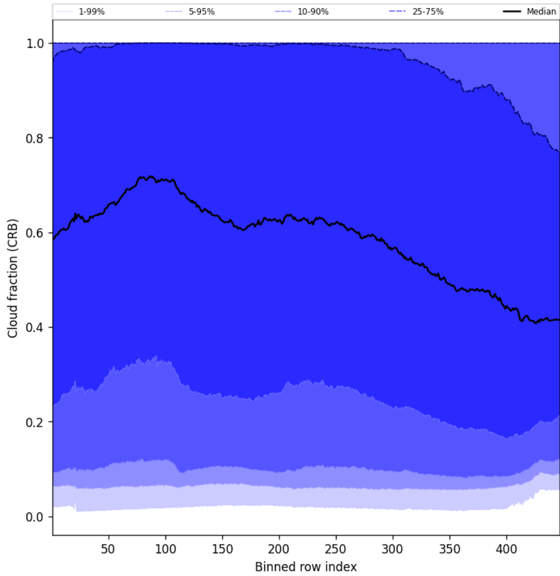
Figure 58: Along track statistics of “Cloud fraction (CRB)” for 2025-05-01 to 2025-05-03
