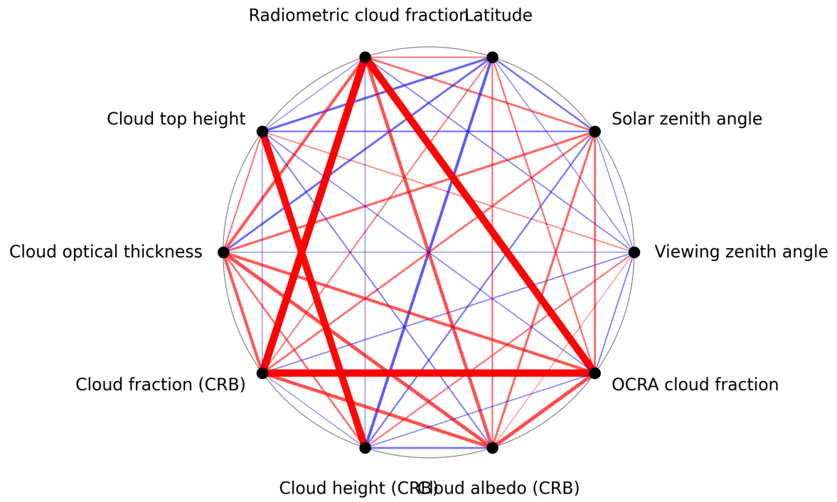
Figure 1: Map of correlation graph for 2025-05-01 to 2025-05-03.
