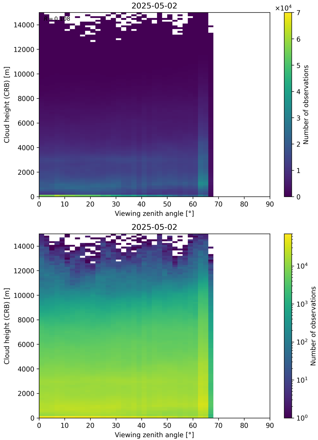
Figure 110: Scatter density plot of “Viewing zenith angle” against “Cloud height (CRB)” for 2025-05-01 to 2025-05-03.
