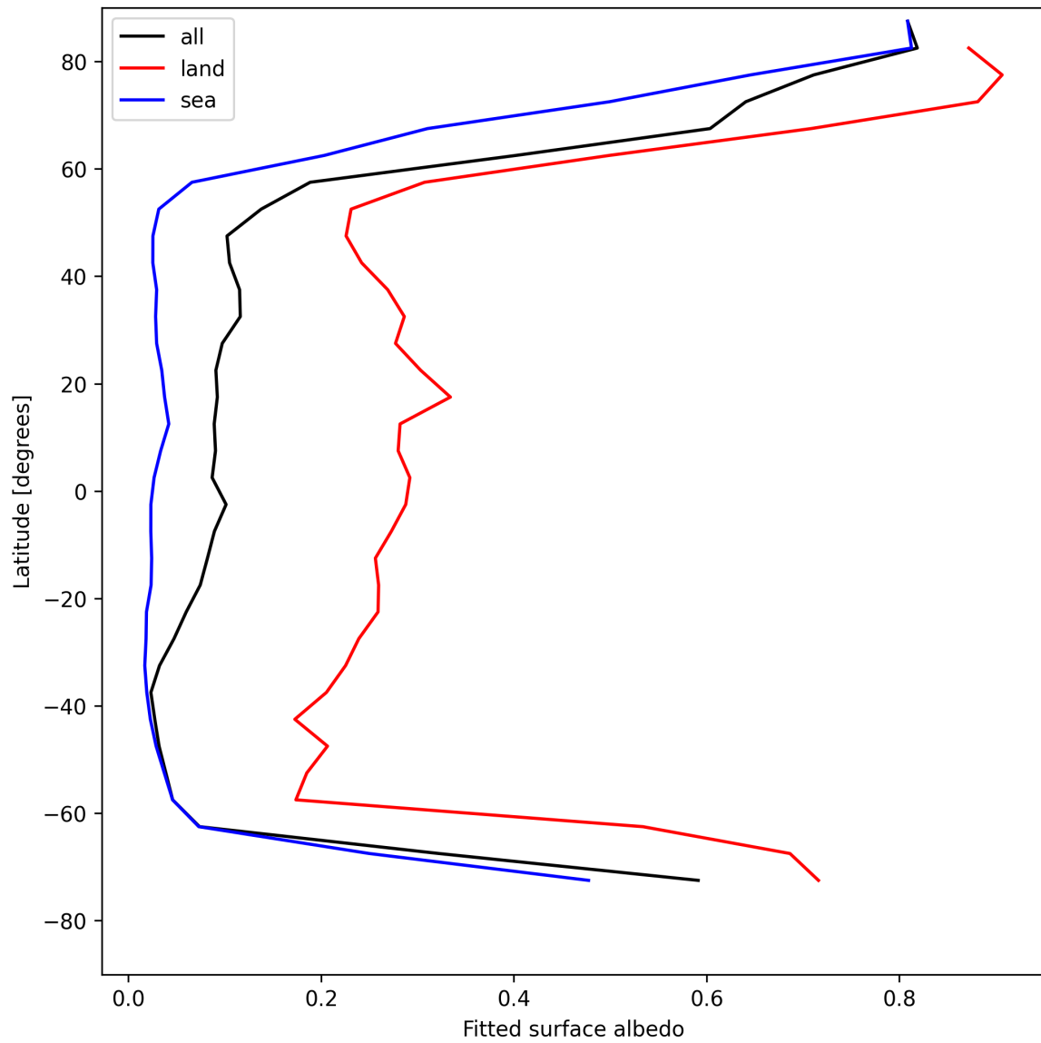
Figure 29: Zonal average of “Fitted surface albedo” for 2025-05-01 to 2025-05-03.
