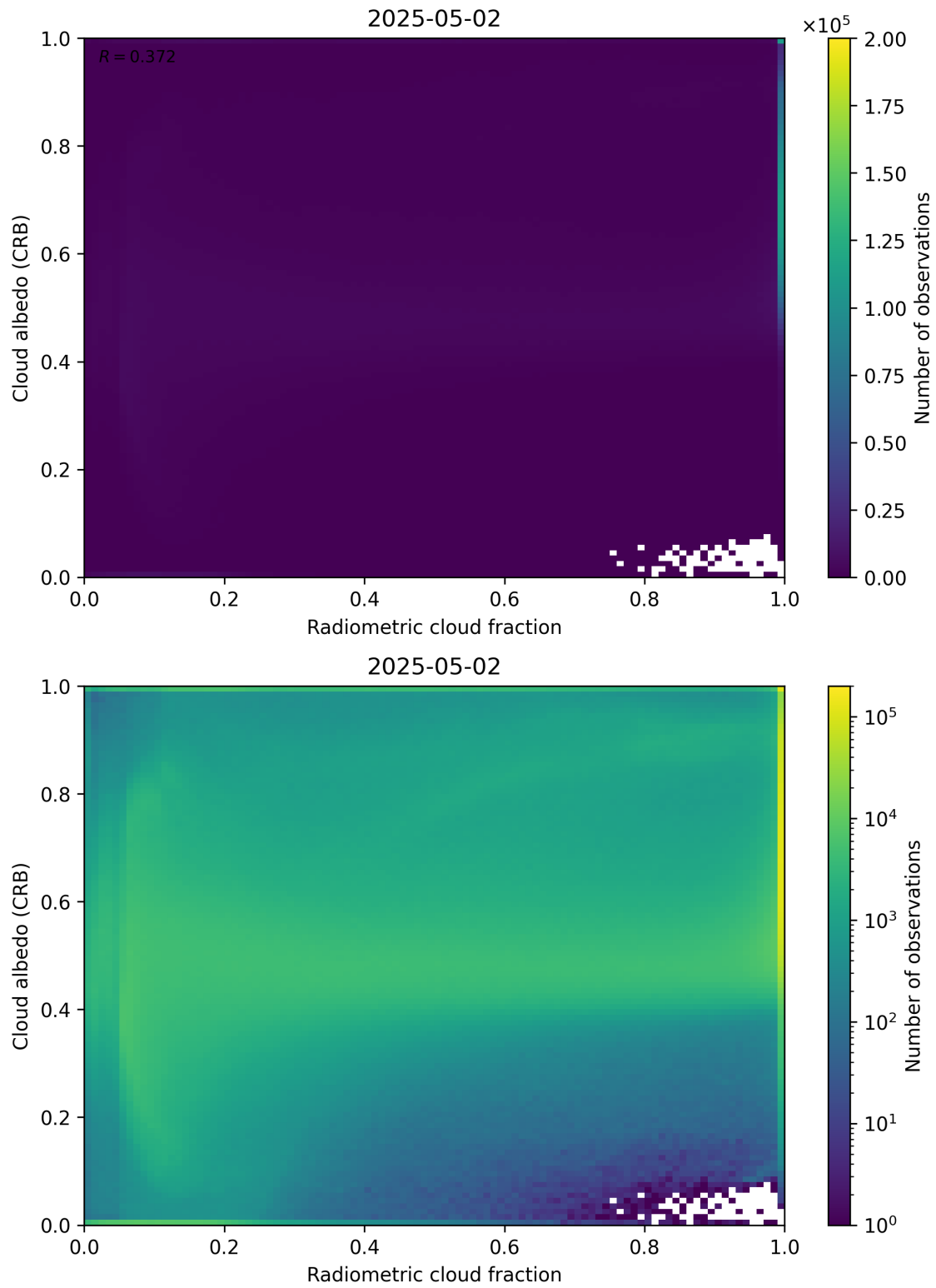
Figure 71: Scatter density plot of “Radiometric cloud fraction” against “Cloud albedo (CRB)” for 2025-05-01 to 2025-05-03.
