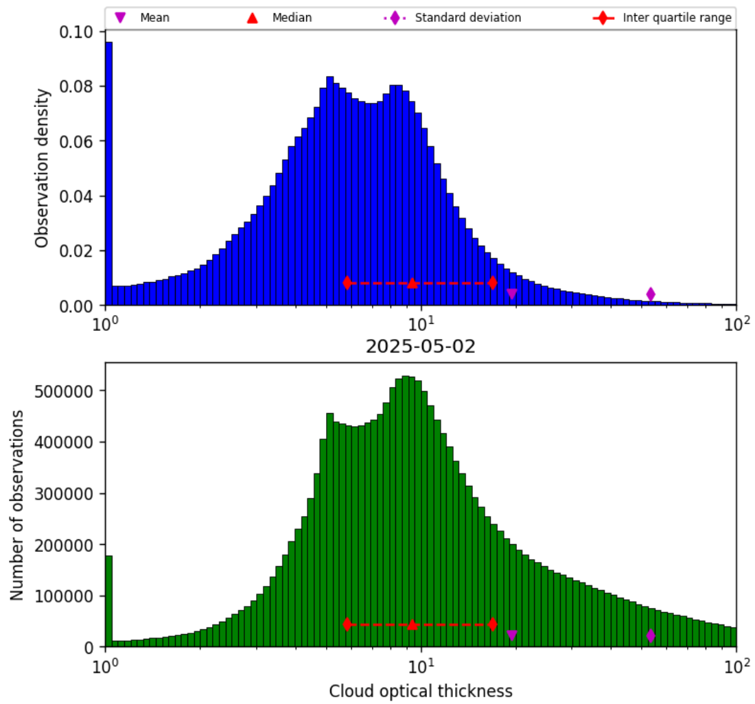
Figure 41: Histogram of “Cloud optical thickness” for 2025-05-01 to 2025-05-03
