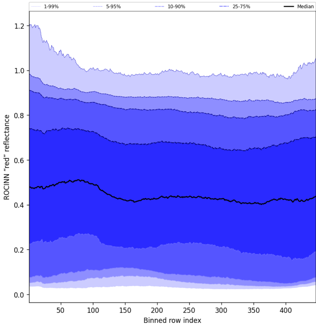
Figure 69: Along track statistics of “ROCINN “red” reflectance” for 2025-05-01 to 2025-05-03
