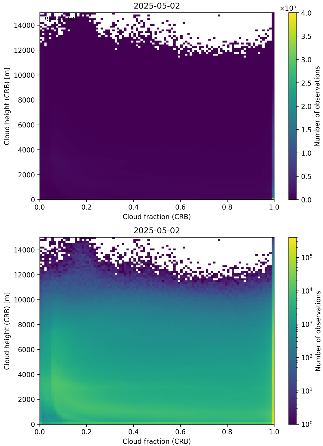
Figure 79: Scatter density plot of “Cloud fraction (CRB)” against “Cloud height (CRB)” for 2025-05-01 to 2025-05-03.
