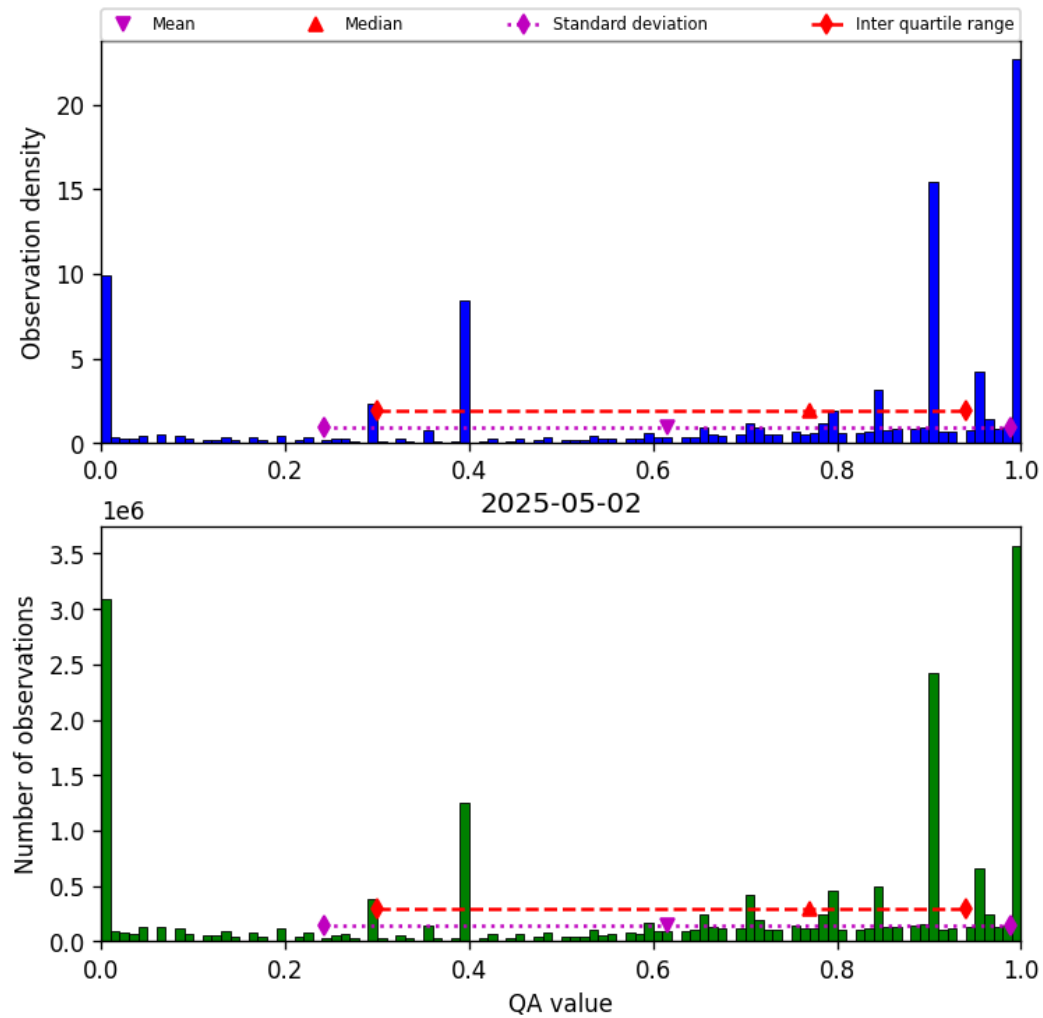
Figure 38: Histogram of “QA value” for 2025-05-01 to 2025-05-03
