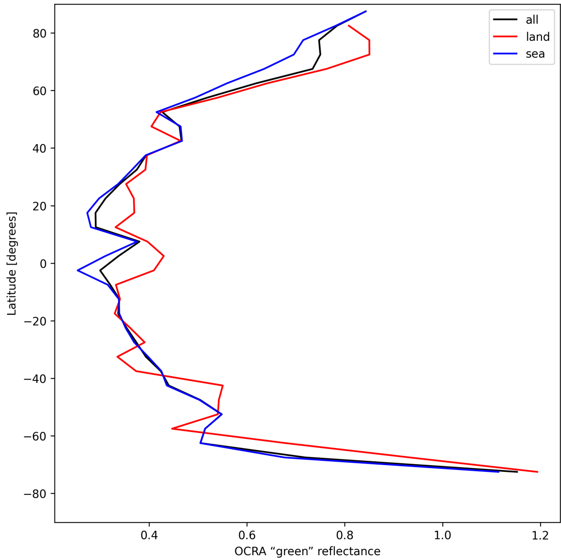
Figure 36: Zonal average of “OCRA “green” reflectance” for 2025-05-01 to 2025-05-03.
