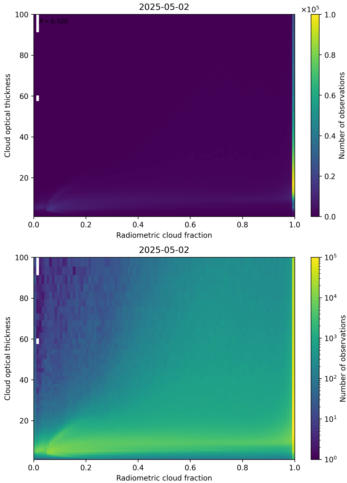
Figure 75: Scatter density plot of “Radiometric cloud fraction” against “Cloud optical thickness” for 2025-05-01 to 2025-05-03.
