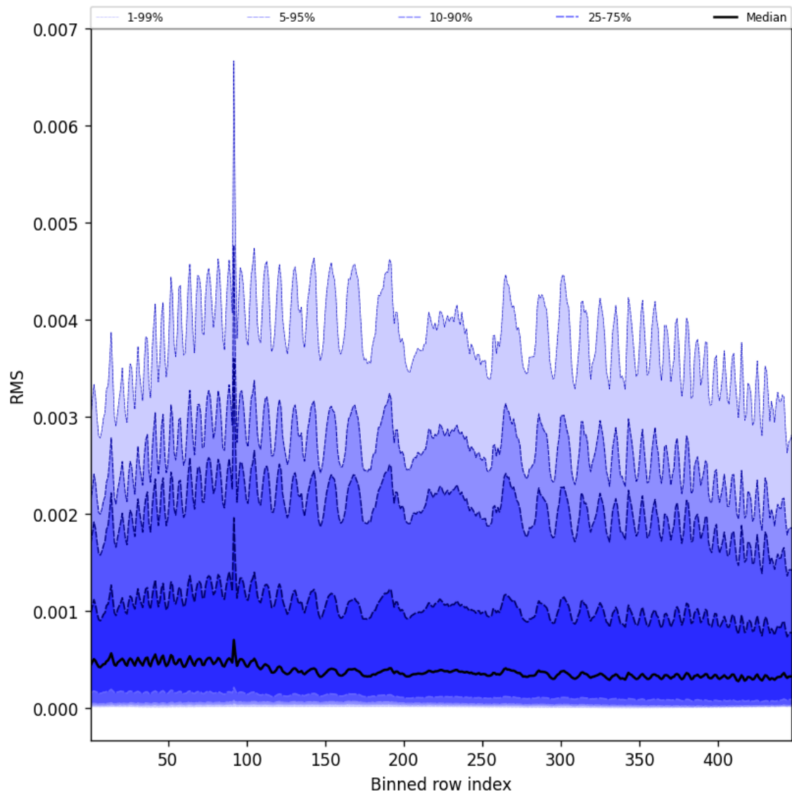
Figure 63: Along track statistics of “RMS” for 2025-05-01 to 2025-05-03
