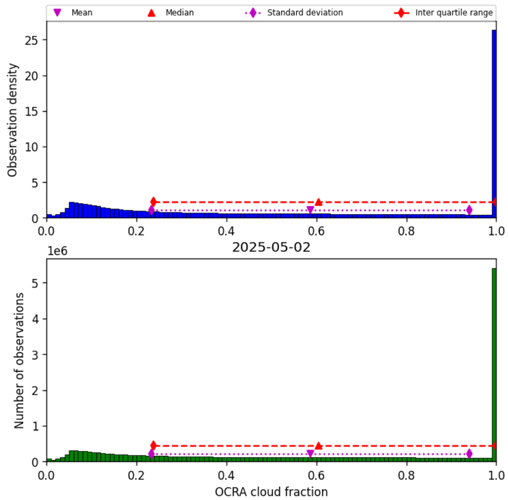
Figure 50: Histogram of “OCRA cloud fraction” for 2025-05-01 to 2025-05-03
