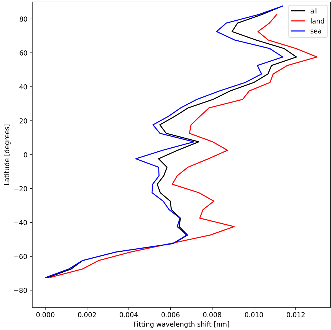
Figure 33: Zonal average of “Fitting wavelength shift” for 2025-05-01 to 2025-05-03.
