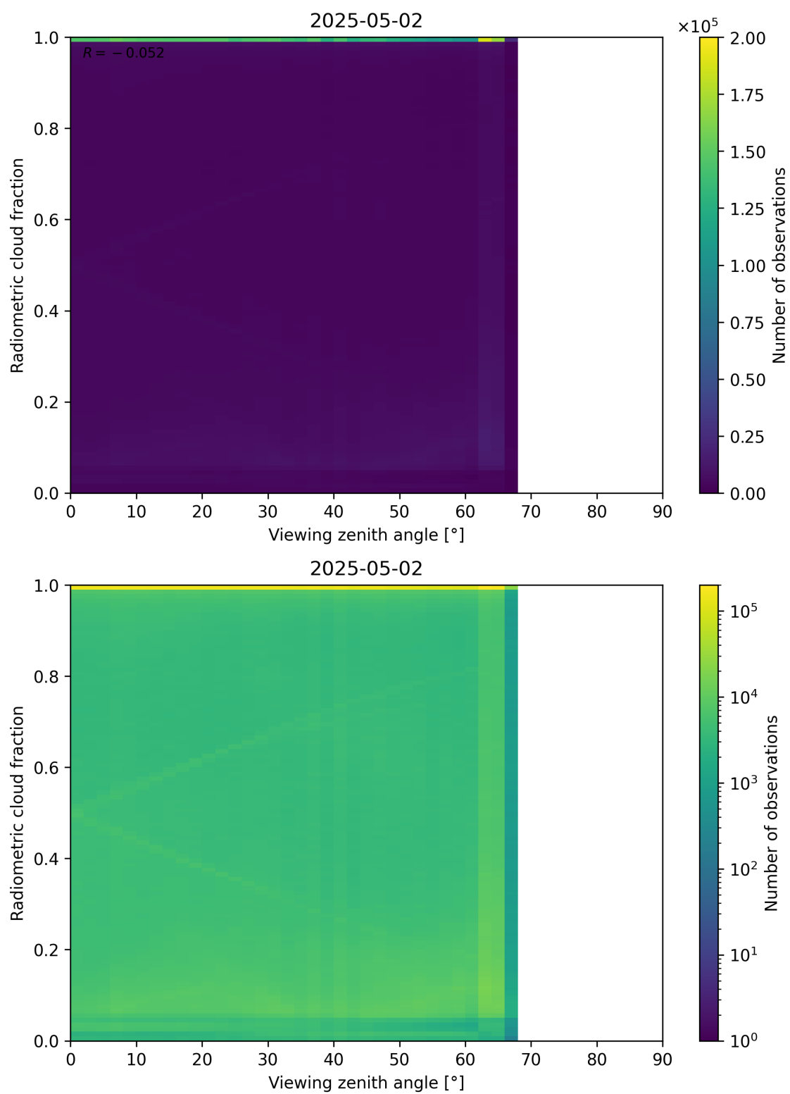
Figure 107: Scatter density plot of “Viewing zenith angle” against “Radiometric cloud fraction” for 2025-05-01 to 2025-05-03.
