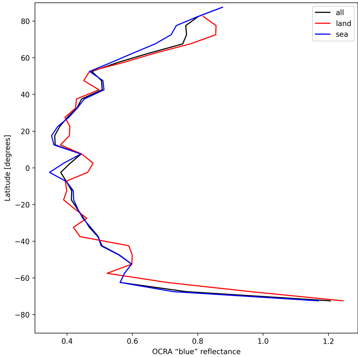
Figure 35: Zonal average of "OCRA "blue" reflectance" for 2025-05-01 to 2025-05-03.
