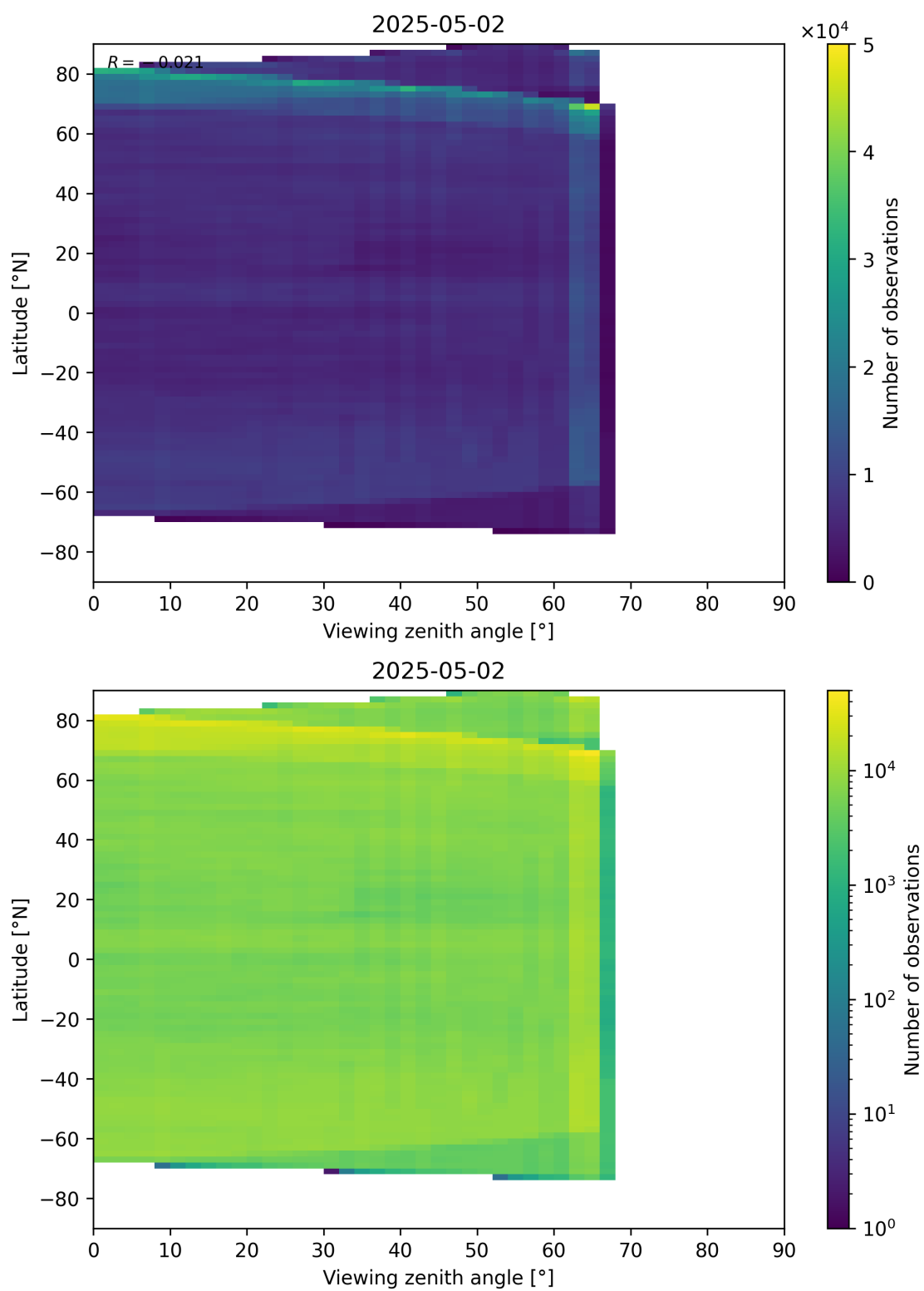
Figure 113: Scatter density plot of “Viewing zenith angle” against “Latitude” for 2025-05-01 to 2025-05-03.
