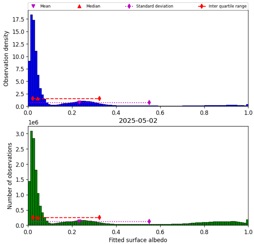
Figure 45: Histogram of “Fitted surface albedo” for 2025-05-01 to 2025-05-03
