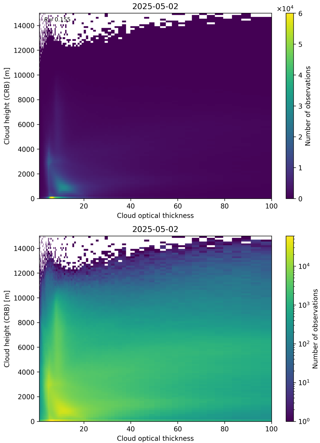
Figure 85: Scatter density plot of “Cloud optical thickness” against “Cloud height (CRB)” for 2025-05-01 to 2025-05-03.
