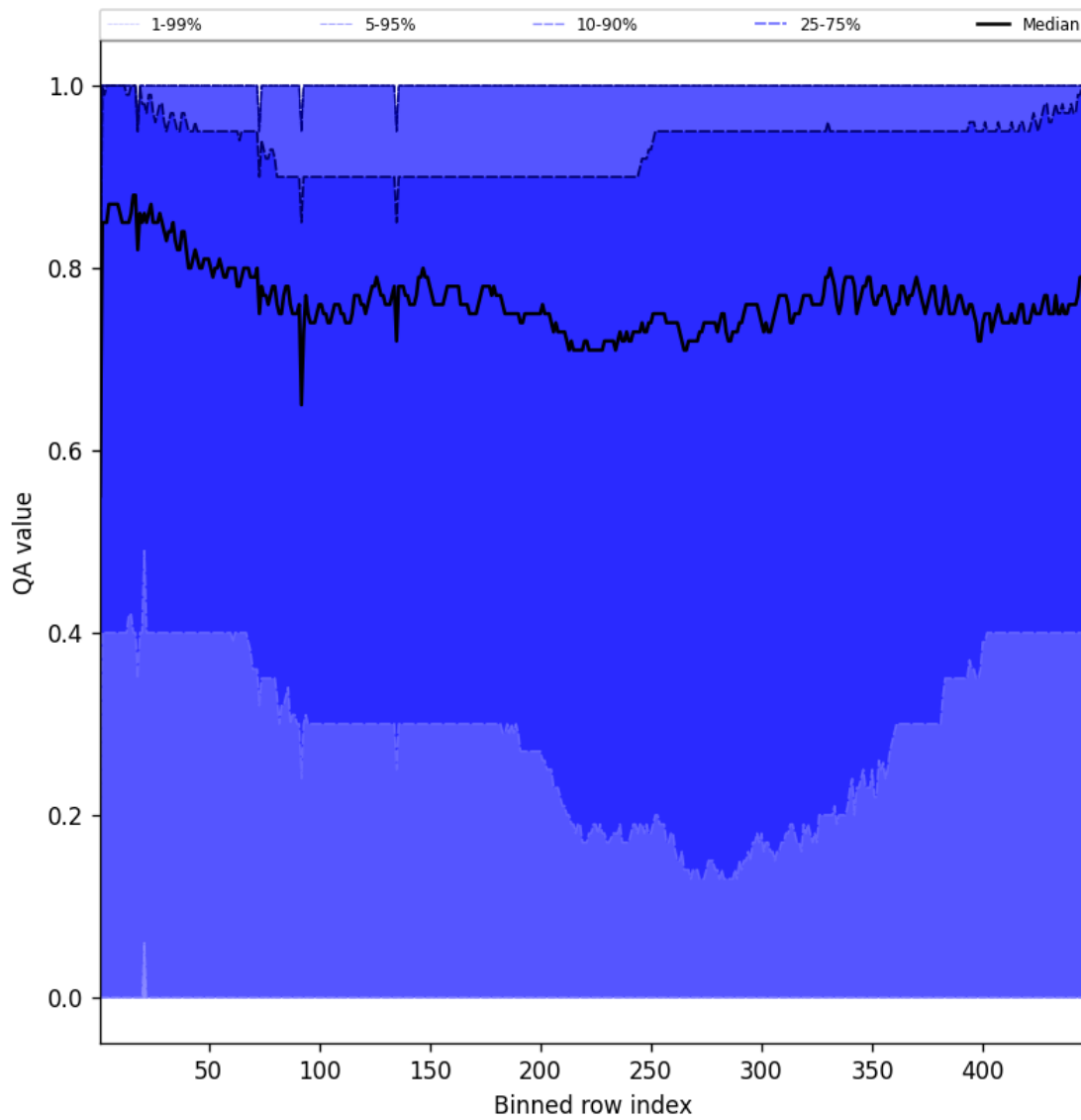
Figure 54: Along track statistics of “QA value” for 2025-05-01 to 2025-05-03
