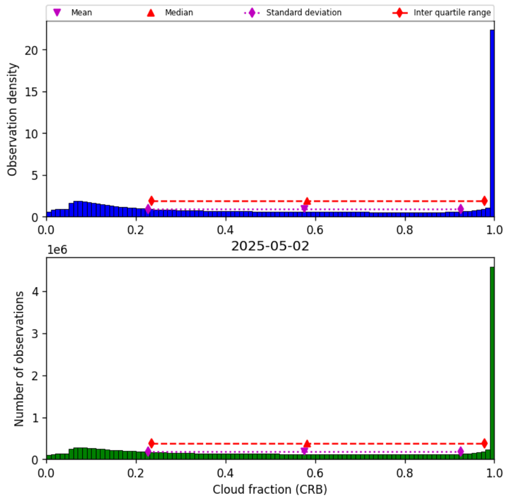
Figure 42: Histogram of “Cloud fraction (CRB)” for 2025-05-01 to 2025-05-03
