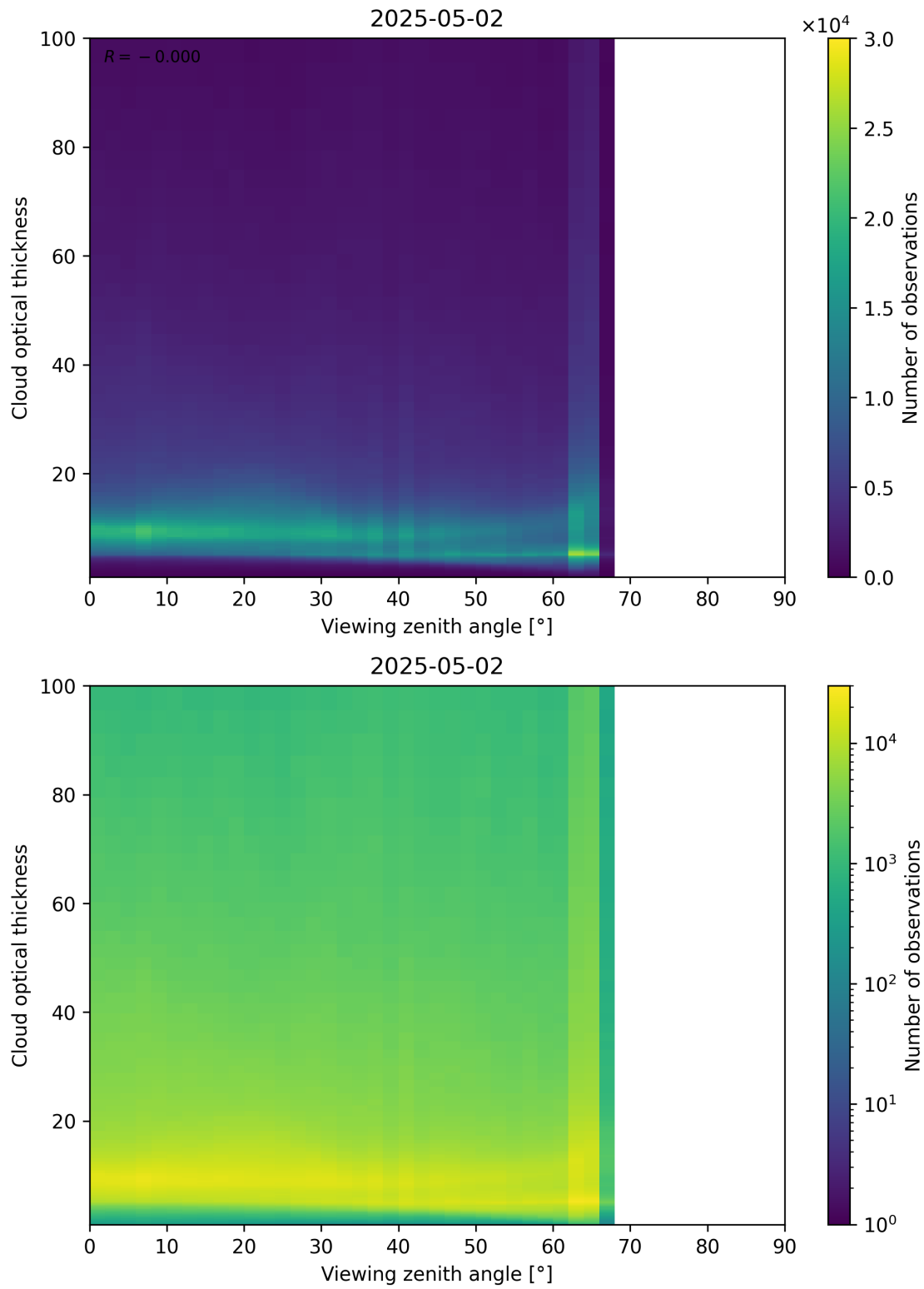
Figure 111: Scatter density plot of “Viewing zenith angle” against “Cloud optical thickness” for 2025-05-01 to 2025-05-03.
