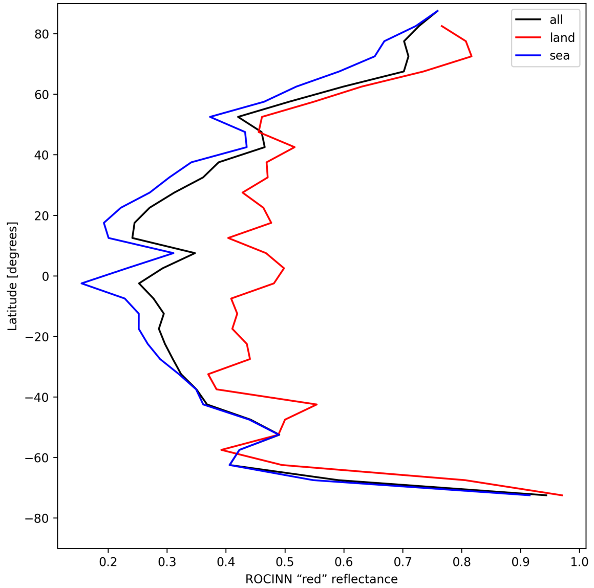
Figure 37: Zonal average of “ROCINN “red” reflectance” for 2025-05-01 to 2025-05-03.
