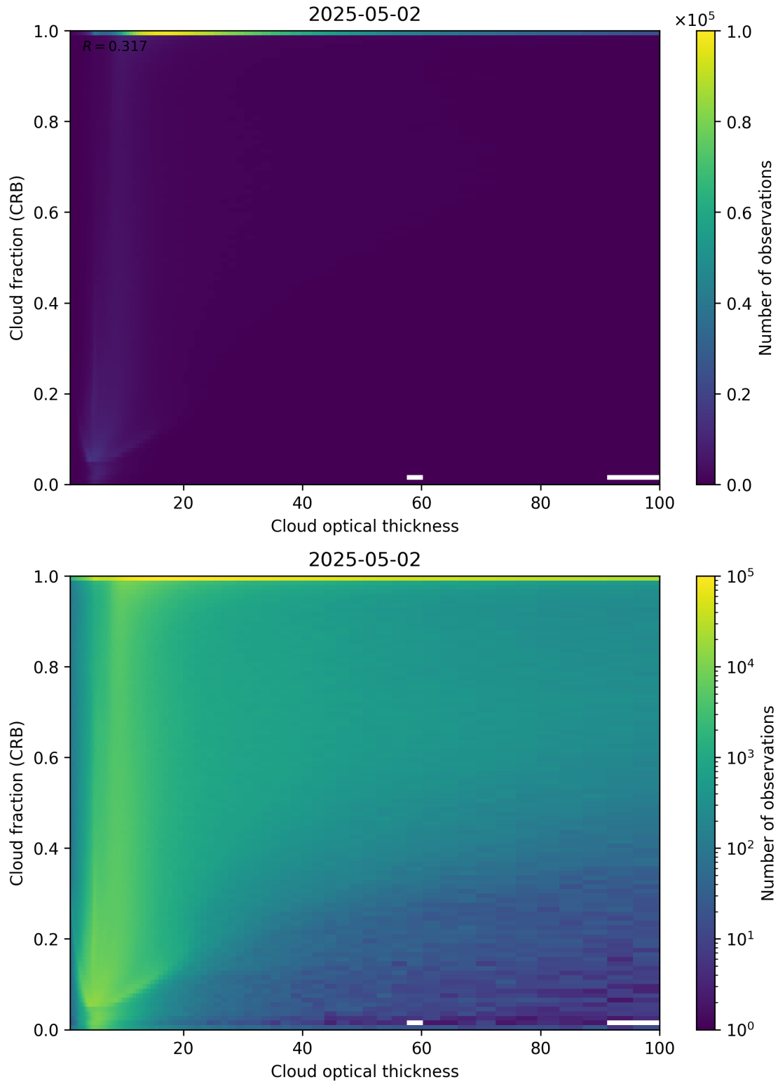
Figure 84: Scatter density plot of “Cloud optical thickness” against “Cloud fraction (CRB)” for 2025-05-01 to 2025-05-03.
