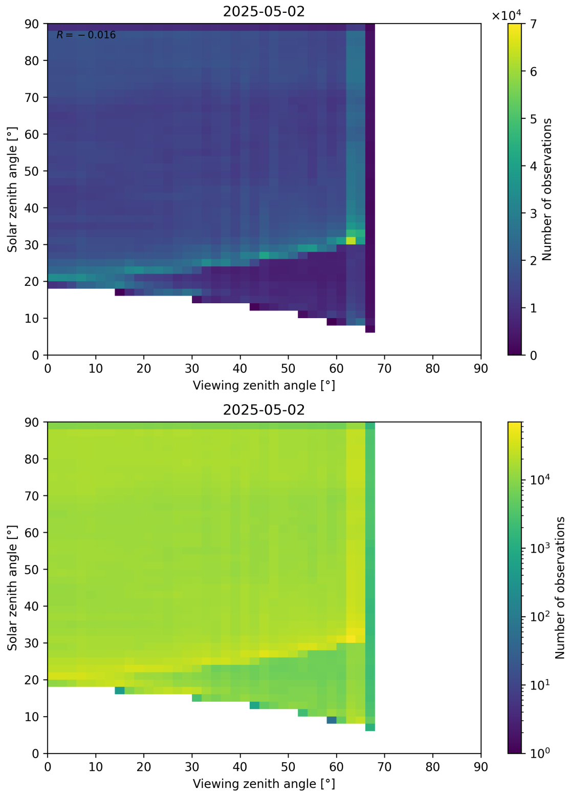
Figure 114: Scatter density plot of “Viewing zenith angle” against “Solar zenith angle” for 2025-05-01 to 2025-05-03.
