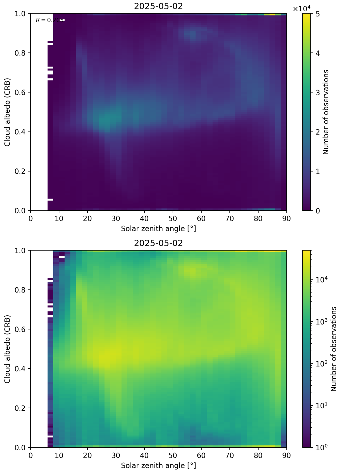
Figure 98: Scatter density plot of “Solar zenith angle” against “Cloud albedo (CRB)” for 2025-05-01 to 2025-05-03.
