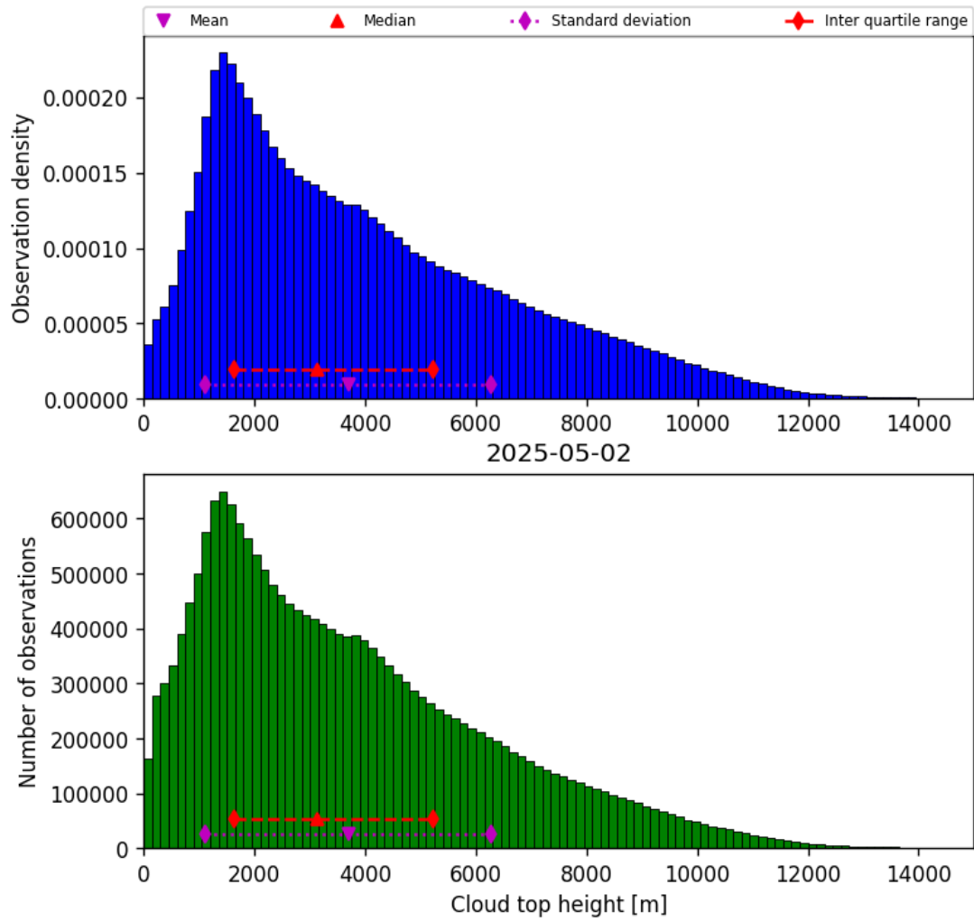
Figure 40: Histogram of “Cloud top height” for 2025-05-01 to 2025-05-03
