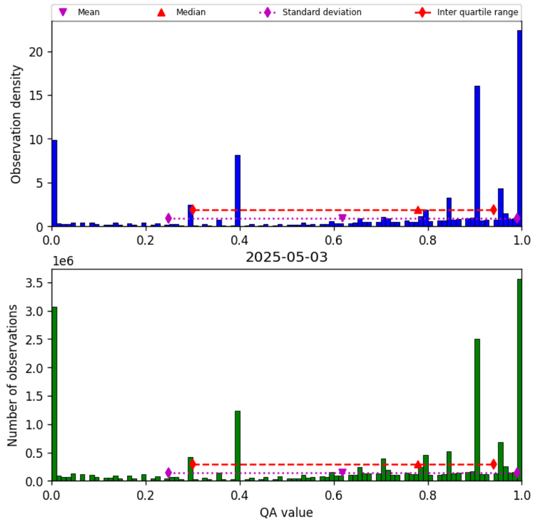
Figure 38: Histogram of “QA value” for 2025-05-02 to 2025-05-04
