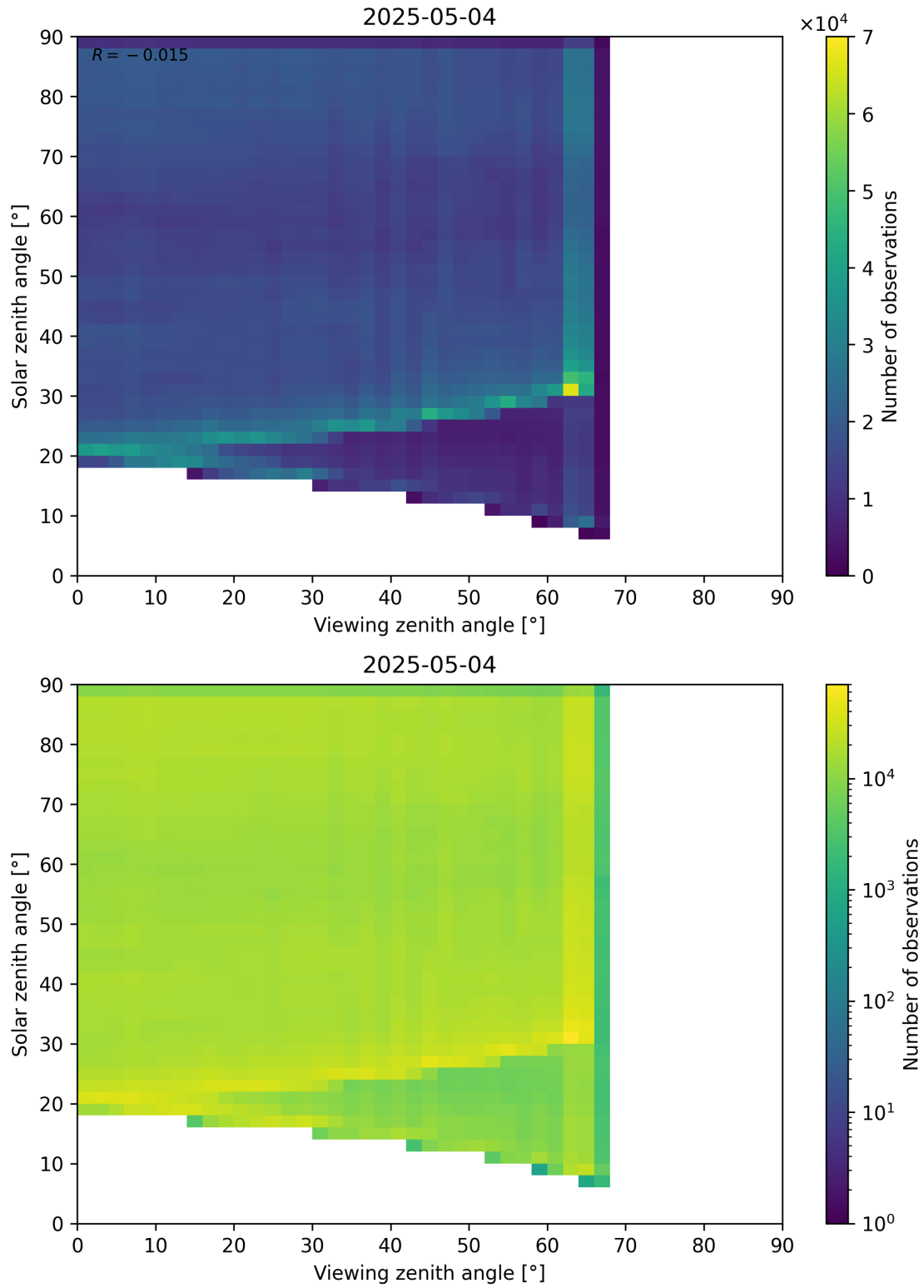
Figure 114: Scatter density plot of “Viewing zenith angle” against “Solar zenith angle” for 2025-05-03 to 2025-05-05.
