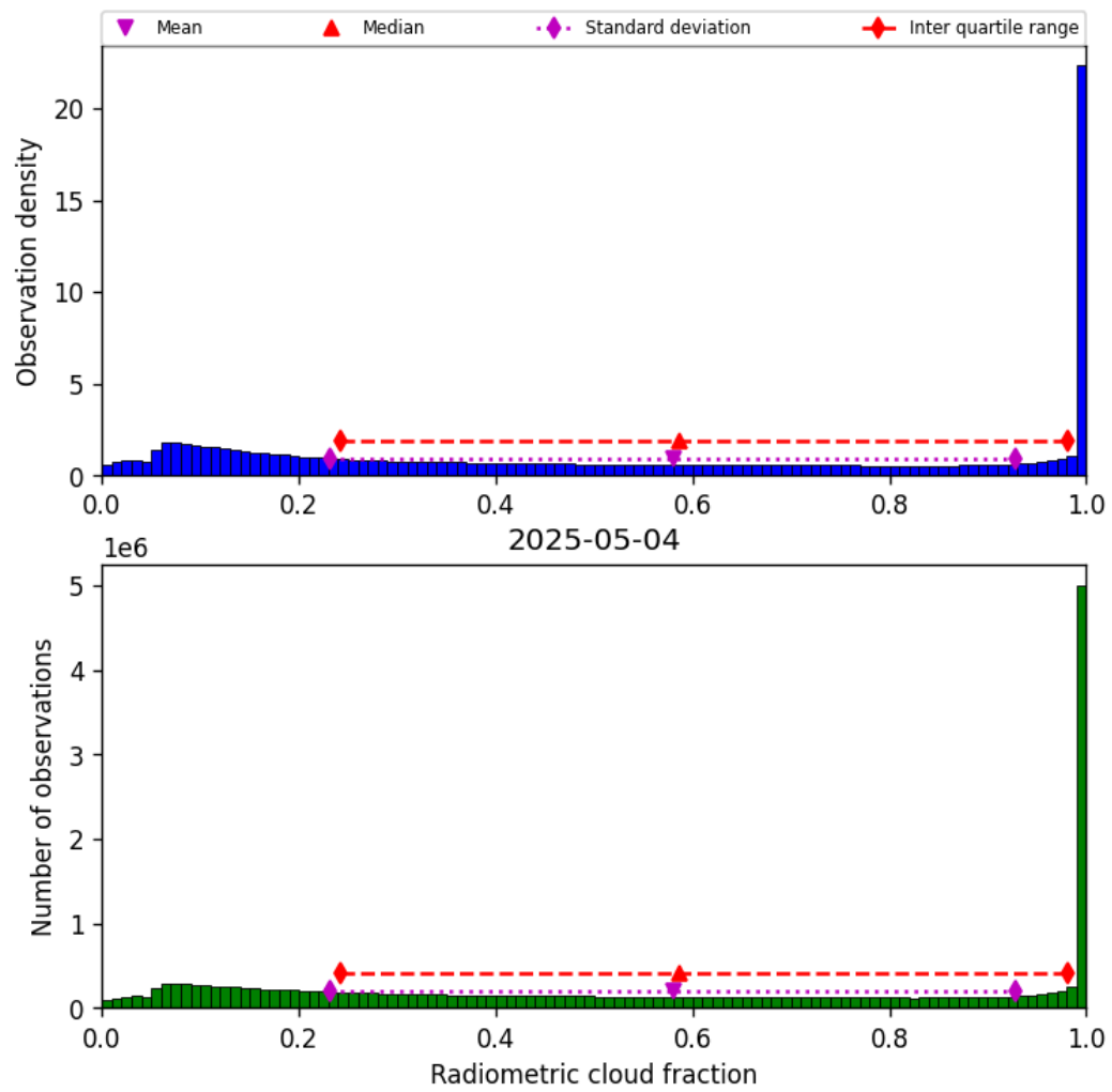
Figure 39: Histogram of “Radiometric cloud fraction” for 2025-05-03 to 2025-05-05
