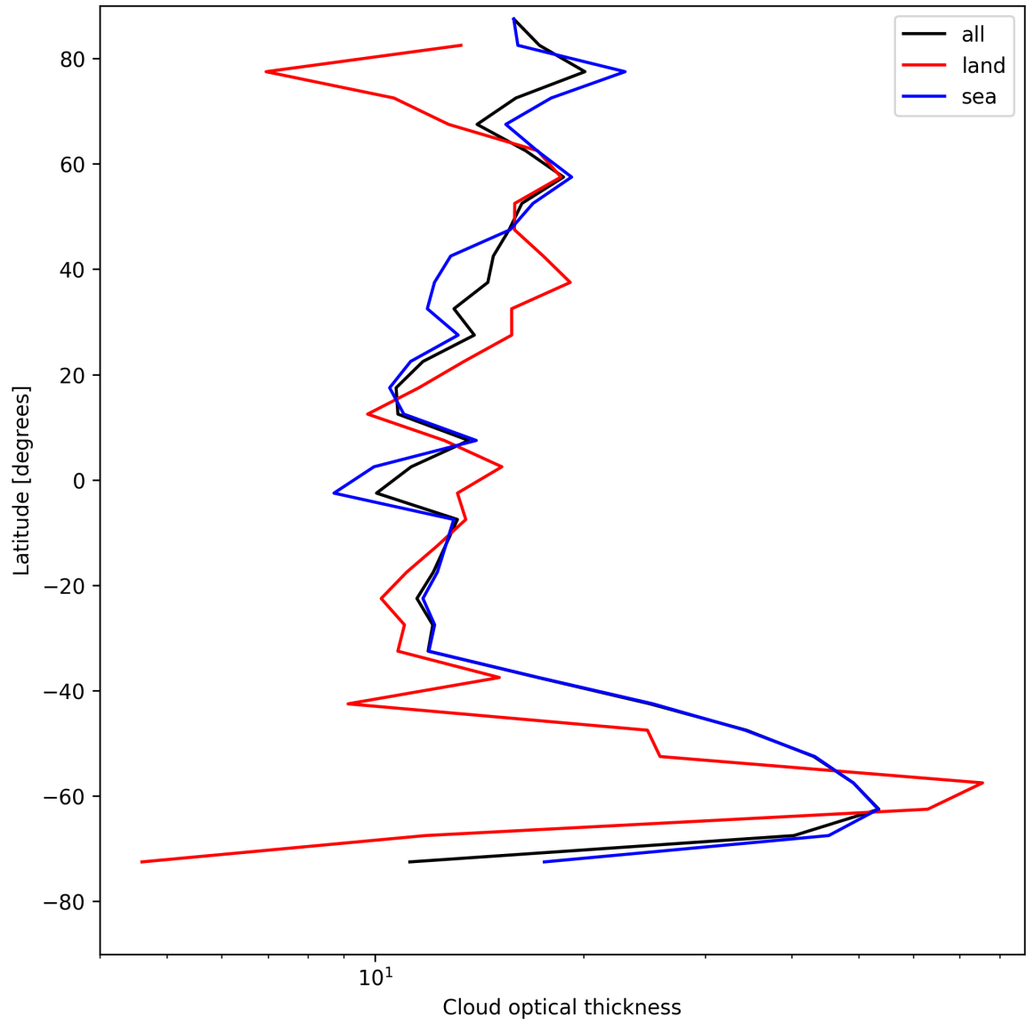
Figure 25: Zonal average of “Cloud optical thickness” for 2025-05-03 to 2025-05-05.
