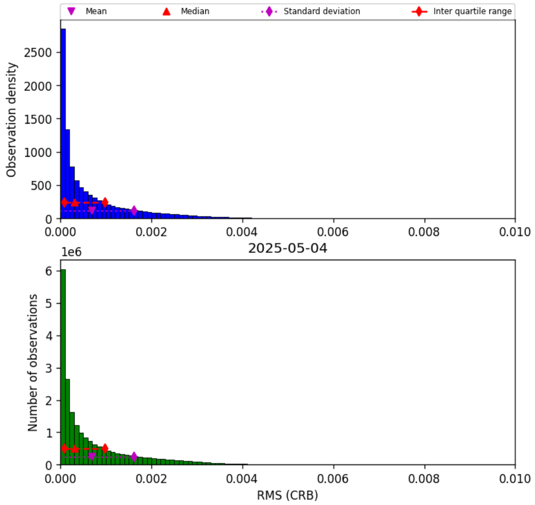
Figure 48: Histogram of “RMS (CRB)” for 2025-05-03 to 2025-05-05
