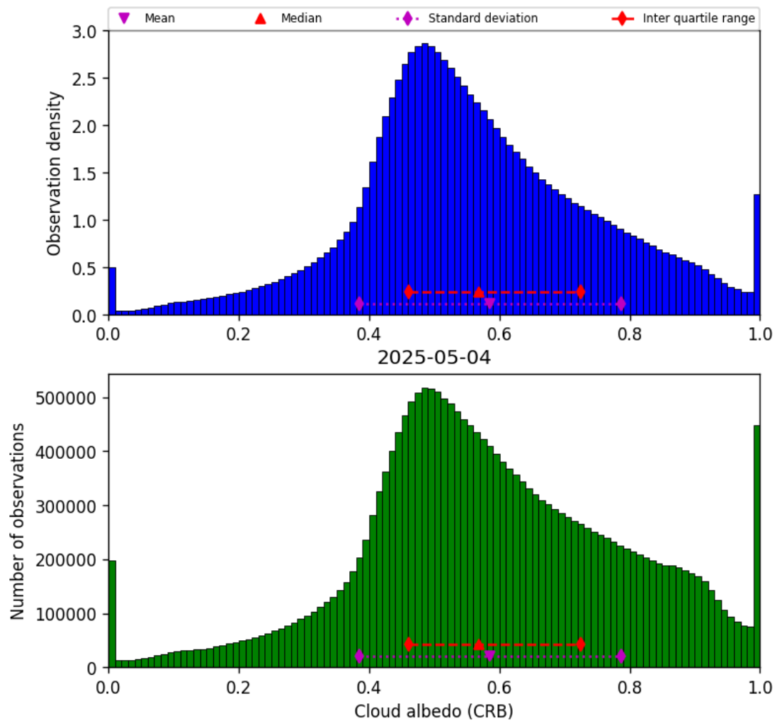
Figure 44: Histogram of “Cloud albedo (CRB)” for 2025-05-03 to 2025-05-05
