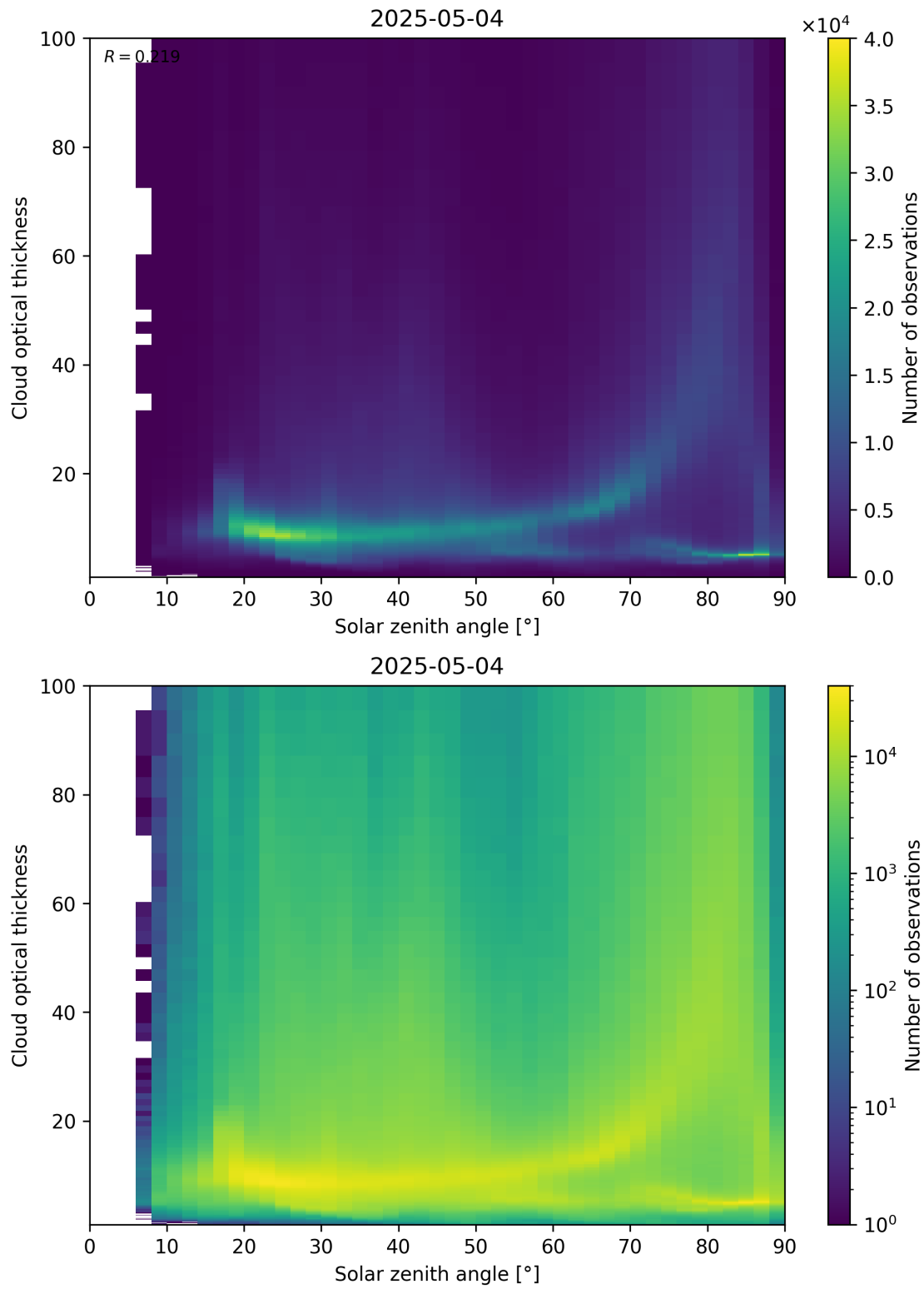
Figure 103: Scatter density plot of “Solar zenith angle” against “Cloud optical thickness” for 2025-05-03 to 2025-05-05.
