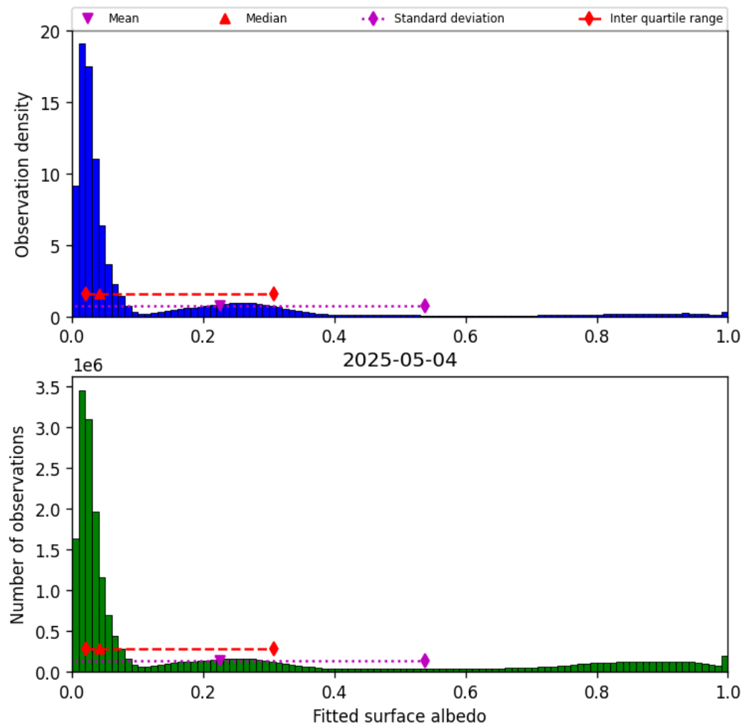
Figure 45: Histogram of “Fitted surface albedo” for 2025-05-03 to 2025-05-05
