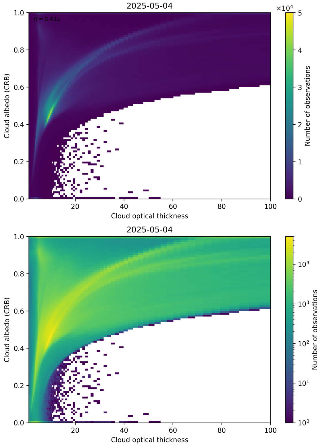
Figure 82: Scatter density plot of “Cloud optical thickness” against “Cloud albedo (CRB)” for 2025-05-03 to 2025-05-05.
