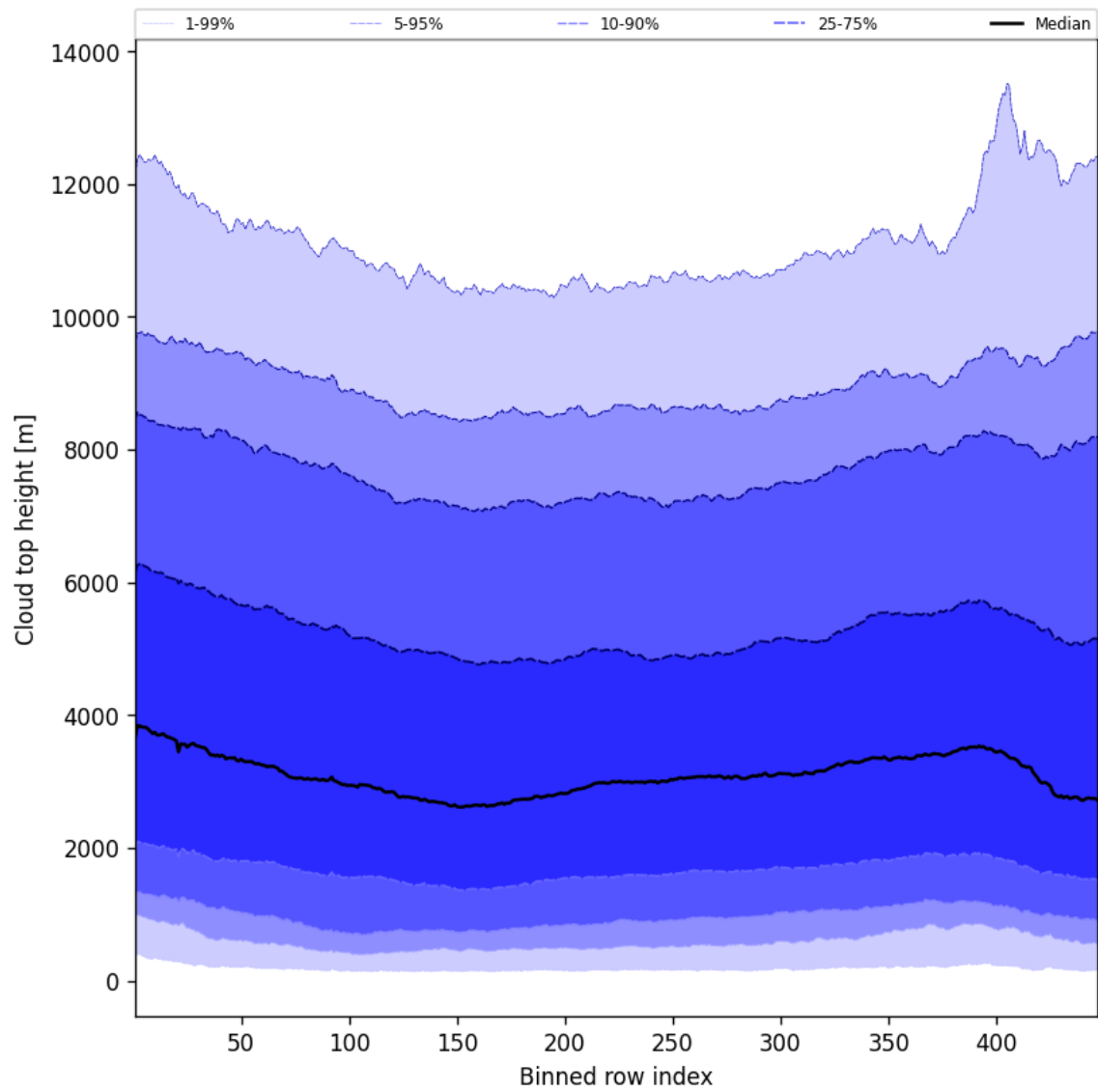
Figure 56: Along track statistics of “Cloud top height” for 2025-05-03 to 2025-05-05
