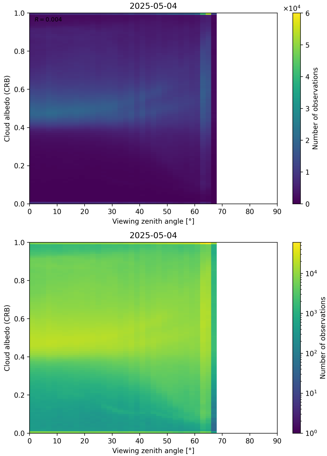
Figure 106: Scatter density plot of “Viewing zenith angle” against “Cloud albedo (CRB)” for 2025-05-03 to 2025-05-05.
