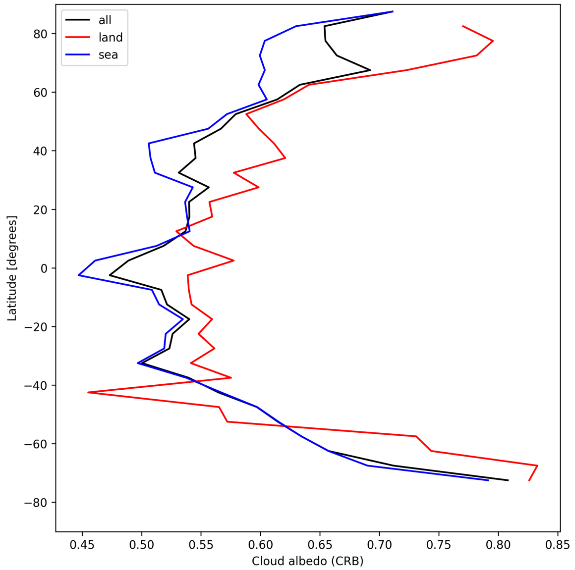
Figure 28: Zonal average of “Cloud albedo (CRB)” for 2025-05-03 to 2025-05-05.
