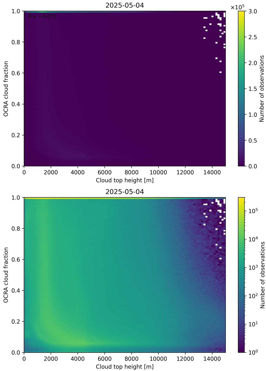
Figure 87: Scatter density plot of “Cloud top height” against “OCRA cloud fraction” for 2025-05-03 to 2025-05-05.
