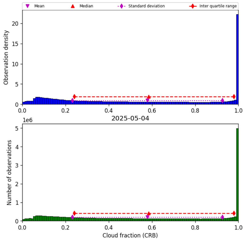
Figure 42: Histogram of “Cloud fraction (CRB)” for 2025-05-03 to 2025-05-05
