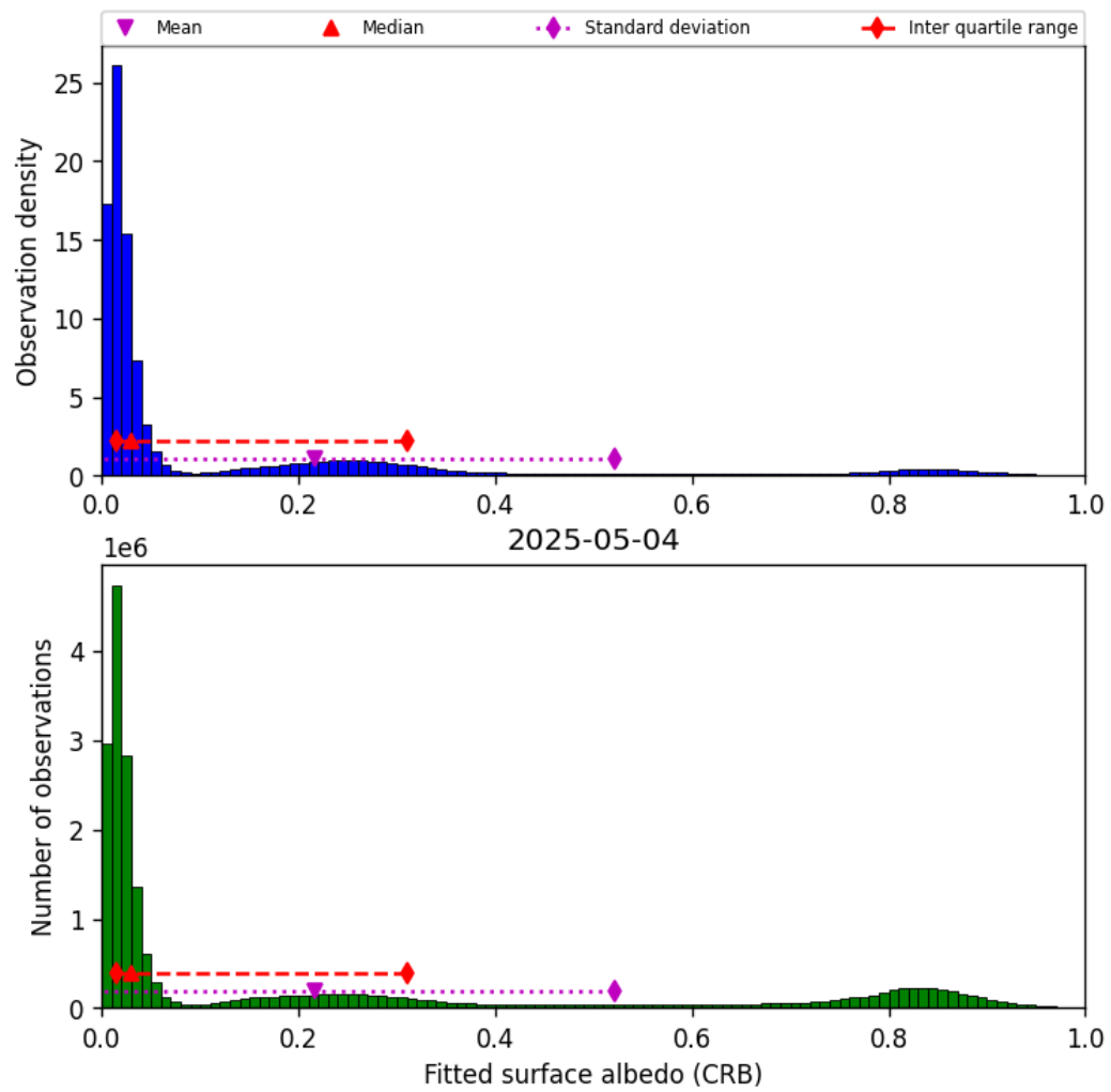
Figure 46: Histogram of “Fitted surface albedo (CRB)” for 2025-05-03 to 2025-05-05
