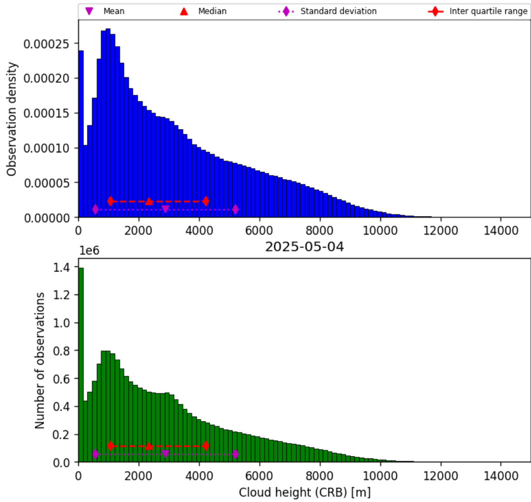
Figure 43: Histogram of “Cloud height (CRB)” for 2025-05-03 to 2025-05-05
