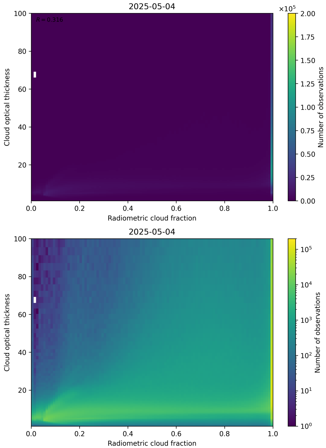
Figure 75: Scatter density plot of “Radiometric cloud fraction” against “Cloud optical thickness” for 2025-05-03 to 2025-05-05.
