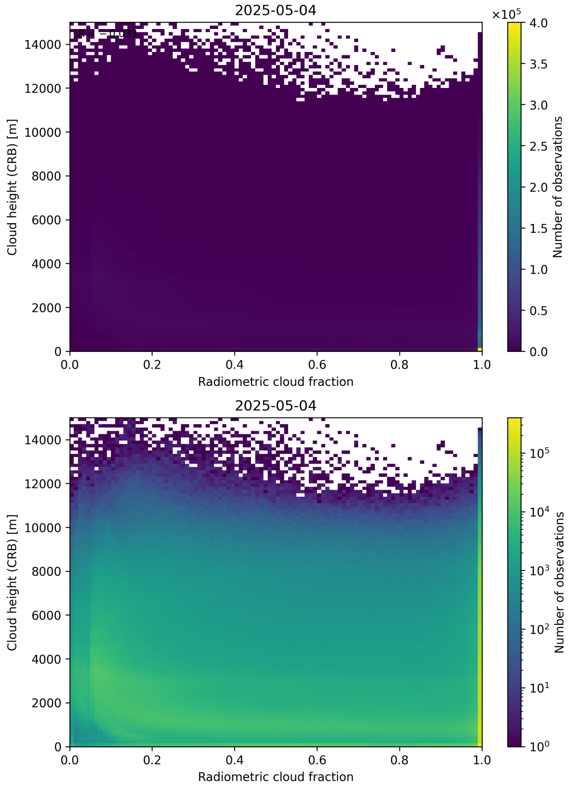
Figure 74: Scatter density plot of “Radiometric cloud fraction” against “Cloud height (CRB)” for 2025-05-03 to 2025-05-05.
