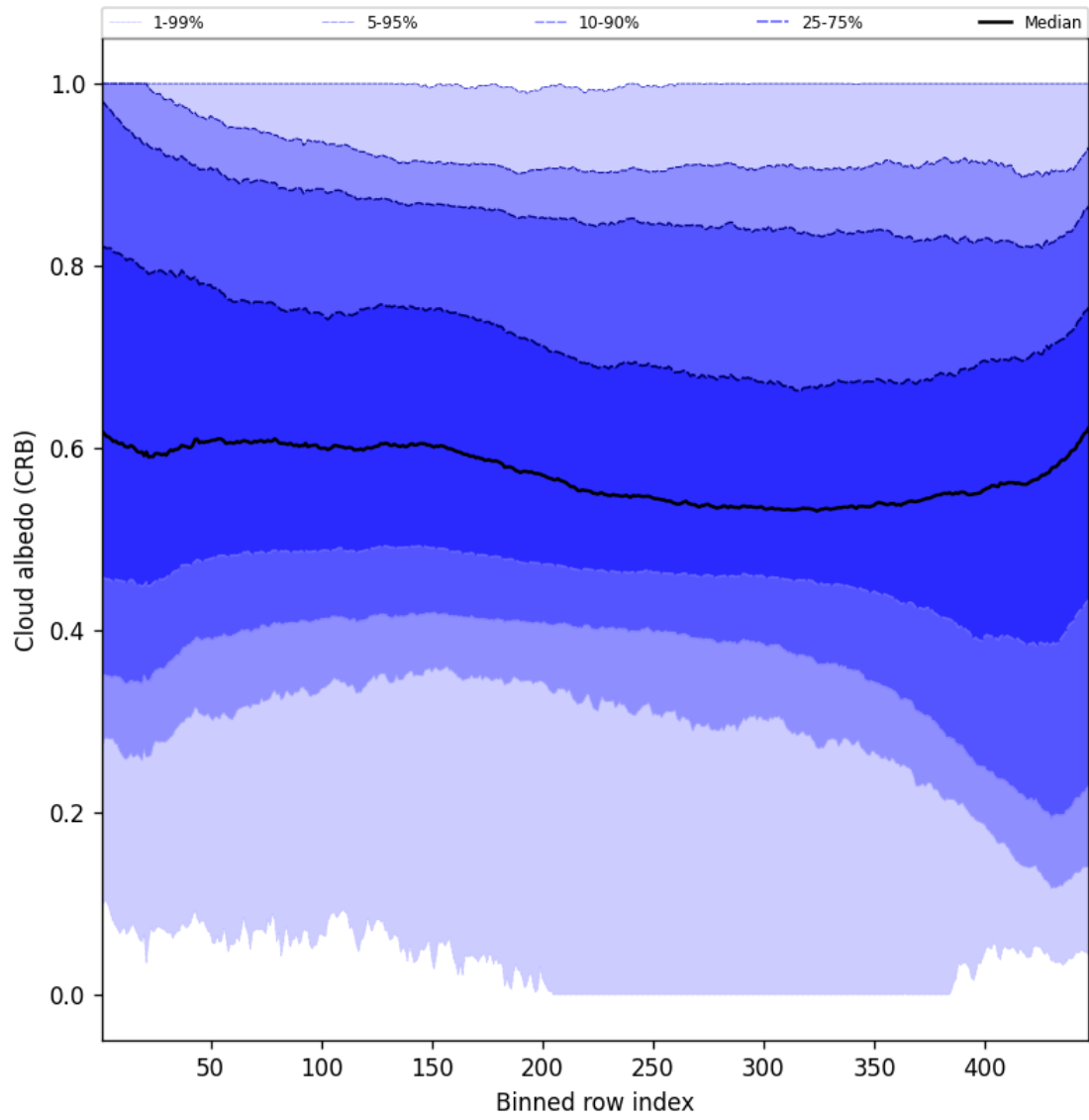
Figure 60: Along track statistics of “Cloud albedo (CRB)” for 2025-05-03 to 2025-05-05
