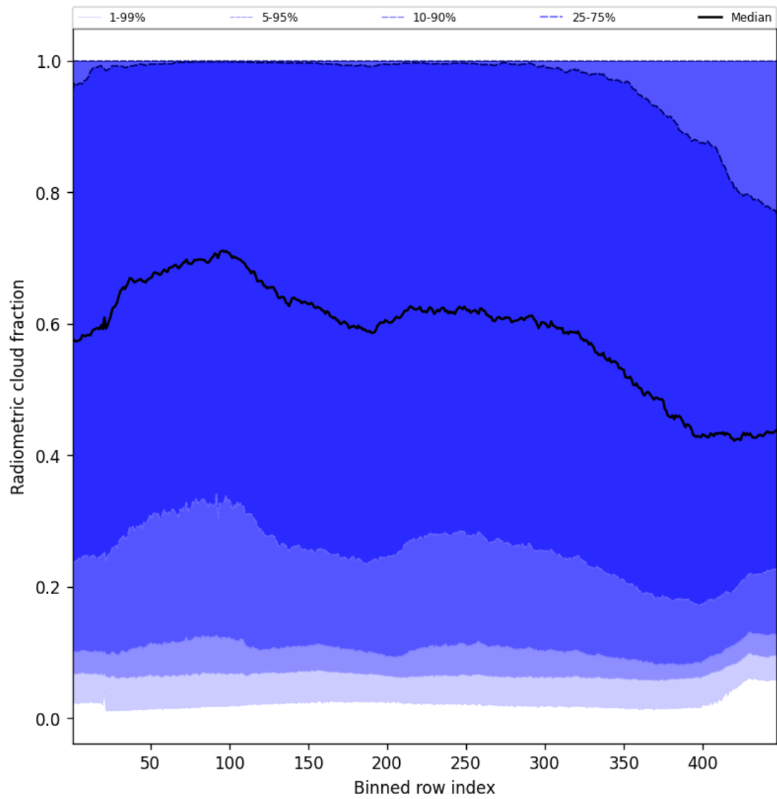
Figure 55: Along track statistics of “Radiometric cloud fraction” for 2025-05-03 to 2025-05-05
