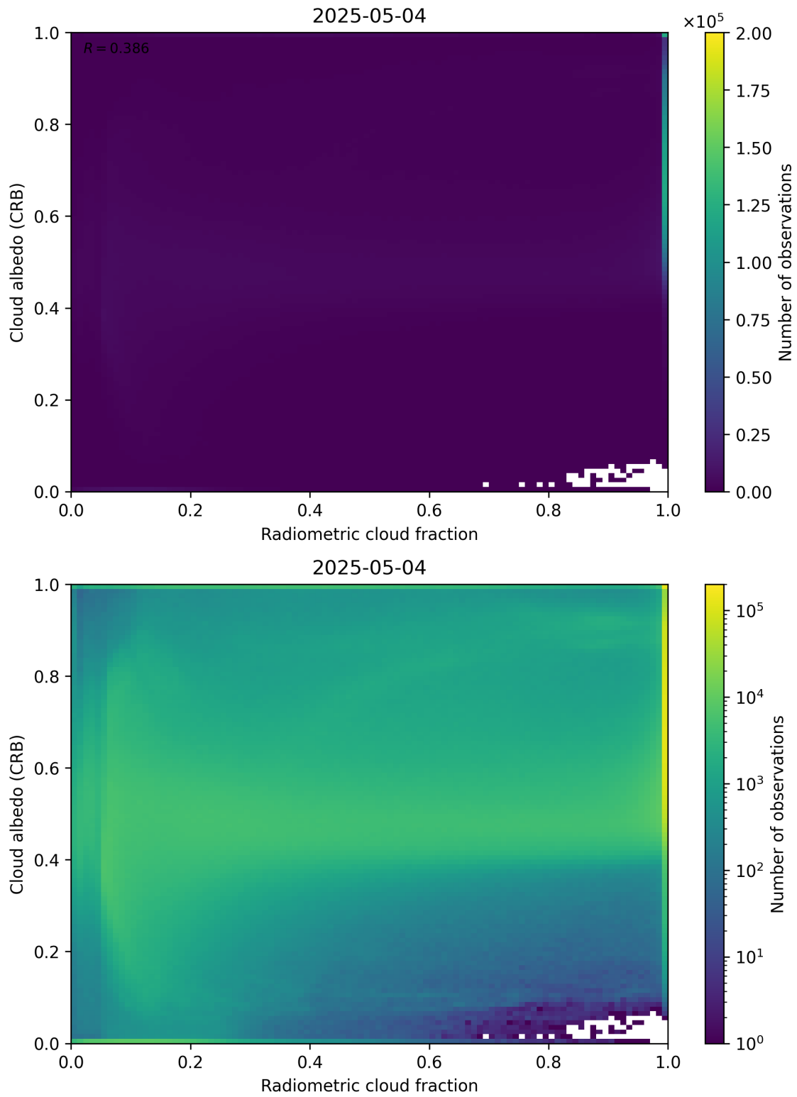
Figure 71: Scatter density plot of “Radiometric cloud fraction” against “Cloud albedo (CRB)” for 2025-05-03 to 2025-05-05.
