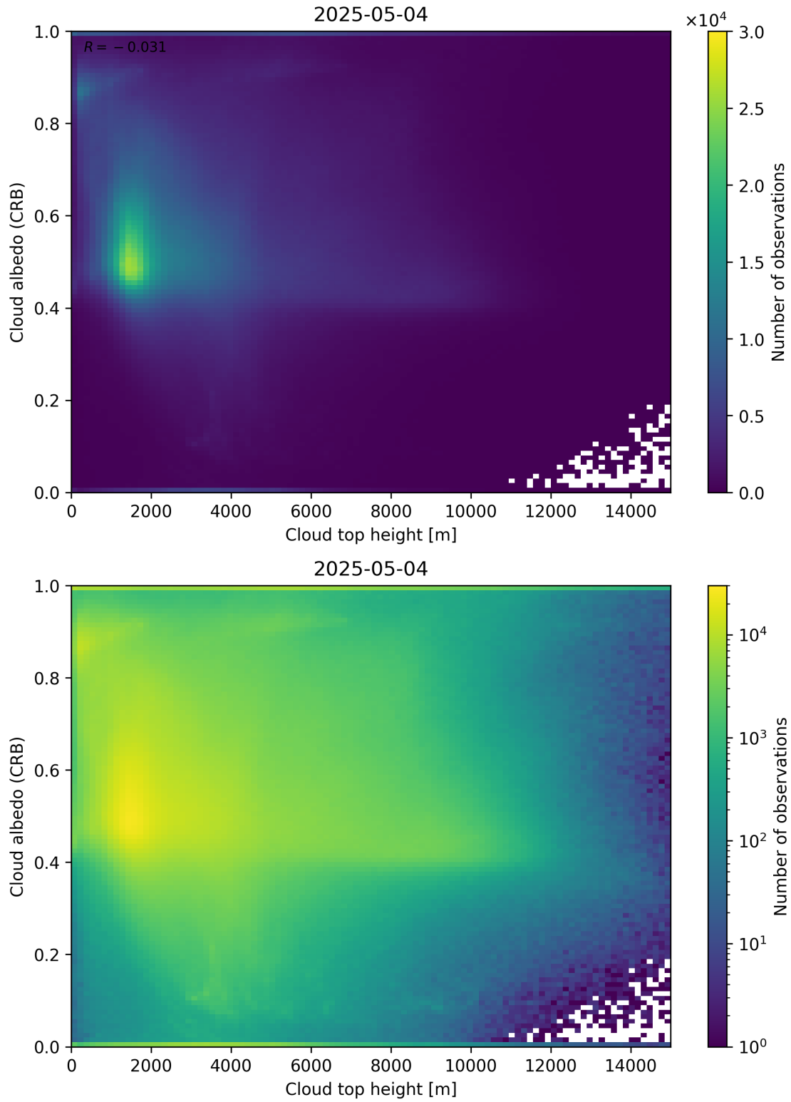
Figure 86: Scatter density plot of “Cloud top height” against “Cloud albedo (CRB)” for 2025-05-03 to 2025-05-05.
