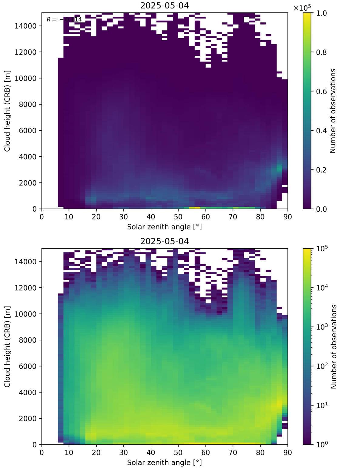
Figure 102: Scatter density plot of “Solar zenith angle” against “Cloud height (CRB)” for 2025-05-03 to 2025-05-05.
