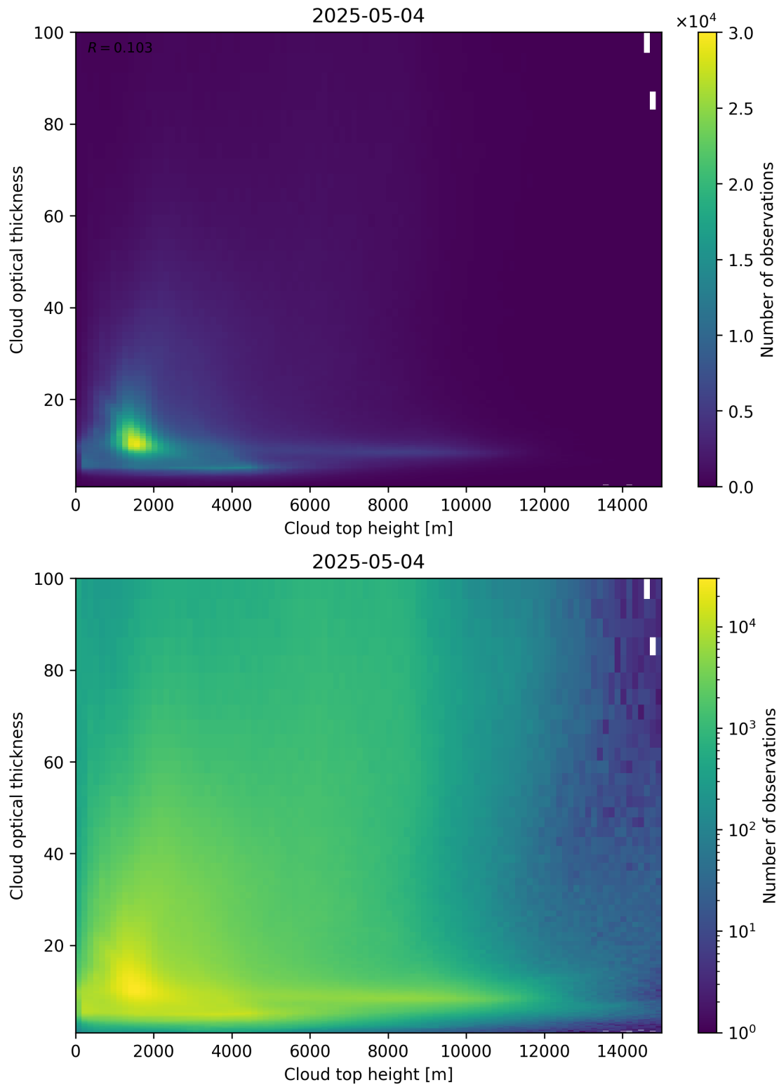
Figure 90: Scatter density plot of “Cloud top height” against “Cloud optical thickness” for 2025-05-03 to 2025-05-05.
