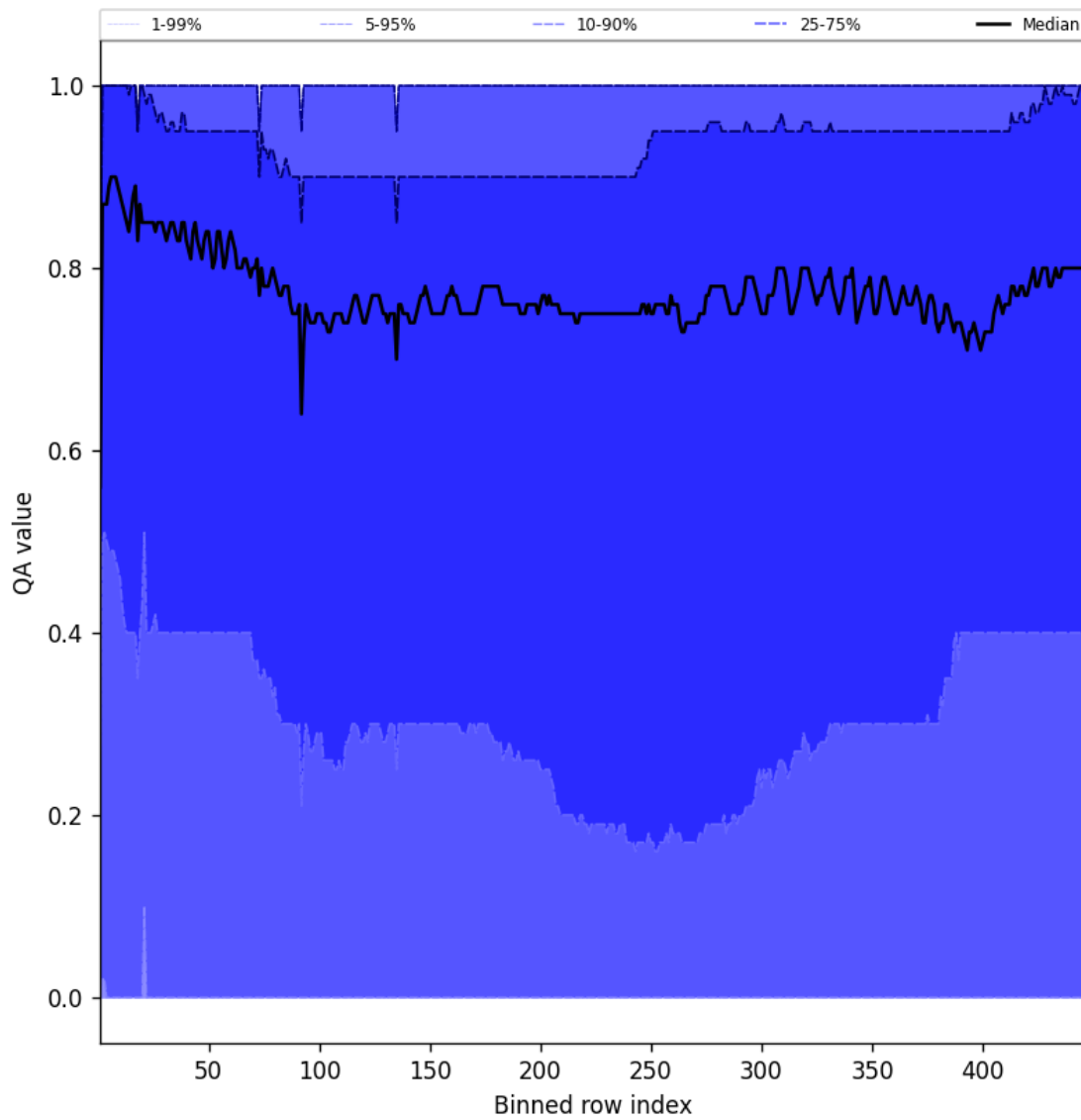
Figure 54: Along track statistics of “QA value” for 2025-05-03 to 2025-05-05
