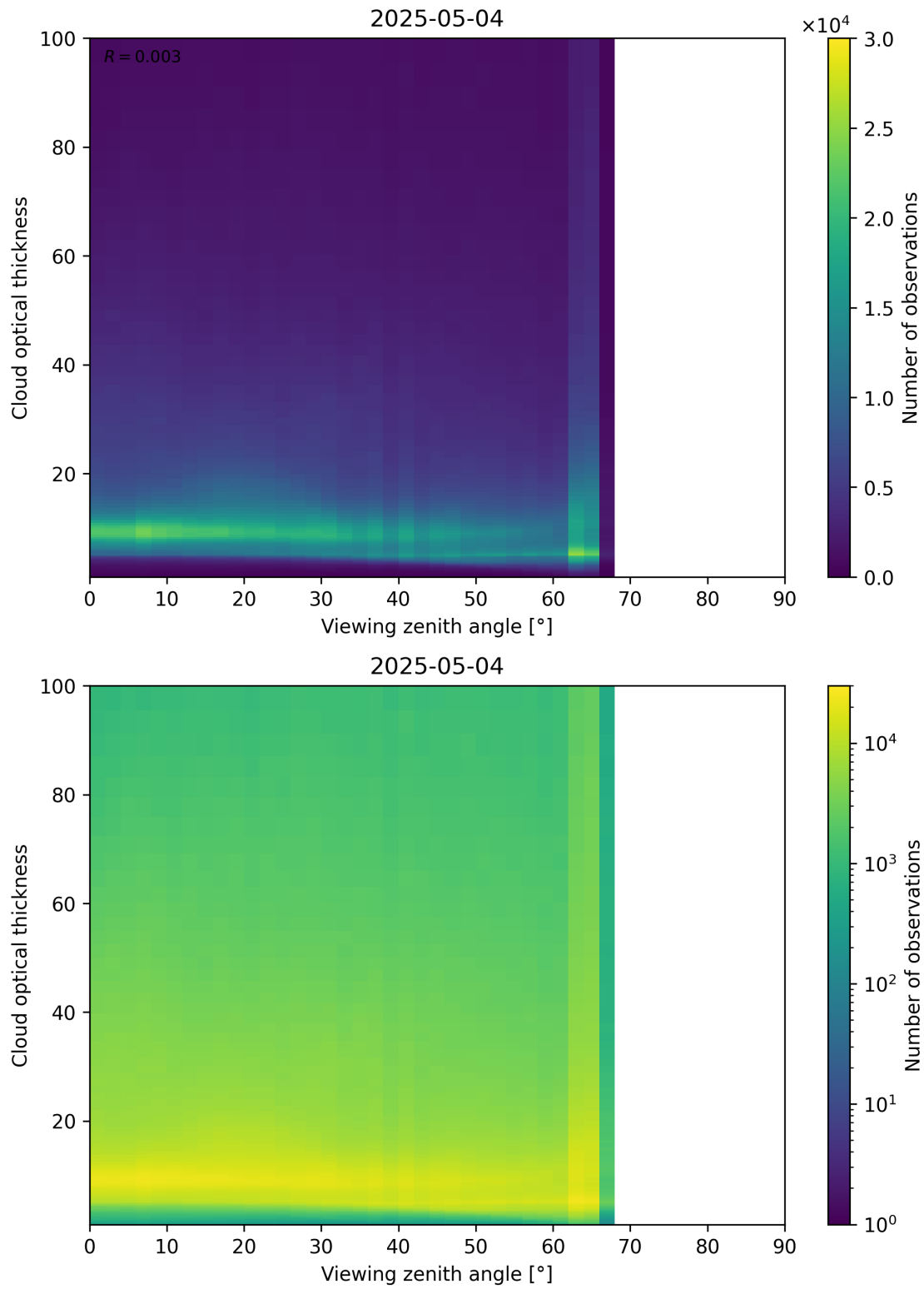
Figure 111: Scatter density plot of “Viewing zenith angle” against “Cloud optical thickness” for 2025-05-03 to 2025-05-05.
