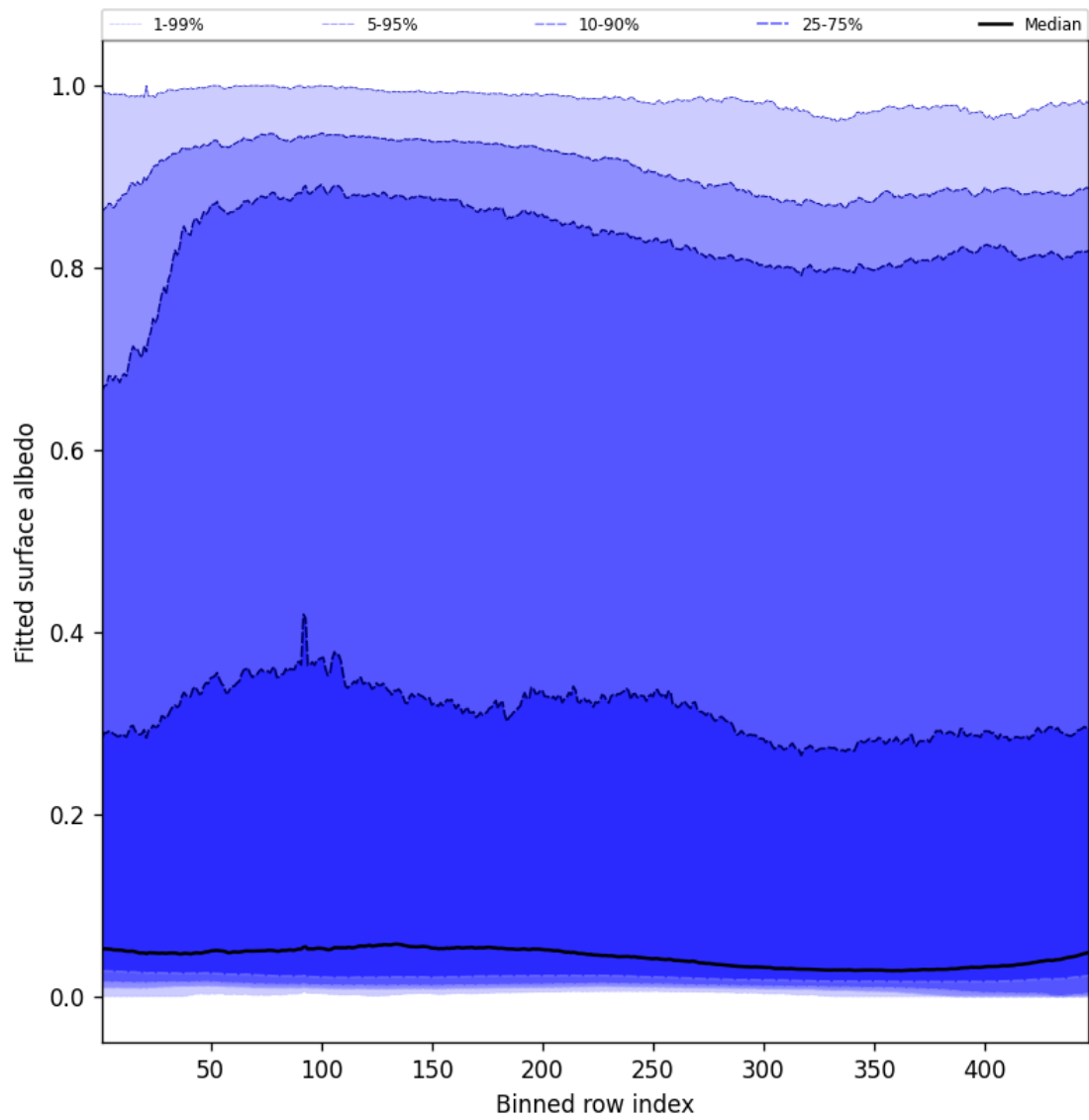
Figure 61: Along track statistics of “Fitted surface albedo” for 2025-05-03 to 2025-05-05
