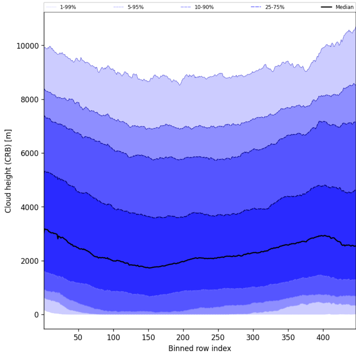
Figure 59: Along track statistics of “Cloud height (CRB)” for 2025-05-03 to 2025-05-05
