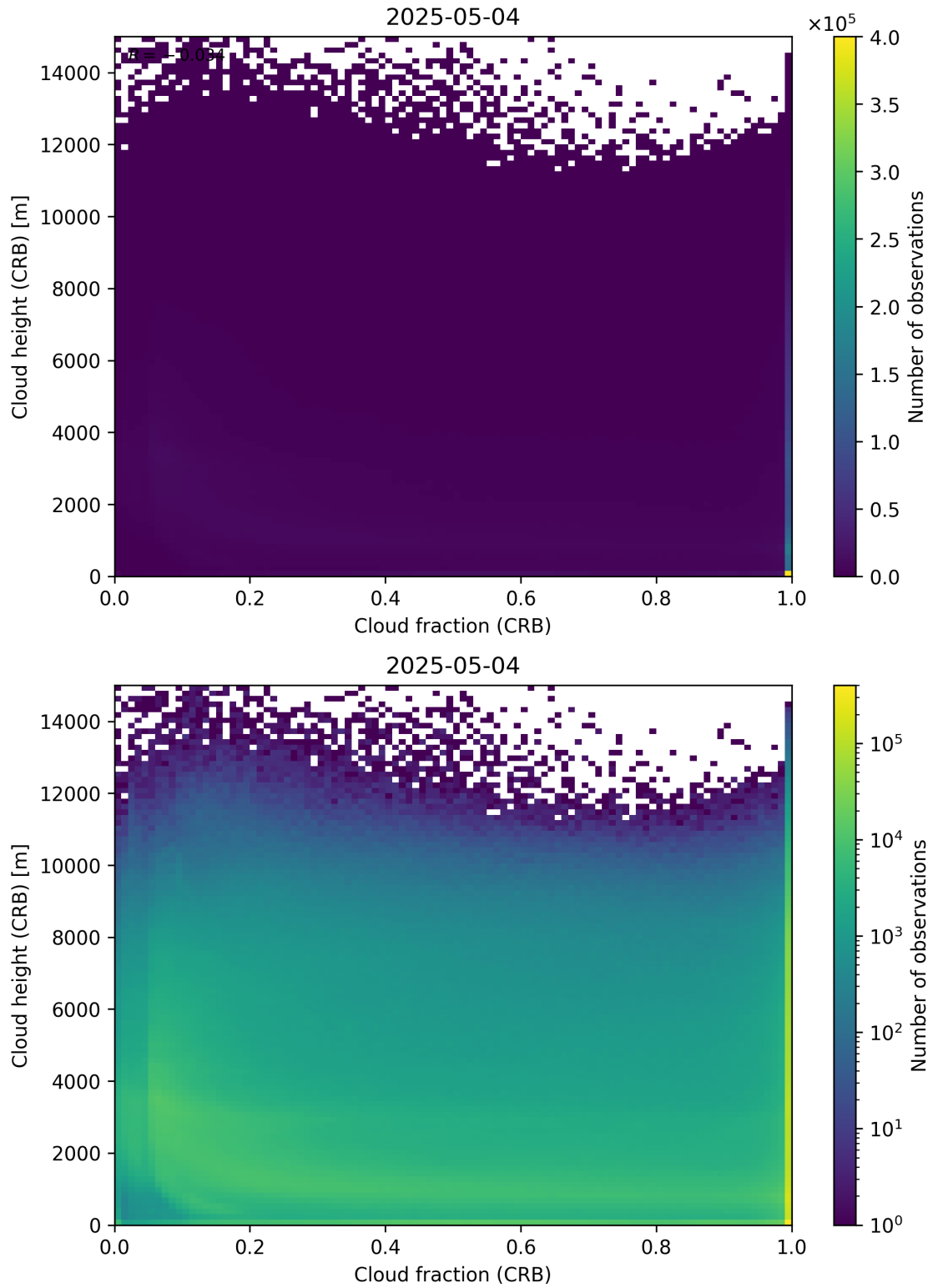
Figure 79: Scatter density plot of “Cloud fraction (CRB)” against “Cloud height (CRB)” for 2025-05-03 to 2025-05-05.
