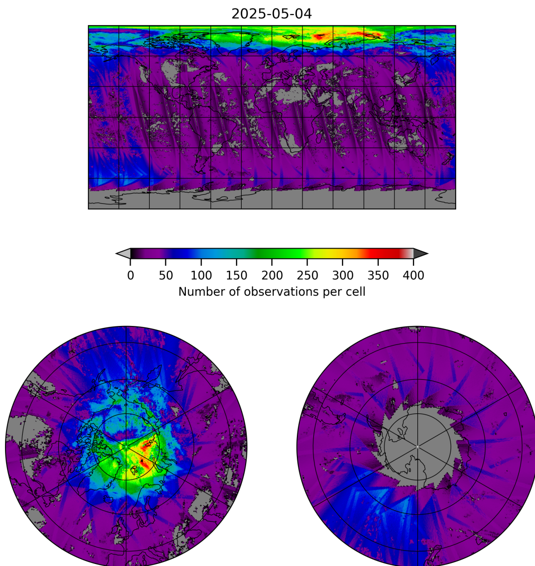
Figure 21: Map of the number of observations for 2025-05-03 to 2025-05-05
