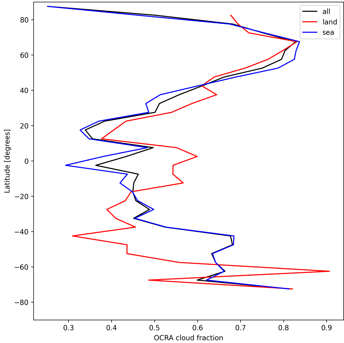
Figure 34: Zonal average of “OCRA cloud fraction” for 2025-05-03 to 2025-05-05.
