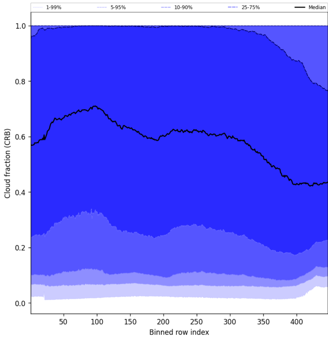
Figure 58: Along track statistics of “Cloud fraction (CRB)” for 2025-05-03 to 2025-05-05
