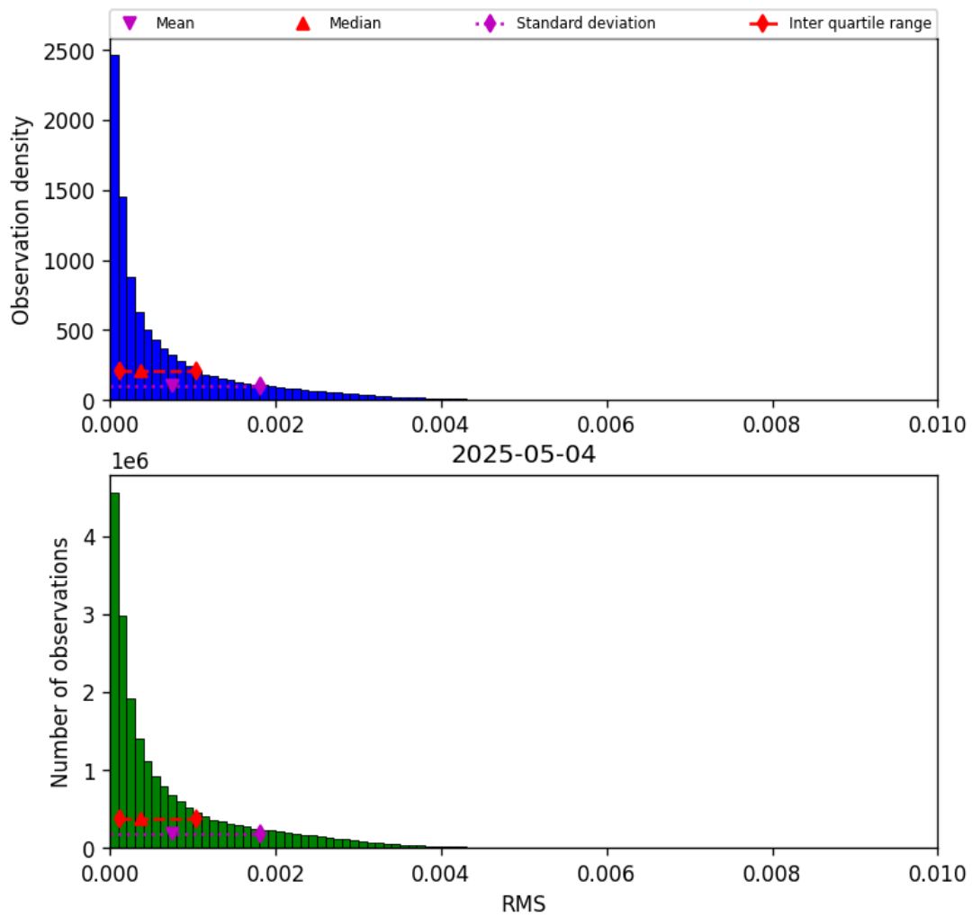
Figure 47: Histogram of “RMS” for 2025-05-03 to 2025-05-05
