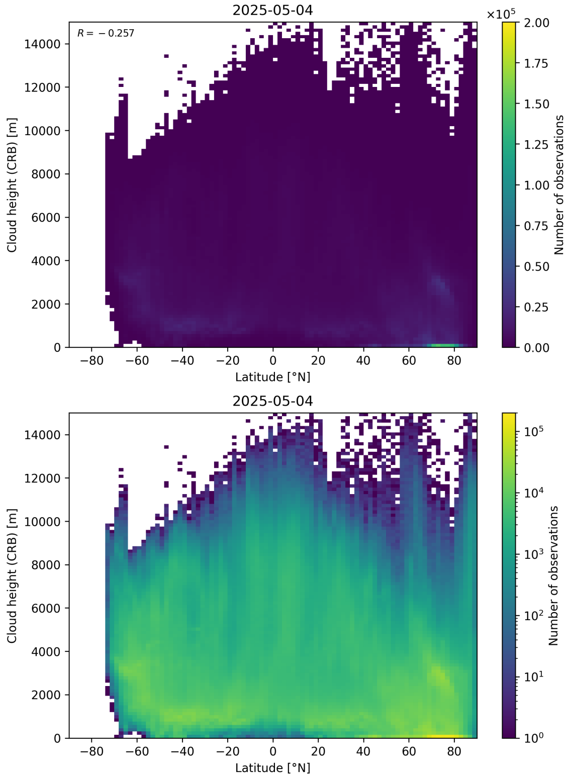
Figure 95: Scatter density plot of “Latitude” against “Cloud height (CRB)” for 2025-05-03 to 2025-05-05.
