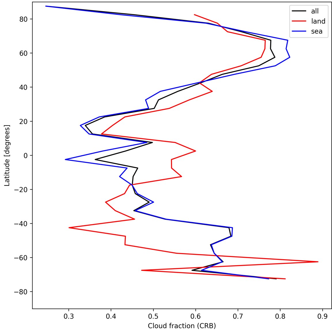
Figure 26: Zonal average of “Cloud fraction (CRB)” for 2025-05-03 to 2025-05-05.
