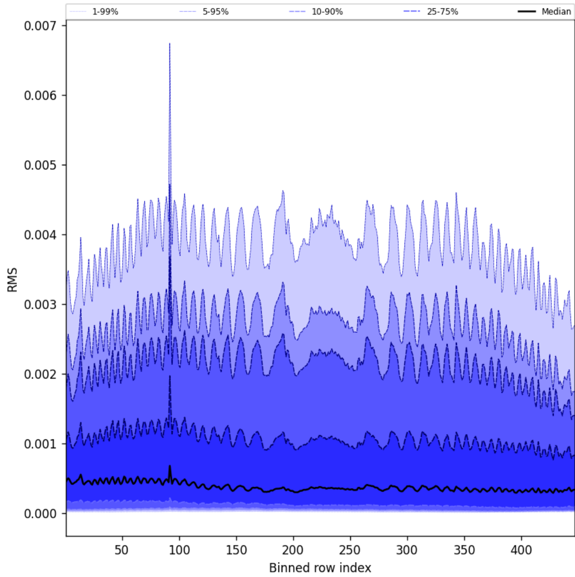
Figure 63: Along track statistics of “RMS” for 2025-05-03 to 2025-05-05
