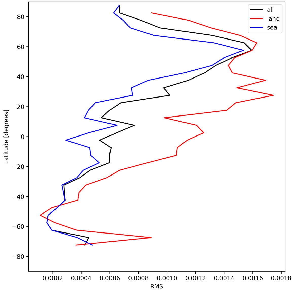
Figure 31: Zonal average of “RMS” for 2025-05-03 to 2025-05-05.
