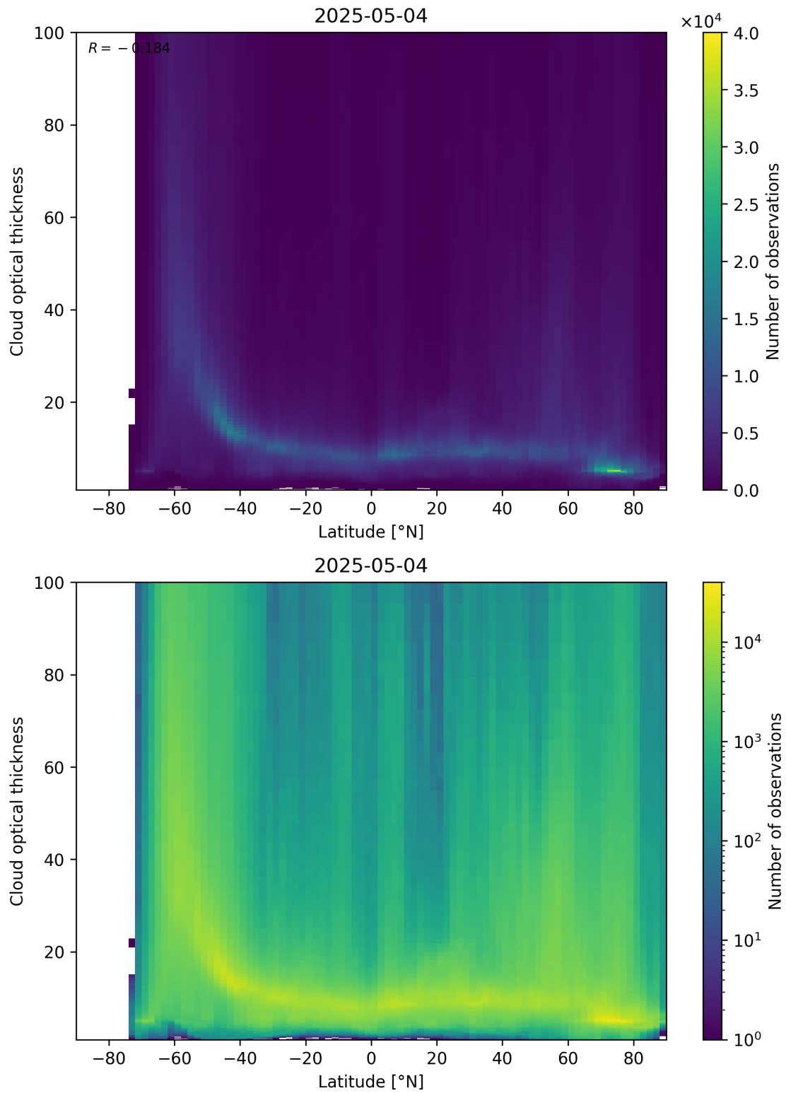
Figure 96: Scatter density plot of “Latitude” against “Cloud optical thickness” for 2025-05-03 to 2025-05-05.
