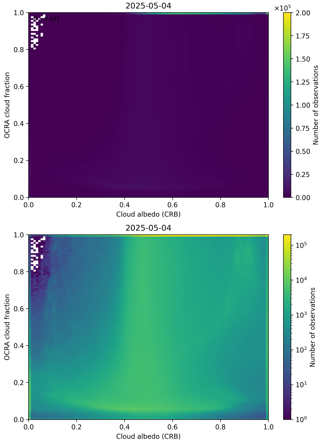
Figure 70: Scatter density plot of “Cloud albedo (CRB)” against “OCRA cloud fraction” for 2025-05-03 to 2025-05-05.
