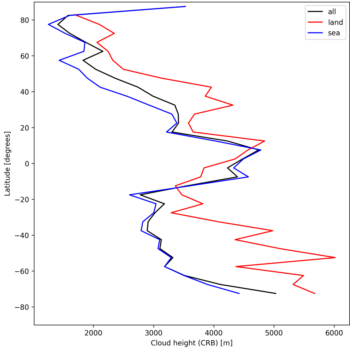
Figure 27: Zonal average of “Cloud height (CRB)” for 2025-05-03 to 2025-05-05.
