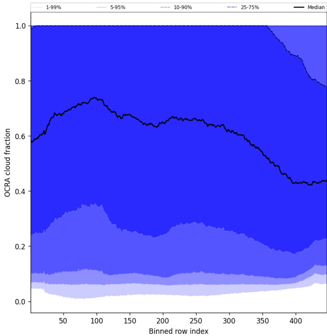
Figure 66: Along track statistics of “OCRA cloud fraction” for 2025-05-03 to 2025-05-05
