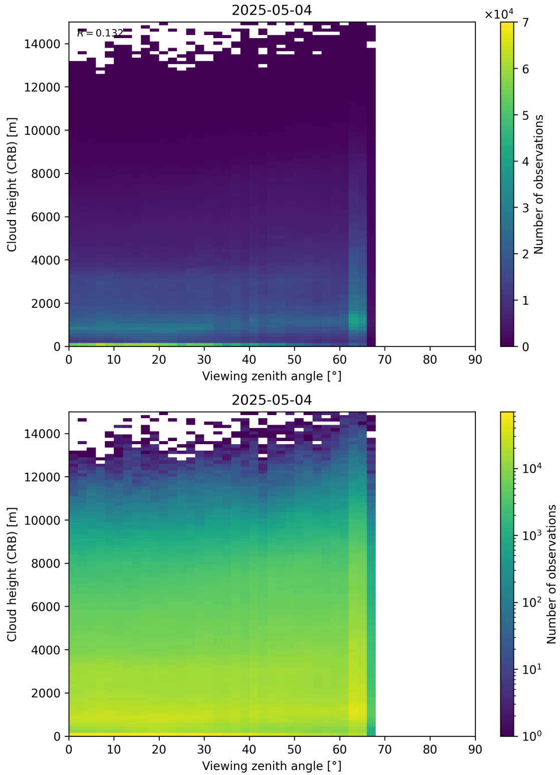
Figure 110: Scatter density plot of “Viewing zenith angle” against “Cloud height (CRB)” for 2025-05-03 to 2025-05-05.
