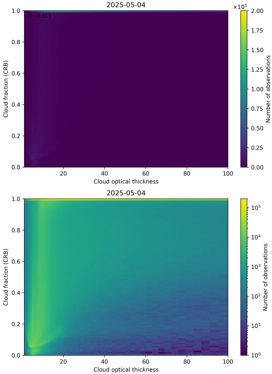
Figure 84: Scatter density plot of “Cloud optical thickness” against “Cloud fraction (CRB)” for 2025-05-03 to 2025-05-05.
