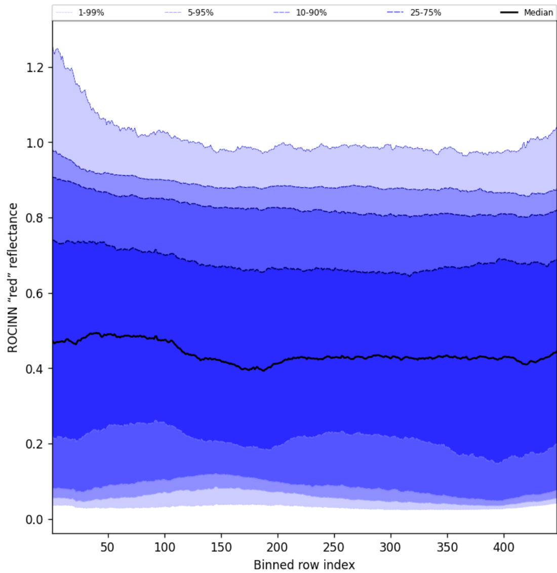
Figure 69: Along track statistics of "ROCINN "red" reflectance" for 2025-05-03 to 2025-05-05
