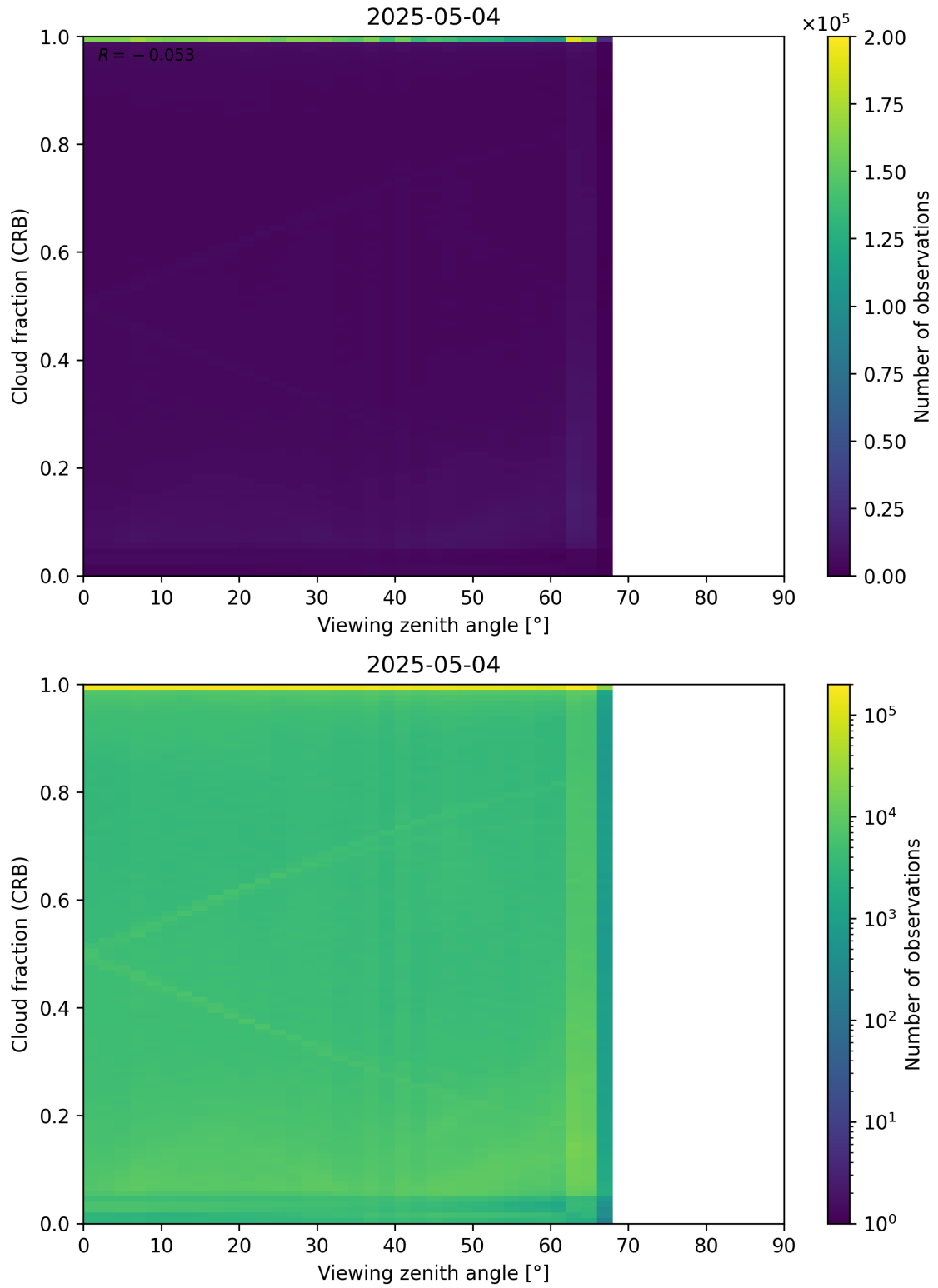
Figure 109: Scatter density plot of “Viewing zenith angle” against “Cloud fraction (CRB)” for 2025-05-03 to 2025-05-05.
