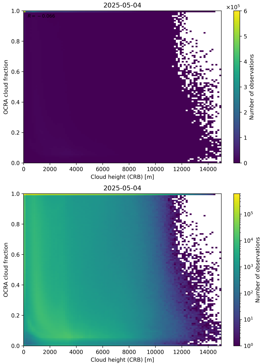
Figure 81: Scatter density plot of “Cloud height (CRB)” against “OCRA cloud fraction” for 2025-05-03 to 2025-05-05.
