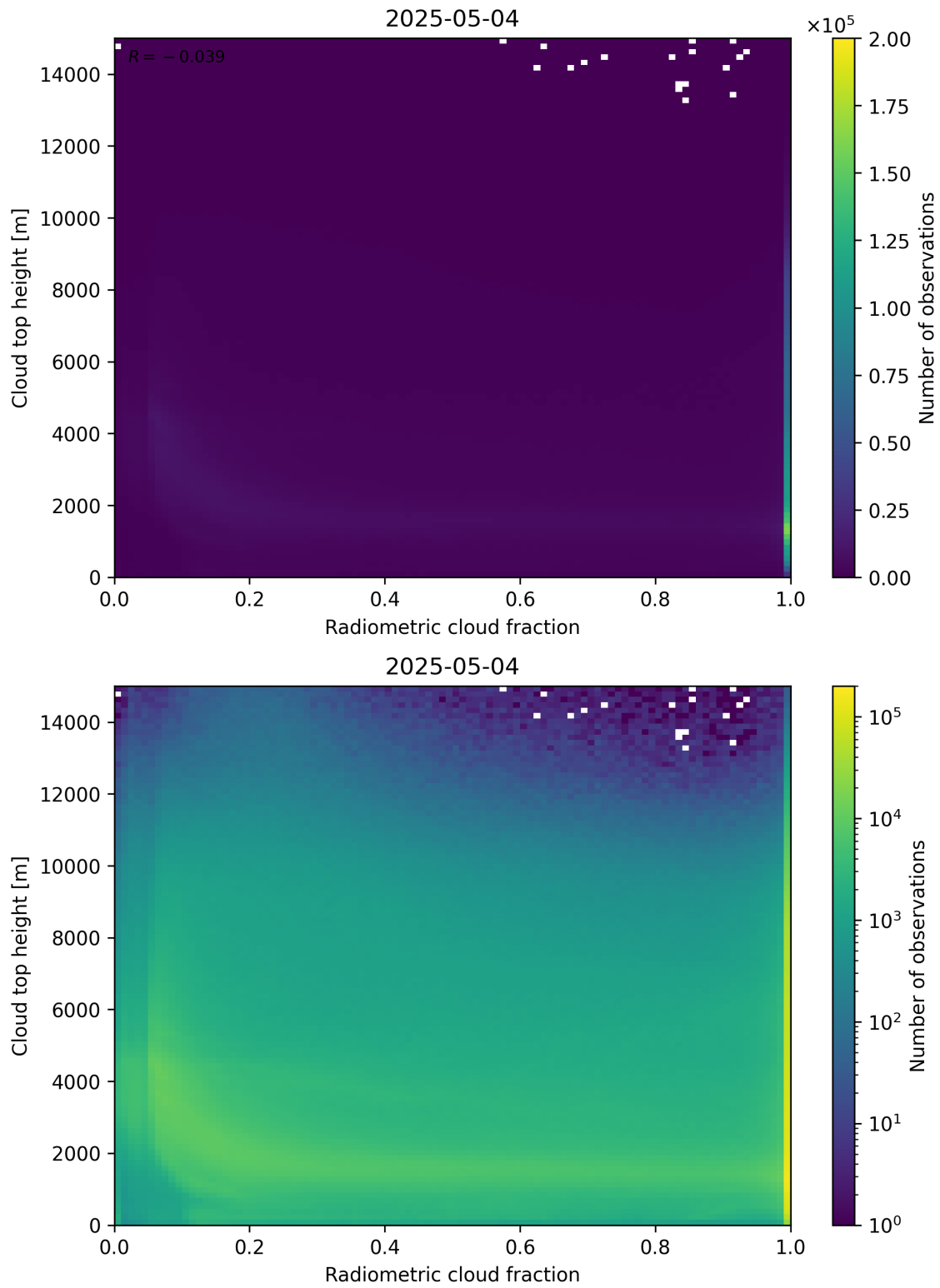
Figure 76: Scatter density plot of “Radiometric cloud fraction” against “Cloud top height” for 2025-05-03 to 2025-05-05.
