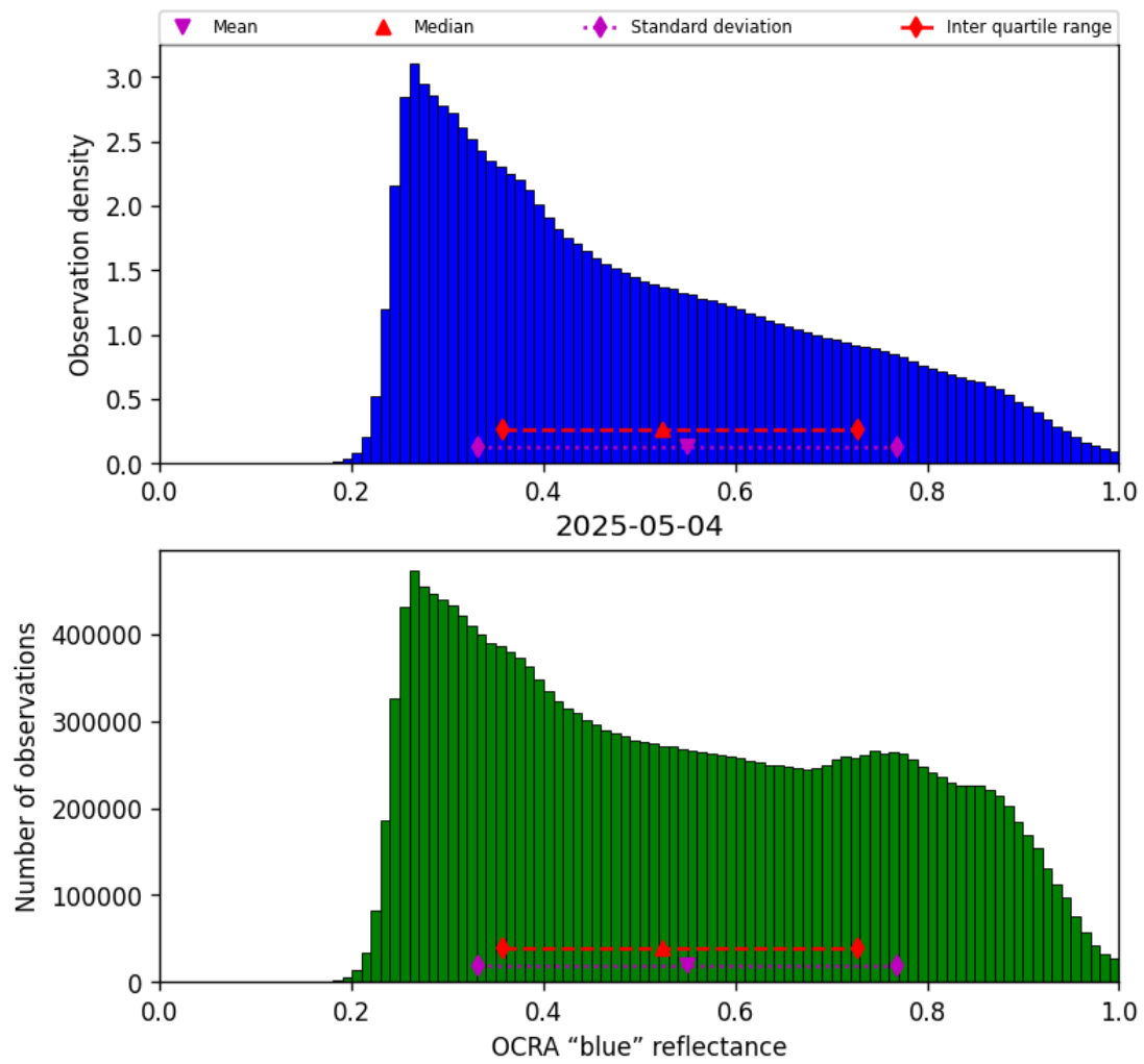
Figure 51: Histogram of “OCRA “blue” reflectance” for 2025-05-03 to 2025-05-05
