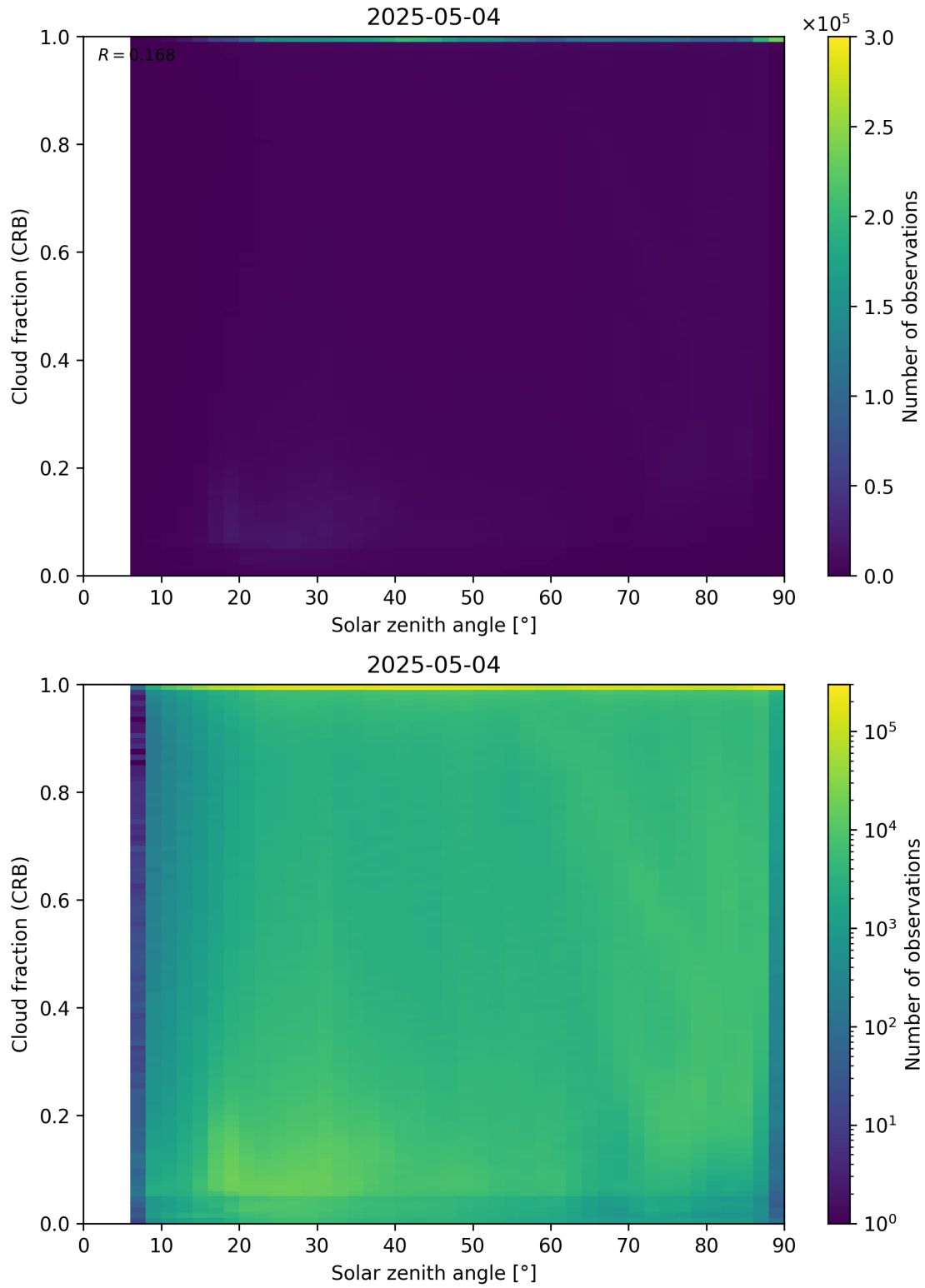
Figure 101: Scatter density plot of “Solar zenith angle” against “Cloud fraction (CRB)” for 2025-05-03 to 2025-05-05.
