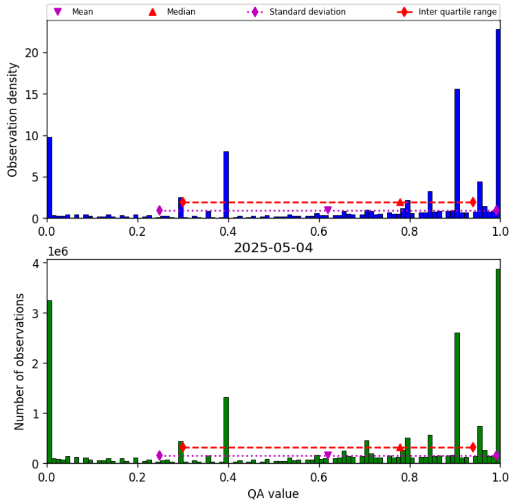
Figure 38: Histogram of “QA value” for 2025-05-03 to 2025-05-05
