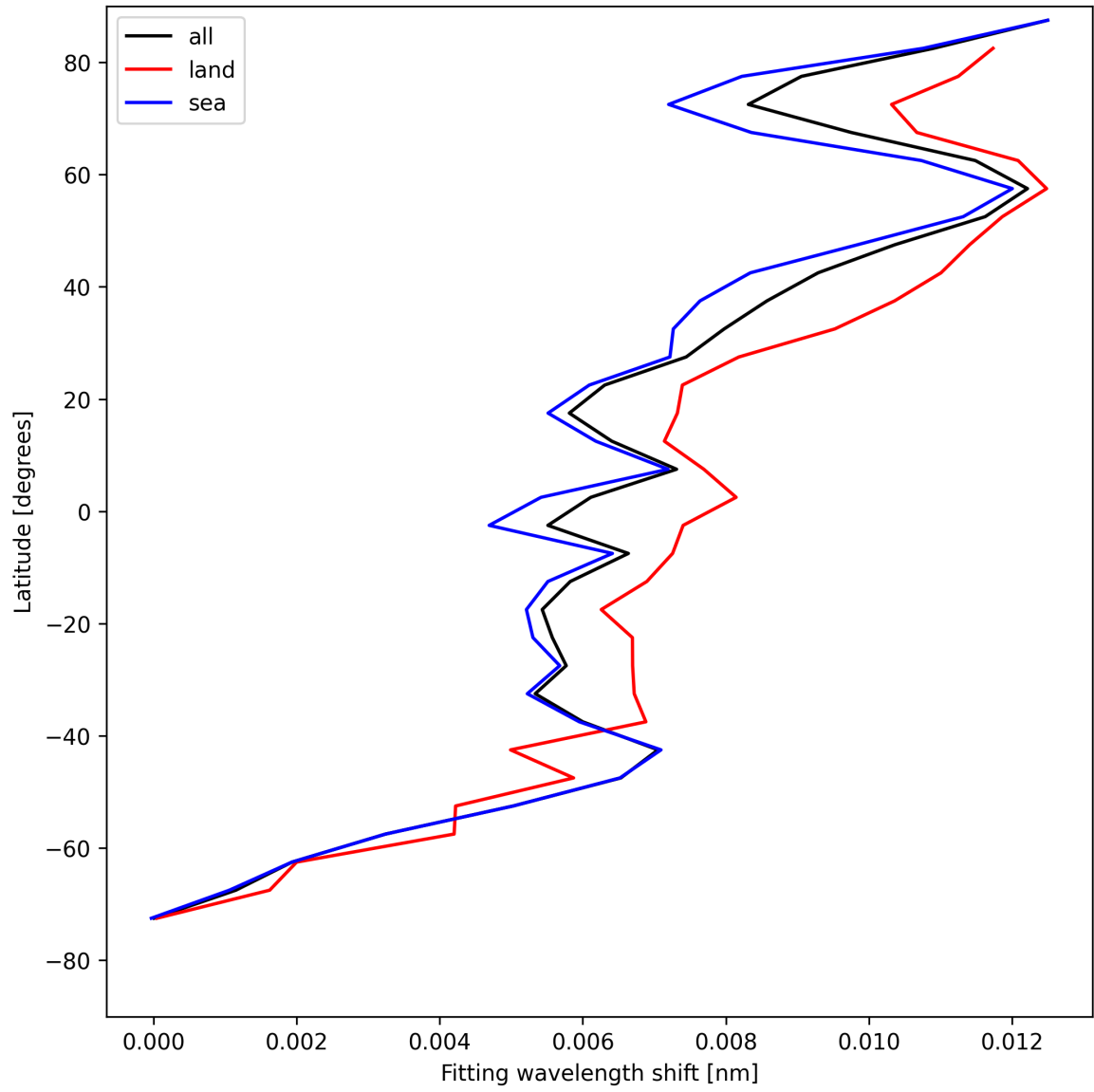
Figure 33: Zonal average of “Fitting wavelength shift” for 2025-05-03 to 2025-05-05.
