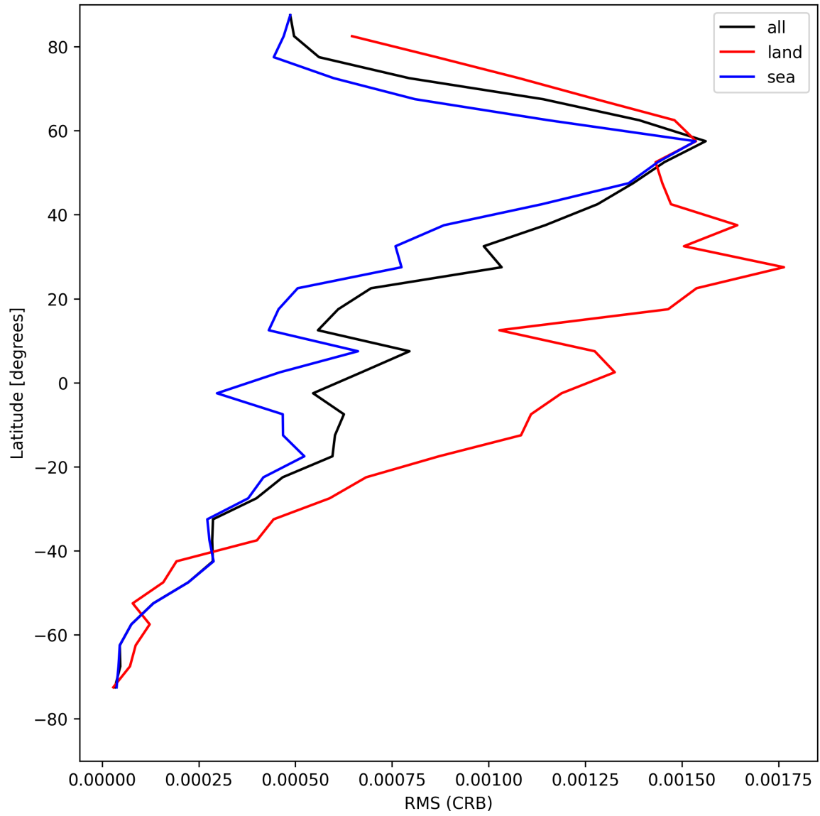
Figure 32: Zonal average of “RMS (CRB)” for 2025-05-03 to 2025-05-05.
