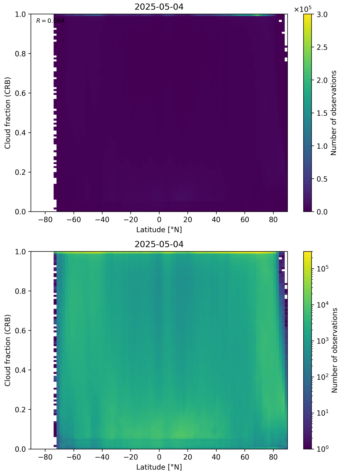
Figure 94: Scatter density plot of “Latitude” against “Cloud fraction (CRB)” for 2025-05-03 to 2025-05-05.
