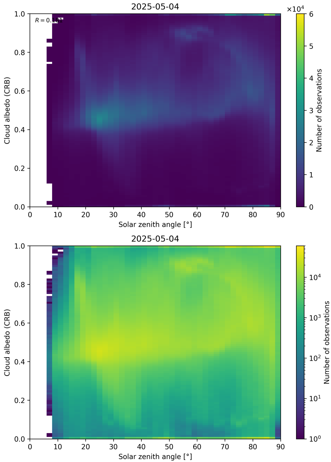
Figure 98: Scatter density plot of “Solar zenith angle” against “Cloud albedo (CRB)” for 2025-05-03 to 2025-05-05.
