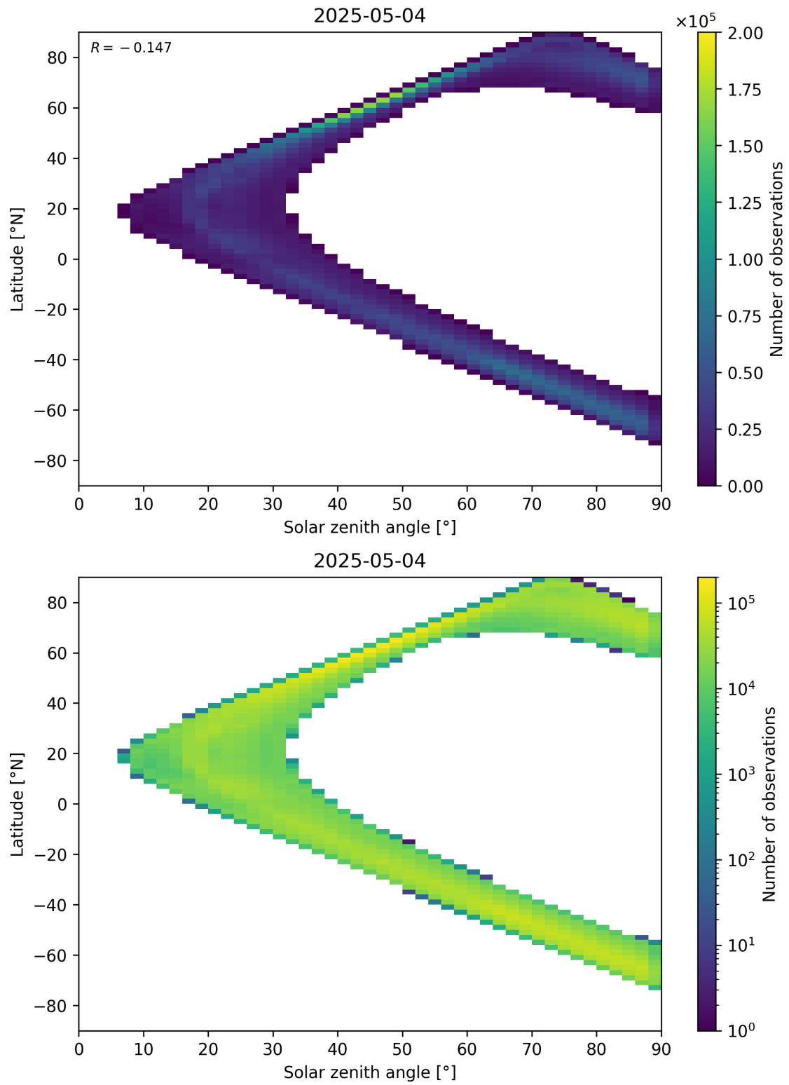
Figure 105: Scatter density plot of “Solar zenith angle” against “Latitude” for 2025-05-03 to 2025-05-05.
