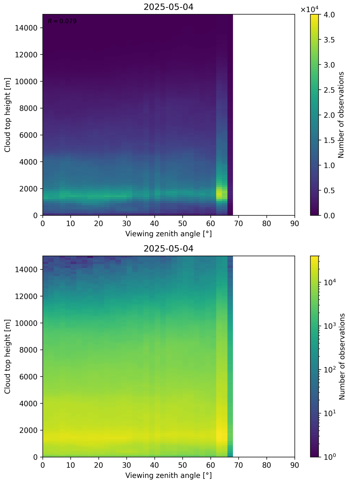
Figure 112: Scatter density plot of “Viewing zenith angle” against “Cloud top height” for 2025-05-03 to 2025-05-05.
