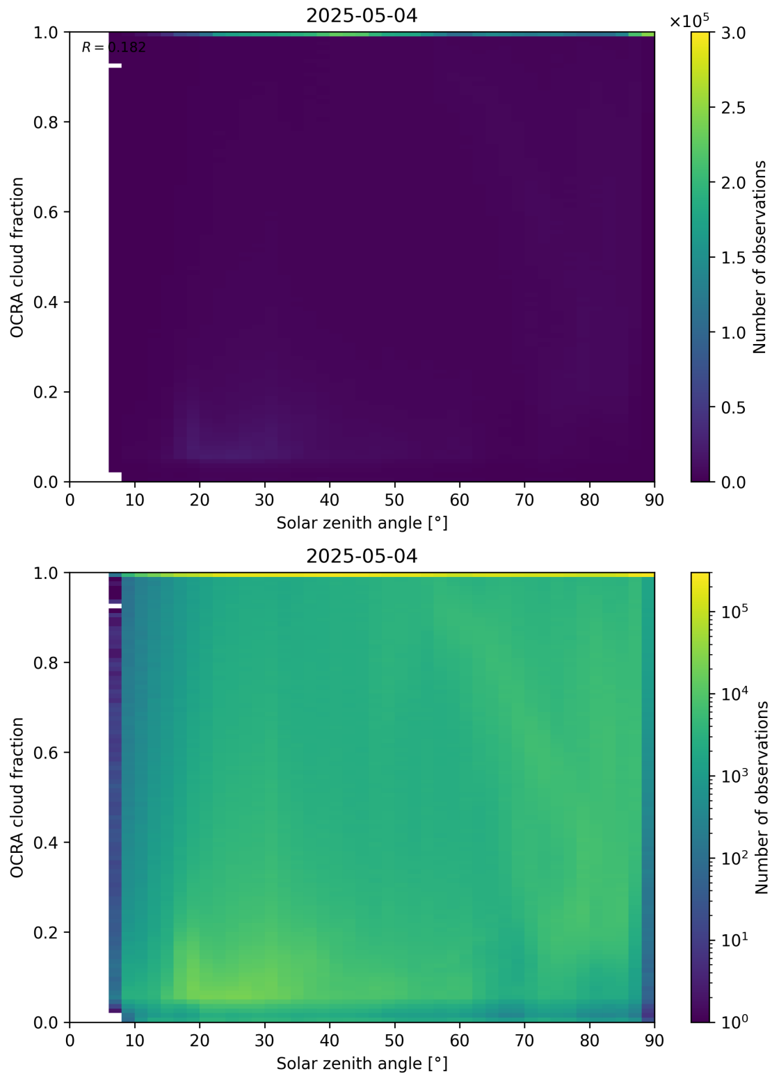
Figure 100: Scatter density plot of “Solar zenith angle” against “OCRA cloud fraction” for 2025-05-03 to 2025-05-05.
