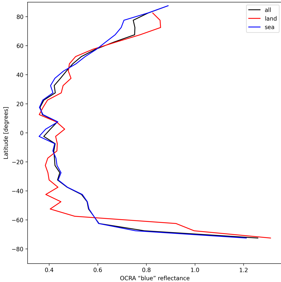
Figure 35: Zonal average of “OCRA “blue” reflectance” for 2025-05-03 to 2025-05-05.
