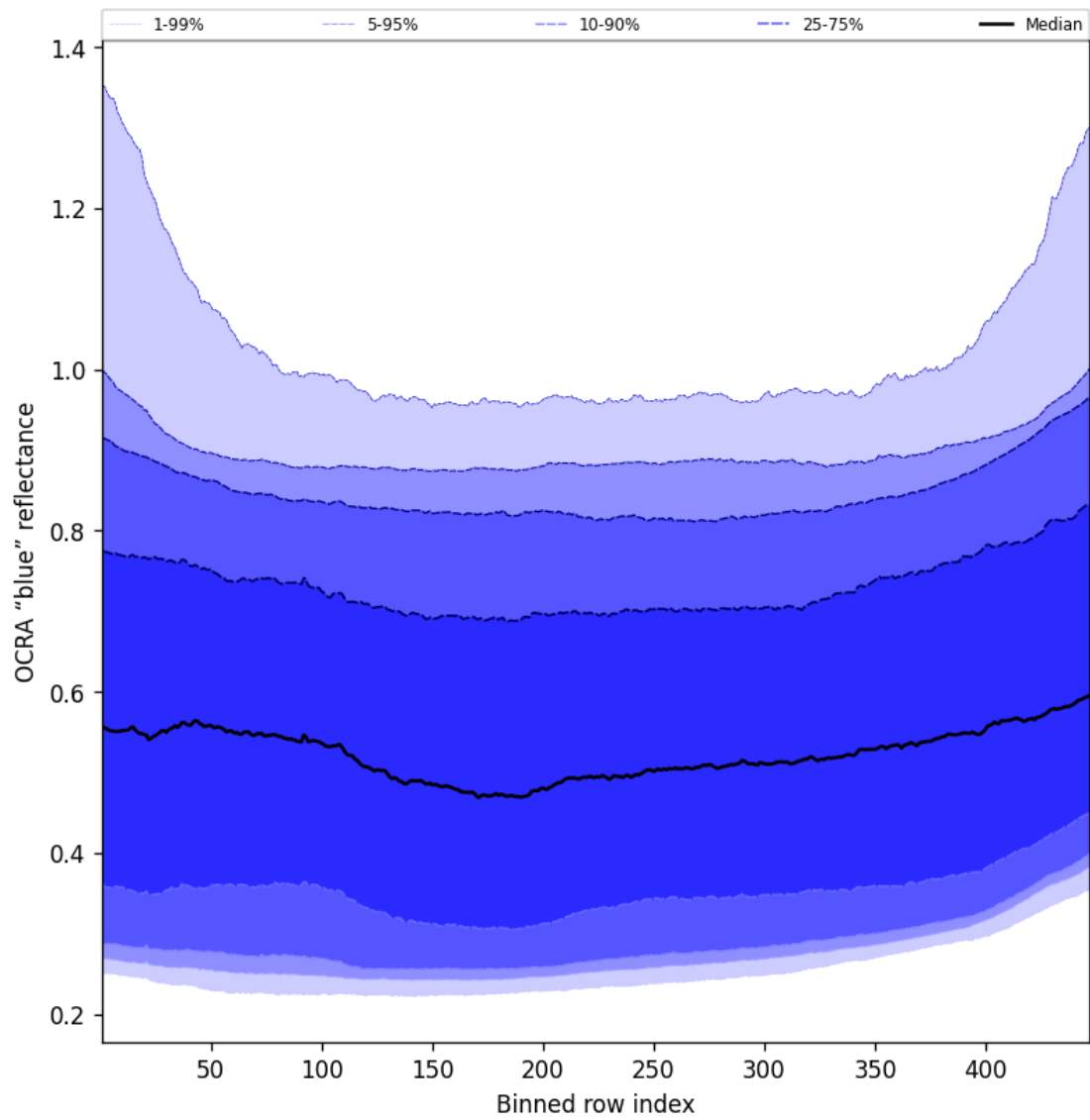
Figure 67: Along track statistics of “OCRA “blue” reflectance” for 2025-05-03 to 2025-05-05
