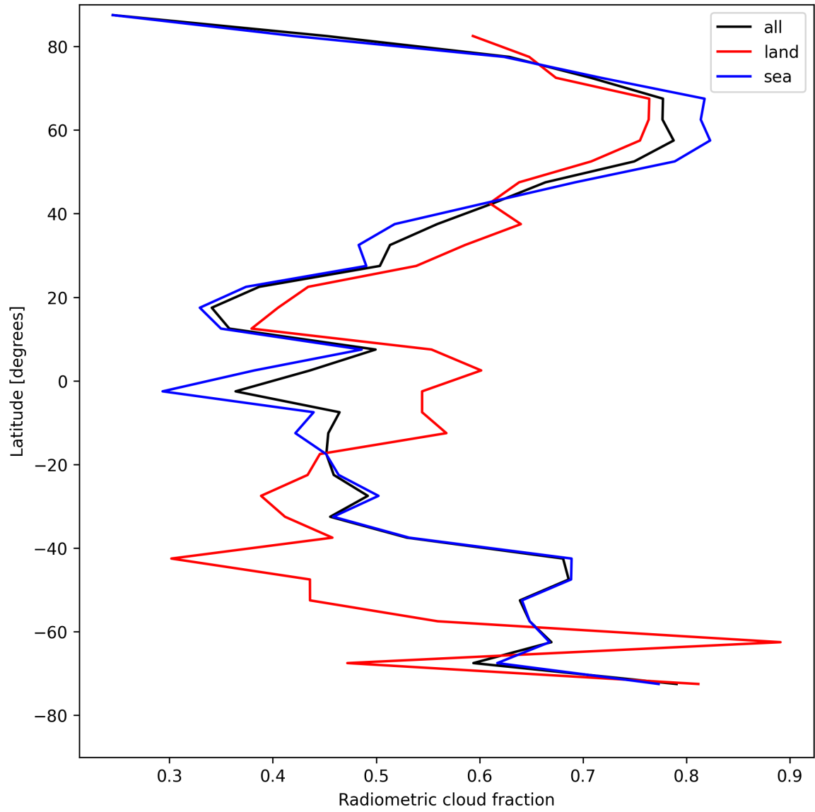
Figure 23: Zonal average of “Radiometric cloud fraction” for 2025-05-03 to 2025-05-05.
