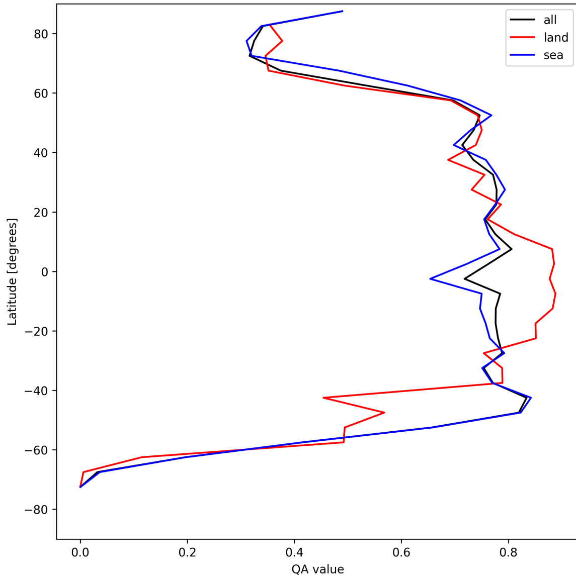
Figure 22: Zonal average of “QA value” for 2025-05-03 to 2025-05-05.
