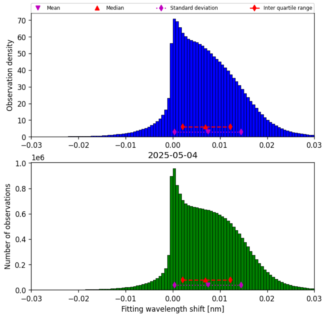
Figure 49: Histogram of “Fitting wavelength shift” for 2025-05-03 to 2025-05-05
