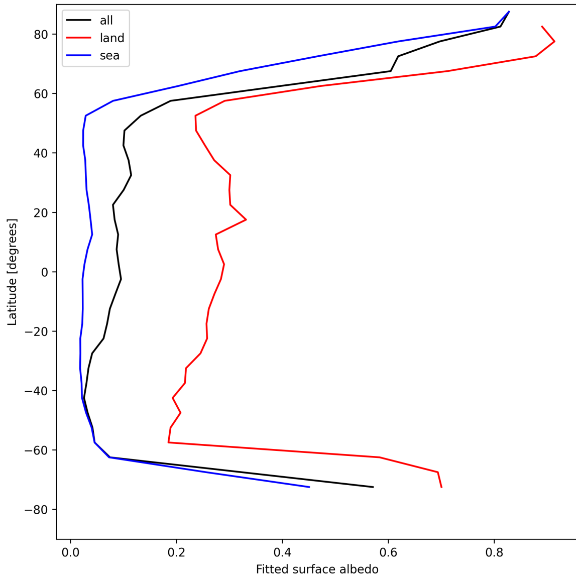
Figure 29: Zonal average of “Fitted surface albedo” for 2025-05-03 to 2025-05-05.
