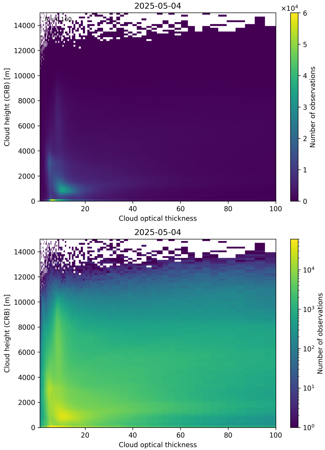
Figure 85: Scatter density plot of “Cloud optical thickness” against “Cloud height (CRB)” for 2025-05-03 to 2025-05-05.
