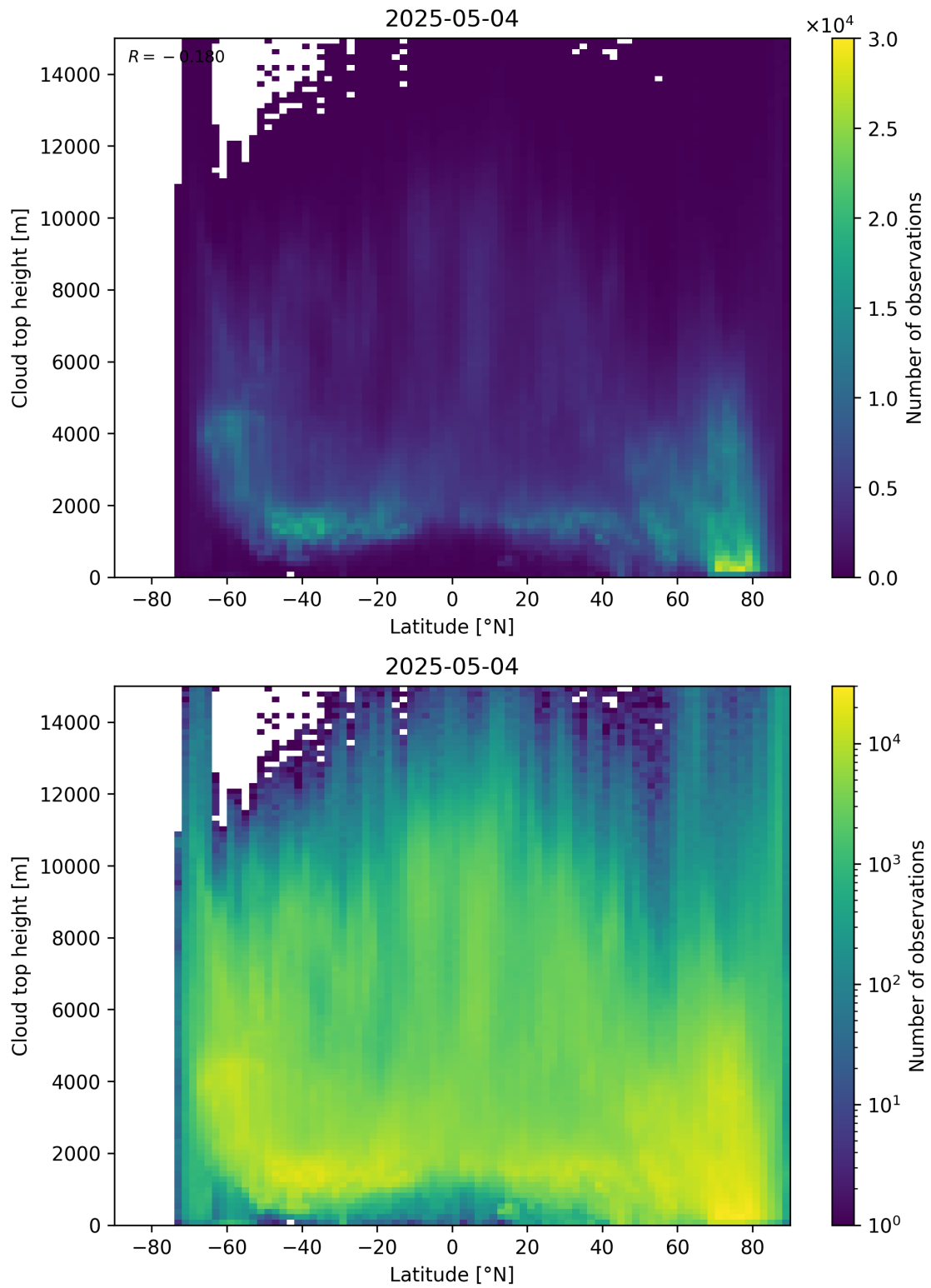
Figure 97: Scatter density plot of “Latitude” against “Cloud top height” for 2025-05-03 to 2025-05-05.
