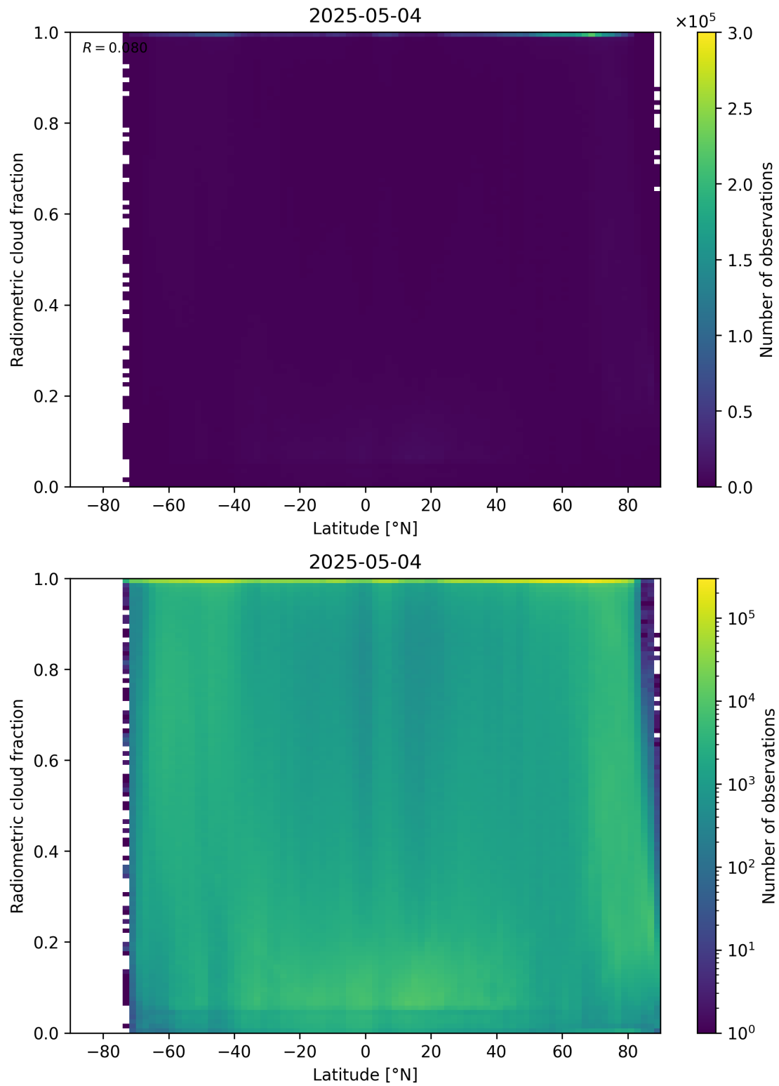
Figure 92: Scatter density plot of “Latitude” against “Radiometric cloud fraction” for 2025-05-03 to 2025-05-05.
