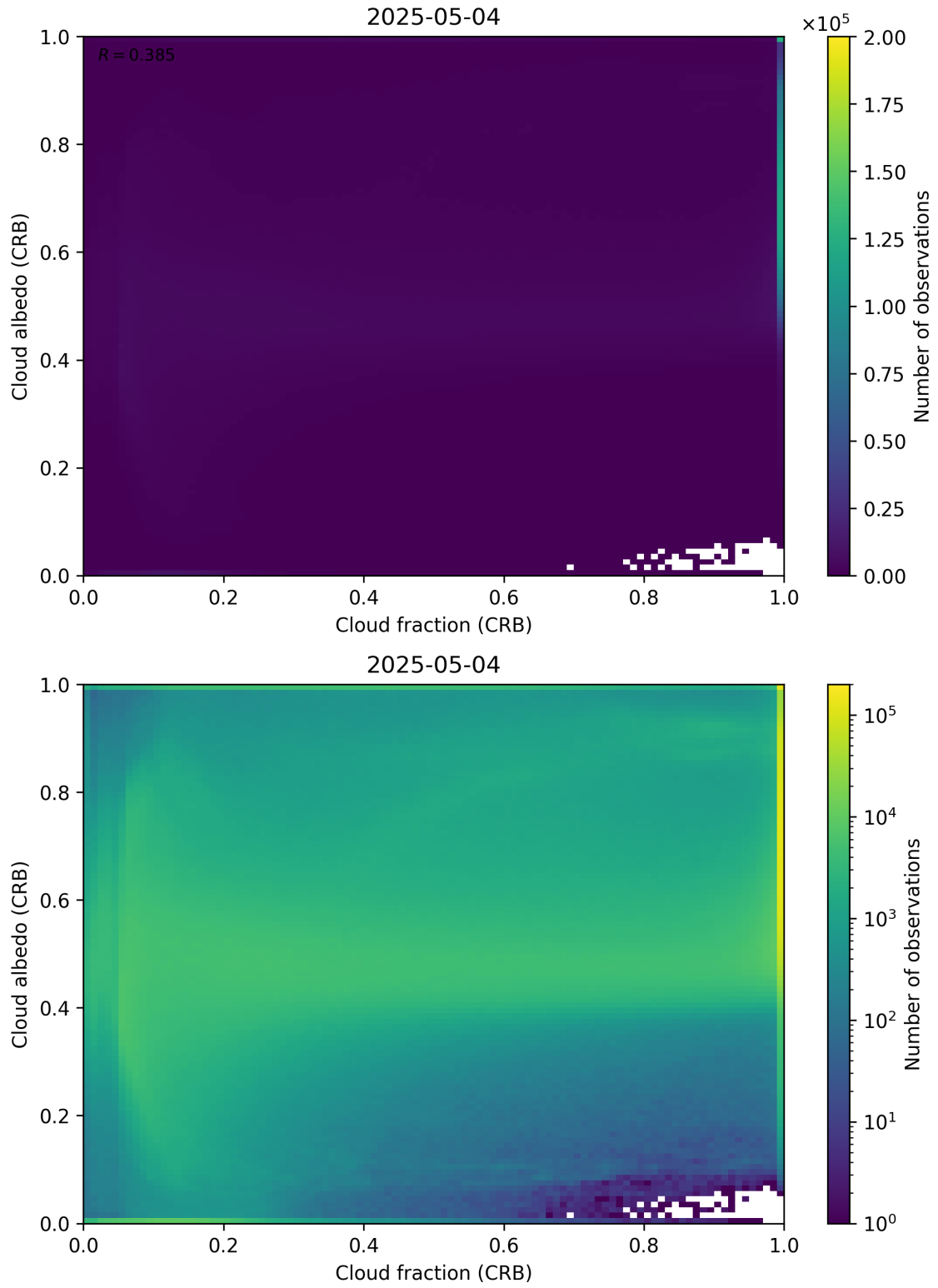
Figure 77: Scatter density plot of “Cloud fraction (CRB)” against “Cloud albedo (CRB)” for 2025-05-03 to 2025-05-05.
