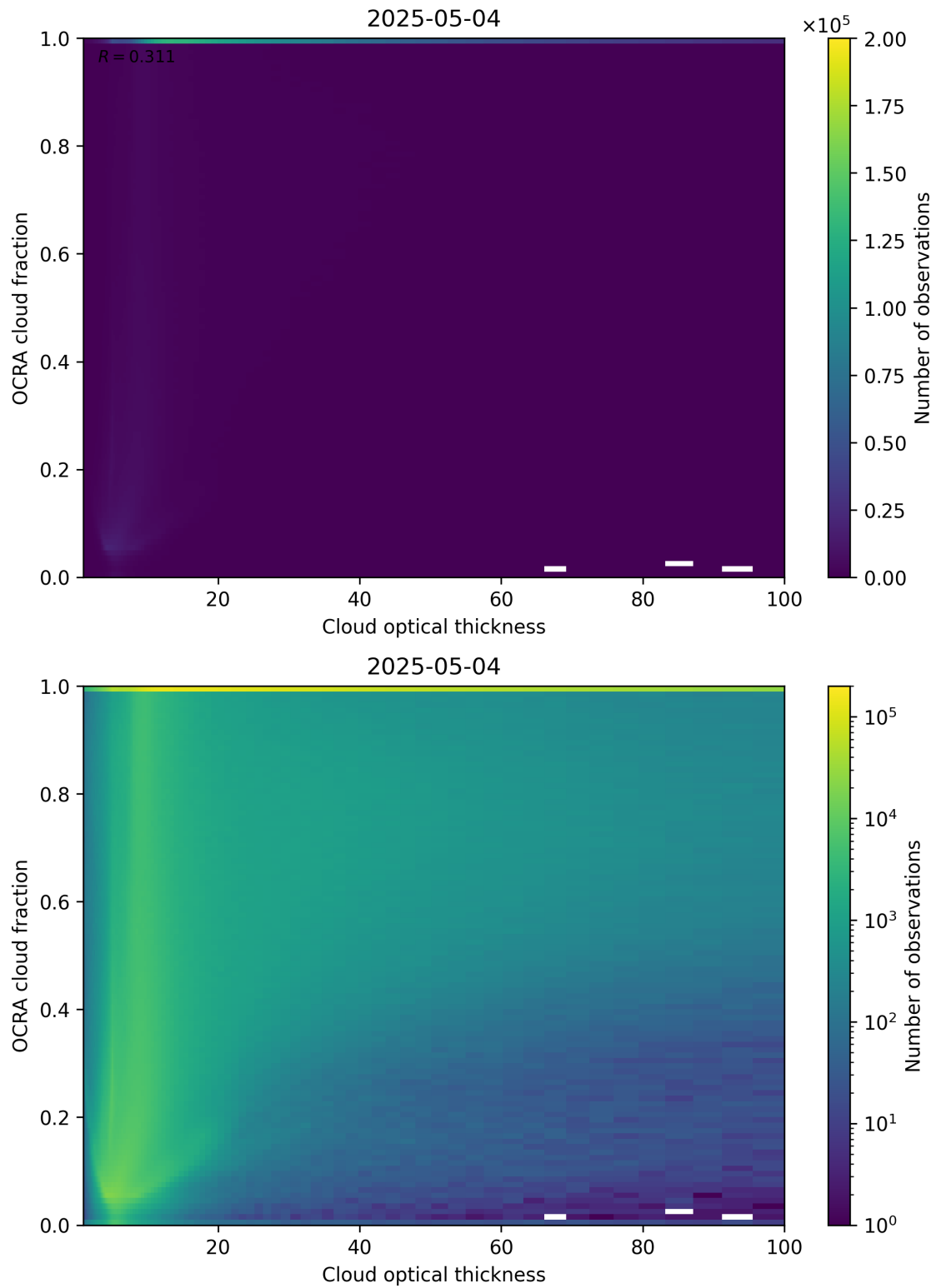
Figure 83: Scatter density plot of “Cloud optical thickness” against “OCRA cloud fraction” for 2025-05-03 to 2025-05-05.
