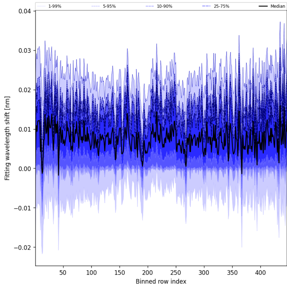
Figure 65: Along track statistics of “Fitting wavelength shift” for 2025-05-03 to 2025-05-05
