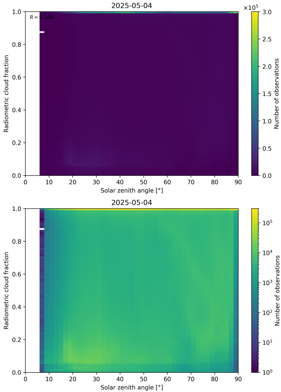
Figure 99: Scatter density plot of “Solar zenith angle” against “Radiometric cloud fraction” for 2025-05-03 to 2025-05-05.
