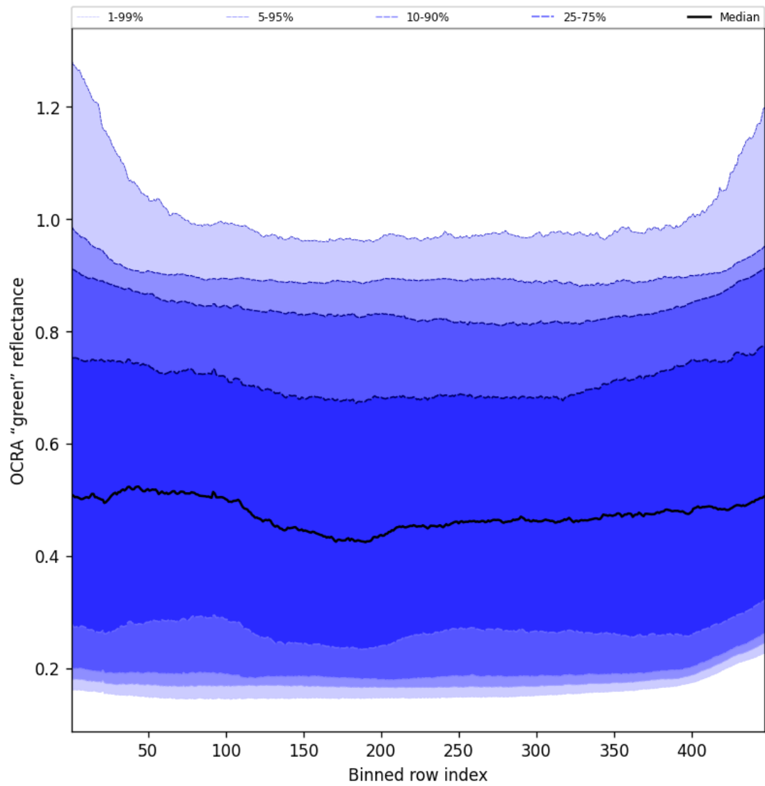
Figure 68: Along track statistics of “OCRA “green” reflectance” for 2025-05-03 to 2025-05-05
