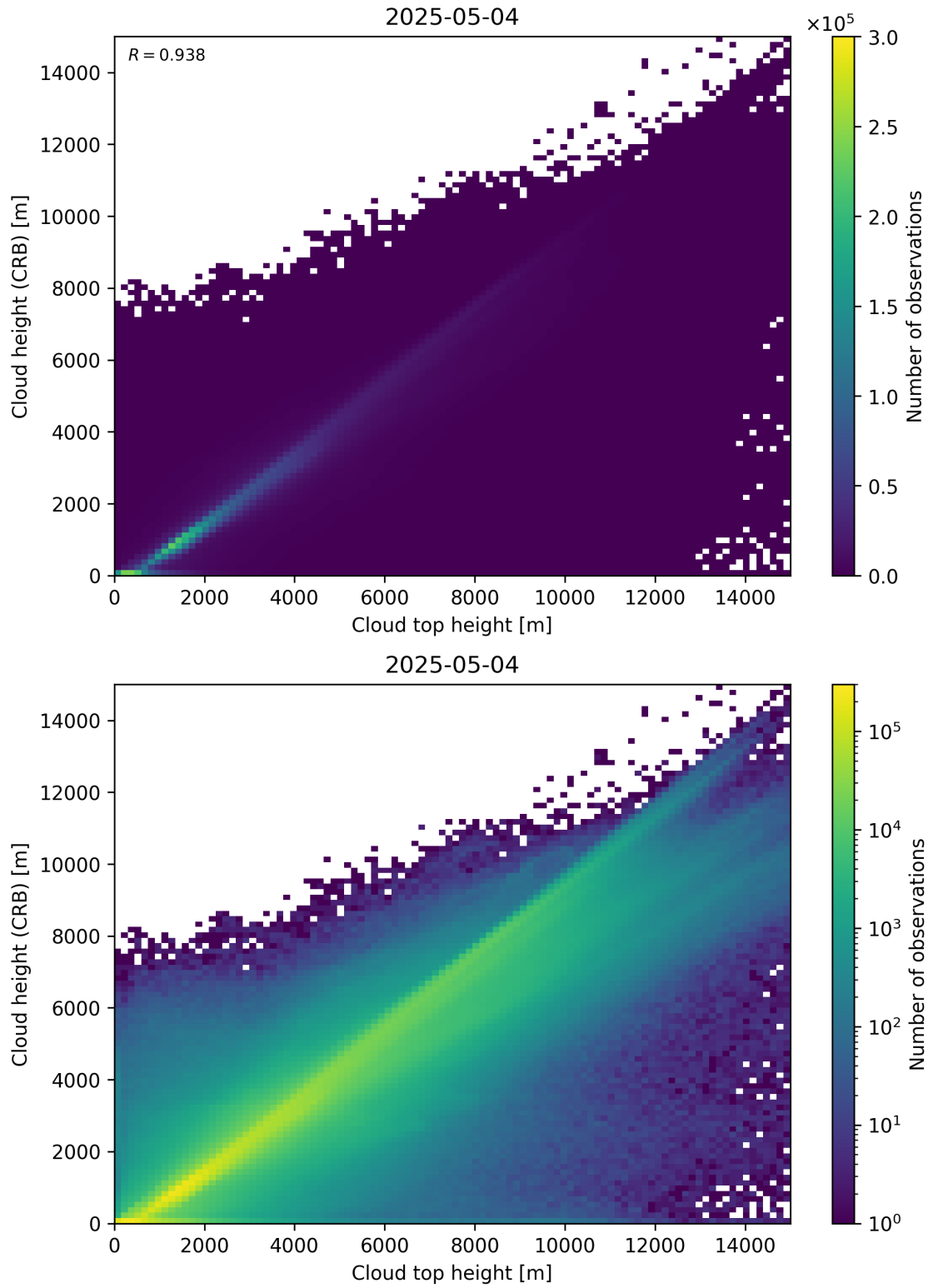
Figure 89: Scatter density plot of “Cloud top height” against “Cloud height (CRB)” for 2025-05-03 to 2025-05-05.
