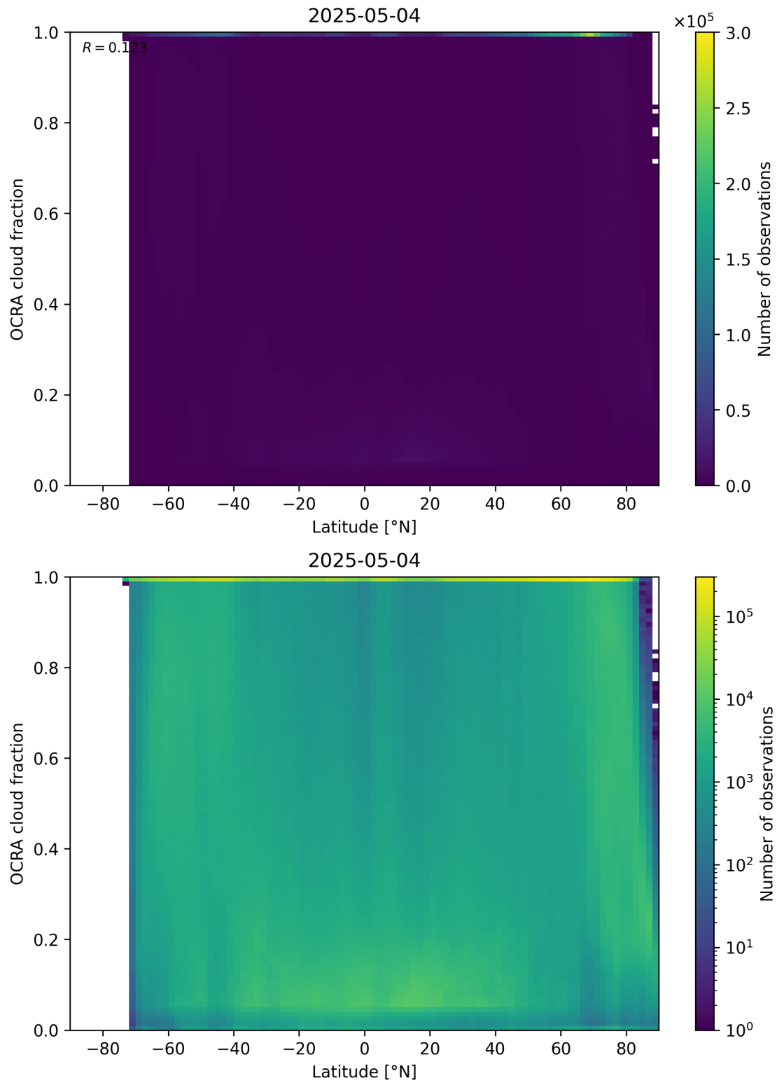
Figure 93: Scatter density plot of “Latitude” against “OCRA cloud fraction” for 2025-05-03 to 2025-05-05.
