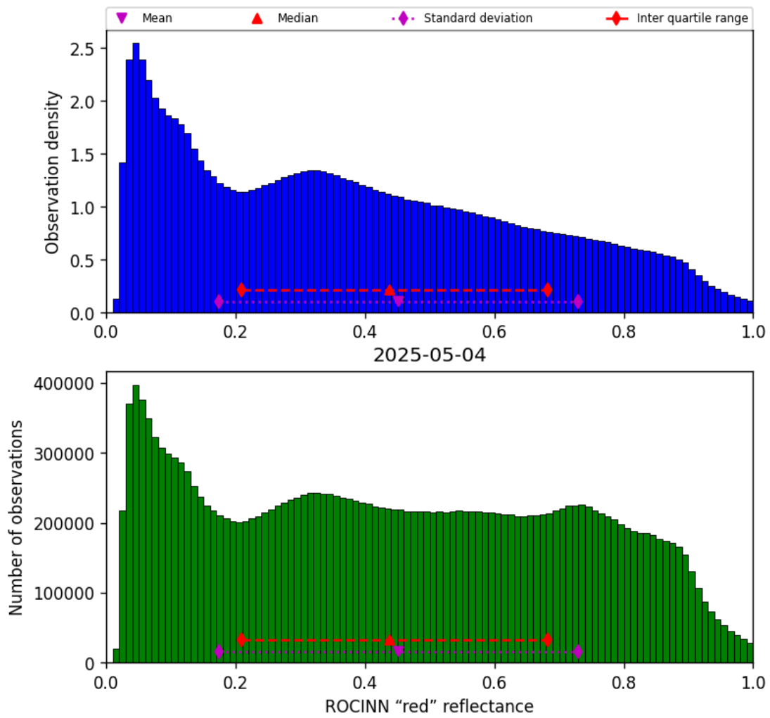
Figure 53: Histogram of “ROCINN “red” reflectance” for 2025-05-03 to 2025-05-05
