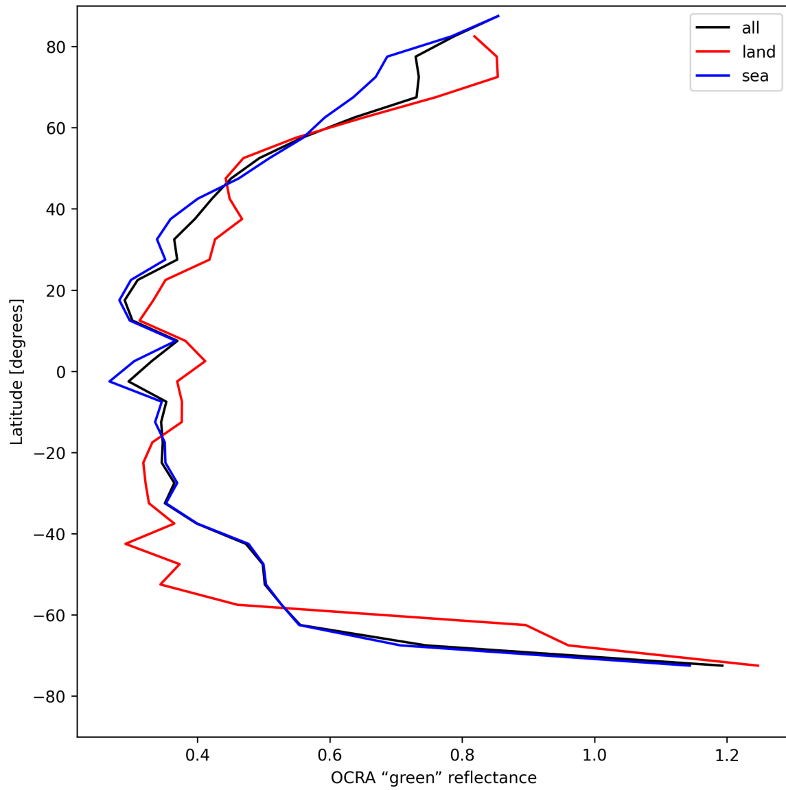
Figure 36: Zonal average of “OCRA “green” reflectance” for 2025-05-03 to 2025-05-05.
