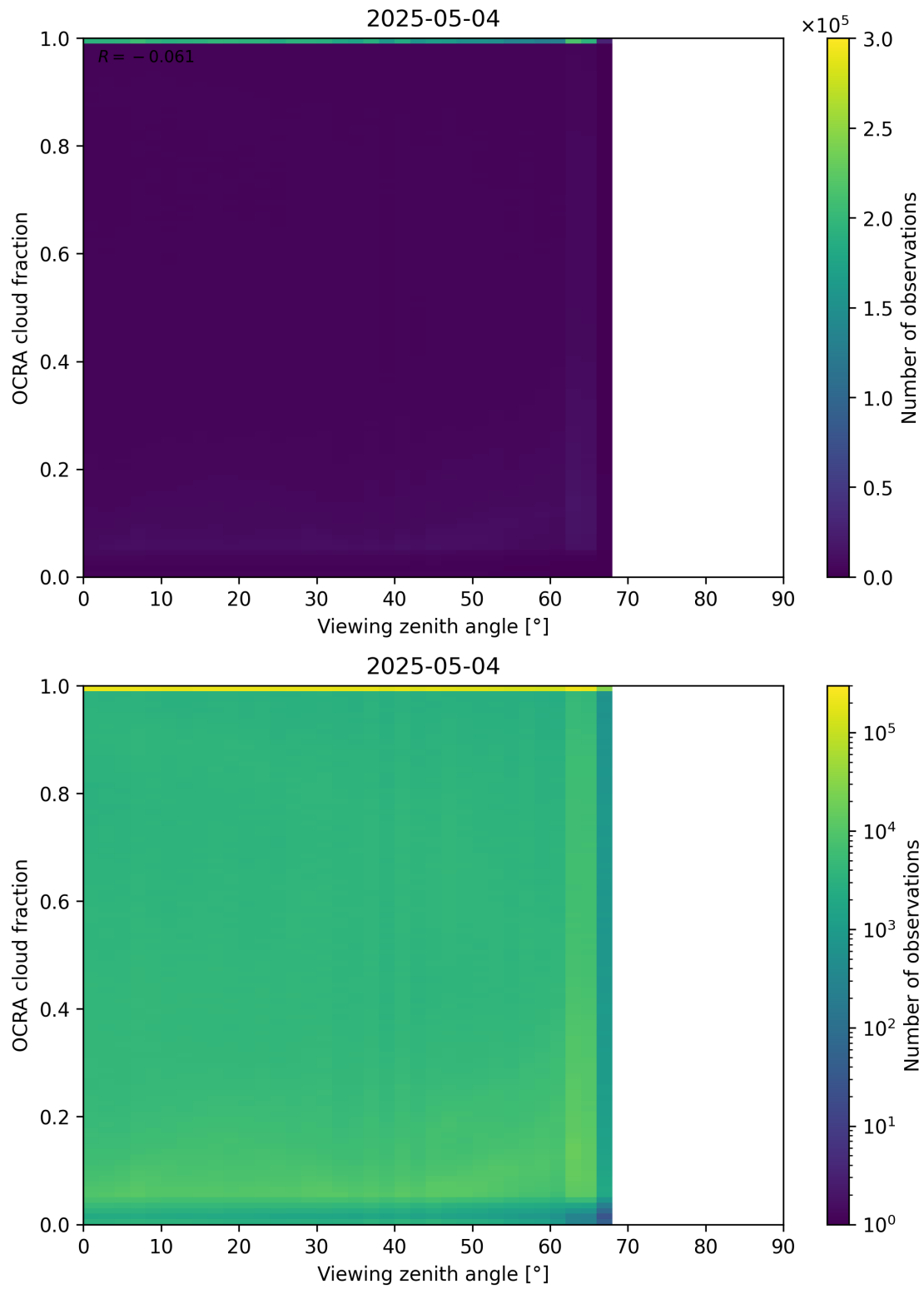
Figure 108: Scatter density plot of “Viewing zenith angle” against “OCRA cloud fraction” for 2025-05-03 to 2025-05-05.
