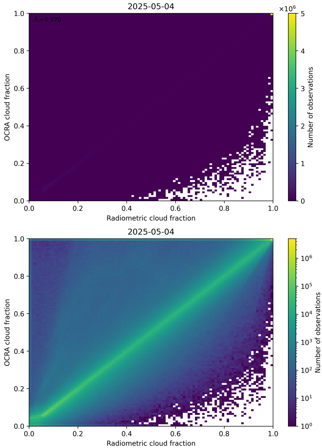
Figure 72: Scatter density plot of “Radiometric cloud fraction” against “OCRA cloud fraction” for 2025-05-03 to 2025-05-05.
