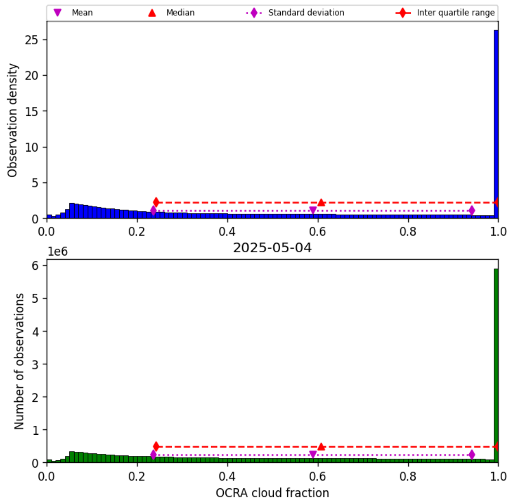
Figure 50: Histogram of “OCRA cloud fraction” for 2025-05-03 to 2025-05-05
