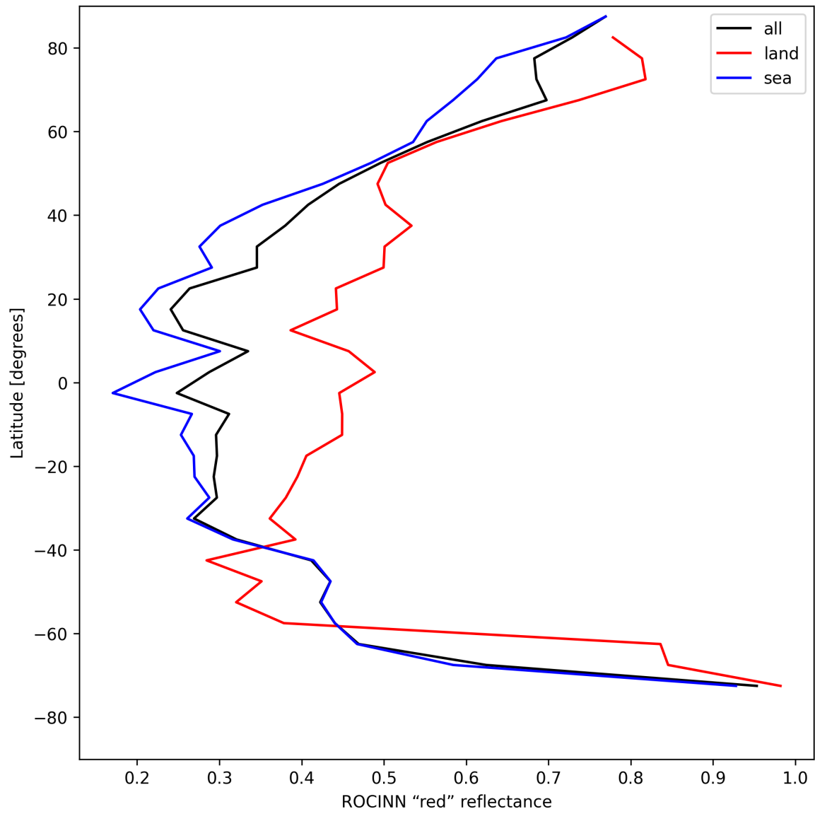
Figure 37: Zonal average of “ROCINN “red” reflectance” for 2025-05-03 to 2025-05-05.
