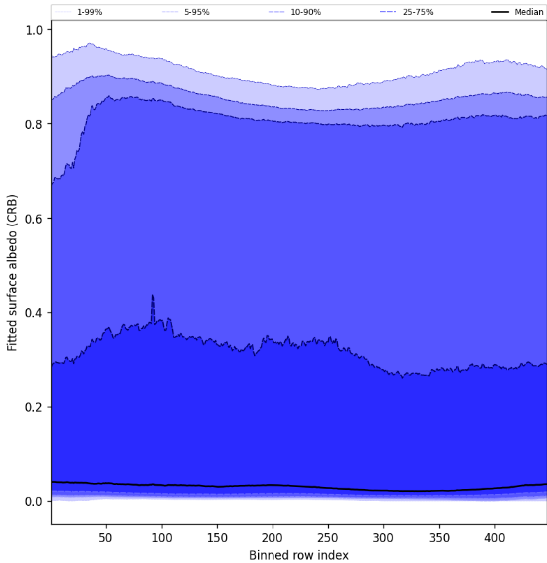
Figure 62: Along track statistics of “Fitted surface albedo (CRB)” for 2025-05-03 to 2025-05-05
