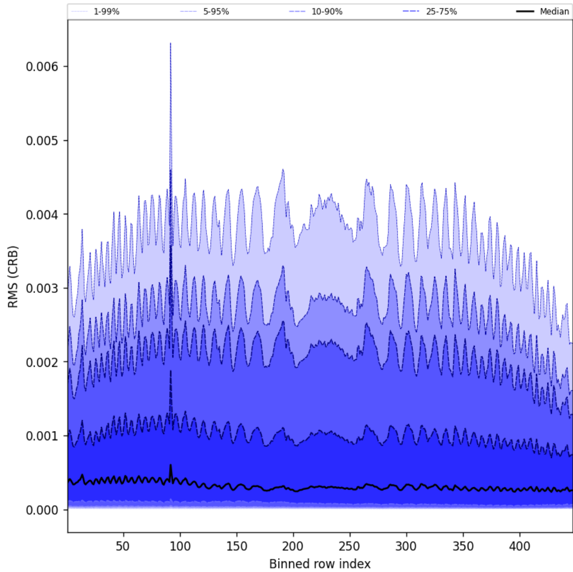
Figure 64: Along track statistics of “RMS (CRB)” for 2025-05-03 to 2025-05-05
