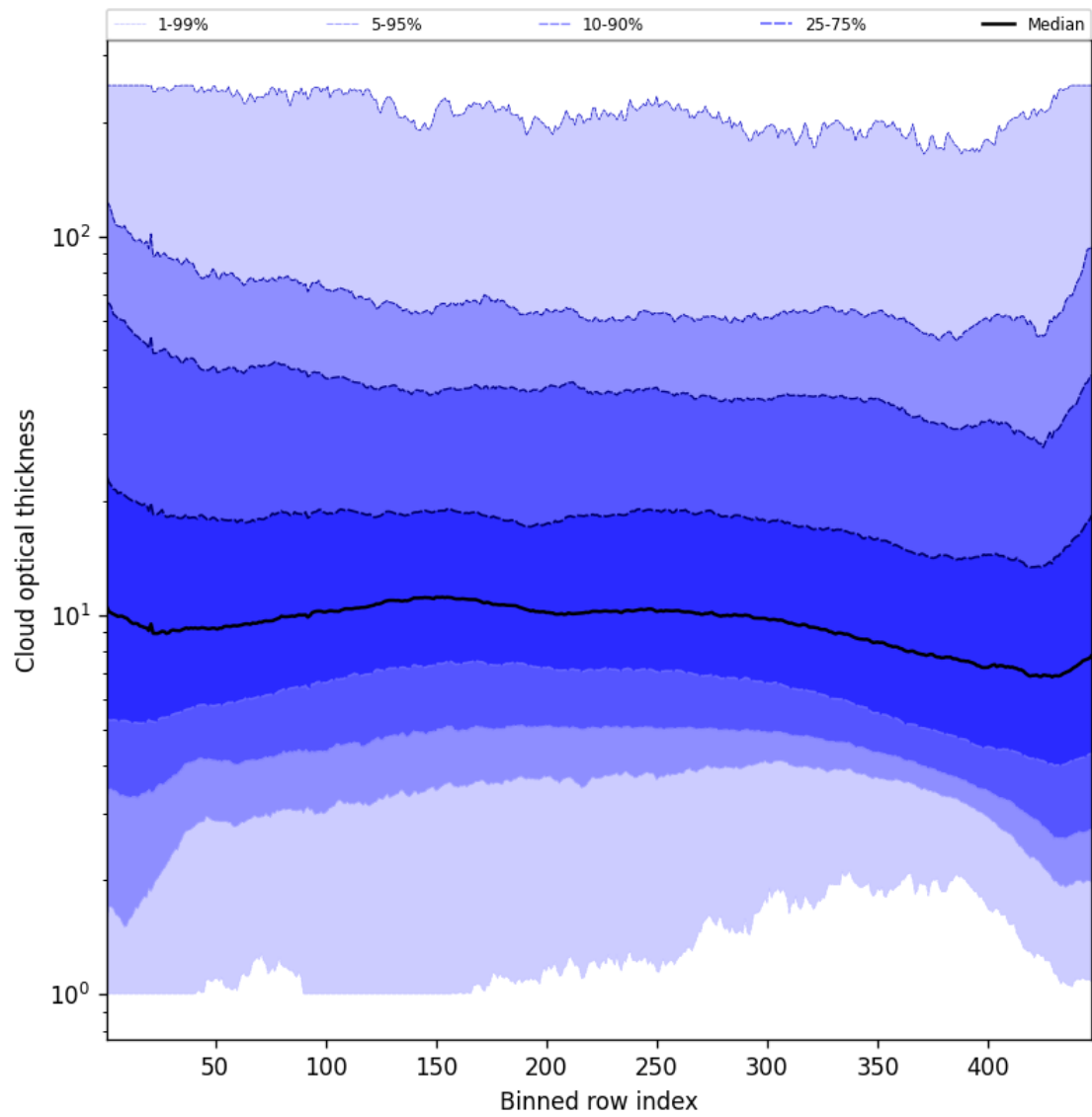
Figure 57: Along track statistics of “Cloud optical thickness” for 2025-05-03 to 2025-05-05
