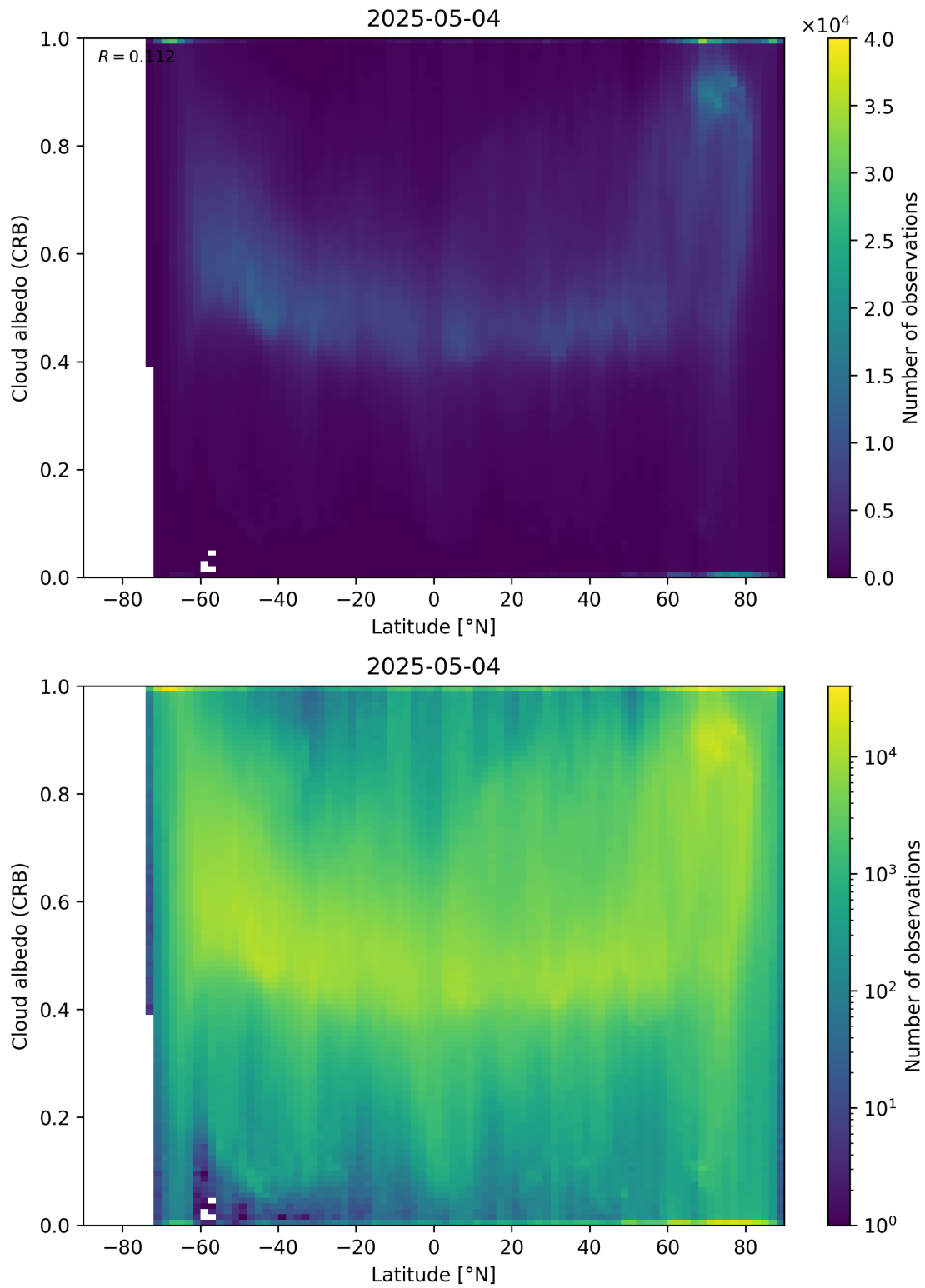
Figure 91: Scatter density plot of “Latitude” against “Cloud albedo (CRB)” for 2025-05-03 to 2025-05-05.
