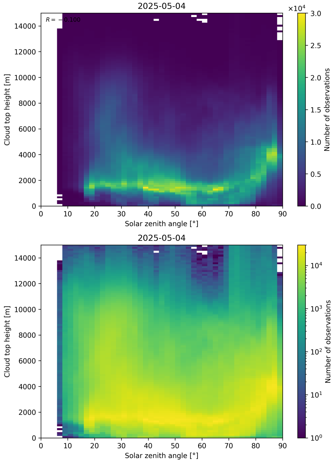
Figure 104: Scatter density plot of “Solar zenith angle” against “Cloud top height” for 2025-05-03 to 2025-05-05.
