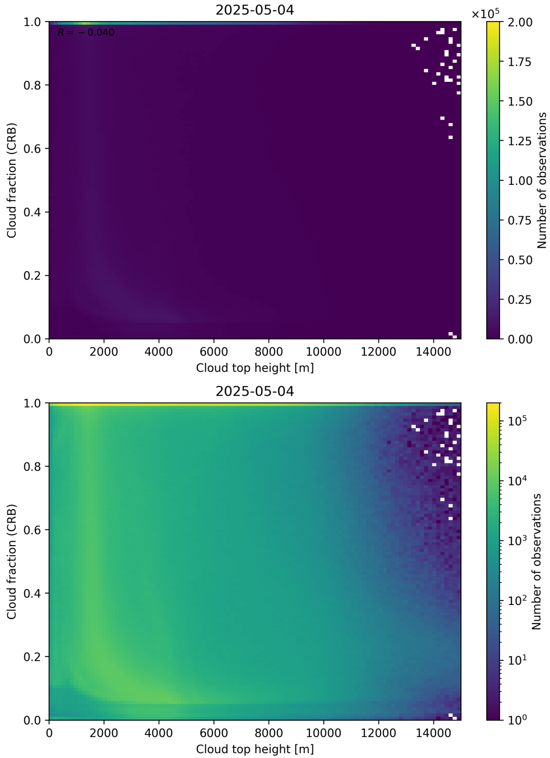
Figure 88: Scatter density plot of “Cloud top height” against “Cloud fraction (CRB)” for 2025-05-03 to 2025-05-05.
