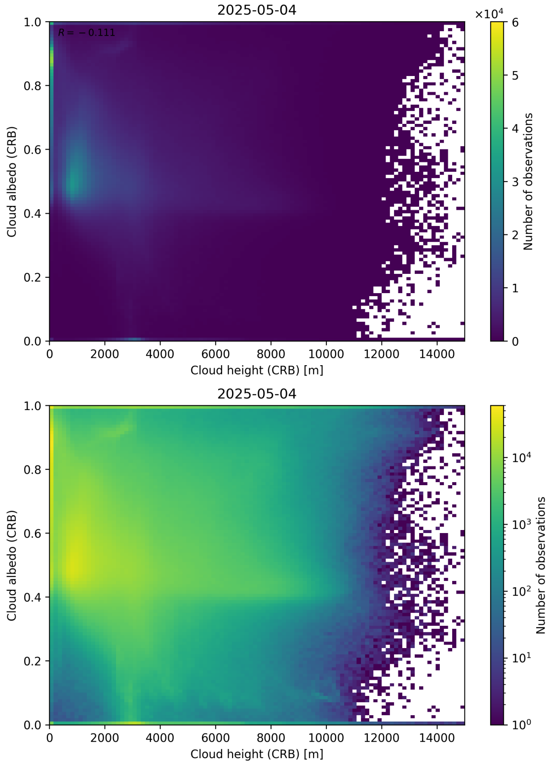
Figure 80: Scatter density plot of “Cloud height (CRB)” against “Cloud albedo (CRB)” for 2025-05-03 to 2025-05-05.
