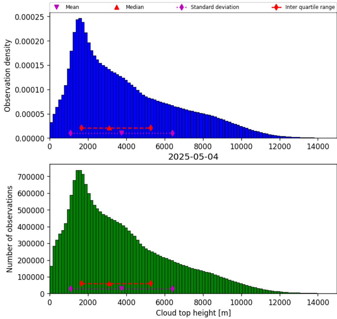
Figure 40: Histogram of “Cloud top height” for 2025-05-03 to 2025-05-05
