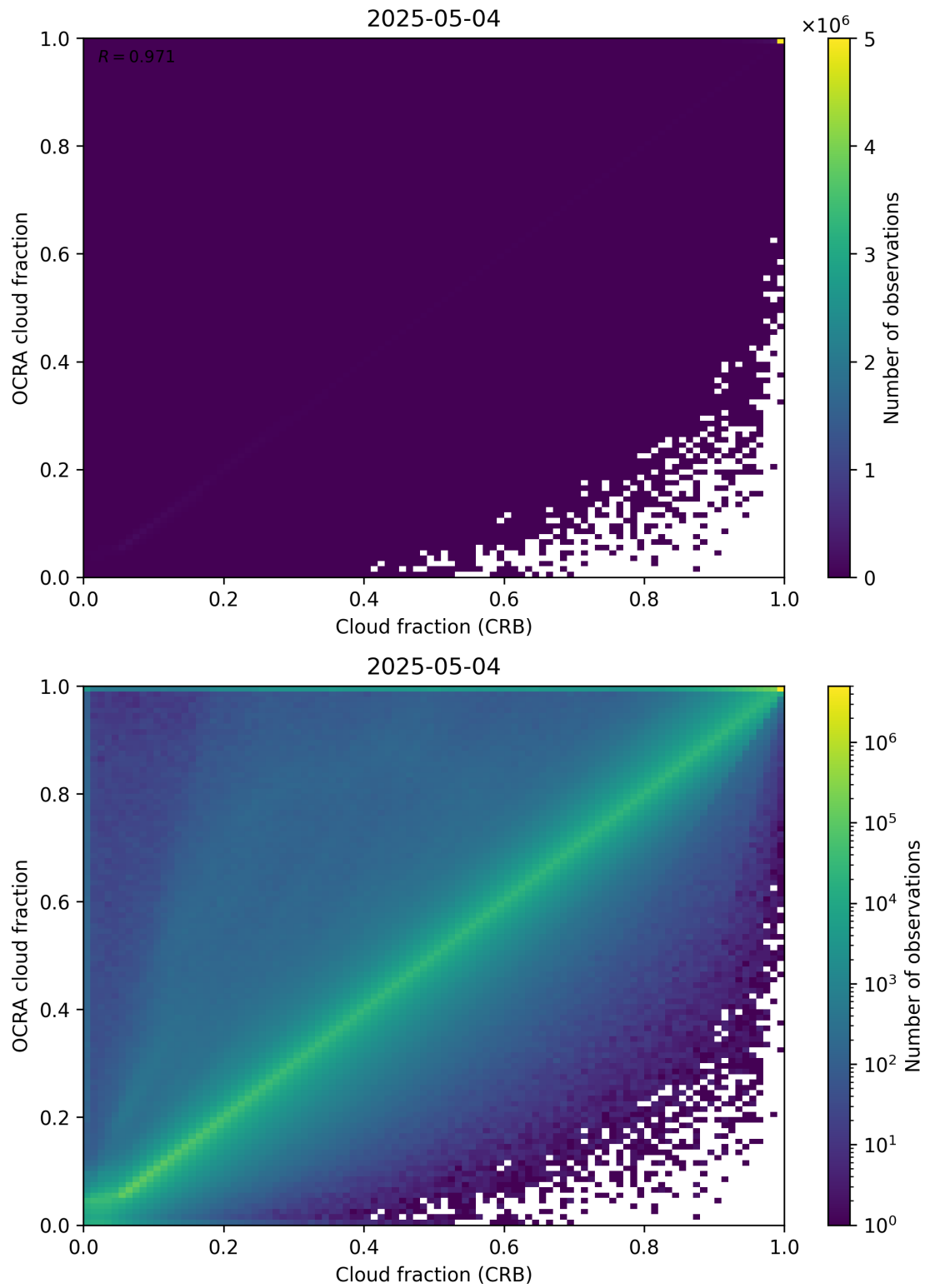
Figure 78: Scatter density plot of “Cloud fraction (CRB)” against “OCRA cloud fraction” for 2025-05-03 to 2025-05-05.
