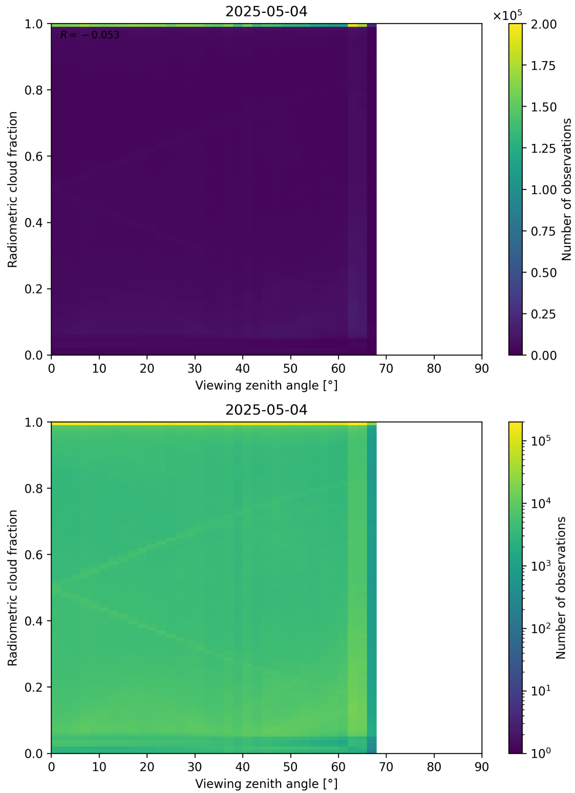
Figure 107: Scatter density plot of “Viewing zenith angle” against “Radiometric cloud fraction” for 2025-05-03 to 2025-05-05.
