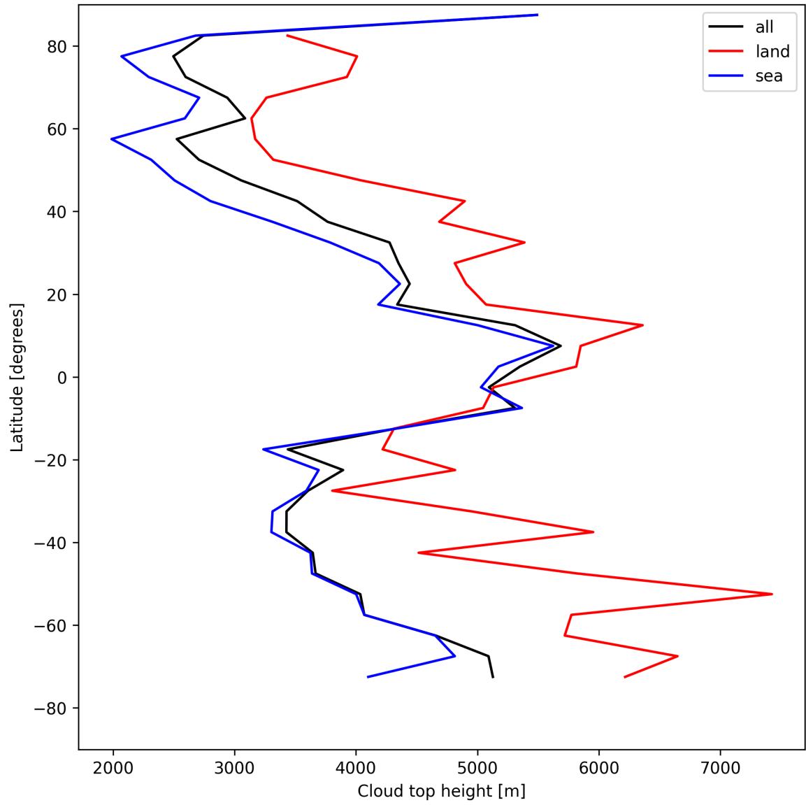
Figure 24: Zonal average of “Cloud top height” for 2025-05-03 to 2025-05-05.
