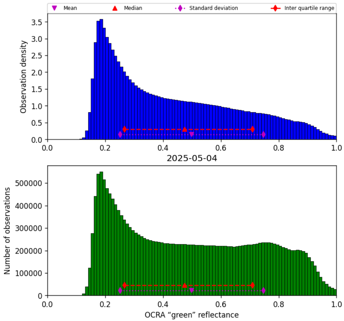
Figure 52: Histogram of “OCRA “green” reflectance” for 2025-05-03 to 2025-05-05
