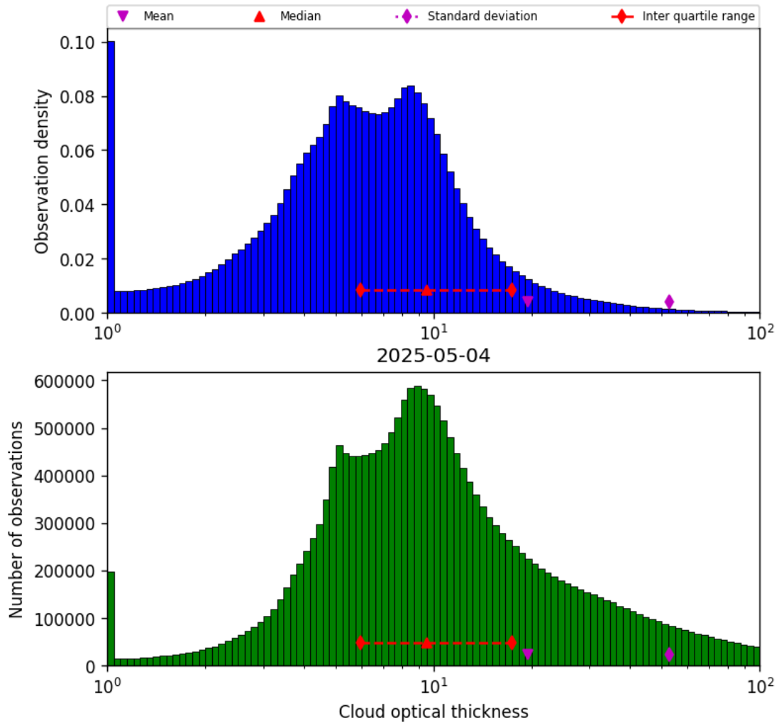
Figure 41: Histogram of “Cloud optical thickness” for 2025-05-03 to 2025-05-05
