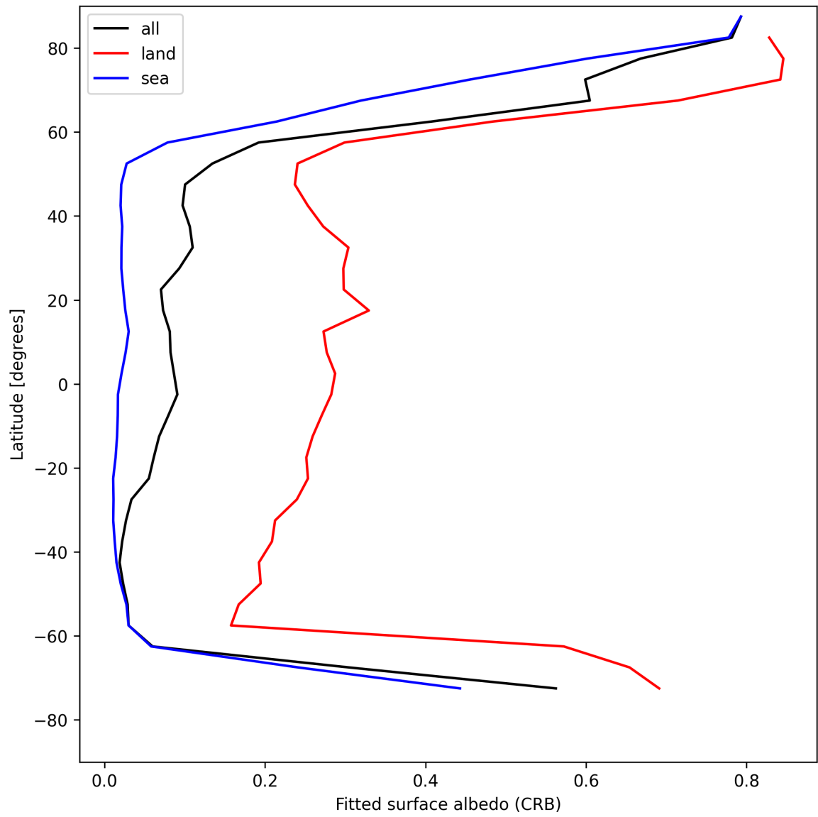
Figure 30: Zonal average of “Fitted surface albedo (CRB)” for 2025-05-03 to 2025-05-05.
