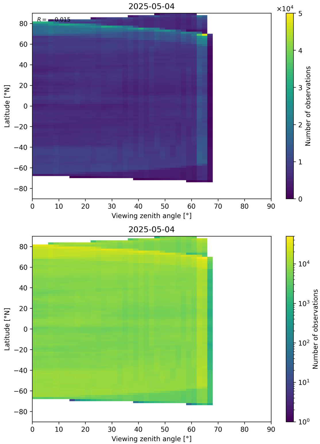
Figure 113: Scatter density plot of “Viewing zenith angle” against “Latitude” for 2025-05-03 to 2025-05-05.
