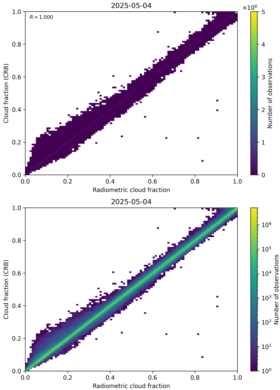
Figure 73: Scatter density plot of “Radiometric cloud fraction” against “Cloud fraction (CRB)” for 2025-05-03 to 2025-05-05.
