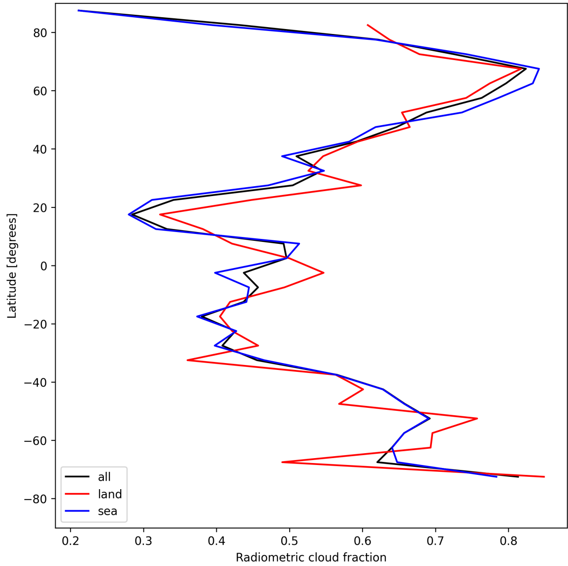
Figure 23: Zonal average of “Radiometric cloud fraction” for 2025-05-05 to 2025-05-07.
