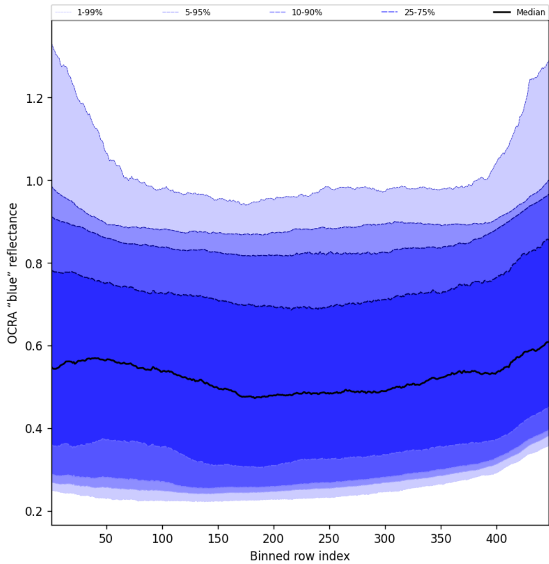
Figure 67: Along track statistics of “OCRA “blue” reflectance” for 2025-05-05 to 2025-05-07
