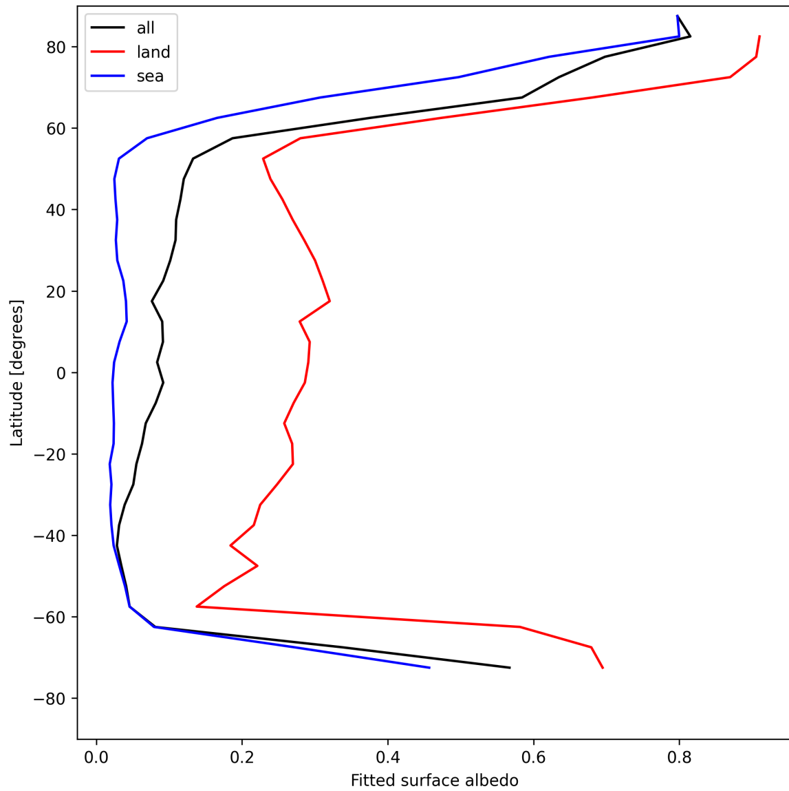
Figure 29: Zonal average of “Fitted surface albedo” for 2025-05-05 to 2025-05-07.
