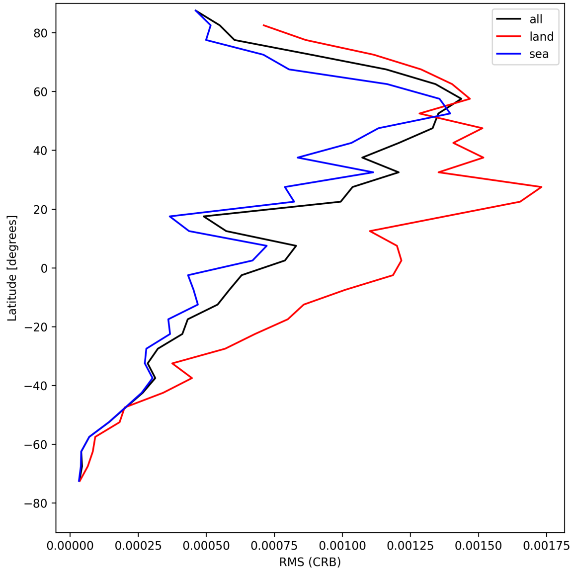
Figure 32: Zonal average of “RMS (CRB)” for 2025-05-05 to 2025-05-07.
