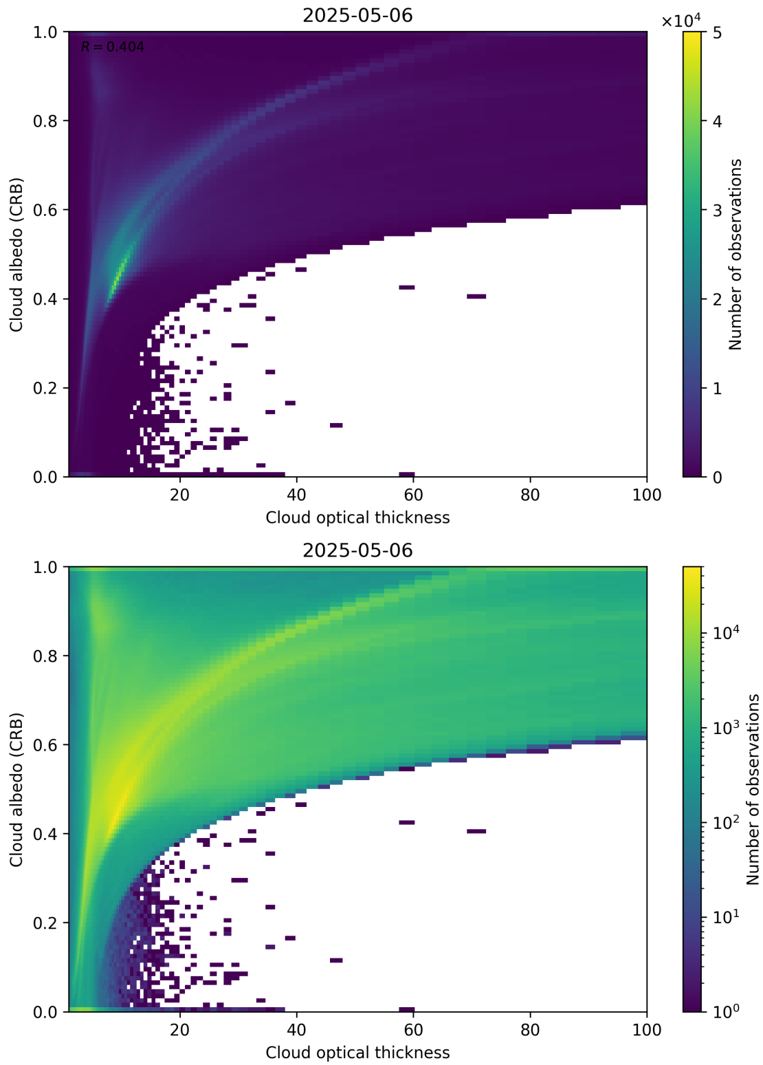
Figure 82: Scatter density plot of “Cloud optical thickness” against “Cloud albedo (CRB)” for 2025-05-05 to 2025-05-07.
