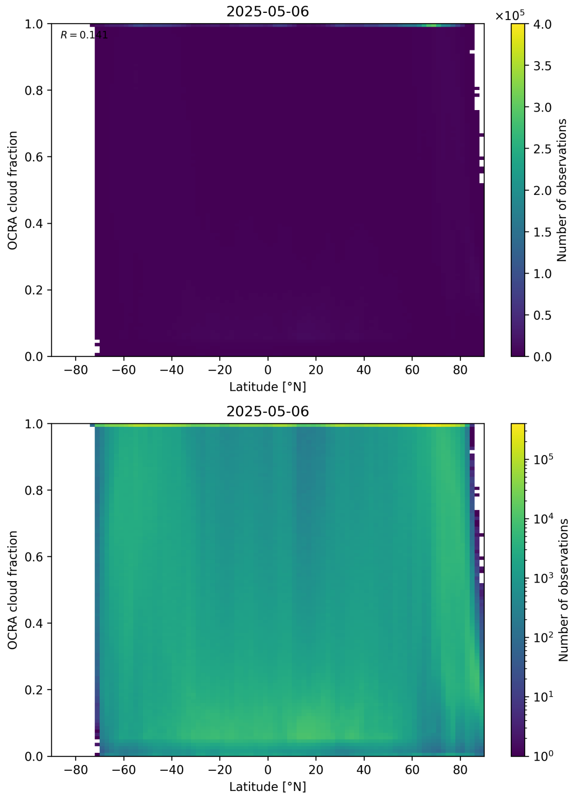
Figure 93: Scatter density plot of “Latitude” against “OCRA cloud fraction” for 2025-05-05 to 2025-05-07.
