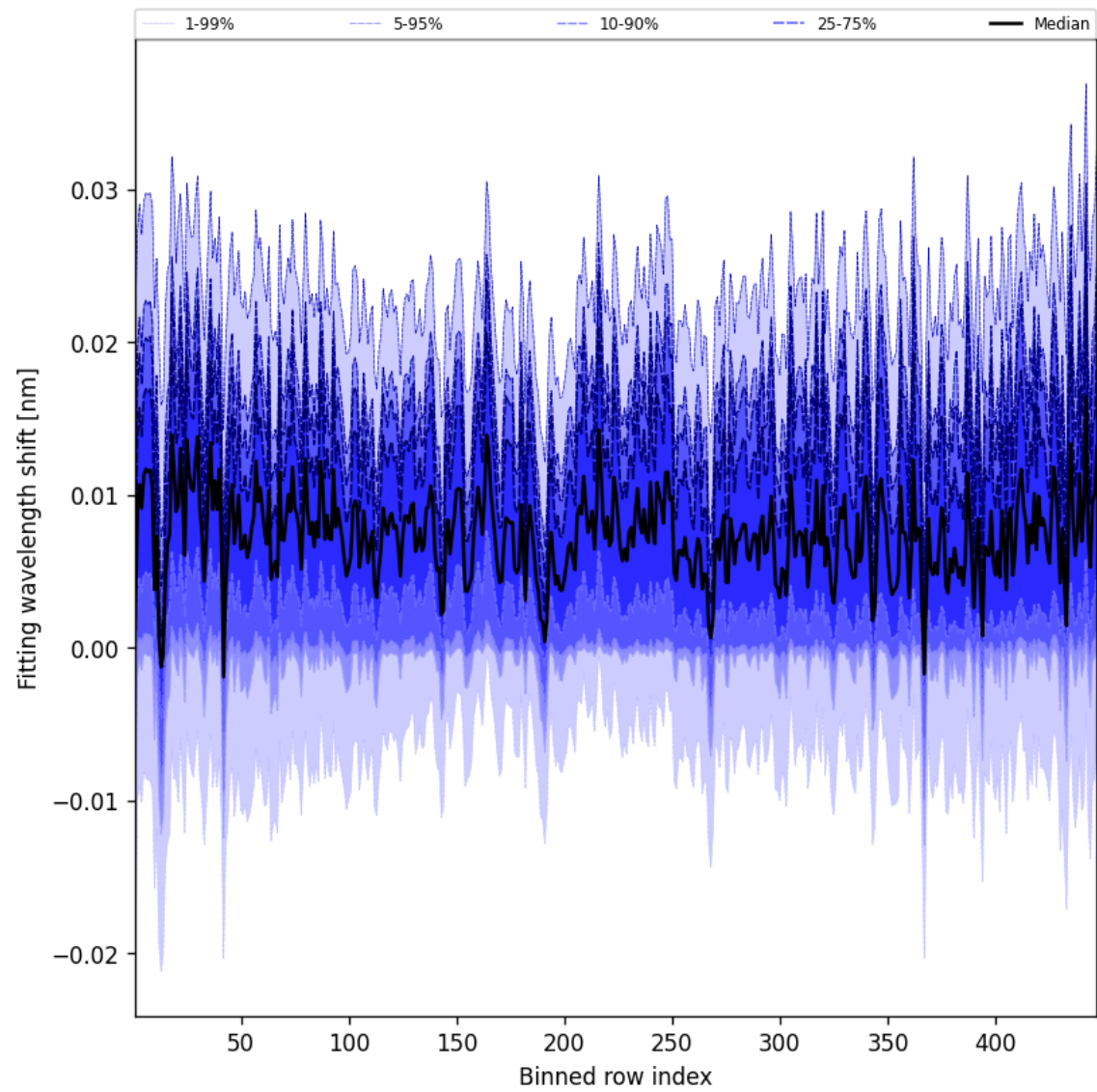
Figure 65: Along track statistics of “Fitting wavelength shift” for 2025-05-05 to 2025-05-07
