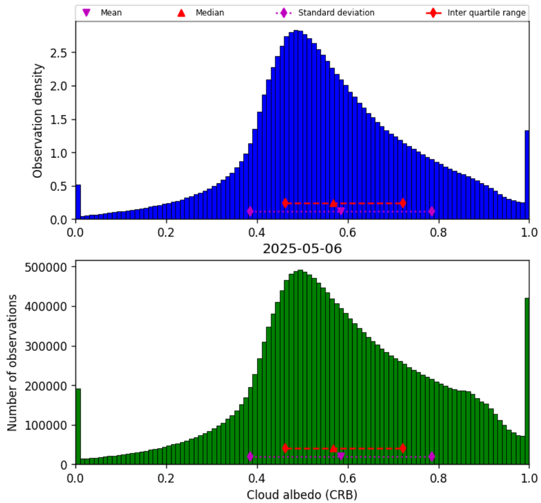
Figure 44: Histogram of “Cloud albedo (CRB)” for 2025-05-05 to 2025-05-07
