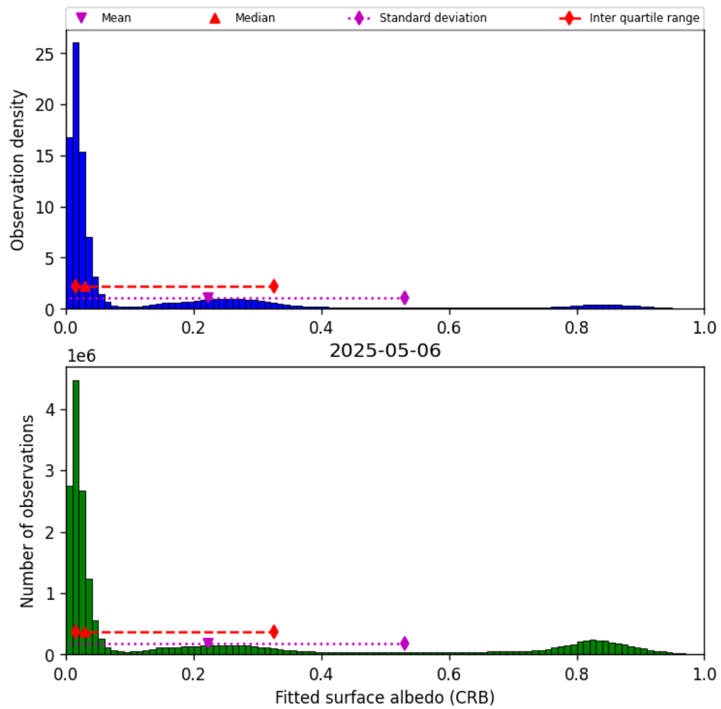
Figure 46: Histogram of “Fitted surface albedo (CRB)” for 2025-05-05 to 2025-05-07
