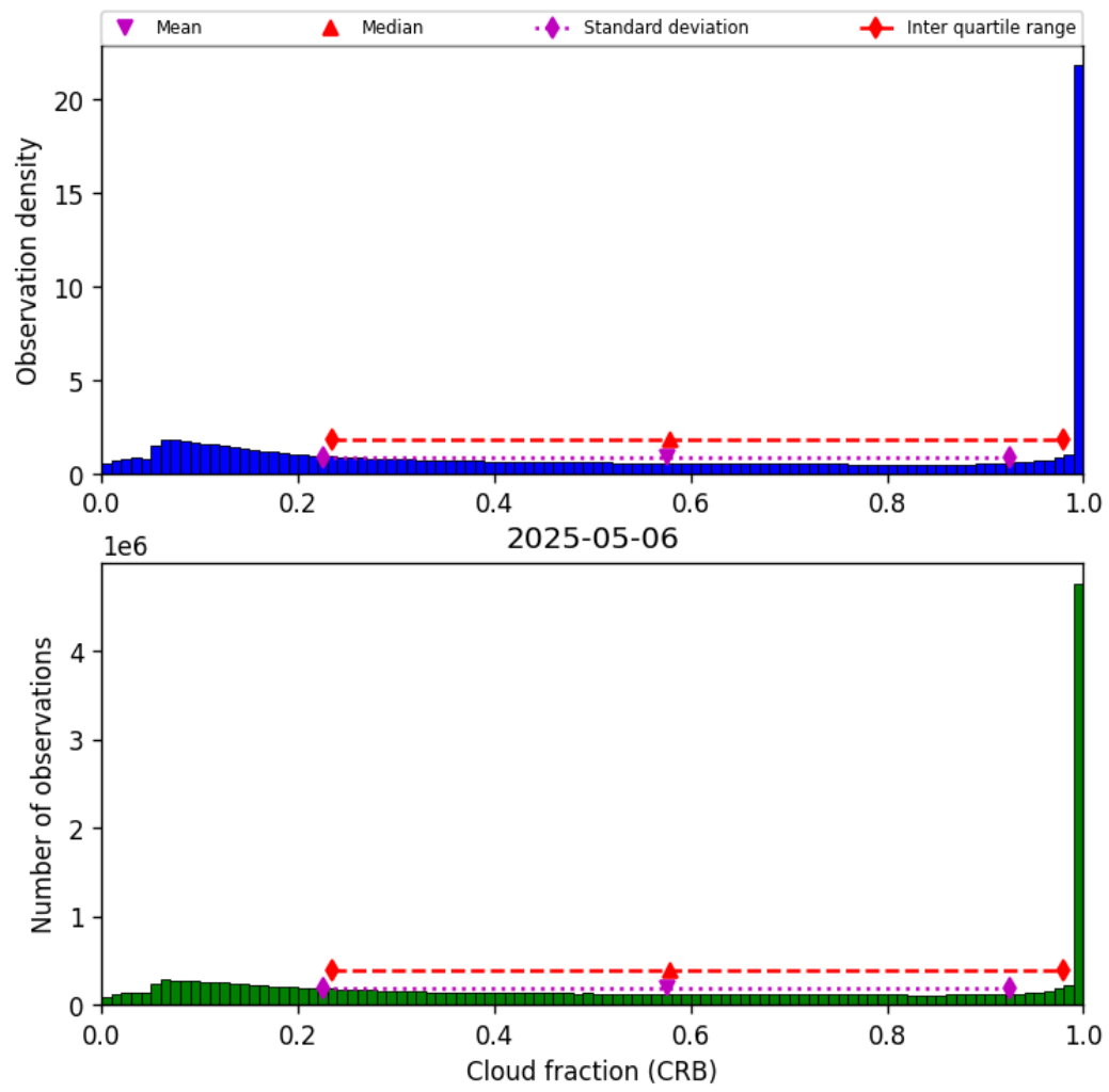
Figure 42: Histogram of “Cloud fraction (CRB)” for 2025-05-05 to 2025-05-07
