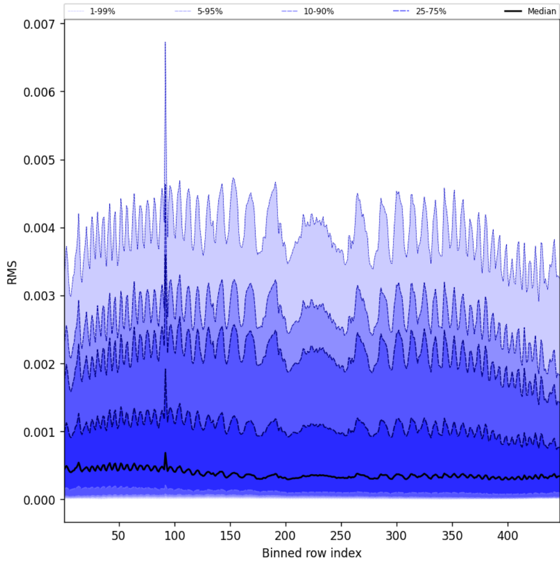
Figure 63: Along track statistics of “RMS” for 2025-05-05 to 2025-05-07
