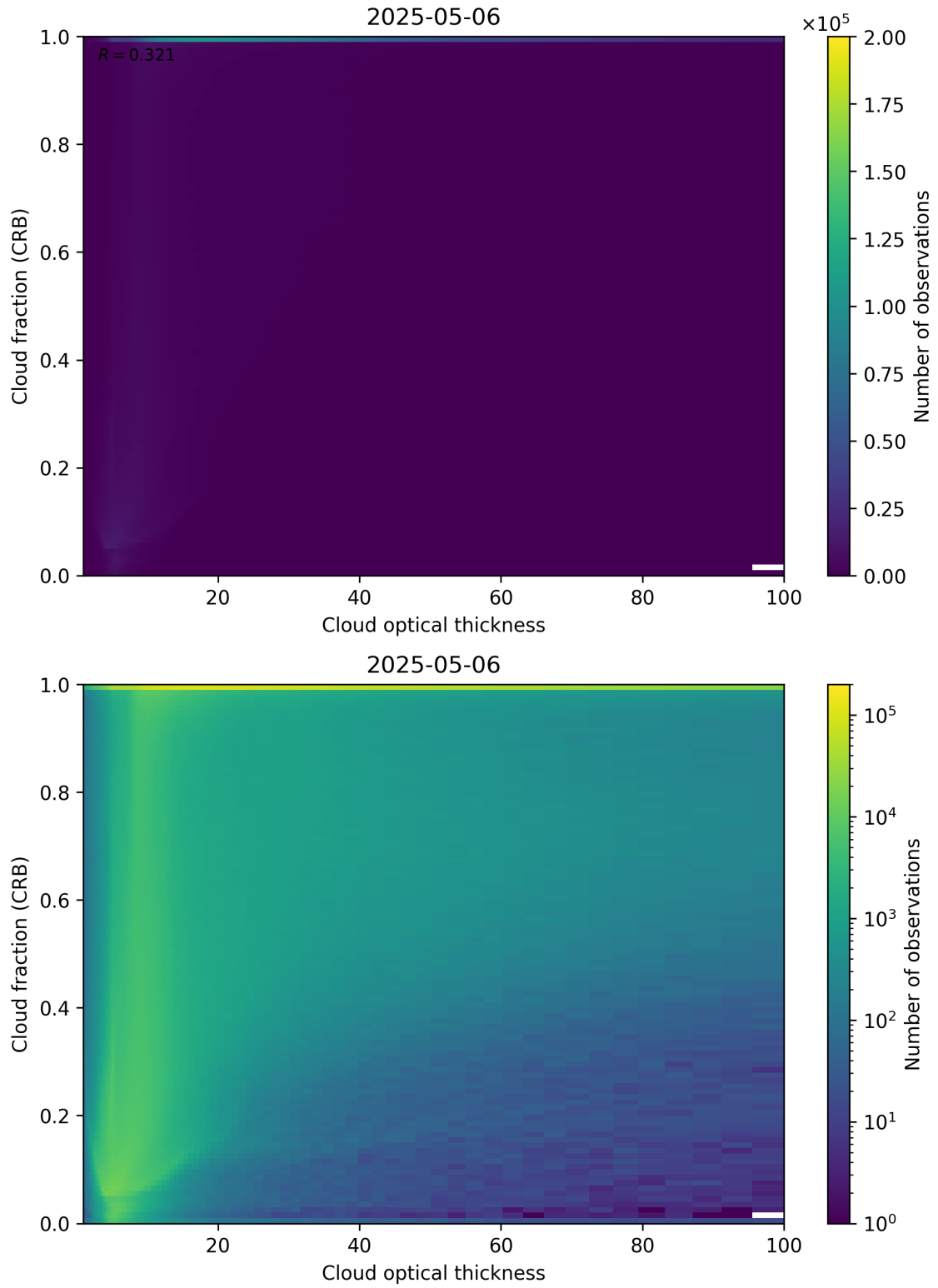
Figure 84: Scatter density plot of “Cloud optical thickness” against “Cloud fraction (CRB)” for 2025-05-05 to 2025-05-07.
