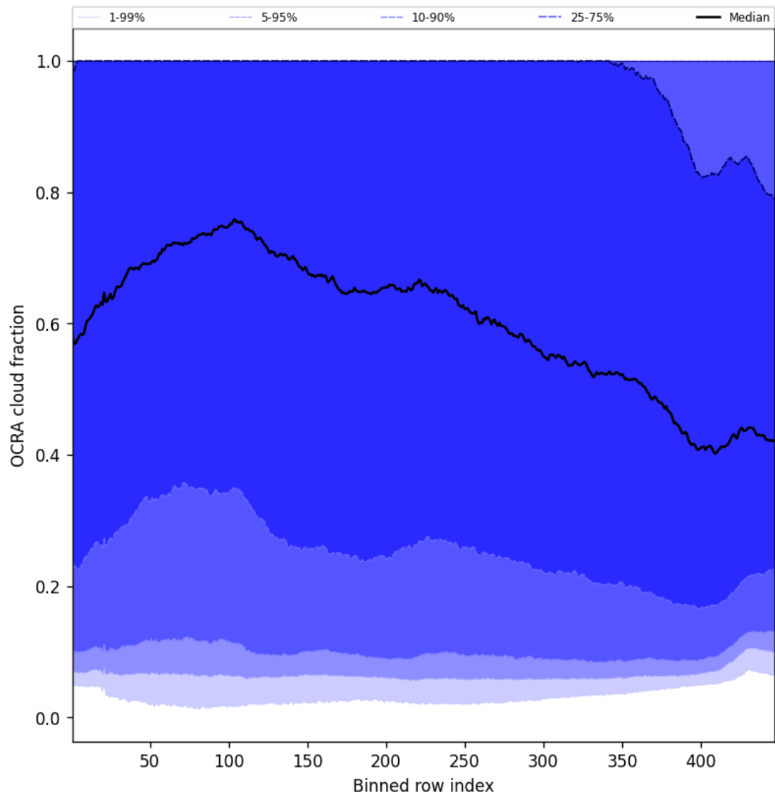
Figure 66: Along track statistics of “OCRA cloud fraction” for 2025-05-05 to 2025-05-07
