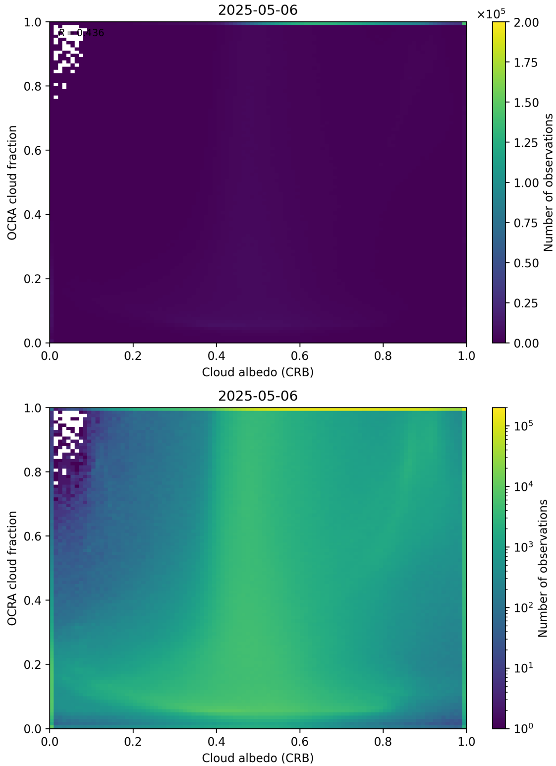
Figure 70: Scatter density plot of “Cloud albedo (CRB)” against “OCRA cloud fraction” for 2025-05-05 to 2025-05-07.
