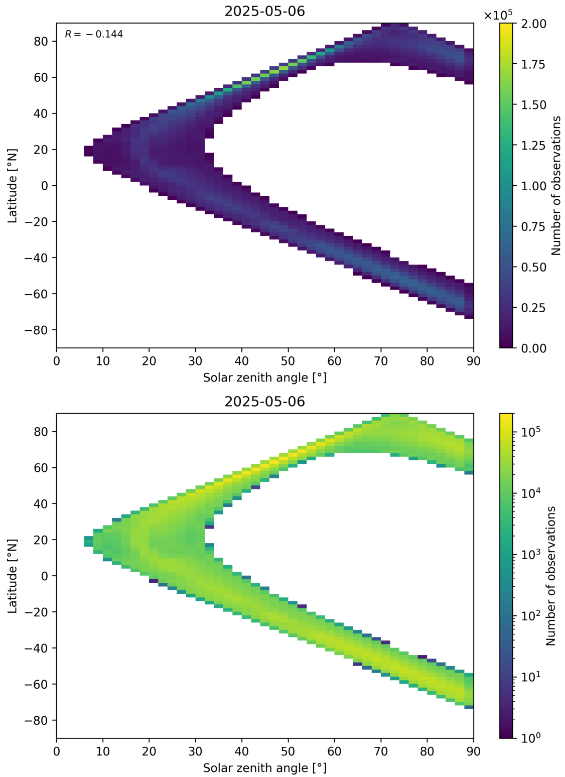
Figure 105: Scatter density plot of “Solar zenith angle” against “Latitude” for 2025-05-05 to 2025-05-07.
