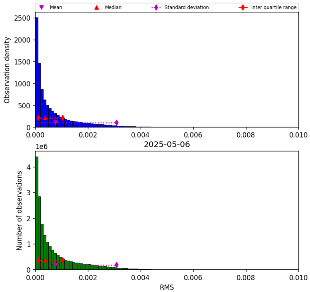
Figure 47: Histogram of “RMS” for 2025-05-05 to 2025-05-07
