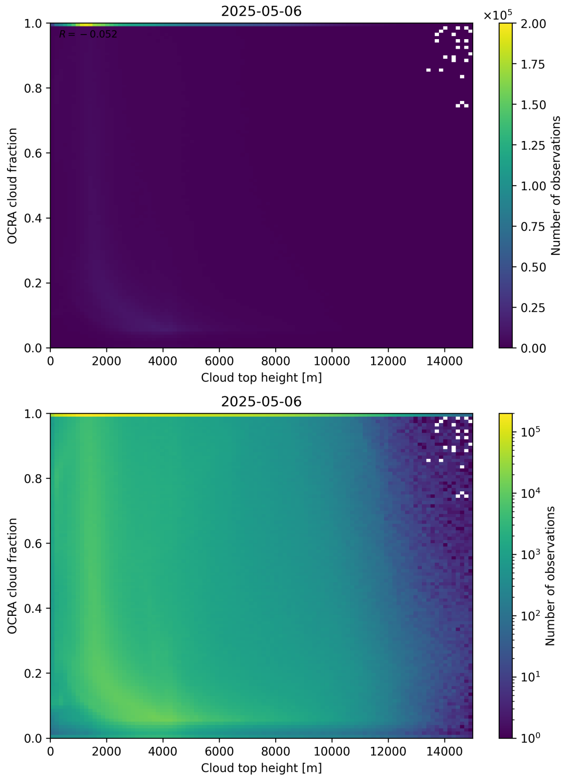
Figure 87: Scatter density plot of “Cloud top height” against “OCRA cloud fraction” for 2025-05-05 to 2025-05-07.
