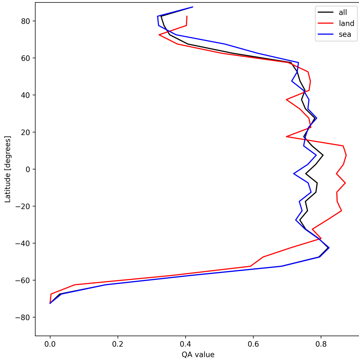
Figure 22: Zonal average of “QA value” for 2025-05-05 to 2025-05-07.
