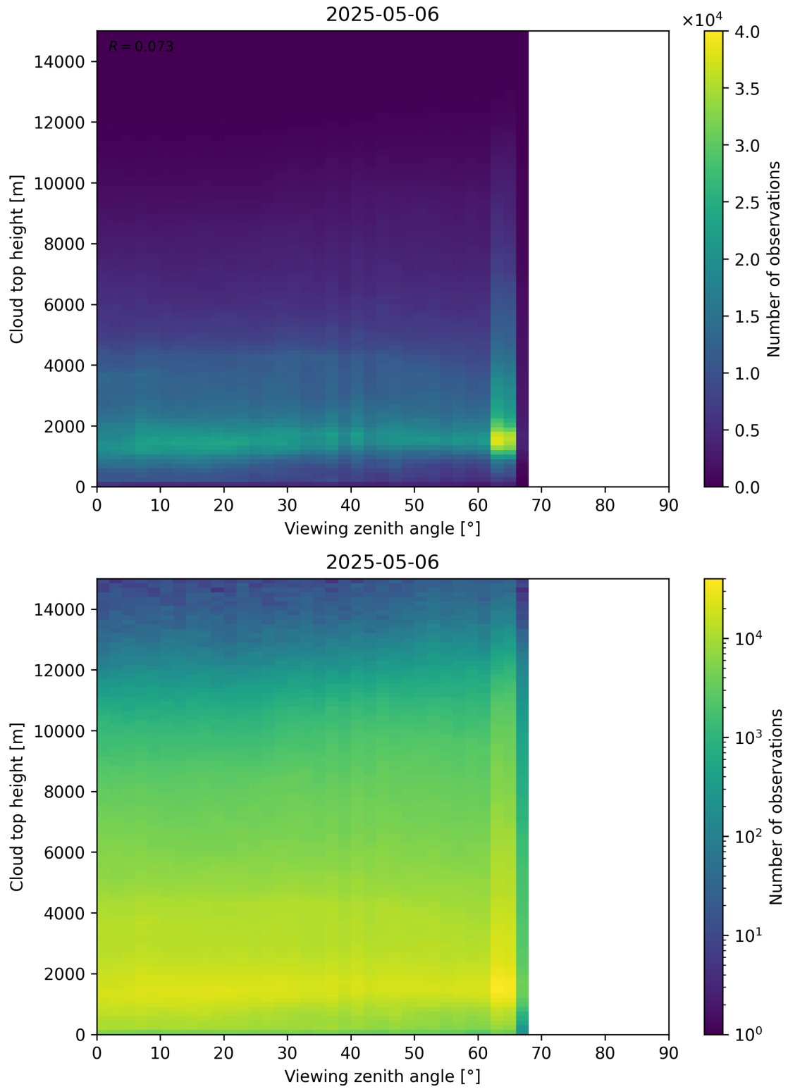
Figure 112: Scatter density plot of “Viewing zenith angle” against “Cloud top height” for 2025-05-05 to 2025-05-07.
