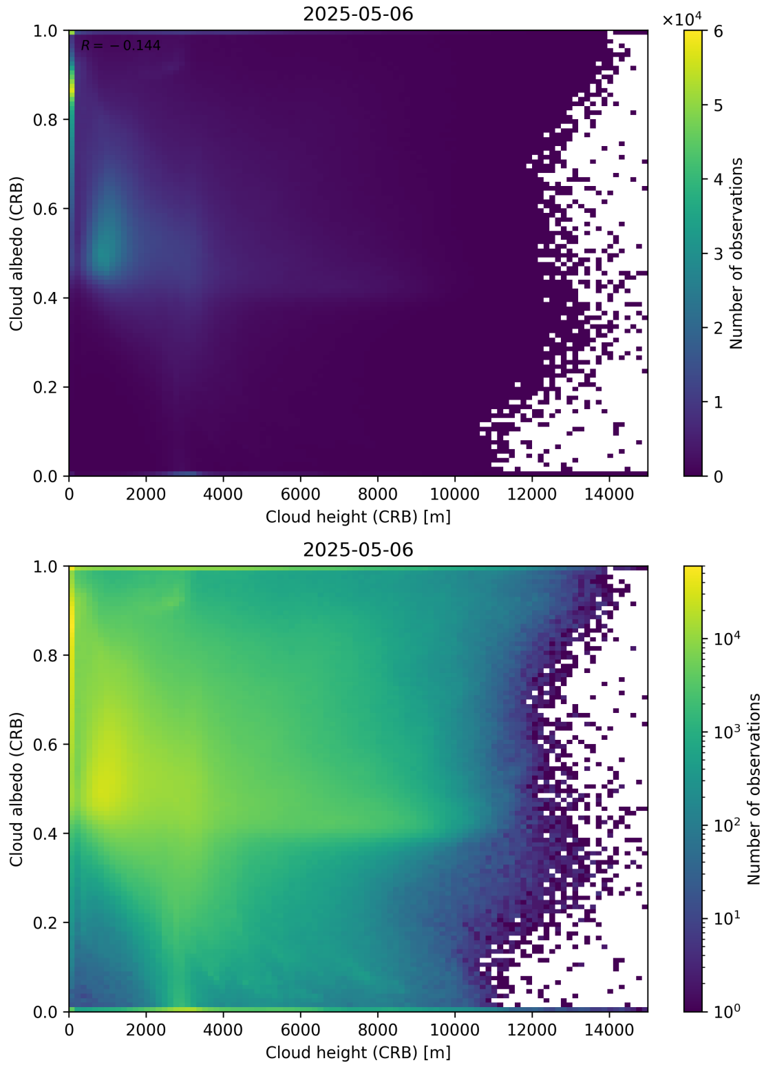
Figure 80: Scatter density plot of “Cloud height (CRB)” against “Cloud albedo (CRB)” for 2025-05-05 to 2025-05-07.
