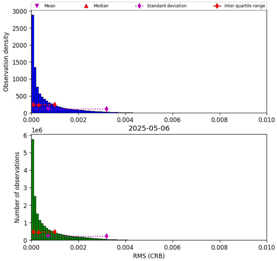
Figure 48: Histogram of “RMS (CRB)” for 2025-05-05 to 2025-05-07
