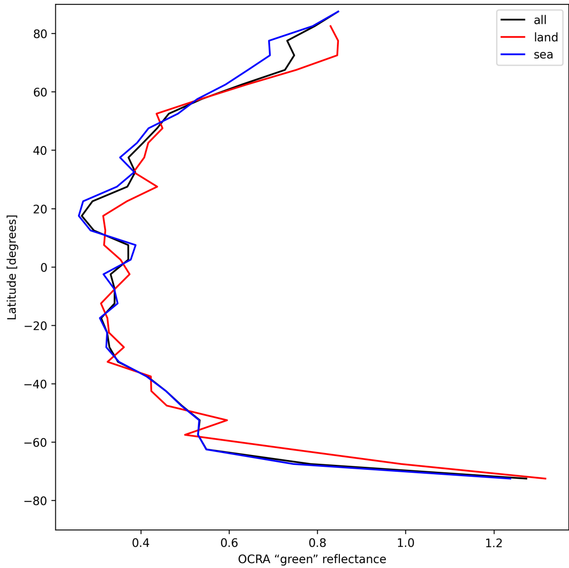
Figure 36: Zonal average of “OCRA “green” reflectance” for 2025-05-05 to 2025-05-07.
