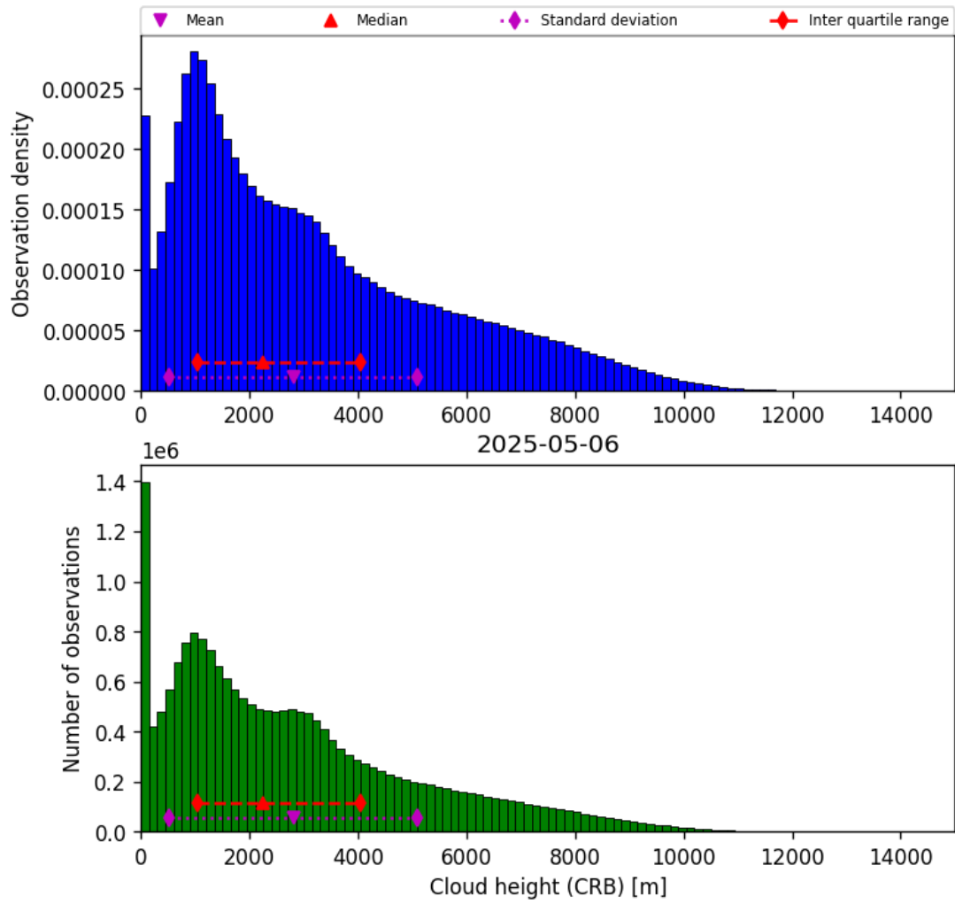
Figure 43: Histogram of “Cloud height (CRB)” for 2025-05-05 to 2025-05-07
