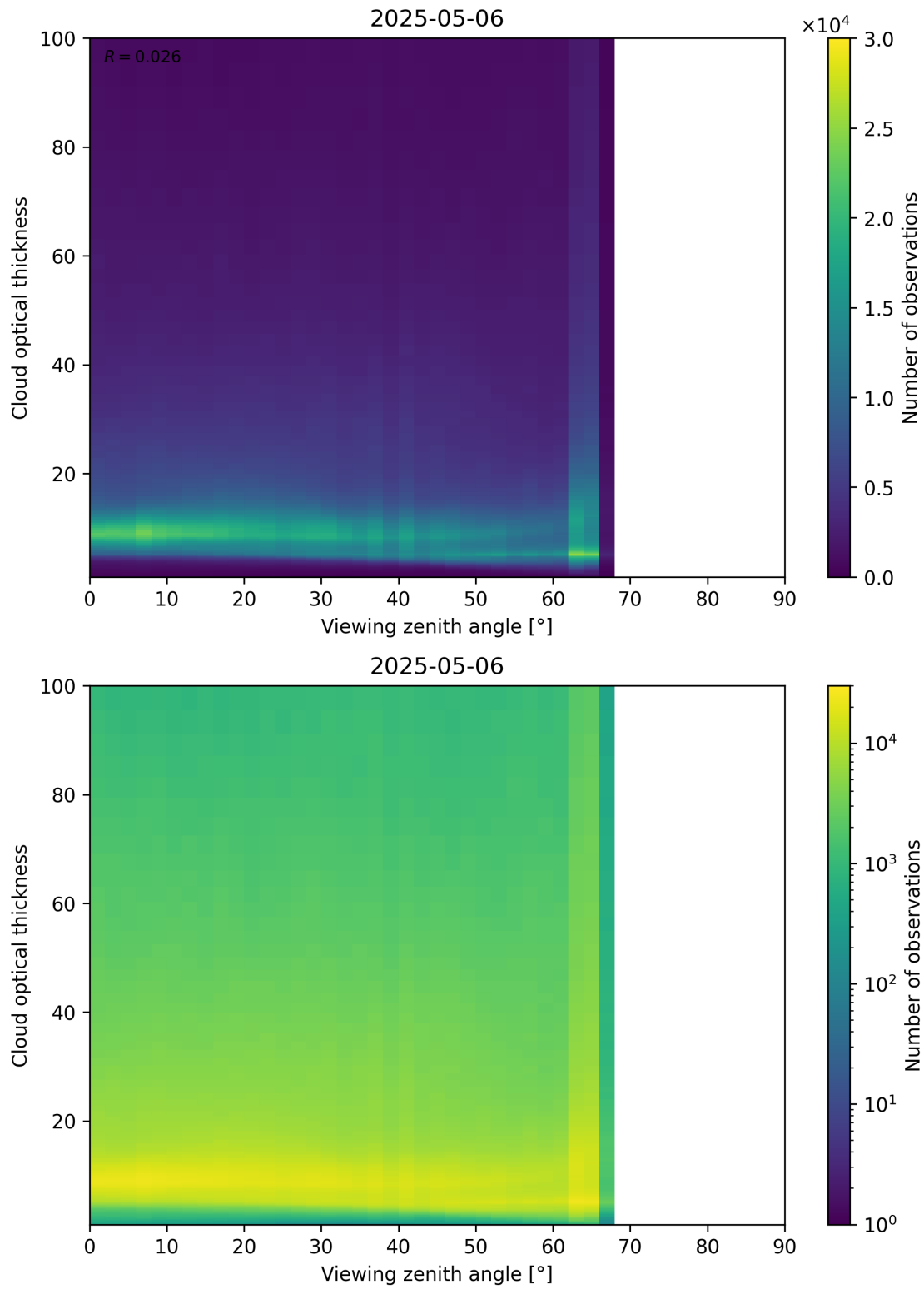
Figure 111: Scatter density plot of “Viewing zenith angle” against “Cloud optical thickness” for 2025-05-05 to 2025-05-07.
