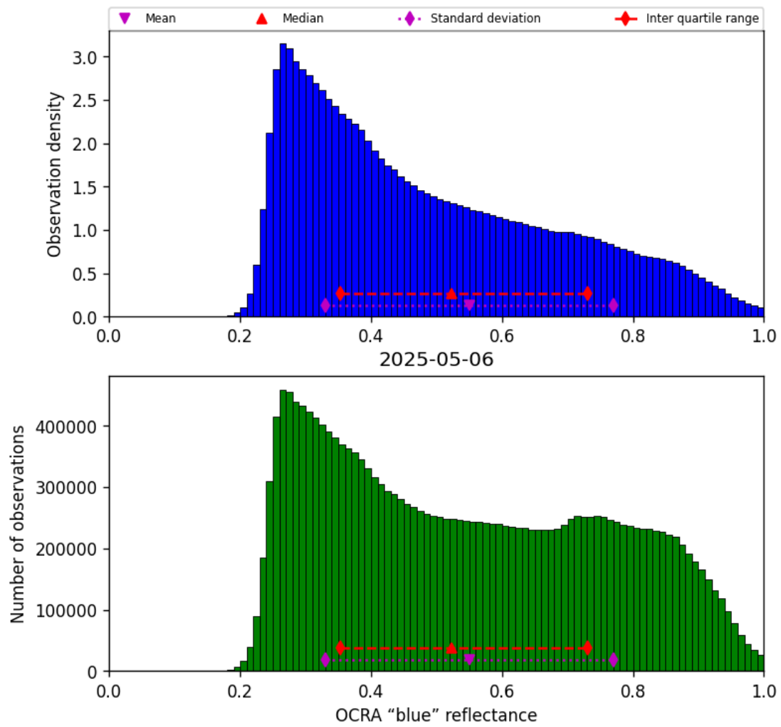
Figure 51: Histogram of “OCRA “blue” reflectance” for 2025-05-05 to 2025-05-07
