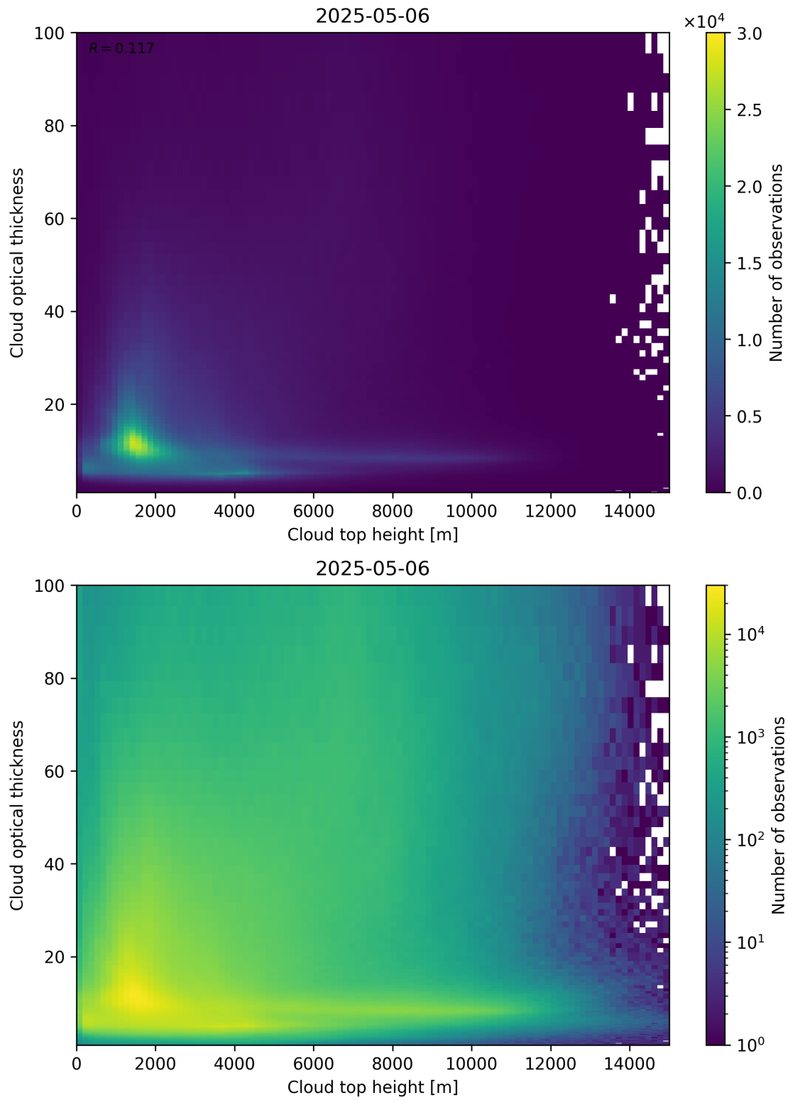
Figure 90: Scatter density plot of “Cloud top height” against “Cloud optical thickness” for 2025-05-05 to 2025-05-07.
