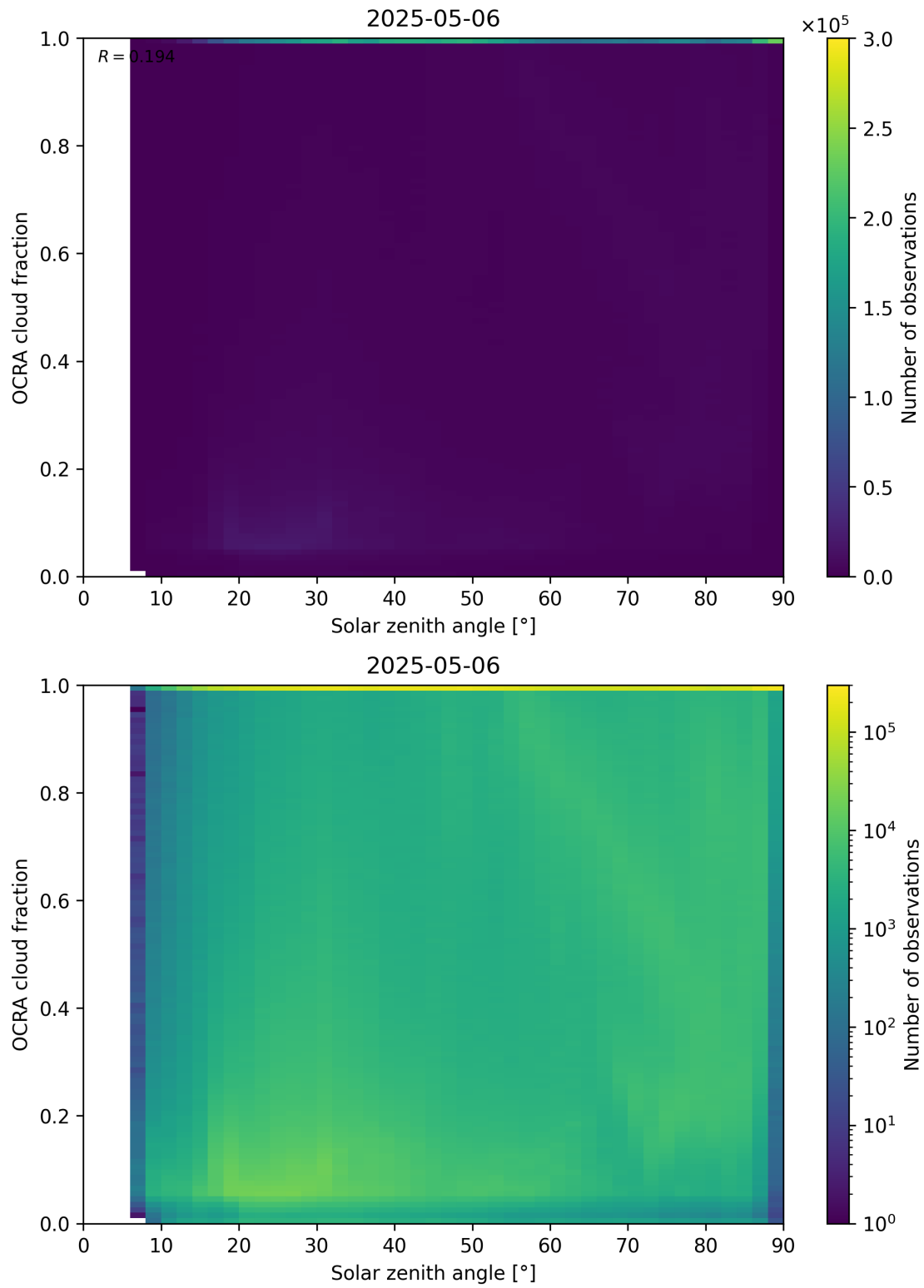
Figure 100: Scatter density plot of “Solar zenith angle” against “OCRA cloud fraction” for 2025-05-05 to 2025-05-07.
