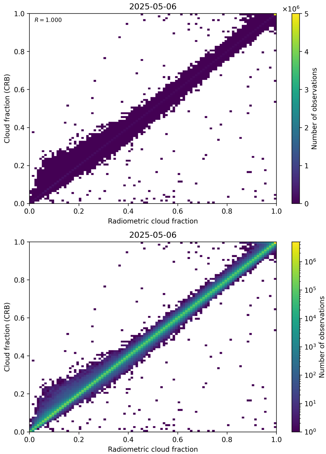
Figure 73: Scatter density plot of “Radiometric cloud fraction” against “Cloud fraction (CRB)” for 2025-05-05 to 2025-05-07.
