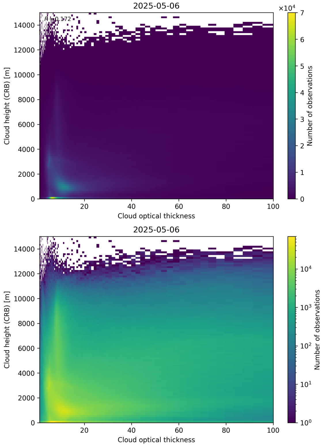
Figure 85: Scatter density plot of “Cloud optical thickness” against “Cloud height (CRB)” for 2025-05-05 to 2025-05-07.
