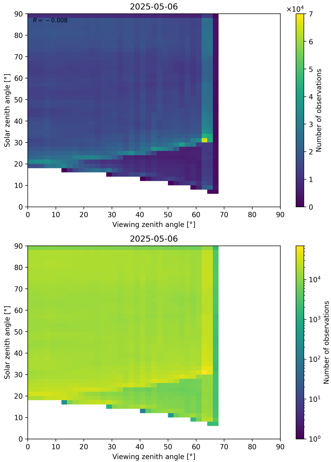
Figure 114: Scatter density plot of “Viewing zenith angle” against “Solar zenith angle” for 2025-05-05 to 2025-05-07.
