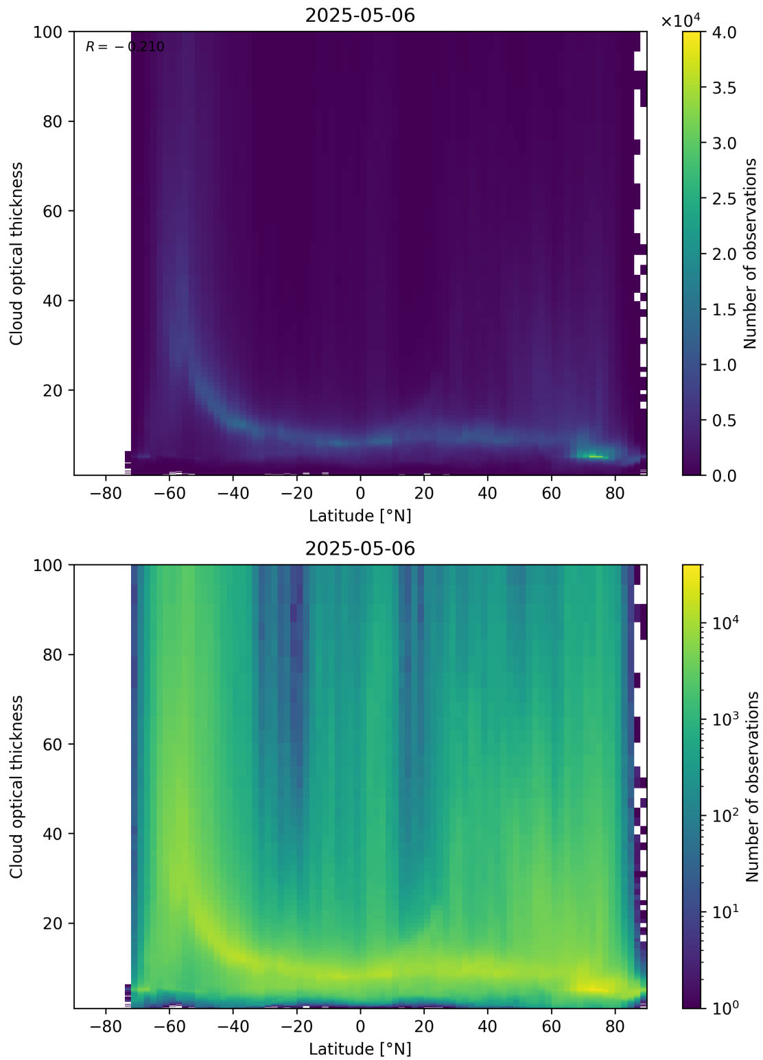
Figure 96: Scatter density plot of “Latitude” against “Cloud optical thickness” for 2025-05-05 to 2025-05-07.
