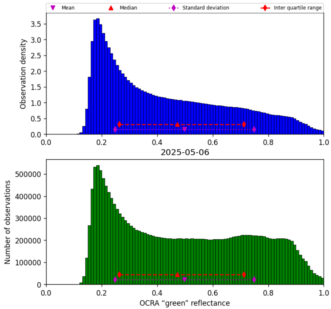
Figure 52: Histogram of “OCRA “green” reflectance” for 2025-05-05 to 2025-05-07
