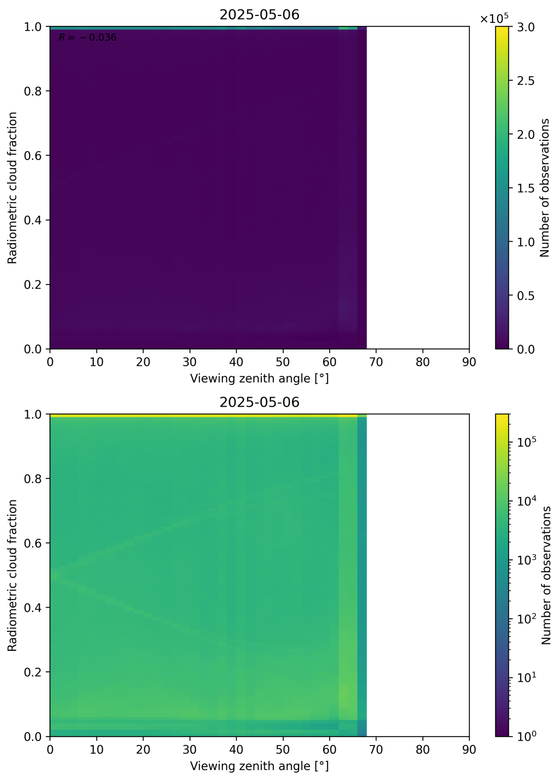
Figure 107: Scatter density plot of “Viewing zenith angle” against “Radiometric cloud fraction” for 2025-05-05 to 2025-05-07.
