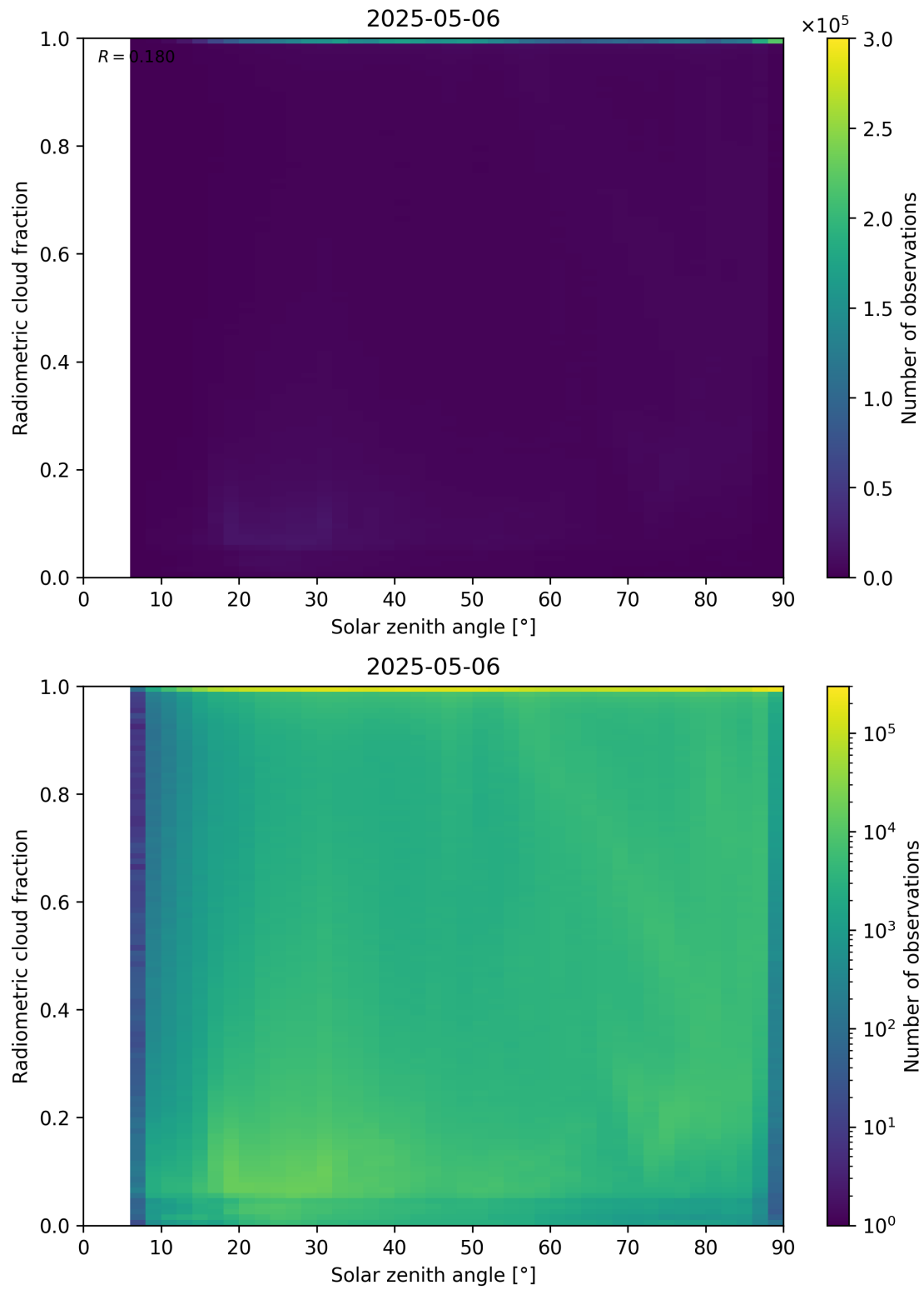
Figure 99: Scatter density plot of “Solar zenith angle” against “Radiometric cloud fraction” for 2025-05-05 to 2025-05-07.
