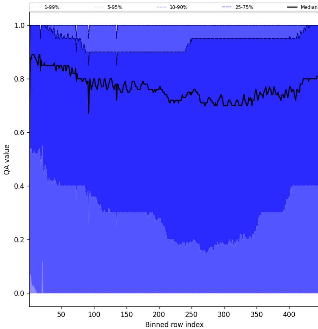
Figure 54: Along track statistics of “QA value” for 2025-05-05 to 2025-05-07
