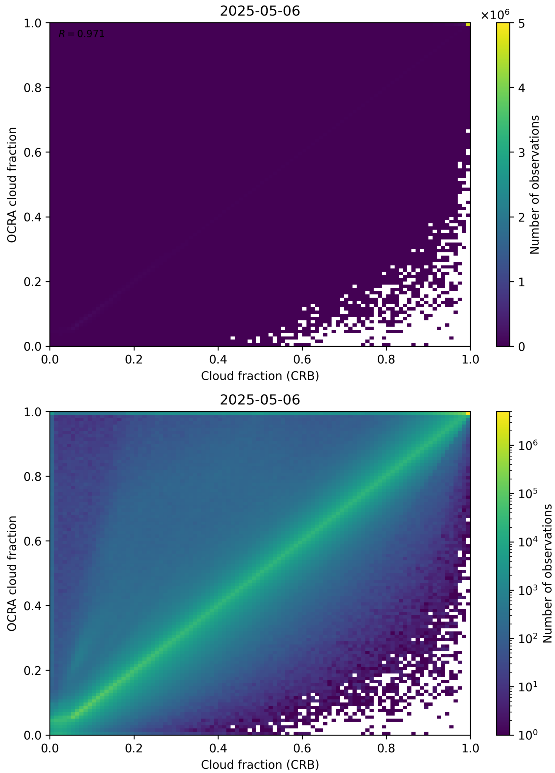
Figure 78: Scatter density plot of “Cloud fraction (CRB)” against “OCRA cloud fraction” for 2025-05-05 to 2025-05-07.
