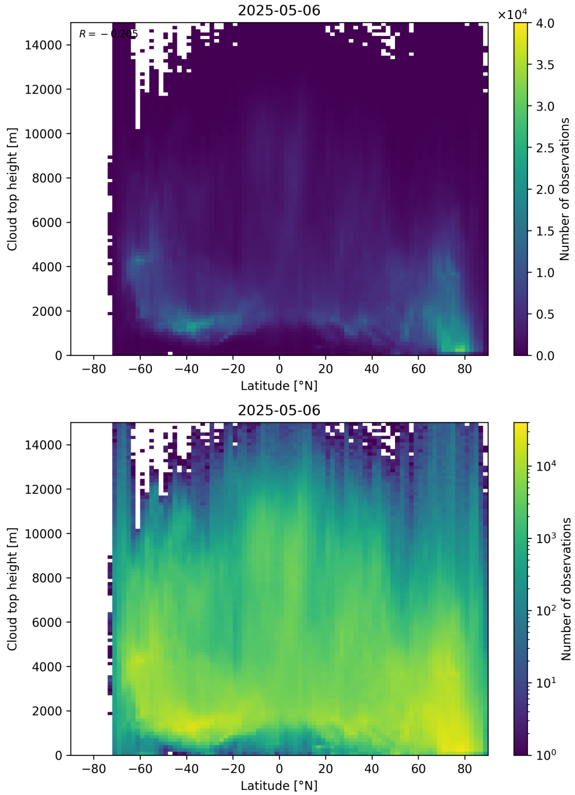
Figure 97: Scatter density plot of “Latitude” against “Cloud top height” for 2025-05-05 to 2025-05-07.
