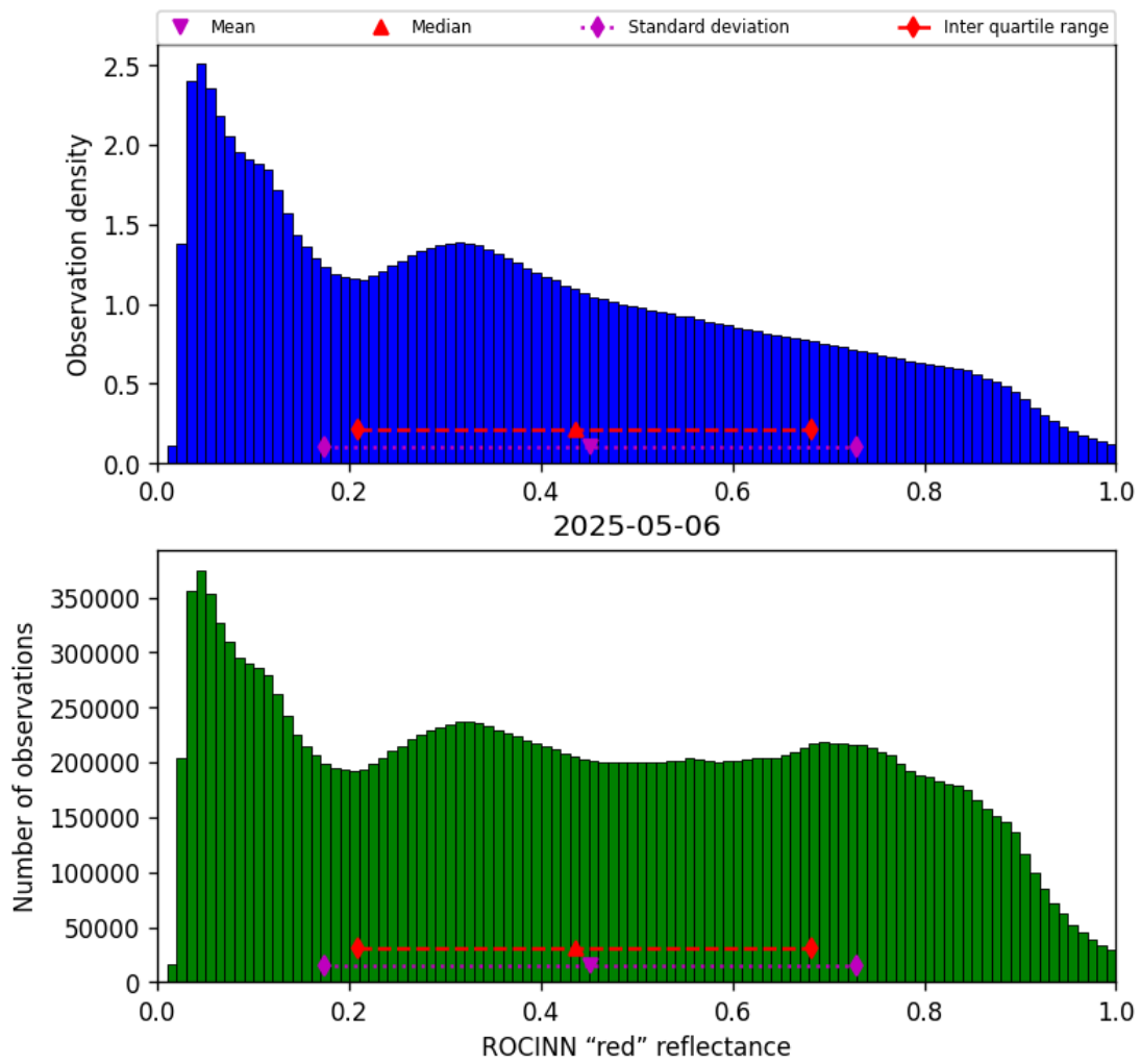
Figure 53: Histogram of “ROCINN “red” reflectance” for 2025-05-05 to 2025-05-07
