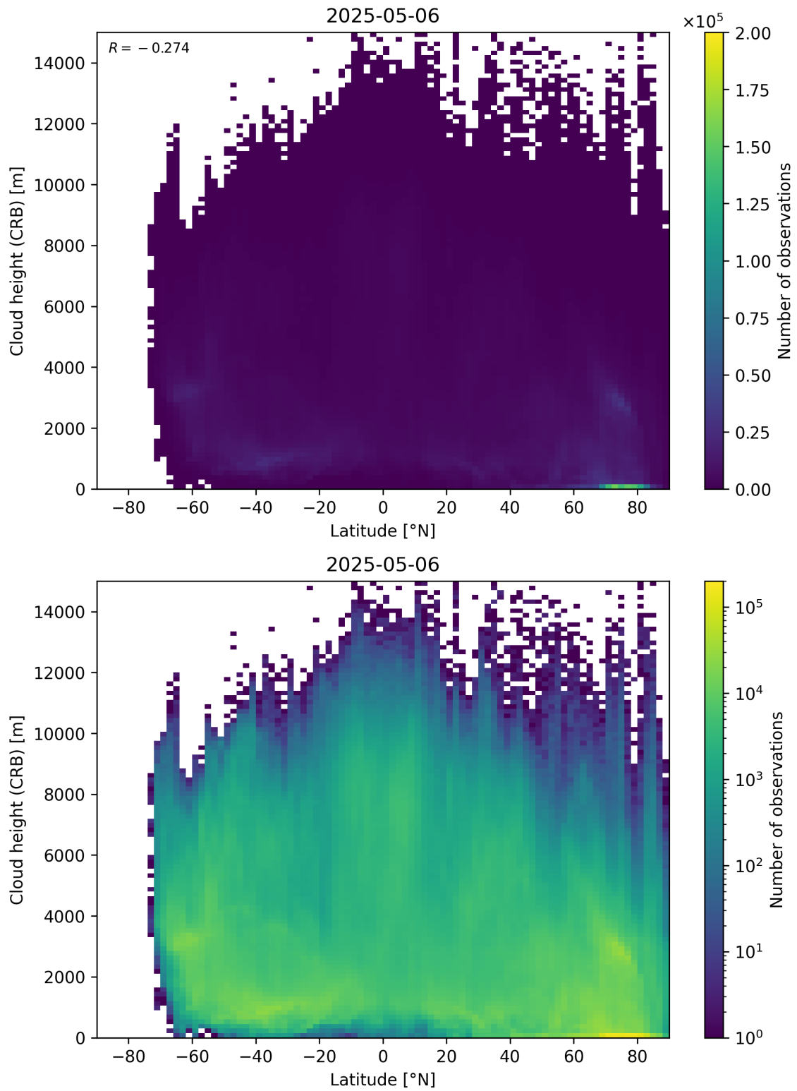
Figure 95: Scatter density plot of “Latitude” against “Cloud height (CRB)” for 2025-05-05 to 2025-05-07.
