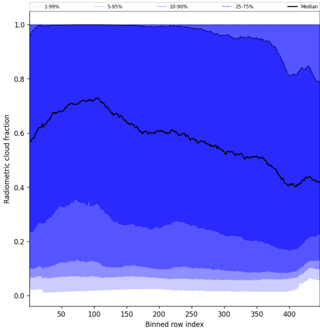
Figure 55: Along track statistics of “Radiometric cloud fraction” for 2025-05-05 to 2025-05-07
