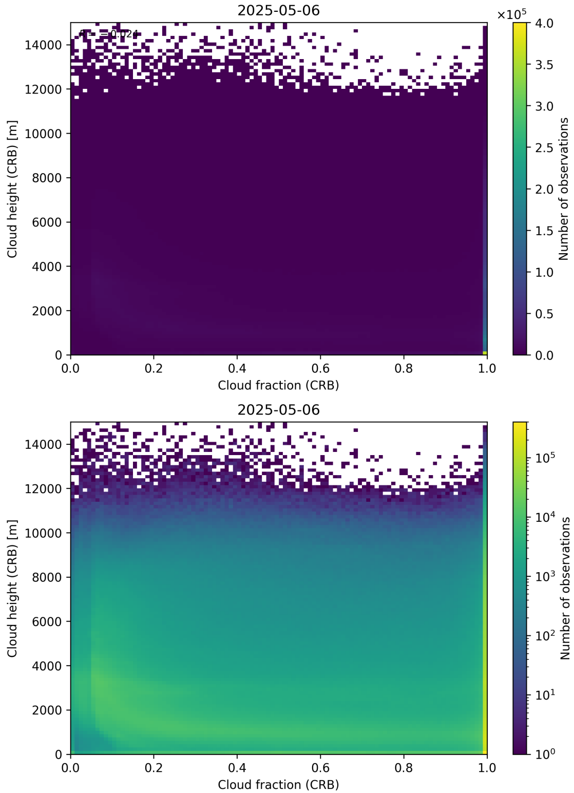
Figure 79: Scatter density plot of “Cloud fraction (CRB)” against “Cloud height (CRB)” for 2025-05-05 to 2025-05-07.
