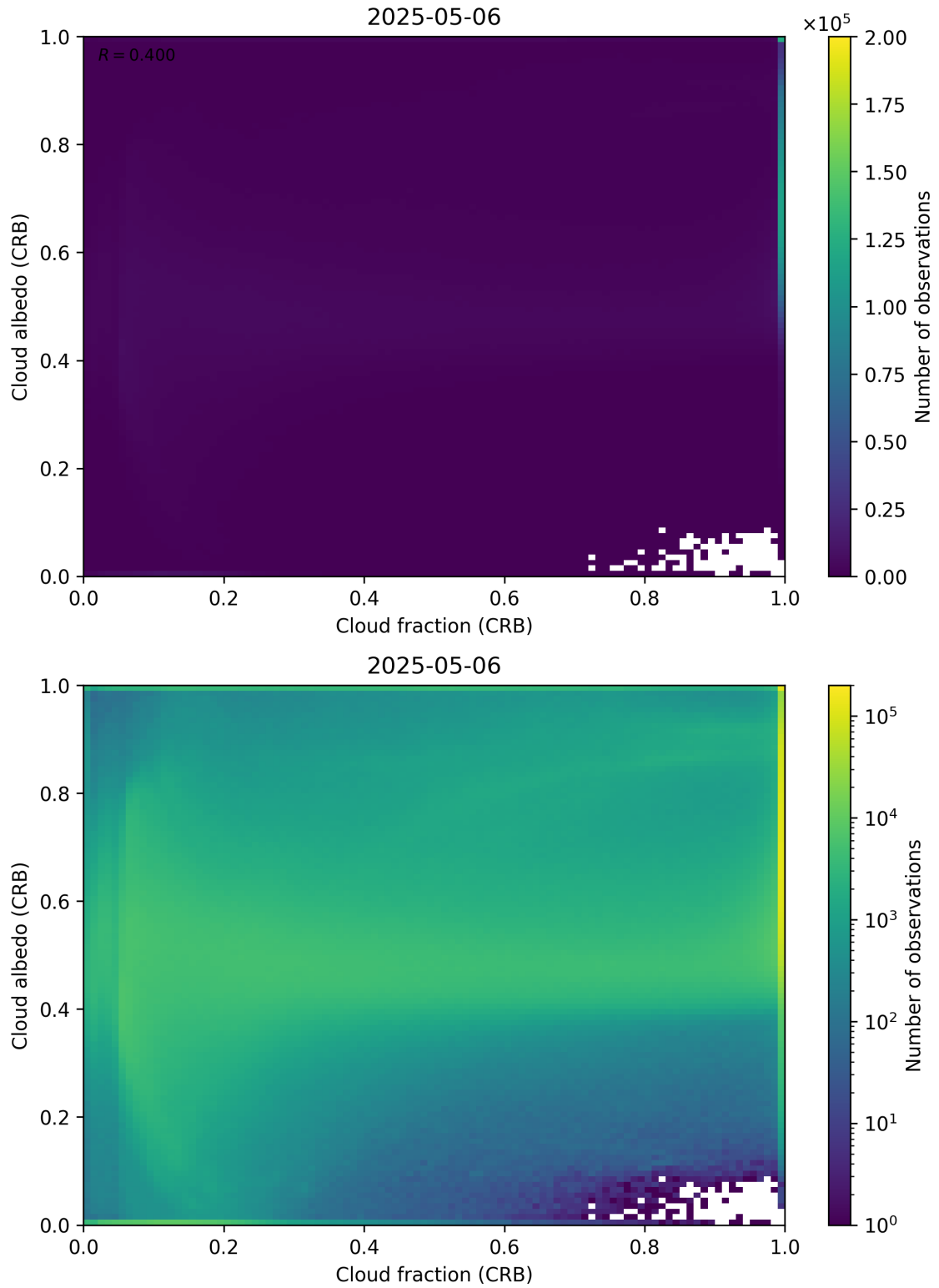
Figure 77: Scatter density plot of “Cloud fraction (CRB)” against “Cloud albedo (CRB)” for 2025-05-05 to 2025-05-07.
