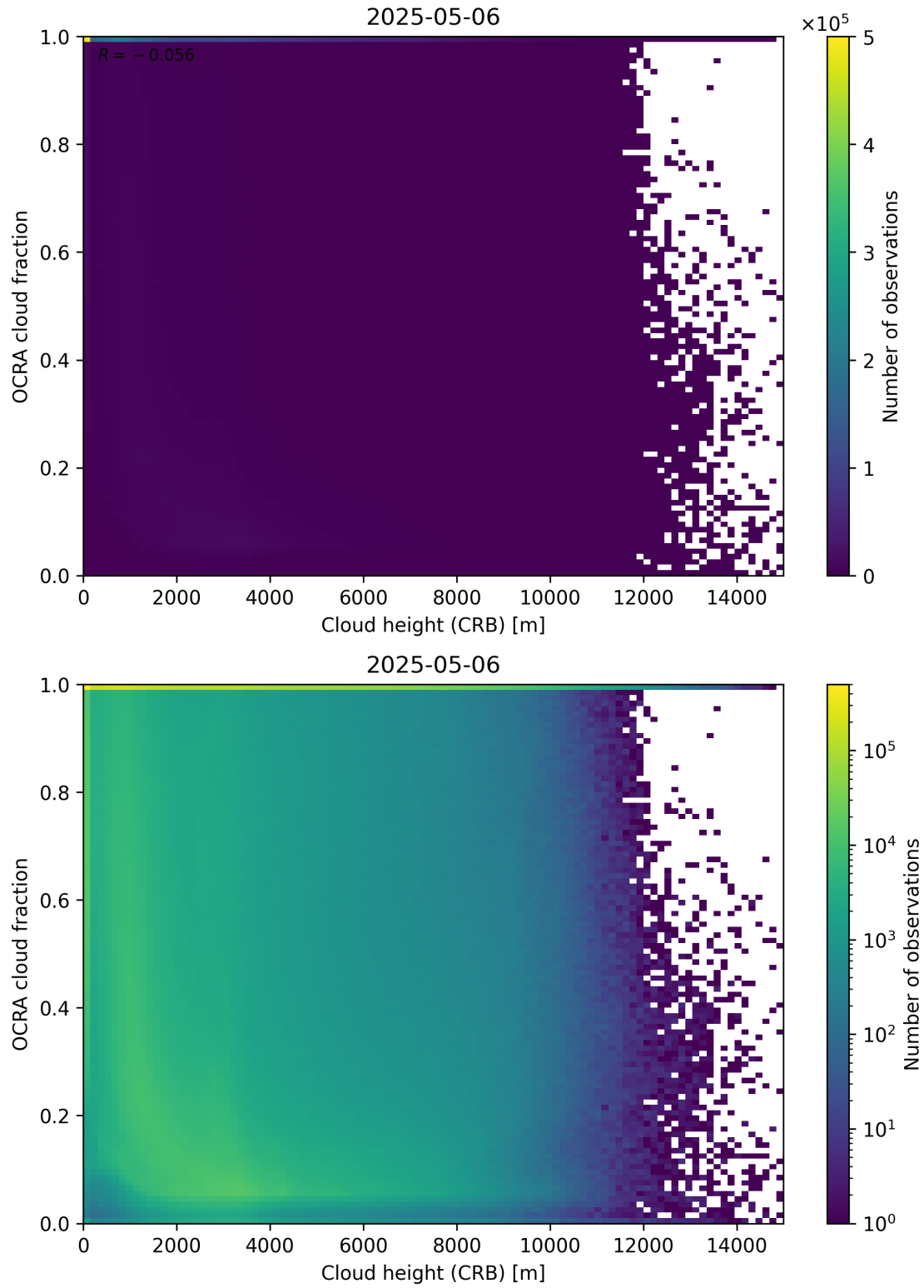
Figure 81: Scatter density plot of “Cloud height (CRB)” against “OCRA cloud fraction” for 2025-05-05 to 2025-05-07.
