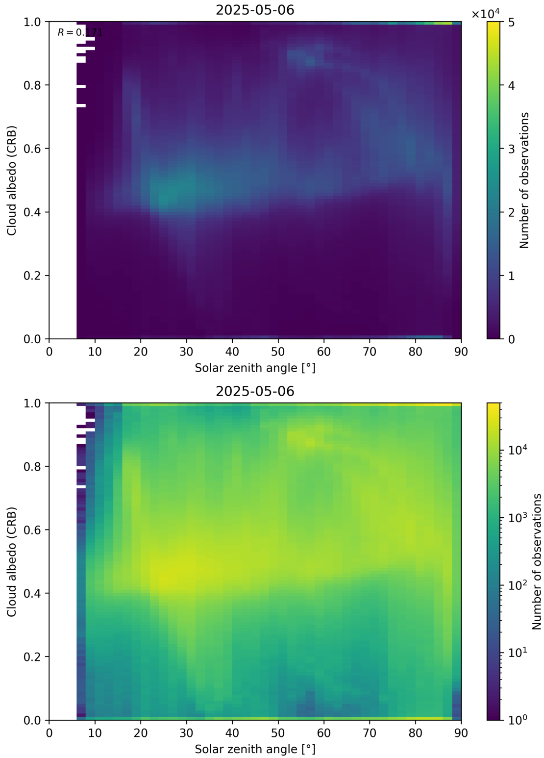
Figure 98: Scatter density plot of “Solar zenith angle” against “Cloud albedo (CRB)” for 2025-05-05 to 2025-05-07.
