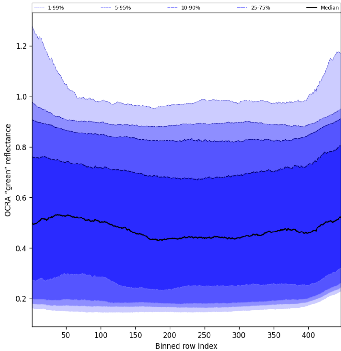
Figure 68: Along track statistics of “OCRA “green” reflectance” for 2025-05-05 to 2025-05-07
