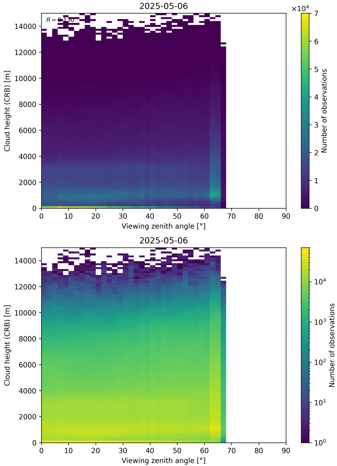
Figure 110: Scatter density plot of “Viewing zenith angle” against “Cloud height (CRB)” for 2025-05-05 to 2025-05-07.
