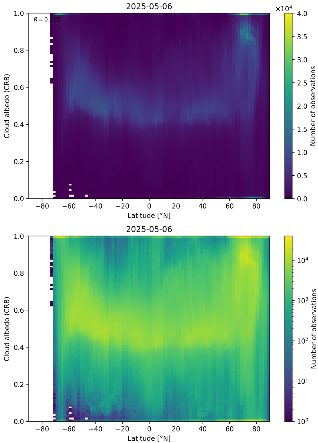
Figure 91: Scatter density plot of “Latitude” against “Cloud albedo (CRB)” for 2025-05-05 to 2025-05-07.
