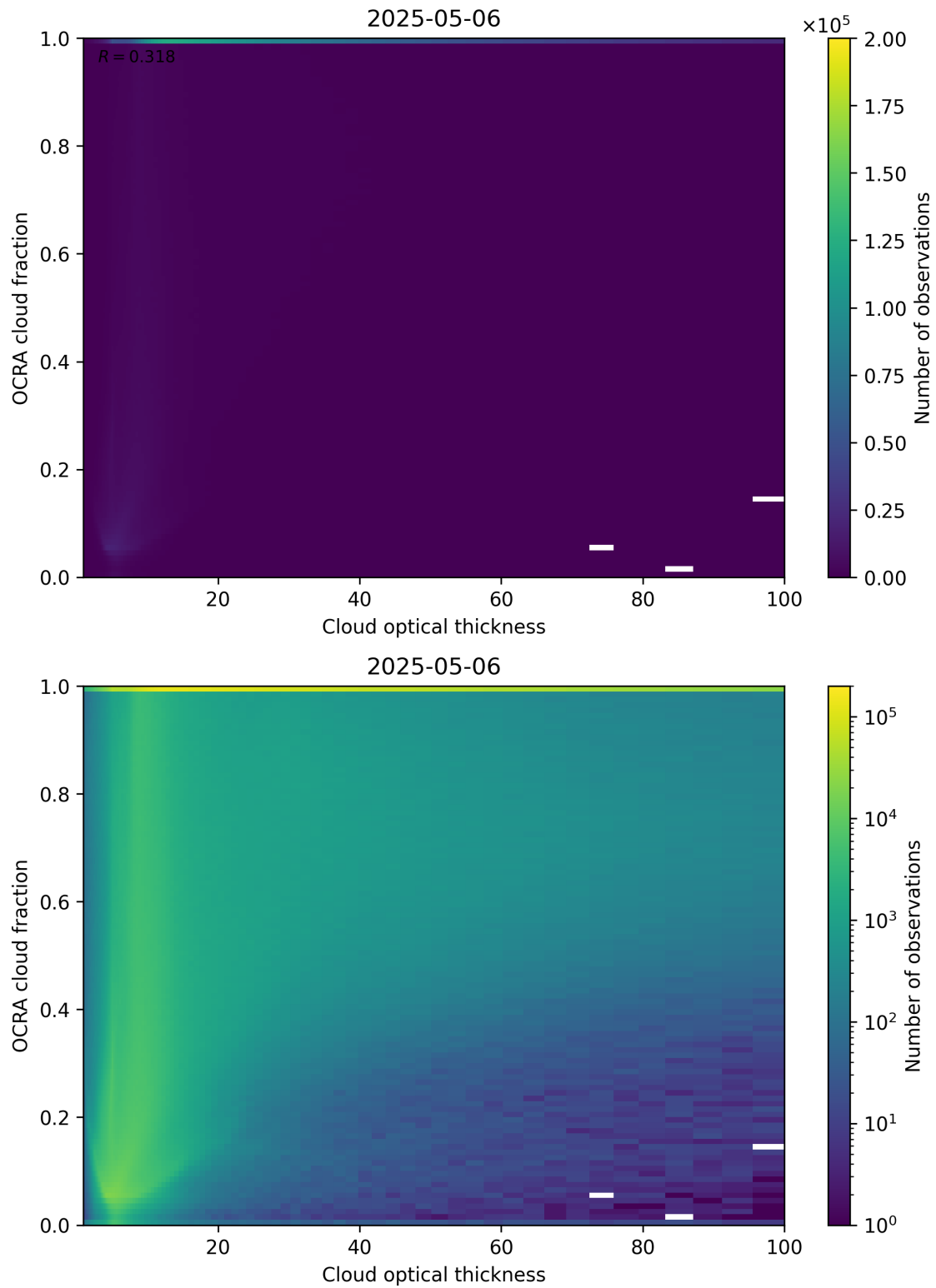
Figure 83: Scatter density plot of “Cloud optical thickness” against “OCRA cloud fraction” for 2025-05-05 to 2025-05-07.
