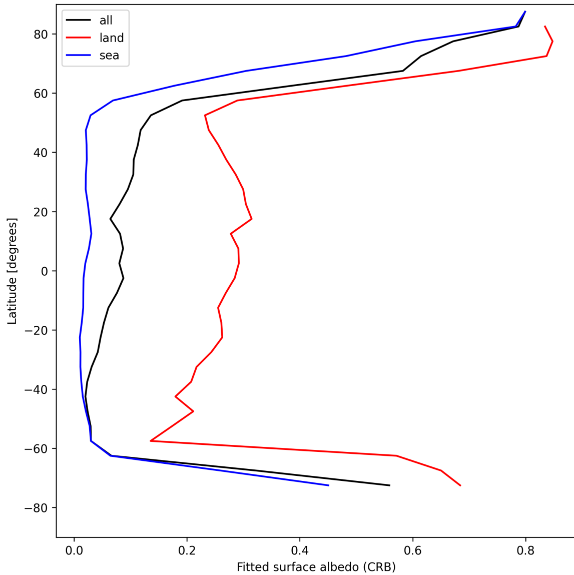
Figure 30: Zonal average of “Fitted surface albedo (CRB)” for 2025-05-05 to 2025-05-07.
