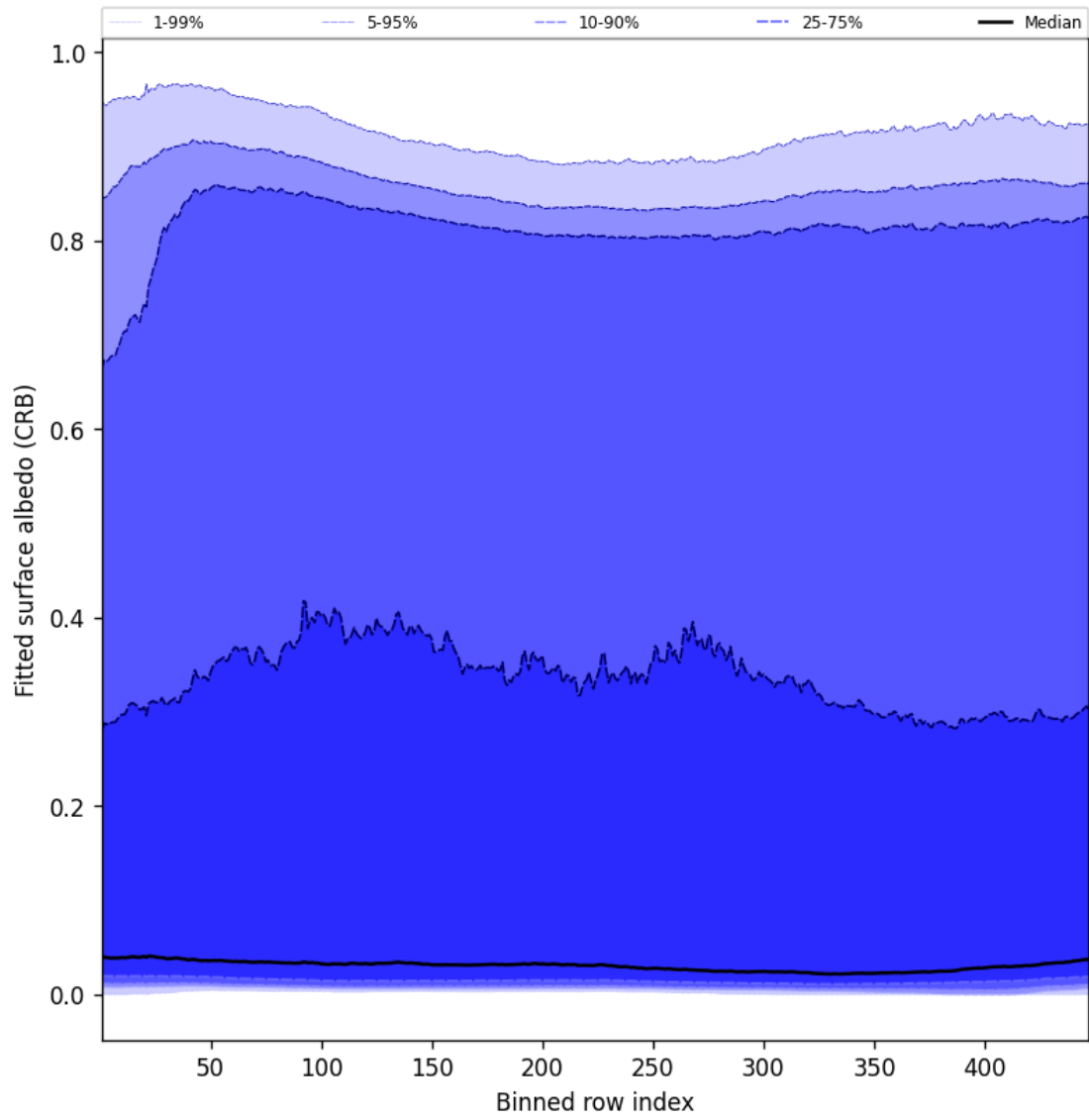
Figure 62: Along track statistics of “Fitted surface albedo (CRB)” for 2025-05-05 to 2025-05-07
