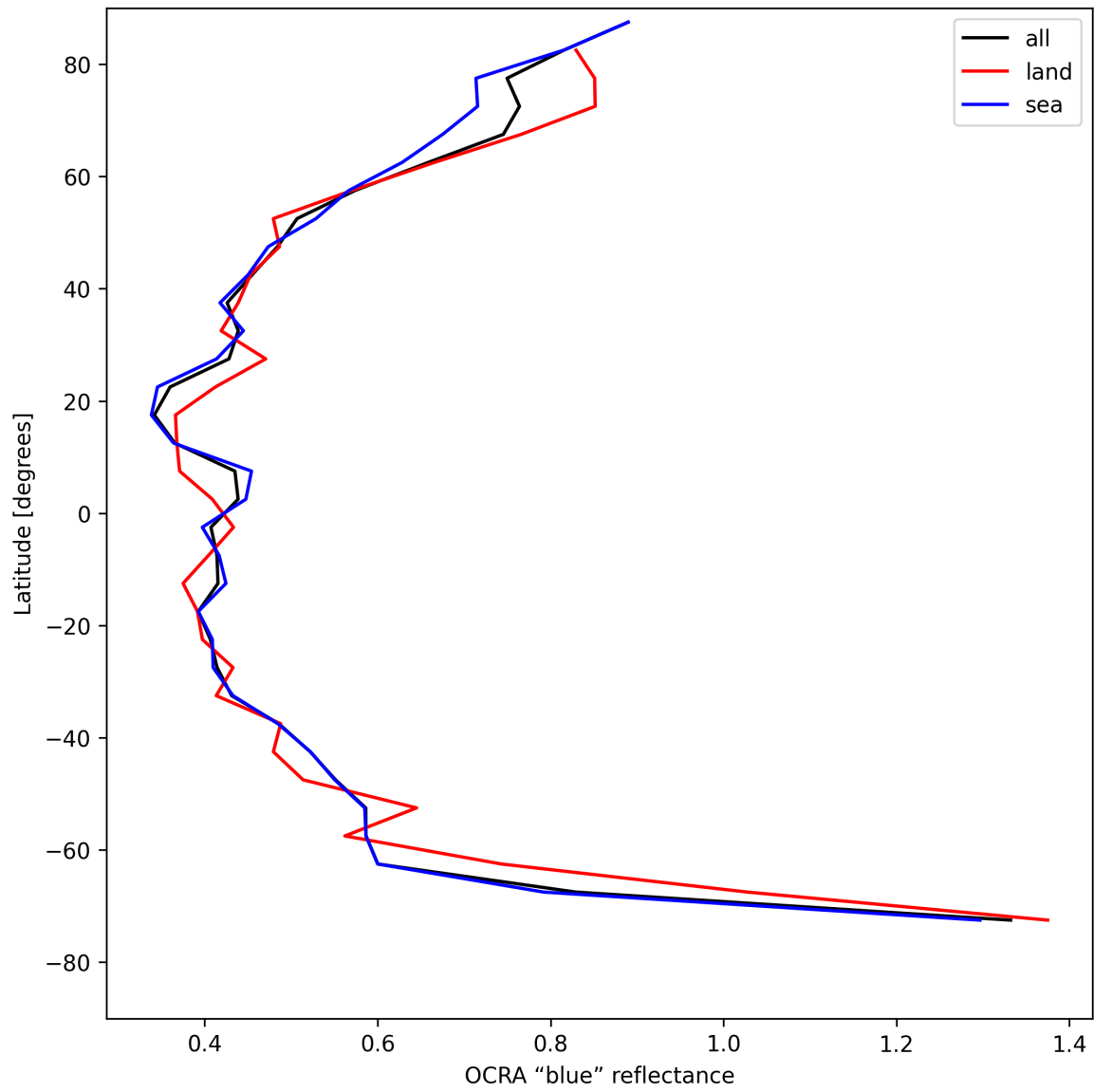
Figure 35: Zonal average of "OCRA "blue" reflectance" for 2025-05-05 to 2025-05-07.
