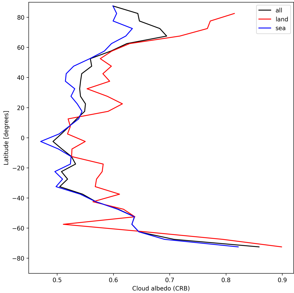
Figure 28: Zonal average of “Cloud albedo (CRB)” for 2025-05-05 to 2025-05-07.
