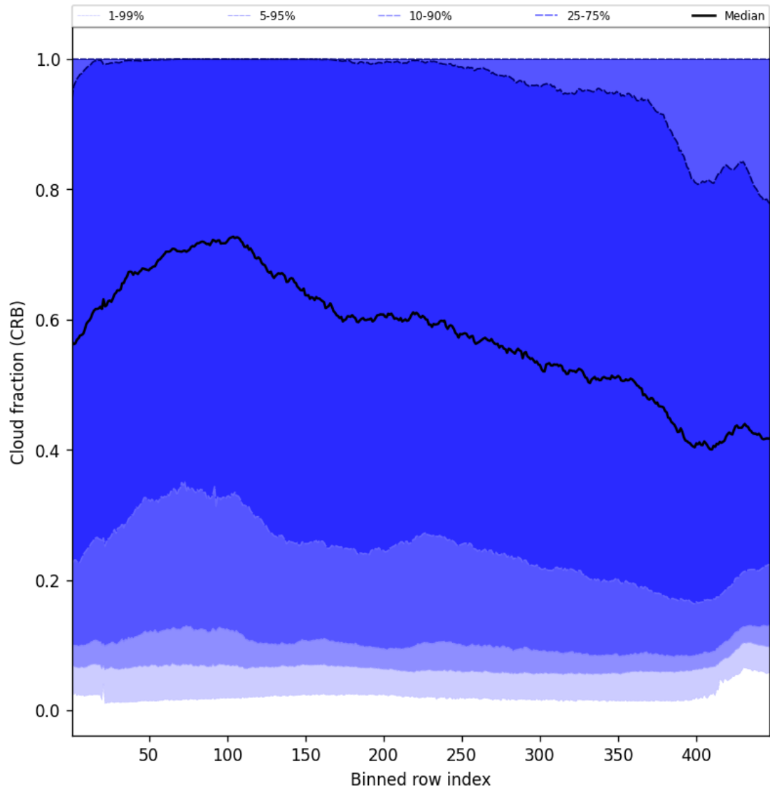
Figure 58: Along track statistics of “Cloud fraction (CRB)” for 2025-05-05 to 2025-05-07
