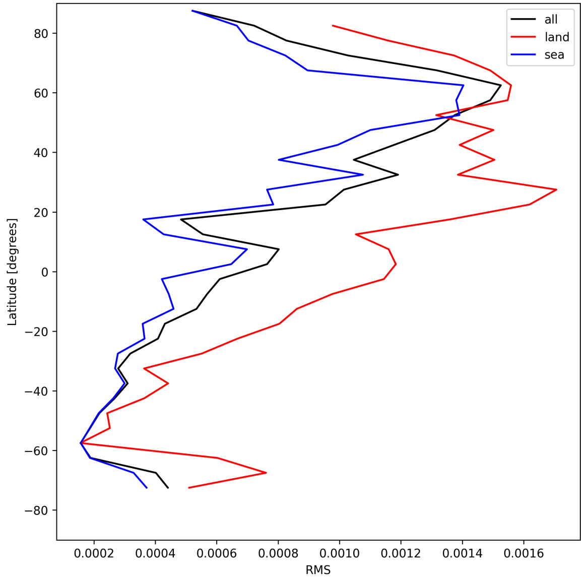
Figure 31: Zonal average of “RMS” for 2025-05-05 to 2025-05-07.
