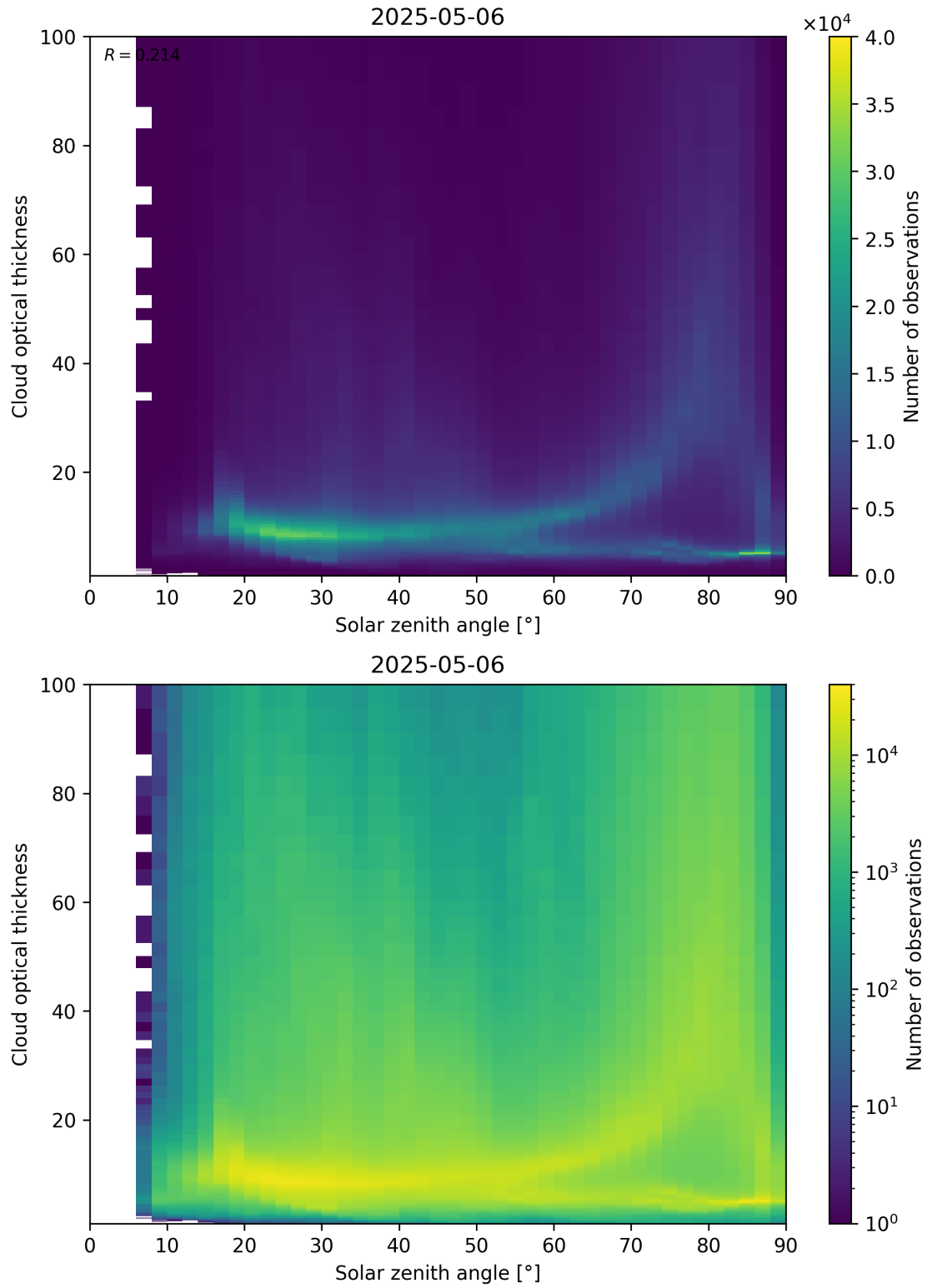
Figure 103: Scatter density plot of “Solar zenith angle” against “Cloud optical thickness” for 2025-05-05 to 2025-05-07.
