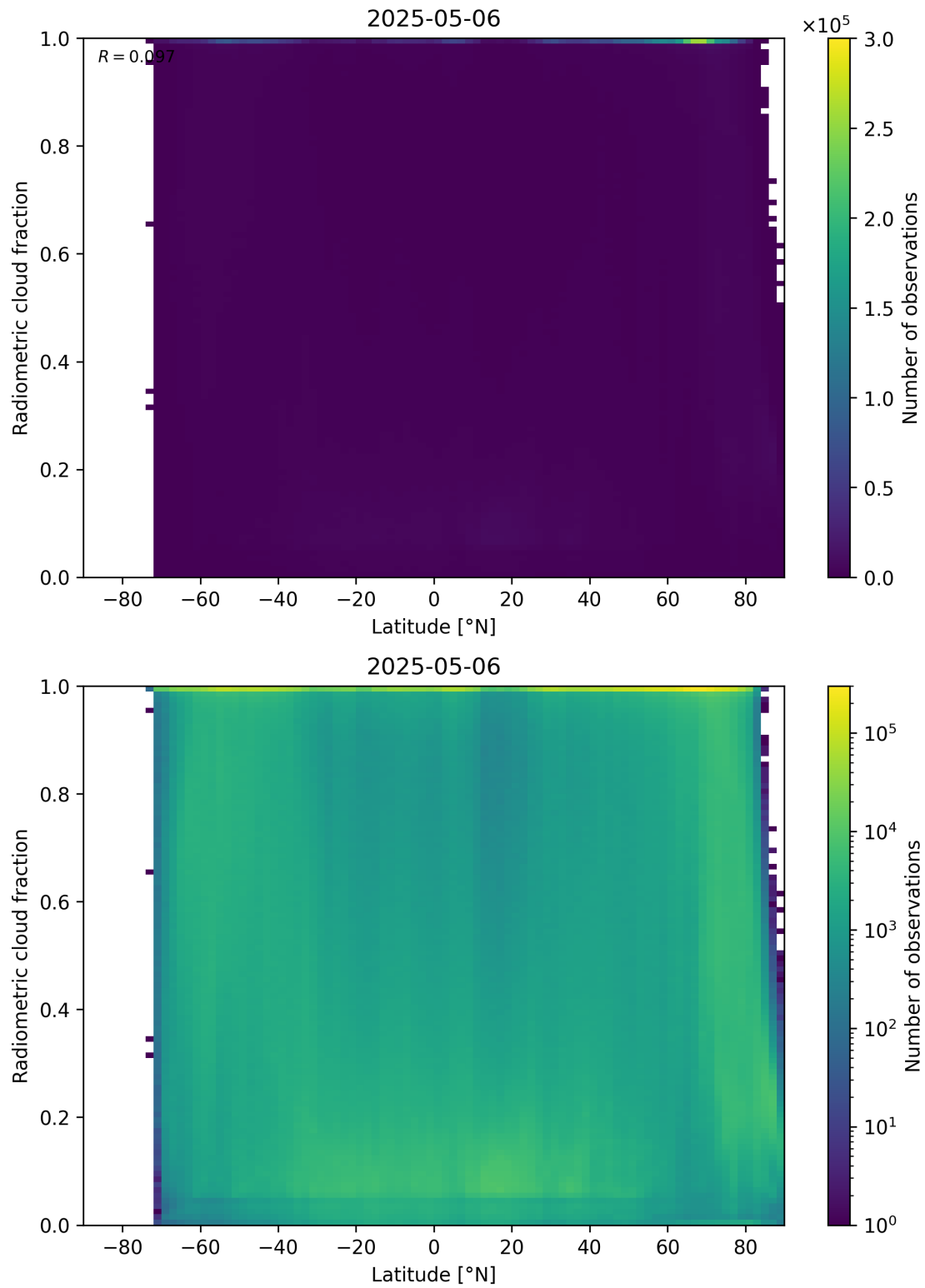
Figure 92: Scatter density plot of “Latitude” against “Radiometric cloud fraction” for 2025-05-05 to 2025-05-07.
