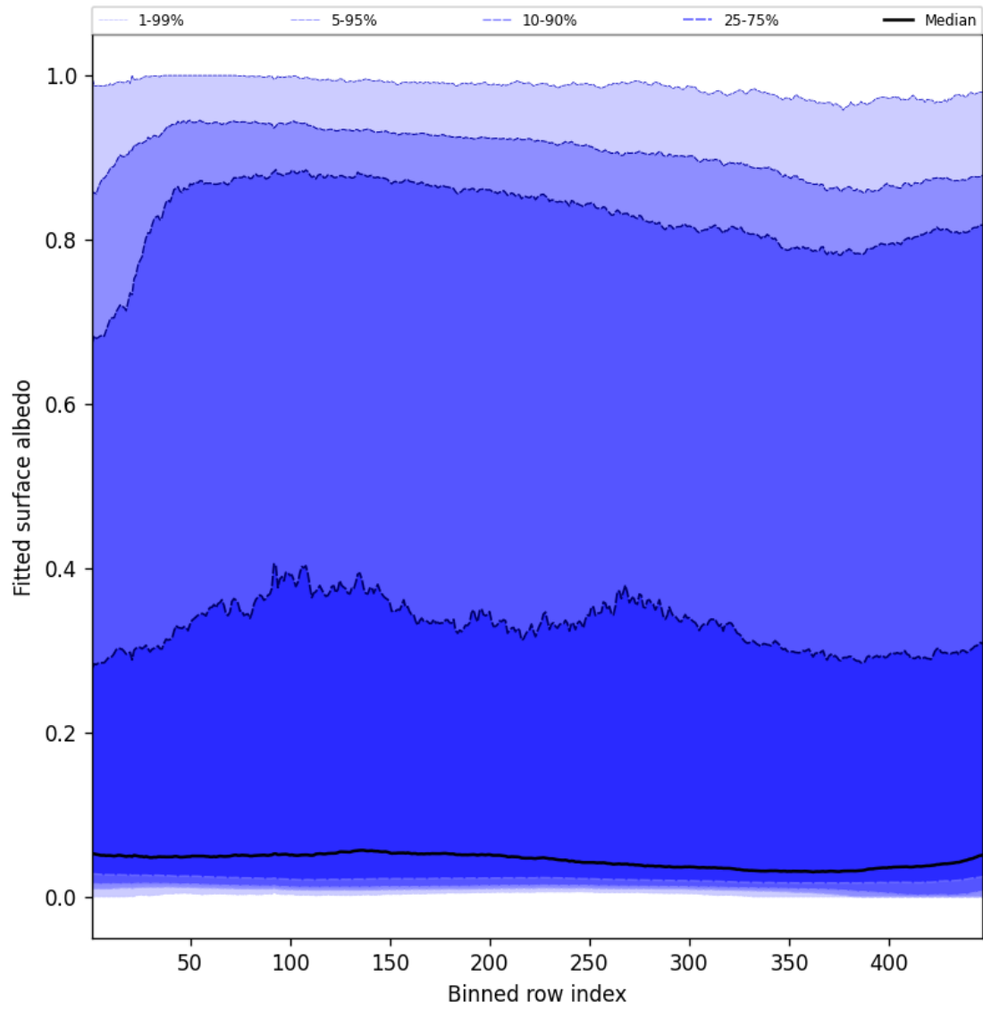
Figure 61: Along track statistics of “Fitted surface albedo” for 2025-05-05 to 2025-05-07
