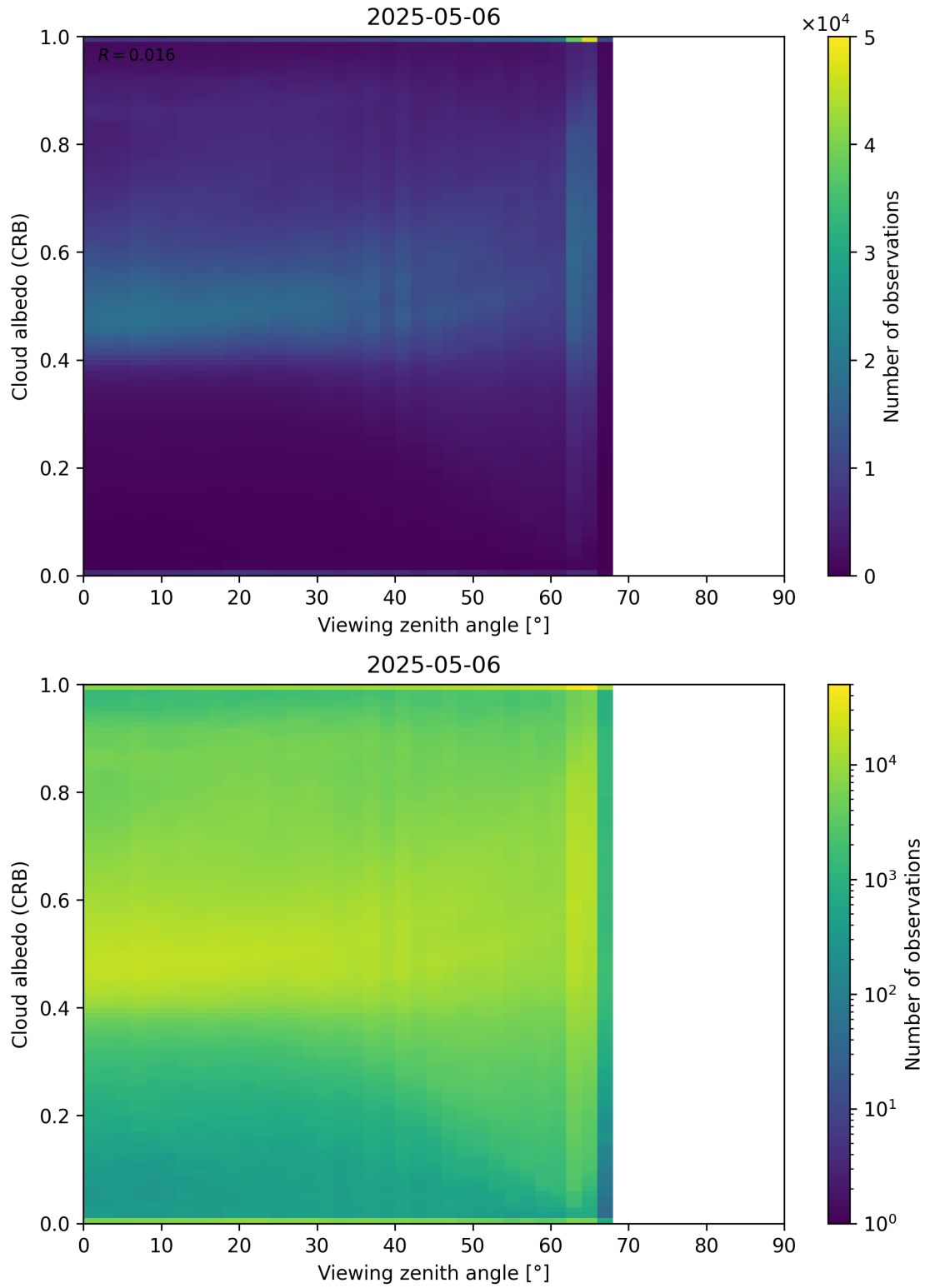
Figure 106: Scatter density plot of “Viewing zenith angle” against “Cloud albedo (CRB)” for 2025-05-05 to 2025-05-07.
