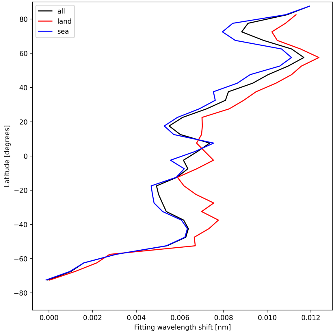
Figure 33: Zonal average of “Fitting wavelength shift” for 2025-05-05 to 2025-05-07.
