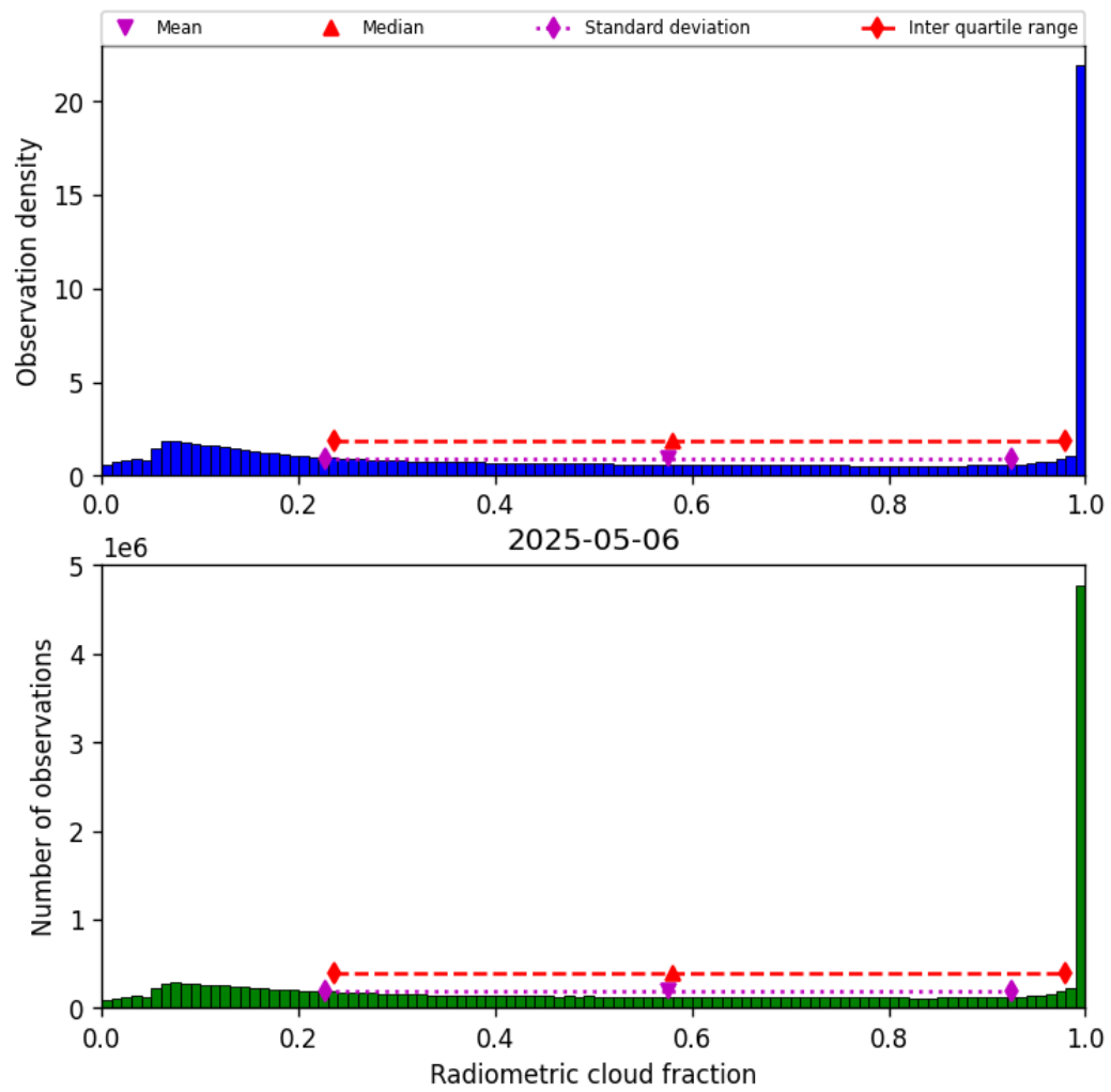
Figure 39: Histogram of “Radiometric cloud fraction” for 2025-05-05 to 2025-05-07
