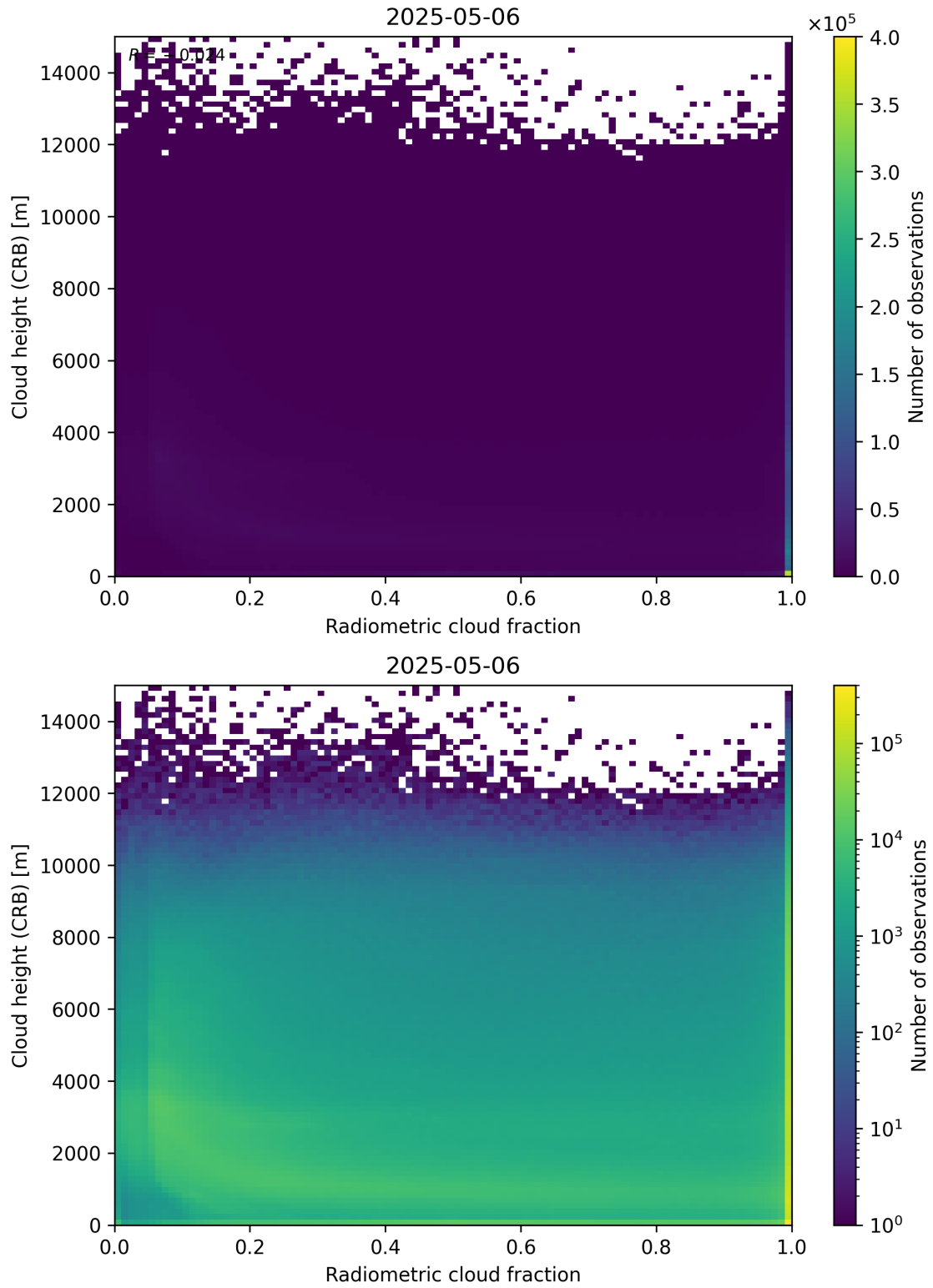
Figure 74: Scatter density plot of “Radiometric cloud fraction” against “Cloud height (CRB)” for 2025-05-05 to 2025-05-07.
