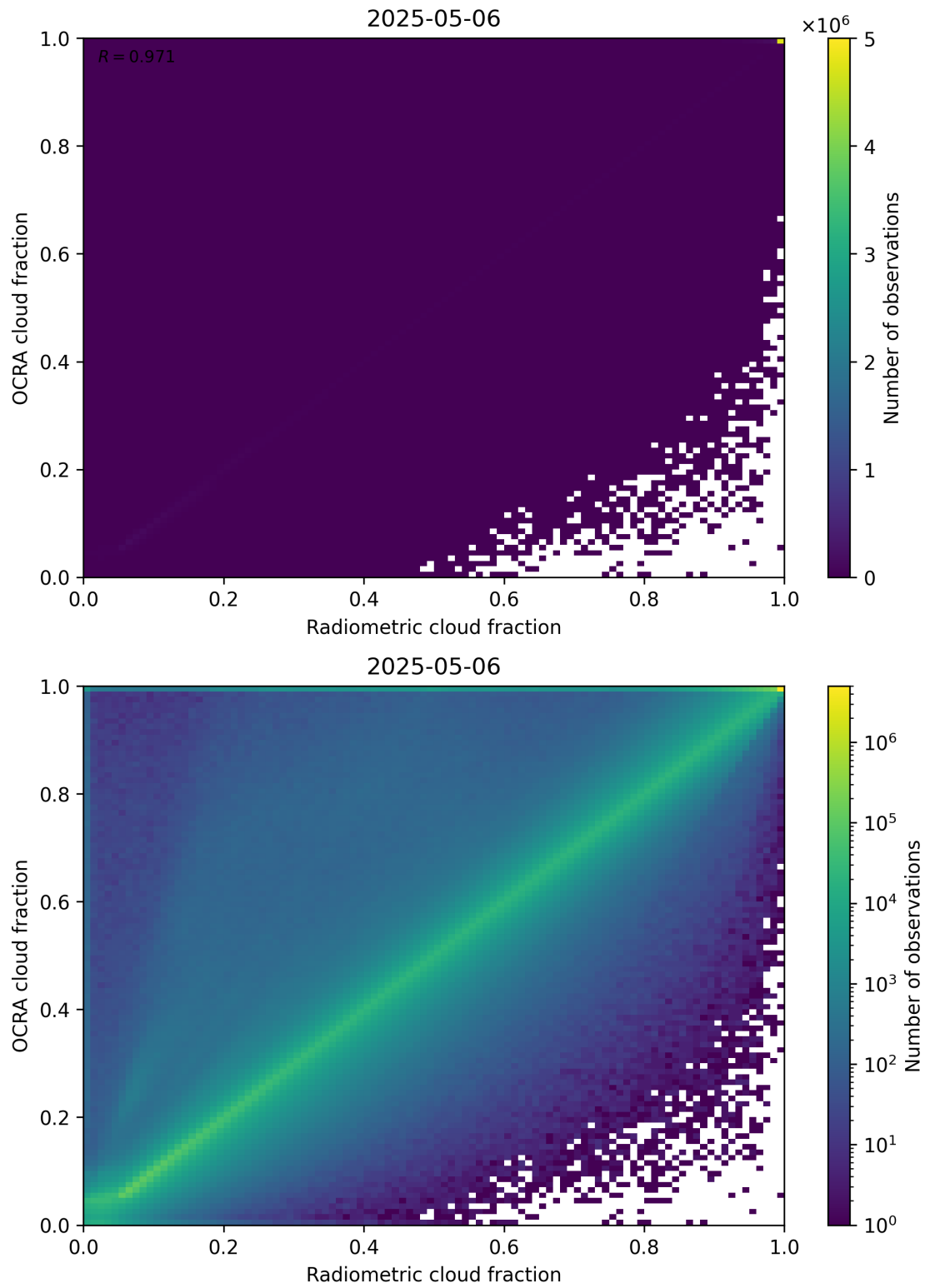
Figure 72: Scatter density plot of “Radiometric cloud fraction” against “OCRA cloud fraction” for 2025-05-05 to 2025-05-07.
