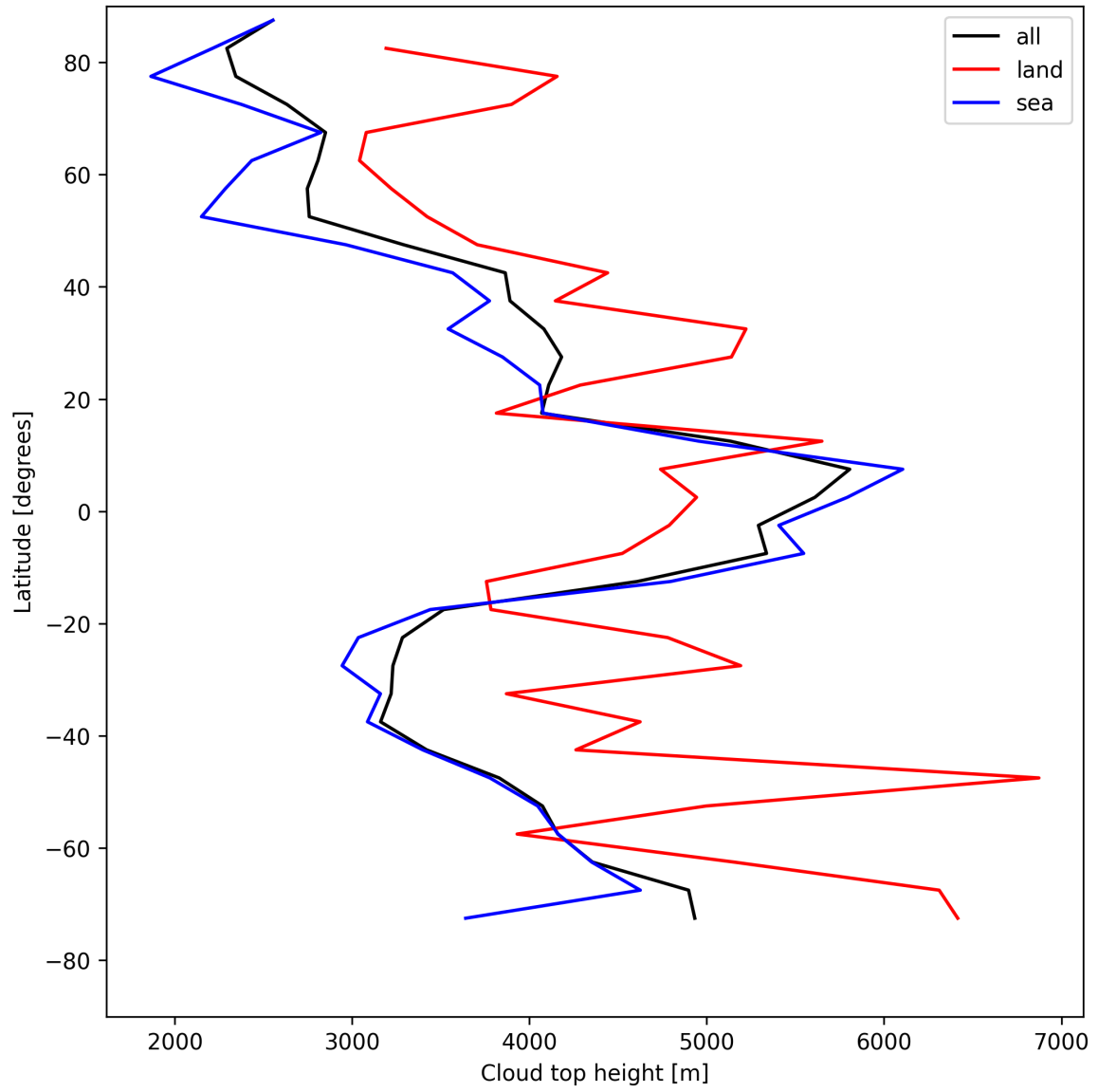
Figure 24: Zonal average of “Cloud top height” for 2025-05-05 to 2025-05-07.
