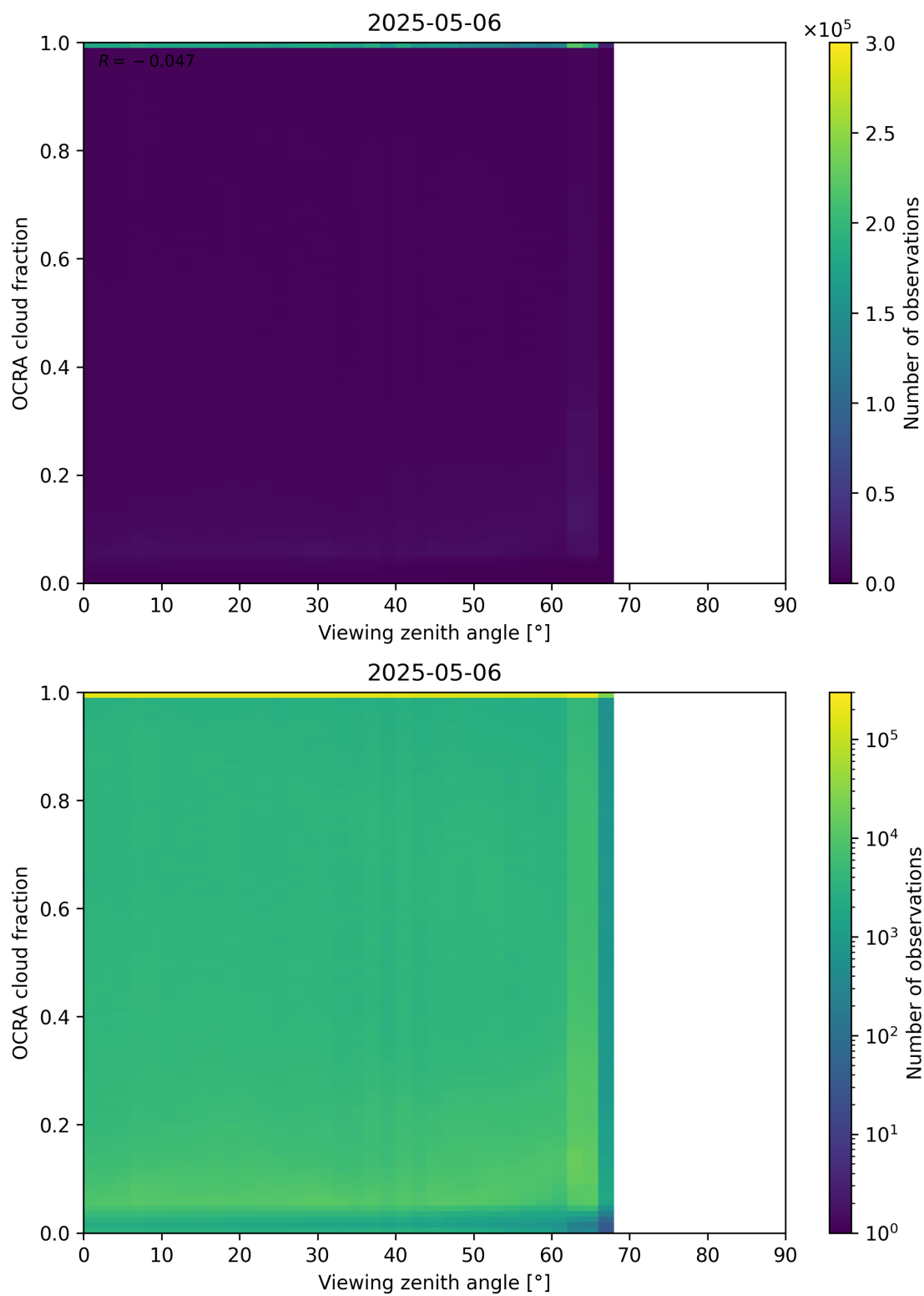
Figure 108: Scatter density plot of “Viewing zenith angle” against “OCRA cloud fraction” for 2025-05-05 to 2025-05-07.
