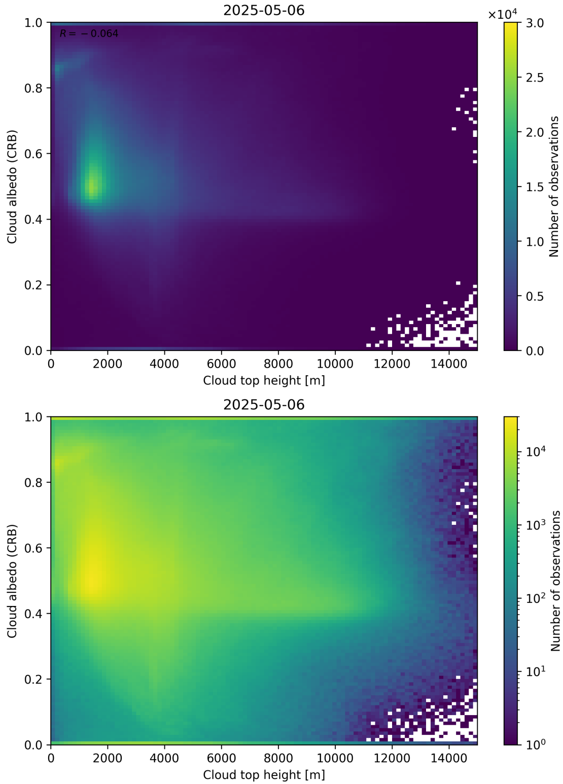
Figure 86: Scatter density plot of “Cloud top height” against “Cloud albedo (CRB)” for 2025-05-05 to 2025-05-07.
