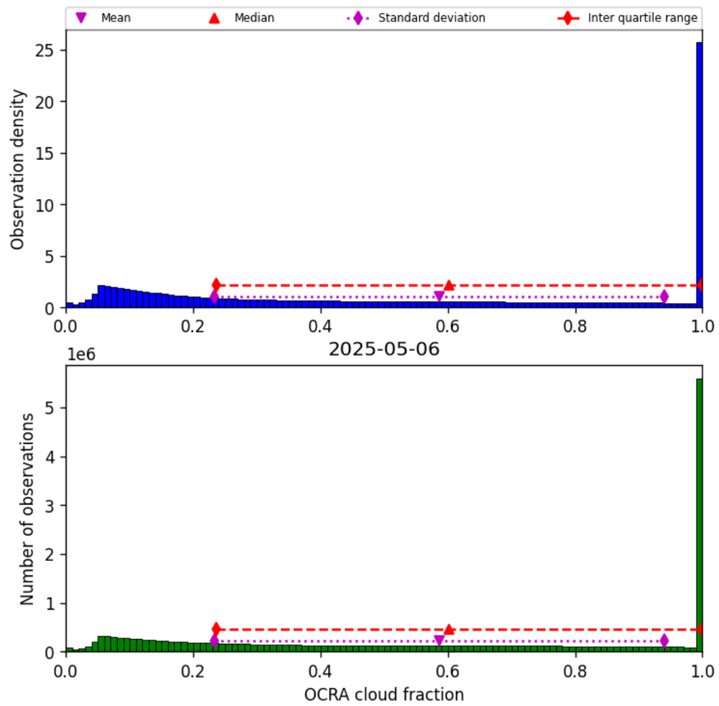
Figure 50: Histogram of “OCRA cloud fraction” for 2025-05-05 to 2025-05-07
