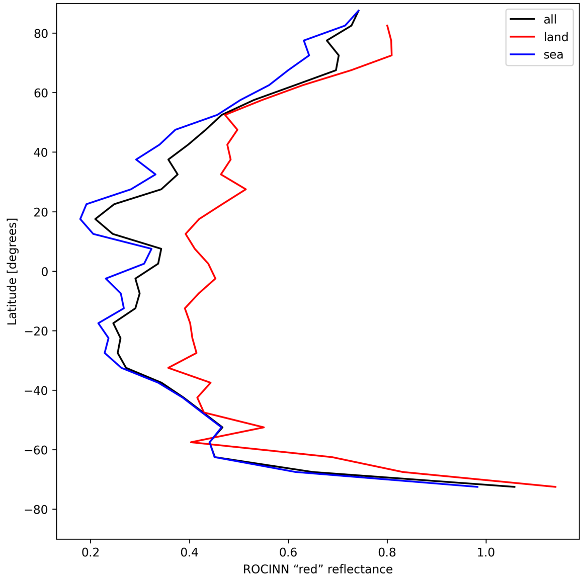
Figure 37: Zonal average of “ROCINN “red” reflectance” for 2025-05-05 to 2025-05-07.
