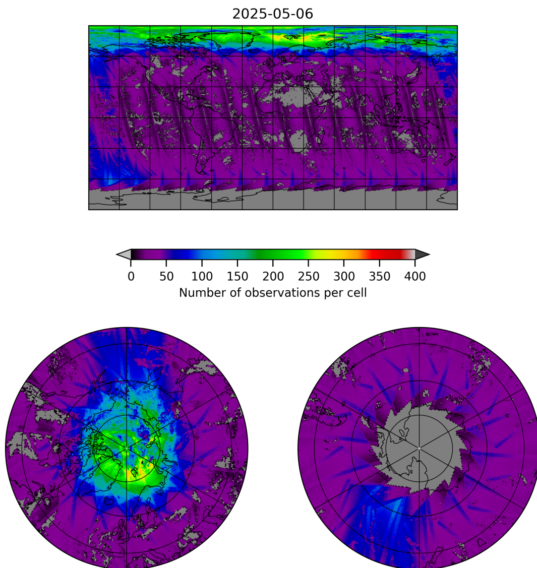
Figure 21: Map of the number of observations for 2025-05-05 to 2025-05-07
