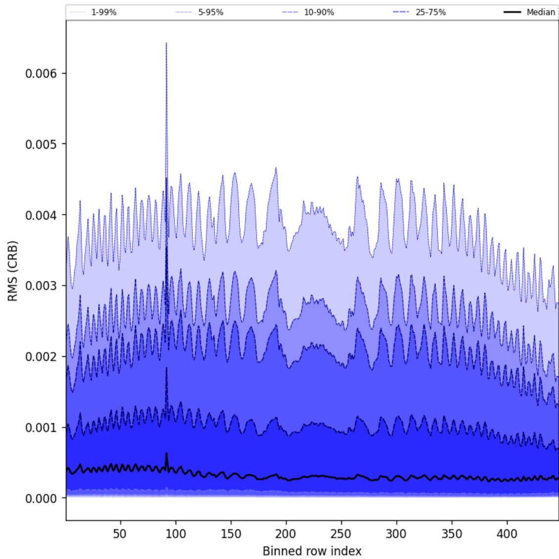
Figure 64: Along track statistics of “RMS (CRB)” for 2025-05-05 to 2025-05-07
