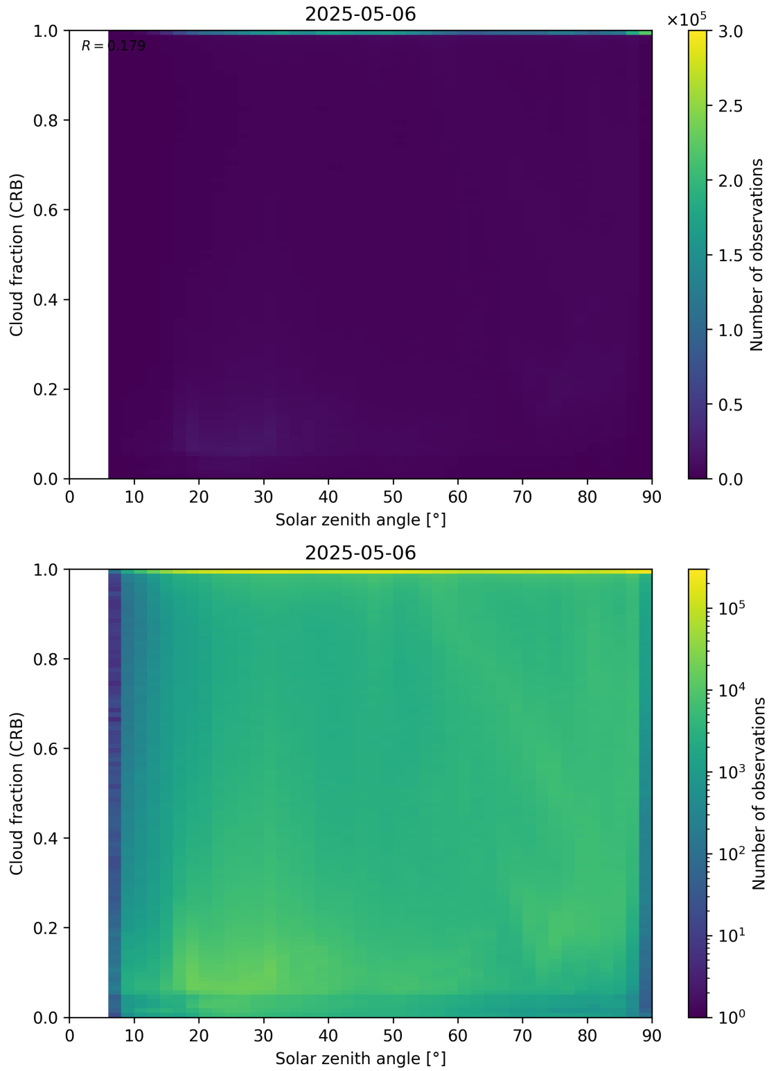
Figure 101: Scatter density plot of “Solar zenith angle” against “Cloud fraction (CRB)” for 2025-05-05 to 2025-05-07.
