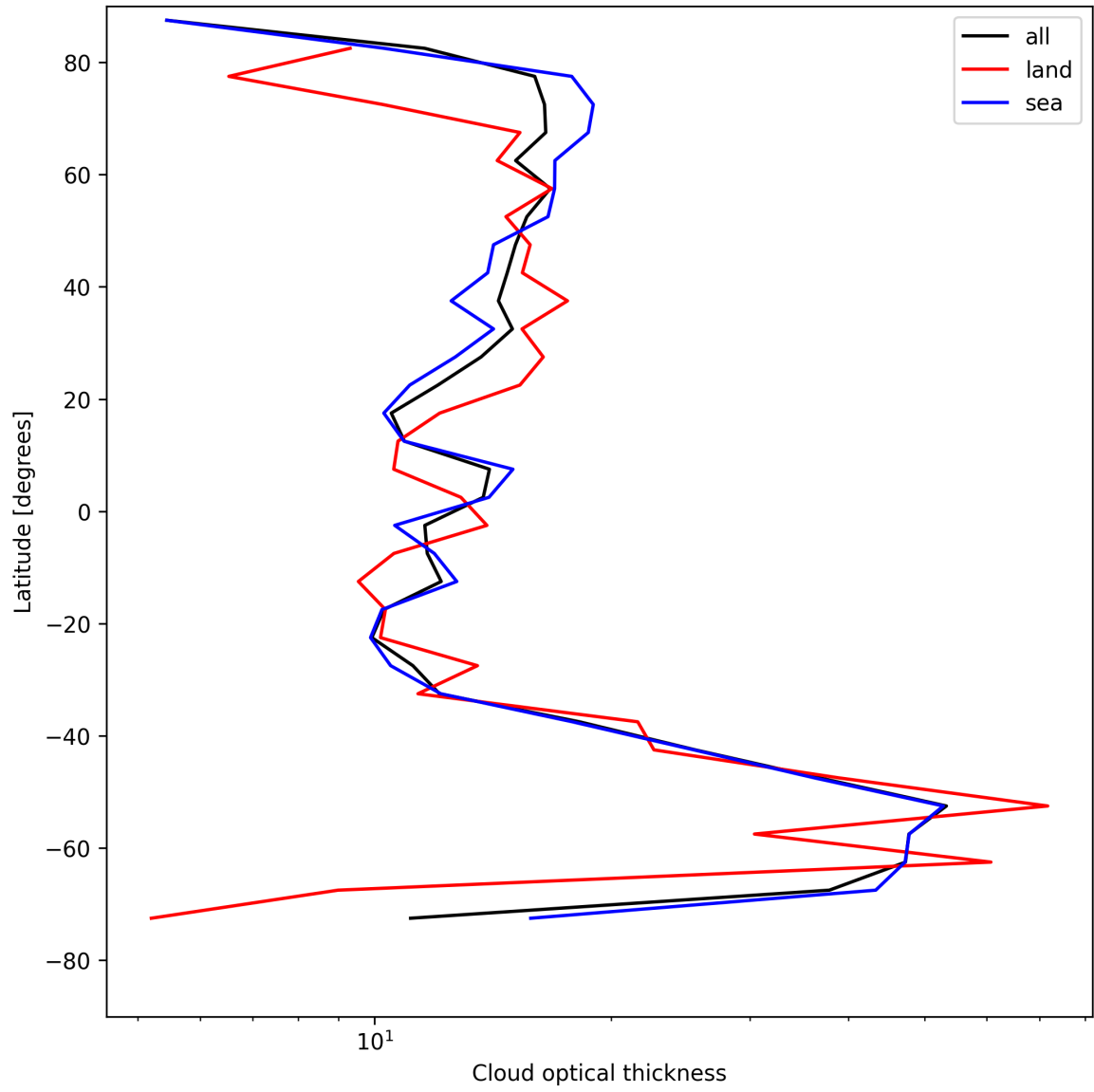
Figure 25: Zonal average of “Cloud optical thickness” for 2025-05-05 to 2025-05-07.
