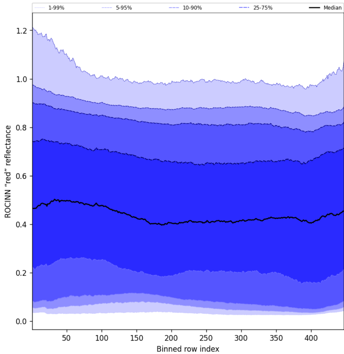
Figure 69: Along track statistics of “ROCINN “red” reflectance” for 2025-05-05 to 2025-05-07
