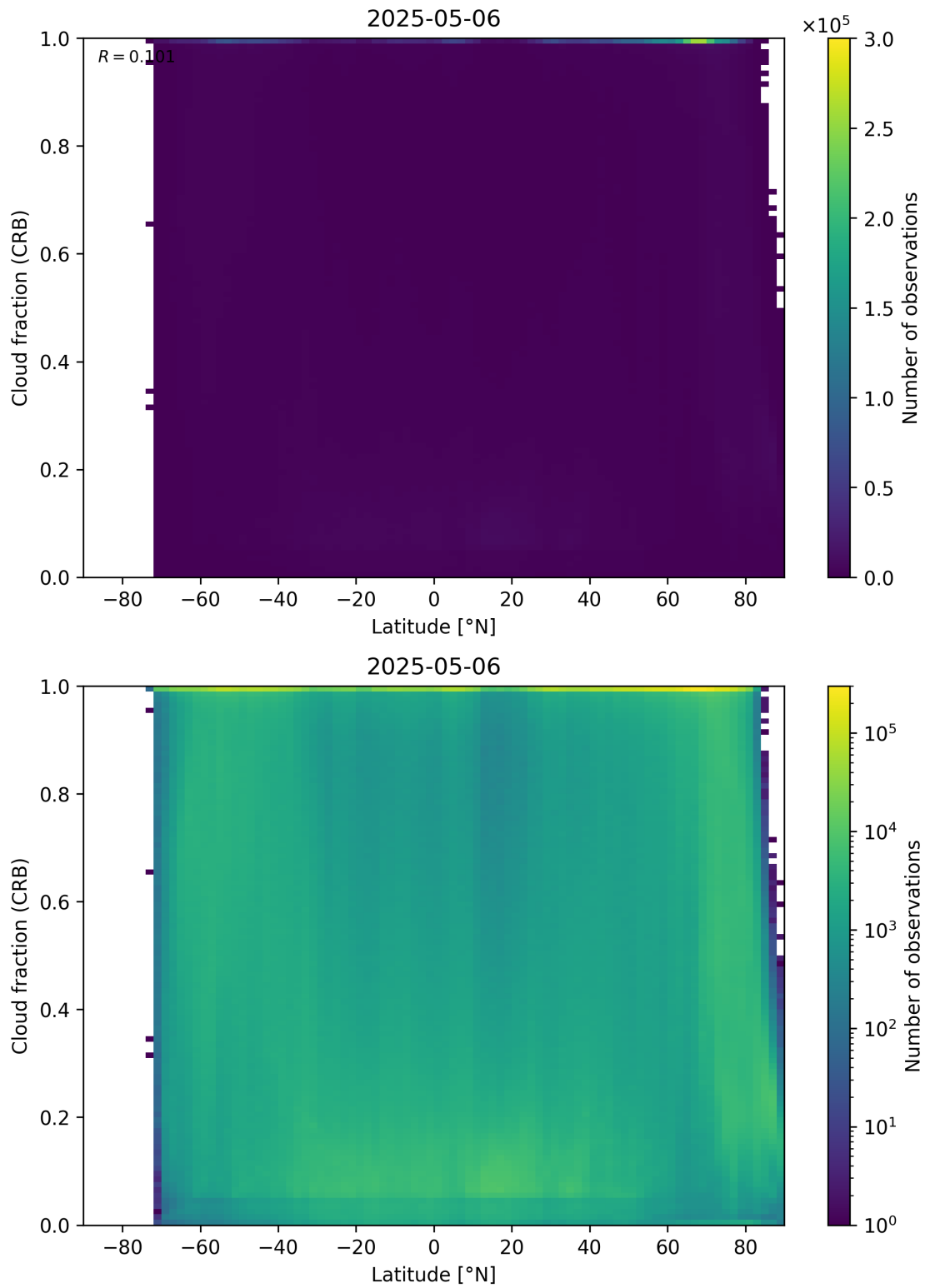
Figure 94: Scatter density plot of “Latitude” against “Cloud fraction (CRB)” for 2025-05-05 to 2025-05-07.
