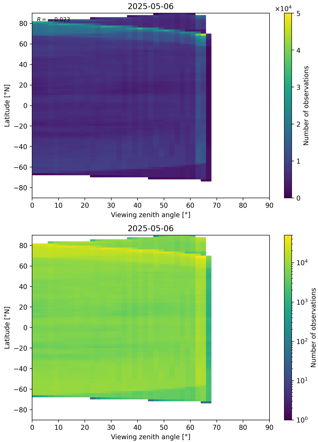
Figure 113: Scatter density plot of “Viewing zenith angle” against “Latitude” for 2025-05-05 to 2025-05-07.
