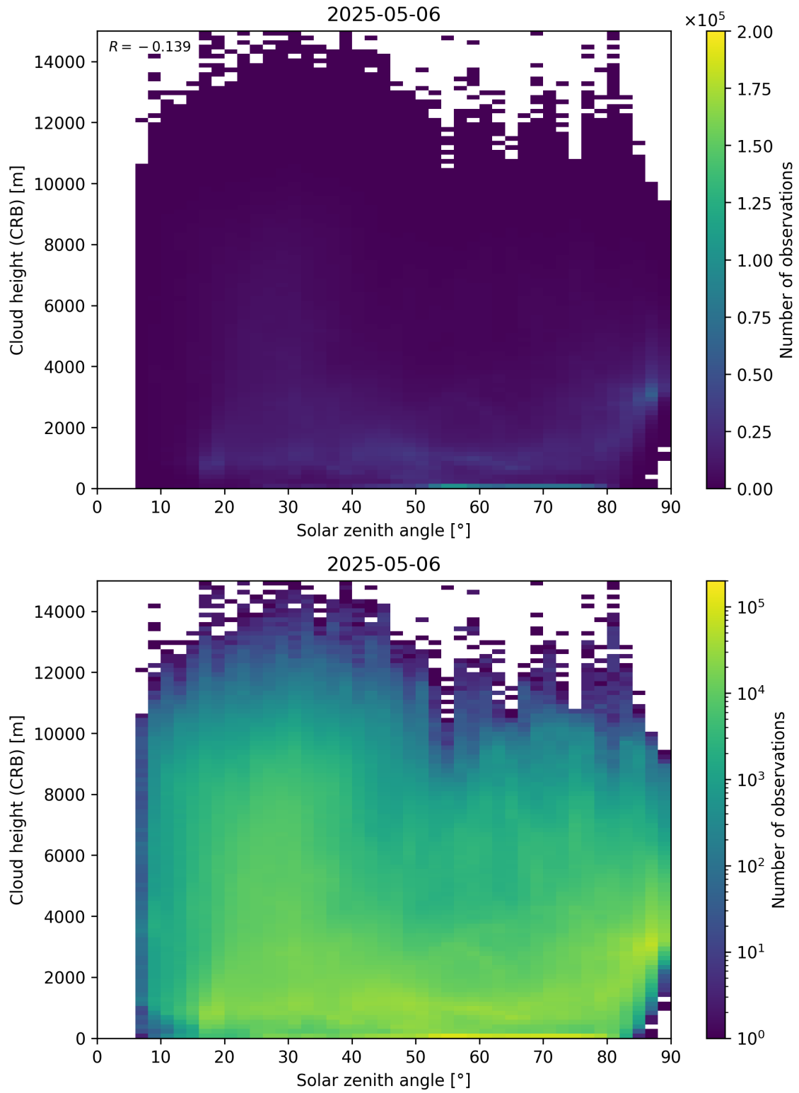
Figure 102: Scatter density plot of “Solar zenith angle” against “Cloud height (CRB)” for 2025-05-05 to 2025-05-07.
