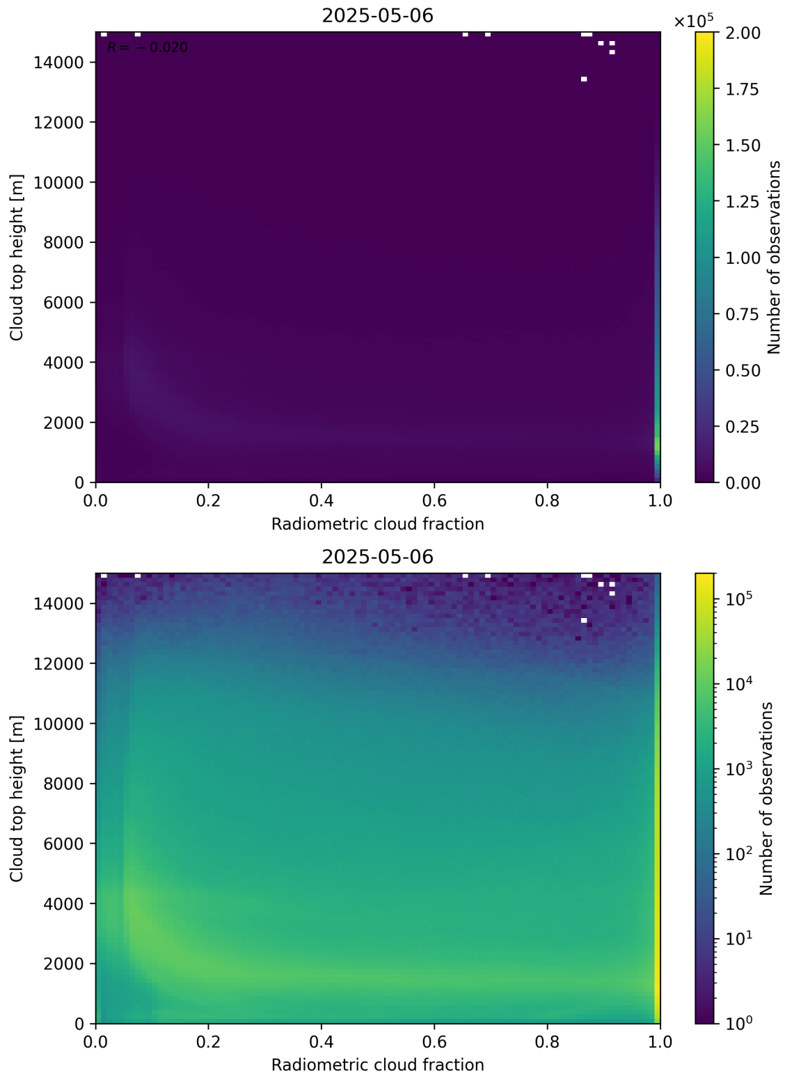
Figure 76: Scatter density plot of “Radiometric cloud fraction” against “Cloud top height” for 2025-05-05 to 2025-05-07.
