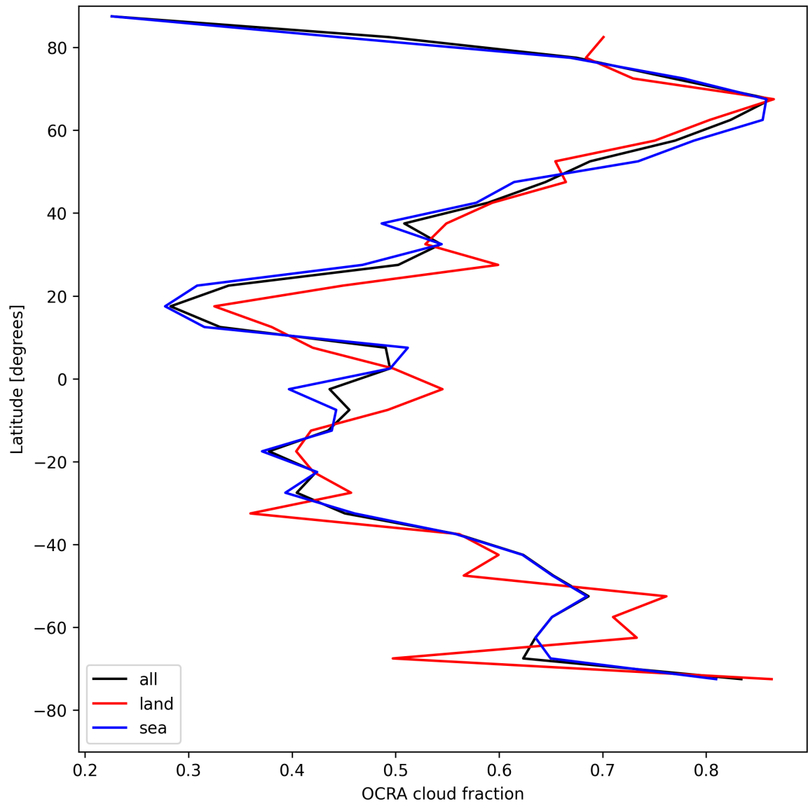
Figure 34: Zonal average of “OCRA cloud fraction” for 2025-05-05 to 2025-05-07.
