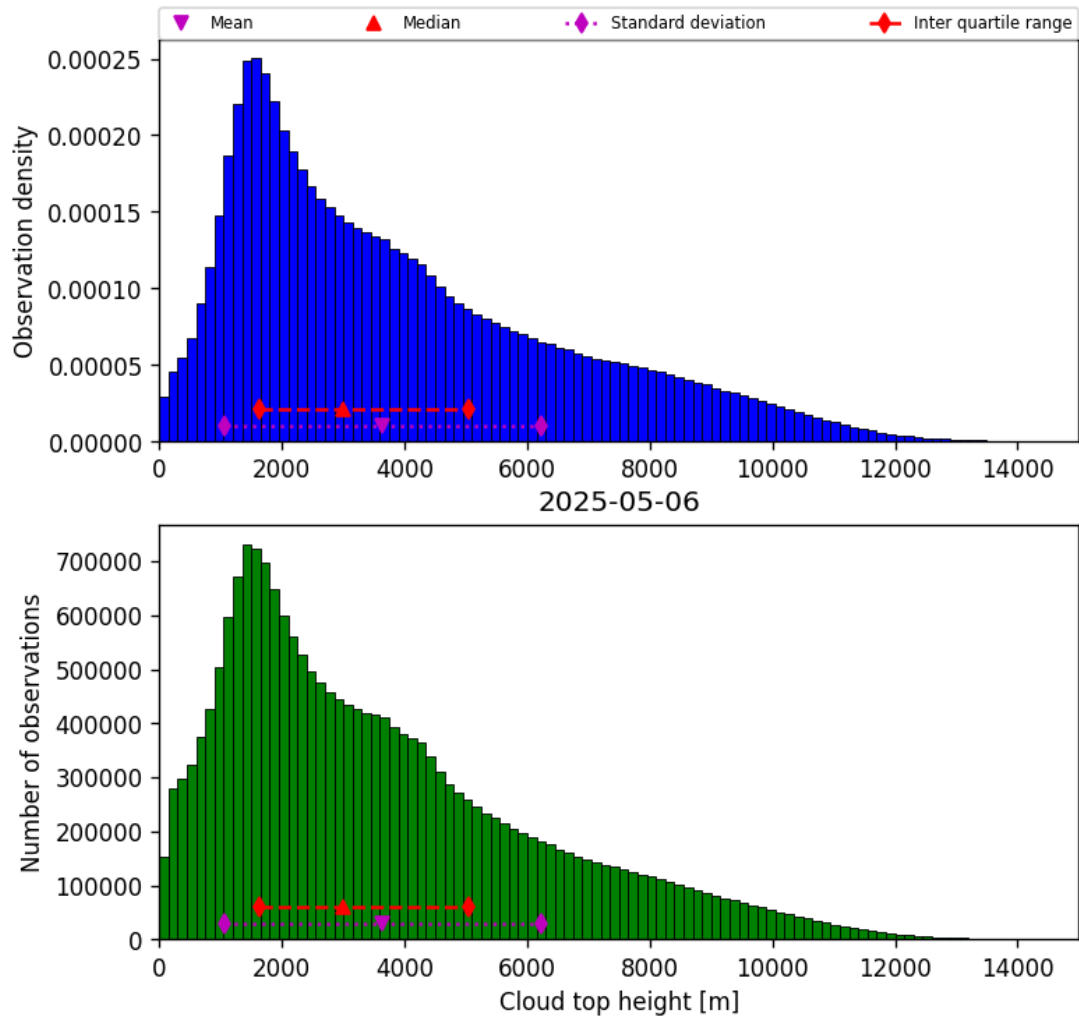
Figure 40: Histogram of “Cloud top height” for 2025-05-05 to 2025-05-07
