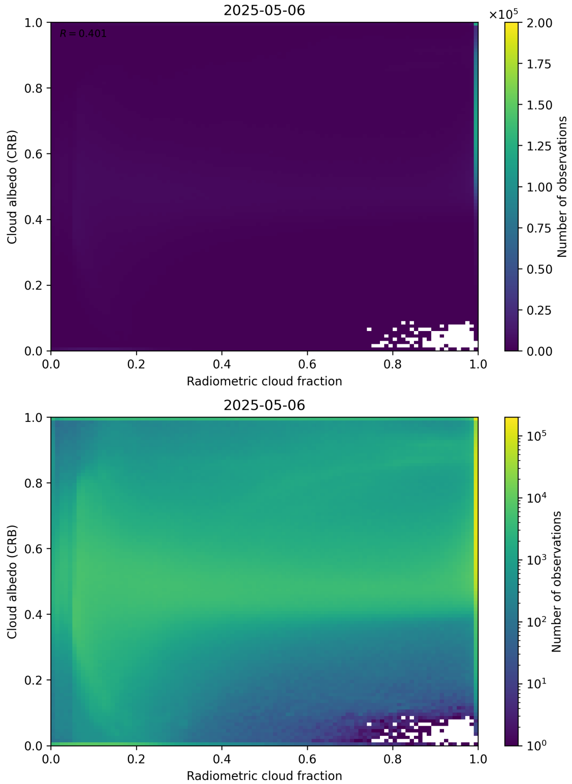
Figure 71: Scatter density plot of “Radiometric cloud fraction” against “Cloud albedo (CRB)” for 2025-05-05 to 2025-05-07.
