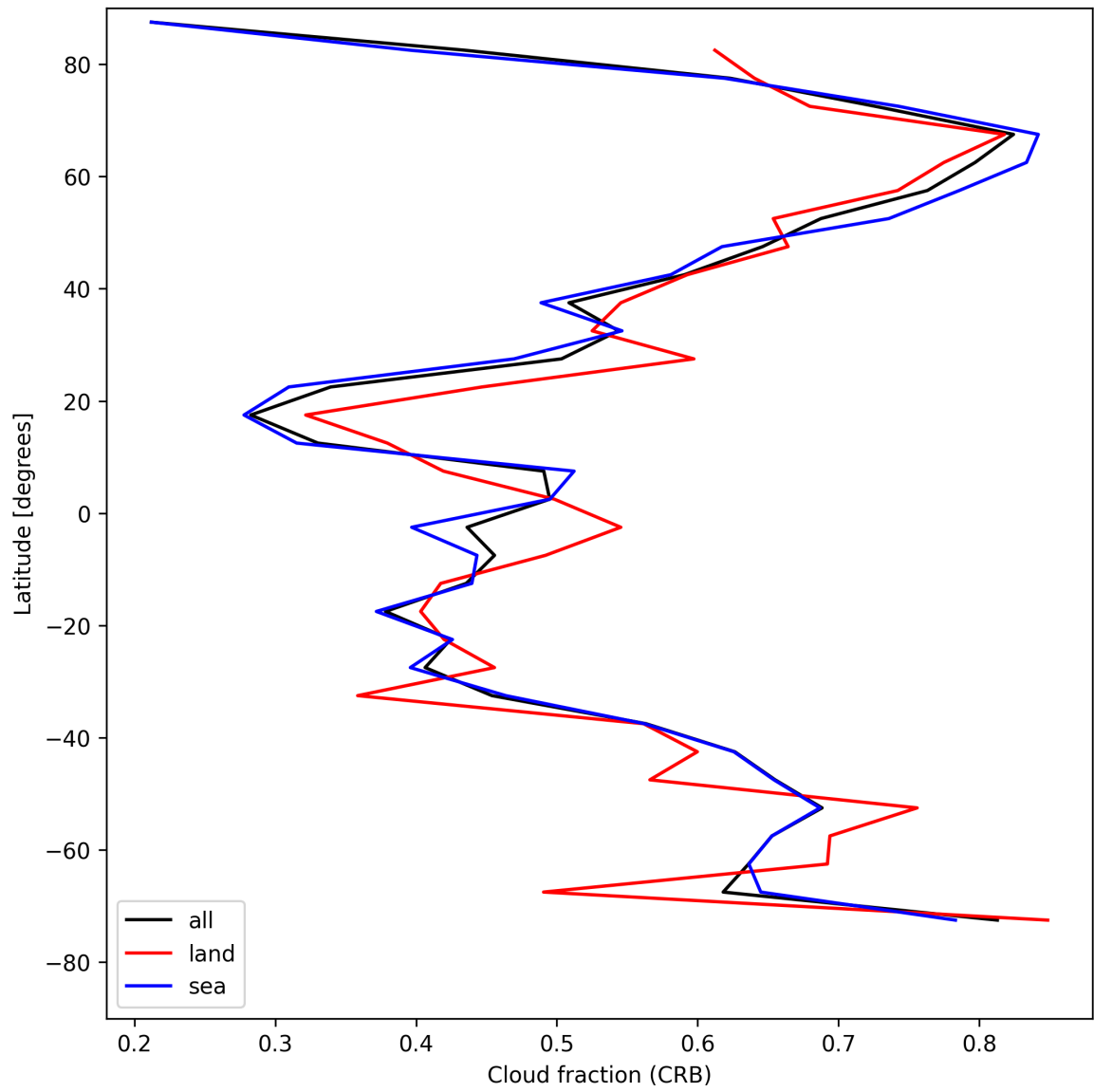
Figure 26: Zonal average of “Cloud fraction (CRB)” for 2025-05-05 to 2025-05-07.
