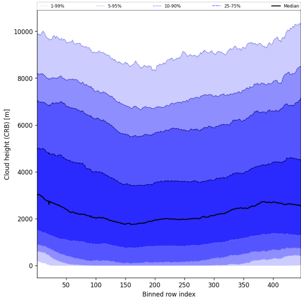
Figure 59: Along track statistics of “Cloud height (CRB)” for 2025-05-05 to 2025-05-07
