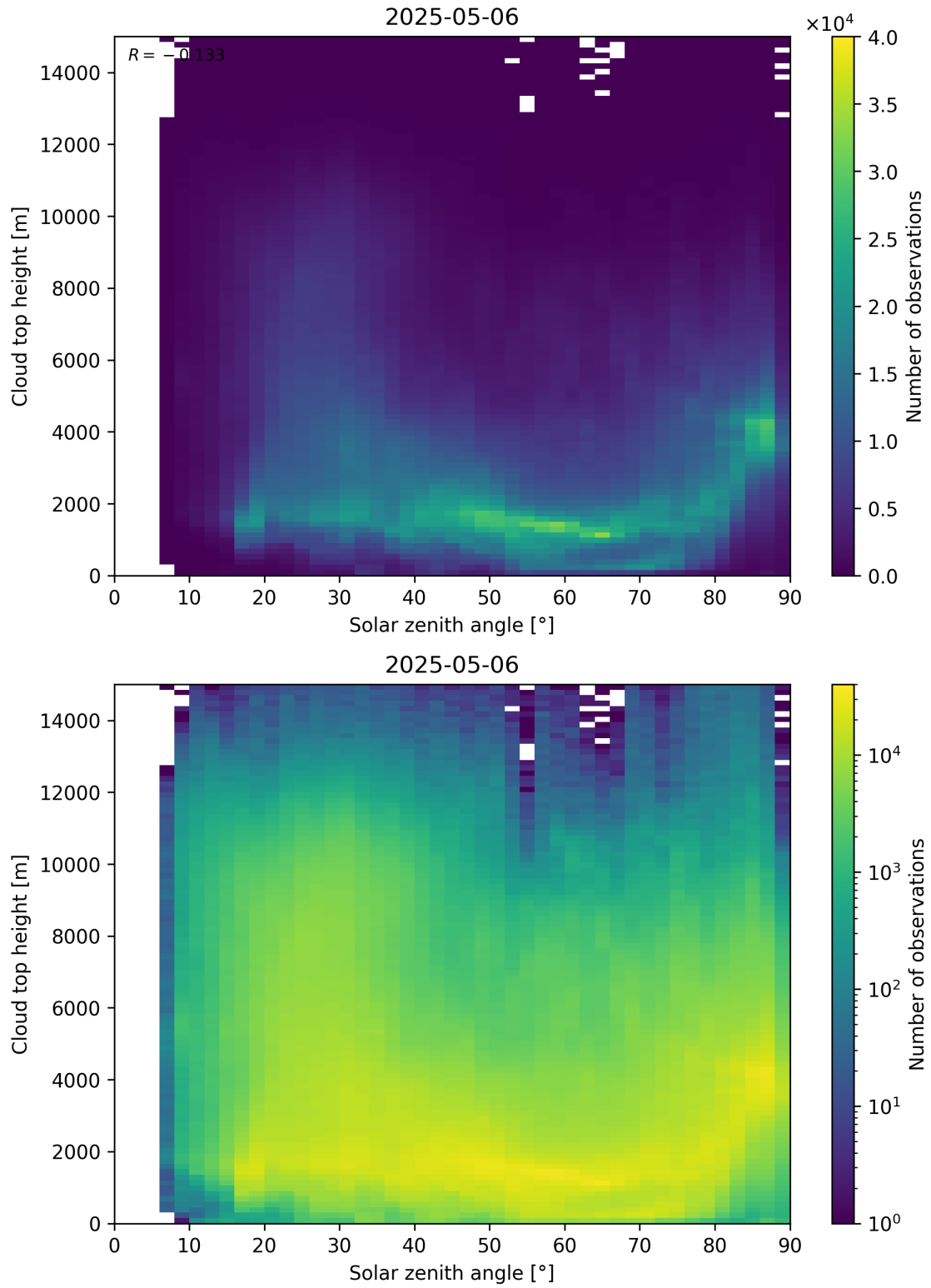
Figure 104: Scatter density plot of “Solar zenith angle” against “Cloud top height” for 2025-05-05 to 2025-05-07.
