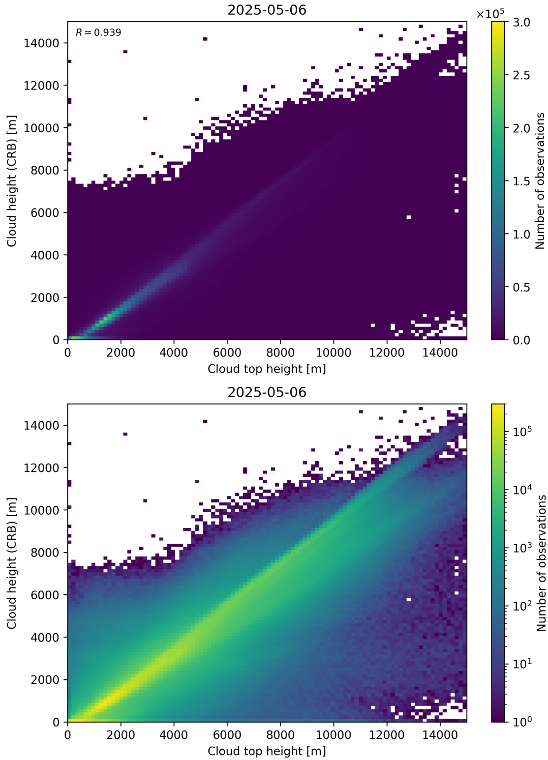
Figure 89: Scatter density plot of “Cloud top height” against “Cloud height (CRB)” for 2025-05-05 to 2025-05-07.
