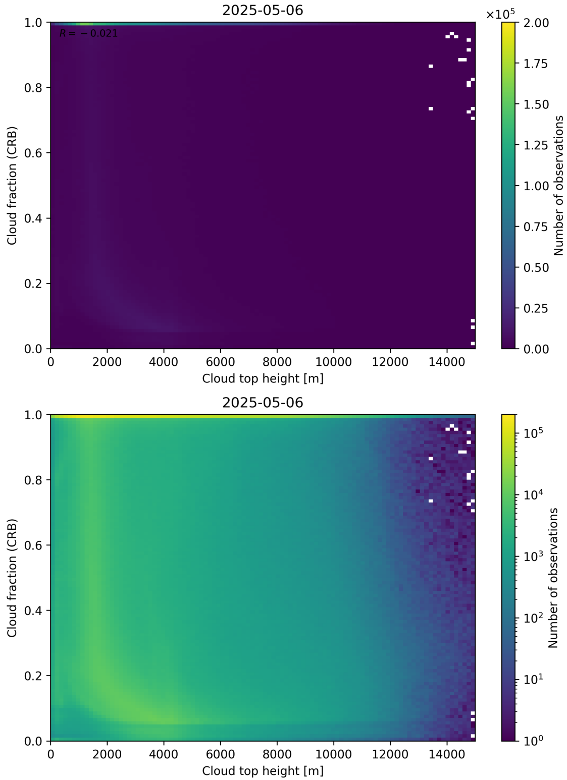
Figure 88: Scatter density plot of “Cloud top height” against “Cloud fraction (CRB)” for 2025-05-05 to 2025-05-07.
