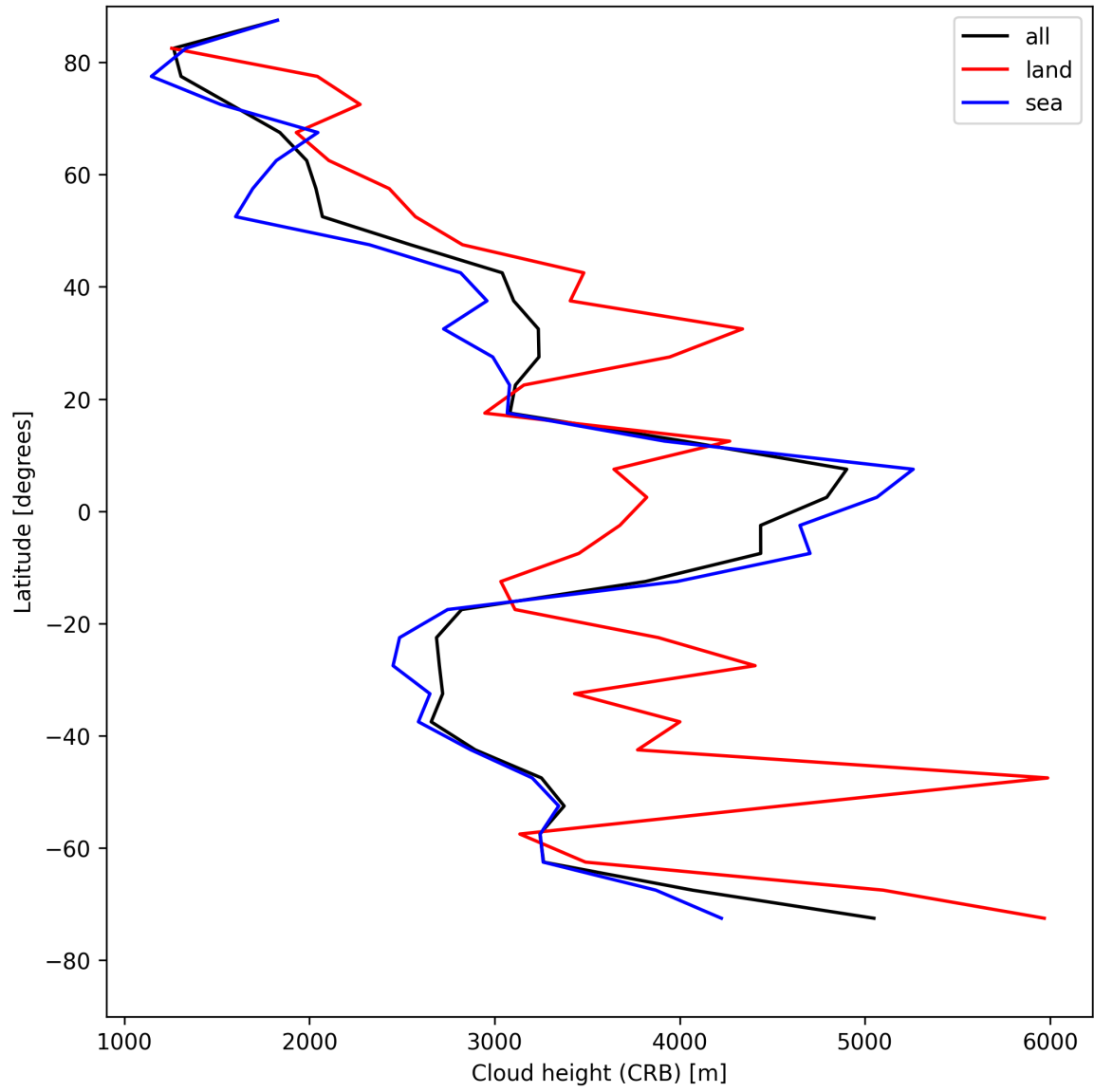
Figure 27: Zonal average of “Cloud height (CRB)” for 2025-05-05 to 2025-05-07.
