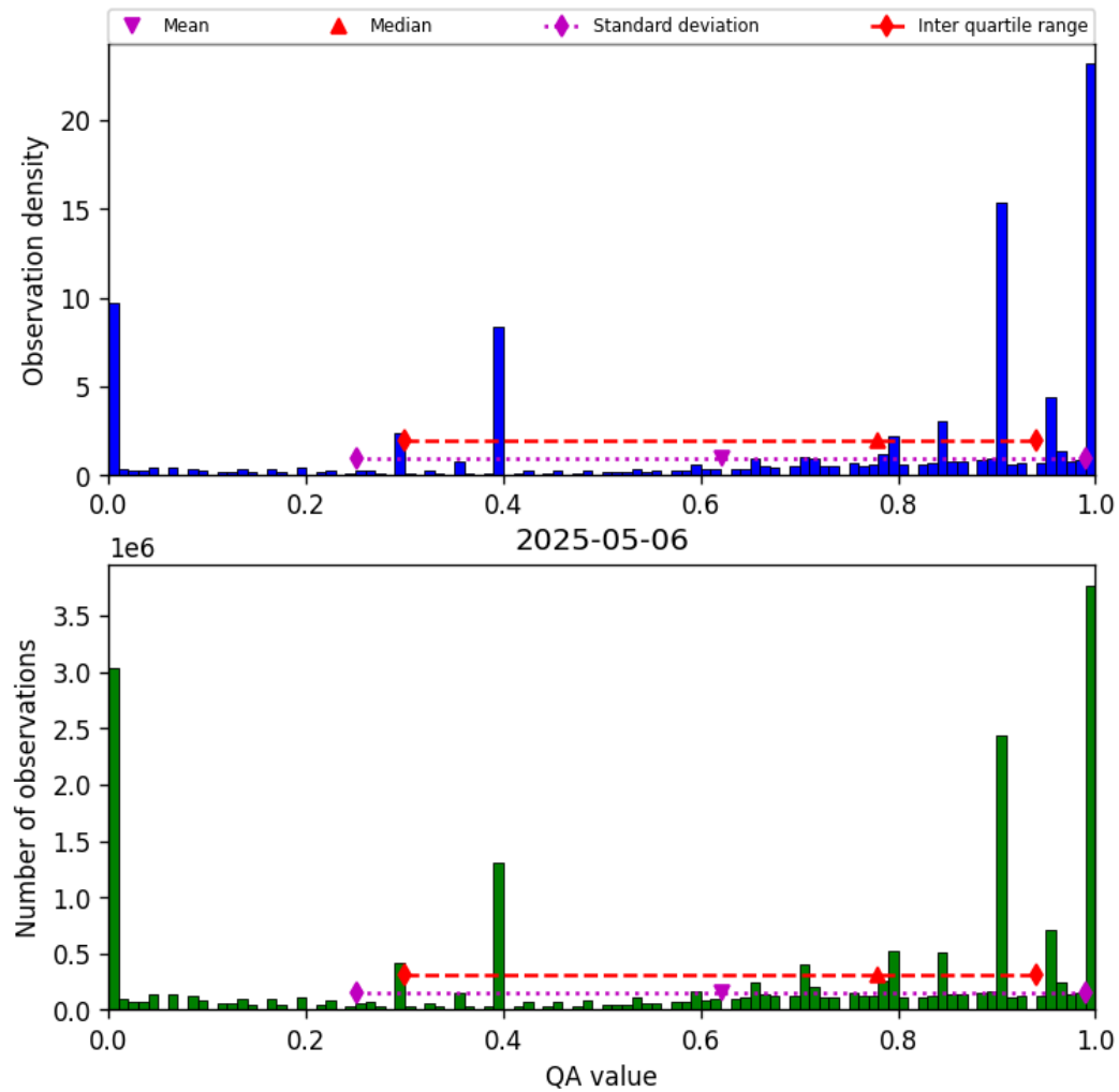
Figure 38: Histogram of “QA value” for 2025-05-05 to 2025-05-07
