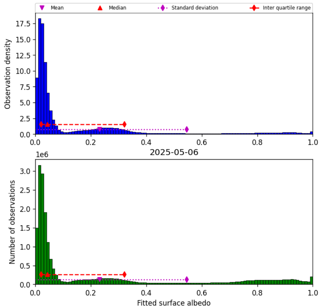
Figure 45: Histogram of “Fitted surface albedo” for 2025-05-05 to 2025-05-07
