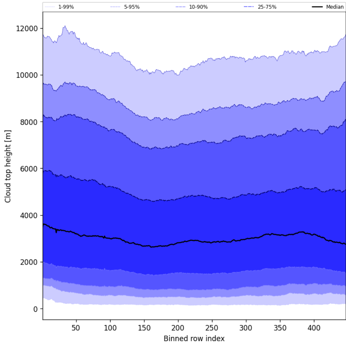
Figure 56: Along track statistics of “Cloud top height” for 2025-05-05 to 2025-05-07
