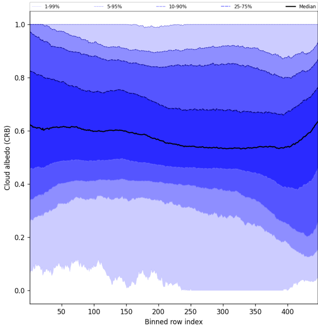
Figure 60: Along track statistics of “Cloud albedo (CRB)” for 2025-05-05 to 2025-05-07
