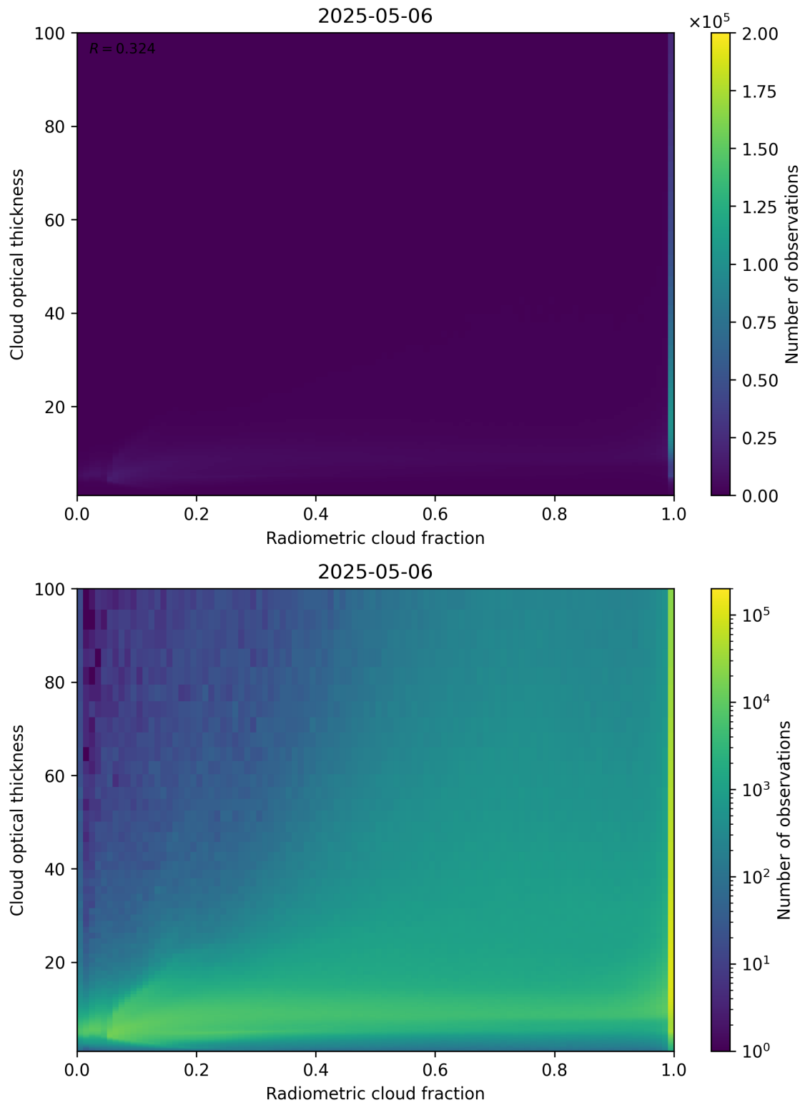
Figure 75: Scatter density plot of “Radiometric cloud fraction” against “Cloud optical thickness” for 2025-05-05 to 2025-05-07.
