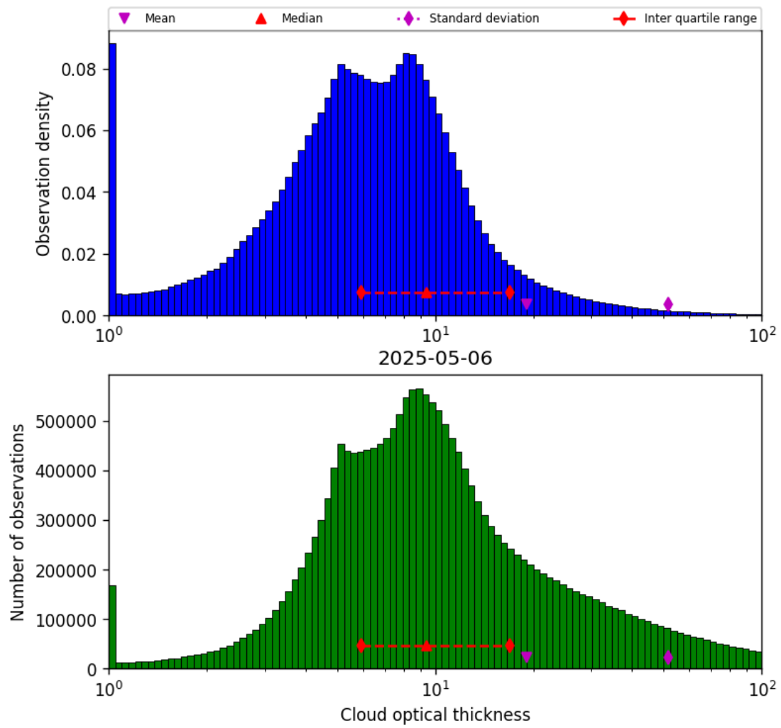
Figure 41: Histogram of “Cloud optical thickness” for 2025-05-05 to 2025-05-07
