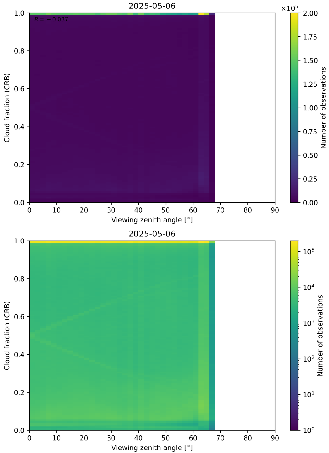
Figure 109: Scatter density plot of “Viewing zenith angle” against “Cloud fraction (CRB)” for 2025-05-05 to 2025-05-07.
