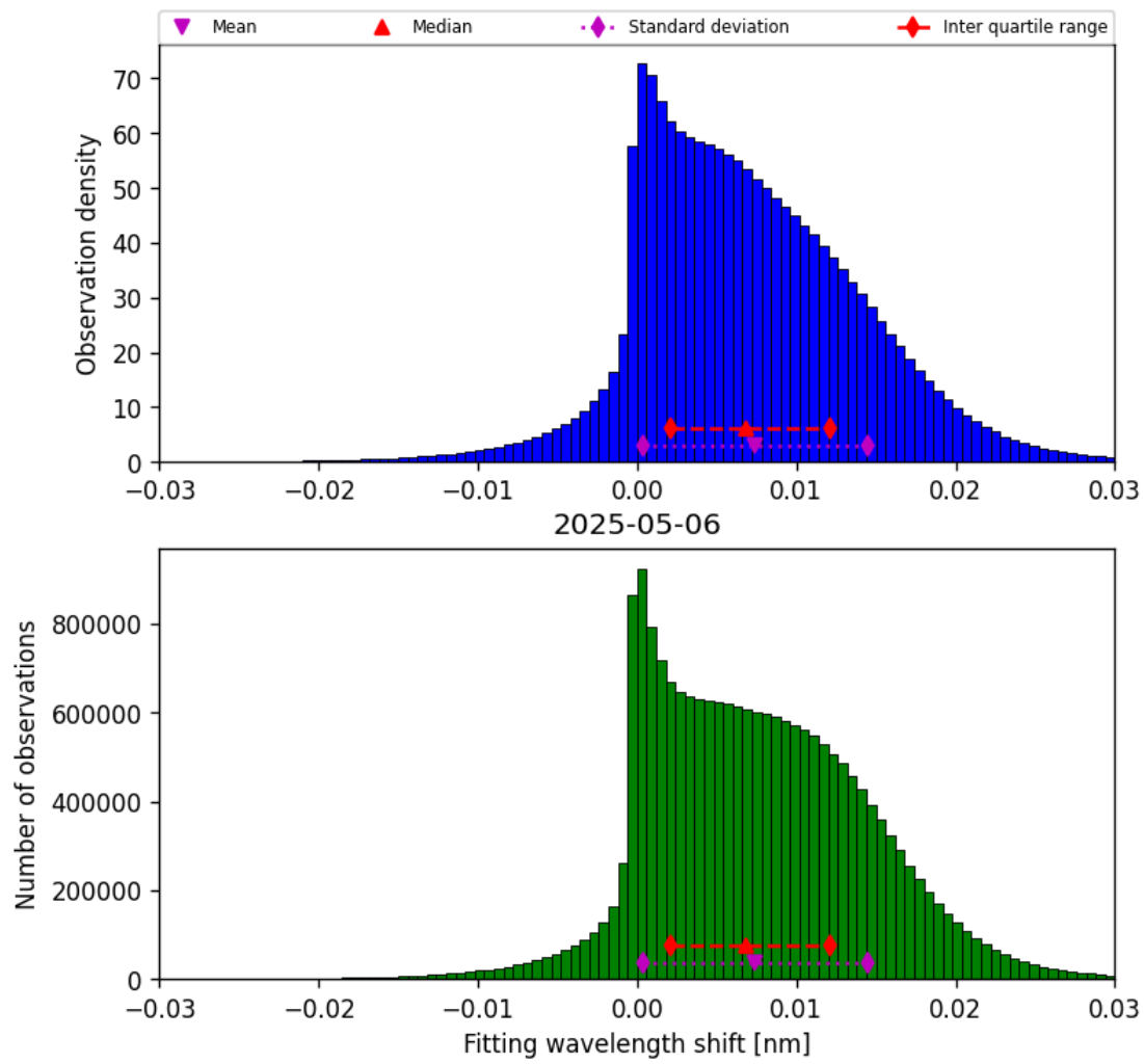
Figure 49: Histogram of “Fitting wavelength shift” for 2025-05-05 to 2025-05-07
