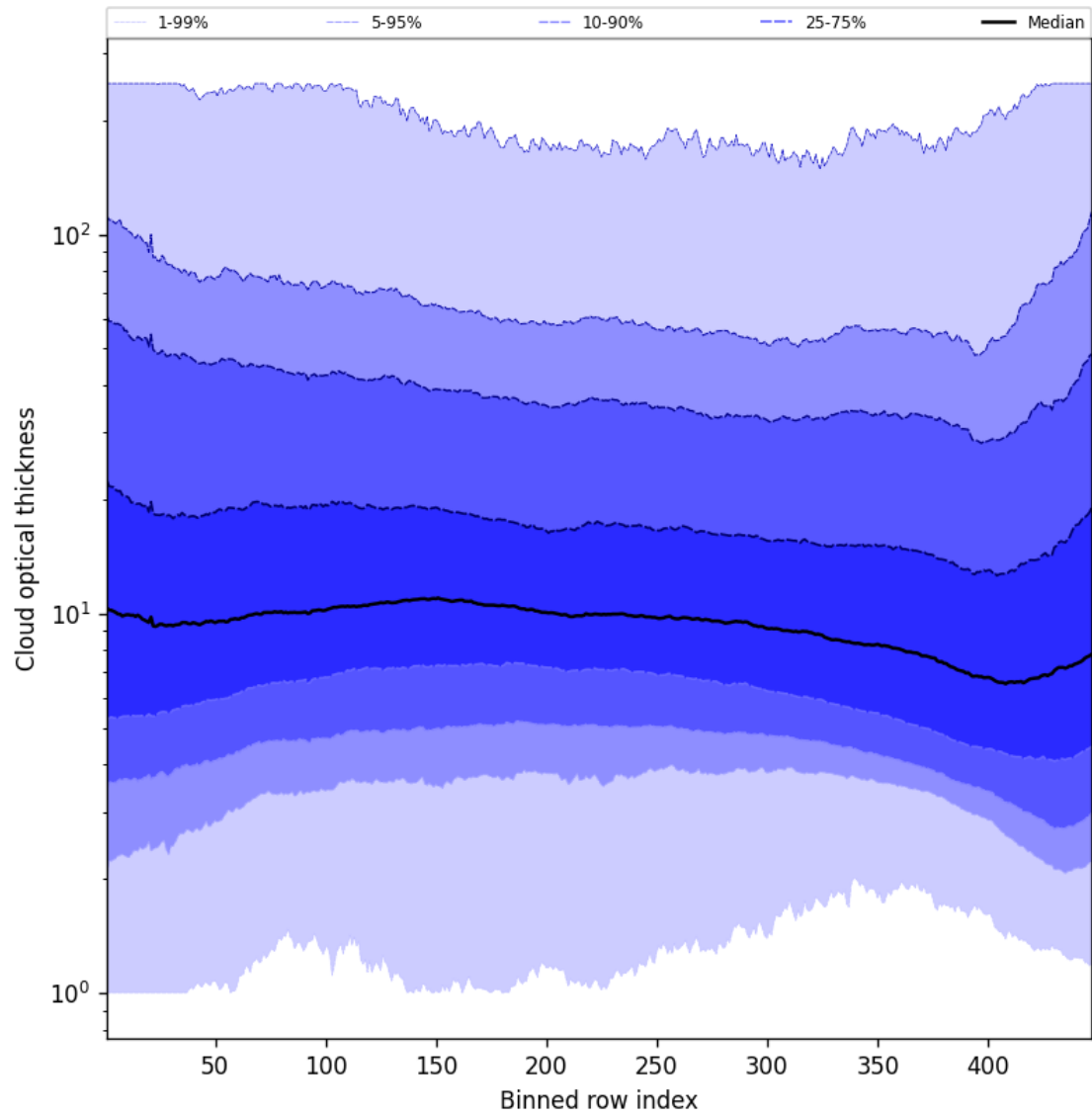
Figure 57: Along track statistics of “Cloud optical thickness” for 2025-05-05 to 2025-05-07
