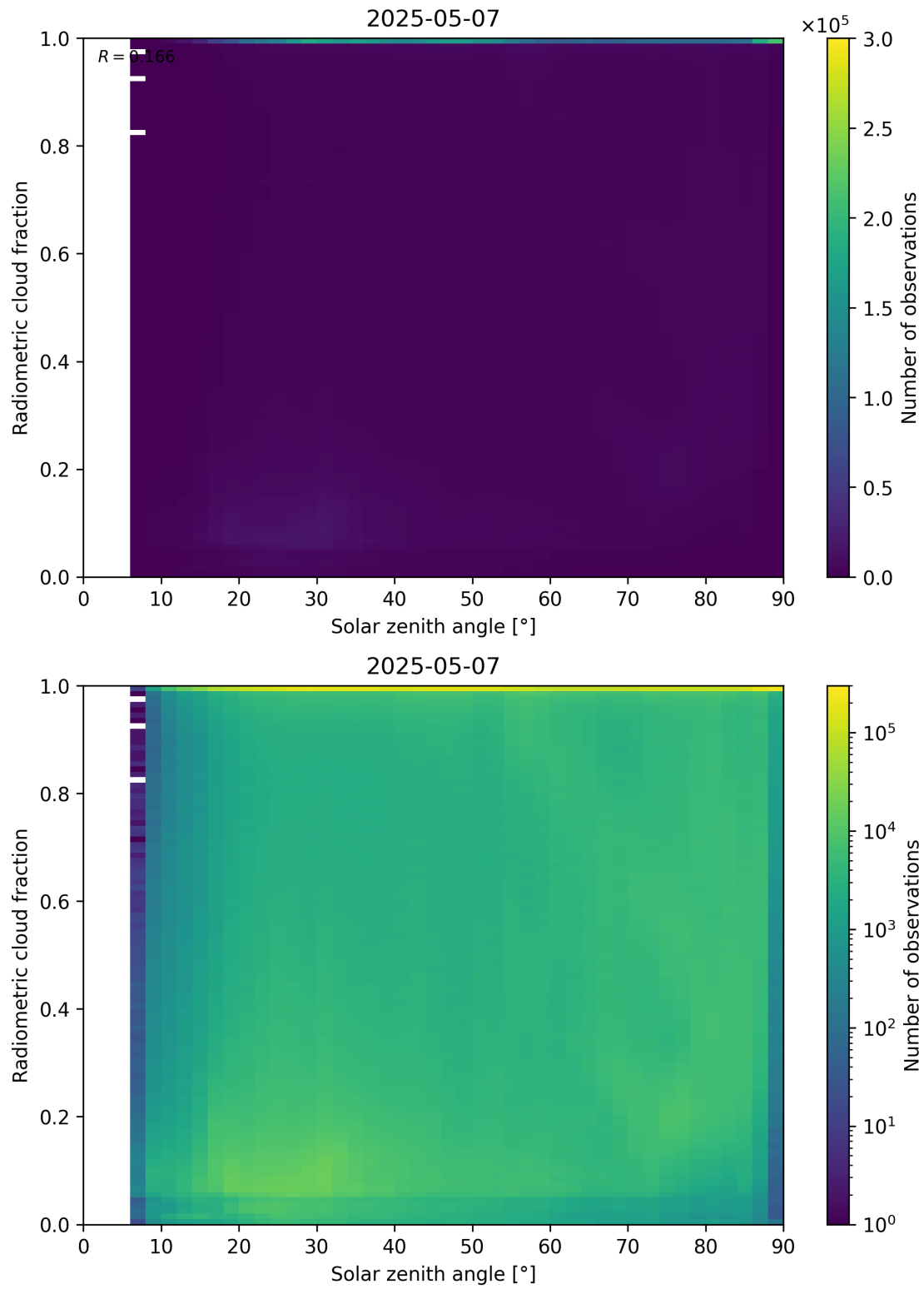
Figure 99: Scatter density plot of “Solar zenith angle” against “Radiometric cloud fraction” for 2025-05-06 to 2025-05-08.
