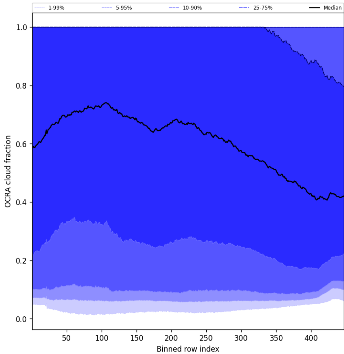
Figure 66: Along track statistics of “OCRA cloud fraction” for 2025-05-06 to 2025-05-08
