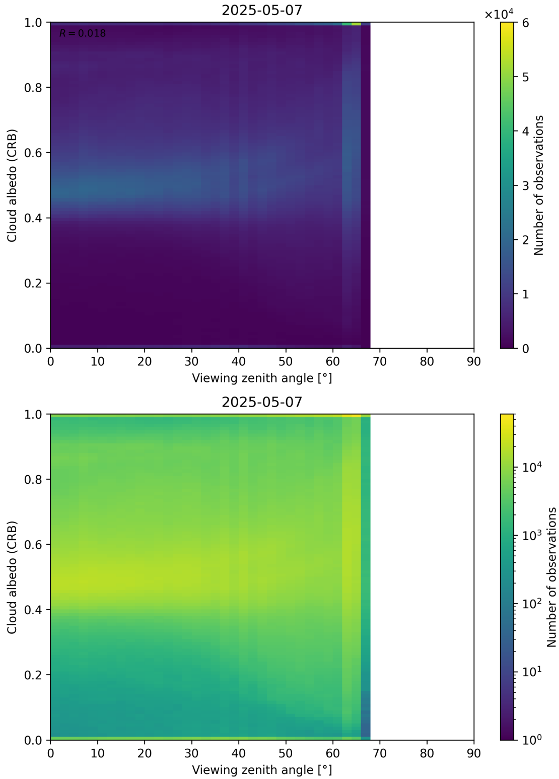
Figure 106: Scatter density plot of “Viewing zenith angle” against “Cloud albedo (CRB)” for 2025-05-06 to 2025-05-08.
