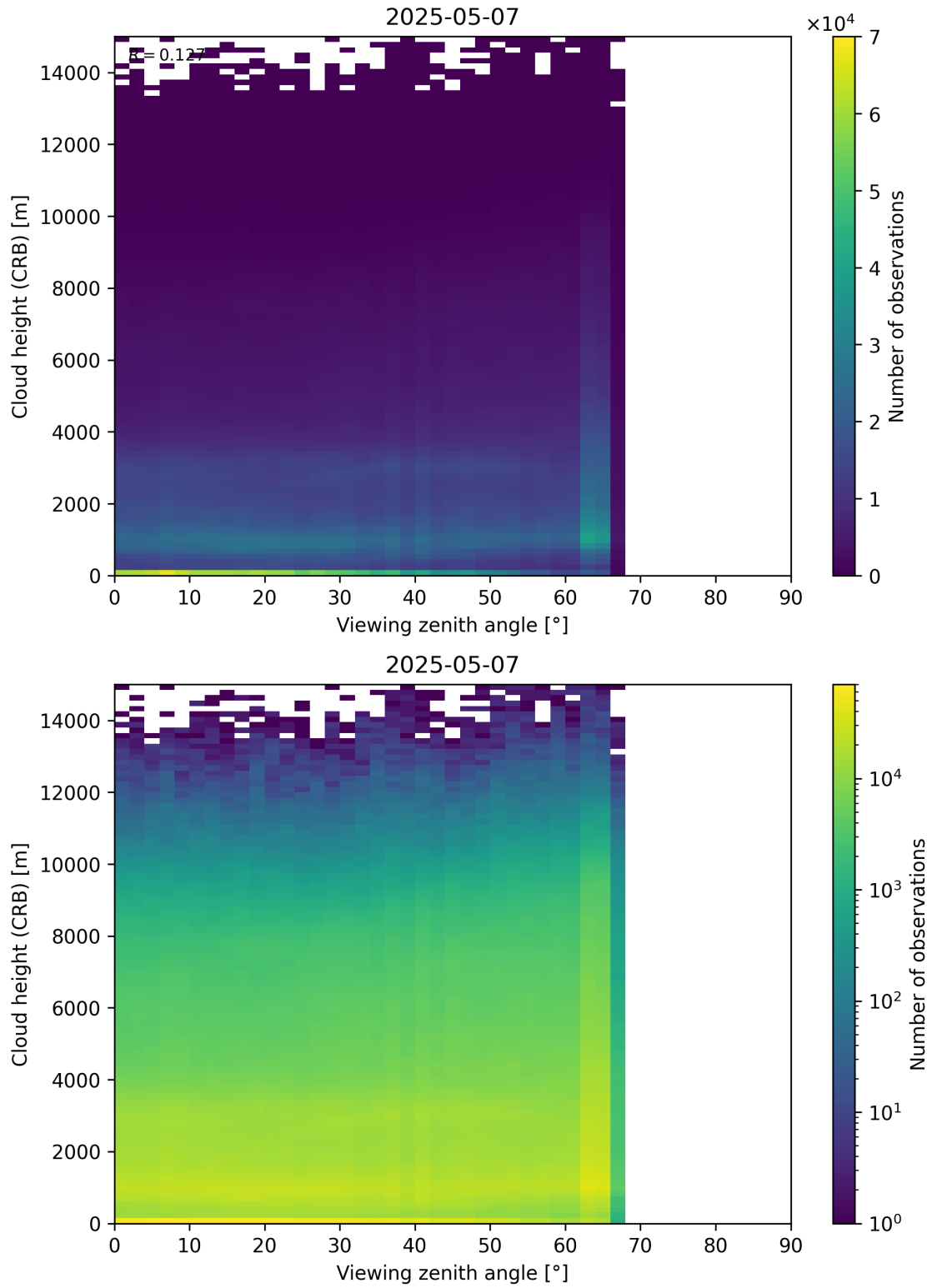
Figure 110: Scatter density plot of “Viewing zenith angle” against “Cloud height (CRB)” for 2025-05-06 to 2025-05-08.
