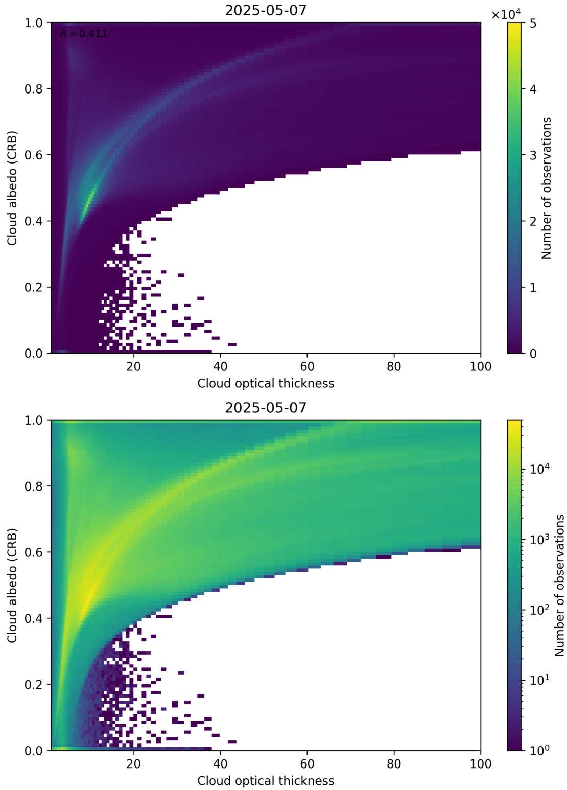
Figure 82: Scatter density plot of “Cloud optical thickness” against “Cloud albedo (CRB)” for 2025-05-06 to 2025-05-08.
