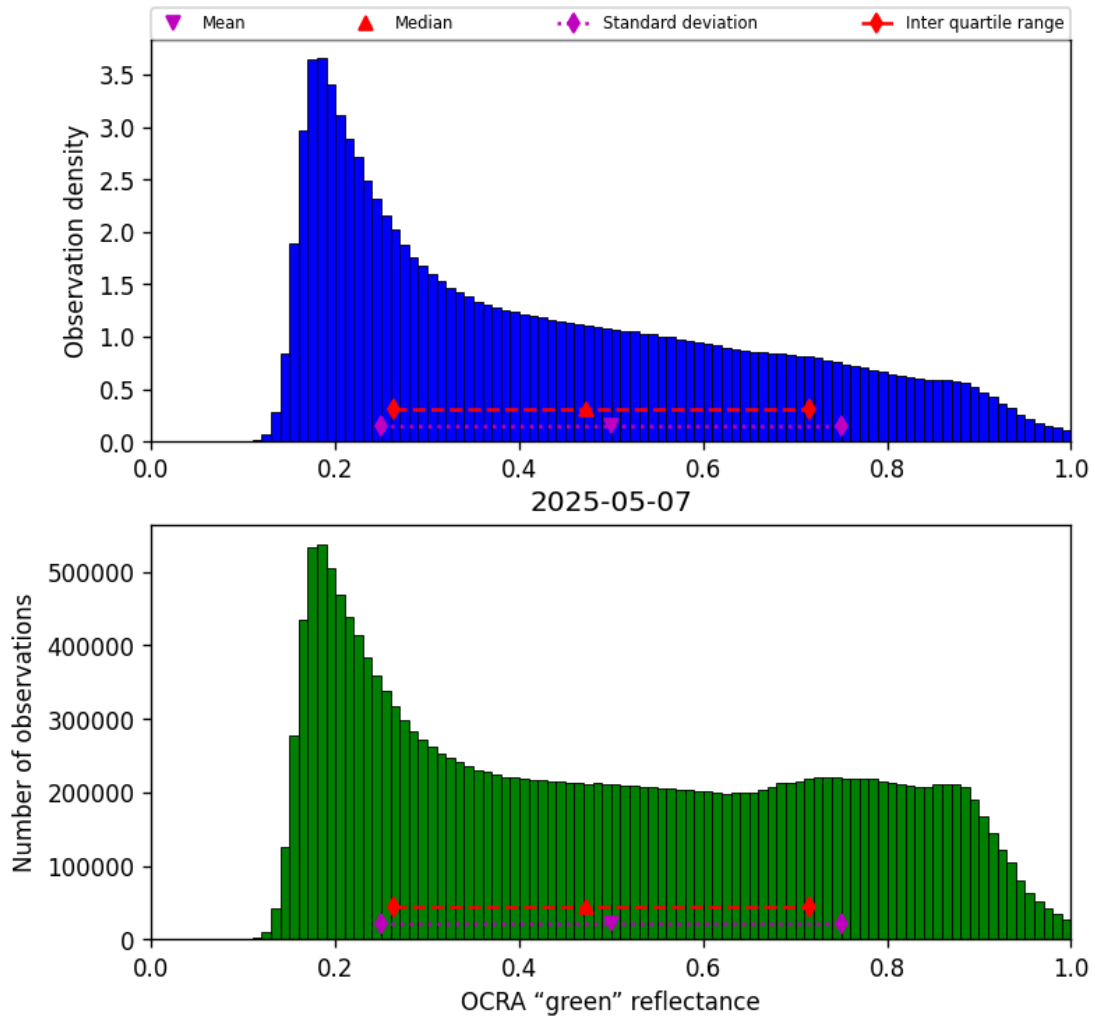
Figure 52: Histogram of “OCRA “green” reflectance” for 2025-05-06 to 2025-05-08
