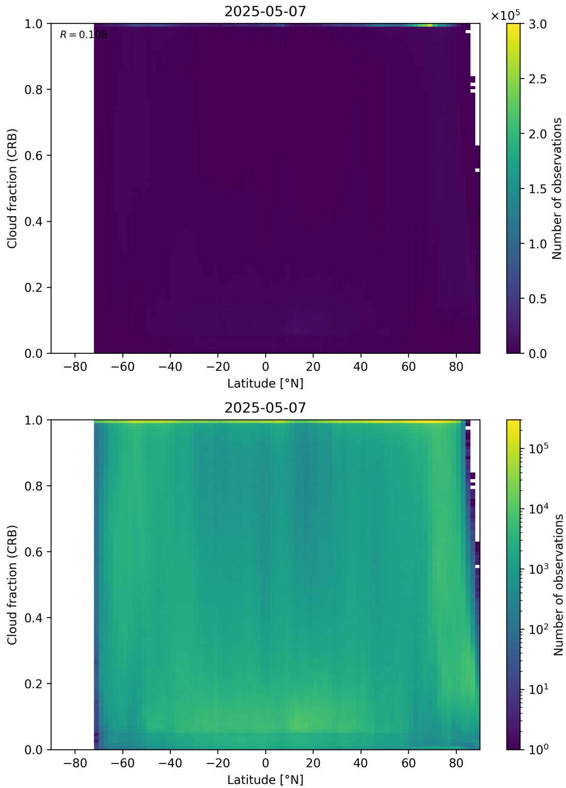
Figure 94: Scatter density plot of “Latitude” against “Cloud fraction (CRB)” for 2025-05-06 to 2025-05-08.
