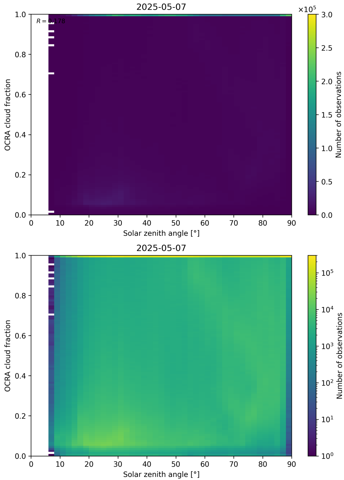
Figure 100: Scatter density plot of “Solar zenith angle” against “OCRA cloud fraction” for 2025-05-06 to 2025-05-08.
