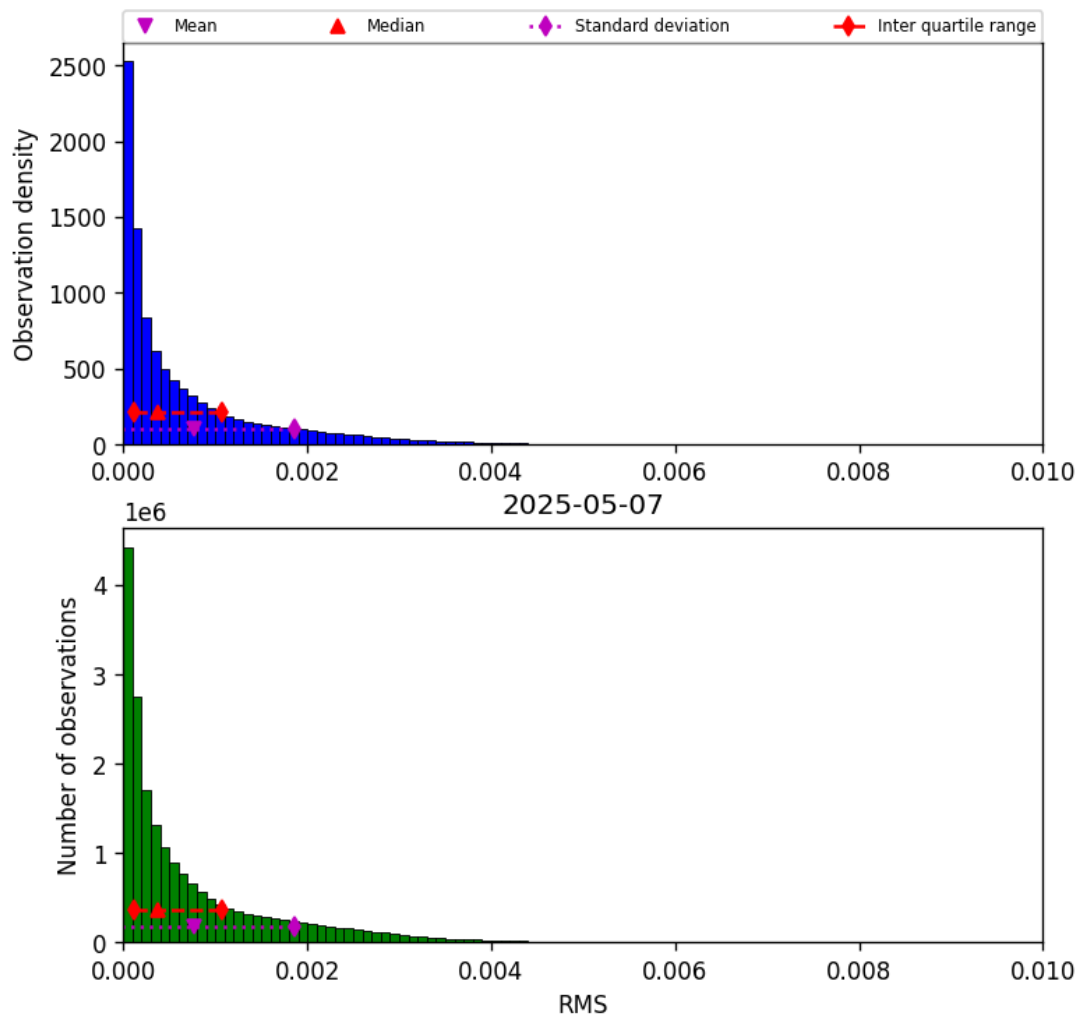
Figure 47: Histogram of “RMS” for 2025-05-06 to 2025-05-08
