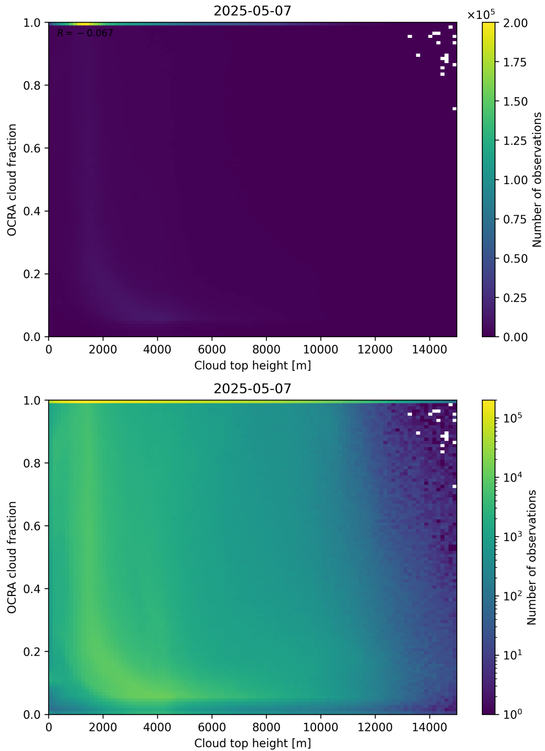
Figure 87: Scatter density plot of “Cloud top height” against “OCRA cloud fraction” for 2025-05-06 to 2025-05-08.
