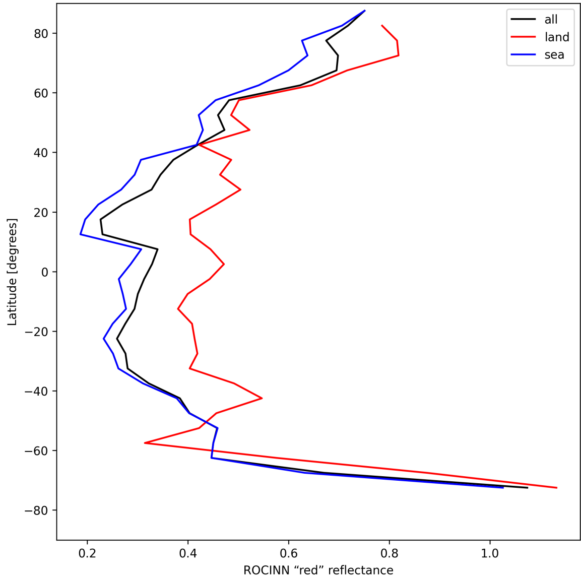
Figure 37: Zonal average of “ROCINN “red” reflectance” for 2025-05-06 to 2025-05-08.
