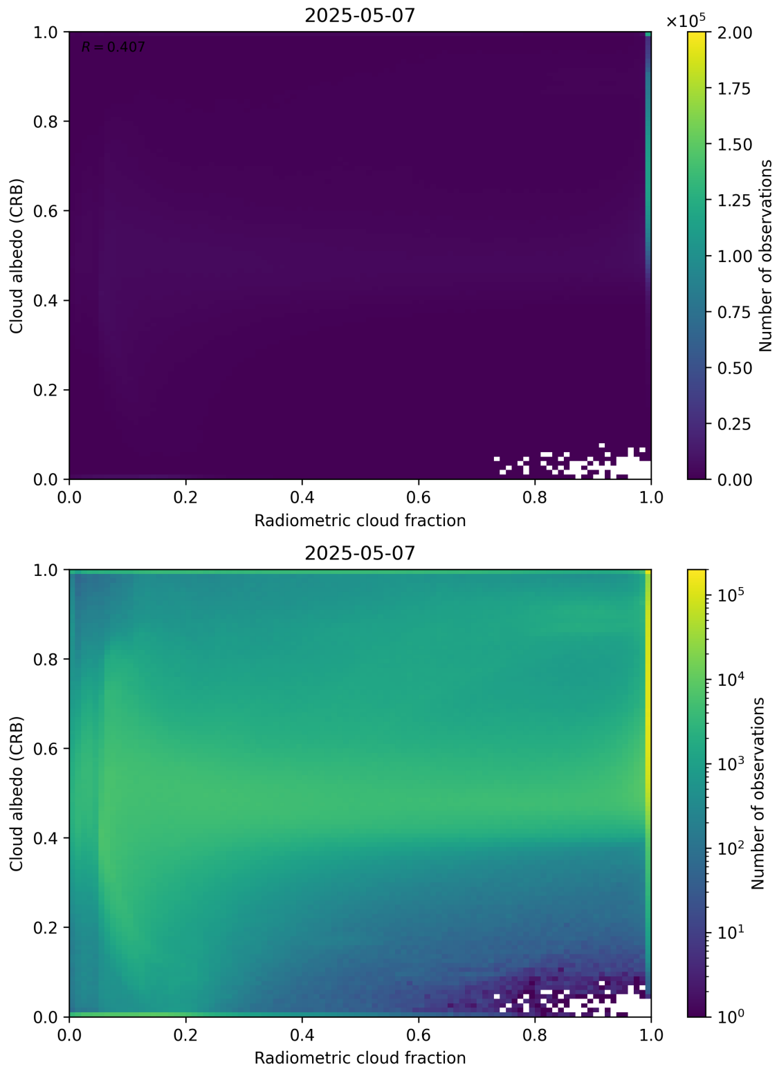
Figure 71: Scatter density plot of “Radiometric cloud fraction” against “Cloud albedo (CRB)” for 2025-05-06 to 2025-05-08.
