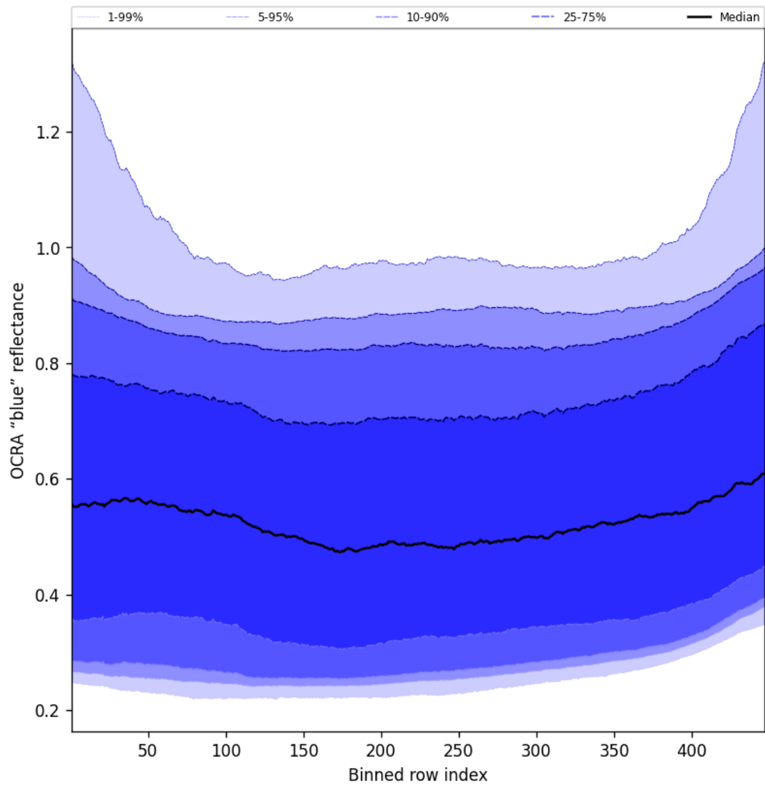
Figure 67: Along track statistics of “OCRA “blue” reflectance” for 2025-05-06 to 2025-05-08
