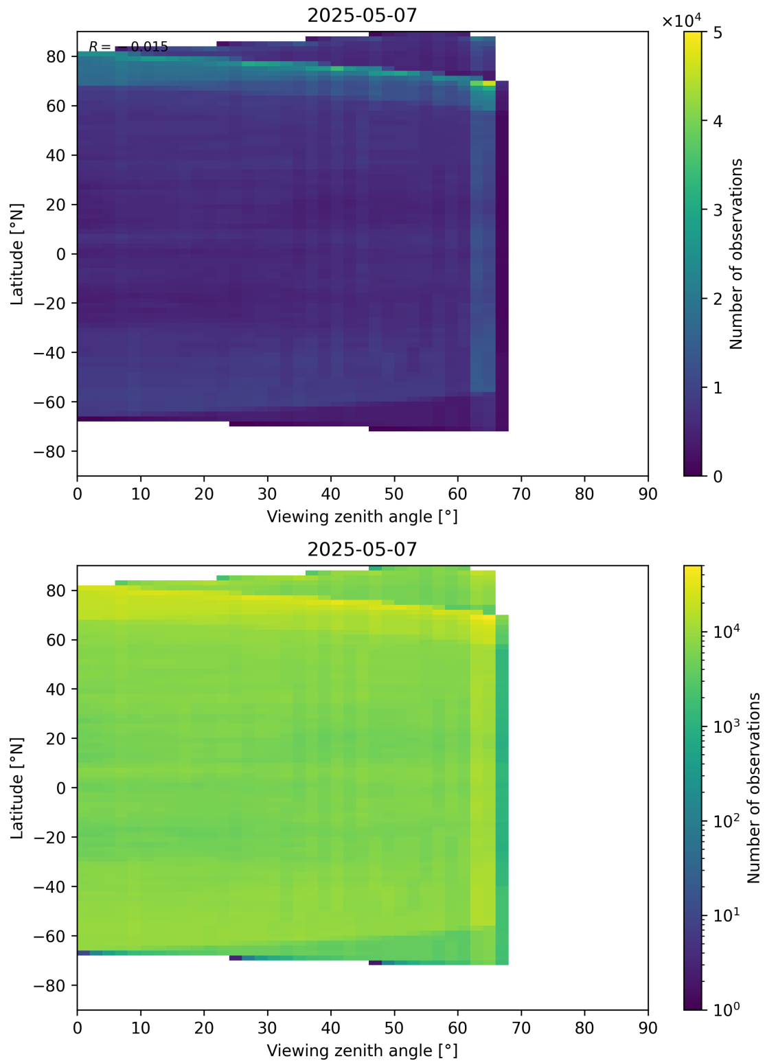
Figure 113: Scatter density plot of “Viewing zenith angle” against “Latitude” for 2025-05-06 to 2025-05-08.
