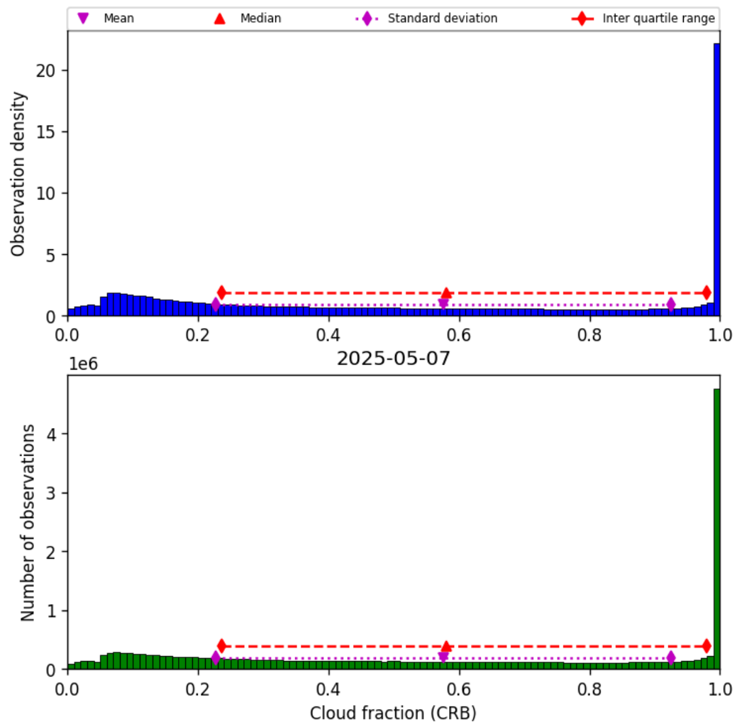
Figure 42: Histogram of “Cloud fraction (CRB)” for 2025-05-06 to 2025-05-08
