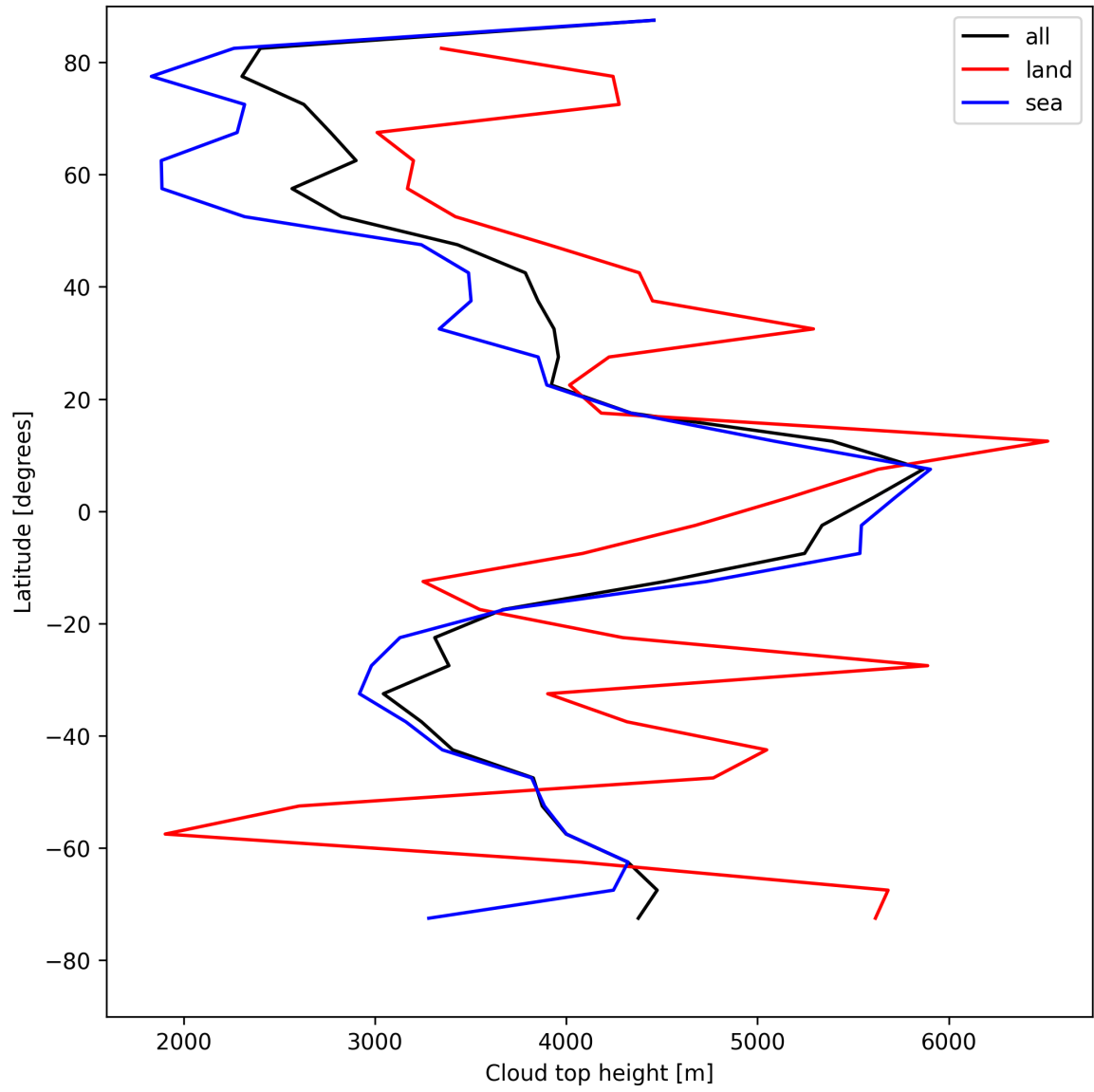
Figure 24: Zonal average of “Cloud top height” for 2025-05-06 to 2025-05-08.
