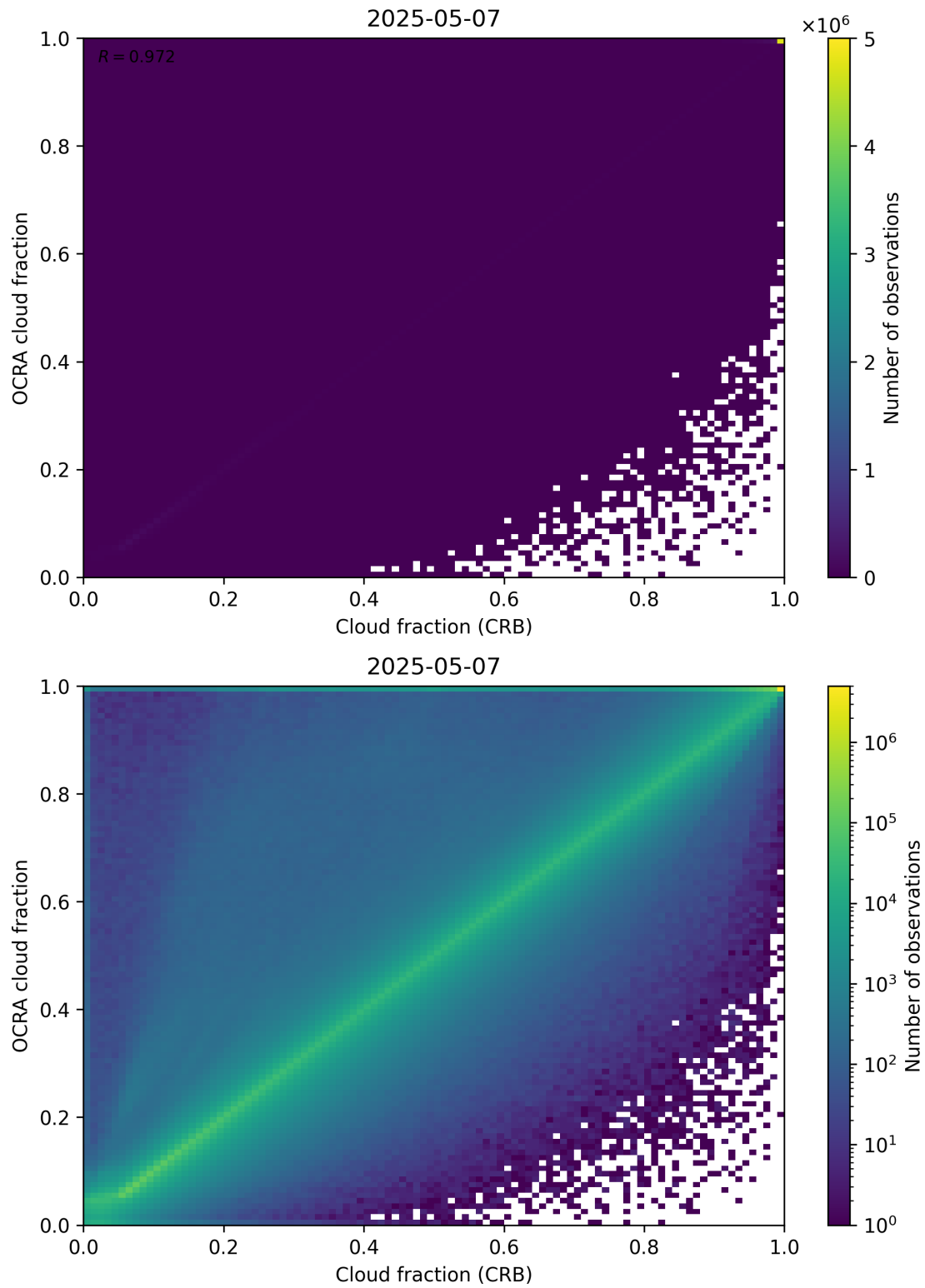
Figure 78: Scatter density plot of “Cloud fraction (CRB)” against “OCRA cloud fraction” for 2025-05-06 to 2025-05-08.
