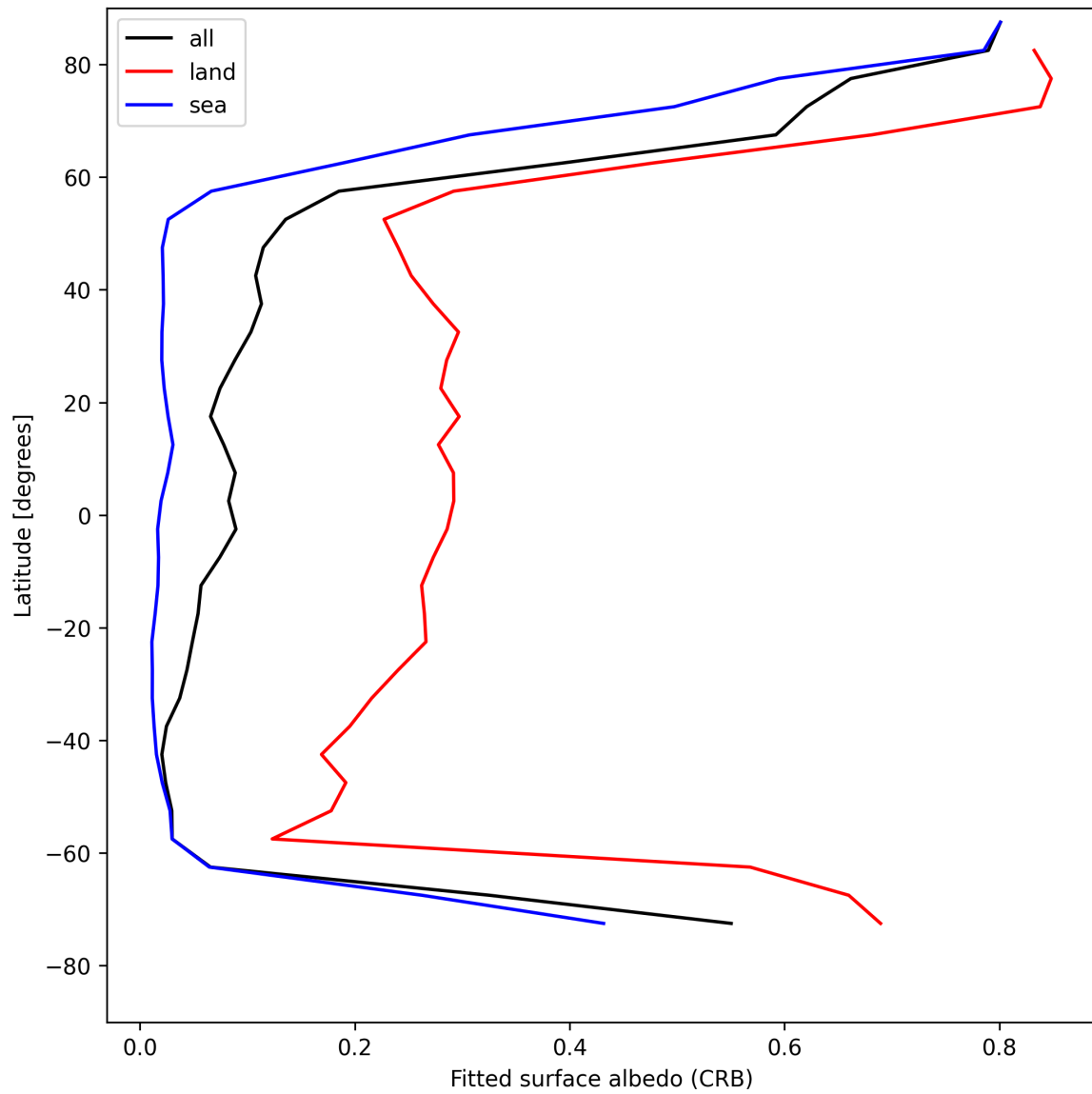
Figure 30: Zonal average of “Fitted surface albedo (CRB)” for 2025-05-06 to 2025-05-08.
