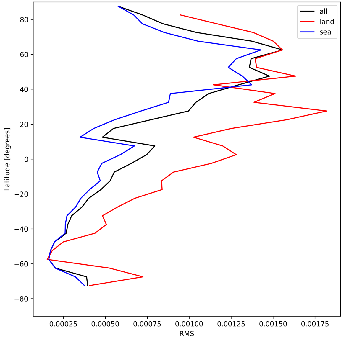
Figure 31: Zonal average of “RMS” for 2025-05-06 to 2025-05-08.
