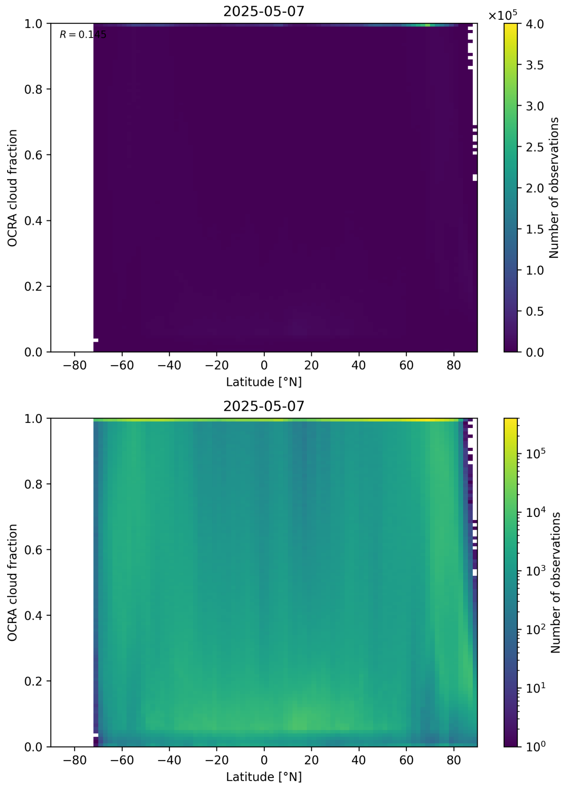
Figure 93: Scatter density plot of “Latitude” against “OCRA cloud fraction” for 2025-05-06 to 2025-05-08.
