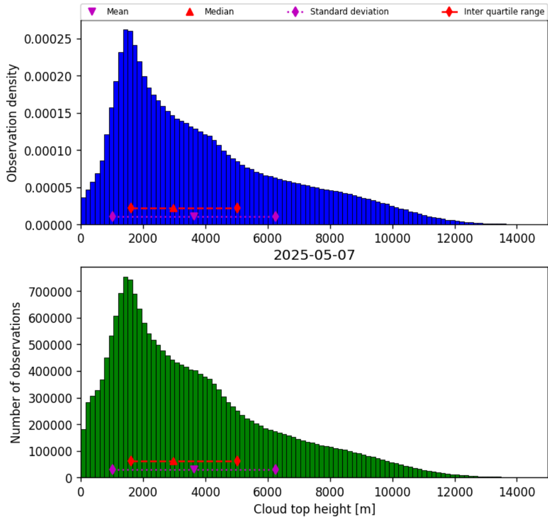
Figure 40: Histogram of “Cloud top height” for 2025-05-06 to 2025-05-08
