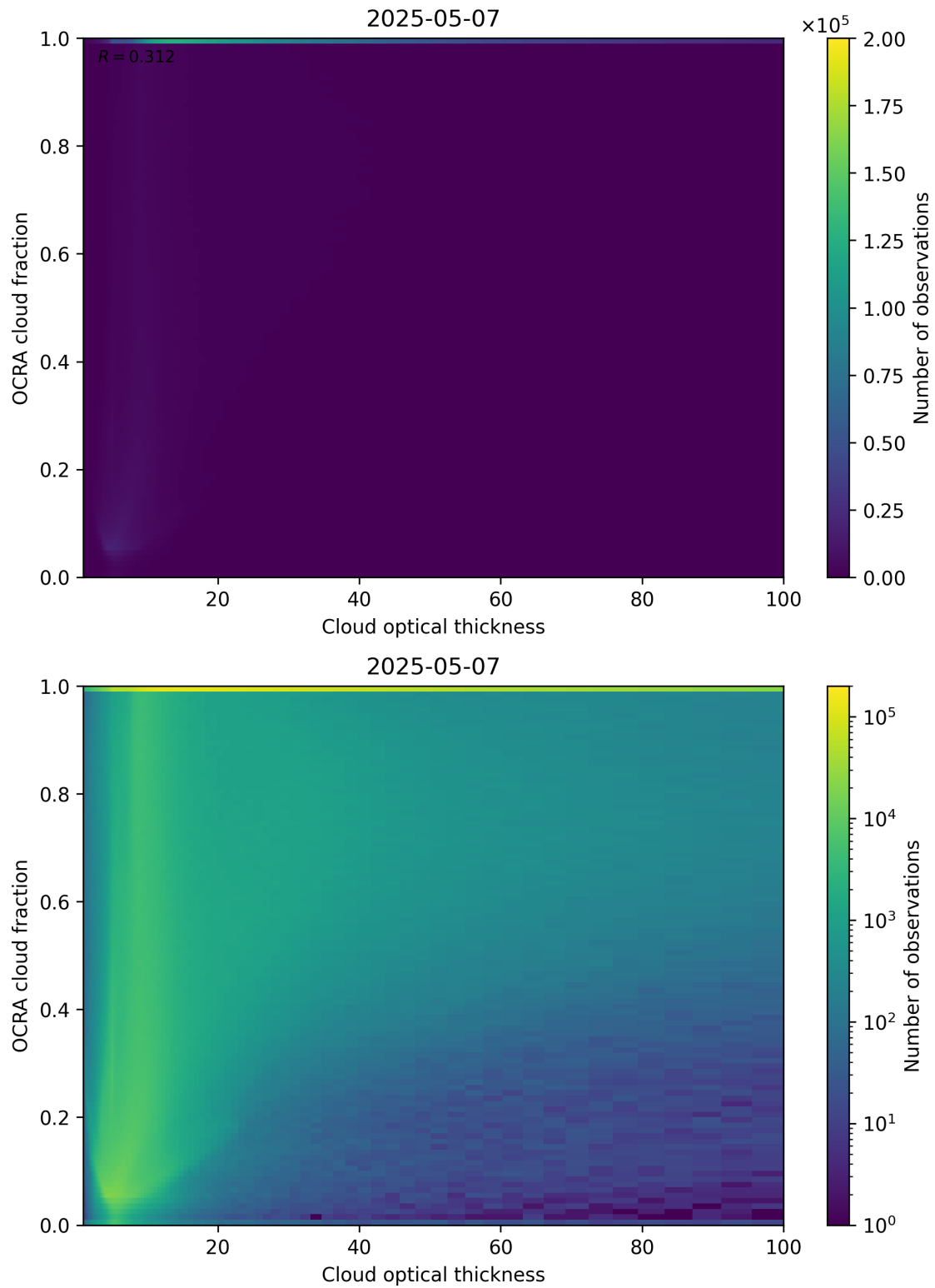
Figure 83: Scatter density plot of “Cloud optical thickness” against “OCRA cloud fraction” for 2025-05-06 to 2025-05-08.
