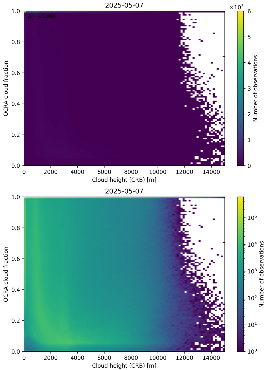
Figure 81: Scatter density plot of “Cloud height (CRB)” against “OCRA cloud fraction” for 2025-05-06 to 2025-05-08.
