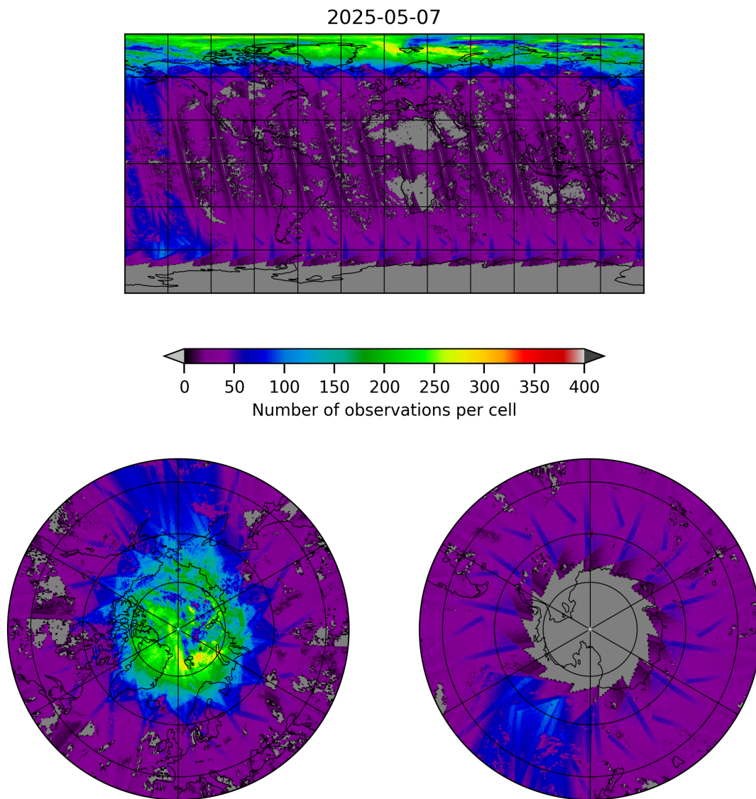
Figure 21: Map of the number of observations for 2025-05-06 to 2025-05-08
