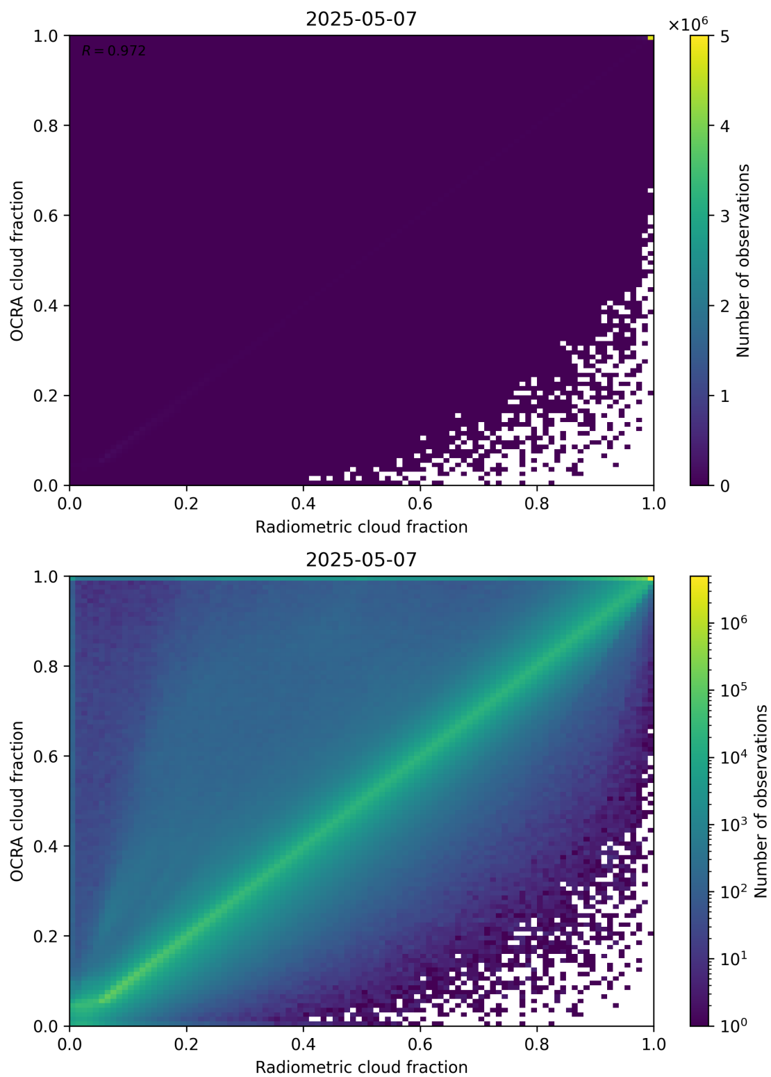
Figure 72: Scatter density plot of “Radiometric cloud fraction” against “OCRA cloud fraction” for 2025-05-06 to 2025-05-08.
