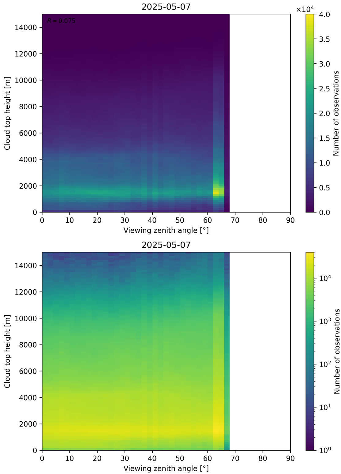
Figure 112: Scatter density plot of “Viewing zenith angle” against “Cloud top height” for 2025-05-06 to 2025-05-08.
