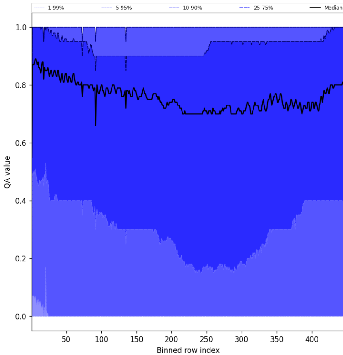
Figure 54: Along track statistics of "QA value" for 2025-05-06 to 2025-05-08
