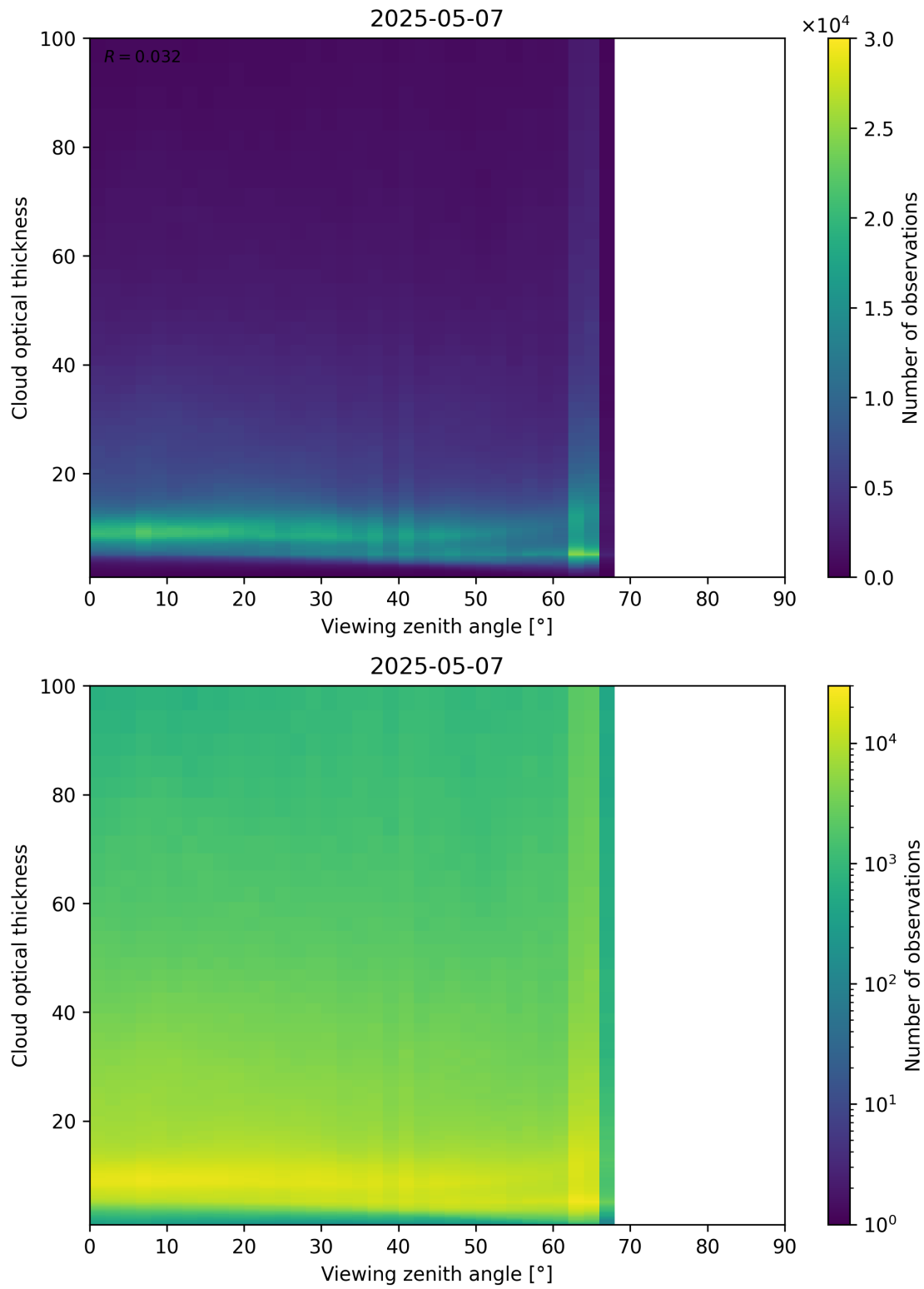
Figure 111: Scatter density plot of “Viewing zenith angle” against “Cloud optical thickness” for 2025-05-06 to 2025-05-08.
