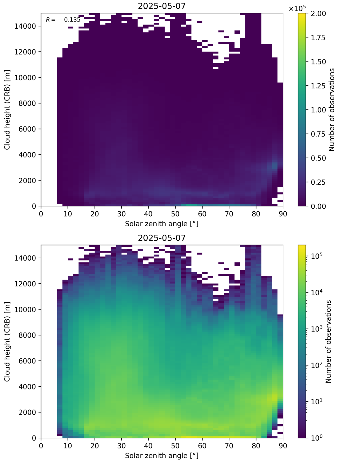
Figure 102: Scatter density plot of “Solar zenith angle” against “Cloud height (CRB)” for 2025-05-06 to 2025-05-08.
