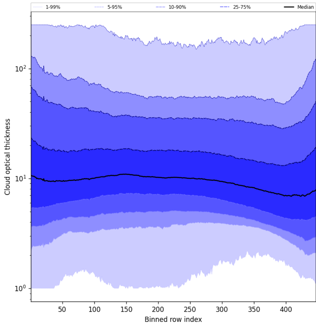
Figure 57: Along track statistics of “Cloud optical thickness” for 2025-05-06 to 2025-05-08
