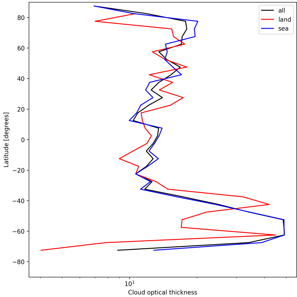
Figure 25: Zonal average of “Cloud optical thickness” for 2025-05-06 to 2025-05-08.
