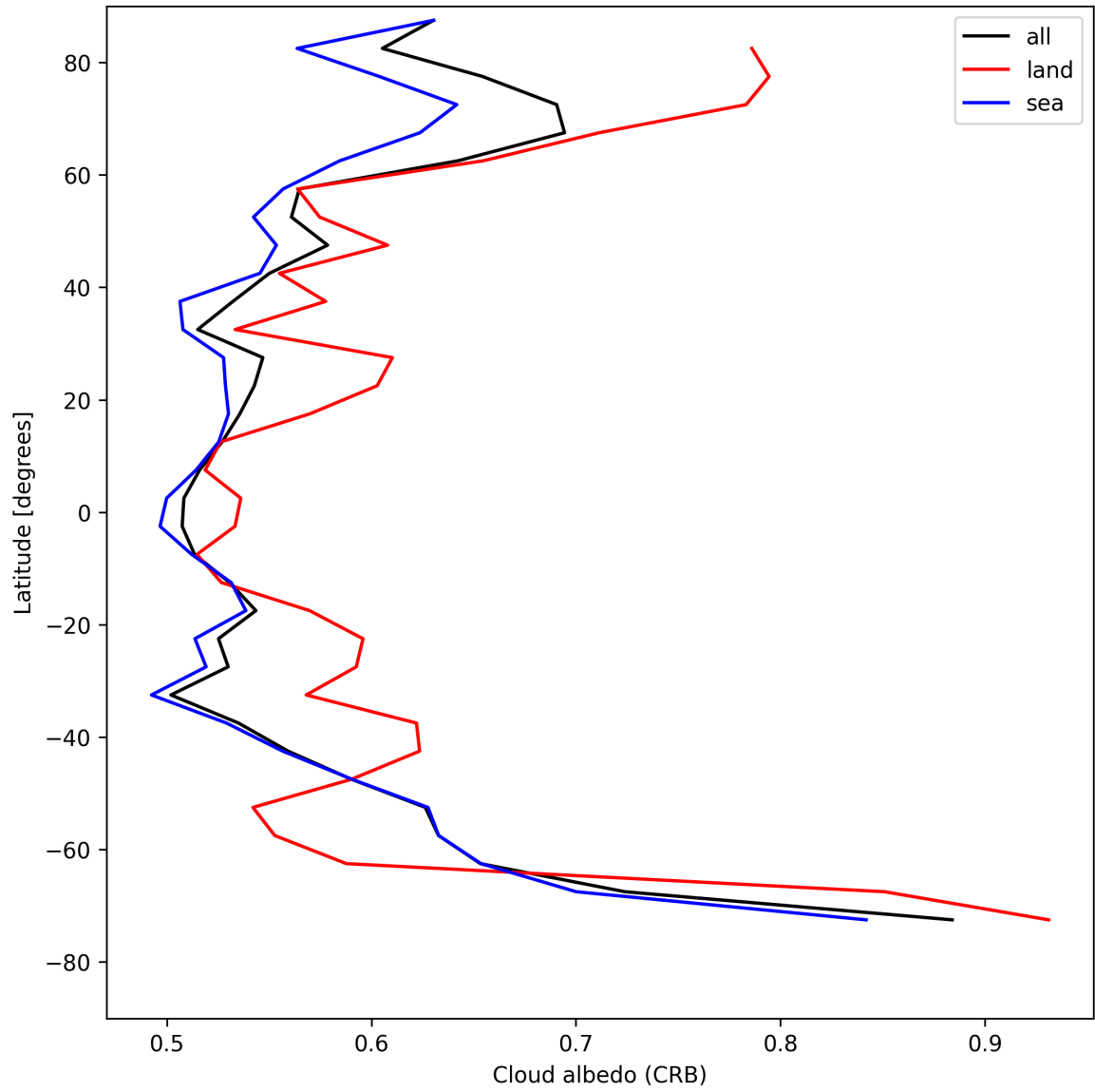
Figure 28: Zonal average of “Cloud albedo (CRB)” for 2025-05-06 to 2025-05-08.
