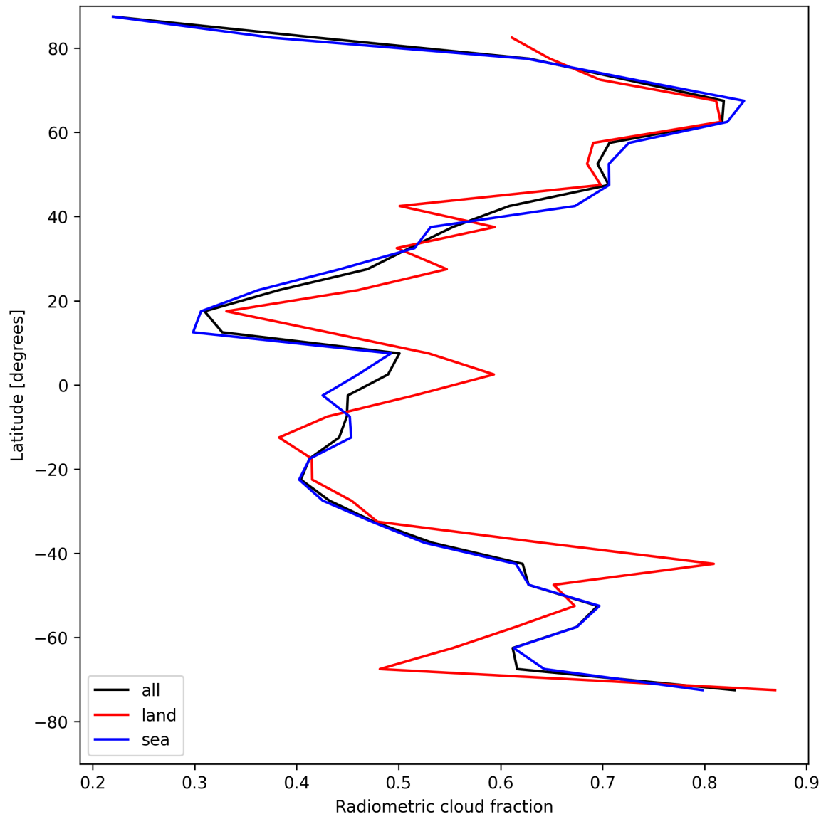
Figure 23: Zonal average of “Radiometric cloud fraction” for 2025-05-06 to 2025-05-08.
