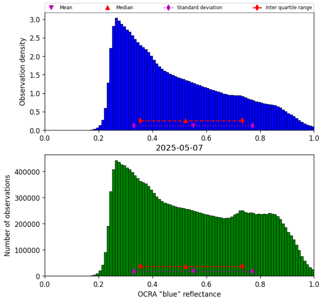
Figure 51: Histogram of “OCRA “blue” reflectance” for 2025-05-06 to 2025-05-08
