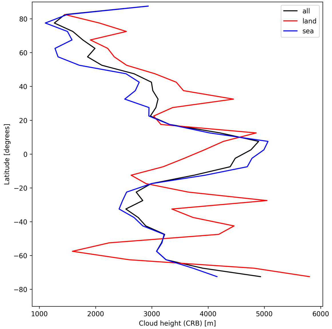
Figure 27: Zonal average of “Cloud height (CRB)” for 2025-05-06 to 2025-05-08.
