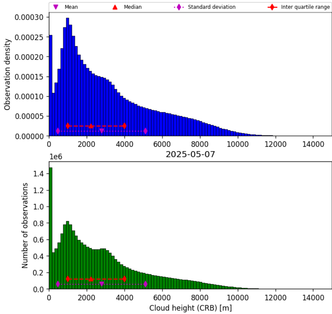
Figure 43: Histogram of “Cloud height (CRB)” for 2025-05-06 to 2025-05-08
