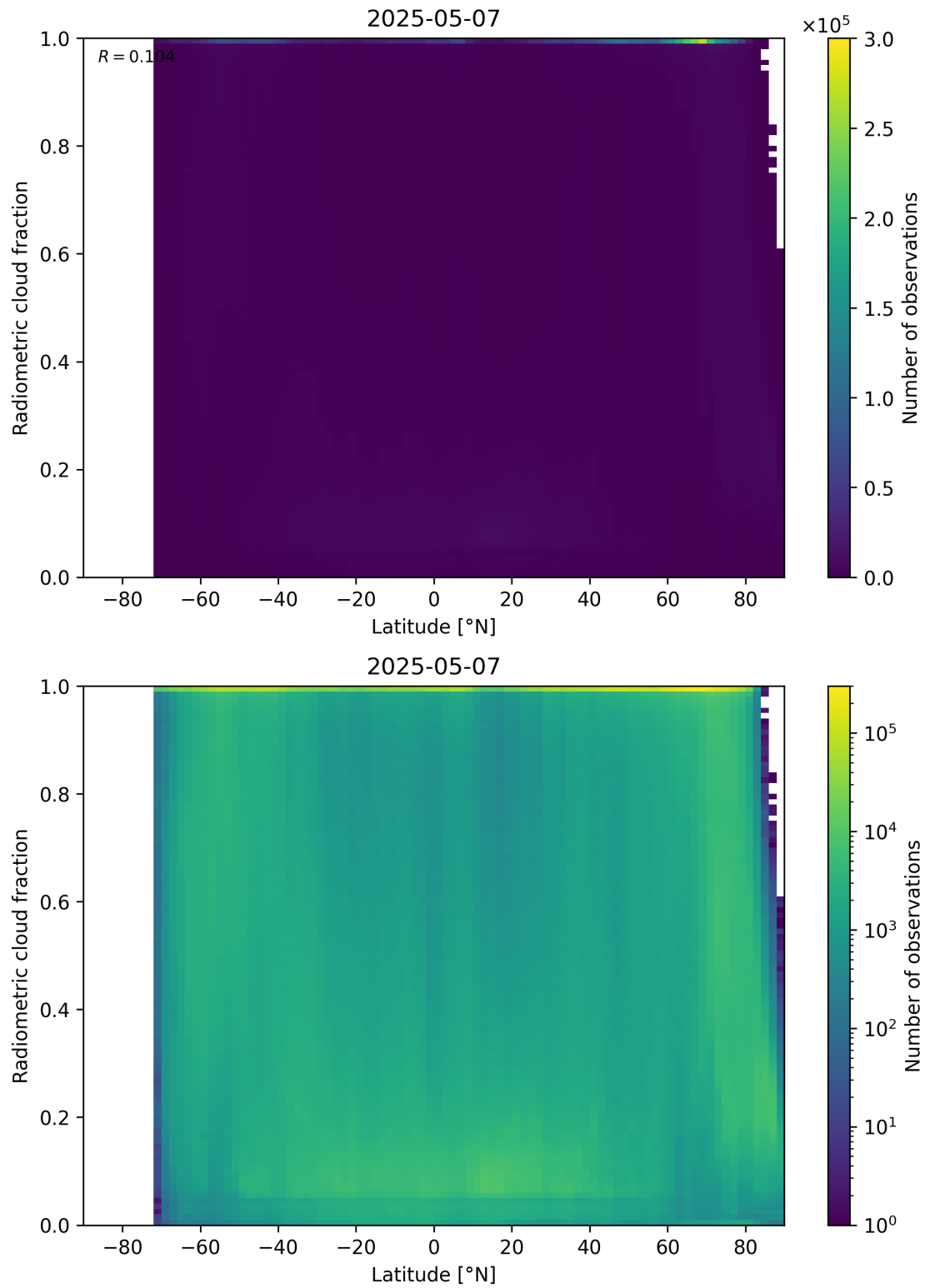
Figure 92: Scatter density plot of “Latitude” against “Radiometric cloud fraction” for 2025-05-06 to 2025-05-08.
