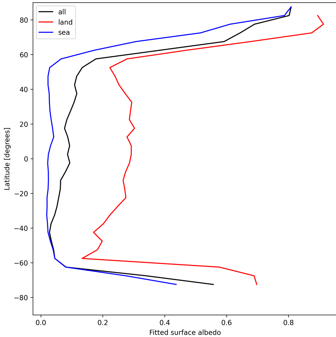
Figure 29: Zonal average of “Fitted surface albedo” for 2025-05-06 to 2025-05-08.
