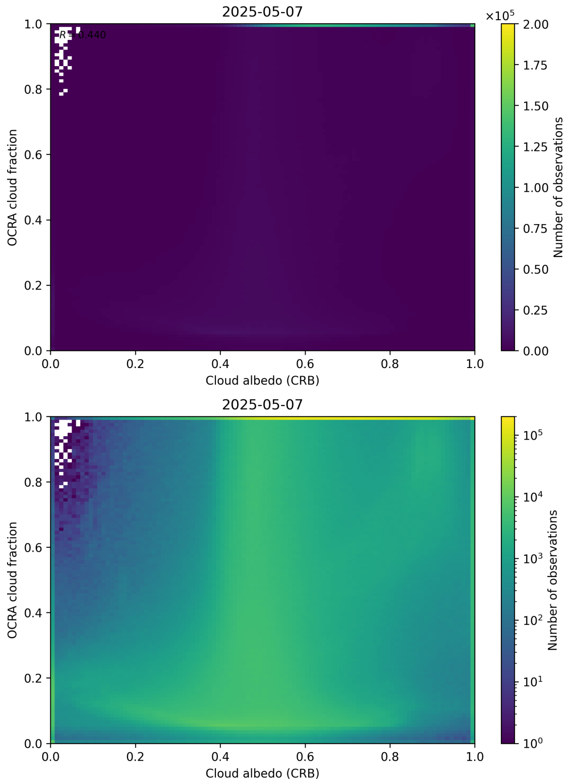
Figure 70: Scatter density plot of “Cloud albedo (CRB)” against “OCRA cloud fraction” for 2025-05-06 to 2025-05-08.
