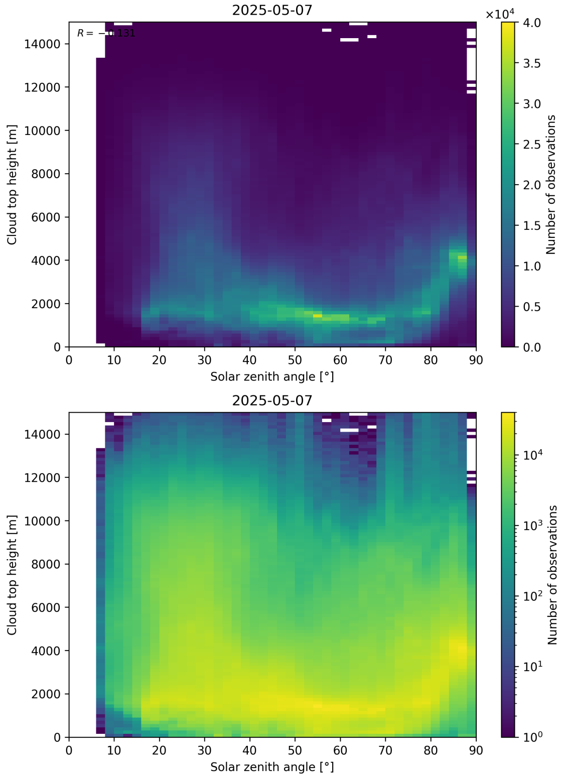
Figure 104: Scatter density plot of “Solar zenith angle” against “Cloud top height” for 2025-05-06 to 2025-05-08.
