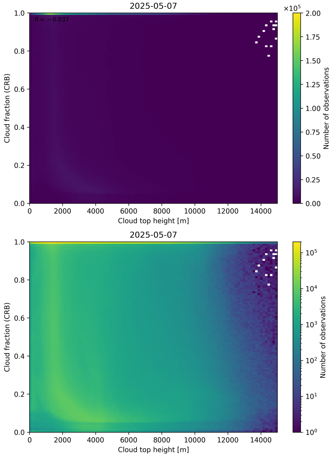
Figure 88: Scatter density plot of “Cloud top height” against “Cloud fraction (CRB)” for 2025-05-06 to 2025-05-08.
