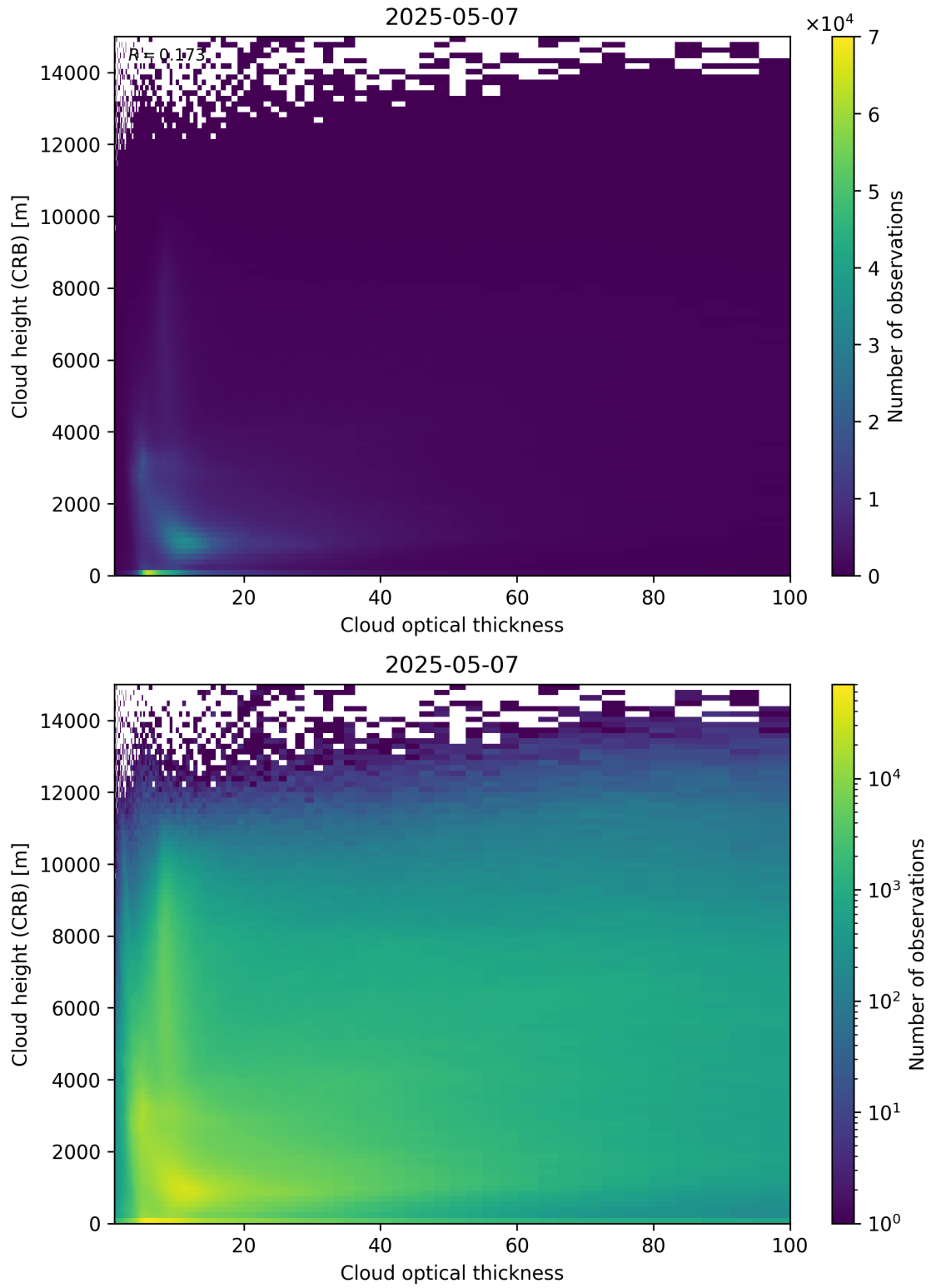
Figure 85: Scatter density plot of “Cloud optical thickness” against “Cloud height (CRB)” for 2025-05-06 to 2025-05-08.
