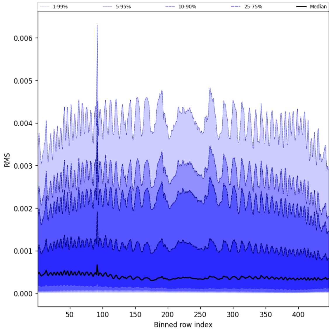
Figure 63: Along track statistics of “RMS” for 2025-05-06 to 2025-05-08
