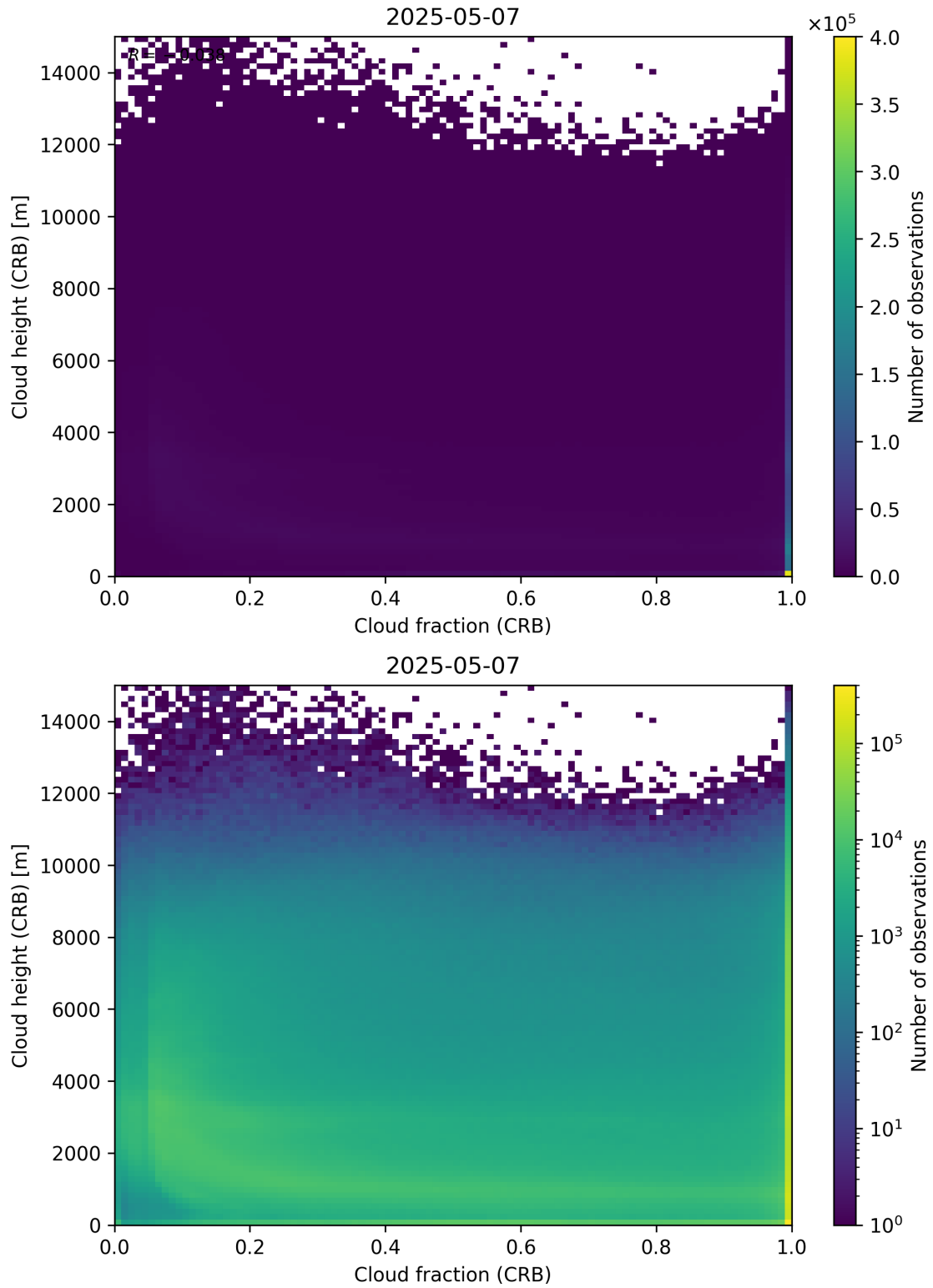
Figure 79: Scatter density plot of “Cloud fraction (CRB)” against “Cloud height (CRB)” for 2025-05-06 to 2025-05-08.
