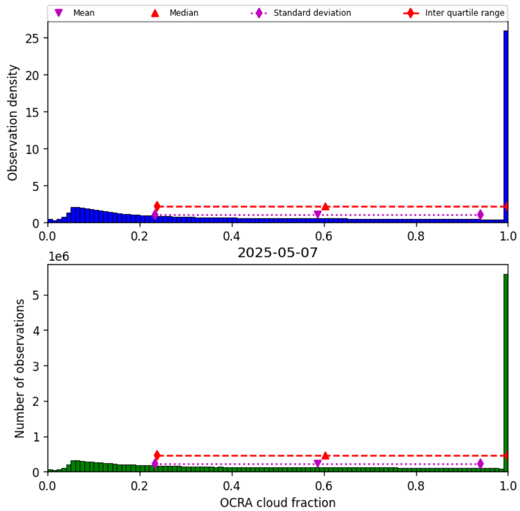
Figure 50: Histogram of “OCRA cloud fraction” for 2025-05-06 to 2025-05-08
