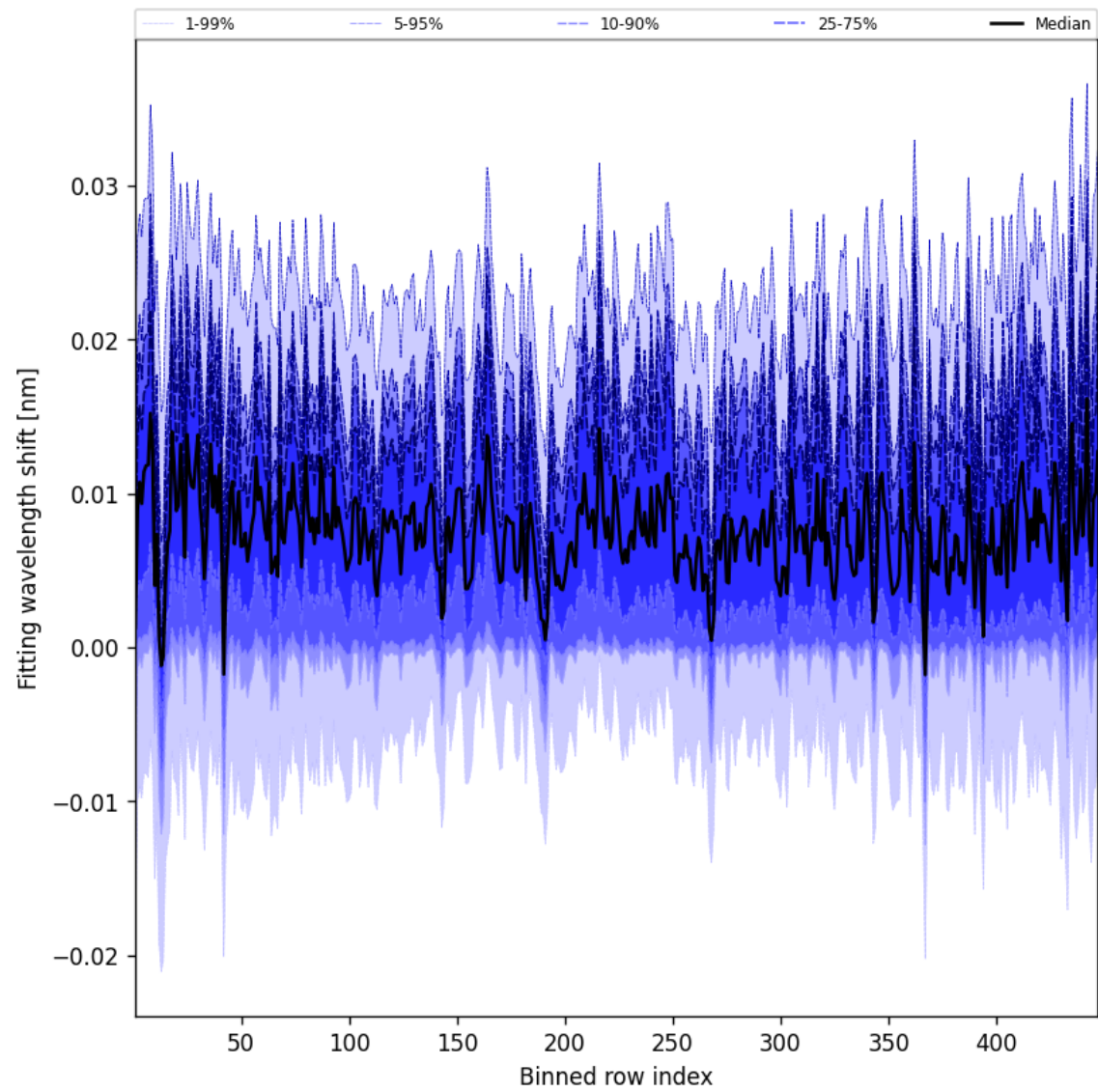
Figure 65: Along track statistics of “Fitting wavelength shift” for 2025-05-06 to 2025-05-08
