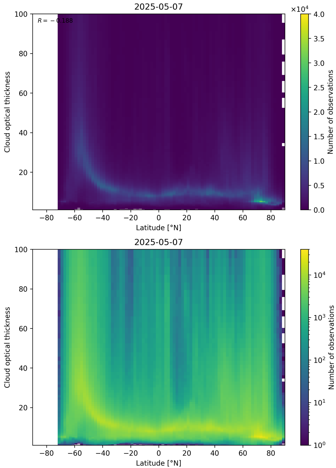
Figure 96: Scatter density plot of “Latitude” against “Cloud optical thickness” for 2025-05-06 to 2025-05-08.
