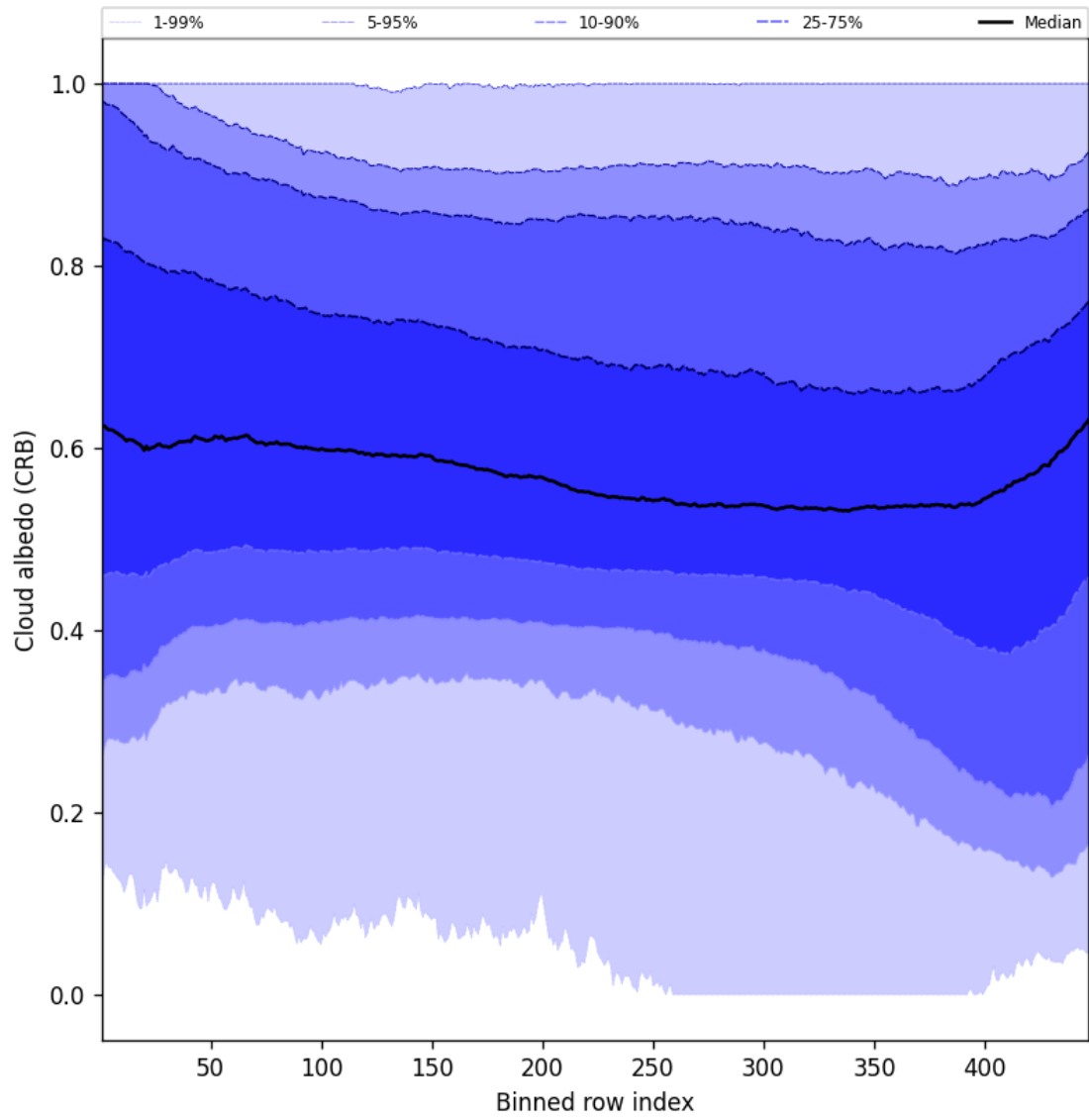
Figure 60: Along track statistics of “Cloud albedo (CRB)” for 2025-05-06 to 2025-05-08
