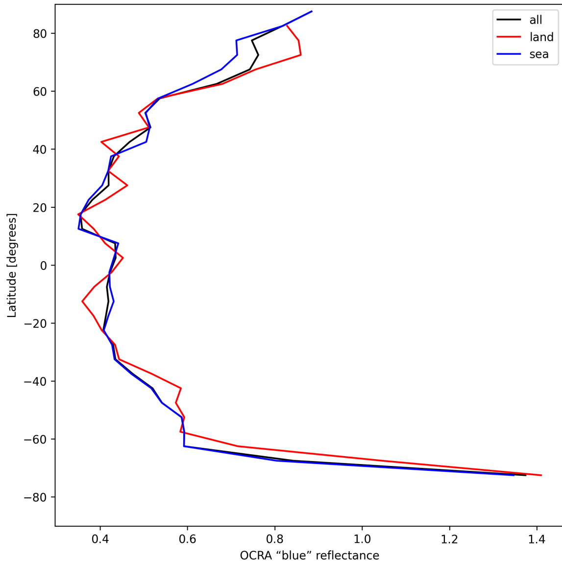
Figure 35: Zonal average of “OCRA “blue” reflectance” for 2025-05-06 to 2025-05-08.
