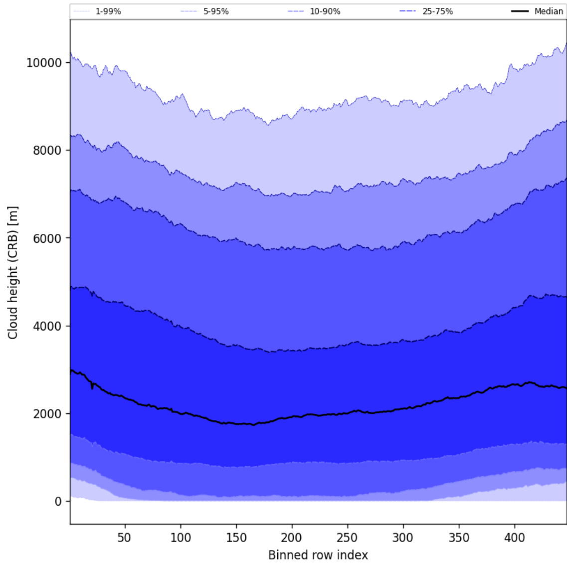
Figure 59: Along track statistics of “Cloud height (CRB)” for 2025-05-06 to 2025-05-08
