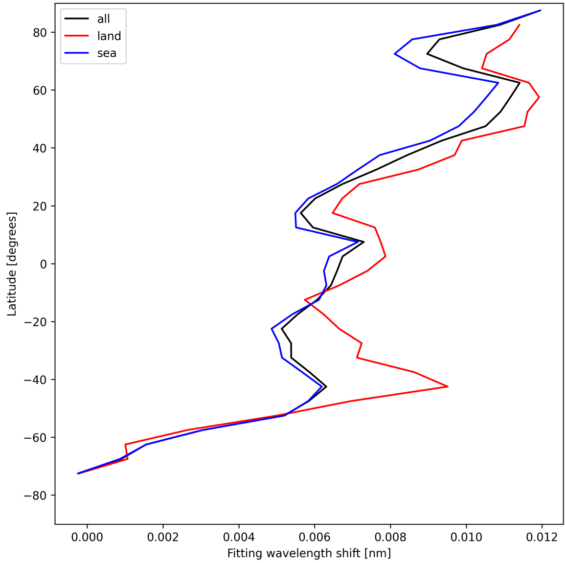
Figure 33: Zonal average of “Fitting wavelength shift” for 2025-05-06 to 2025-05-08.
