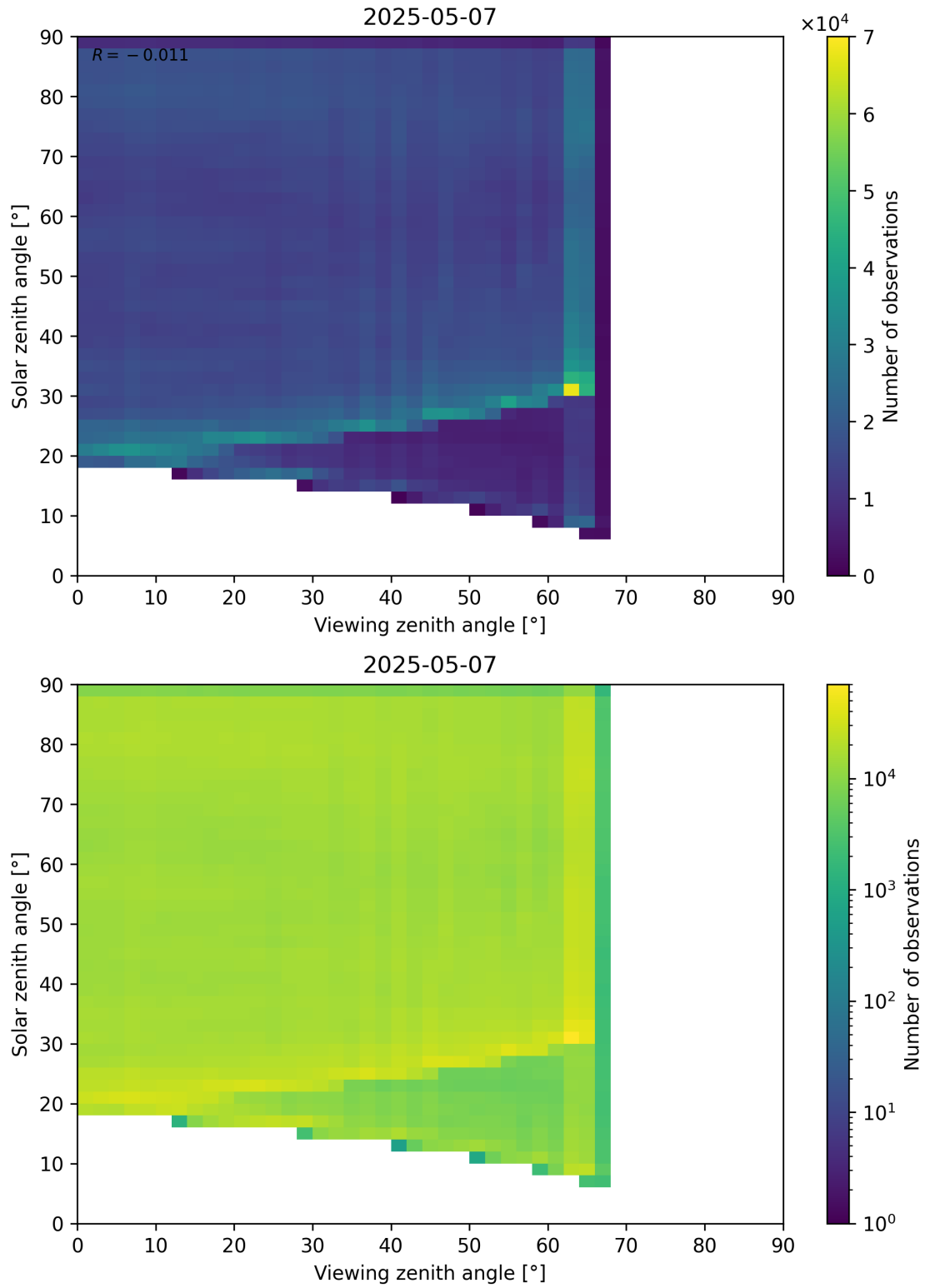
Figure 114: Scatter density plot of “Viewing zenith angle” against “Solar zenith angle” for 2025-05-06 to 2025-05-08.
