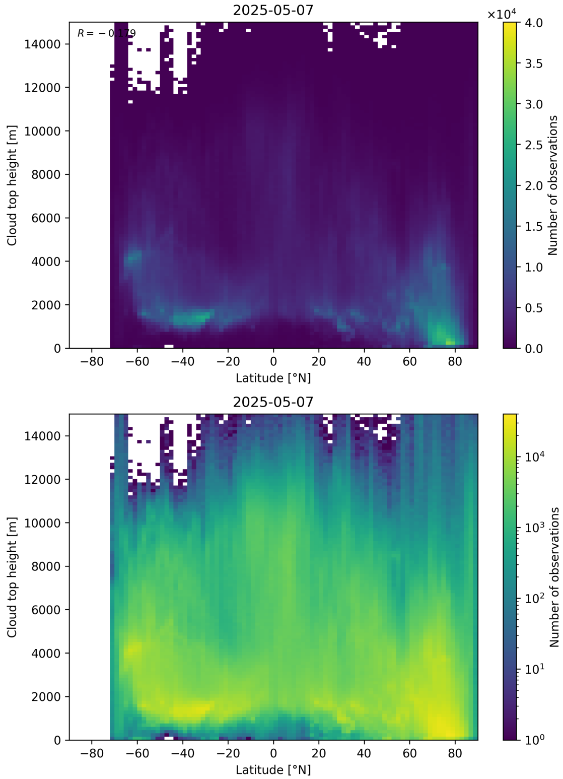
Figure 97: Scatter density plot of “Latitude” against “Cloud top height” for 2025-05-06 to 2025-05-08.
