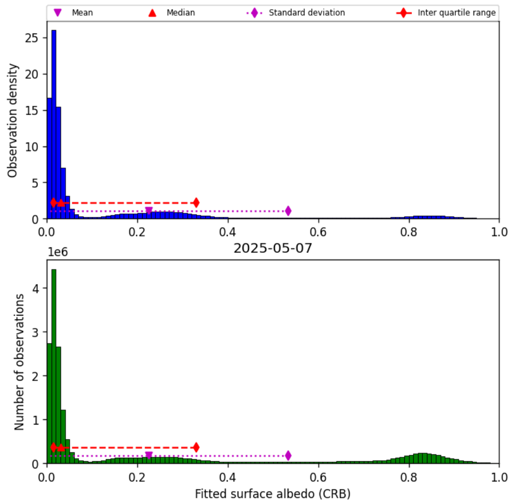
Figure 46: Histogram of “Fitted surface albedo (CRB)” for 2025-05-06 to 2025-05-08
