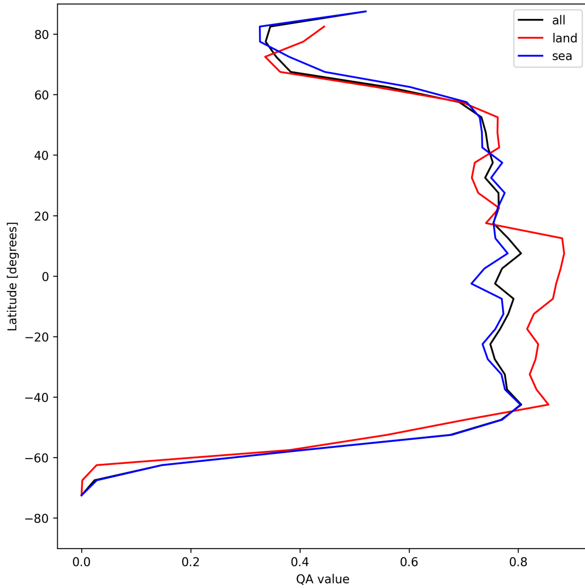
Figure 22: Zonal average of “QA value” for 2025-05-06 to 2025-05-08.
