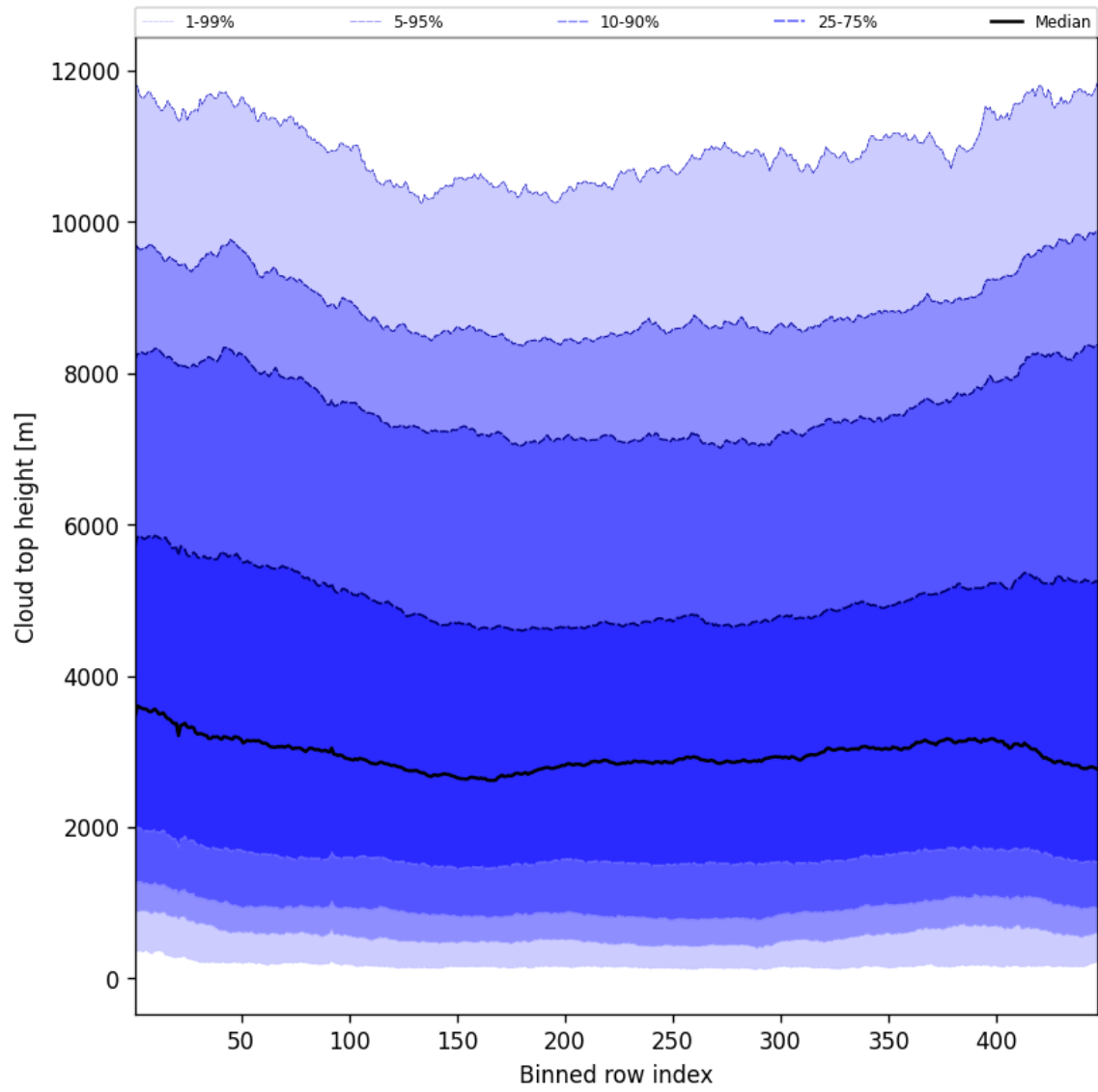
Figure 56: Along track statistics of “Cloud top height” for 2025-05-06 to 2025-05-08
