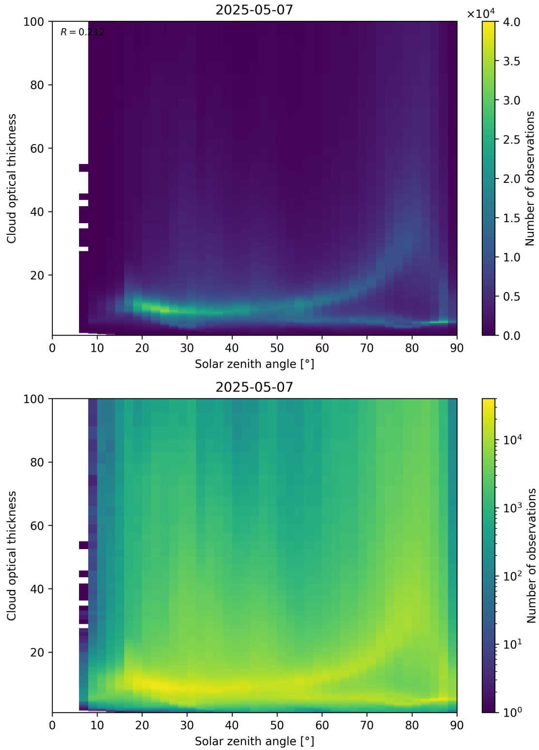
Figure 103: Scatter density plot of “Solar zenith angle” against “Cloud optical thickness” for 2025-05-06 to 2025-05-08.
