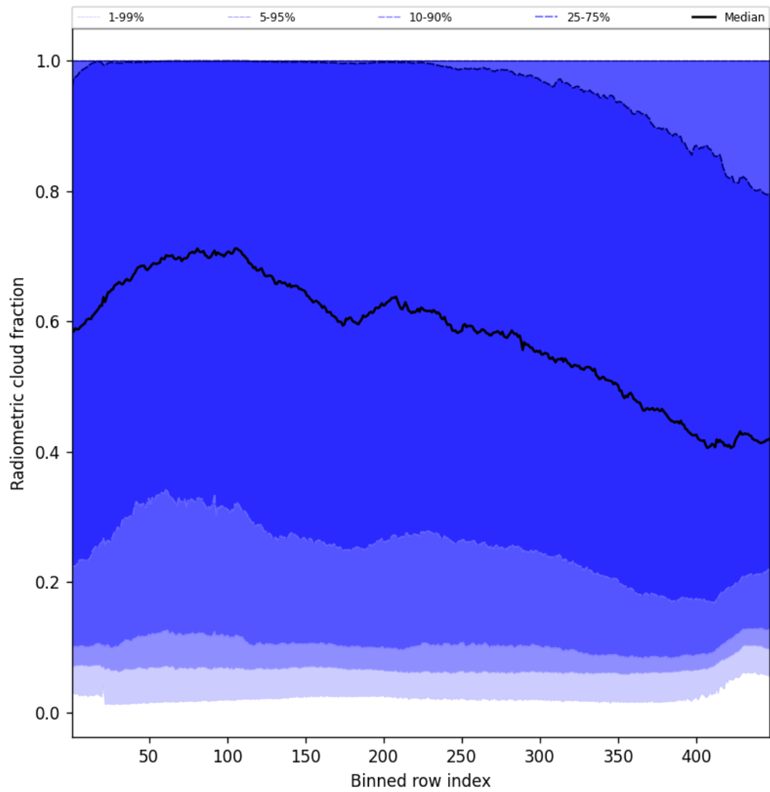
Figure 55: Along track statistics of “Radiometric cloud fraction” for 2025-05-06 to 2025-05-08
