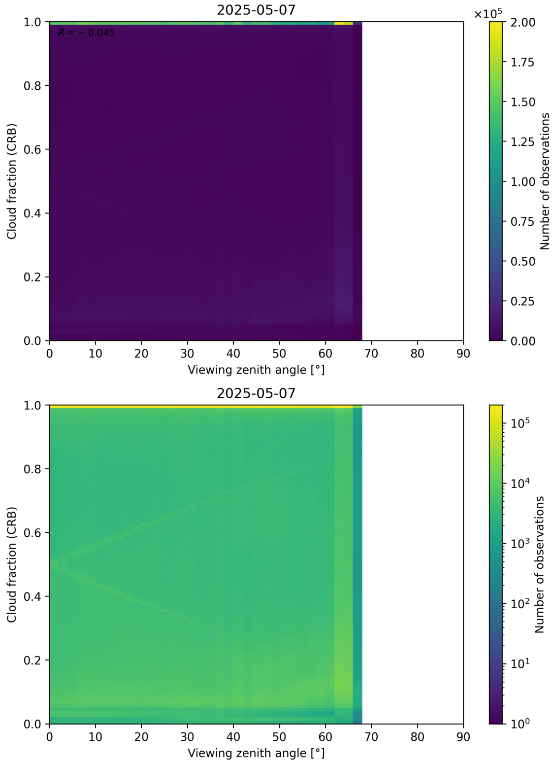
Figure 109: Scatter density plot of “Viewing zenith angle” against “Cloud fraction (CRB)” for 2025-05-06 to 2025-05-08.
