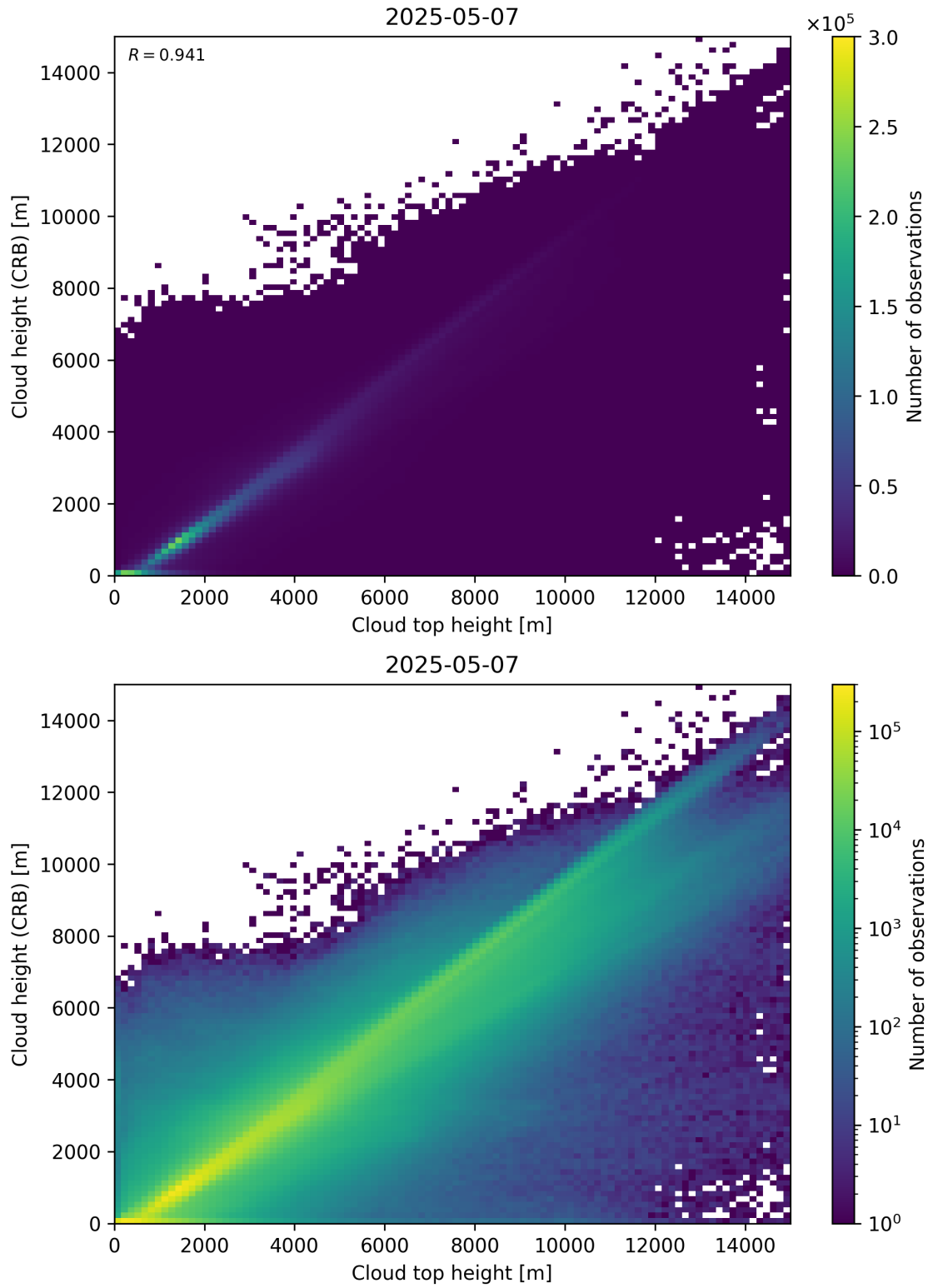
Figure 89: Scatter density plot of “Cloud top height” against “Cloud height (CRB)” for 2025-05-06 to 2025-05-08.
