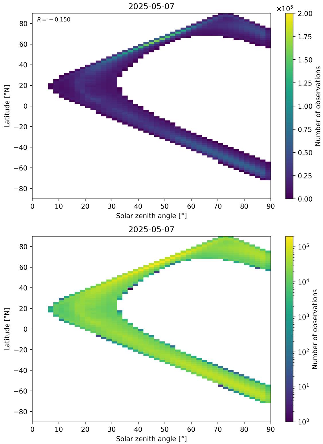
Figure 105: Scatter density plot of “Solar zenith angle” against “Latitude” for 2025-05-06 to 2025-05-08.
