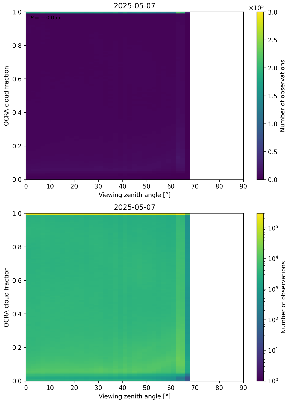
Figure 108: Scatter density plot of “Viewing zenith angle” against “OCRA cloud fraction” for 2025-05-06 to 2025-05-08.
