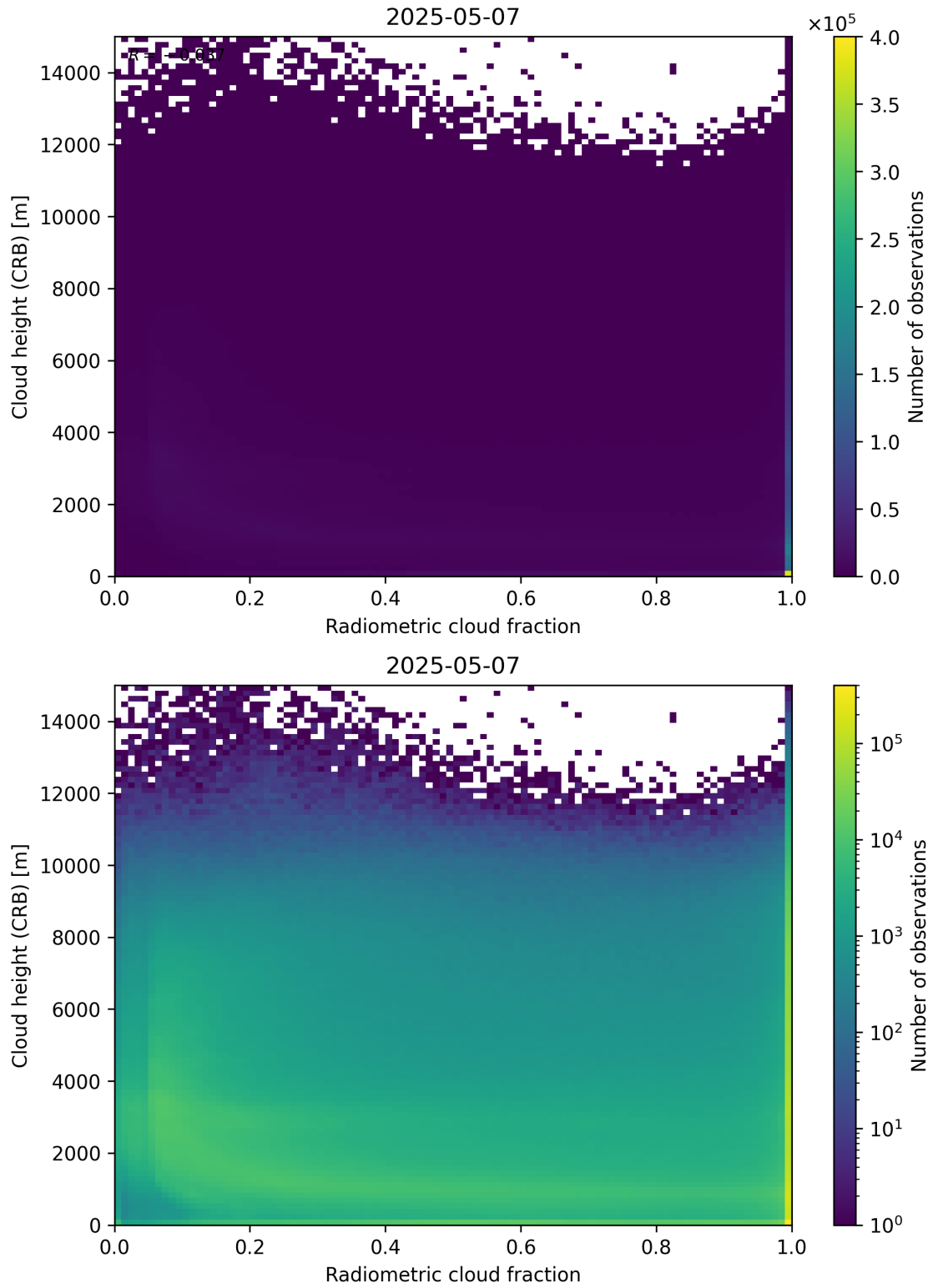
Figure 74: Scatter density plot of “Radiometric cloud fraction” against “Cloud height (CRB)” for 2025-05-06 to 2025-05-08.
