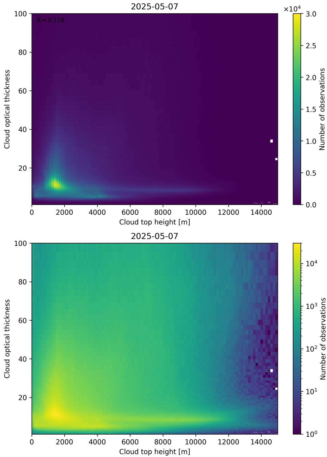
Figure 90: Scatter density plot of “Cloud top height” against “Cloud optical thickness” for 2025-05-06 to 2025-05-08.
