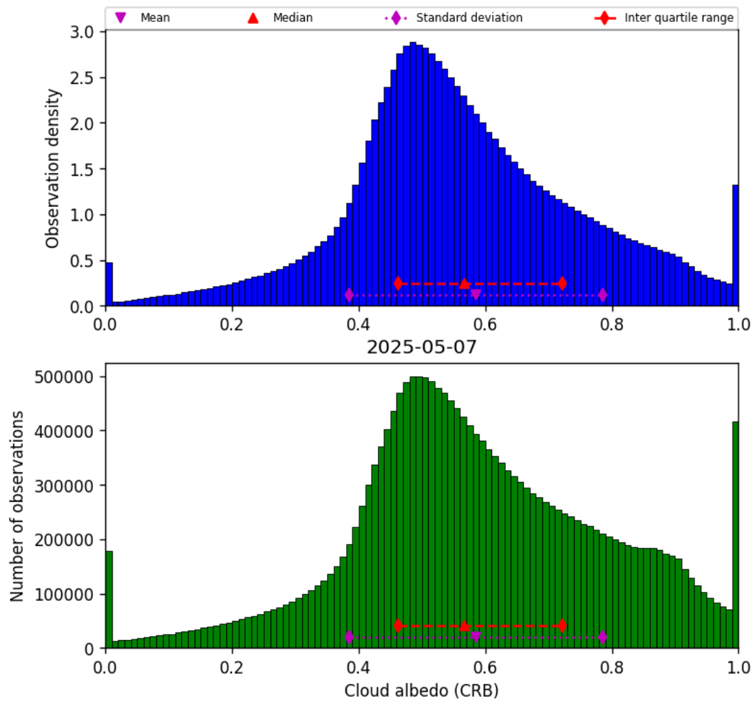
Figure 44: Histogram of “Cloud albedo (CRB)” for 2025-05-06 to 2025-05-08
