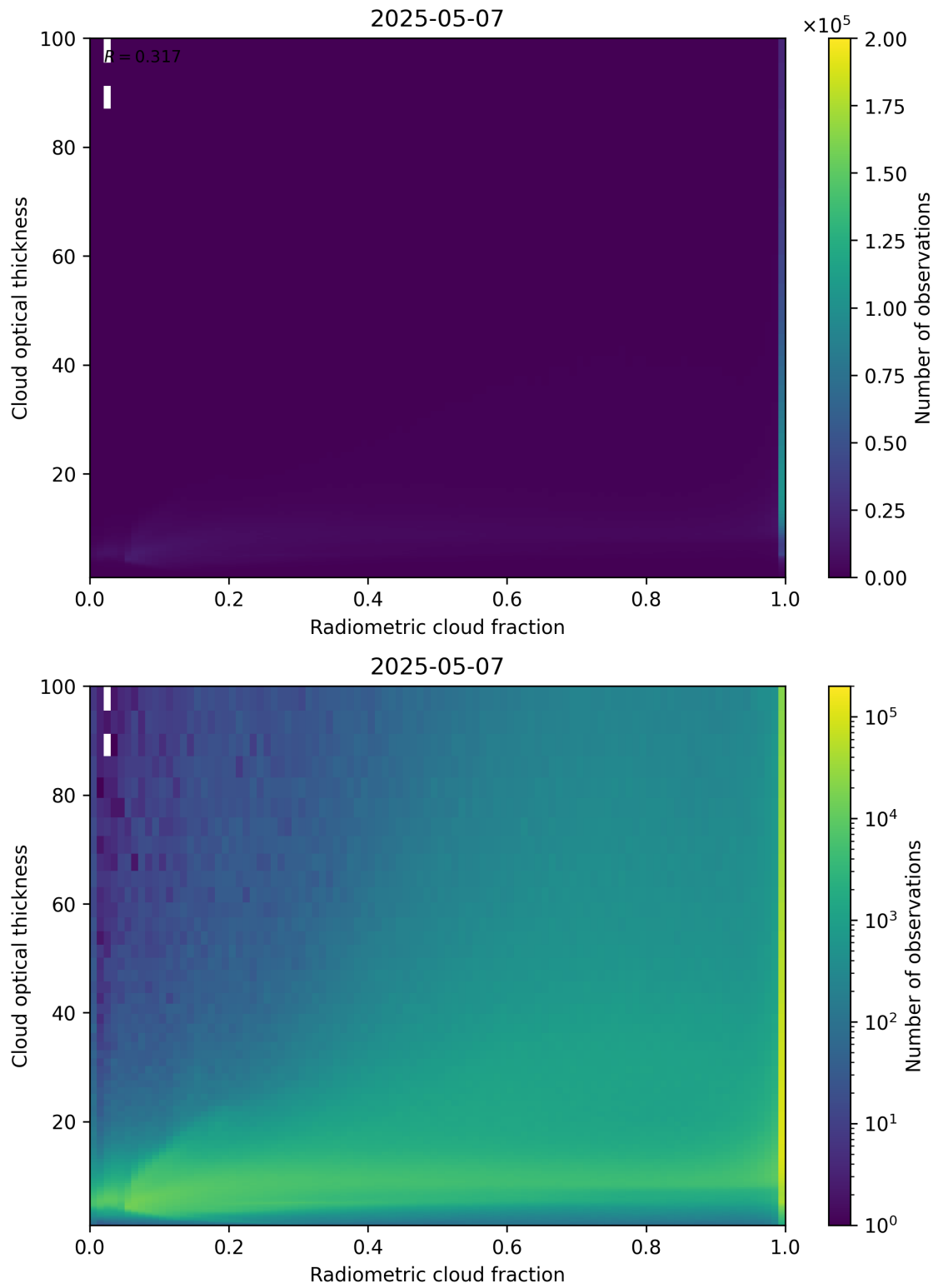
Figure 75: Scatter density plot of “Radiometric cloud fraction” against “Cloud optical thickness” for 2025-05-06 to 2025-05-08.
