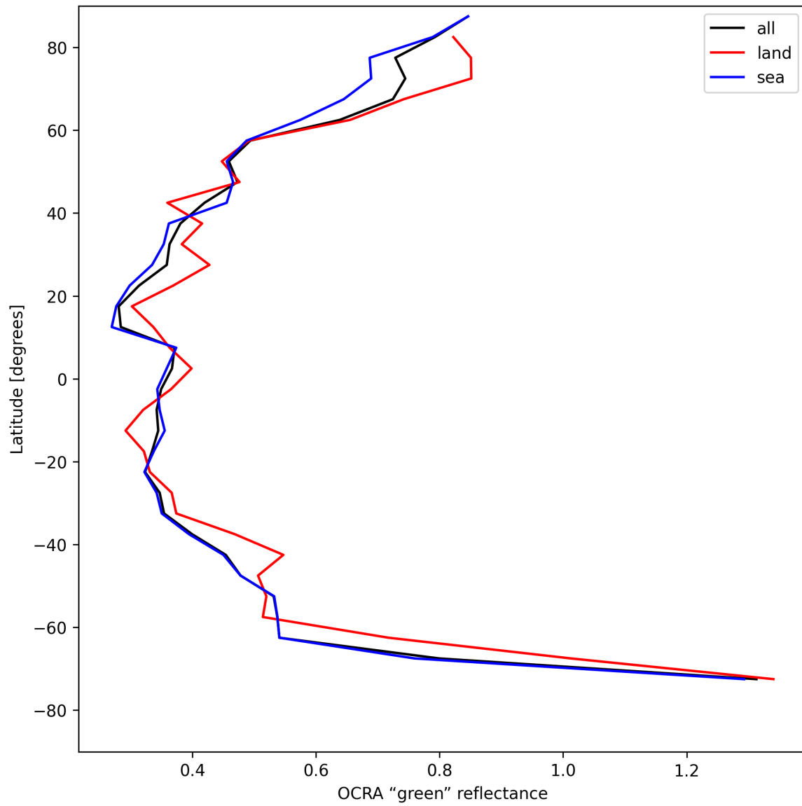
Figure 36: Zonal average of “OCRA “green” reflectance” for 2025-05-06 to 2025-05-08.
