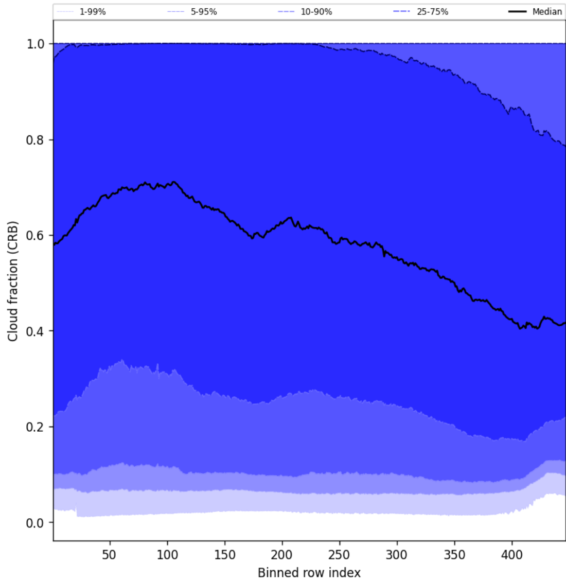
Figure 58: Along track statistics of “Cloud fraction (CRB)” for 2025-05-06 to 2025-05-08
