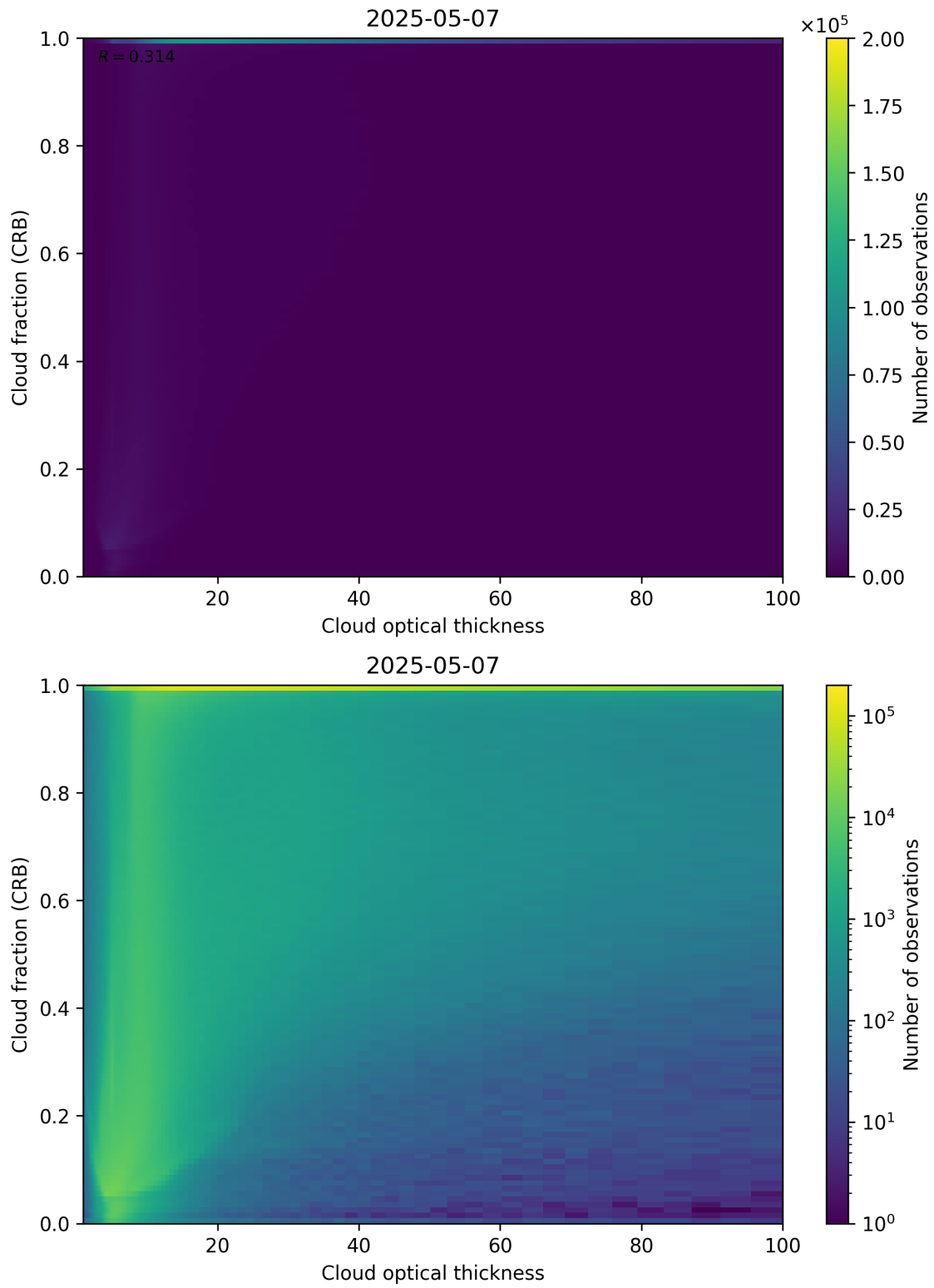
Figure 84: Scatter density plot of “Cloud optical thickness” against “Cloud fraction (CRB)” for 2025-05-06 to 2025-05-08.
