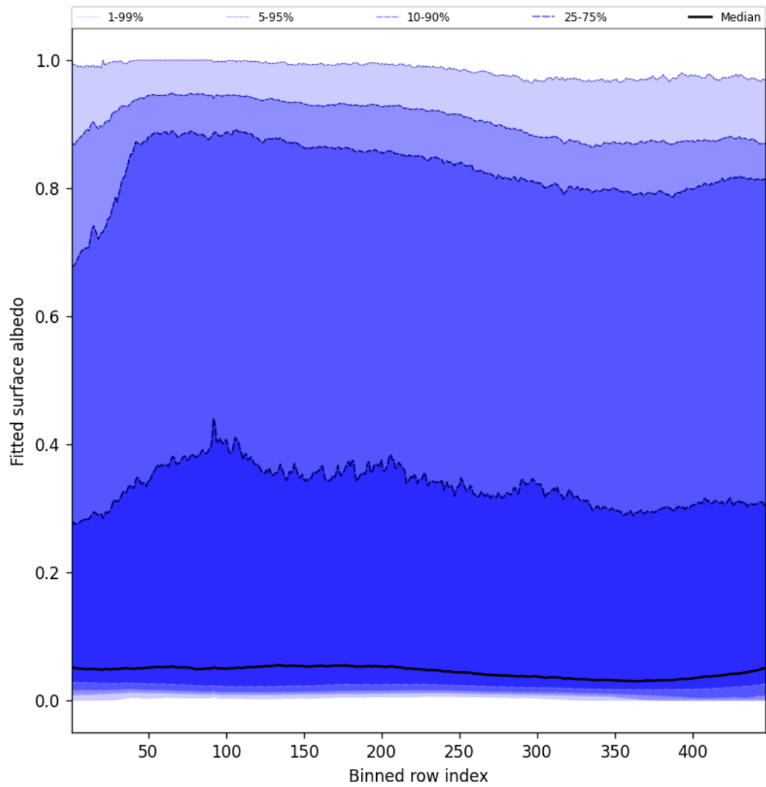
Figure 61: Along track statistics of “Fitted surface albedo” for 2025-05-06 to 2025-05-08
