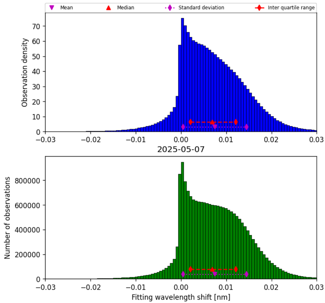
Figure 49: Histogram of “Fitting wavelength shift” for 2025-05-06 to 2025-05-08
