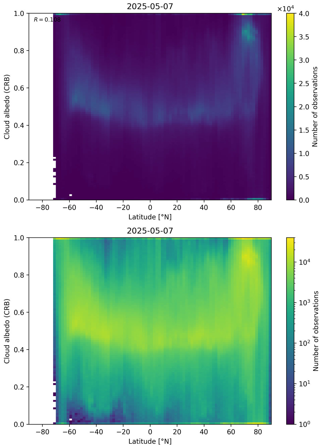
Figure 91: Scatter density plot of “Latitude” against “Cloud albedo (CRB)” for 2025-05-06 to 2025-05-08.
