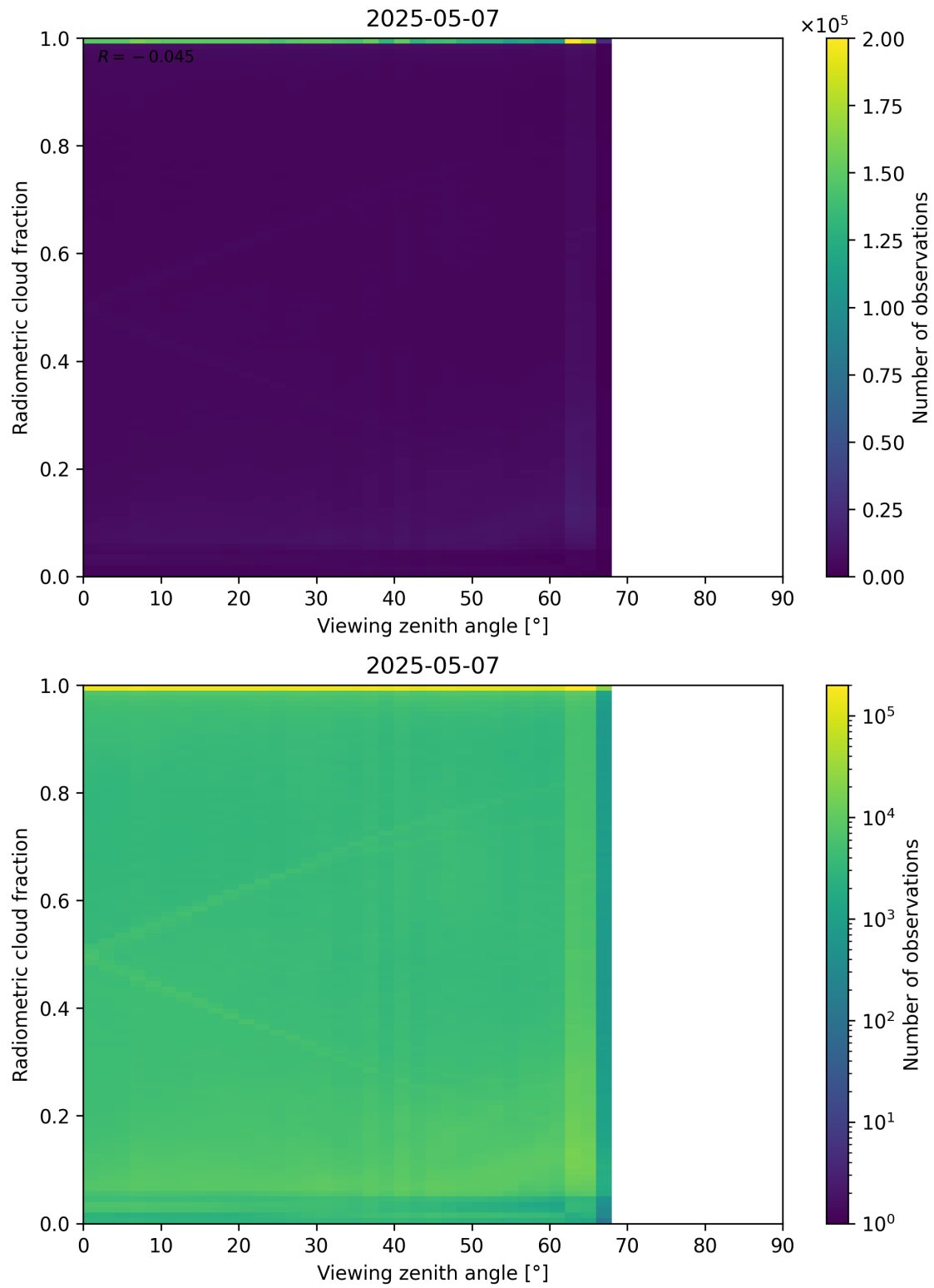
Figure 107: Scatter density plot of “Viewing zenith angle” against “Radiometric cloud fraction” for 2025-05-06 to 2025-05-08.
