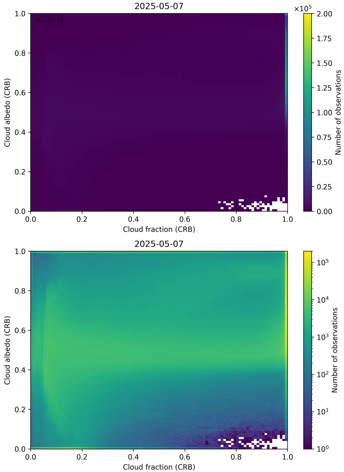
Figure 77: Scatter density plot of “Cloud fraction (CRB)” against “Cloud albedo (CRB)” for 2025-05-06 to 2025-05-08.
