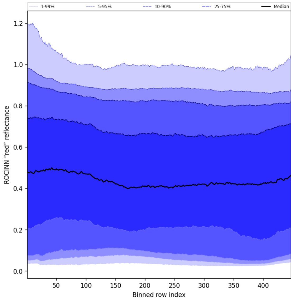
Figure 69: Along track statistics of “ROCINN “red” reflectance” for 2025-05-06 to 2025-05-08
