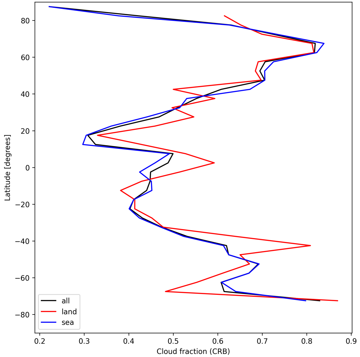
Figure 26: Zonal average of “Cloud fraction (CRB)” for 2025-05-06 to 2025-05-08.
