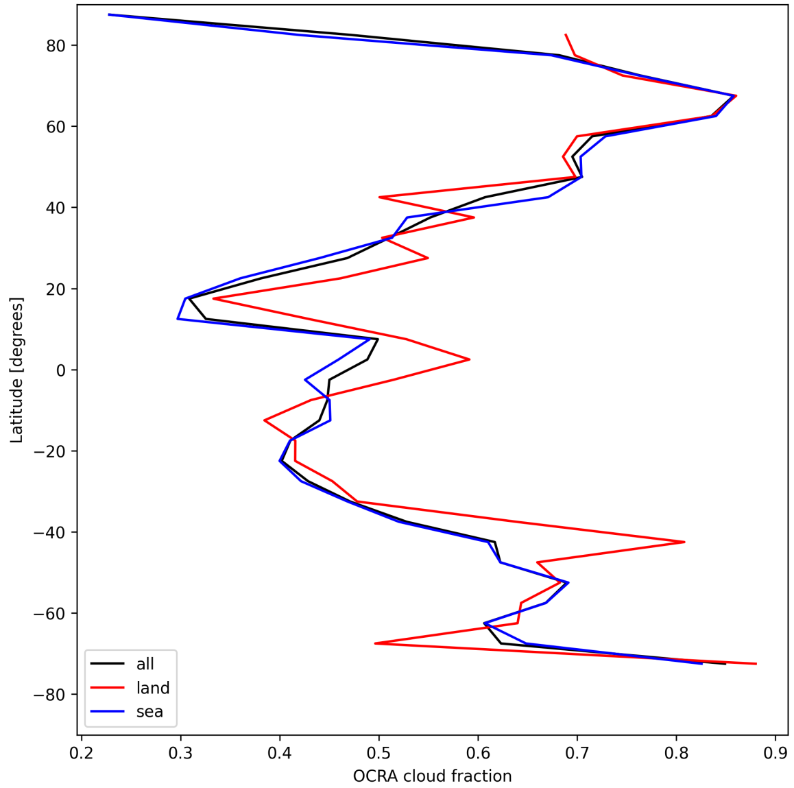
Figure 34: Zonal average of “OCRA cloud fraction” for 2025-05-06 to 2025-05-08.
