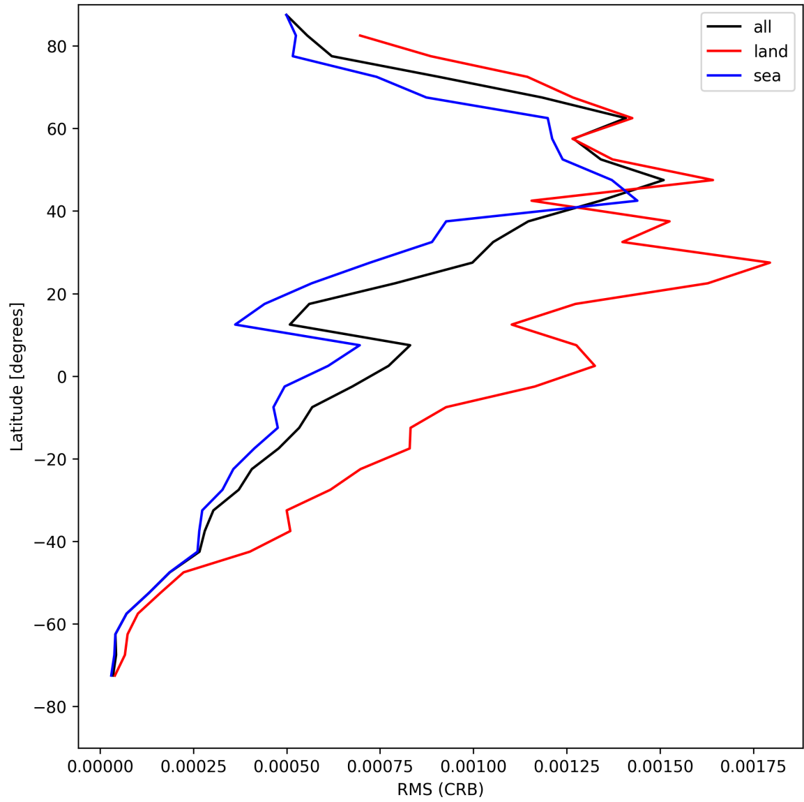
Figure 32: Zonal average of “RMS (CRB)” for 2025-05-06 to 2025-05-08.
