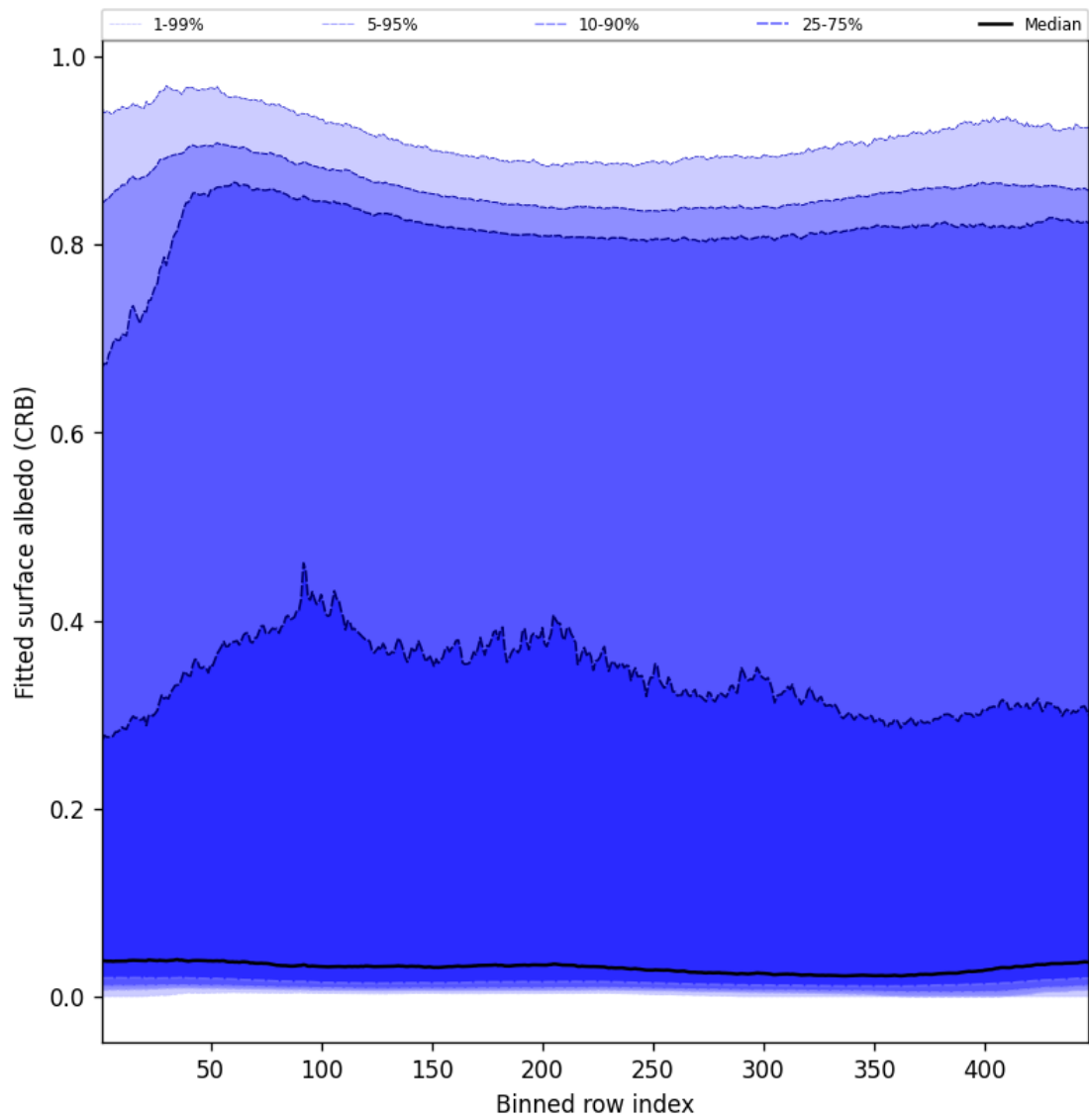
Figure 62: Along track statistics of “Fitted surface albedo (CRB)” for 2025-05-06 to 2025-05-08
