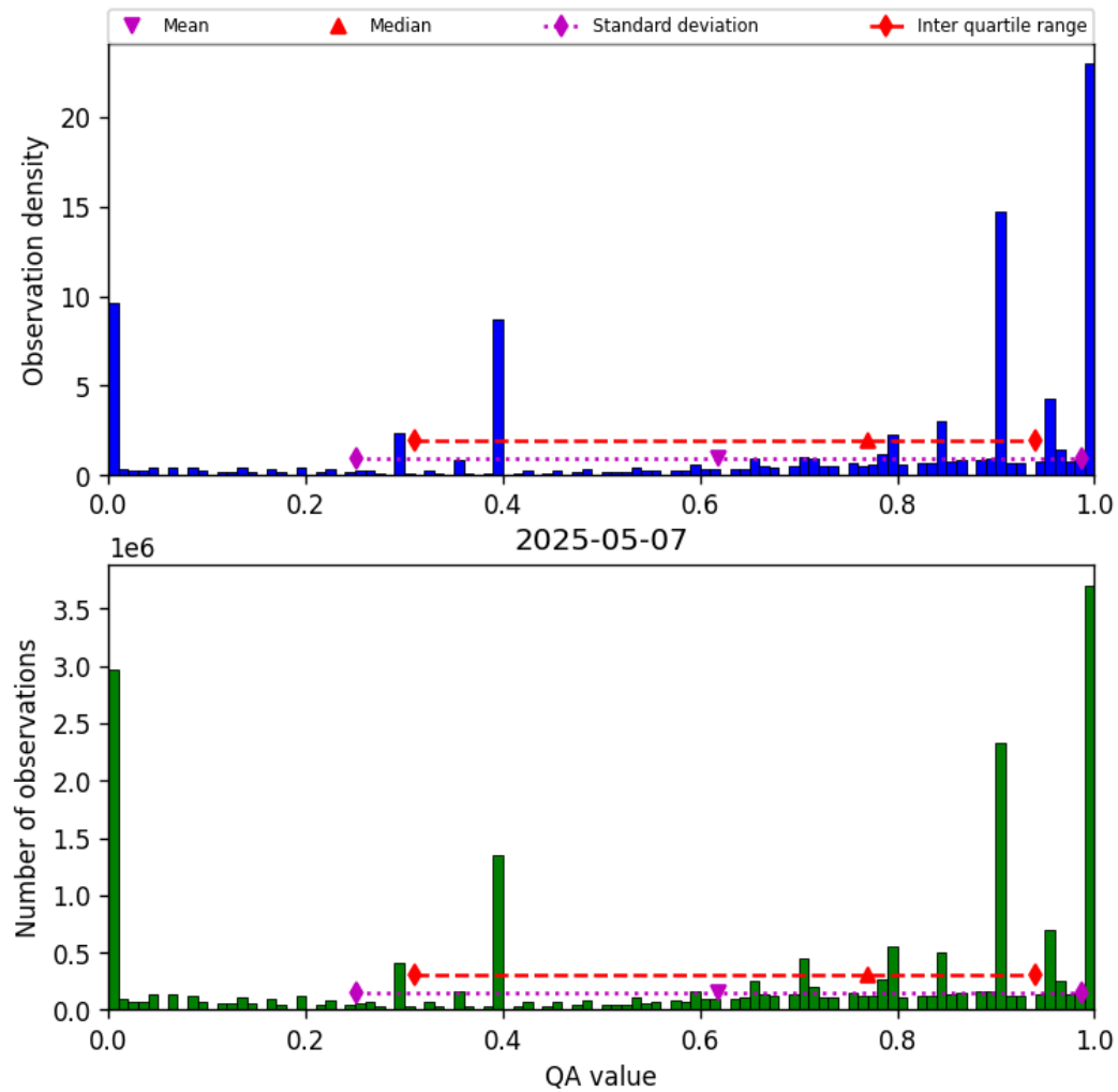
Figure 38: Histogram of “QA value” for 2025-05-06 to 2025-05-08
