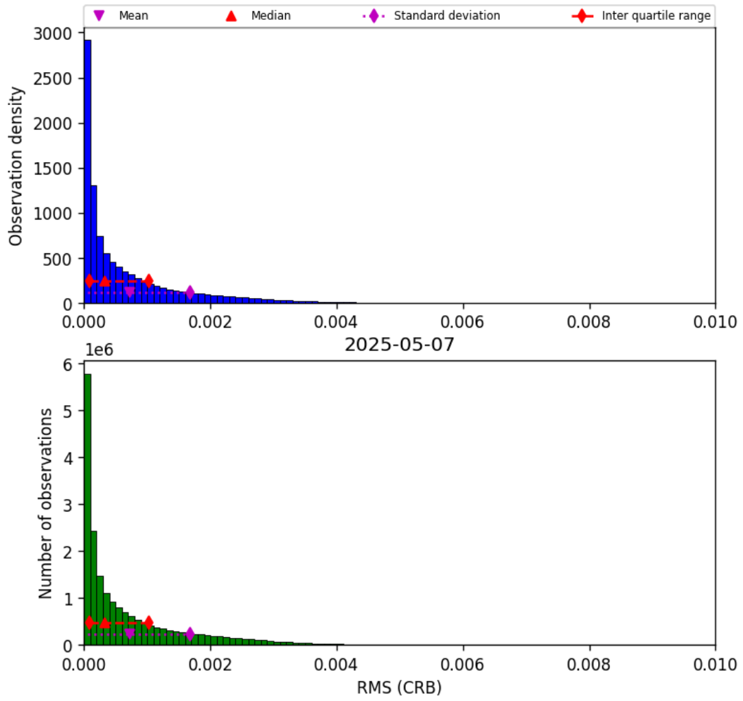
Figure 48: Histogram of “RMS (CRB)” for 2025-05-06 to 2025-05-08
