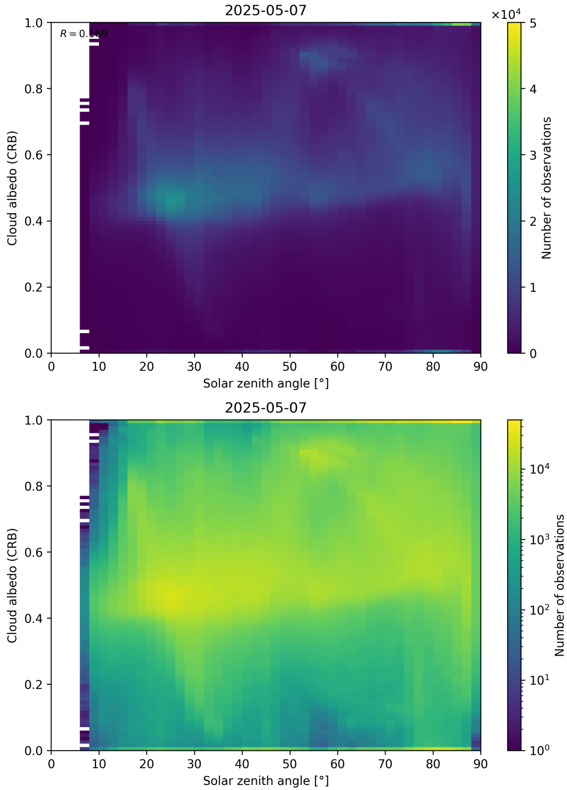
Figure 98: Scatter density plot of “Solar zenith angle” against “Cloud albedo (CRB)” for 2025-05-06 to 2025-05-08.
