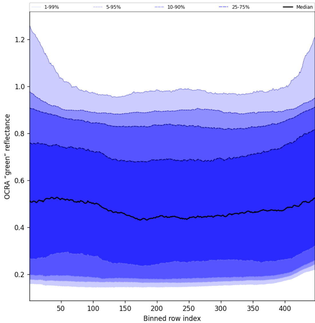
Figure 68: Along track statistics of “OCRA “green” reflectance” for 2025-05-06 to 2025-05-08
