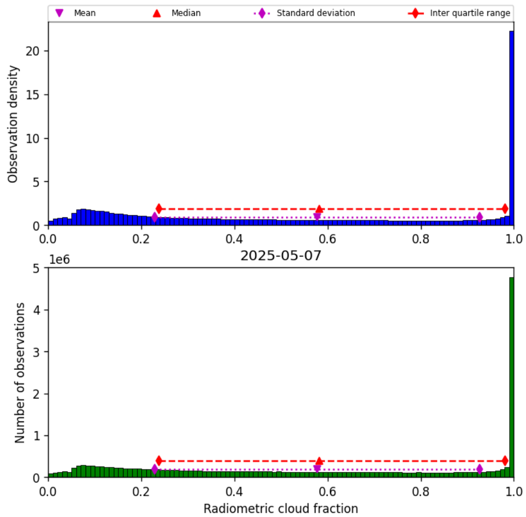
Figure 39: Histogram of “Radiometric cloud fraction” for 2025-05-06 to 2025-05-08
