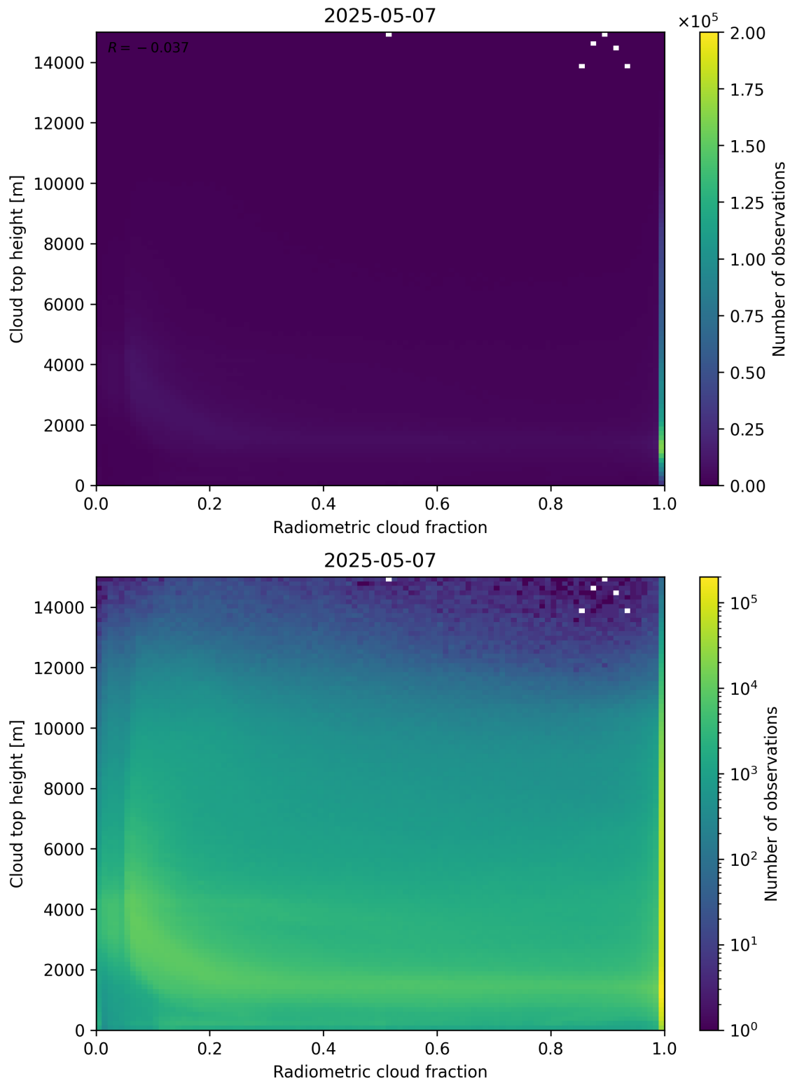
Figure 76: Scatter density plot of “Radiometric cloud fraction” against “Cloud top height” for 2025-05-06 to 2025-05-08.
