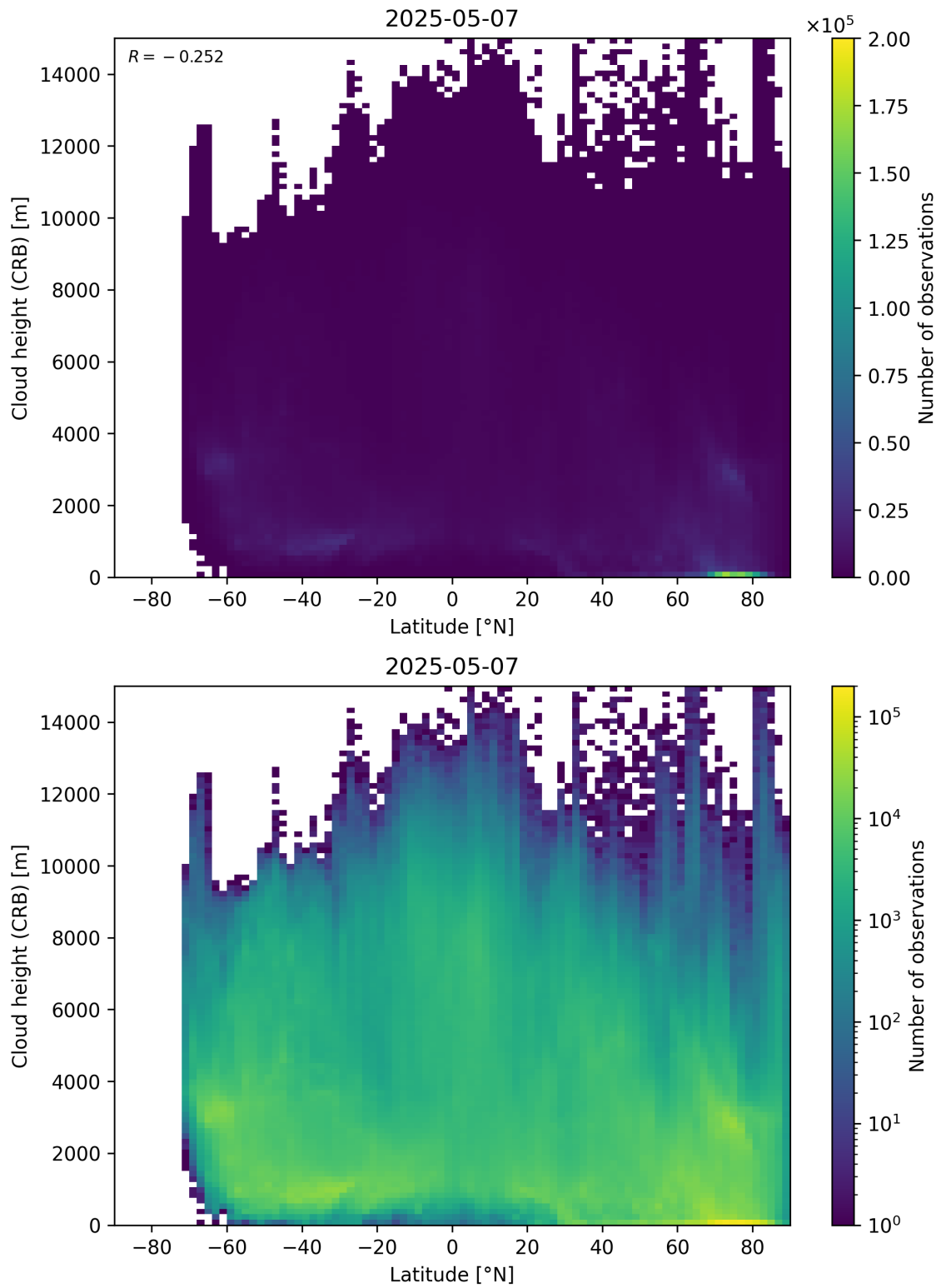
Figure 95: Scatter density plot of “Latitude” against “Cloud height (CRB)” for 2025-05-06 to 2025-05-08.
