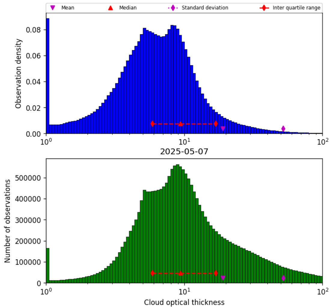
Figure 41: Histogram of “Cloud optical thickness” for 2025-05-06 to 2025-05-08
