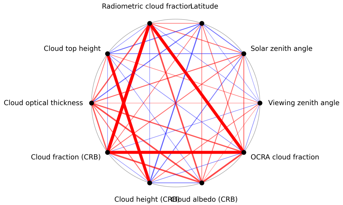
Figure 1: Map of correlation graph for 2025-05-06 to 2025-05-08.
