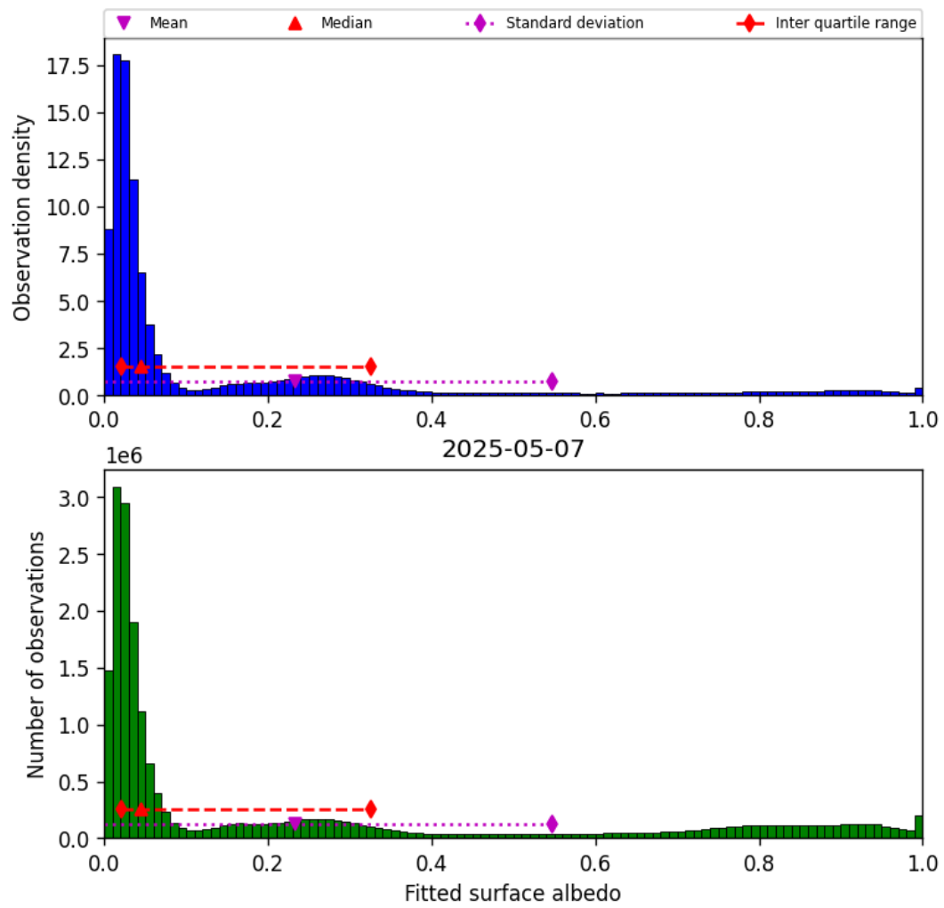
Figure 45: Histogram of “Fitted surface albedo” for 2025-05-06 to 2025-05-08
