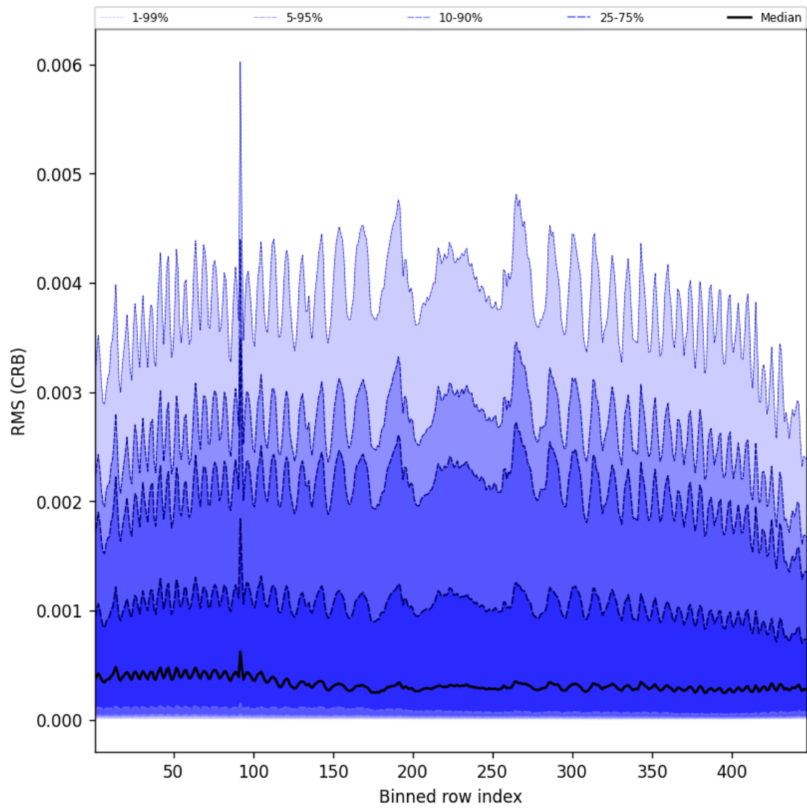
Figure 64: Along track statistics of “RMS (CRB)” for 2025-05-06 to 2025-05-08
