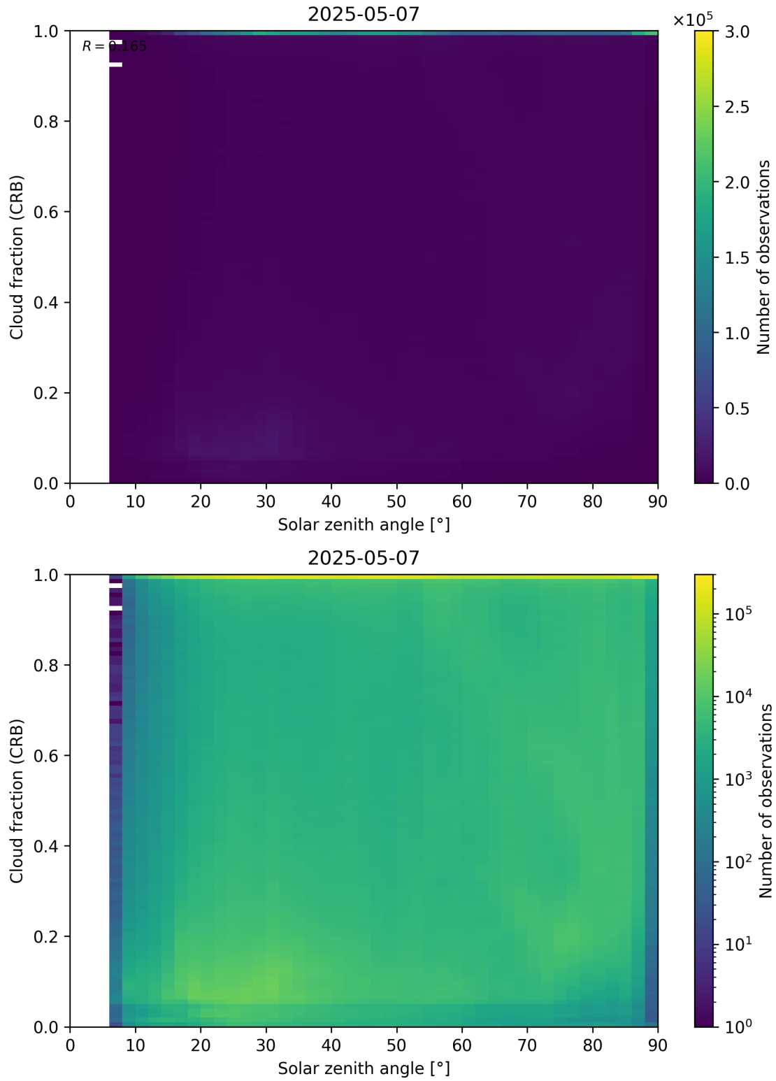
Figure 101: Scatter density plot of “Solar zenith angle” against “Cloud fraction (CRB)” for 2025-05-06 to 2025-05-08.
