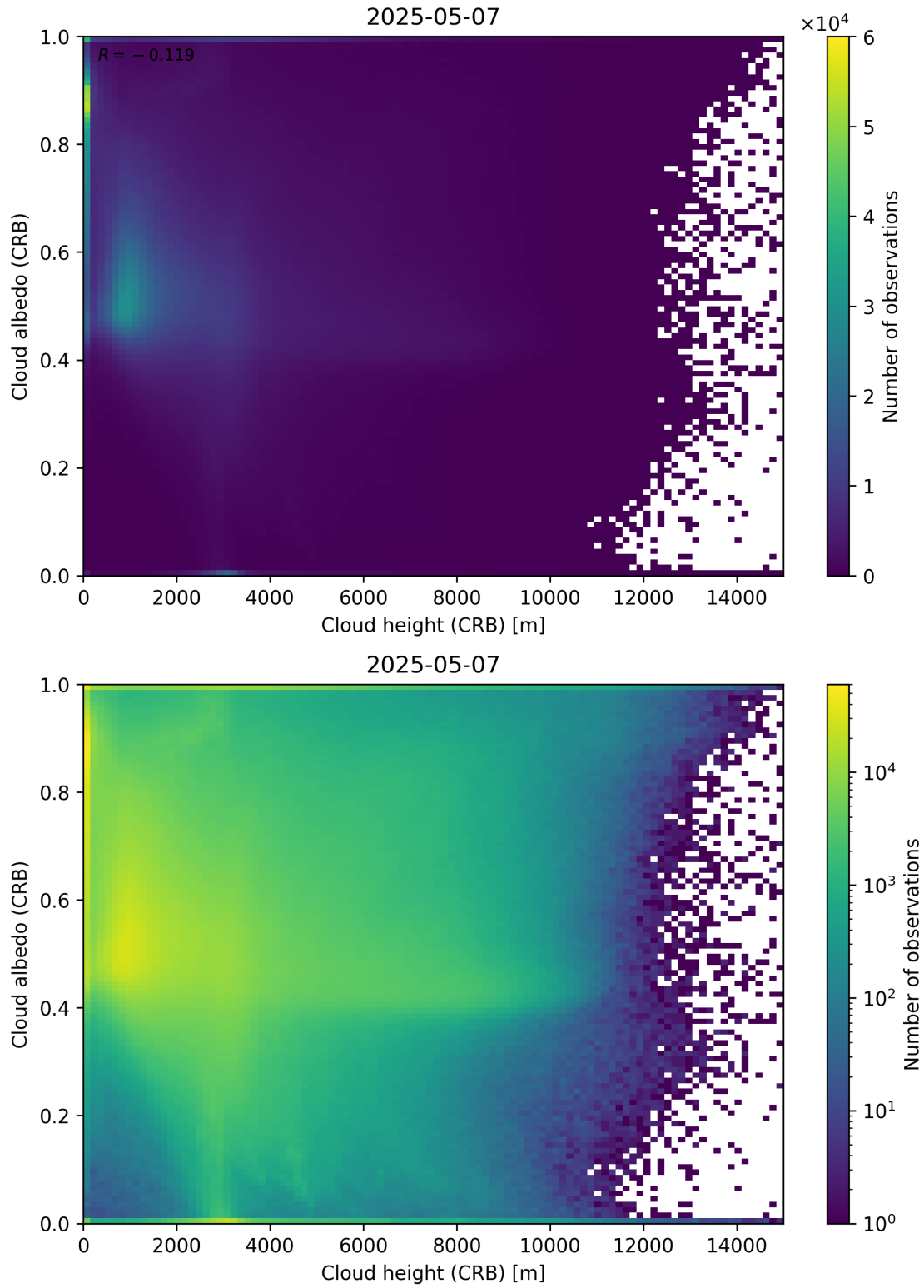
Figure 80: Scatter density plot of “Cloud height (CRB)” against “Cloud albedo (CRB)” for 2025-05-06 to 2025-05-08.
