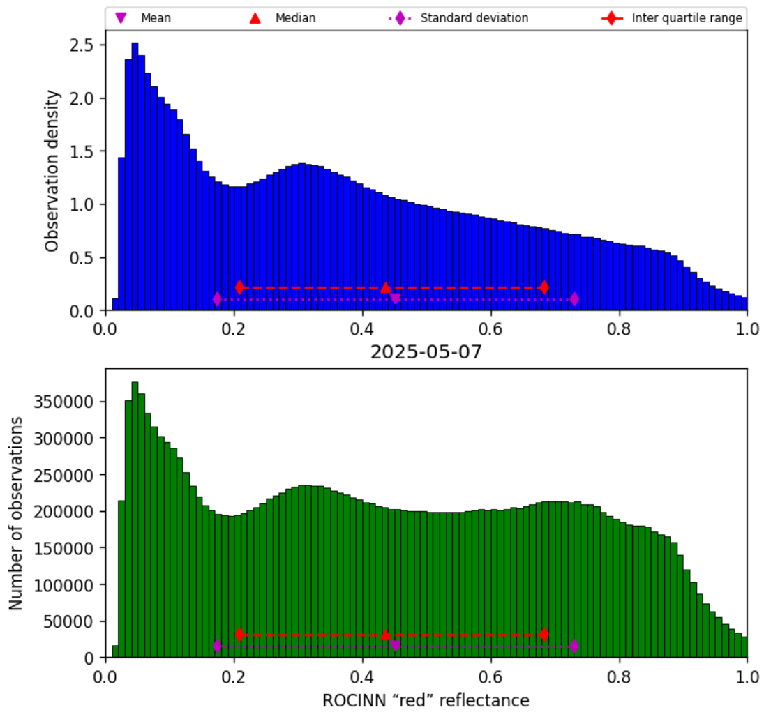
Figure 53: Histogram of “ROCINN “red” reflectance” for 2025-05-06 to 2025-05-08
