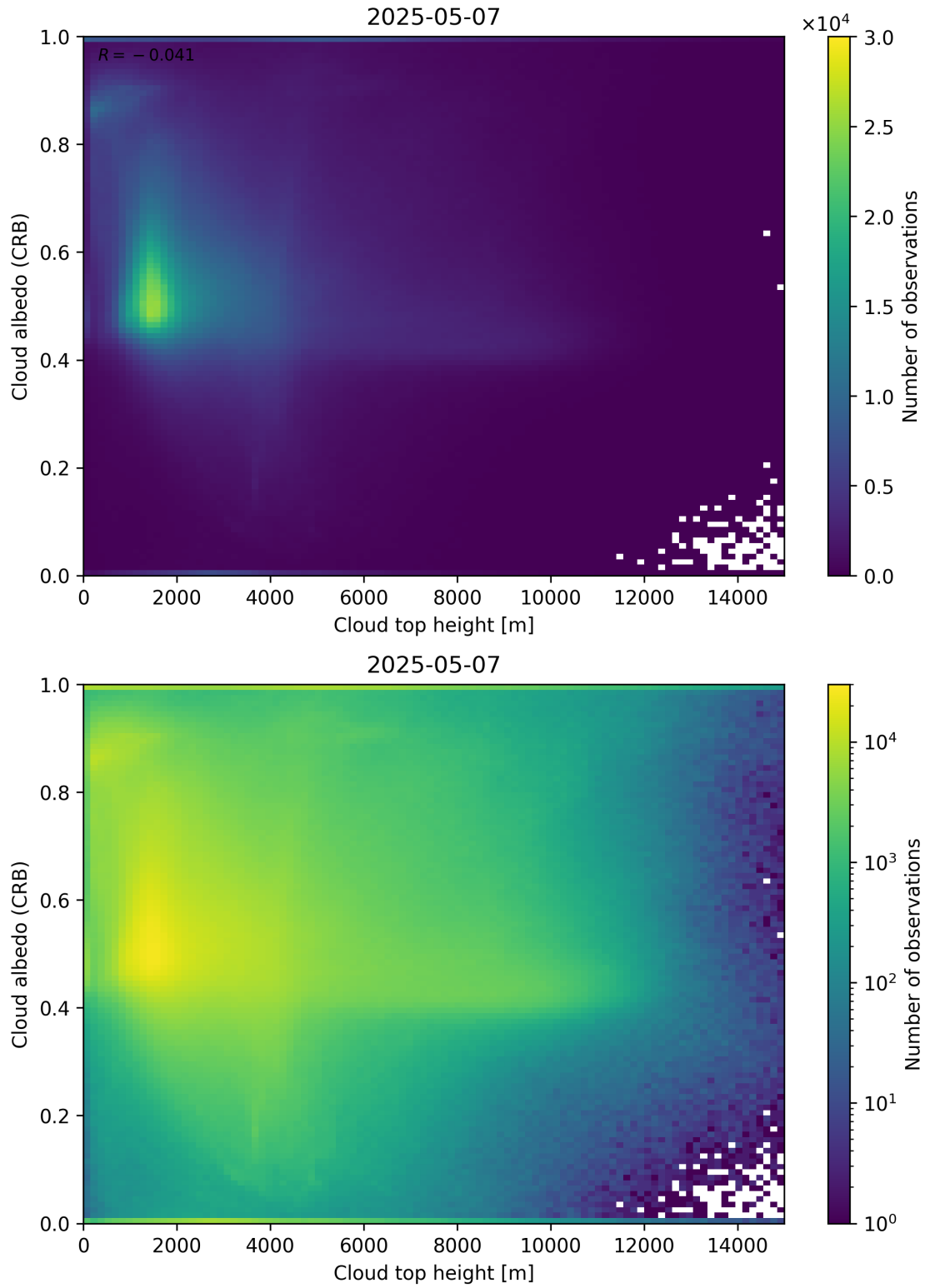
Figure 86: Scatter density plot of “Cloud top height” against “Cloud albedo (CRB)” for 2025-05-06 to 2025-05-08.
