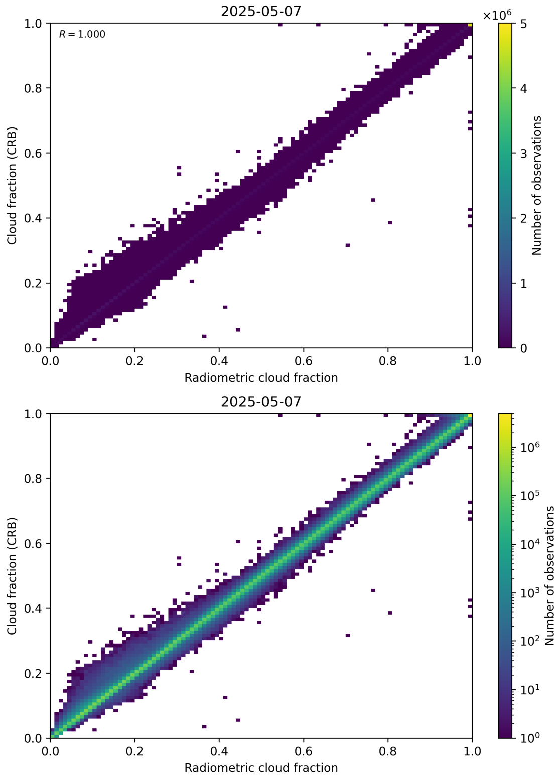
Figure 73: Scatter density plot of “Radiometric cloud fraction” against “Cloud fraction (CRB)” for 2025-05-06 to 2025-05-08.
