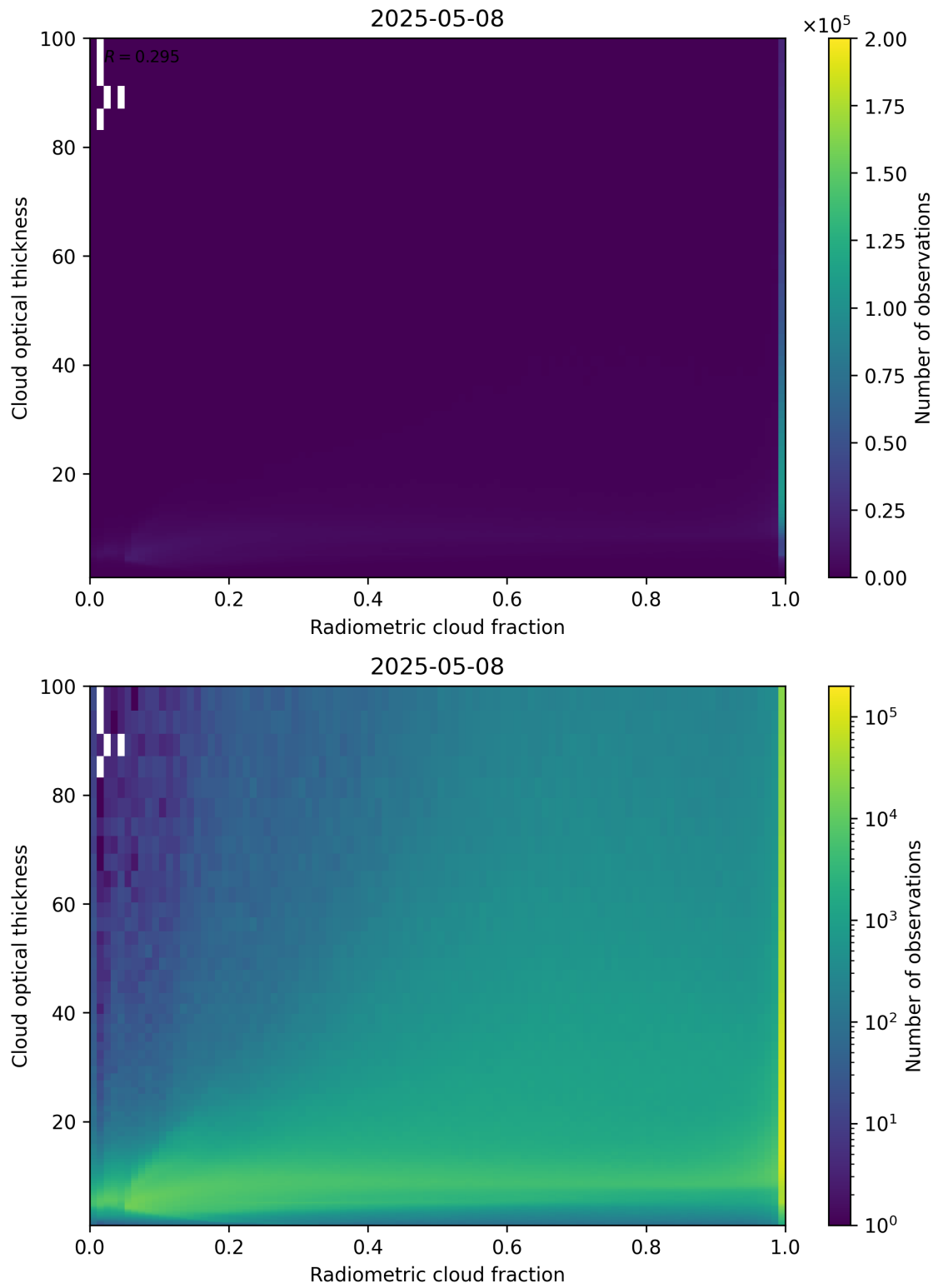
Figure 75: Scatter density plot of “Radiometric cloud fraction” against “Cloud optical thickness” for 2025-05-07 to 2025-05-09.
