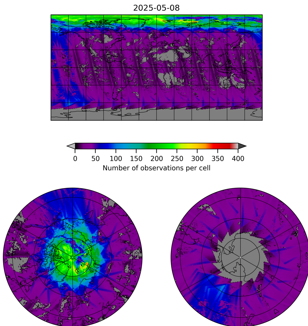
Figure 21: Map of the number of observations for 2025-05-07 to 2025-05-09
