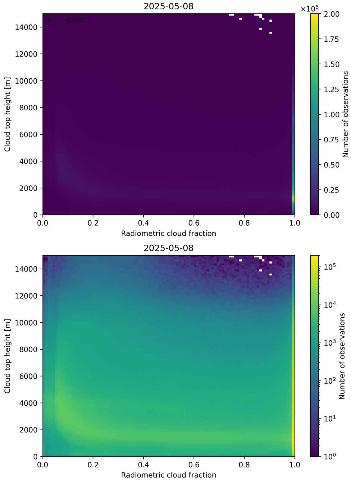
Figure 76: Scatter density plot of “Radiometric cloud fraction” against “Cloud top height” for 2025-05-07 to 2025-05-09.
