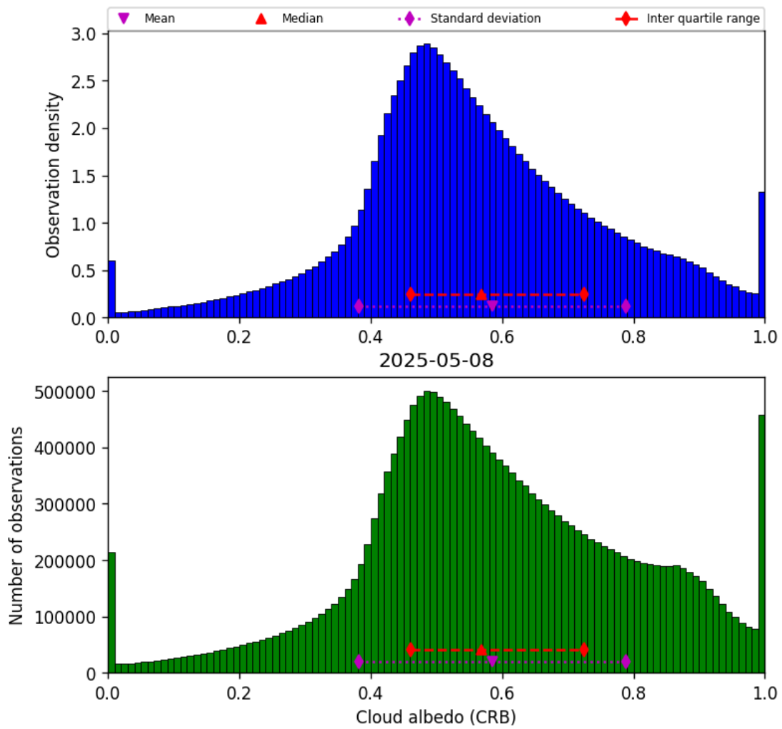
Figure 44: Histogram of “Cloud albedo (CRB)” for 2025-05-07 to 2025-05-09
