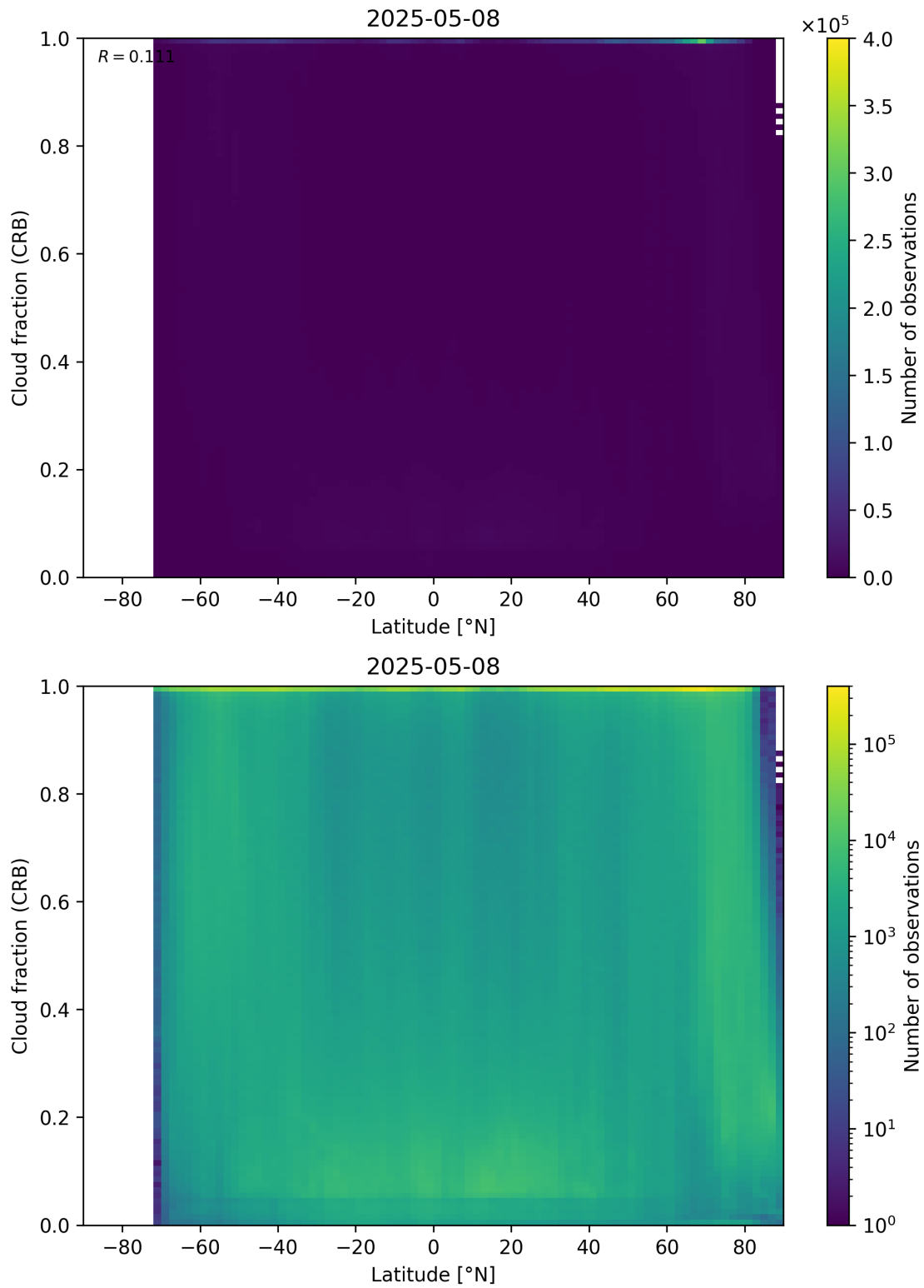
Figure 94: Scatter density plot of “Latitude” against “Cloud fraction (CRB)” for 2025-05-07 to 2025-05-09.
