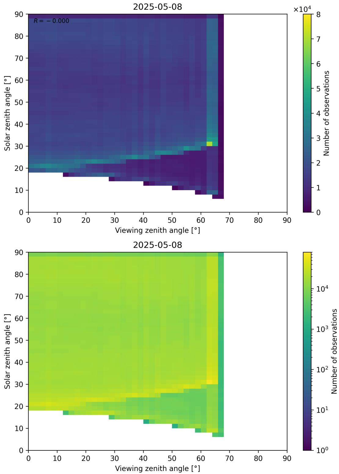
Figure 114: Scatter density plot of “Viewing zenith angle” against “Solar zenith angle” for 2025-05-07 to 2025-05-09.
