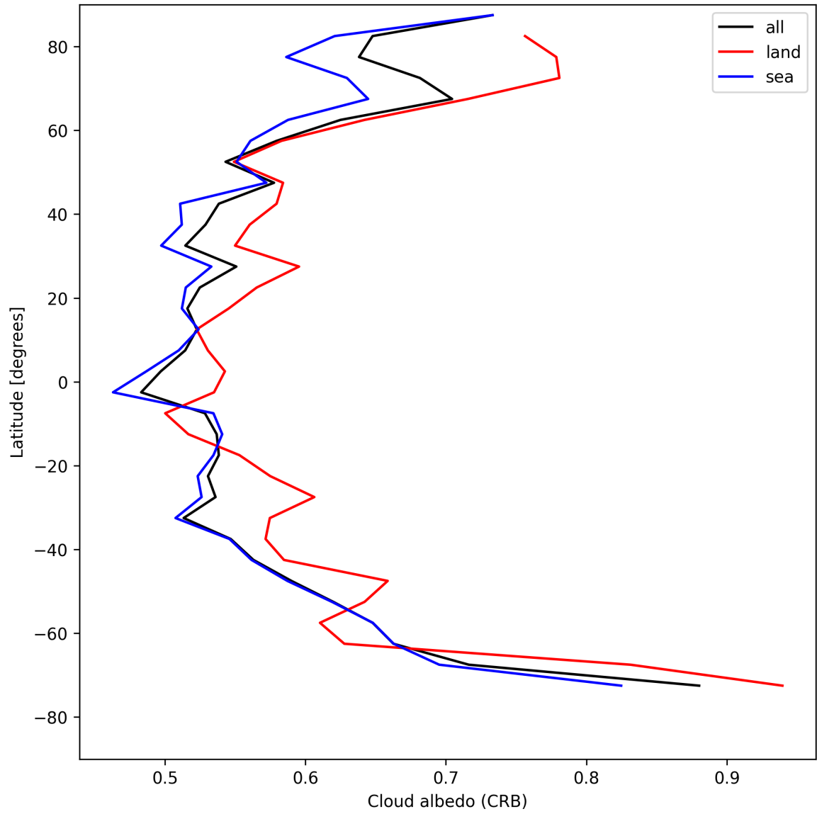
Figure 28: Zonal average of “Cloud albedo (CRB)” for 2025-05-07 to 2025-05-09.
