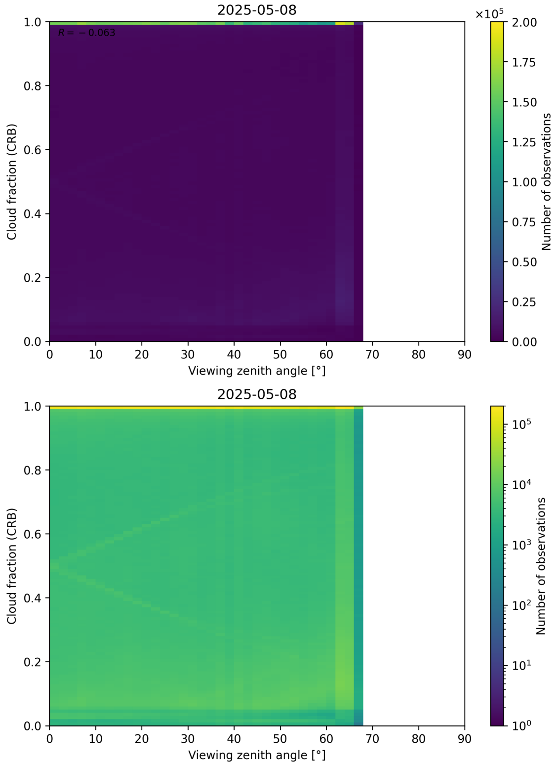
Figure 109: Scatter density plot of “Viewing zenith angle” against “Cloud fraction (CRB)” for 2025-05-07 to 2025-05-09.
