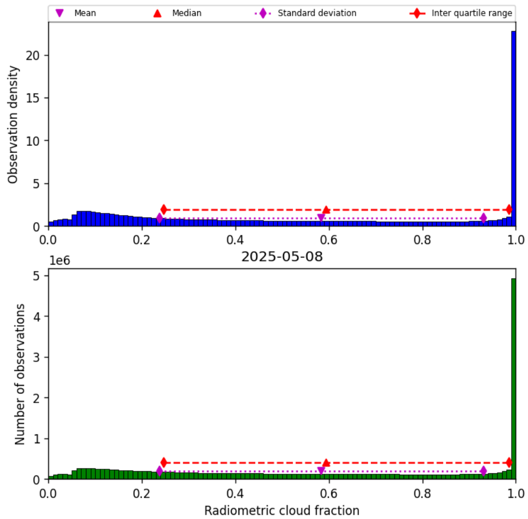
Figure 39: Histogram of “Radiometric cloud fraction” for 2025-05-07 to 2025-05-09
