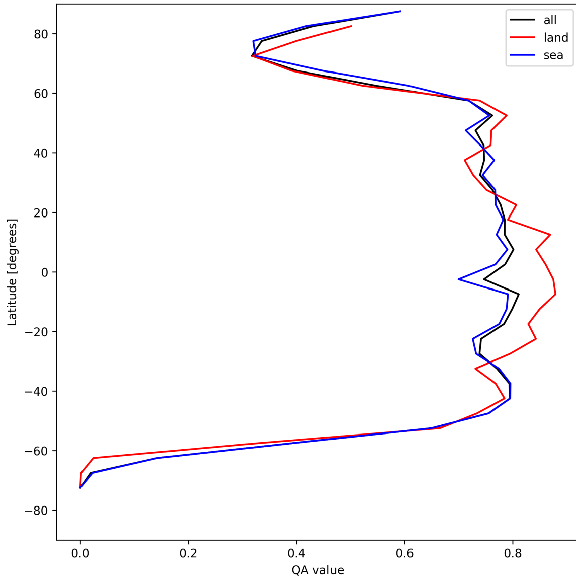
Figure 22: Zonal average of “QA value” for 2025-05-07 to 2025-05-09.
