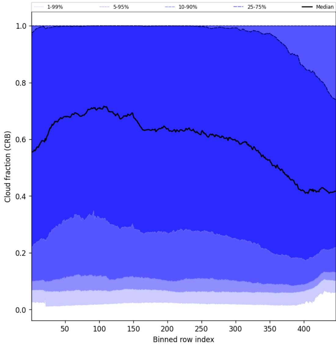
Figure 58: Along track statistics of “Cloud fraction (CRB)” for 2025-05-07 to 2025-05-09
