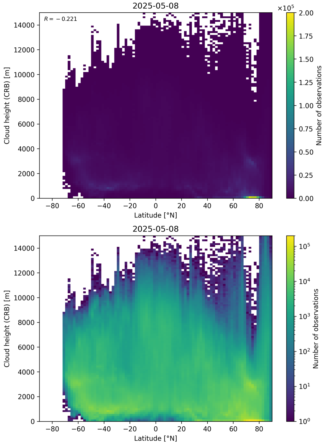
Figure 95: Scatter density plot of “Latitude” against “Cloud height (CRB)” for 2025-05-07 to 2025-05-09.
