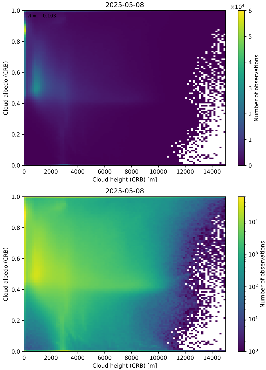
Figure 80: Scatter density plot of “Cloud height (CRB)” against “Cloud albedo (CRB)” for 2025-05-07 to 2025-05-09.
