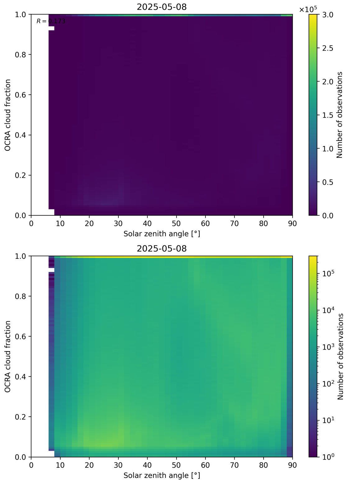
Figure 100: Scatter density plot of “Solar zenith angle” against “OCRA cloud fraction” for 2025-05-07 to 2025-05-09.
