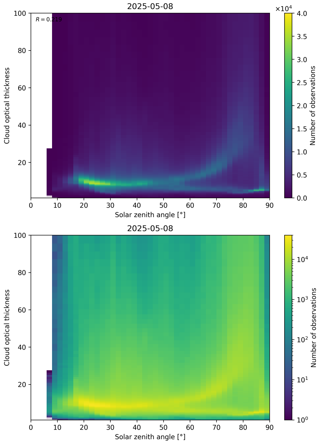
Figure 103: Scatter density plot of “Solar zenith angle” against “Cloud optical thickness” for 2025-05-07 to 2025-05-09.
