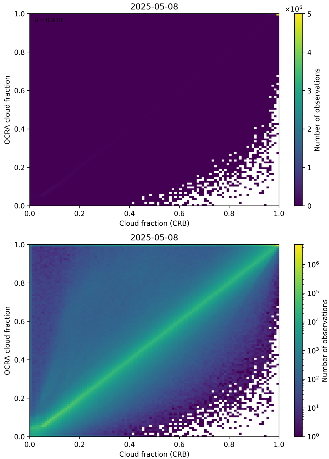
Figure 78: Scatter density plot of “Cloud fraction (CRB)” against “OCRA cloud fraction” for 2025-05-07 to 2025-05-09.
