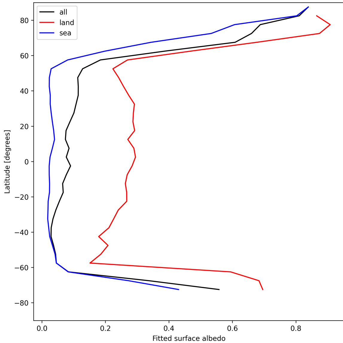
Figure 29: Zonal average of “Fitted surface albedo” for 2025-05-07 to 2025-05-09.
