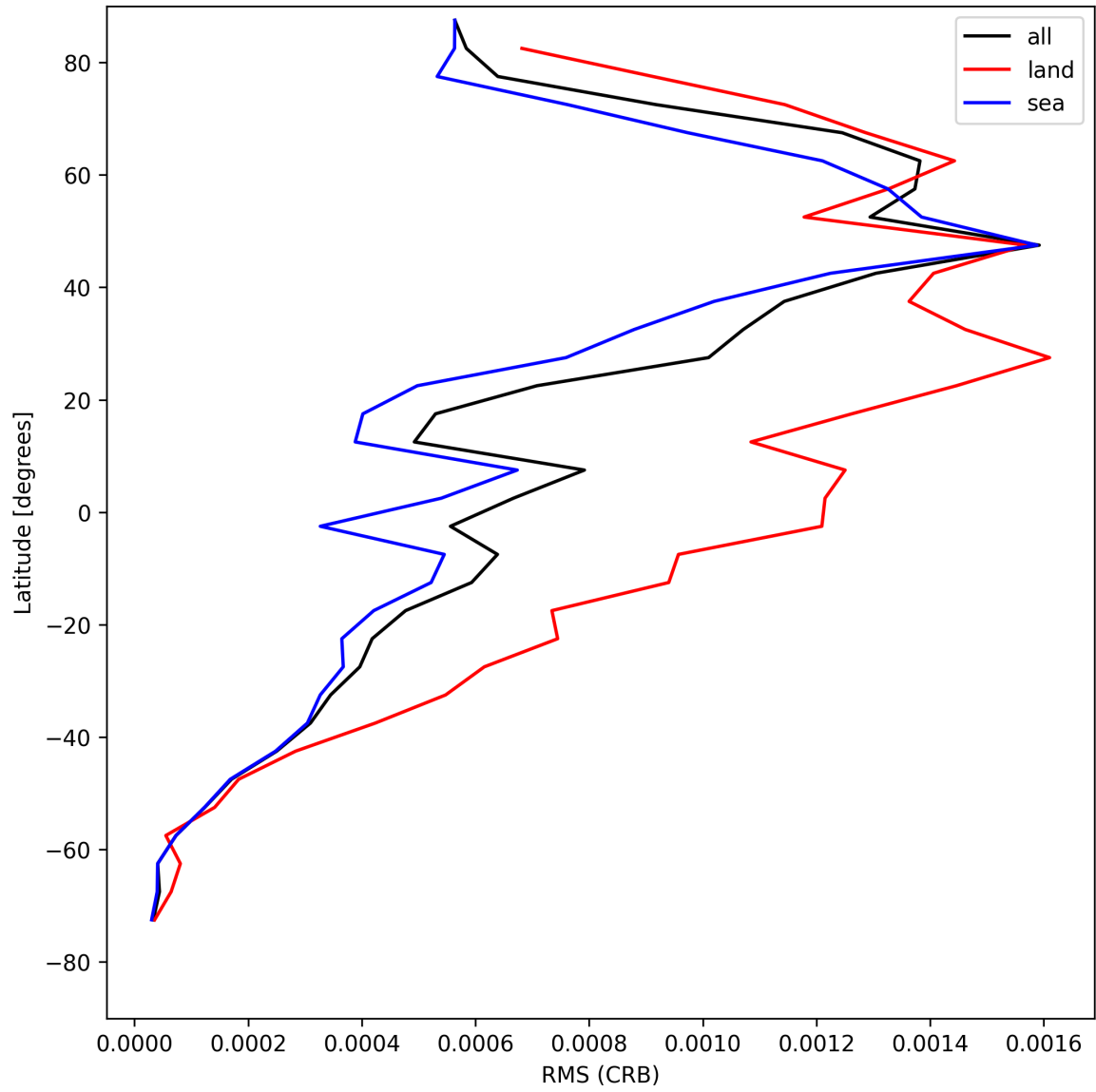
Figure 32: Zonal average of “RMS (CRB)” for 2025-05-07 to 2025-05-09.
