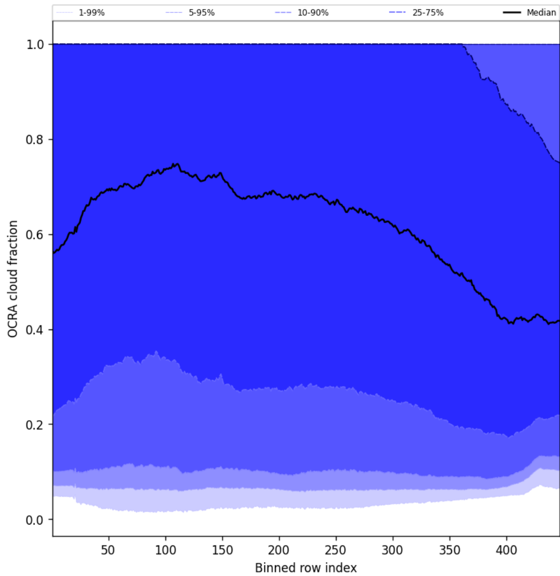
Figure 66: Along track statistics of “OCRA cloud fraction” for 2025-05-07 to 2025-05-09
