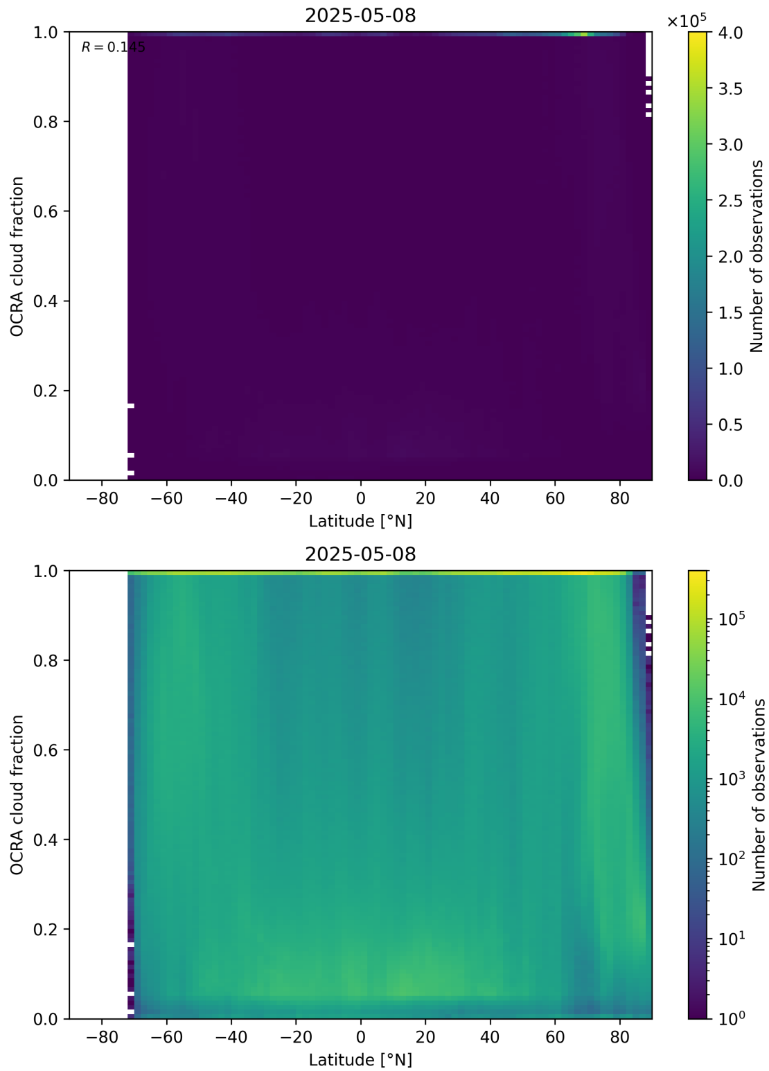
Figure 93: Scatter density plot of “Latitude” against “OCRA cloud fraction” for 2025-05-07 to 2025-05-09.
