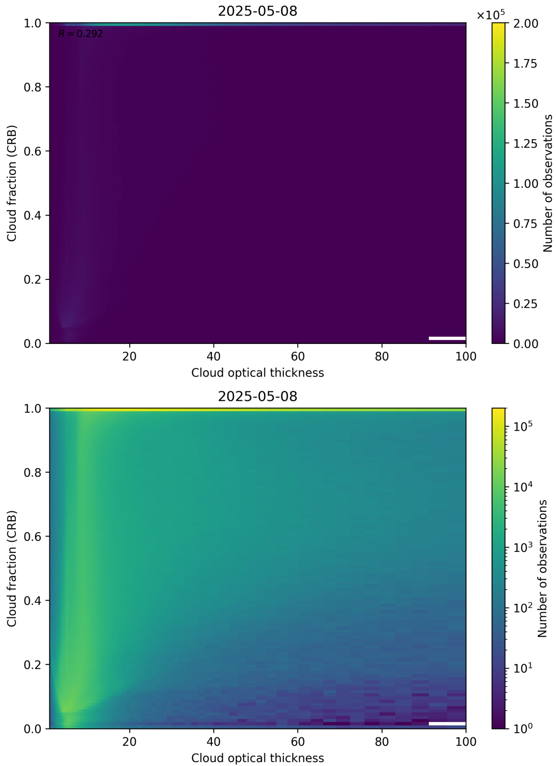
Figure 84: Scatter density plot of “Cloud optical thickness” against “Cloud fraction (CRB)” for 2025-05-07 to 2025-05-09.
