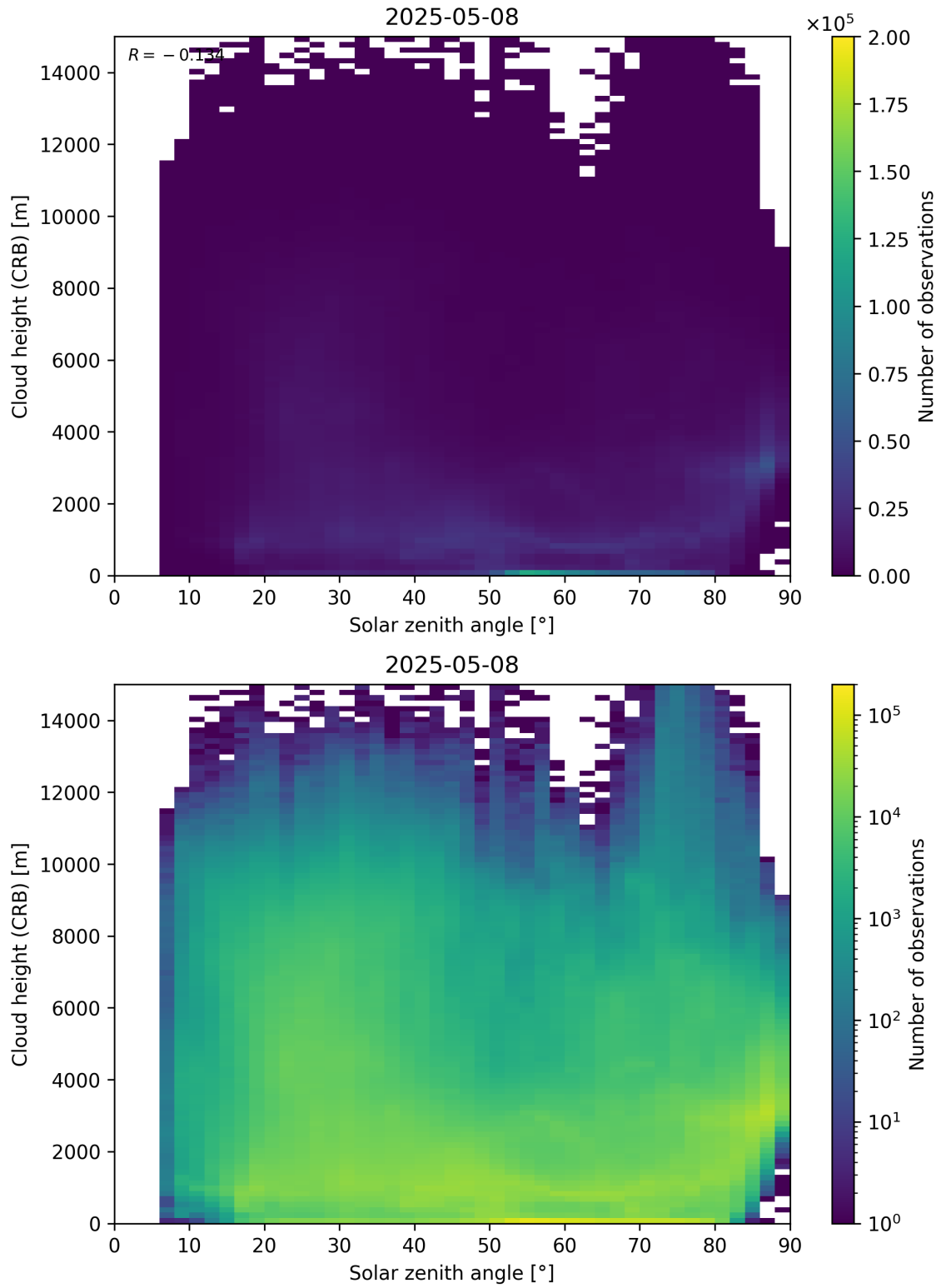
Figure 102: Scatter density plot of “Solar zenith angle” against “Cloud height (CRB)” for 2025-05-07 to 2025-05-09.
