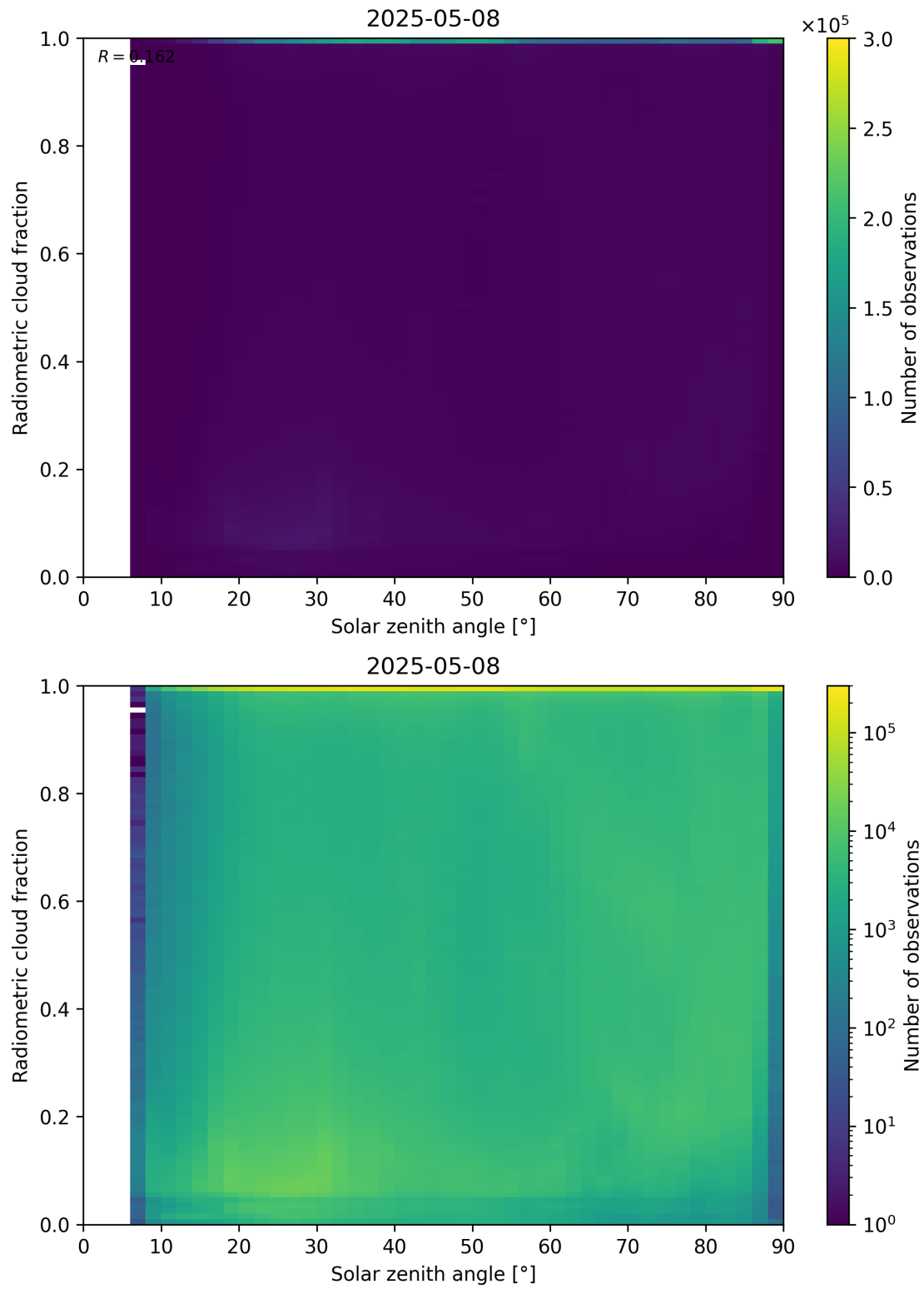
Figure 99: Scatter density plot of “Solar zenith angle” against “Radiometric cloud fraction” for 2025-05-07 to 2025-05-09.
