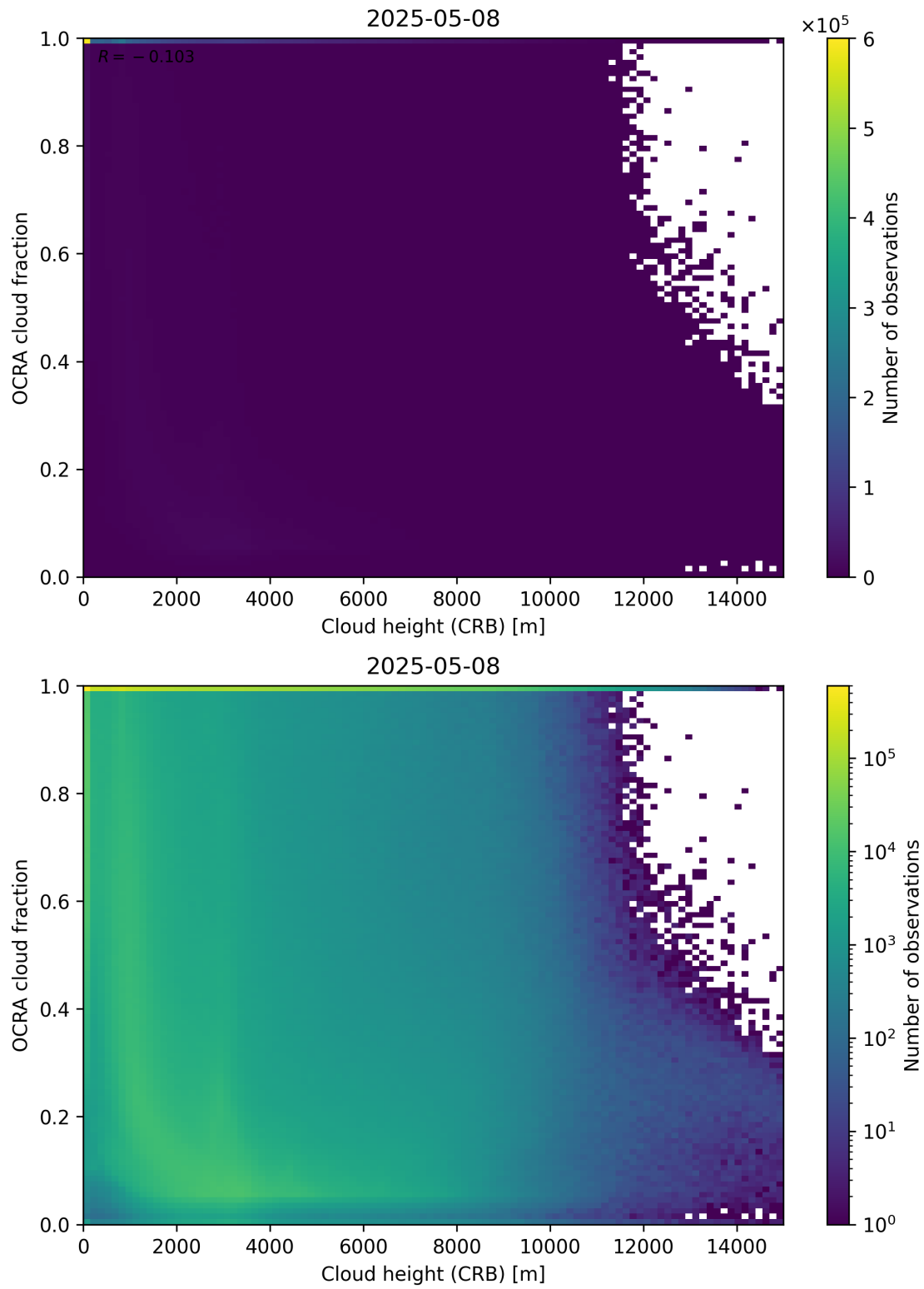
Figure 81: Scatter density plot of “Cloud height (CRB)” against “OCRA cloud fraction” for 2025-05-07 to 2025-05-09.
