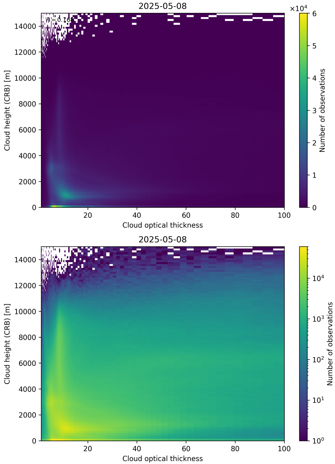
Figure 85: Scatter density plot of “Cloud optical thickness” against “Cloud height (CRB)” for 2025-05-07 to 2025-05-09.
