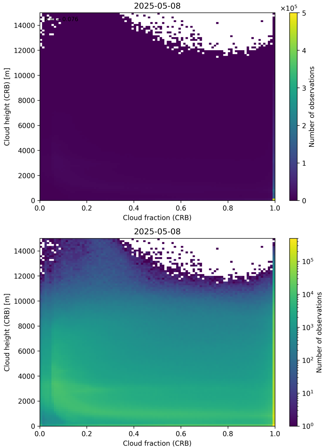
Figure 79: Scatter density plot of “Cloud fraction (CRB)” against “Cloud height (CRB)” for 2025-05-07 to 2025-05-09.
