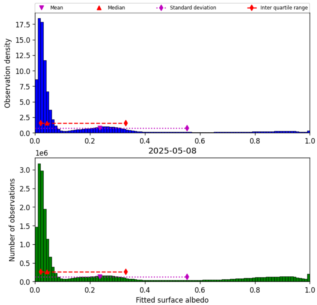
Figure 45: Histogram of “Fitted surface albedo” for 2025-05-07 to 2025-05-09
