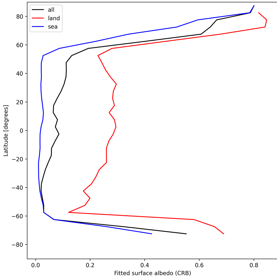
Figure 30: Zonal average of “Fitted surface albedo (CRB)” for 2025-05-07 to 2025-05-09.
