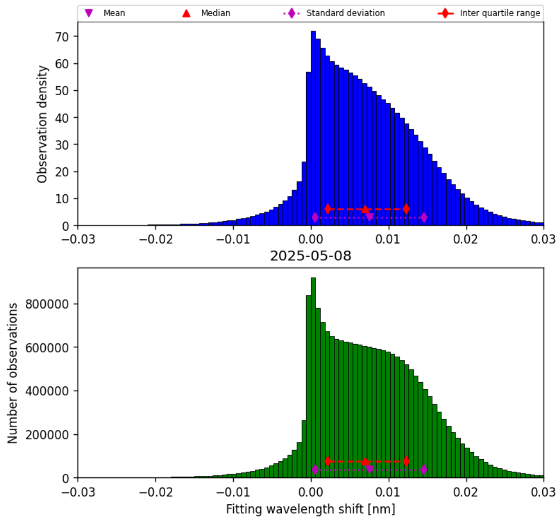
Figure 49: Histogram of “Fitting wavelength shift” for 2025-05-07 to 2025-05-09
