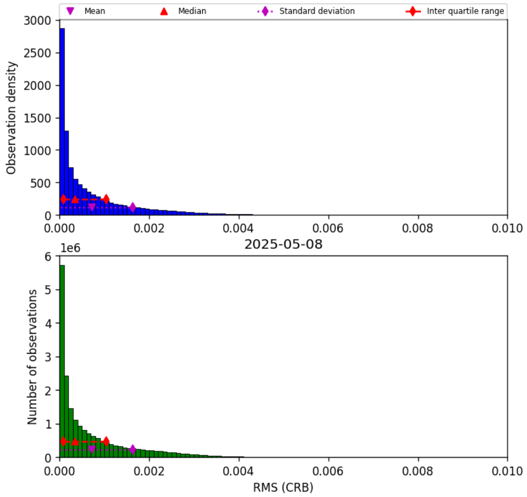
Figure 48: Histogram of “RMS (CRB)” for 2025-05-07 to 2025-05-09
