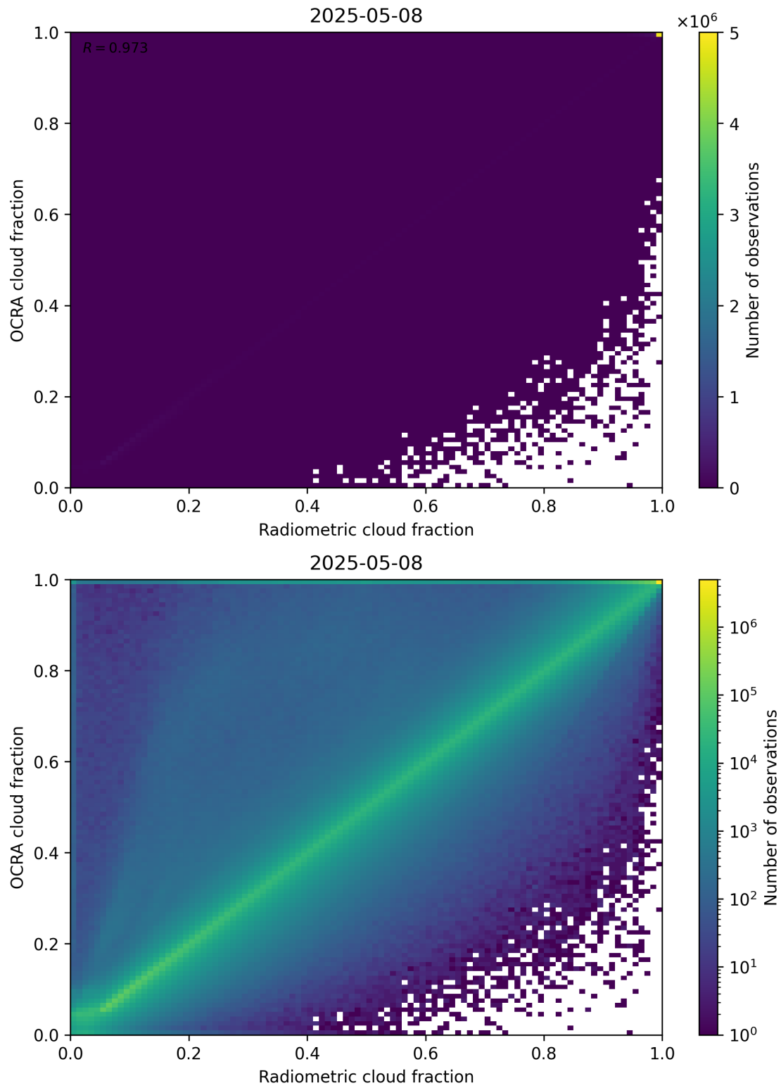
Figure 72: Scatter density plot of “Radiometric cloud fraction” against “OCRA cloud fraction” for 2025-05-07 to 2025-05-09.
