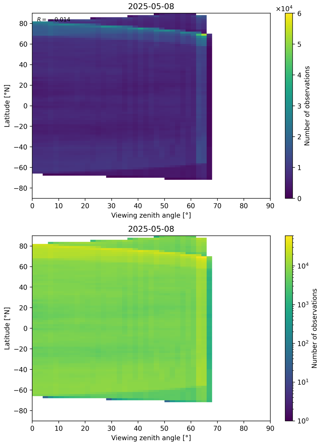
Figure 113: Scatter density plot of “Viewing zenith angle” against “Latitude” for 2025-05-07 to 2025-05-09.
