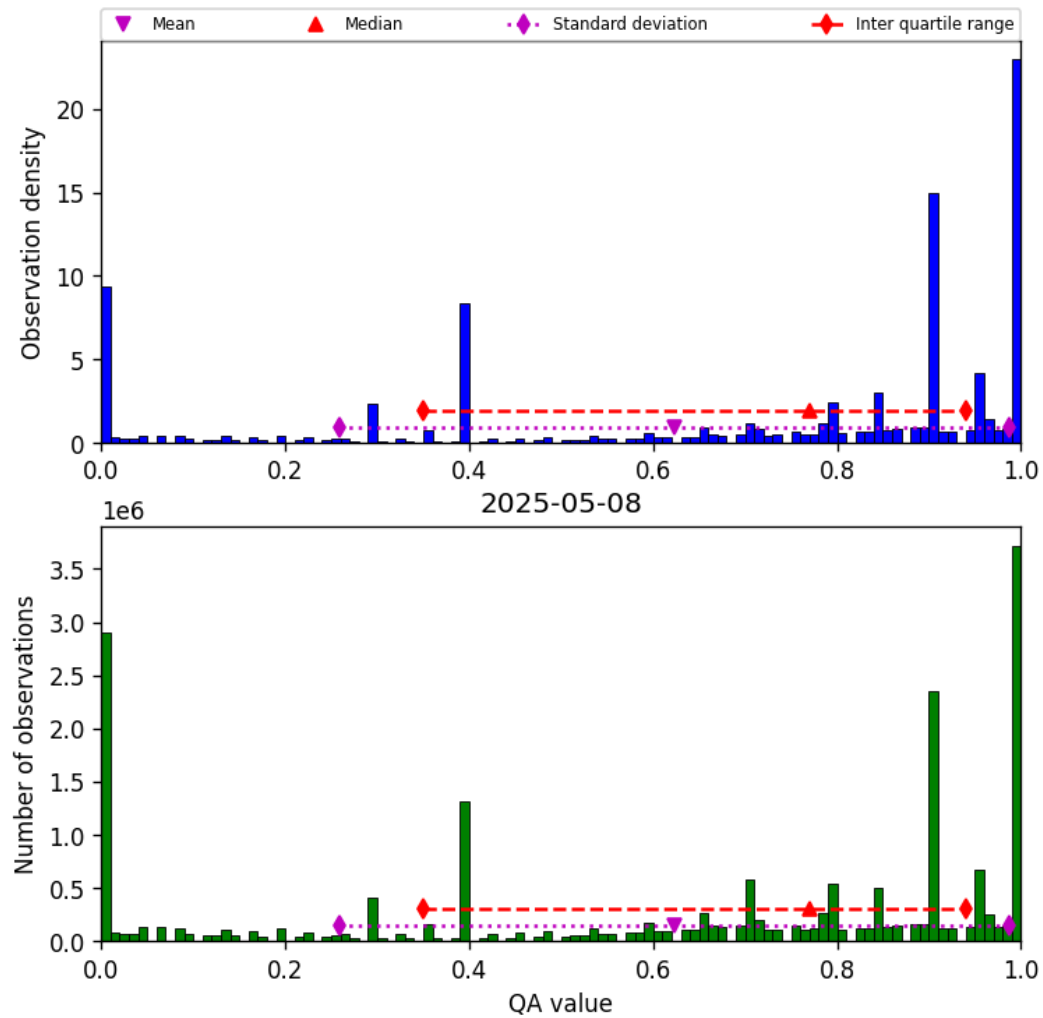
Figure 38: Histogram of “QA value” for 2025-05-07 to 2025-05-09
