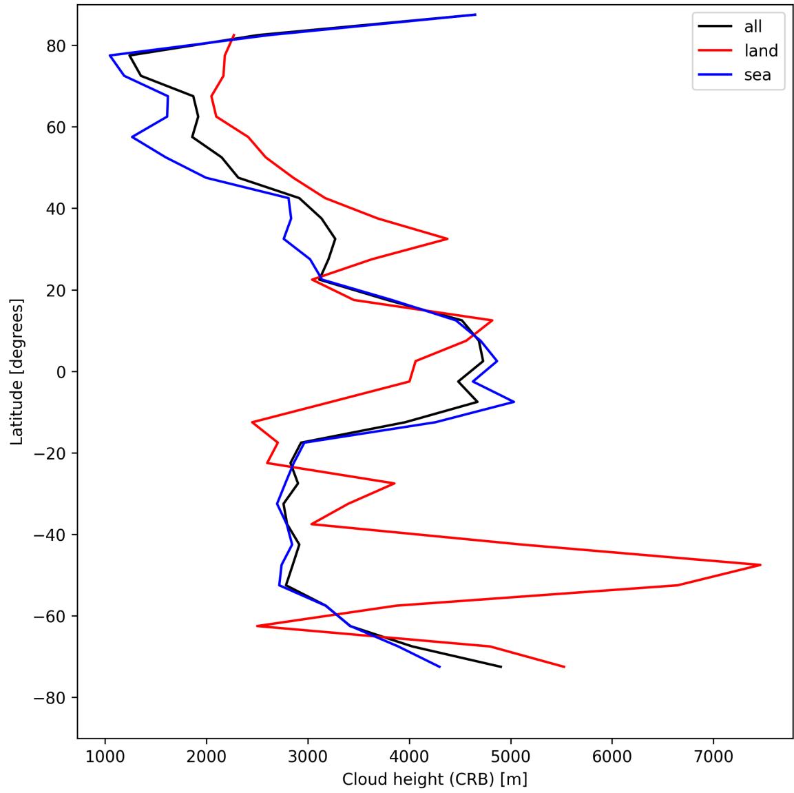
Figure 27: Zonal average of “Cloud height (CRB)” for 2025-05-07 to 2025-05-09.
