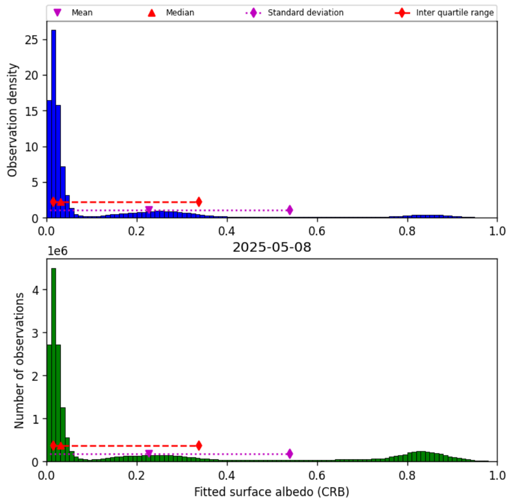
Figure 46: Histogram of “Fitted surface albedo (CRB)” for 2025-05-07 to 2025-05-09
