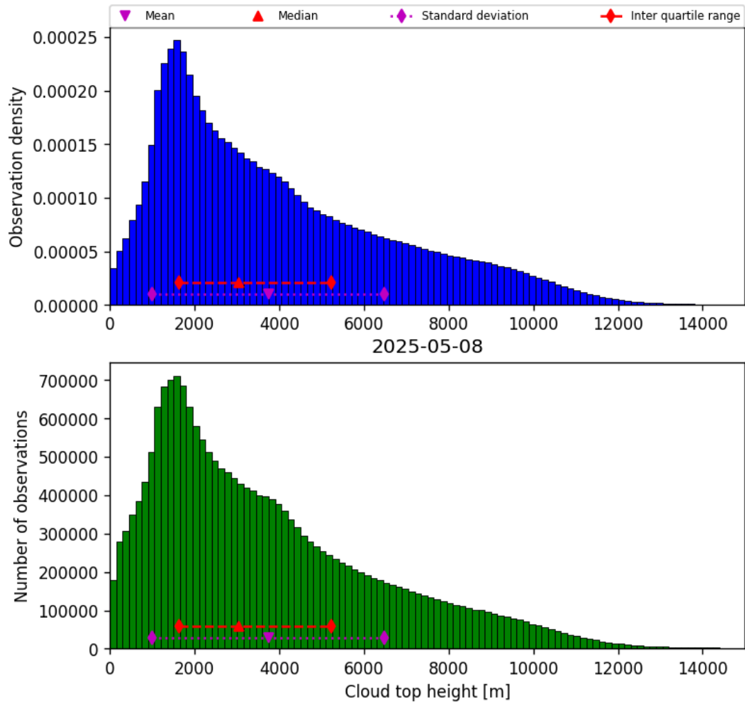
Figure 40: Histogram of “Cloud top height” for 2025-05-07 to 2025-05-09
