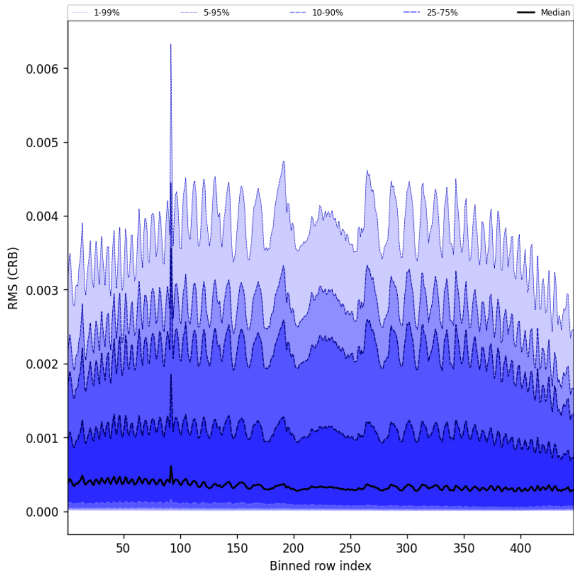
Figure 64: Along track statistics of “RMS (CRB)” for 2025-05-07 to 2025-05-09
