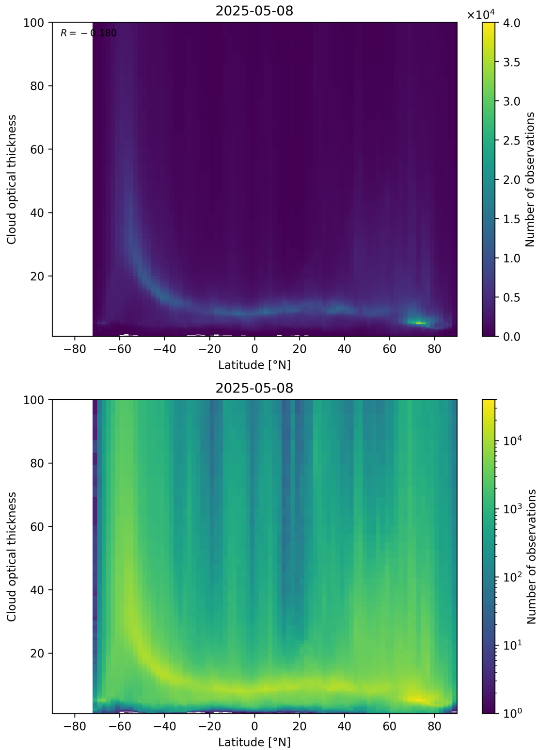
Figure 96: Scatter density plot of “Latitude” against “Cloud optical thickness” for 2025-05-07 to 2025-05-09.
