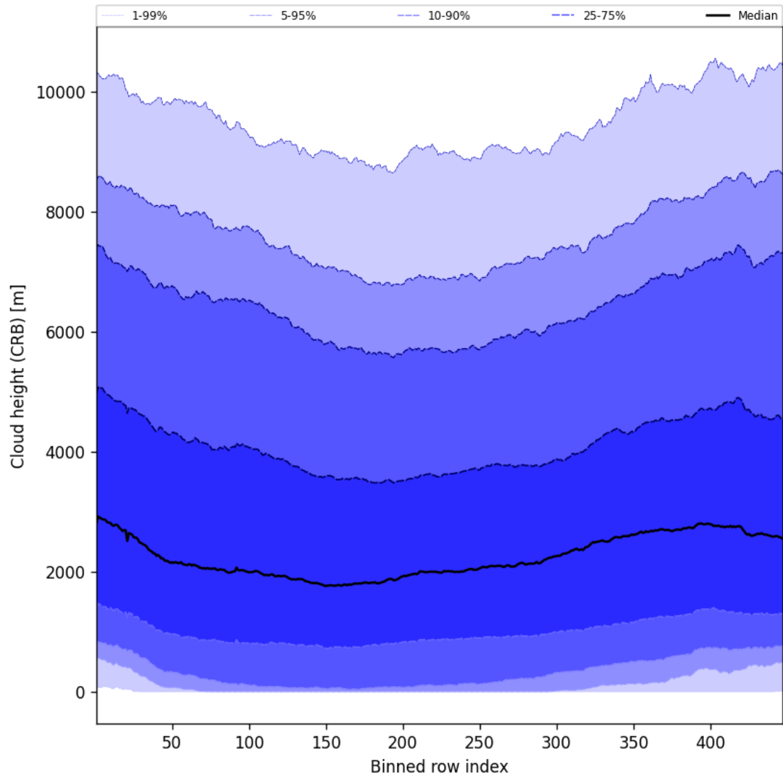
Figure 59: Along track statistics of “Cloud height (CRB)” for 2025-05-07 to 2025-05-09
