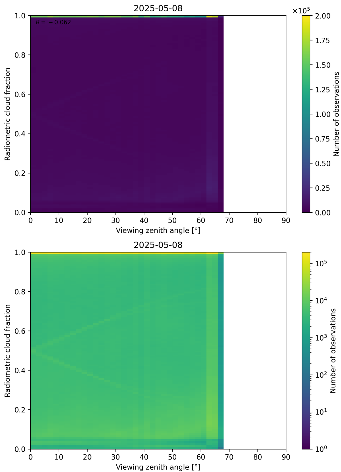
Figure 107: Scatter density plot of “Viewing zenith angle” against “Radiometric cloud fraction” for 2025-05-07 to 2025-05-09.
