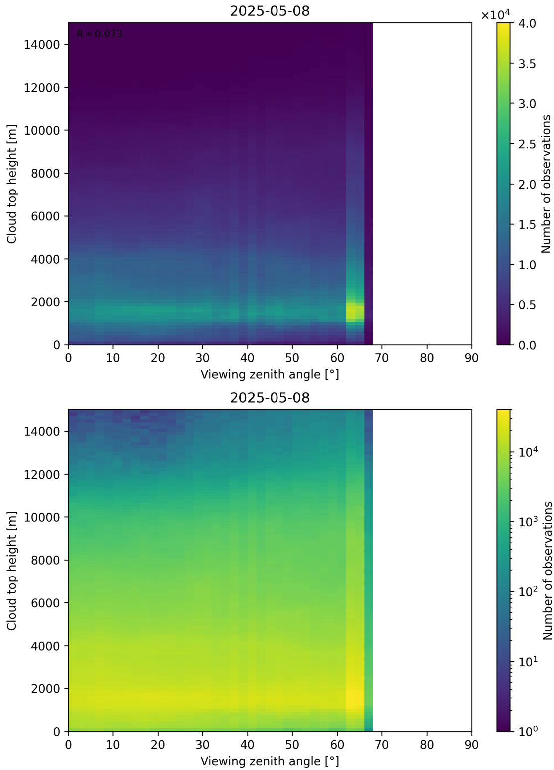
Figure 112: Scatter density plot of “Viewing zenith angle” against “Cloud top height” for 2025-05-07 to 2025-05-09.
