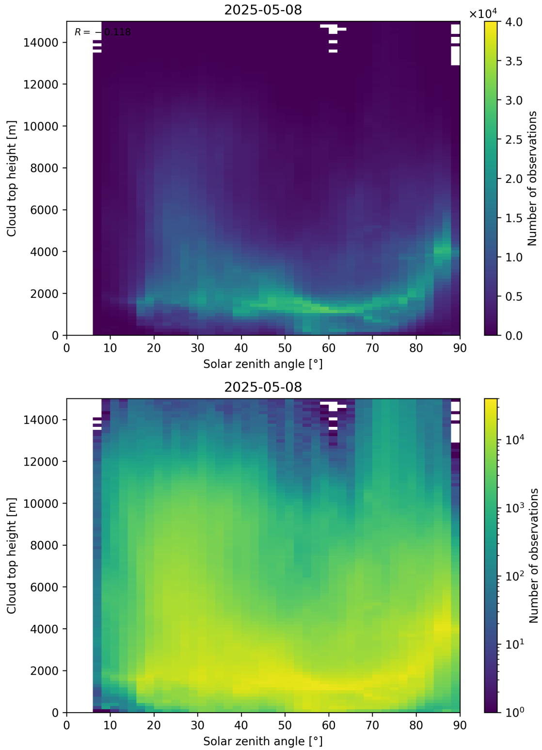
Figure 104: Scatter density plot of “Solar zenith angle” against “Cloud top height” for 2025-05-07 to 2025-05-09.
