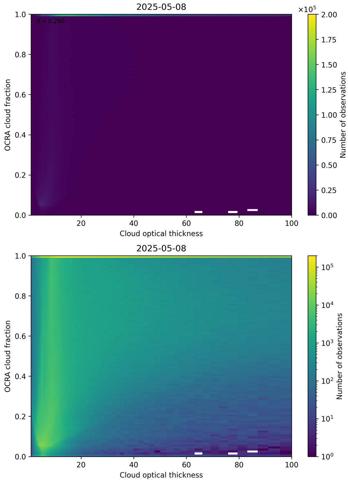
Figure 83: Scatter density plot of “Cloud optical thickness” against “OCRA cloud fraction” for 2025-05-07 to 2025-05-09.
