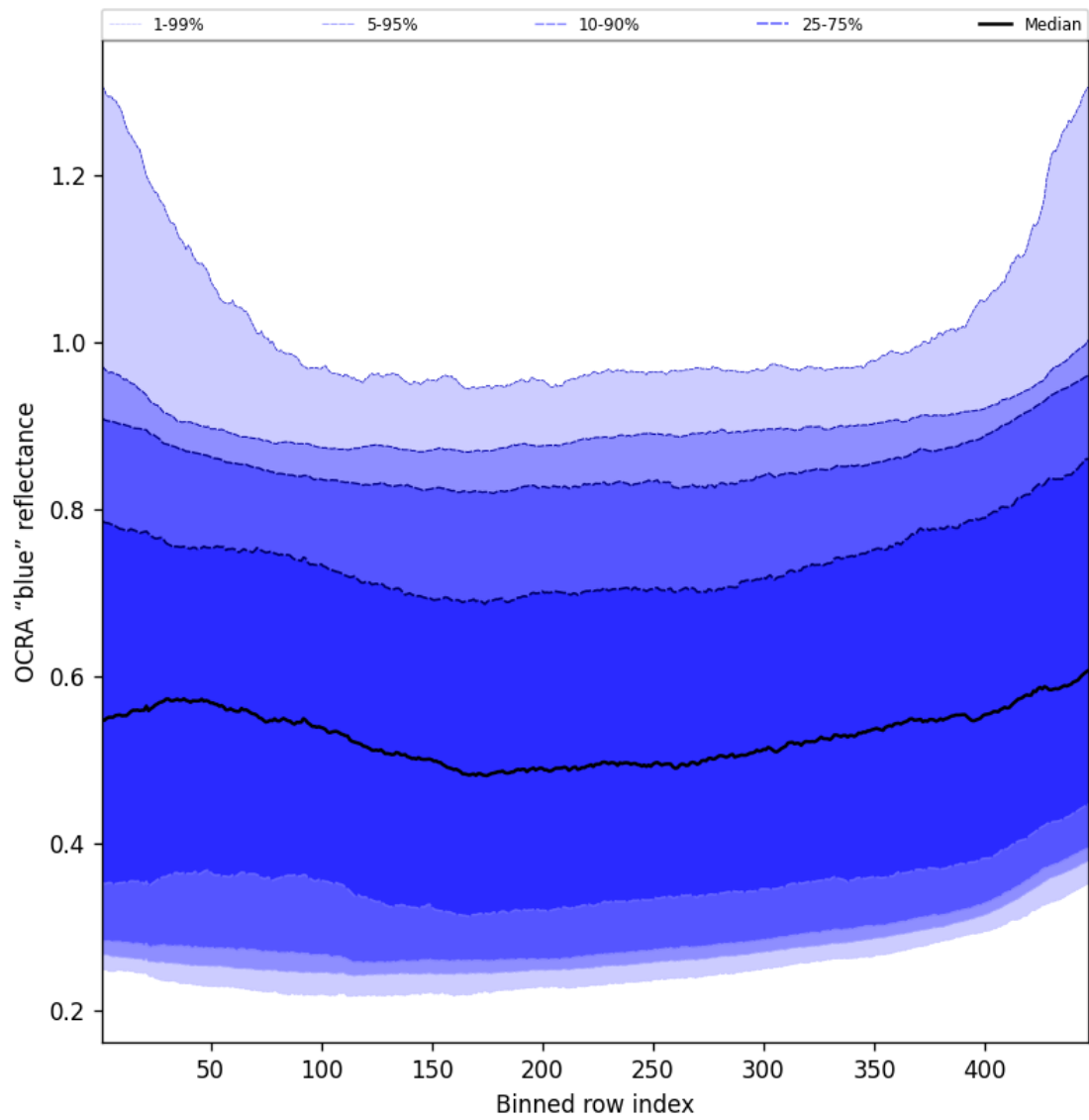
Figure 67: Along track statistics of “OCRA “blue” reflectance” for 2025-05-07 to 2025-05-09
