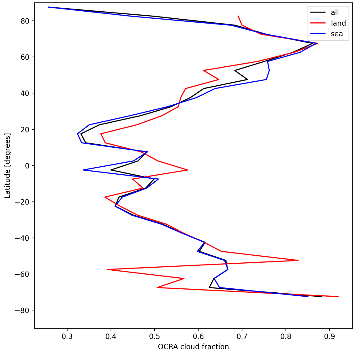
Figure 34: Zonal average of “OCRA cloud fraction” for 2025-05-07 to 2025-05-09.
