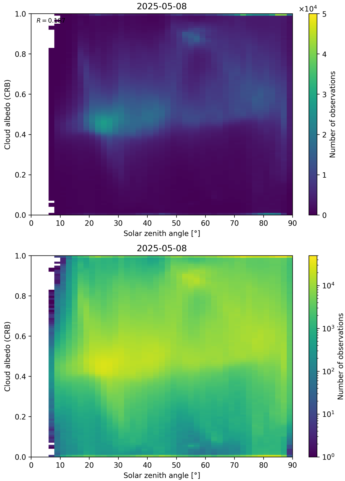
Figure 98: Scatter density plot of “Solar zenith angle” against “Cloud albedo (CRB)” for 2025-05-07 to 2025-05-09.
