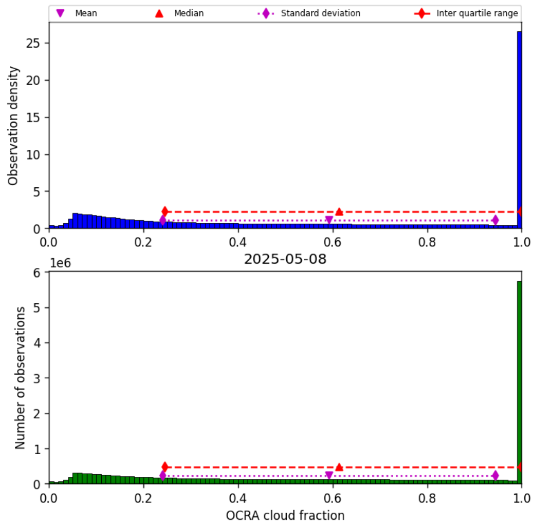
Figure 50: Histogram of “OCRA cloud fraction” for 2025-05-07 to 2025-05-09
