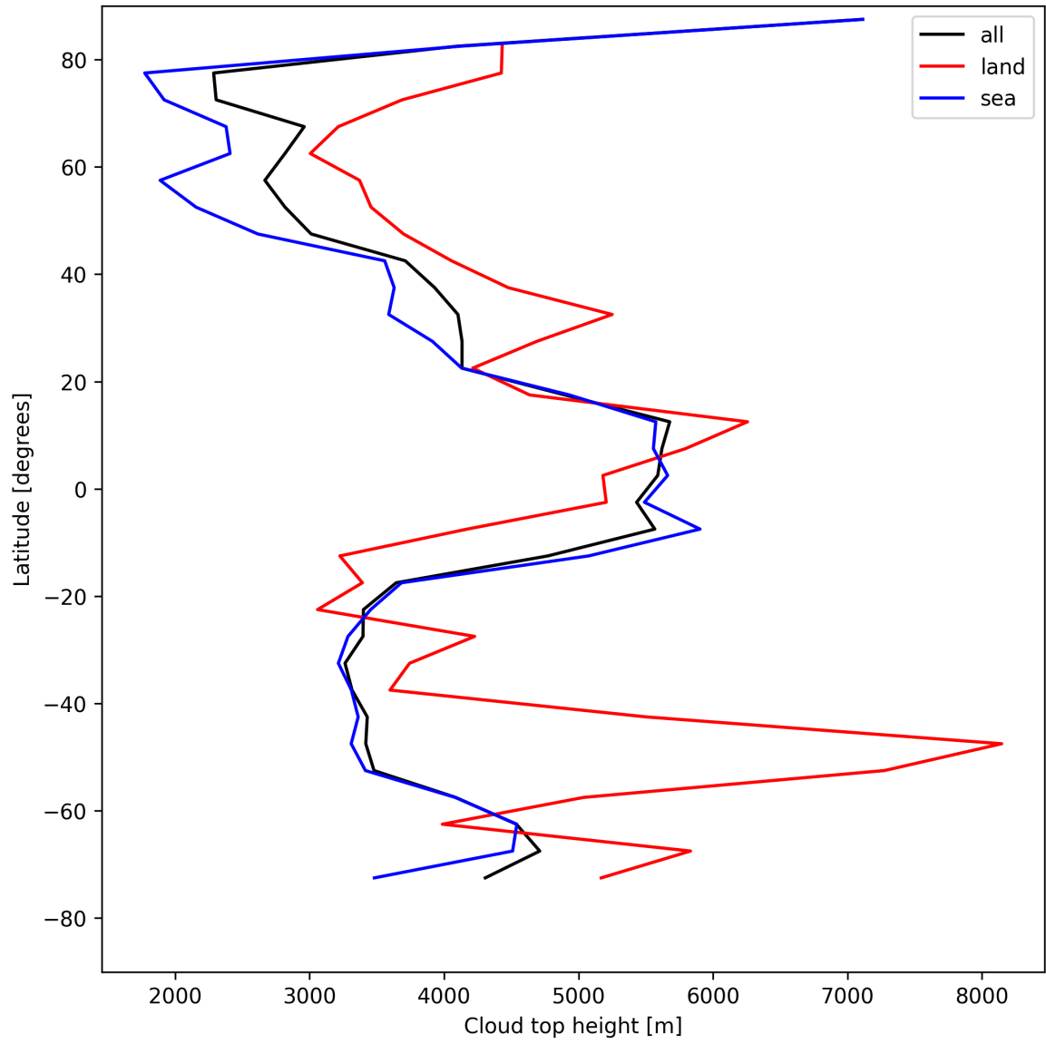
Figure 24: Zonal average of “Cloud top height” for 2025-05-07 to 2025-05-09.
