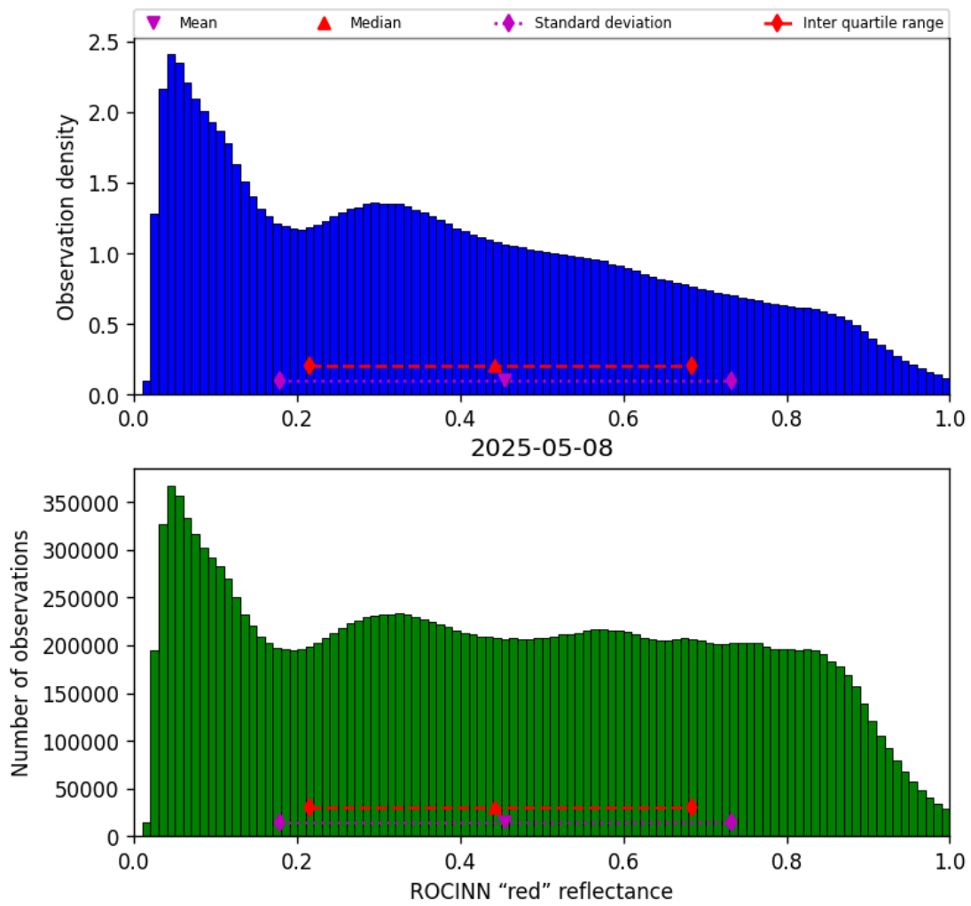
Figure 53: Histogram of “ROCINN “red” reflectance” for 2025-05-07 to 2025-05-09
