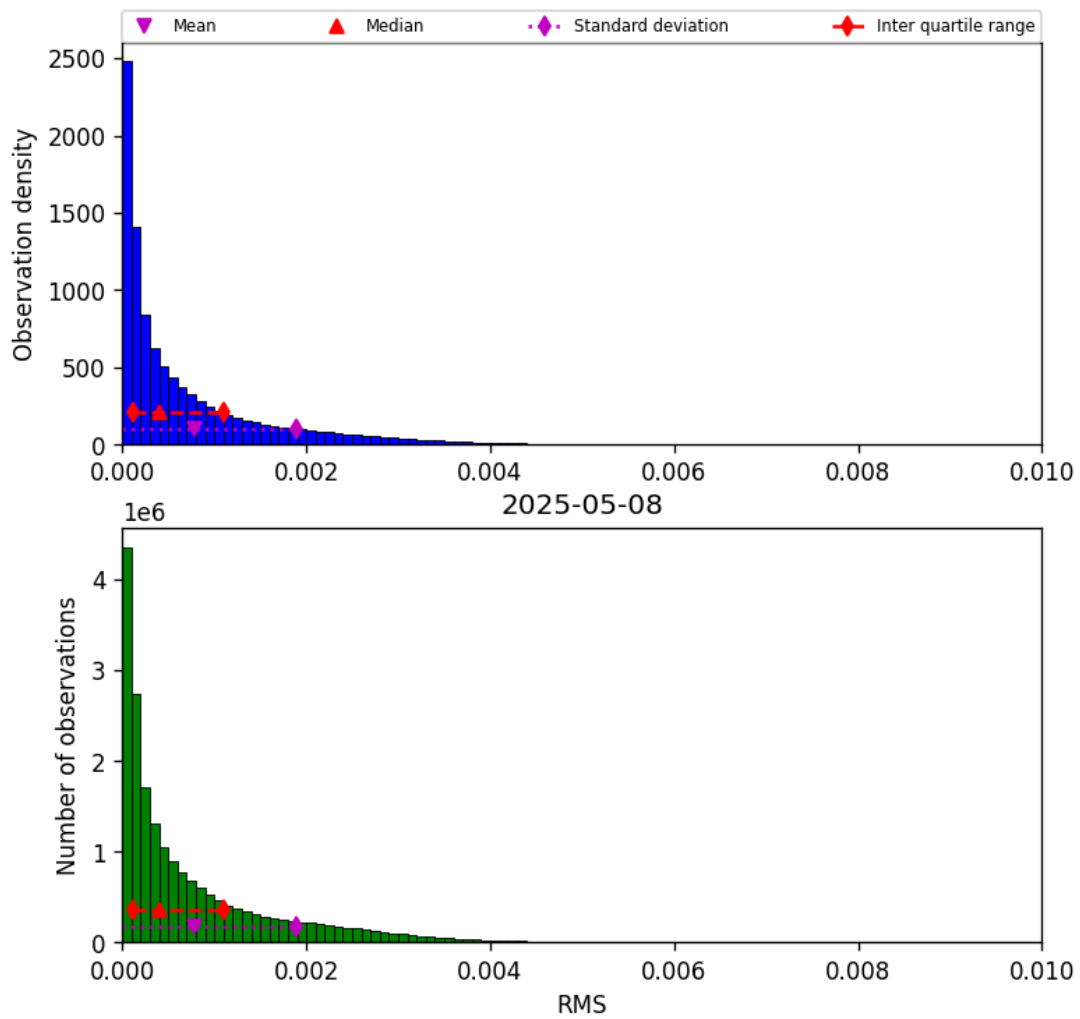
Figure 47: Histogram of “RMS” for 2025-05-07 to 2025-05-09
