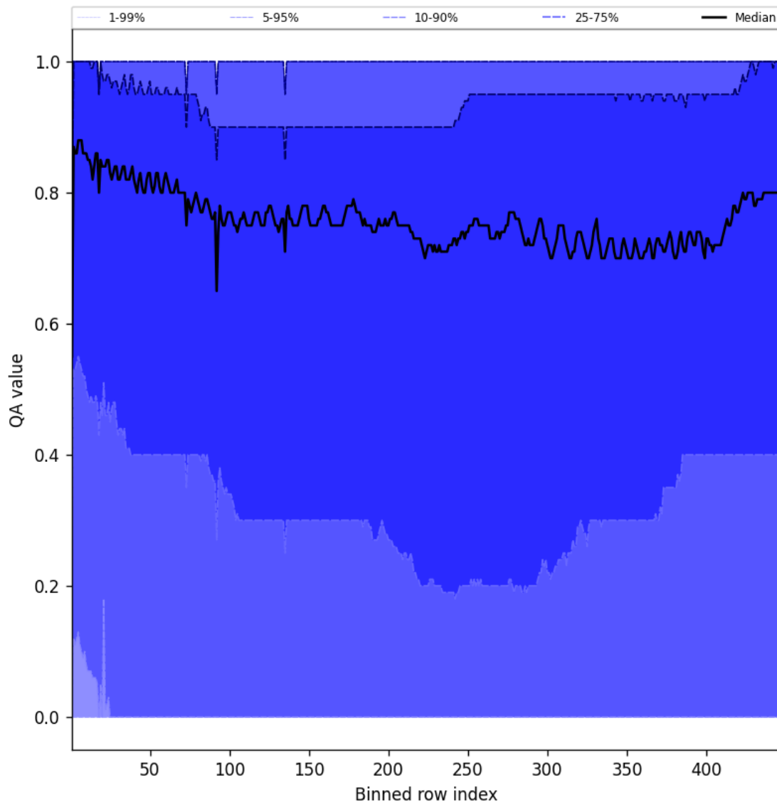
Figure 54: Along track statistics of “QA value” for 2025-05-07 to 2025-05-09
