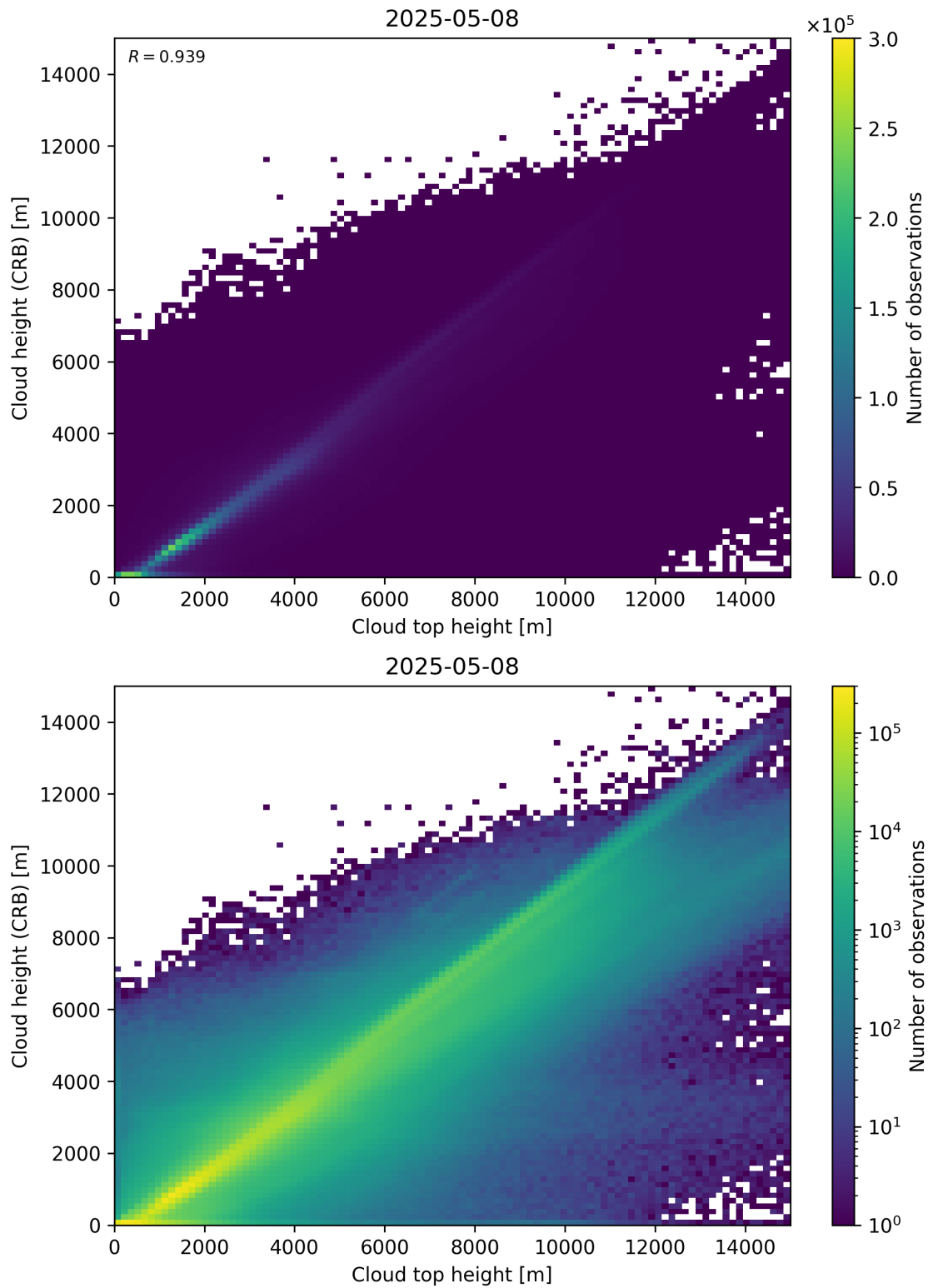
Figure 89: Scatter density plot of “Cloud top height” against “Cloud height (CRB)” for 2025-05-07 to 2025-05-09.
