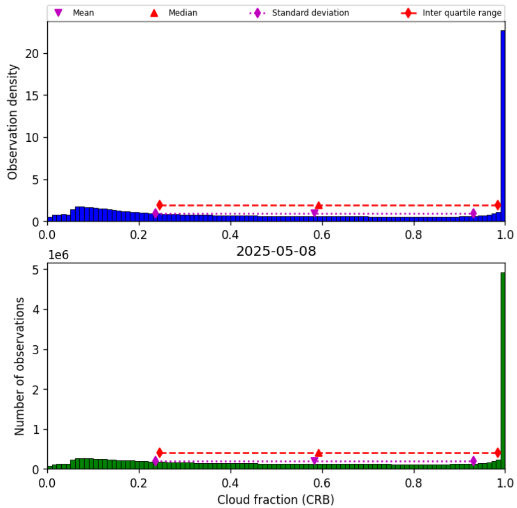
Figure 42: Histogram of “Cloud fraction (CRB)” for 2025-05-07 to 2025-05-09
