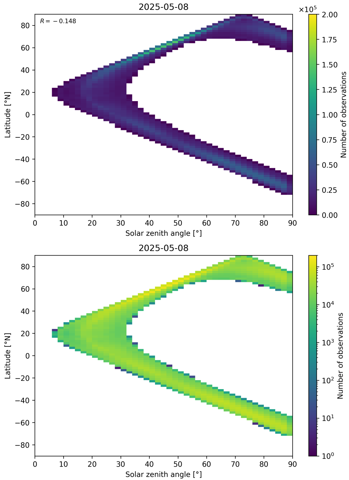
Figure 105: Scatter density plot of “Solar zenith angle” against “Latitude” for 2025-05-07 to 2025-05-09.
