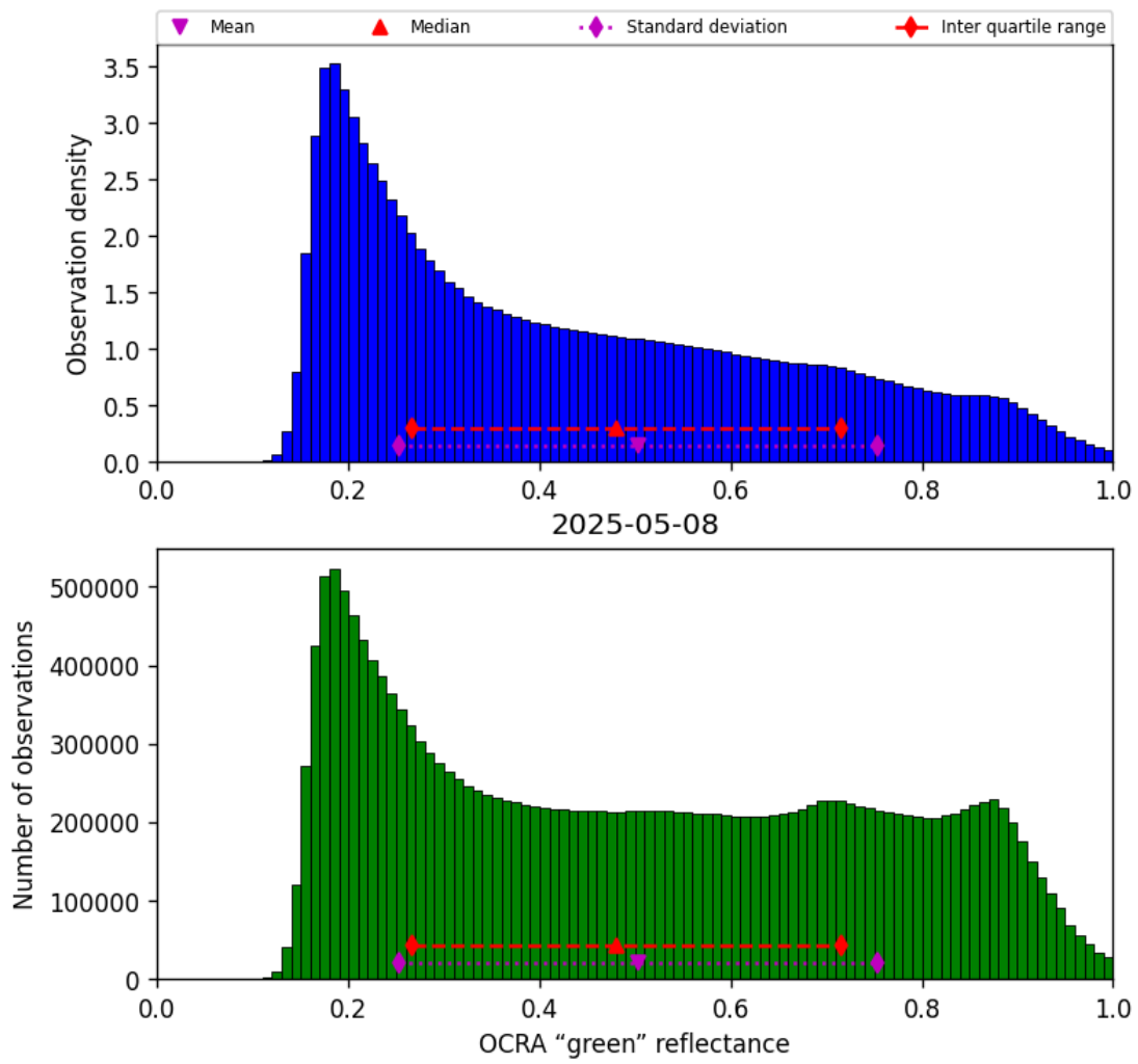
Figure 52: Histogram of “OCRA “green” reflectance” for 2025-05-07 to 2025-05-09
