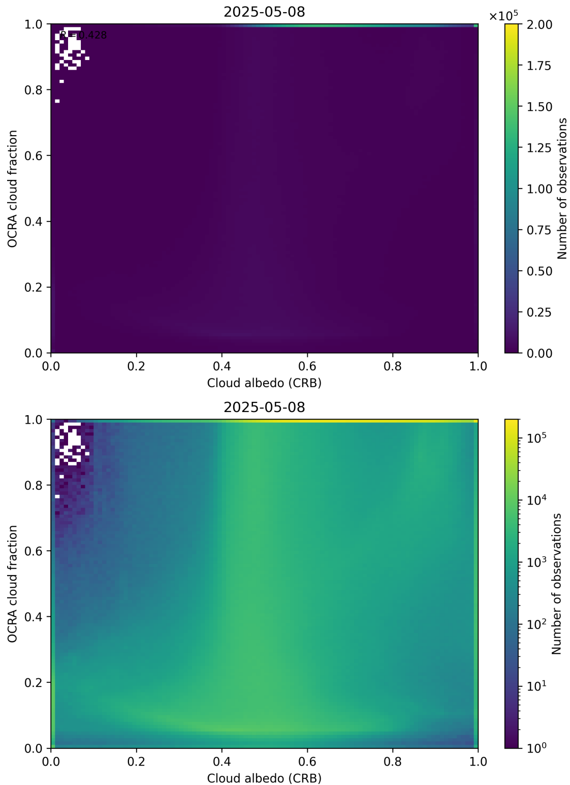
Figure 70: Scatter density plot of “Cloud albedo (CRB)” against “OCRA cloud fraction” for 2025-05-07 to 2025-05-09.
