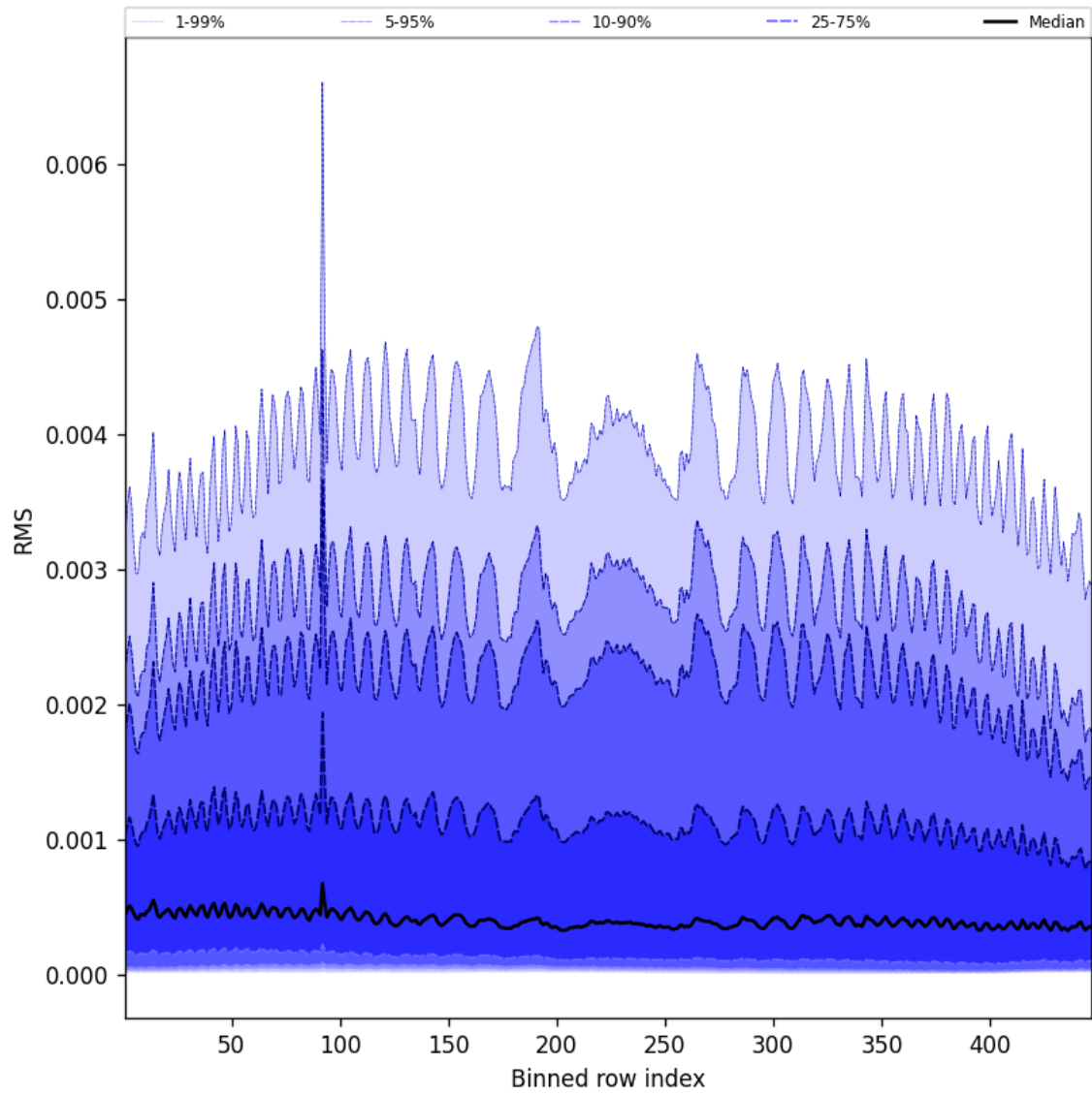
Figure 63: Along track statistics of “RMS” for 2025-05-07 to 2025-05-09
