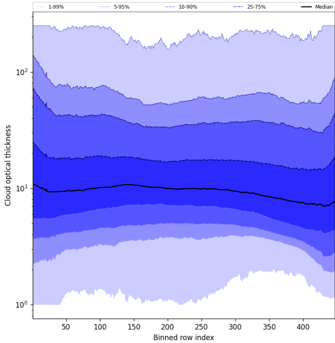
Figure 57: Along track statistics of “Cloud optical thickness” for 2025-05-07 to 2025-05-09
