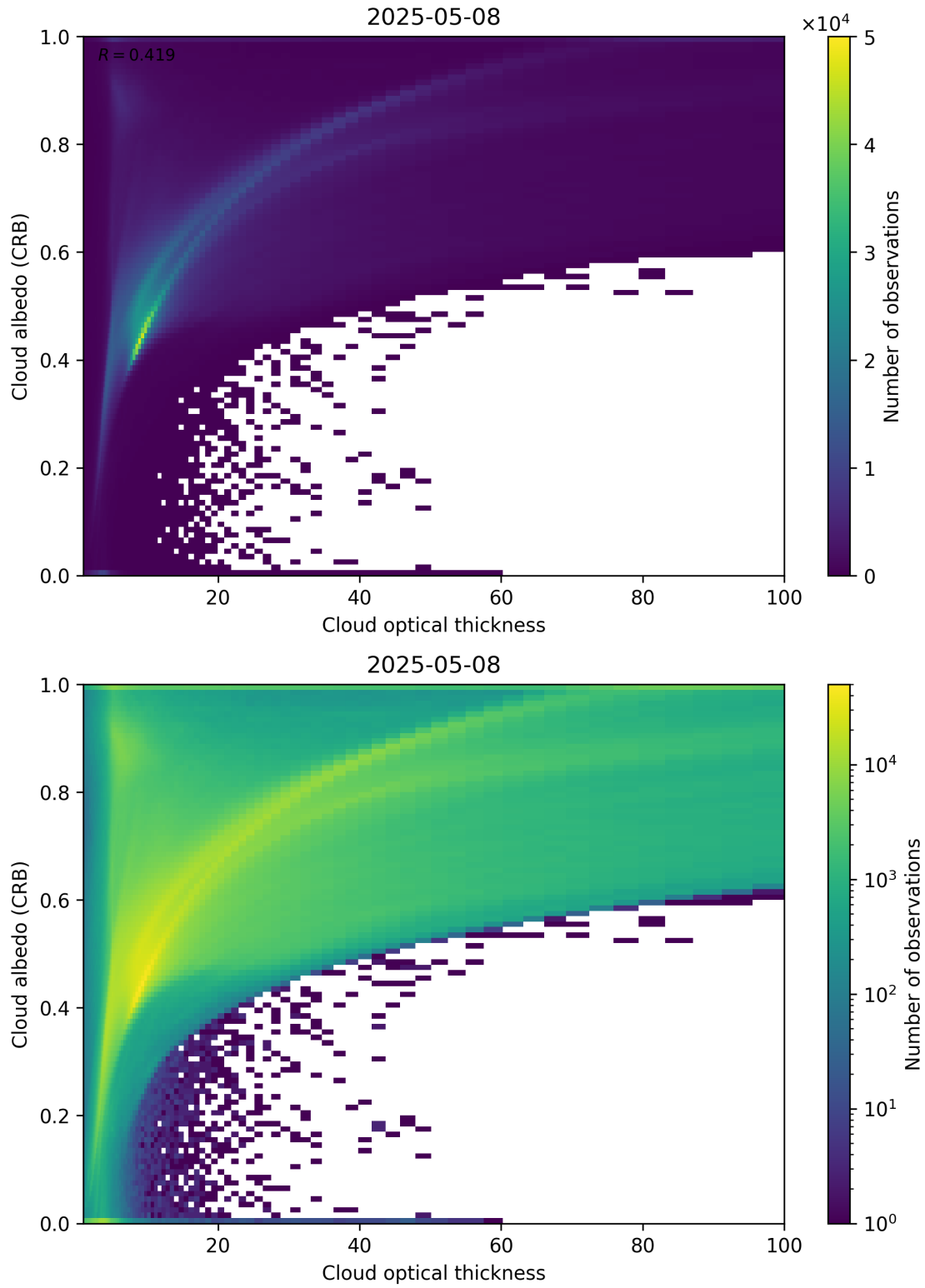
Figure 82: Scatter density plot of “Cloud optical thickness” against “Cloud albedo (CRB)” for 2025-05-07 to 2025-05-09.
