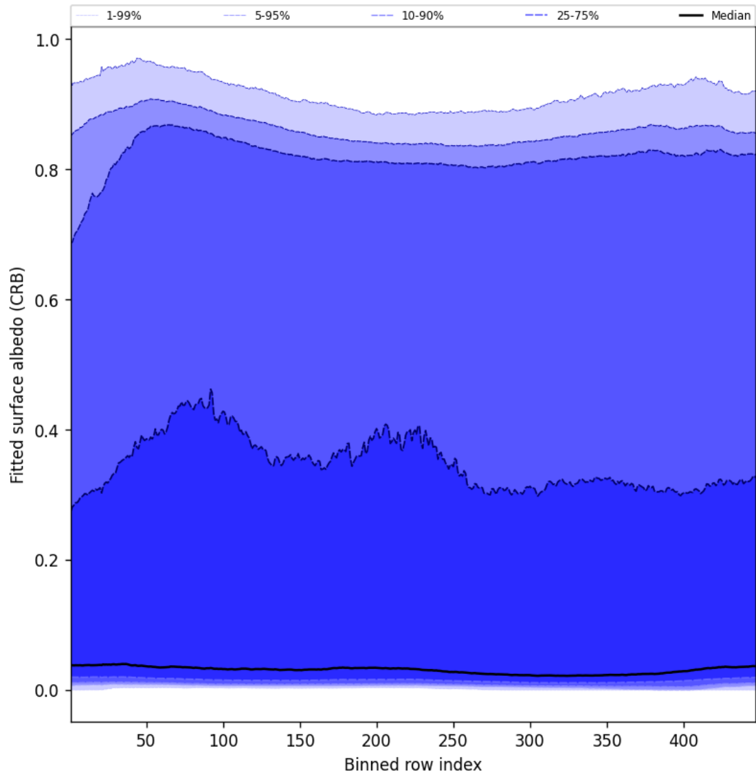
Figure 62: Along track statistics of “Fitted surface albedo (CRB)” for 2025-05-07 to 2025-05-09
