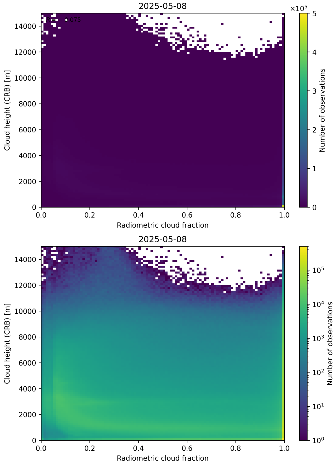
Figure 74: Scatter density plot of “Radiometric cloud fraction” against “Cloud height (CRB)” for 2025-05-07 to 2025-05-09.
