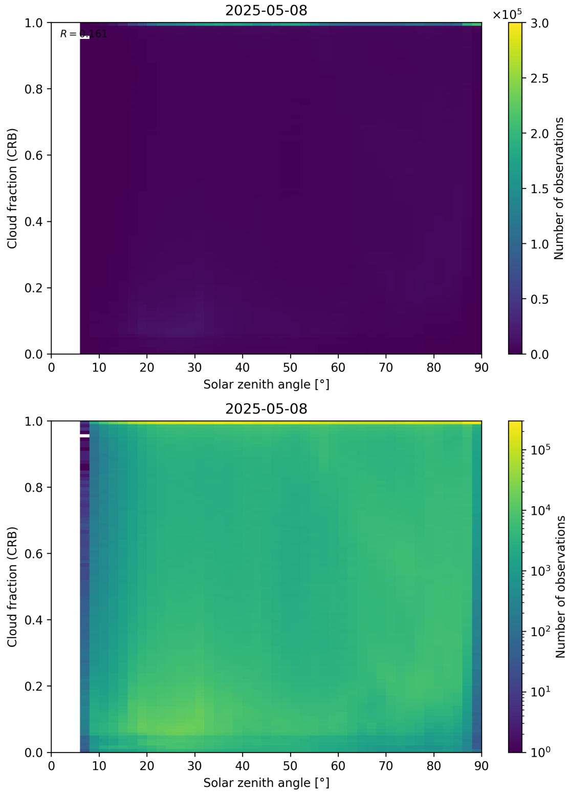
Figure 101: Scatter density plot of “Solar zenith angle” against “Cloud fraction (CRB)” for 2025-05-07 to 2025-05-09.
