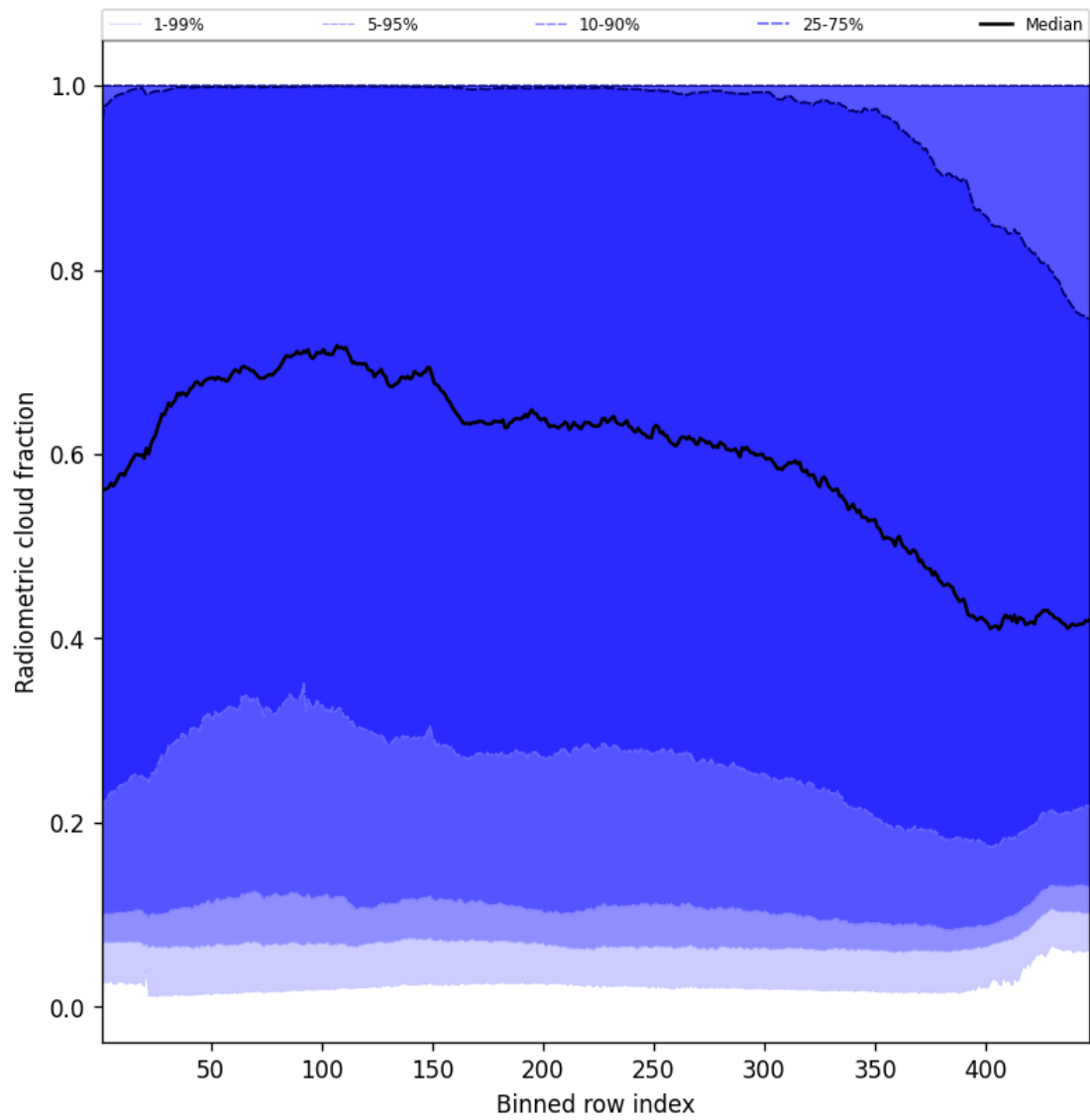
Figure 55: Along track statistics of “Radiometric cloud fraction” for 2025-05-07 to 2025-05-09
