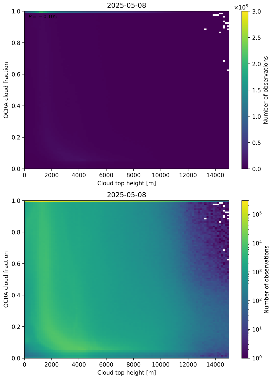
Figure 87: Scatter density plot of “Cloud top height” against “OCRA cloud fraction” for 2025-05-07 to 2025-05-09.
