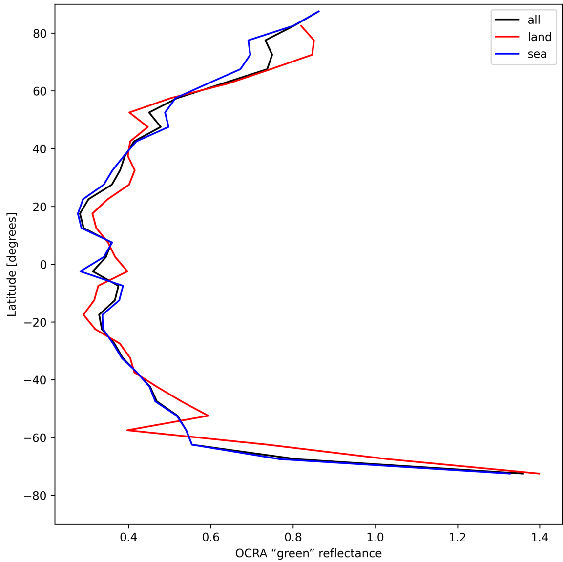
Figure 36: Zonal average of “OCRA “green” reflectance” for 2025-05-07 to 2025-05-09.
