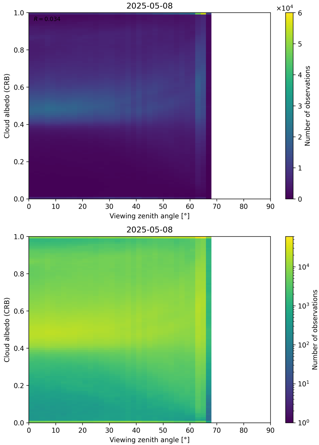
Figure 106: Scatter density plot of “Viewing zenith angle” against “Cloud albedo (CRB)” for 2025-05-07 to 2025-05-09.
