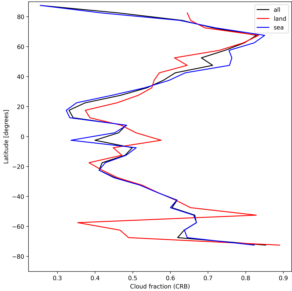
Figure 26: Zonal average of “Cloud fraction (CRB)” for 2025-05-07 to 2025-05-09.
