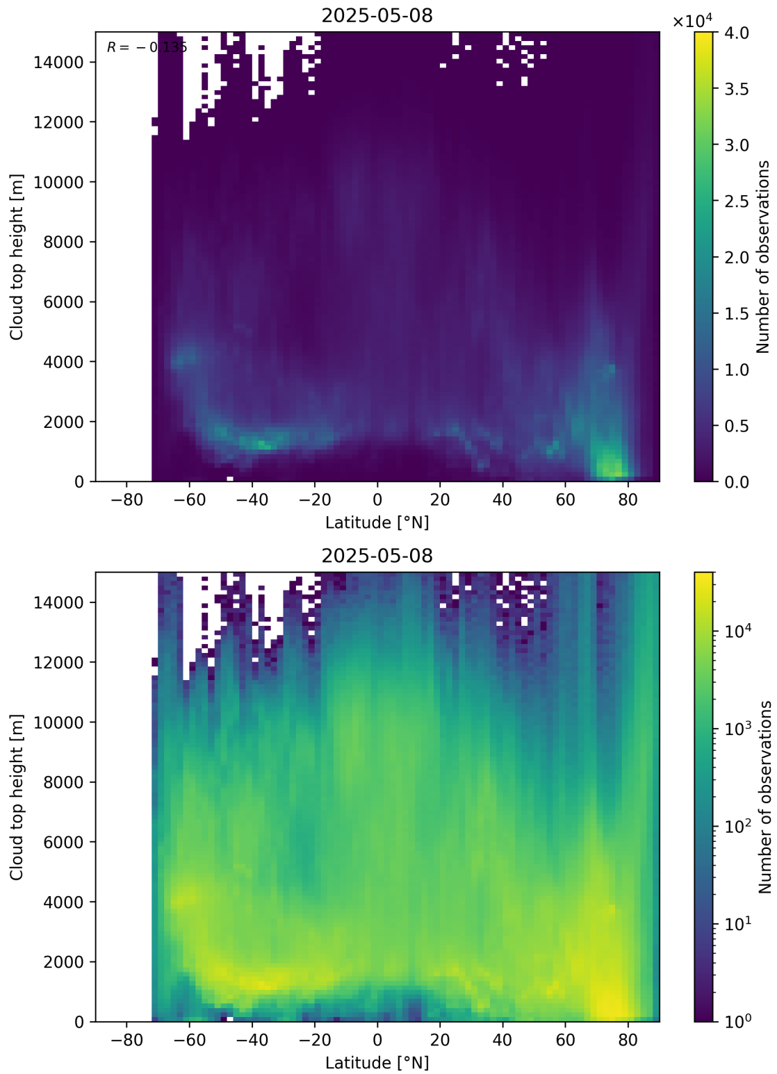
Figure 97: Scatter density plot of “Latitude” against “Cloud top height” for 2025-05-07 to 2025-05-09.
