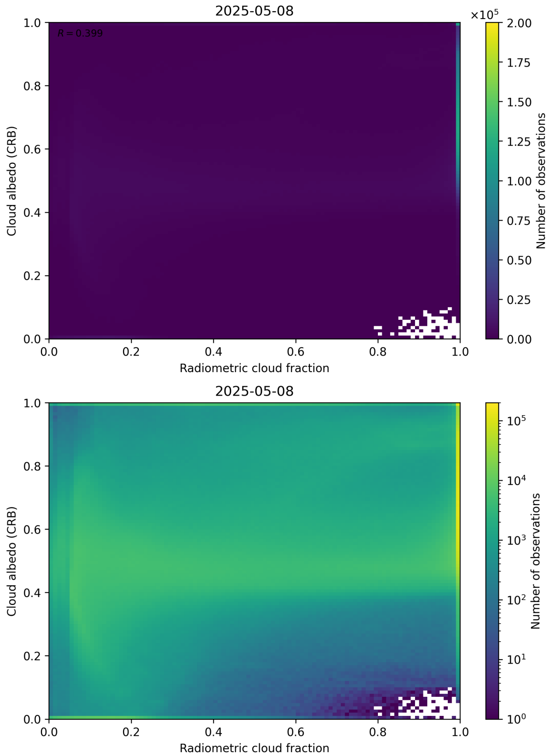
Figure 71: Scatter density plot of “Radiometric cloud fraction” against “Cloud albedo (CRB)” for 2025-05-07 to 2025-05-09.
