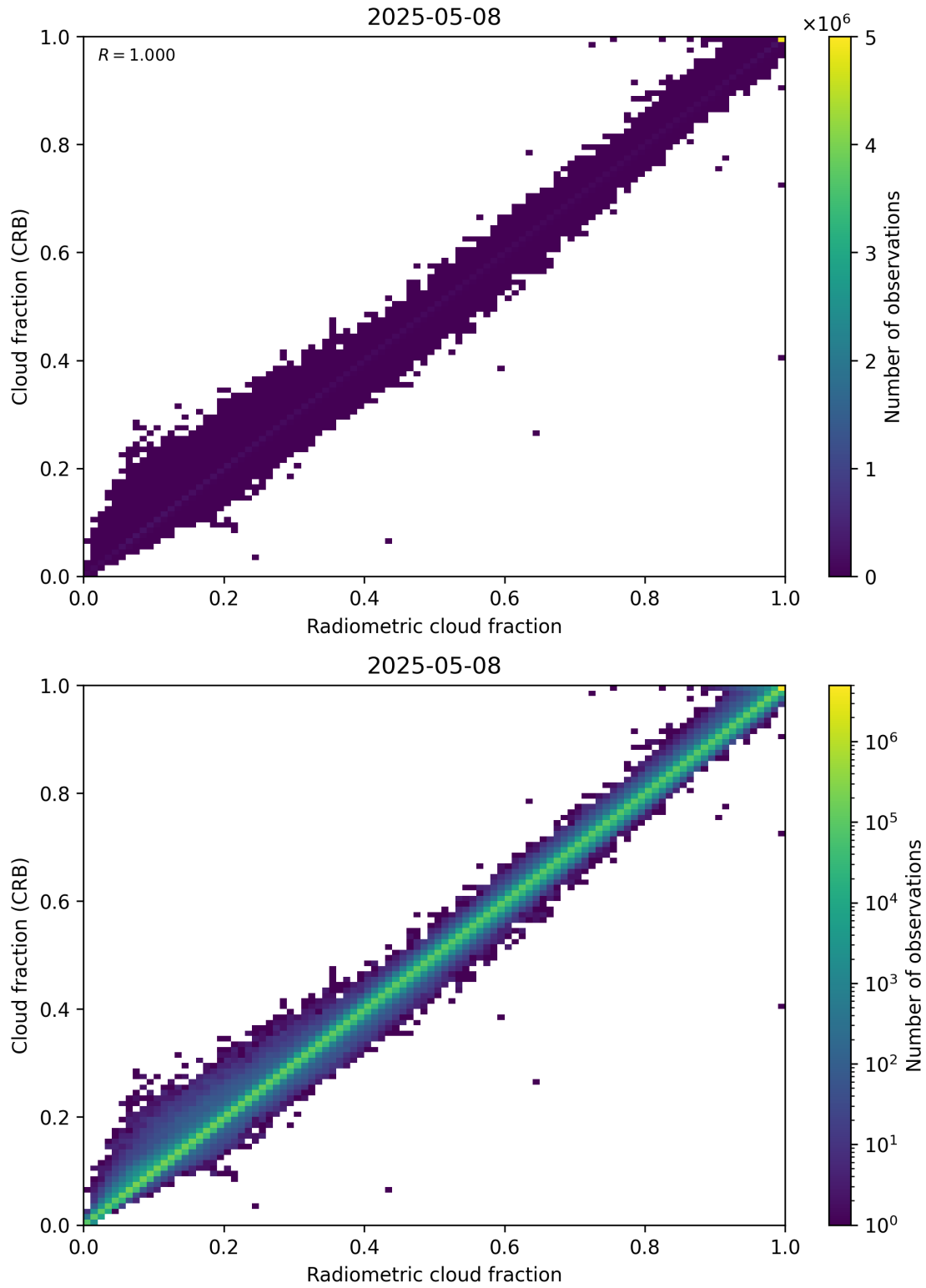
Figure 73: Scatter density plot of “Radiometric cloud fraction” against “Cloud fraction (CRB)” for 2025-05-07 to 2025-05-09.
