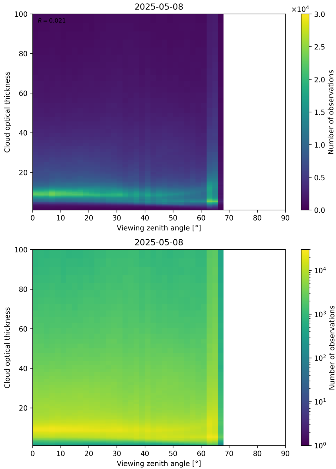
Figure 111: Scatter density plot of “Viewing zenith angle” against “Cloud optical thickness” for 2025-05-07 to 2025-05-09.
