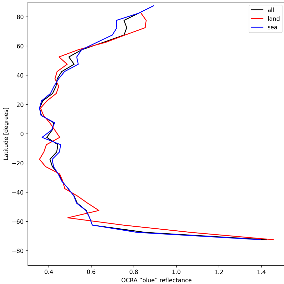
Figure 35: Zonal average of “OCRA “blue” reflectance” for 2025-05-07 to 2025-05-09.
