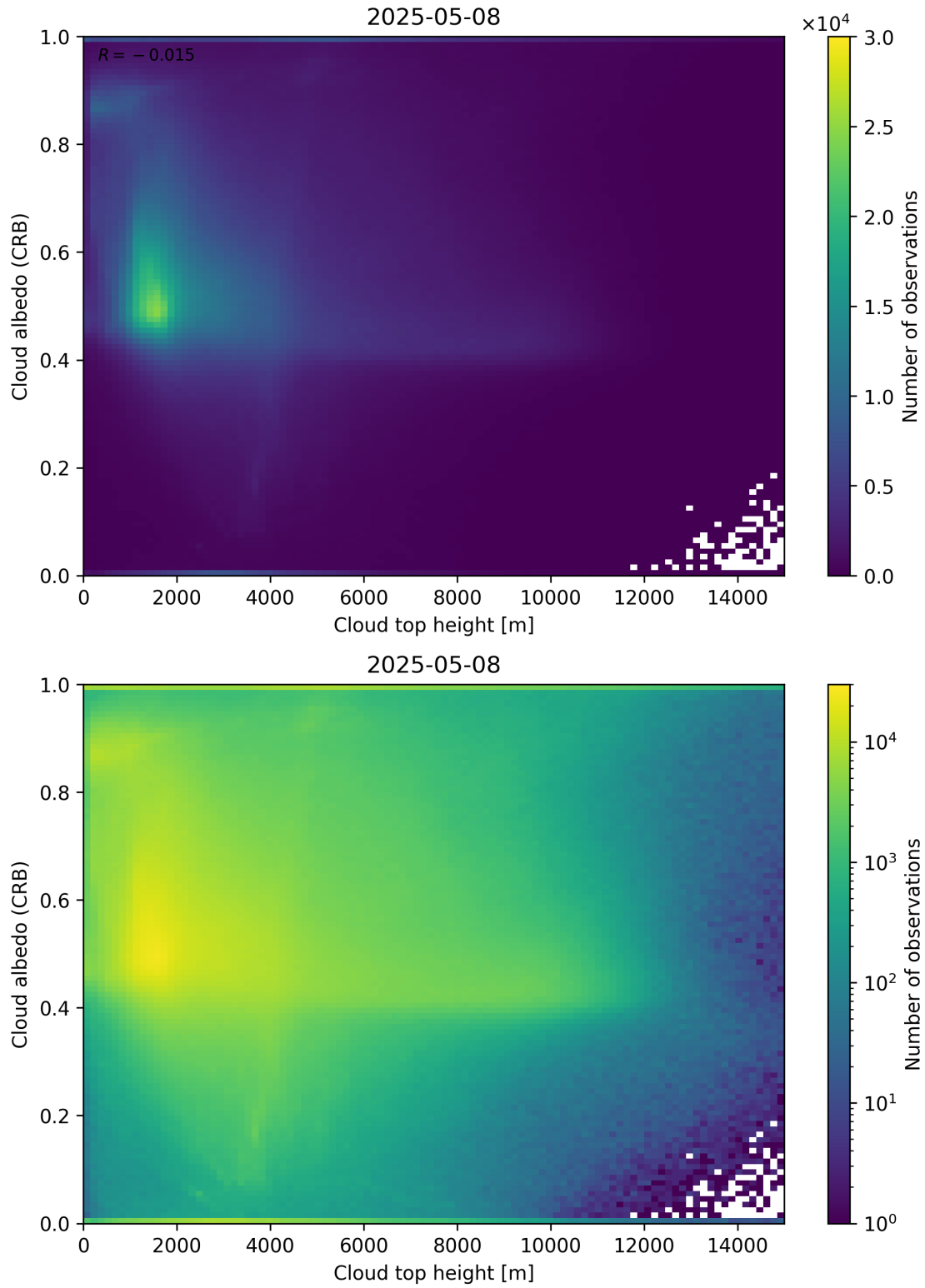
Figure 86: Scatter density plot of “Cloud top height” against “Cloud albedo (CRB)” for 2025-05-07 to 2025-05-09.
