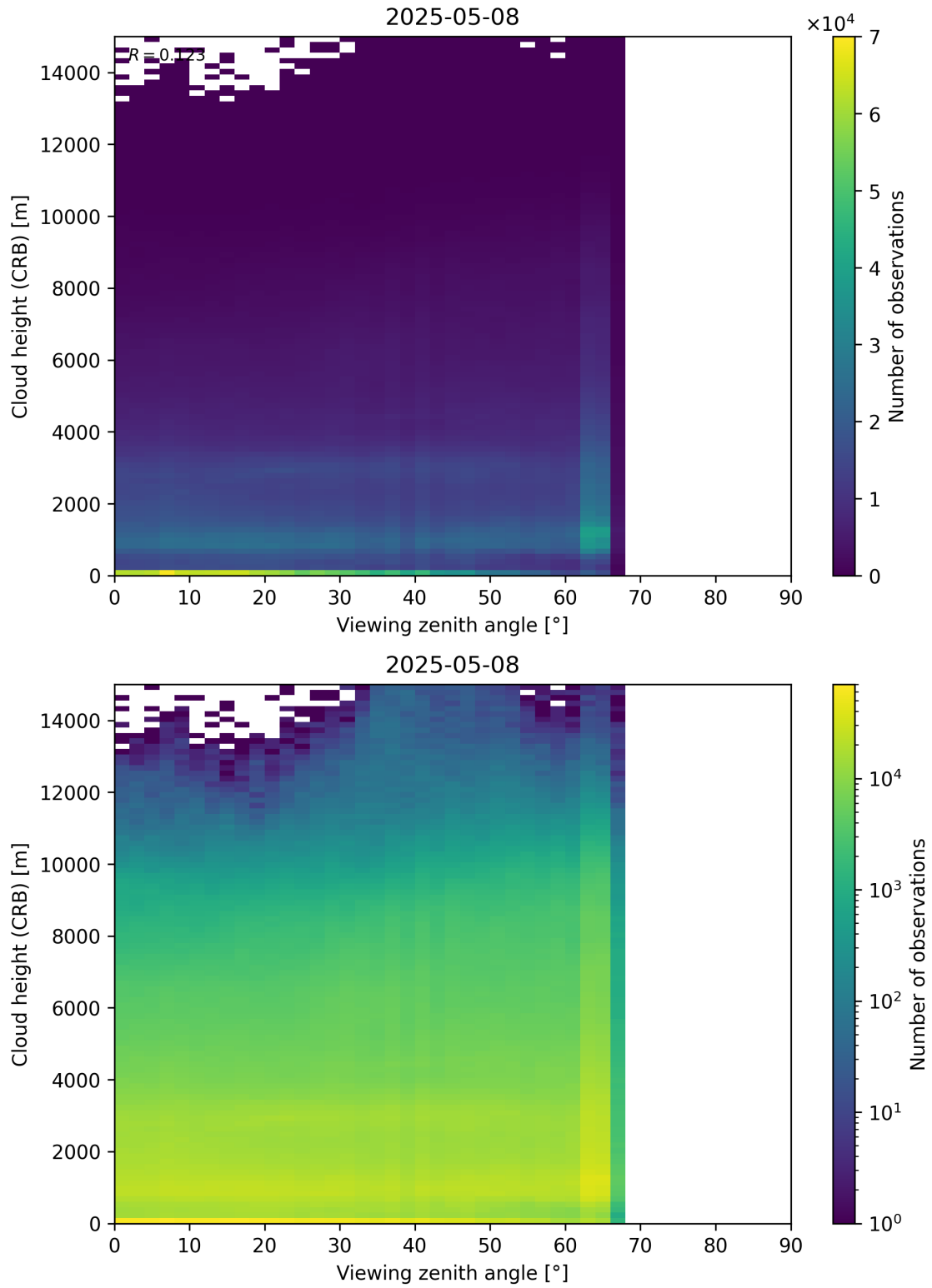
Figure 110: Scatter density plot of “Viewing zenith angle” against “Cloud height (CRB)” for 2025-05-07 to 2025-05-09.
