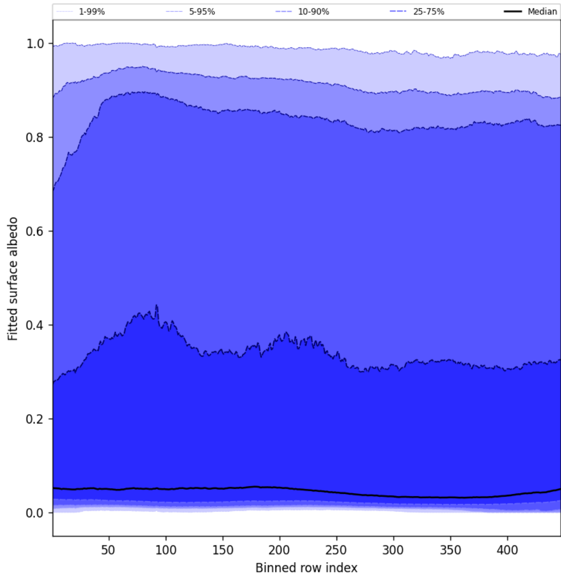
Figure 61: Along track statistics of “Fitted surface albedo” for 2025-05-07 to 2025-05-09
