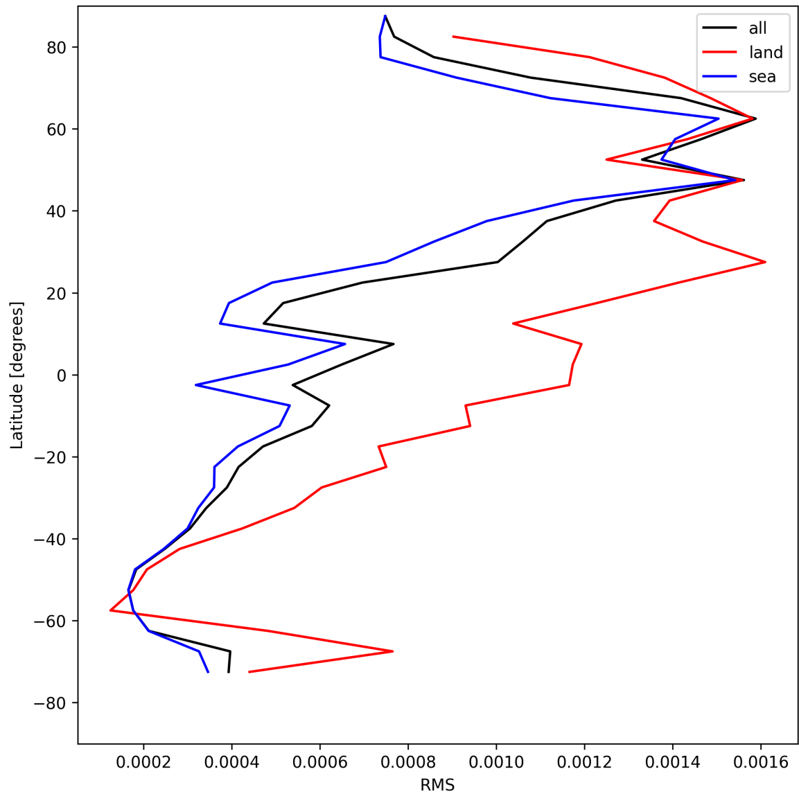
Figure 31: Zonal average of “RMS” for 2025-05-07 to 2025-05-09.
