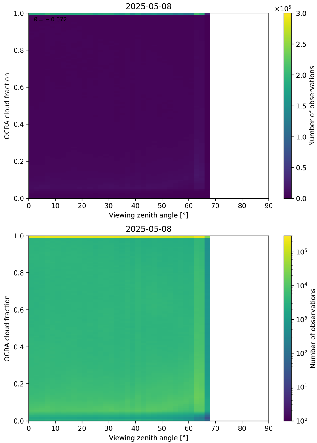
Figure 108: Scatter density plot of “Viewing zenith angle” against “OCRA cloud fraction” for 2025-05-07 to 2025-05-09.
