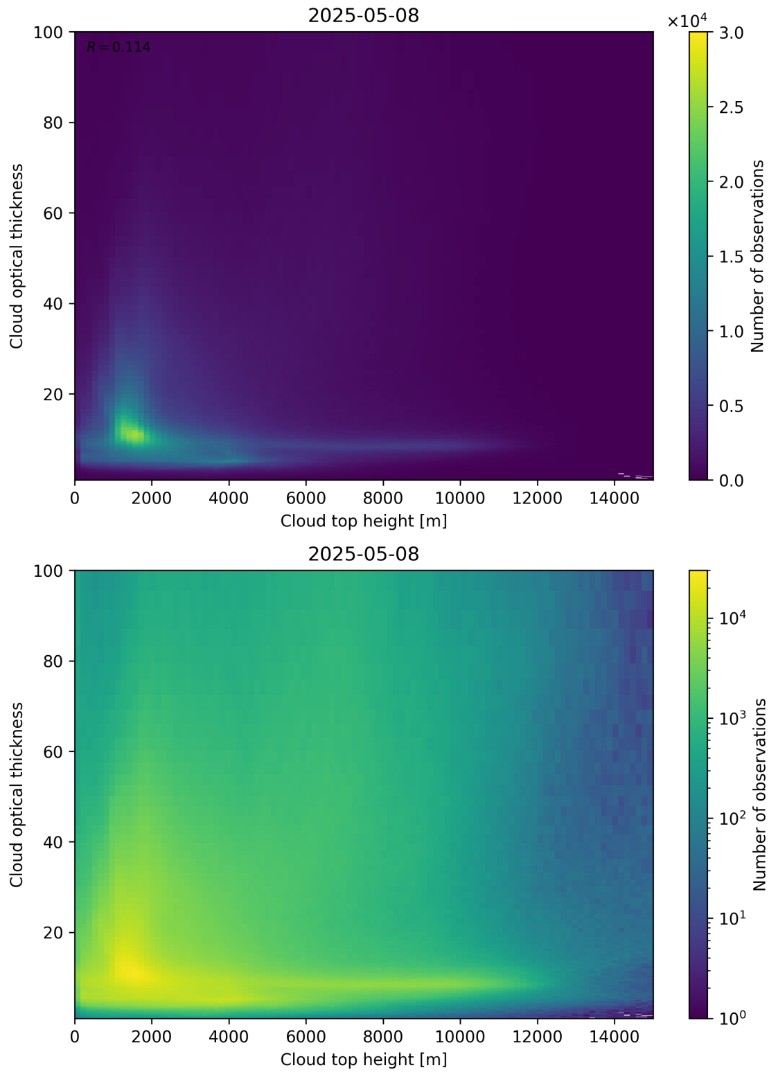
Figure 90: Scatter density plot of “Cloud top height” against “Cloud optical thickness” for 2025-05-07 to 2025-05-09.
