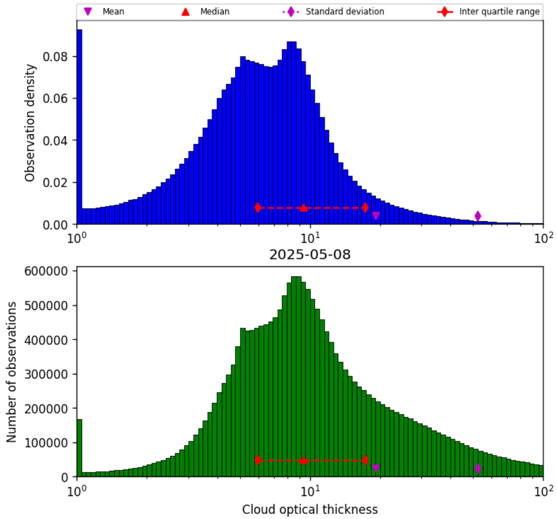
Figure 41: Histogram of “Cloud optical thickness” for 2025-05-07 to 2025-05-09
