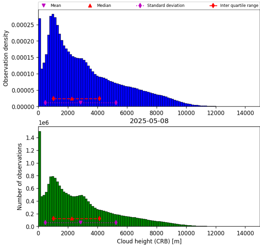
Figure 43: Histogram of “Cloud height (CRB)” for 2025-05-07 to 2025-05-09
