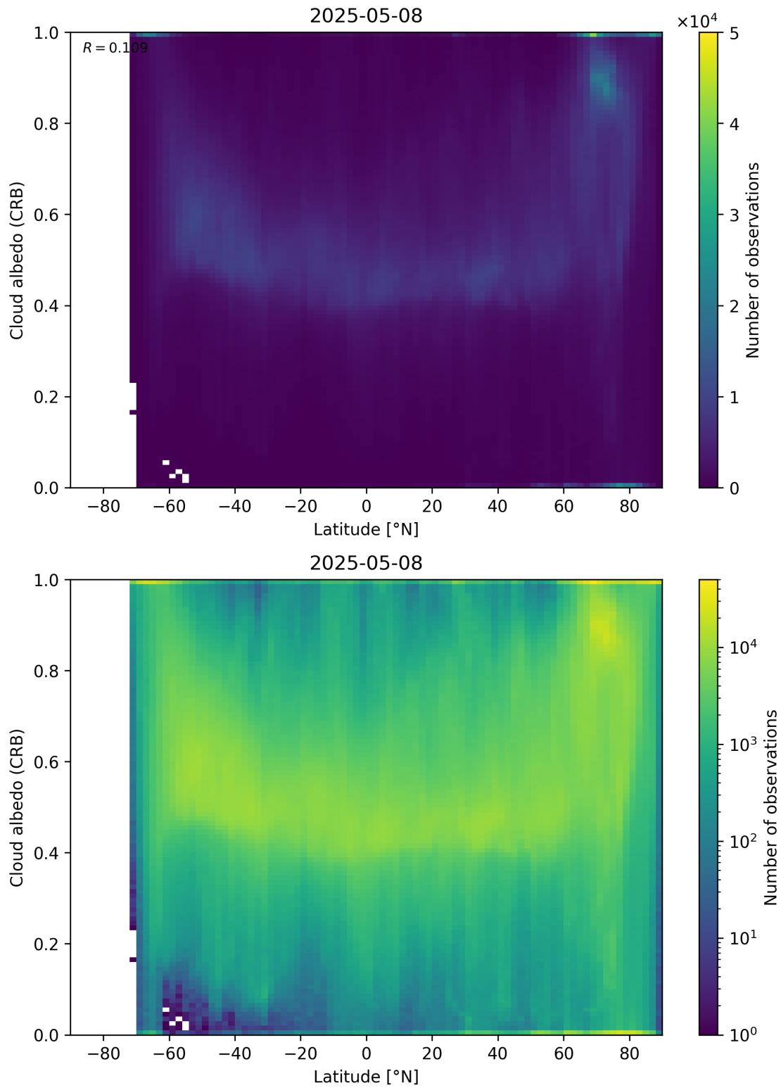
Figure 91: Scatter density plot of “Latitude” against “Cloud albedo (CRB)” for 2025-05-07 to 2025-05-09.
