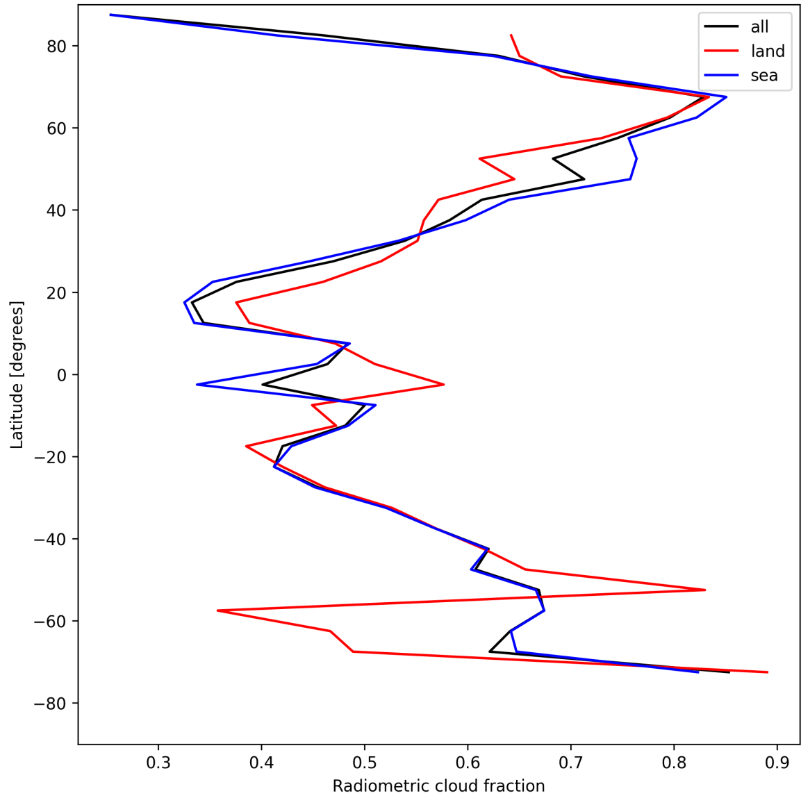
Figure 23: Zonal average of “Radiometric cloud fraction” for 2025-05-07 to 2025-05-09.
