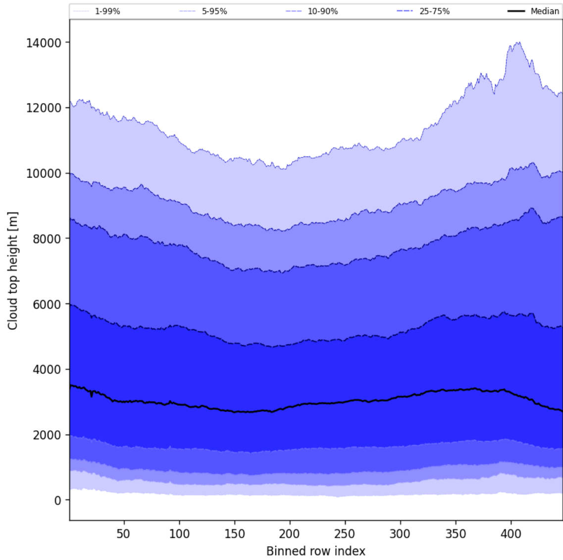
Figure 56: Along track statistics of “Cloud top height” for 2025-05-07 to 2025-05-09
