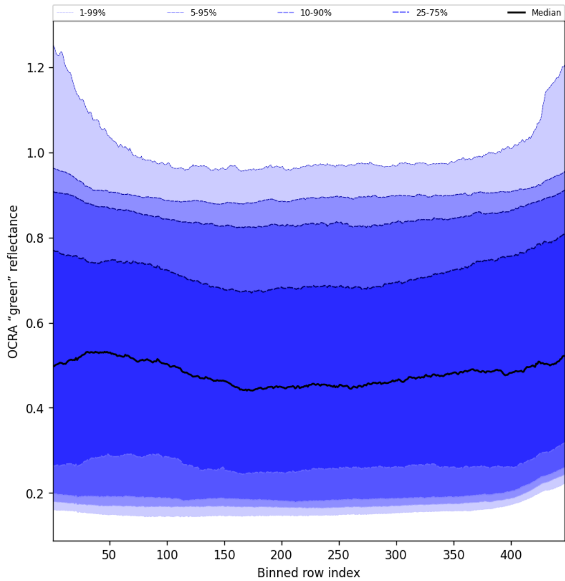
Figure 68: Along track statistics of “OCRA “green” reflectance” for 2025-05-07 to 2025-05-09
