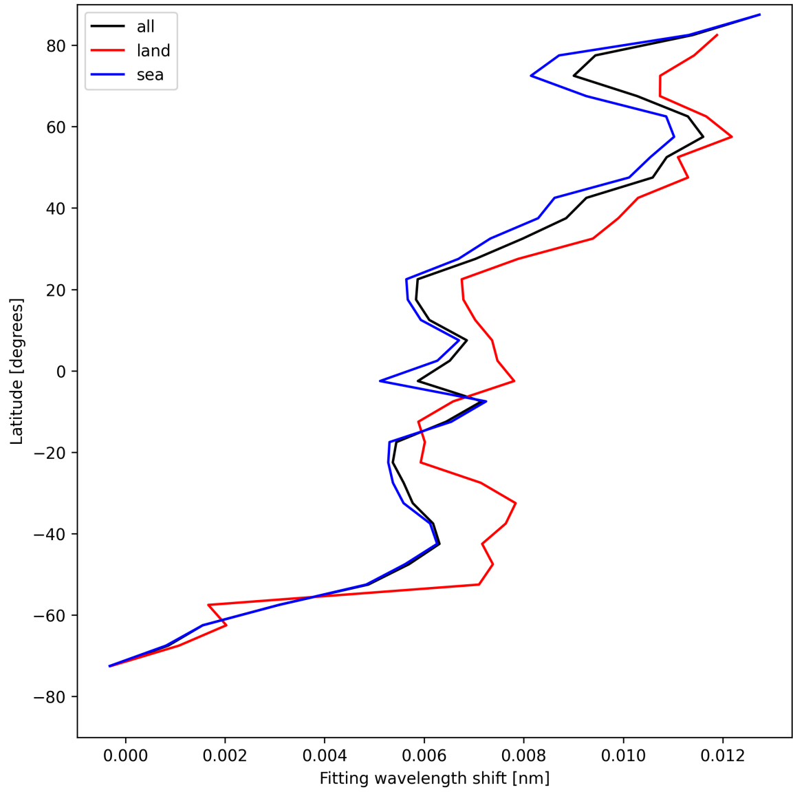
Figure 33: Zonal average of “Fitting wavelength shift” for 2025-05-07 to 2025-05-09.
