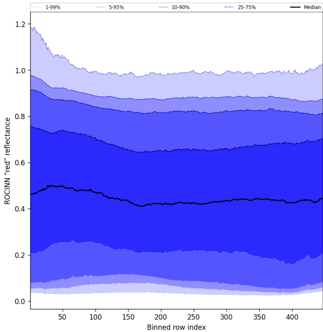
Figure 69: Along track statistics of “ROCINN “red” reflectance” for 2025-05-07 to 2025-05-09
