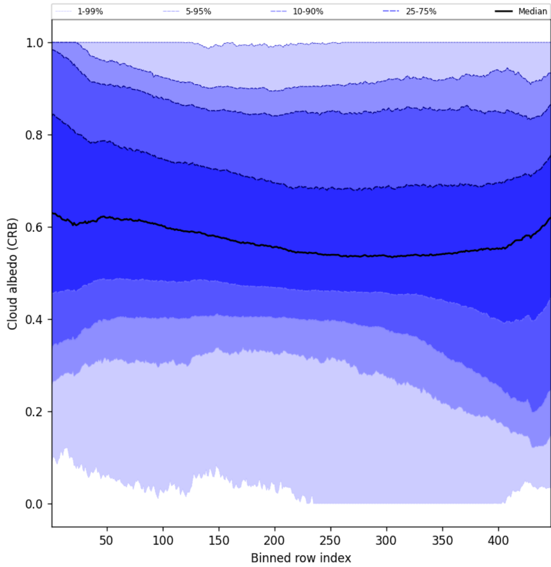
Figure 60: Along track statistics of “Cloud albedo (CRB)” for 2025-05-07 to 2025-05-09
