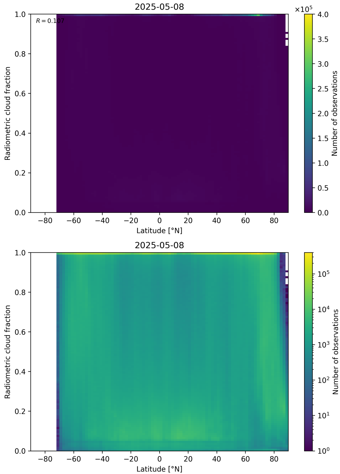
Figure 92: Scatter density plot of “Latitude” against “Radiometric cloud fraction” for 2025-05-07 to 2025-05-09.
