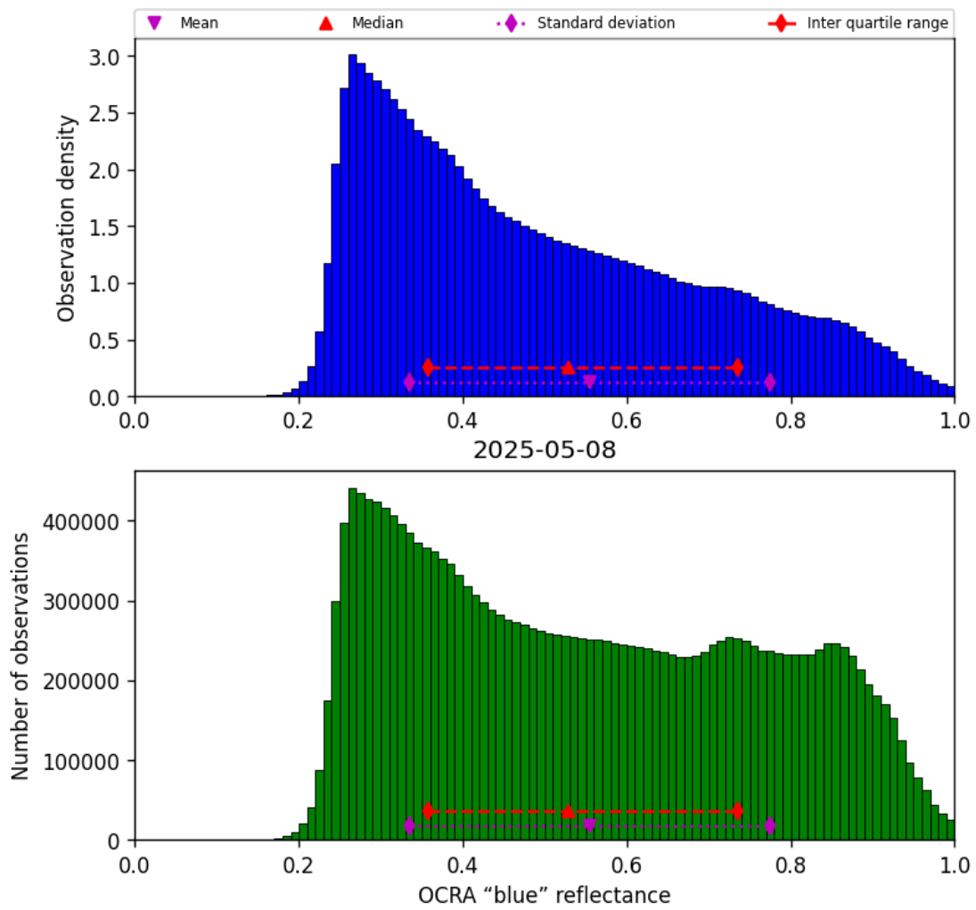
Figure 51: Histogram of “OCRA “blue” reflectance” for 2025-05-07 to 2025-05-09
