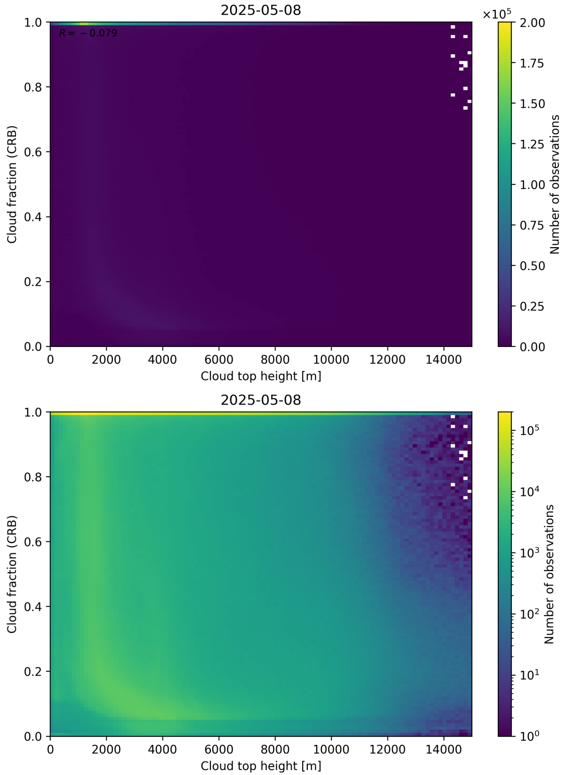
Figure 88: Scatter density plot of “Cloud top height” against “Cloud fraction (CRB)” for 2025-05-07 to 2025-05-09.
