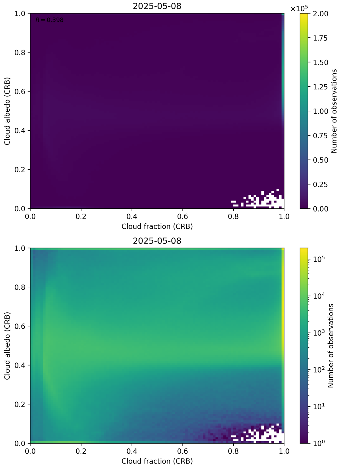
Figure 77: Scatter density plot of “Cloud fraction (CRB)” against “Cloud albedo (CRB)” for 2025-05-07 to 2025-05-09.
