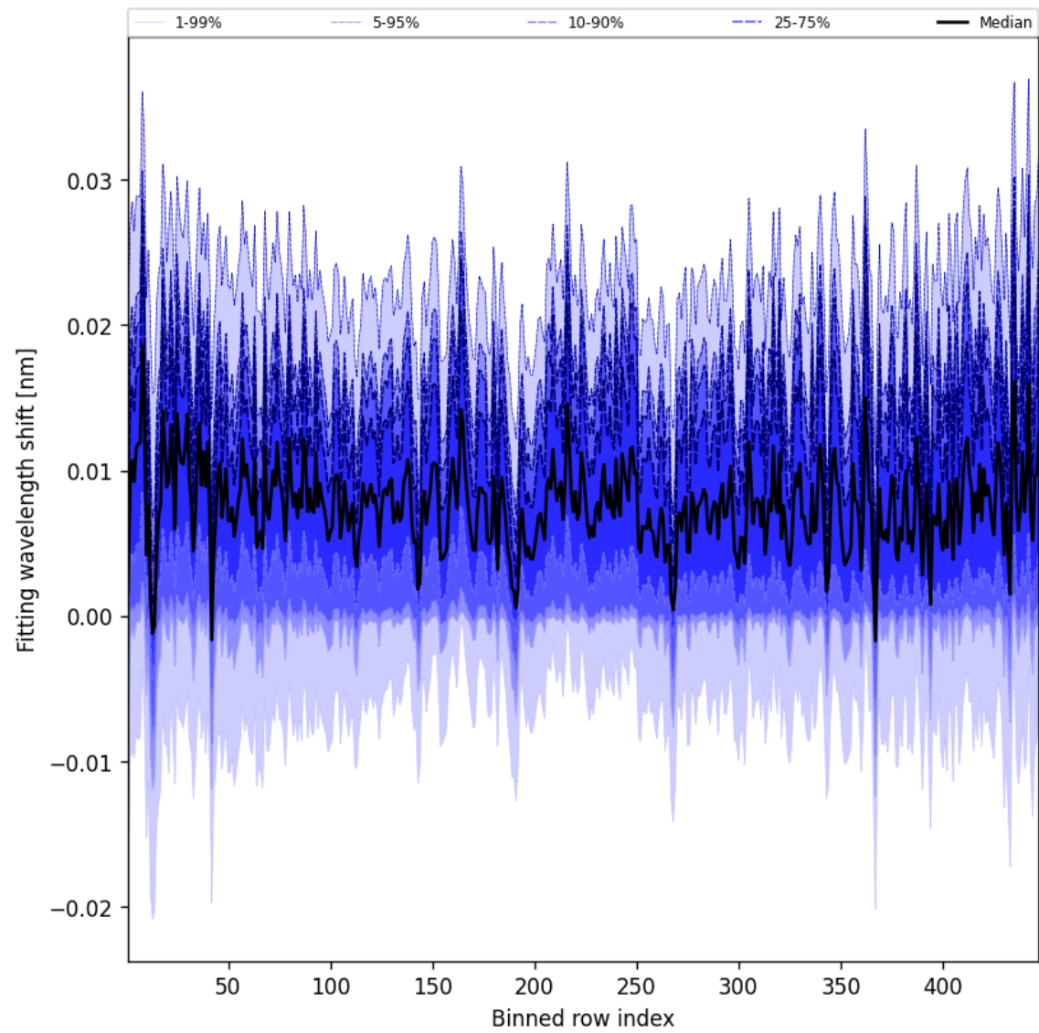
Figure 65: Along track statistics of “Fitting wavelength shift” for 2025-05-07 to 2025-05-09
