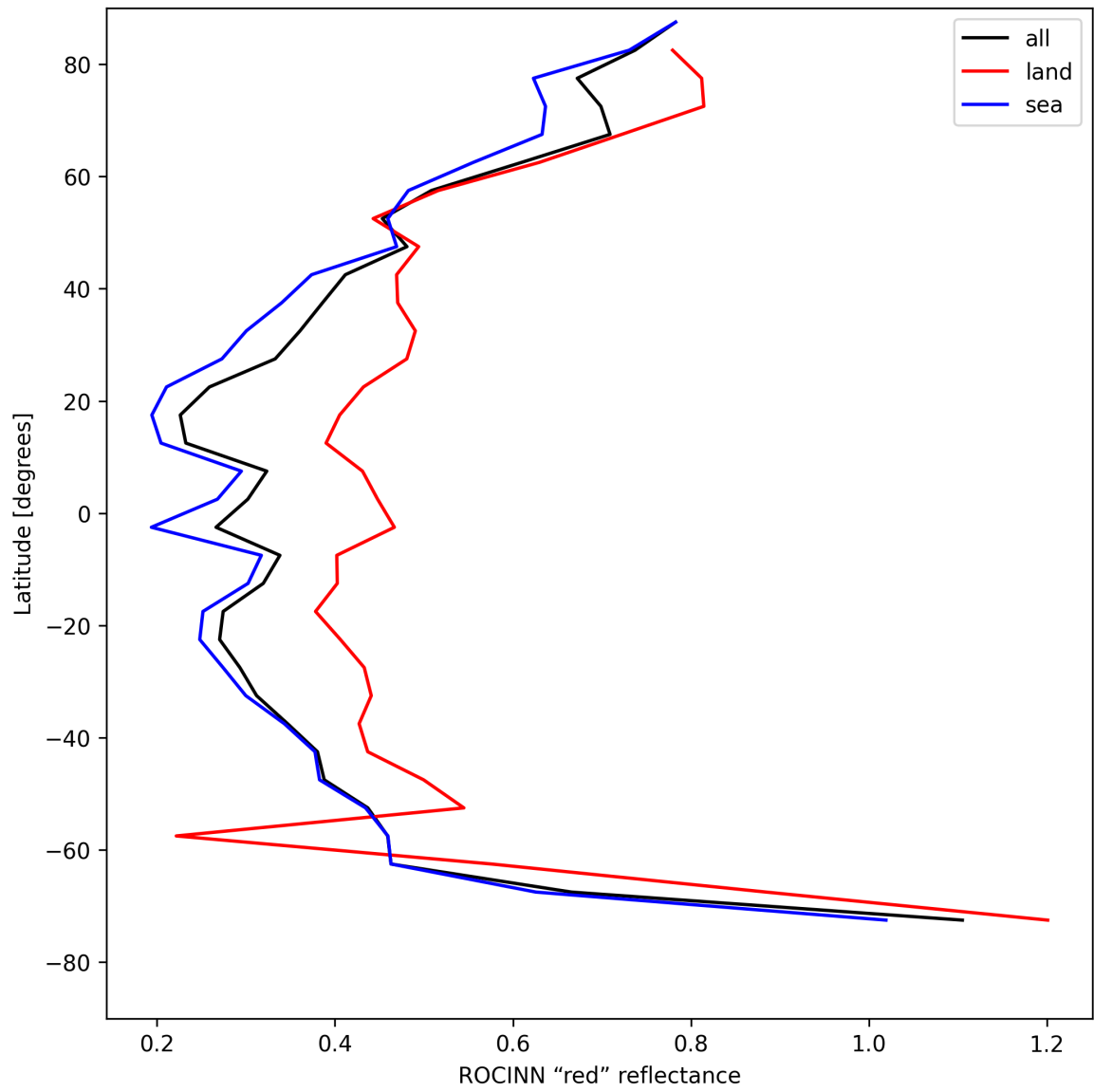
Figure 37: Zonal average of “ROCINN “red” reflectance” for 2025-05-07 to 2025-05-09.
