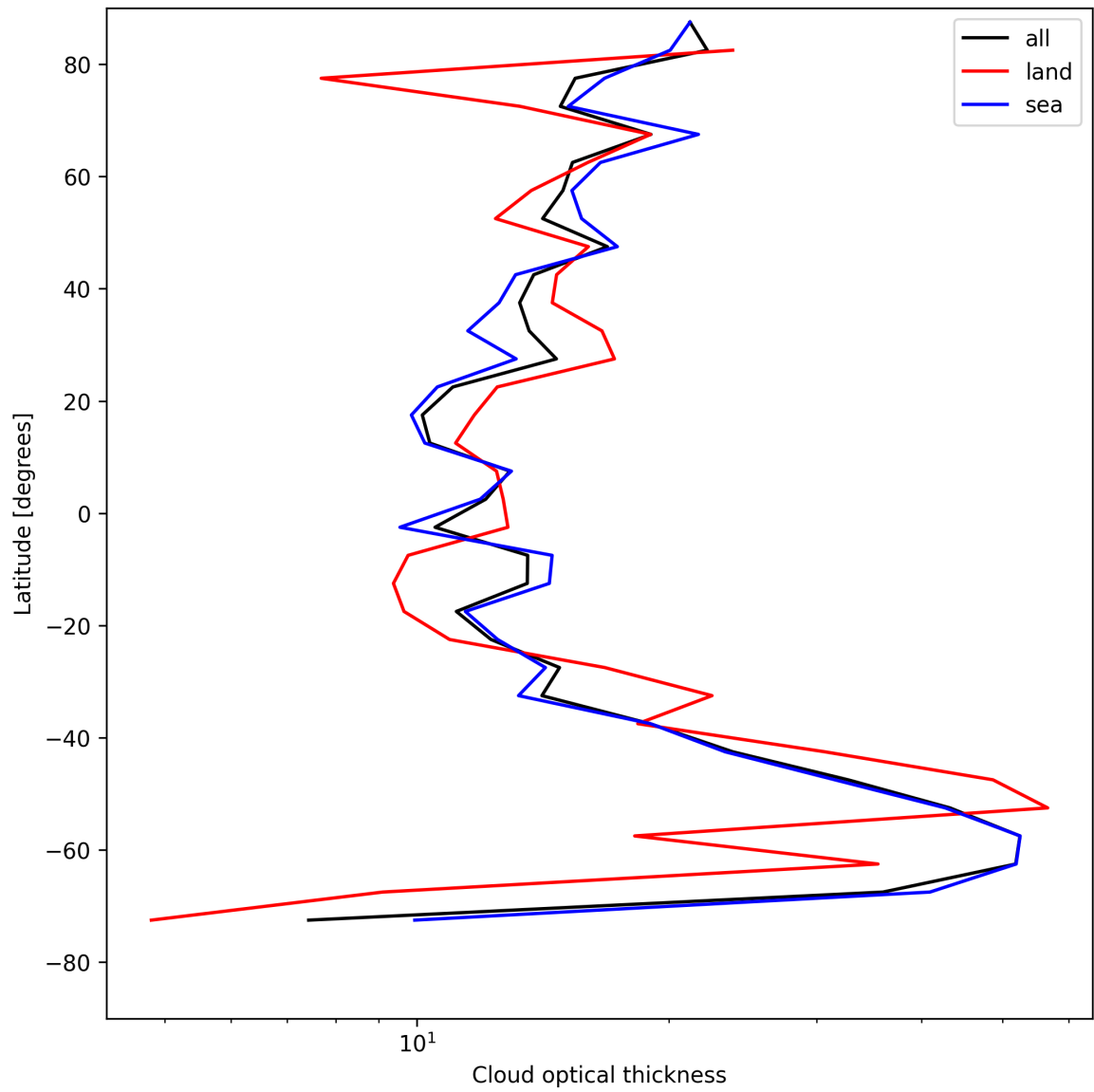
Figure 25: Zonal average of “Cloud optical thickness” for 2025-05-07 to 2025-05-09.
