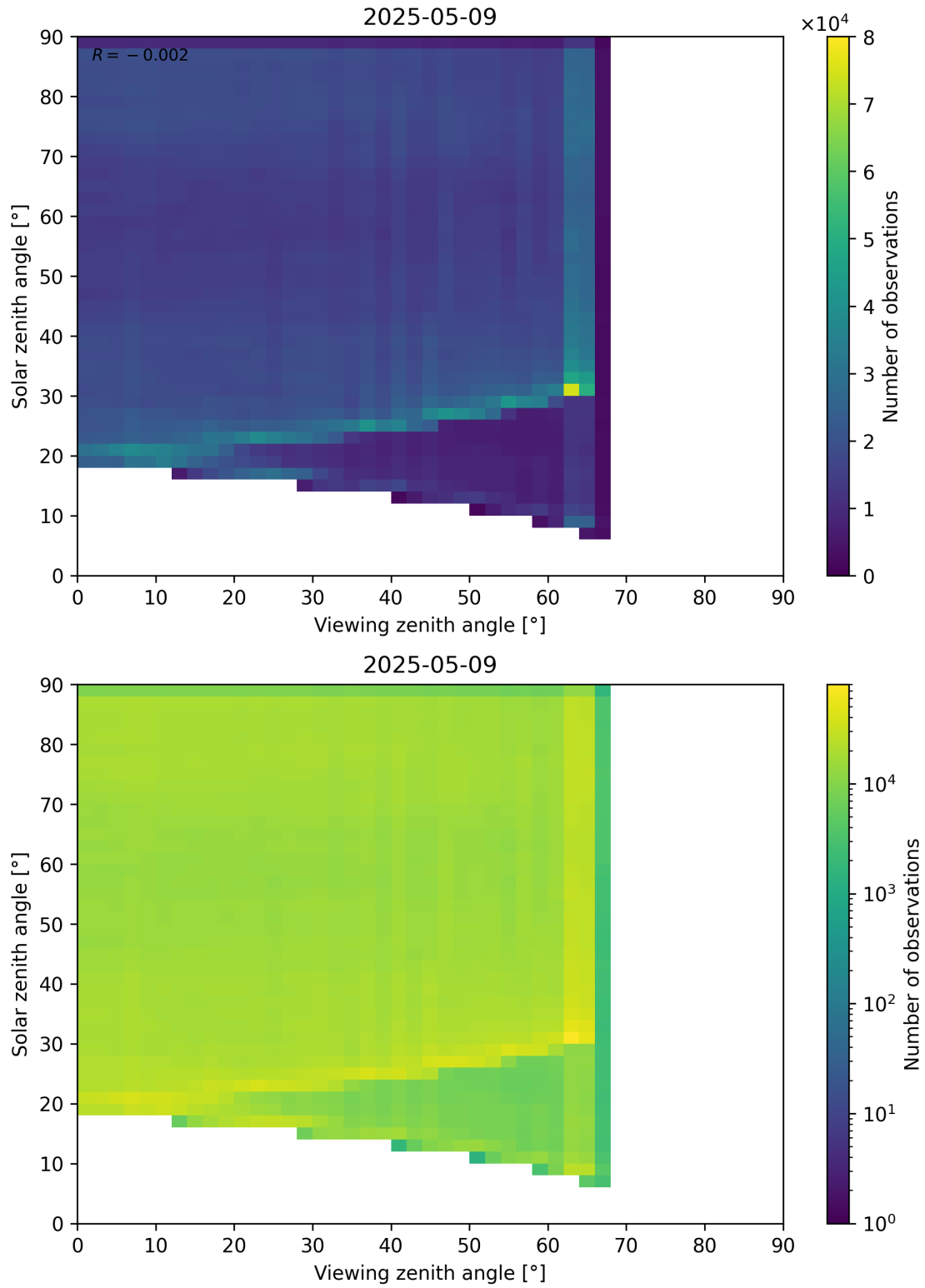
Figure 114: Scatter density plot of “Viewing zenith angle” against “Solar zenith angle” for 2025-05-08 to 2025-05-10.
