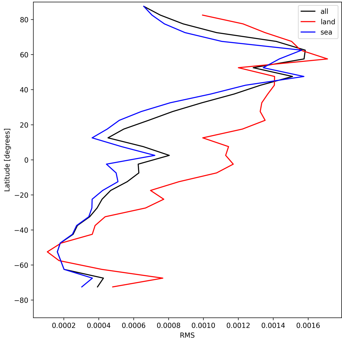
Figure 31: Zonal average of “RMS” for 2025-05-08 to 2025-05-10.
