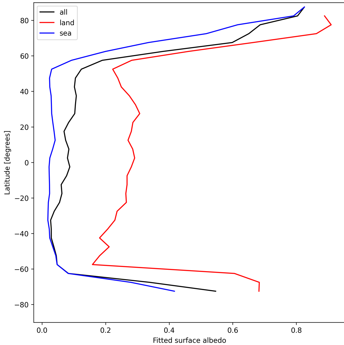
Figure 29: Zonal average of “Fitted surface albedo” for 2025-05-08 to 2025-05-10.
