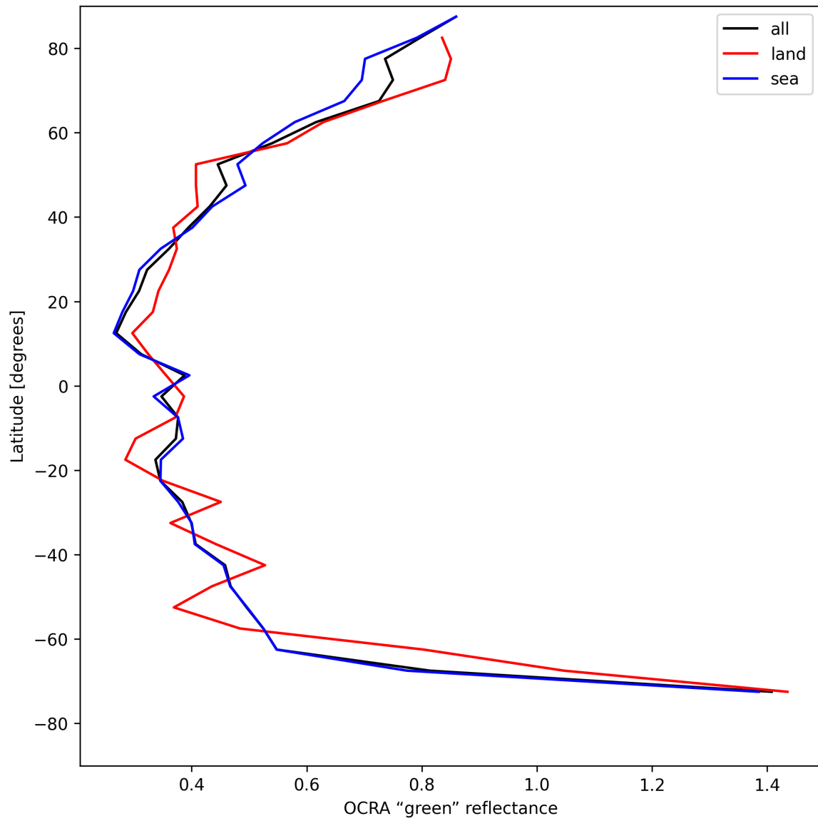
Figure 36: Zonal average of “OCRA “green” reflectance” for 2025-05-08 to 2025-05-10.
