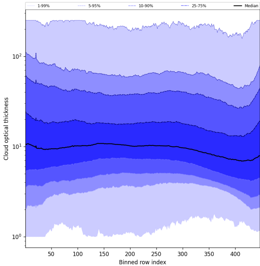
Figure 57: Along track statistics of “Cloud optical thickness” for 2025-05-08 to 2025-05-10
