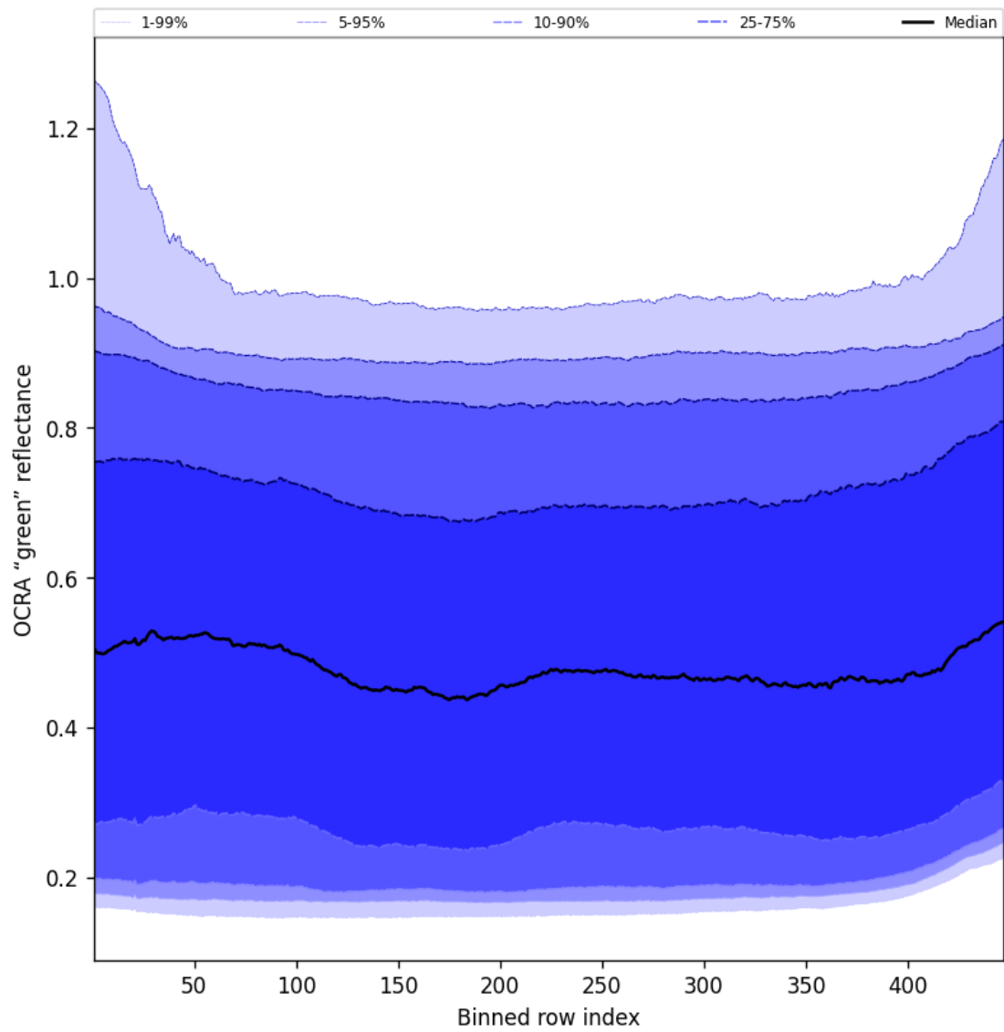
Figure 68: Along track statistics of "OCRA "green" reflectance" for 2025-05-08 to 2025-05-10
