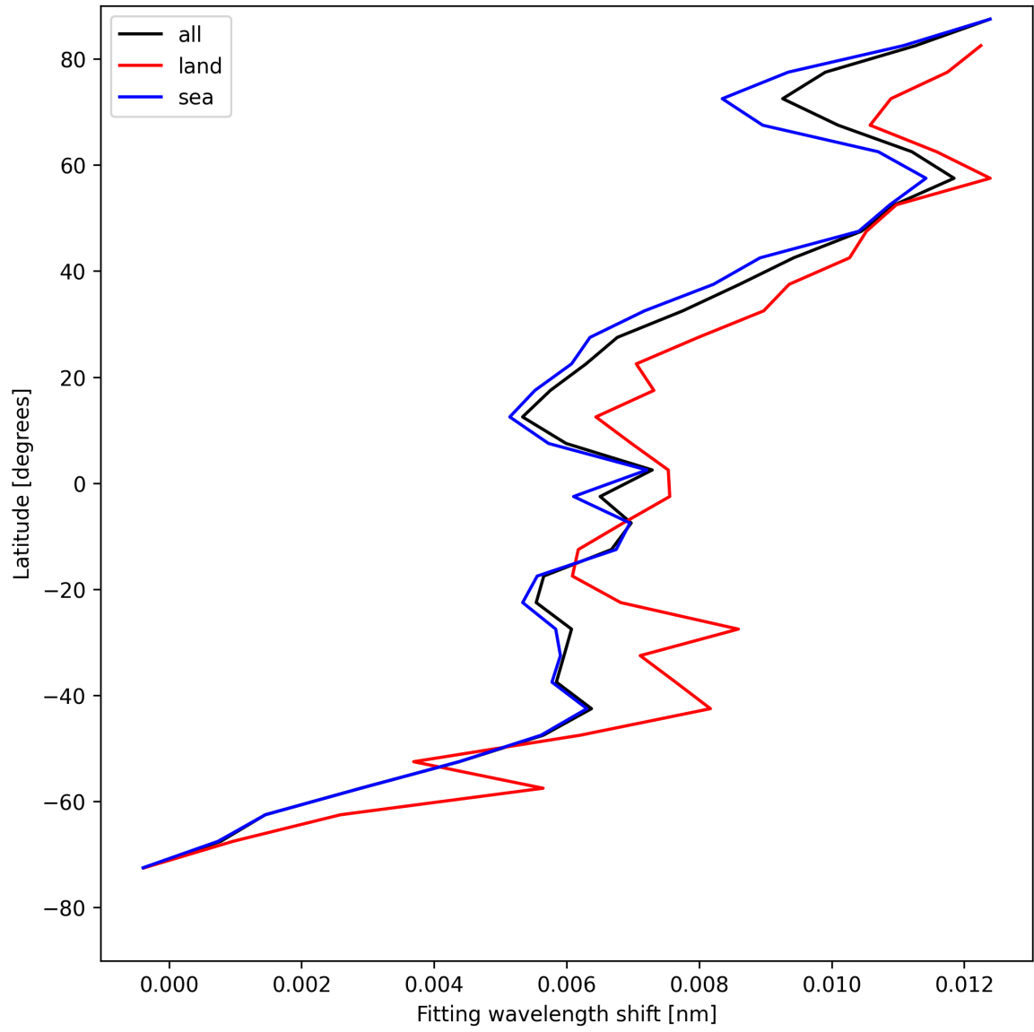
Figure 33: Zonal average of “Fitting wavelength shift” for 2025-05-08 to 2025-05-10.
