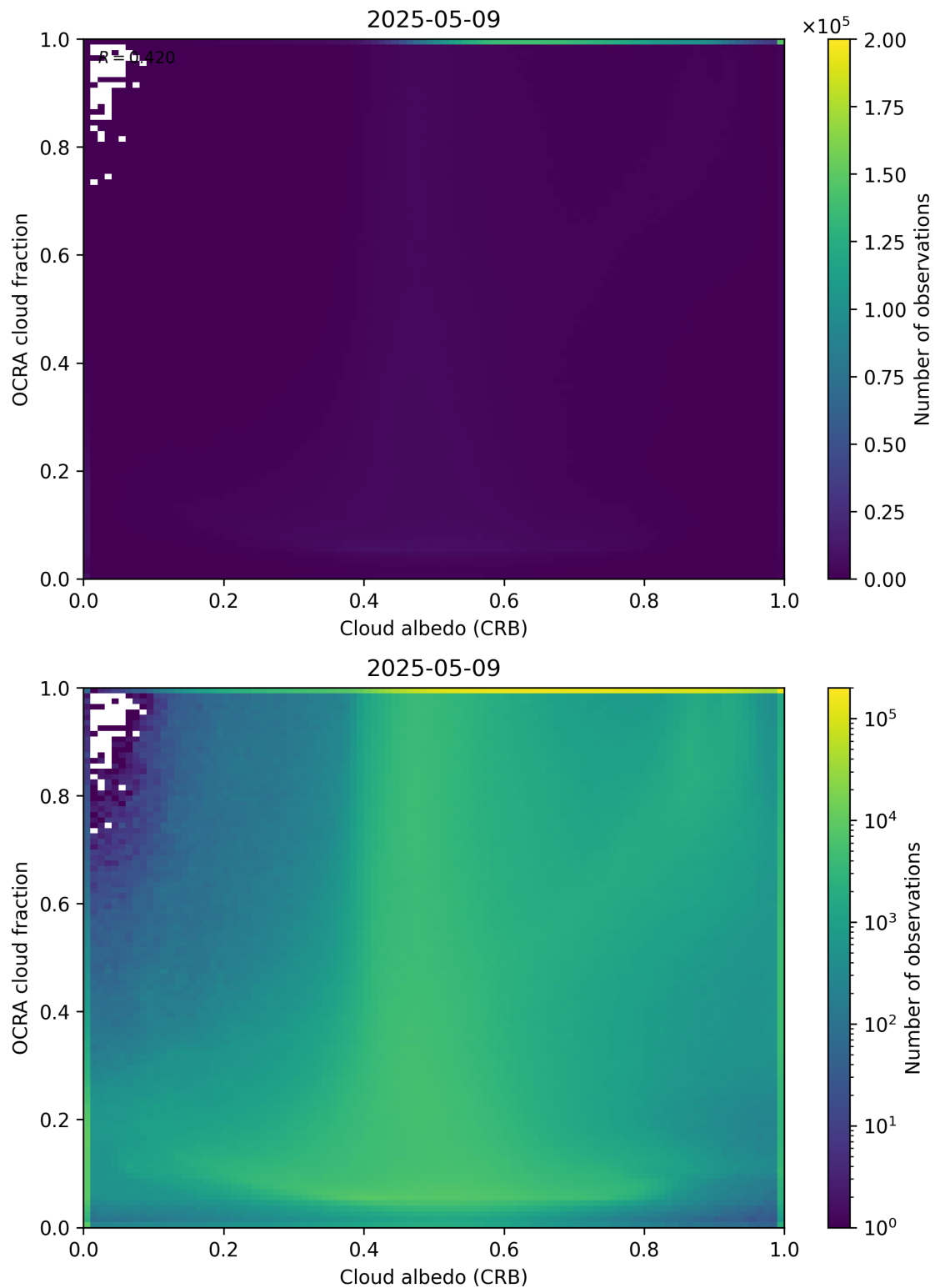
Figure 70: Scatter density plot of “Cloud albedo (CRB)” against “OCRA cloud fraction” for 2025-05-08 to 2025-05-10.
