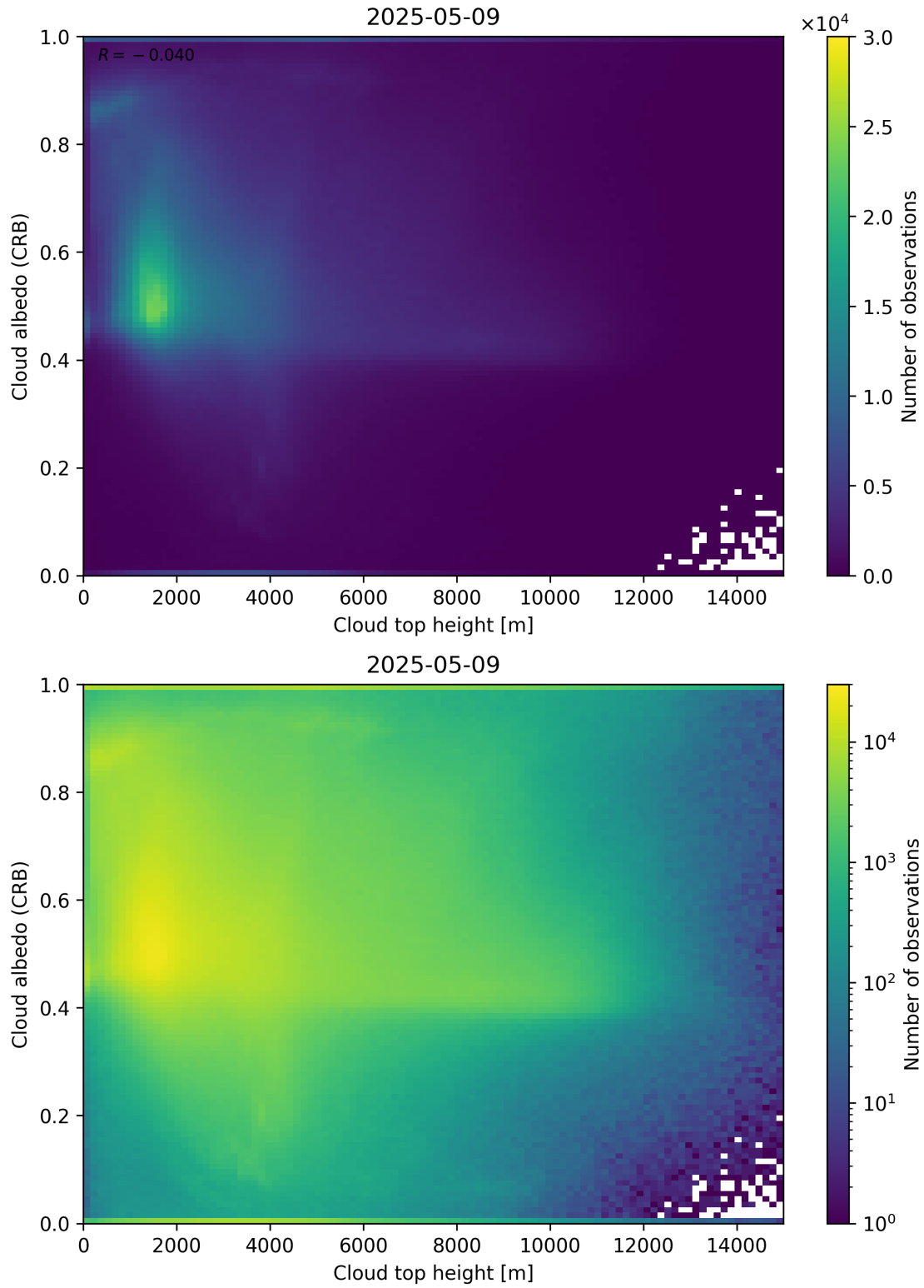
Figure 86: Scatter density plot of “Cloud top height” against “Cloud albedo (CRB)” for 2025-05-08 to 2025-05-10.
