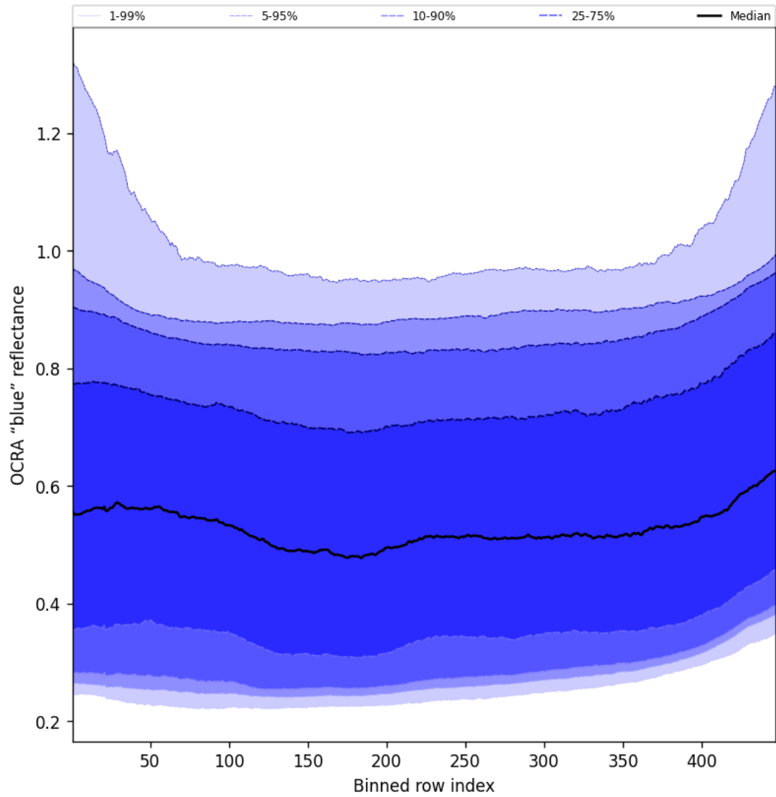
Figure 67: Along track statistics of “OCRA “blue” reflectance” for 2025-05-08 to 2025-05-10
