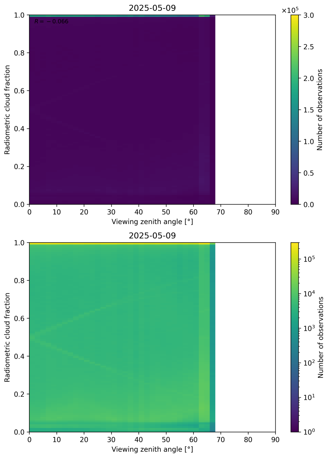
Figure 107: Scatter density plot of “Viewing zenith angle” against “Radiometric cloud fraction” for 2025-05-08 to 2025-05-10.
