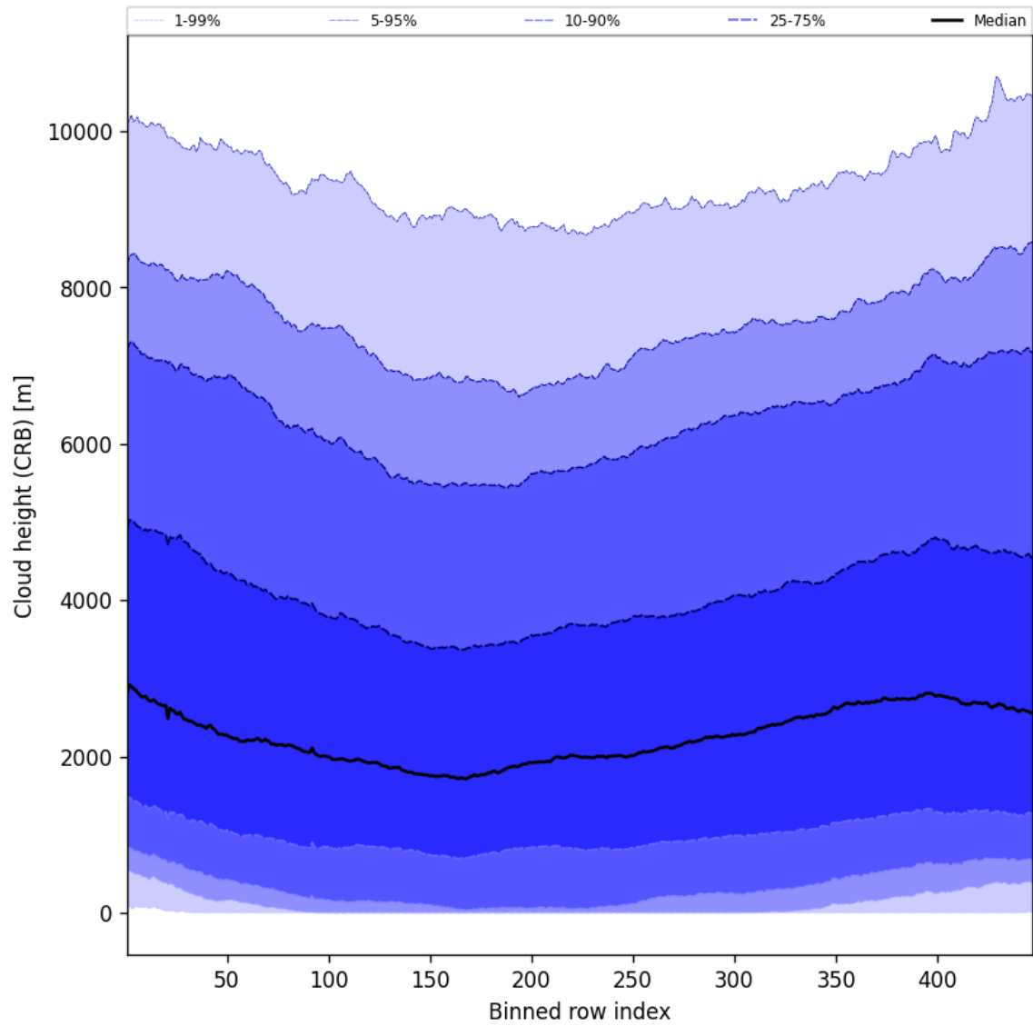
Figure 59: Along track statistics of “Cloud height (CRB)” for 2025-05-08 to 2025-05-10
