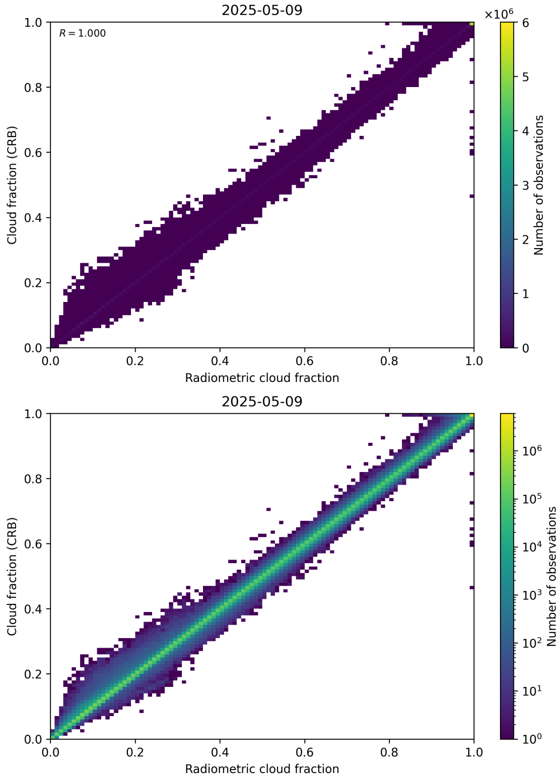
Figure 73: Scatter density plot of “Radiometric cloud fraction” against “Cloud fraction (CRB)” for 2025-05-08 to 2025-05-10.
