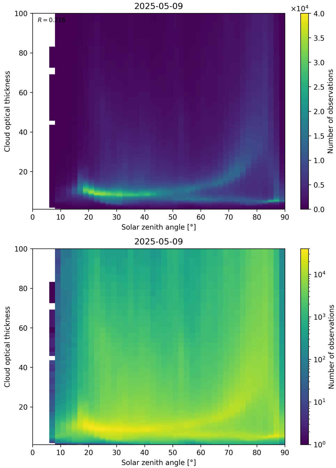
Figure 103: Scatter density plot of “Solar zenith angle” against “Cloud optical thickness” for 2025-05-08 to 2025-05-10.
