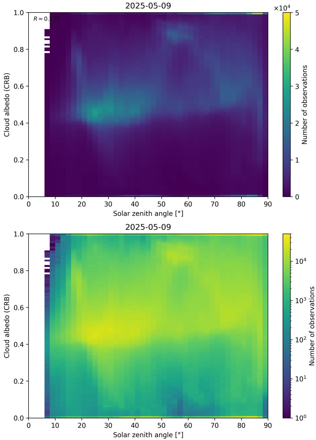
Figure 98: Scatter density plot of “Solar zenith angle” against “Cloud albedo (CRB)” for 2025-05-08 to 2025-05-10.
