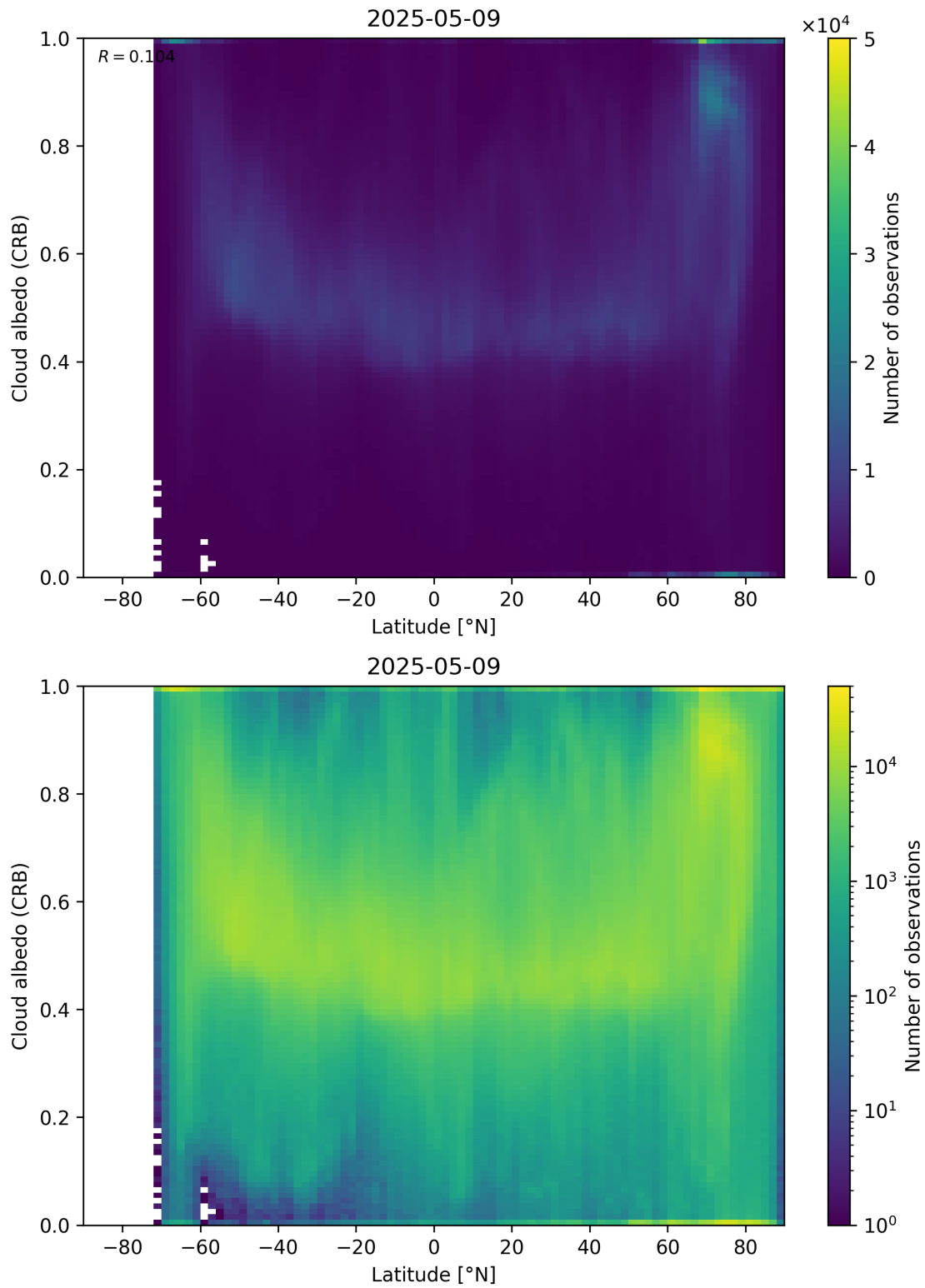
Figure 91: Scatter density plot of “Latitude” against “Cloud albedo (CRB)” for 2025-05-08 to 2025-05-10.
