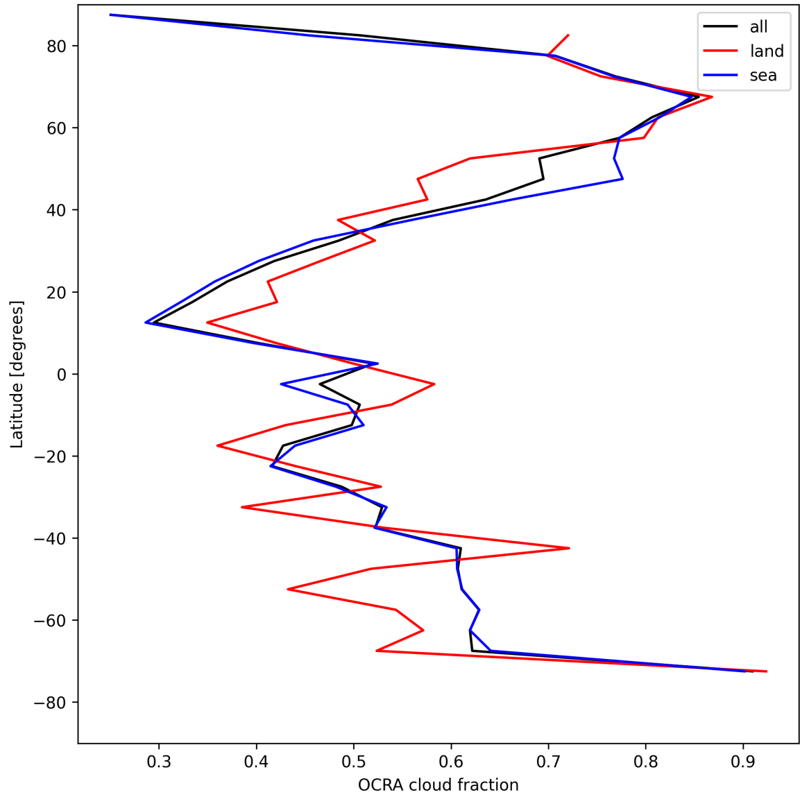
Figure 34: Zonal average of “OCRA cloud fraction” for 2025-05-08 to 2025-05-10.
