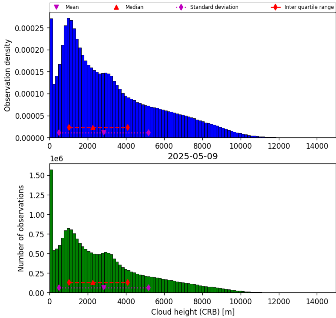
Figure 43: Histogram of “Cloud height (CRB)” for 2025-05-08 to 2025-05-10
