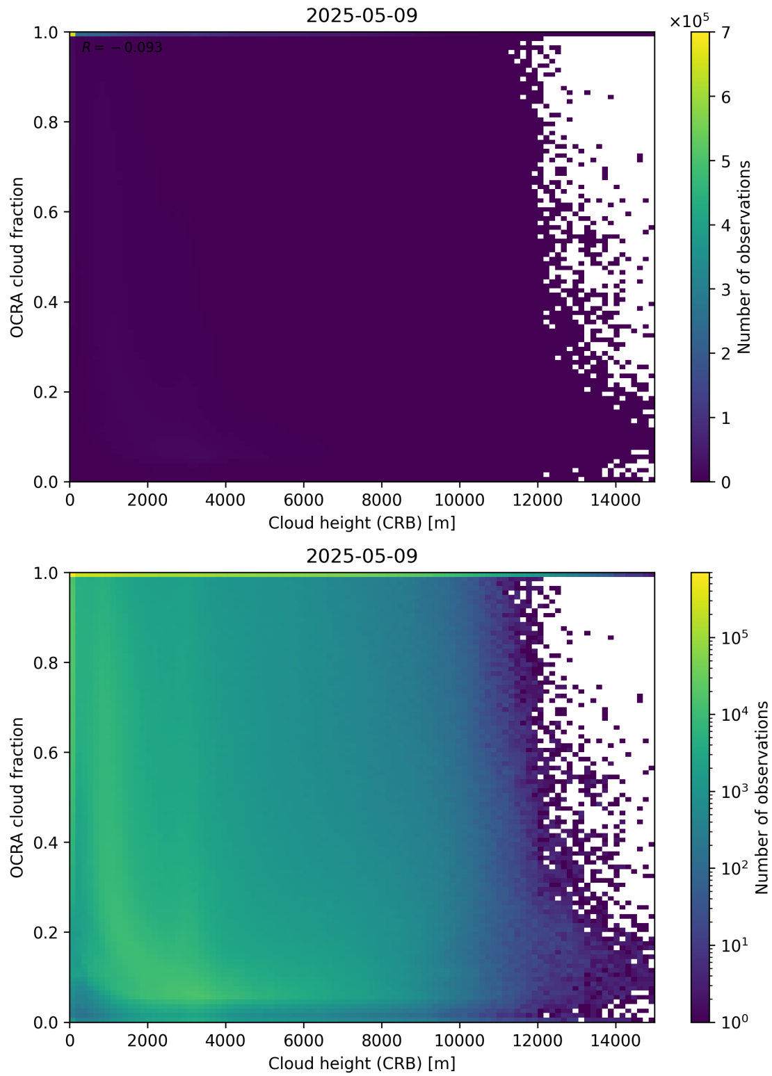
Figure 81: Scatter density plot of “Cloud height (CRB)” against “OCRA cloud fraction” for 2025-05-08 to 2025-05-10.
