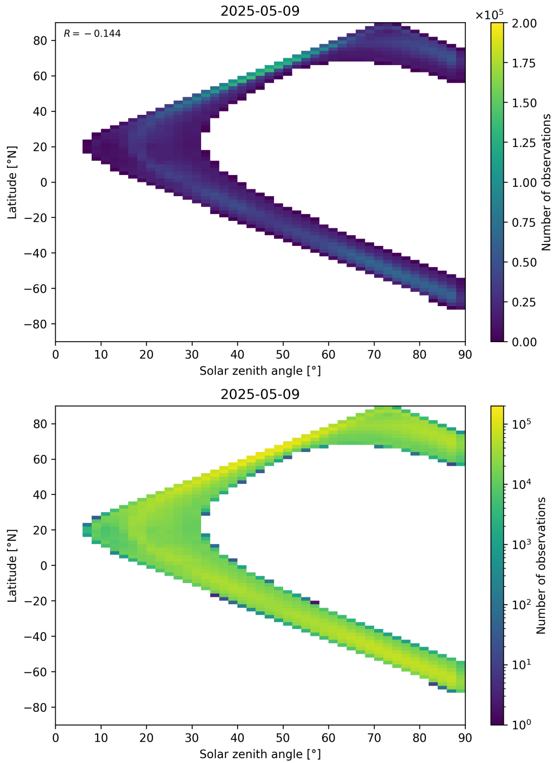
Figure 105: Scatter density plot of “Solar zenith angle” against “Latitude” for 2025-05-08 to 2025-05-10.
