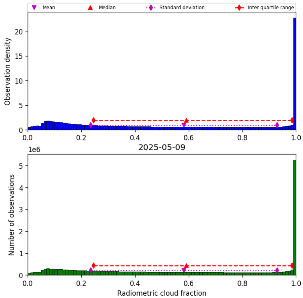
Figure 39: Histogram of “Radiometric cloud fraction” for 2025-05-08 to 2025-05-10
