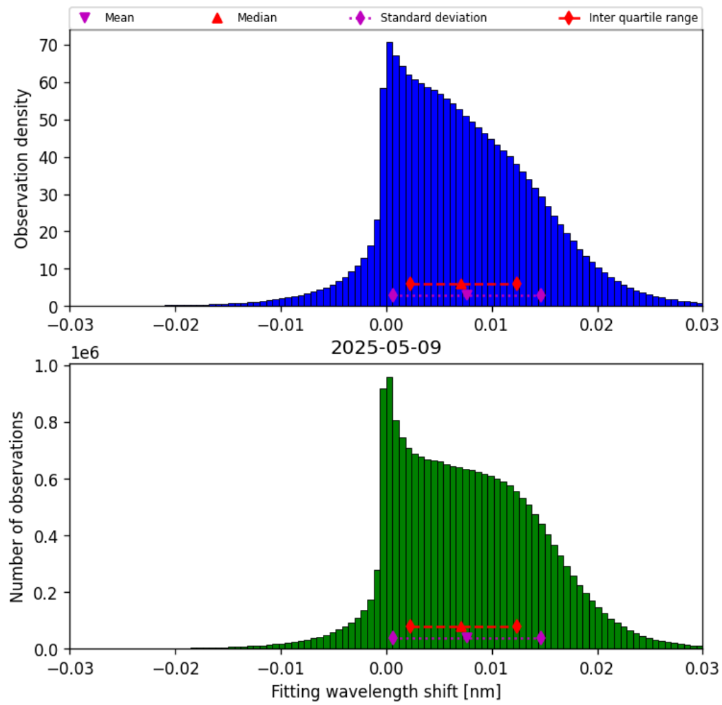
Figure 49: Histogram of “Fitting wavelength shift” for 2025-05-08 to 2025-05-10
