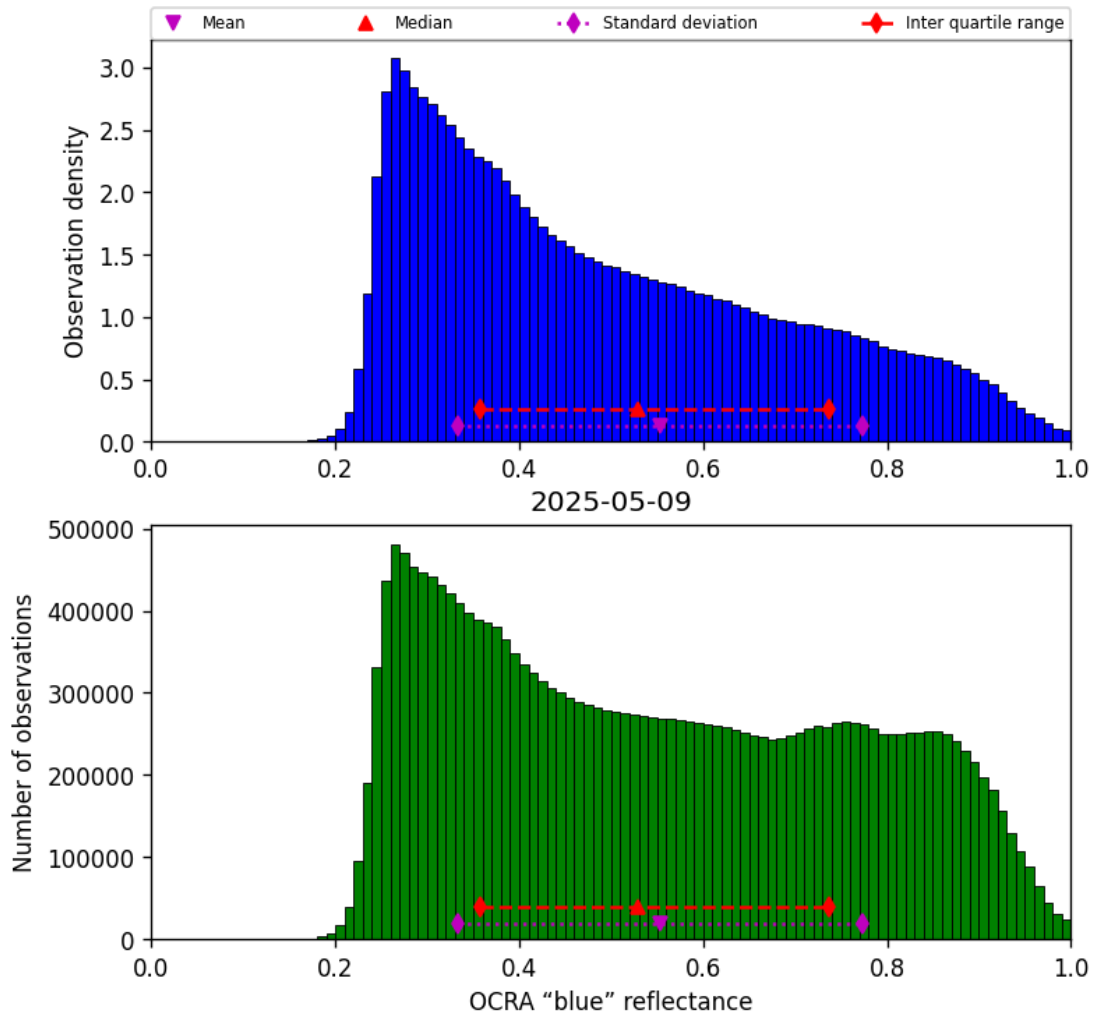
Figure 51: Histogram of “OCRA “blue” reflectance” for 2025-05-08 to 2025-05-10
