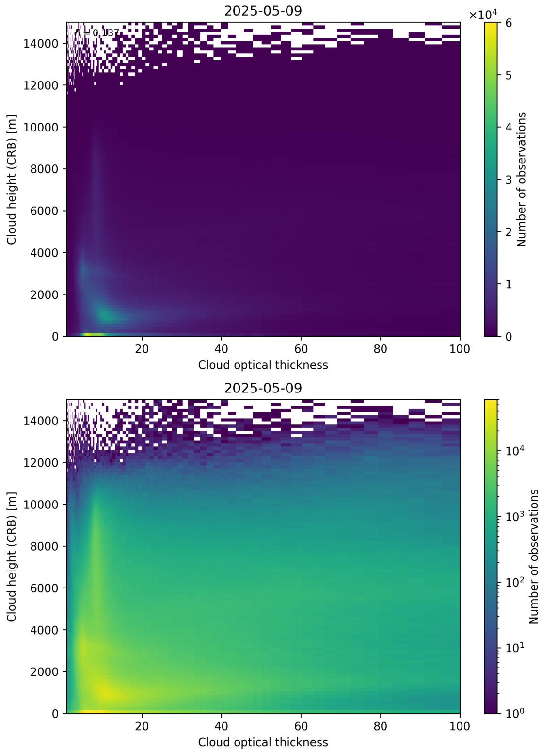
Figure 85: Scatter density plot of “Cloud optical thickness” against “Cloud height (CRB)” for 2025-05-08 to 2025-05-10.
