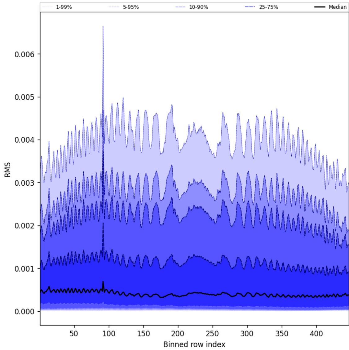
Figure 63: Along track statistics of “RMS” for 2025-05-08 to 2025-05-10
