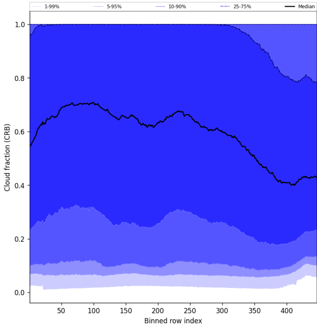
Figure 58: Along track statistics of “Cloud fraction (CRB)” for 2025-05-08 to 2025-05-10
