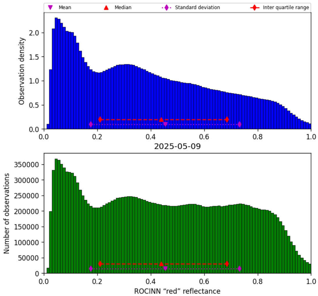
Figure 53: Histogram of “ROCINN “red” reflectance” for 2025-05-08 to 2025-05-10
