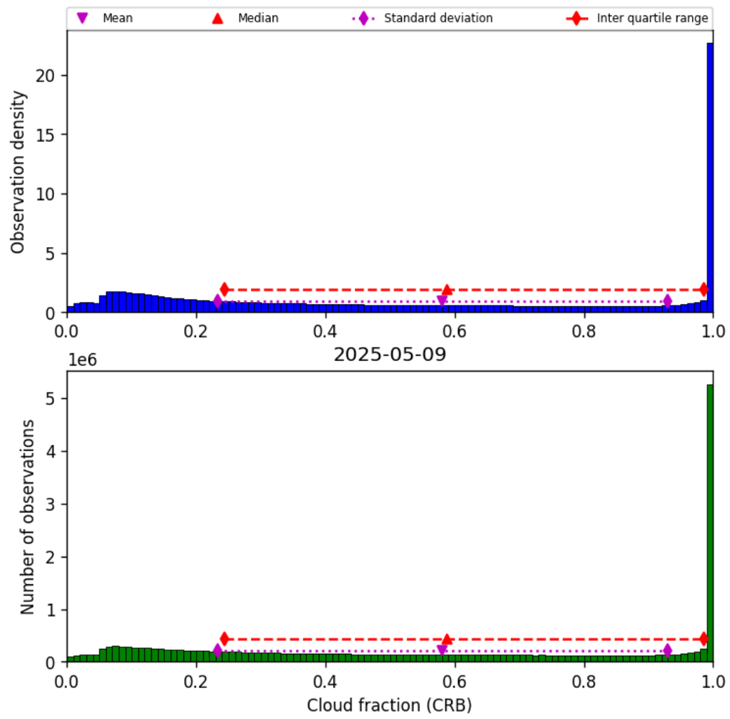
Figure 42: Histogram of “Cloud fraction (CRB)” for 2025-05-08 to 2025-05-10
