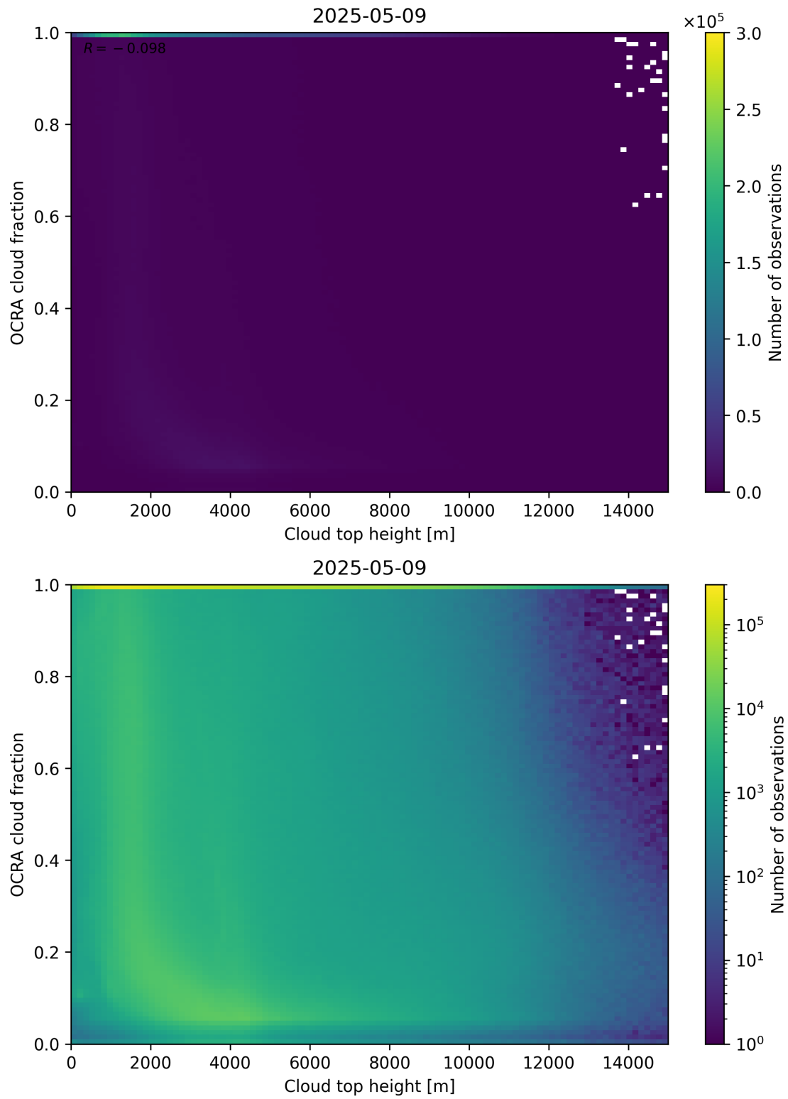
Figure 87: Scatter density plot of “Cloud top height” against “OCRA cloud fraction” for 2025-05-08 to 2025-05-10.
