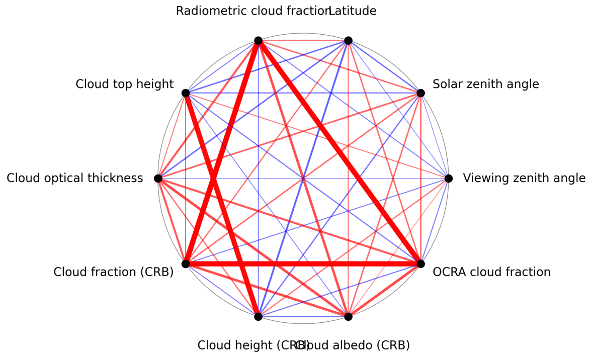
Figure 1: Map of correlation graph for 2025-05-08 to 2025-05-10.
