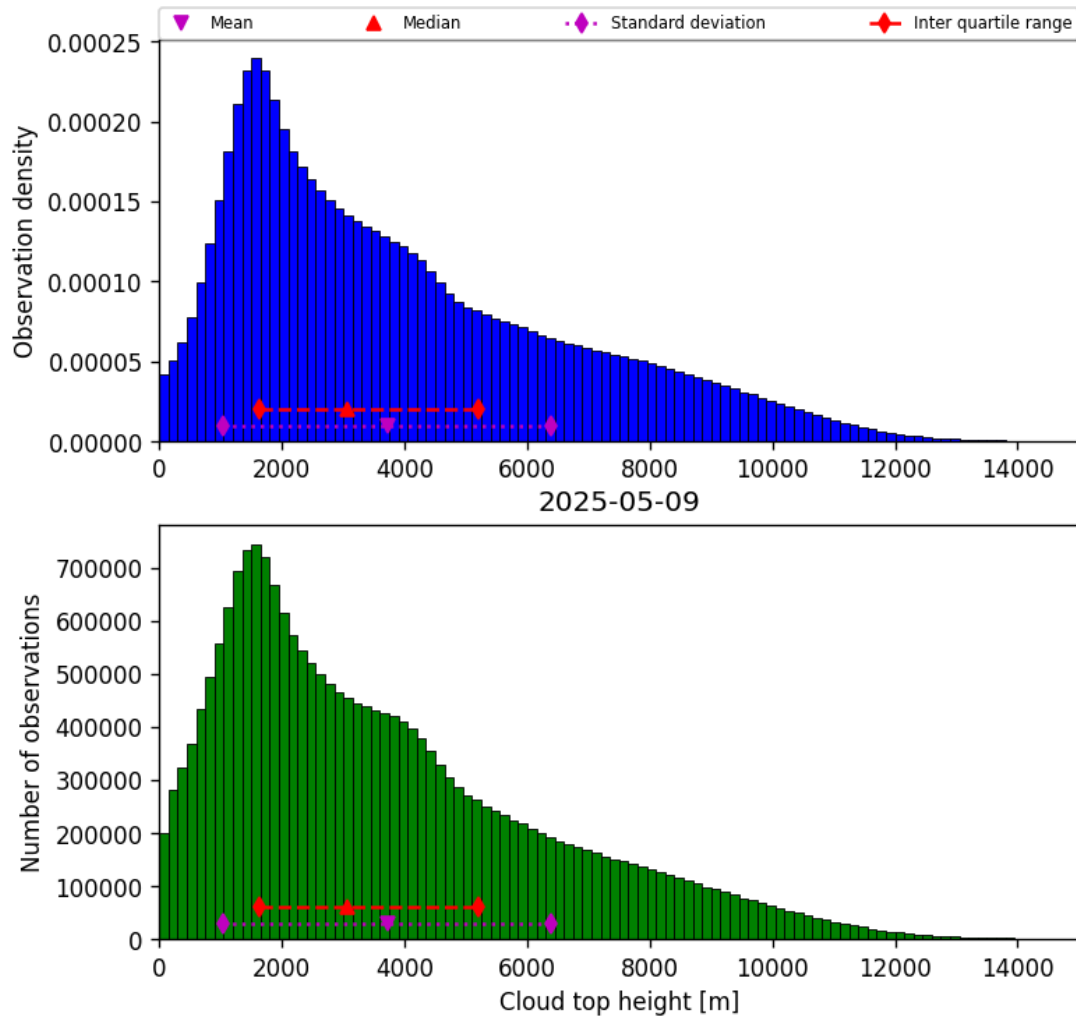
Figure 40: Histogram of “Cloud top height” for 2025-05-08 to 2025-05-10
