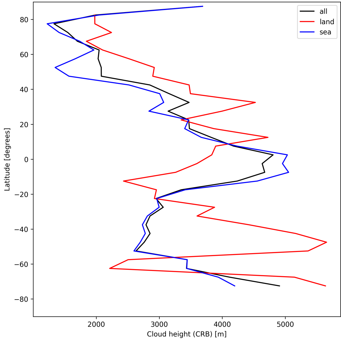
Figure 27: Zonal average of “Cloud height (CRB)” for 2025-05-08 to 2025-05-10.
