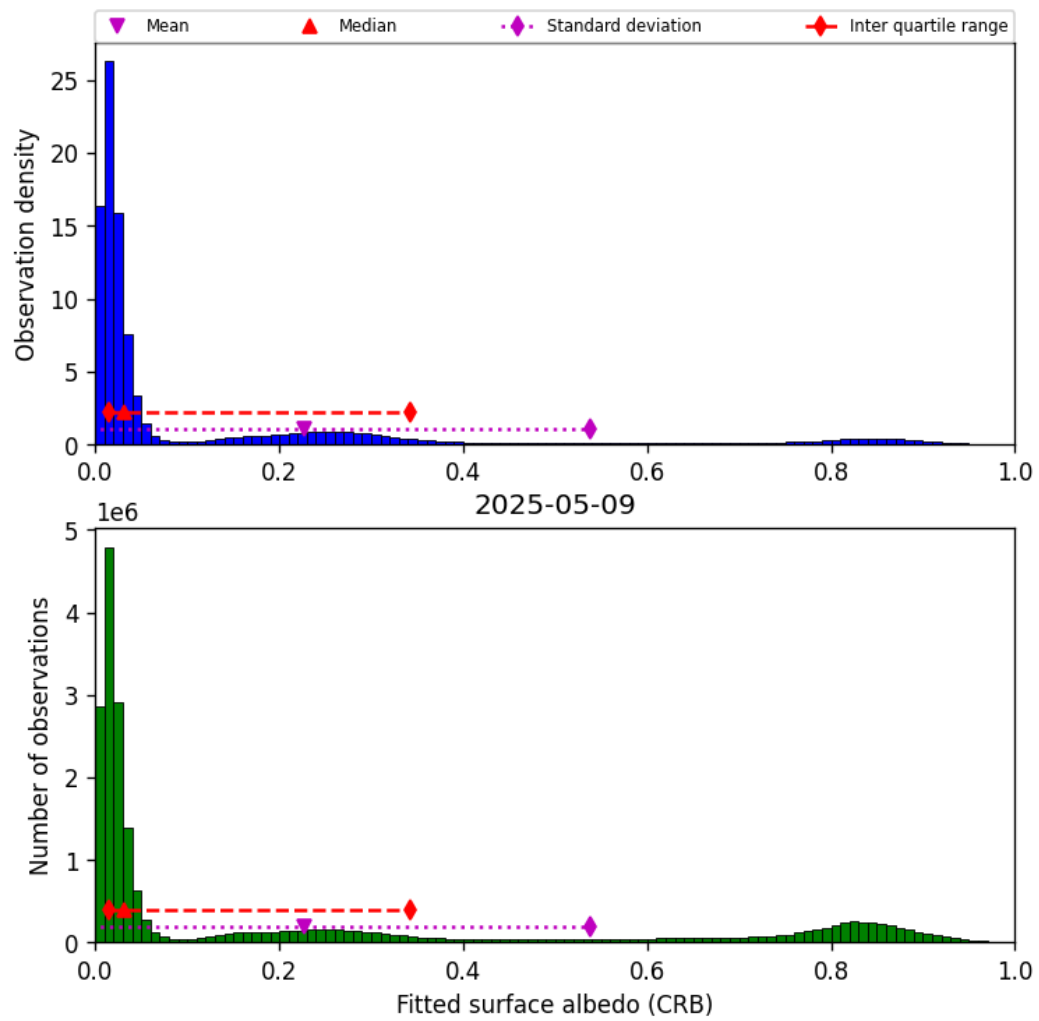
Figure 46: Histogram of “Fitted surface albedo (CRB)” for 2025-05-08 to 2025-05-10
