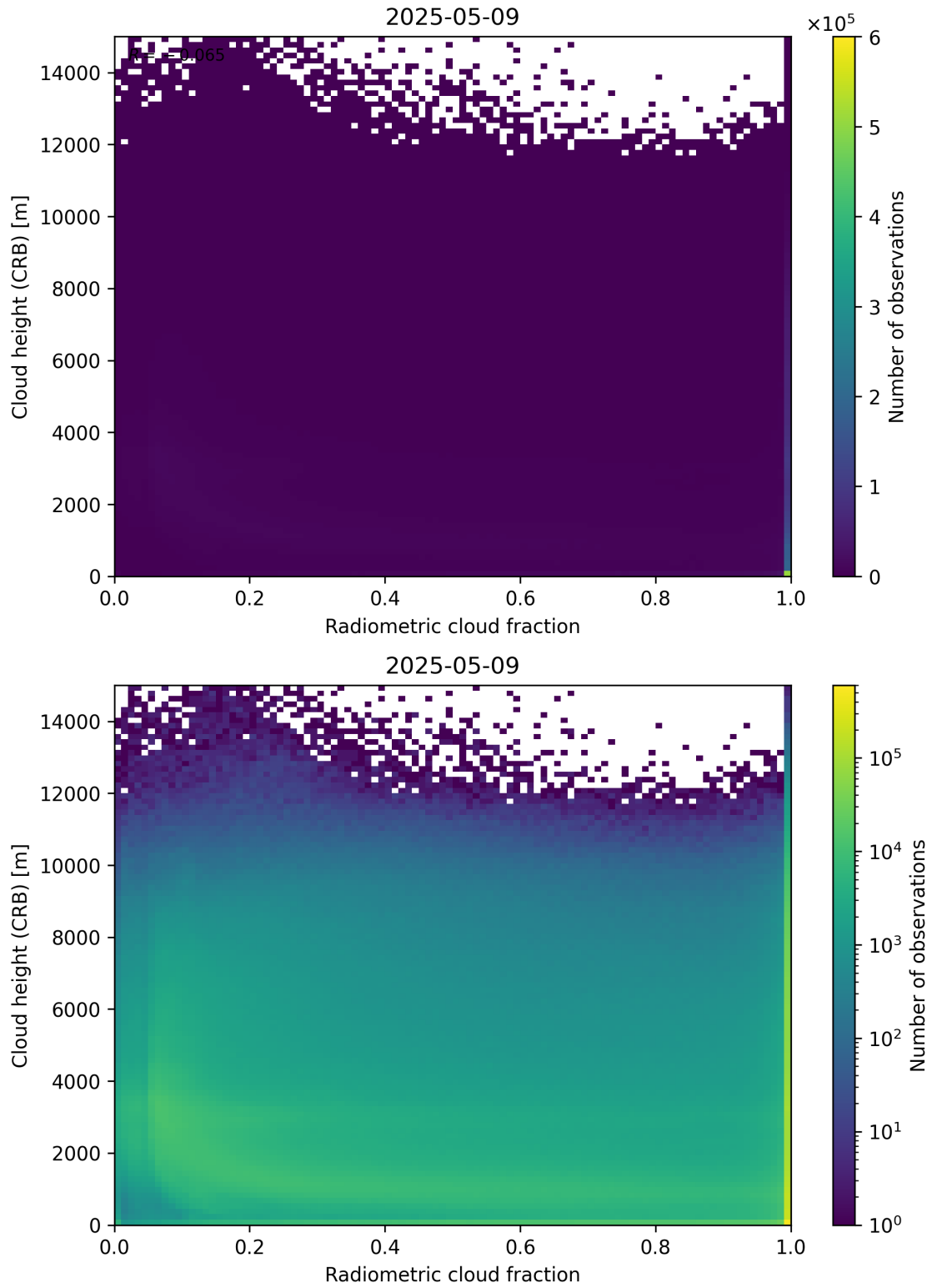
Figure 74: Scatter density plot of “Radiometric cloud fraction” against “Cloud height (CRB)” for 2025-05-08 to 2025-05-10.
