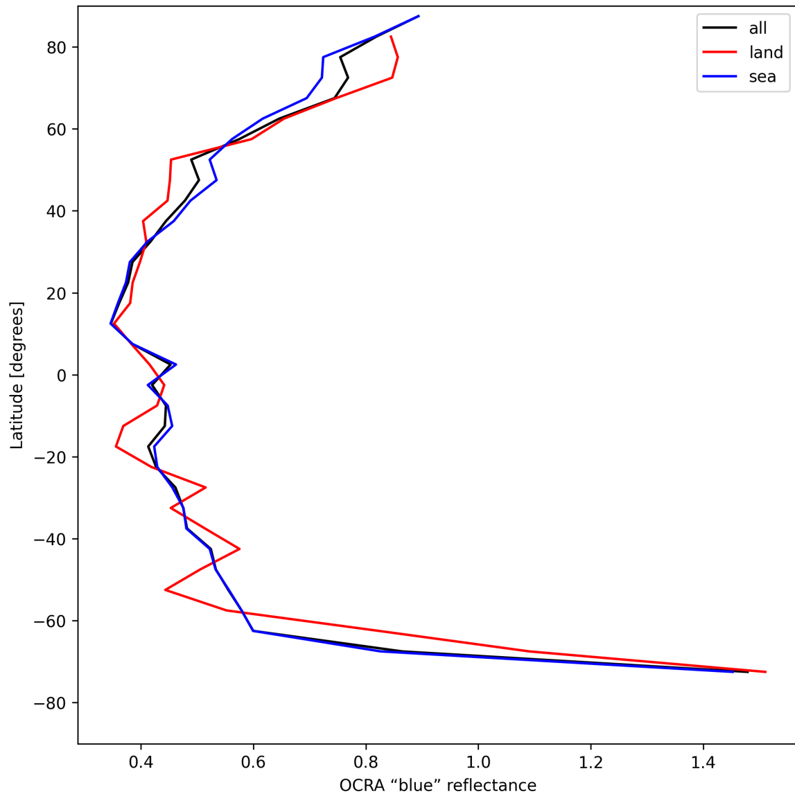
Figure 35: Zonal average of “OCRA “blue” reflectance” for 2025-05-08 to 2025-05-10.
