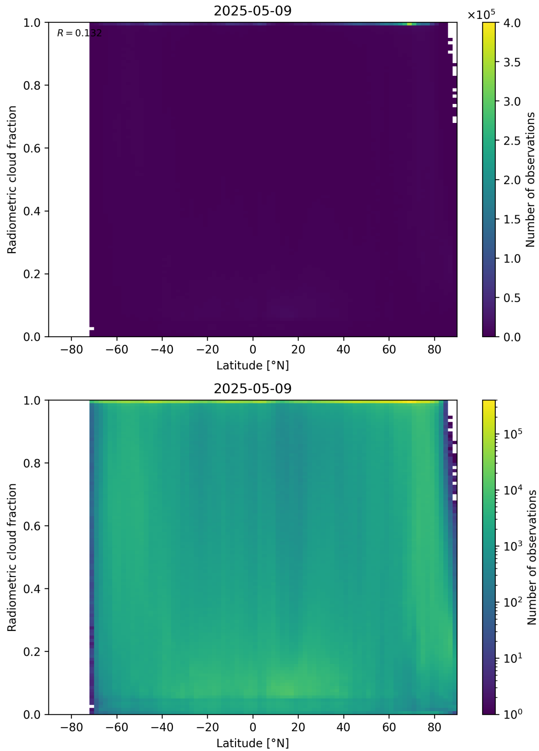
Figure 92: Scatter density plot of “Latitude” against “Radiometric cloud fraction” for 2025-05-08 to 2025-05-10.
