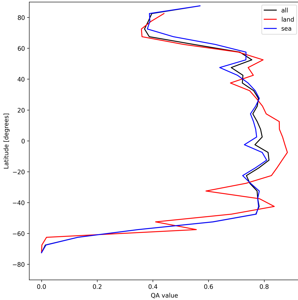
Figure 22: Zonal average of “QA value” for 2025-05-08 to 2025-05-10.
