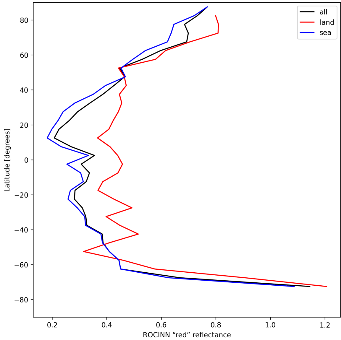
Figure 37: Zonal average of “ROCINN “red” reflectance” for 2025-05-08 to 2025-05-10.
