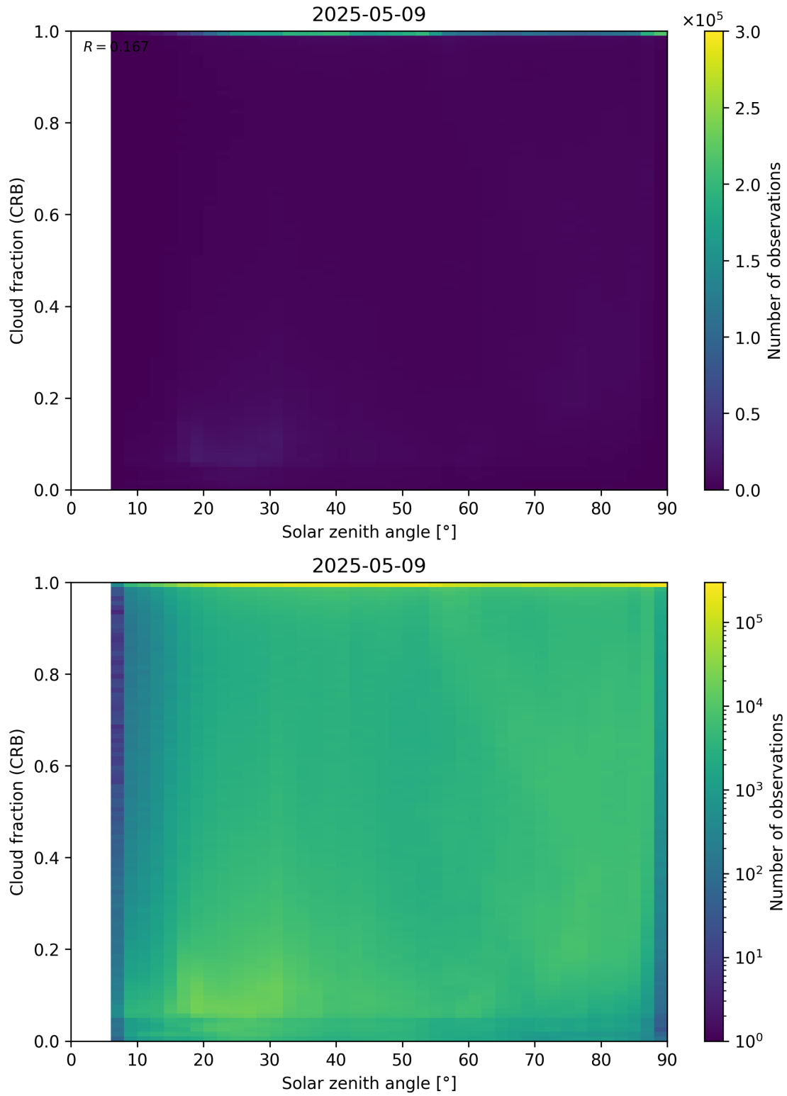
Figure 101: Scatter density plot of “Solar zenith angle” against “Cloud fraction (CRB)” for 2025-05-08 to 2025-05-10.
