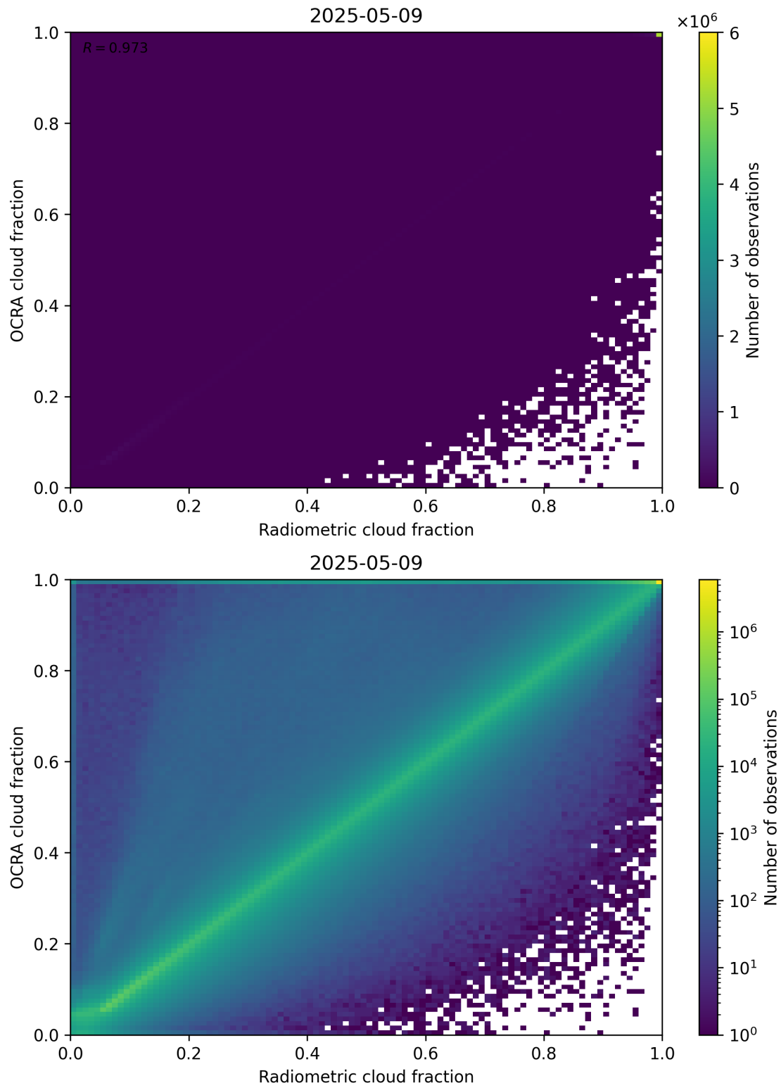
Figure 72: Scatter density plot of “Radiometric cloud fraction” against “OCRA cloud fraction” for 2025-05-08 to 2025-05-10.
