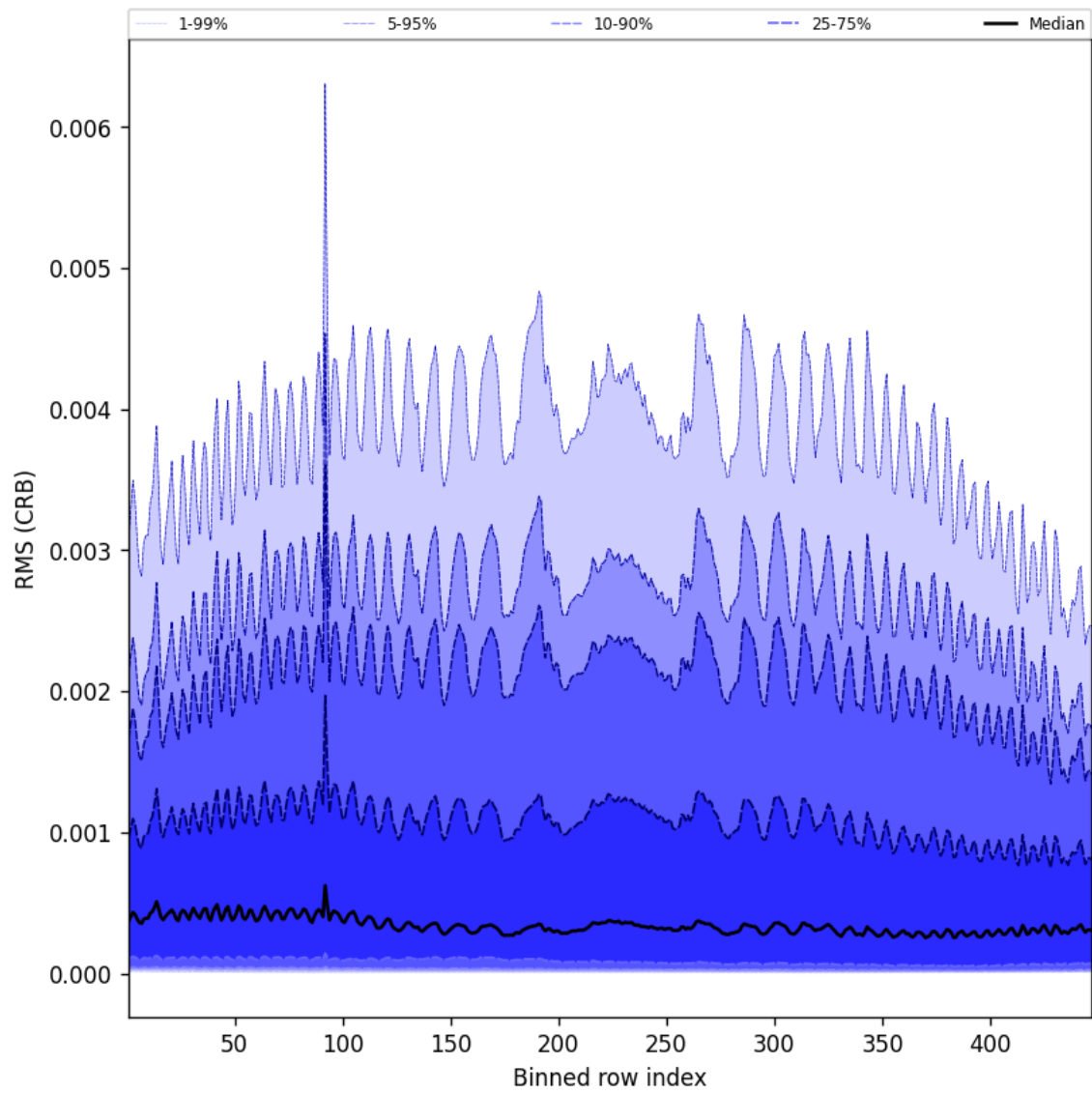
Figure 64: Along track statistics of “RMS (CRB)” for 2025-05-08 to 2025-05-10
