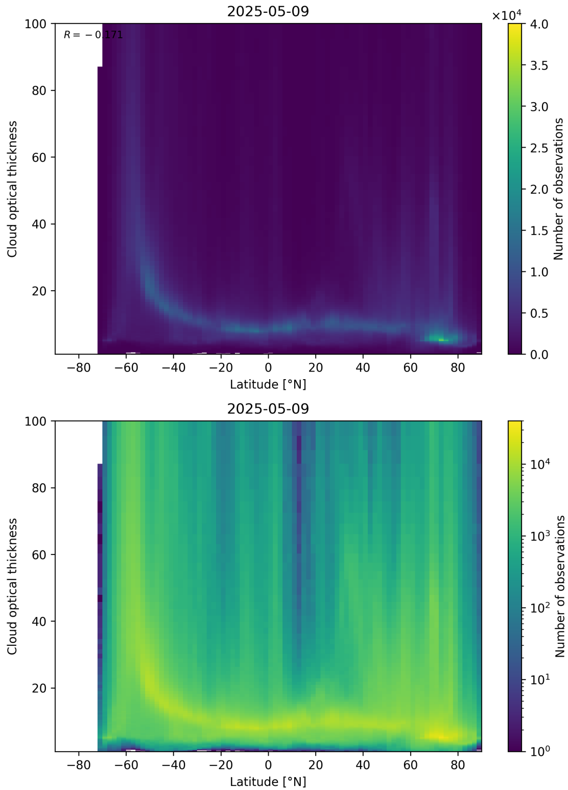
Figure 96: Scatter density plot of “Latitude” against “Cloud optical thickness” for 2025-05-08 to 2025-05-10.
