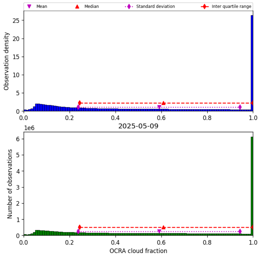
Figure 50: Histogram of “OCRA cloud fraction” for 2025-05-08 to 2025-05-10
