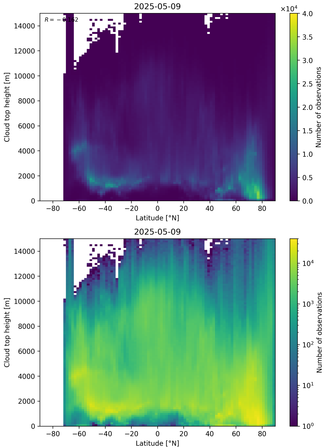
Figure 97: Scatter density plot of “Latitude” against “Cloud top height” for 2025-05-08 to 2025-05-10.
