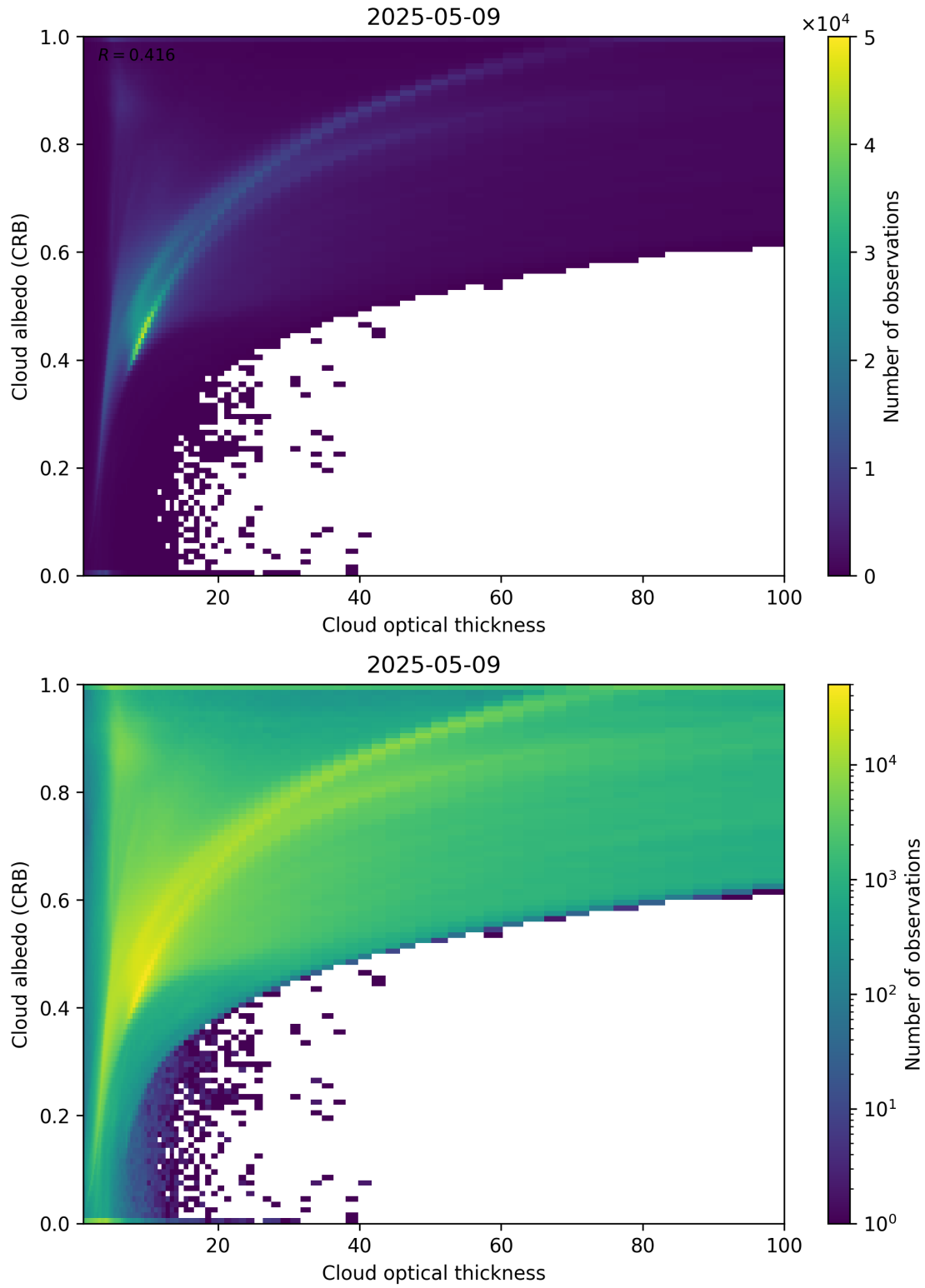
Figure 82: Scatter density plot of “Cloud optical thickness” against “Cloud albedo (CRB)” for 2025-05-08 to 2025-05-10.
