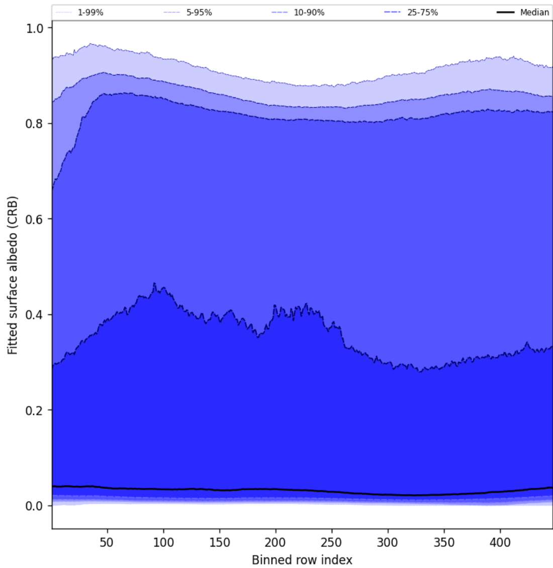
Figure 62: Along track statistics of “Fitted surface albedo (CRB)” for 2025-05-08 to 2025-05-10
