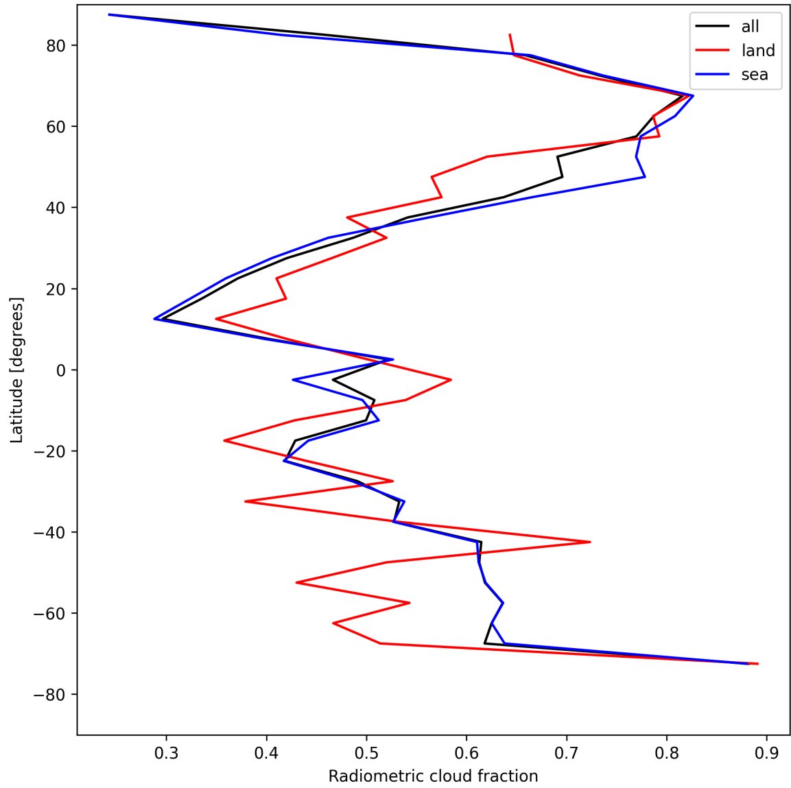
Figure 23: Zonal average of “Radiometric cloud fraction” for 2025-05-08 to 2025-05-10.
