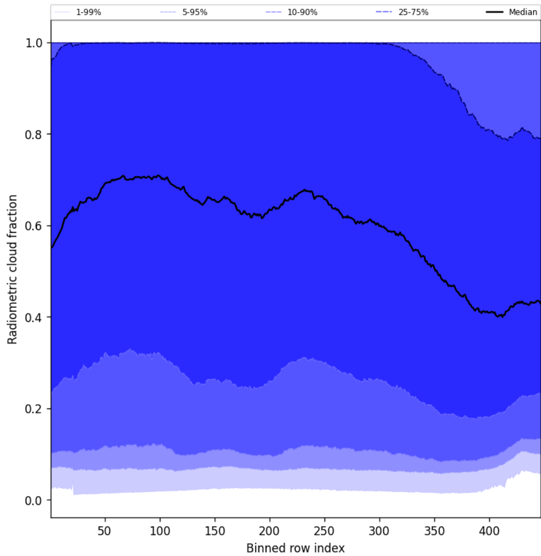
Figure 55: Along track statistics of “Radiometric cloud fraction” for 2025-05-08 to 2025-05-10
