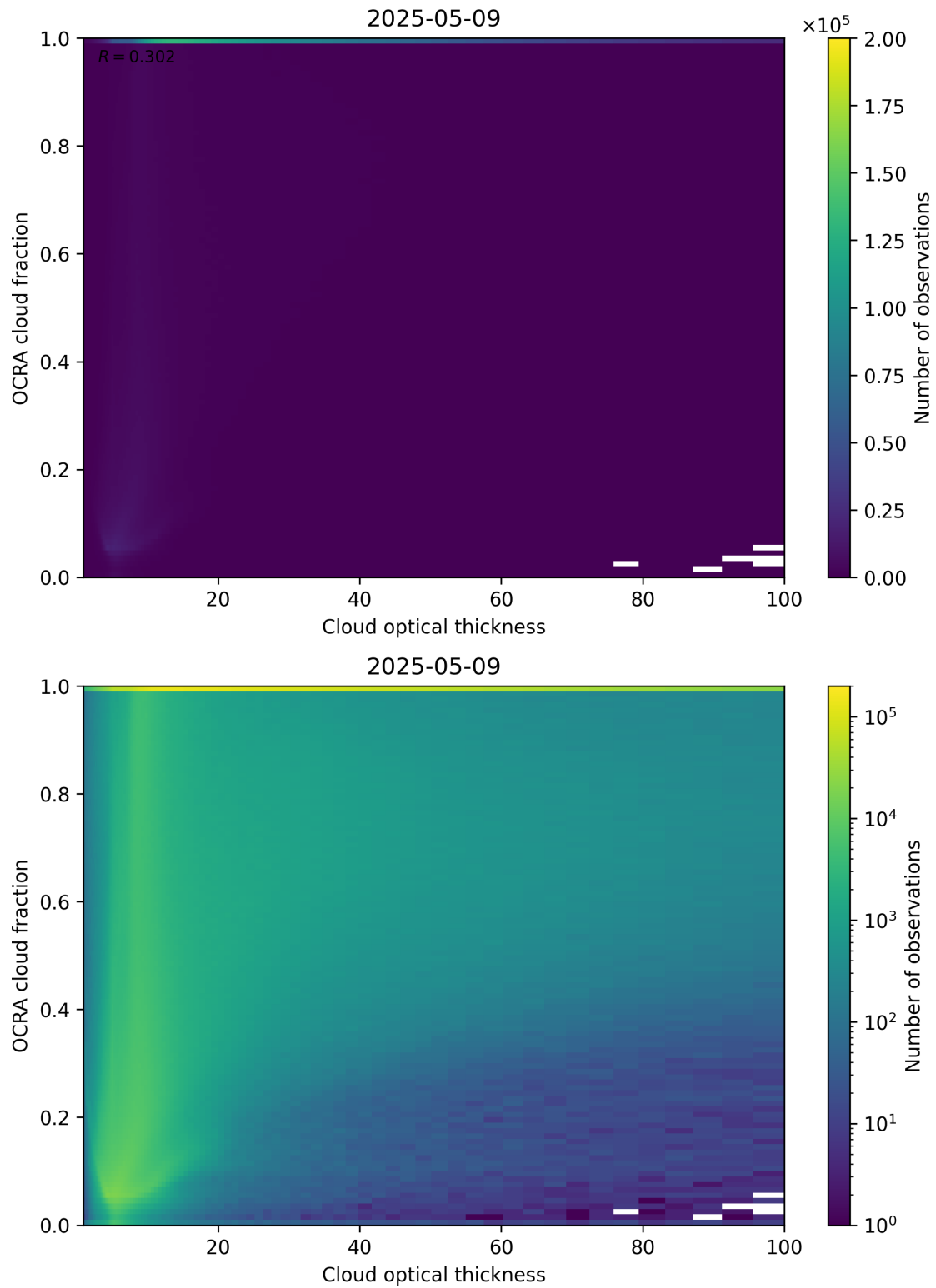
Figure 83: Scatter density plot of “Cloud optical thickness” against “OCRA cloud fraction” for 2025-05-08 to 2025-05-10.
