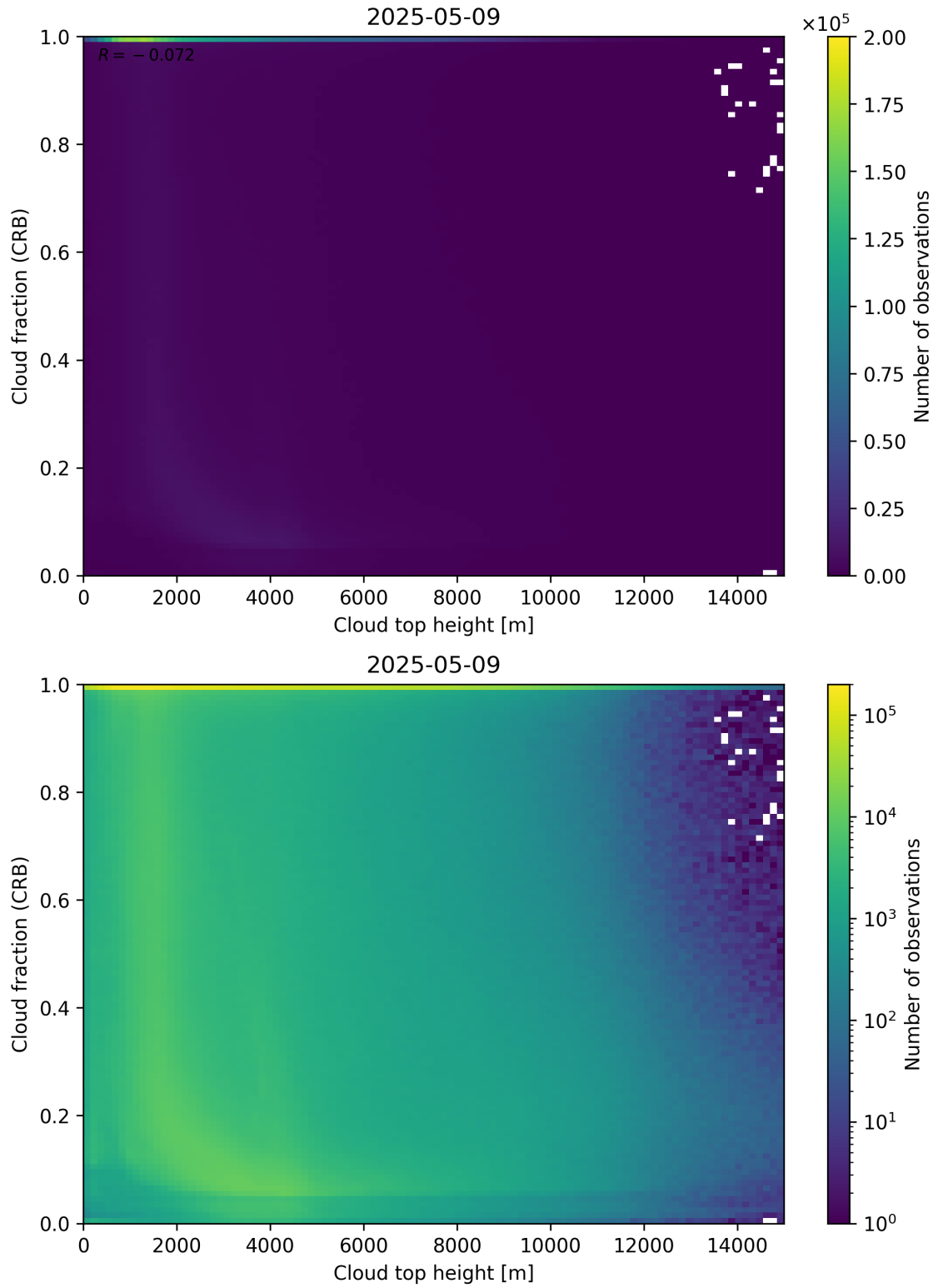
Figure 88: Scatter density plot of “Cloud top height” against “Cloud fraction (CRB)” for 2025-05-08 to 2025-05-10.
