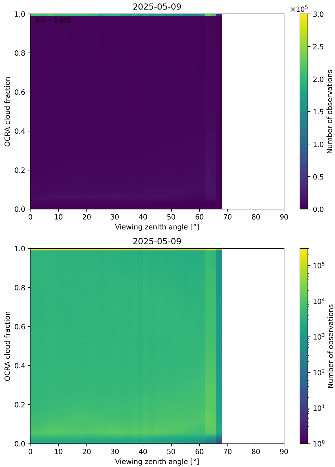
Figure 108: Scatter density plot of “Viewing zenith angle” against “OCRA cloud fraction” for 2025-05-08 to 2025-05-10.
