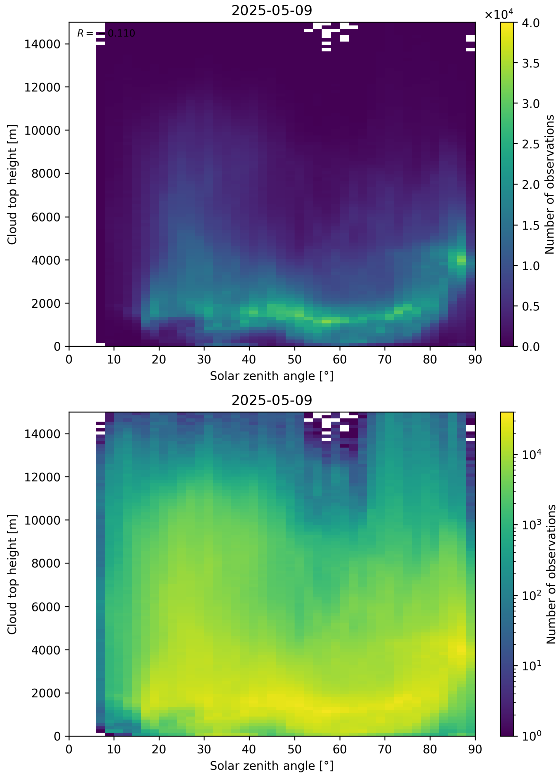
Figure 104: Scatter density plot of “Solar zenith angle” against “Cloud top height” for 2025-05-08 to 2025-05-10.
