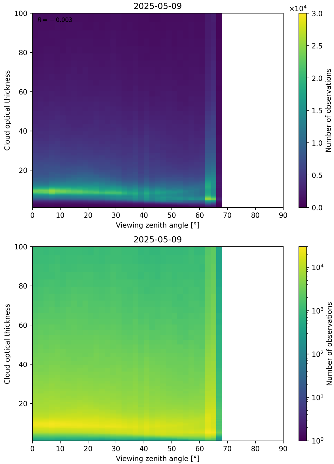
Figure 111: Scatter density plot of “Viewing zenith angle” against “Cloud optical thickness” for 2025-05-08 to 2025-05-10.
