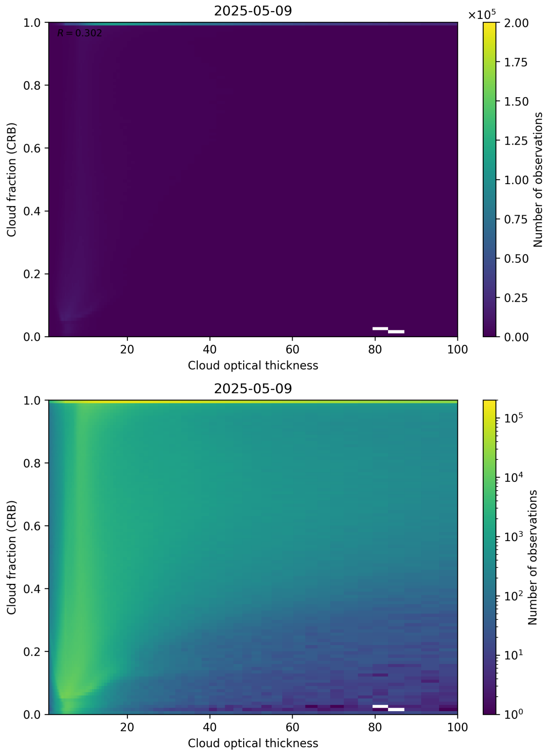
Figure 84: Scatter density plot of “Cloud optical thickness” against “Cloud fraction (CRB)” for 2025-05-08 to 2025-05-10.
