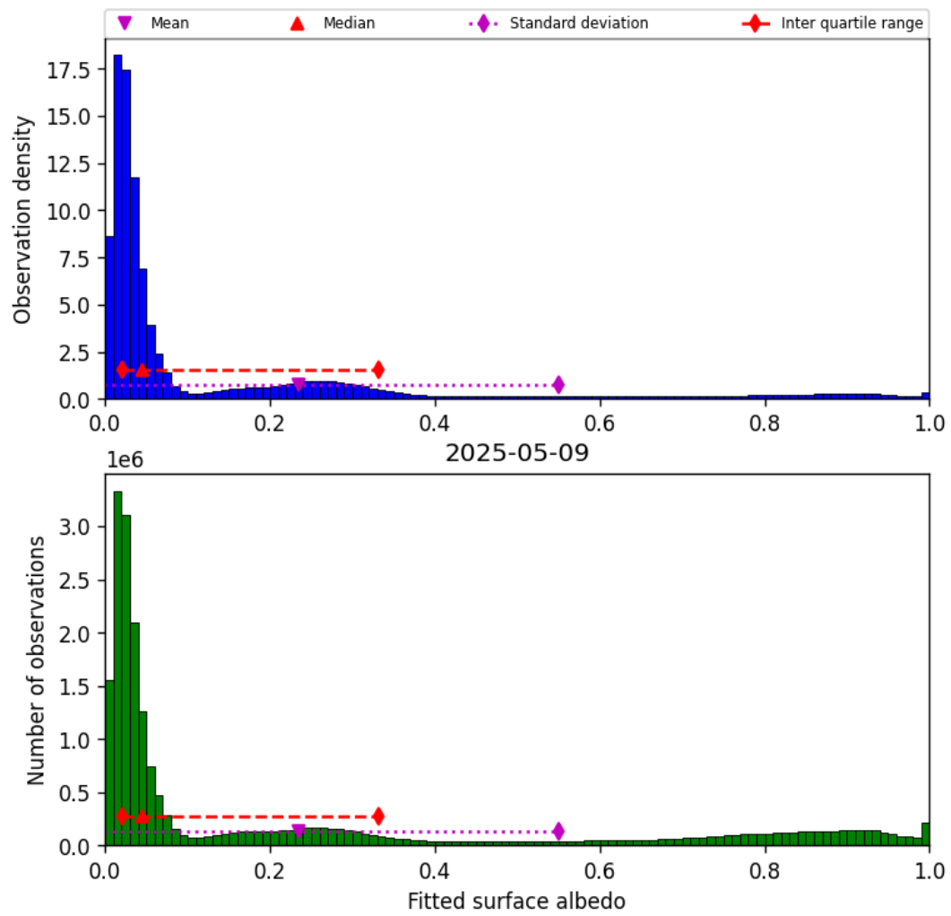
Figure 45: Histogram of “Fitted surface albedo” for 2025-05-08 to 2025-05-10
