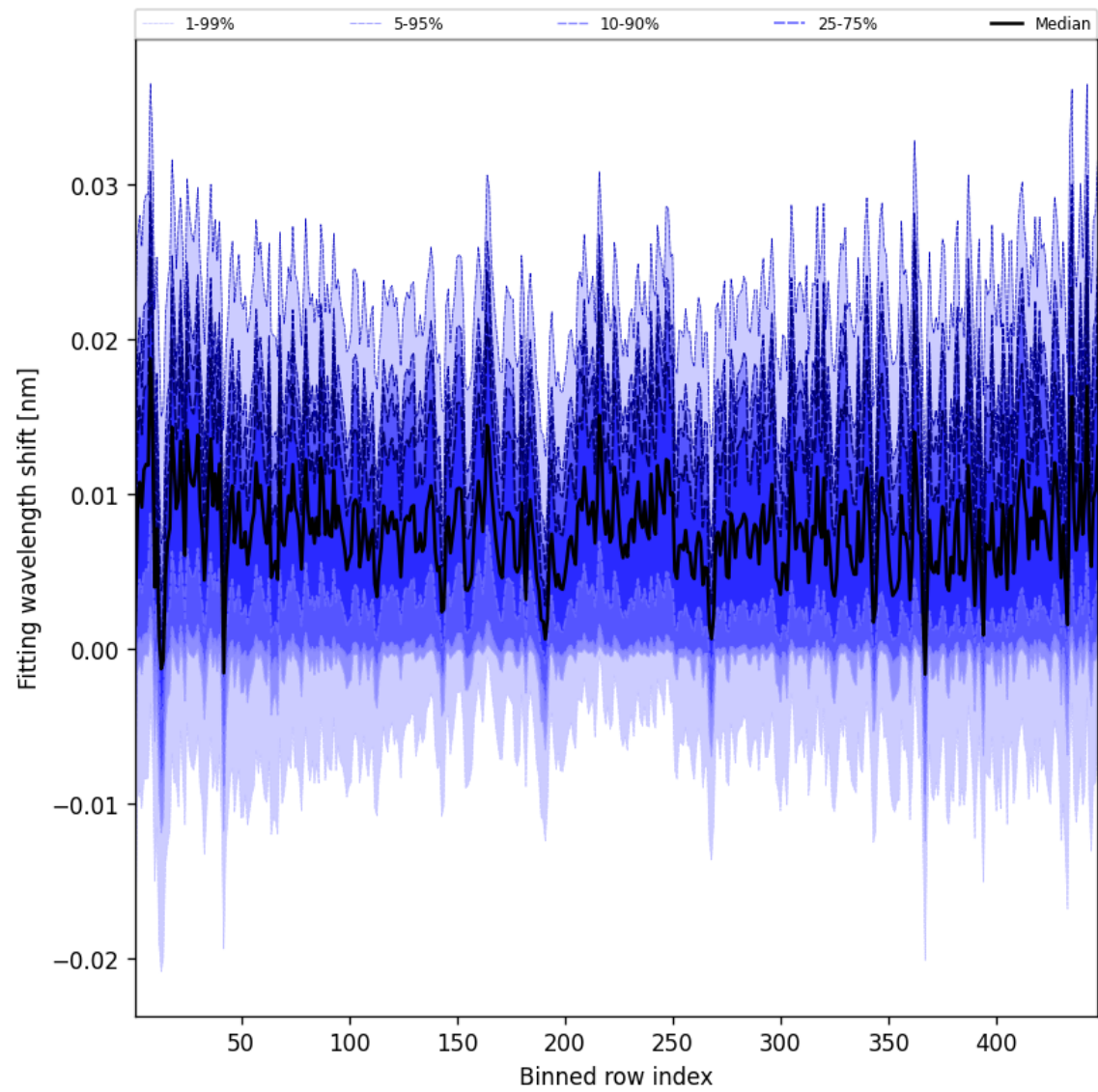
Figure 65: Along track statistics of “Fitting wavelength shift” for 2025-05-08 to 2025-05-10
