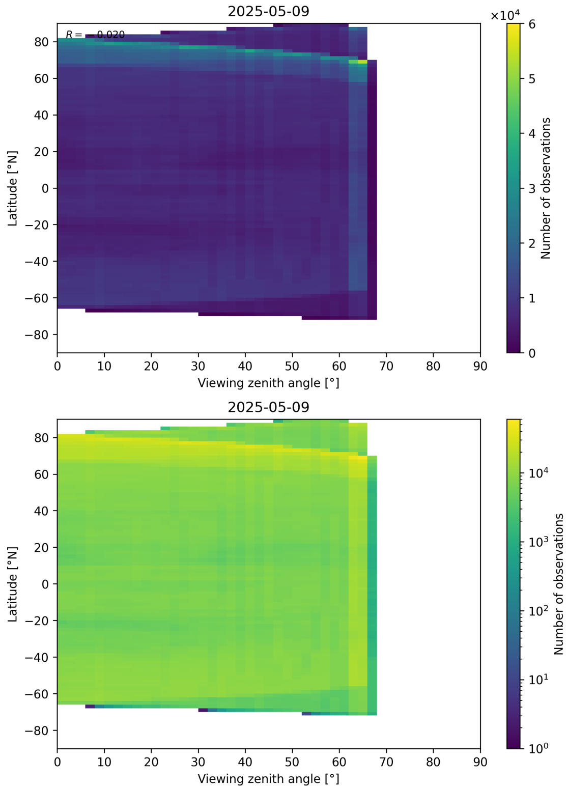
Figure 113: Scatter density plot of “Viewing zenith angle” against “Latitude” for 2025-05-08 to 2025-05-10.
