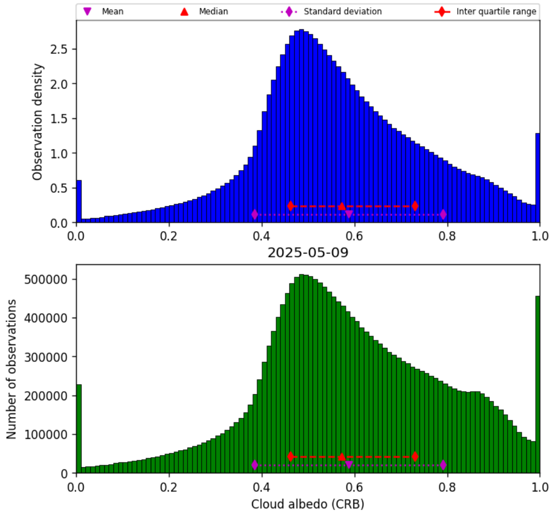
Figure 44: Histogram of “Cloud albedo (CRB)” for 2025-05-08 to 2025-05-10
