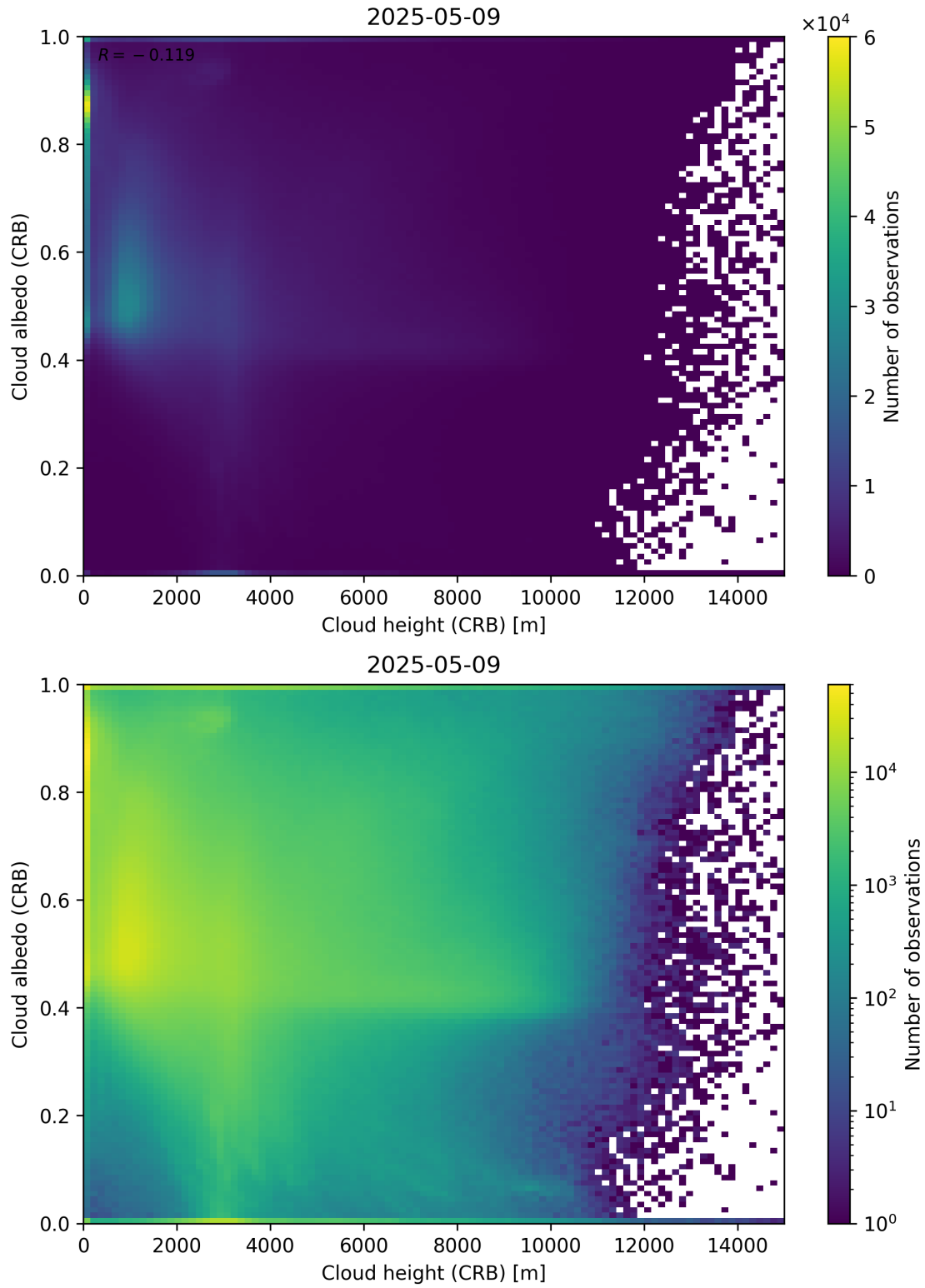
Figure 80: Scatter density plot of “Cloud height (CRB)” against “Cloud albedo (CRB)” for 2025-05-08 to 2025-05-10.
