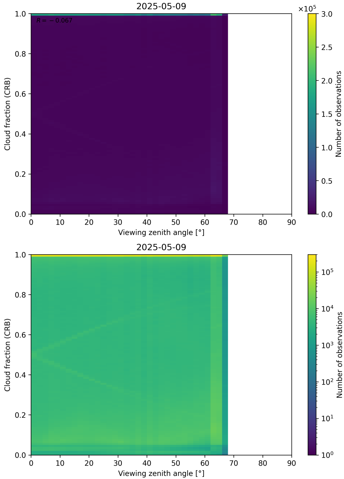
Figure 109: Scatter density plot of “Viewing zenith angle” against “Cloud fraction (CRB)” for 2025-05-08 to 2025-05-10.
