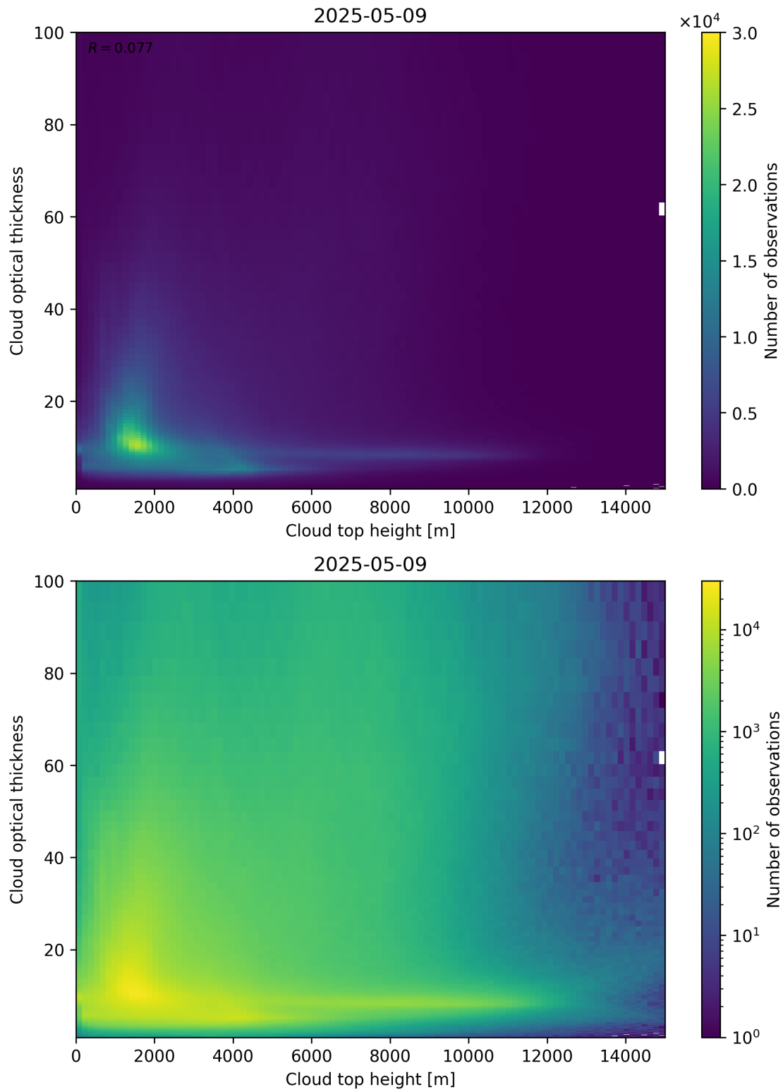
Figure 90: Scatter density plot of “Cloud top height” against “Cloud optical thickness” for 2025-05-08 to 2025-05-10.
