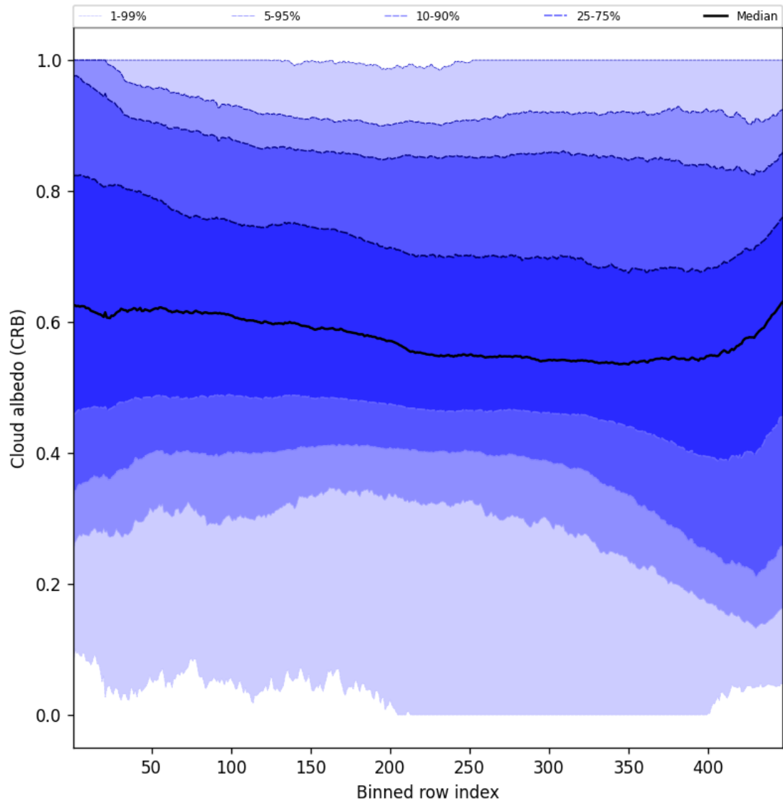
Figure 60: Along track statistics of “Cloud albedo (CRB)” for 2025-05-08 to 2025-05-10
