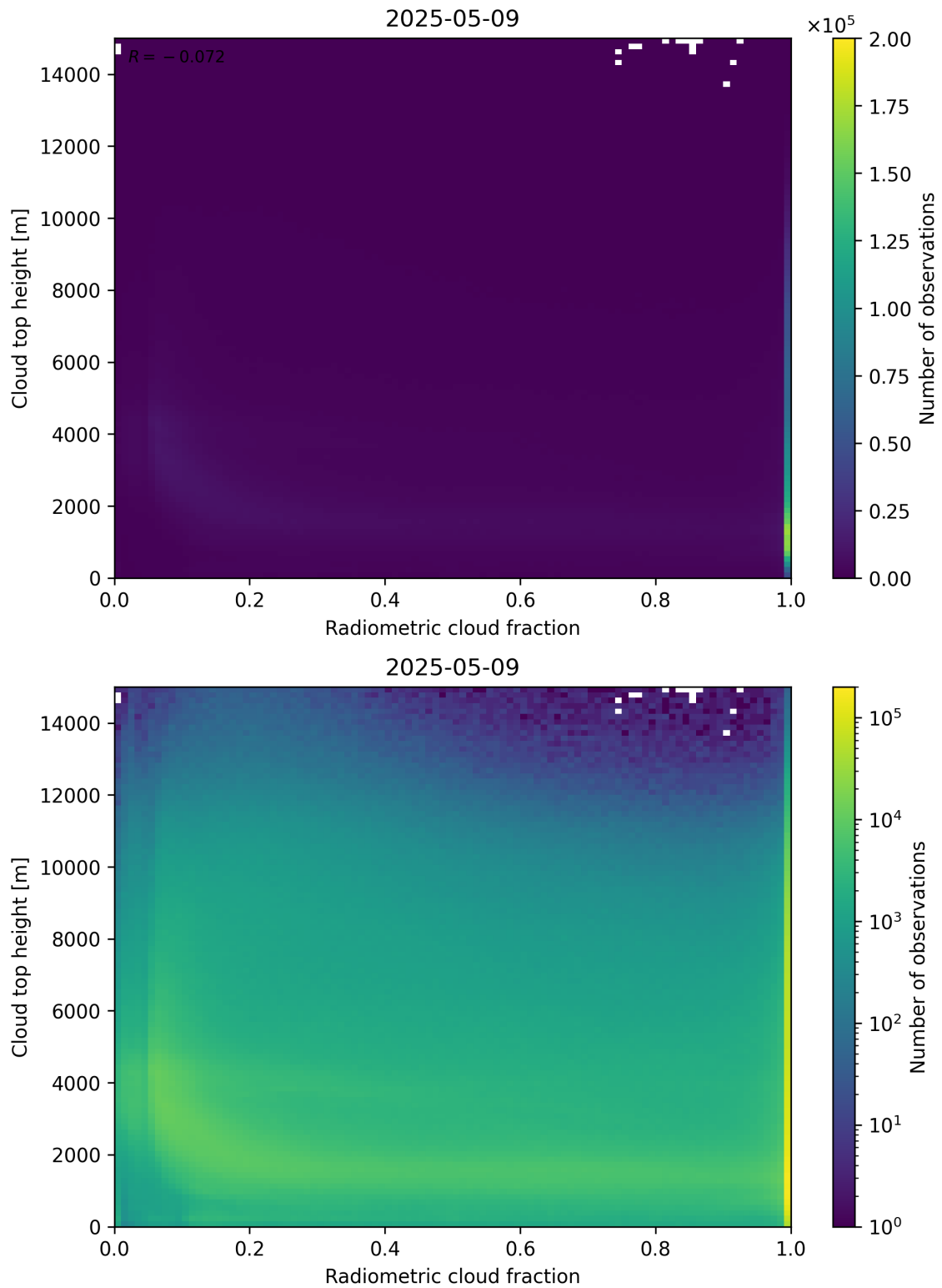
Figure 76: Scatter density plot of “Radiometric cloud fraction” against “Cloud top height” for 2025-05-08 to 2025-05-10.
