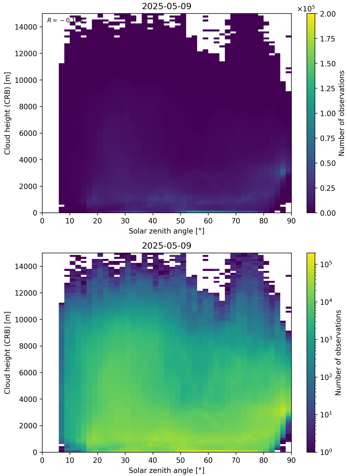
Figure 102: Scatter density plot of “Solar zenith angle” against “Cloud height (CRB)” for 2025-05-08 to 2025-05-10.
