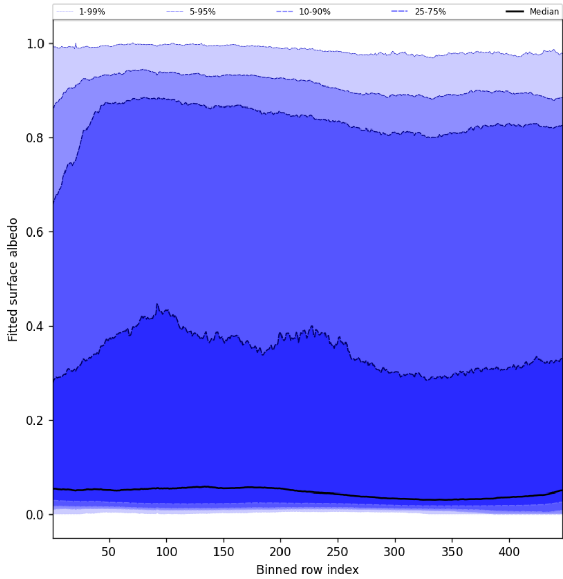
Figure 61: Along track statistics of “Fitted surface albedo” for 2025-05-08 to 2025-05-10
