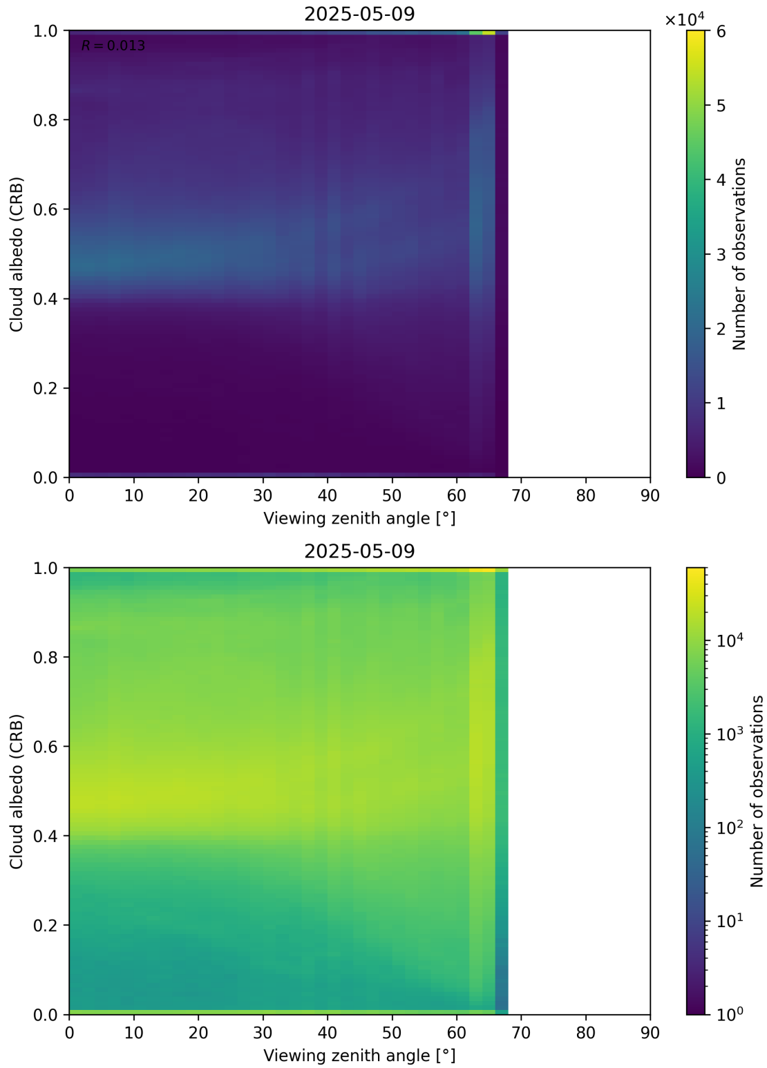
Figure 106: Scatter density plot of “Viewing zenith angle” against “Cloud albedo (CRB)” for 2025-05-08 to 2025-05-10.
