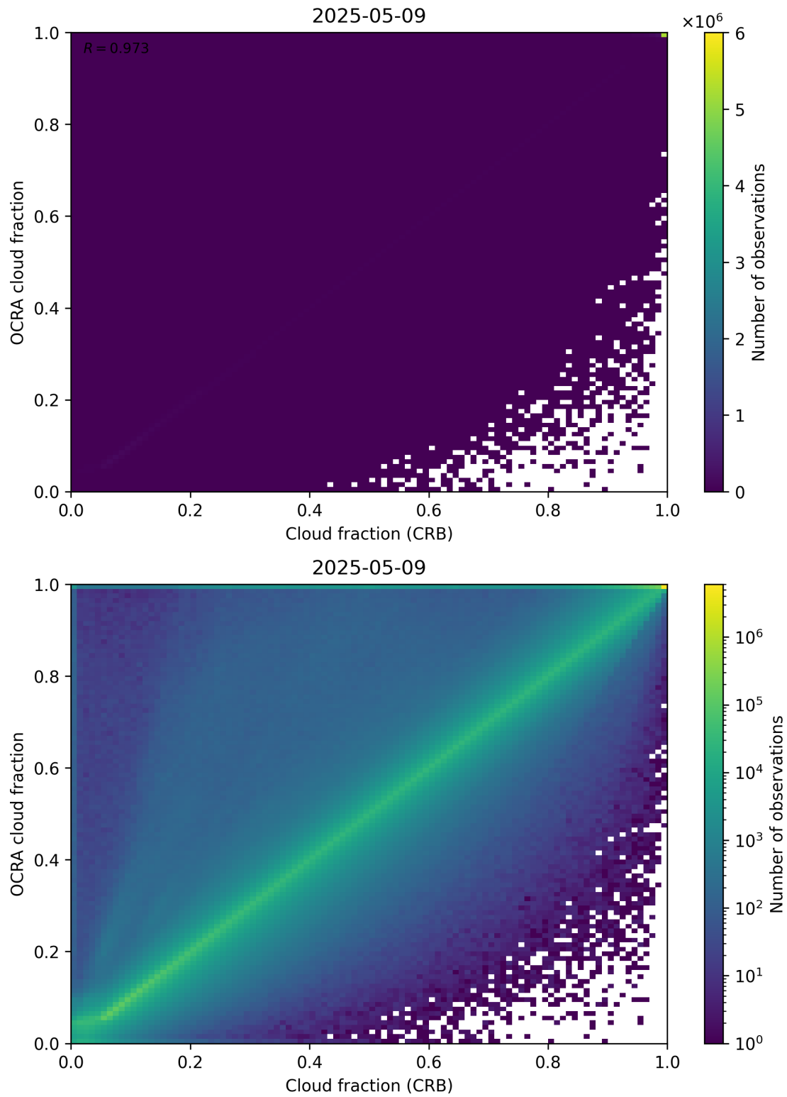
Figure 78: Scatter density plot of “Cloud fraction (CRB)” against “OCRA cloud fraction” for 2025-05-08 to 2025-05-10.
