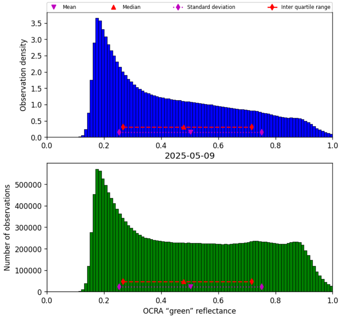
Figure 52: Histogram of “OCRA “green” reflectance” for 2025-05-08 to 2025-05-10
