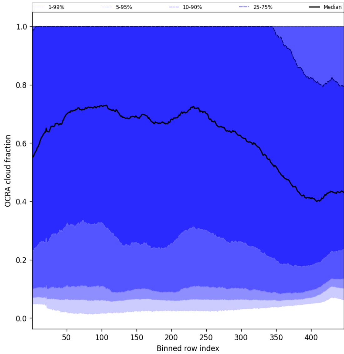
Figure 66: Along track statistics of “OCRA cloud fraction” for 2025-05-08 to 2025-05-10
