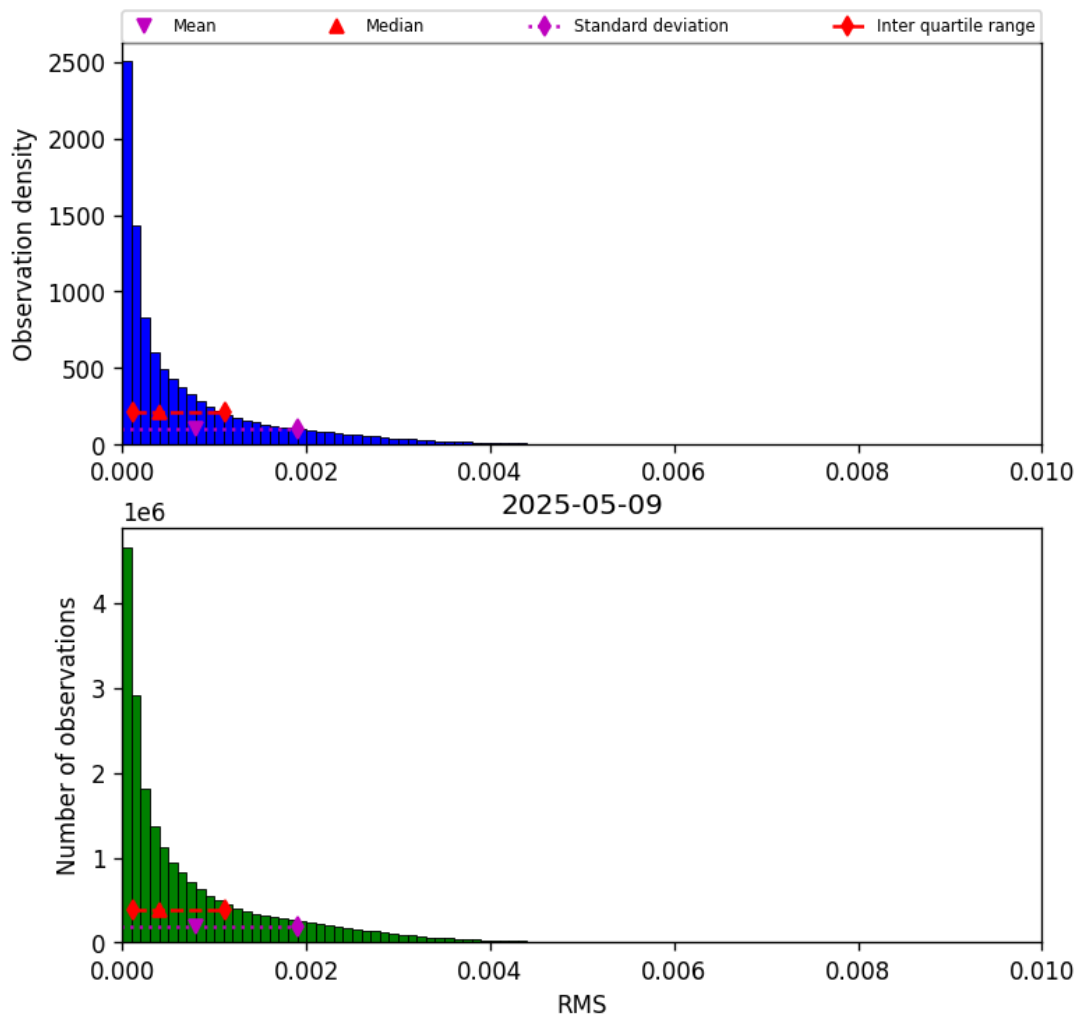
Figure 47: Histogram of “RMS” for 2025-05-08 to 2025-05-10
