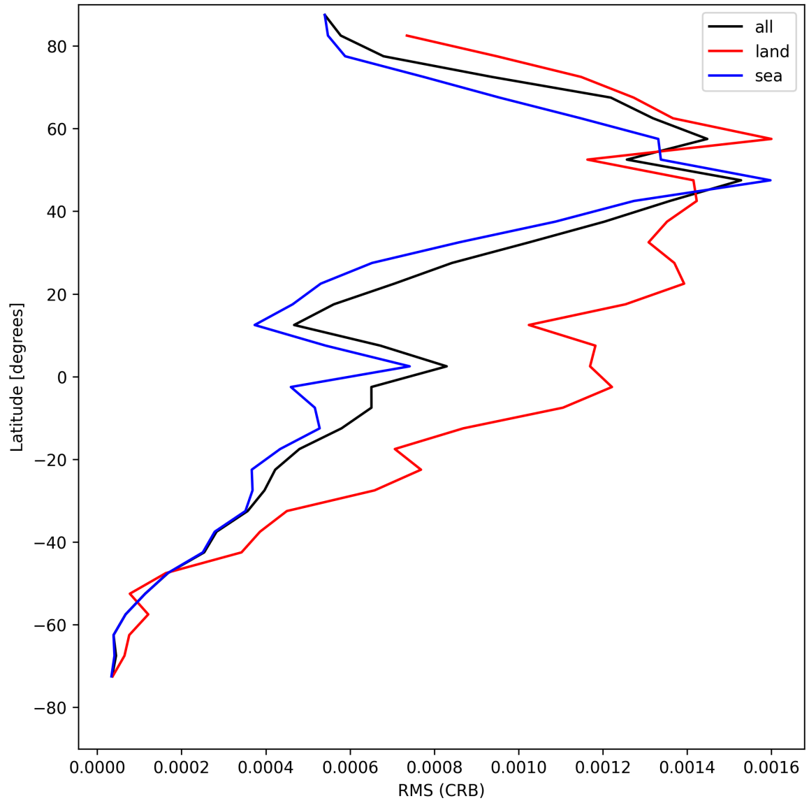
Figure 32: Zonal average of “RMS (CRB)” for 2025-05-08 to 2025-05-10.
