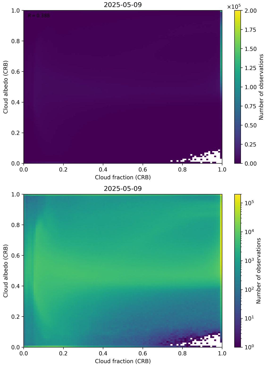
Figure 77: Scatter density plot of “Cloud fraction (CRB)” against “Cloud albedo (CRB)” for 2025-05-08 to 2025-05-10.
