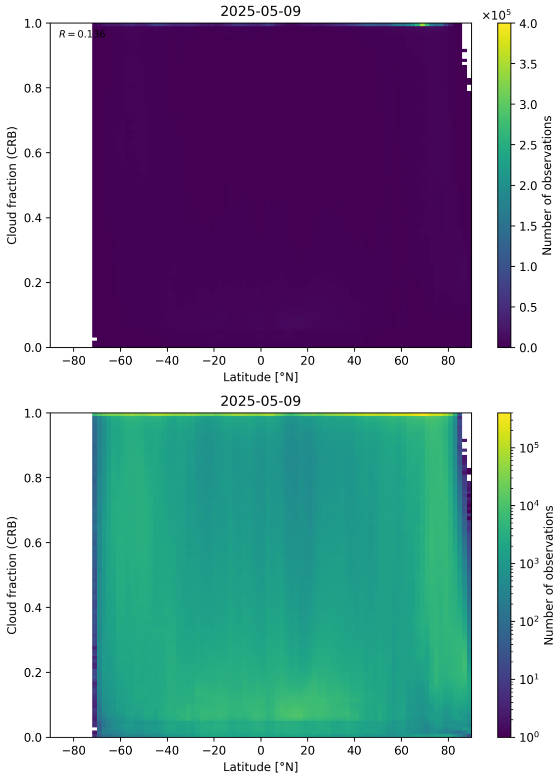
Figure 94: Scatter density plot of “Latitude” against “Cloud fraction (CRB)” for 2025-05-08 to 2025-05-10.
