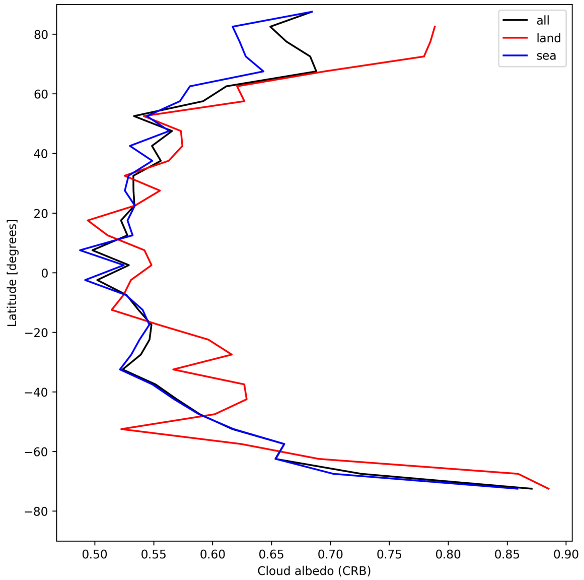
Figure 28: Zonal average of “Cloud albedo (CRB)” for 2025-05-08 to 2025-05-10.
