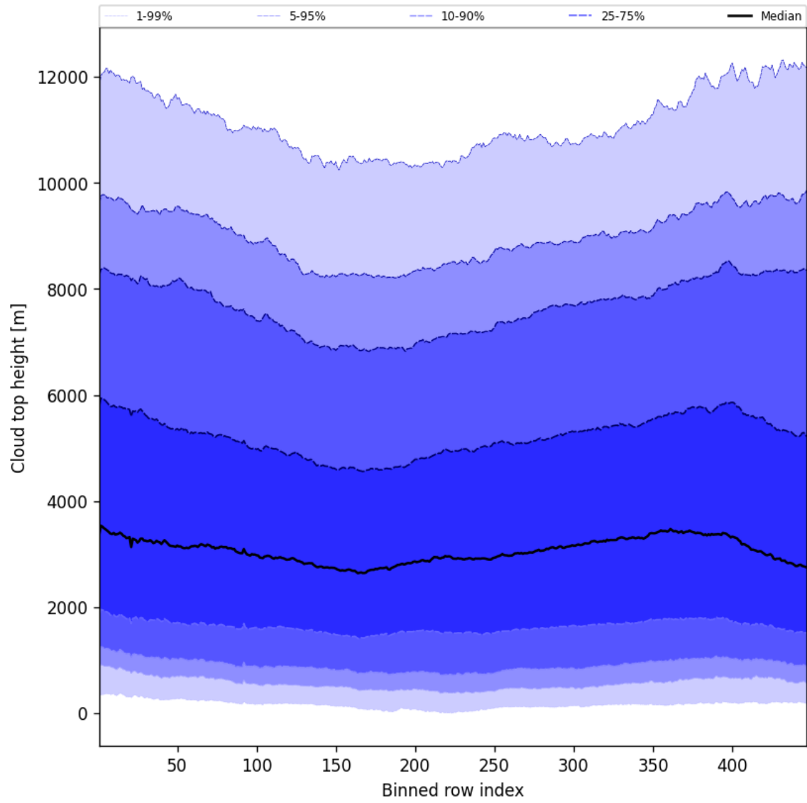
Figure 56: Along track statistics of “Cloud top height” for 2025-05-08 to 2025-05-10
