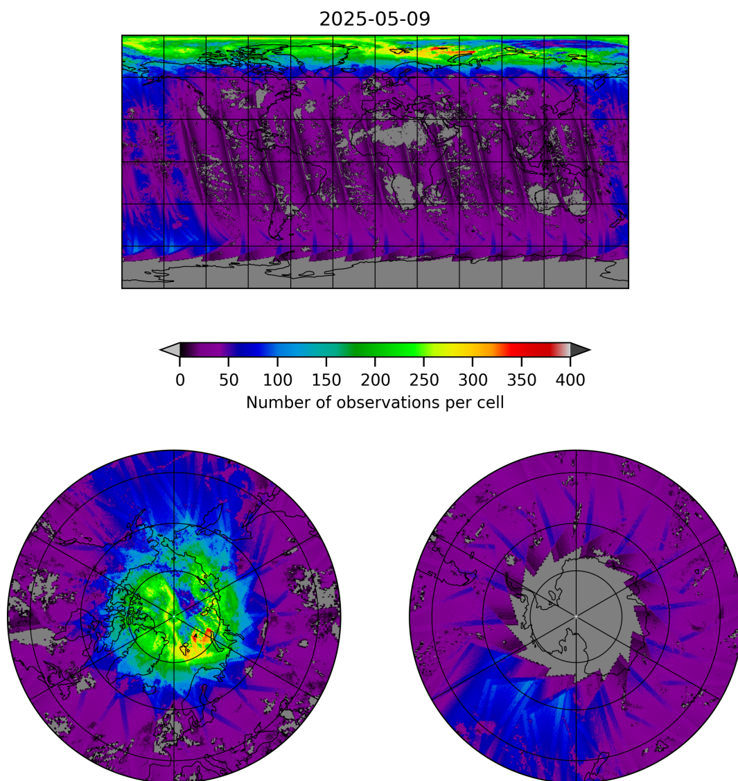
Figure 21: Map of the number of observations for 2025-05-08 to 2025-05-10
