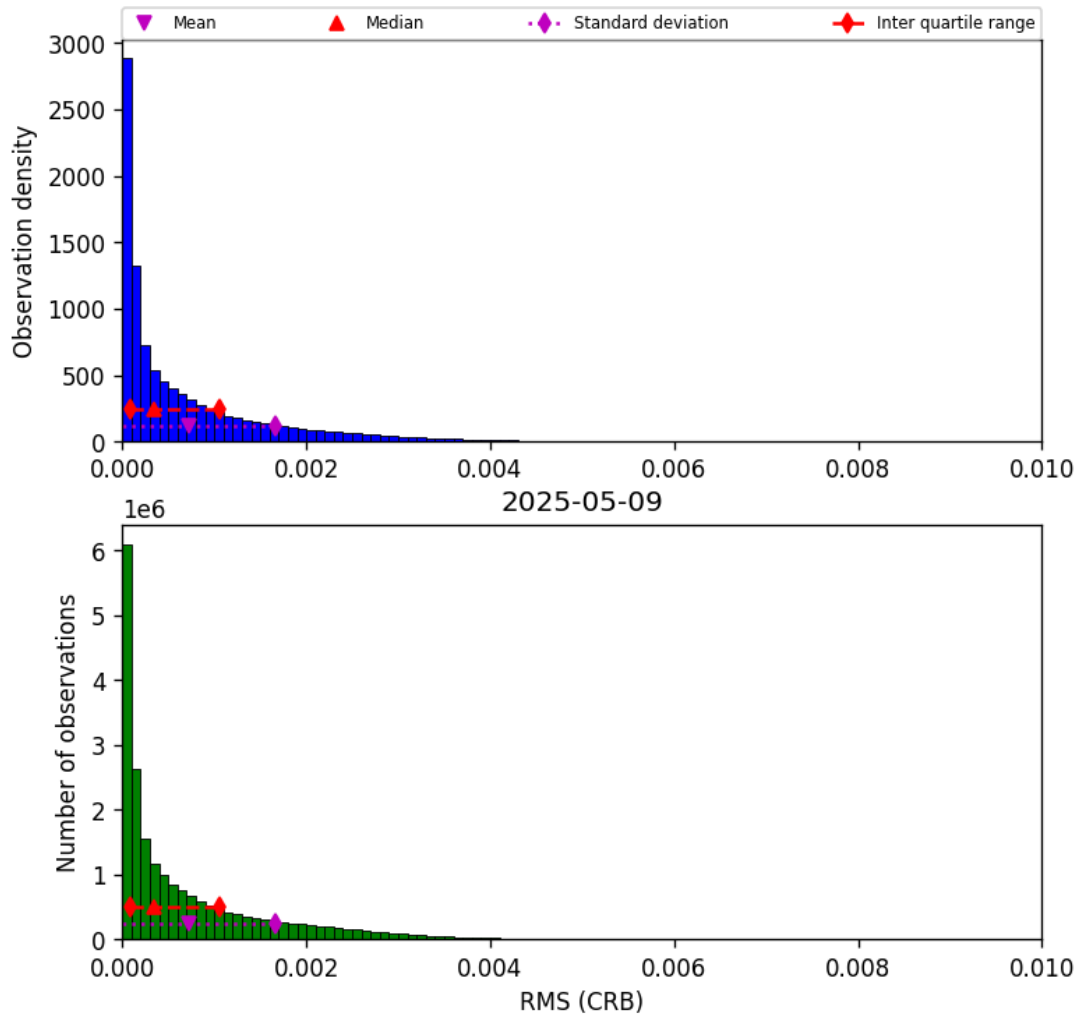
Figure 48: Histogram of “RMS (CRB)” for 2025-05-08 to 2025-05-10
