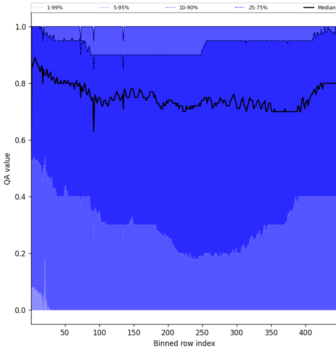
Figure 54: Along track statistics of “QA value” for 2025-05-08 to 2025-05-10
