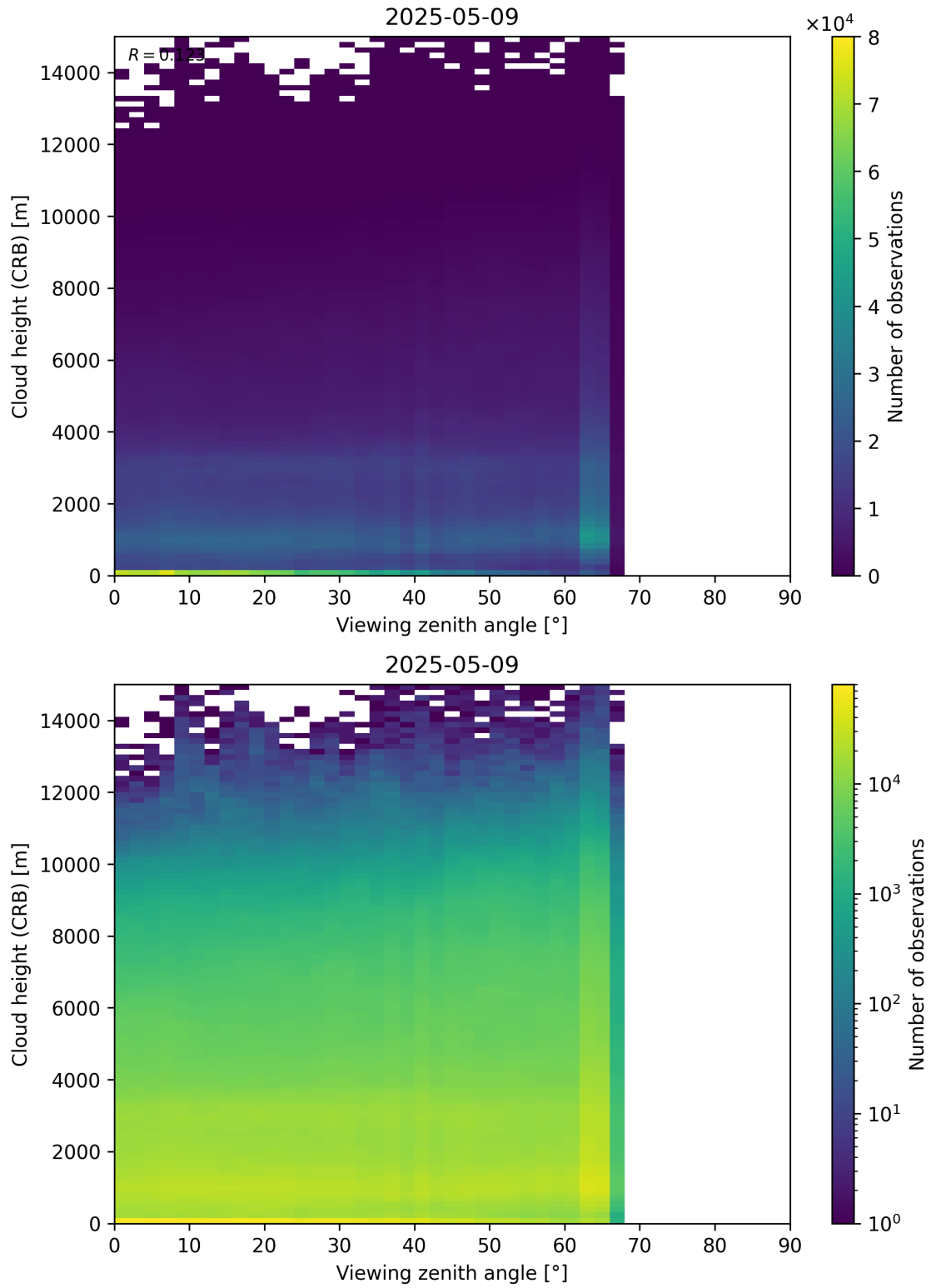
Figure 110: Scatter density plot of “Viewing zenith angle” against “Cloud height (CRB)” for 2025-05-08 to 2025-05-10.
