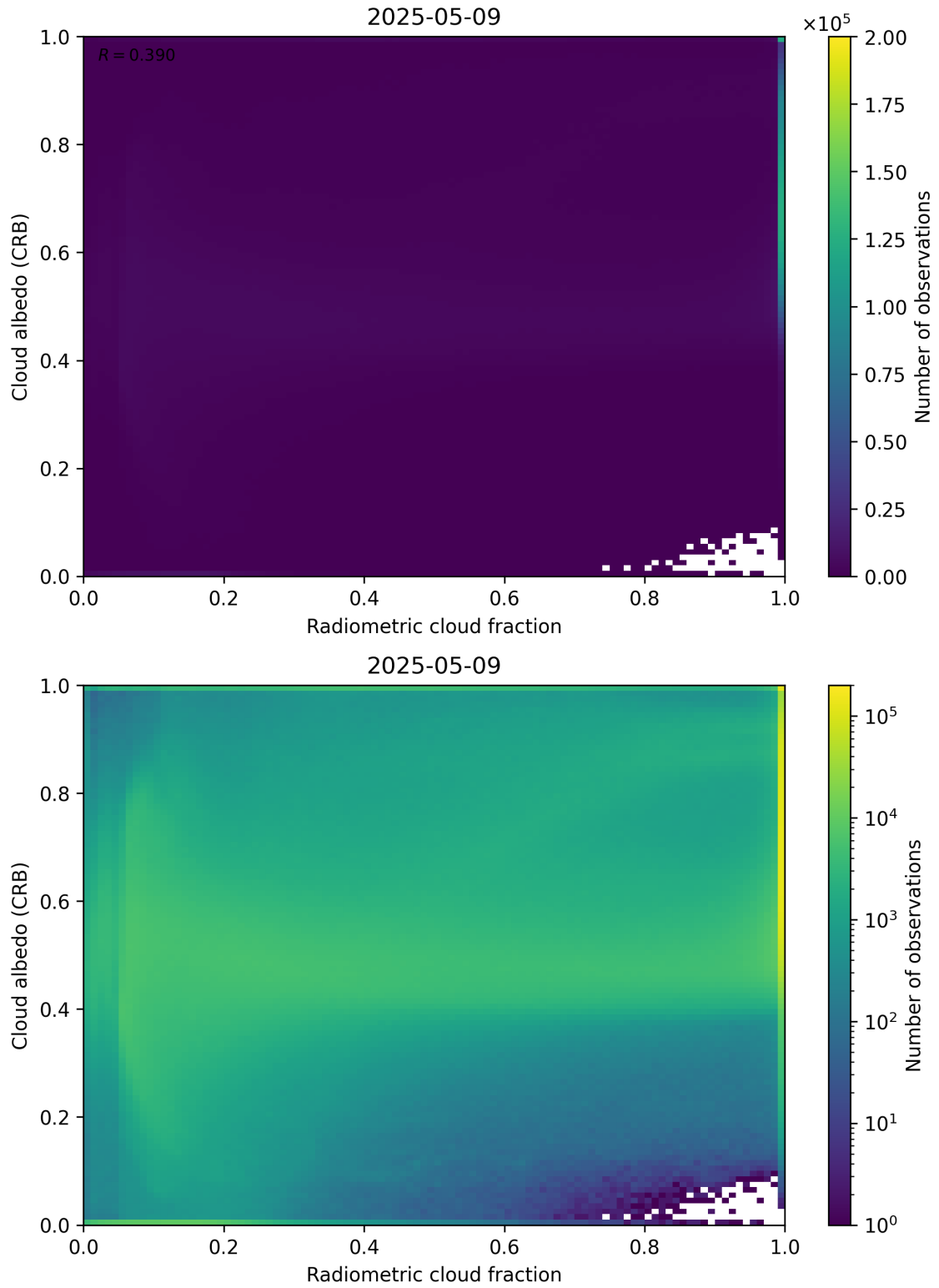
Figure 71: Scatter density plot of “Radiometric cloud fraction” against “Cloud albedo (CRB)” for 2025-05-08 to 2025-05-10.
