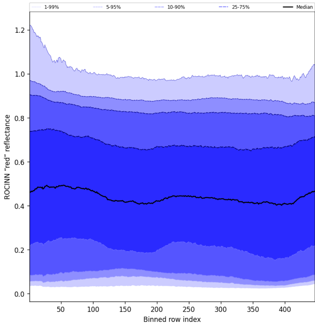
Figure 69: Along track statistics of “ROCINN “red” reflectance” for 2025-05-08 to 2025-05-10
