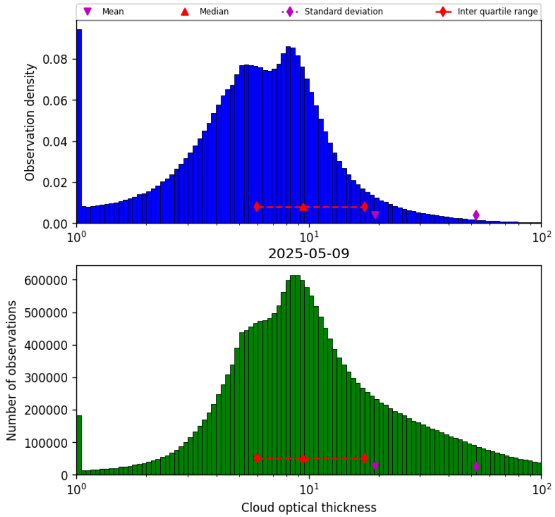
Figure 41: Histogram of “Cloud optical thickness” for 2025-05-08 to 2025-05-10
