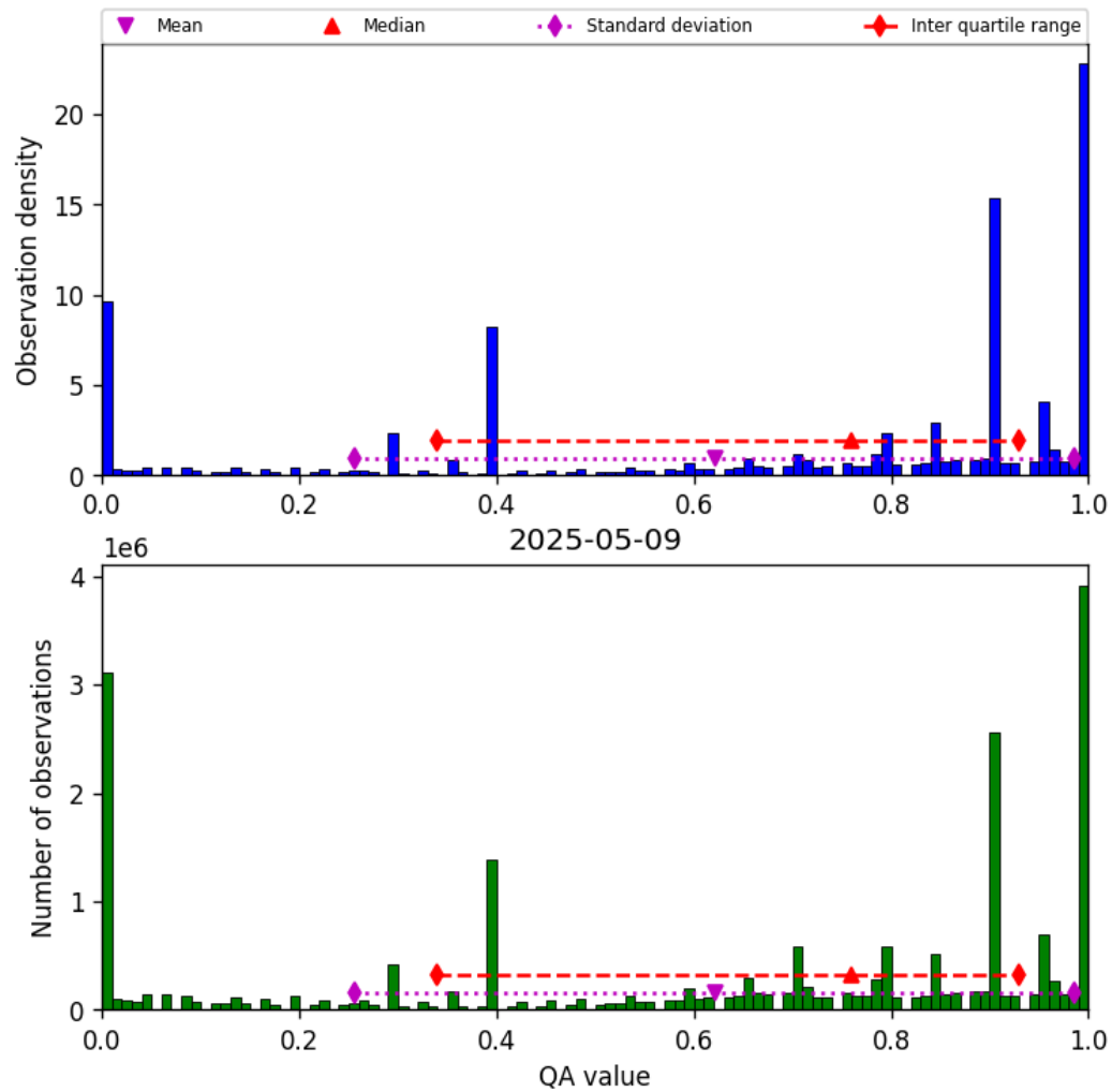
Figure 38: Histogram of “QA value” for 2025-05-08 to 2025-05-10
