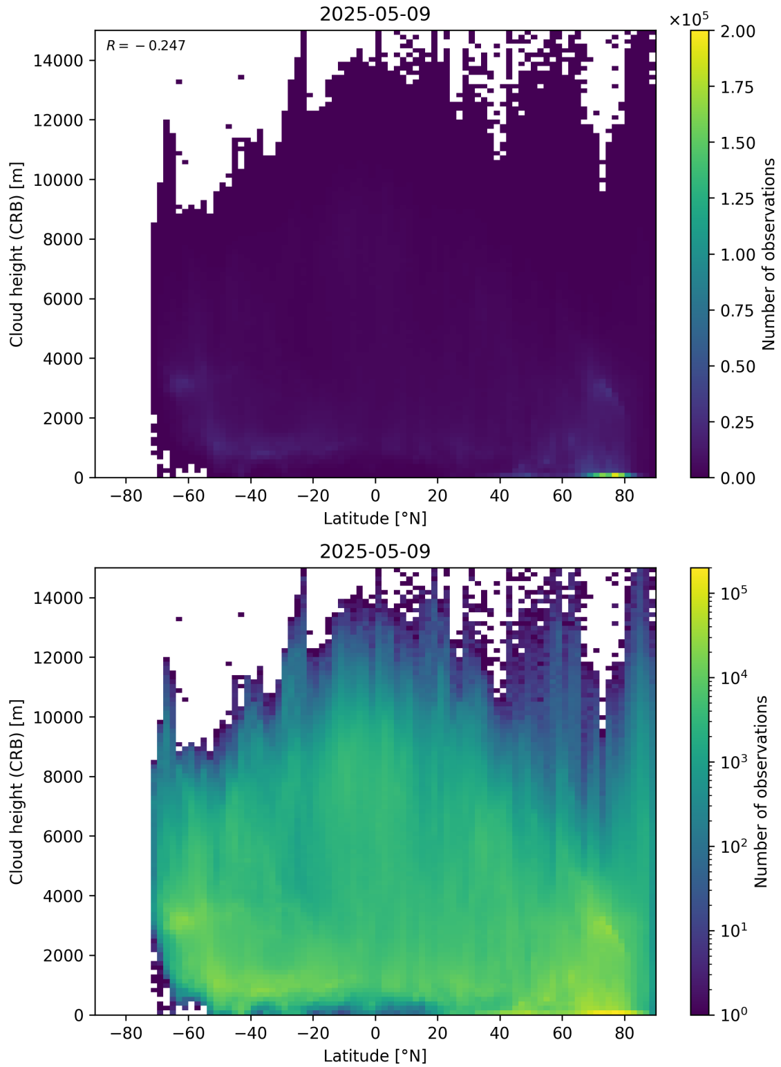
Figure 95: Scatter density plot of “Latitude” against “Cloud height (CRB)” for 2025-05-08 to 2025-05-10.
