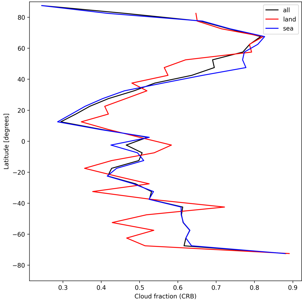
Figure 26: Zonal average of “Cloud fraction (CRB)” for 2025-05-08 to 2025-05-10.
