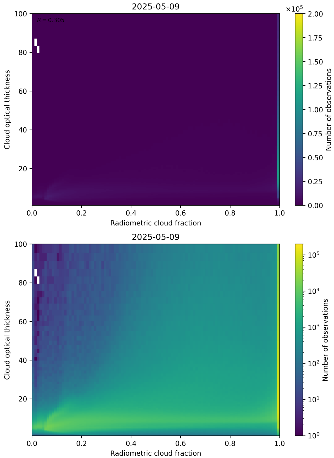
Figure 75: Scatter density plot of “Radiometric cloud fraction” against “Cloud optical thickness” for 2025-05-08 to 2025-05-10.
