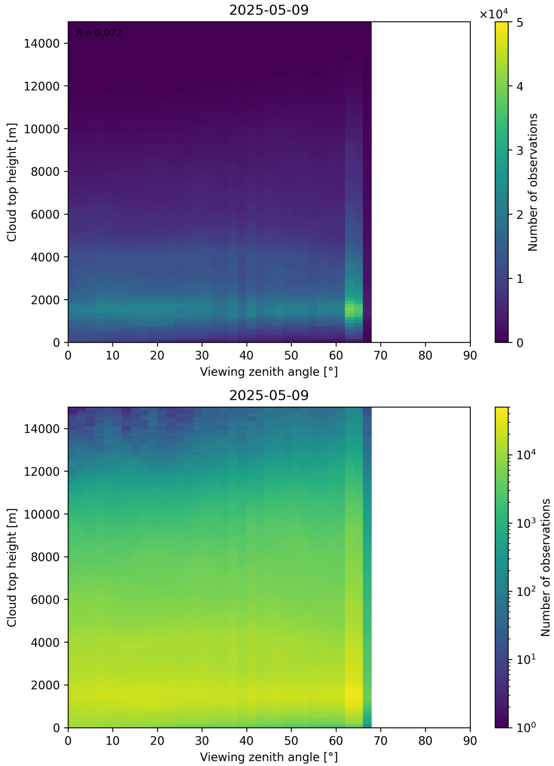
Figure 112: Scatter density plot of “Viewing zenith angle” against “Cloud top height” for 2025-05-08 to 2025-05-10.
