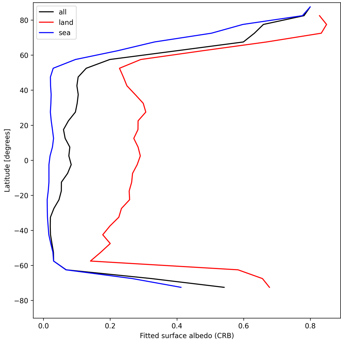
Figure 30: Zonal average of “Fitted surface albedo (CRB)” for 2025-05-08 to 2025-05-10.
