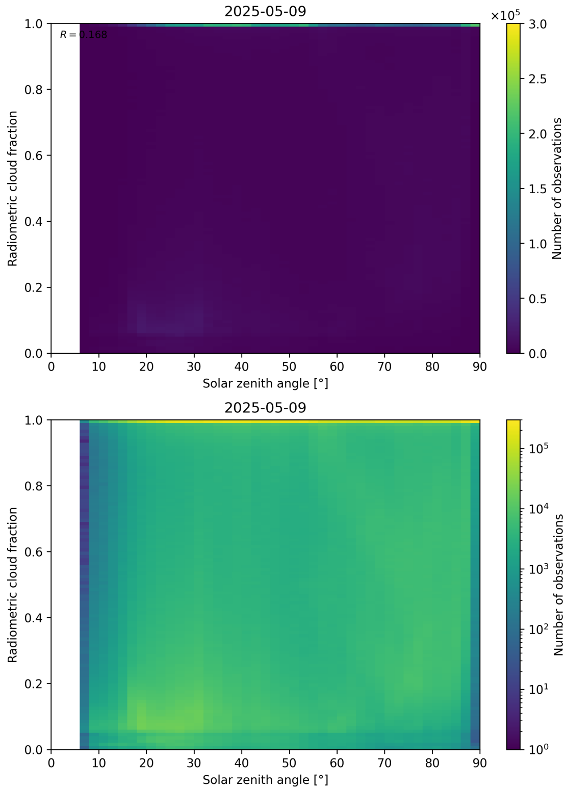
Figure 99: Scatter density plot of “Solar zenith angle” against “Radiometric cloud fraction” for 2025-05-08 to 2025-05-10.
