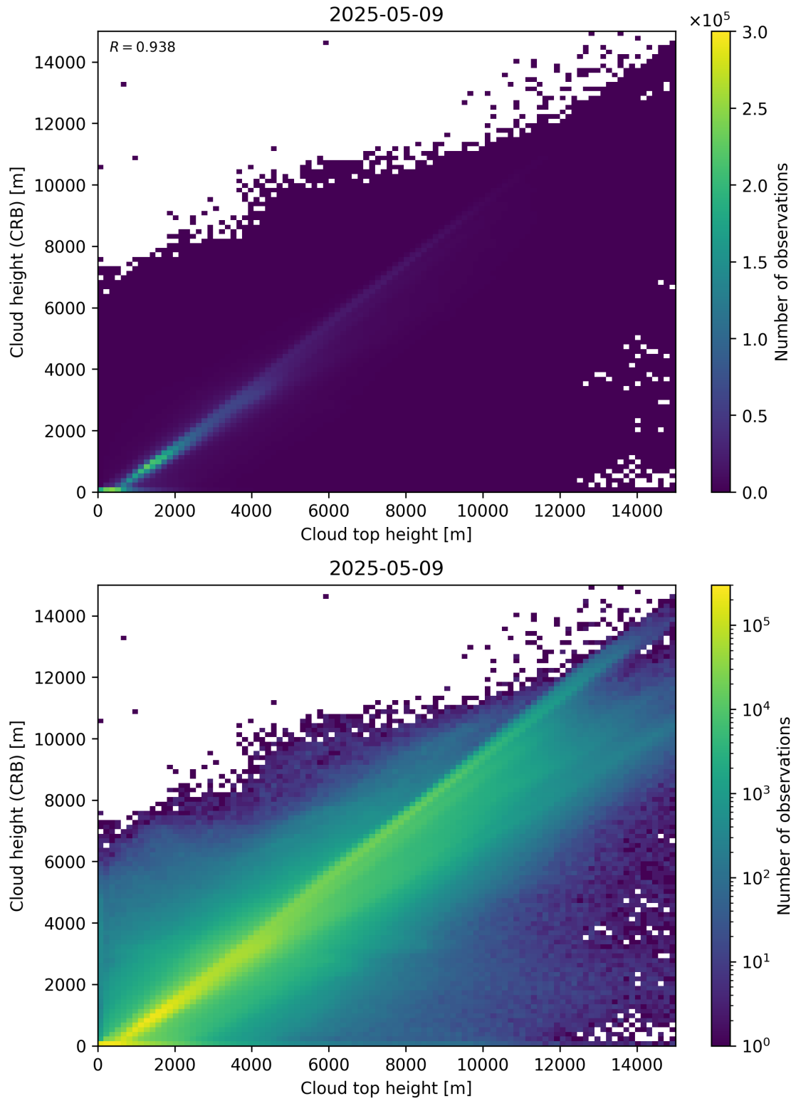
Figure 89: Scatter density plot of “Cloud top height” against “Cloud height (CRB)” for 2025-05-08 to 2025-05-10.
