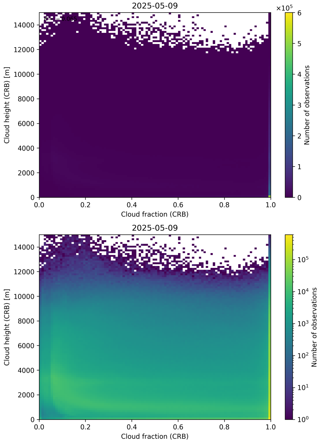
Figure 79: Scatter density plot of “Cloud fraction (CRB)” against “Cloud height (CRB)” for 2025-05-08 to 2025-05-10.
