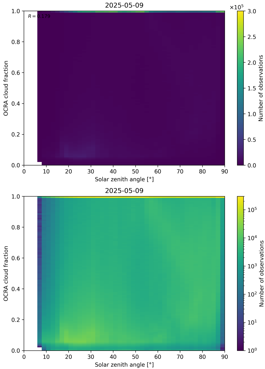
Figure 100: Scatter density plot of “Solar zenith angle” against “OCRA cloud fraction” for 2025-05-08 to 2025-05-10.
