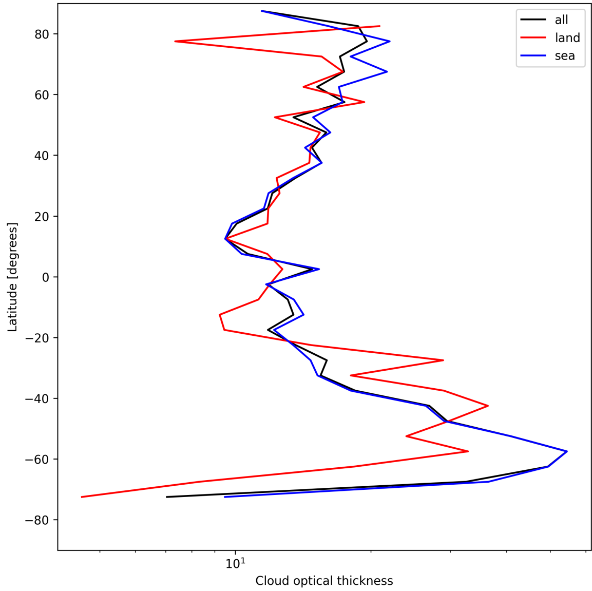
Figure 25: Zonal average of “Cloud optical thickness” for 2025-05-08 to 2025-05-10.
