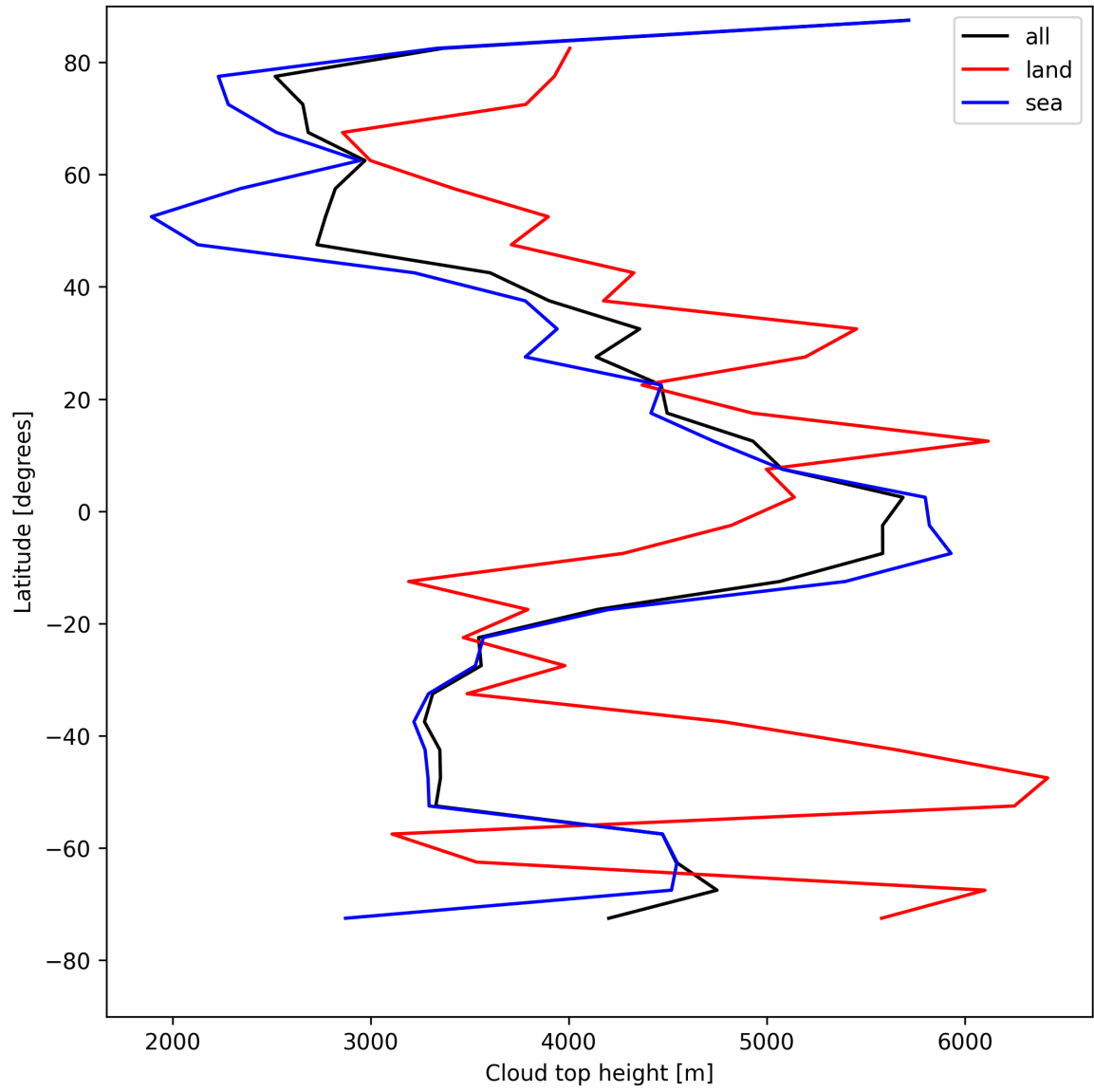
Figure 24: Zonal average of “Cloud top height” for 2025-05-08 to 2025-05-10.
