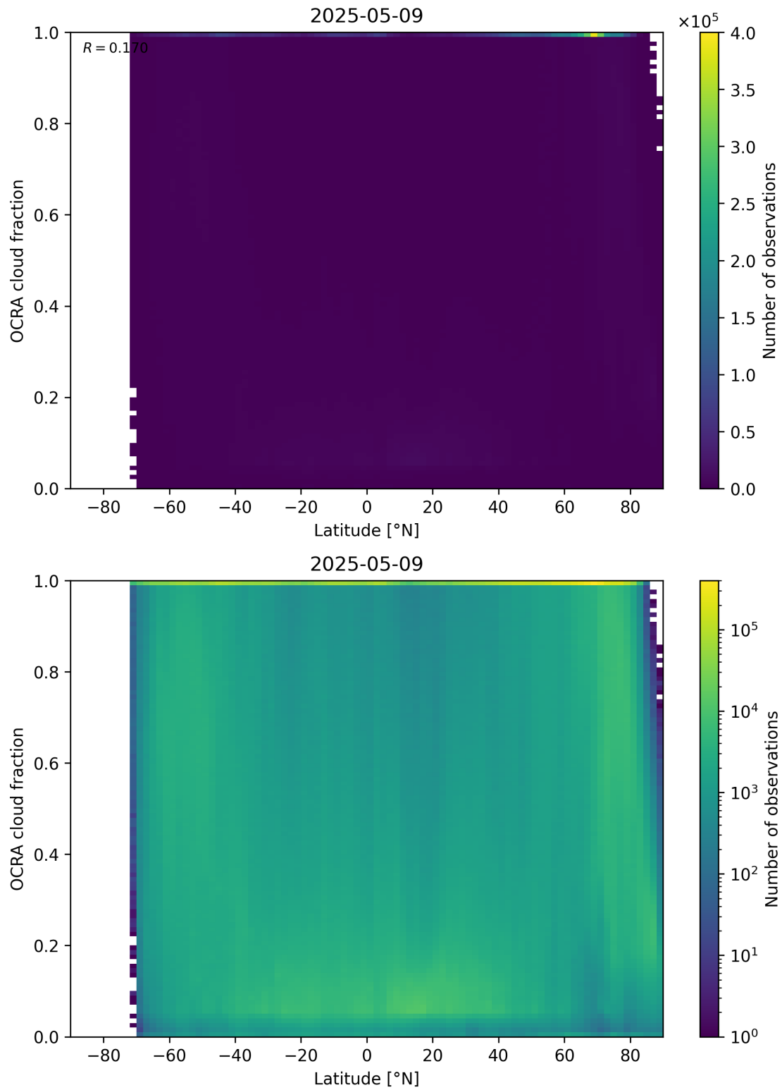
Figure 93: Scatter density plot of “Latitude” against “OCRA cloud fraction” for 2025-05-08 to 2025-05-10.
