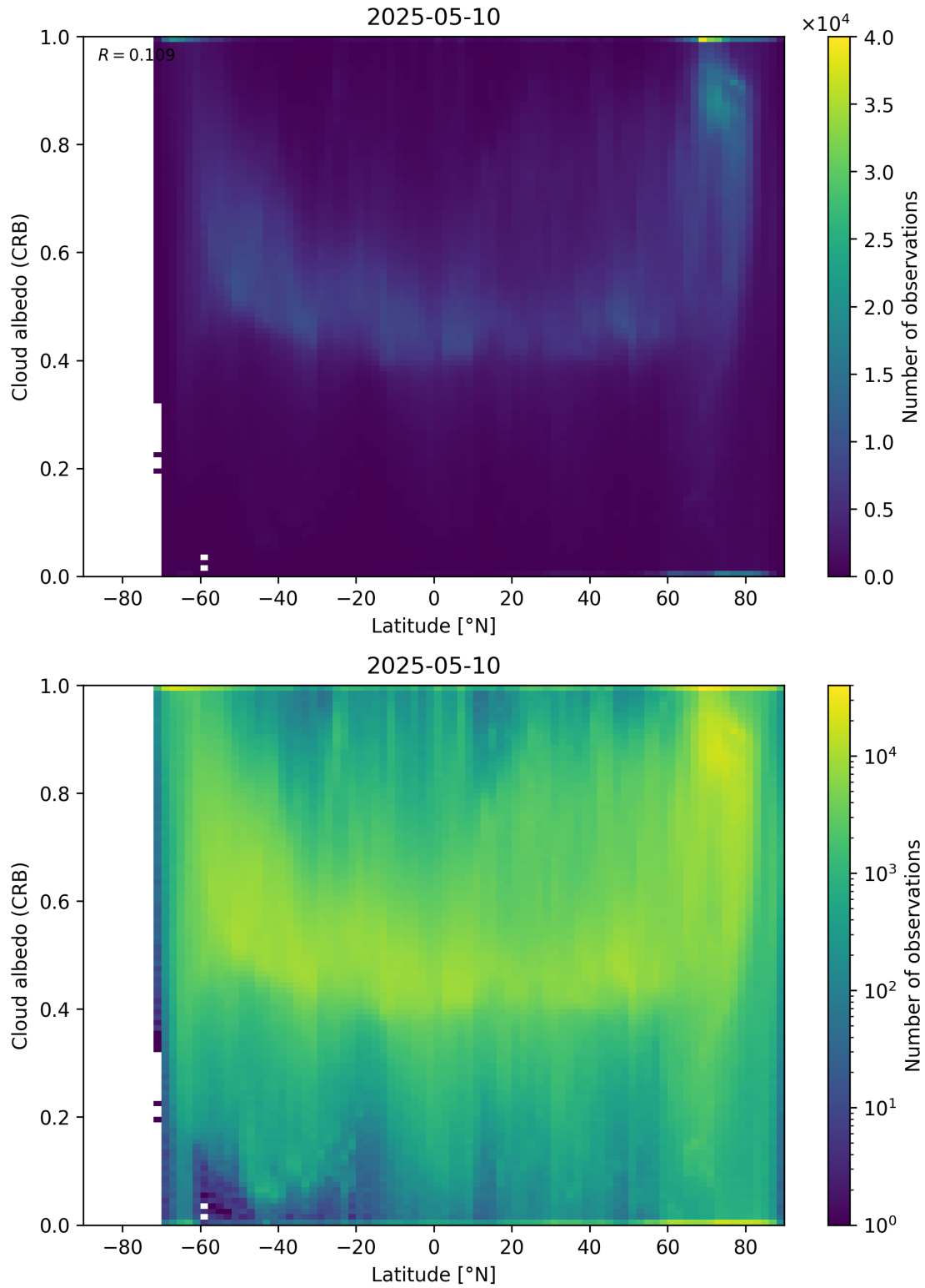
Figure 91: Scatter density plot of “Latitude” against “Cloud albedo (CRB)” for 2025-05-10 to 2025-05-11.
