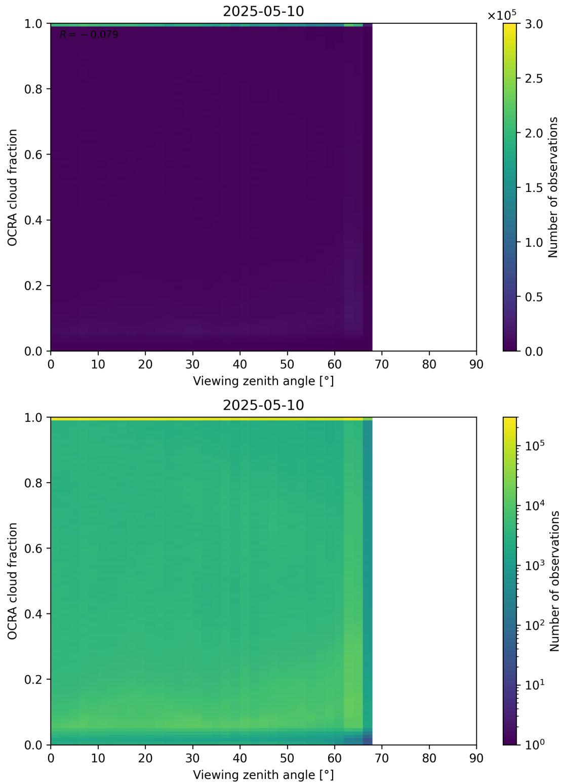
Figure 108: Scatter density plot of “Viewing zenith angle” against “OCRA cloud fraction” for 2025-05-10 to 2025-05-11.
