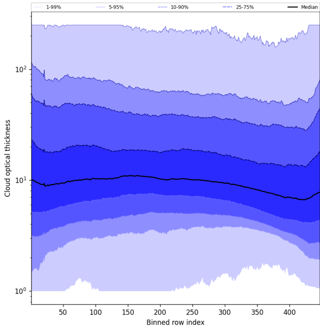
Figure 57: Along track statistics of “Cloud optical thickness” for 2025-05-10 to 2025-05-11
