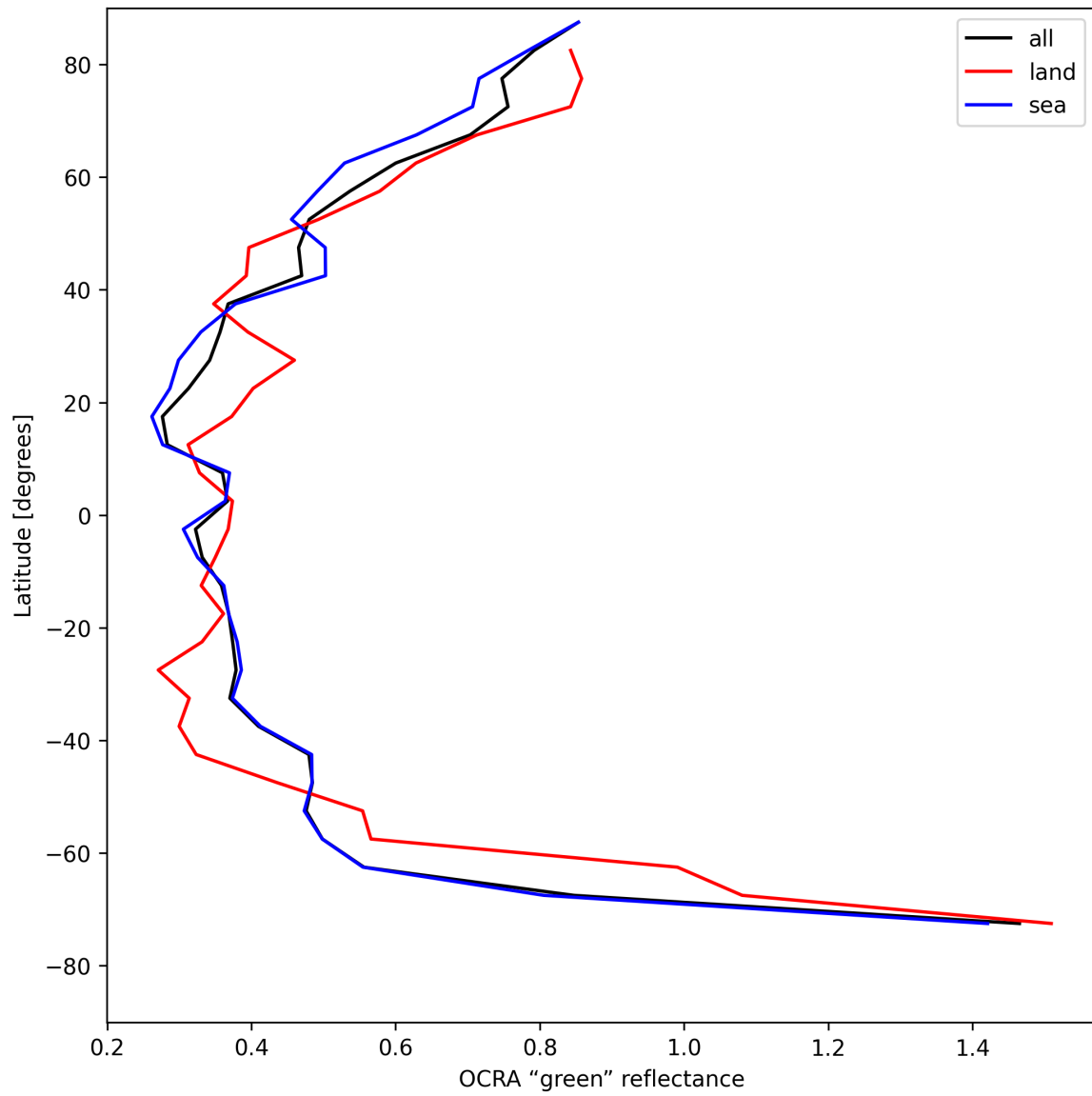
Figure 36: Zonal average of “OCRA “green” reflectance” for 2025-05-10 to 2025-05-11.
