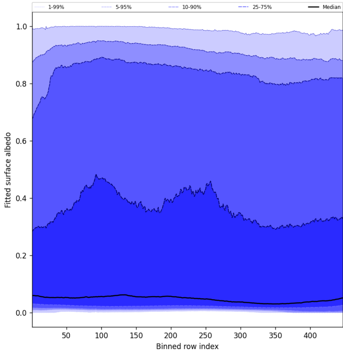
Figure 61: Along track statistics of “Fitted surface albedo” for 2025-05-10 to 2025-05-11
