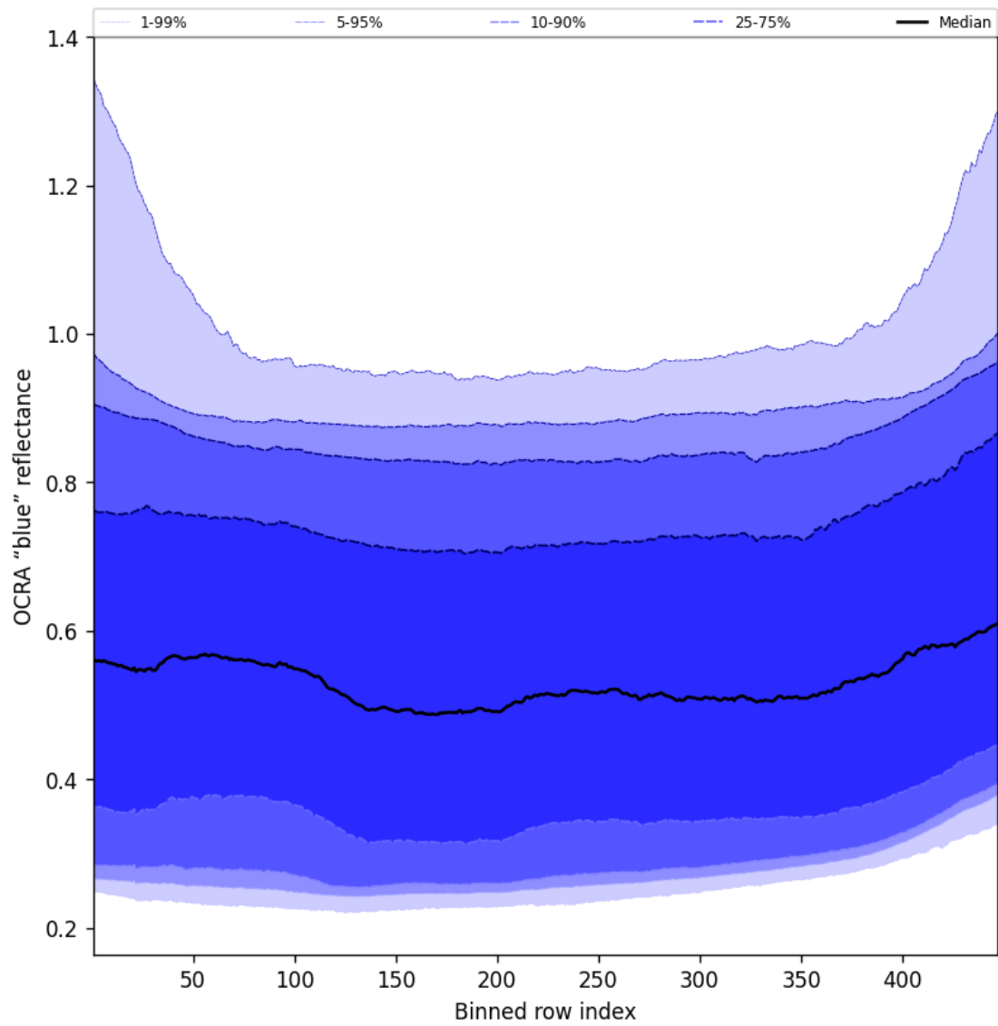
Figure 67: Along track statistics of “OCRA “blue” reflectance” for 2025-05-10 to 2025-05-11
