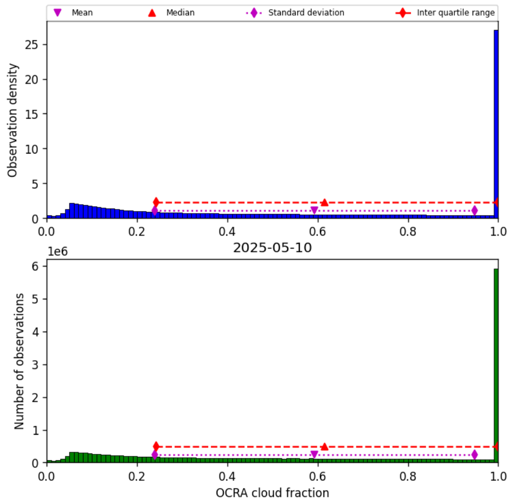
Figure 50: Histogram of “OCRA cloud fraction” for 2025-05-10 to 2025-05-11
