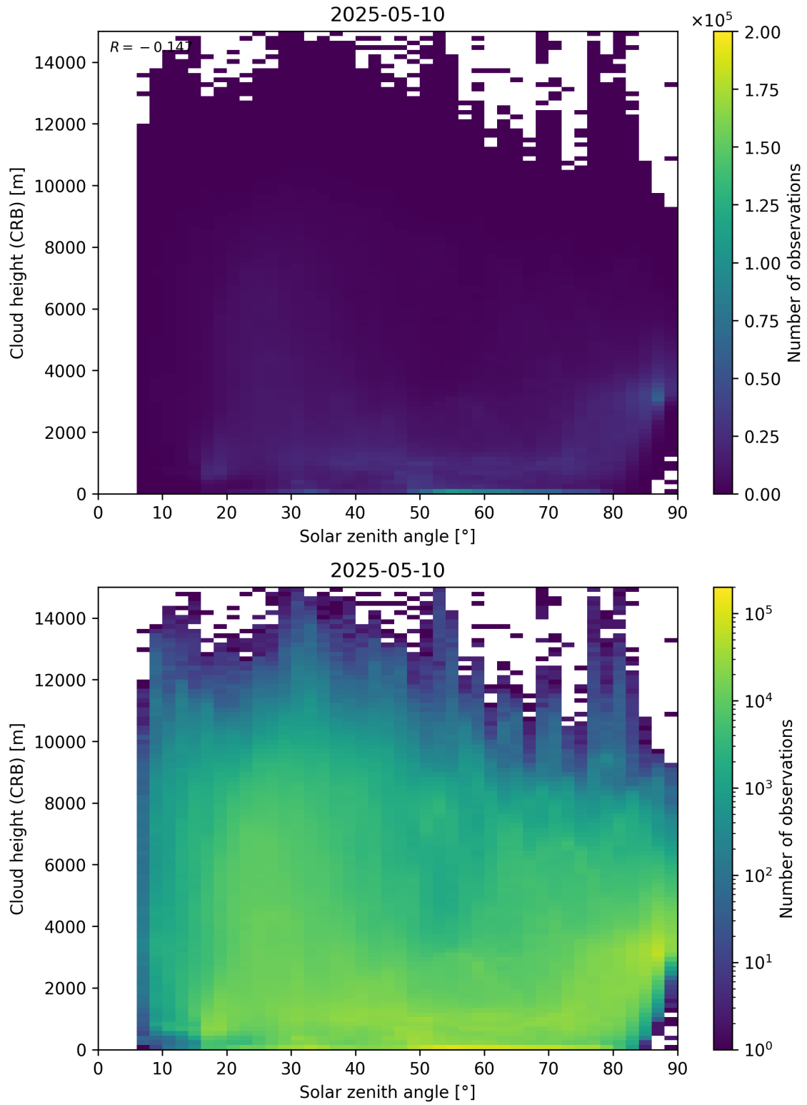
Figure 102: Scatter density plot of “Solar zenith angle” against “Cloud height (CRB)” for 2025-05-10 to 2025-05-11.
