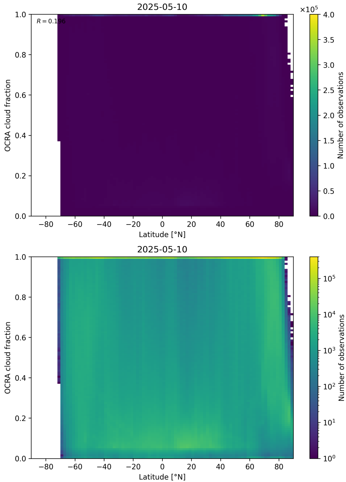
Figure 93: Scatter density plot of “Latitude” against “OCRA cloud fraction” for 2025-05-10 to 2025-05-11.
