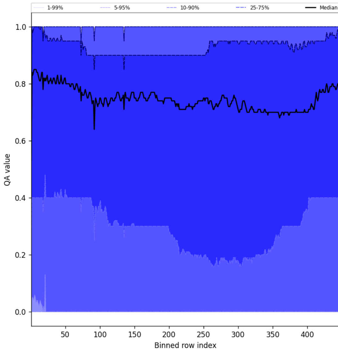
Figure 54: Along track statistics of "QA value" for 2025-05-10 to 2025-05-11
