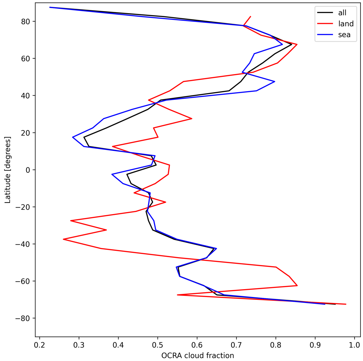
Figure 34: Zonal average of “OCRA cloud fraction” for 2025-05-10 to 2025-05-11.
