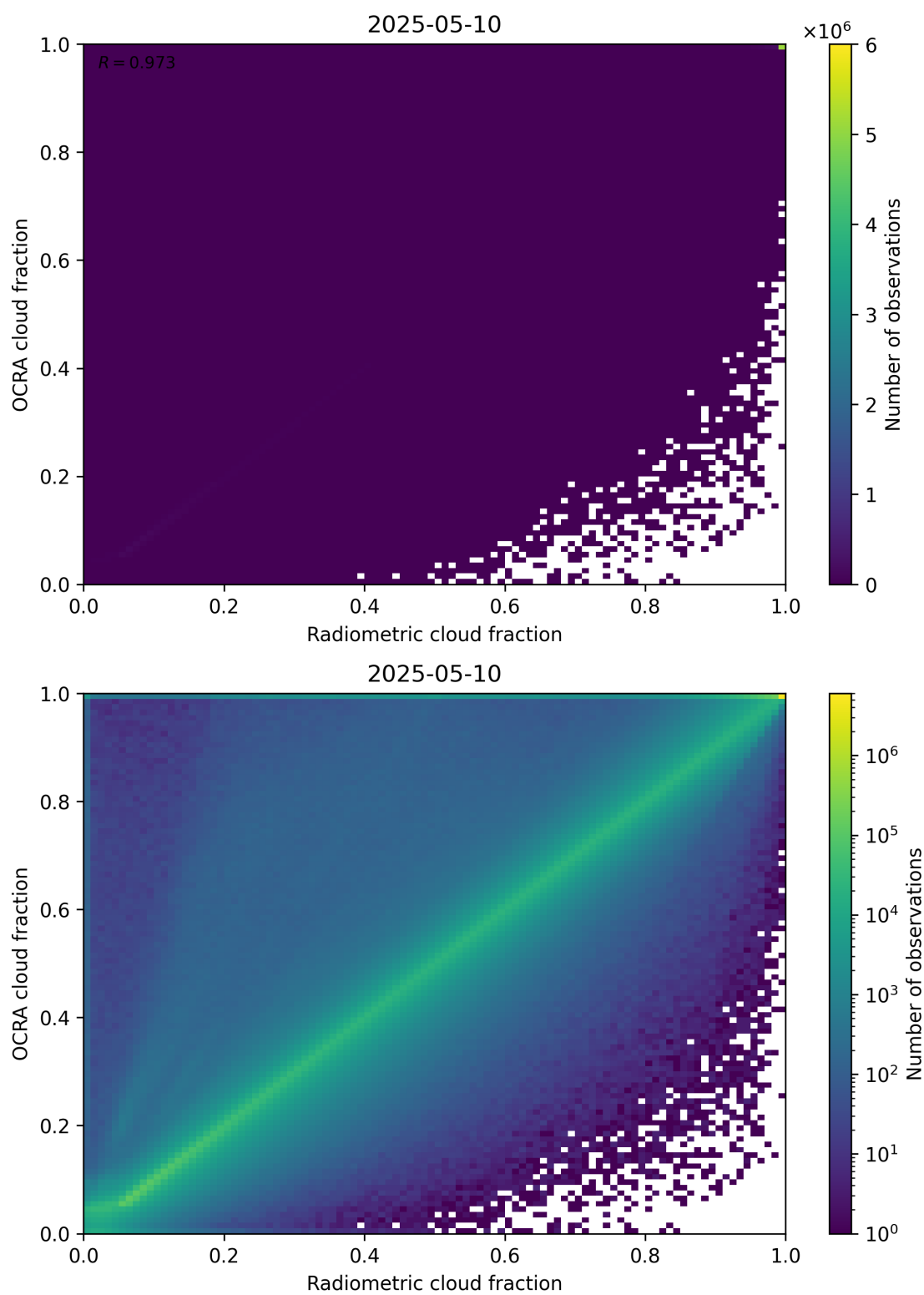
Figure 72: Scatter density plot of “Radiometric cloud fraction” against “OCRA cloud fraction” for 2025-05-10 to 2025-05-11.
