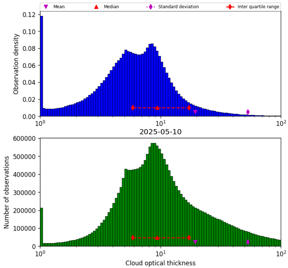
Figure 41: Histogram of “Cloud optical thickness” for 2025-05-10 to 2025-05-11
