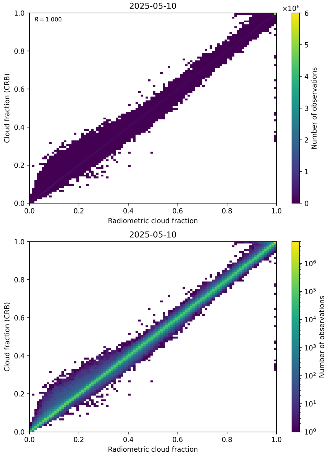
Figure 73: Scatter density plot of “Radiometric cloud fraction” against “Cloud fraction (CRB)” for 2025-05-10 to 2025-05-11.
