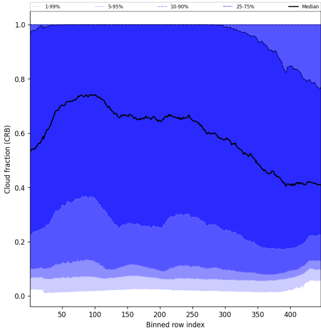
Figure 58: Along track statistics of “Cloud fraction (CRB)” for 2025-05-10 to 2025-05-11
