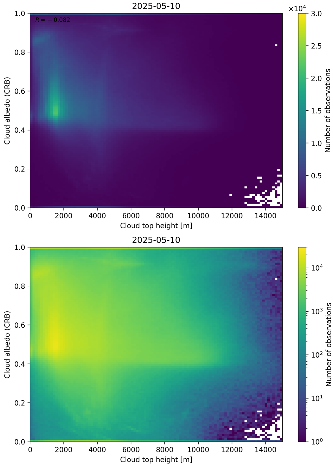
Figure 86: Scatter density plot of “Cloud top height” against “Cloud albedo (CRB)” for 2025-05-10 to 2025-05-11.
