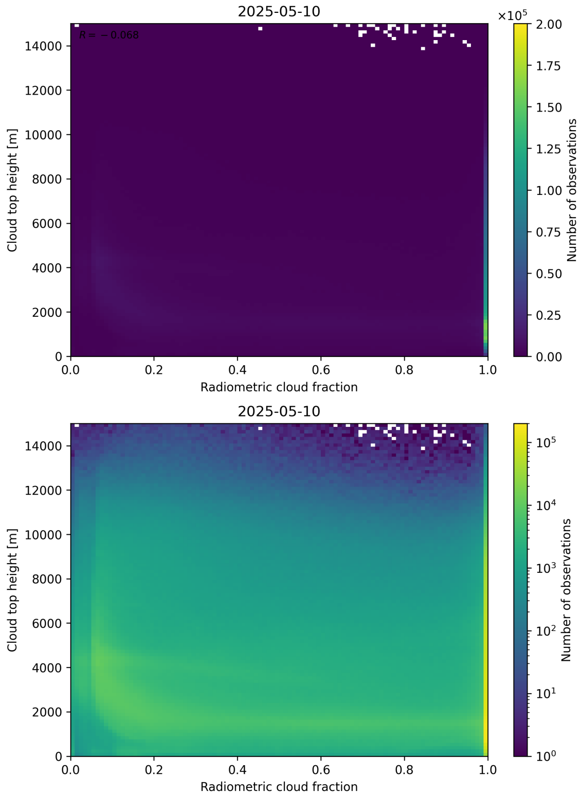
Figure 76: Scatter density plot of “Radiometric cloud fraction” against “Cloud top height” for 2025-05-10 to 2025-05-11.
