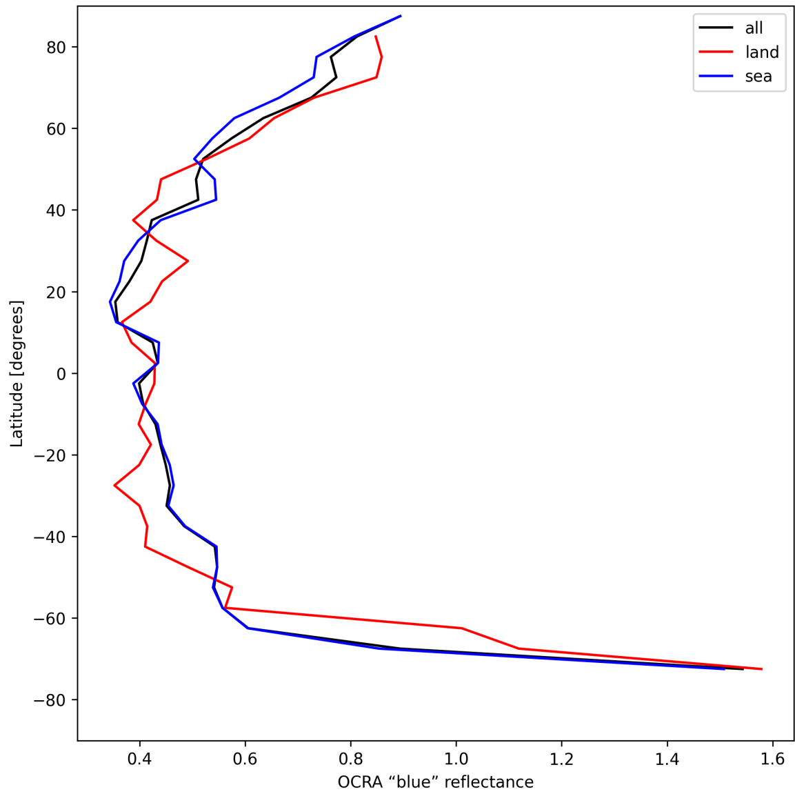
Figure 35: Zonal average of “OCRA “blue” reflectance” for 2025-05-10 to 2025-05-11.
