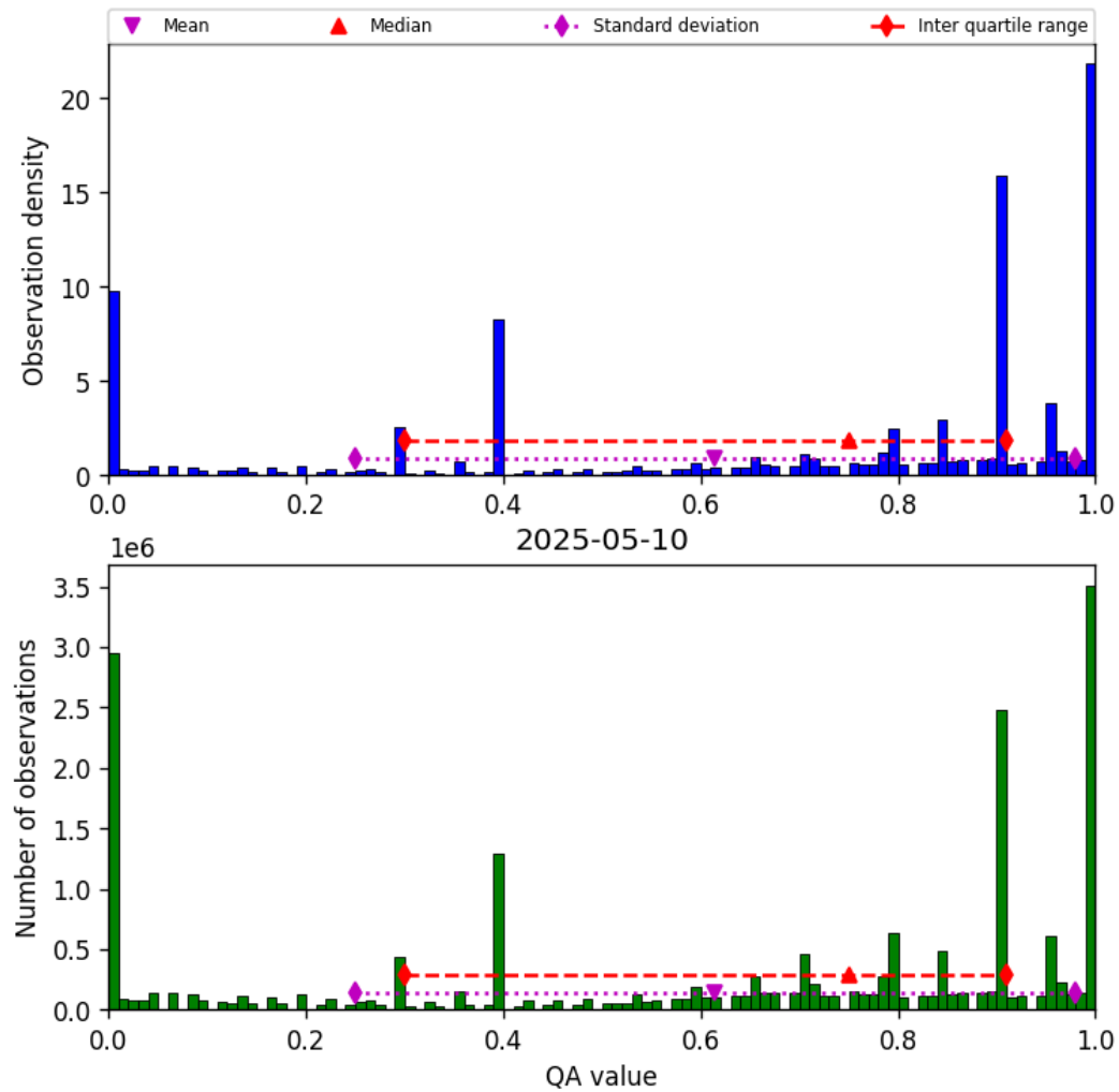
Figure 38: Histogram of “QA value” for 2025-05-10 to 2025-05-11
