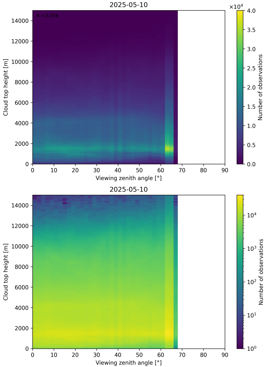
Figure 112: Scatter density plot of “Viewing zenith angle” against “Cloud top height” for 2025-05-10 to 2025-05-11.
