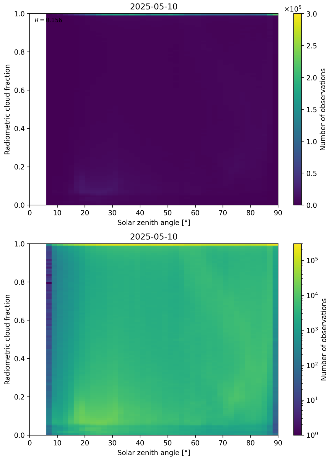
Figure 99: Scatter density plot of “Solar zenith angle” against “Radiometric cloud fraction” for 2025-05-10 to 2025-05-11.
