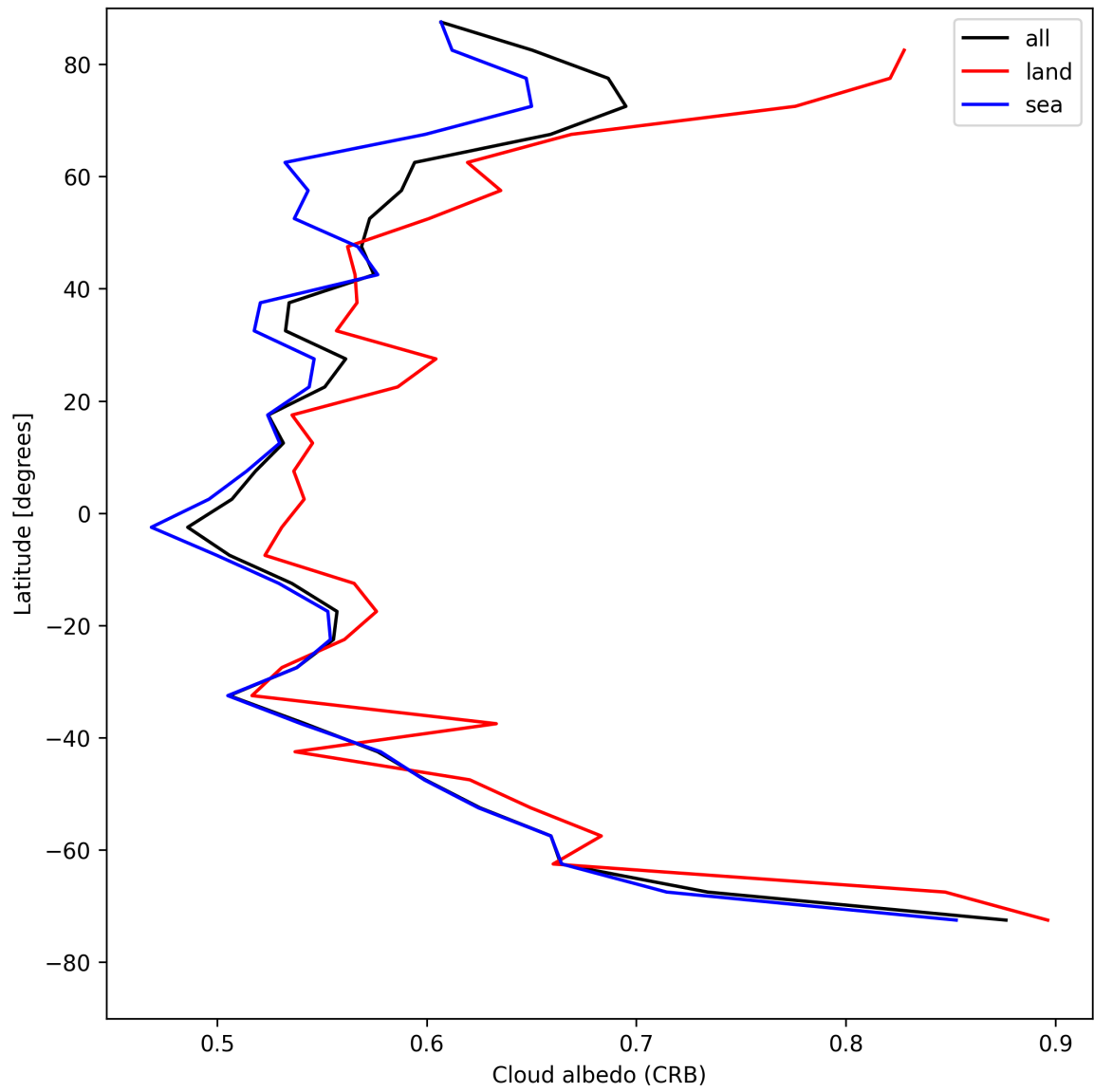
Figure 28: Zonal average of “Cloud albedo (CRB)” for 2025-05-10 to 2025-05-11.
