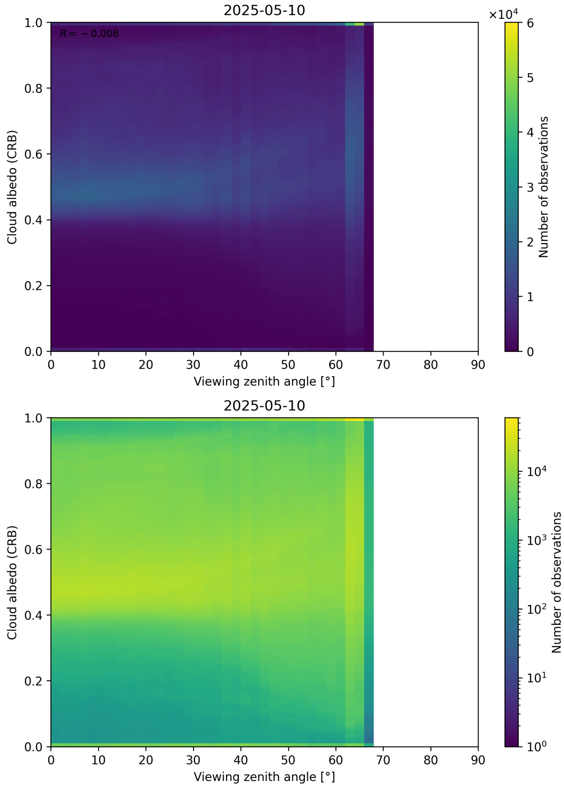
Figure 106: Scatter density plot of “Viewing zenith angle” against “Cloud albedo (CRB)” for 2025-05-10 to 2025-05-11.
