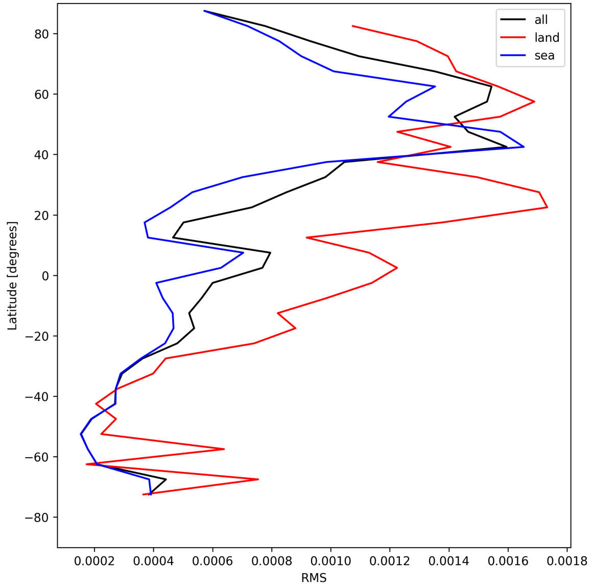
Figure 31: Zonal average of “RMS” for 2025-05-10 to 2025-05-11.
