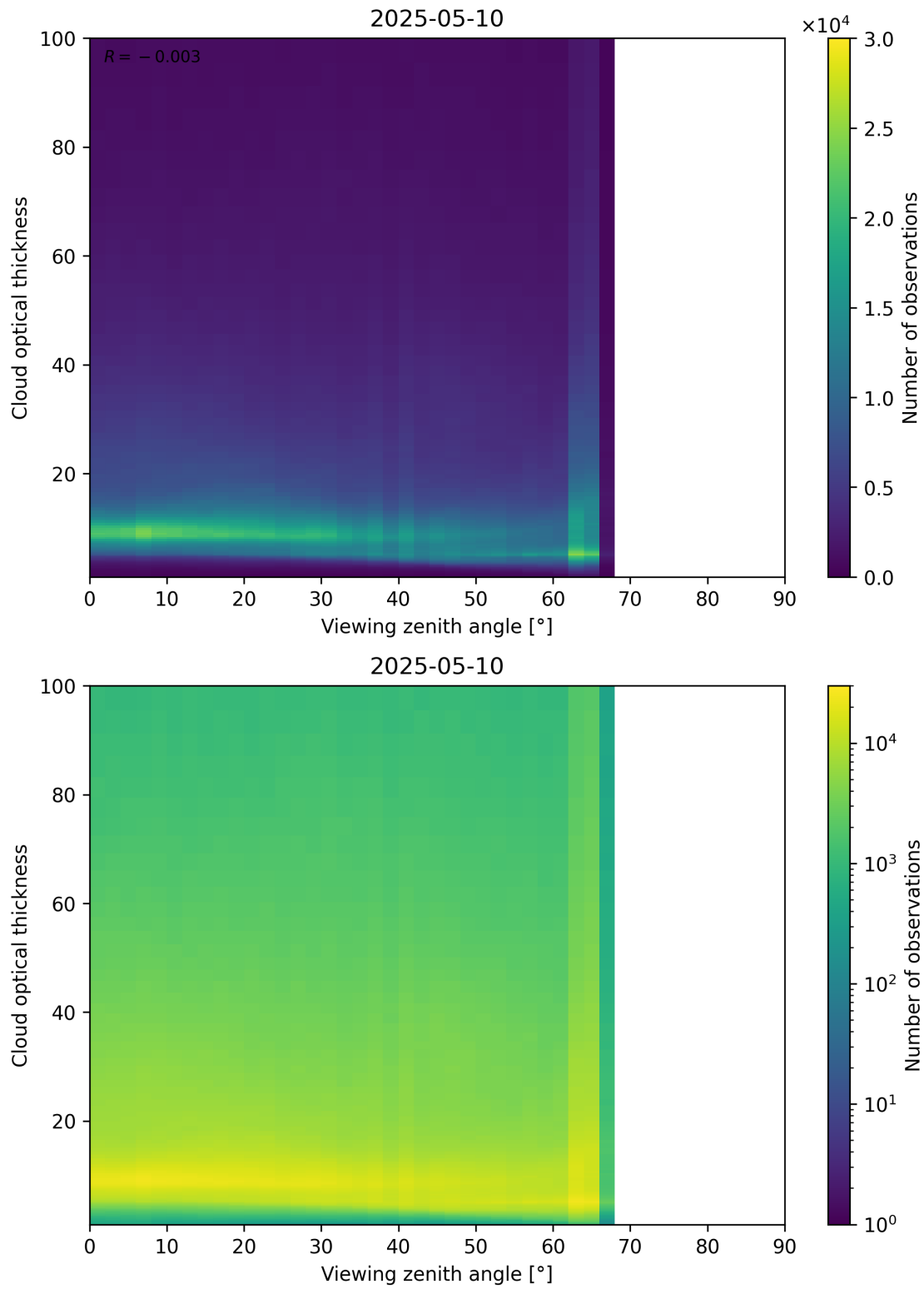
Figure 111: Scatter density plot of “Viewing zenith angle” against “Cloud optical thickness” for 2025-05-10 to 2025-05-11.
