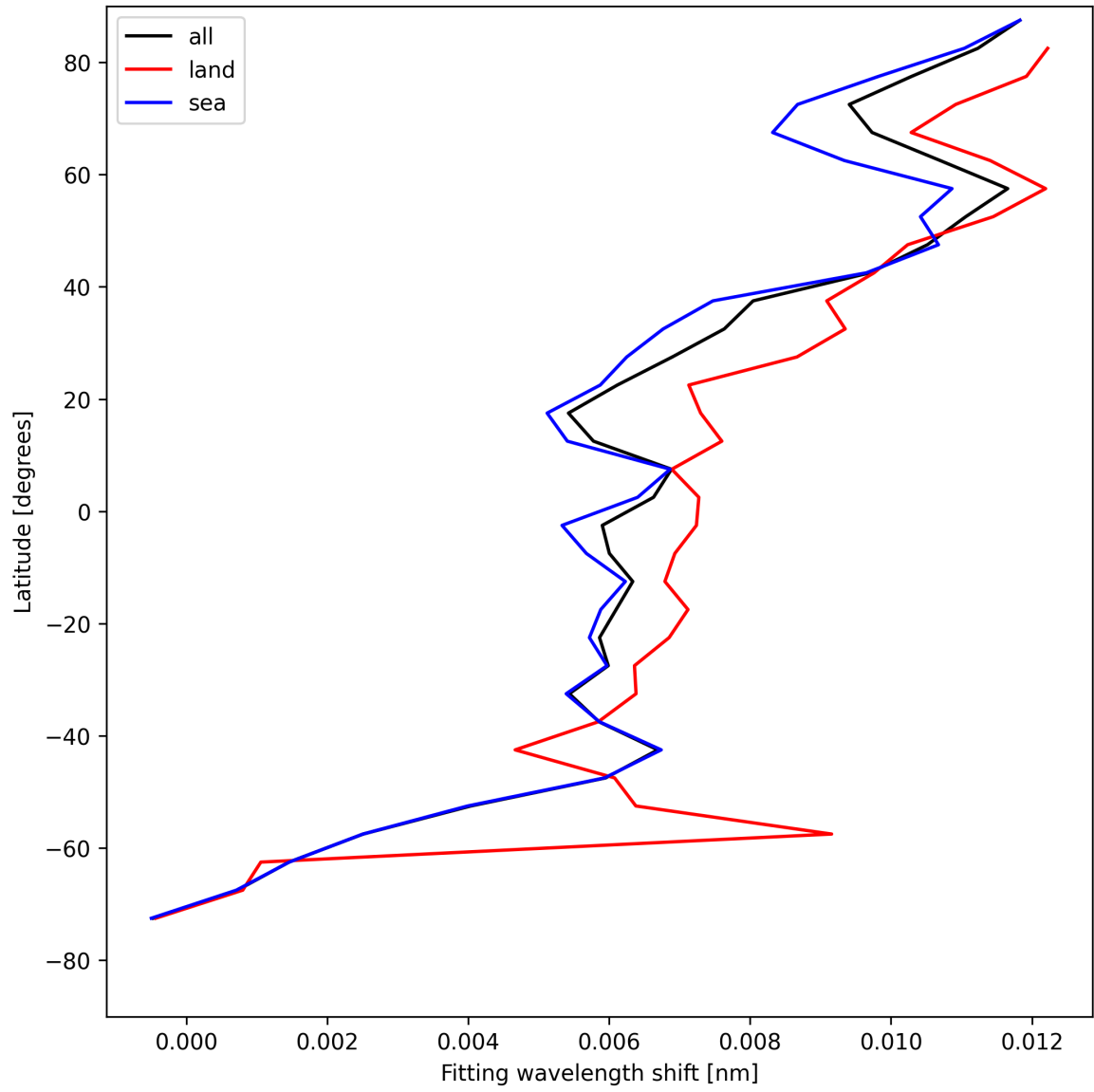
Figure 33: Zonal average of “Fitting wavelength shift” for 2025-05-10 to 2025-05-11.
