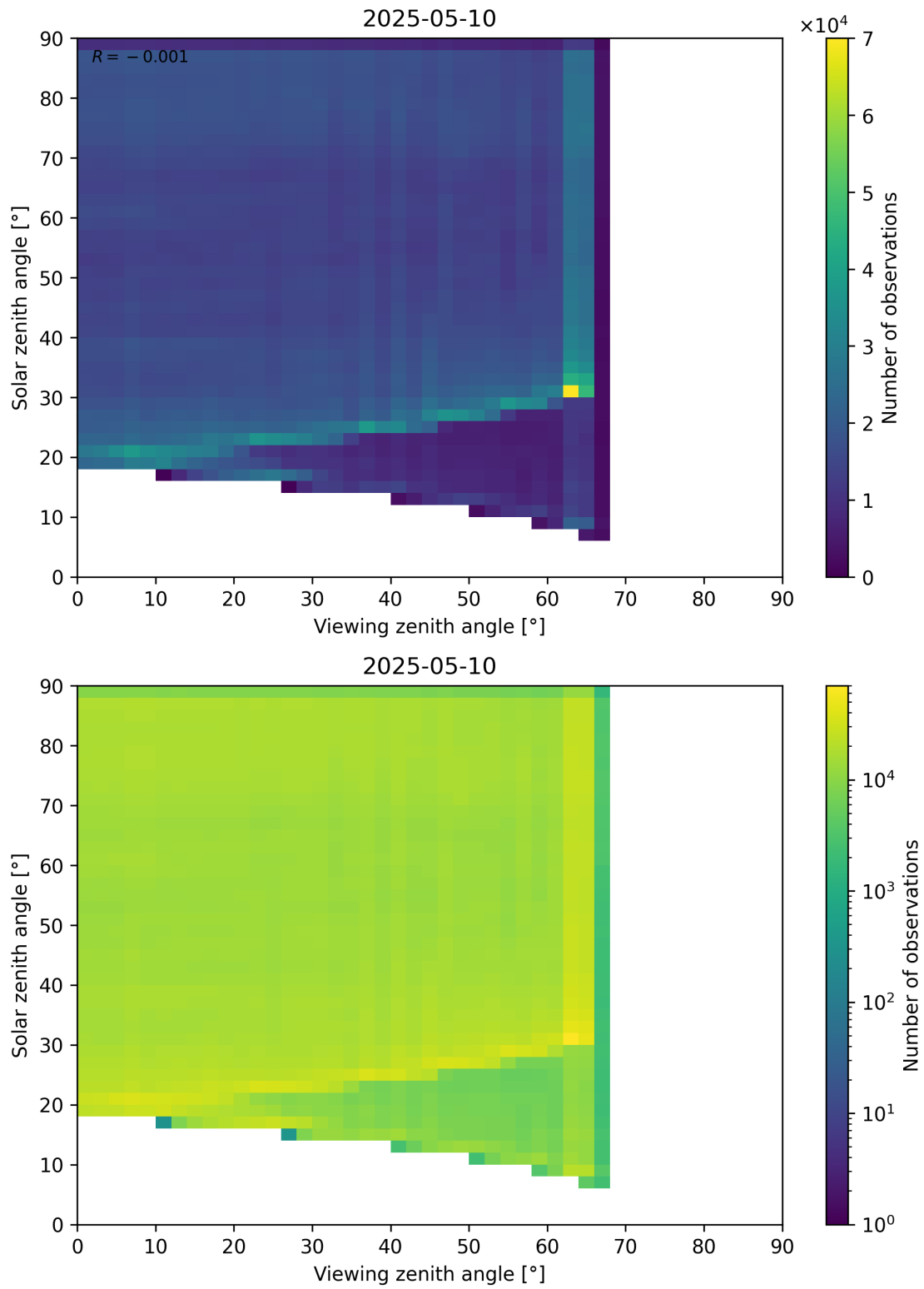
Figure 114: Scatter density plot of “Viewing zenith angle” against “Solar zenith angle” for 2025-05-10 to 2025-05-11.
