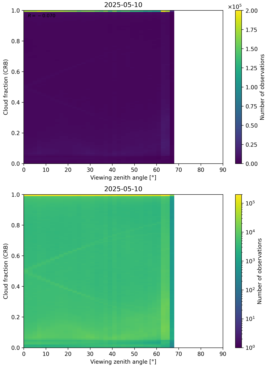
Figure 109: Scatter density plot of “Viewing zenith angle” against “Cloud fraction (CRB)” for 2025-05-10 to 2025-05-11.
