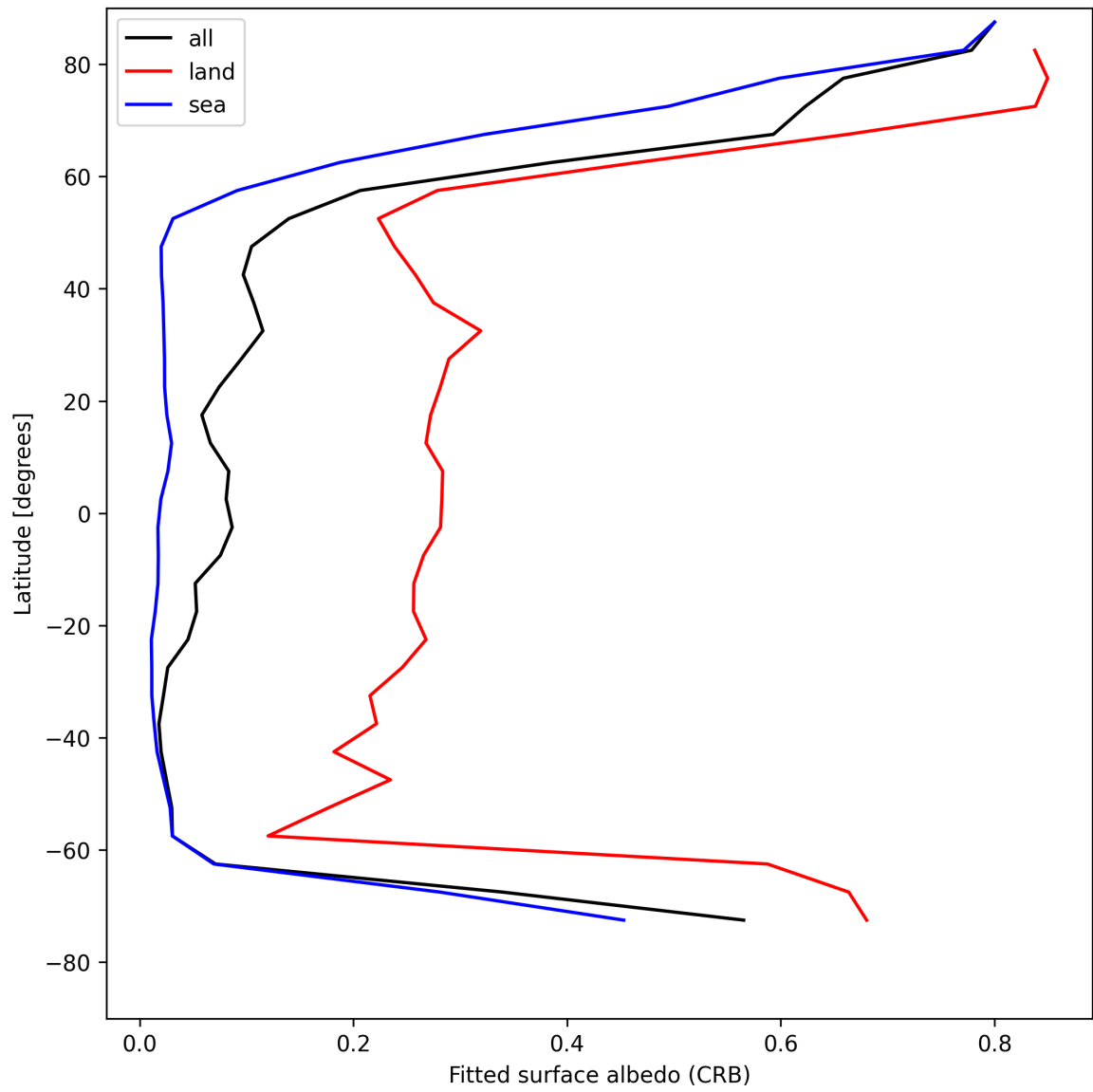
Figure 30: Zonal average of “Fitted surface albedo (CRB)” for 2025-05-10 to 2025-05-11.
