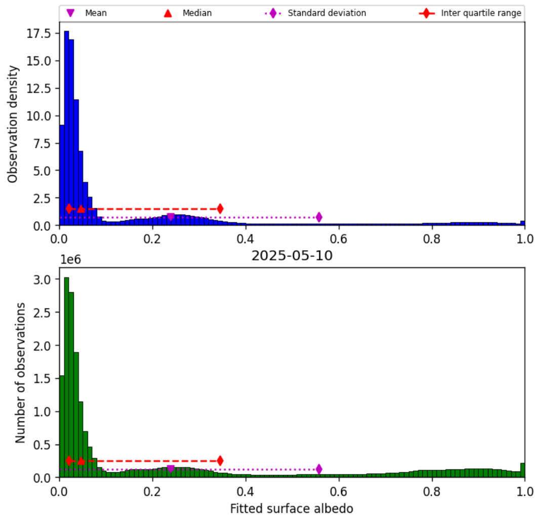
Figure 45: Histogram of “Fitted surface albedo” for 2025-05-10 to 2025-05-11
