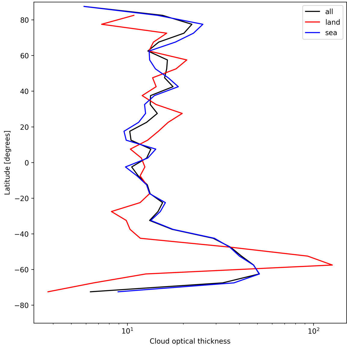
Figure 25: Zonal average of “Cloud optical thickness” for 2025-05-10 to 2025-05-11.
