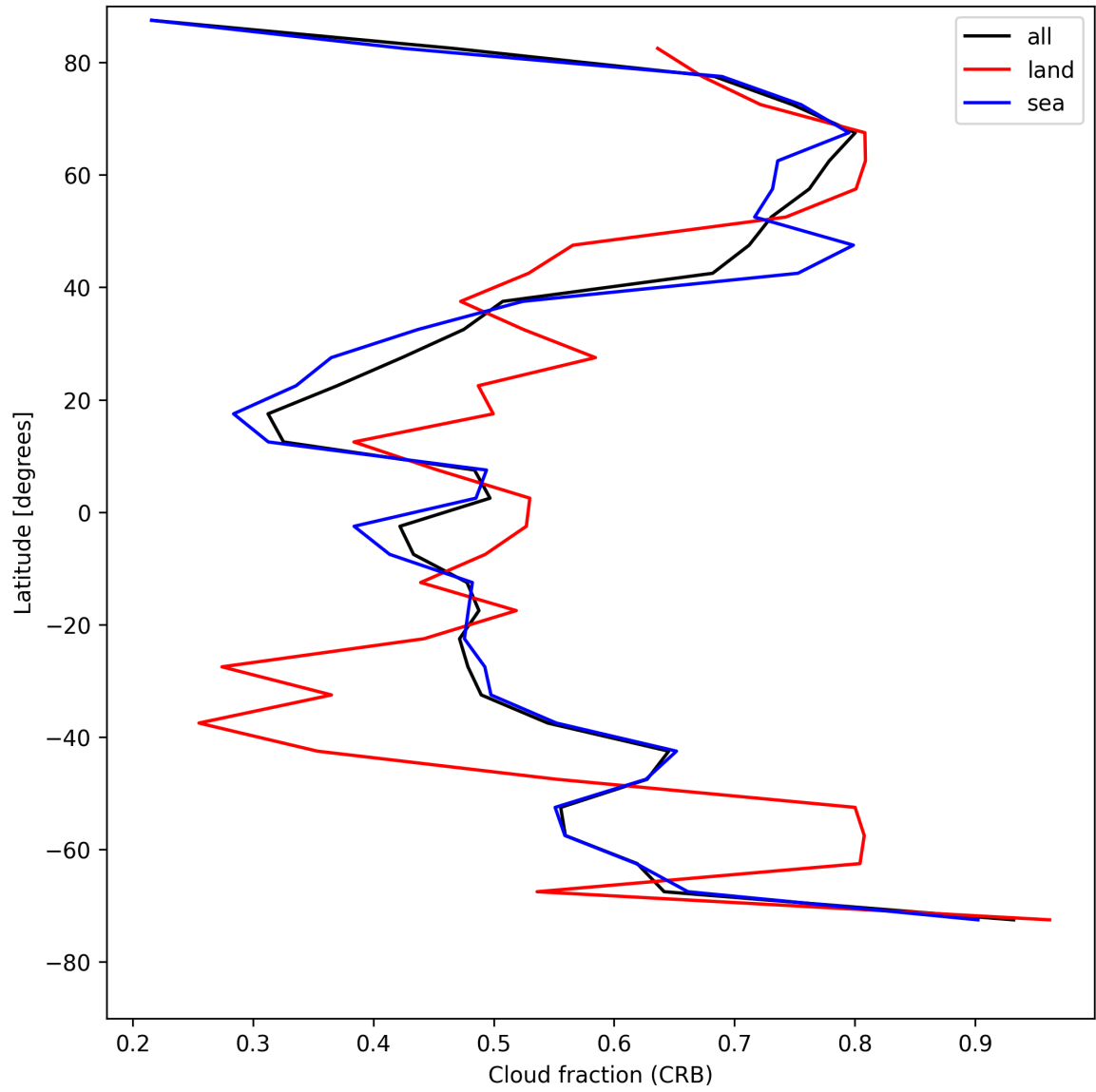
Figure 26: Zonal average of “Cloud fraction (CRB)” for 2025-05-10 to 2025-05-11.
