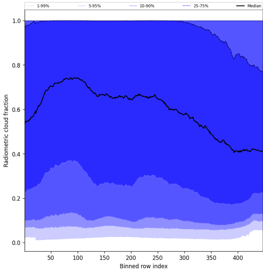
Figure 55: Along track statistics of “Radiometric cloud fraction” for 2025-05-10 to 2025-05-11
