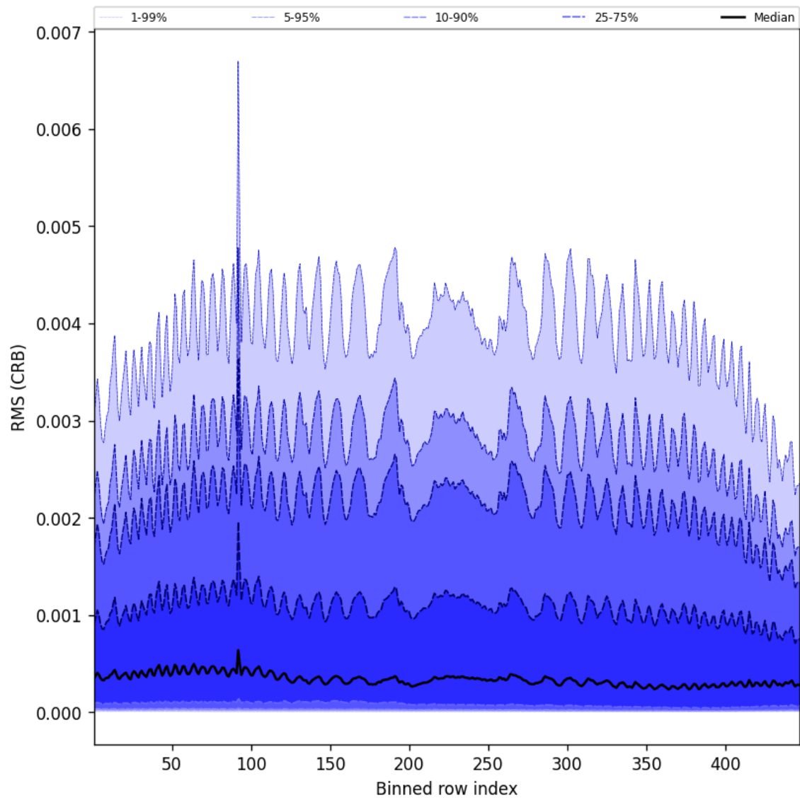
Figure 64: Along track statistics of “RMS (CRB)” for 2025-05-10 to 2025-05-11
