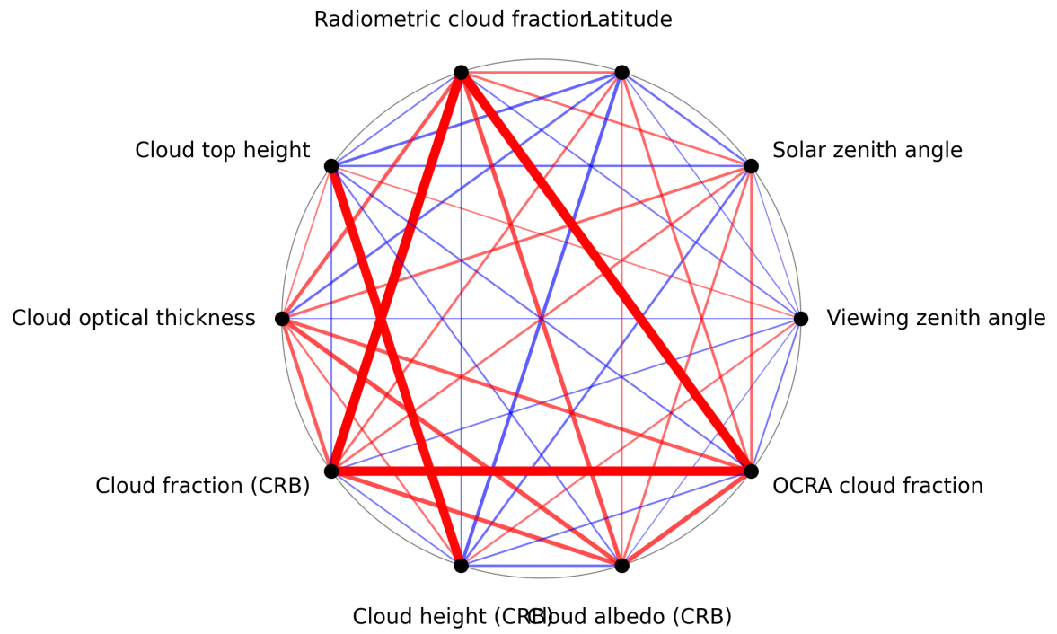
Figure 1: Map of correlation graph for 2025-05-10 to 2025-05-11.
