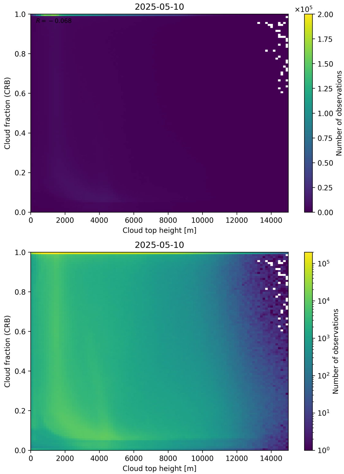
Figure 88: Scatter density plot of “Cloud top height” against “Cloud fraction (CRB)” for 2025-05-10 to 2025-05-11.
