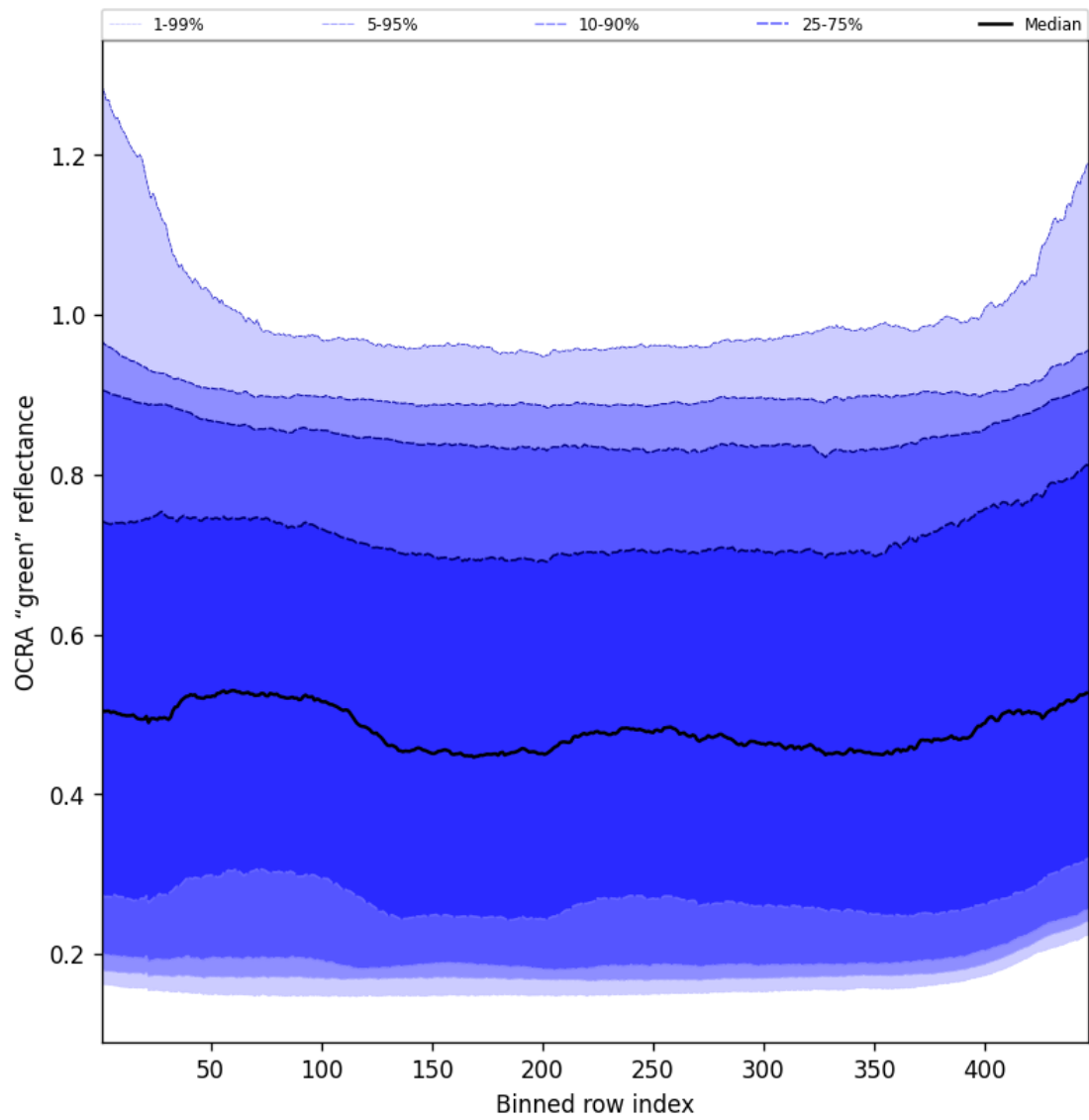
Figure 68: Along track statistics of “OCRA “green” reflectance” for 2025-05-10 to 2025-05-11
