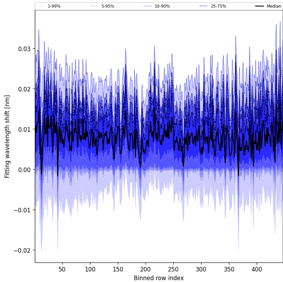
Figure 65: Along track statistics of “Fitting wavelength shift” for 2025-05-10 to 2025-05-11
