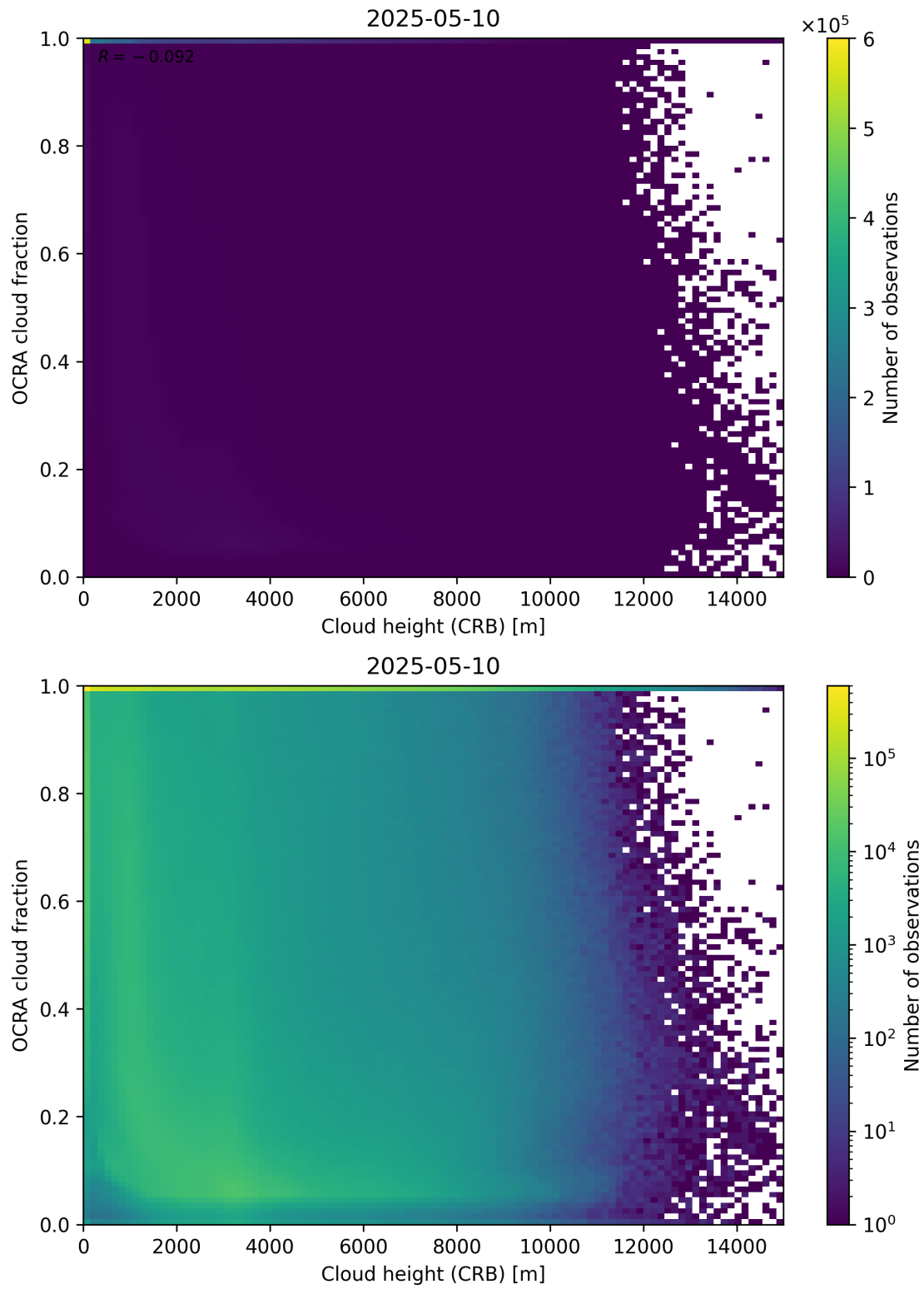
Figure 81: Scatter density plot of “Cloud height (CRB)” against “OCRA cloud fraction” for 2025-05-10 to 2025-05-11.
