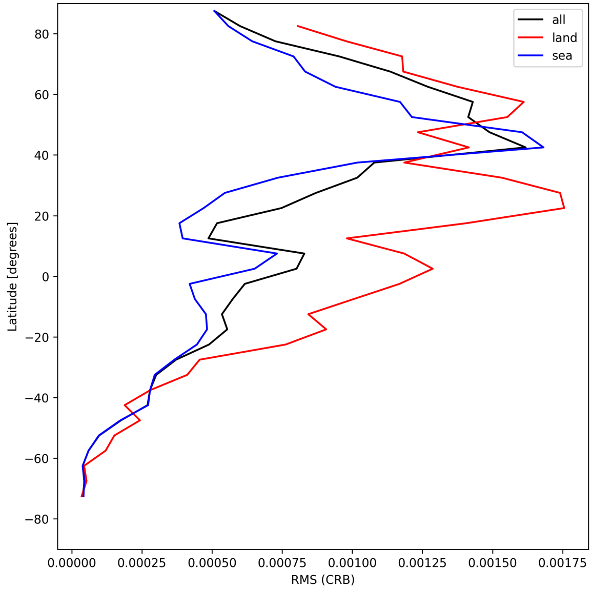
Figure 32: Zonal average of “RMS (CRB)” for 2025-05-10 to 2025-05-11.
