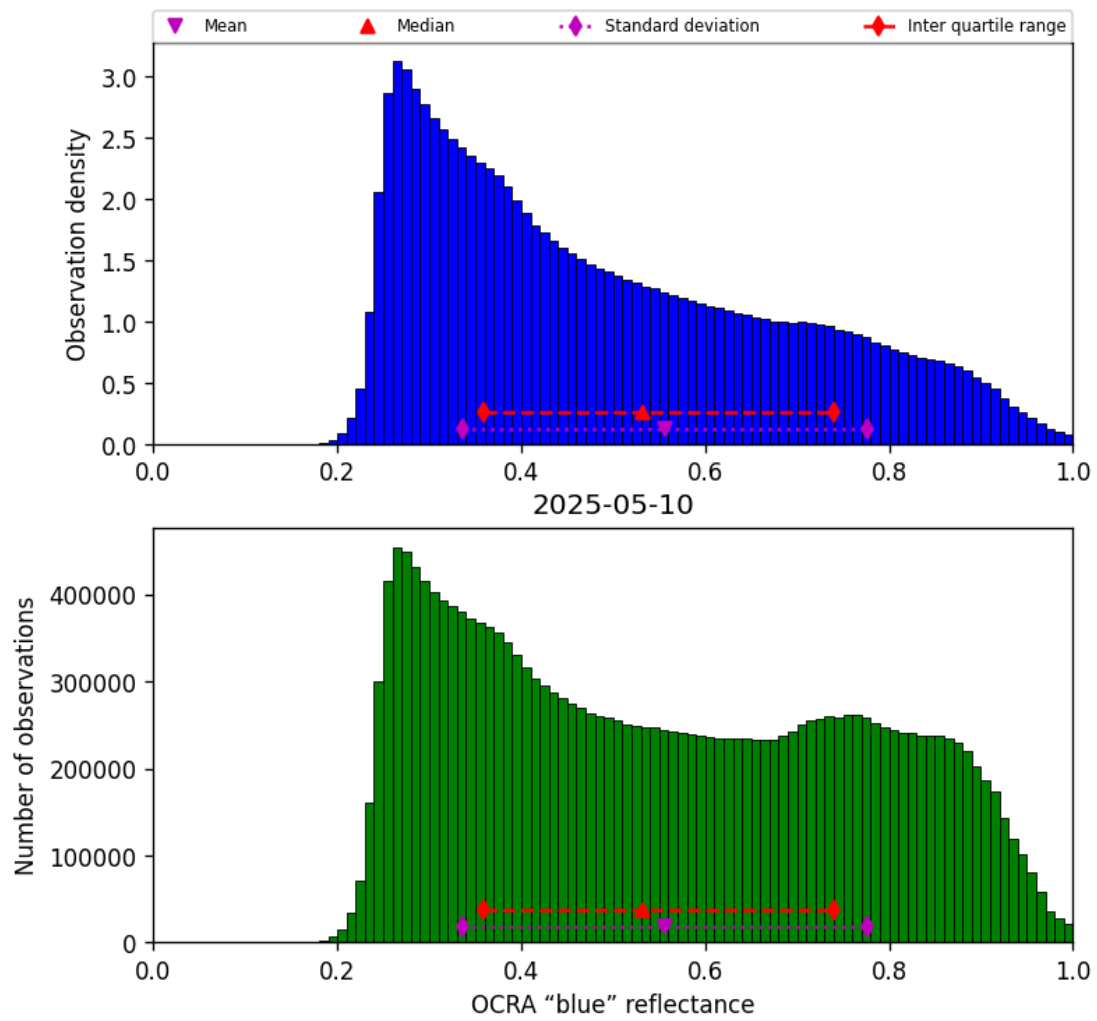
Figure 51: Histogram of “OCRA “blue” reflectance” for 2025-05-10 to 2025-05-11
