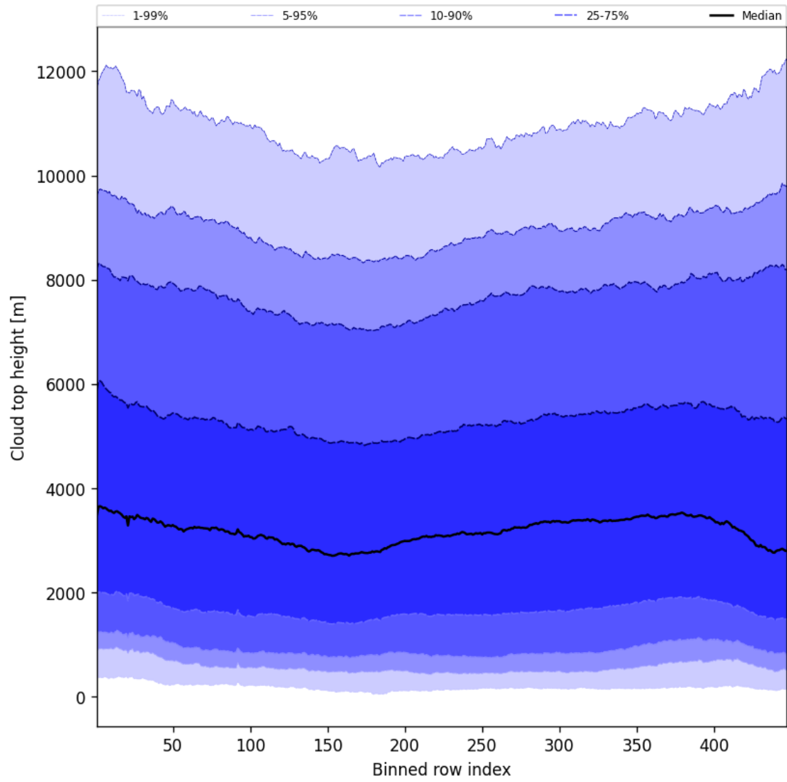
Figure 56: Along track statistics of “Cloud top height” for 2025-05-10 to 2025-05-11
