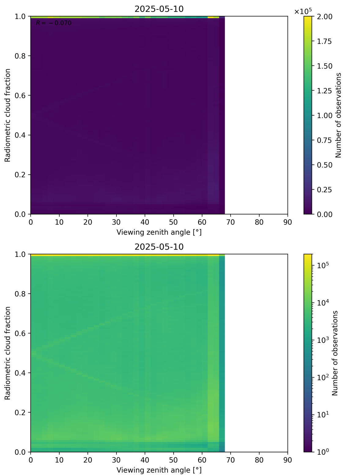
Figure 107: Scatter density plot of “Viewing zenith angle” against “Radiometric cloud fraction” for 2025-05-10 to 2025-05-11.
