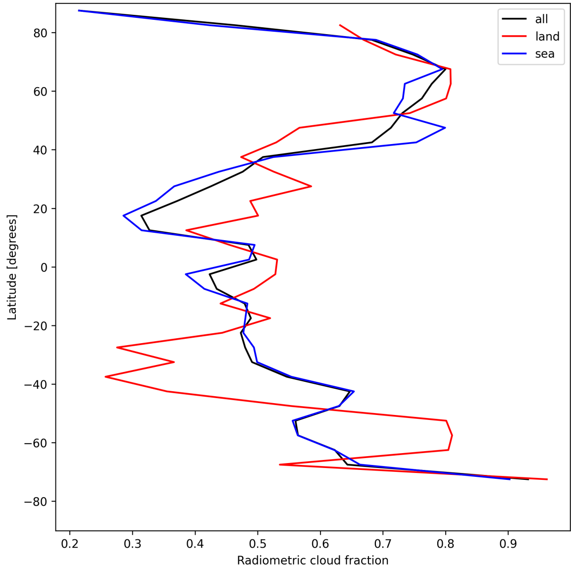
Figure 23: Zonal average of “Radiometric cloud fraction” for 2025-05-10 to 2025-05-11.
