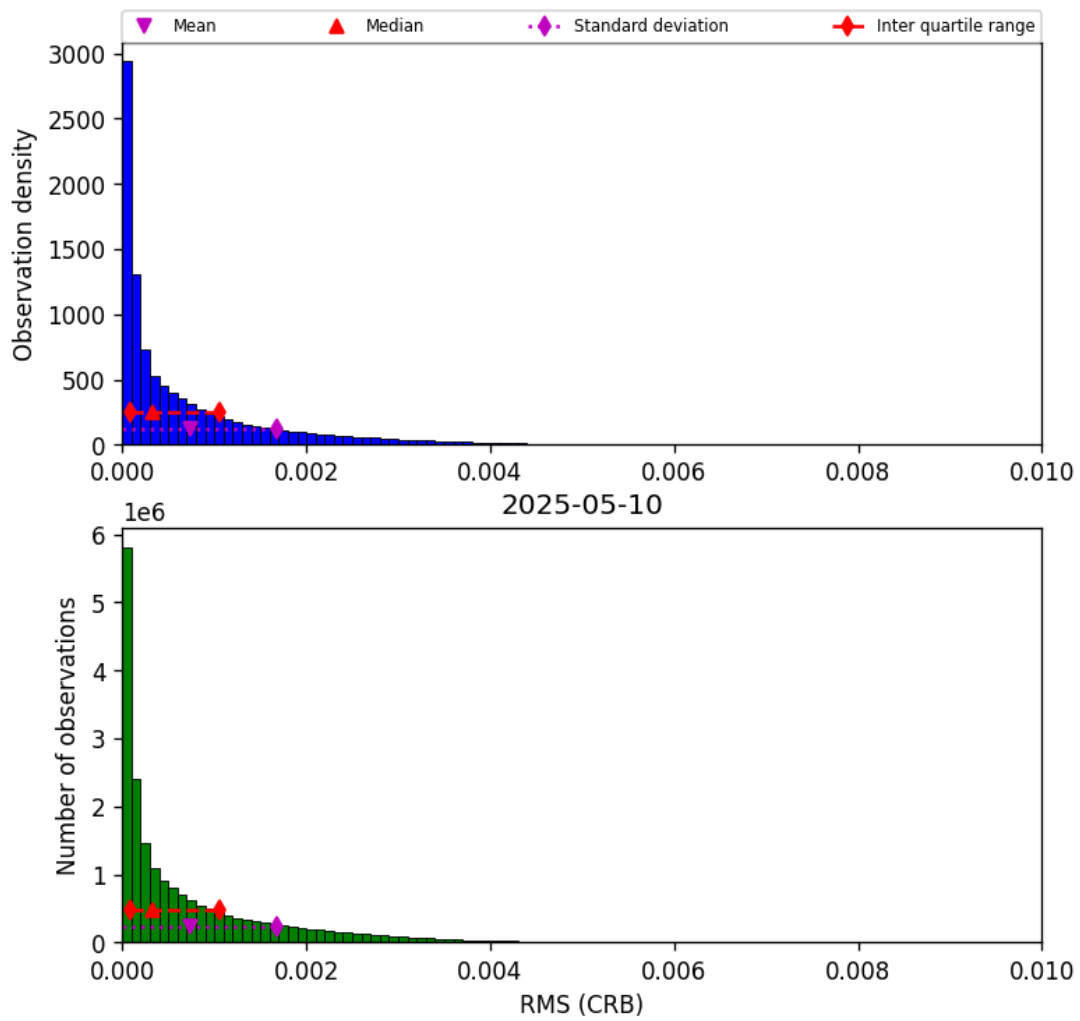
Figure 48: Histogram of “RMS (CRB)” for 2025-05-10 to 2025-05-11
