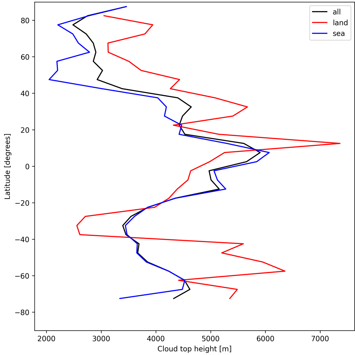
Figure 24: Zonal average of “Cloud top height” for 2025-05-10 to 2025-05-11.
