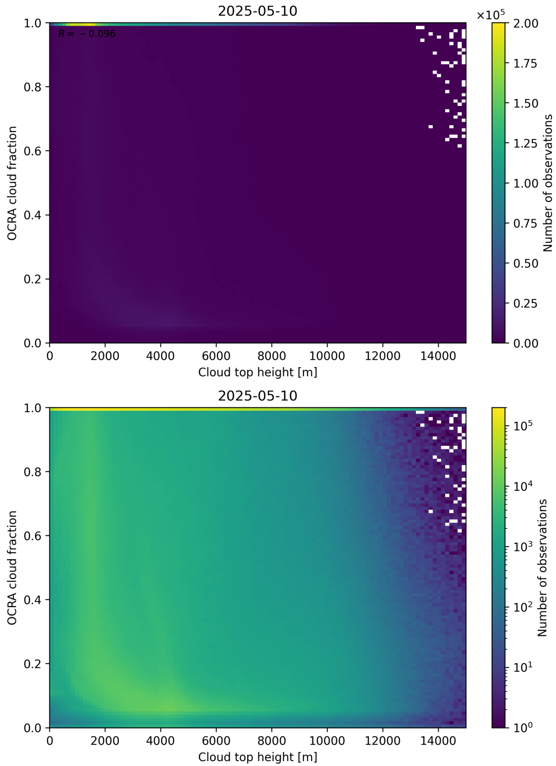
Figure 87: Scatter density plot of “Cloud top height” against “OCRA cloud fraction” for 2025-05-10 to 2025-05-11.
