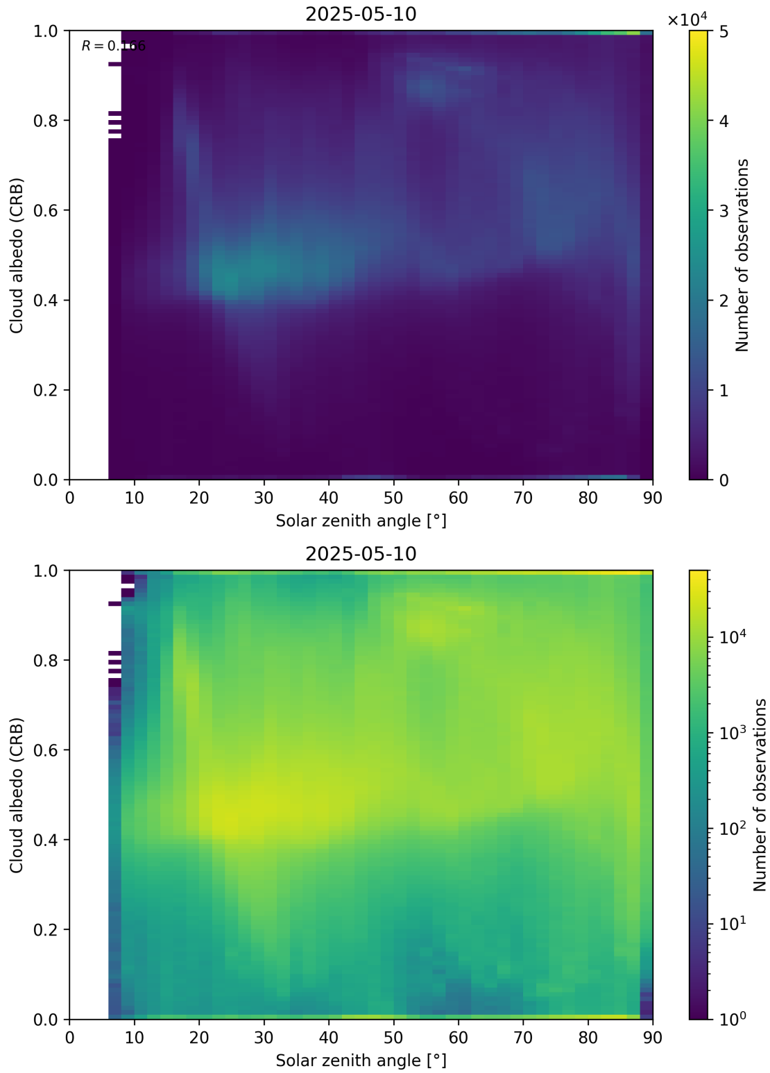
Figure 98: Scatter density plot of “Solar zenith angle” against “Cloud albedo (CRB)” for 2025-05-10 to 2025-05-11.
