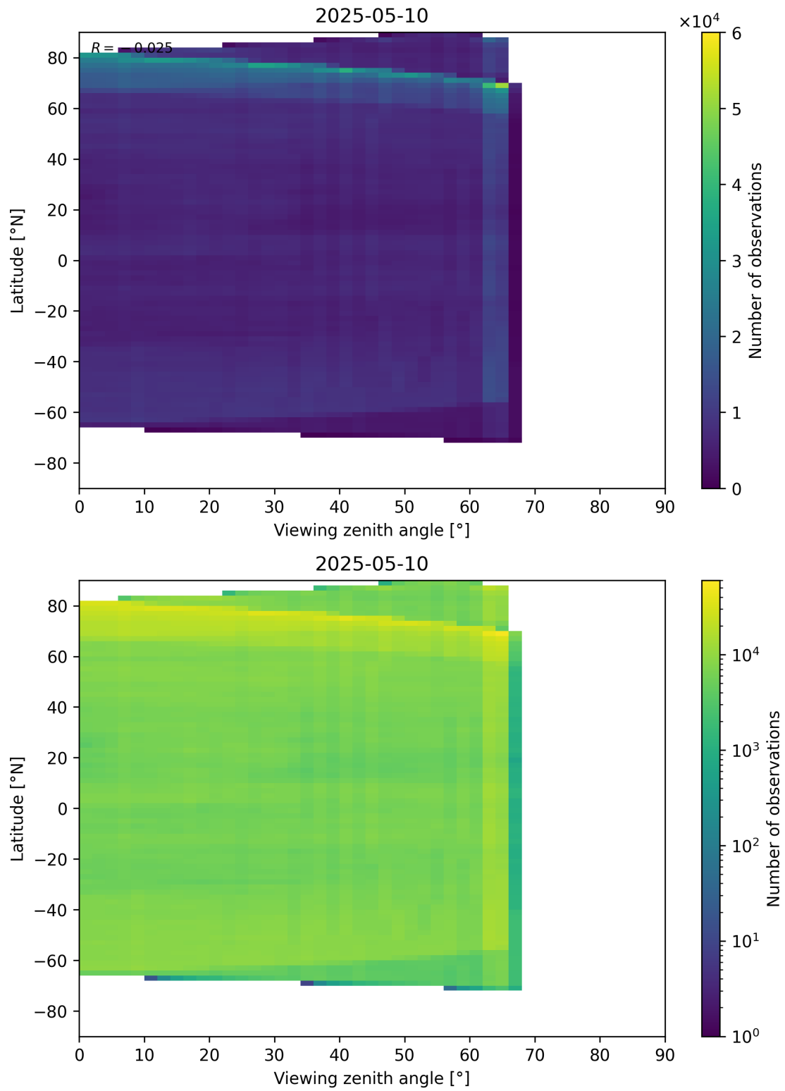
Figure 113: Scatter density plot of “Viewing zenith angle” against “Latitude” for 2025-05-10 to 2025-05-11.
