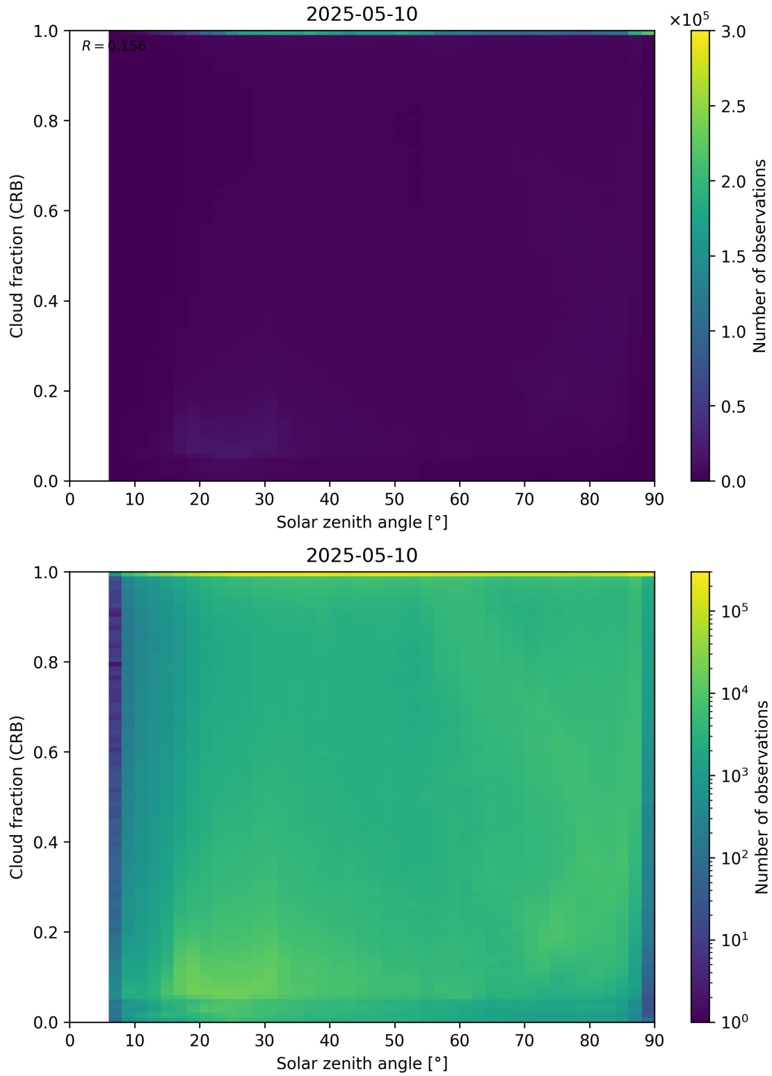
Figure 101: Scatter density plot of “Solar zenith angle” against “Cloud fraction (CRB)” for 2025-05-10 to 2025-05-11.
