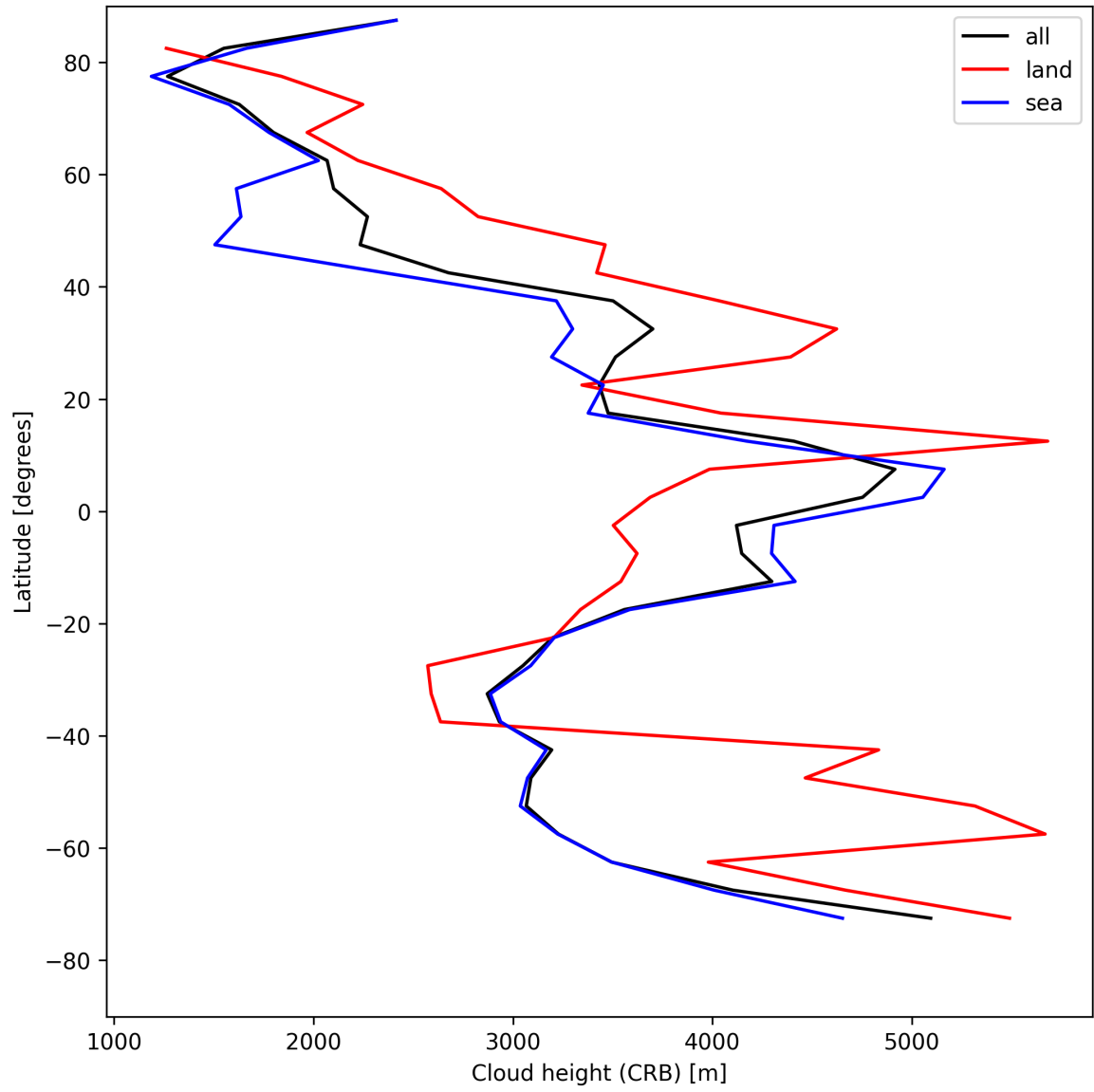
Figure 27: Zonal average of “Cloud height (CRB)” for 2025-05-10 to 2025-05-11.
