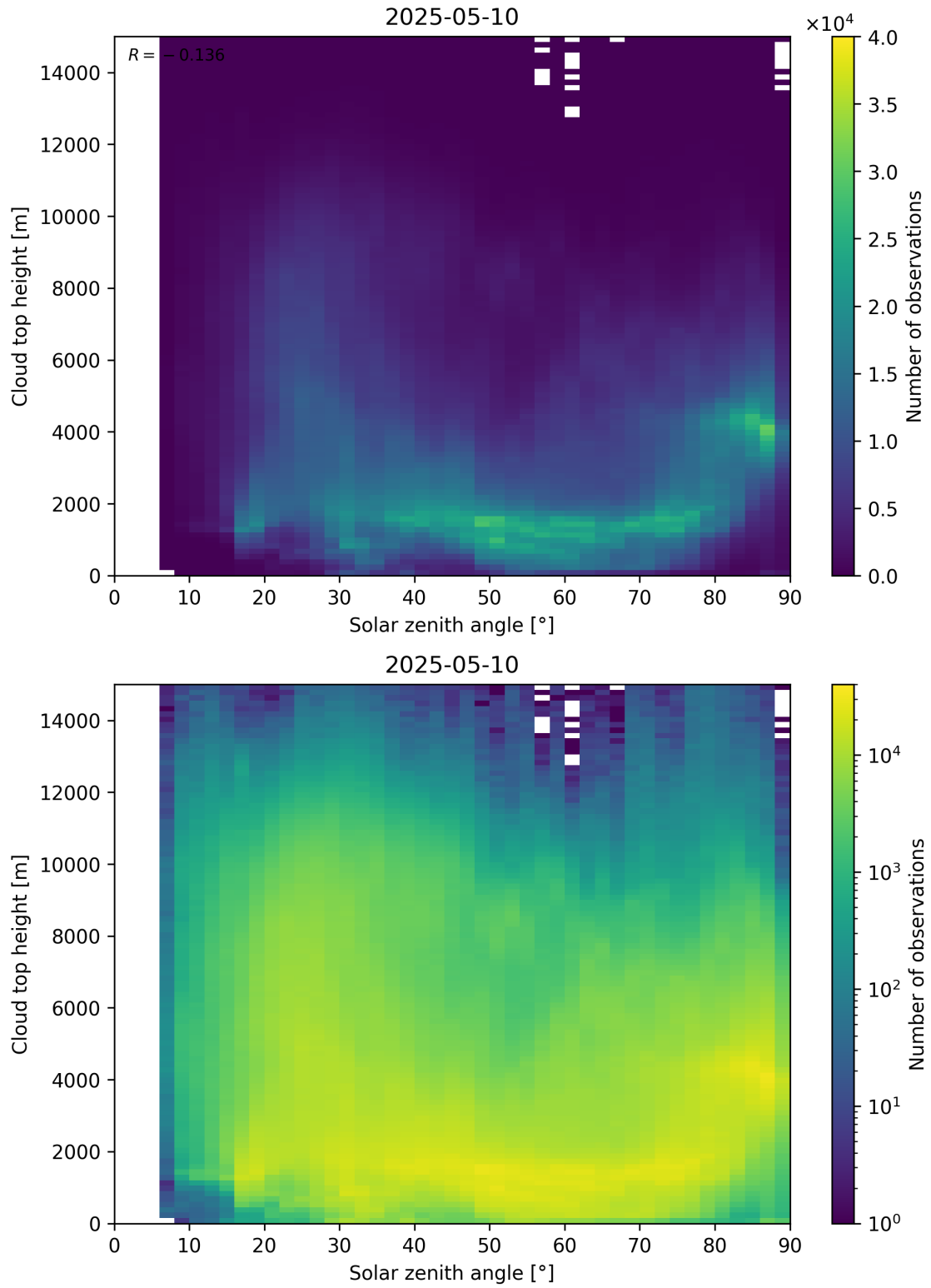
Figure 104: Scatter density plot of “Solar zenith angle” against “Cloud top height” for 2025-05-10 to 2025-05-11.
