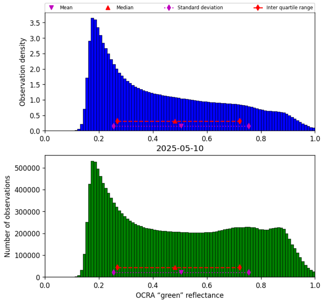
Figure 52: Histogram of “OCRA “green” reflectance” for 2025-05-10 to 2025-05-11
