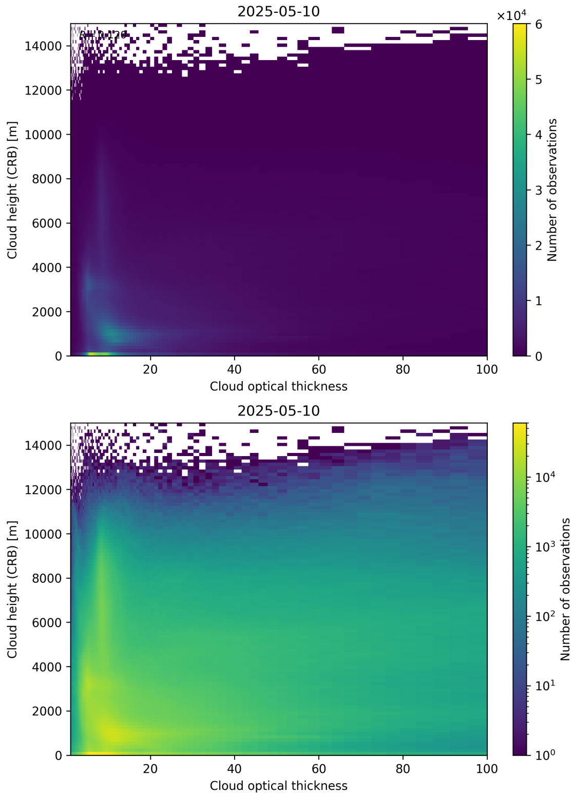
Figure 85: Scatter density plot of “Cloud optical thickness” against “Cloud height (CRB)” for 2025-05-10 to 2025-05-11.
