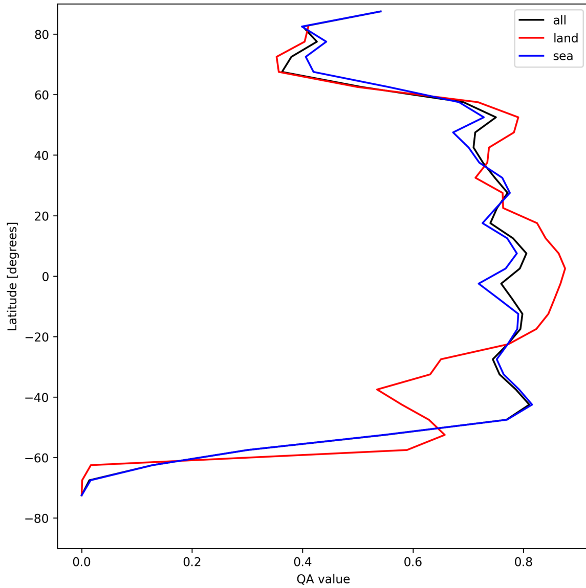
Figure 22: Zonal average of “QA value” for 2025-05-10 to 2025-05-11.
