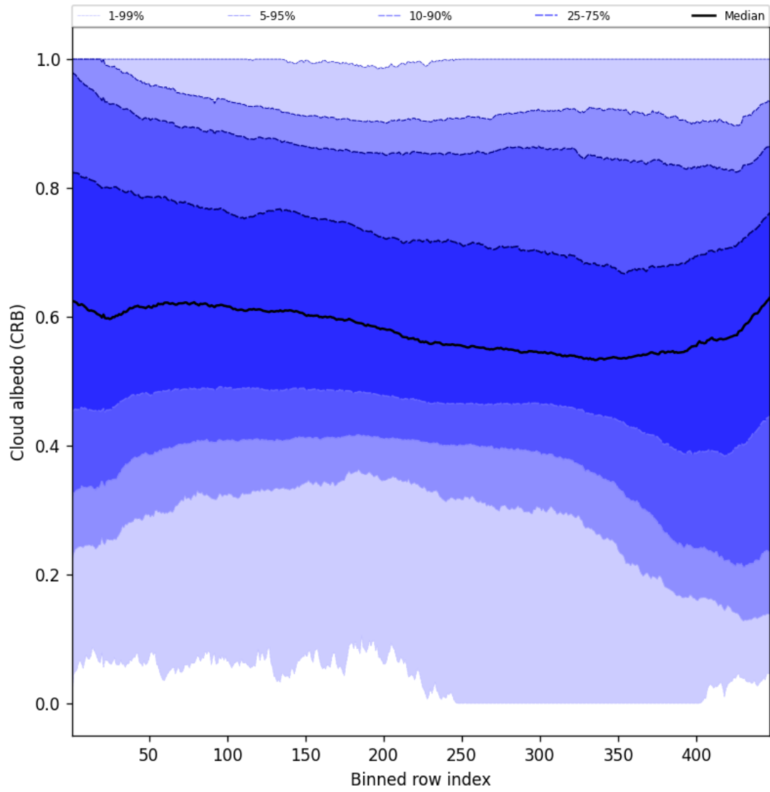
Figure 60: Along track statistics of “Cloud albedo (CRB)” for 2025-05-10 to 2025-05-11
