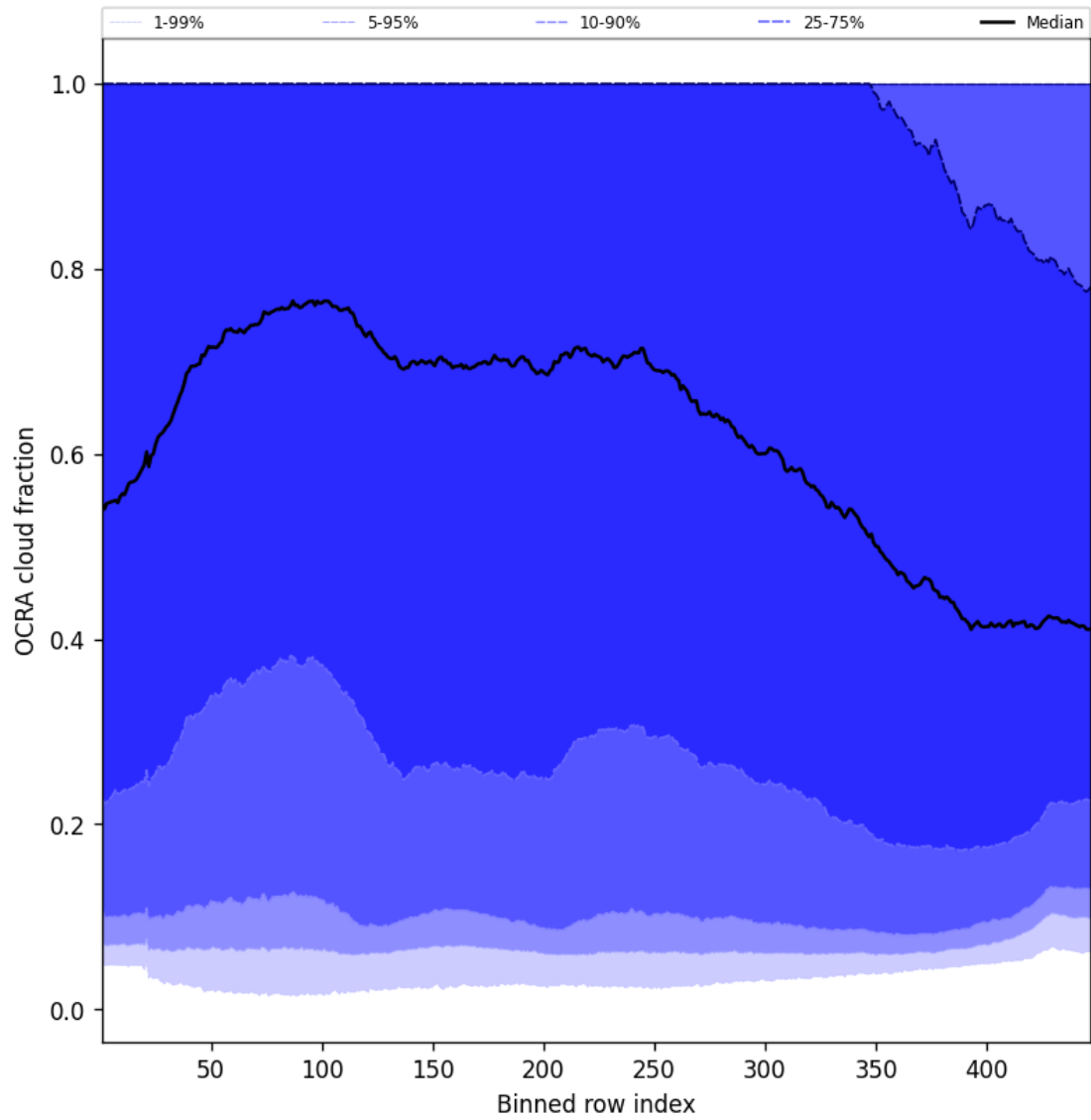
Figure 66: Along track statistics of “OCRA cloud fraction” for 2025-05-10 to 2025-05-11
