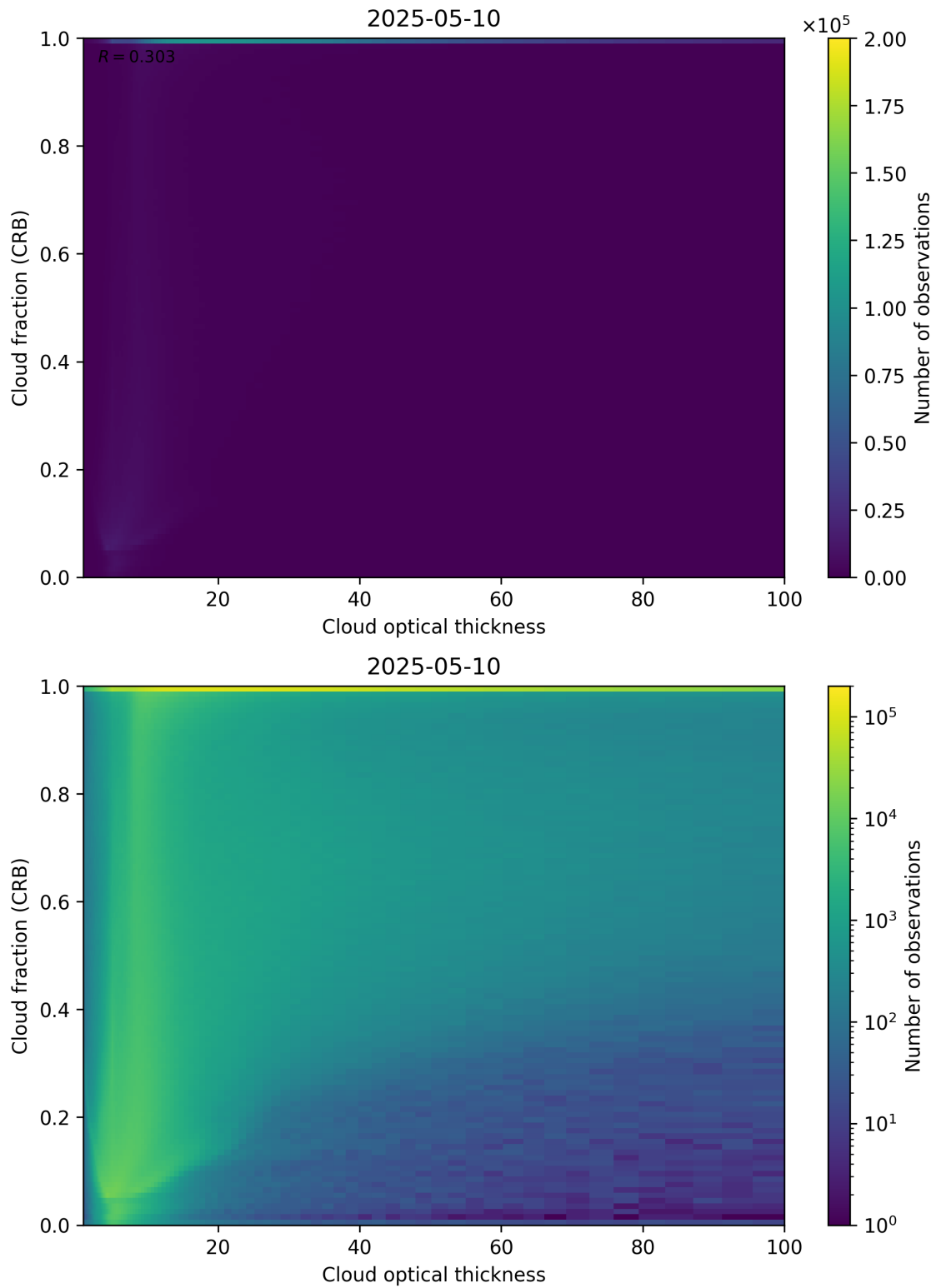
Figure 84: Scatter density plot of “Cloud optical thickness” against “Cloud fraction (CRB)” for 2025-05-10 to 2025-05-11.
