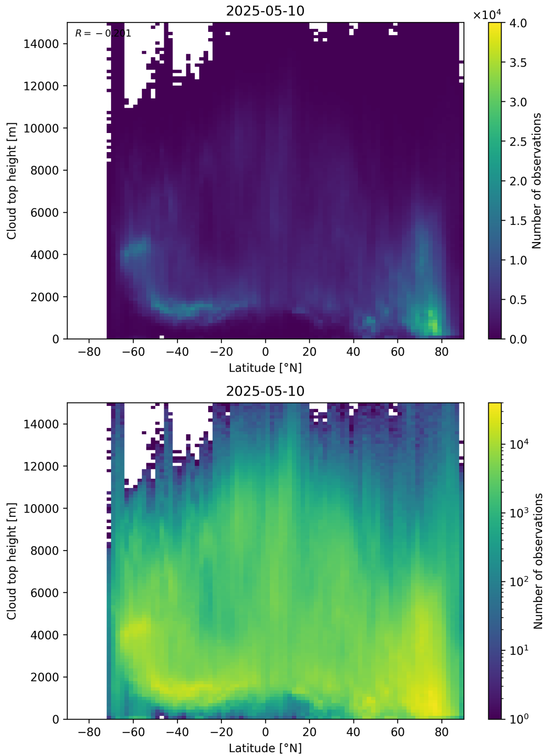
Figure 97: Scatter density plot of “Latitude” against “Cloud top height” for 2025-05-10 to 2025-05-11.
