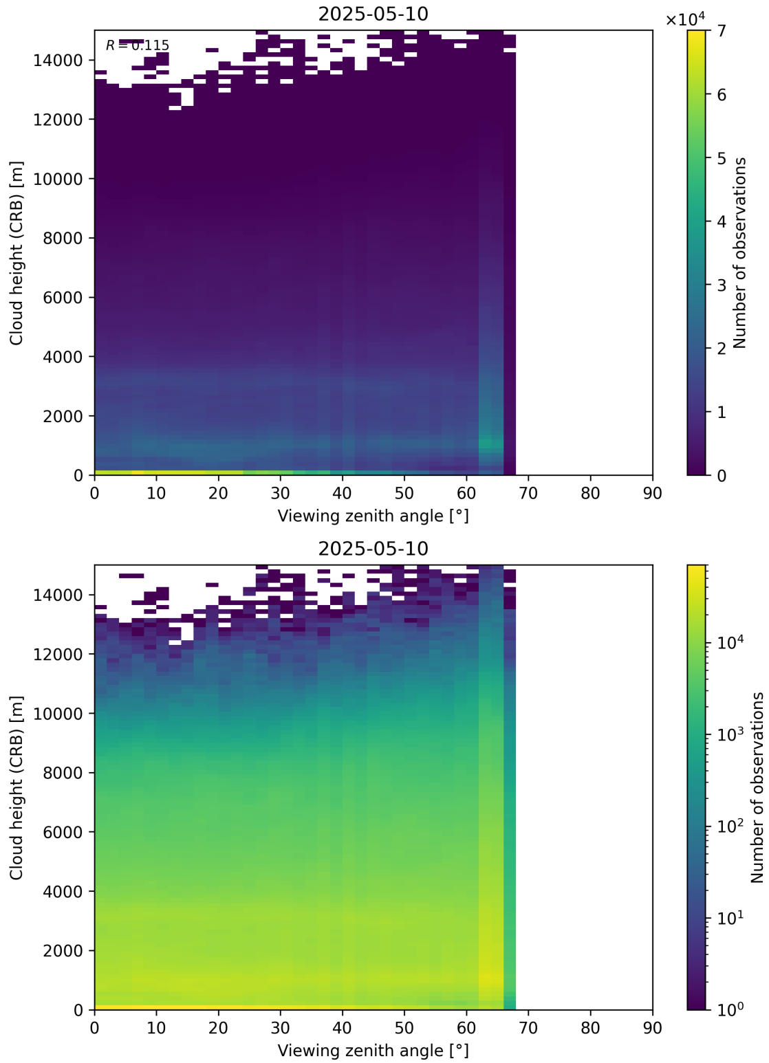
Figure 110: Scatter density plot of “Viewing zenith angle” against “Cloud height (CRB)” for 2025-05-10 to 2025-05-11.
