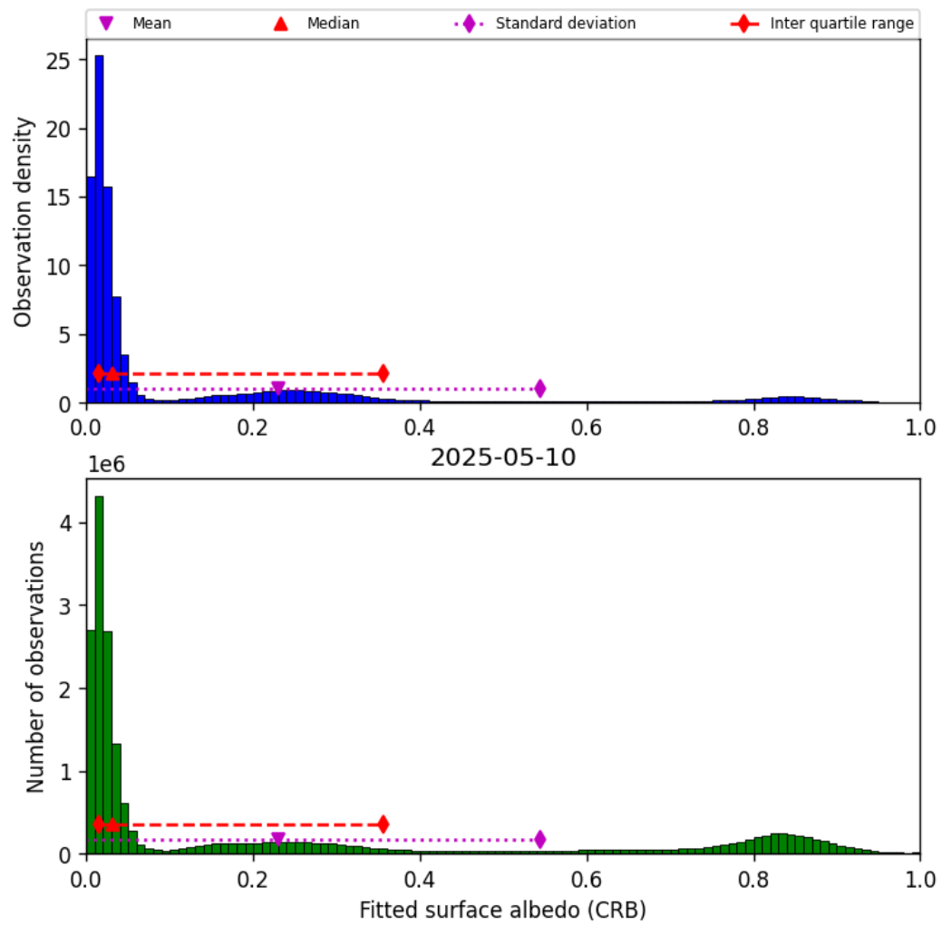
Figure 46: Histogram of “Fitted surface albedo (CRB)” for 2025-05-10 to 2025-05-11
