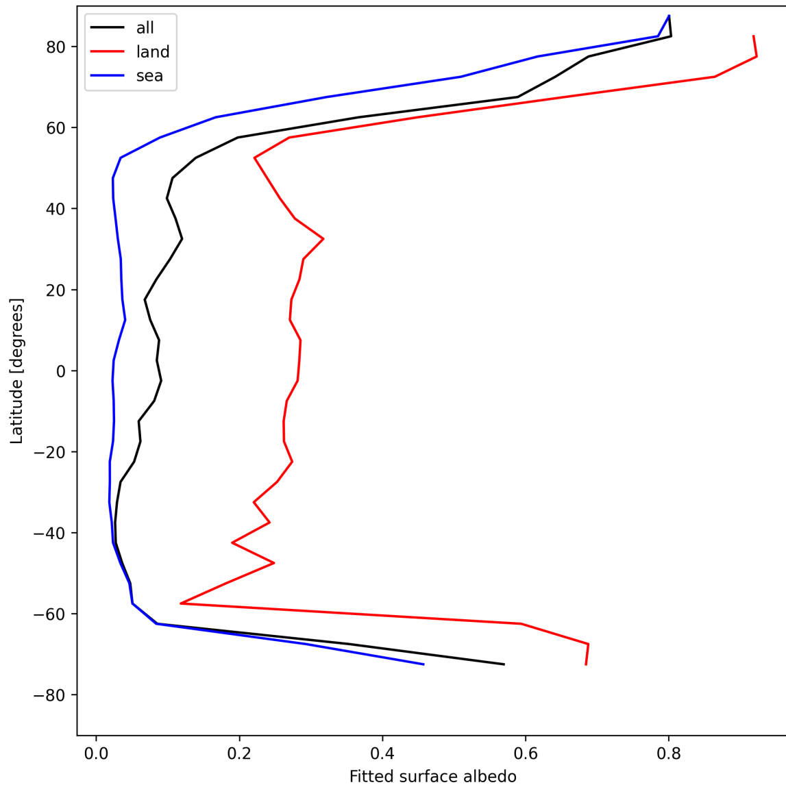
Figure 29: Zonal average of “Fitted surface albedo” for 2025-05-10 to 2025-05-11.
