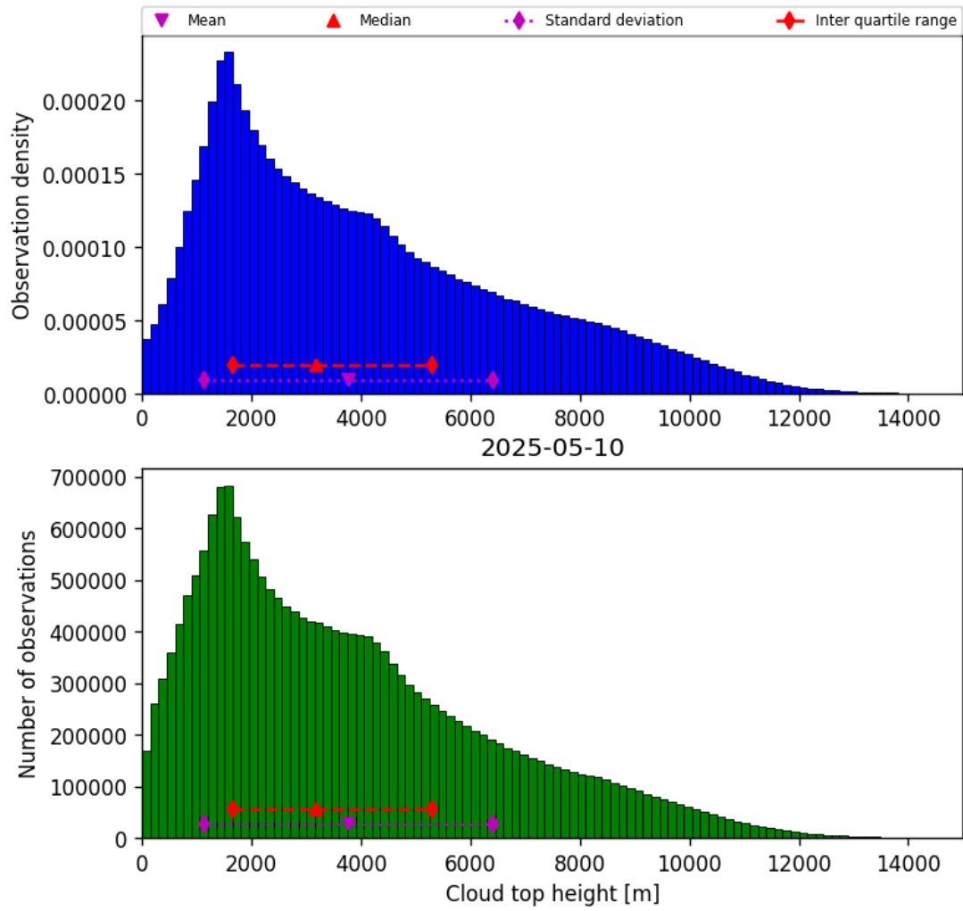
Figure 40: Histogram of “Cloud top height” for 2025-05-10 to 2025-05-11
