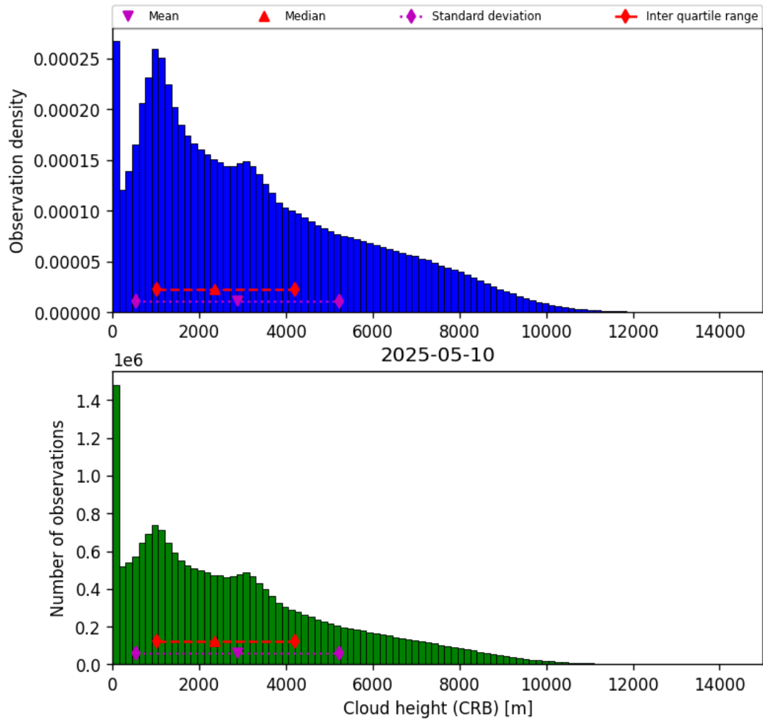
Figure 43: Histogram of “Cloud height (CRB)” for 2025-05-10 to 2025-05-11
