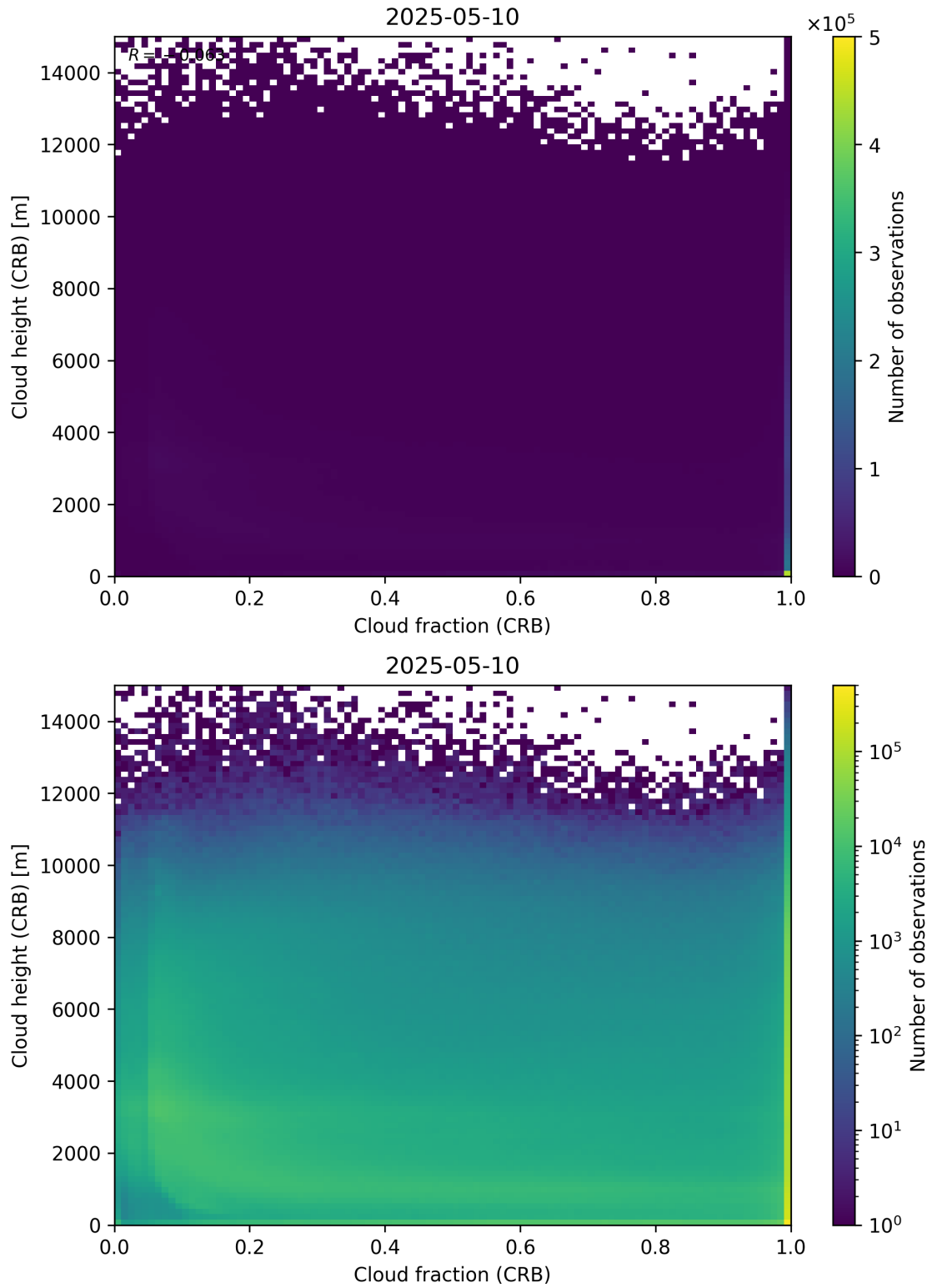
Figure 79: Scatter density plot of “Cloud fraction (CRB)” against “Cloud height (CRB)” for 2025-05-10 to 2025-05-11.
