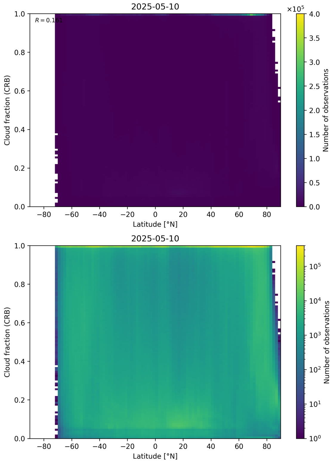
Figure 94: Scatter density plot of “Latitude” against “Cloud fraction (CRB)” for 2025-05-10 to 2025-05-11.
