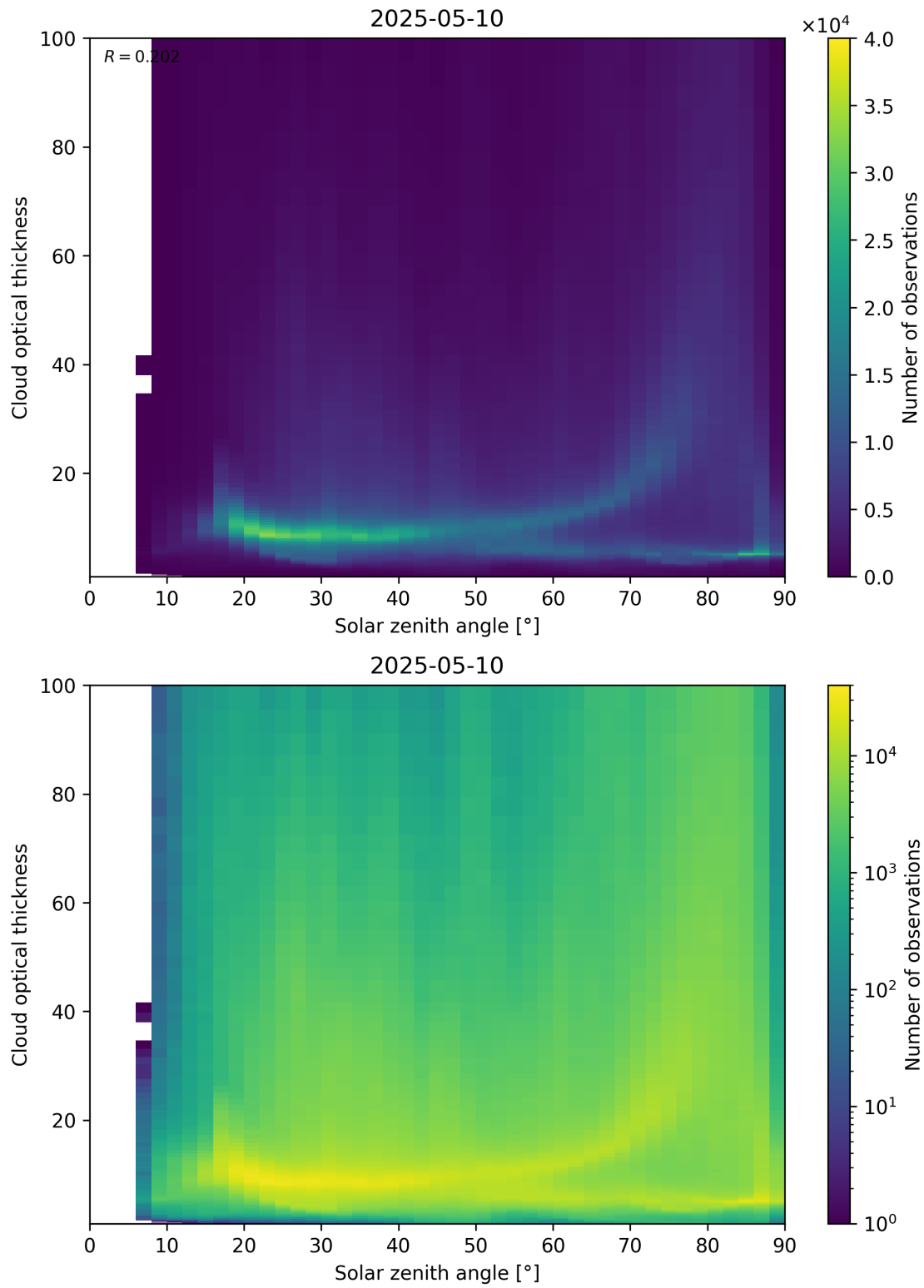
Figure 103: Scatter density plot of “Solar zenith angle” against “Cloud optical thickness” for 2025-05-10 to 2025-05-11.
