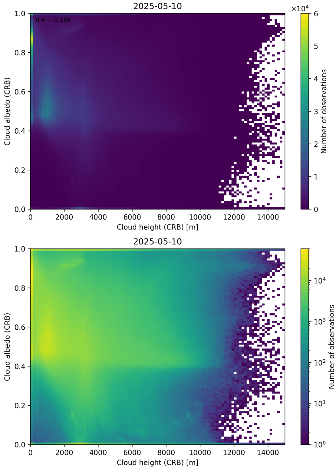
Figure 80: Scatter density plot of “Cloud height (CRB)” against “Cloud albedo (CRB)” for 2025-05-10 to 2025-05-11.
