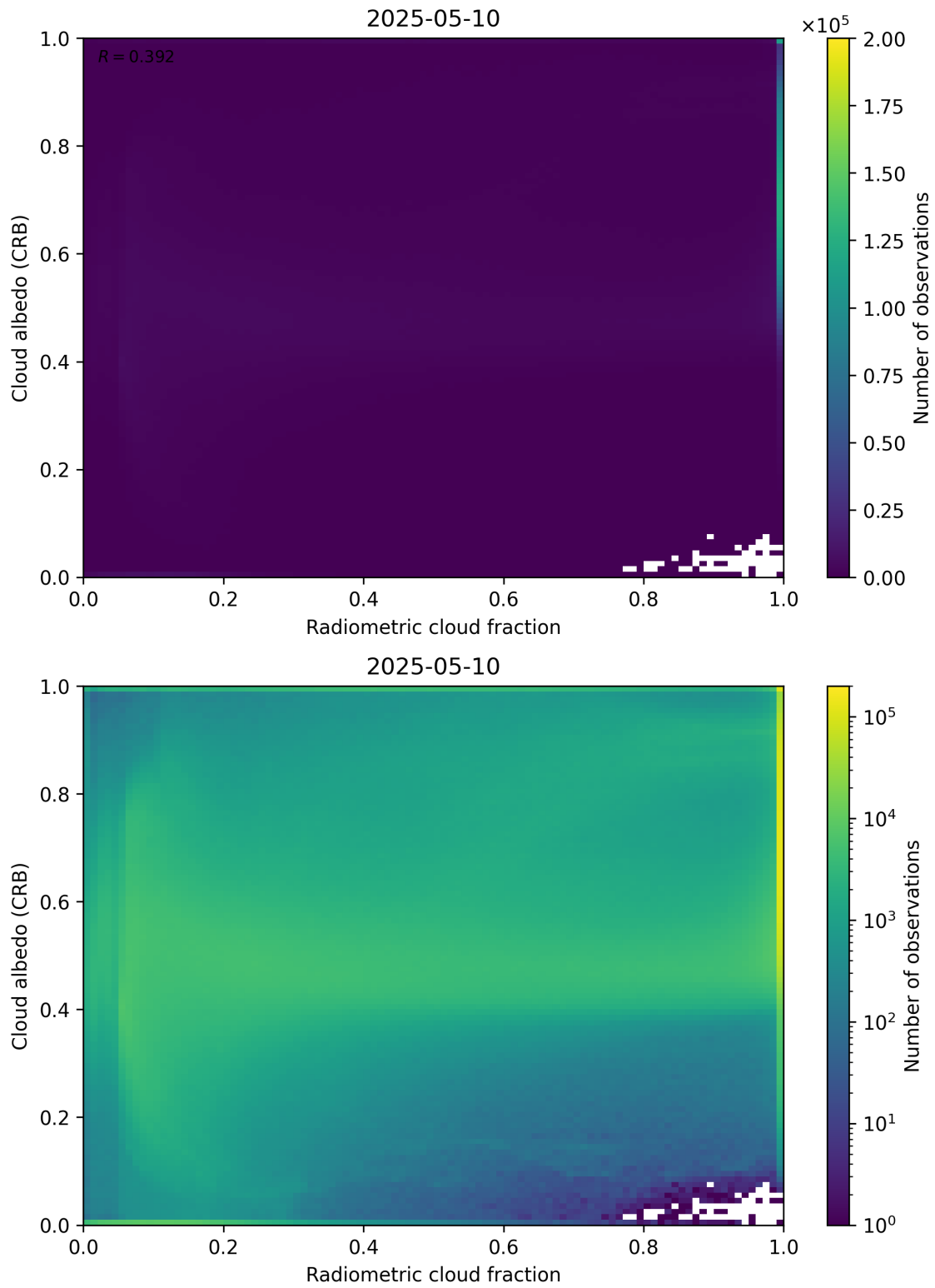
Figure 71: Scatter density plot of “Radiometric cloud fraction” against “Cloud albedo (CRB)” for 2025-05-10 to 2025-05-11.
