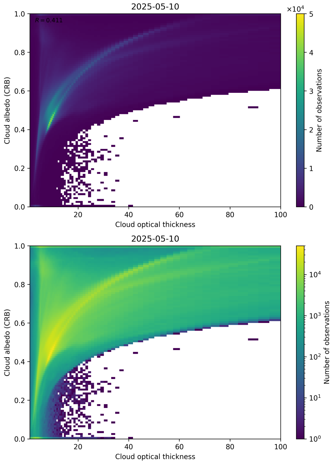
Figure 82: Scatter density plot of “Cloud optical thickness” against “Cloud albedo (CRB)” for 2025-05-10 to 2025-05-11.
