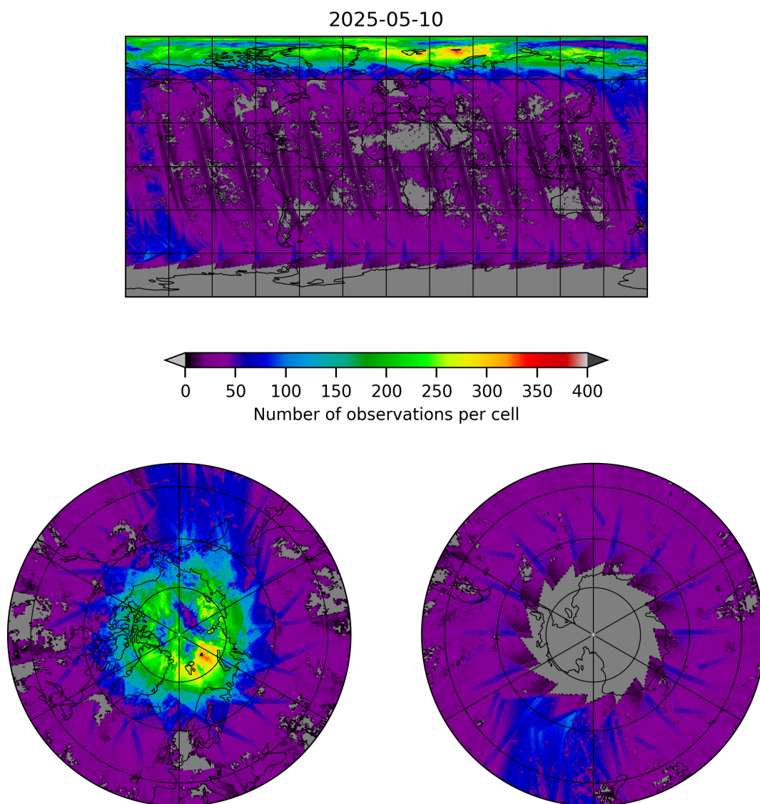
Figure 21: Map of the number of observations for 2025-05-10 to 2025-05-11
