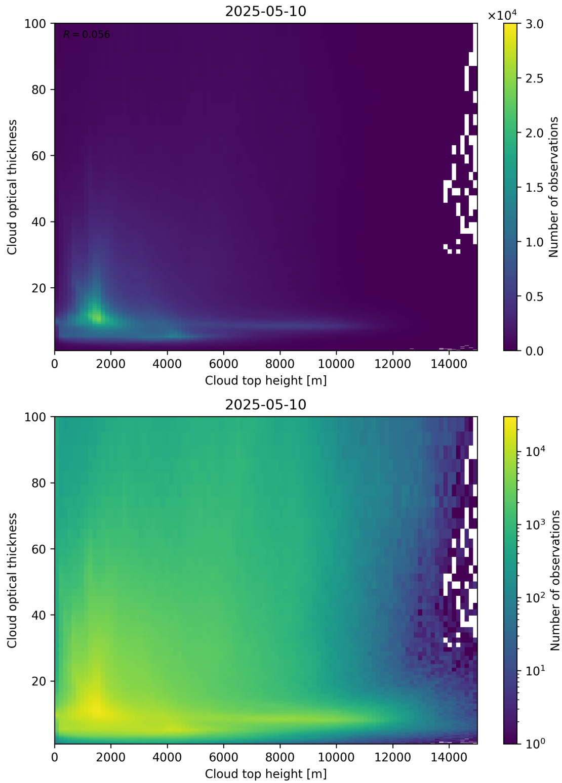
Figure 90: Scatter density plot of “Cloud top height” against “Cloud optical thickness” for 2025-05-10 to 2025-05-11.
