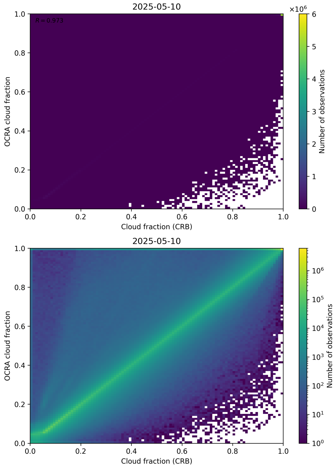
Figure 78: Scatter density plot of “Cloud fraction (CRB)” against “OCRA cloud fraction” for 2025-05-10 to 2025-05-11.
