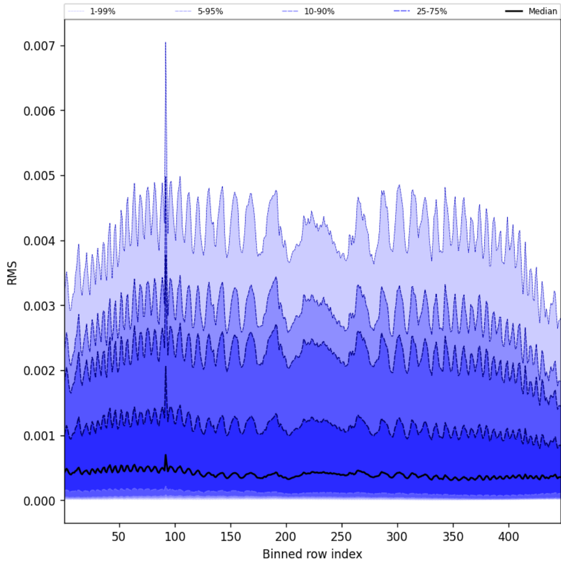
Figure 63: Along track statistics of “RMS” for 2025-05-10 to 2025-05-11
