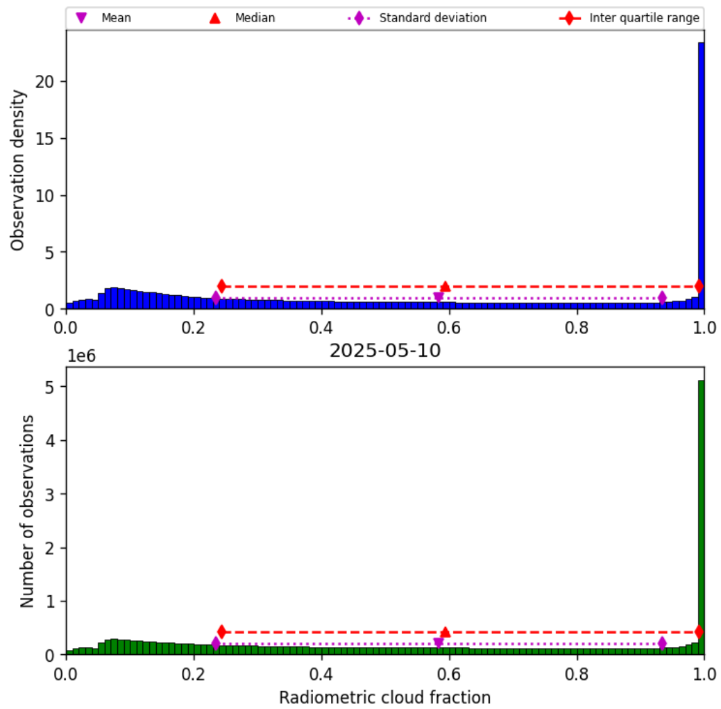
Figure 39: Histogram of “Radiometric cloud fraction” for 2025-05-10 to 2025-05-11
