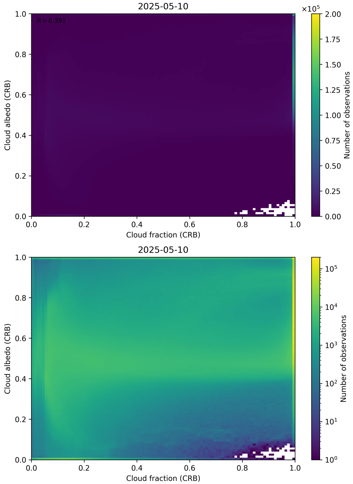
Figure 77: Scatter density plot of “Cloud fraction (CRB)” against “Cloud albedo (CRB)” for 2025-05-10 to 2025-05-11.
