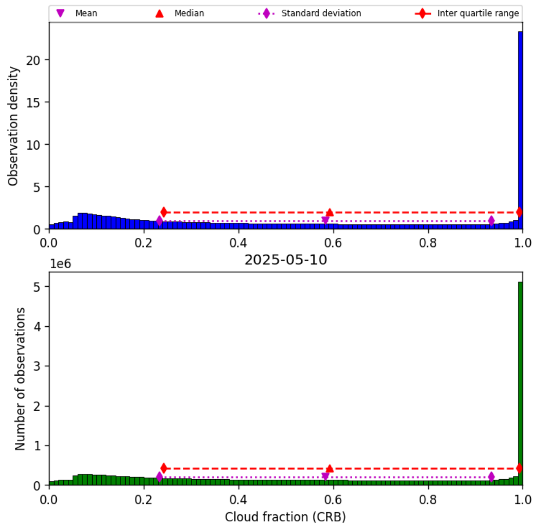
Figure 42: Histogram of “Cloud fraction (CRB)” for 2025-05-10 to 2025-05-11
