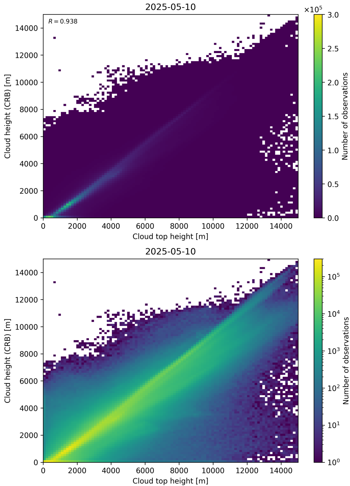
Figure 89: Scatter density plot of “Cloud top height” against “Cloud height (CRB)” for 2025-05-10 to 2025-05-11.
