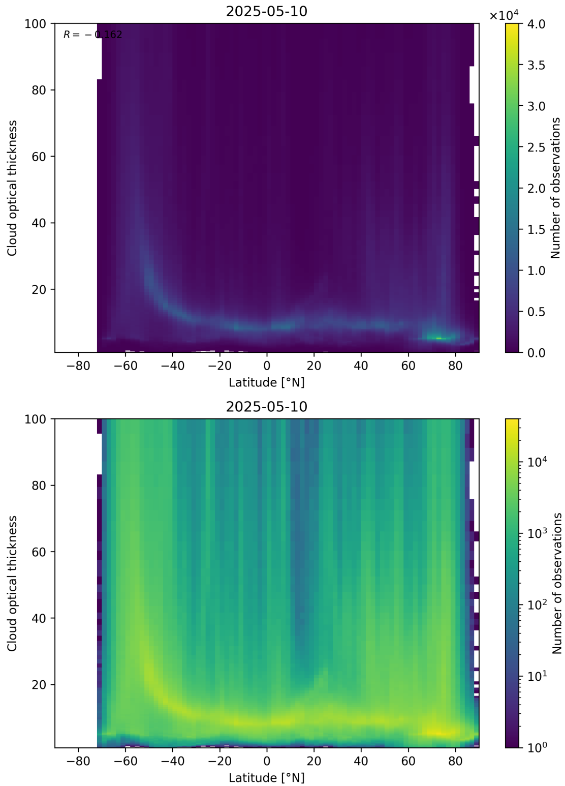
Figure 96: Scatter density plot of “Latitude” against “Cloud optical thickness” for 2025-05-10 to 2025-05-11.
