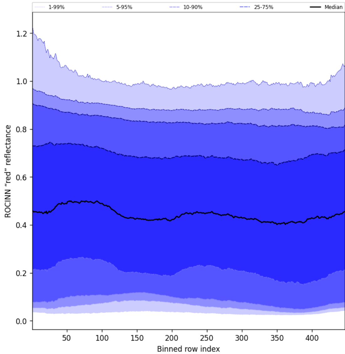
Figure 69: Along track statistics of "ROCINN "red" reflectance" for 2025-05-10 to 2025-05-11
