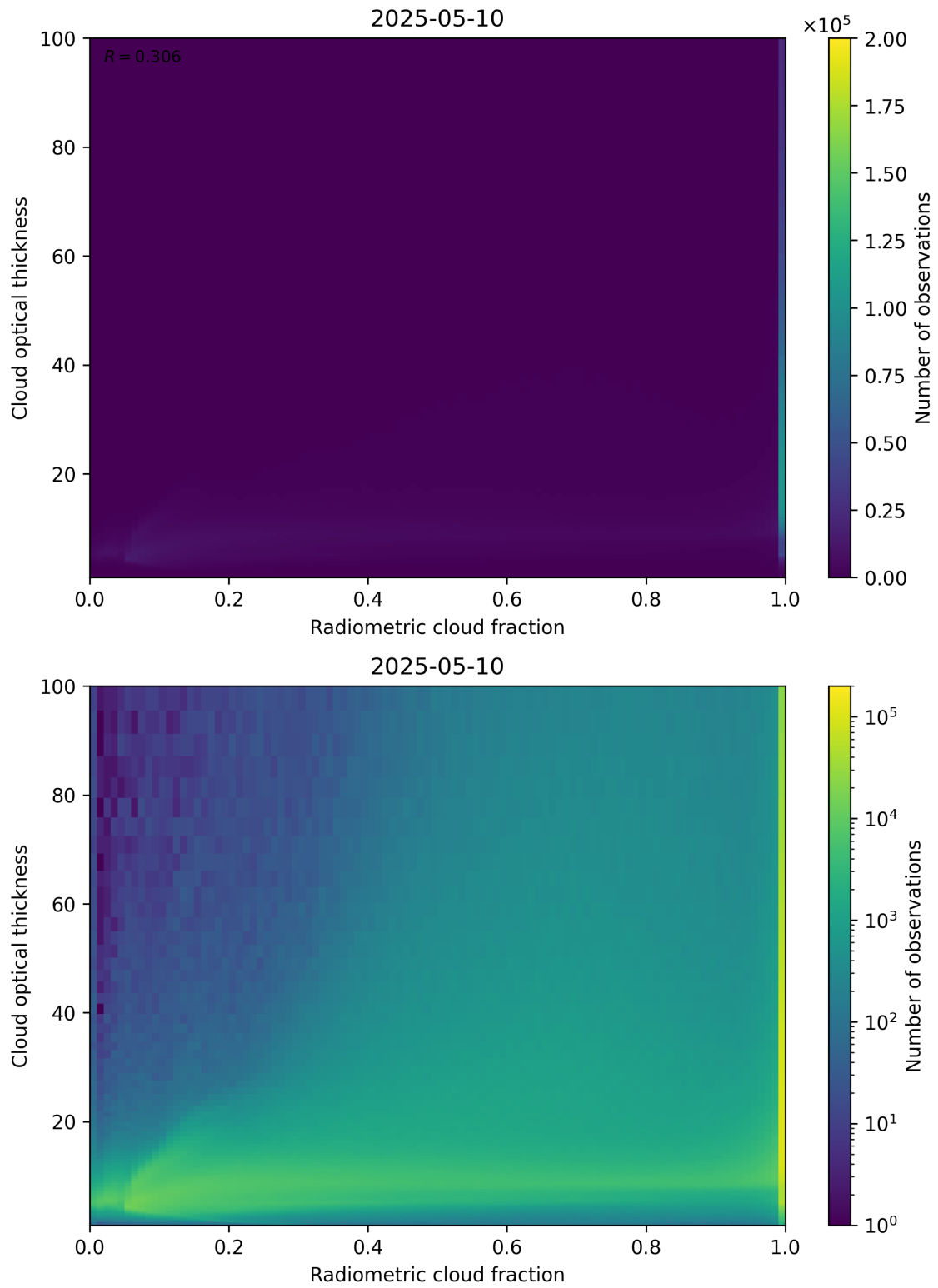
Figure 75: Scatter density plot of “Radiometric cloud fraction” against “Cloud optical thickness” for 2025-05-10 to 2025-05-11.
