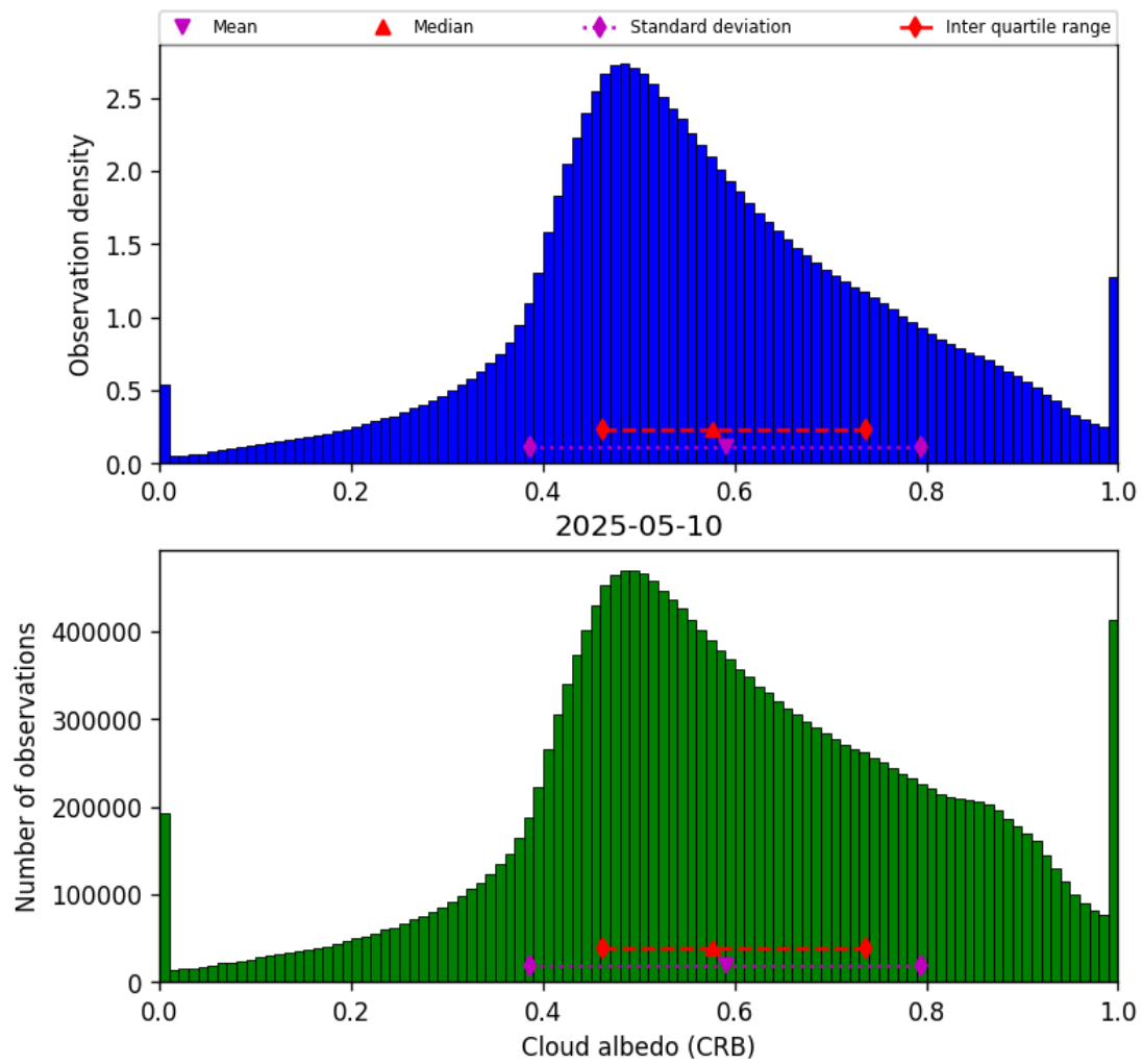
Figure 44: Histogram of “Cloud albedo (CRB)” for 2025-05-10 to 2025-05-11
