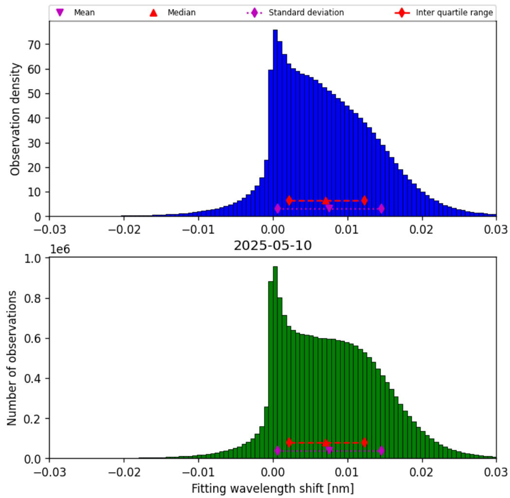
Figure 49: Histogram of “Fitting wavelength shift” for 2025-05-10 to 2025-05-11
