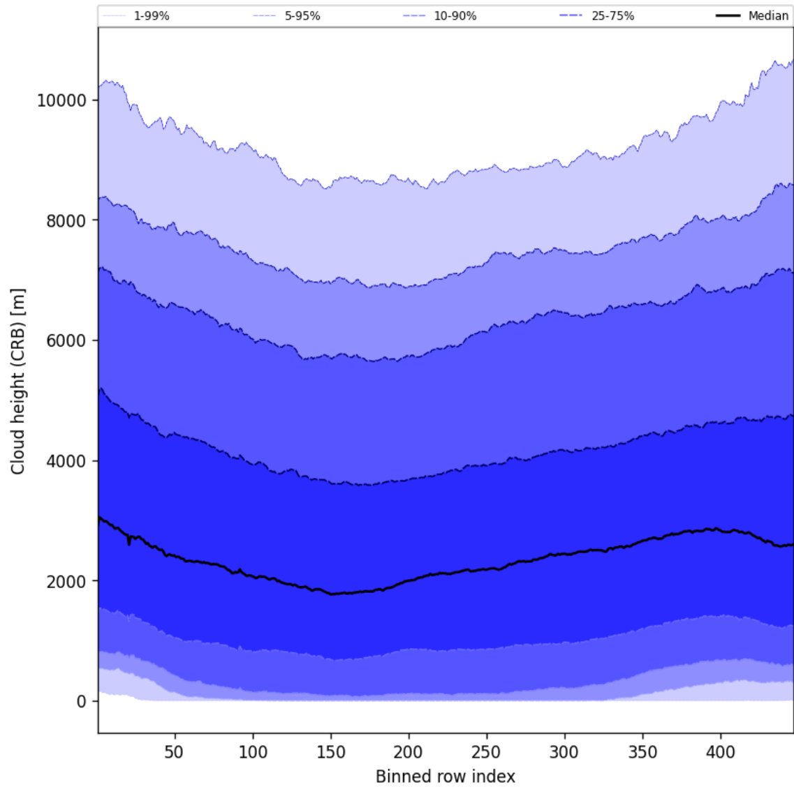
Figure 59: Along track statistics of “Cloud height (CRB)” for 2025-05-10 to 2025-05-11
