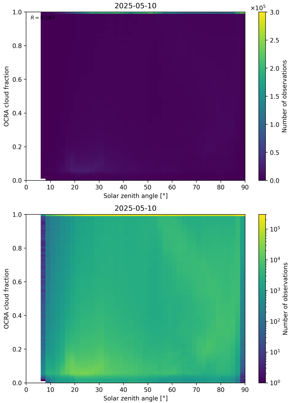
Figure 100: Scatter density plot of “Solar zenith angle” against “OCRA cloud fraction” for 2025-05-10 to 2025-05-11.
