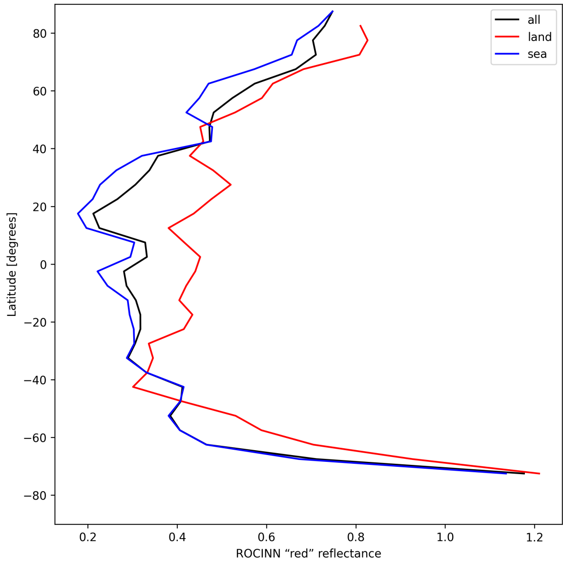
Figure 37: Zonal average of “ROCINN “red” reflectance” for 2025-05-10 to 2025-05-11.
