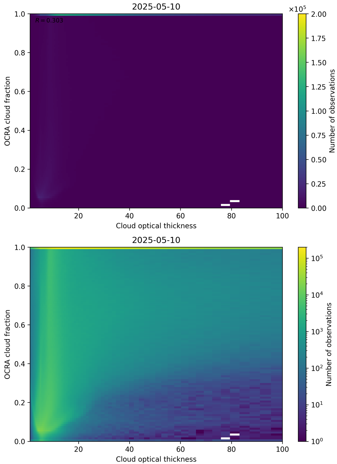
Figure 83: Scatter density plot of “Cloud optical thickness” against “OCRA cloud fraction” for 2025-05-10 to 2025-05-11.
