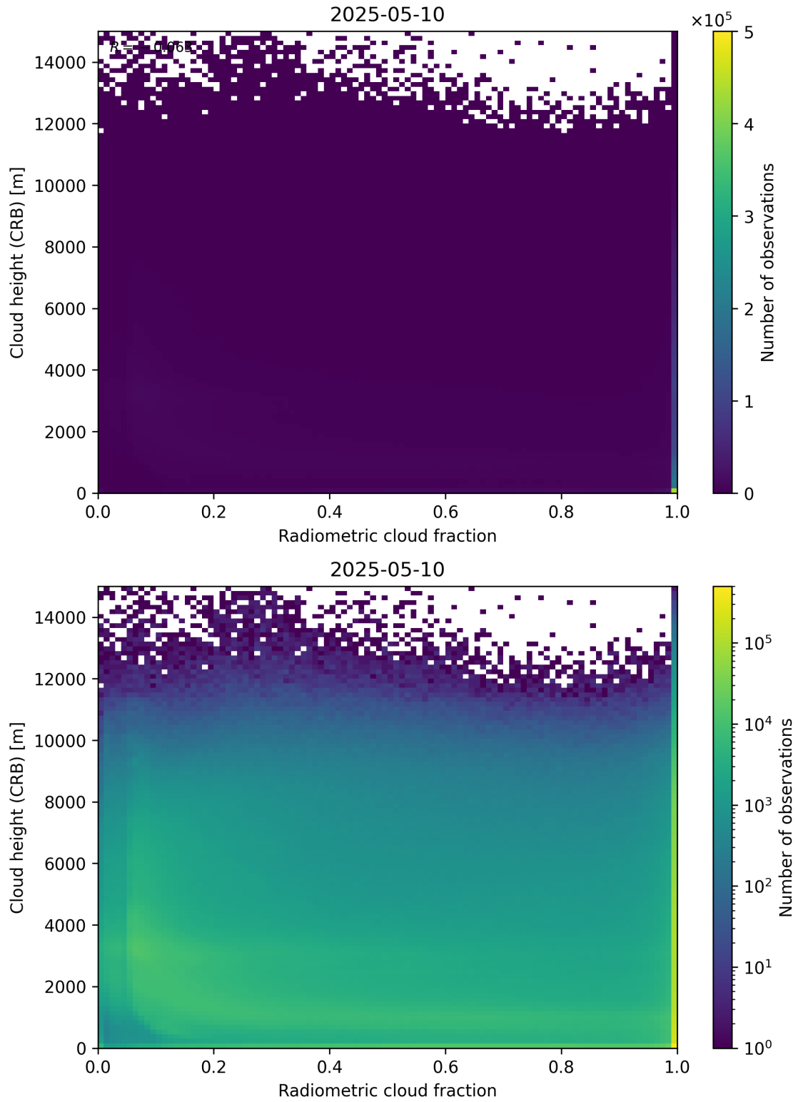
Figure 74: Scatter density plot of “Radiometric cloud fraction” against “Cloud height (CRB)” for 2025-05-10 to 2025-05-11.
