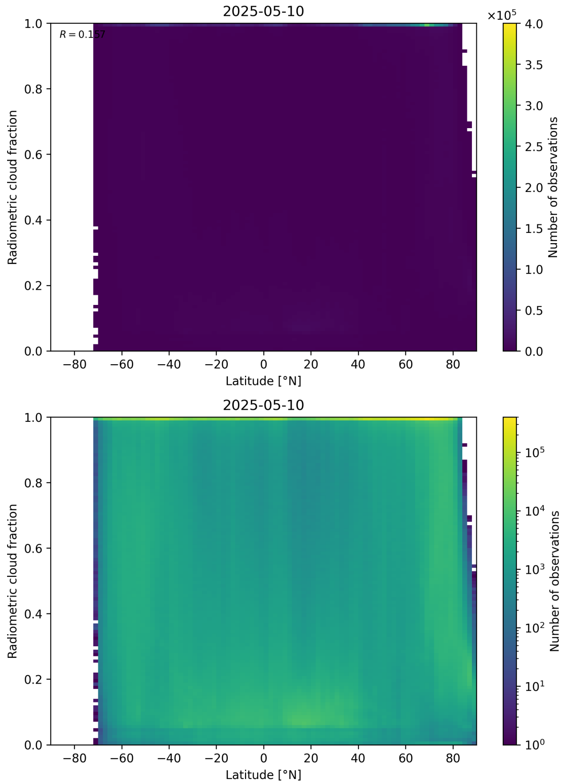
Figure 92: Scatter density plot of “Latitude” against “Radiometric cloud fraction” for 2025-05-10 to 2025-05-11.
