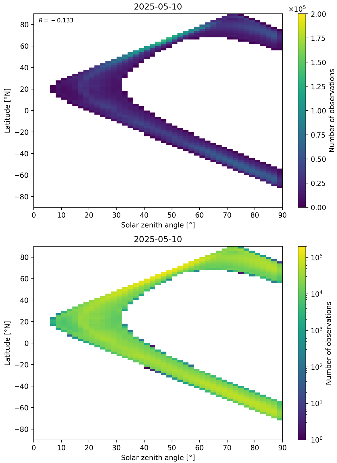
Figure 105: Scatter density plot of “Solar zenith angle” against “Latitude” for 2025-05-10 to 2025-05-11.
