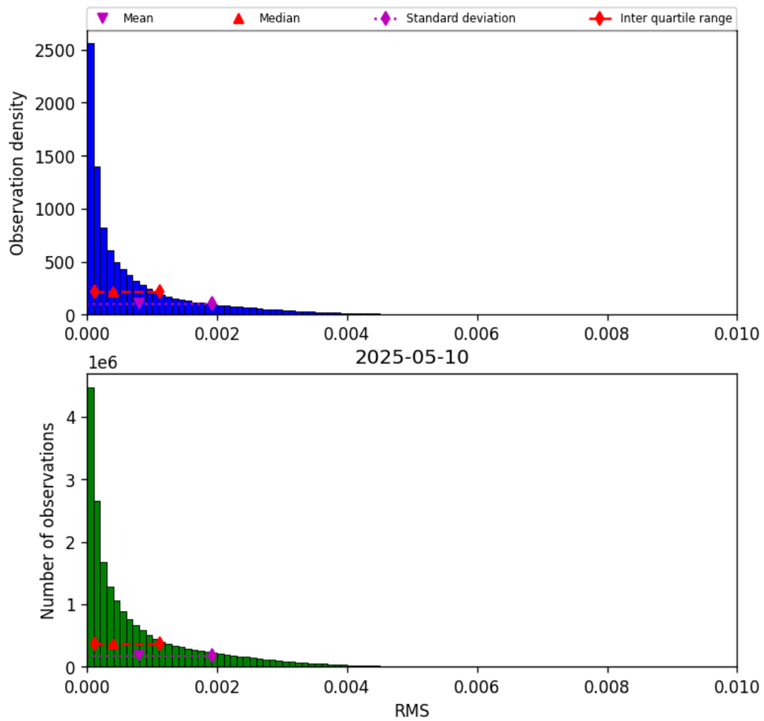
Figure 47: Histogram of “RMS” for 2025-05-10 to 2025-05-11
