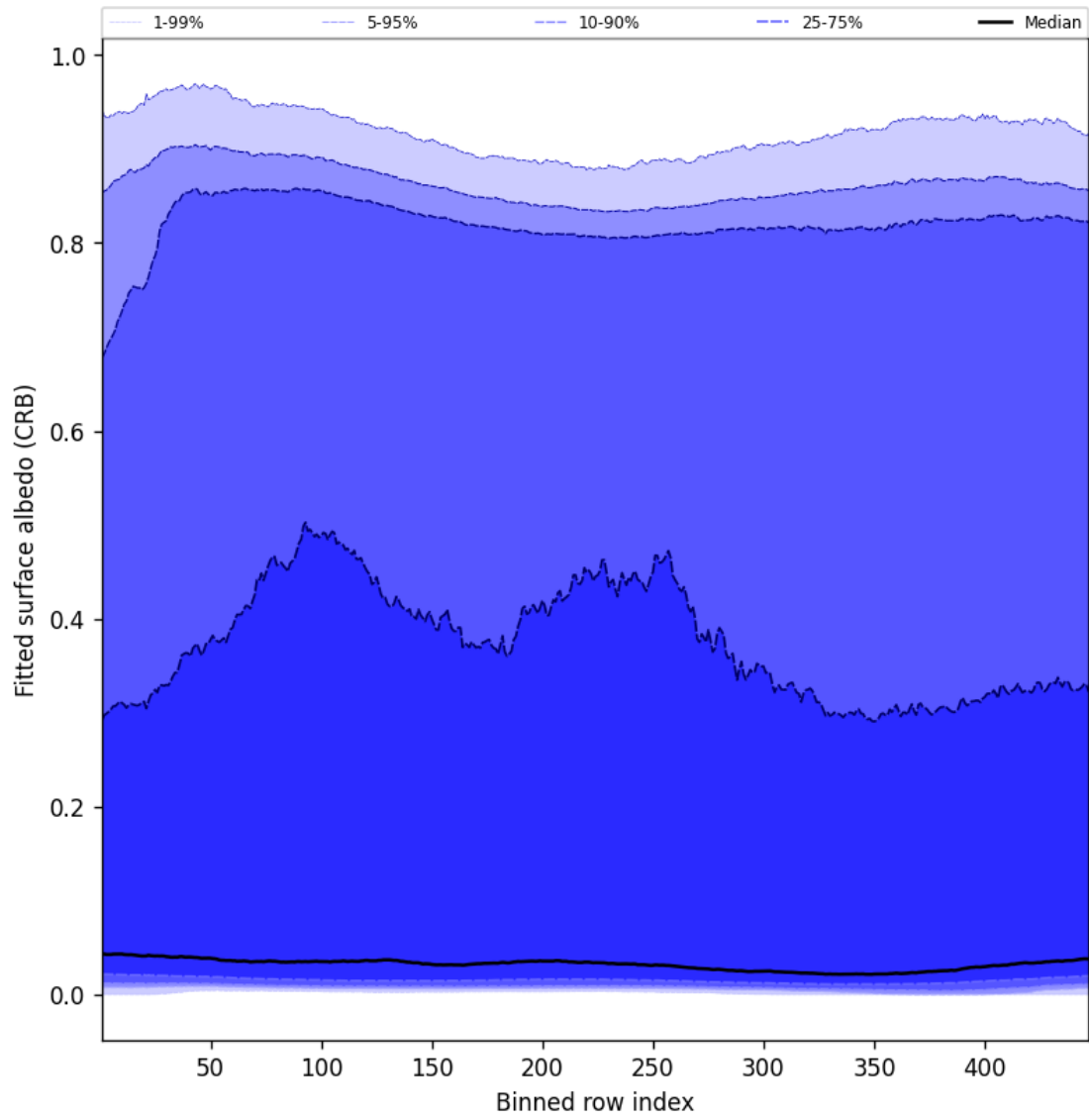
Figure 62: Along track statistics of “Fitted surface albedo (CRB)” for 2025-05-10 to 2025-05-11
