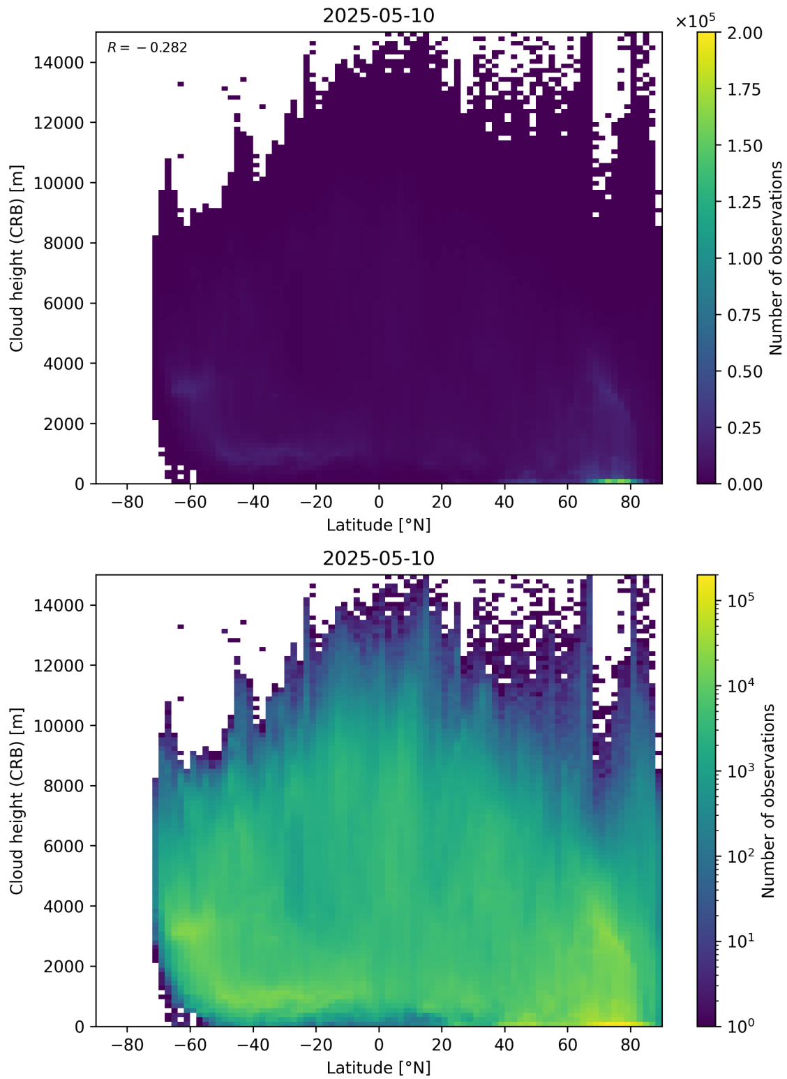
Figure 95: Scatter density plot of “Latitude” against “Cloud height (CRB)” for 2025-05-10 to 2025-05-11.
