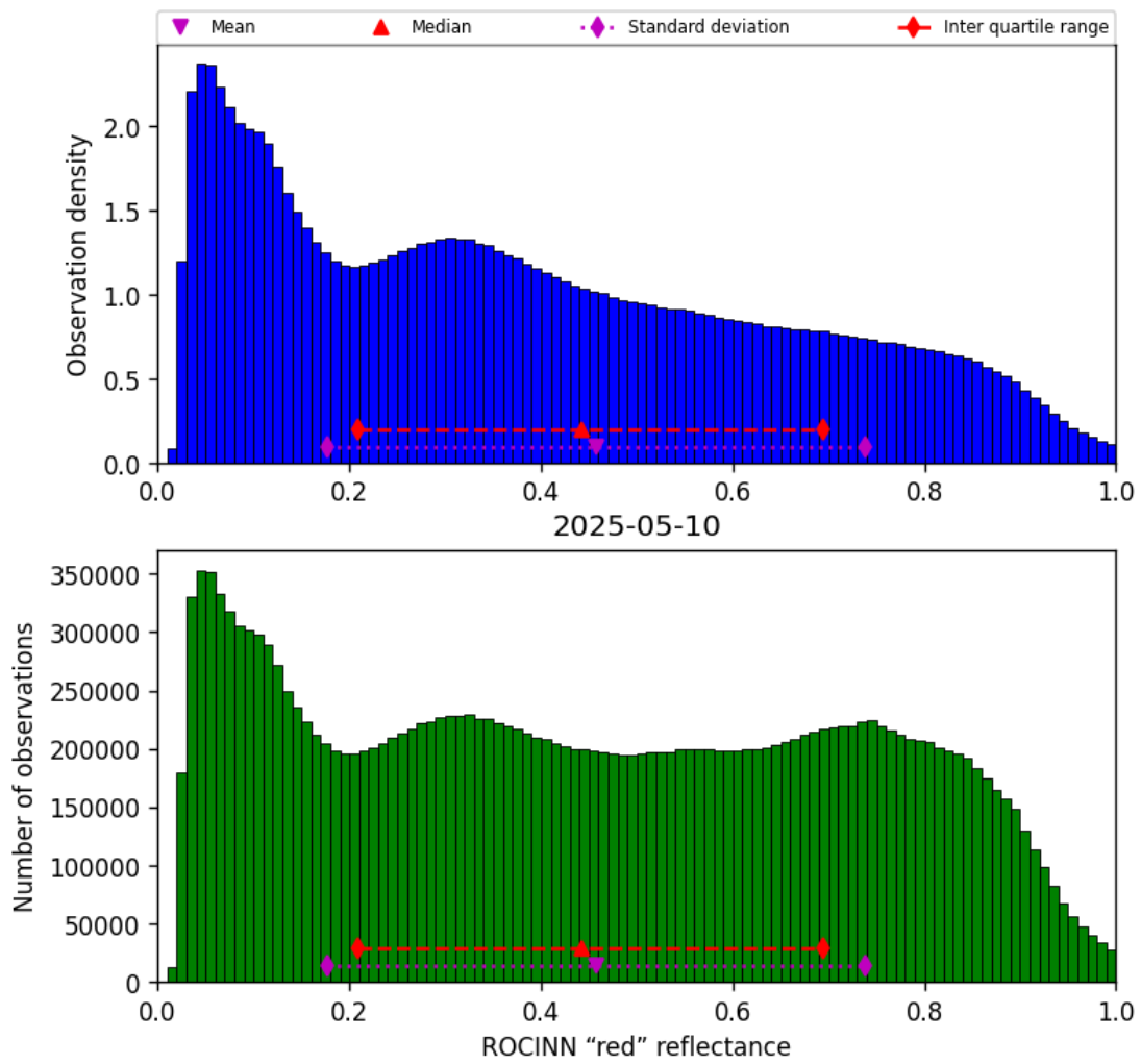
Figure 53: Histogram of “ROCINN “red” reflectance” for 2025-05-10 to 2025-05-11
