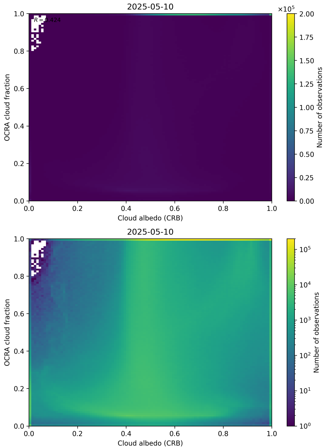
Figure 70: Scatter density plot of “Cloud albedo (CRB)” against “OCRA cloud fraction” for 2025-05-10 to 2025-05-11.
