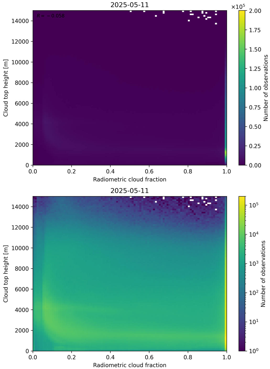
Figure 76: Scatter density plot of “Radiometric cloud fraction” against “Cloud top height” for 2025-05-10 to 2025-05-12.
