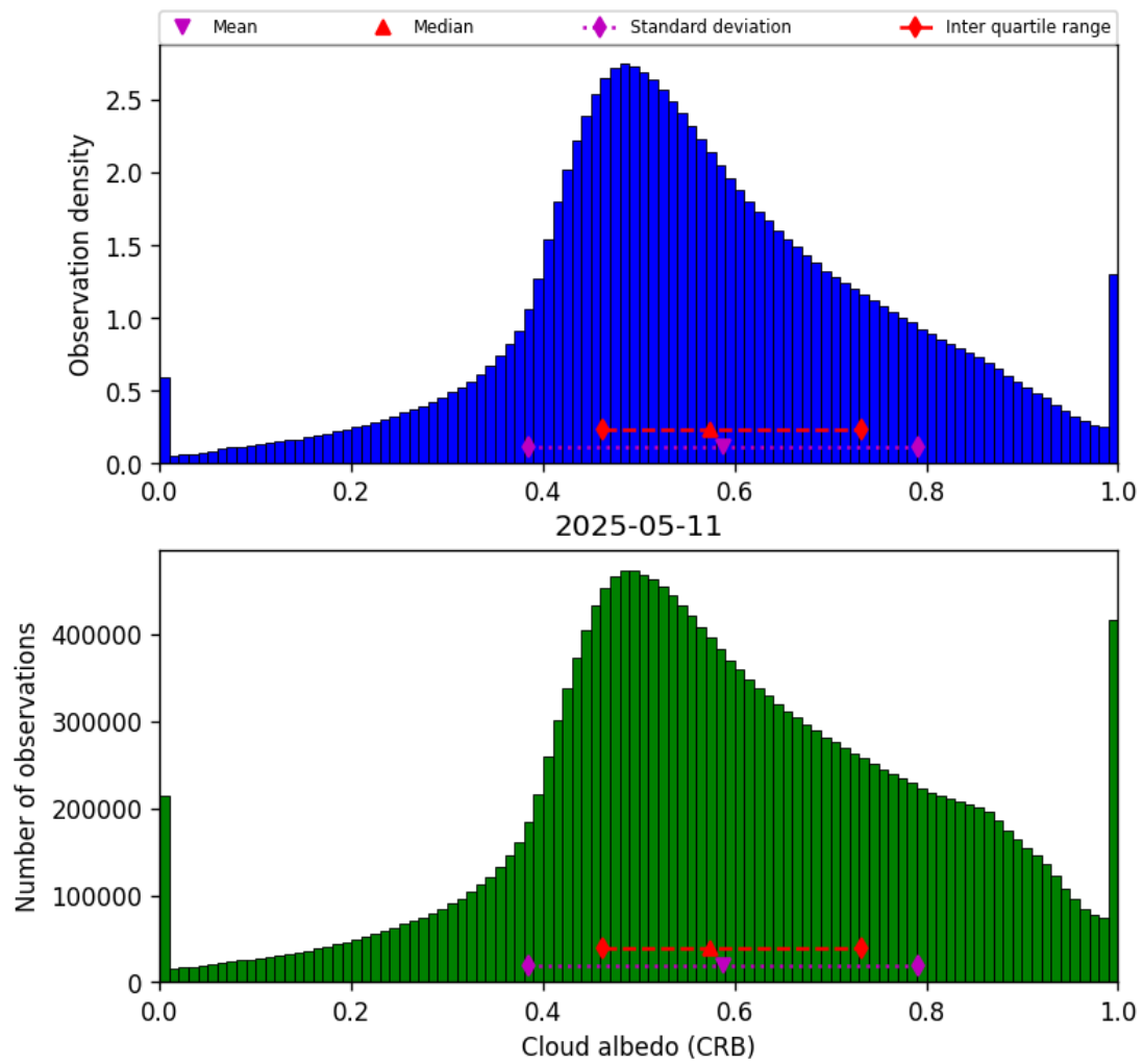
Figure 44: Histogram of “Cloud albedo (CRB)” for 2025-05-10 to 2025-05-12
