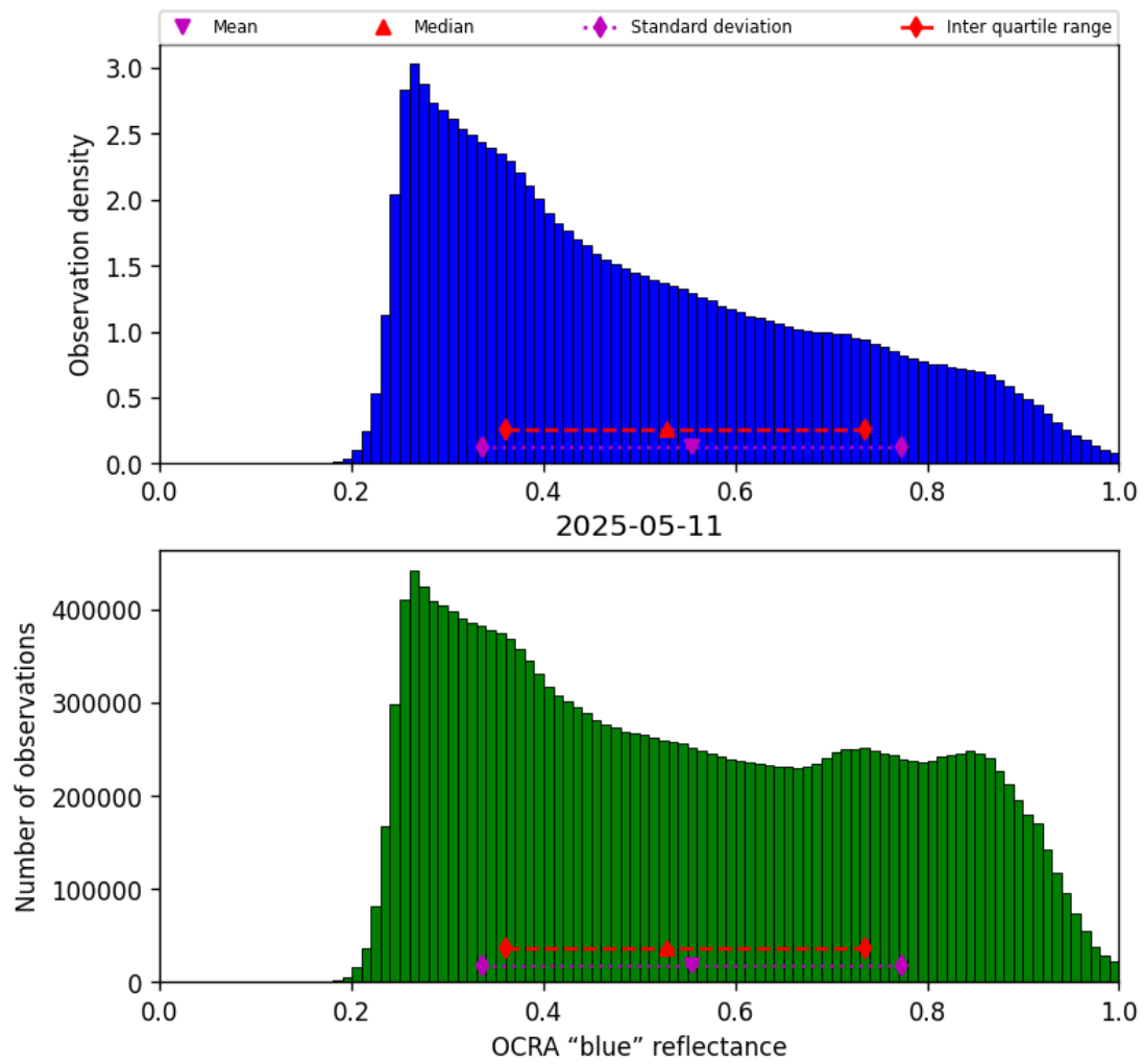
Figure 51: Histogram of “OCRA “blue” reflectance” for 2025-05-10 to 2025-05-12
