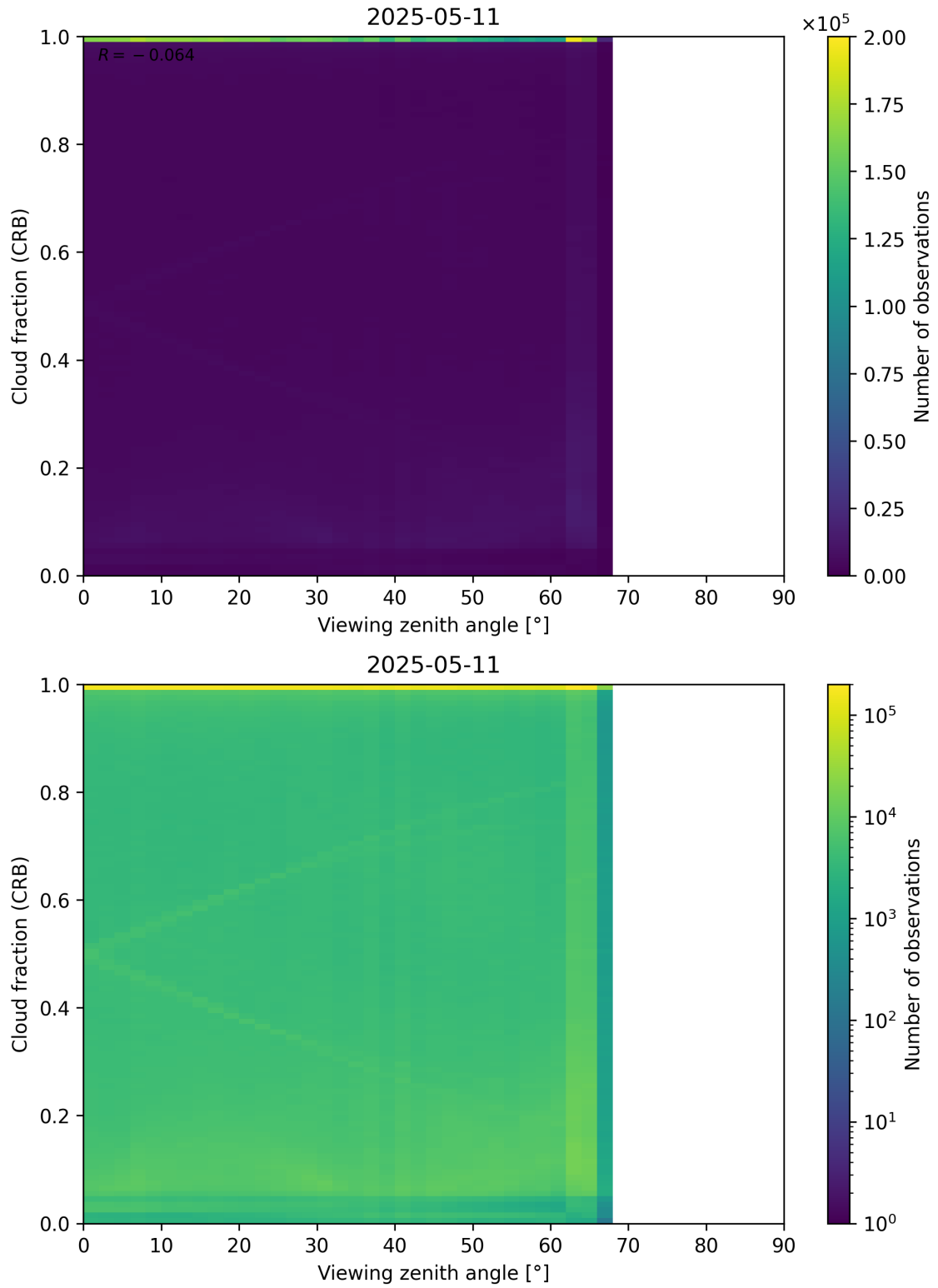
Figure 109: Scatter density plot of “Viewing zenith angle” against “Cloud fraction (CRB)” for 2025-05-10 to 2025-05-12.
