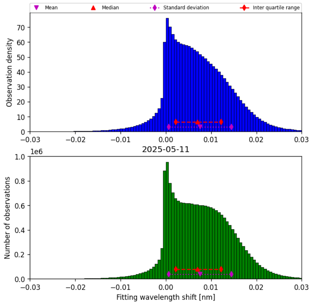
Figure 49: Histogram of “Fitting wavelength shift” for 2025-05-10 to 2025-05-12
