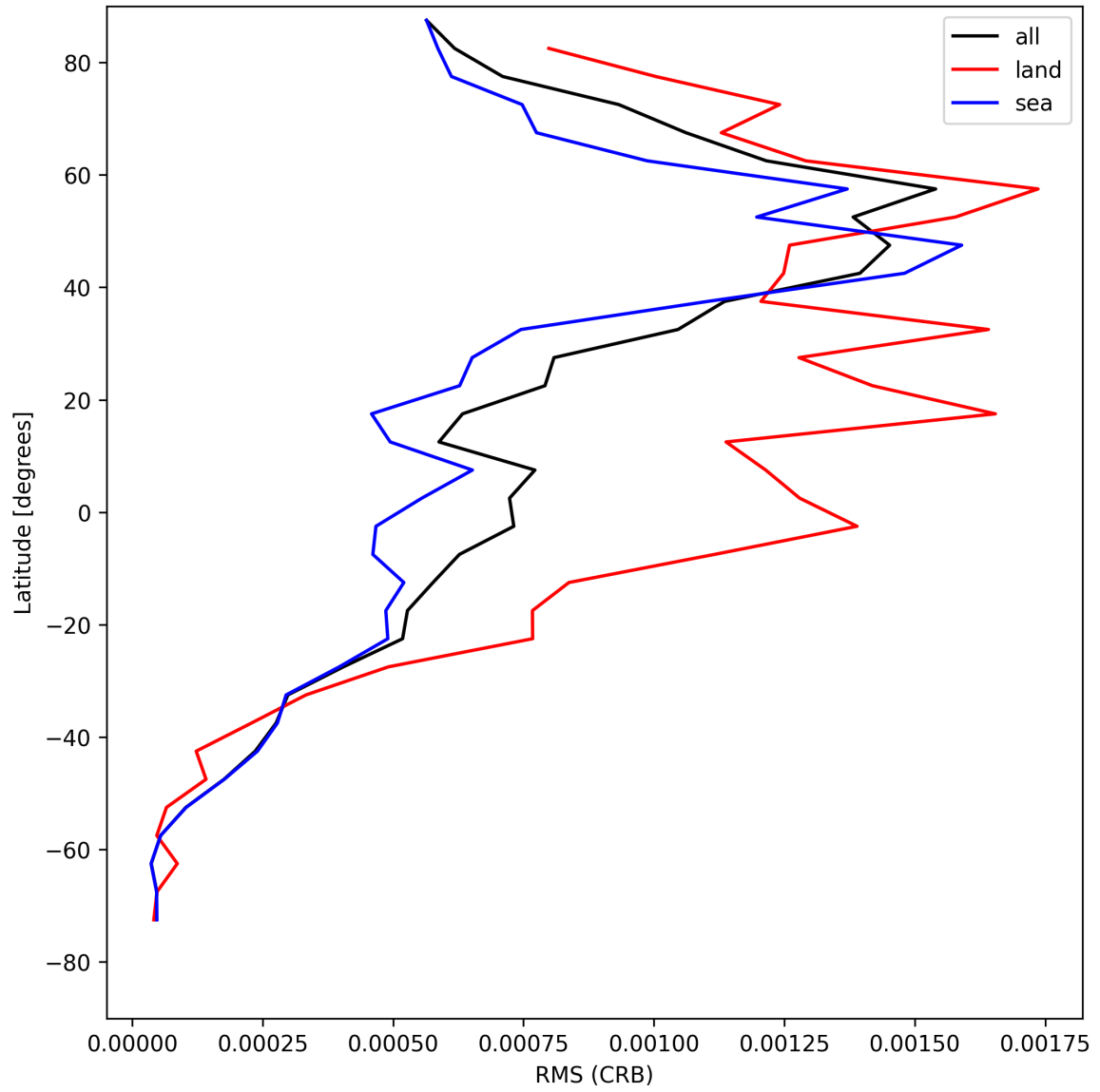
Figure 32: Zonal average of “RMS (CRB)” for 2025-05-10 to 2025-05-12.
