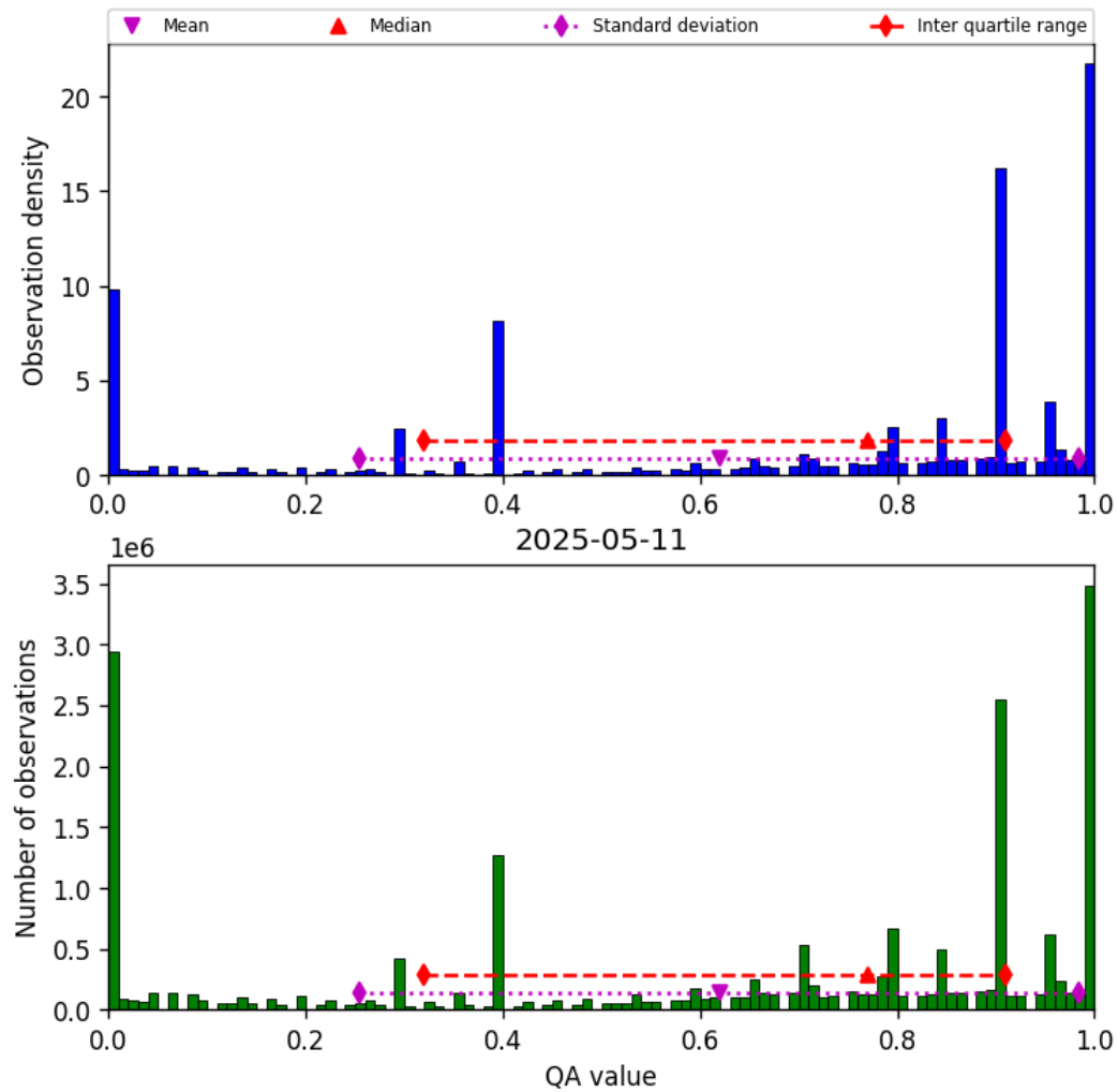
Figure 38: Histogram of “QA value” for 2025-05-10 to 2025-05-12
