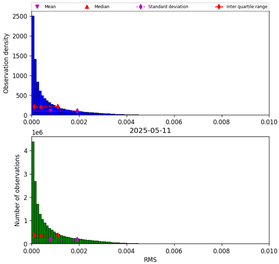
Figure 47: Histogram of “RMS” for 2025-05-10 to 2025-05-12
