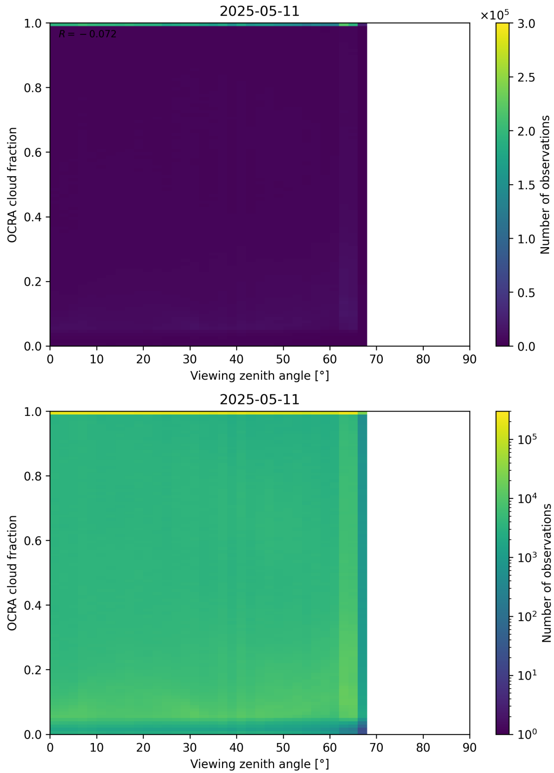
Figure 108: Scatter density plot of “Viewing zenith angle” against “OCRA cloud fraction” for 2025-05-10 to 2025-05-12.
