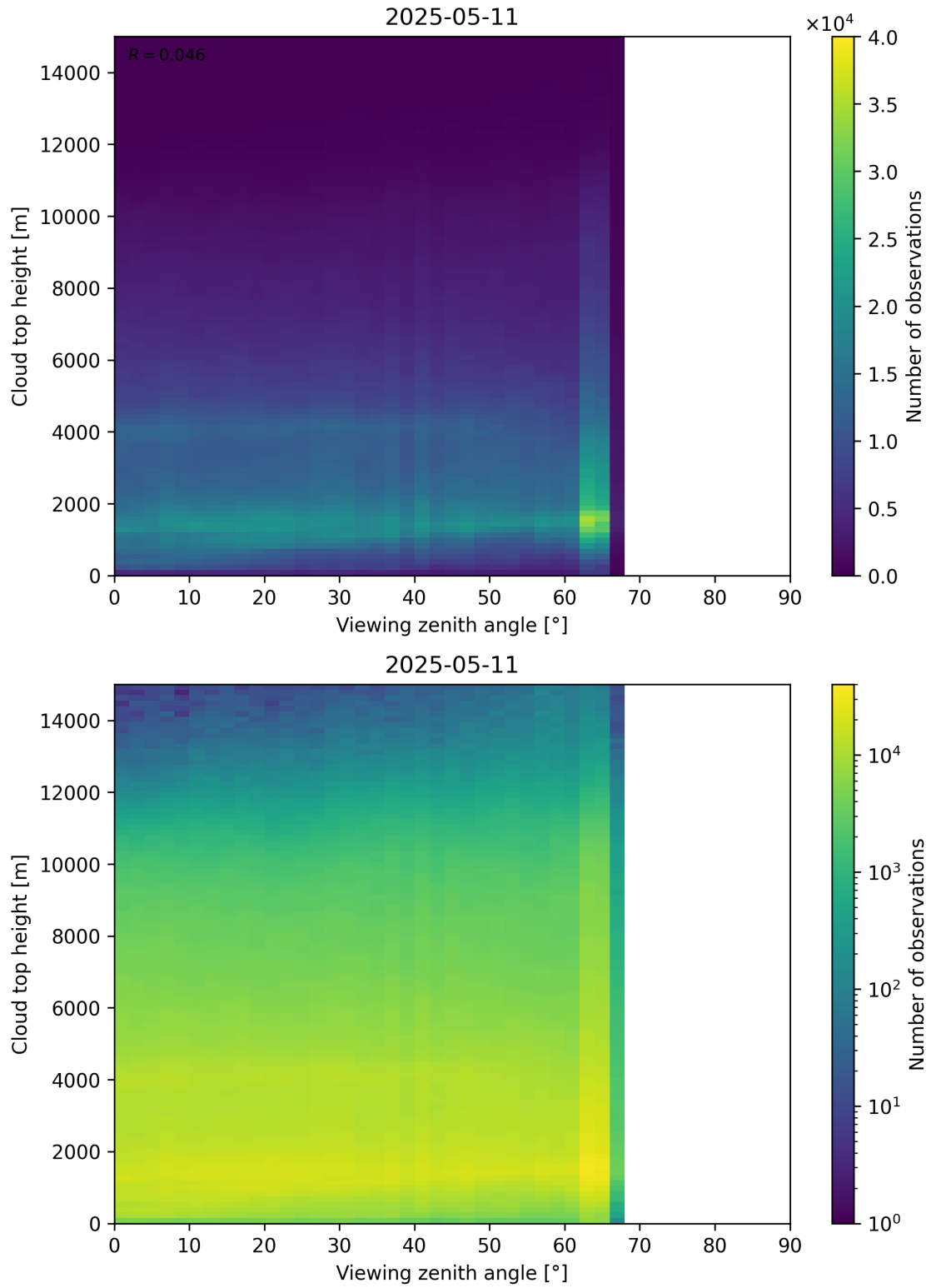
Figure 112: Scatter density plot of “Viewing zenith angle” against “Cloud top height” for 2025-05-10 to 2025-05-12.
