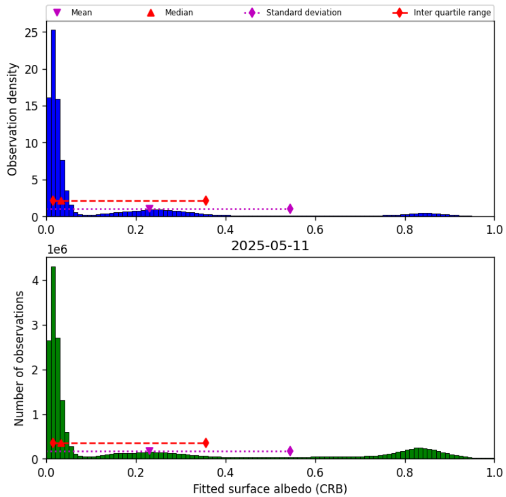
Figure 46: Histogram of “Fitted surface albedo (CRB)” for 2025-05-10 to 2025-05-12
