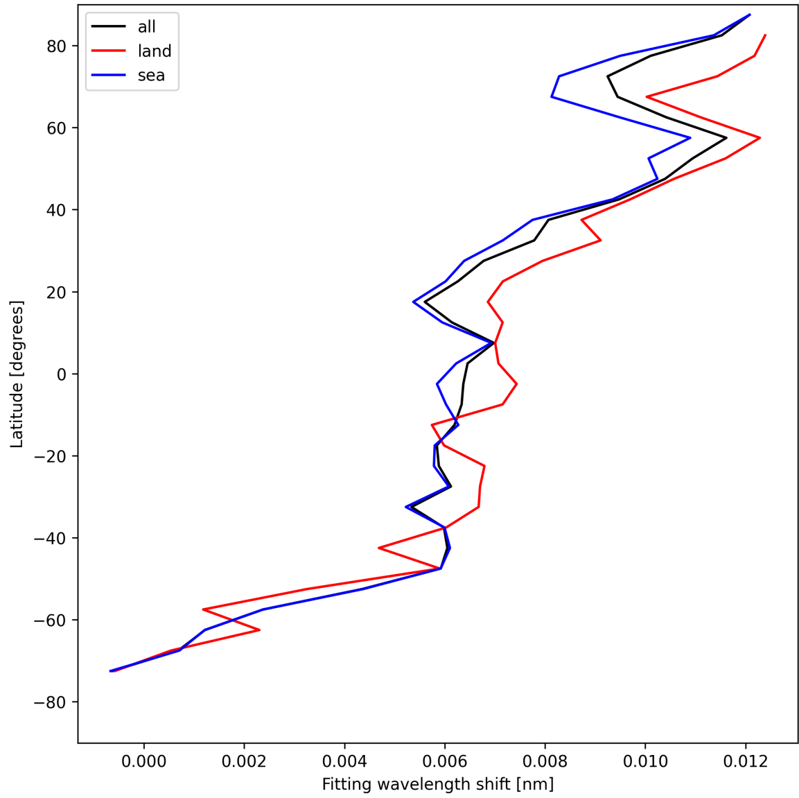
Figure 33: Zonal average of “Fitting wavelength shift” for 2025-05-10 to 2025-05-12.
