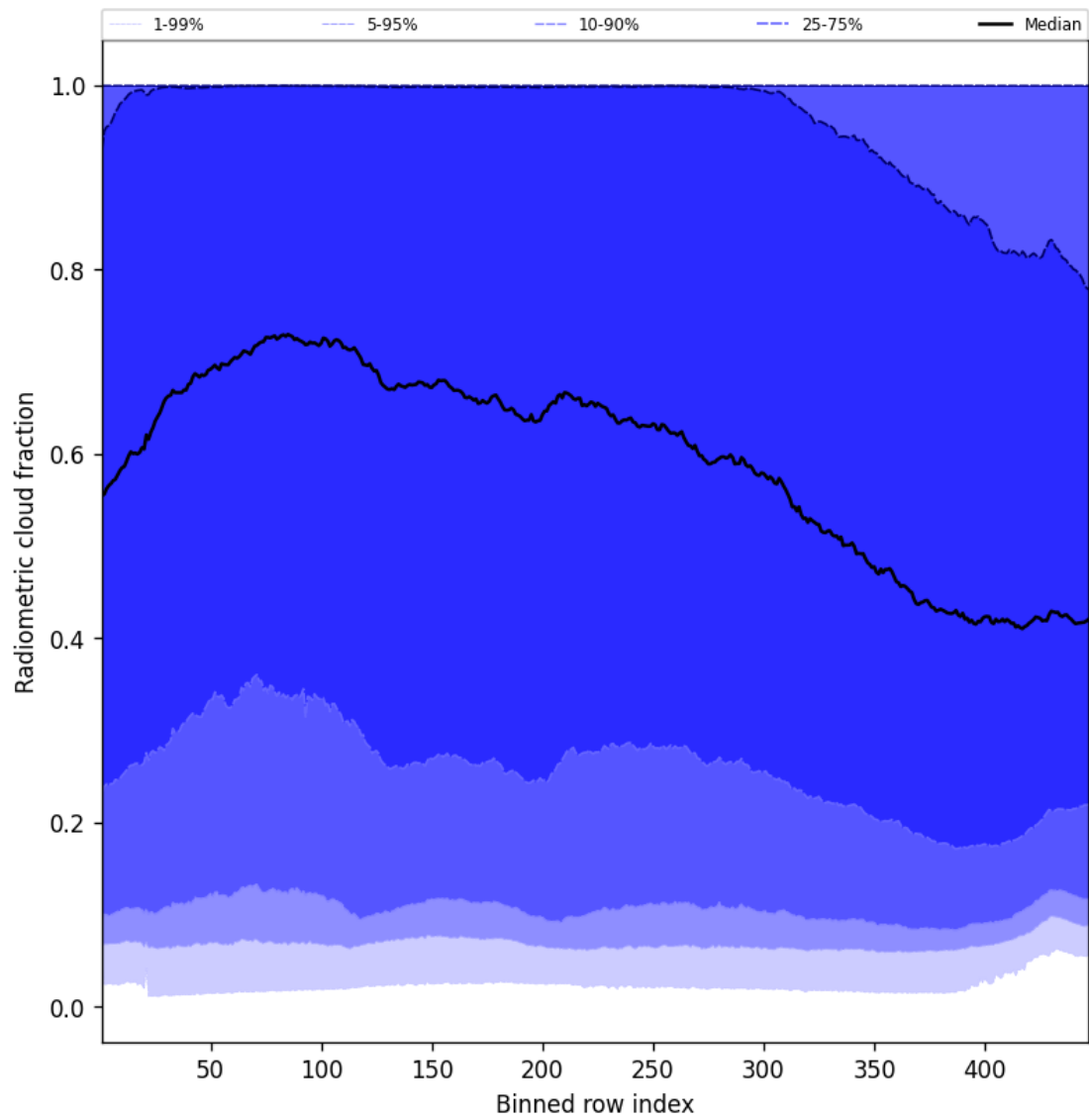
Figure 55: Along track statistics of "Radiometric cloud fraction" for 2025-05-10 to 2025-05-12
