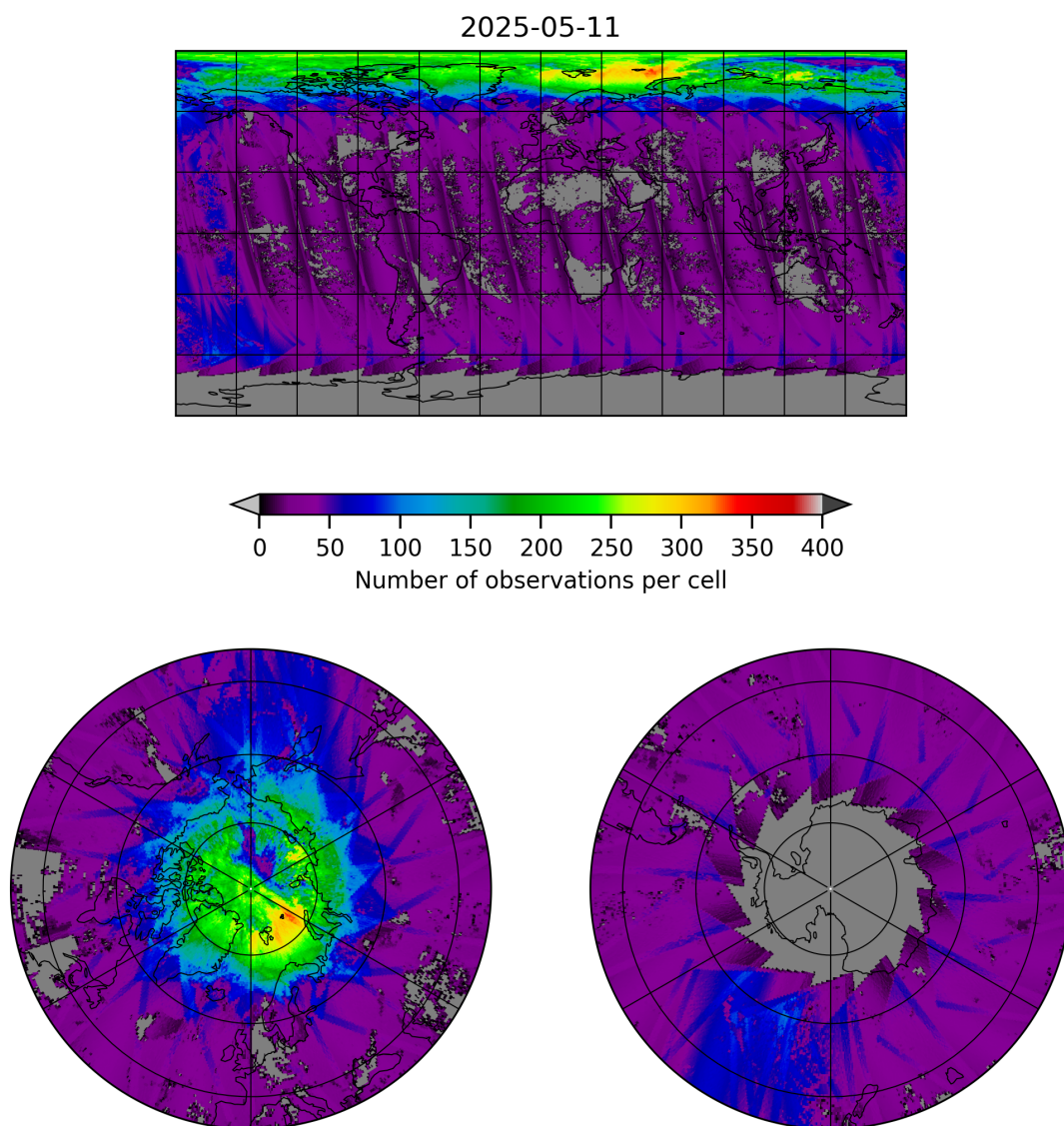
Figure 21: Map of the number of observations for 2025-05-10 to 2025-05-12
