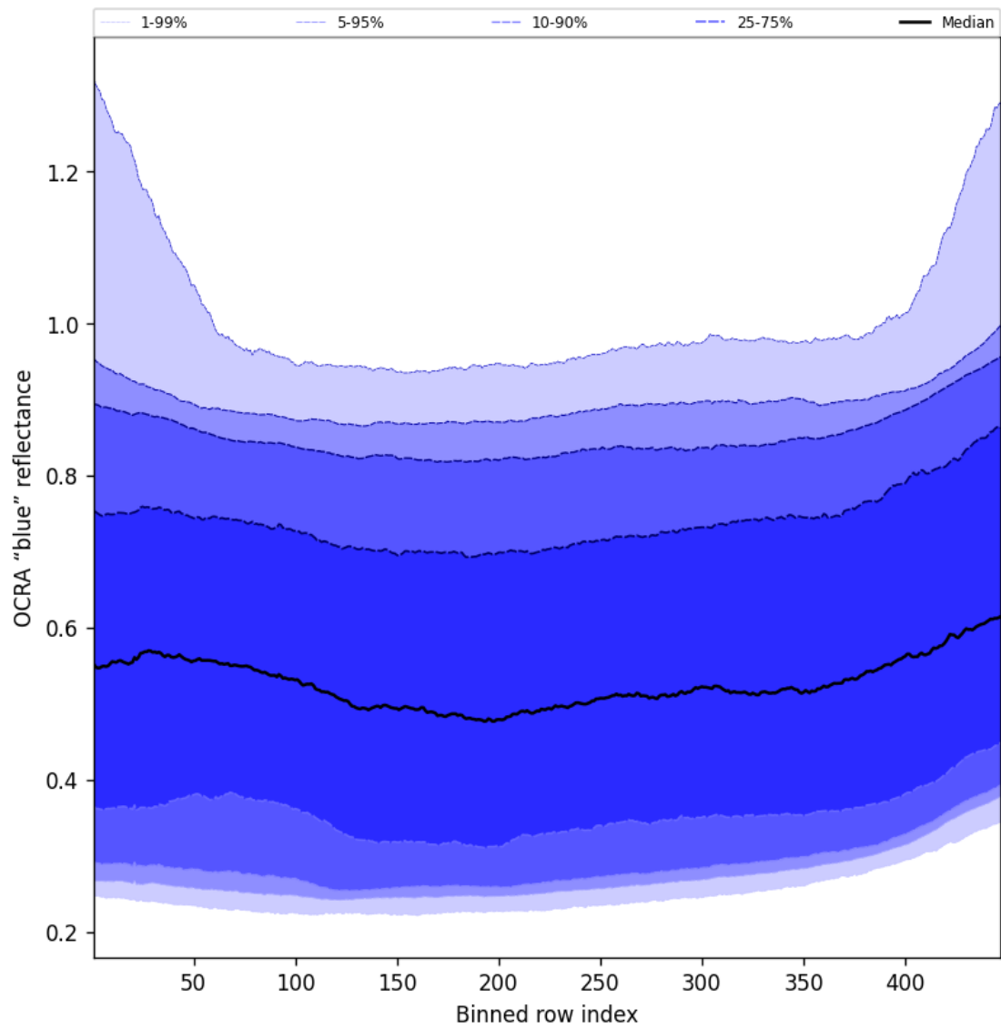
Figure 67: Along track statistics of “OCRA “blue” reflectance” for 2025-05-10 to 2025-05-12
