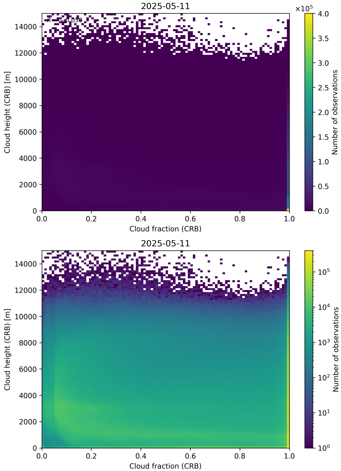
Figure 79: Scatter density plot of “Cloud fraction (CRB)” against “Cloud height (CRB)” for 2025-05-10 to 2025-05-12.
