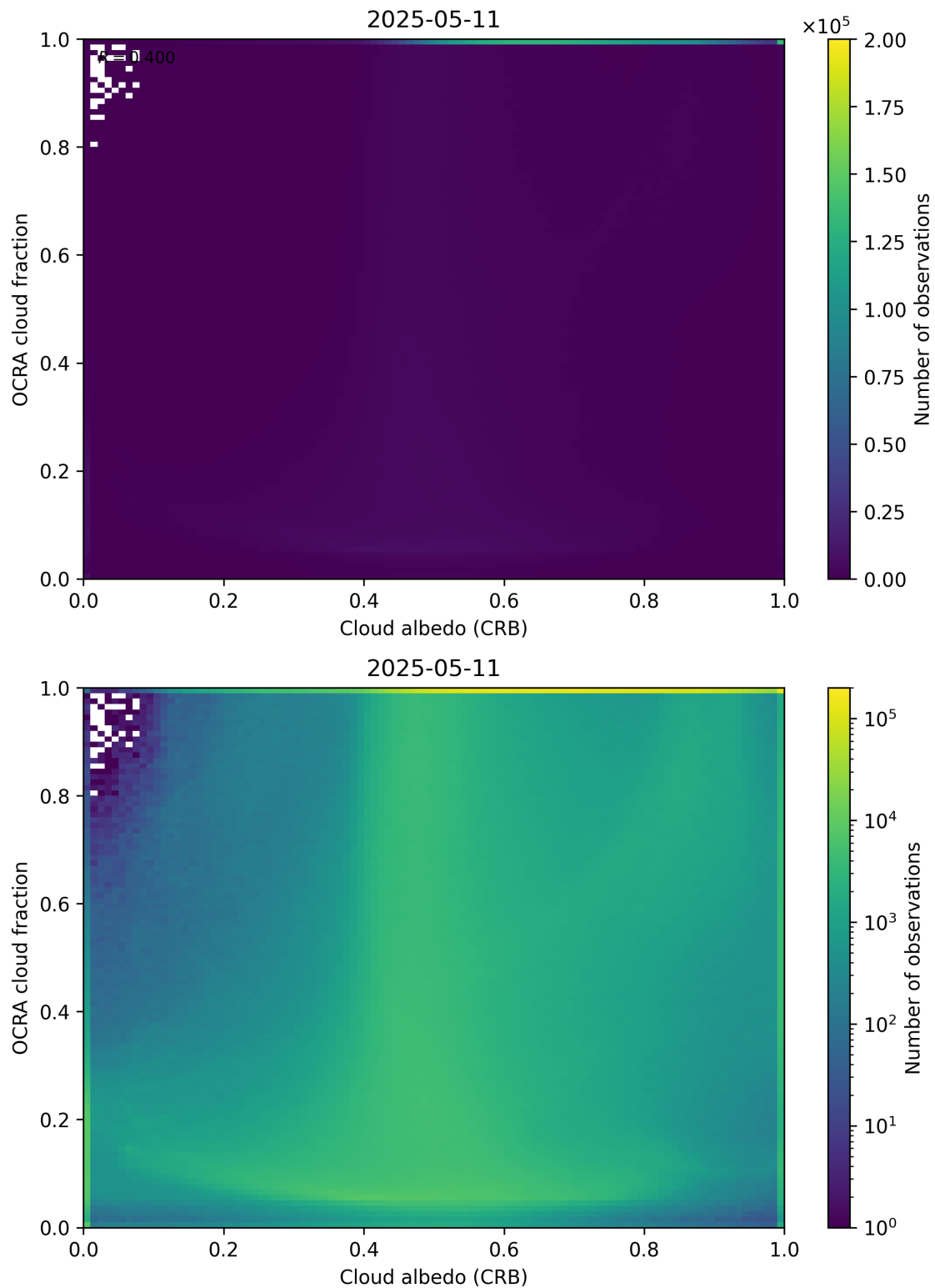
Figure 70: Scatter density plot of “Cloud albedo (CRB)” against “OCRA cloud fraction” for 2025-05-10 to 2025-05-12.
