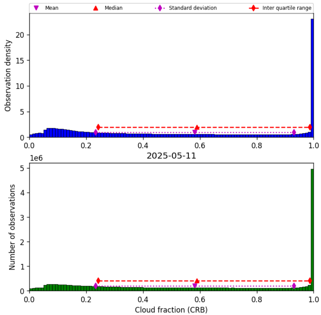
Figure 42: Histogram of “Cloud fraction (CRB)” for 2025-05-10 to 2025-05-12
