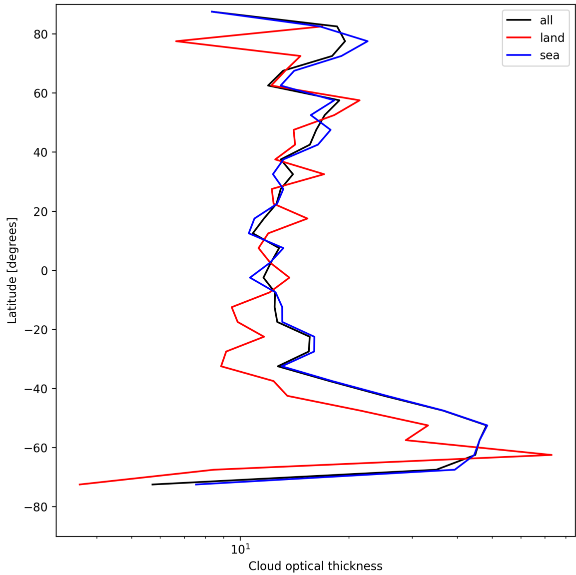
Figure 25: Zonal average of “Cloud optical thickness” for 2025-05-10 to 2025-05-12.
