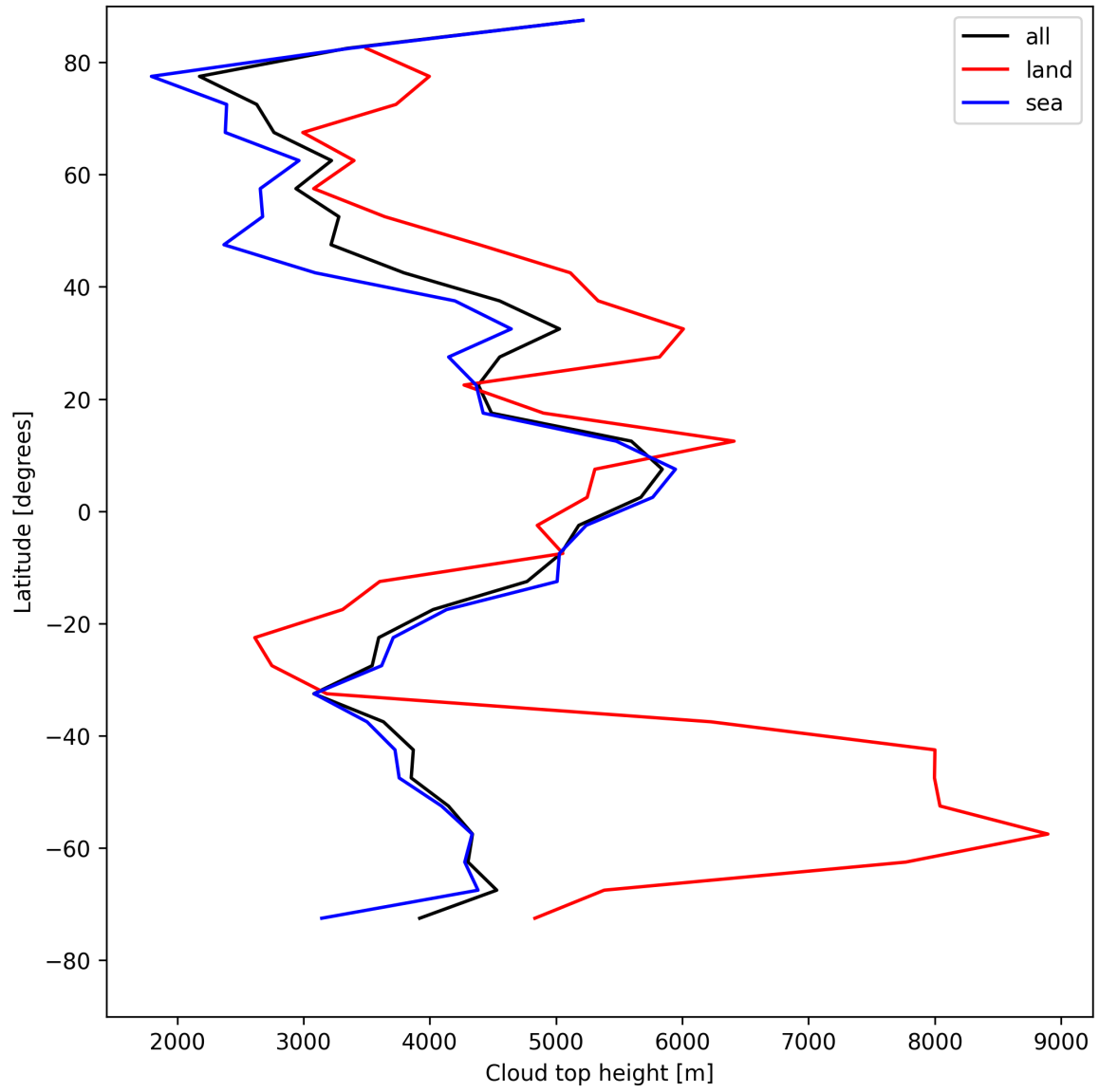
Figure 24: Zonal average of “Cloud top height” for 2025-05-10 to 2025-05-12.
