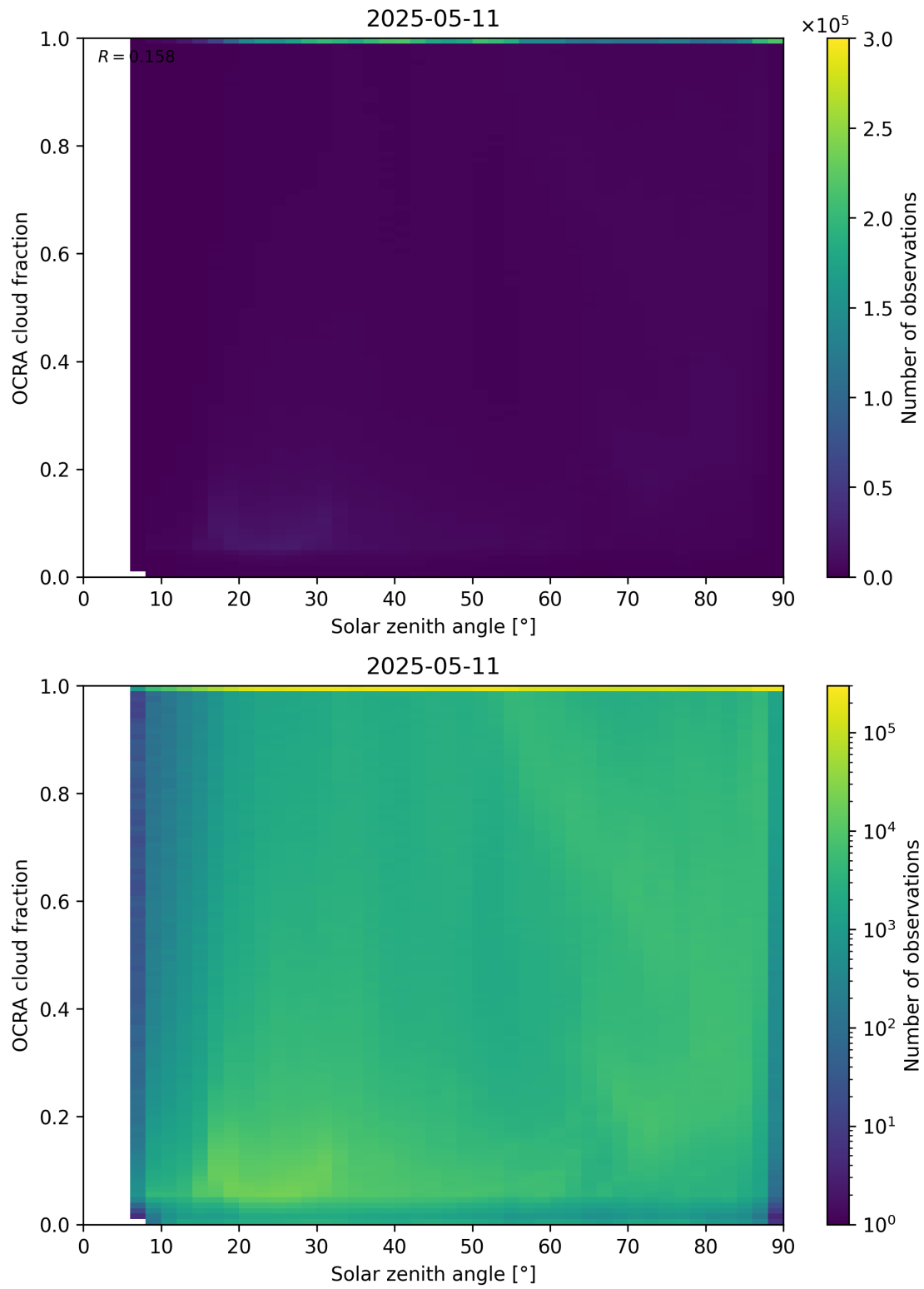
Figure 100: Scatter density plot of “Solar zenith angle” against “OCRA cloud fraction” for 2025-05-10 to 2025-05-12.
