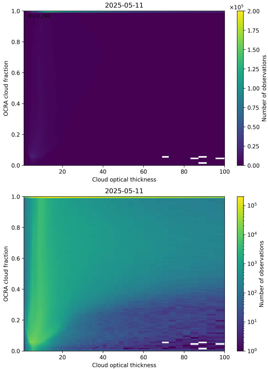
Figure 83: Scatter density plot of “Cloud optical thickness” against “OCRA cloud fraction” for 2025-05-10 to 2025-05-12.
