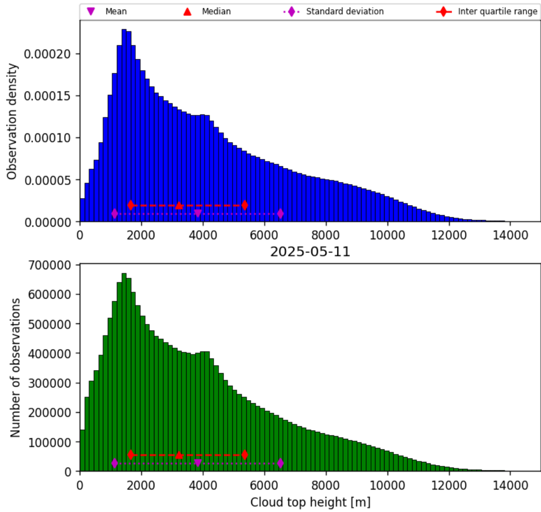
Figure 40: Histogram of “Cloud top height” for 2025-05-10 to 2025-05-12
