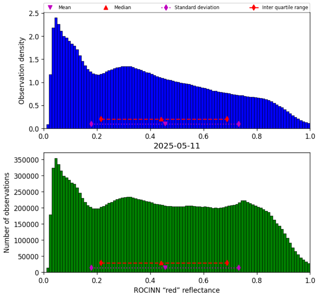
Figure 53: Histogram of “ROCINN “red” reflectance” for 2025-05-10 to 2025-05-12
