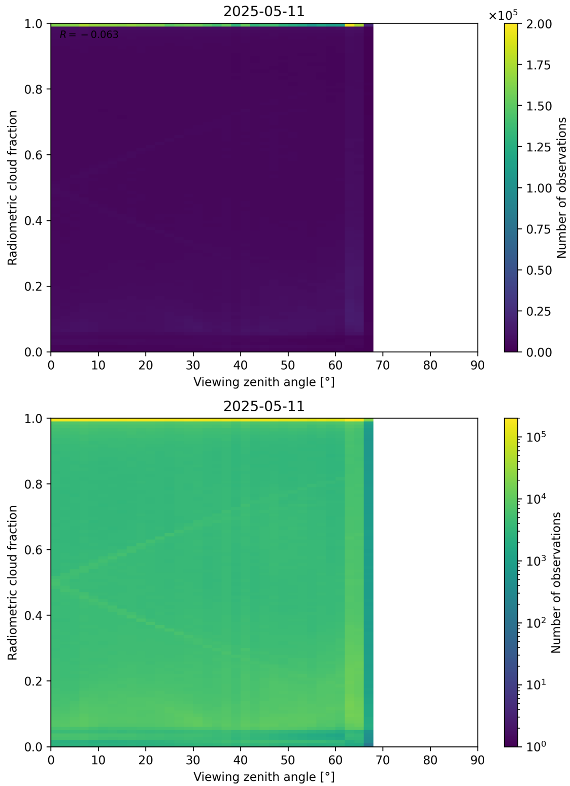
Figure 107: Scatter density plot of “Viewing zenith angle” against “Radiometric cloud fraction” for 2025-05-10 to 2025-05-12.
