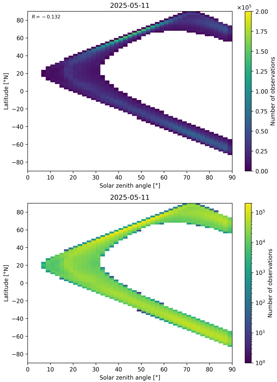
Figure 105: Scatter density plot of “Solar zenith angle” against “Latitude” for 2025-05-10 to 2025-05-12.
