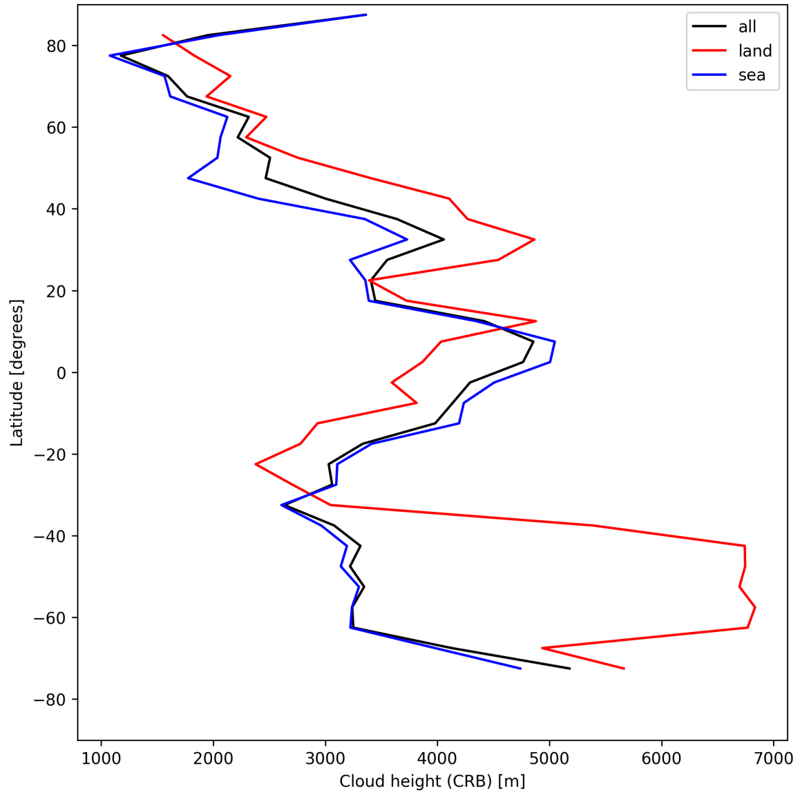
Figure 27: Zonal average of “Cloud height (CRB)” for 2025-05-10 to 2025-05-12.
