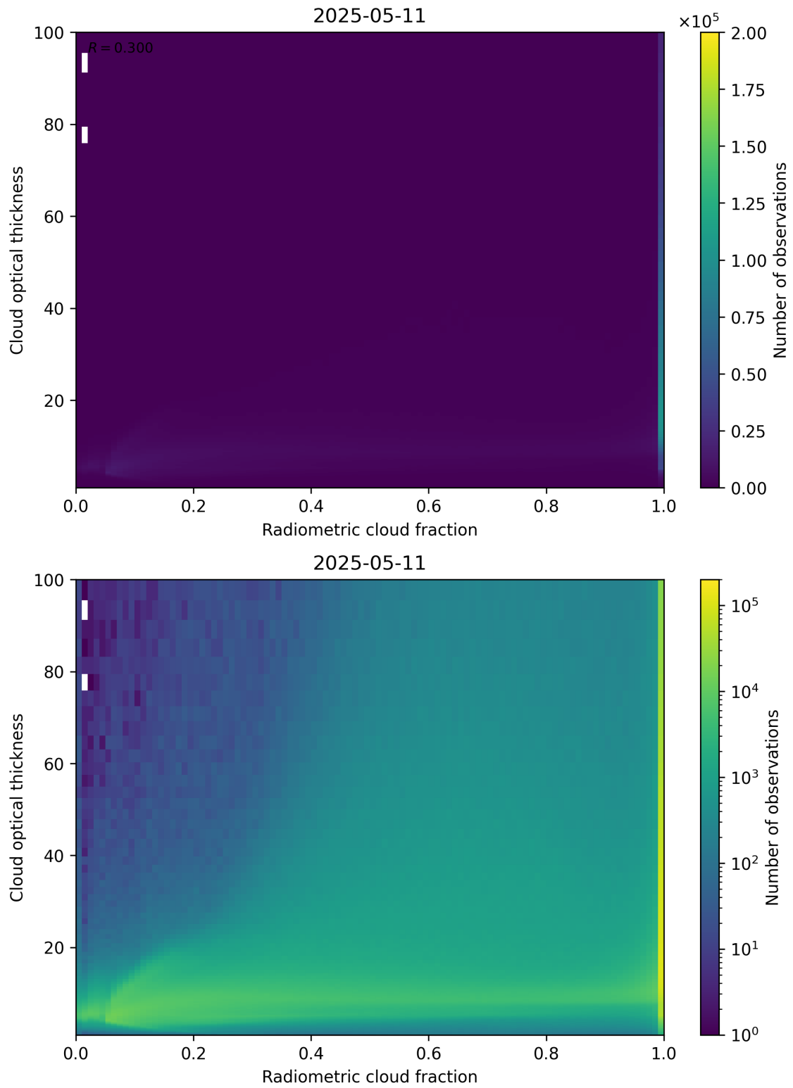
Figure 75: Scatter density plot of “Radiometric cloud fraction” against “Cloud optical thickness” for 2025-05-10 to 2025-05-12.
