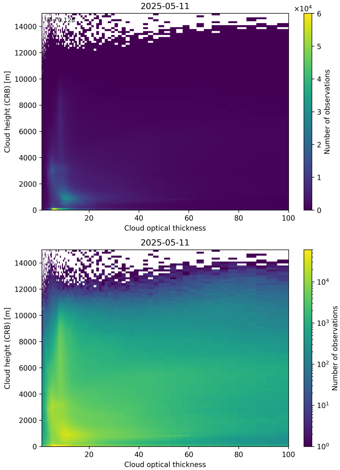
Figure 85: Scatter density plot of “Cloud optical thickness” against “Cloud height (CRB)” for 2025-05-10 to 2025-05-12.
