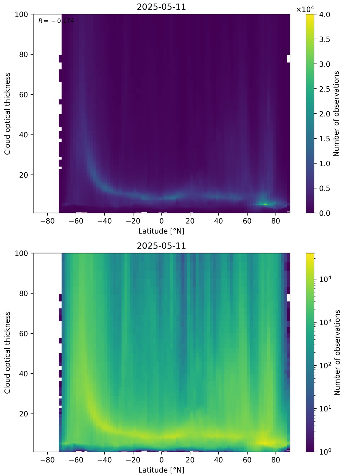
Figure 96: Scatter density plot of “Latitude” against “Cloud optical thickness” for 2025-05-10 to 2025-05-12.
