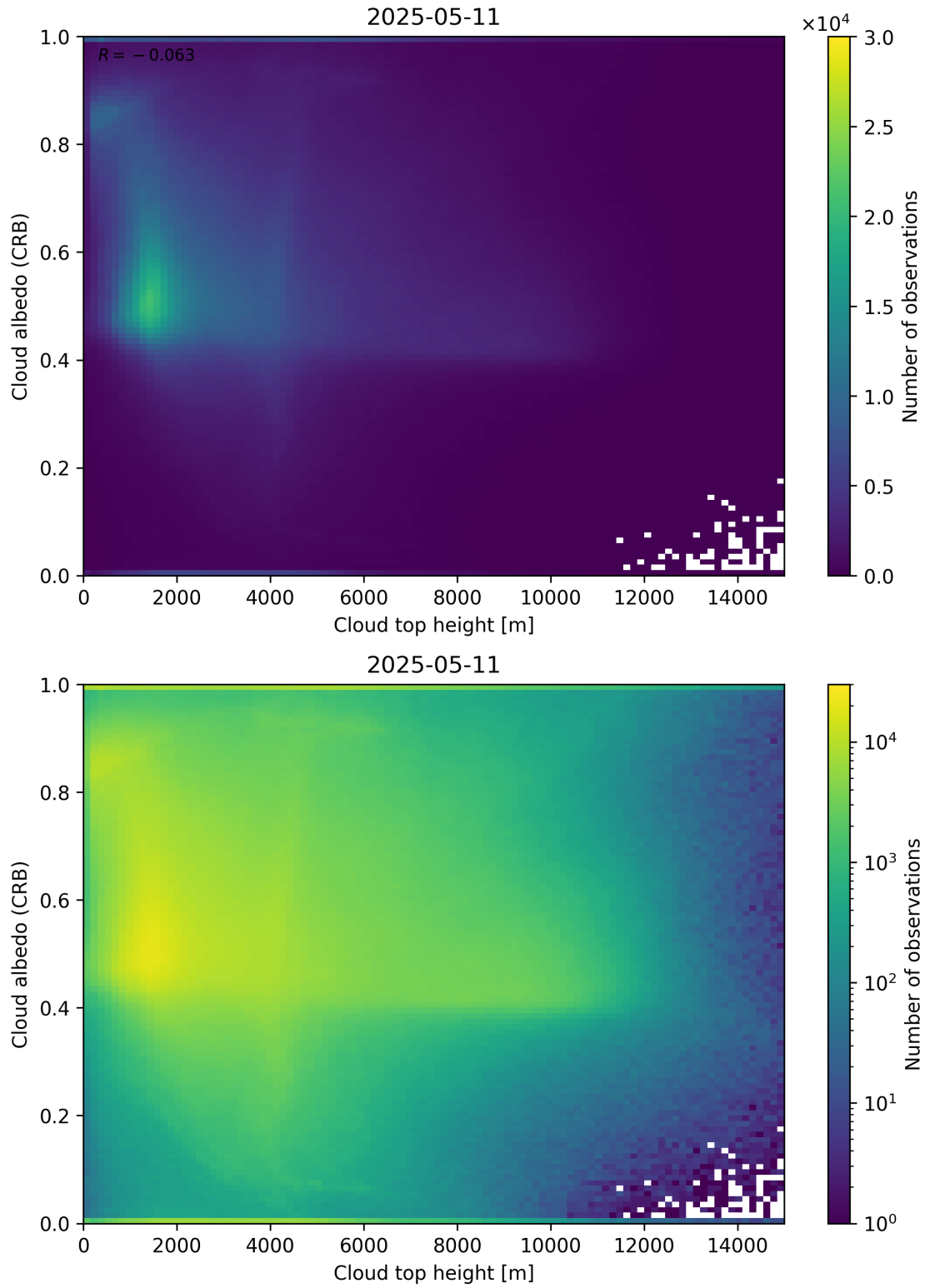
Figure 86: Scatter density plot of “Cloud top height” against “Cloud albedo (CRB)” for 2025-05-10 to 2025-05-12.
