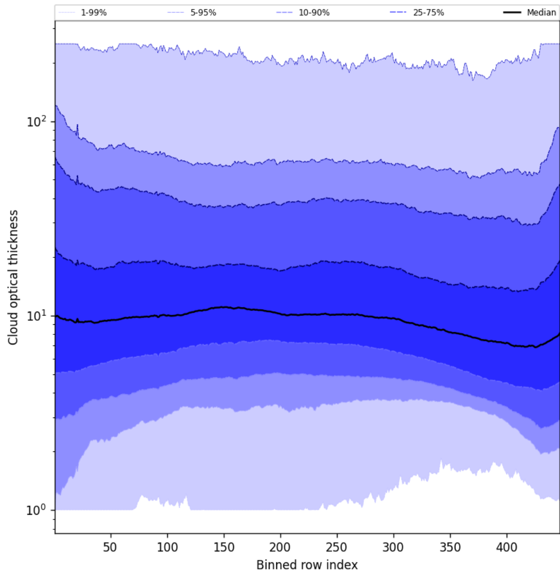
Figure 57: Along track statistics of “Cloud optical thickness” for 2025-05-10 to 2025-05-12
