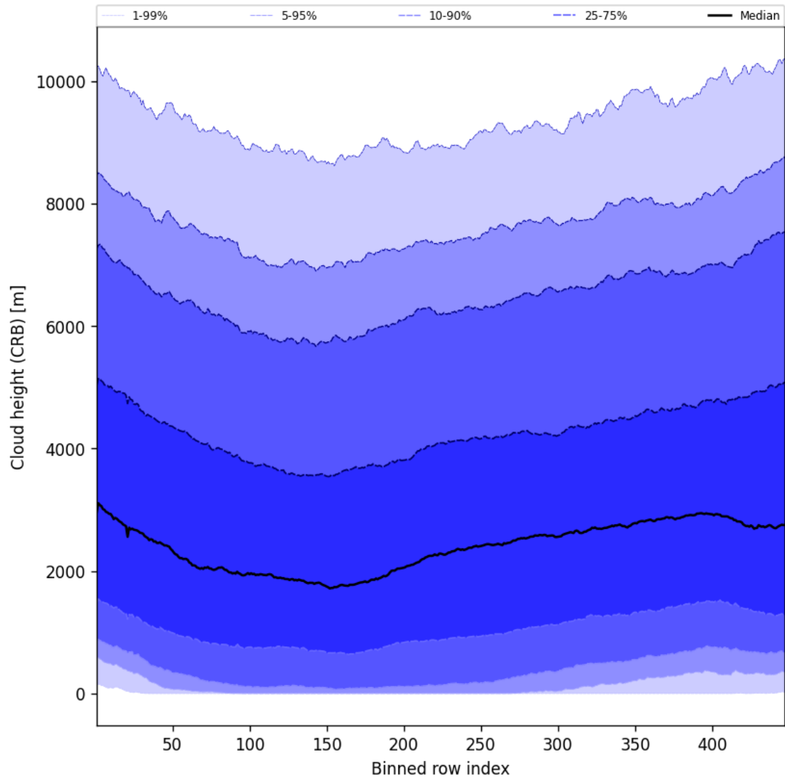
Figure 59: Along track statistics of “Cloud height (CRB)” for 2025-05-10 to 2025-05-12
