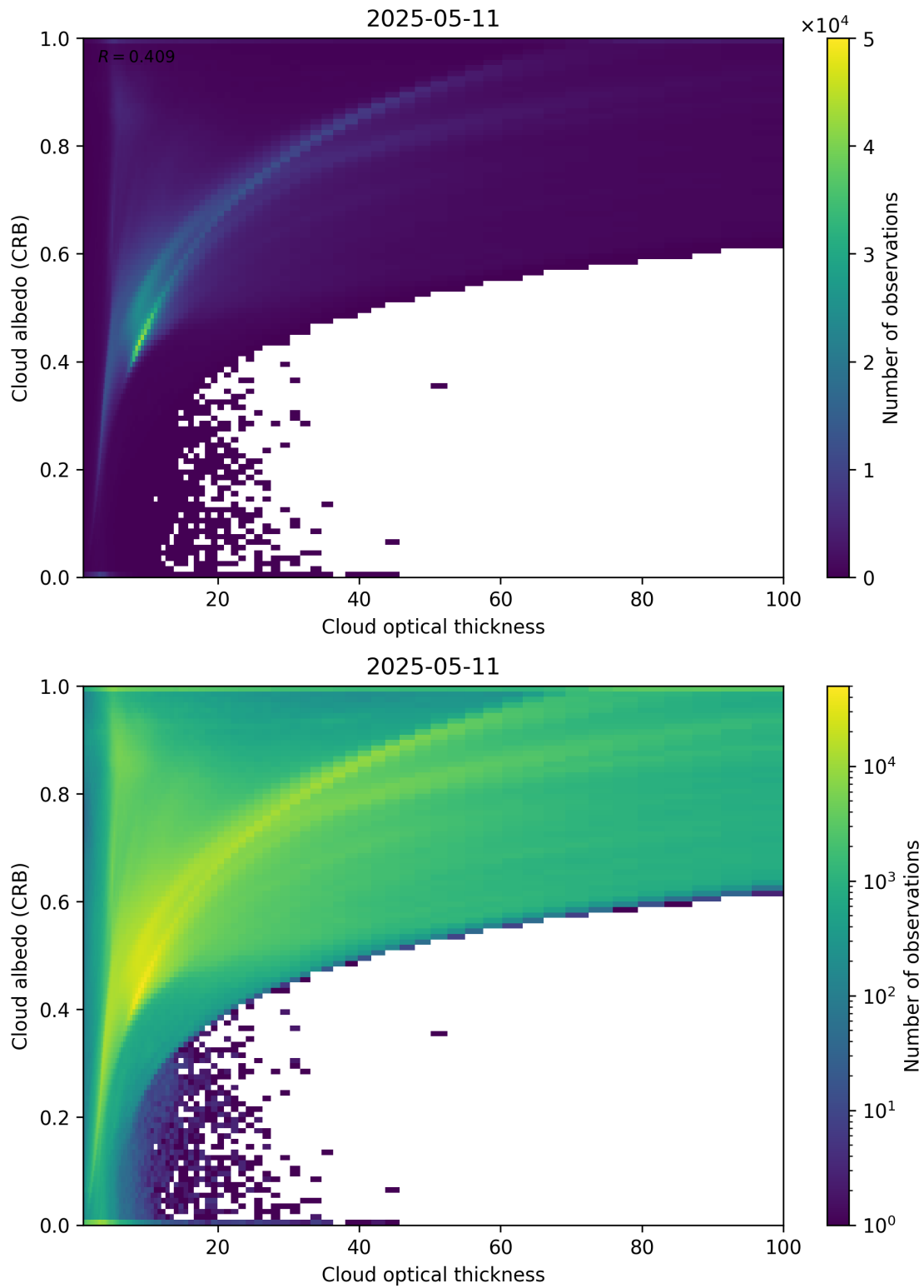
Figure 82: Scatter density plot of “Cloud optical thickness” against “Cloud albedo (CRB)” for 2025-05-10 to 2025-05-12.
