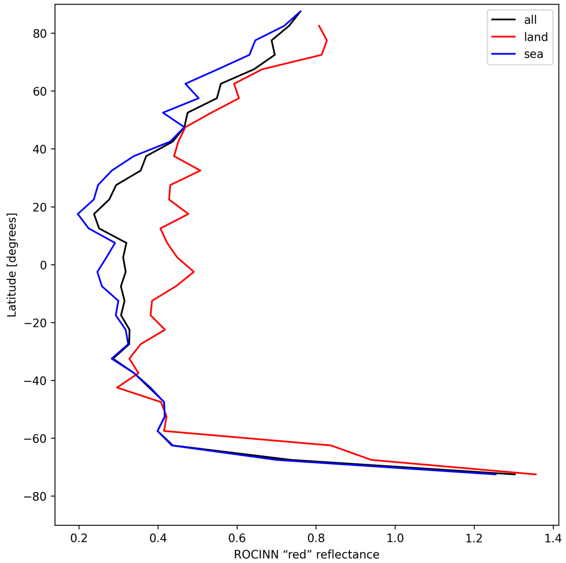
Figure 37: Zonal average of “ROCINN “red” reflectance” for 2025-05-10 to 2025-05-12.
