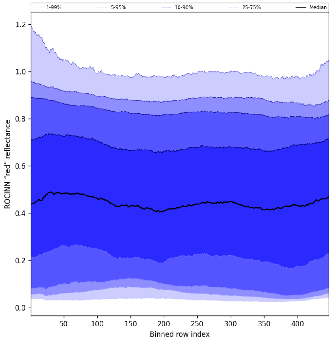
Figure 69: Along track statistics of “ROCINN “red” reflectance” for 2025-05-10 to 2025-05-12
