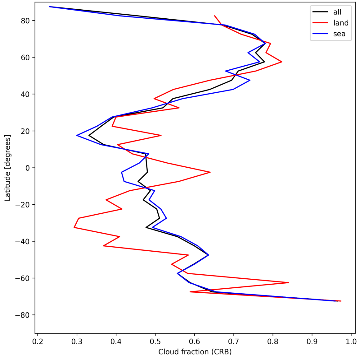
Figure 26: Zonal average of “Cloud fraction (CRB)” for 2025-05-10 to 2025-05-12.
