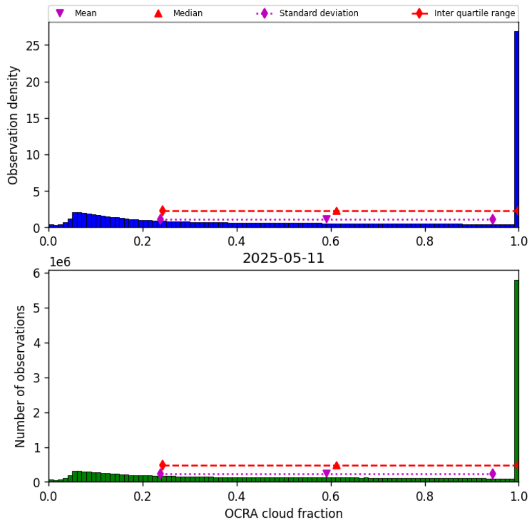
Figure 50: Histogram of “OCRA cloud fraction” for 2025-05-10 to 2025-05-12
