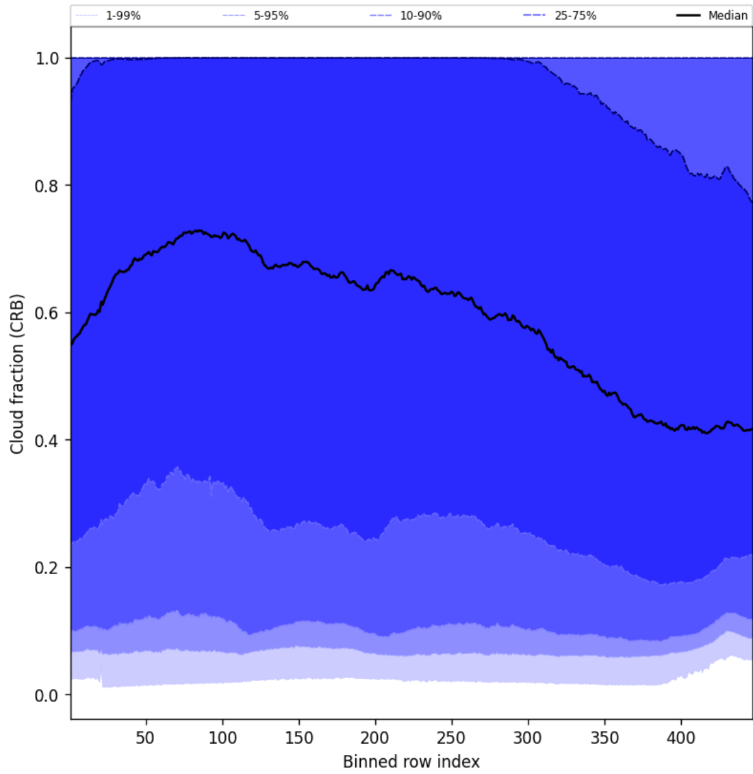
Figure 58: Along track statistics of “Cloud fraction (CRB)” for 2025-05-10 to 2025-05-12
