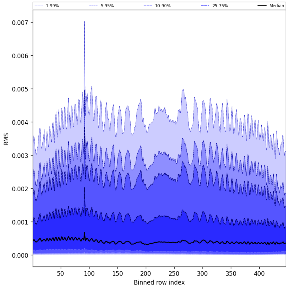
Figure 63: Along track statistics of “RMS” for 2025-05-10 to 2025-05-12
