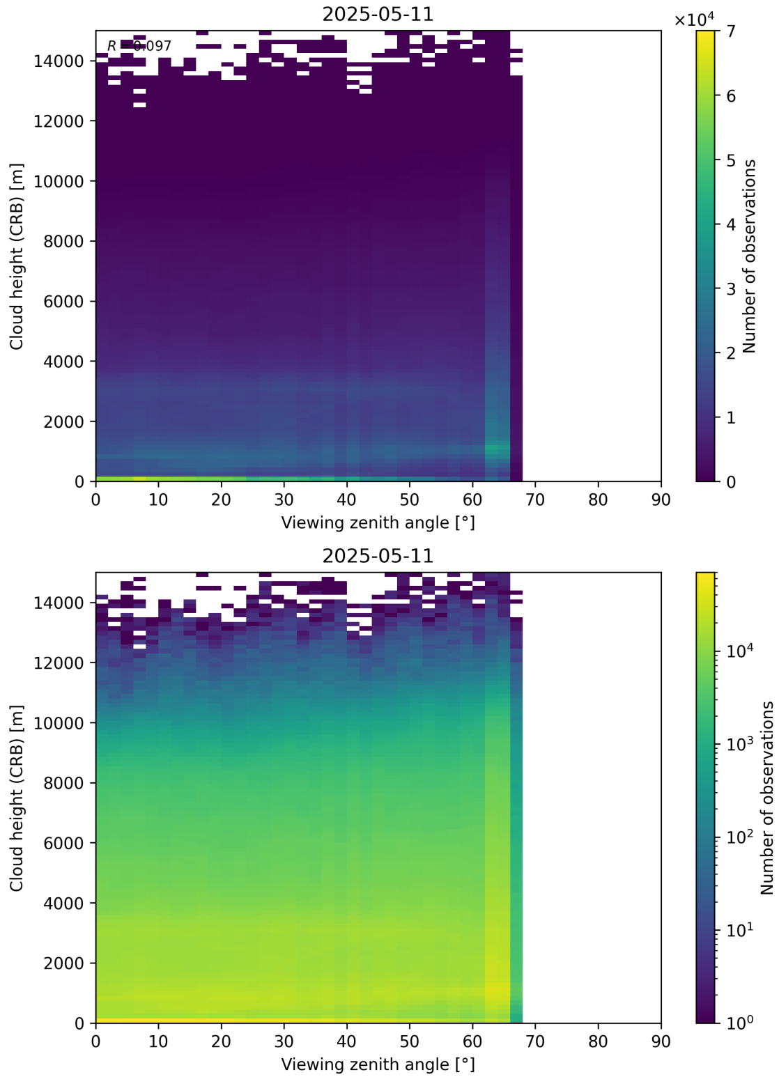
Figure 110: Scatter density plot of “Viewing zenith angle” against “Cloud height (CRB)” for 2025-05-10 to 2025-05-12.
