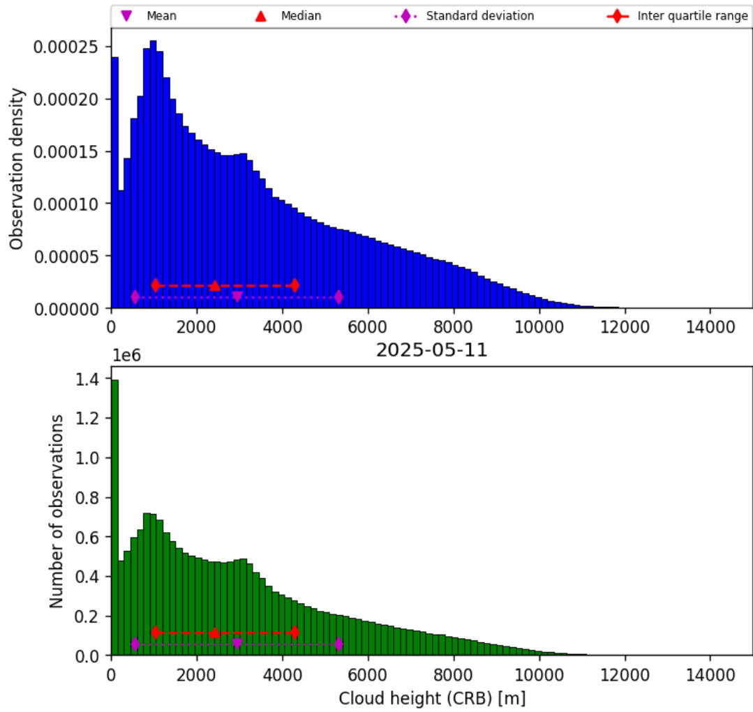
Figure 43: Histogram of “Cloud height (CRB)” for 2025-05-10 to 2025-05-12
