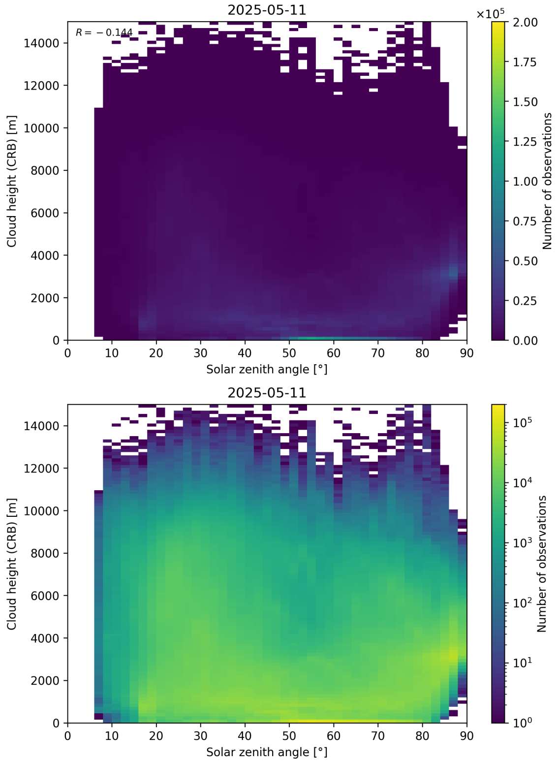
Figure 102: Scatter density plot of “Solar zenith angle” against “Cloud height (CRB)” for 2025-05-10 to 2025-05-12.
