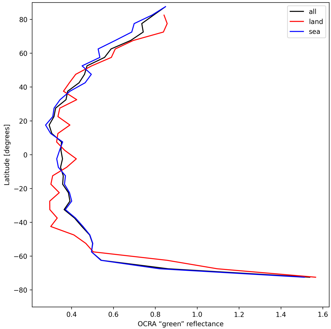
Figure 36: Zonal average of “OCRA “green” reflectance” for 2025-05-10 to 2025-05-12.
