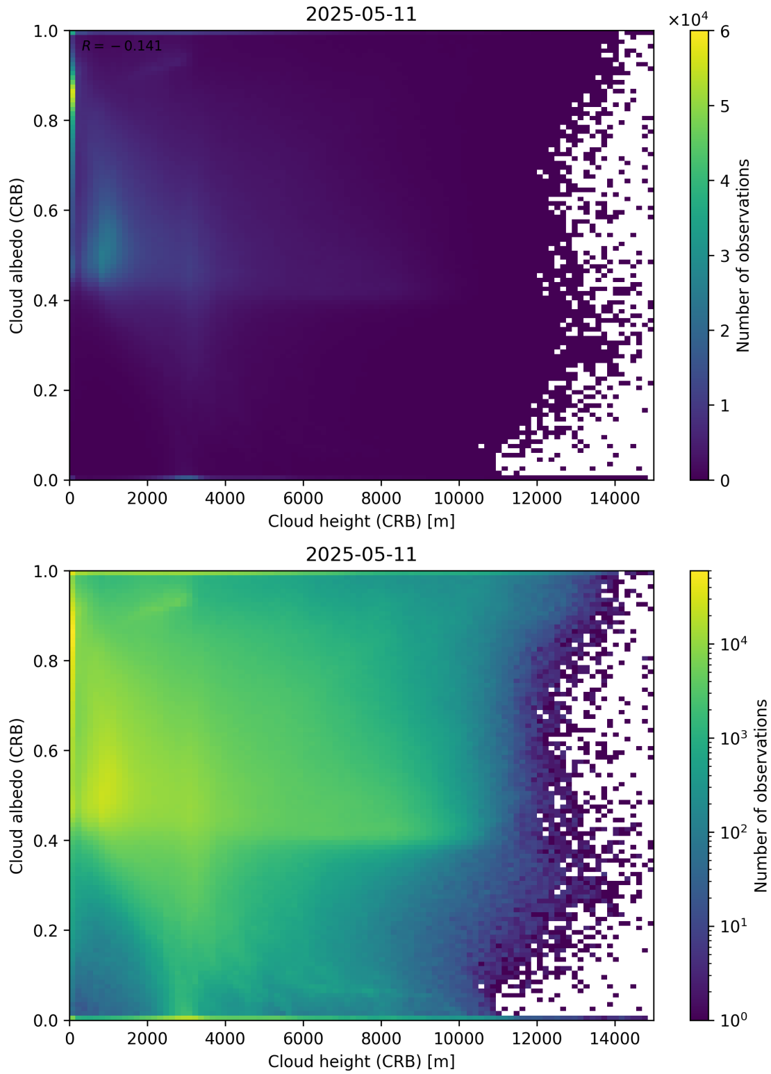
Figure 80: Scatter density plot of “Cloud height (CRB)” against “Cloud albedo (CRB)” for 2025-05-10 to 2025-05-12.
