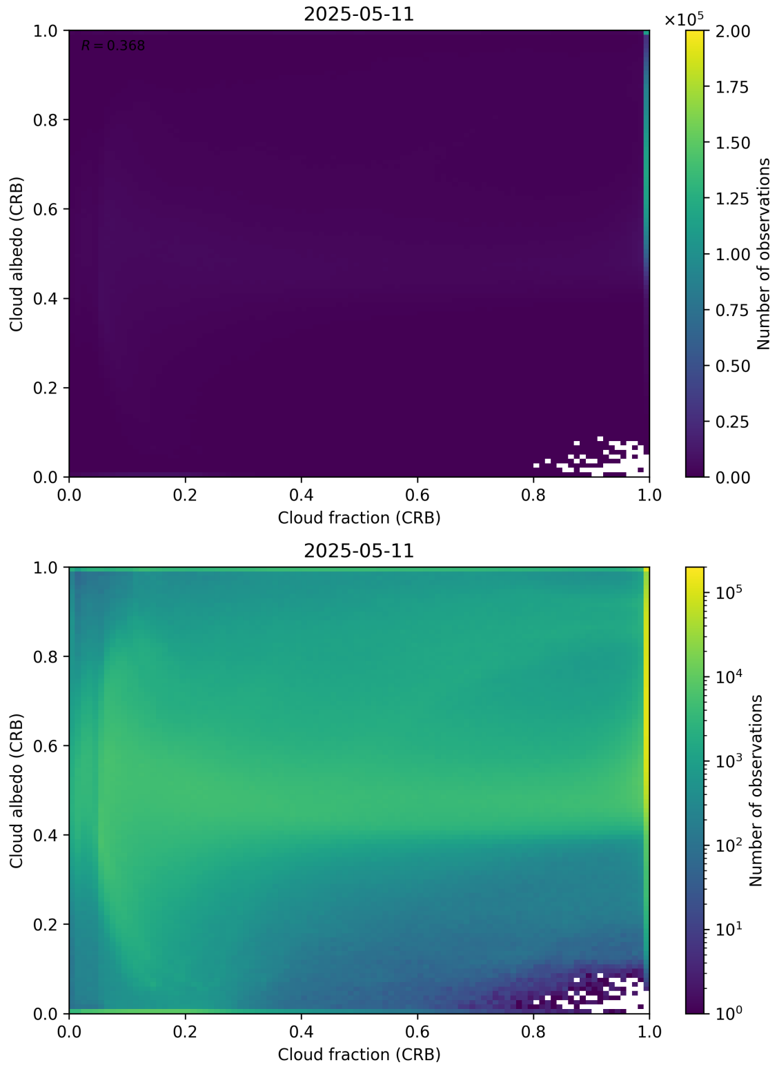
Figure 77: Scatter density plot of “Cloud fraction (CRB)” against “Cloud albedo (CRB)” for 2025-05-10 to 2025-05-12.
