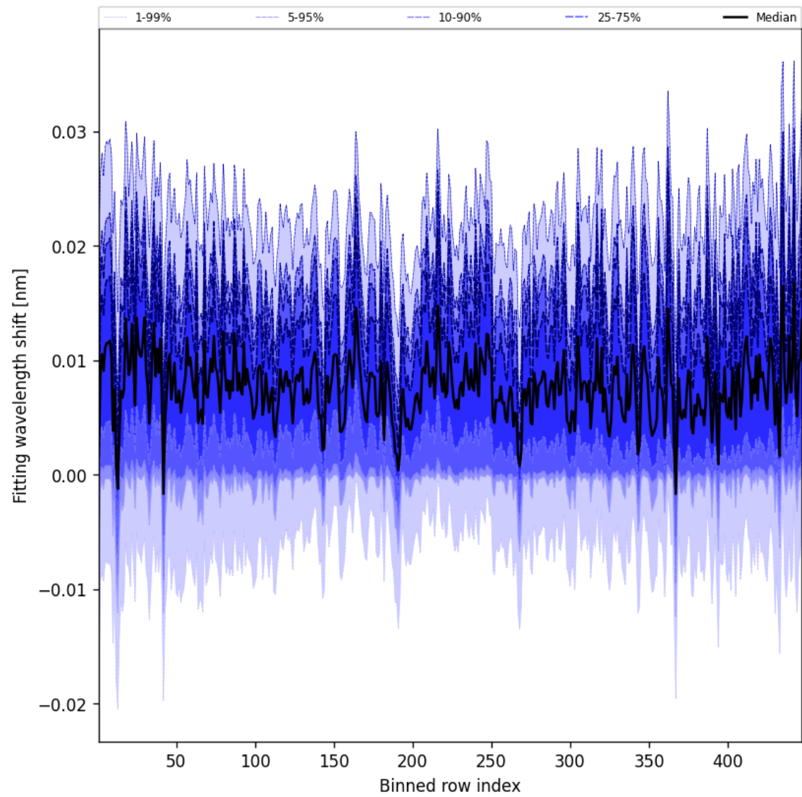
Figure 65: Along track statistics of “Fitting wavelength shift” for 2025-05-10 to 2025-05-12
