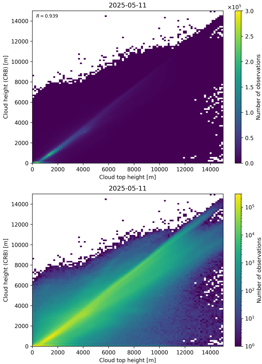
Figure 89: Scatter density plot of “Cloud top height” against “Cloud height (CRB)” for 2025-05-10 to 2025-05-12.
