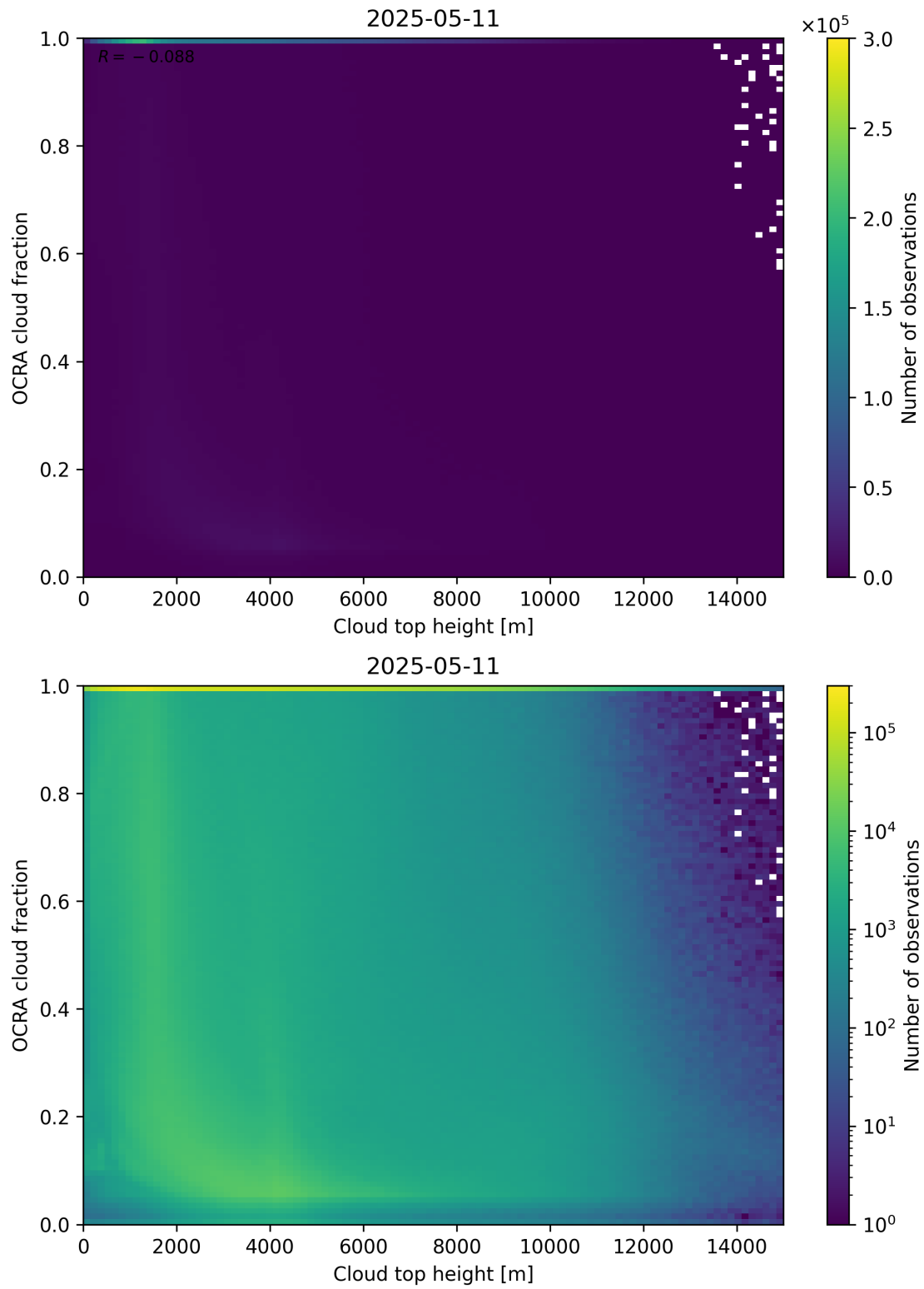
Figure 87: Scatter density plot of “Cloud top height” against “OCRA cloud fraction” for 2025-05-10 to 2025-05-12.
