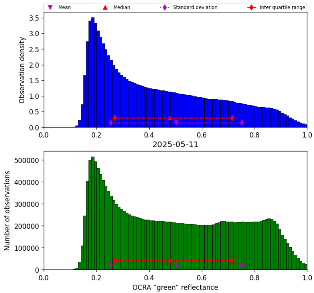
Figure 52: Histogram of “OCRA “green” reflectance” for 2025-05-10 to 2025-05-12
