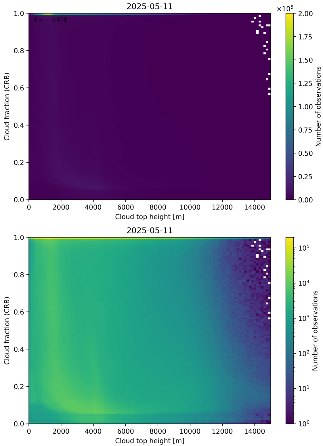
Figure 88: Scatter density plot of “Cloud top height” against “Cloud fraction (CRB)” for 2025-05-10 to 2025-05-12.
