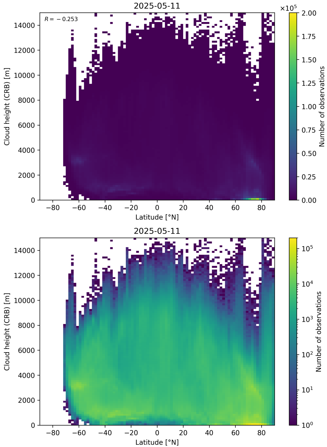
Figure 95: Scatter density plot of “Latitude” against “Cloud height (CRB)” for 2025-05-10 to 2025-05-12.
