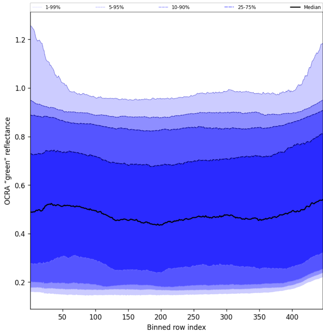
Figure 68: Along track statistics of “OCRA “green” reflectance” for 2025-05-10 to 2025-05-12
