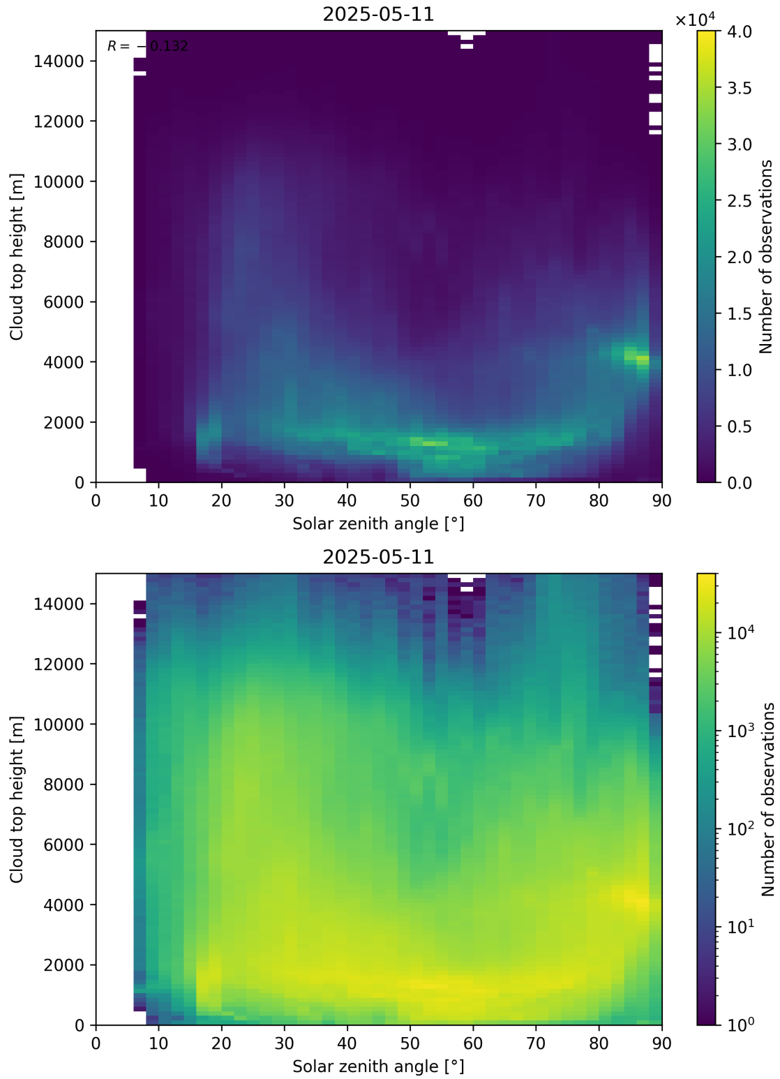
Figure 104: Scatter density plot of “Solar zenith angle” against “Cloud top height” for 2025-05-10 to 2025-05-12.
