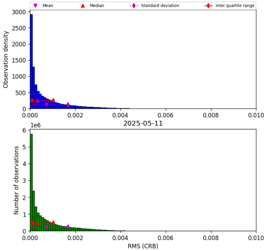
Figure 48: Histogram of “RMS (CRB)” for 2025-05-10 to 2025-05-12
