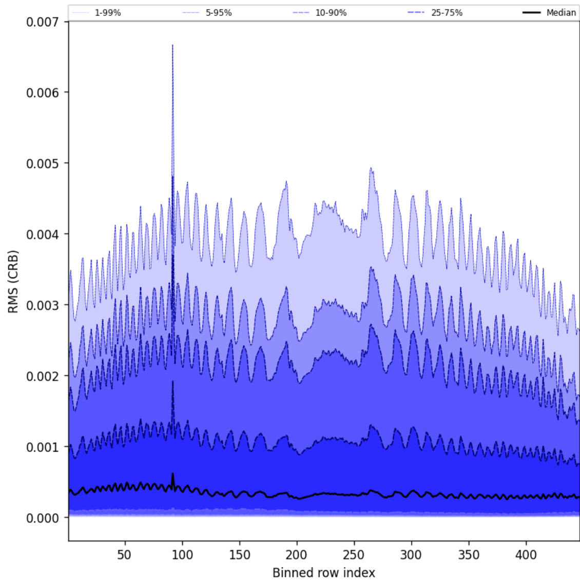
Figure 64: Along track statistics of “RMS (CRB)” for 2025-05-10 to 2025-05-12
