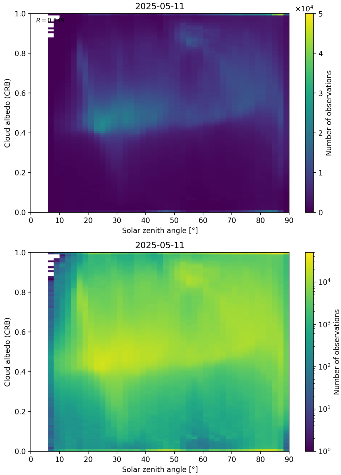
Figure 98: Scatter density plot of “Solar zenith angle” against “Cloud albedo (CRB)” for 2025-05-10 to 2025-05-12.
