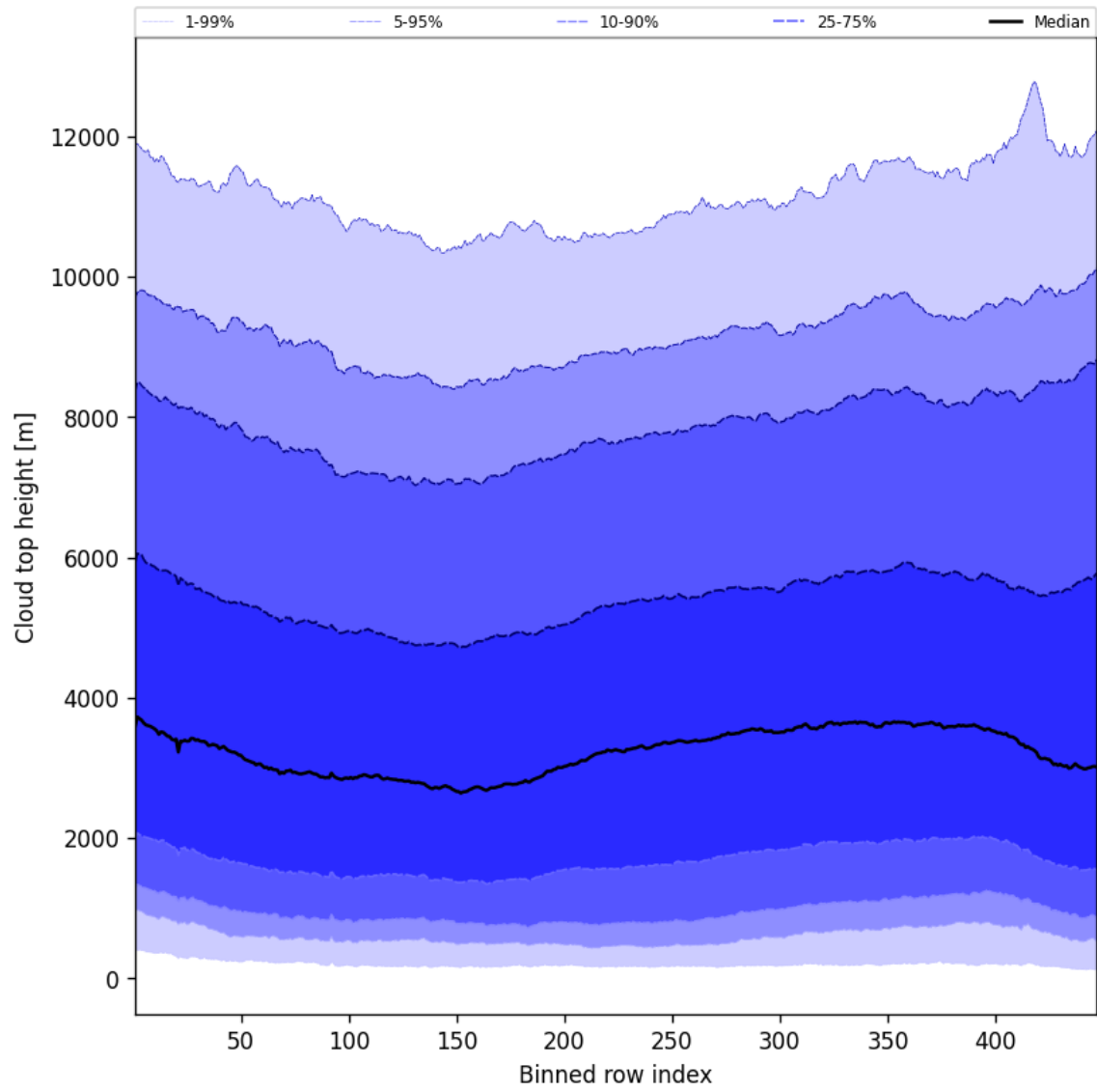
Figure 56: Along track statistics of “Cloud top height” for 2025-05-10 to 2025-05-12
