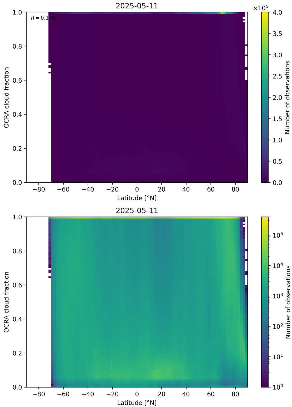
Figure 93: Scatter density plot of “Latitude” against “OCRA cloud fraction” for 2025-05-10 to 2025-05-12.
