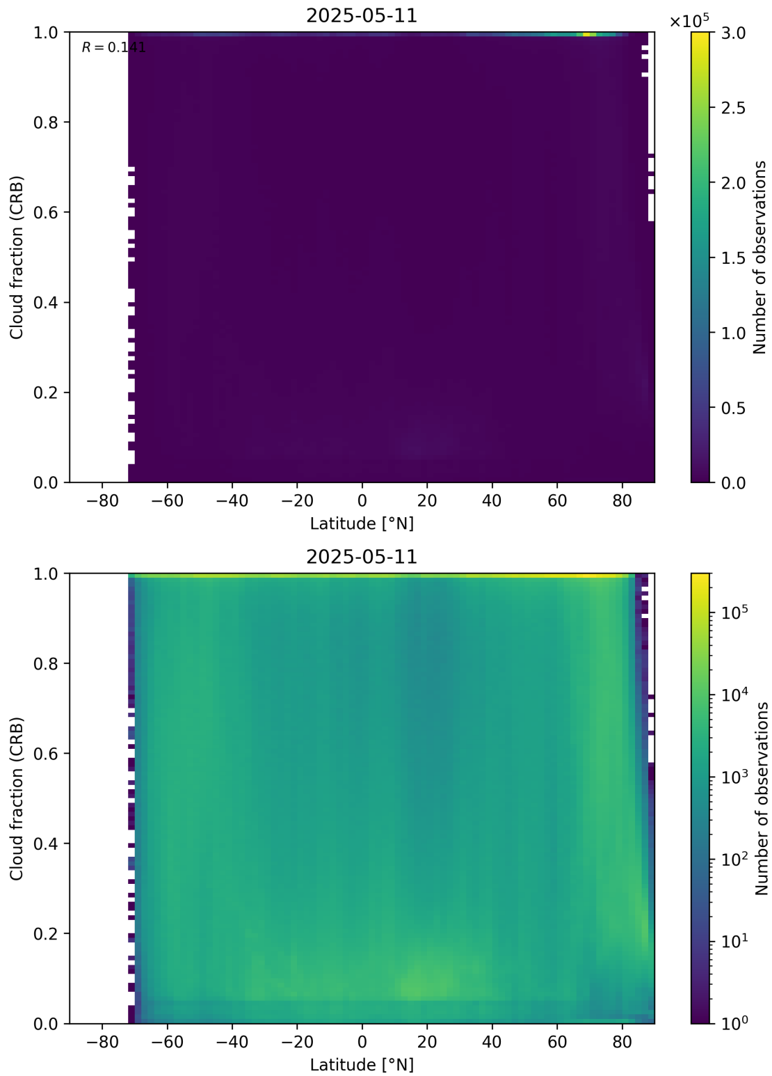
Figure 94: Scatter density plot of “Latitude” against “Cloud fraction (CRB)” for 2025-05-10 to 2025-05-12.
