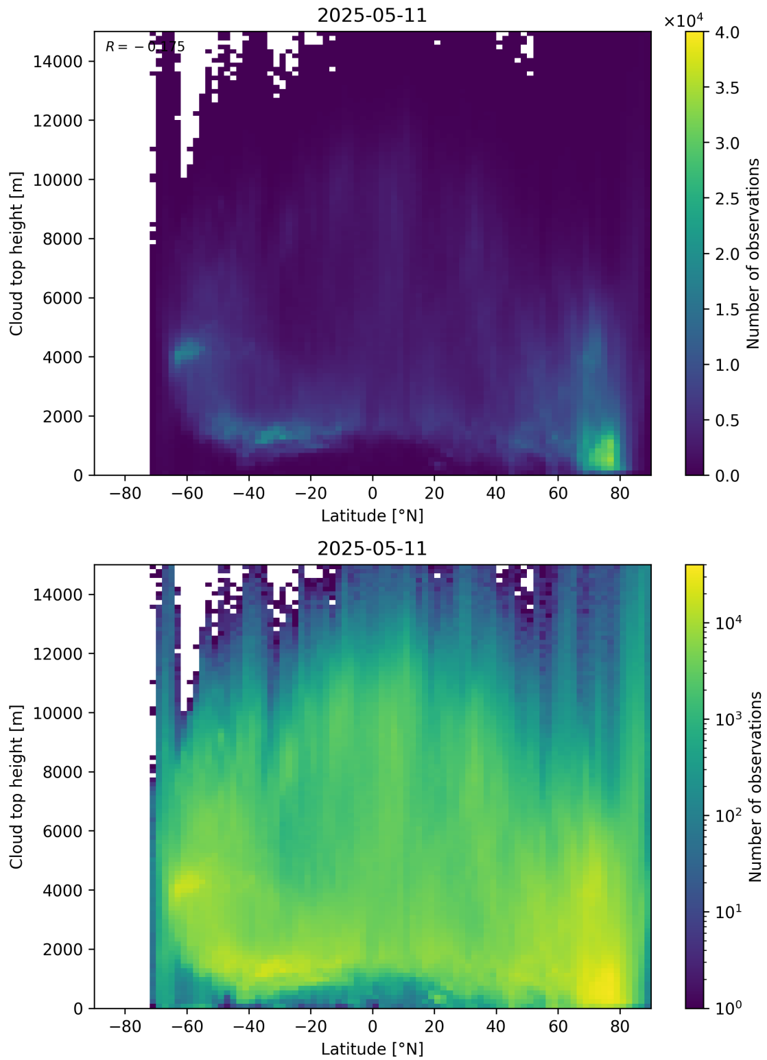
Figure 97: Scatter density plot of “Latitude” against “Cloud top height” for 2025-05-10 to 2025-05-12.
