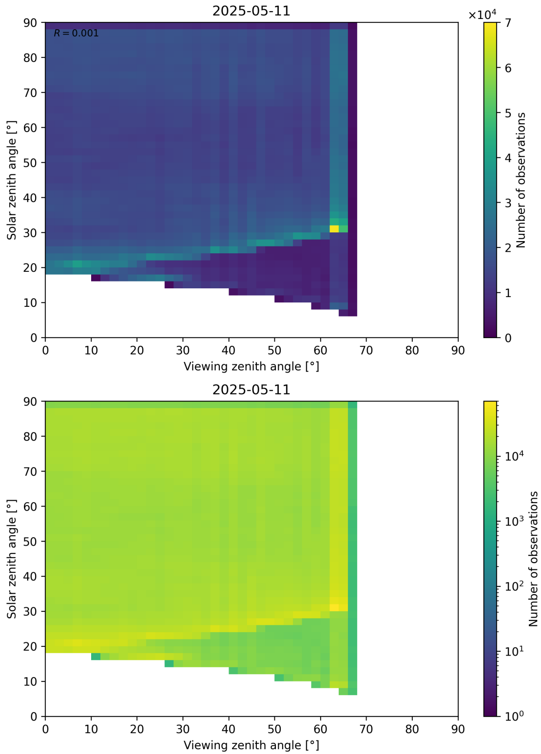
Figure 114: Scatter density plot of “Viewing zenith angle” against “Solar zenith angle” for 2025-05-10 to 2025-05-12.
