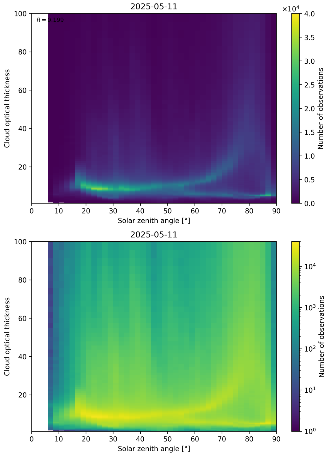
Figure 103: Scatter density plot of “Solar zenith angle” against “Cloud optical thickness” for 2025-05-10 to 2025-05-12.
