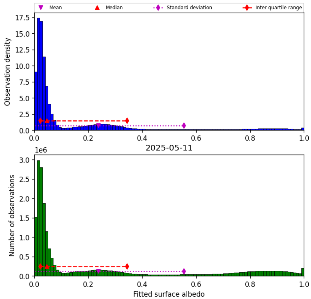
Figure 45: Histogram of “Fitted surface albedo” for 2025-05-10 to 2025-05-12
