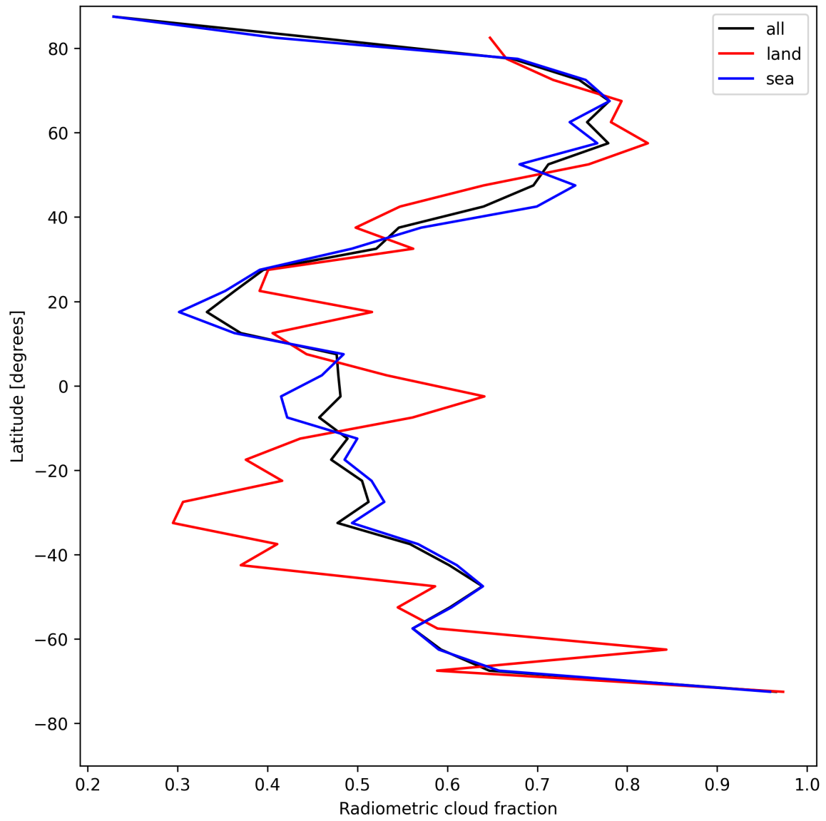
Figure 23: Zonal average of “Radiometric cloud fraction” for 2025-05-10 to 2025-05-12.
