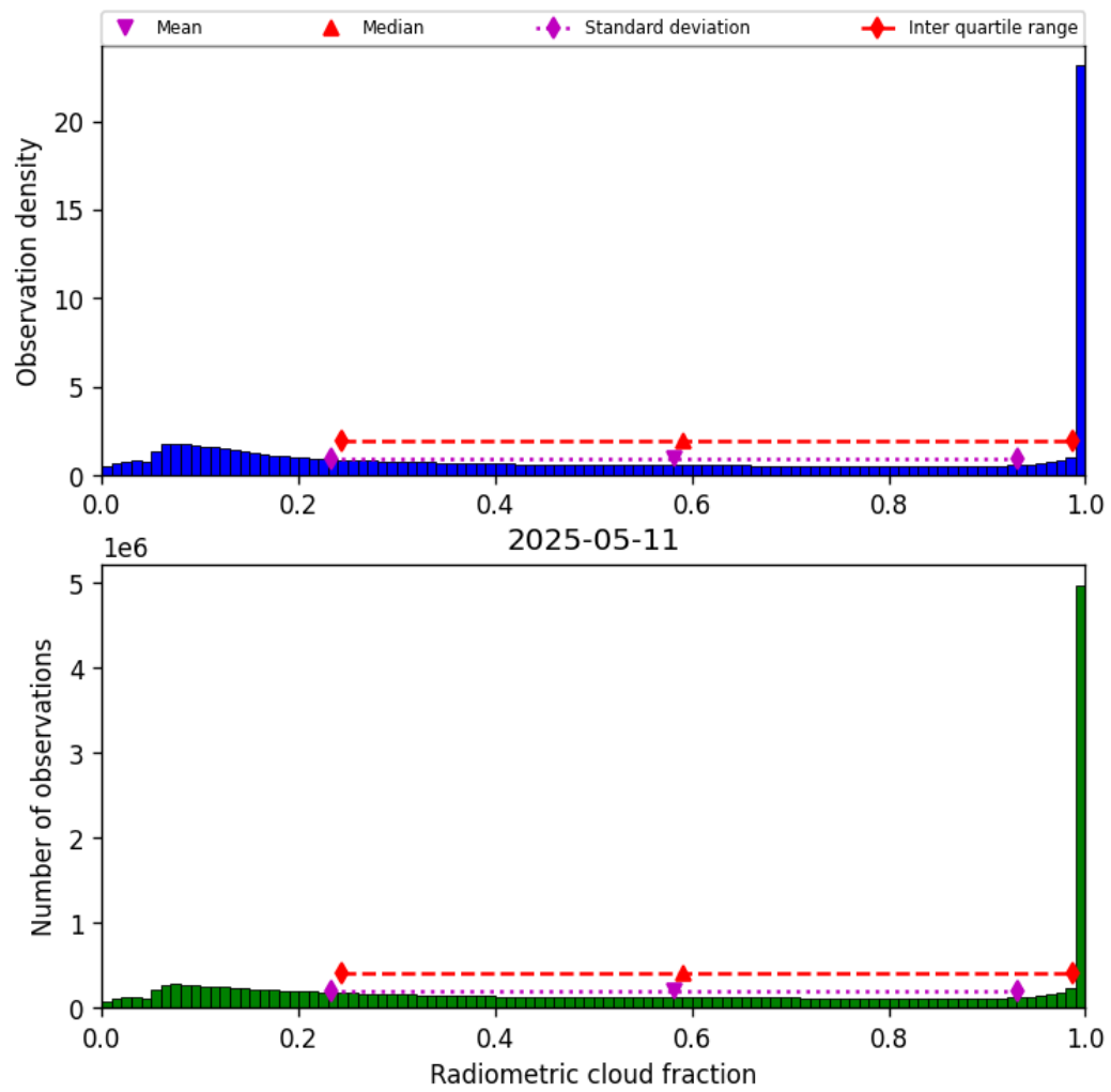
Figure 39: Histogram of “Radiometric cloud fraction” for 2025-05-10 to 2025-05-12
