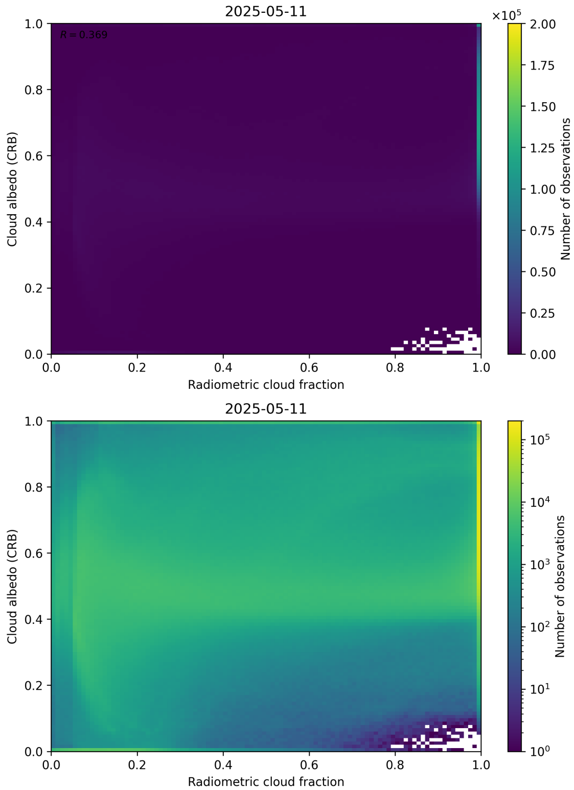
Figure 71: Scatter density plot of “Radiometric cloud fraction” against “Cloud albedo (CRB)” for 2025-05-10 to 2025-05-12.
