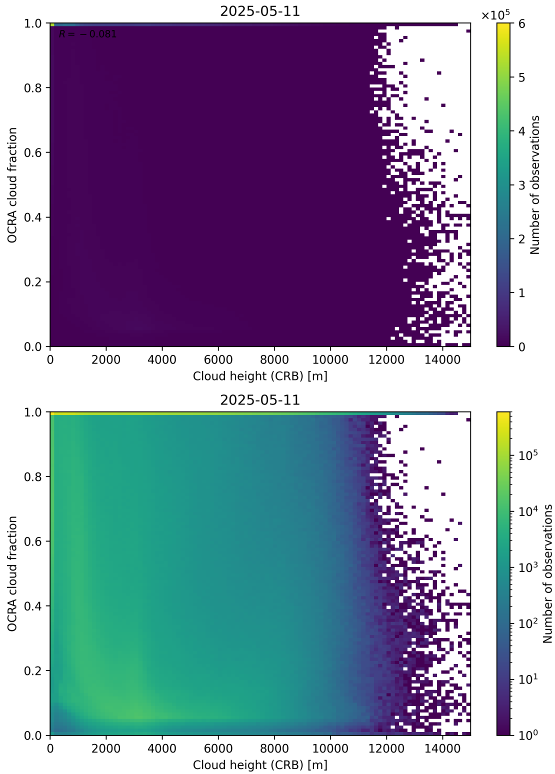
Figure 81: Scatter density plot of “Cloud height (CRB)” against “OCRA cloud fraction” for 2025-05-10 to 2025-05-12.
