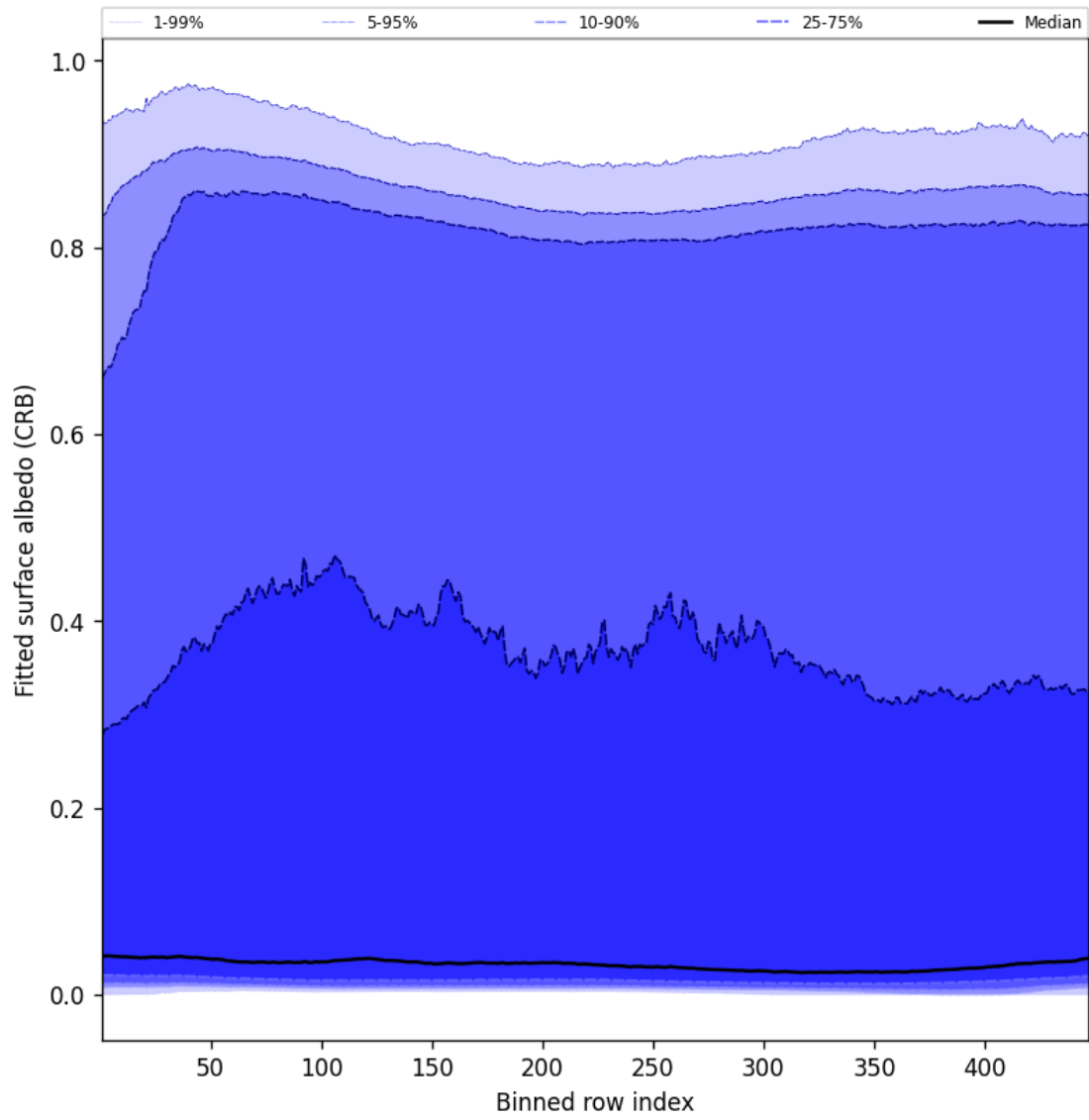
Figure 62: Along track statistics of “Fitted surface albedo (CRB)” for 2025-05-10 to 2025-05-12
