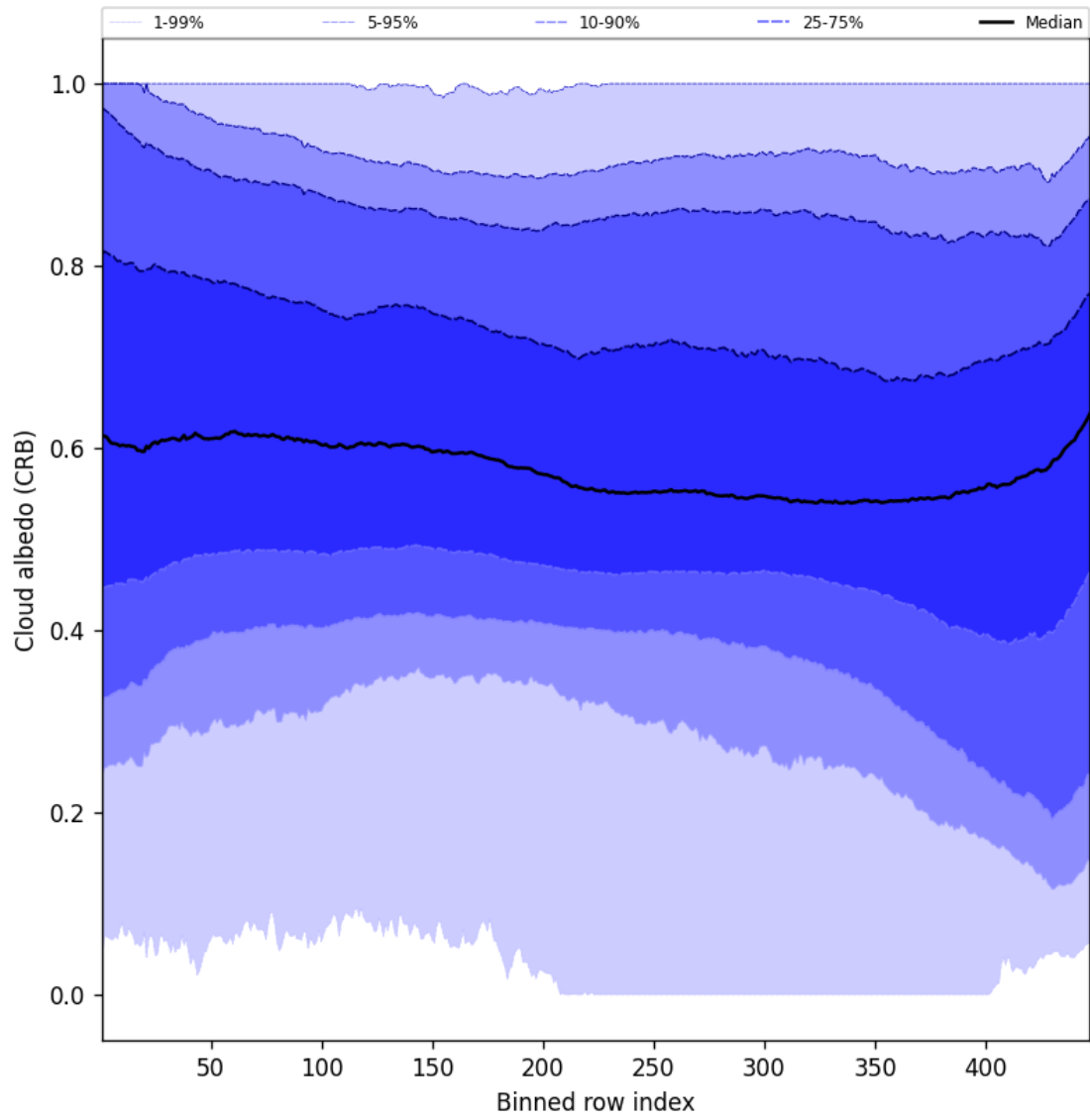
Figure 60: Along track statistics of “Cloud albedo (CRB)” for 2025-05-10 to 2025-05-12
