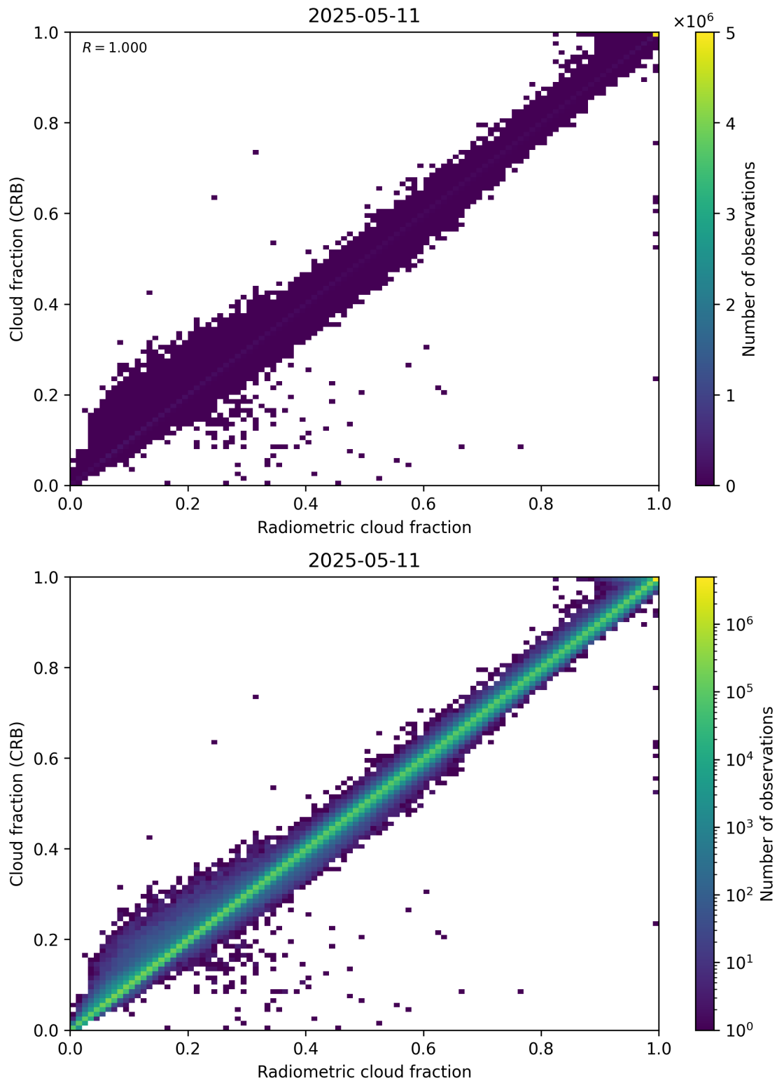
Figure 73: Scatter density plot of “Radiometric cloud fraction” against “Cloud fraction (CRB)” for 2025-05-10 to 2025-05-12.
