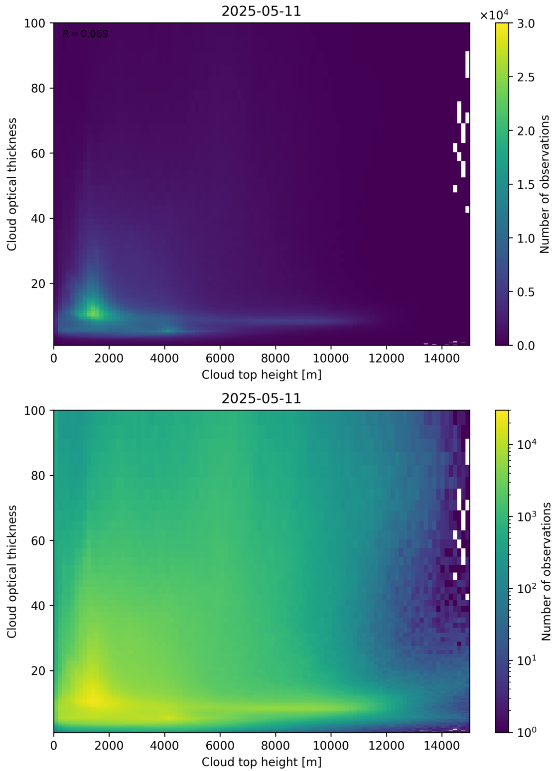
Figure 90: Scatter density plot of “Cloud top height” against “Cloud optical thickness” for 2025-05-10 to 2025-05-12.
