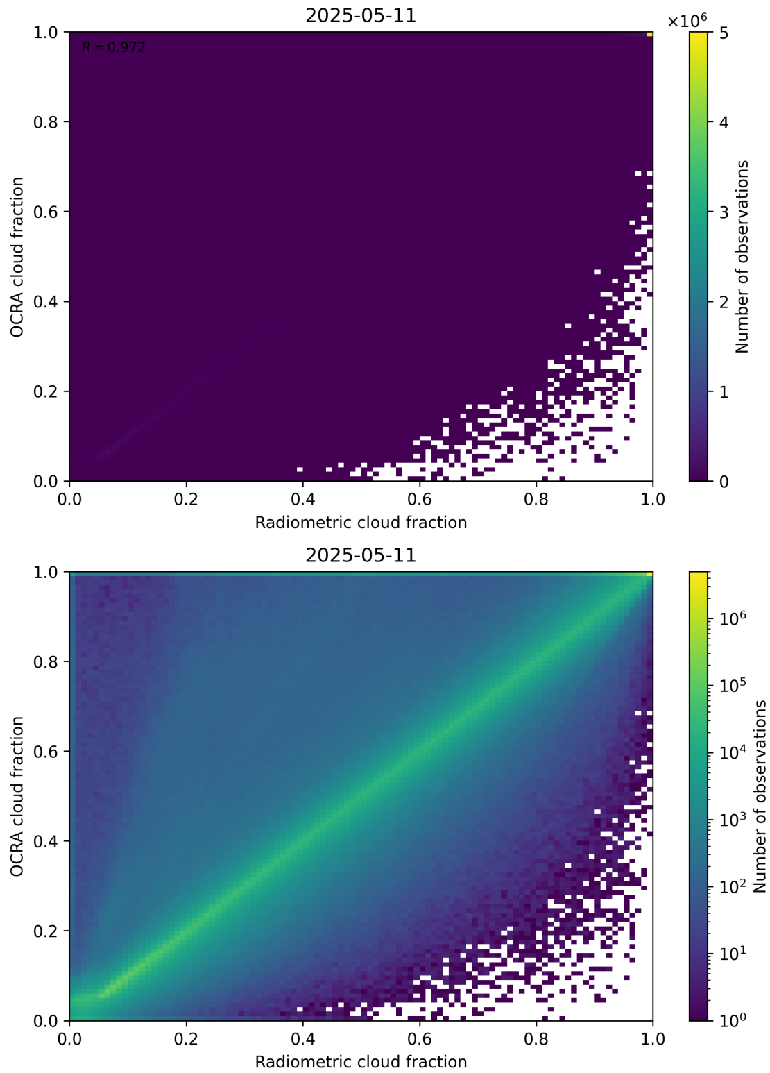
Figure 72: Scatter density plot of “Radiometric cloud fraction” against “OCRA cloud fraction” for 2025-05-10 to 2025-05-12.
