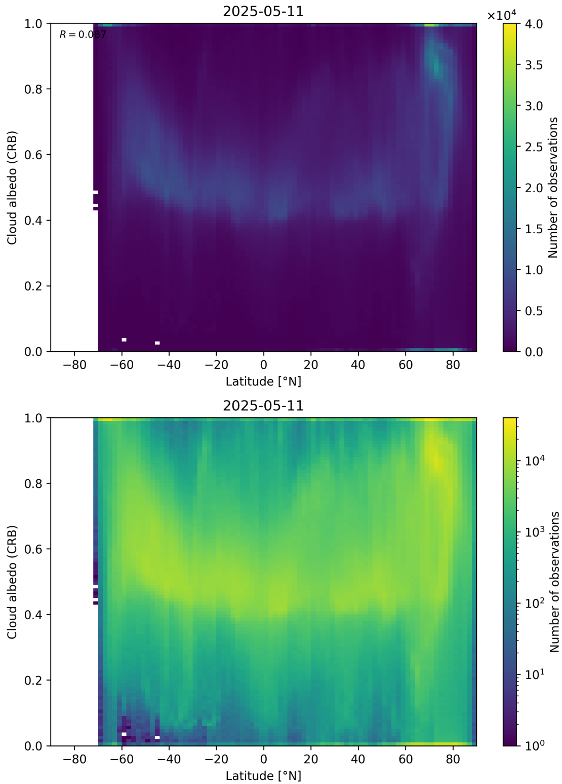
Figure 91: Scatter density plot of “Latitude” against “Cloud albedo (CRB)” for 2025-05-10 to 2025-05-12.
