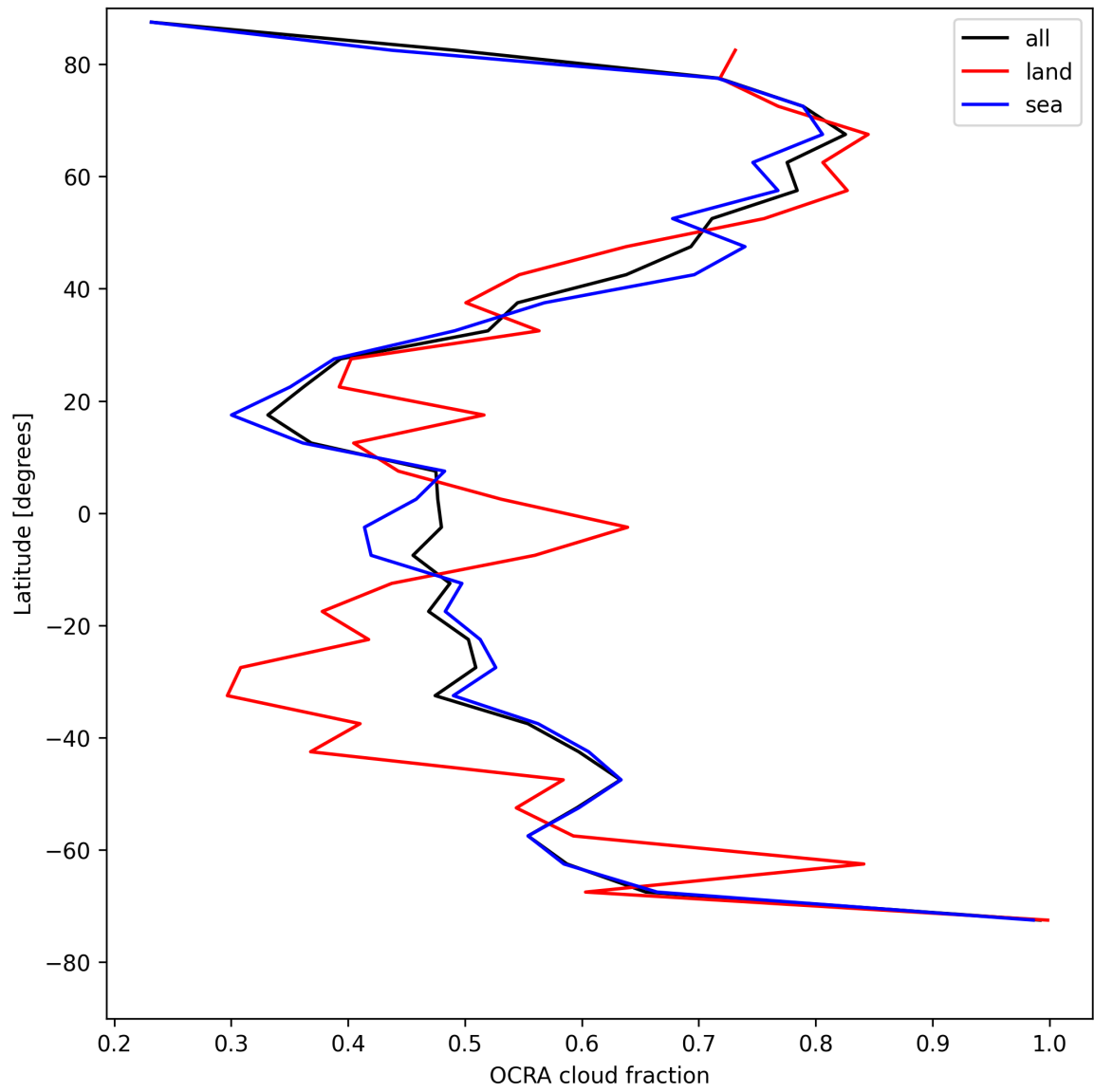
Figure 34: Zonal average of “OCRA cloud fraction” for 2025-05-10 to 2025-05-12.
