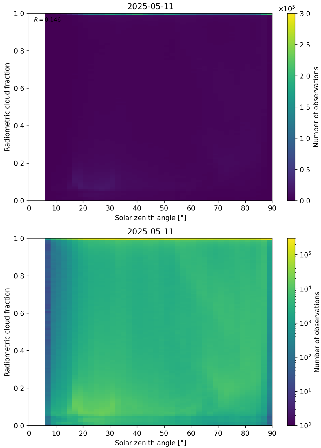
Figure 99: Scatter density plot of “Solar zenith angle” against “Radiometric cloud fraction” for 2025-05-10 to 2025-05-12.
