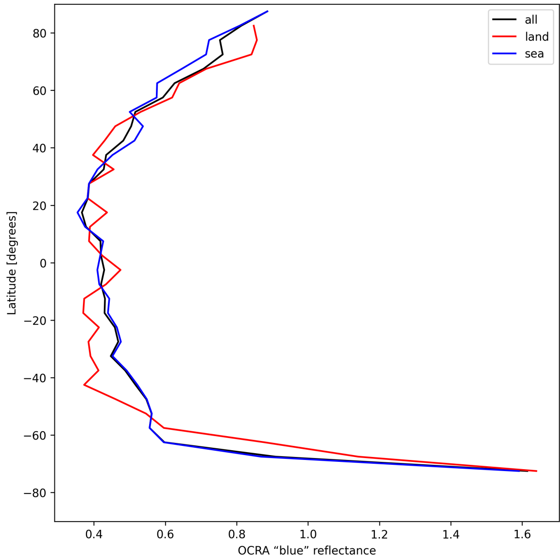
Figure 35: Zonal average of “OCRA “blue” reflectance” for 2025-05-10 to 2025-05-12.
