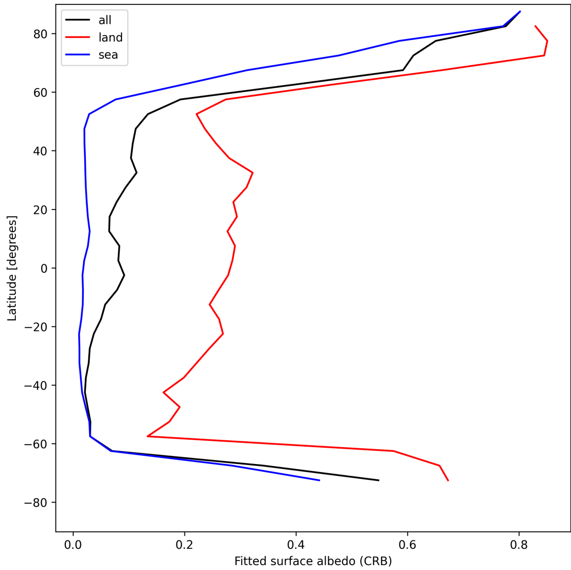
Figure 30: Zonal average of “Fitted surface albedo (CRB)” for 2025-05-10 to 2025-05-12.
