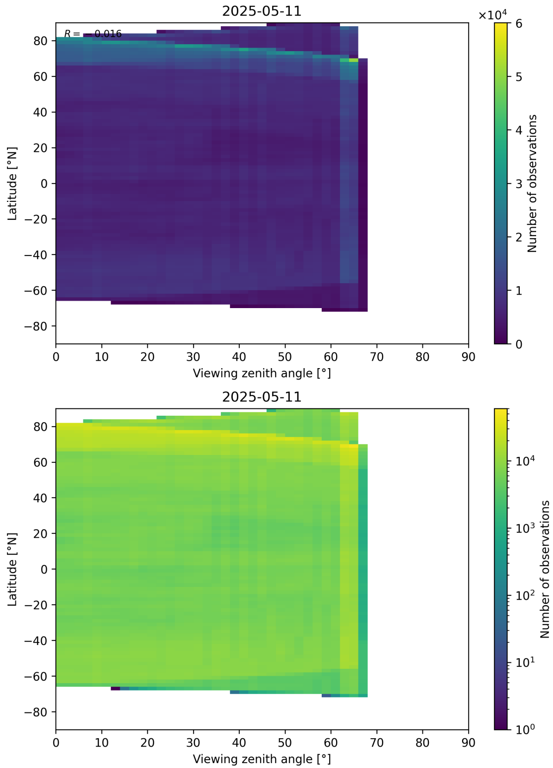
Figure 113: Scatter density plot of “Viewing zenith angle” against “Latitude” for 2025-05-10 to 2025-05-12.
