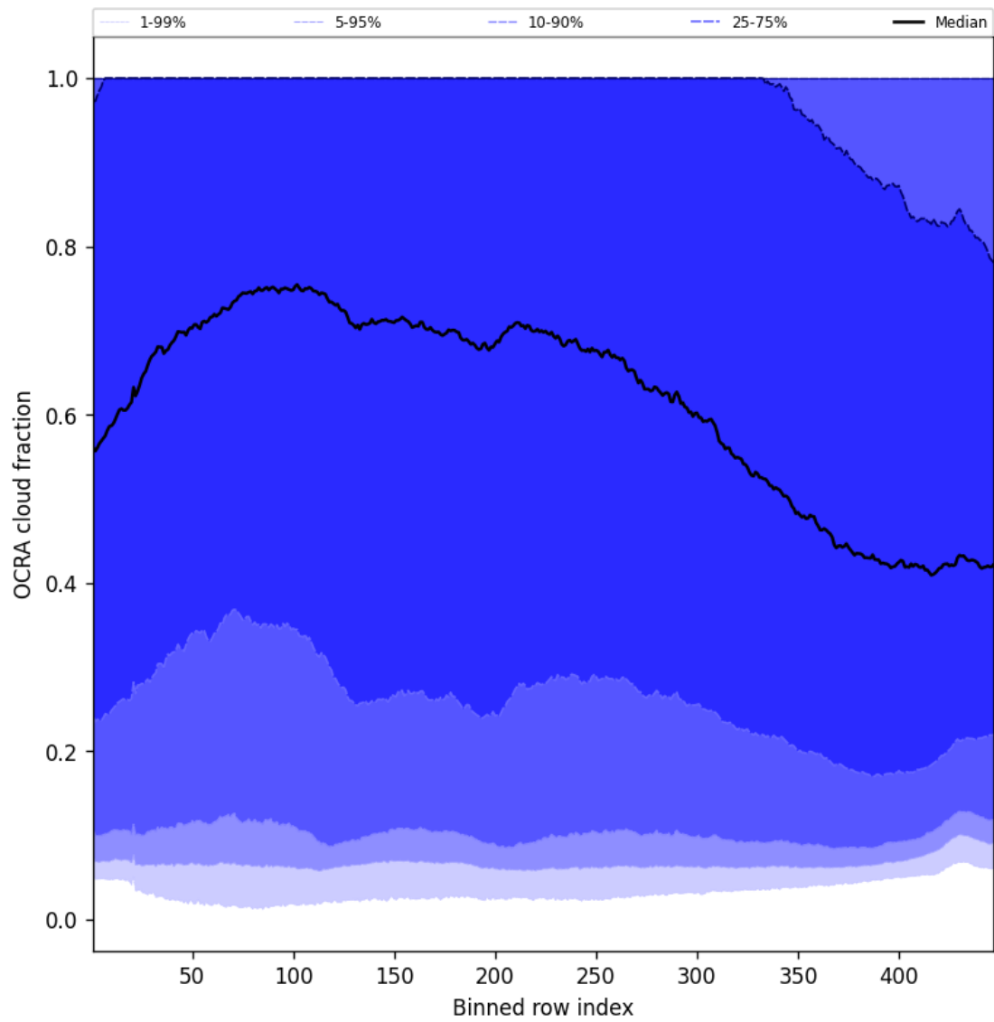
Figure 66: Along track statistics of “OCRA cloud fraction” for 2025-05-10 to 2025-05-12
