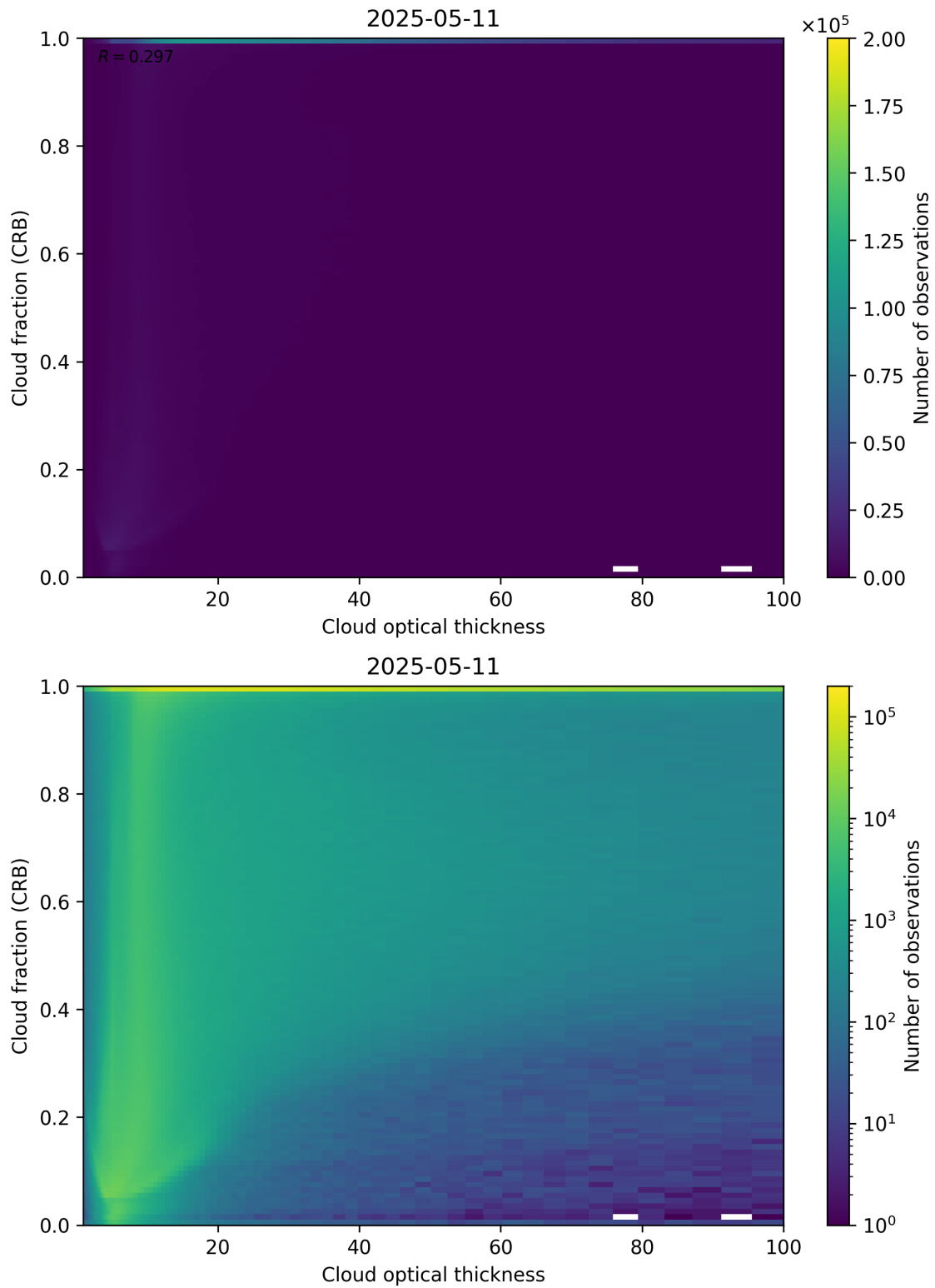
Figure 84: Scatter density plot of “Cloud optical thickness” against “Cloud fraction (CRB)” for 2025-05-10 to 2025-05-12.
