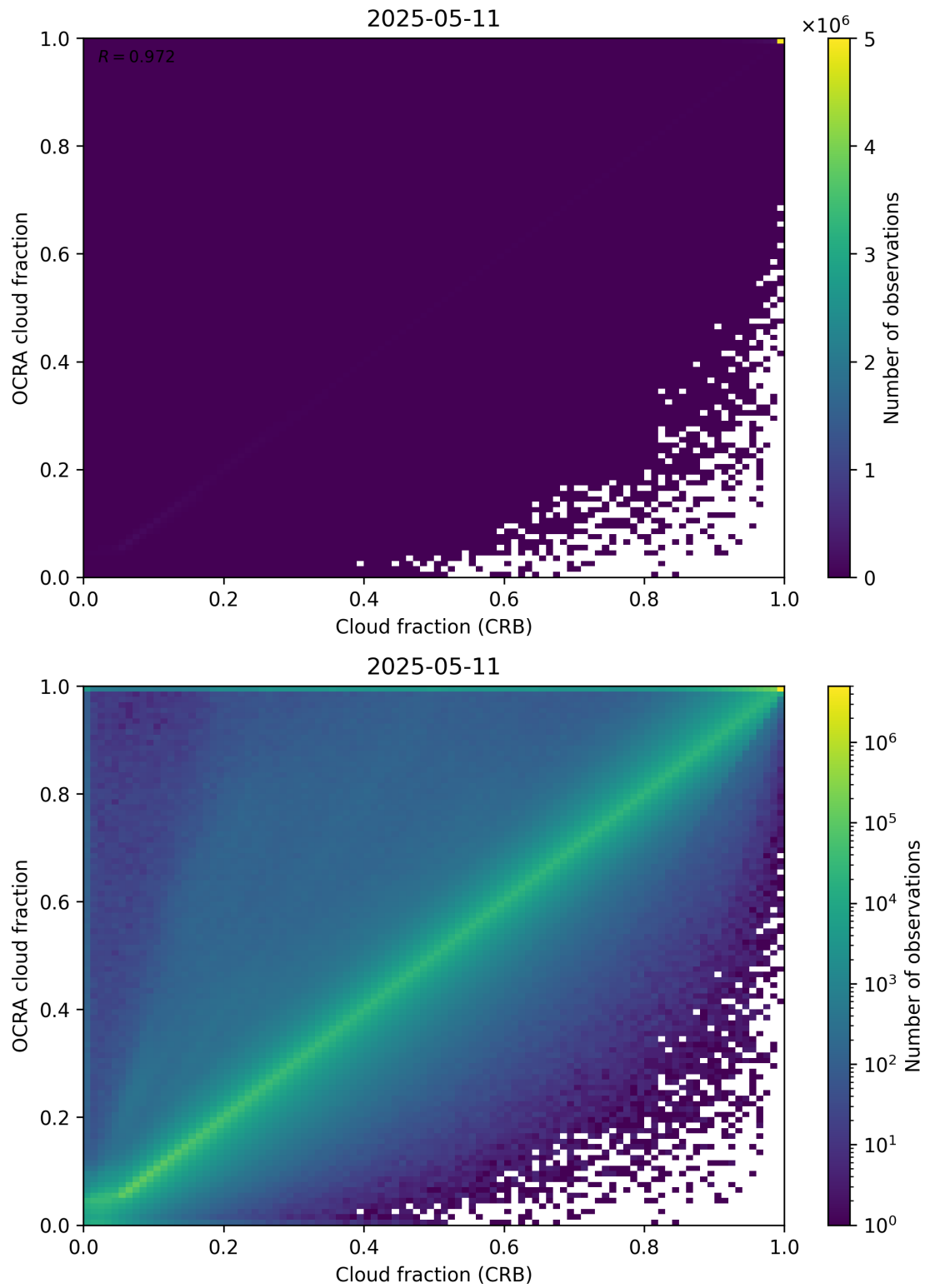
Figure 78: Scatter density plot of “Cloud fraction (CRB)” against “OCRA cloud fraction” for 2025-05-10 to 2025-05-12.
