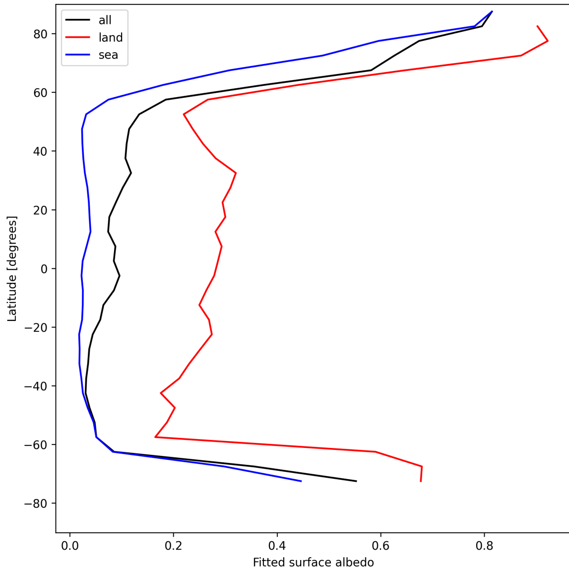
Figure 29: Zonal average of “Fitted surface albedo” for 2025-05-10 to 2025-05-12.
