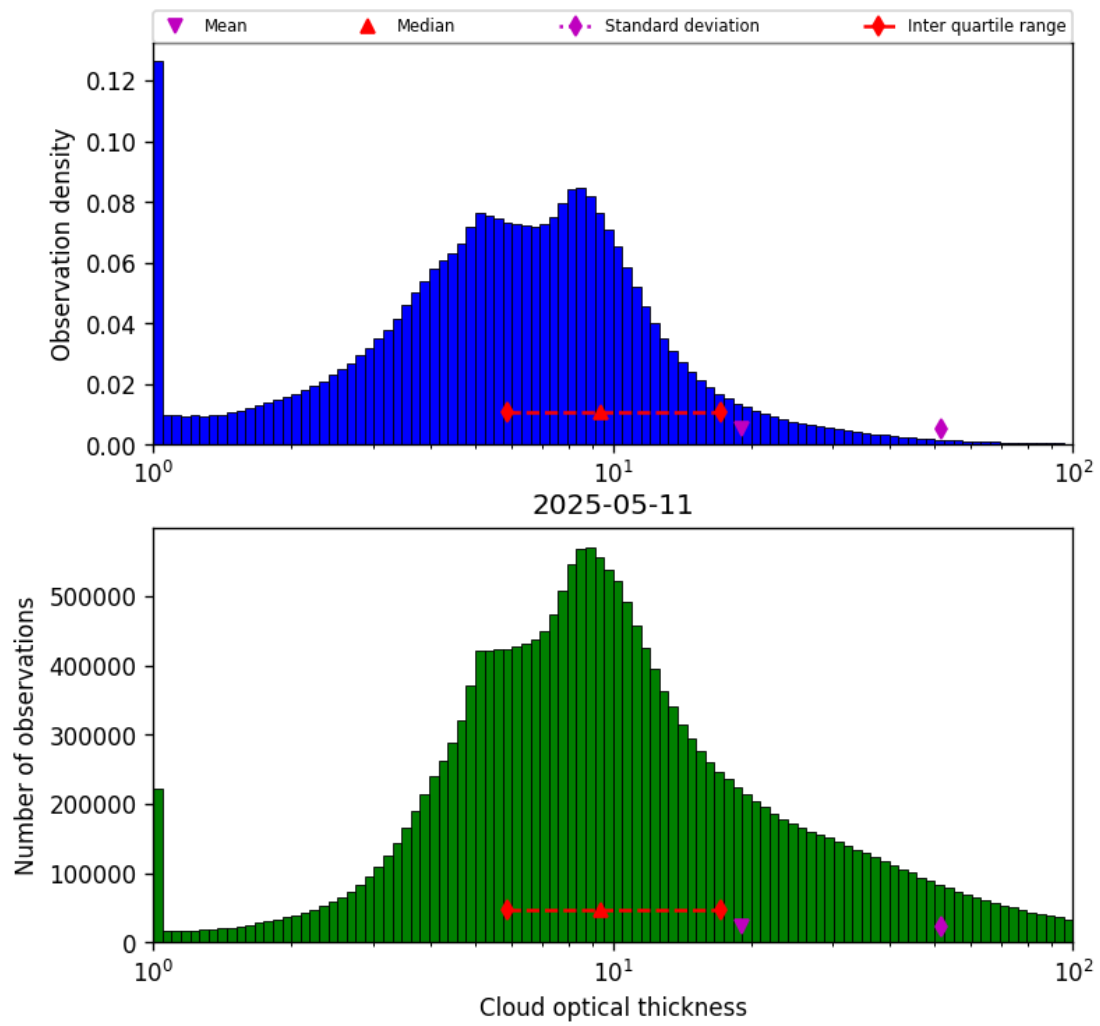
Figure 41: Histogram of “Cloud optical thickness” for 2025-05-10 to 2025-05-12
