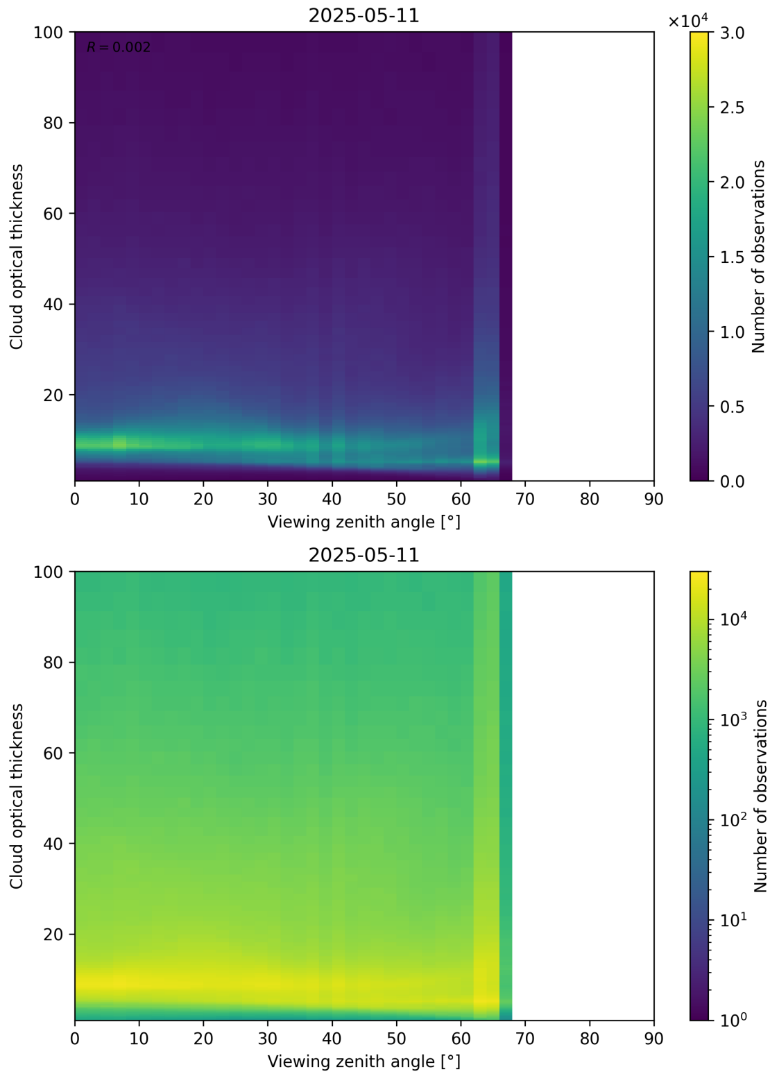
Figure 111: Scatter density plot of “Viewing zenith angle” against “Cloud optical thickness” for 2025-05-10 to 2025-05-12.
