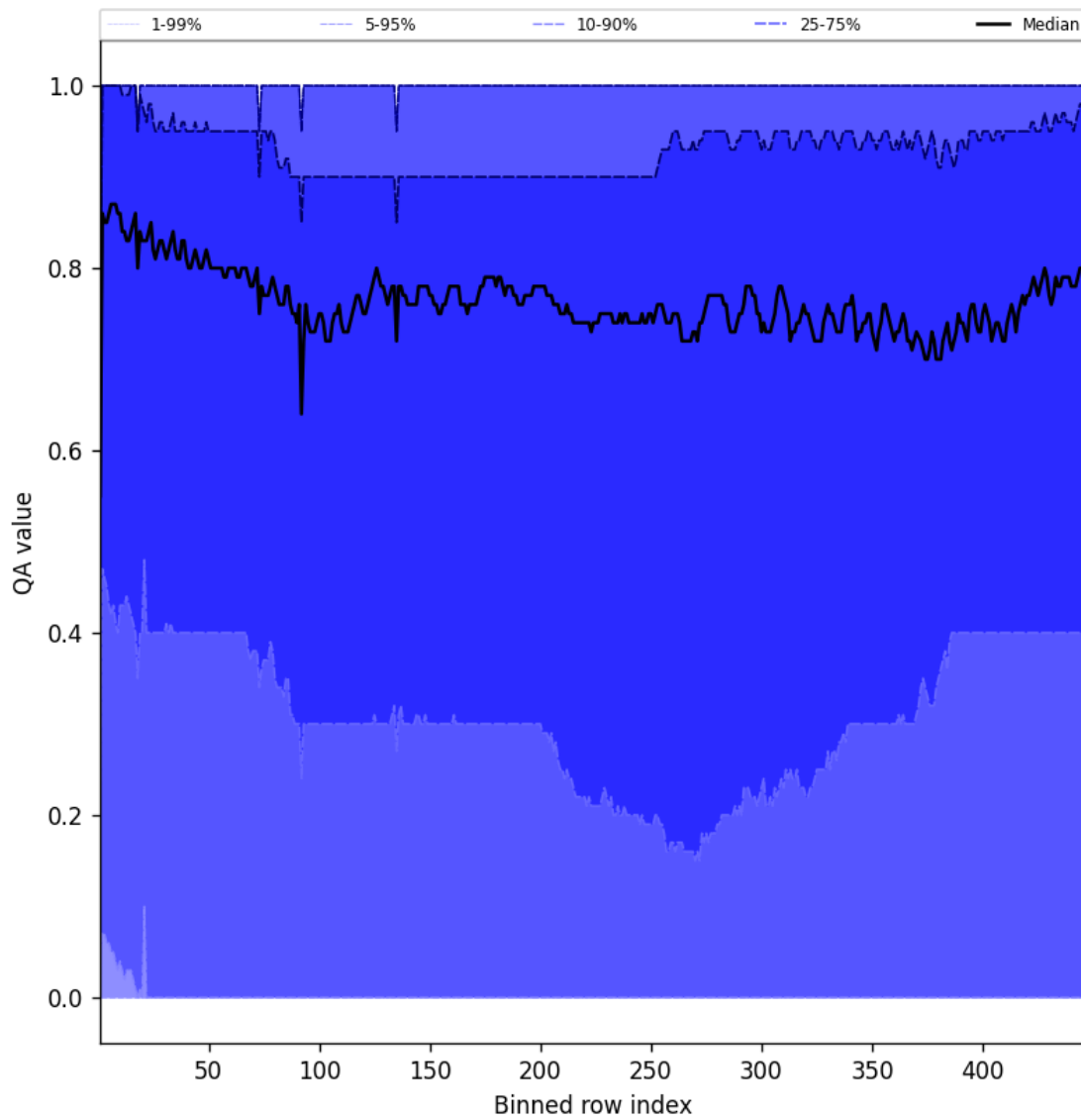
Figure 54: Along track statistics of “QA value” for 2025-05-10 to 2025-05-12
