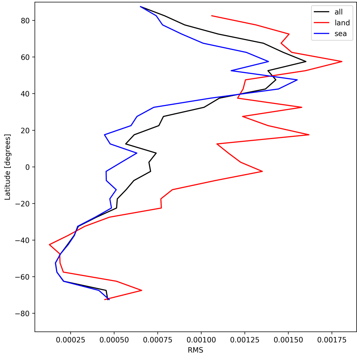
Figure 31: Zonal average of “RMS” for 2025-05-10 to 2025-05-12.
