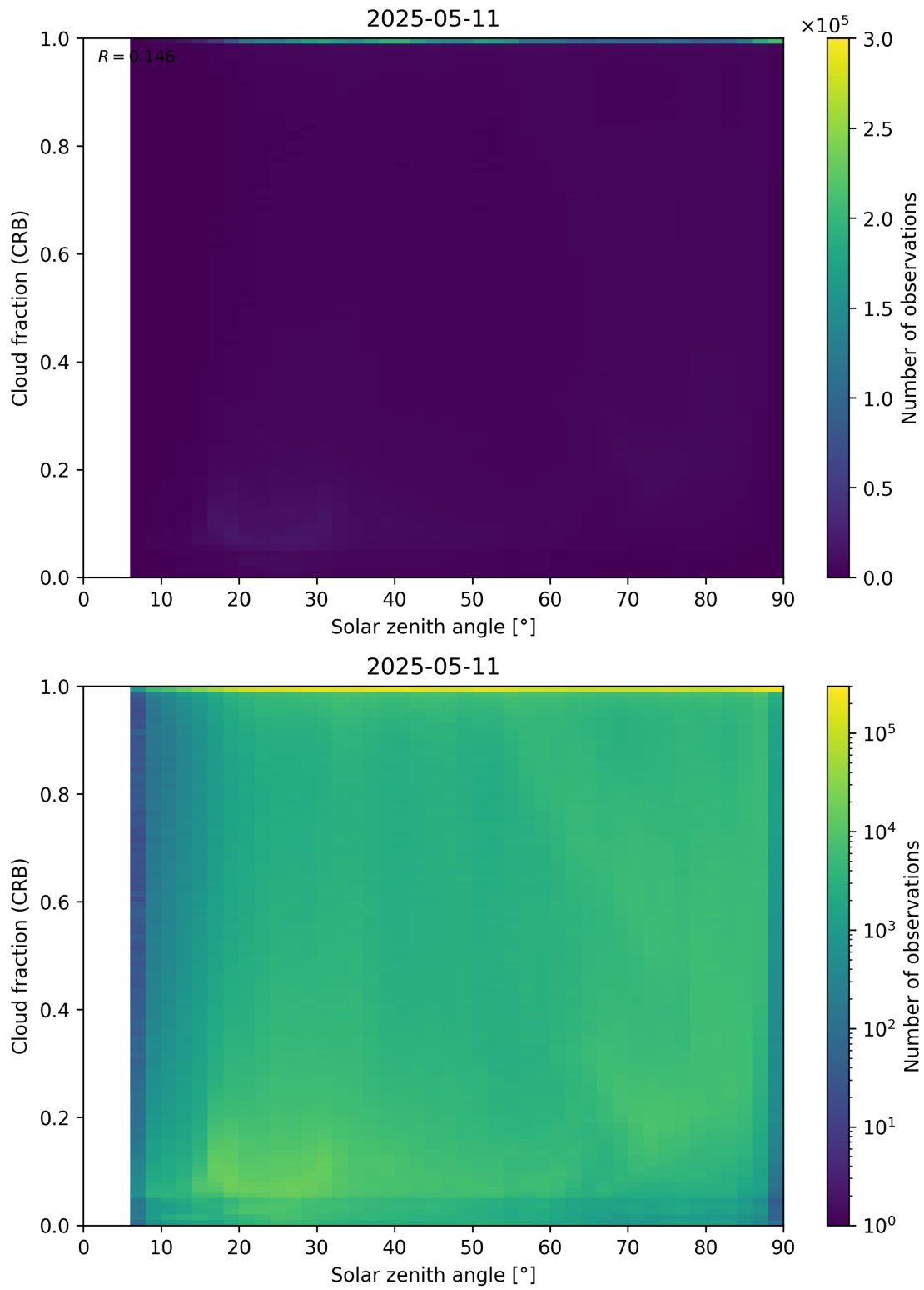
Figure 101: Scatter density plot of “Solar zenith angle” against “Cloud fraction (CRB)” for 2025-05-10 to 2025-05-12.
