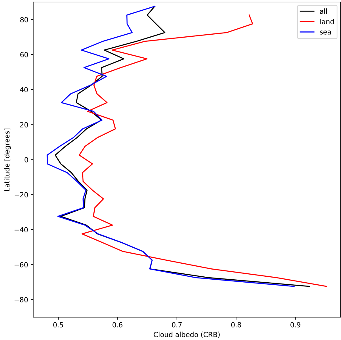
Figure 28: Zonal average of “Cloud albedo (CRB)” for 2025-05-10 to 2025-05-12.
