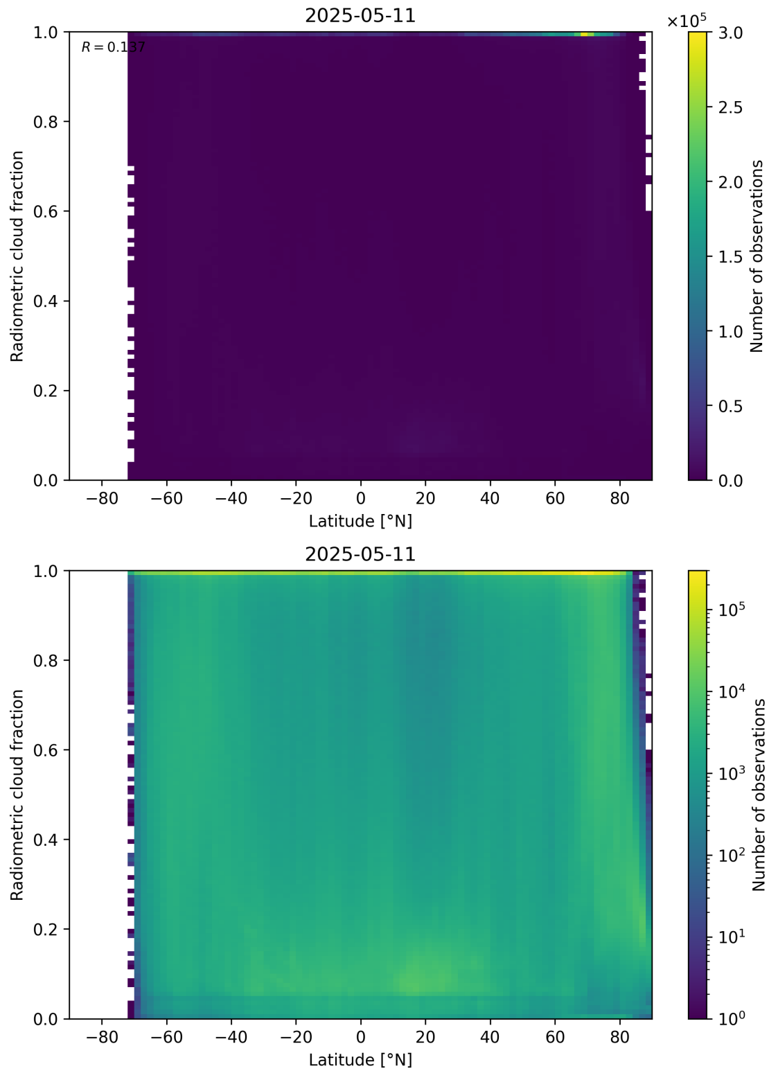
Figure 92: Scatter density plot of “Latitude” against “Radiometric cloud fraction” for 2025-05-10 to 2025-05-12.
