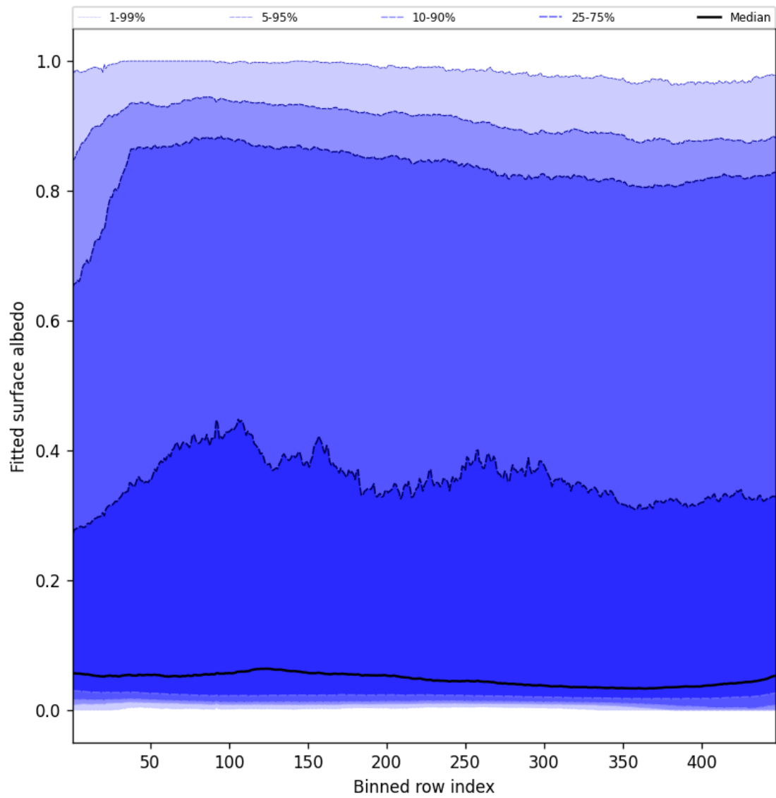
Figure 61: Along track statistics of “Fitted surface albedo” for 2025-05-10 to 2025-05-12
