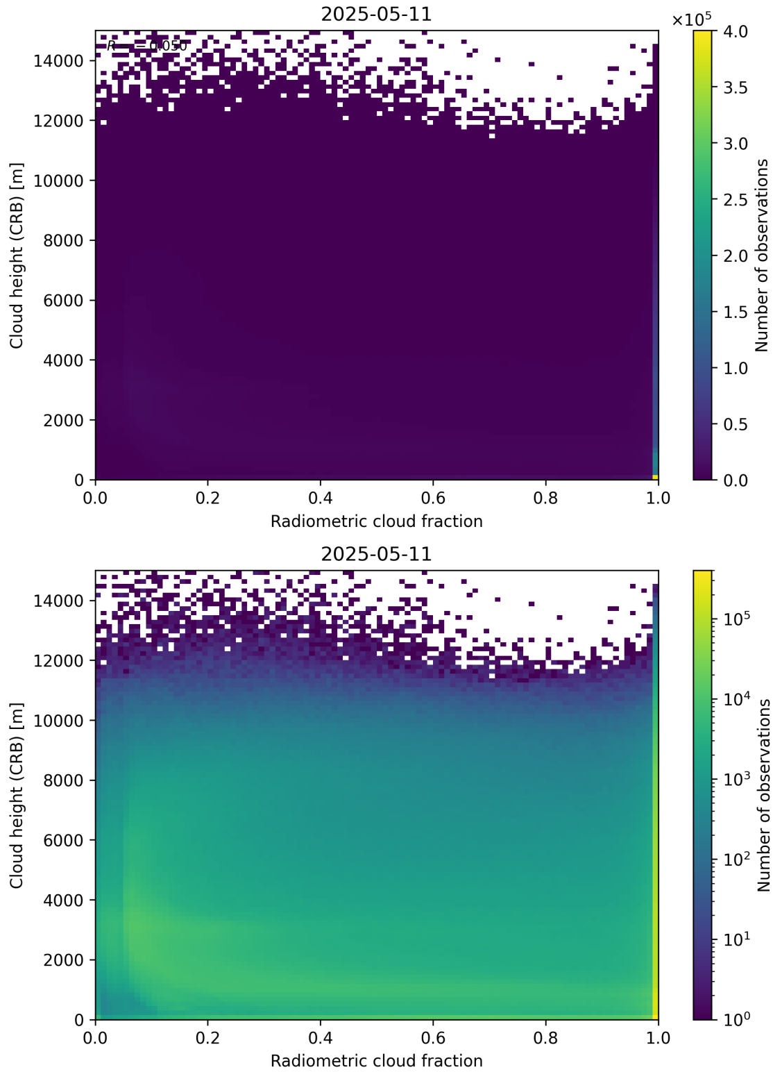
Figure 74: Scatter density plot of “Radiometric cloud fraction” against “Cloud height (CRB)” for 2025-05-10 to 2025-05-12.
