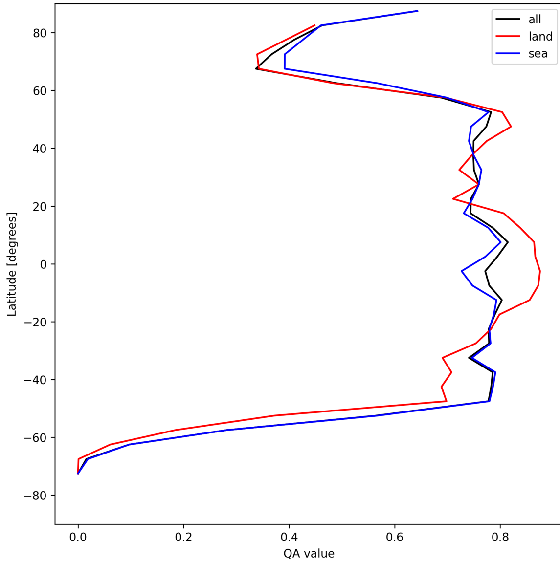
Figure 22: Zonal average of “QA value” for 2025-05-10 to 2025-05-12.
