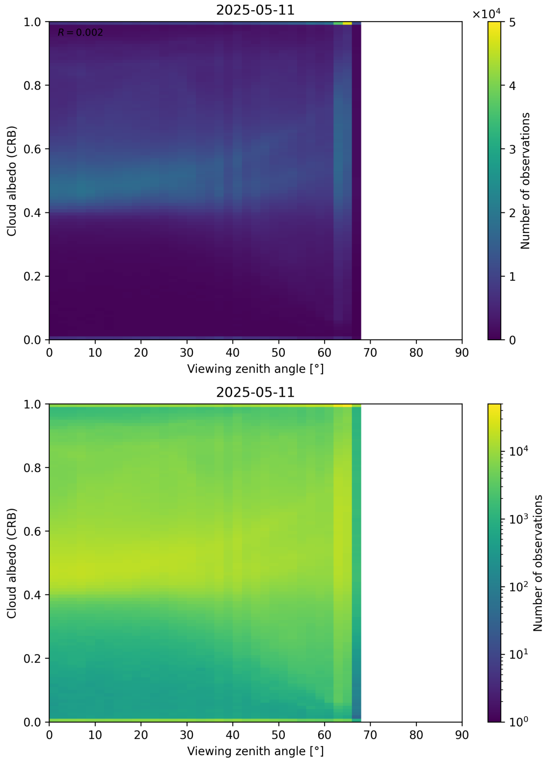
Figure 106: Scatter density plot of “Viewing zenith angle” against “Cloud albedo (CRB)” for 2025-05-10 to 2025-05-12.
