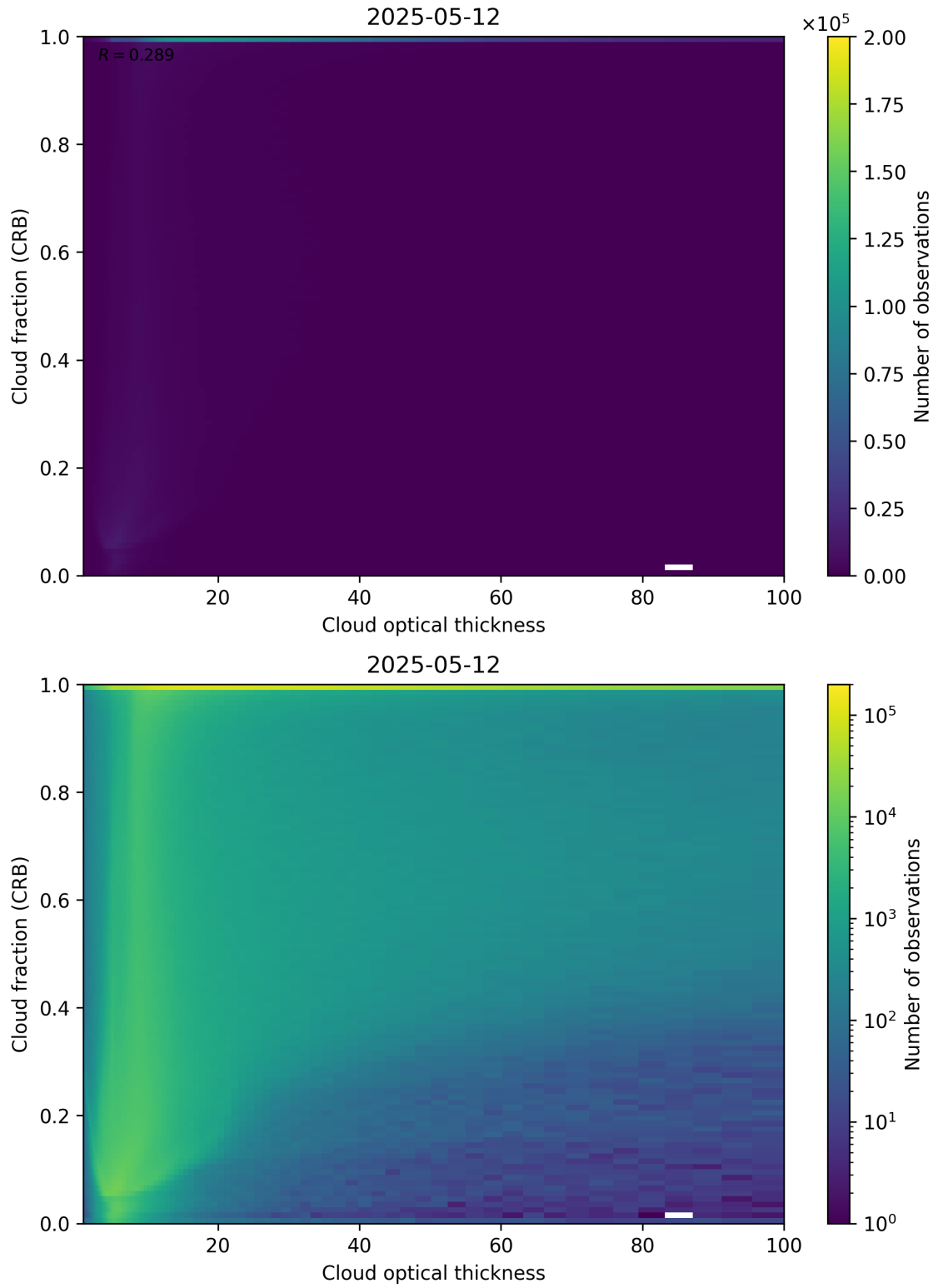
Figure 84: Scatter density plot of “Cloud optical thickness” against “Cloud fraction (CRB)” for 2025-05-11 to 2025-05-13.
