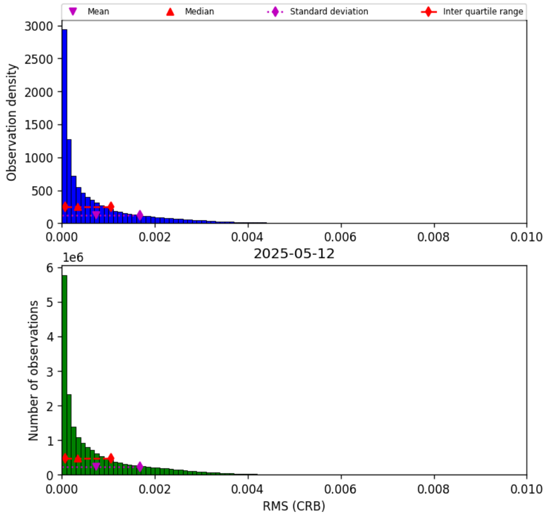
Figure 48: Histogram of “RMS (CRB)” for 2025-05-11 to 2025-05-13
