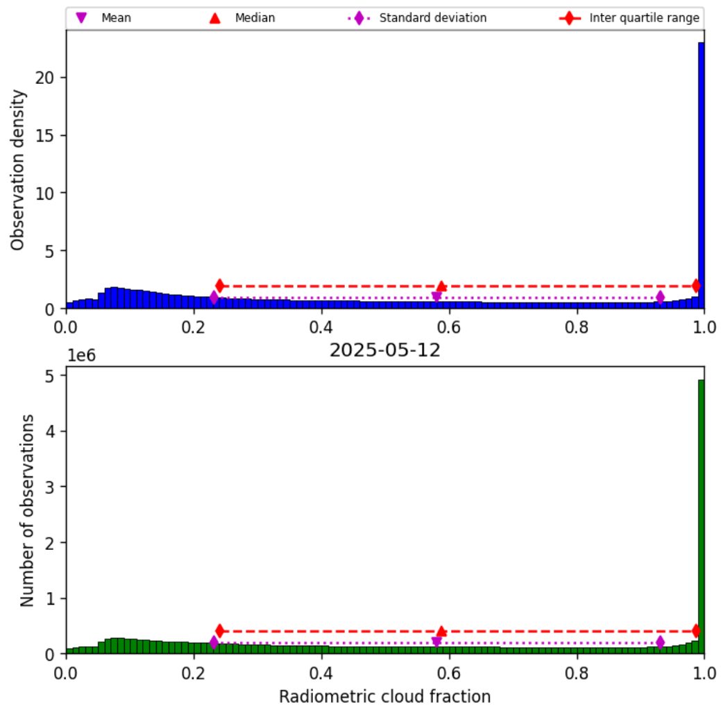
Figure 39: Histogram of “Radiometric cloud fraction” for 2025-05-11 to 2025-05-13
