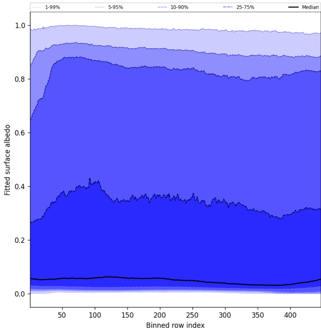
Figure 61: Along track statistics of “Fitted surface albedo” for 2025-05-11 to 2025-05-13
