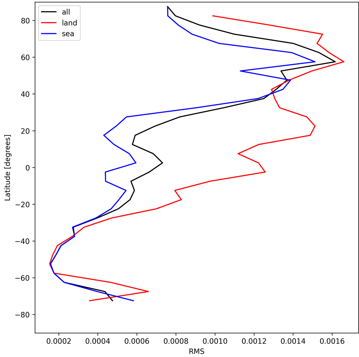
Figure 31: Zonal average of “RMS” for 2025-05-11 to 2025-05-13.
