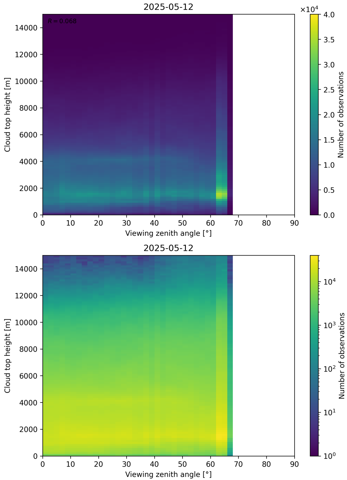
Figure 112: Scatter density plot of “Viewing zenith angle” against “Cloud top height” for 2025-05-11 to 2025-05-13.
