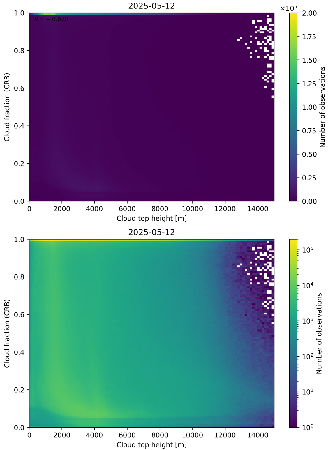
Figure 88: Scatter density plot of “Cloud top height” against “Cloud fraction (CRB)” for 2025-05-11 to 2025-05-13.
