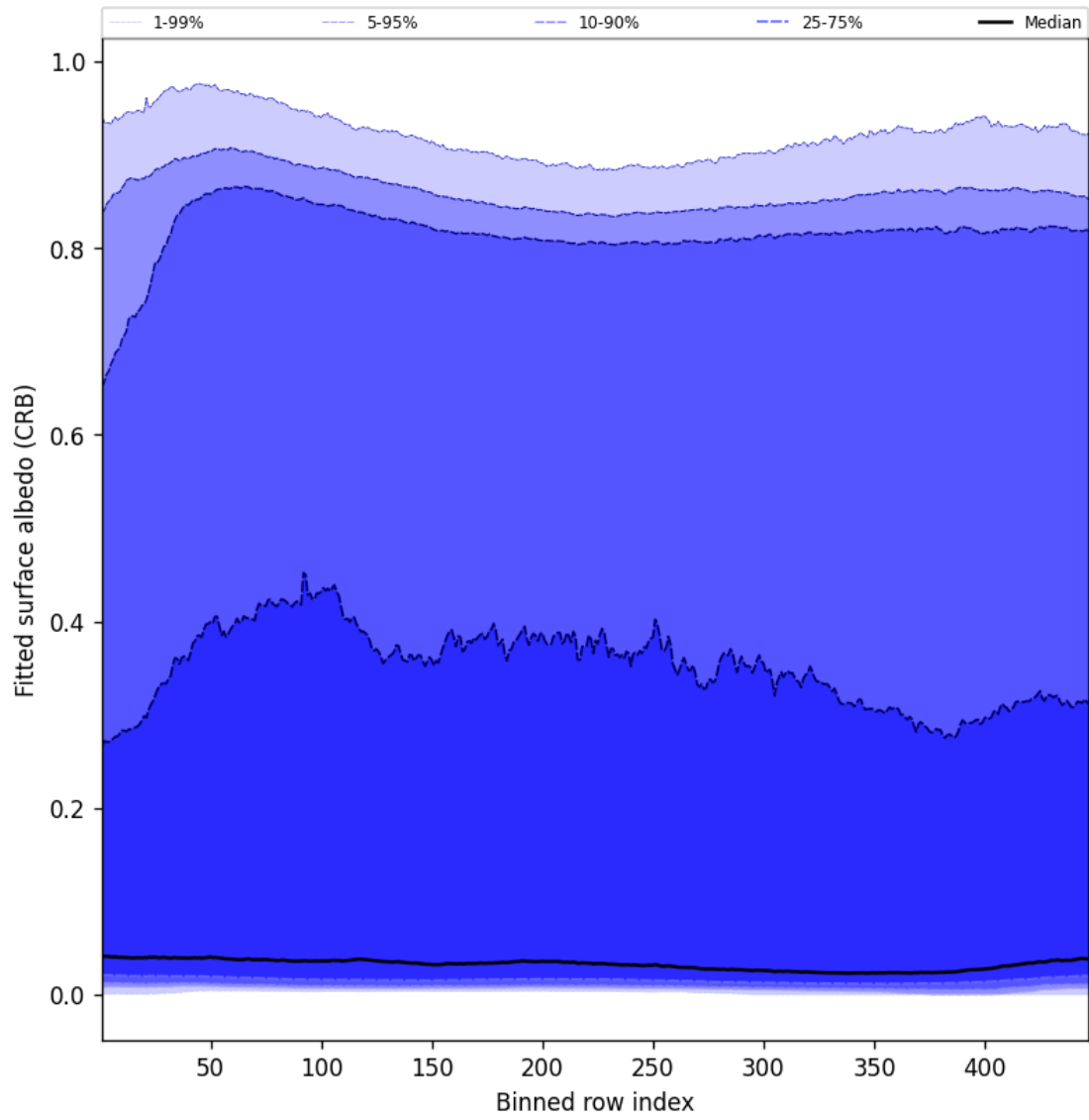
Figure 62: Along track statistics of “Fitted surface albedo (CRB)” for 2025-05-11 to 2025-05-13
