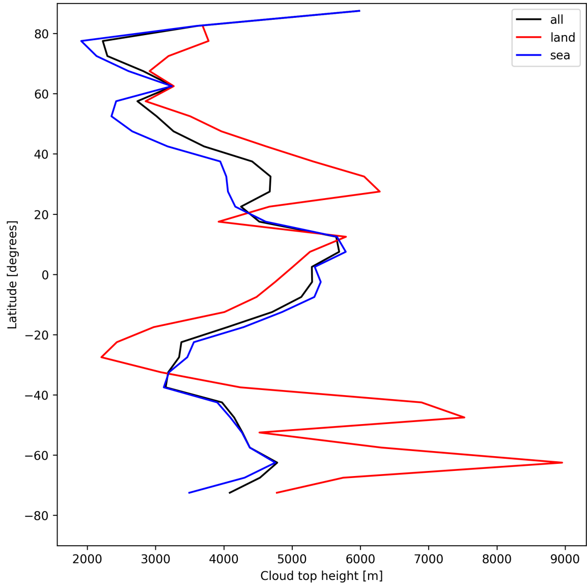
Figure 24: Zonal average of “Cloud top height” for 2025-05-11 to 2025-05-13.
