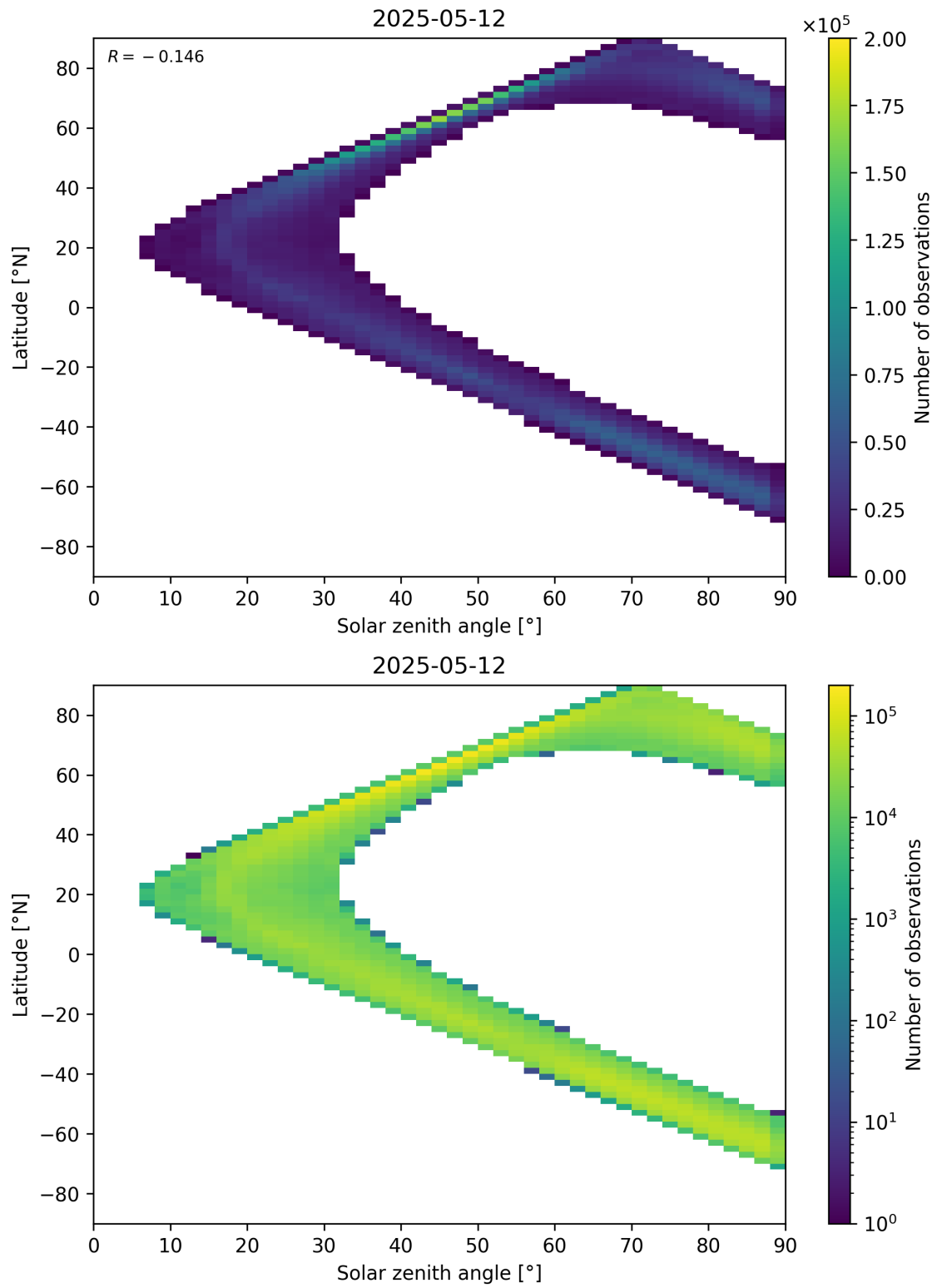
Figure 105: Scatter density plot of “Solar zenith angle” against “Latitude” for 2025-05-11 to 2025-05-13.
