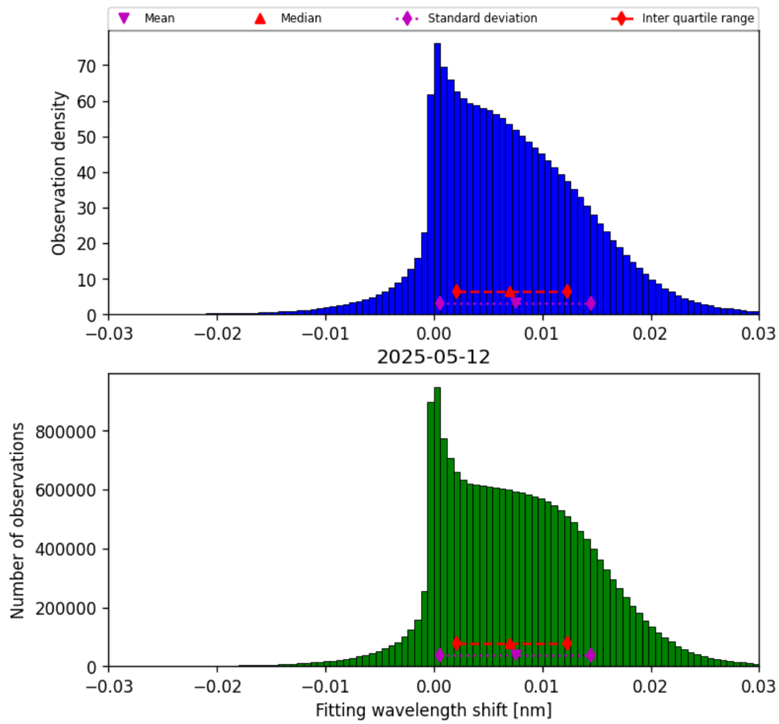
Figure 49: Histogram of “Fitting wavelength shift” for 2025-05-11 to 2025-05-13
