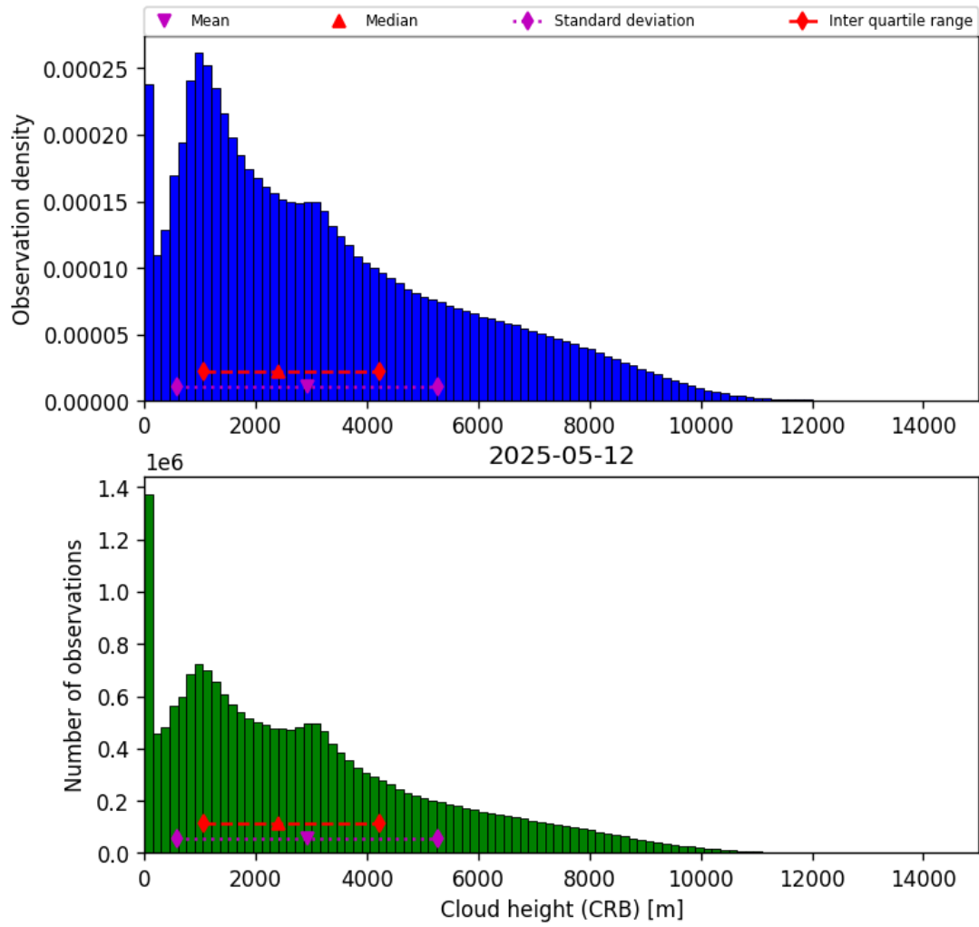
Figure 43: Histogram of “Cloud height (CRB)” for 2025-05-11 to 2025-05-13
