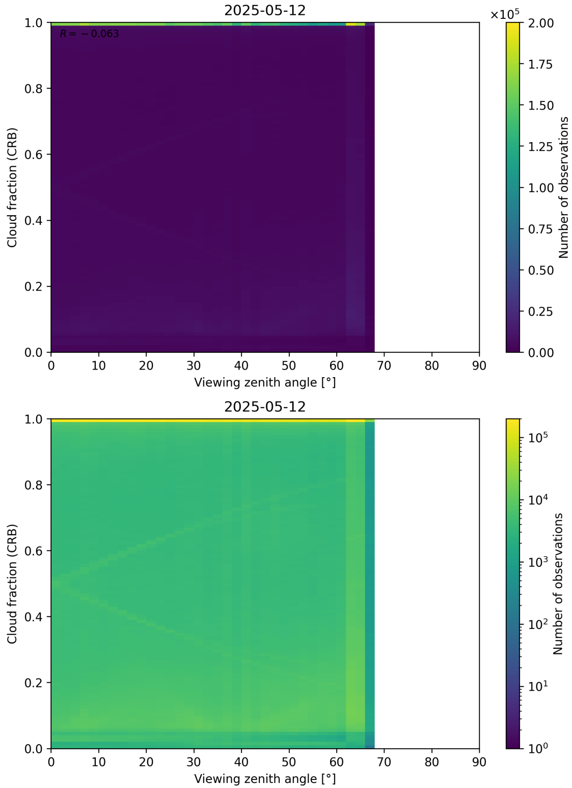
Figure 109: Scatter density plot of “Viewing zenith angle” against “Cloud fraction (CRB)” for 2025-05-11 to 2025-05-13.
