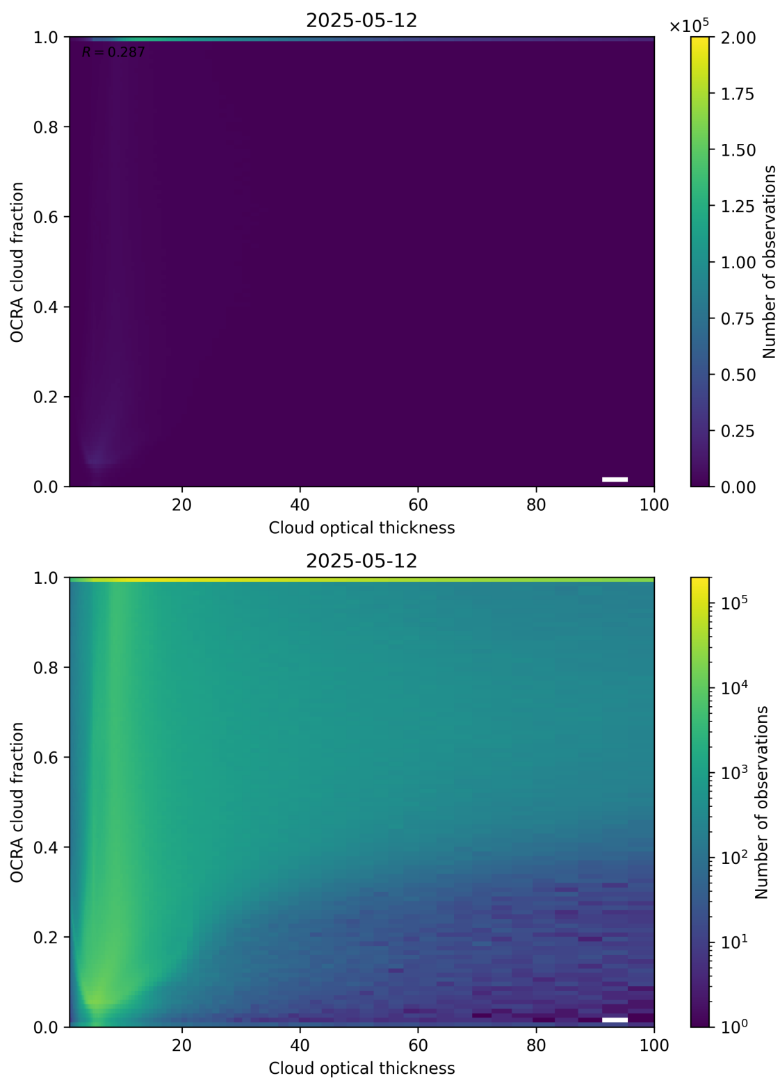
Figure 83: Scatter density plot of “Cloud optical thickness” against “OCRA cloud fraction” for 2025-05-11 to 2025-05-13.
