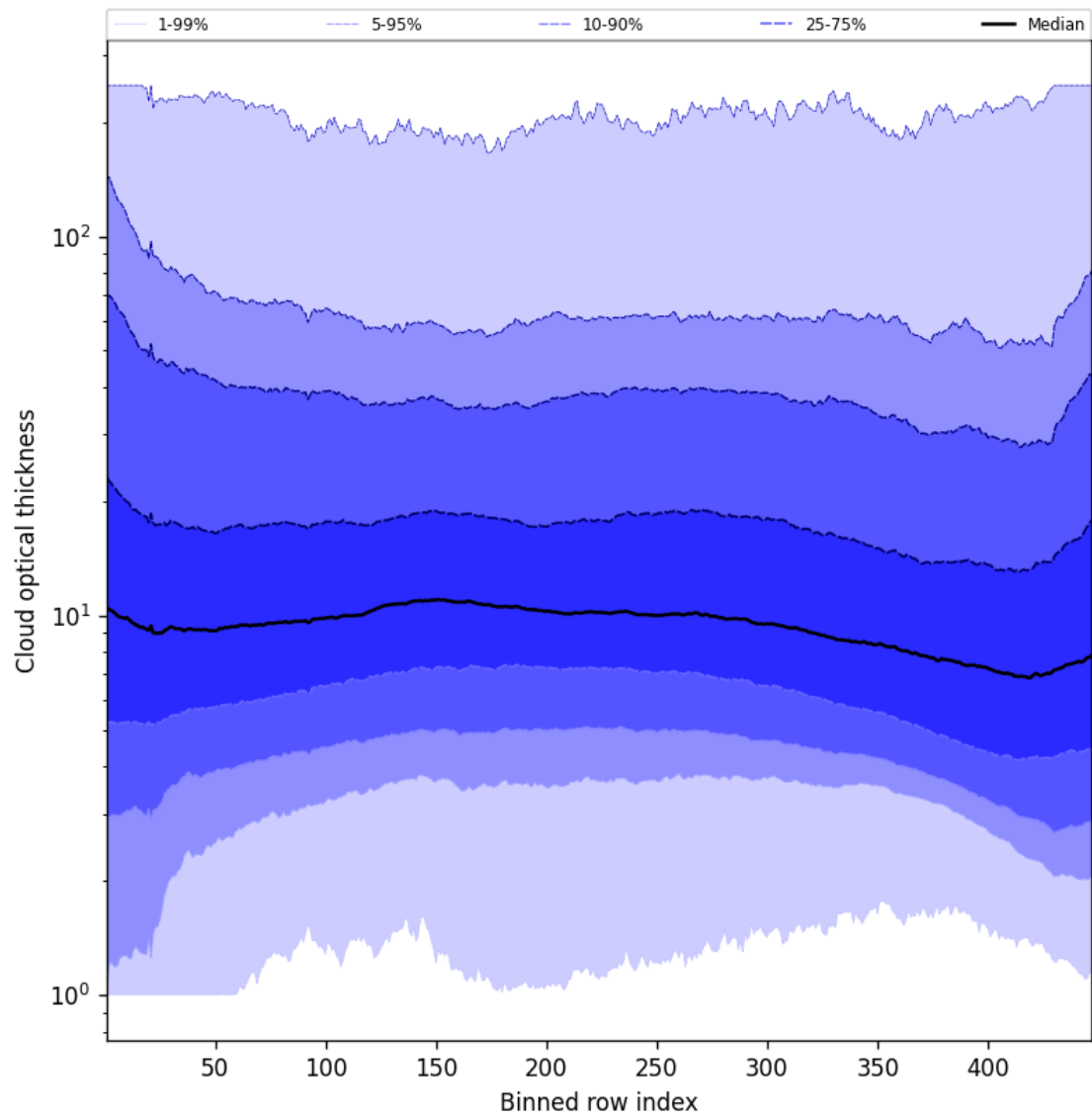
Figure 57: Along track statistics of “Cloud optical thickness” for 2025-05-11 to 2025-05-13
