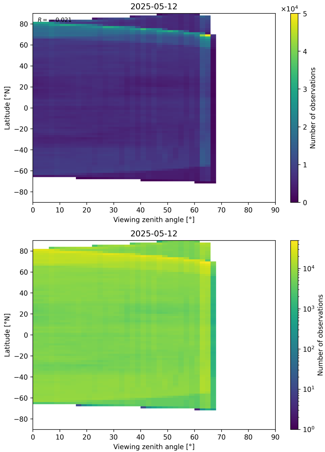
Figure 113: Scatter density plot of “Viewing zenith angle” against “Latitude” for 2025-05-11 to 2025-05-13.
