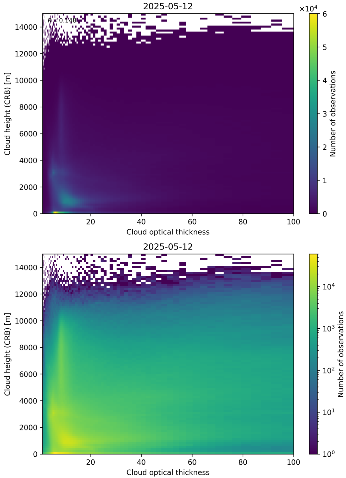
Figure 85: Scatter density plot of “Cloud optical thickness” against “Cloud height (CRB)” for 2025-05-11 to 2025-05-13.
