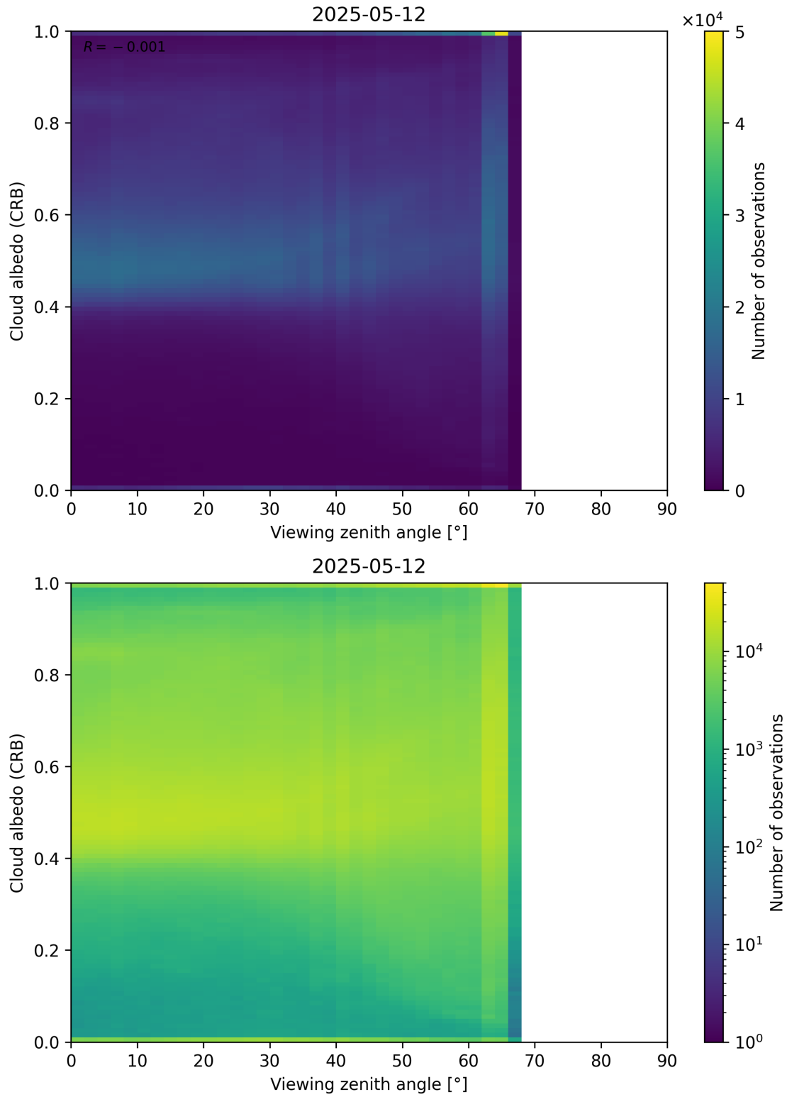
Figure 106: Scatter density plot of “Viewing zenith angle” against “Cloud albedo (CRB)” for 2025-05-11 to 2025-05-13.
