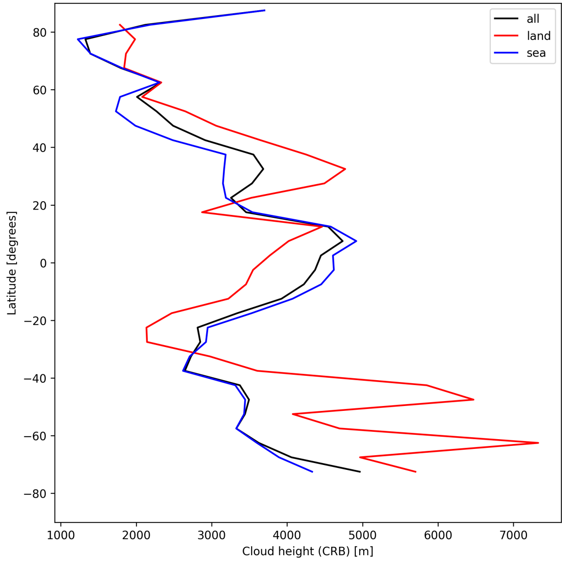
Figure 27: Zonal average of “Cloud height (CRB)” for 2025-05-11 to 2025-05-13.
