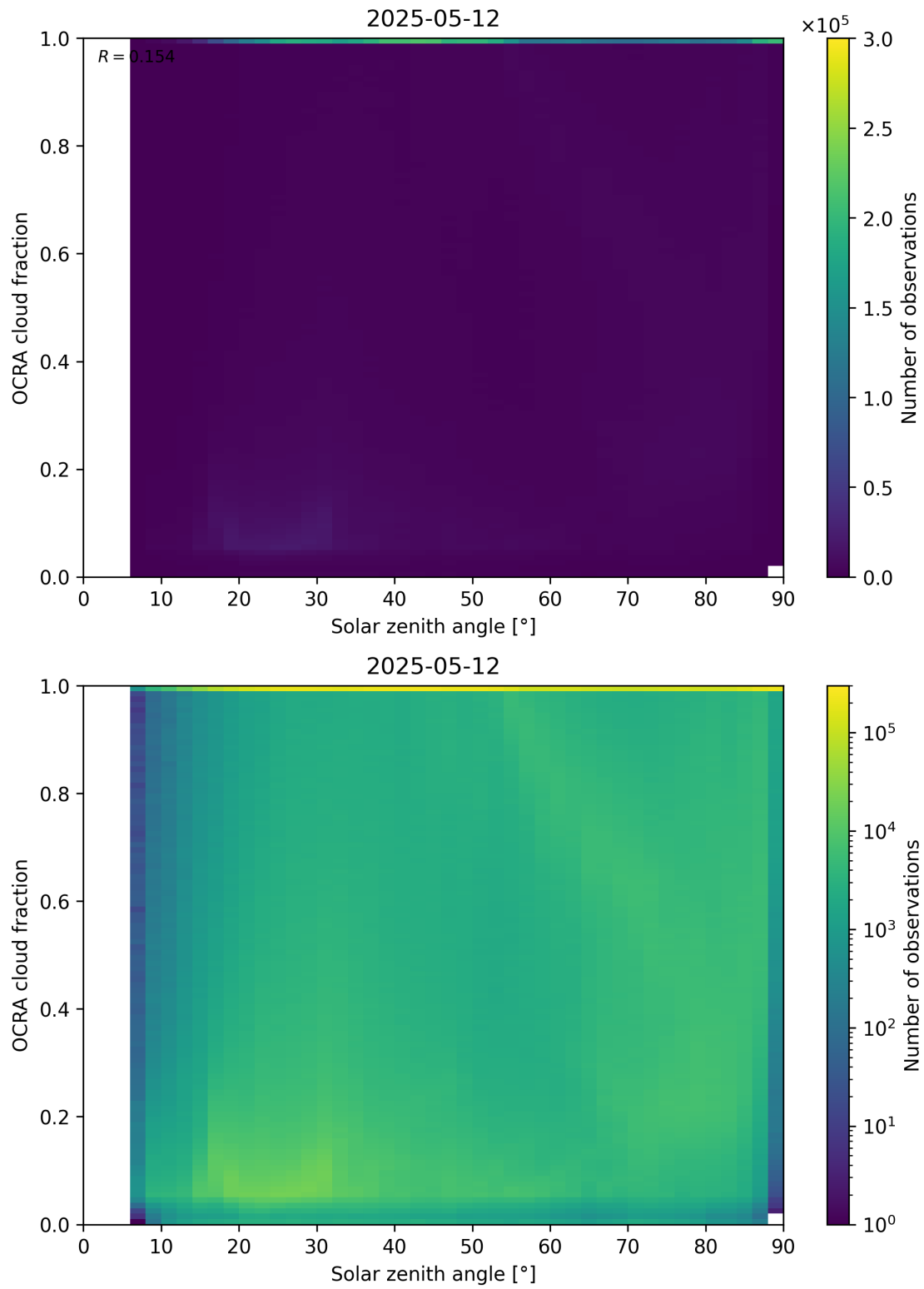
Figure 100: Scatter density plot of “Solar zenith angle” against “OCRA cloud fraction” for 2025-05-11 to 2025-05-13.
