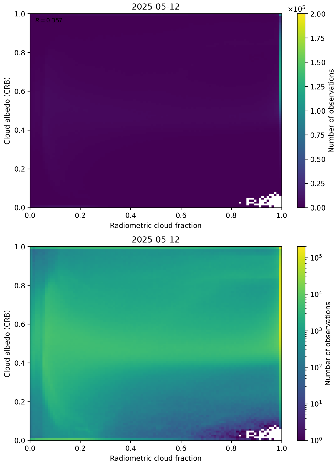
Figure 71: Scatter density plot of “Radiometric cloud fraction” against “Cloud albedo (CRB)” for 2025-05-11 to 2025-05-13.
