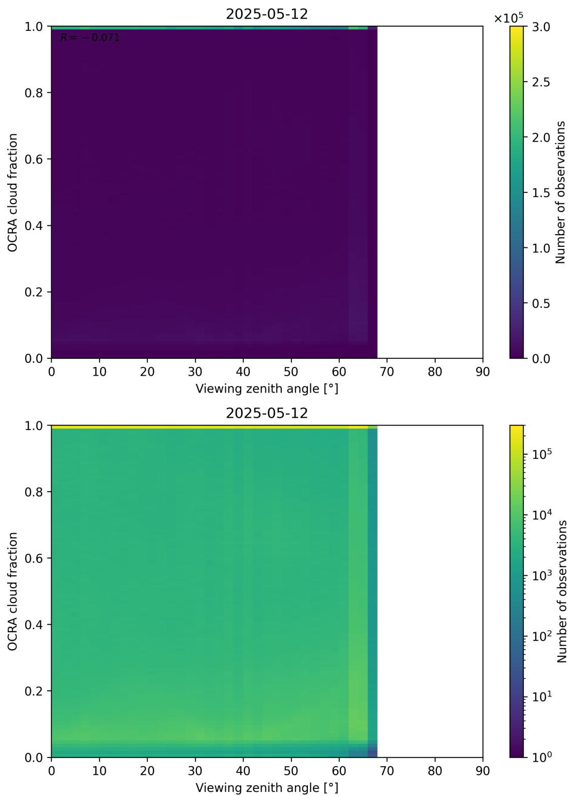
Figure 108: Scatter density plot of “Viewing zenith angle” against “OCRA cloud fraction” for 2025-05-11 to 2025-05-13.
