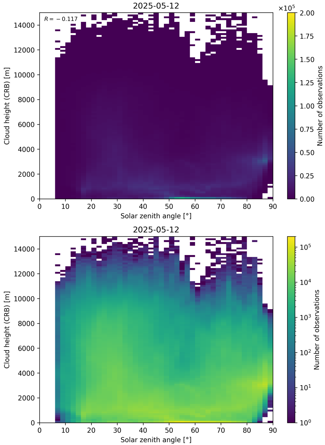
Figure 102: Scatter density plot of “Solar zenith angle” against “Cloud height (CRB)” for 2025-05-11 to 2025-05-13.
