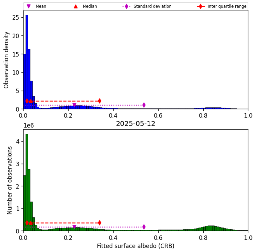
Figure 46: Histogram of “Fitted surface albedo (CRB)” for 2025-05-11 to 2025-05-13
