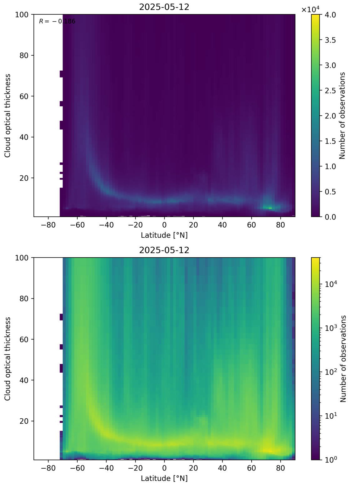
Figure 96: Scatter density plot of “Latitude” against “Cloud optical thickness” for 2025-05-11 to 2025-05-13.
