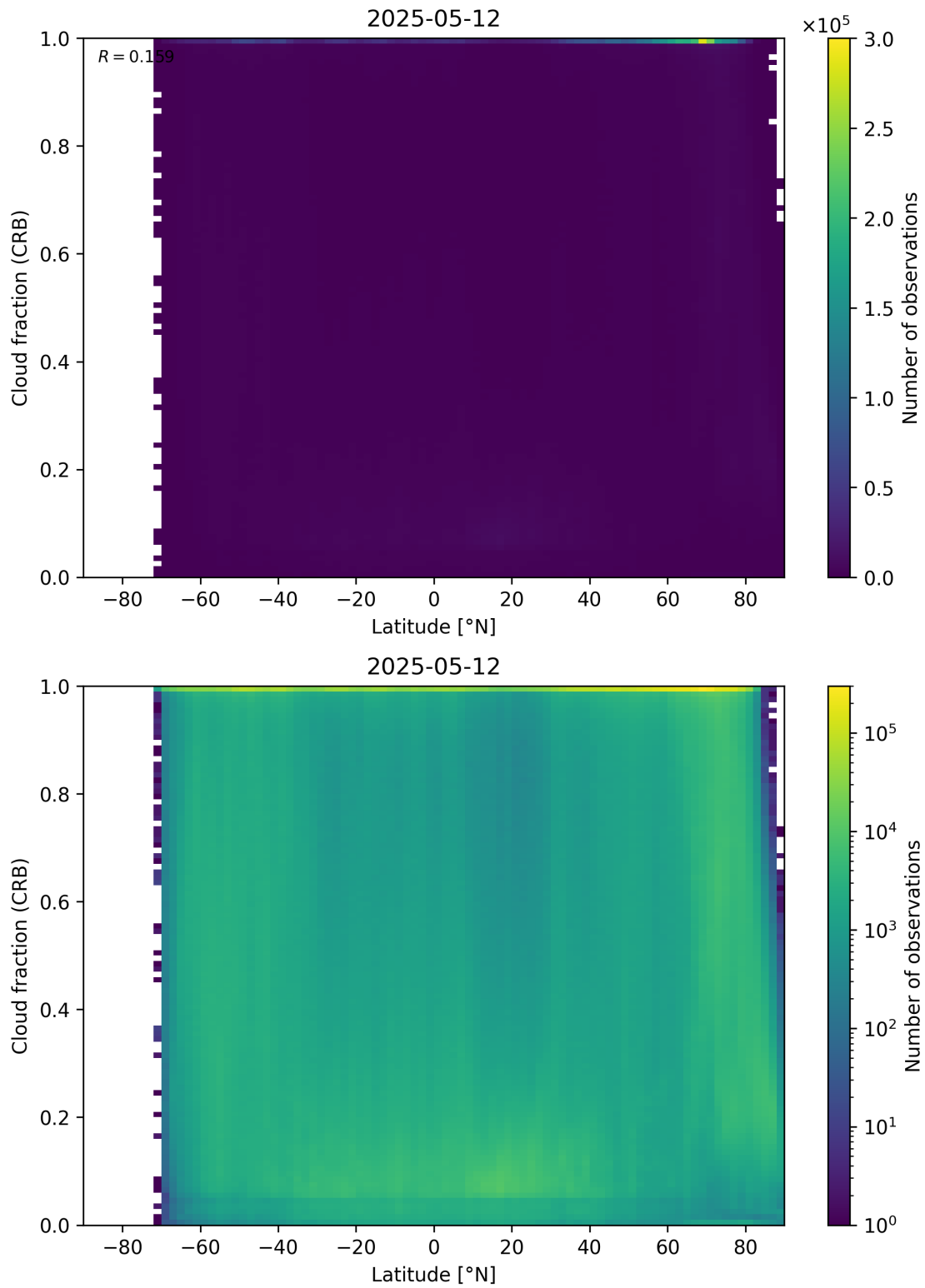
Figure 94: Scatter density plot of “Latitude” against “Cloud fraction (CRB)” for 2025-05-11 to 2025-05-13.
