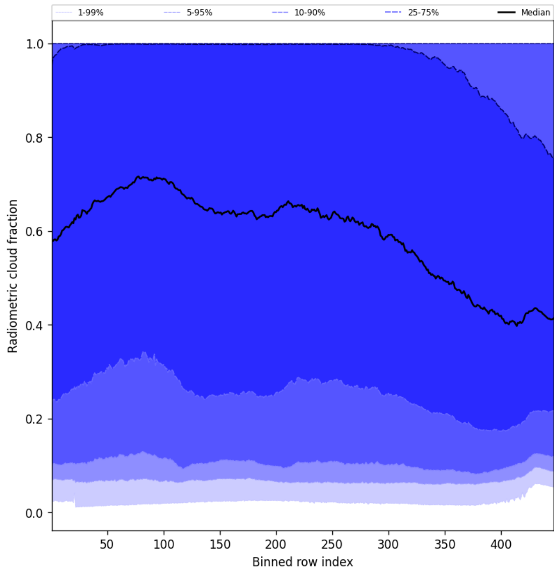
Figure 55: Along track statistics of “Radiometric cloud fraction” for 2025-05-11 to 2025-05-13
