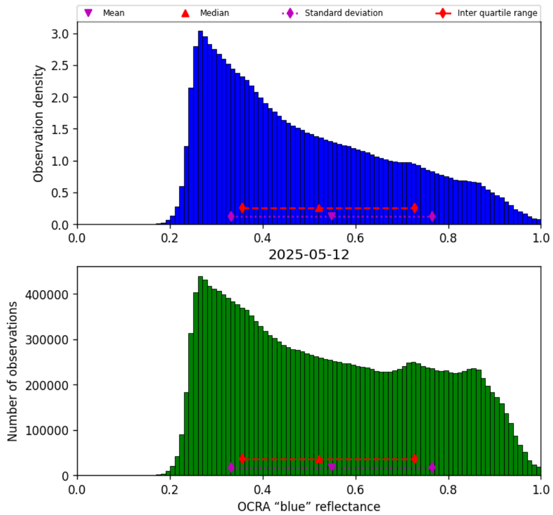
Figure 51: Histogram of “OCRA “blue” reflectance” for 2025-05-11 to 2025-05-13
