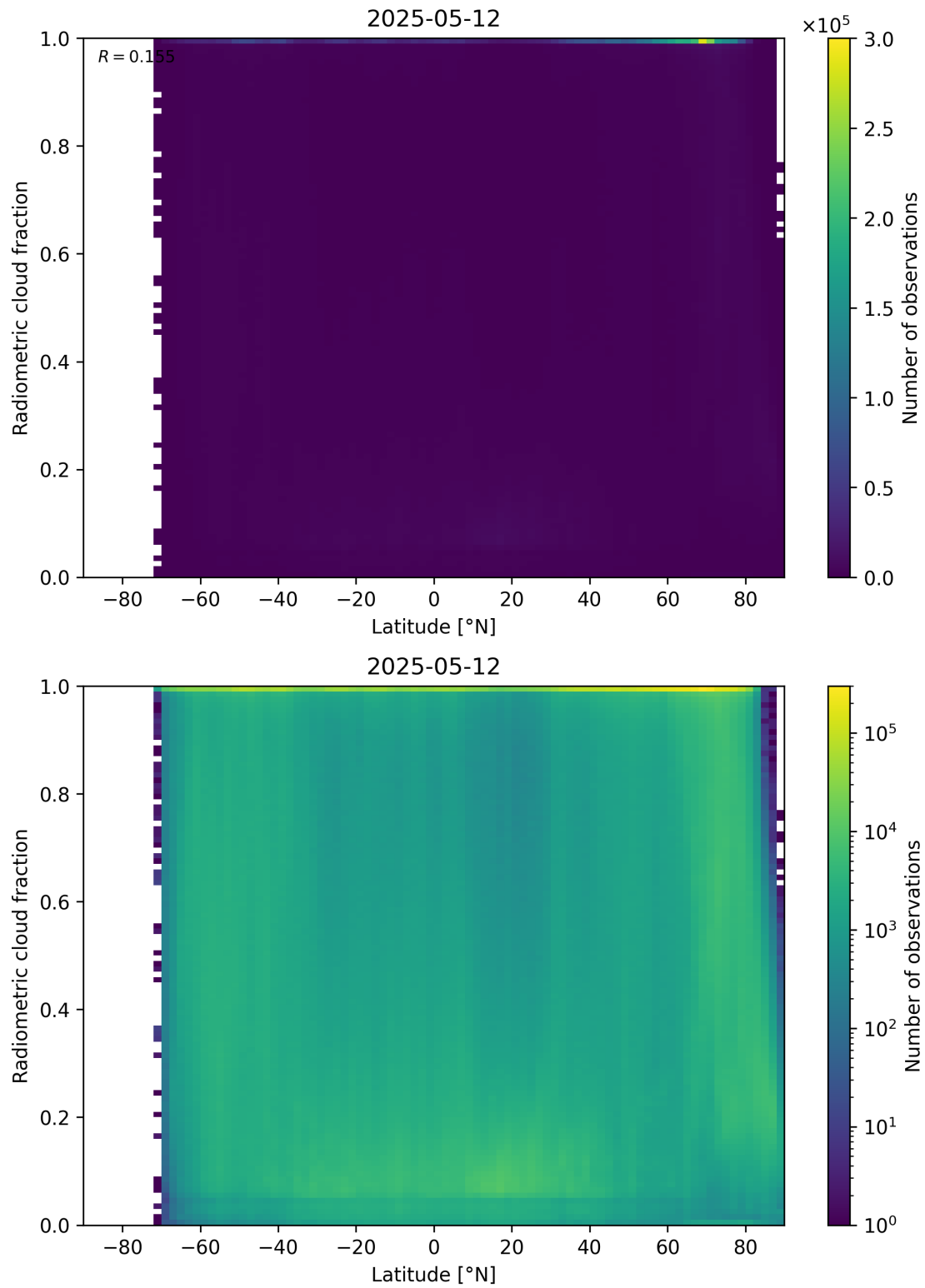
Figure 92: Scatter density plot of “Latitude” against “Radiometric cloud fraction” for 2025-05-11 to 2025-05-13.
