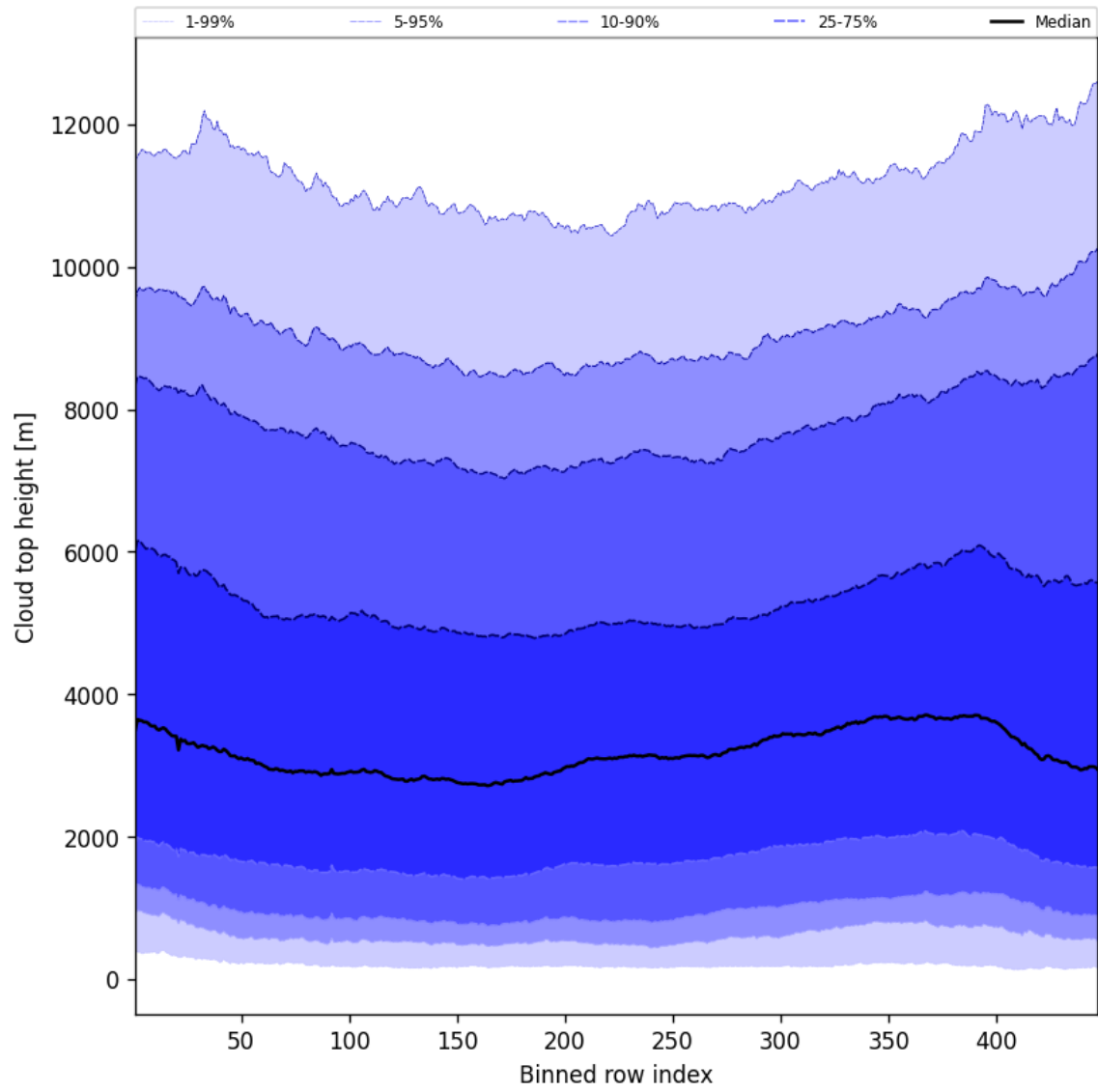
Figure 56: Along track statistics of “Cloud top height” for 2025-05-11 to 2025-05-13
