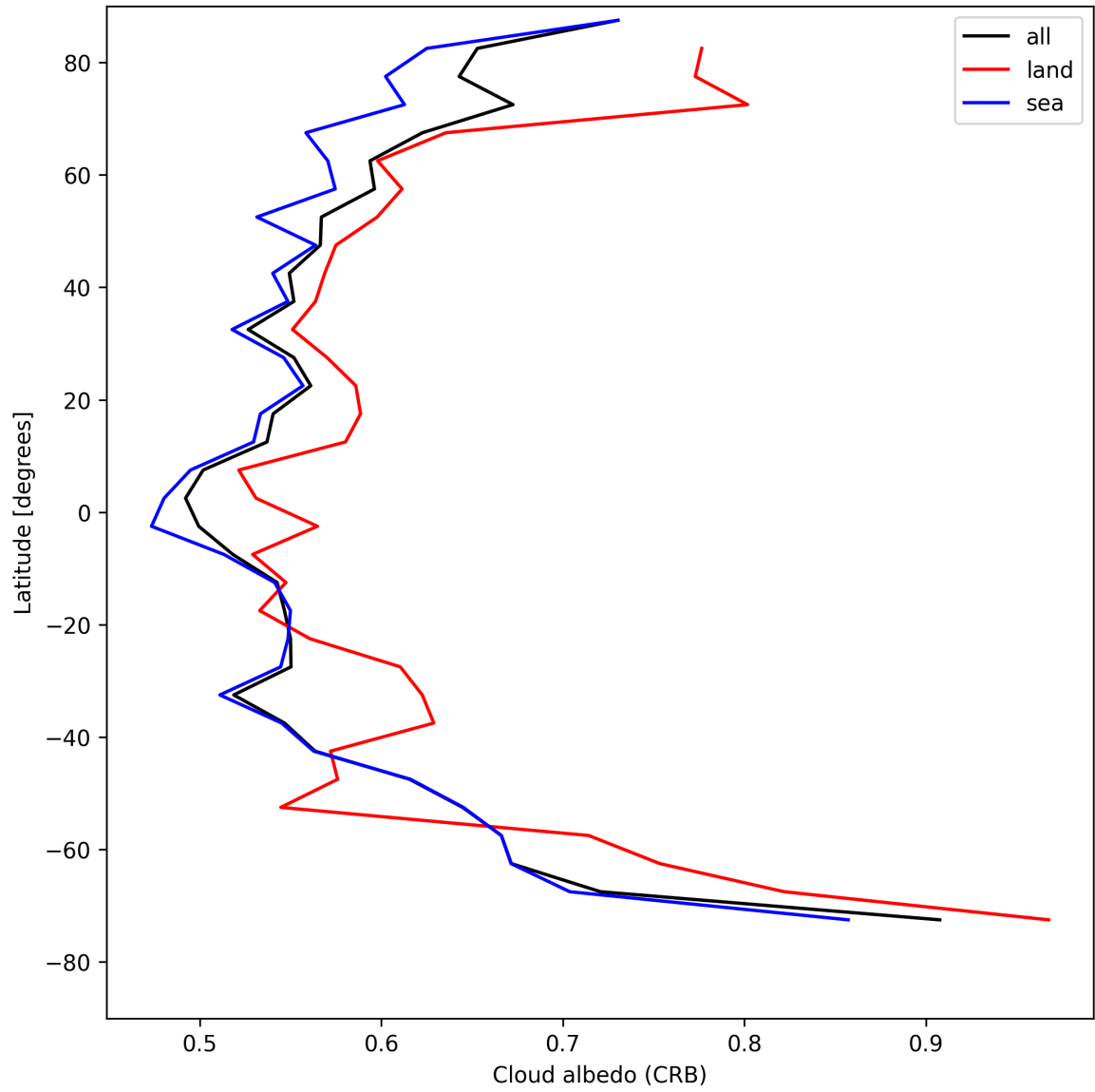
Figure 28: Zonal average of “Cloud albedo (CRB)” for 2025-05-11 to 2025-05-13.
