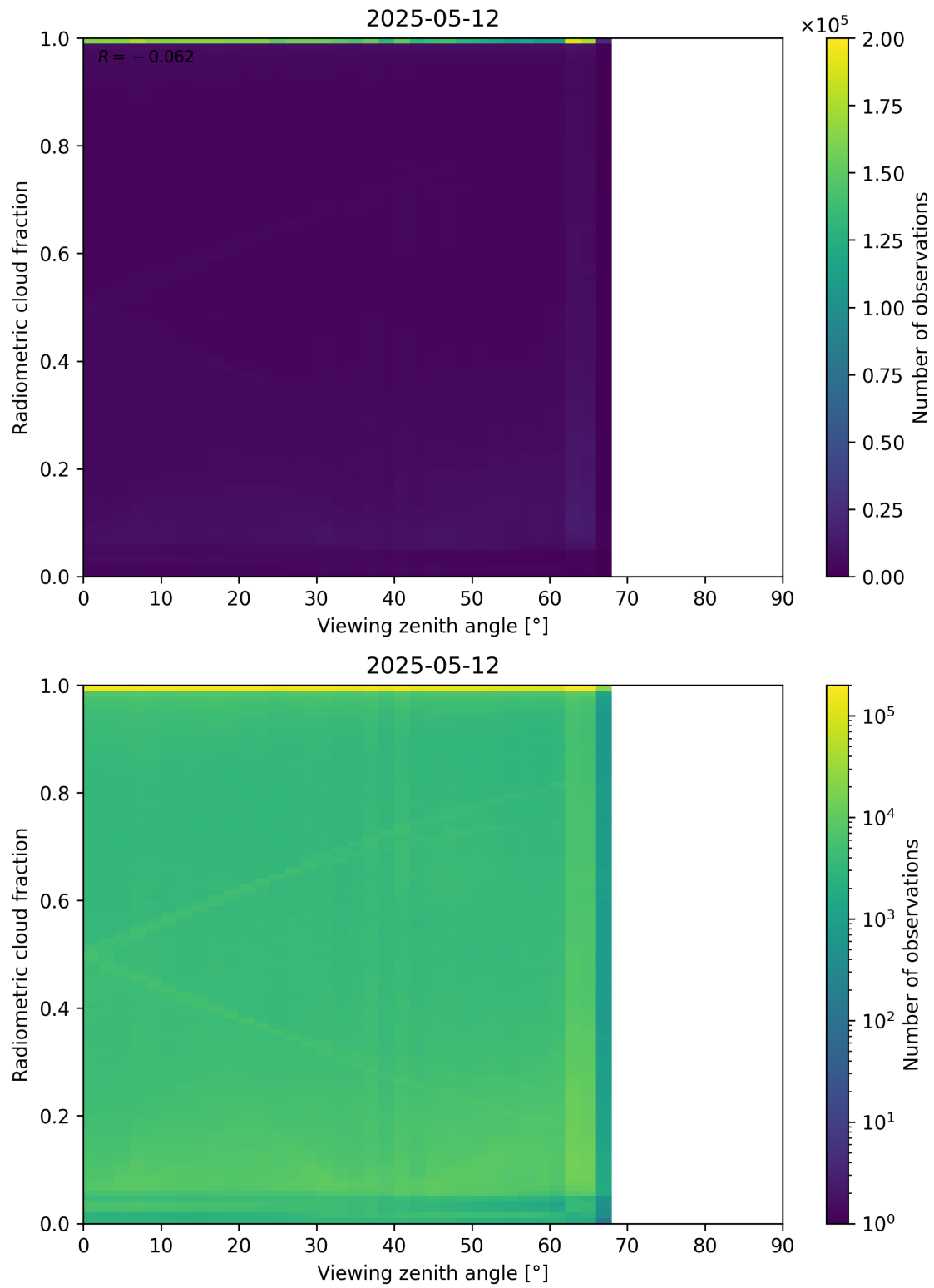
Figure 107: Scatter density plot of “Viewing zenith angle” against “Radiometric cloud fraction” for 2025-05-11 to 2025-05-13.
