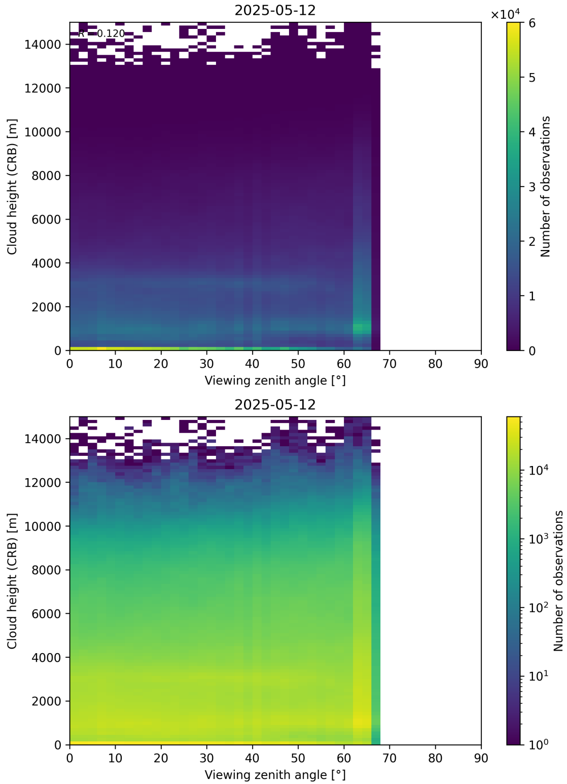
Figure 110: Scatter density plot of “Viewing zenith angle” against “Cloud height (CRB)” for 2025-05-11 to 2025-05-13.
