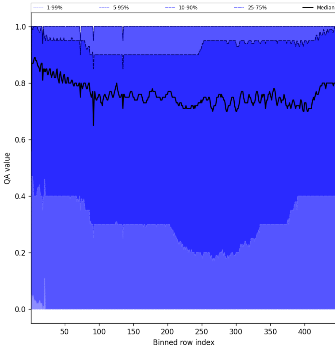
Figure 54: Along track statistics of “QA value” for 2025-05-11 to 2025-05-13
