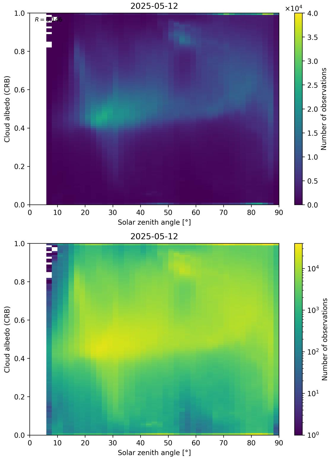
Figure 98: Scatter density plot of “Solar zenith angle” against “Cloud albedo (CRB)” for 2025-05-11 to 2025-05-13.
