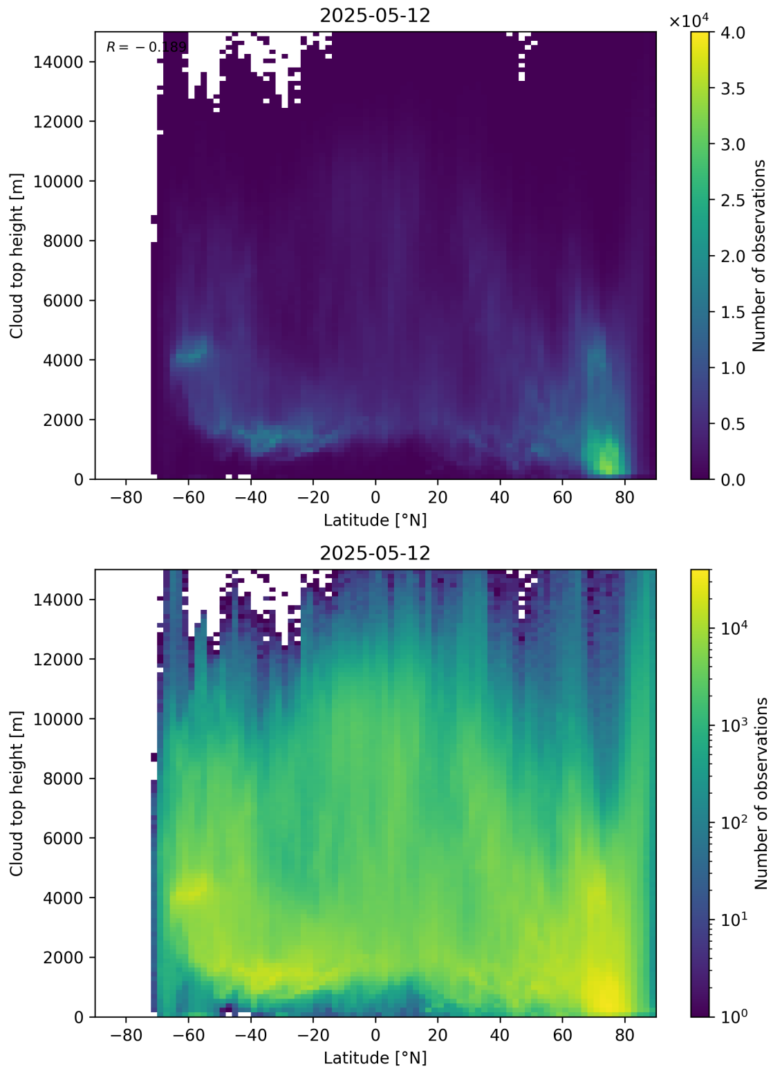
Figure 97: Scatter density plot of “Latitude” against “Cloud top height” for 2025-05-11 to 2025-05-13.
