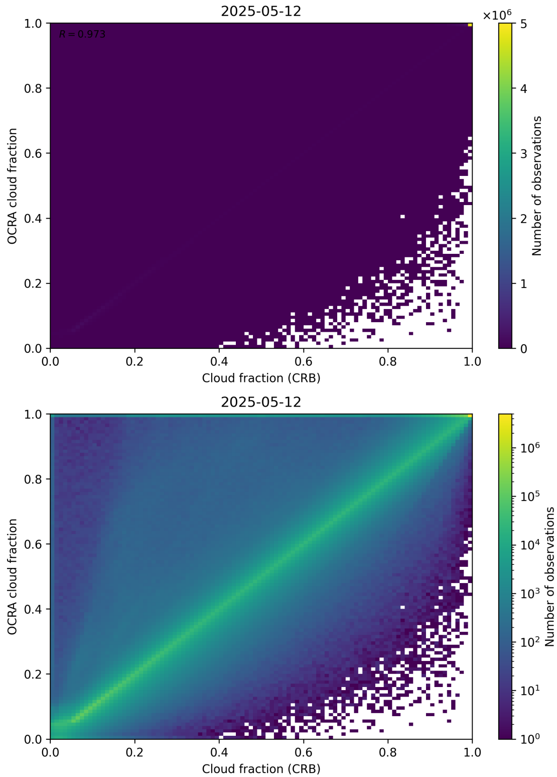
Figure 78: Scatter density plot of “Cloud fraction (CRB)” against “OCRA cloud fraction” for 2025-05-11 to 2025-05-13.
