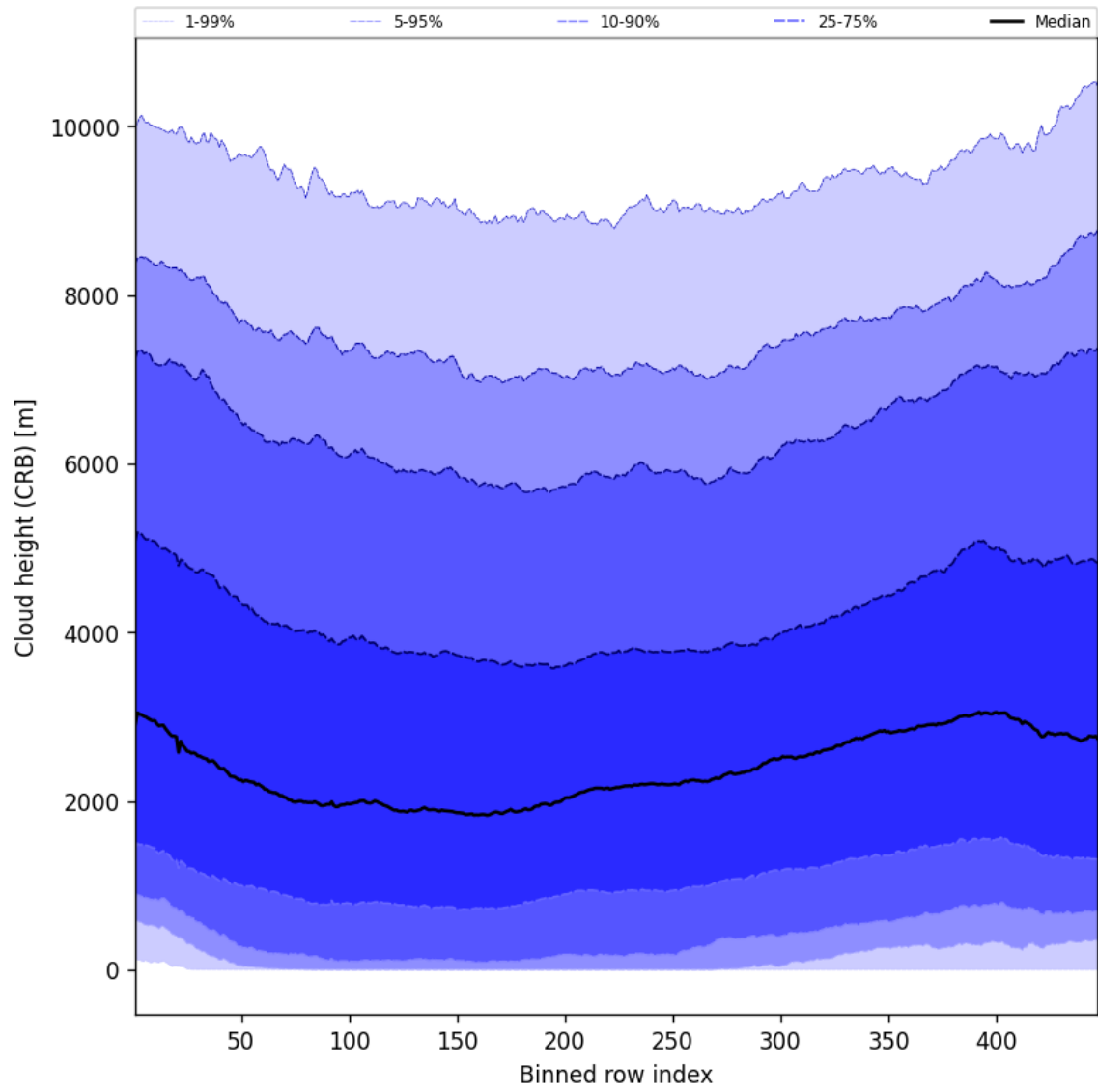
Figure 59: Along track statistics of “Cloud height (CRB)” for 2025-05-11 to 2025-05-13
