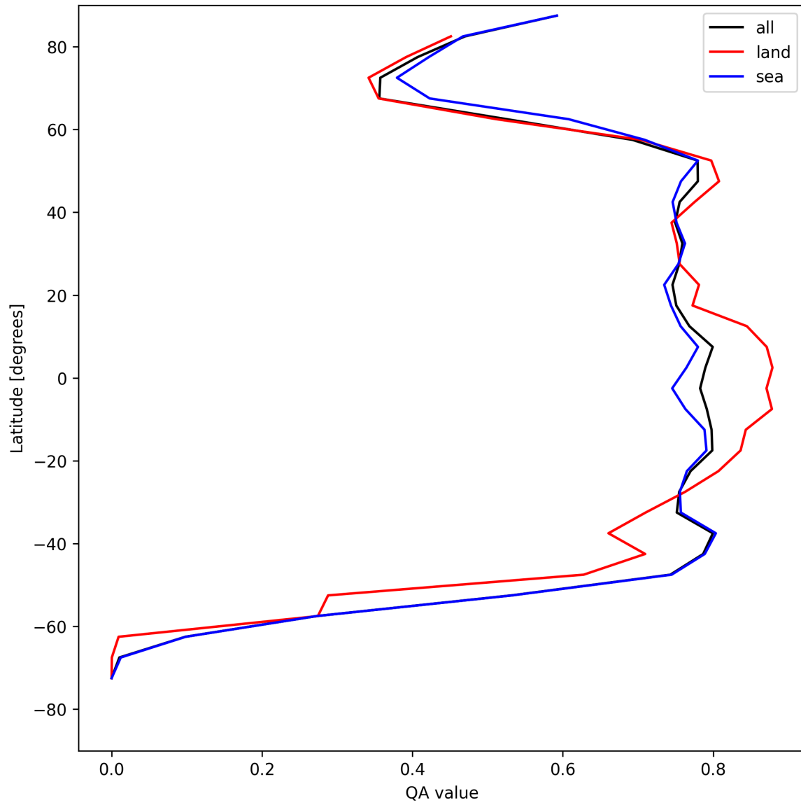
Figure 22: Zonal average of “QA value” for 2025-05-11 to 2025-05-13.
