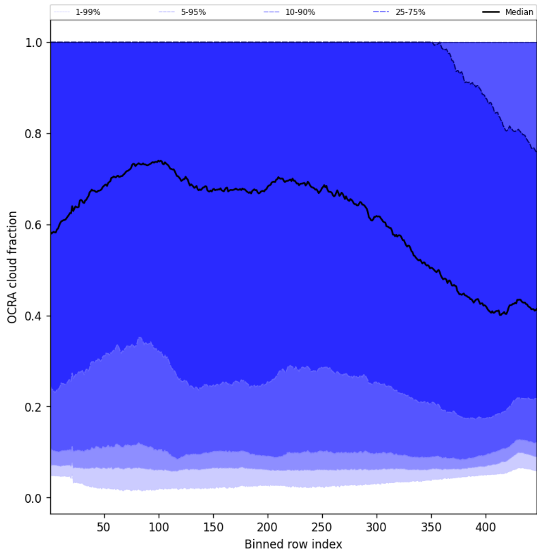
Figure 66: Along track statistics of “OCRA cloud fraction” for 2025-05-11 to 2025-05-13
