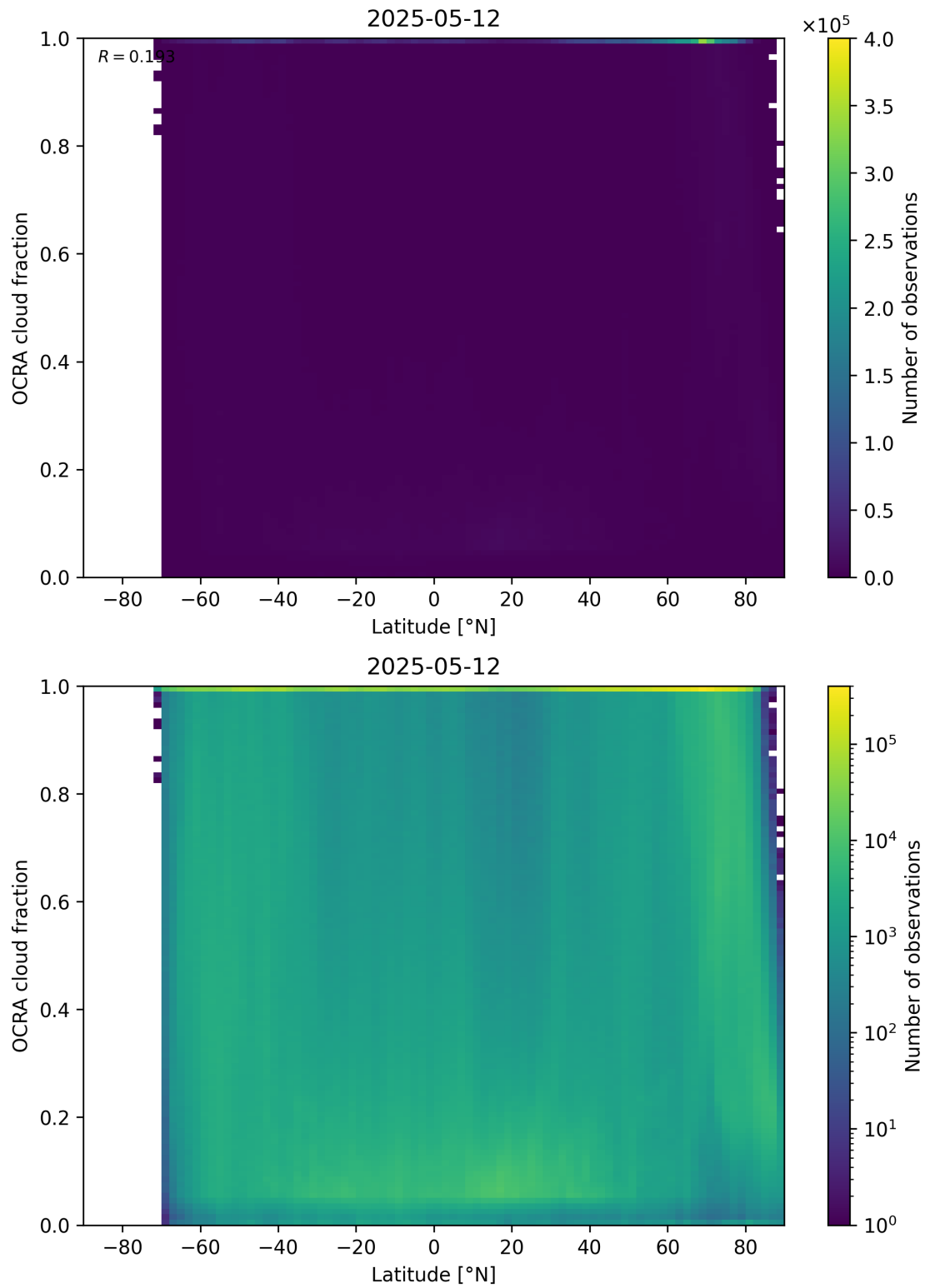
Figure 93: Scatter density plot of “Latitude” against “OCRA cloud fraction” for 2025-05-11 to 2025-05-13.
