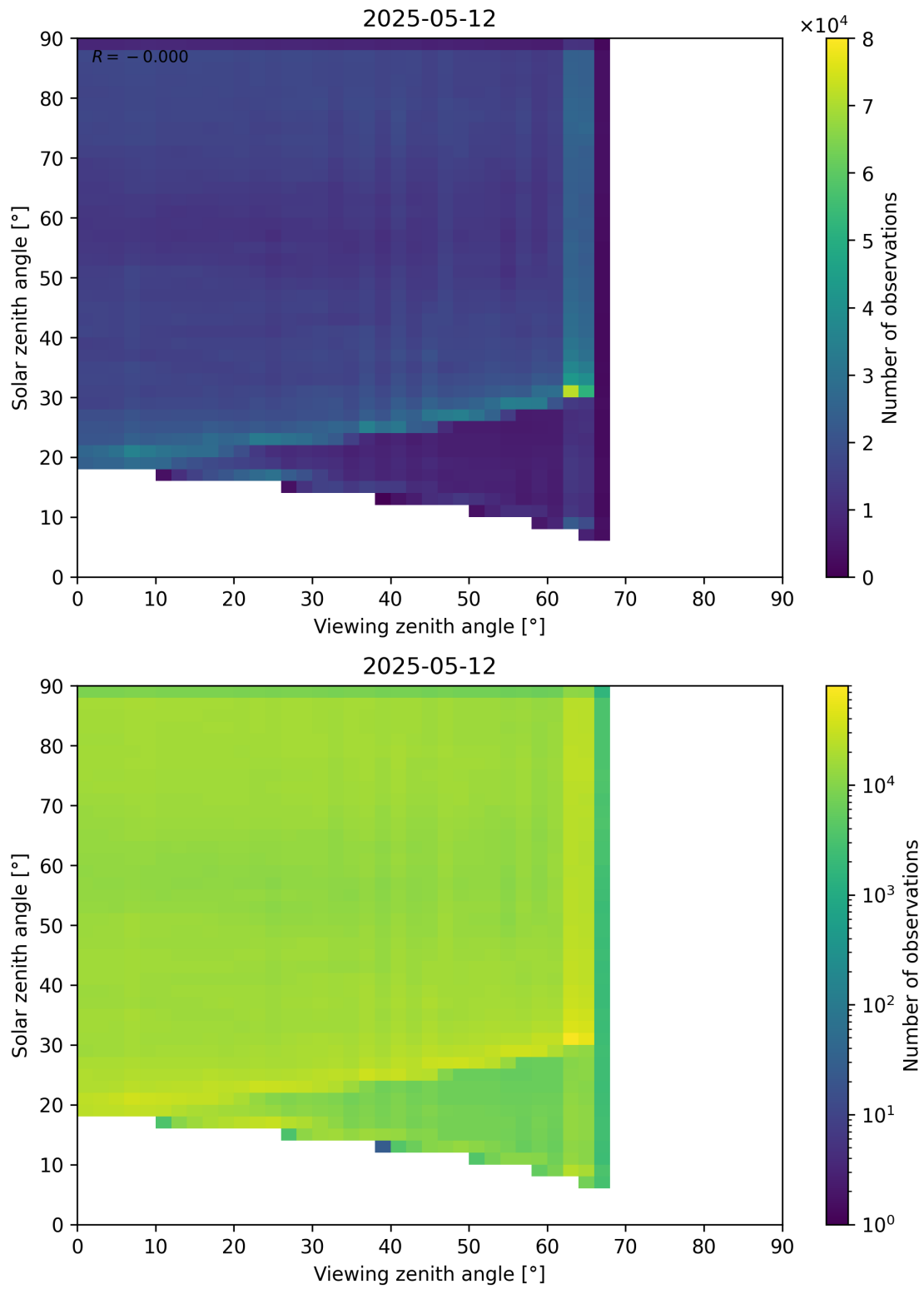
Figure 114: Scatter density plot of “Viewing zenith angle” against “Solar zenith angle” for 2025-05-11 to 2025-05-13.
