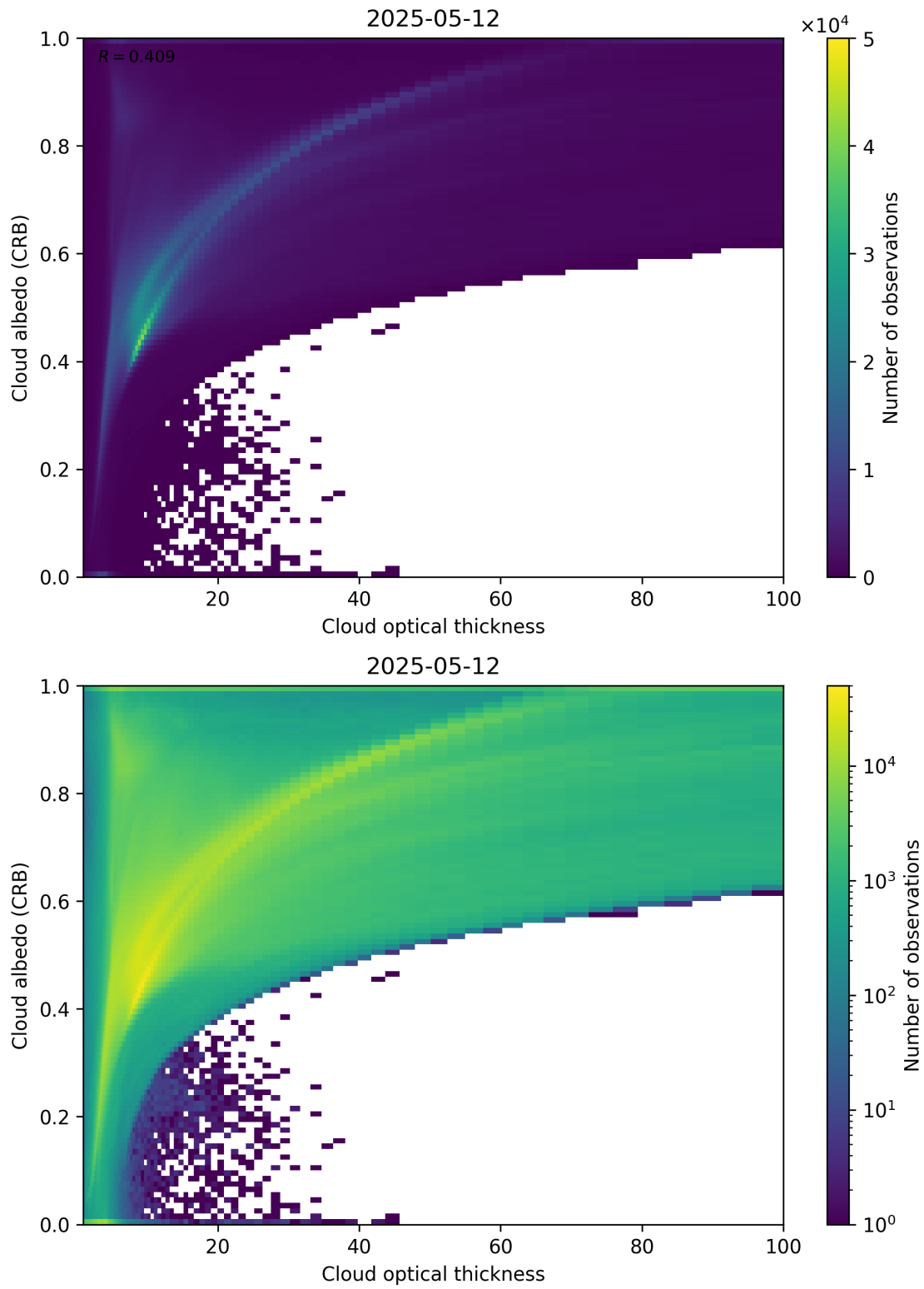
Figure 82: Scatter density plot of “Cloud optical thickness” against “Cloud albedo (CRB)” for 2025-05-11 to 2025-05-13.
