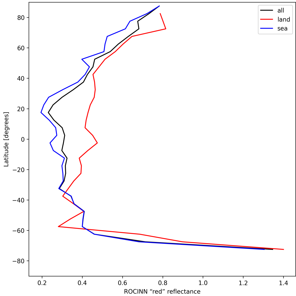
Figure 37: Zonal average of “ROCINN “red” reflectance” for 2025-05-11 to 2025-05-13.
