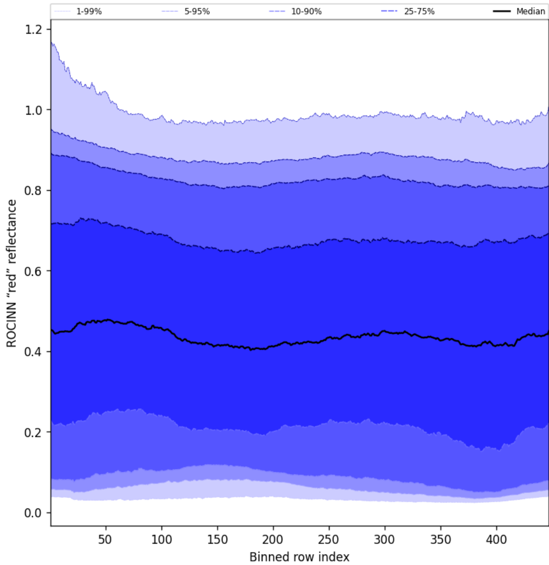
Figure 69: Along track statistics of “ROCINN “red” reflectance” for 2025-05-11 to 2025-05-13
