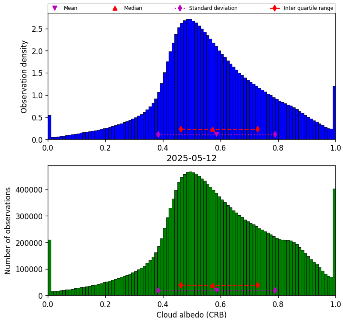
Figure 44: Histogram of “Cloud albedo (CRB)” for 2025-05-11 to 2025-05-13
