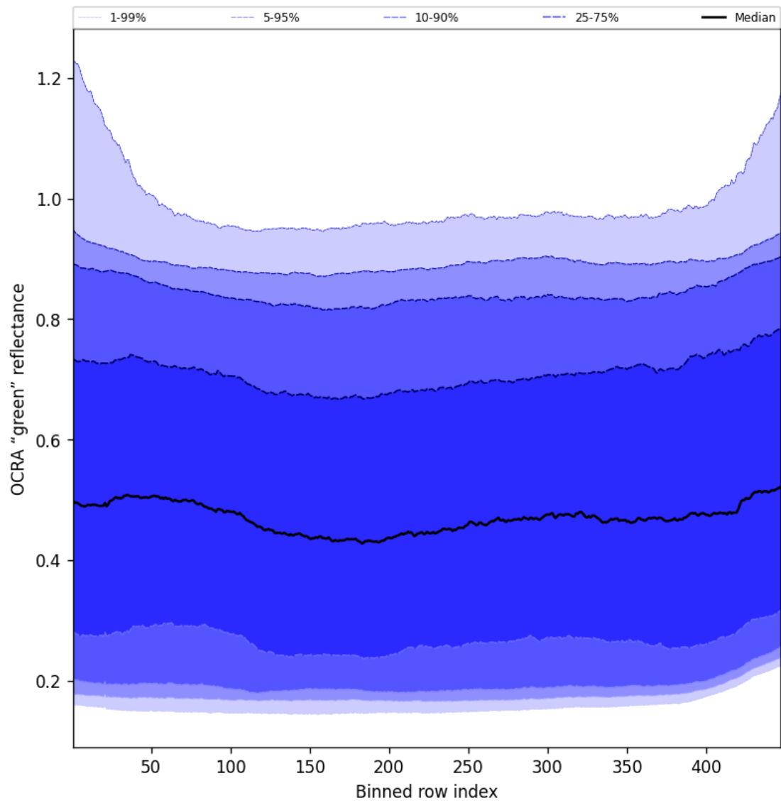
Figure 68: Along track statistics of "OCRA "green" reflectance" for 2025-05-11 to 2025-05-13
