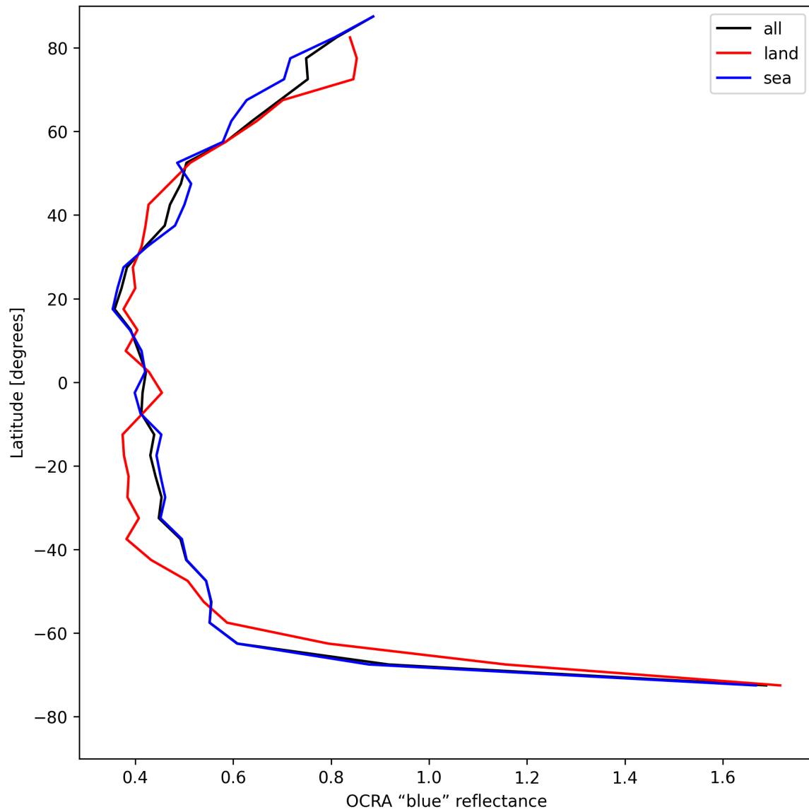
Figure 35: Zonal average of “OCRA “blue” reflectance” for 2025-05-11 to 2025-05-13.
