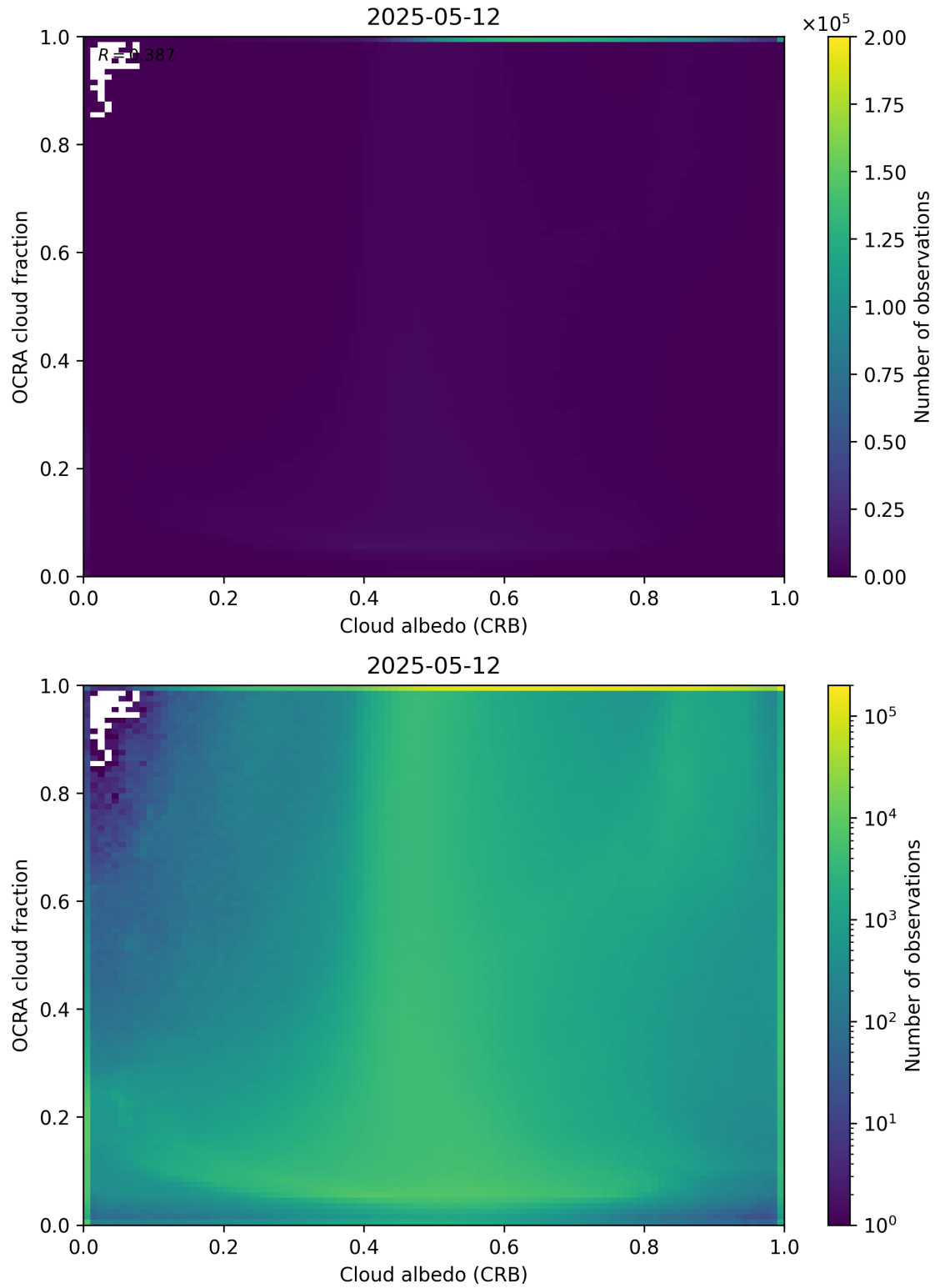
Figure 70: Scatter density plot of “Cloud albedo (CRB)” against “OCRA cloud fraction” for 2025-05-11 to 2025-05-13.
