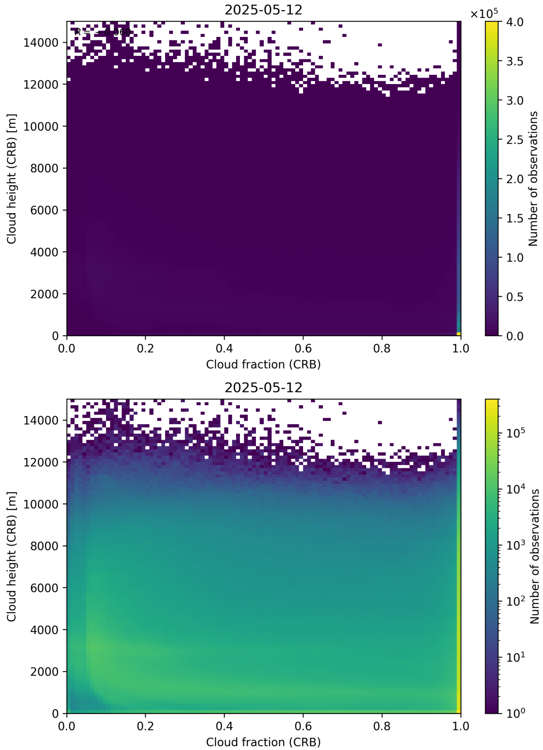
Figure 79: Scatter density plot of “Cloud fraction (CRB)” against “Cloud height (CRB)” for 2025-05-11 to 2025-05-13.
