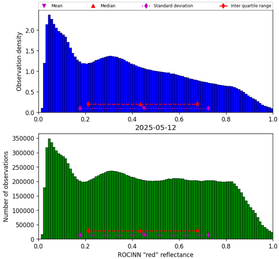
Figure 53: Histogram of “ROCINN “red” reflectance” for 2025-05-11 to 2025-05-13
