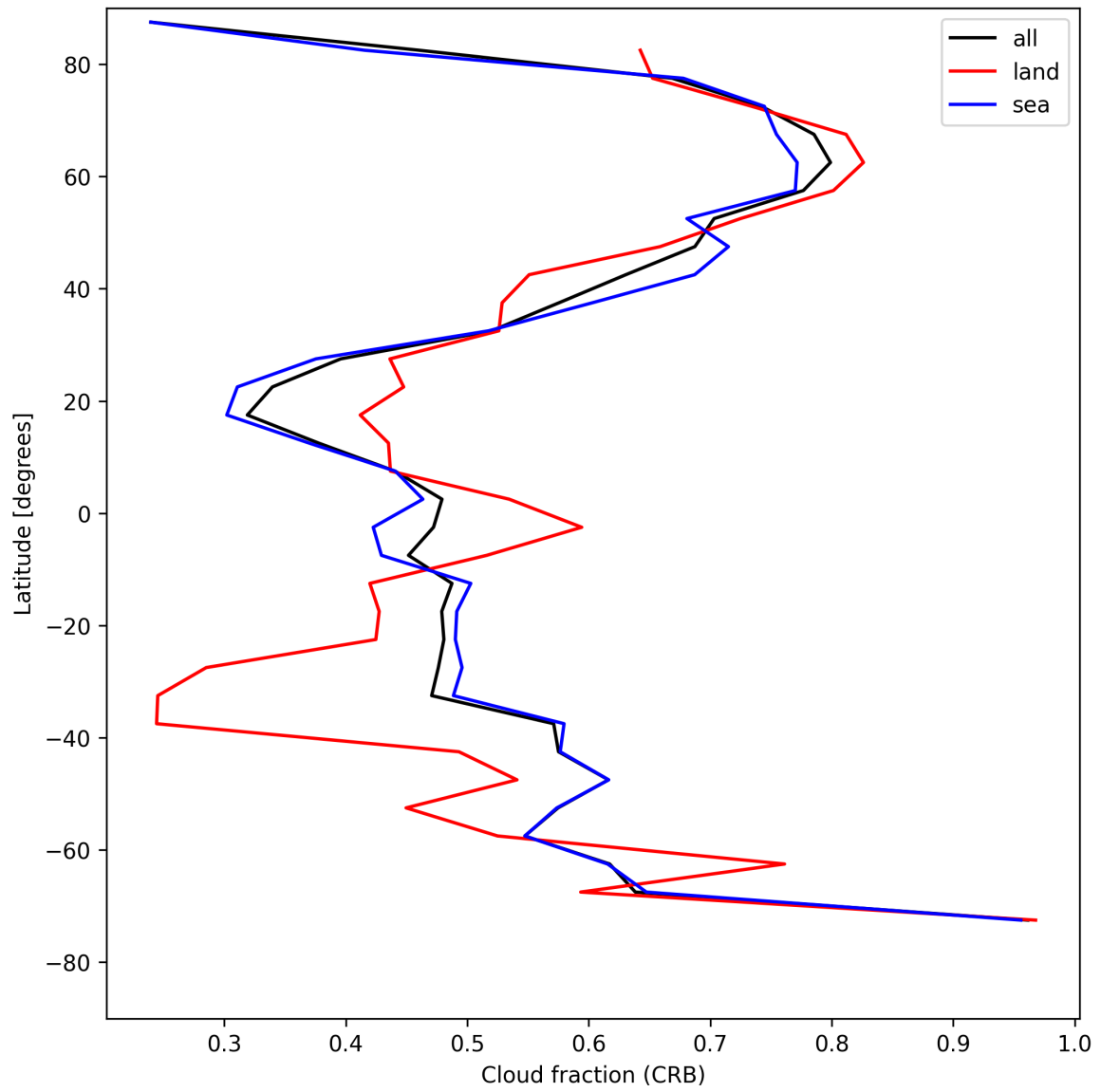
Figure 26: Zonal average of “Cloud fraction (CRB)” for 2025-05-11 to 2025-05-13.
