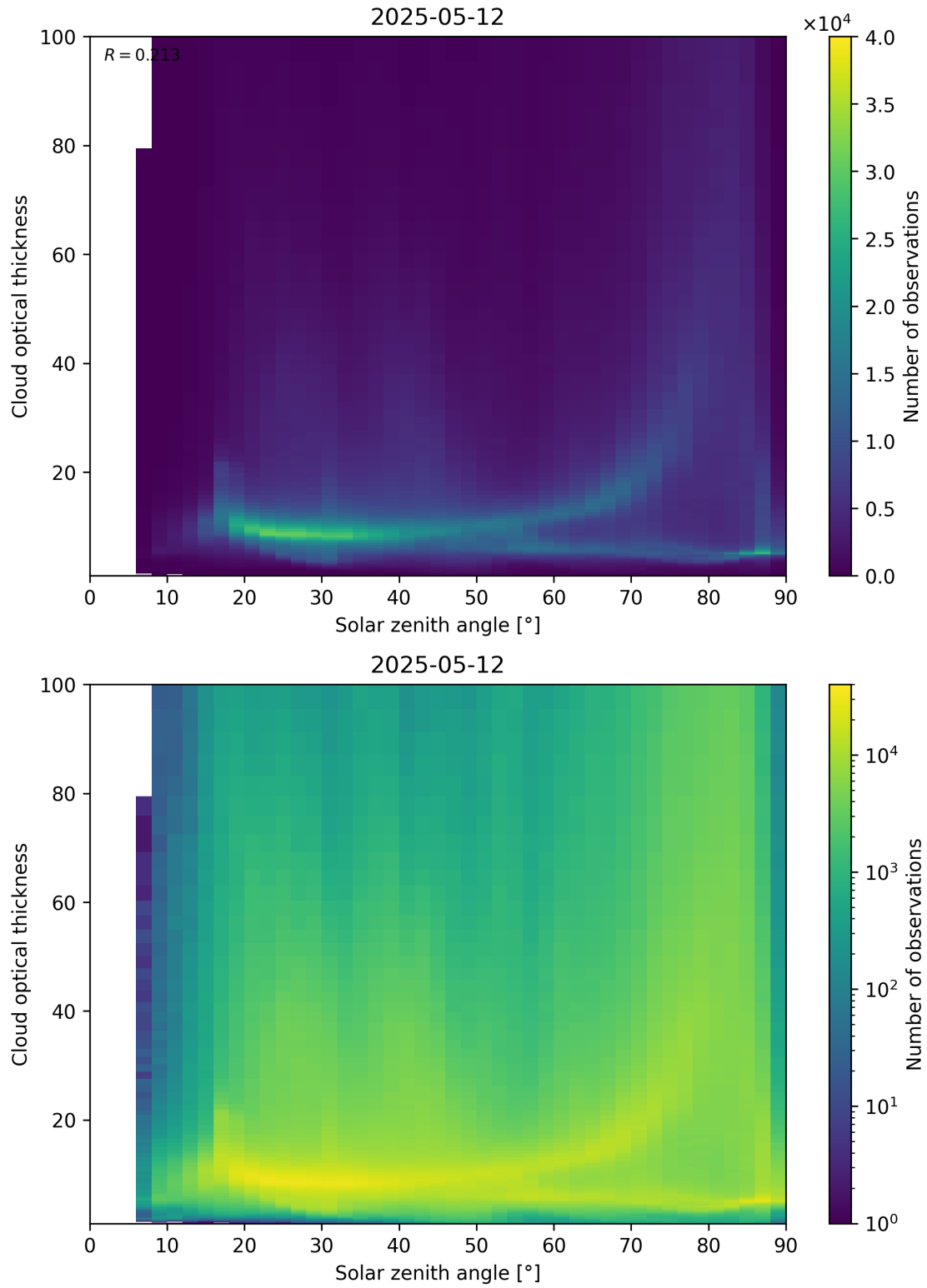
Figure 103: Scatter density plot of “Solar zenith angle” against “Cloud optical thickness” for 2025-05-11 to 2025-05-13.
