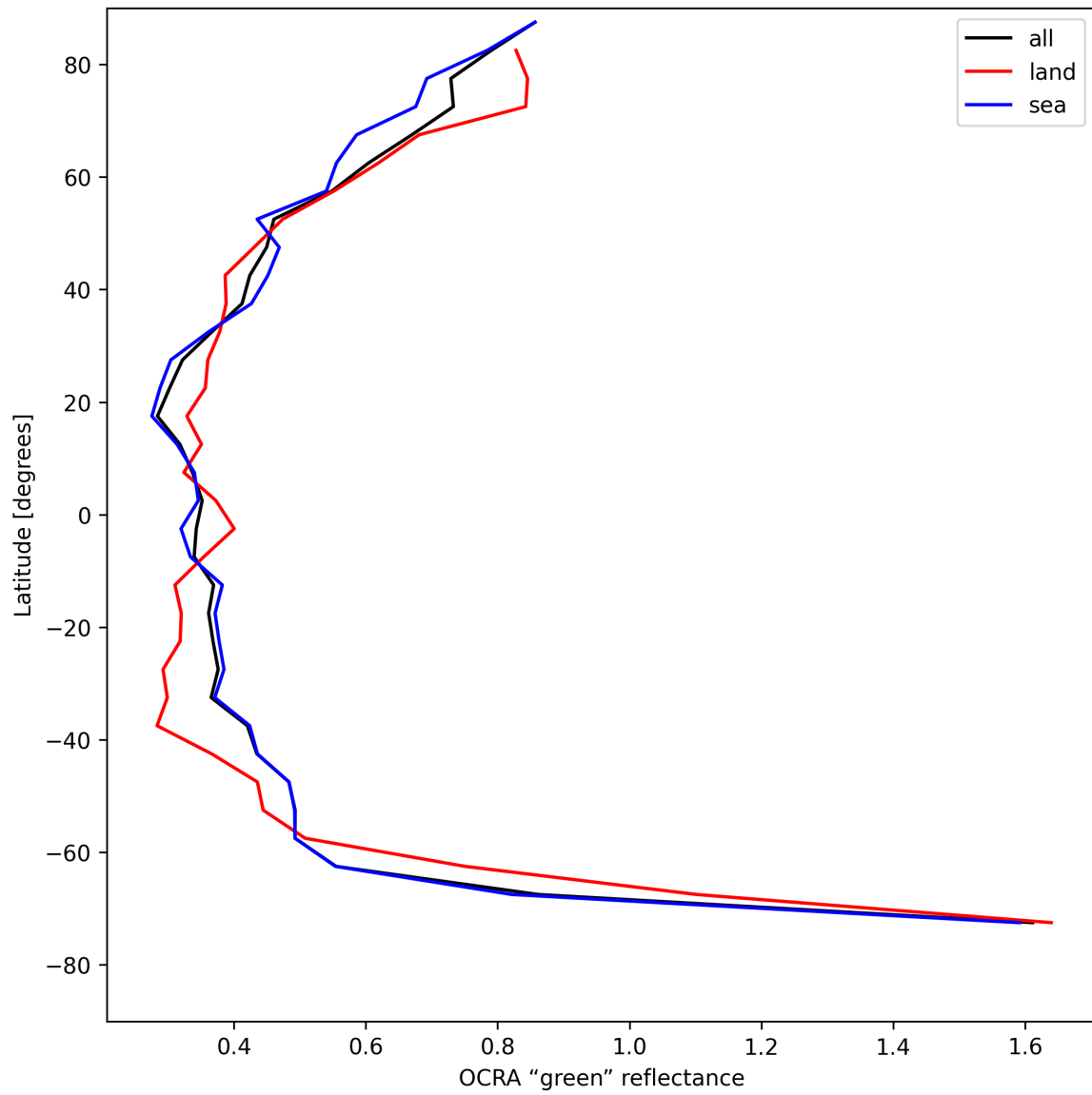
Figure 36: Zonal average of “OCRA “green” reflectance” for 2025-05-11 to 2025-05-13.
