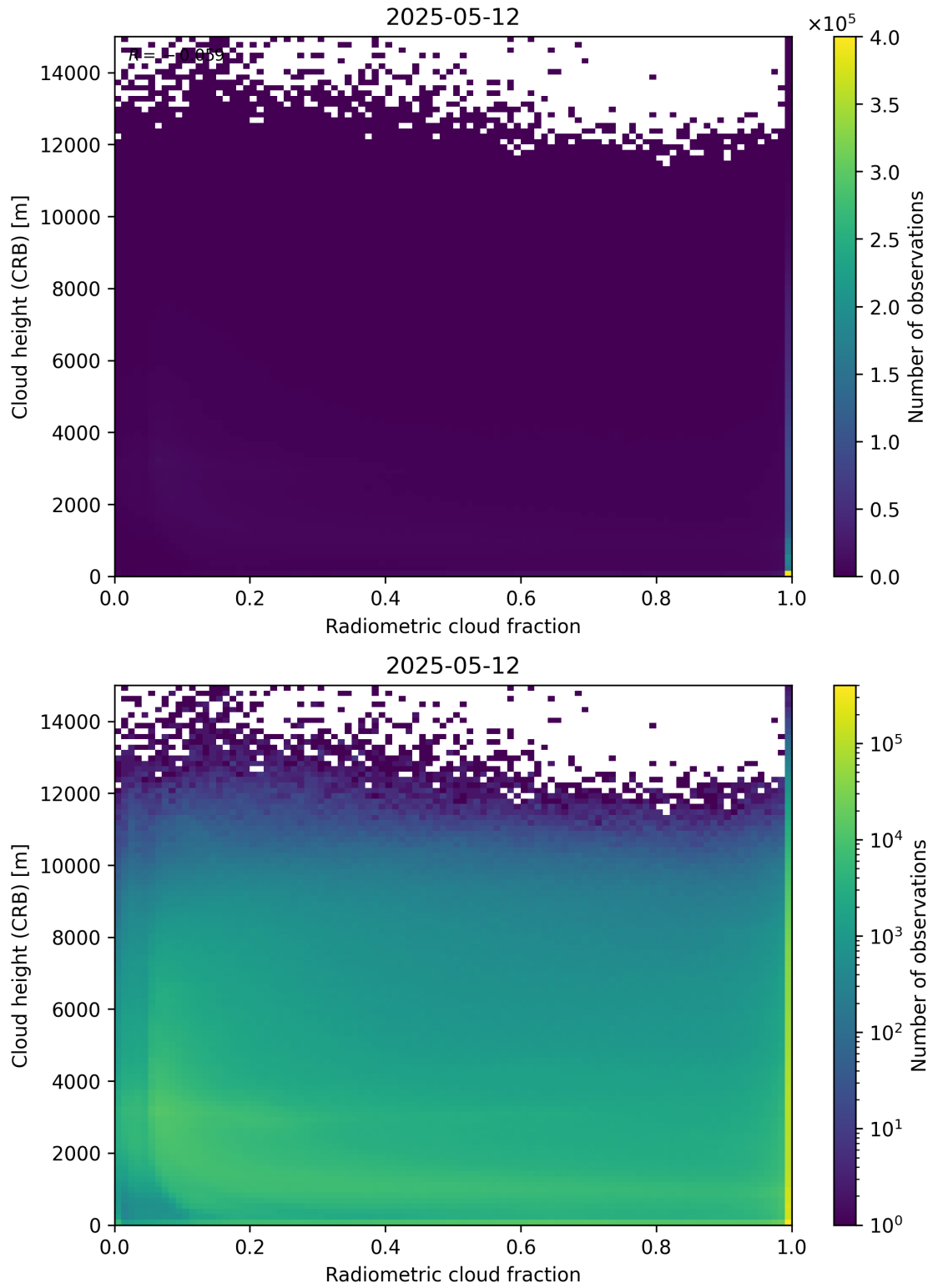
Figure 74: Scatter density plot of “Radiometric cloud fraction” against “Cloud height (CRB)” for 2025-05-11 to 2025-05-13.
