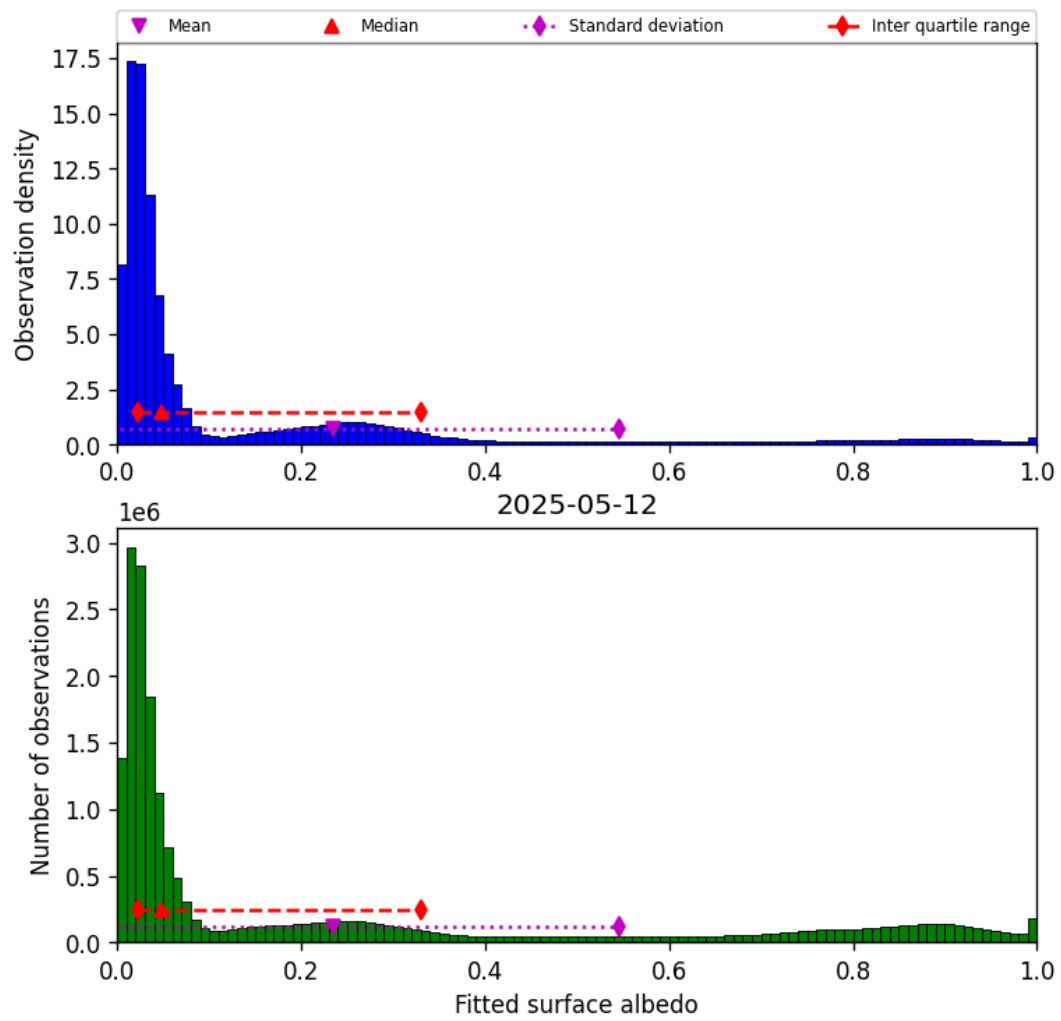
Figure 45: Histogram of “Fitted surface albedo” for 2025-05-11 to 2025-05-13
