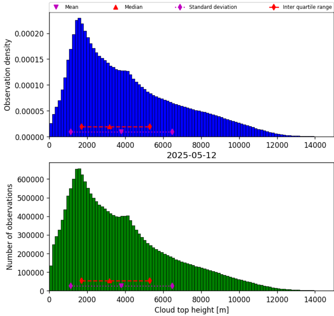
Figure 40: Histogram of “Cloud top height” for 2025-05-11 to 2025-05-13
