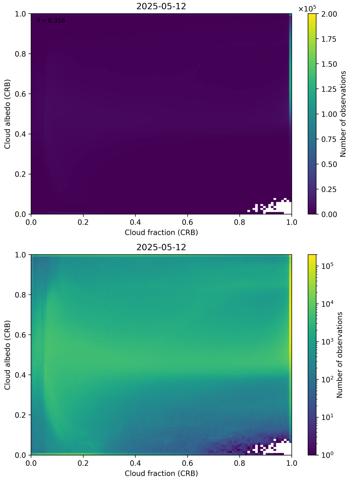
Figure 77: Scatter density plot of “Cloud fraction (CRB)” against “Cloud albedo (CRB)” for 2025-05-11 to 2025-05-13.
