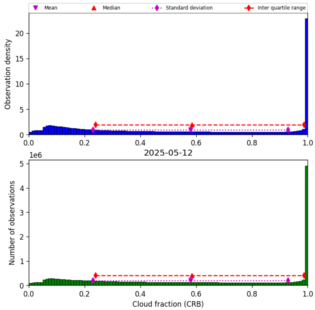
Figure 42: Histogram of “Cloud fraction (CRB)” for 2025-05-11 to 2025-05-13
