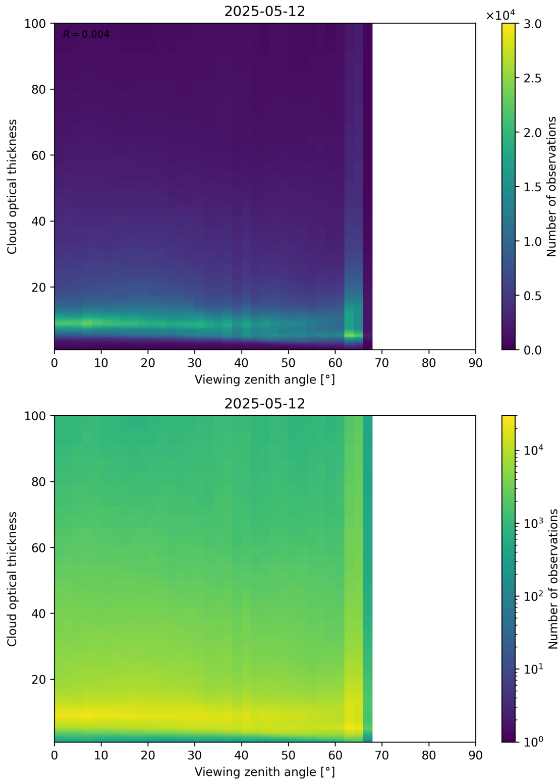
Figure 111: Scatter density plot of “Viewing zenith angle” against “Cloud optical thickness” for 2025-05-11 to 2025-05-13.
