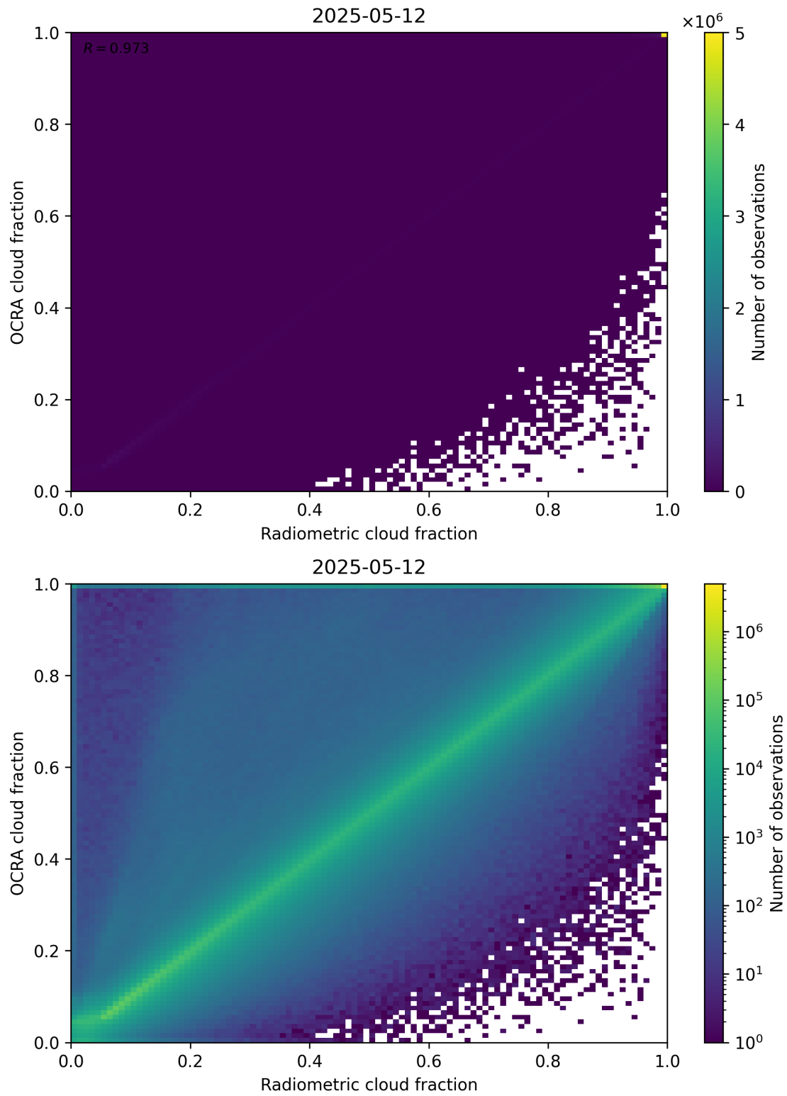
Figure 72: Scatter density plot of “Radiometric cloud fraction” against “OCRA cloud fraction” for 2025-05-11 to 2025-05-13.
