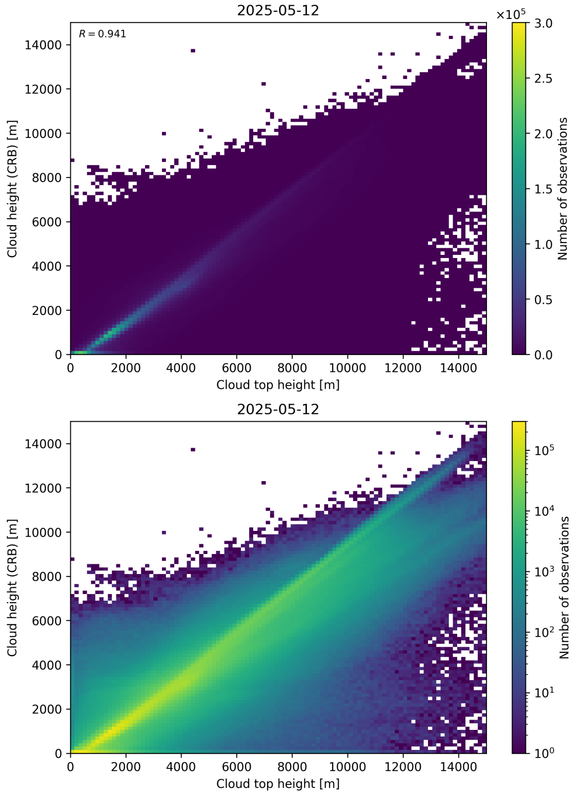
Figure 89: Scatter density plot of “Cloud top height” against “Cloud height (CRB)” for 2025-05-11 to 2025-05-13.
