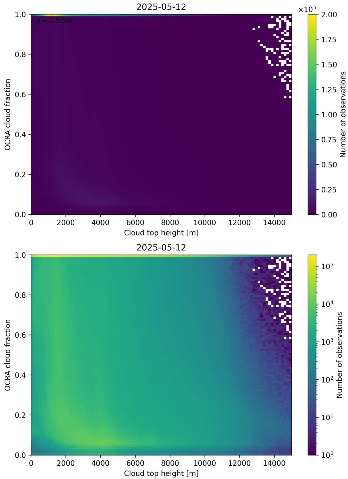
Figure 87: Scatter density plot of “Cloud top height” against “OCRA cloud fraction” for 2025-05-11 to 2025-05-13.
