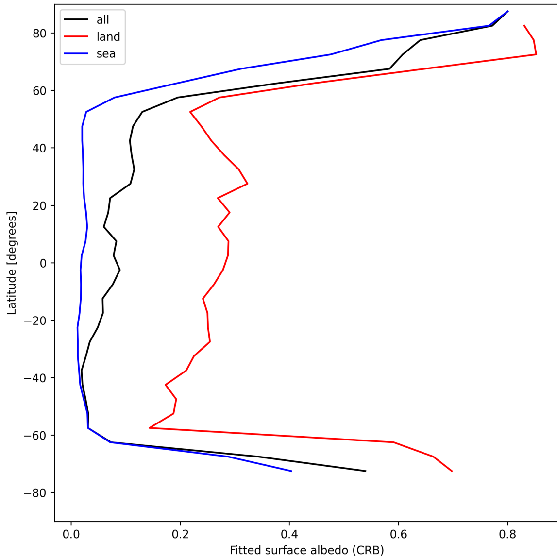
Figure 30: Zonal average of “Fitted surface albedo (CRB)” for 2025-05-11 to 2025-05-13.
