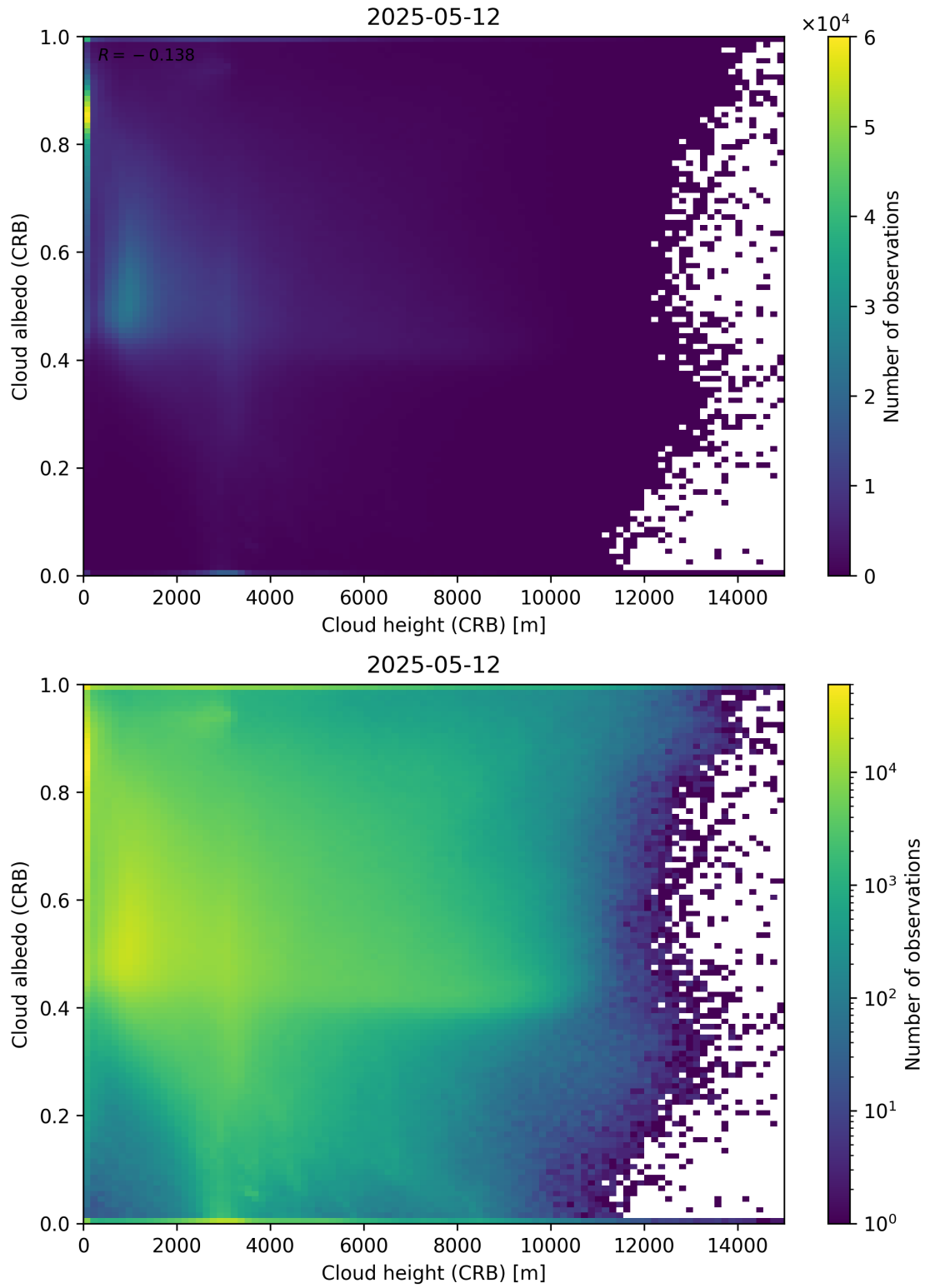
Figure 80: Scatter density plot of “Cloud height (CRB)” against “Cloud albedo (CRB)” for 2025-05-11 to 2025-05-13.
