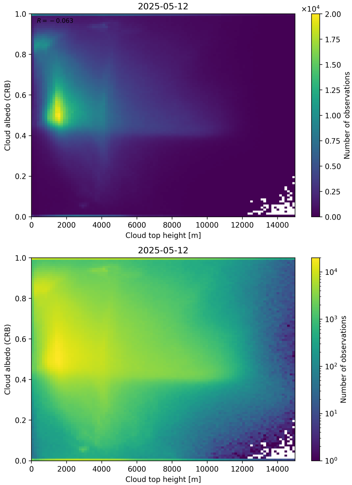
Figure 86: Scatter density plot of “Cloud top height” against “Cloud albedo (CRB)” for 2025-05-11 to 2025-05-13.
