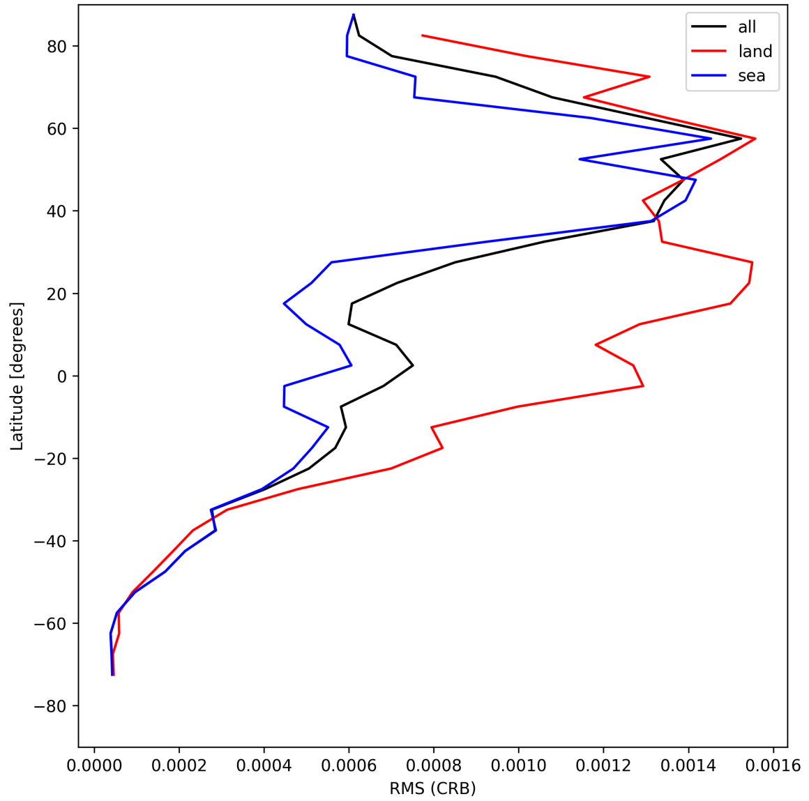
Figure 32: Zonal average of “RMS (CRB)” for 2025-05-11 to 2025-05-13.
