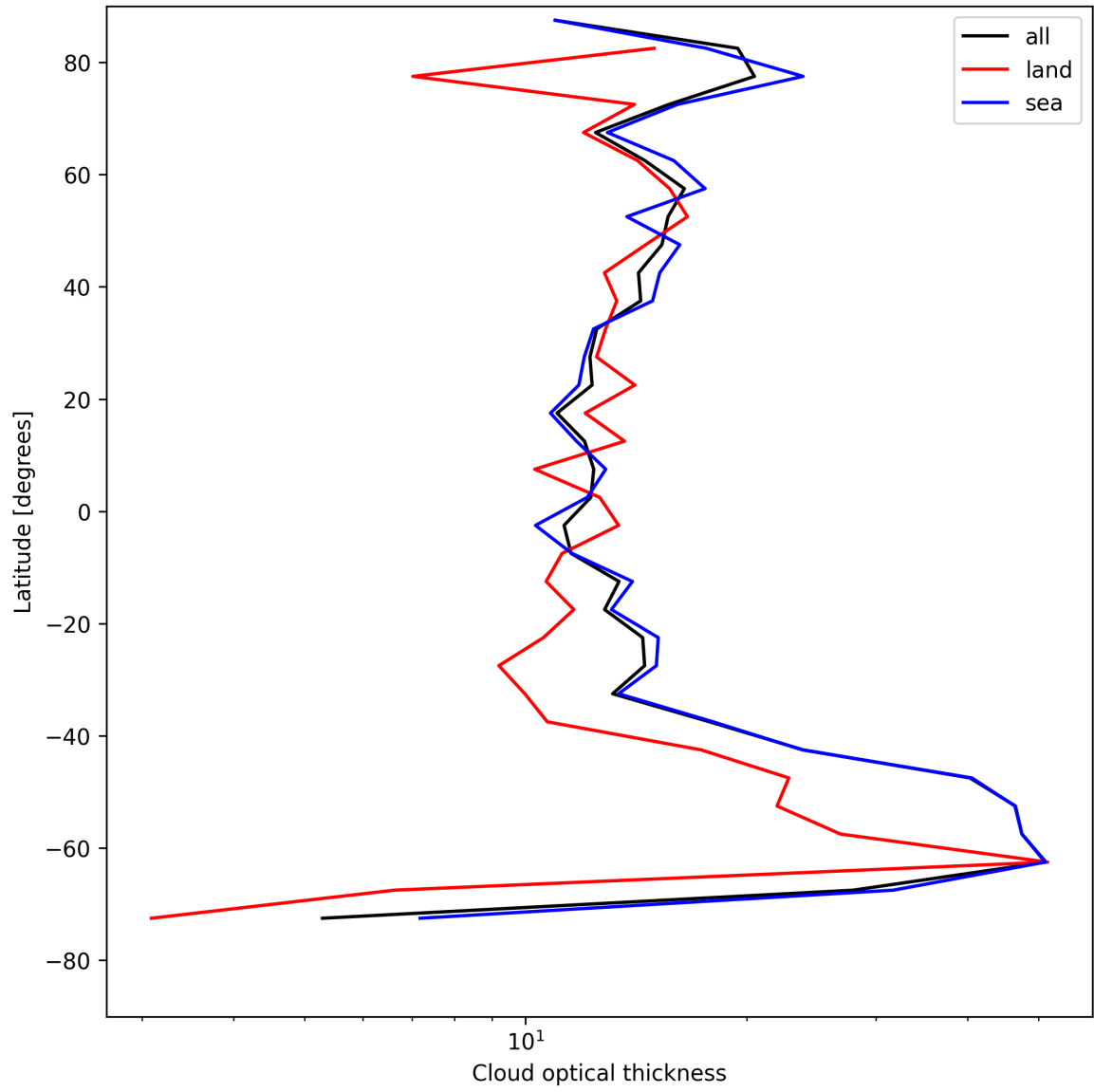
Figure 25: Zonal average of “Cloud optical thickness” for 2025-05-11 to 2025-05-13.
