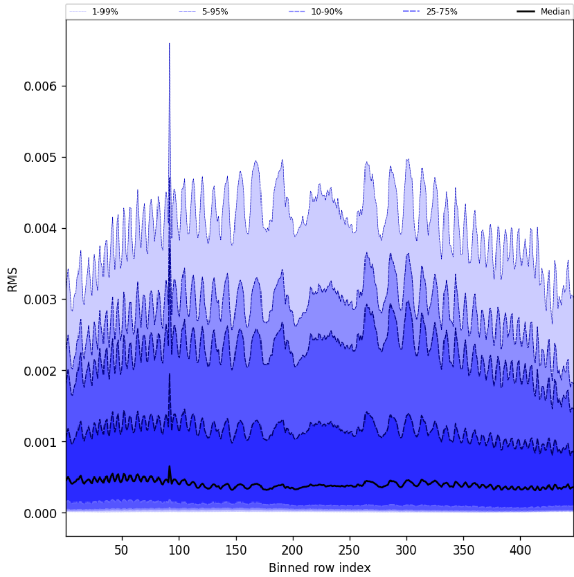
Figure 63: Along track statistics of “RMS” for 2025-05-11 to 2025-05-13
