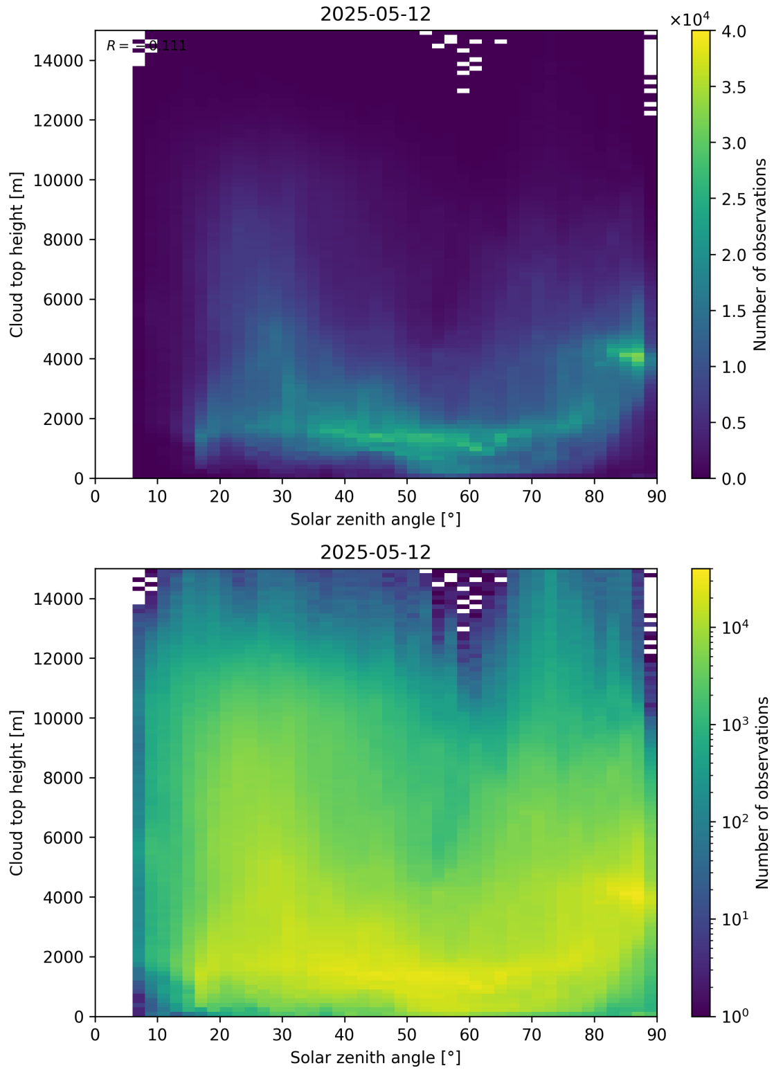
Figure 104: Scatter density plot of “Solar zenith angle” against “Cloud top height” for 2025-05-11 to 2025-05-13.
