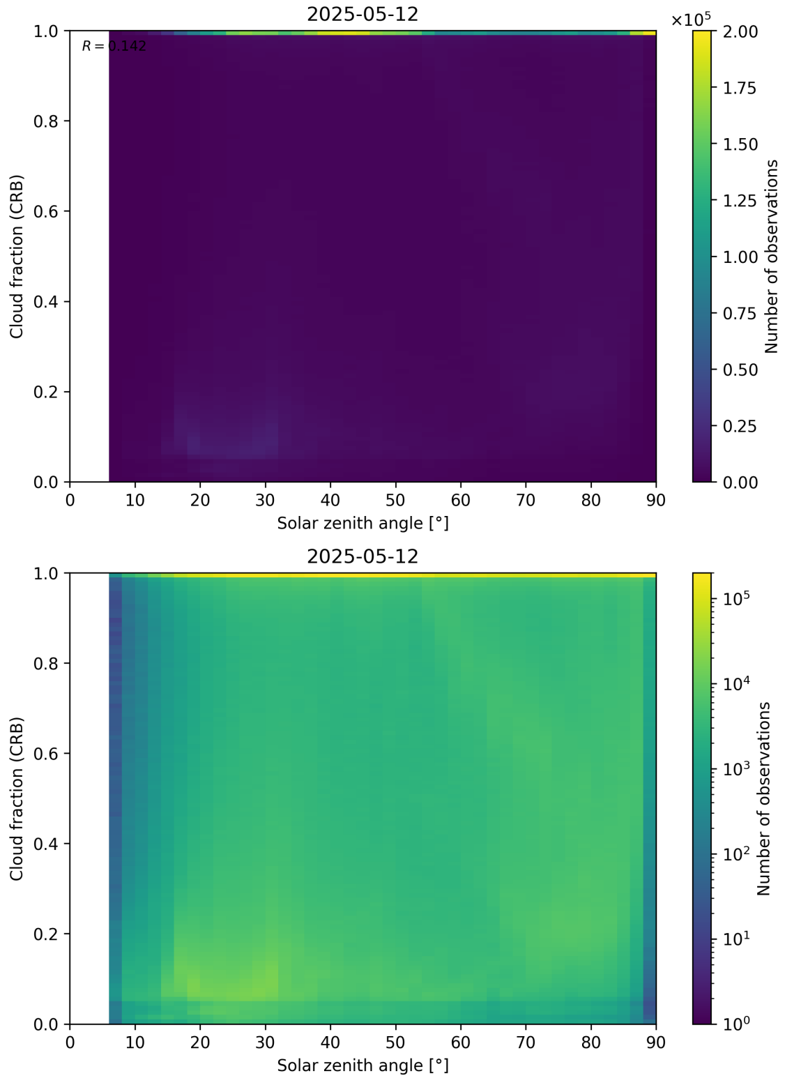
Figure 101: Scatter density plot of “Solar zenith angle” against “Cloud fraction (CRB)” for 2025-05-11 to 2025-05-13.
