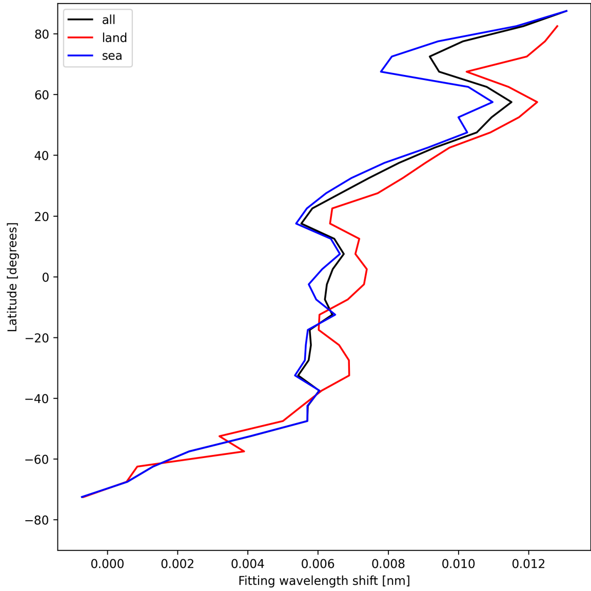
Figure 33: Zonal average of “Fitting wavelength shift” for 2025-05-11 to 2025-05-13.
