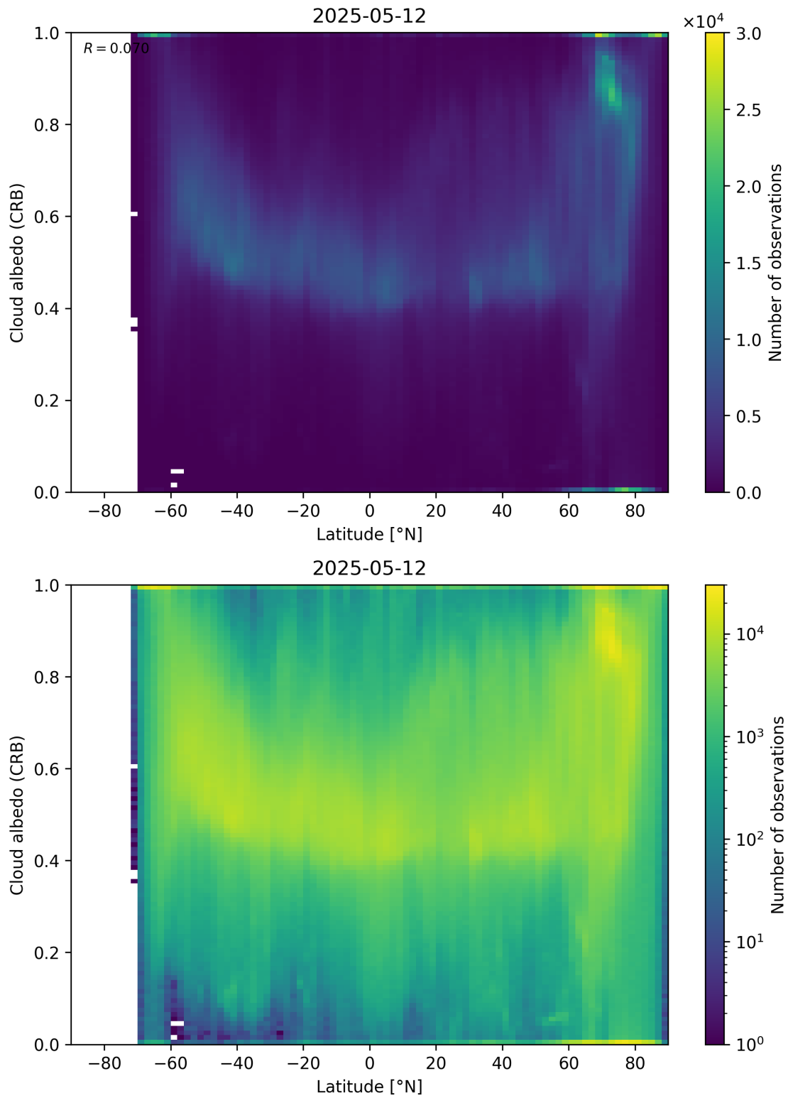
Figure 91: Scatter density plot of “Latitude” against “Cloud albedo (CRB)” for 2025-05-11 to 2025-05-13.
