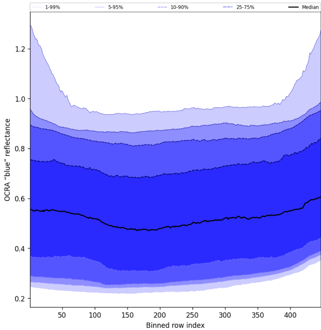
Figure 67: Along track statistics of “OCRA “blue” reflectance” for 2025-05-11 to 2025-05-13
