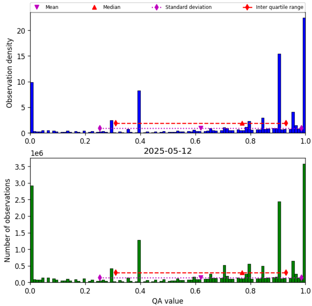
Figure 38: Histogram of “QA value” for 2025-05-11 to 2025-05-13
