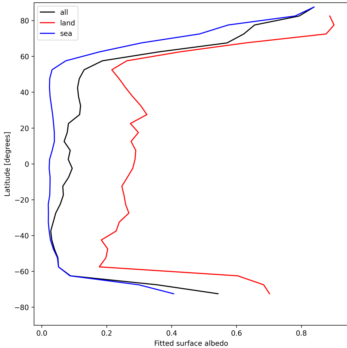
Figure 29: Zonal average of “Fitted surface albedo” for 2025-05-11 to 2025-05-13.
