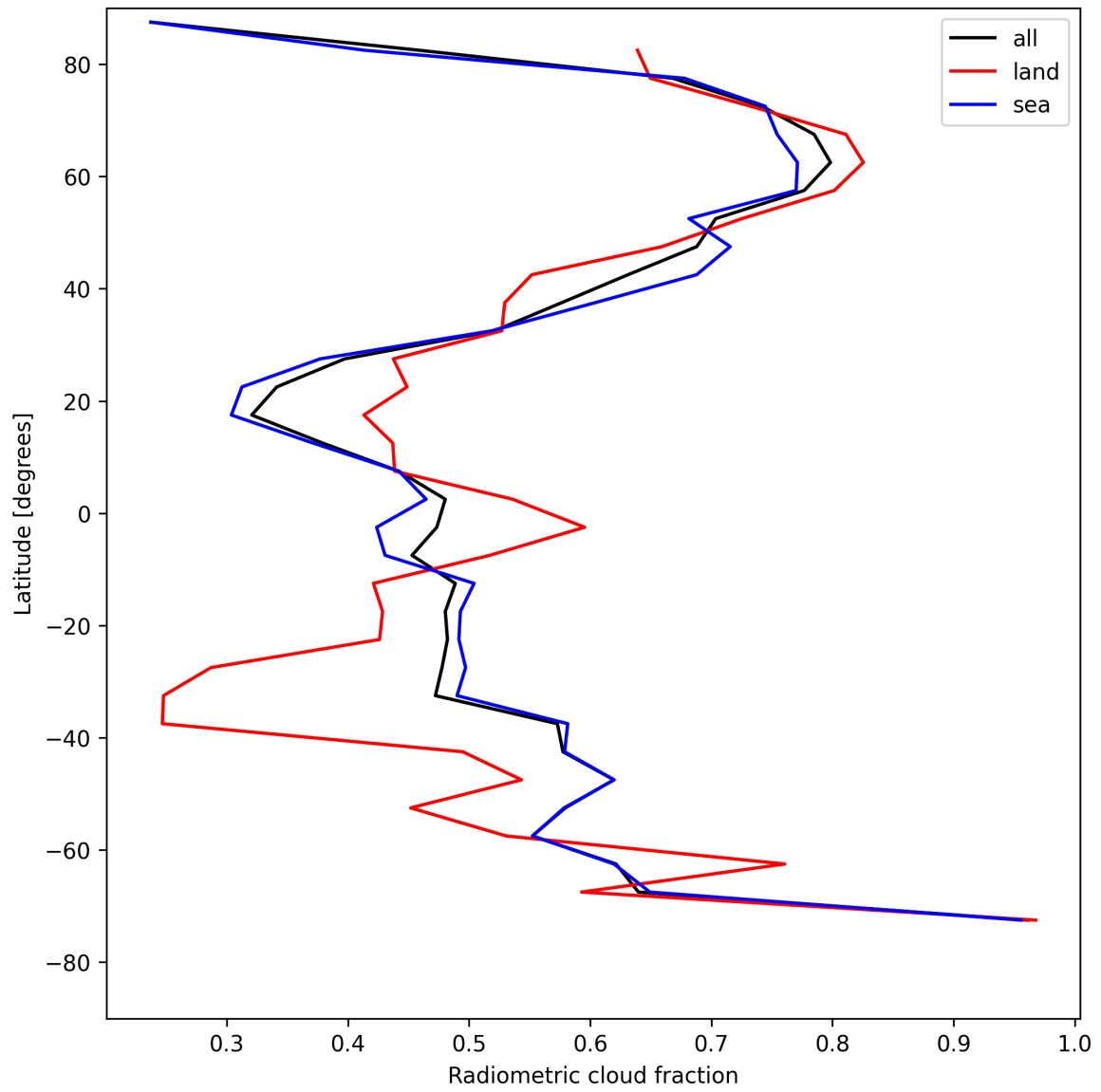
Figure 23: Zonal average of “Radiometric cloud fraction” for 2025-05-11 to 2025-05-13.
