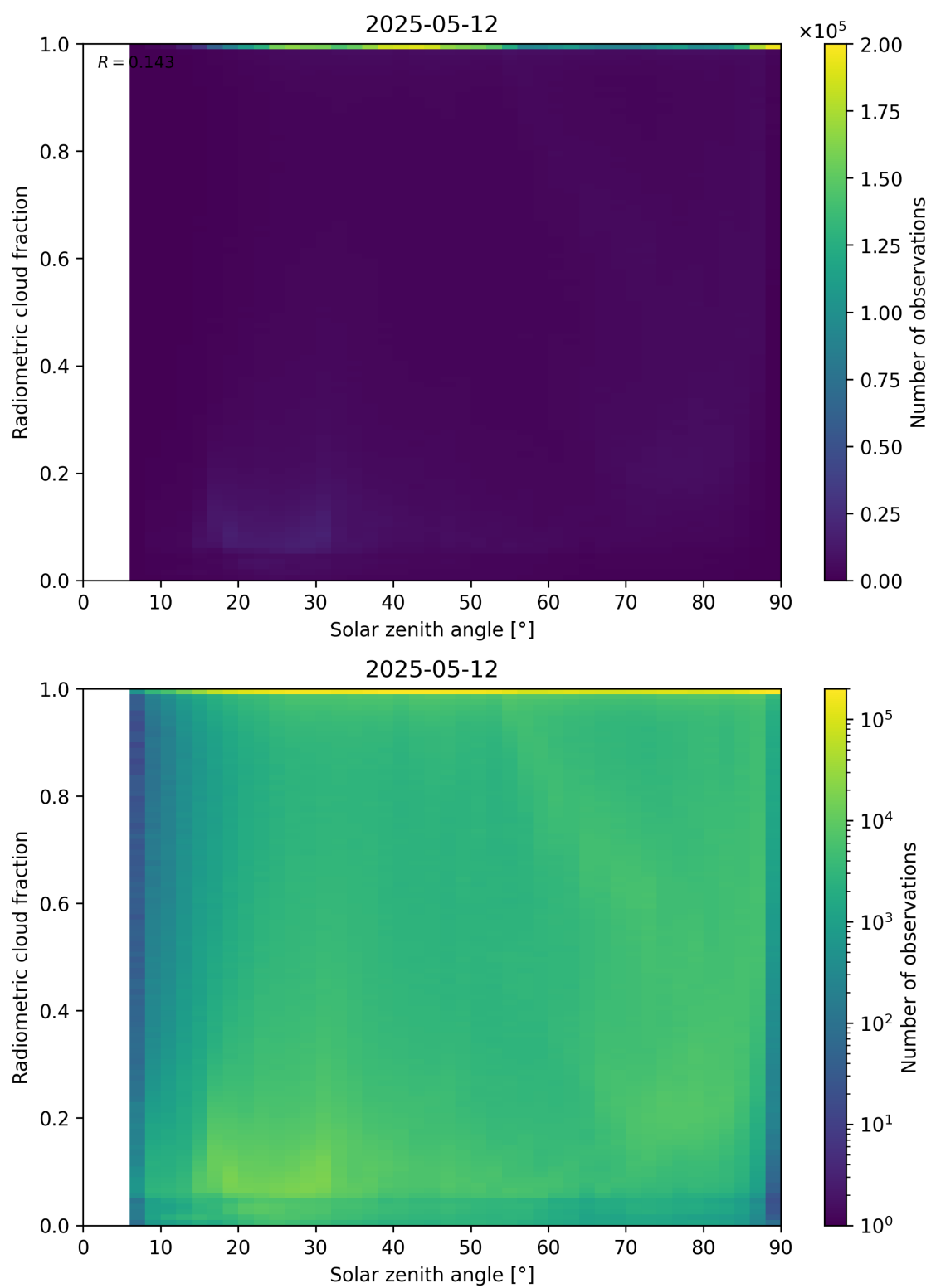
Figure 99: Scatter density plot of “Solar zenith angle” against “Radiometric cloud fraction” for 2025-05-11 to 2025-05-13.
