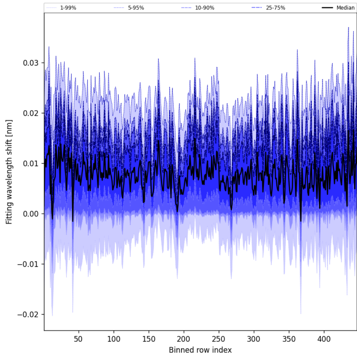
Figure 65: Along track statistics of “Fitting wavelength shift” for 2025-05-11 to 2025-05-13
