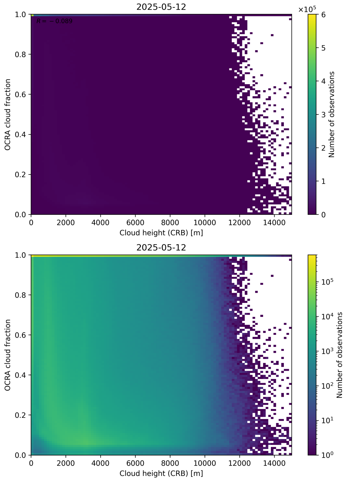
Figure 81: Scatter density plot of “Cloud height (CRB)” against “OCRA cloud fraction” for 2025-05-11 to 2025-05-13.
