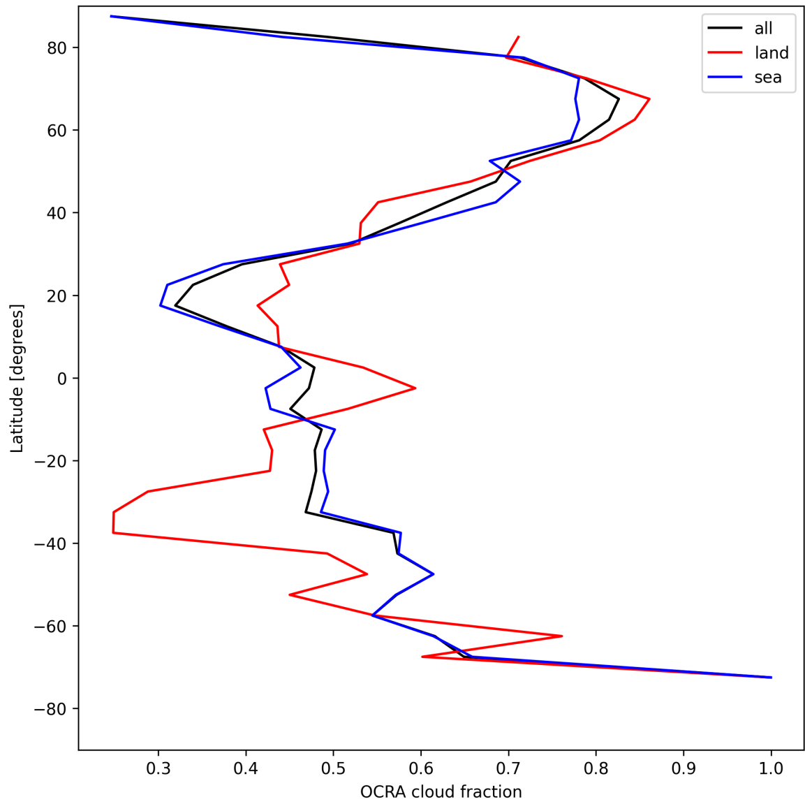
Figure 34: Zonal average of “OCRA cloud fraction” for 2025-05-11 to 2025-05-13.
