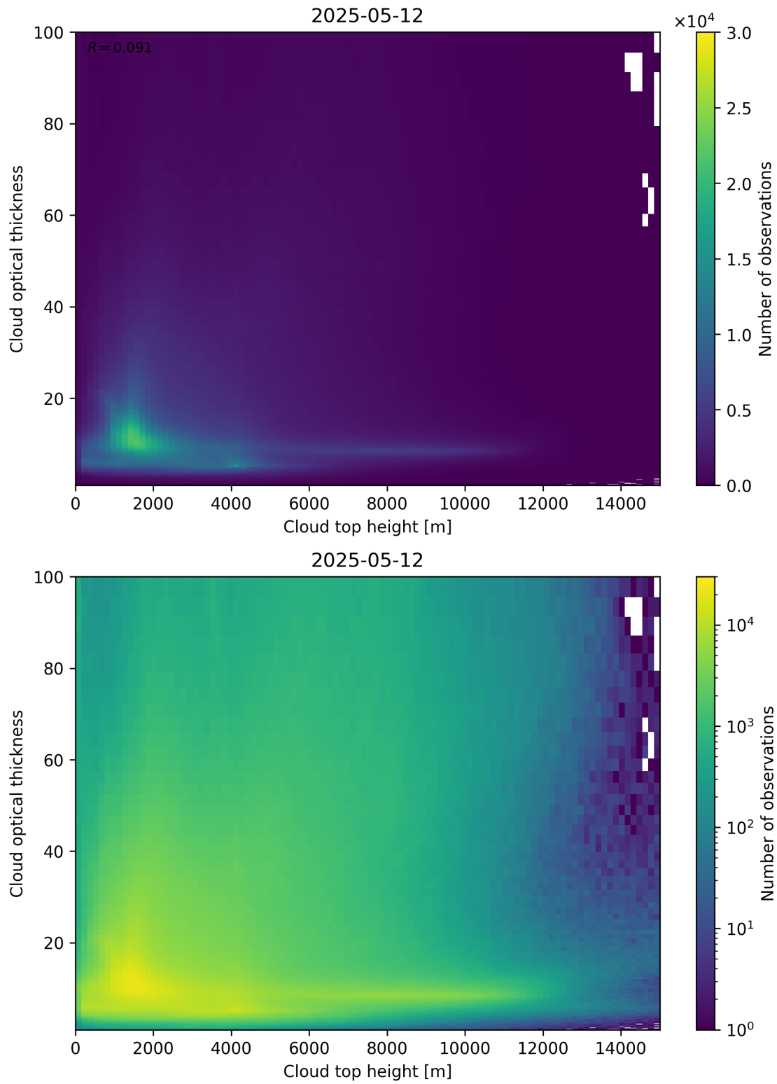
Figure 90: Scatter density plot of “Cloud top height” against “Cloud optical thickness” for 2025-05-11 to 2025-05-13.
