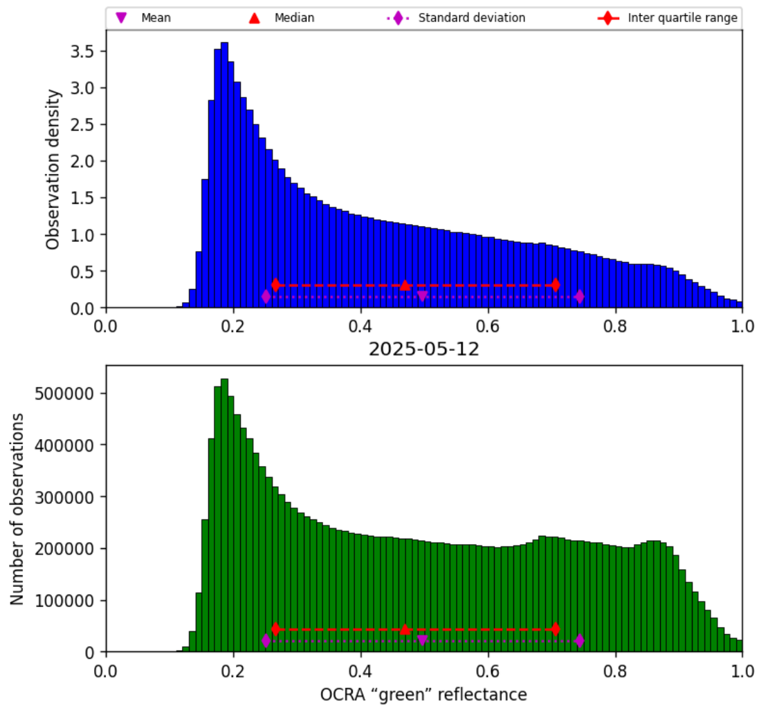
Figure 52: Histogram of “OCRA “green” reflectance” for 2025-05-11 to 2025-05-13
