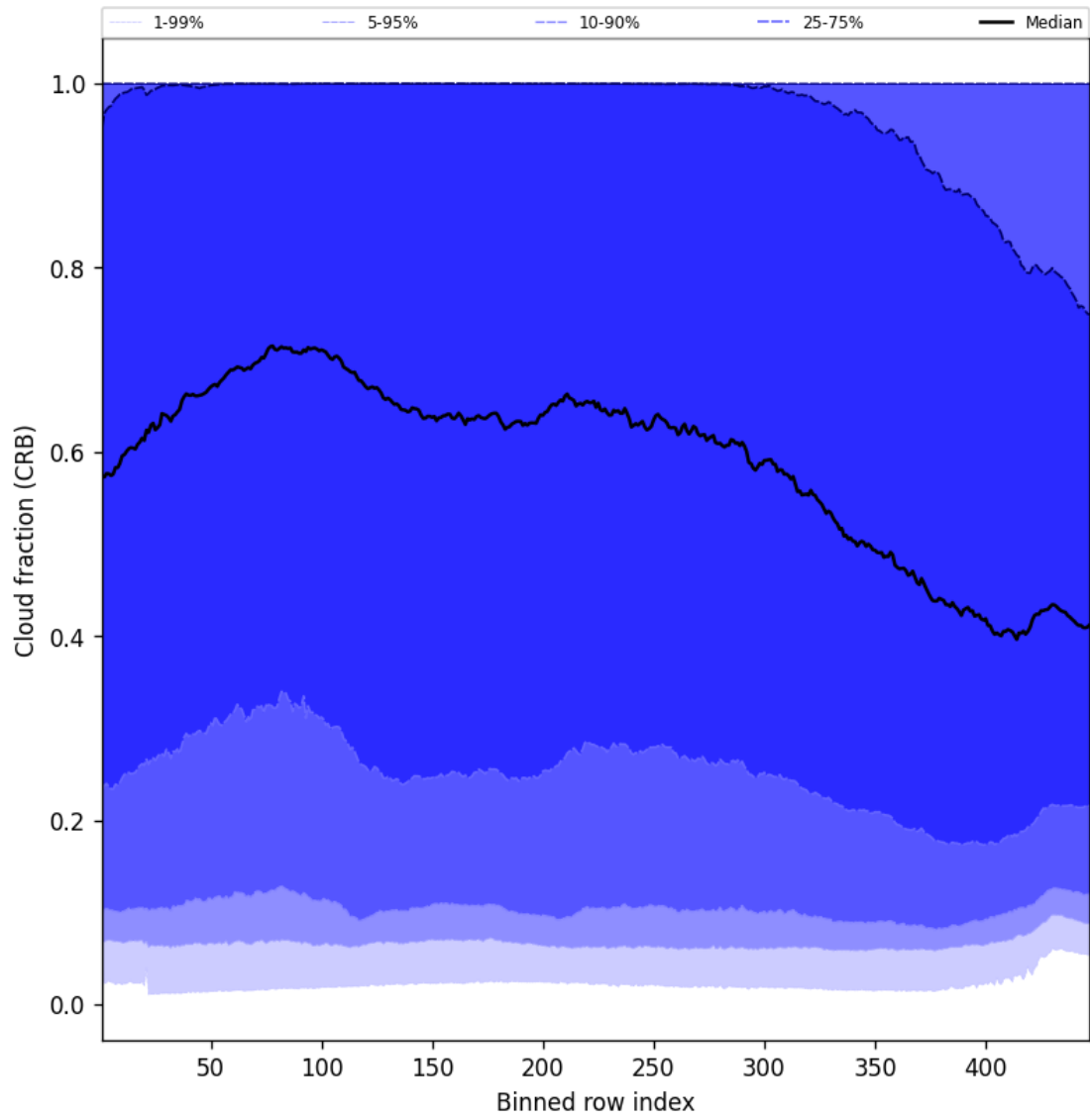
Figure 58: Along track statistics of “Cloud fraction (CRB)” for 2025-05-11 to 2025-05-13
