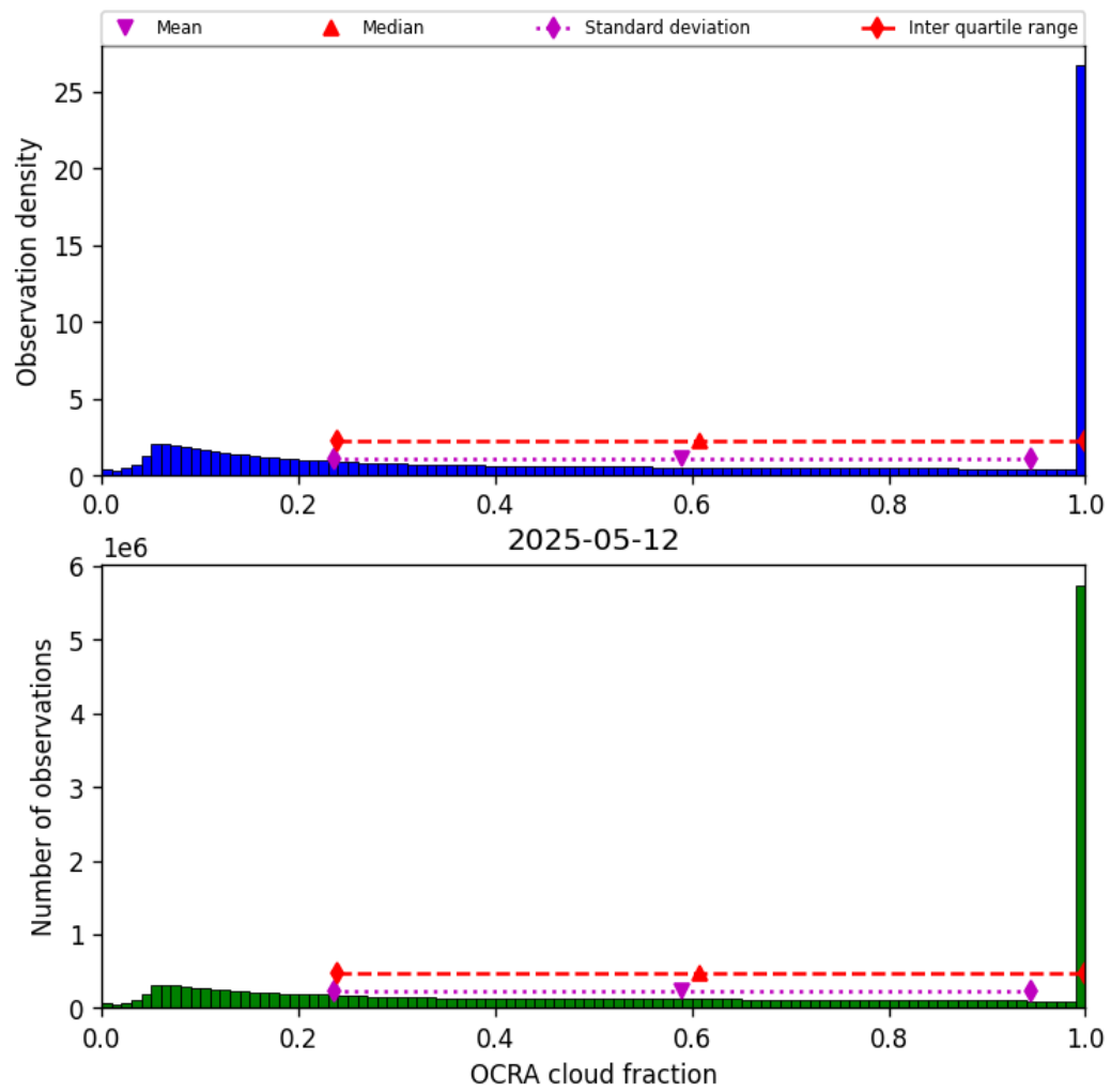
Figure 50: Histogram of “OCRA cloud fraction” for 2025-05-11 to 2025-05-13
