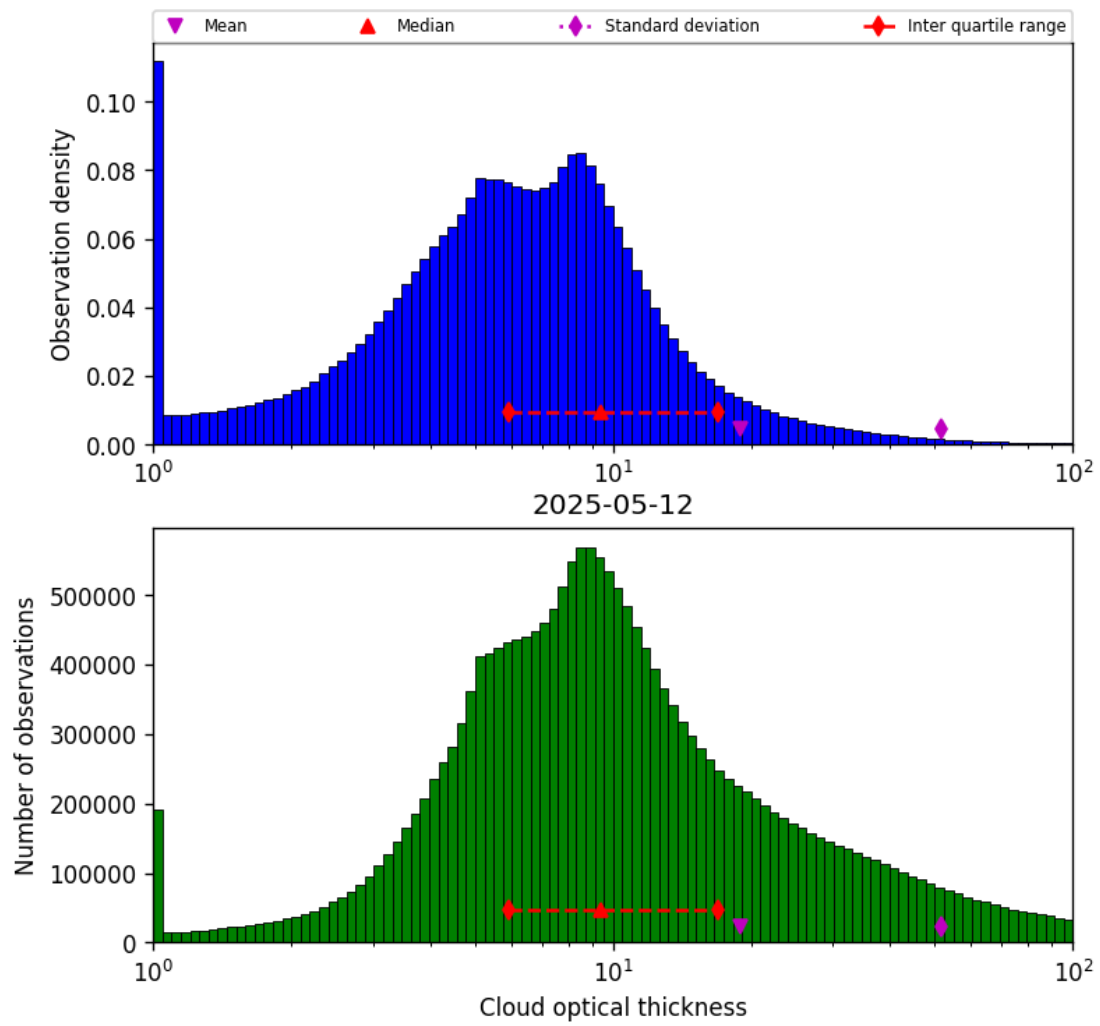
Figure 41: Histogram of “Cloud optical thickness” for 2025-05-11 to 2025-05-13
