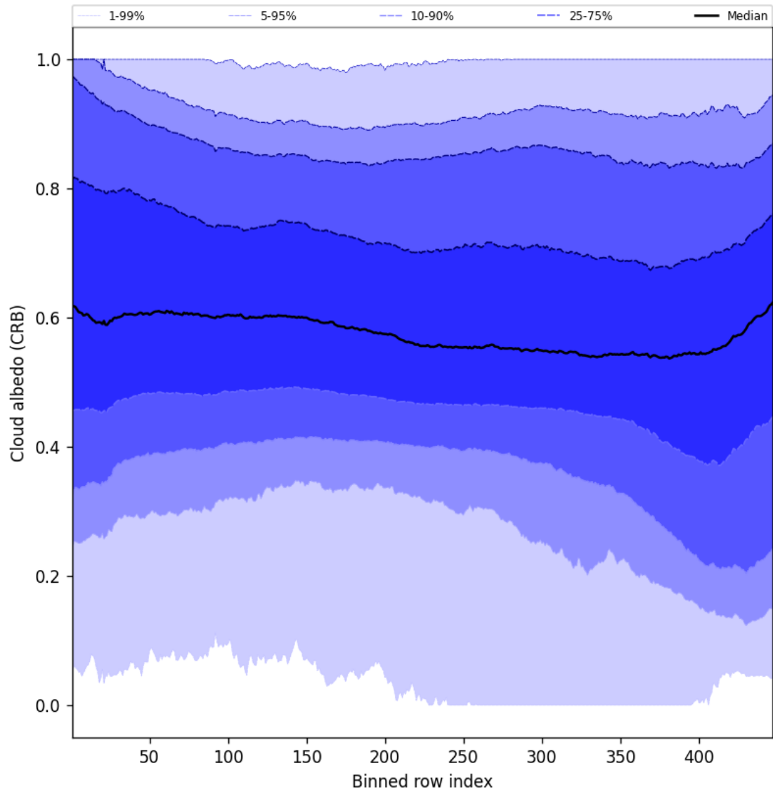
Figure 60: Along track statistics of “Cloud albedo (CRB)” for 2025-05-11 to 2025-05-13
