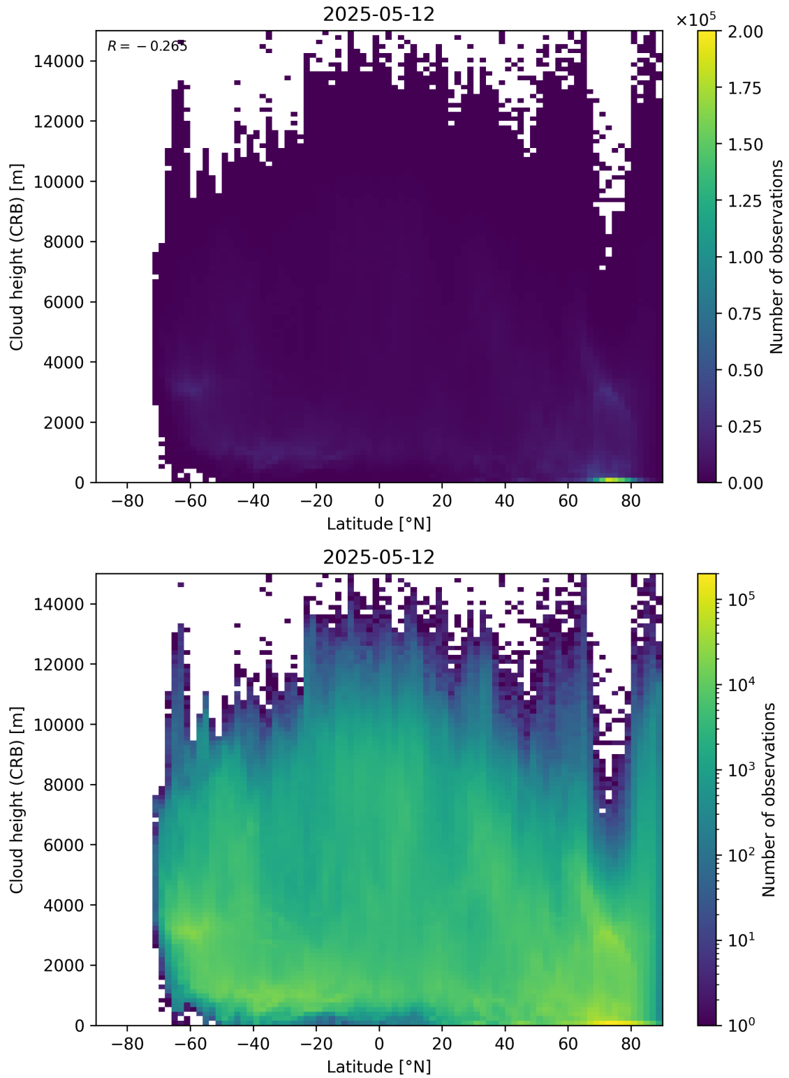
Figure 95: Scatter density plot of “Latitude” against “Cloud height (CRB)” for 2025-05-11 to 2025-05-13.
