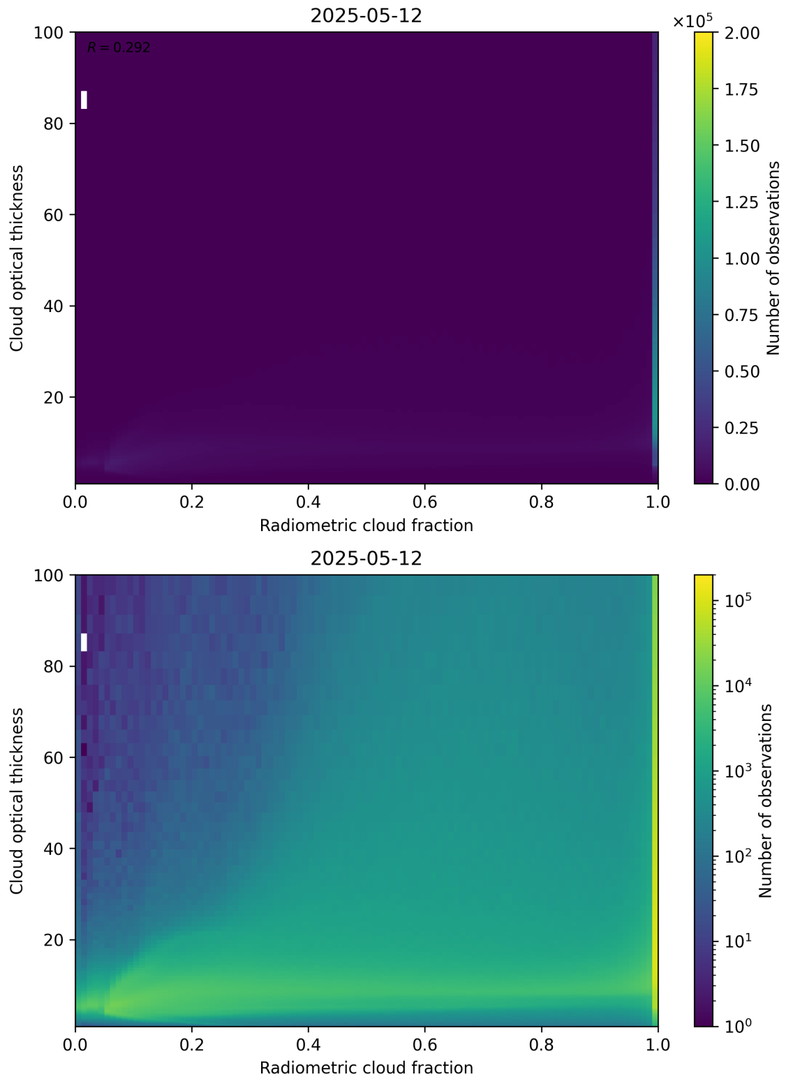
Figure 75: Scatter density plot of “Radiometric cloud fraction” against “Cloud optical thickness” for 2025-05-11 to 2025-05-13.
