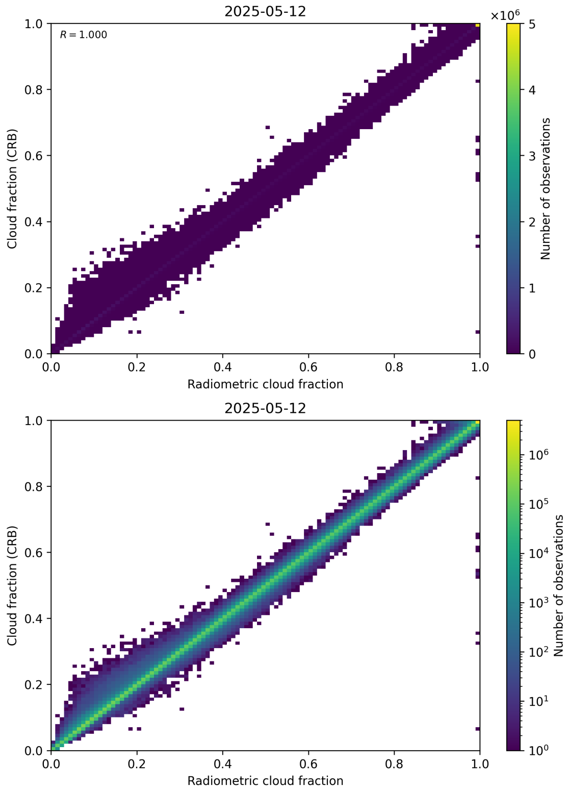
Figure 73: Scatter density plot of “Radiometric cloud fraction” against “Cloud fraction (CRB)” for 2025-05-11 to 2025-05-13.
