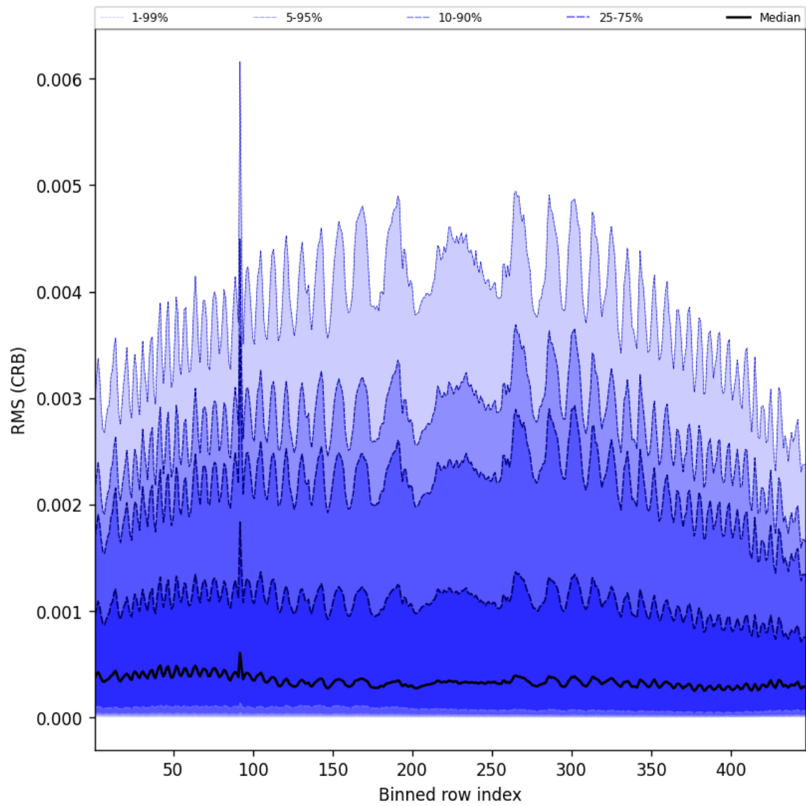
Figure 64: Along track statistics of “RMS (CRB)” for 2025-05-11 to 2025-05-13
