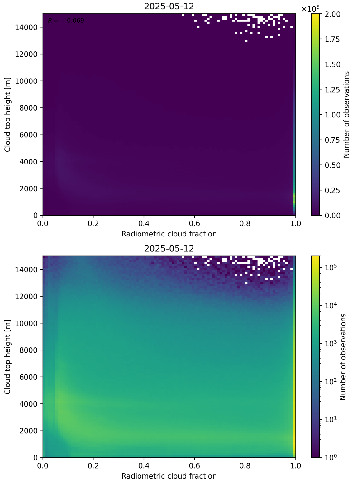
Figure 76: Scatter density plot of “Radiometric cloud fraction” against “Cloud top height” for 2025-05-11 to 2025-05-13.
