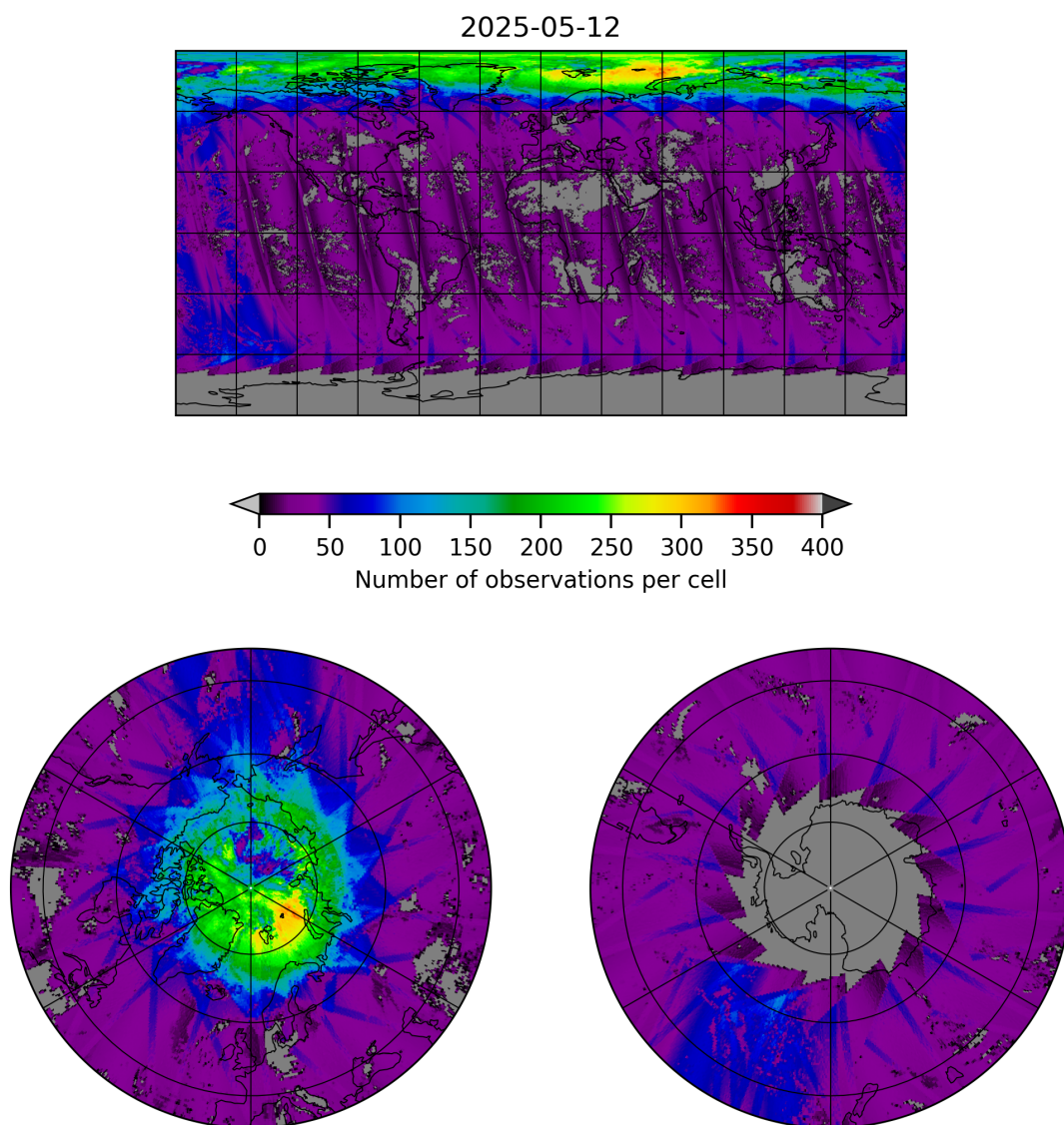
Figure 21: Map of the number of observations for 2025-05-11 to 2025-05-13
