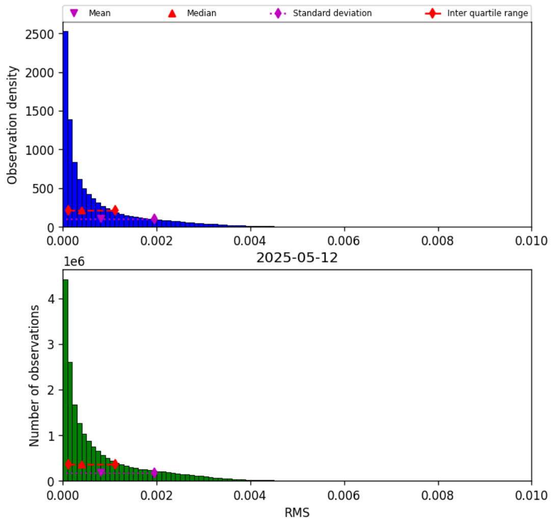
Figure 47: Histogram of “RMS” for 2025-05-11 to 2025-05-13
