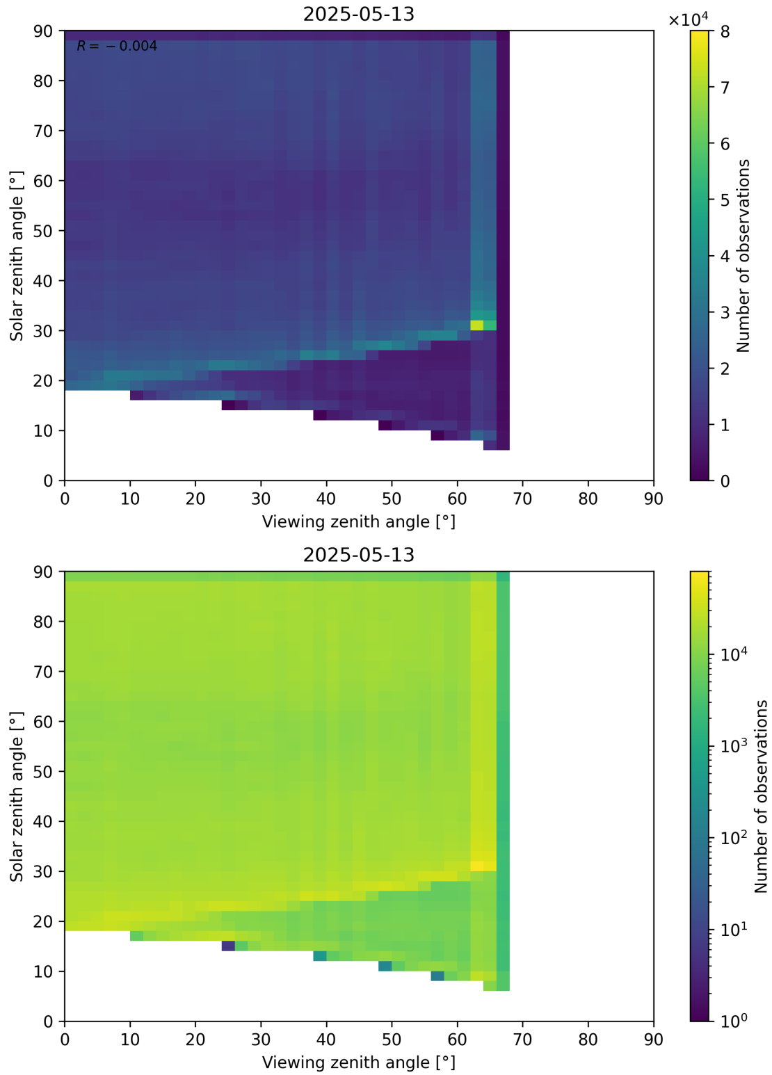
Figure 114: Scatter density plot of “Viewing zenith angle” against “Solar zenith angle” for 2025-05-12 to 2025-05-14.
