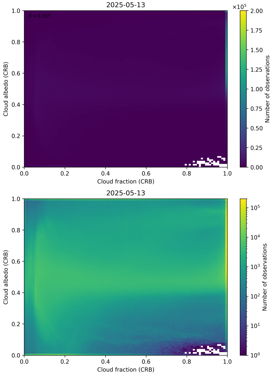
Figure 77: Scatter density plot of “Cloud fraction (CRB)” against “Cloud albedo (CRB)” for 2025-05-12 to 2025-05-14.
