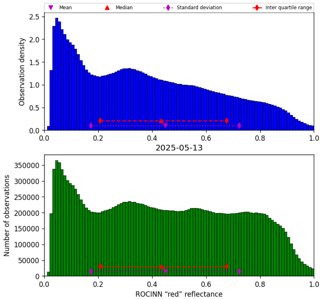
Figure 53: Histogram of “ROCINN “red” reflectance” for 2025-05-12 to 2025-05-14
