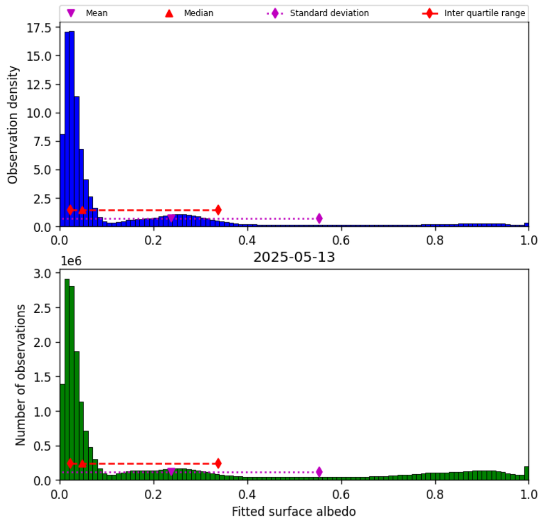
Figure 45: Histogram of “Fitted surface albedo” for 2025-05-12 to 2025-05-14
