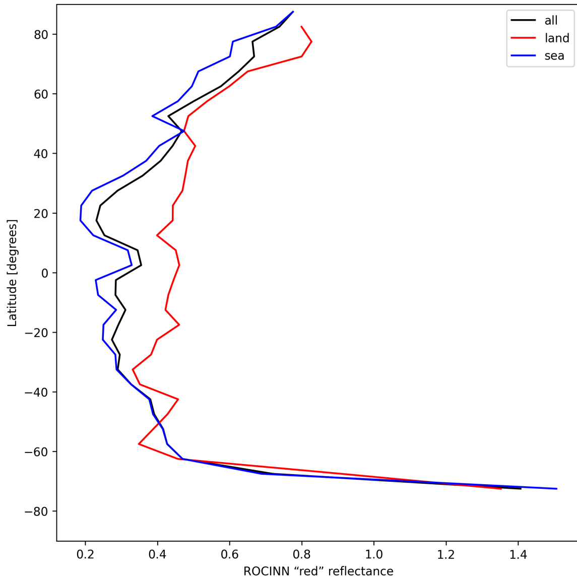
Figure 37: Zonal average of “ROCINN “red” reflectance” for 2025-05-12 to 2025-05-14.
