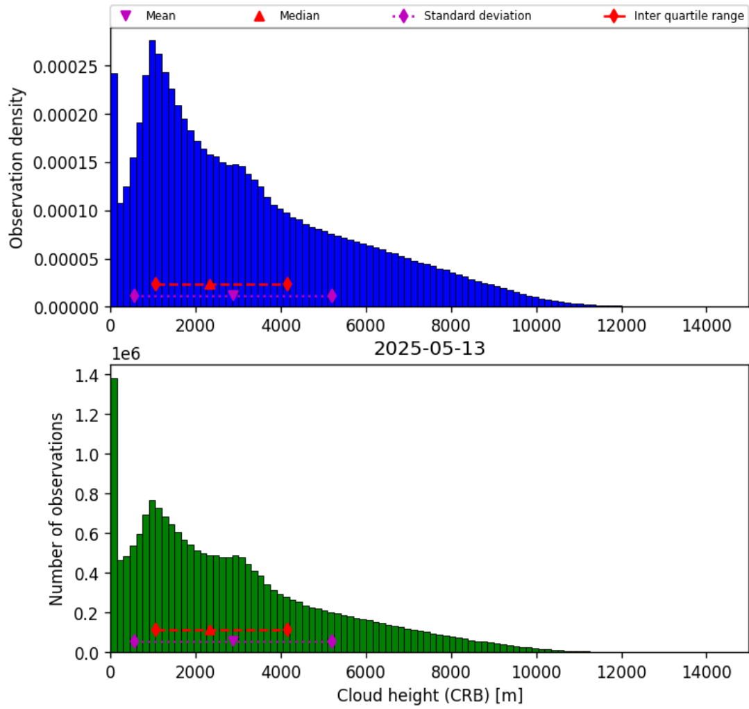
Figure 43: Histogram of “Cloud height (CRB)” for 2025-05-12 to 2025-05-14
