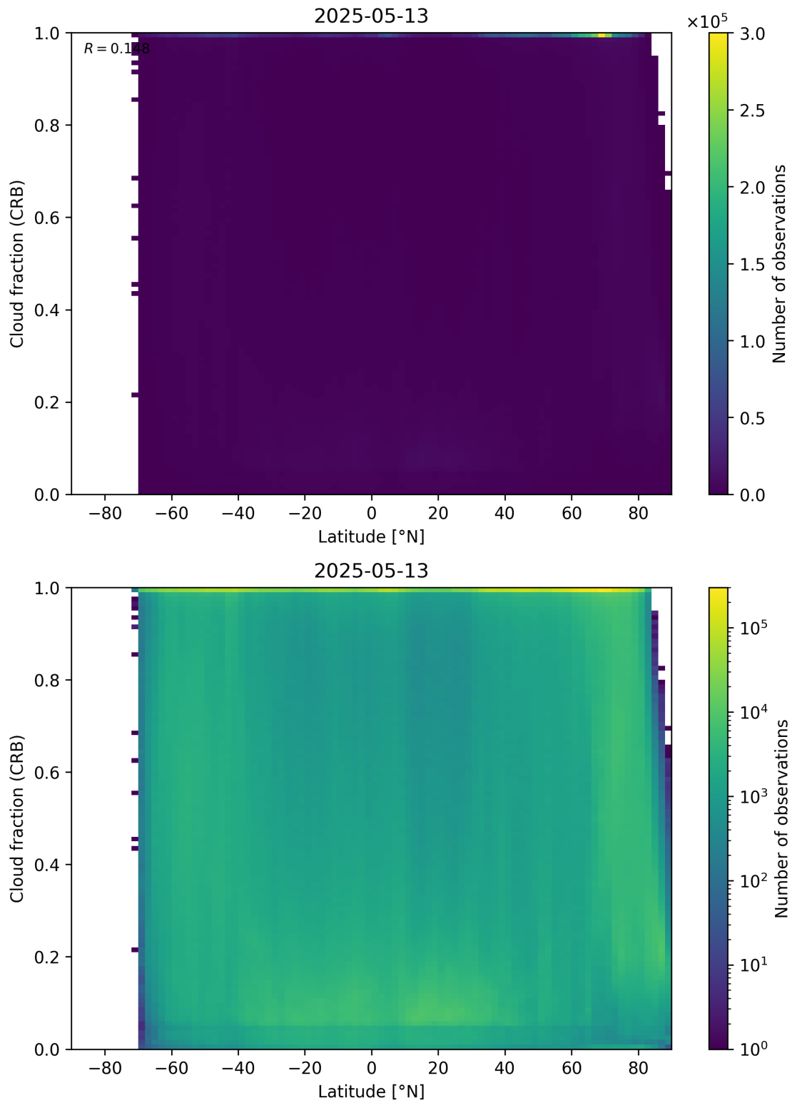
Figure 94: Scatter density plot of “Latitude” against “Cloud fraction (CRB)” for 2025-05-12 to 2025-05-14.
