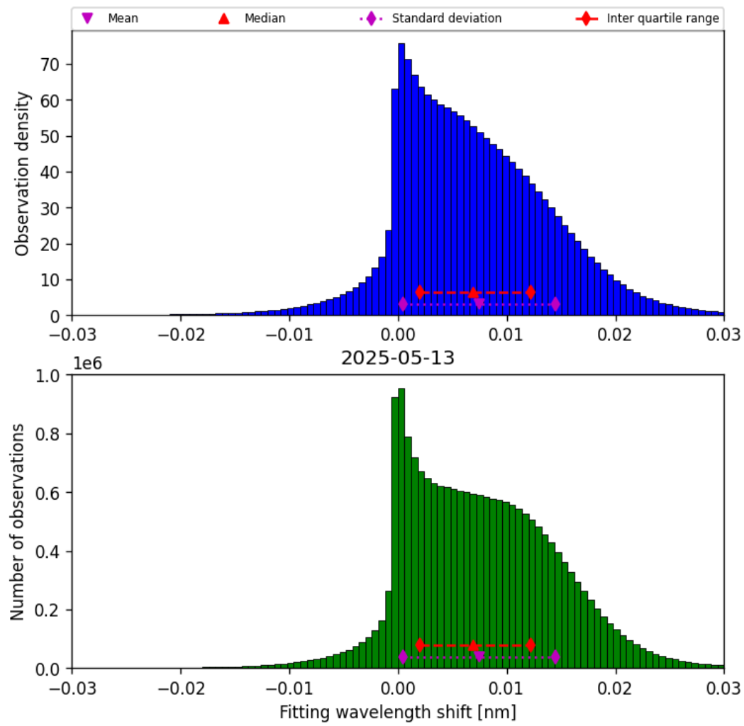
Figure 49: Histogram of “Fitting wavelength shift” for 2025-05-12 to 2025-05-14
