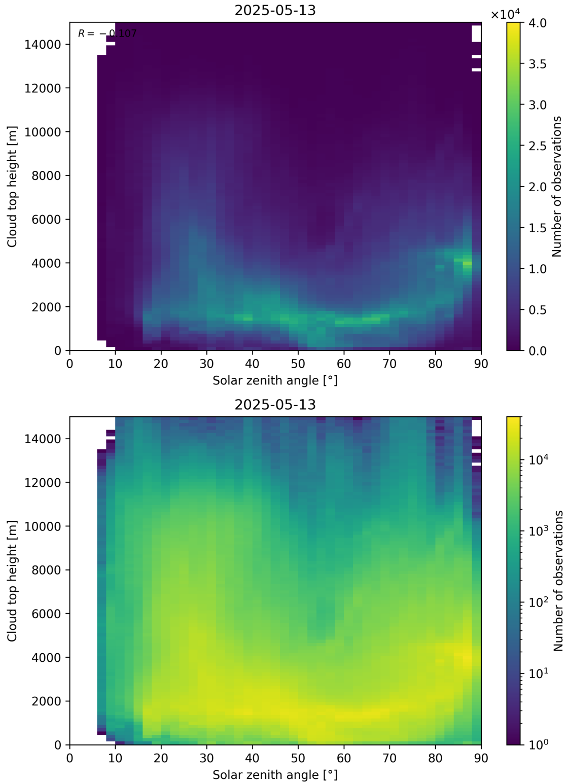
Figure 104: Scatter density plot of “Solar zenith angle” against “Cloud top height” for 2025-05-12 to 2025-05-14.
