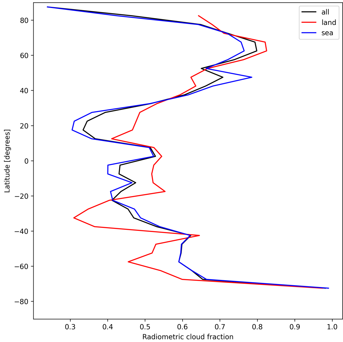
Figure 23: Zonal average of “Radiometric cloud fraction” for 2025-05-12 to 2025-05-14.
