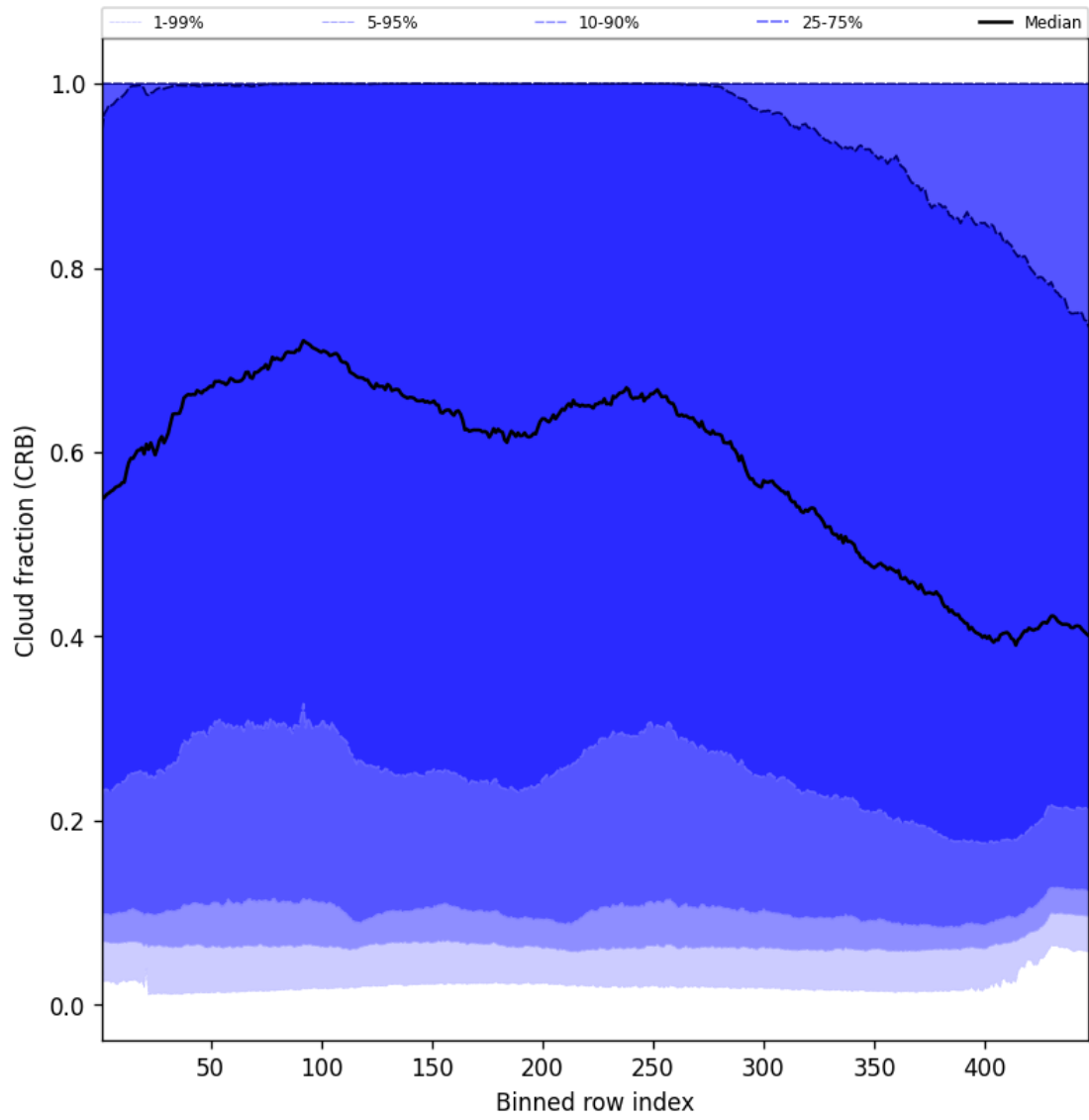
Figure 58: Along track statistics of “Cloud fraction (CRB)” for 2025-05-12 to 2025-05-14
