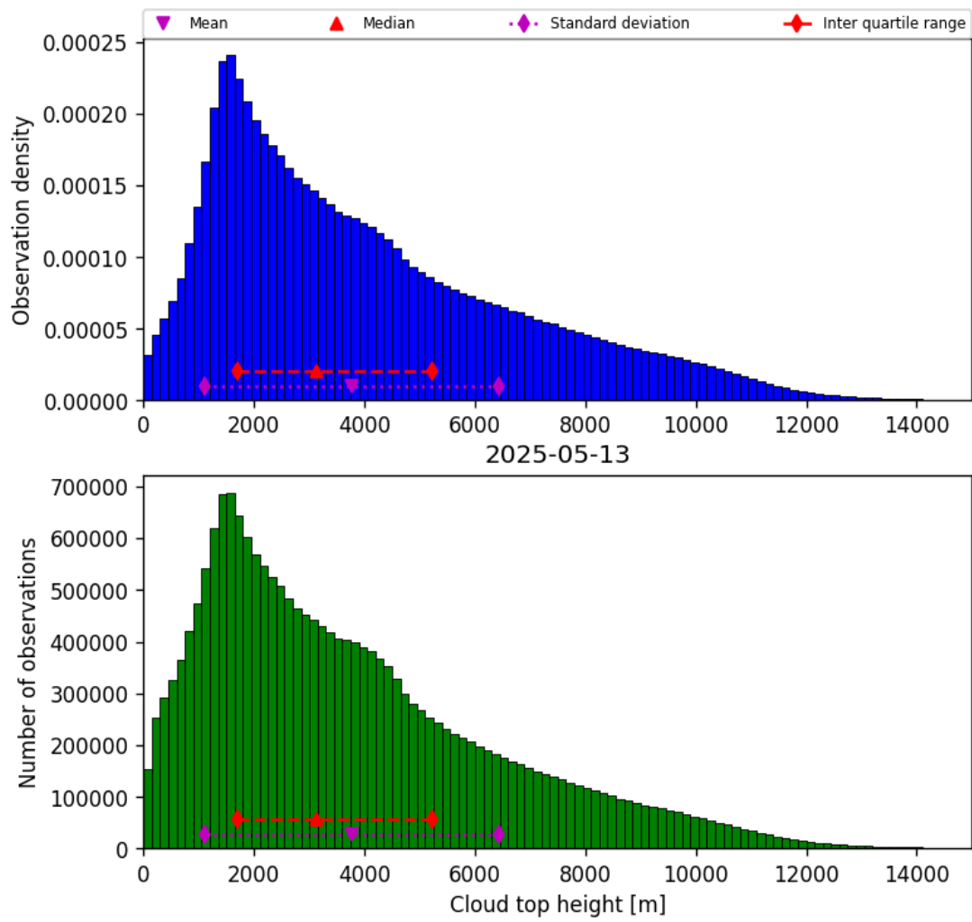
Figure 40: Histogram of “Cloud top height” for 2025-05-12 to 2025-05-14
