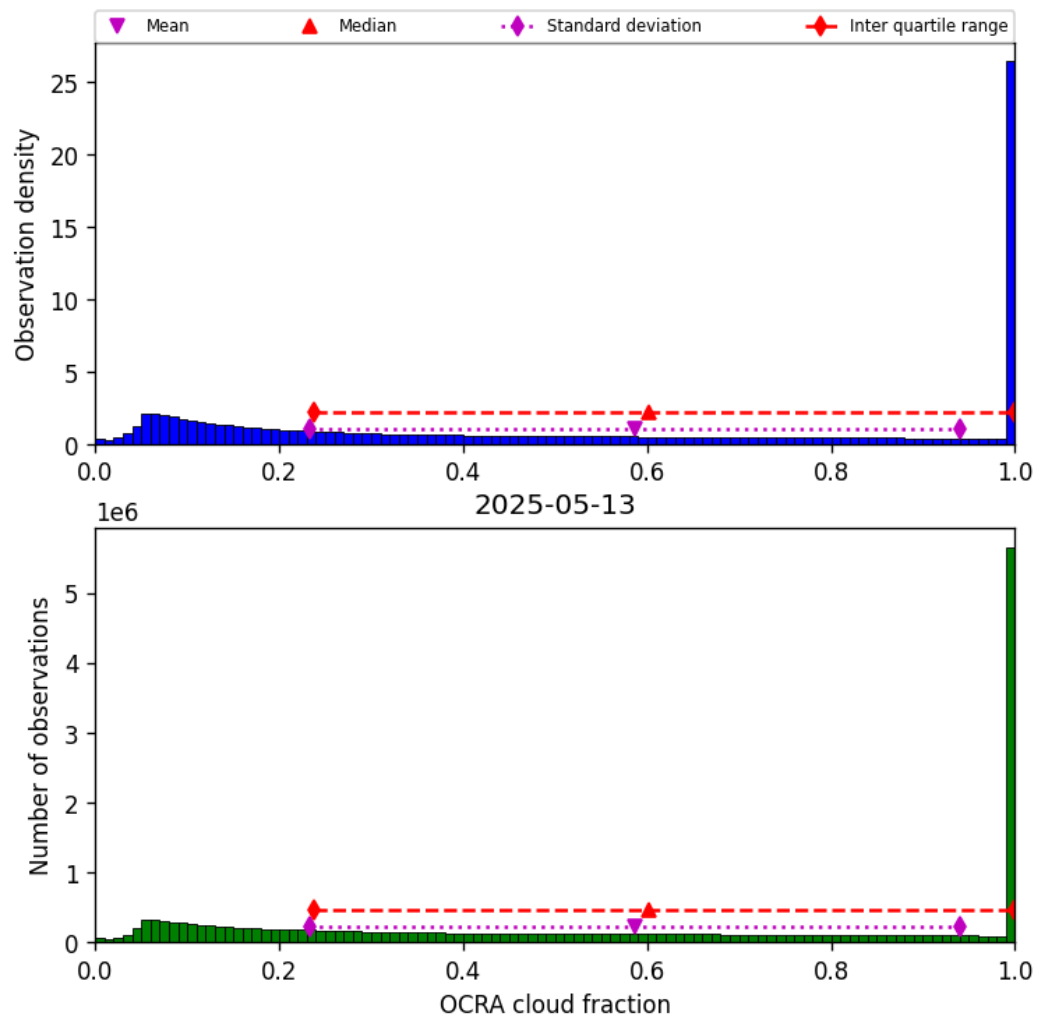
Figure 50: Histogram of “OCRA cloud fraction” for 2025-05-12 to 2025-05-14
