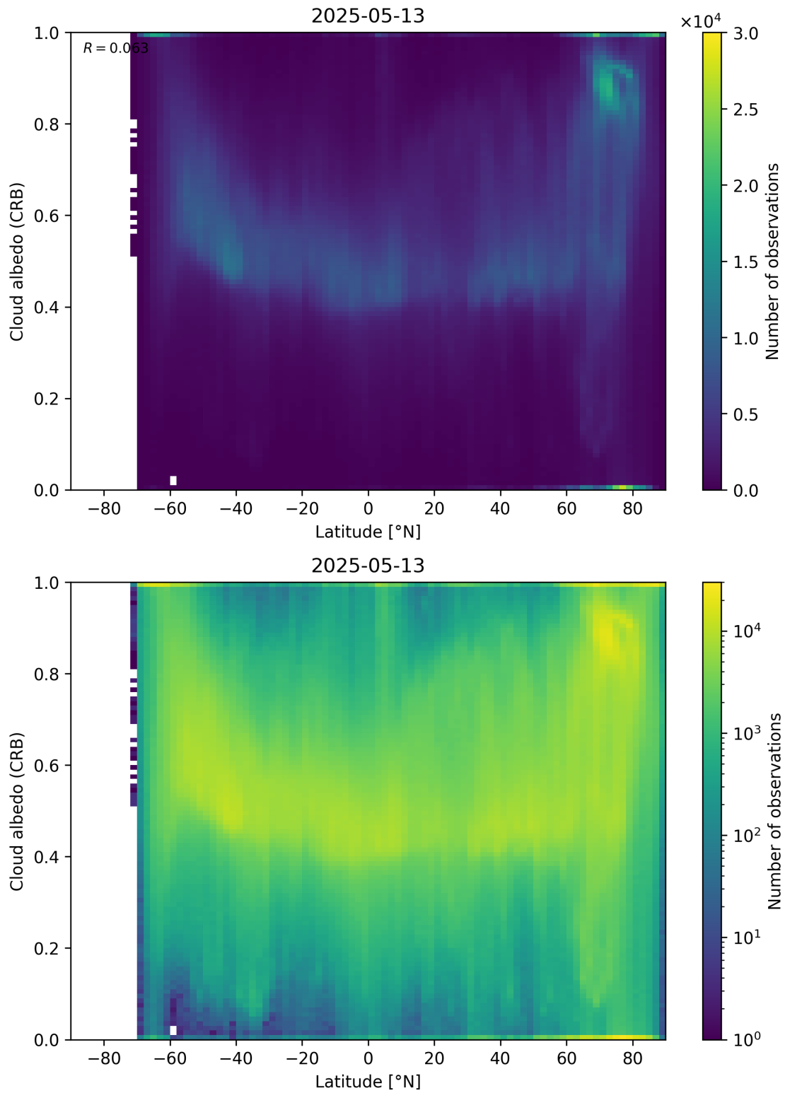
Figure 91: Scatter density plot of “Latitude” against “Cloud albedo (CRB)” for 2025-05-12 to 2025-05-14.
