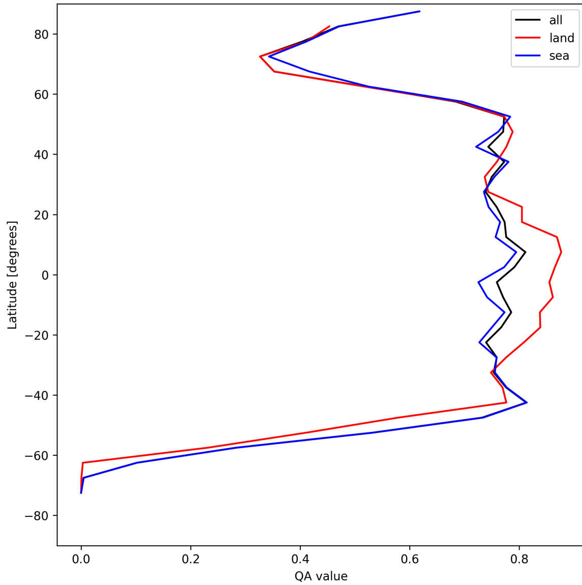
Figure 22: Zonal average of “QA value” for 2025-05-12 to 2025-05-14.
