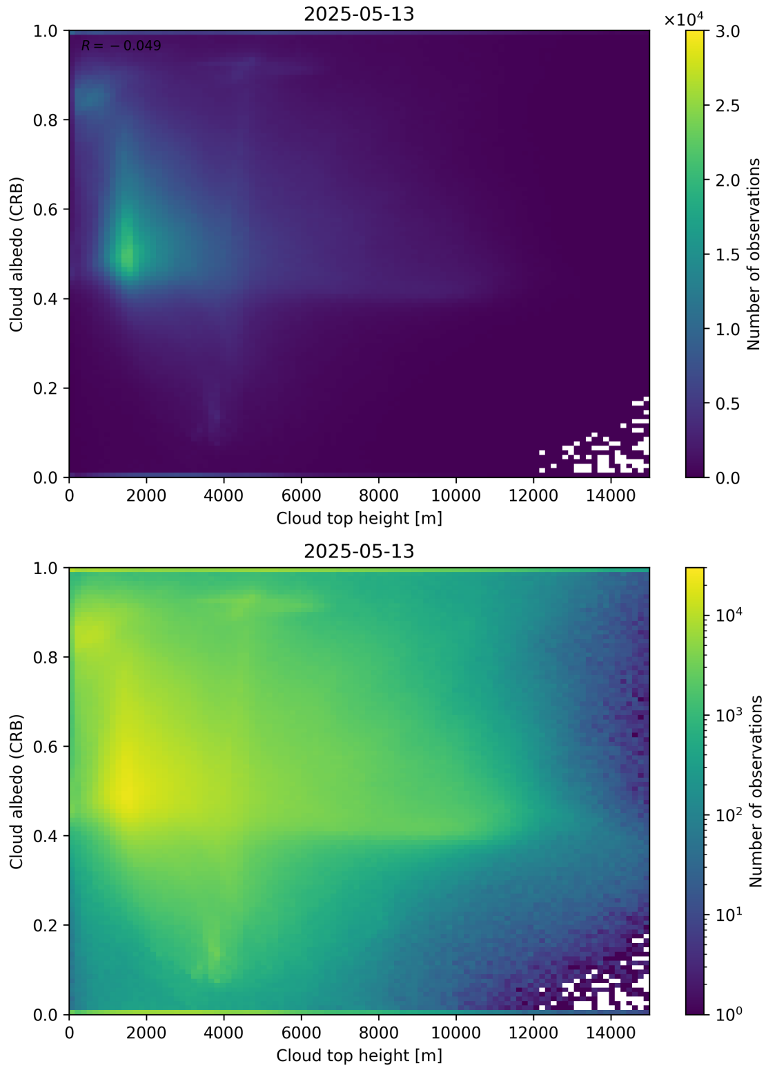
Figure 86: Scatter density plot of “Cloud top height” against “Cloud albedo (CRB)” for 2025-05-12 to 2025-05-14.
