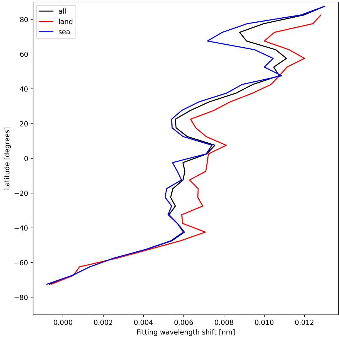
Figure 33: Zonal average of “Fitting wavelength shift” for 2025-05-12 to 2025-05-14.
