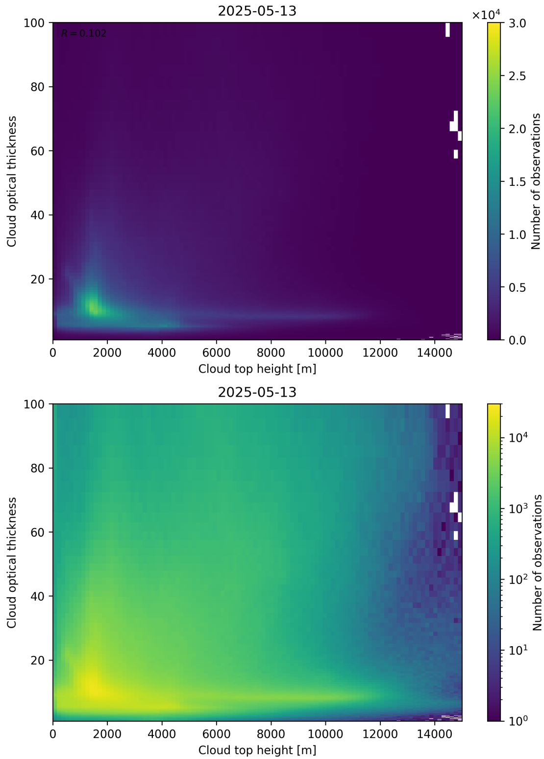
Figure 90: Scatter density plot of “Cloud top height” against “Cloud optical thickness” for 2025-05-12 to 2025-05-14.
