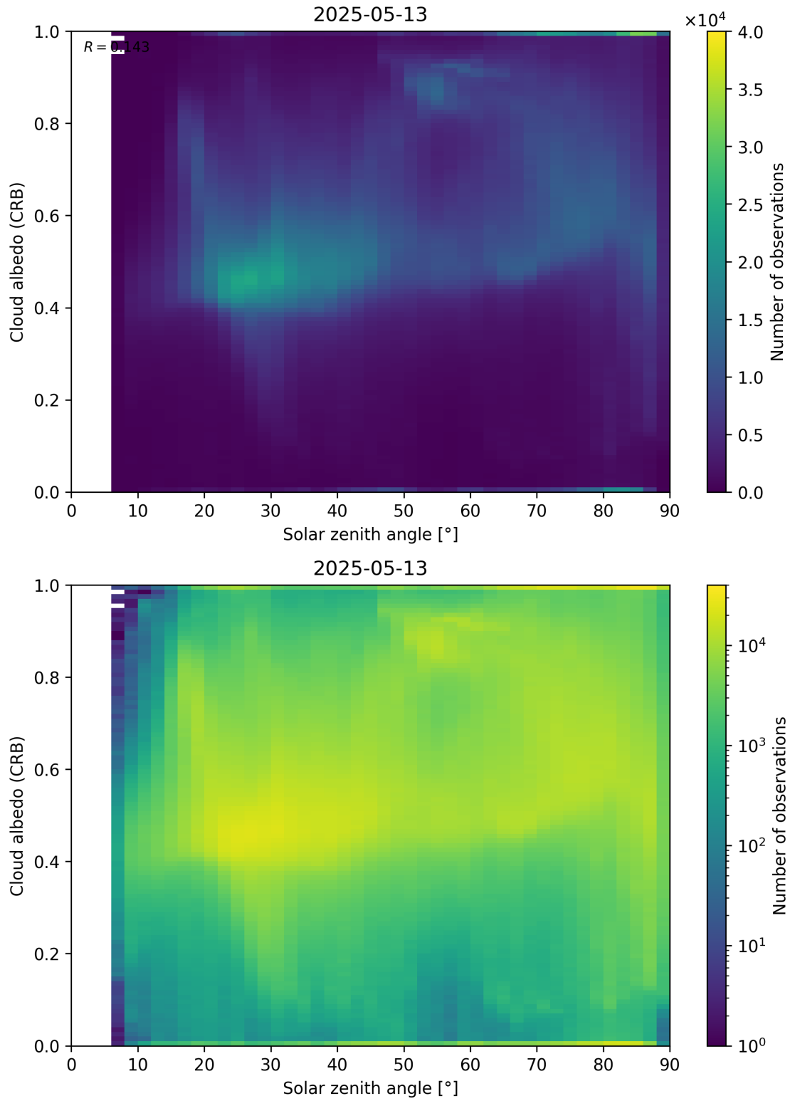
Figure 98: Scatter density plot of “Solar zenith angle” against “Cloud albedo (CRB)” for 2025-05-12 to 2025-05-14.
