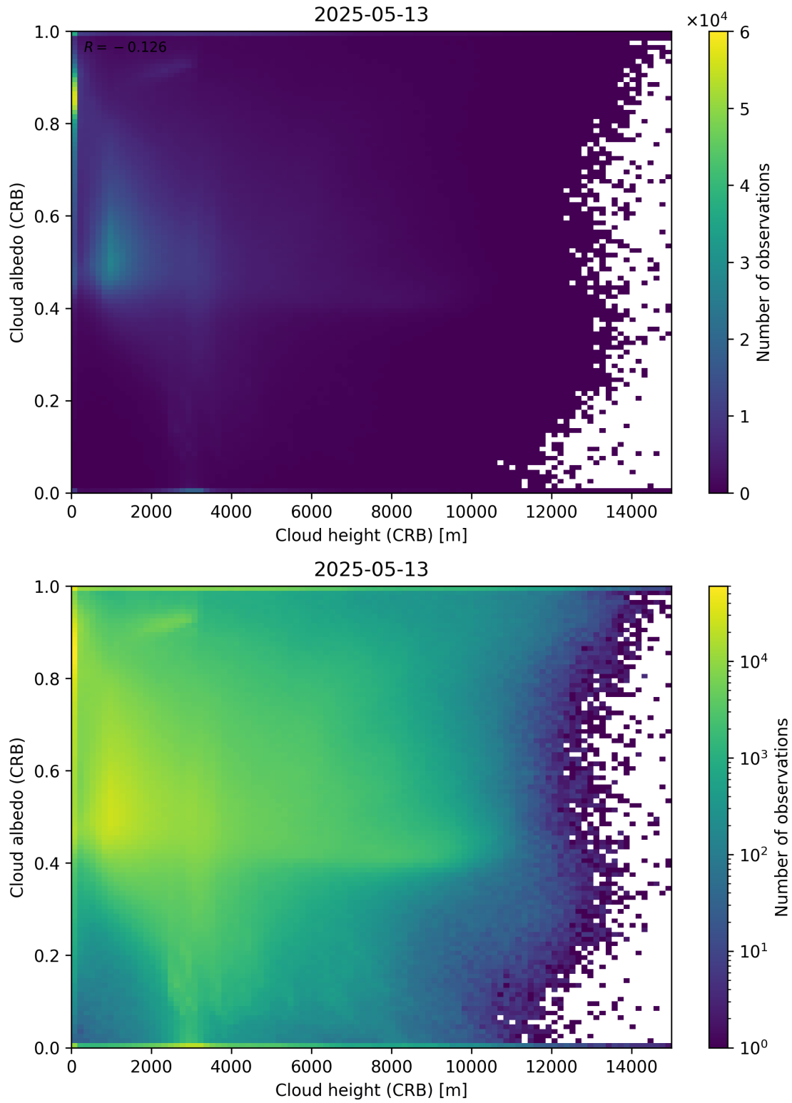
Figure 80: Scatter density plot of “Cloud height (CRB)” against “Cloud albedo (CRB)” for 2025-05-12 to 2025-05-14.
