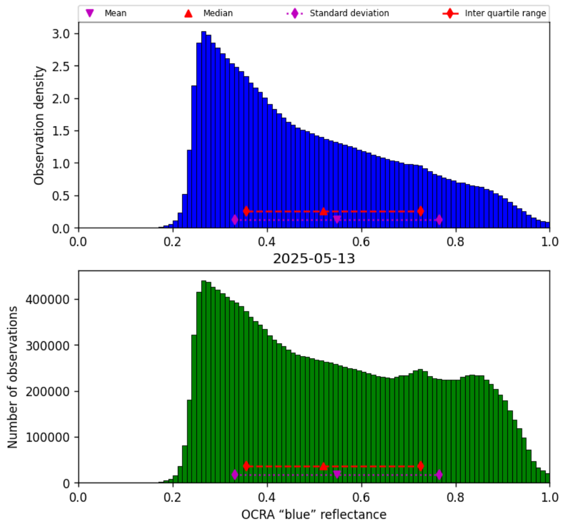
Figure 51: Histogram of “OCRA “blue” reflectance” for 2025-05-12 to 2025-05-14
