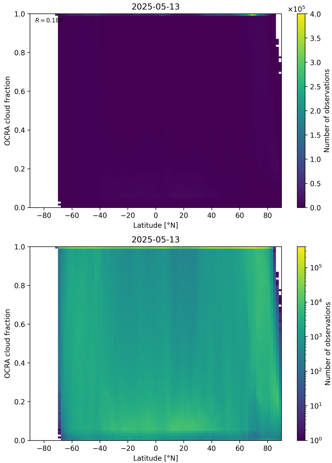
Figure 93: Scatter density plot of “Latitude” against “OCRA cloud fraction” for 2025-05-12 to 2025-05-14.
