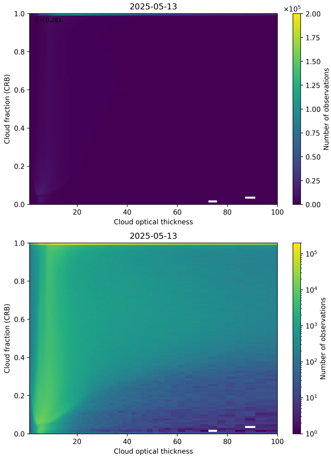
Figure 84: Scatter density plot of “Cloud optical thickness” against “Cloud fraction (CRB)” for 2025-05-12 to 2025-05-14.
