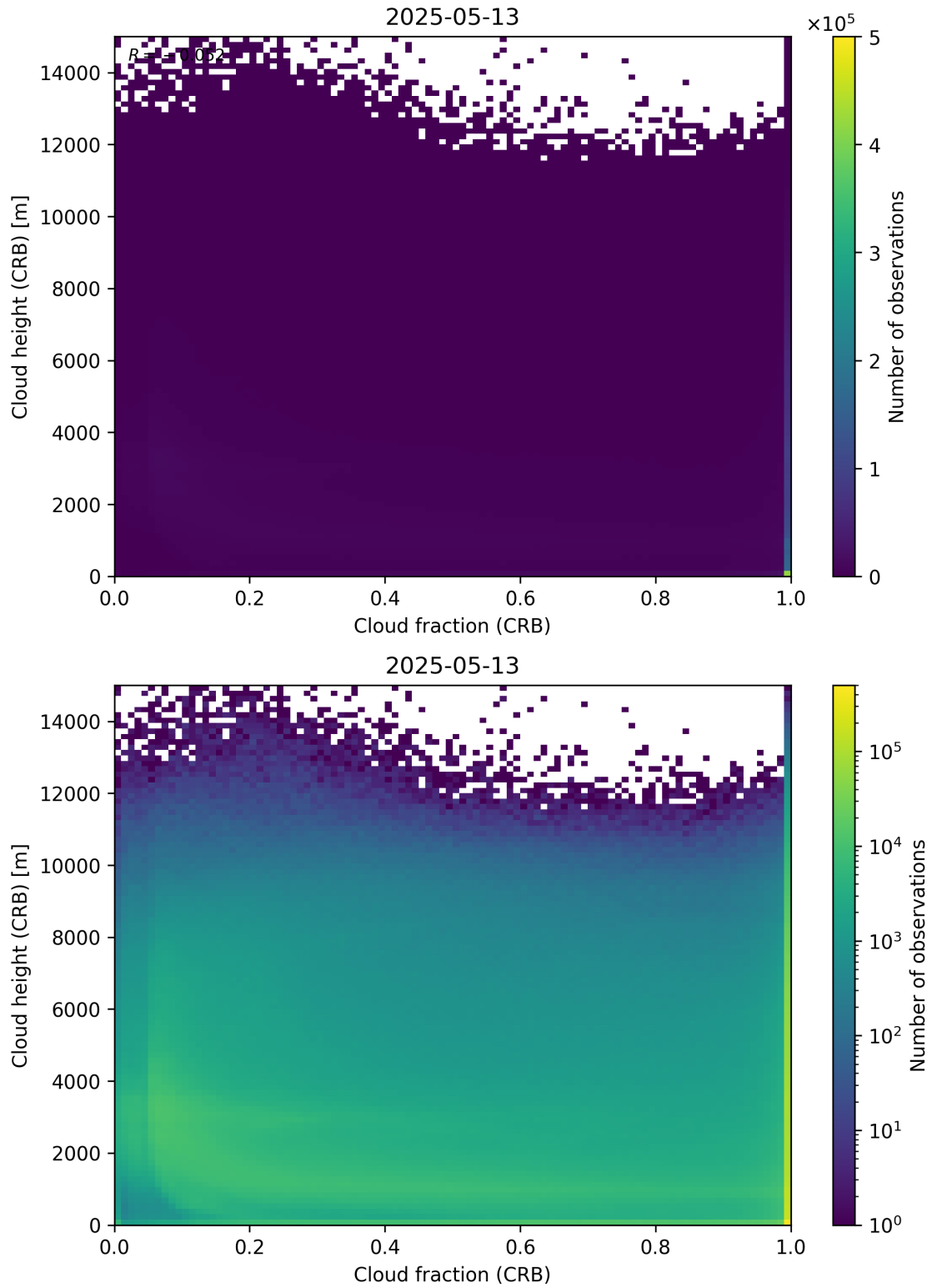
Figure 79: Scatter density plot of “Cloud fraction (CRB)” against “Cloud height (CRB)” for 2025-05-12 to 2025-05-14.
