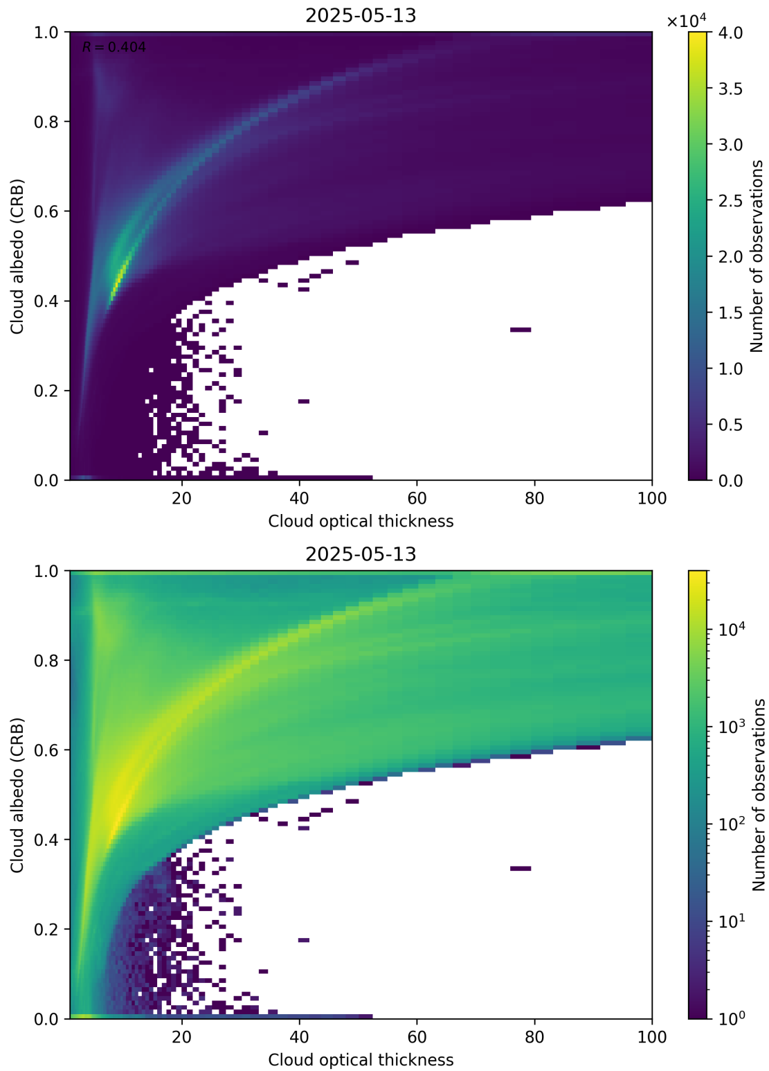
Figure 82: Scatter density plot of “Cloud optical thickness” against “Cloud albedo (CRB)” for 2025-05-12 to 2025-05-14.
