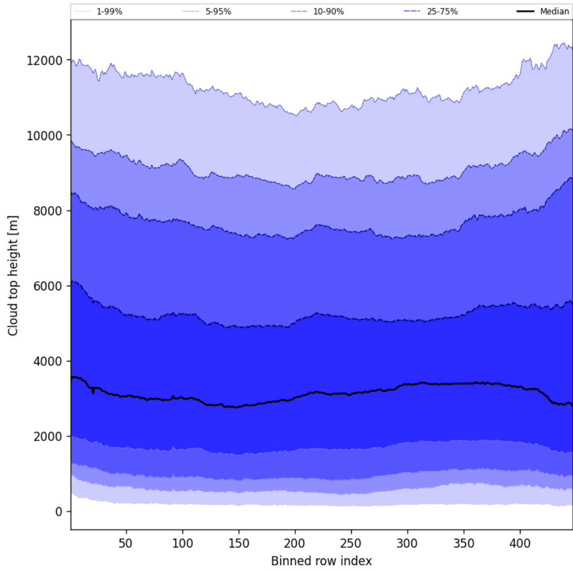
Figure 56: Along track statistics of “Cloud top height” for 2025-05-12 to 2025-05-14
