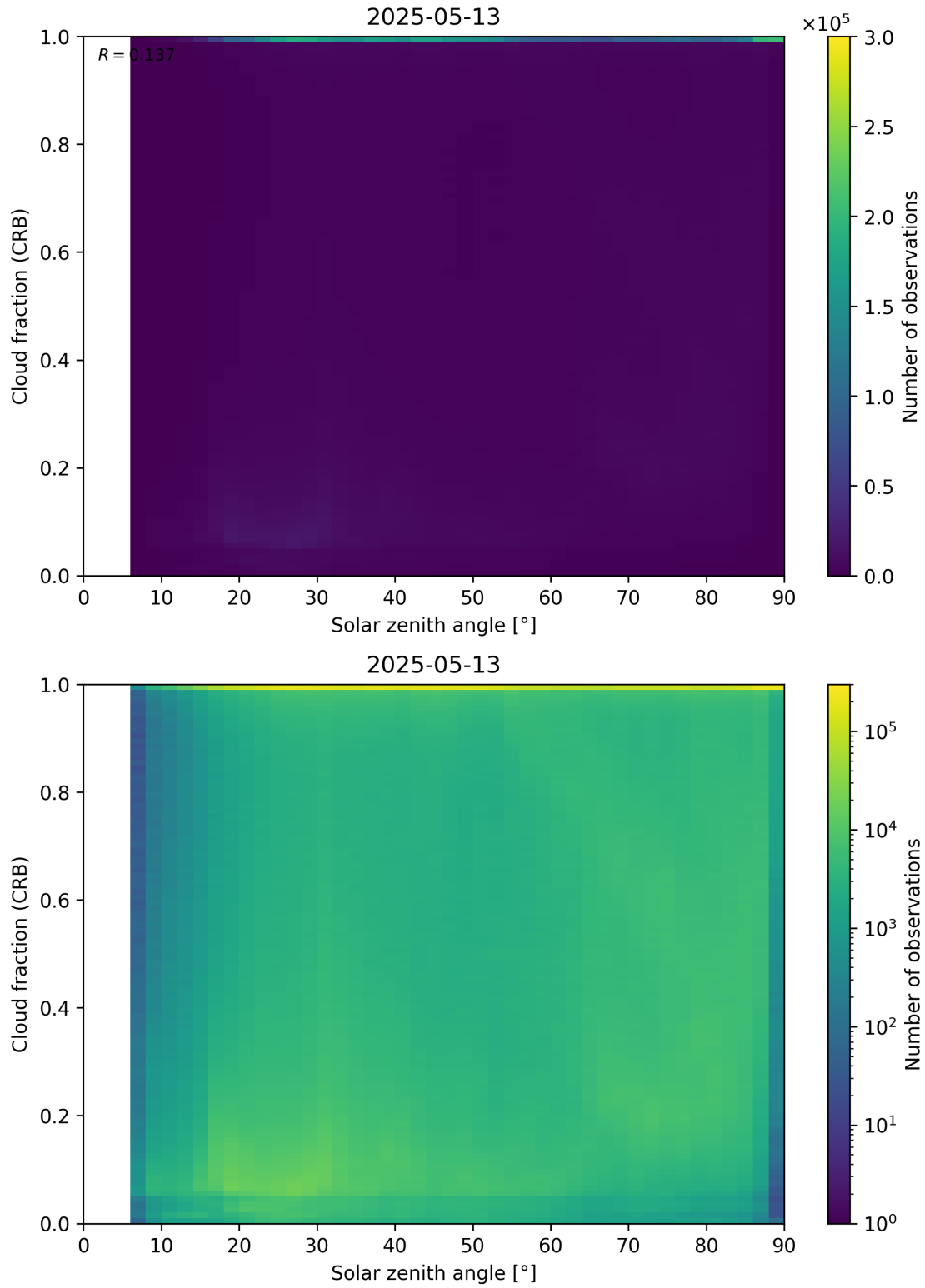
Figure 101: Scatter density plot of “Solar zenith angle” against “Cloud fraction (CRB)” for 2025-05-12 to 2025-05-14.
