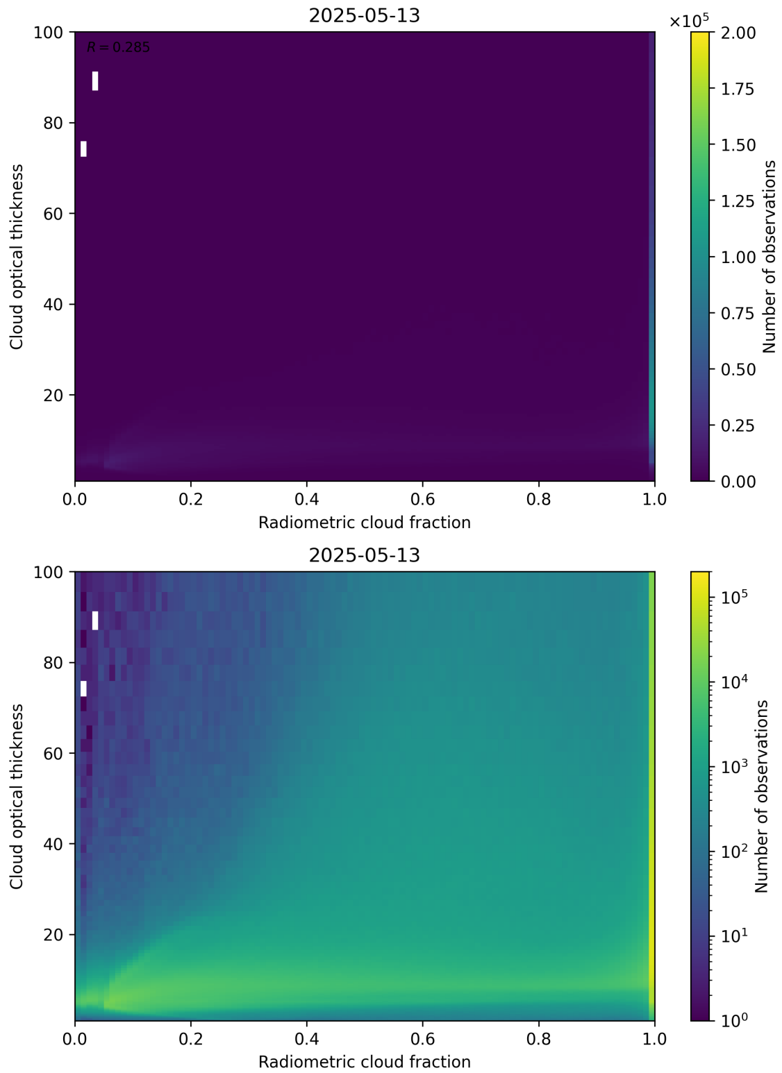
Figure 75: Scatter density plot of “Radiometric cloud fraction” against “Cloud optical thickness” for 2025-05-12 to 2025-05-14.
