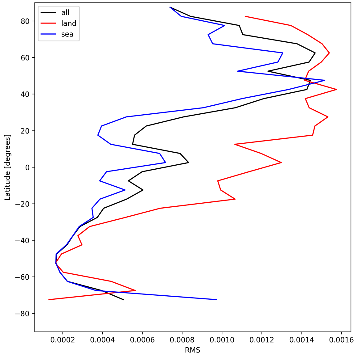
Figure 31: Zonal average of “RMS” for 2025-05-12 to 2025-05-14.
