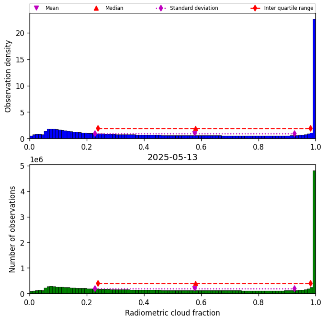
Figure 39: Histogram of “Radiometric cloud fraction” for 2025-05-12 to 2025-05-14
