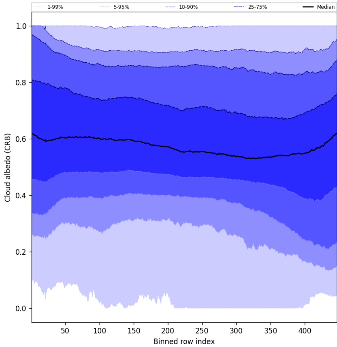
Figure 60: Along track statistics of “Cloud albedo (CRB)” for 2025-05-12 to 2025-05-14
