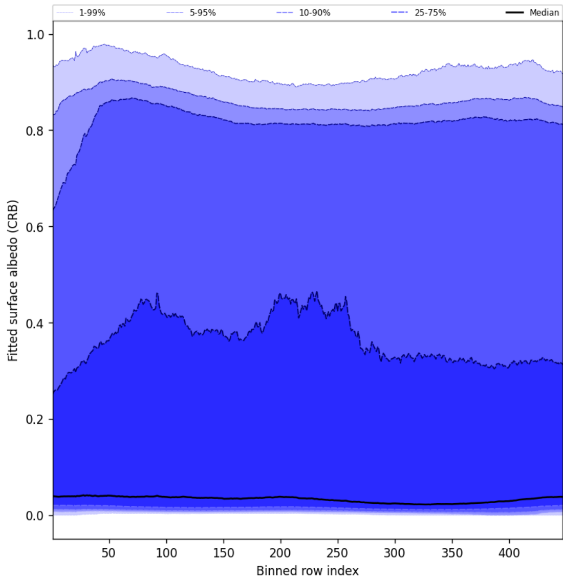
Figure 62: Along track statistics of “Fitted surface albedo (CRB)” for 2025-05-12 to 2025-05-14
