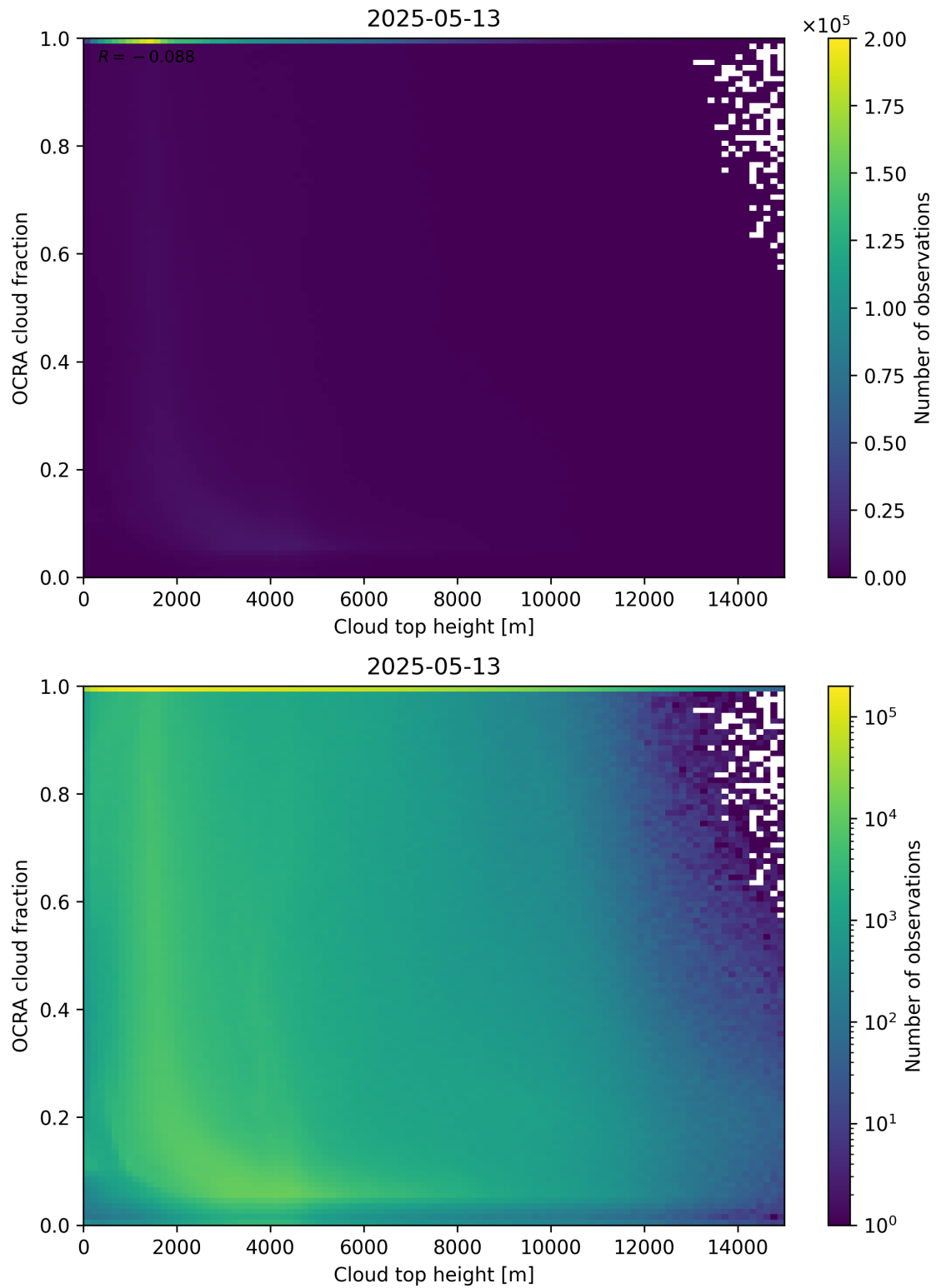
Figure 87: Scatter density plot of “Cloud top height” against “OCRA cloud fraction” for 2025-05-12 to 2025-05-14.
