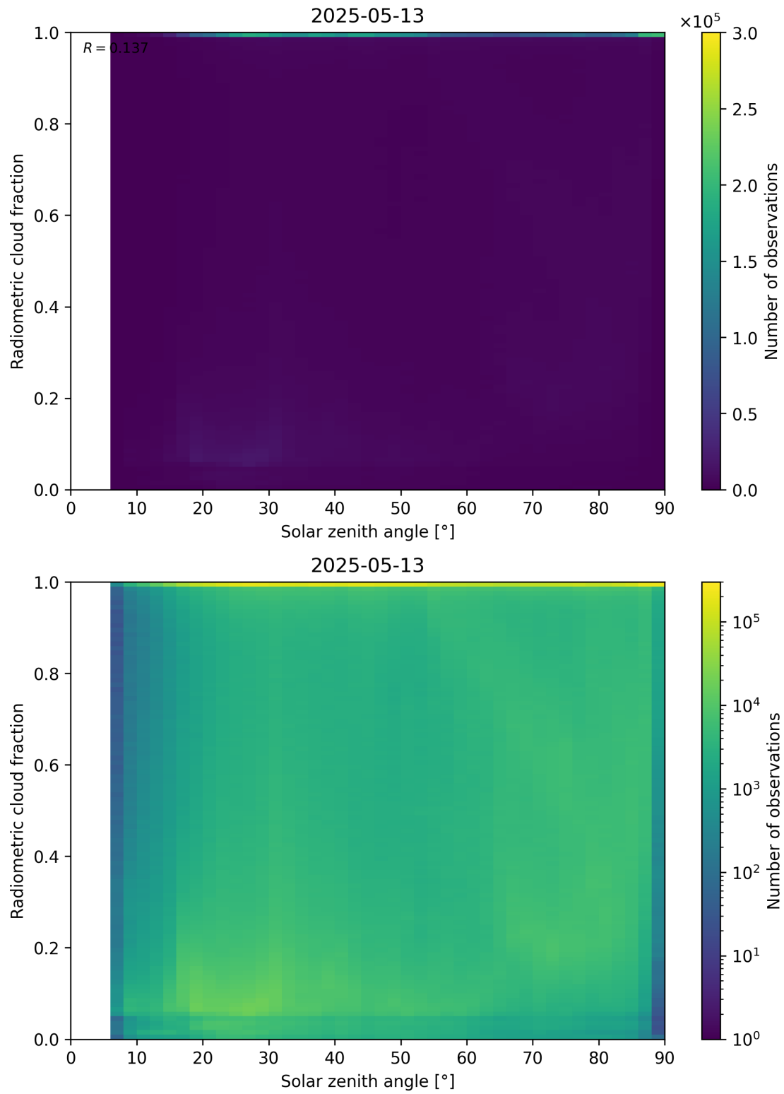
Figure 99: Scatter density plot of “Solar zenith angle” against “Radiometric cloud fraction” for 2025-05-12 to 2025-05-14.
