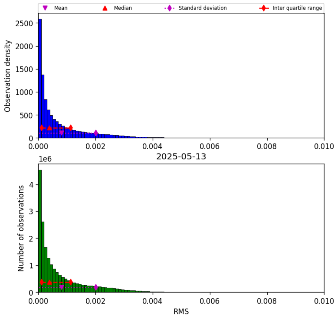
Figure 47: Histogram of “RMS” for 2025-05-12 to 2025-05-14
