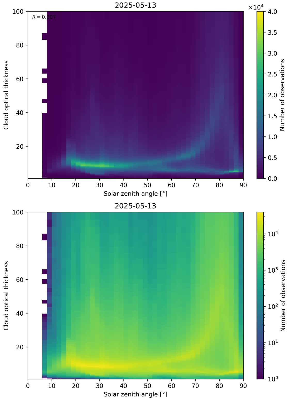
Figure 103: Scatter density plot of “Solar zenith angle” against “Cloud optical thickness” for 2025-05-12 to 2025-05-14.
