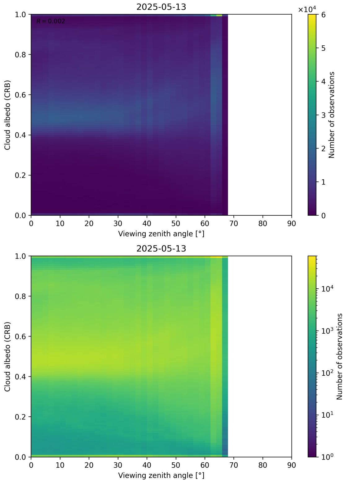
Figure 106: Scatter density plot of “Viewing zenith angle” against “Cloud albedo (CRB)” for 2025-05-12 to 2025-05-14.
