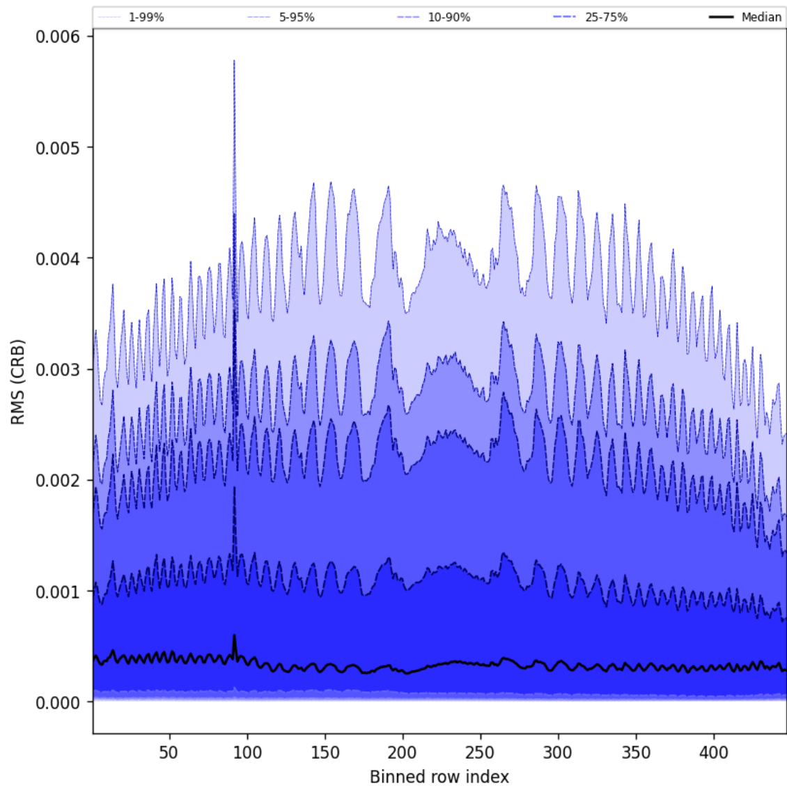
Figure 64: Along track statistics of “RMS (CRB)” for 2025-05-12 to 2025-05-14
