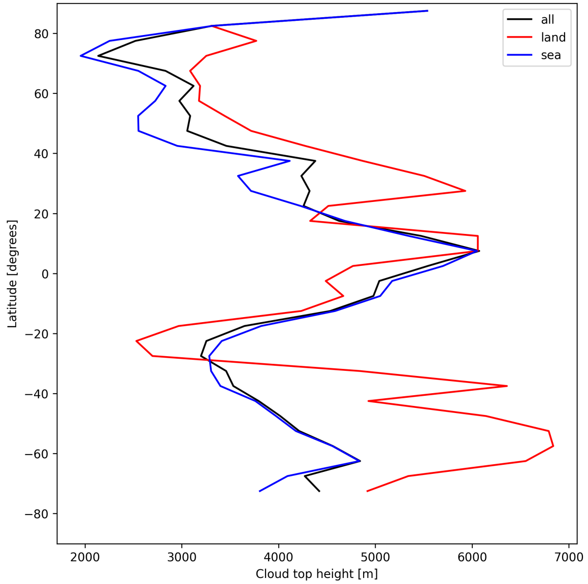
Figure 24: Zonal average of “Cloud top height” for 2025-05-12 to 2025-05-14.
