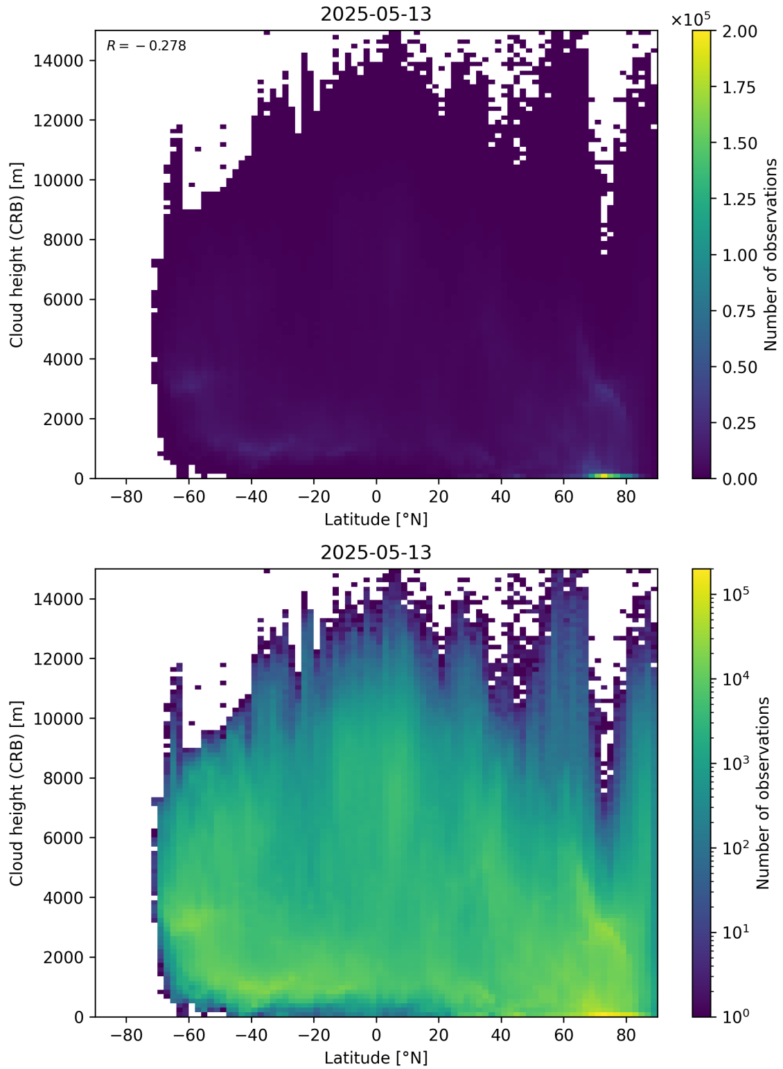
Figure 95: Scatter density plot of “Latitude” against “Cloud height (CRB)” for 2025-05-12 to 2025-05-14.
