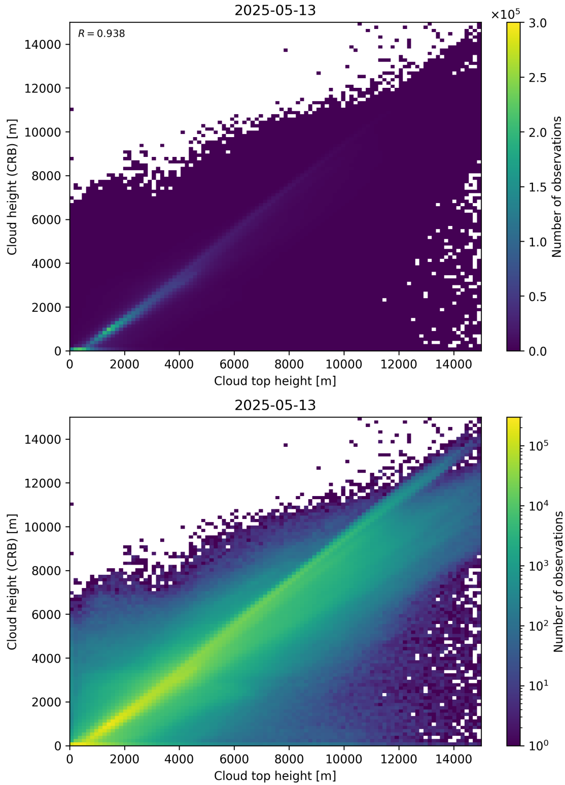
Figure 89: Scatter density plot of “Cloud top height” against “Cloud height (CRB)” for 2025-05-12 to 2025-05-14.
