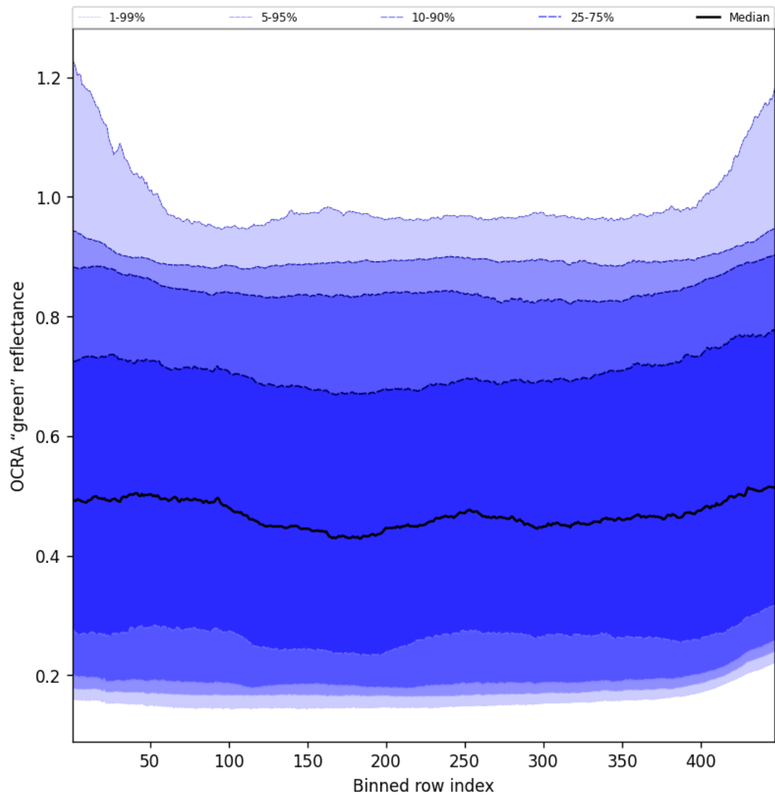
Figure 68: Along track statistics of “OCRA “green” reflectance” for 2025-05-12 to 2025-05-14
