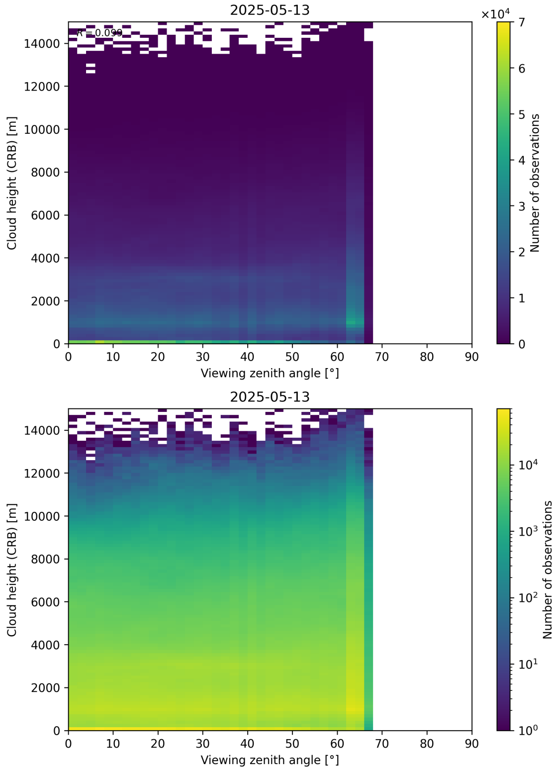
Figure 110: Scatter density plot of “Viewing zenith angle” against “Cloud height (CRB)” for 2025-05-12 to 2025-05-14.
