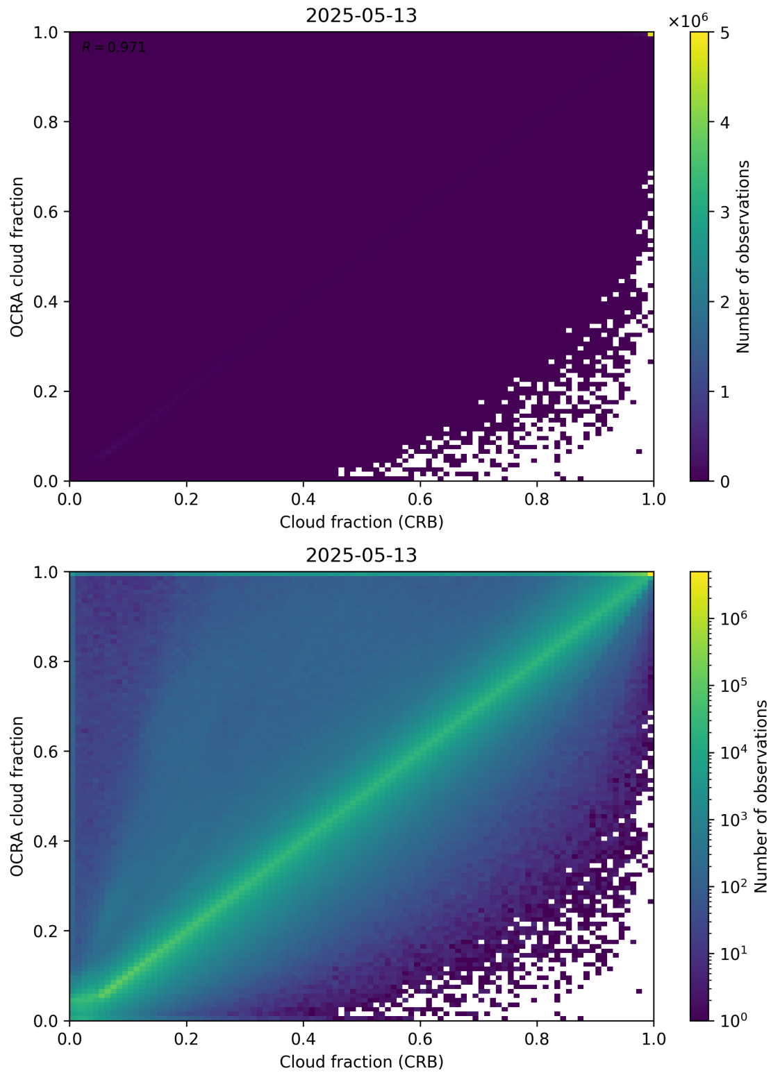
Figure 78: Scatter density plot of “Cloud fraction (CRB)” against “OCRA cloud fraction” for 2025-05-12 to 2025-05-14.
