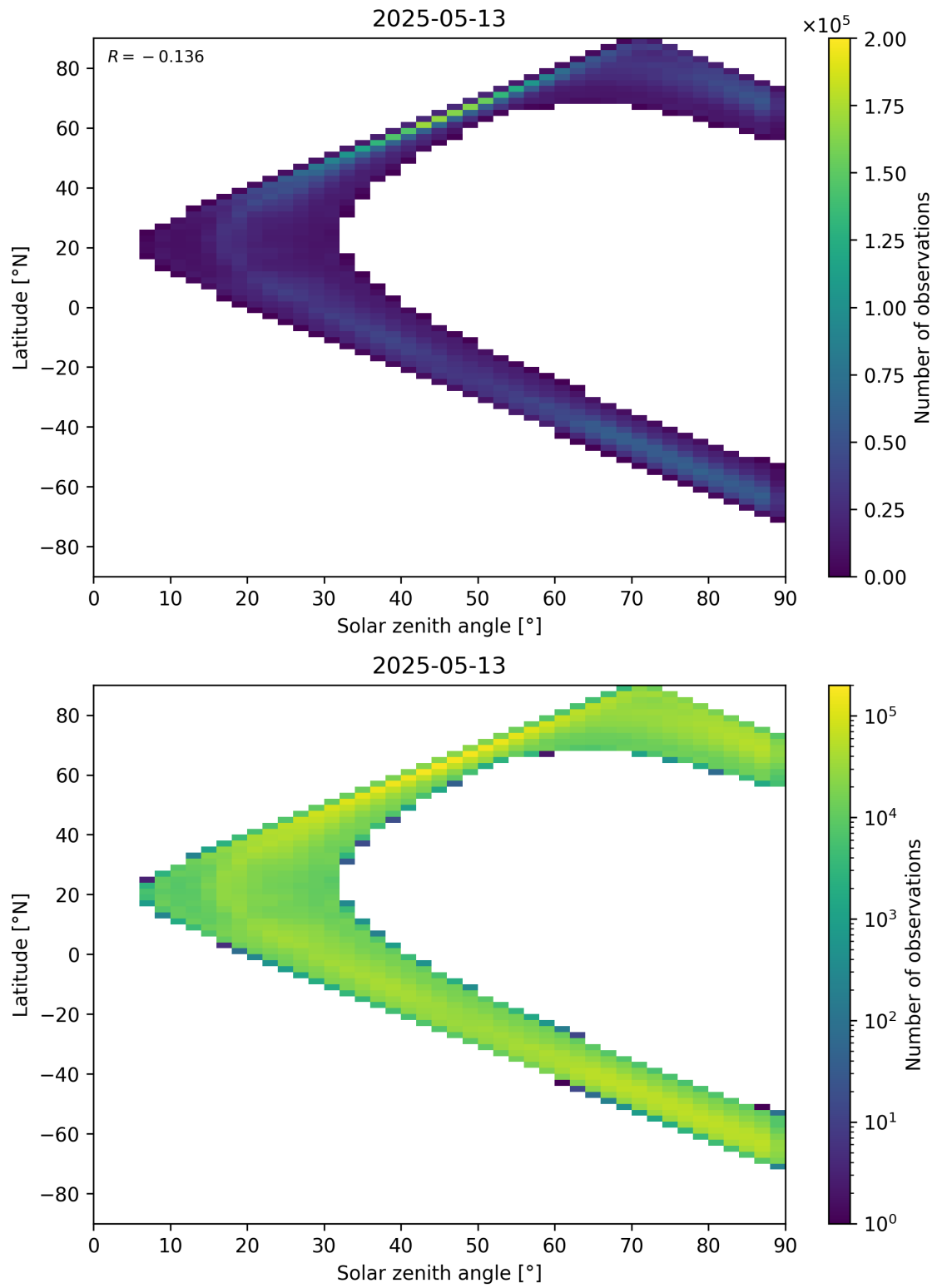
Figure 105: Scatter density plot of “Solar zenith angle” against “Latitude” for 2025-05-12 to 2025-05-14.
