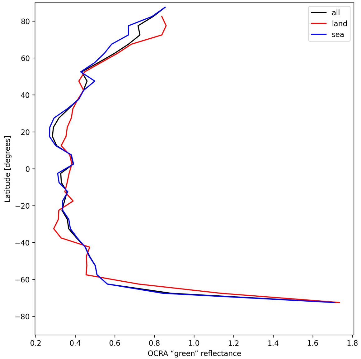
Figure 36: Zonal average of “OCRA “green” reflectance” for 2025-05-12 to 2025-05-14.
