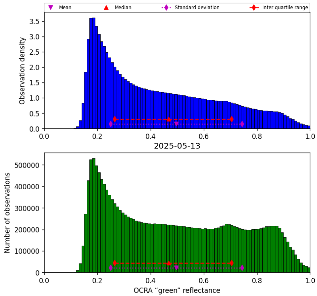
Figure 52: Histogram of “OCRA “green” reflectance” for 2025-05-12 to 2025-05-14
