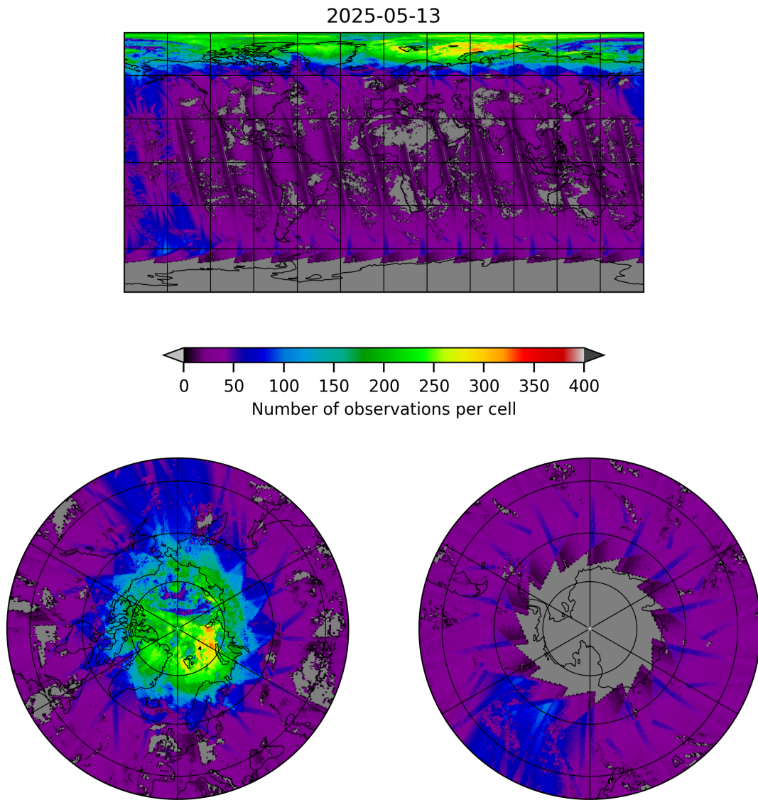
Figure 21: Map of the number of observations for 2025-05-12 to 2025-05-14
