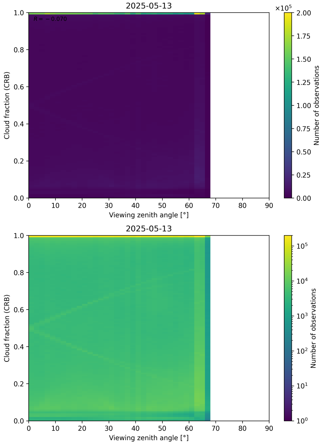
Figure 109: Scatter density plot of “Viewing zenith angle” against “Cloud fraction (CRB)” for 2025-05-12 to 2025-05-14.
