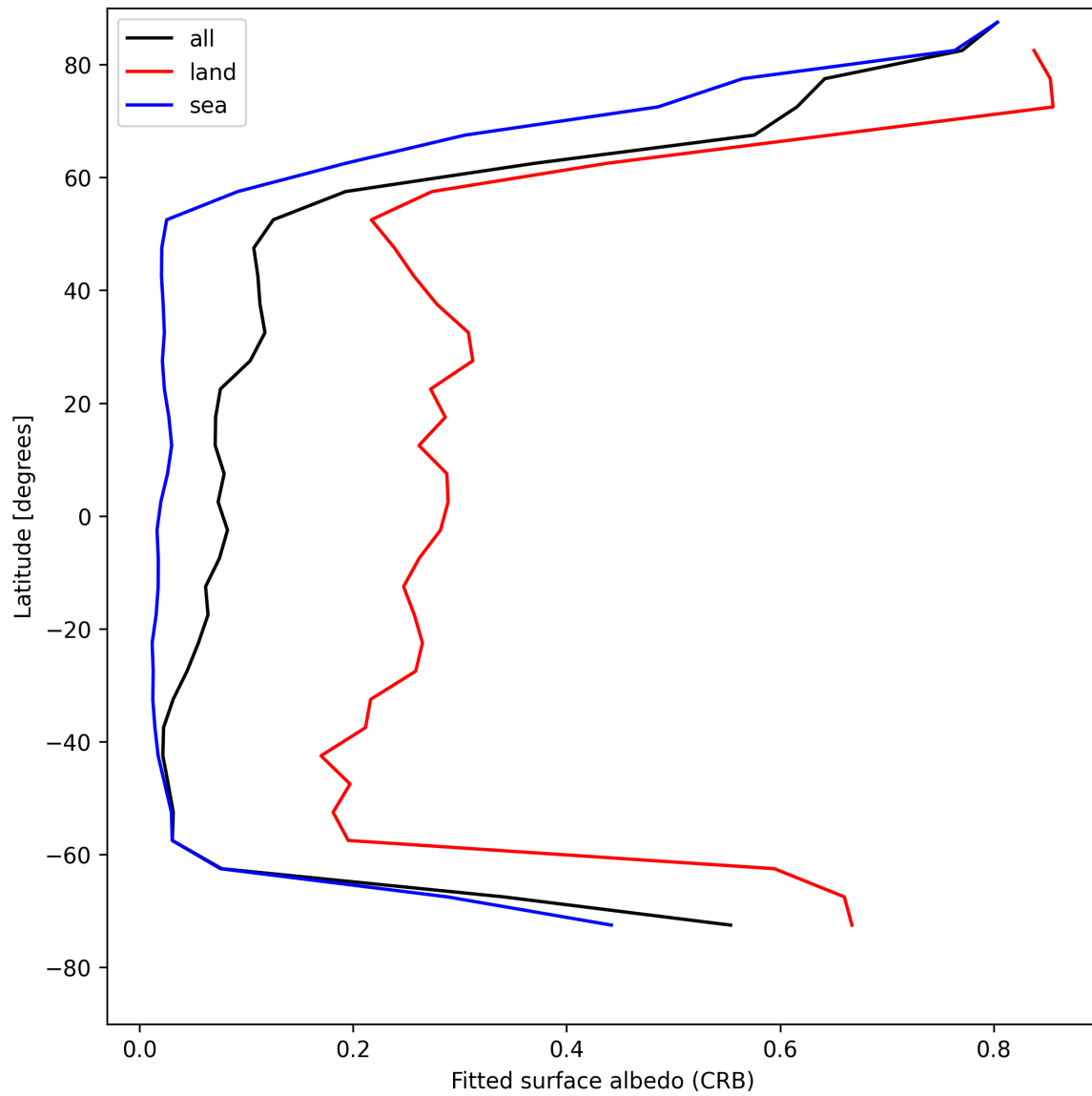
Figure 30: Zonal average of “Fitted surface albedo (CRB)” for 2025-05-12 to 2025-05-14.
