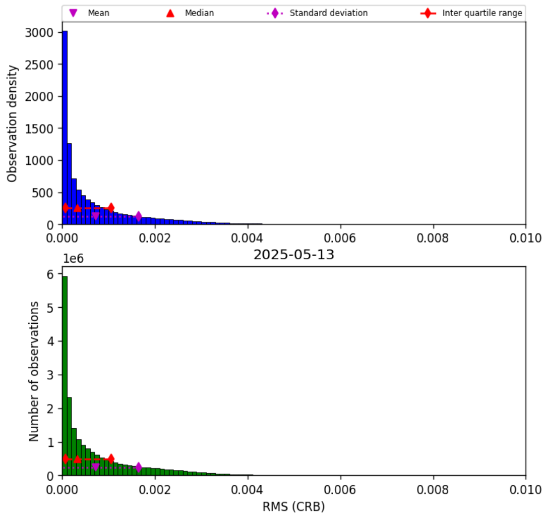
Figure 48: Histogram of “RMS (CRB)” for 2025-05-12 to 2025-05-14
