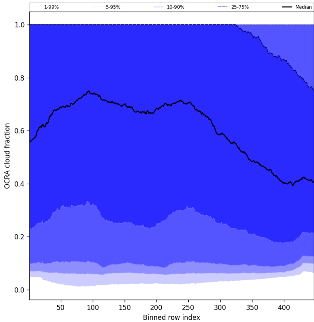
Figure 66: Along track statistics of “OCRA cloud fraction” for 2025-05-12 to 2025-05-14
