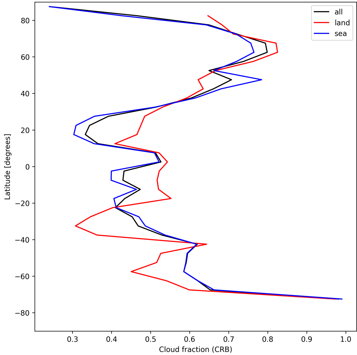
Figure 26: Zonal average of “Cloud fraction (CRB)” for 2025-05-12 to 2025-05-14.
