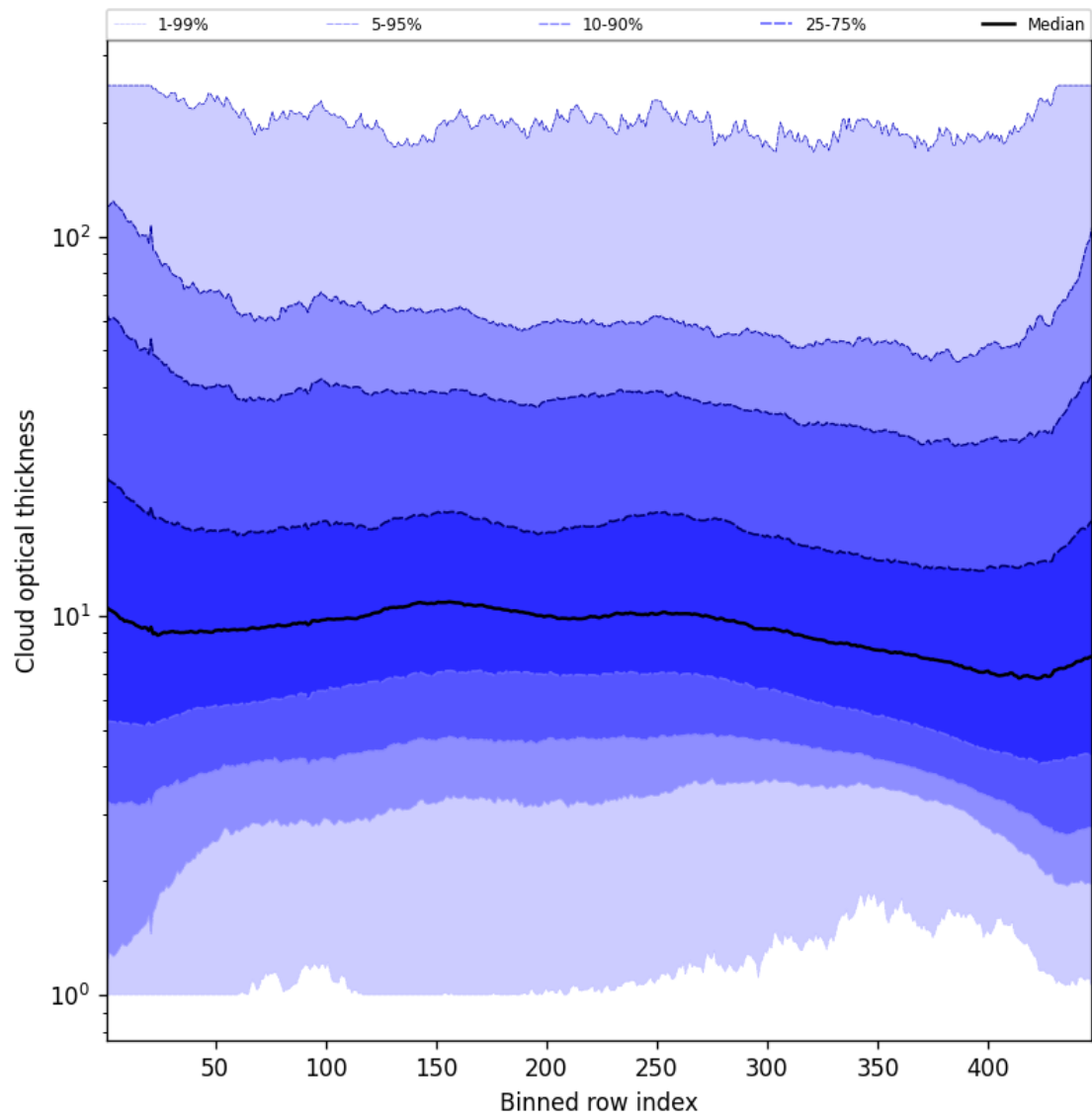
Figure 57: Along track statistics of “Cloud optical thickness” for 2025-05-12 to 2025-05-14
