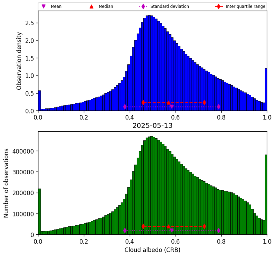
Figure 44: Histogram of “Cloud albedo (CRB)” for 2025-05-12 to 2025-05-14
