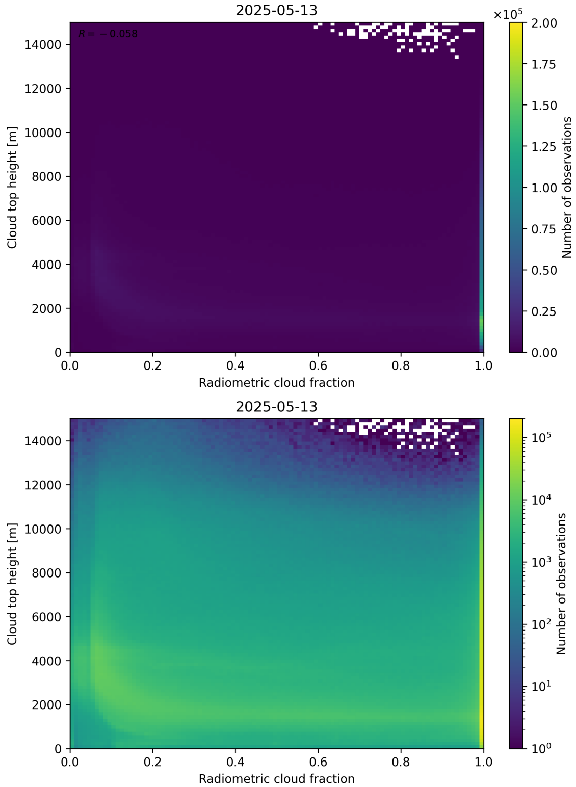
Figure 76: Scatter density plot of “Radiometric cloud fraction” against “Cloud top height” for 2025-05-12 to 2025-05-14.
