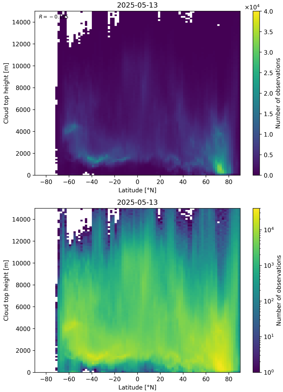
Figure 97: Scatter density plot of “Latitude” against “Cloud top height” for 2025-05-12 to 2025-05-14.
