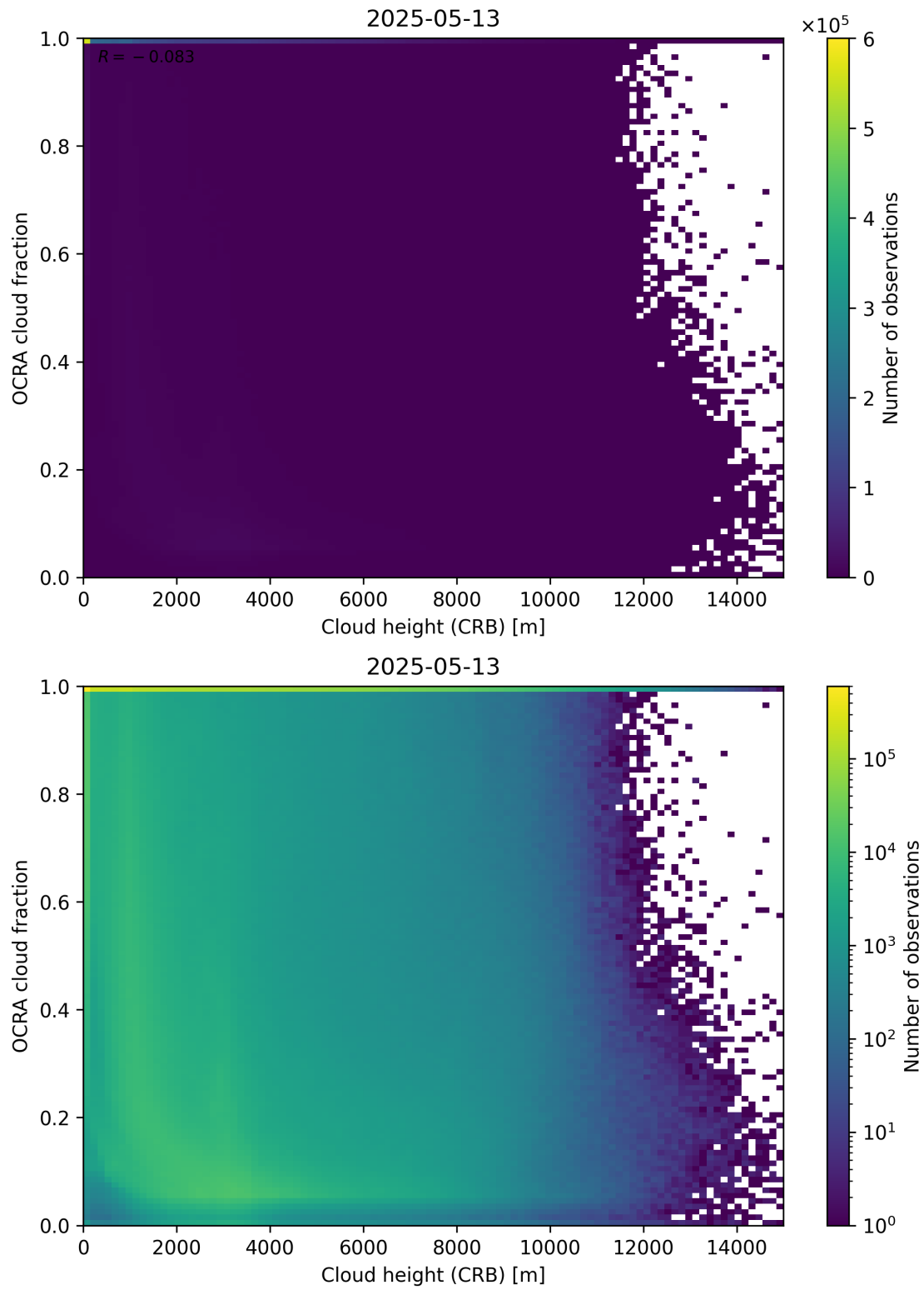
Figure 81: Scatter density plot of “Cloud height (CRB)” against “OCRA cloud fraction” for 2025-05-12 to 2025-05-14.
