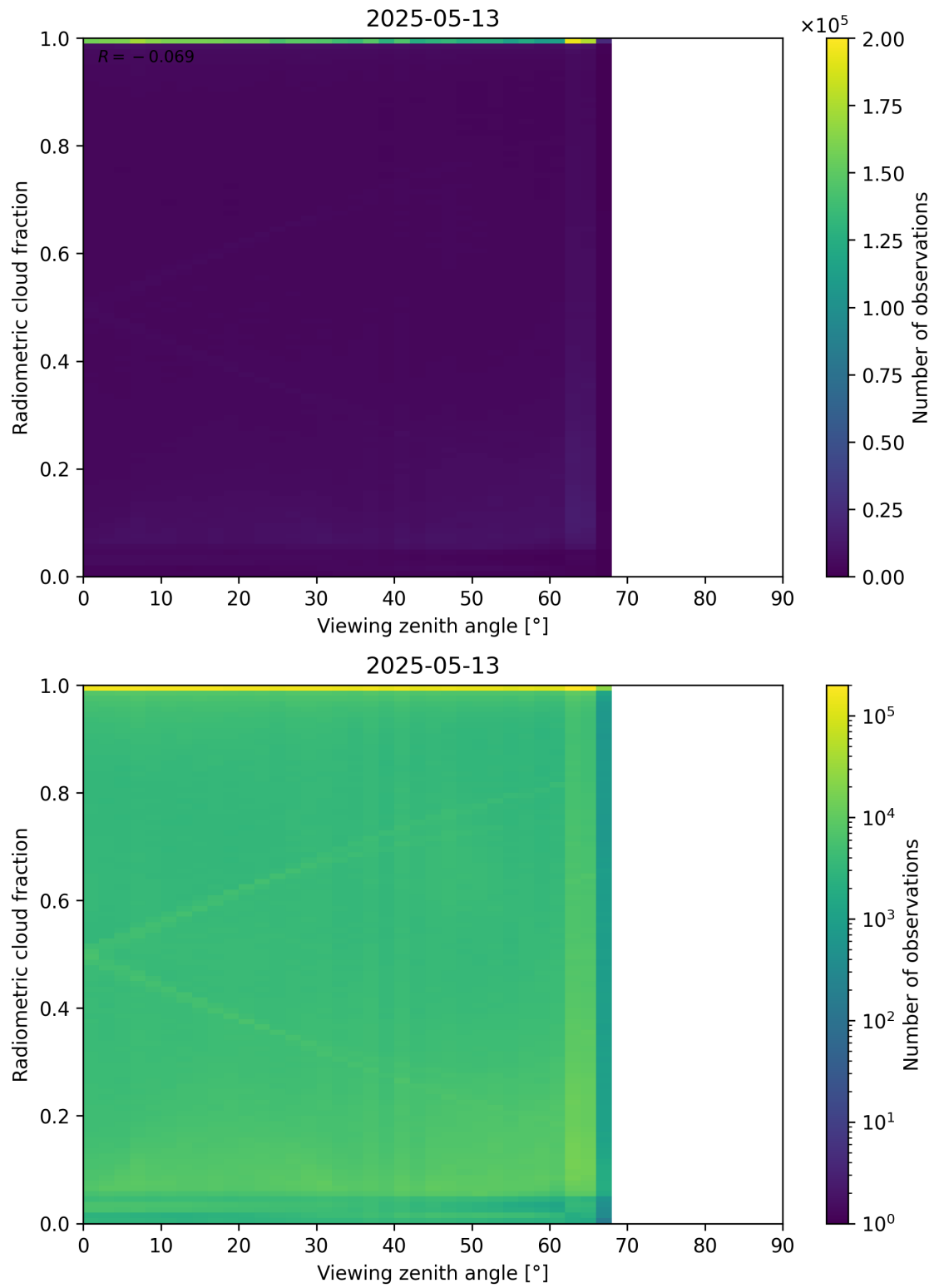
Figure 107: Scatter density plot of “Viewing zenith angle” against “Radiometric cloud fraction” for 2025-05-12 to 2025-05-14.
