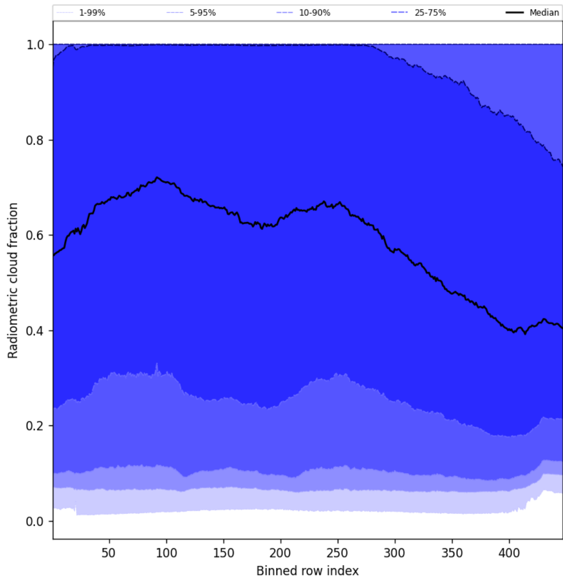
Figure 55: Along track statistics of “Radiometric cloud fraction” for 2025-05-12 to 2025-05-14
