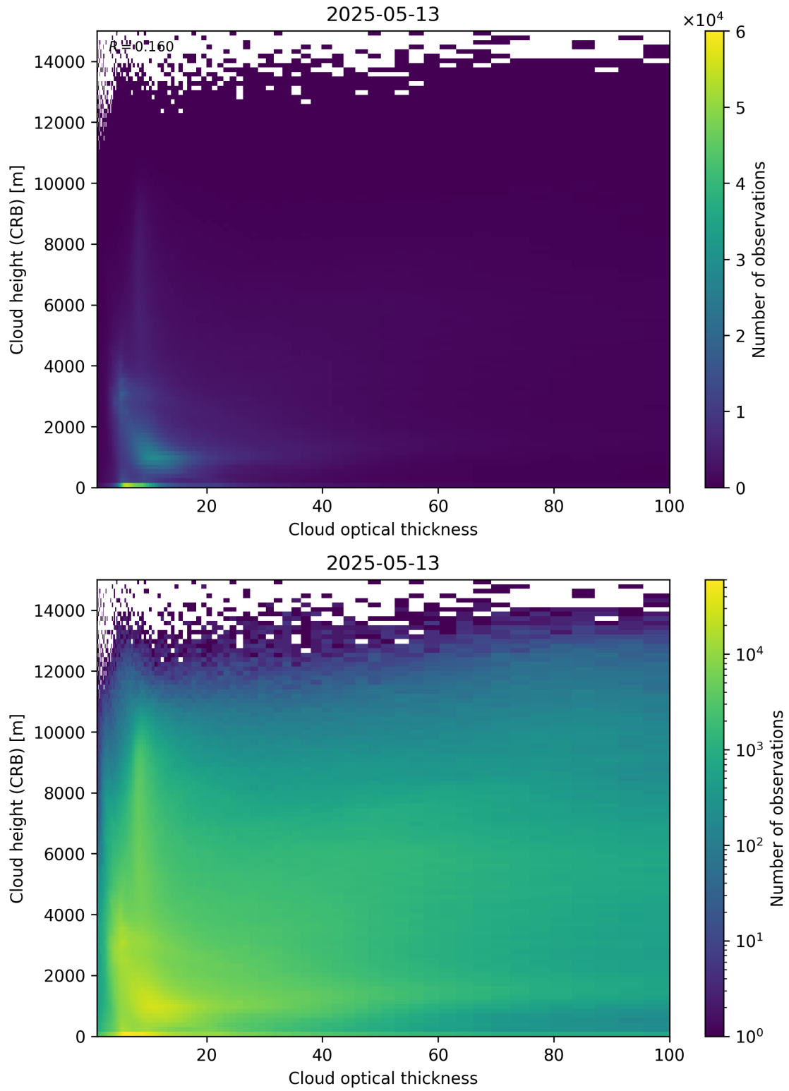
Figure 85: Scatter density plot of “Cloud optical thickness” against “Cloud height (CRB)” for 2025-05-12 to 2025-05-14.
