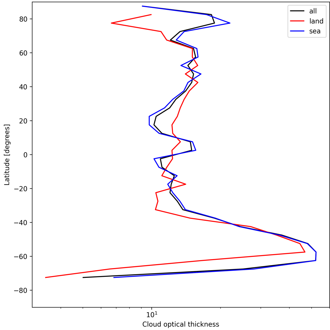
Figure 25: Zonal average of “Cloud optical thickness” for 2025-05-12 to 2025-05-14.
