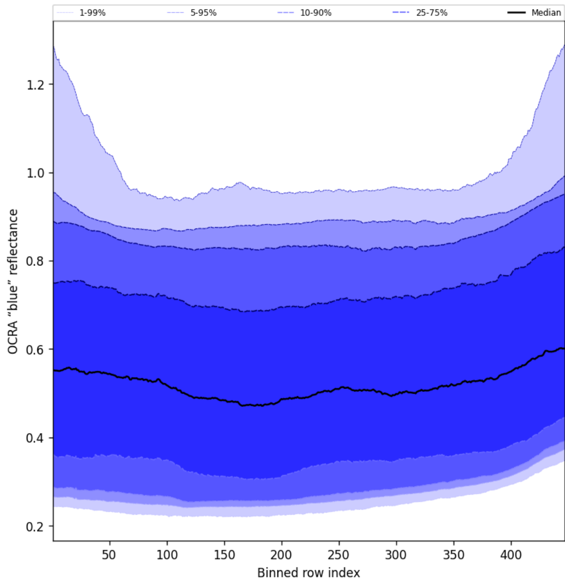
Figure 67: Along track statistics of "OCRA "blue" reflectance" for 2025-05-12 to 2025-05-14
