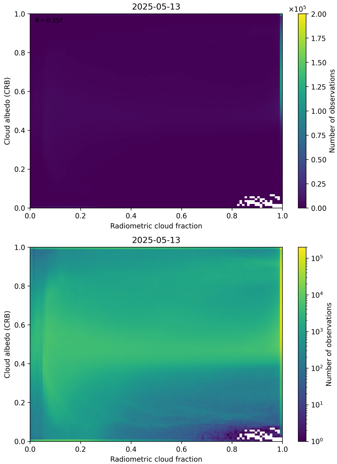
Figure 71: Scatter density plot of “Radiometric cloud fraction” against “Cloud albedo (CRB)” for 2025-05-12 to 2025-05-14.
