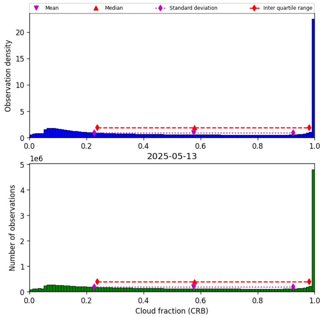
Figure 42: Histogram of “Cloud fraction (CRB)” for 2025-05-12 to 2025-05-14
