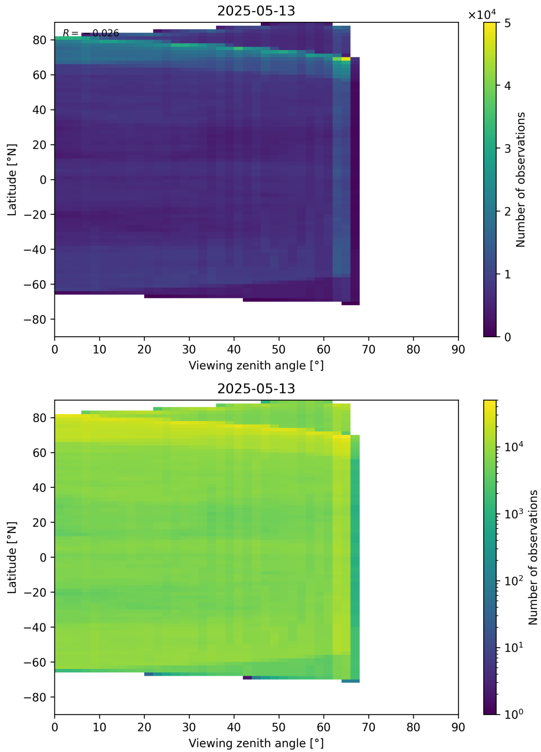
Figure 113: Scatter density plot of “Viewing zenith angle” against “Latitude” for 2025-05-12 to 2025-05-14.
