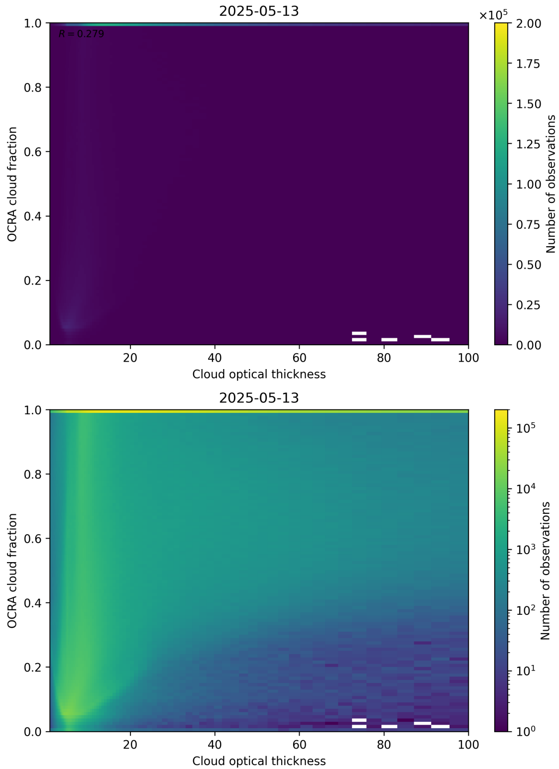
Figure 83: Scatter density plot of “Cloud optical thickness” against “OCRA cloud fraction” for 2025-05-12 to 2025-05-14.
