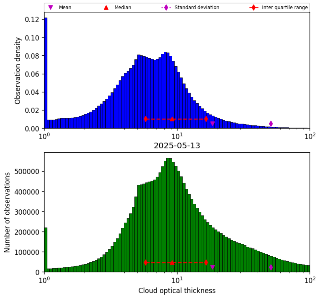
Figure 41: Histogram of “Cloud optical thickness” for 2025-05-12 to 2025-05-14
