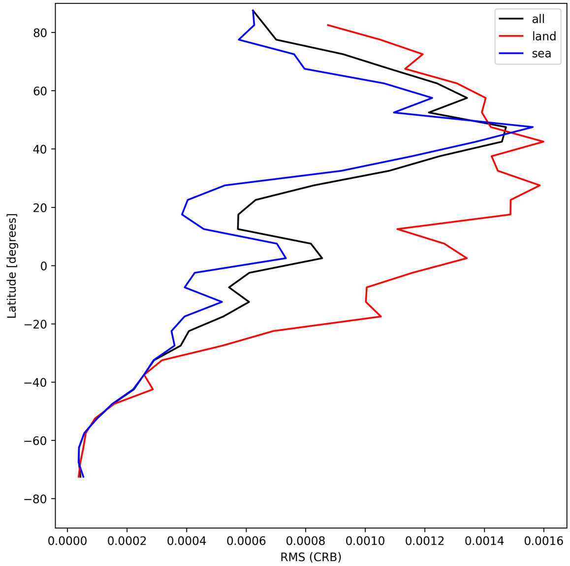
Figure 32: Zonal average of “RMS (CRB)” for 2025-05-12 to 2025-05-14.
