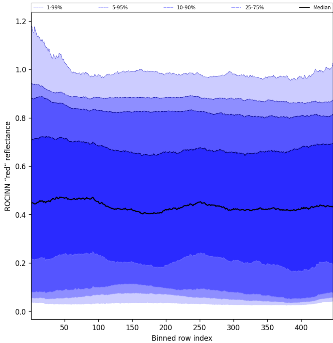
Figure 69: Along track statistics of "ROCINN "red" reflectance" for 2025-05-12 to 2025-05-14
