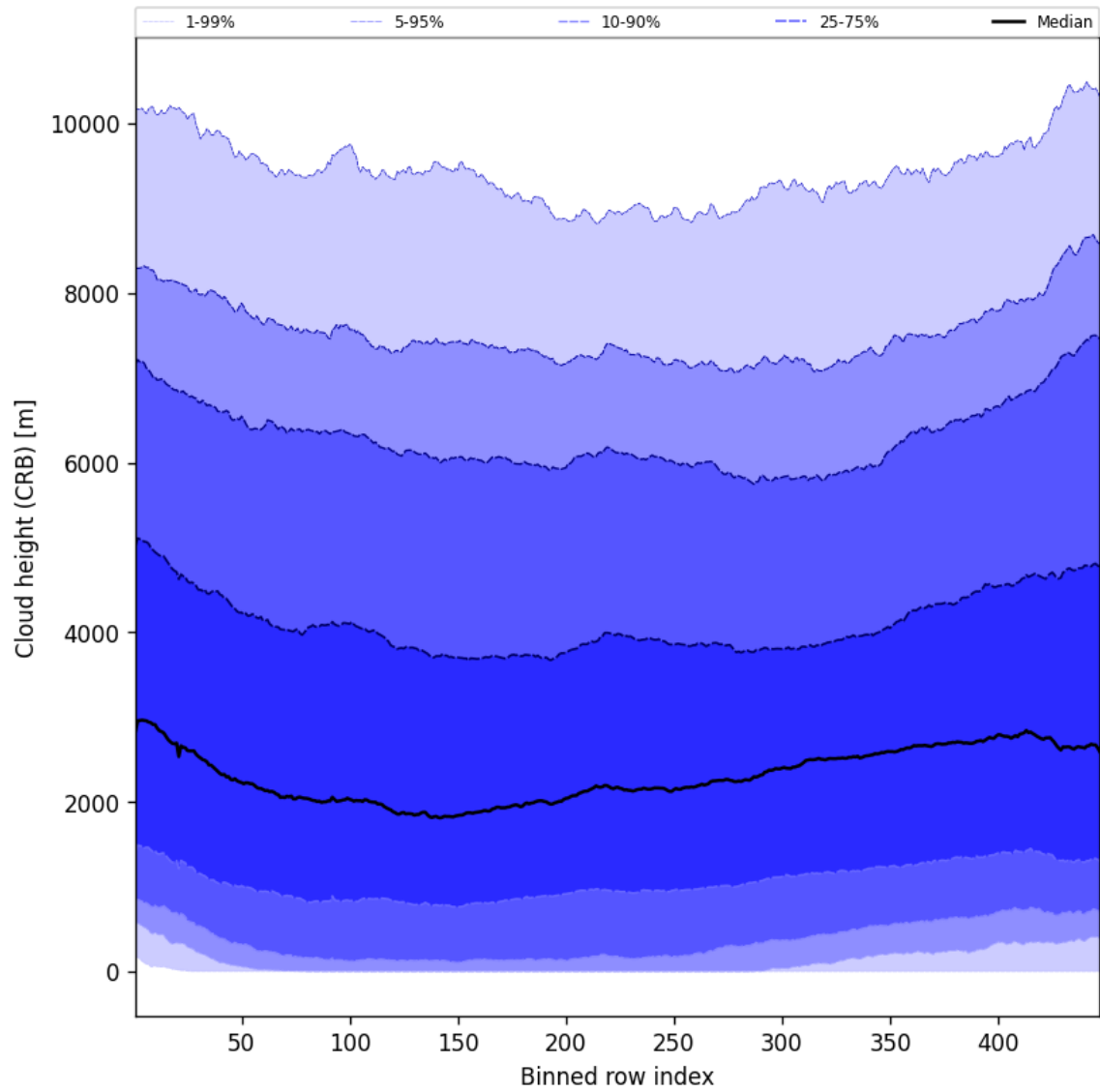
Figure 59: Along track statistics of “Cloud height (CRB)” for 2025-05-12 to 2025-05-14
