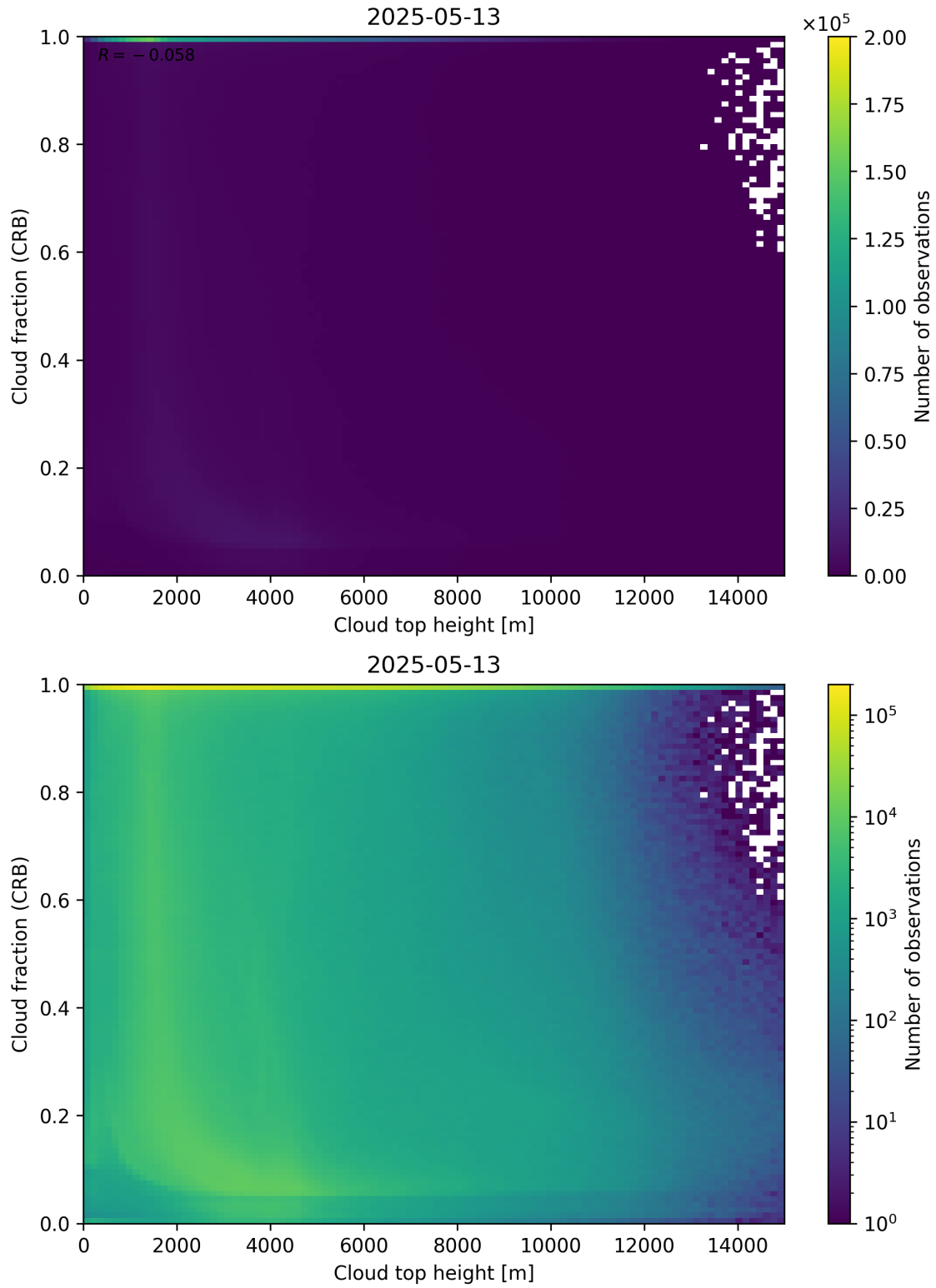
Figure 88: Scatter density plot of “Cloud top height” against “Cloud fraction (CRB)” for 2025-05-12 to 2025-05-14.
