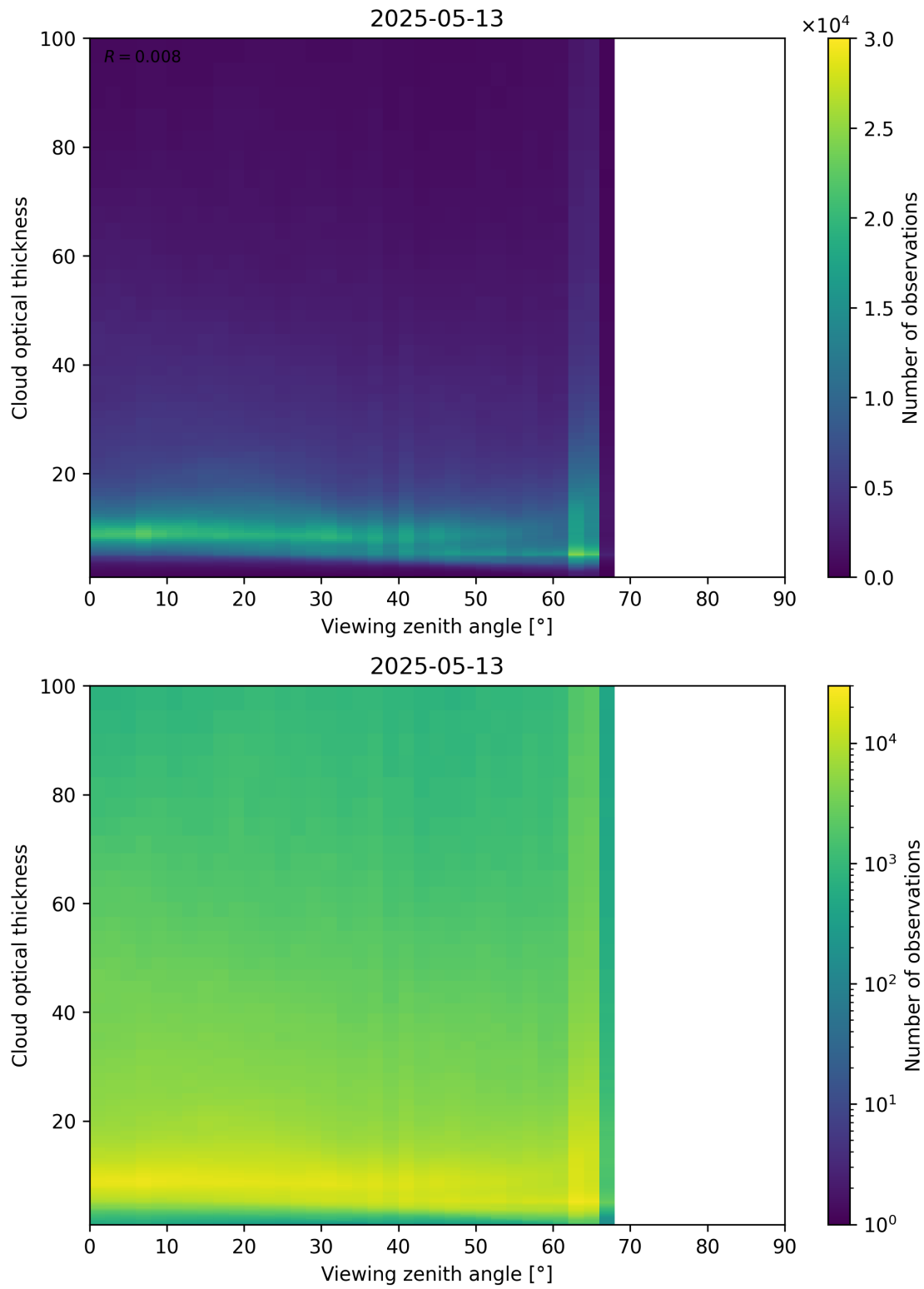
Figure 111: Scatter density plot of “Viewing zenith angle” against “Cloud optical thickness” for 2025-05-12 to 2025-05-14.
