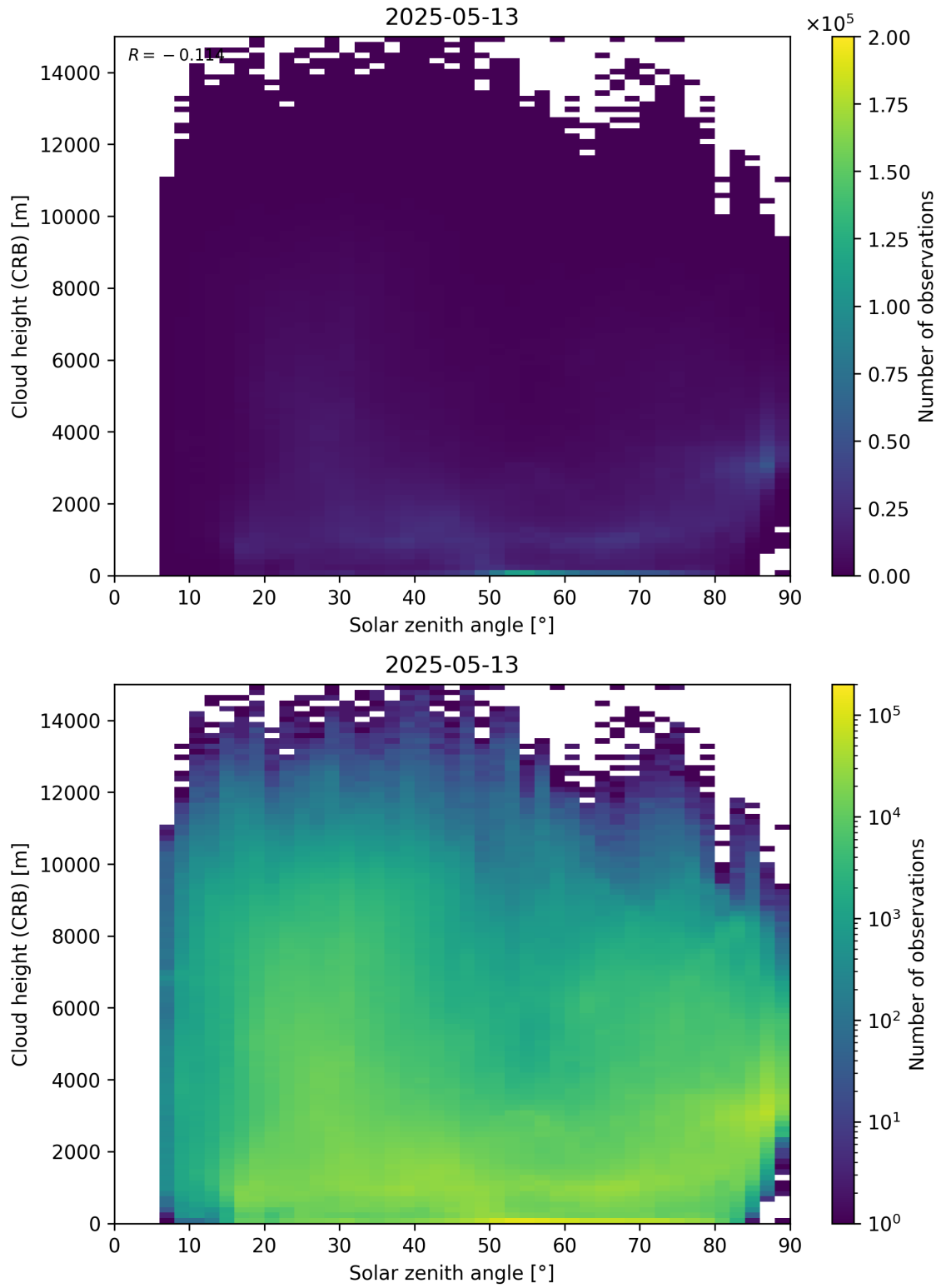
Figure 102: Scatter density plot of “Solar zenith angle” against “Cloud height (CRB)” for 2025-05-12 to 2025-05-14.
