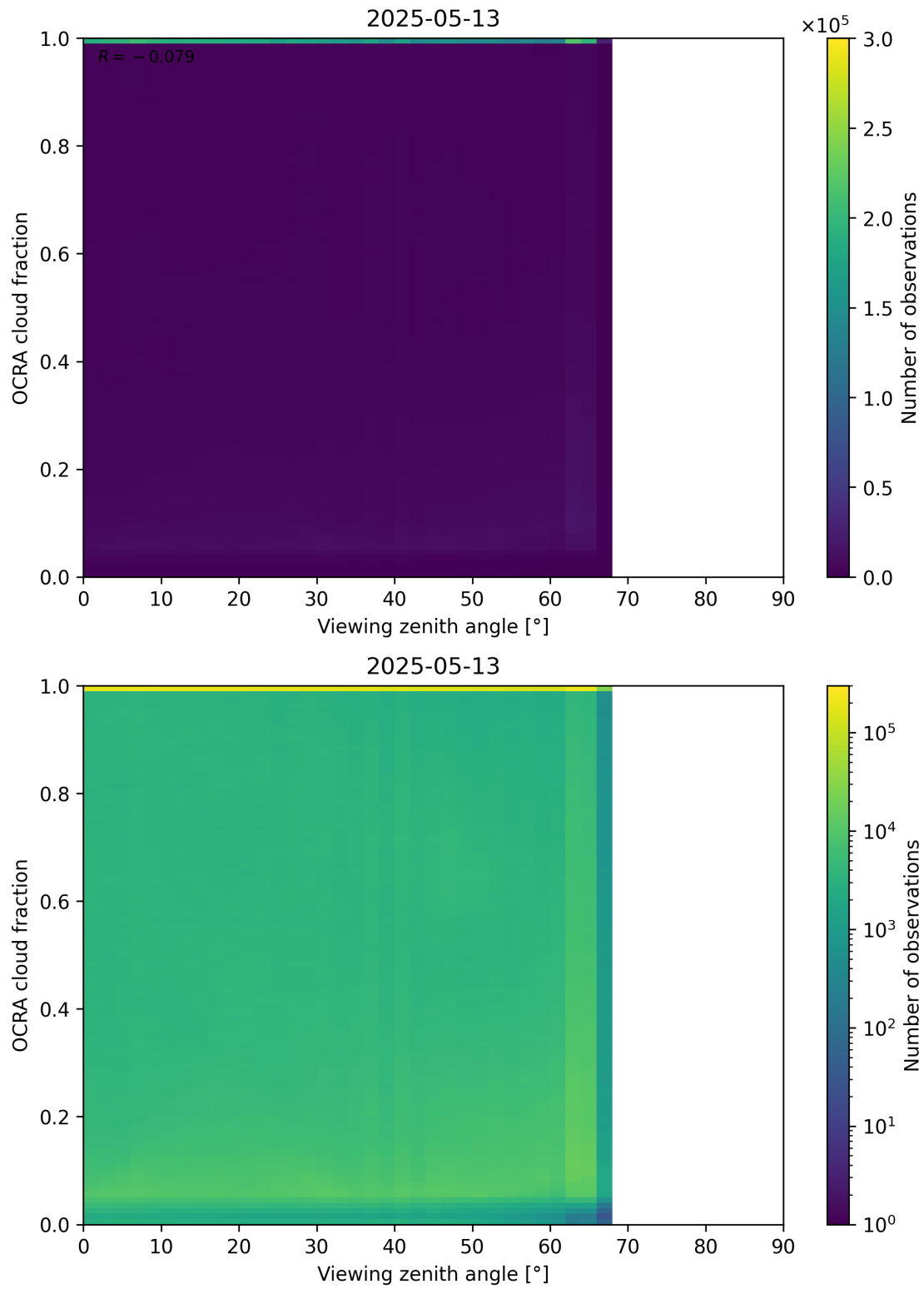
Figure 108: Scatter density plot of “Viewing zenith angle” against “OCRA cloud fraction” for 2025-05-12 to 2025-05-14.
