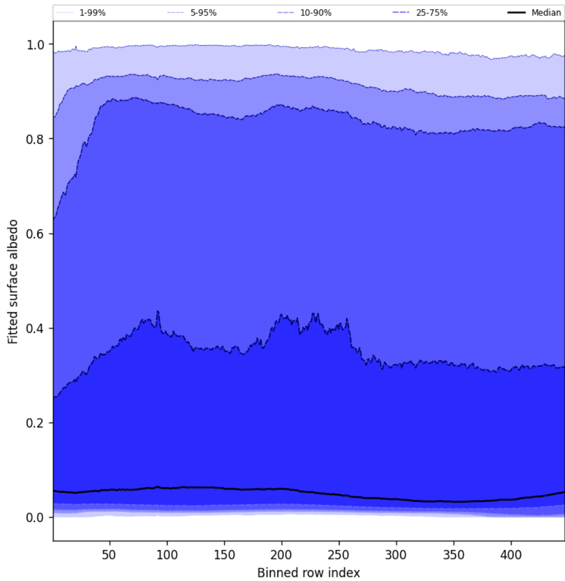
Figure 61: Along track statistics of “Fitted surface albedo” for 2025-05-12 to 2025-05-14
