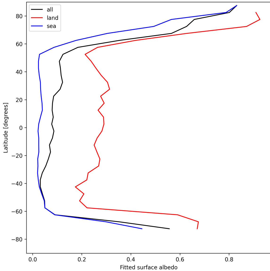
Figure 29: Zonal average of “Fitted surface albedo” for 2025-05-12 to 2025-05-14.
