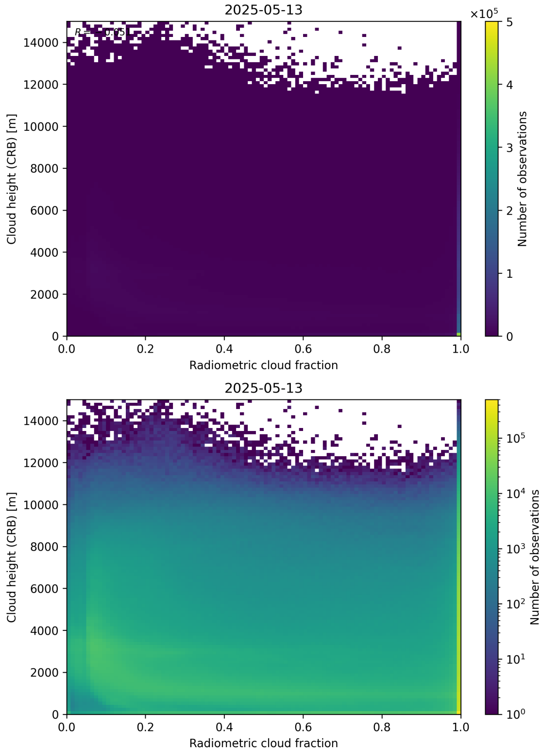
Figure 74: Scatter density plot of “Radiometric cloud fraction” against “Cloud height (CRB)” for 2025-05-12 to 2025-05-14.
