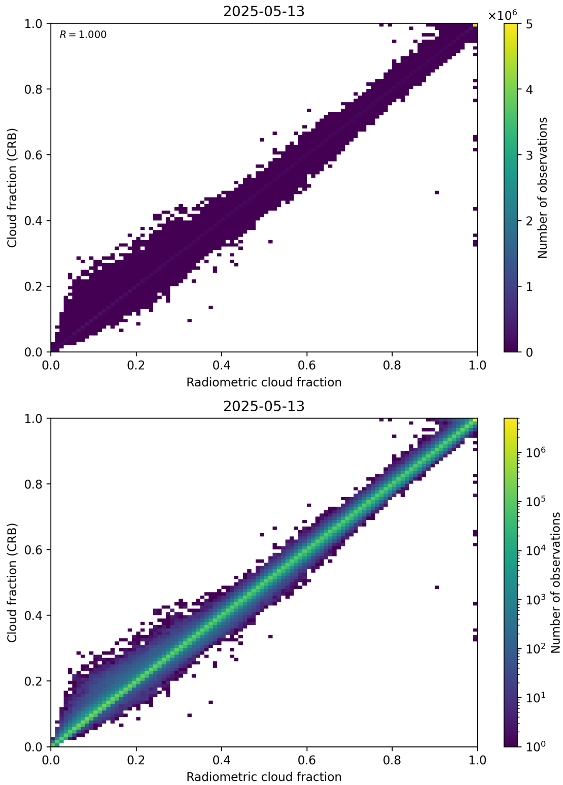
Figure 73: Scatter density plot of “Radiometric cloud fraction” against “Cloud fraction (CRB)” for 2025-05-12 to 2025-05-14.
