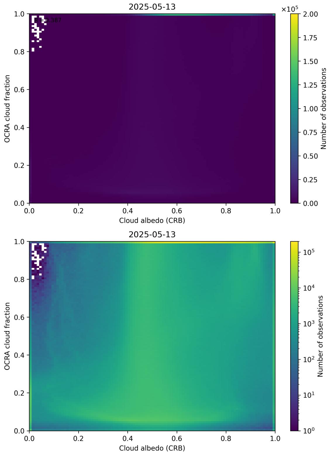
Figure 70: Scatter density plot of “Cloud albedo (CRB)” against “OCRA cloud fraction” for 2025-05-12 to 2025-05-14.
