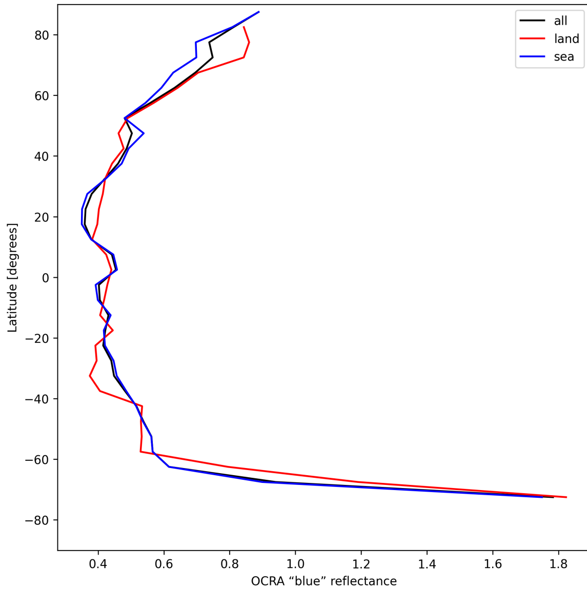
Figure 35: Zonal average of “OCRA “blue” reflectance” for 2025-05-12 to 2025-05-14.
