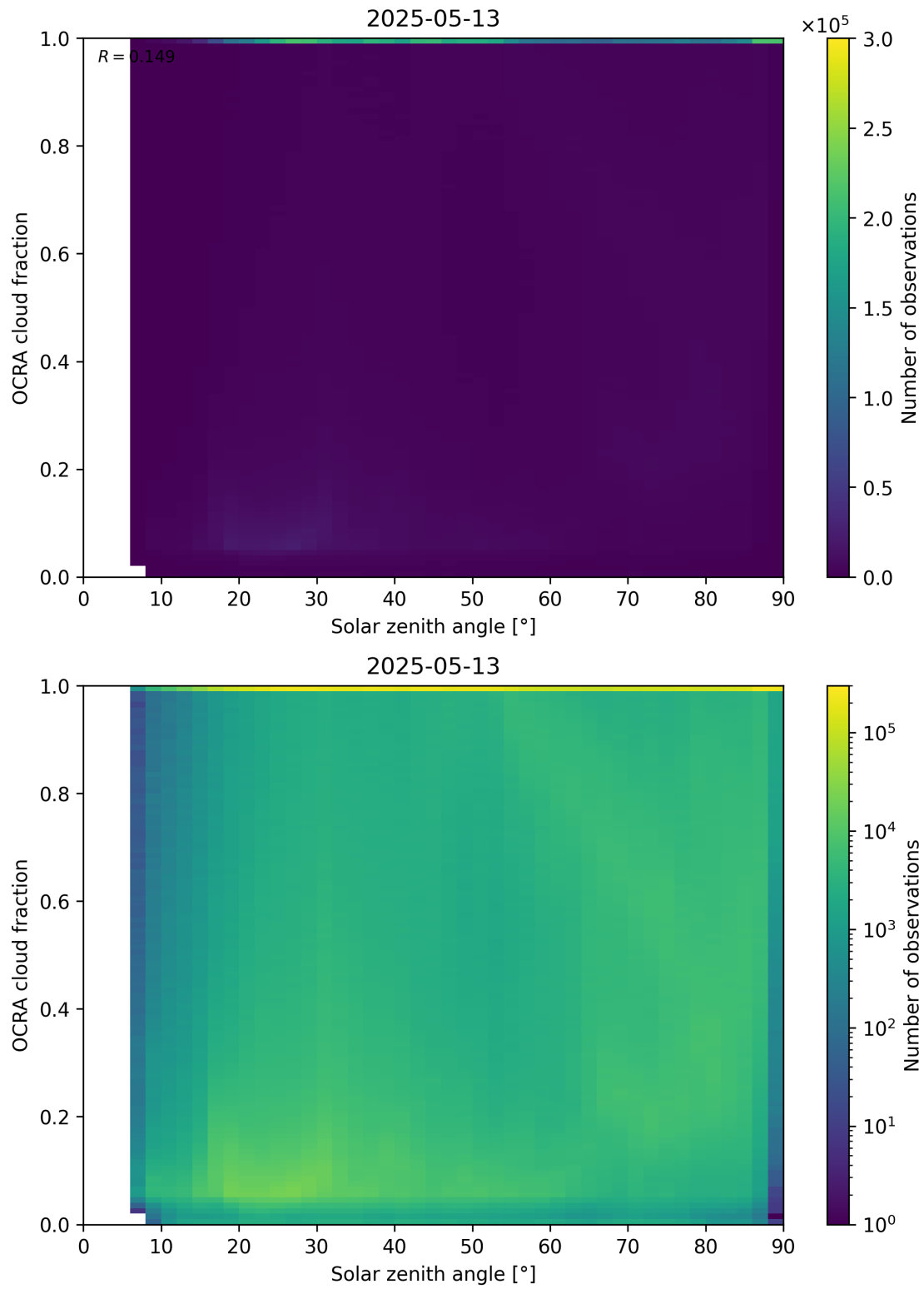
Figure 100: Scatter density plot of “Solar zenith angle” against “OCRA cloud fraction” for 2025-05-12 to 2025-05-14.
