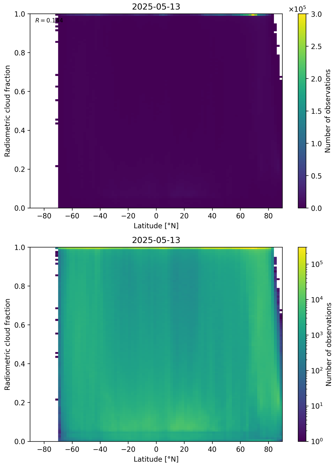
Figure 92: Scatter density plot of “Latitude” against “Radiometric cloud fraction” for 2025-05-12 to 2025-05-14.
