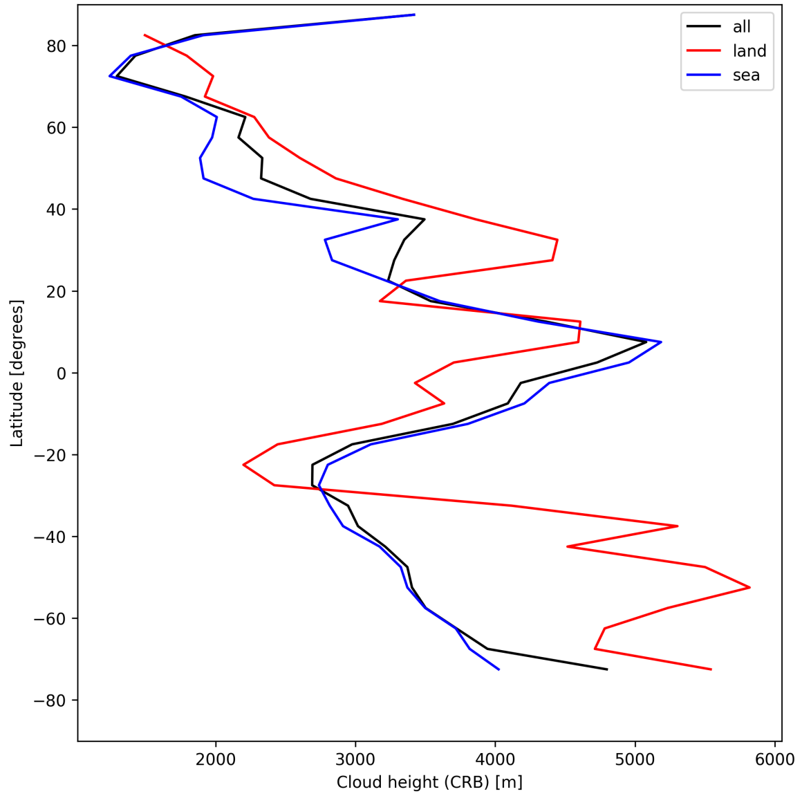
Figure 27: Zonal average of “Cloud height (CRB)” for 2025-05-12 to 2025-05-14.
