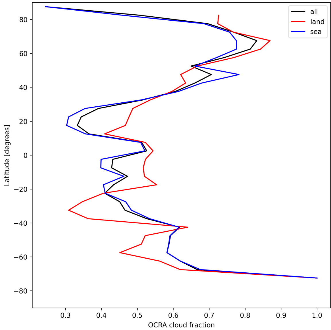
Figure 34: Zonal average of “OCRA cloud fraction” for 2025-05-12 to 2025-05-14.
