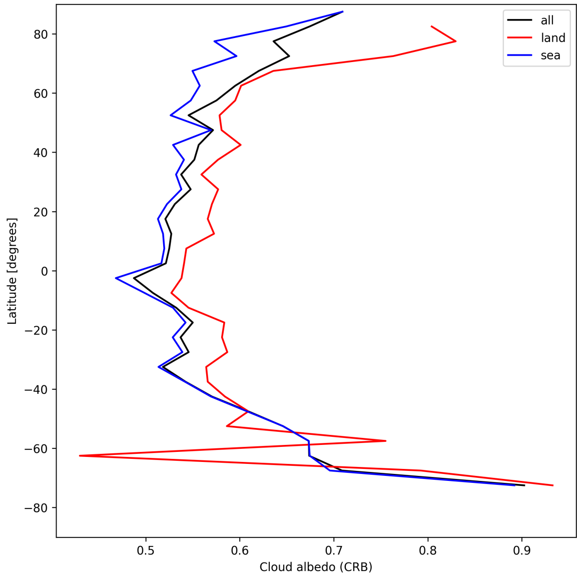
Figure 28: Zonal average of “Cloud albedo (CRB)” for 2025-05-12 to 2025-05-14.
