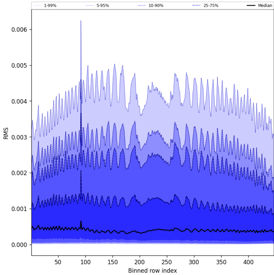
Figure 63: Along track statistics of “RMS” for 2025-05-12 to 2025-05-14
