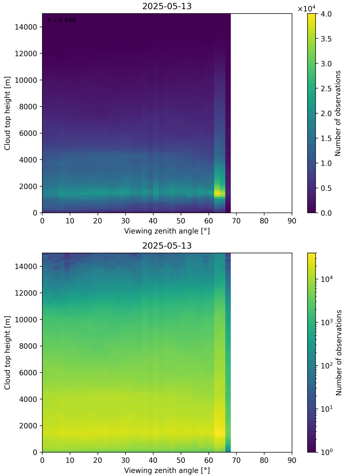
Figure 112: Scatter density plot of “Viewing zenith angle” against “Cloud top height” for 2025-05-12 to 2025-05-14.
