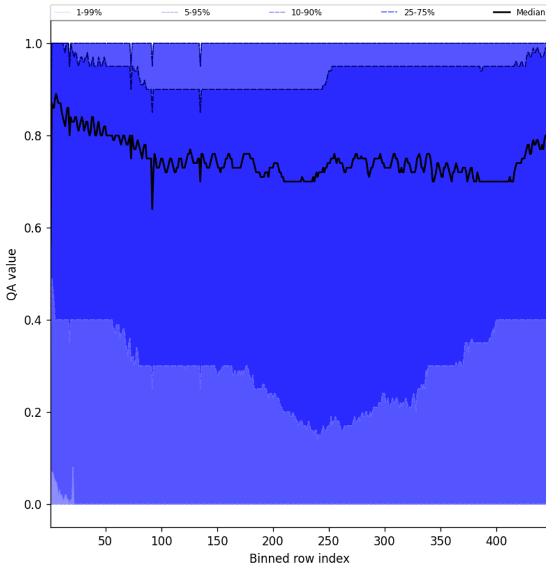
Figure 54: Along track statistics of “QA value” for 2025-05-12 to 2025-05-14
