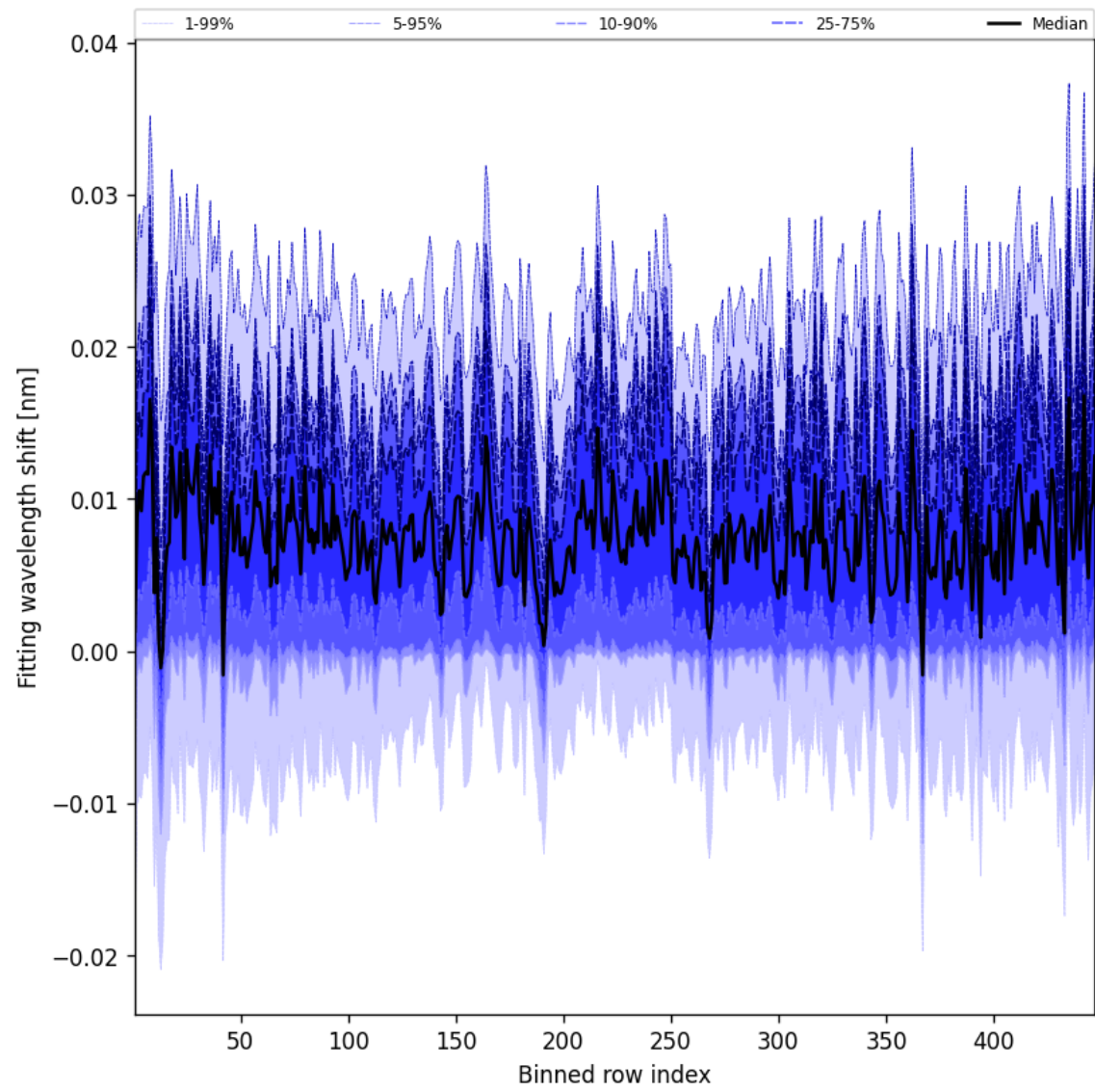
Figure 65: Along track statistics of “Fitting wavelength shift” for 2025-05-12 to 2025-05-14
