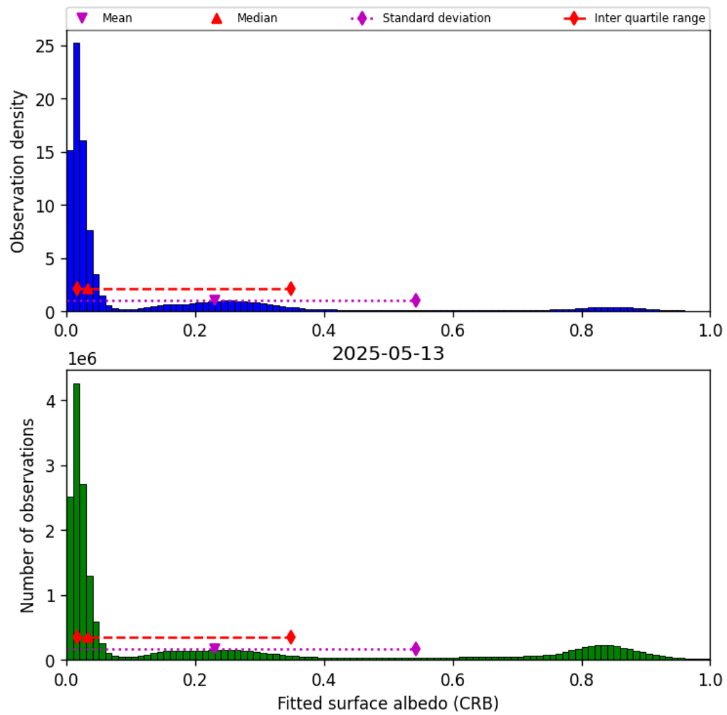
Figure 46: Histogram of “Fitted surface albedo (CRB)” for 2025-05-12 to 2025-05-14
