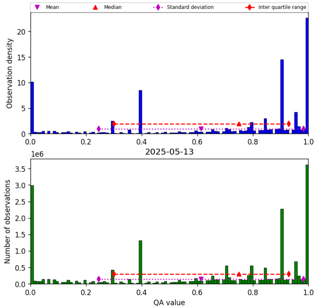
Figure 38: Histogram of “QA value” for 2025-05-12 to 2025-05-14
