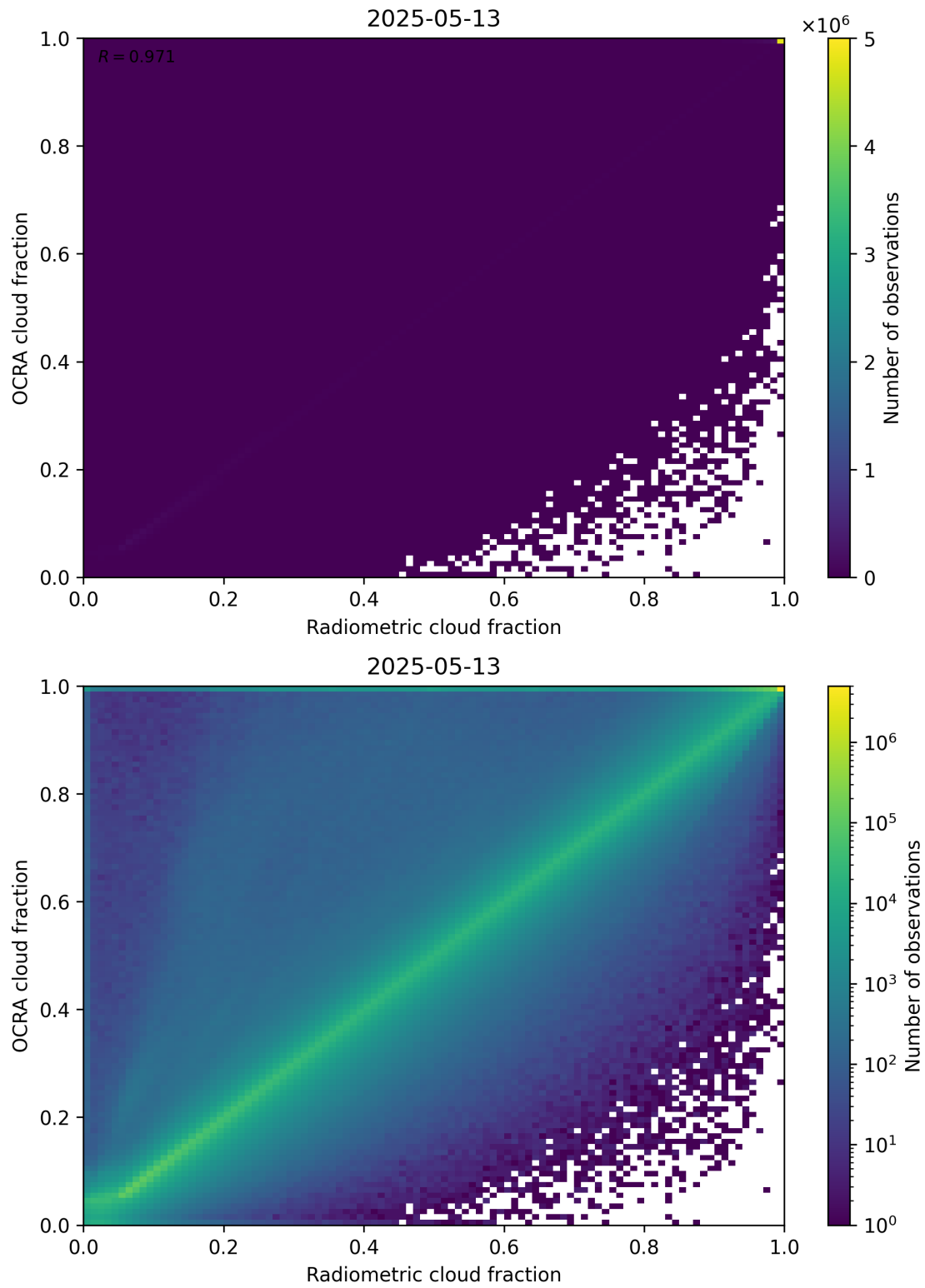
Figure 72: Scatter density plot of “Radiometric cloud fraction” against “OCRA cloud fraction” for 2025-05-12 to 2025-05-14.
