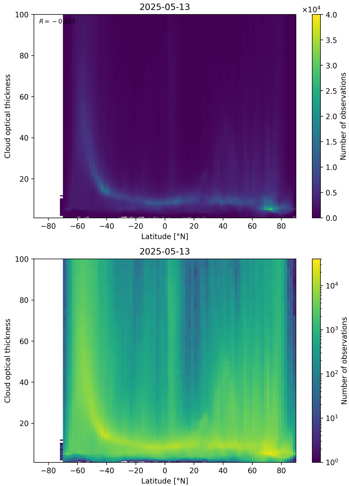
Figure 96: Scatter density plot of “Latitude” against “Cloud optical thickness” for 2025-05-12 to 2025-05-14.
