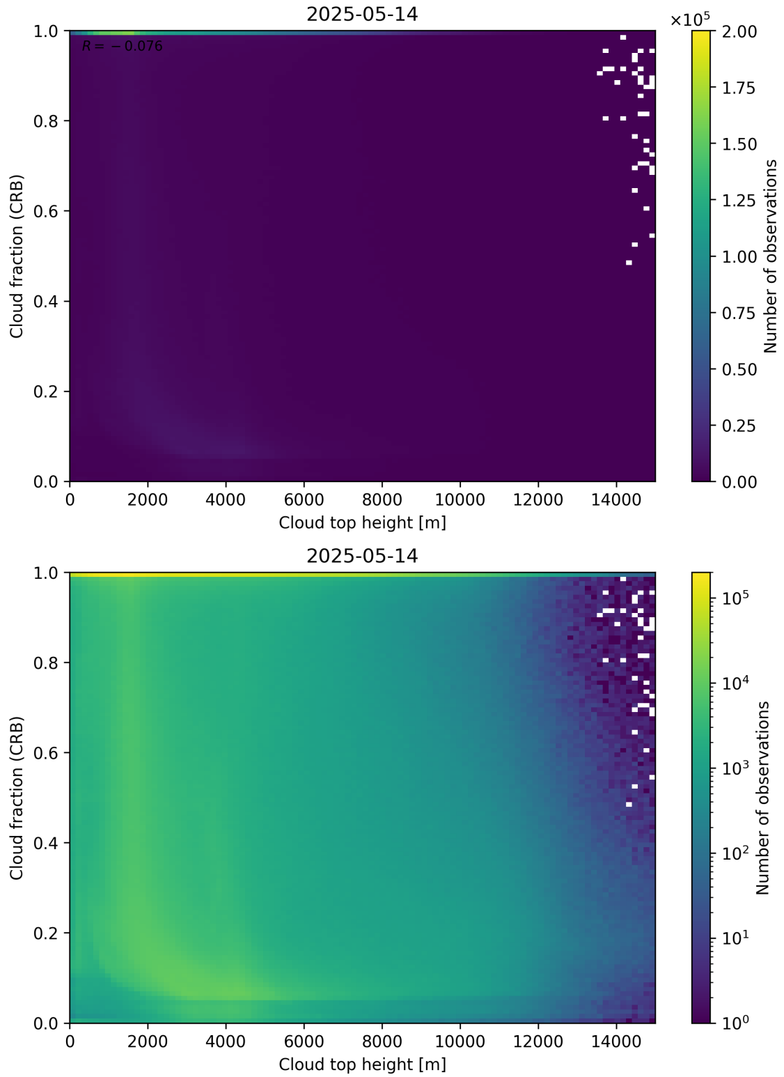
Figure 88: Scatter density plot of “Cloud top height” against “Cloud fraction (CRB)” for 2025-05-13 to 2025-05-15.
