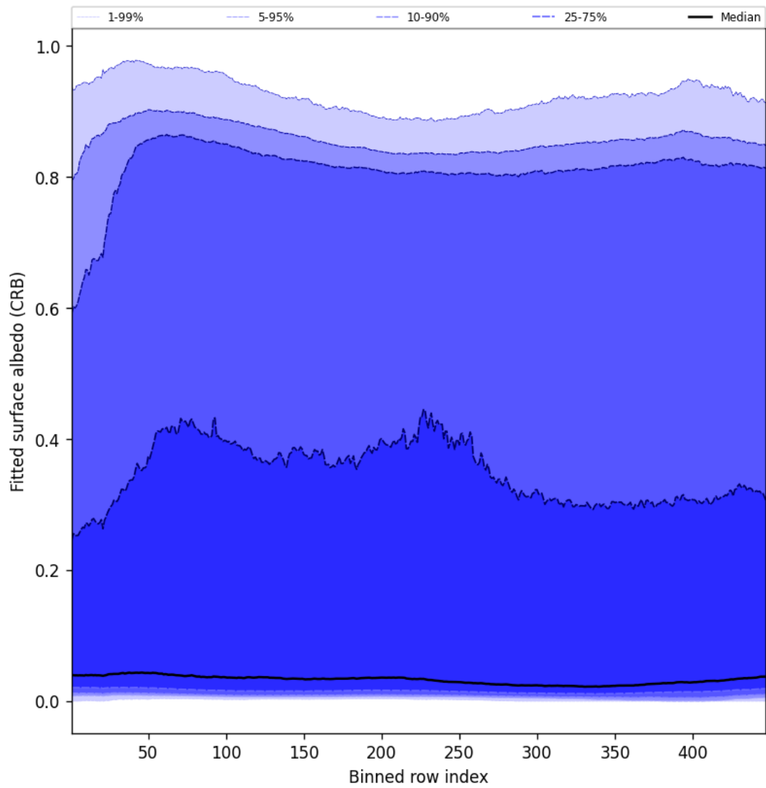
Figure 62: Along track statistics of “Fitted surface albedo (CRB)” for 2025-05-13 to 2025-05-15
