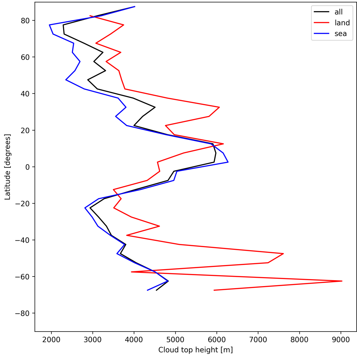
Figure 24: Zonal average of “Cloud top height” for 2025-05-13 to 2025-05-15.
