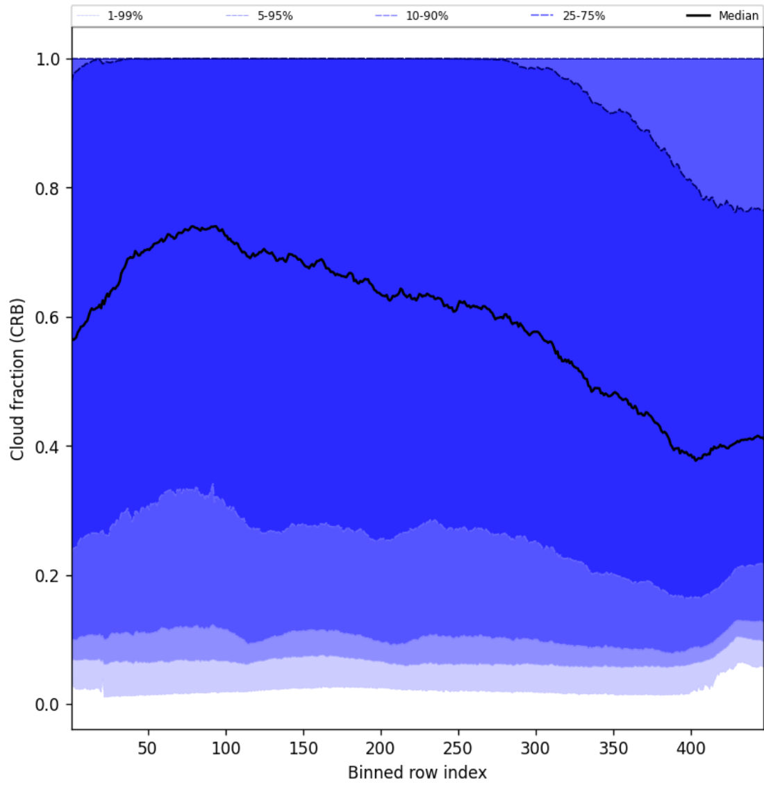
Figure 58: Along track statistics of “Cloud fraction (CRB)” for 2025-05-13 to 2025-05-15
