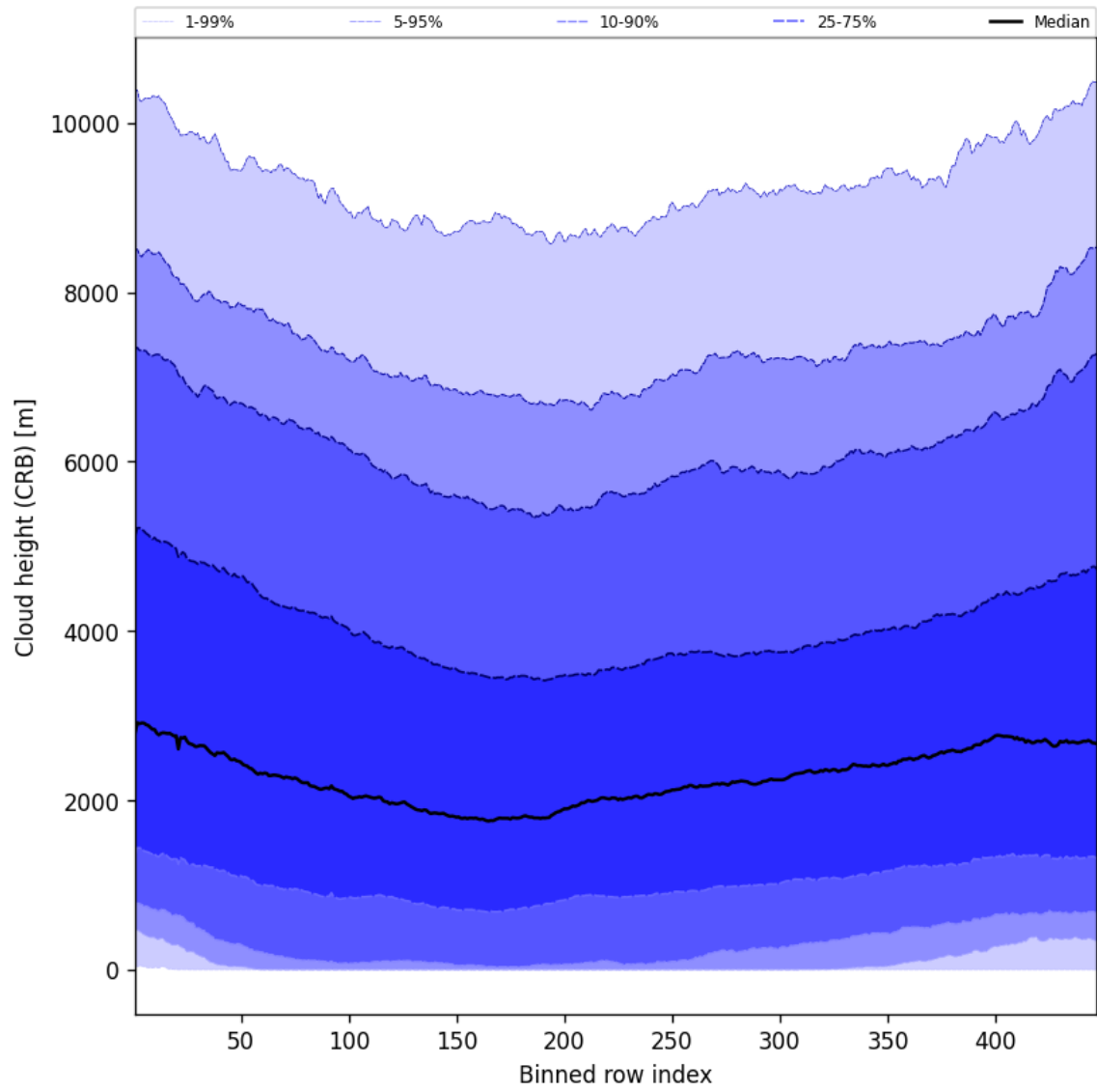
Figure 59: Along track statistics of “Cloud height (CRB)” for 2025-05-13 to 2025-05-15
