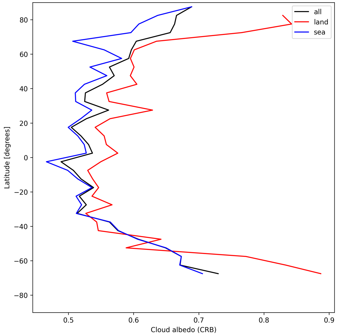
Figure 28: Zonal average of “Cloud albedo (CRB)” for 2025-05-13 to 2025-05-15.
