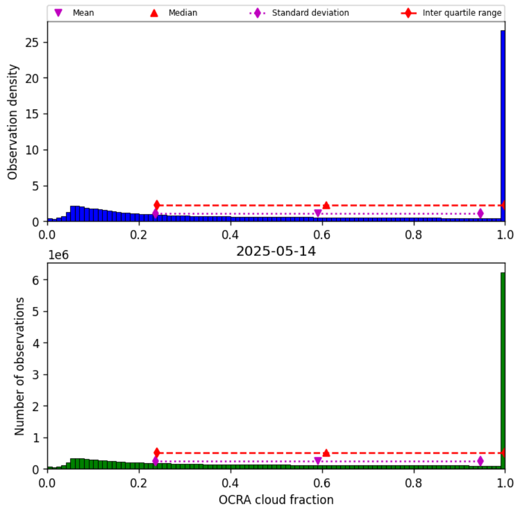
Figure 50: Histogram of “OCRA cloud fraction” for 2025-05-13 to 2025-05-15
