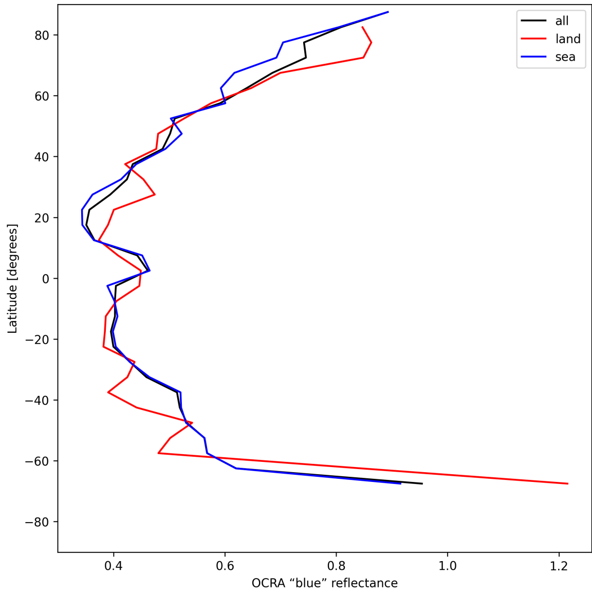
Figure 35: Zonal average of “OCRA “blue” reflectance” for 2025-05-13 to 2025-05-15.
