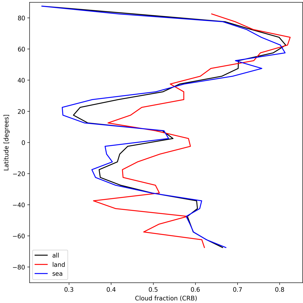
Figure 26: Zonal average of “Cloud fraction (CRB)” for 2025-05-13 to 2025-05-15.
