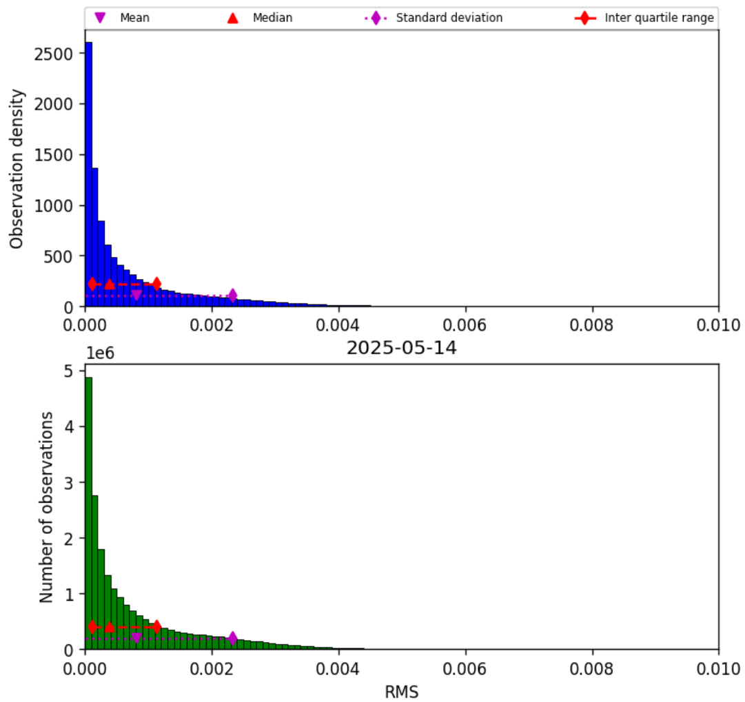
Figure 47: Histogram of “RMS” for 2025-05-13 to 2025-05-15
