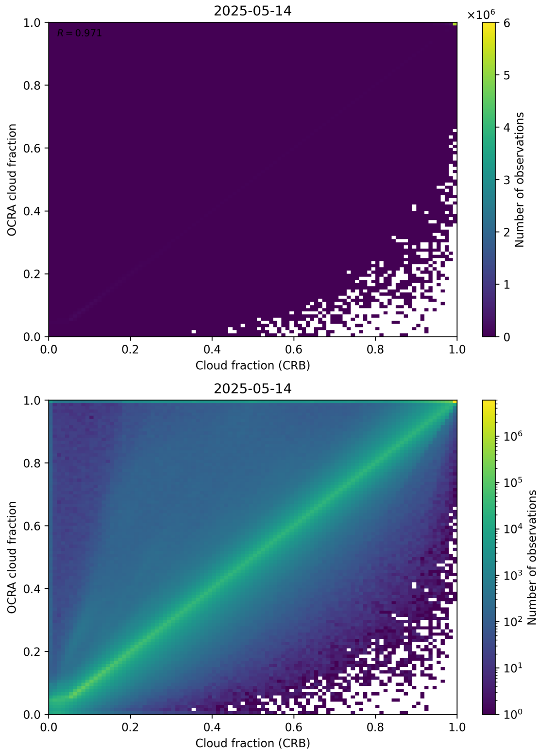
Figure 78: Scatter density plot of “Cloud fraction (CRB)” against “OCRA cloud fraction” for 2025-05-13 to 2025-05-15.
