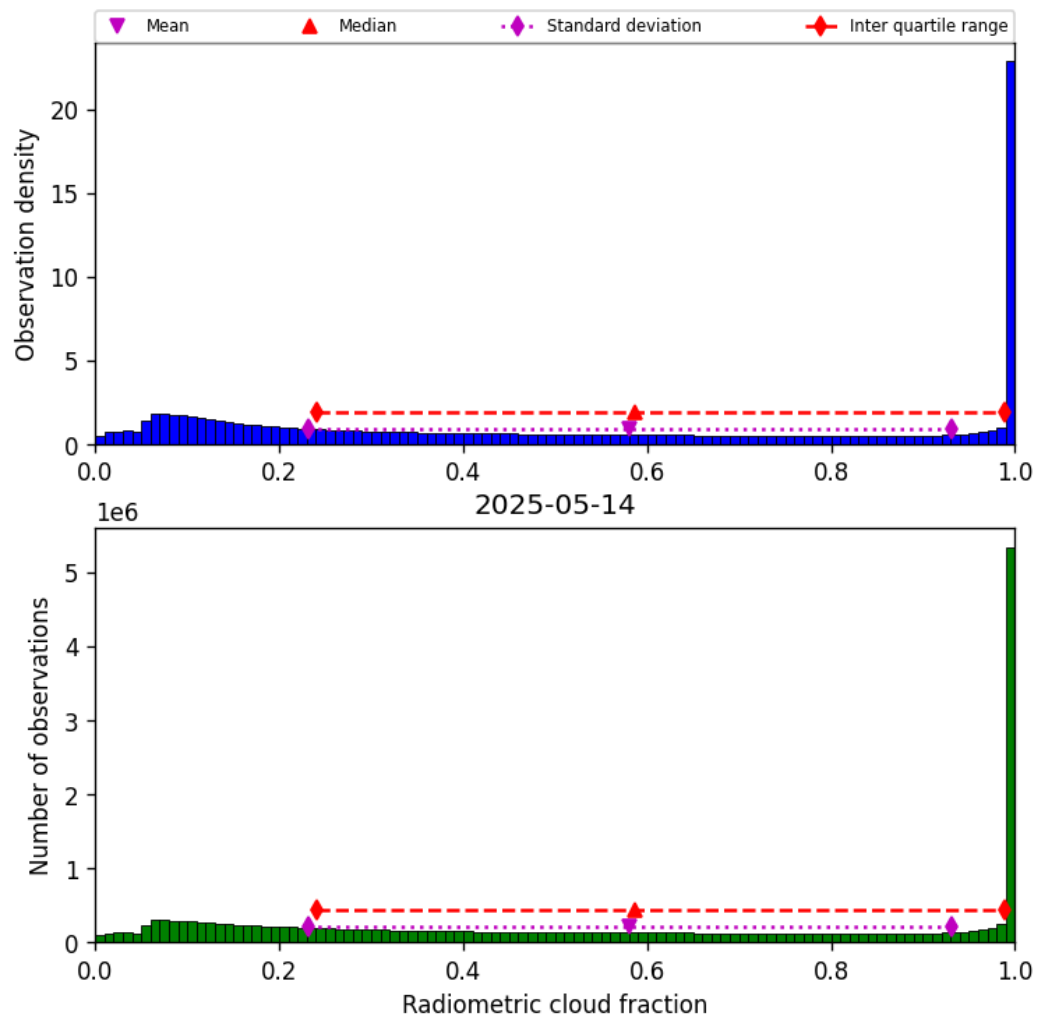
Figure 39: Histogram of “Radiometric cloud fraction” for 2025-05-13 to 2025-05-15
