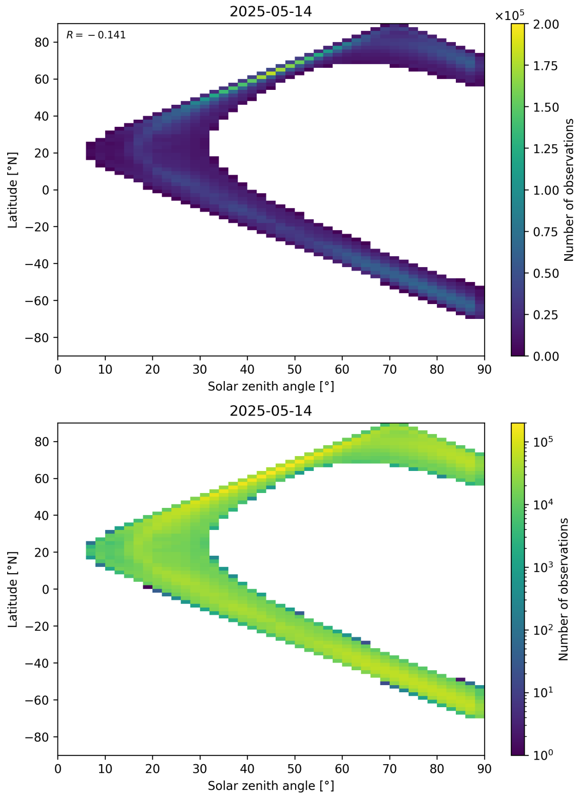
Figure 105: Scatter density plot of “Solar zenith angle” against “Latitude” for 2025-05-13 to 2025-05-15.
