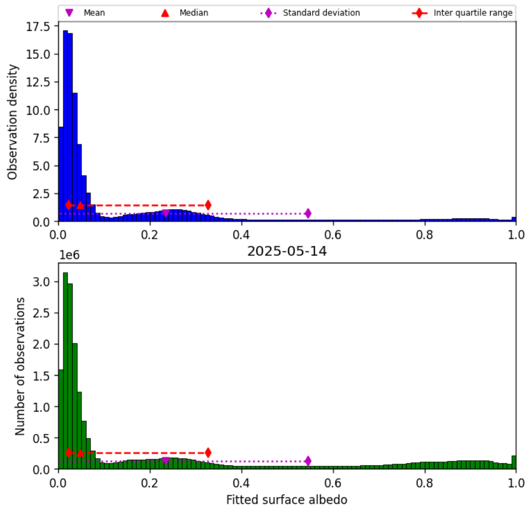
Figure 45: Histogram of “Fitted surface albedo” for 2025-05-13 to 2025-05-15
