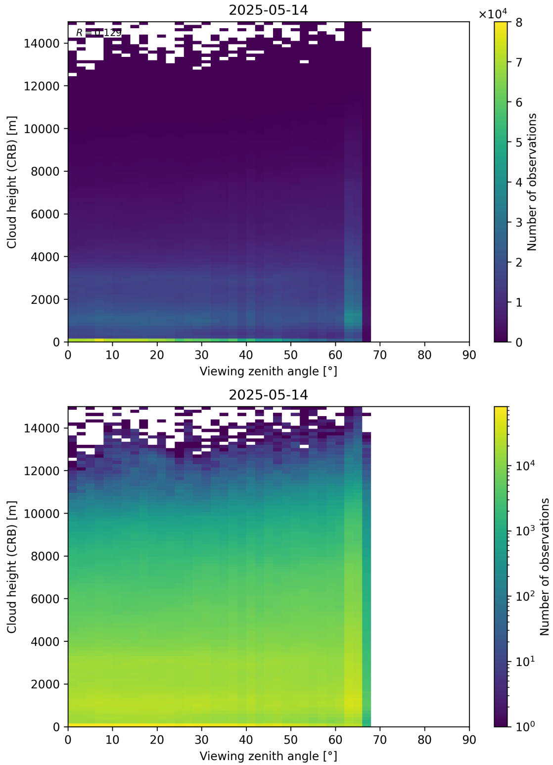
Figure 110: Scatter density plot of “Viewing zenith angle” against “Cloud height (CRB)” for 2025-05-13 to 2025-05-15.
