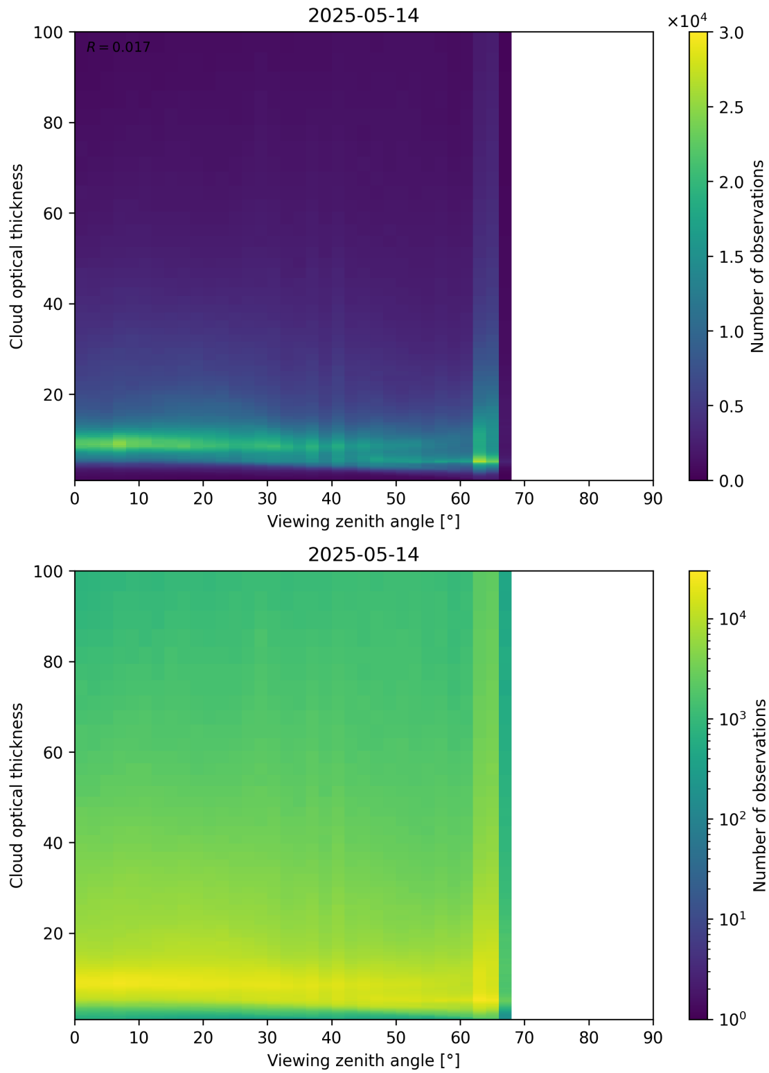
Figure 111: Scatter density plot of “Viewing zenith angle” against “Cloud optical thickness” for 2025-05-13 to 2025-05-15.
