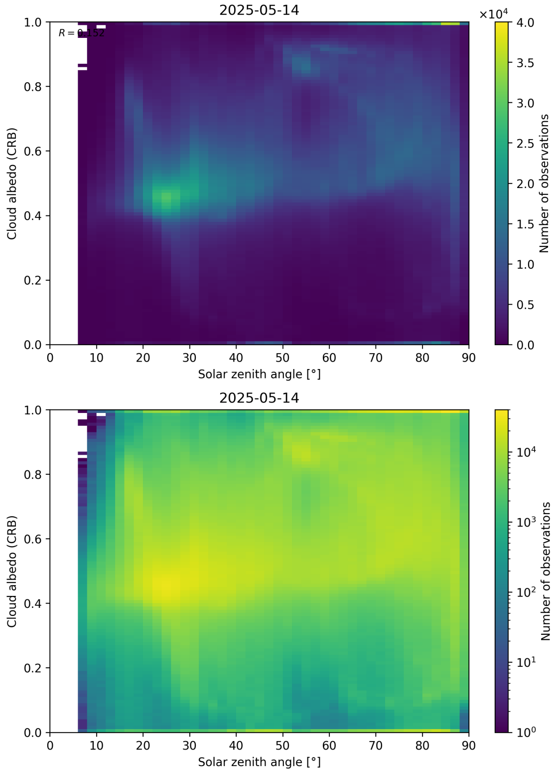
Figure 98: Scatter density plot of “Solar zenith angle” against “Cloud albedo (CRB)” for 2025-05-13 to 2025-05-15.
