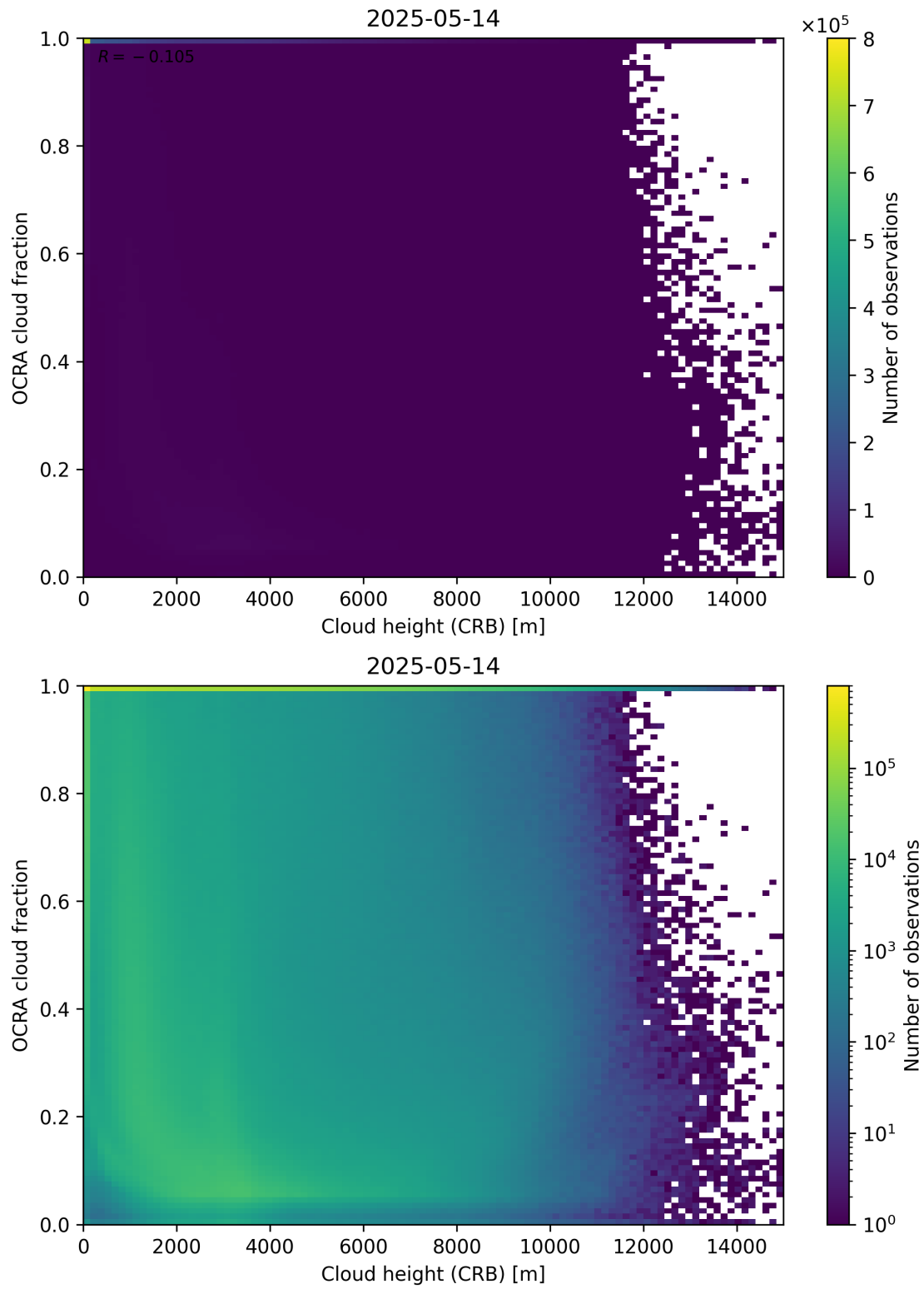
Figure 81: Scatter density plot of “Cloud height (CRB)” against “OCRA cloud fraction” for 2025-05-13 to 2025-05-15.
