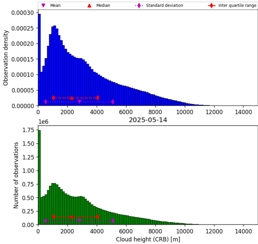
Figure 43: Histogram of “Cloud height (CRB)” for 2025-05-13 to 2025-05-15
