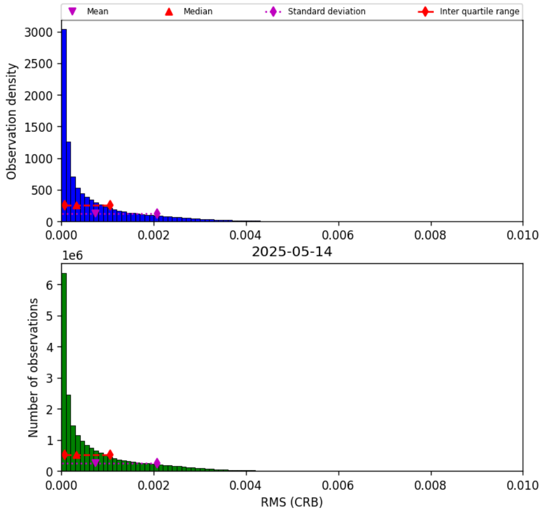
Figure 48: Histogram of “RMS (CRB)” for 2025-05-13 to 2025-05-15
