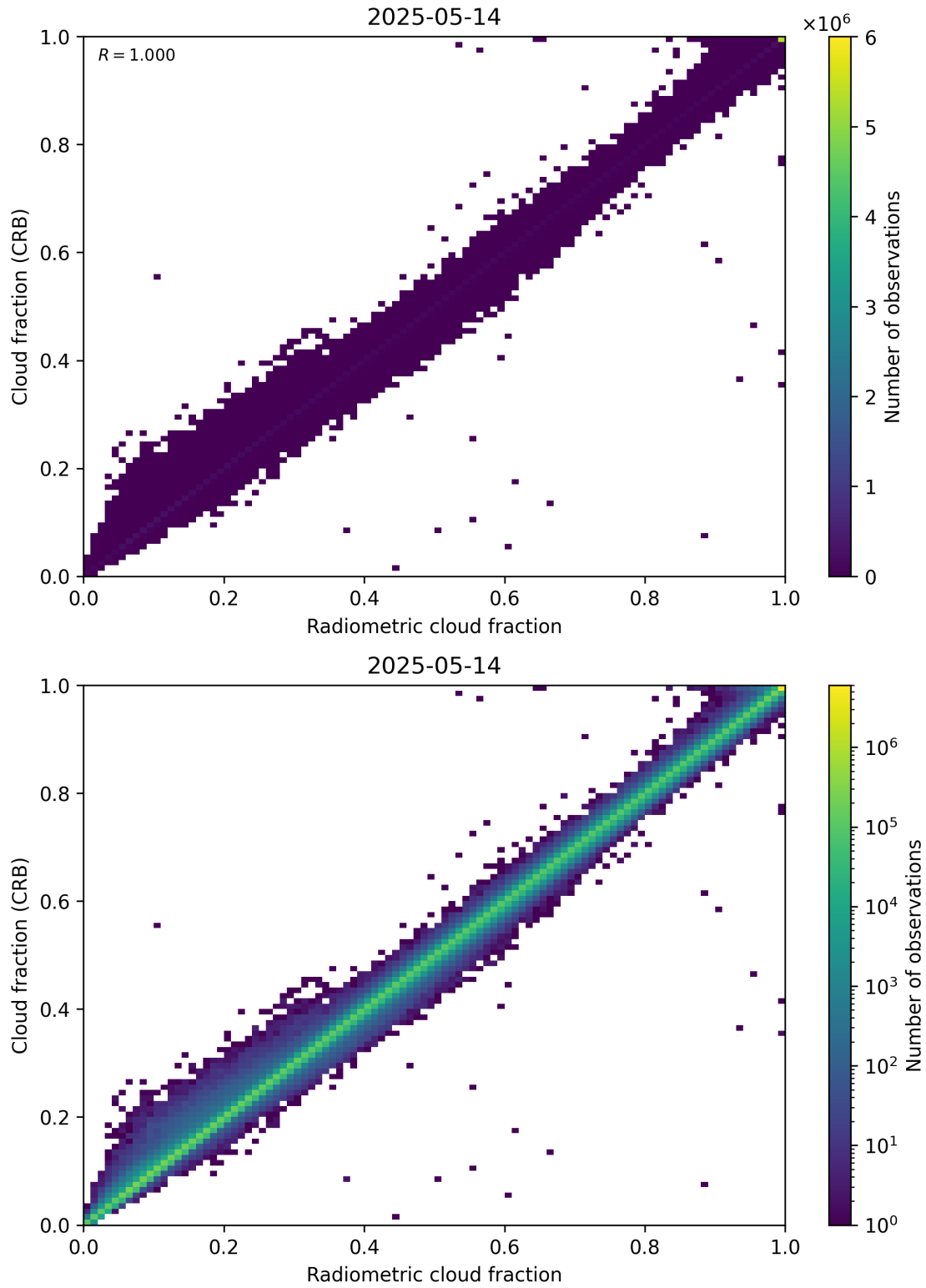
Figure 73: Scatter density plot of “Radiometric cloud fraction” against “Cloud fraction (CRB)” for 2025-05-13 to 2025-05-15.
