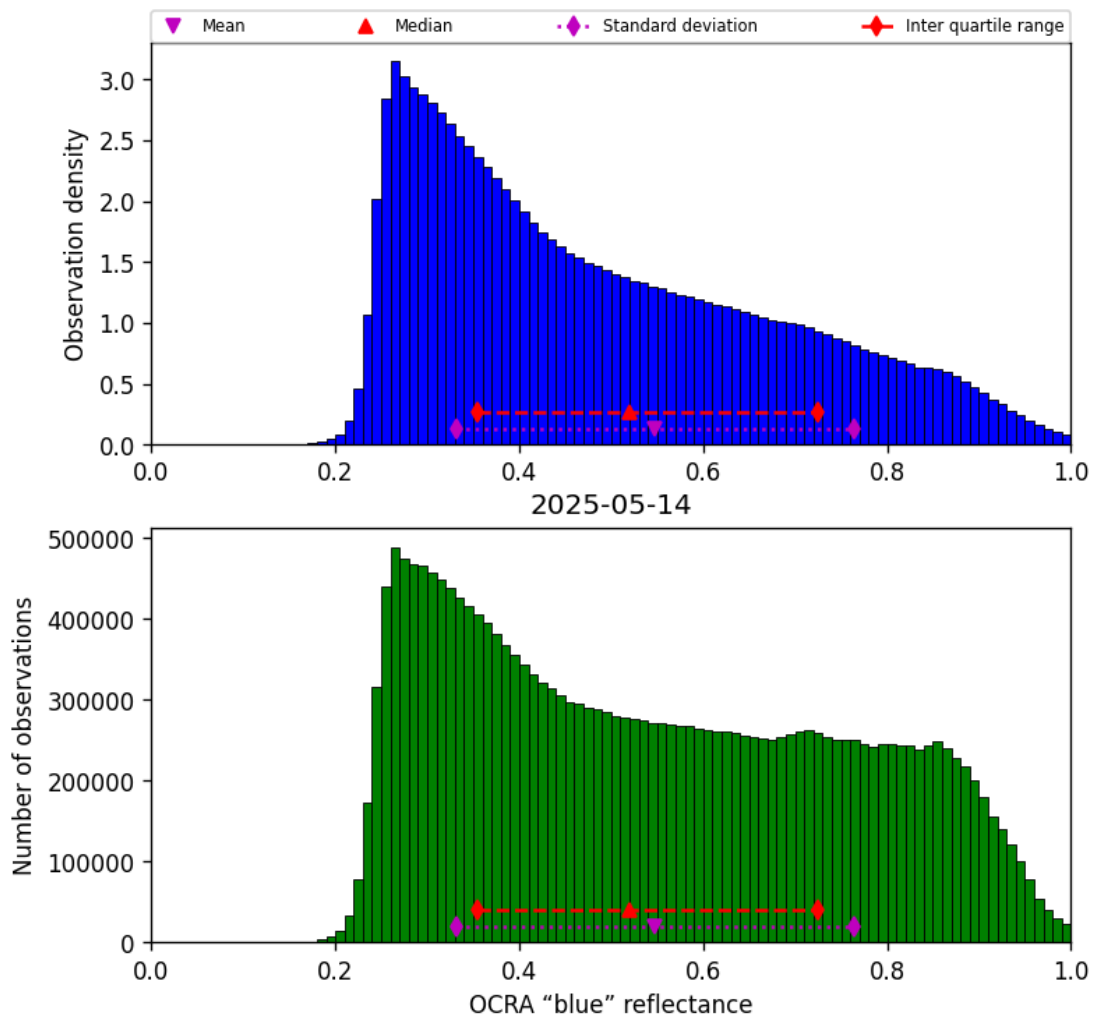
Figure 51: Histogram of “OCRA “blue” reflectance” for 2025-05-13 to 2025-05-15
