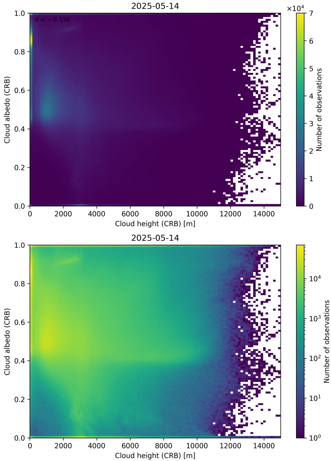
Figure 80: Scatter density plot of “Cloud height (CRB)” against “Cloud albedo (CRB)” for 2025-05-13 to 2025-05-15.
