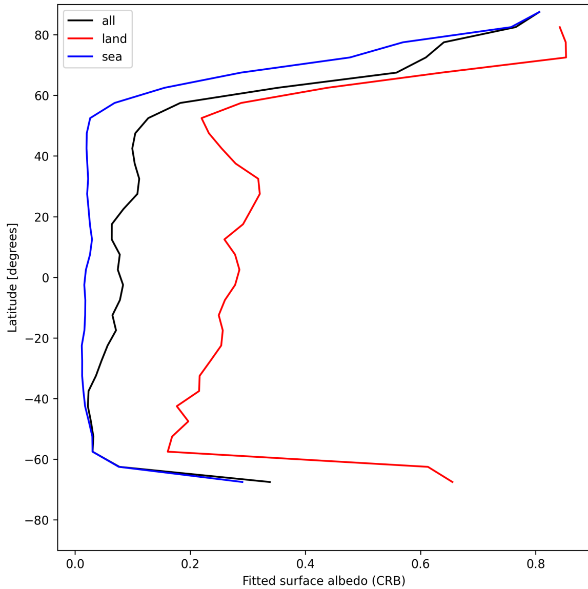
Figure 30: Zonal average of "Fitted surface albedo (CRB)" for 2025-05-13 to 2025-05-15.
