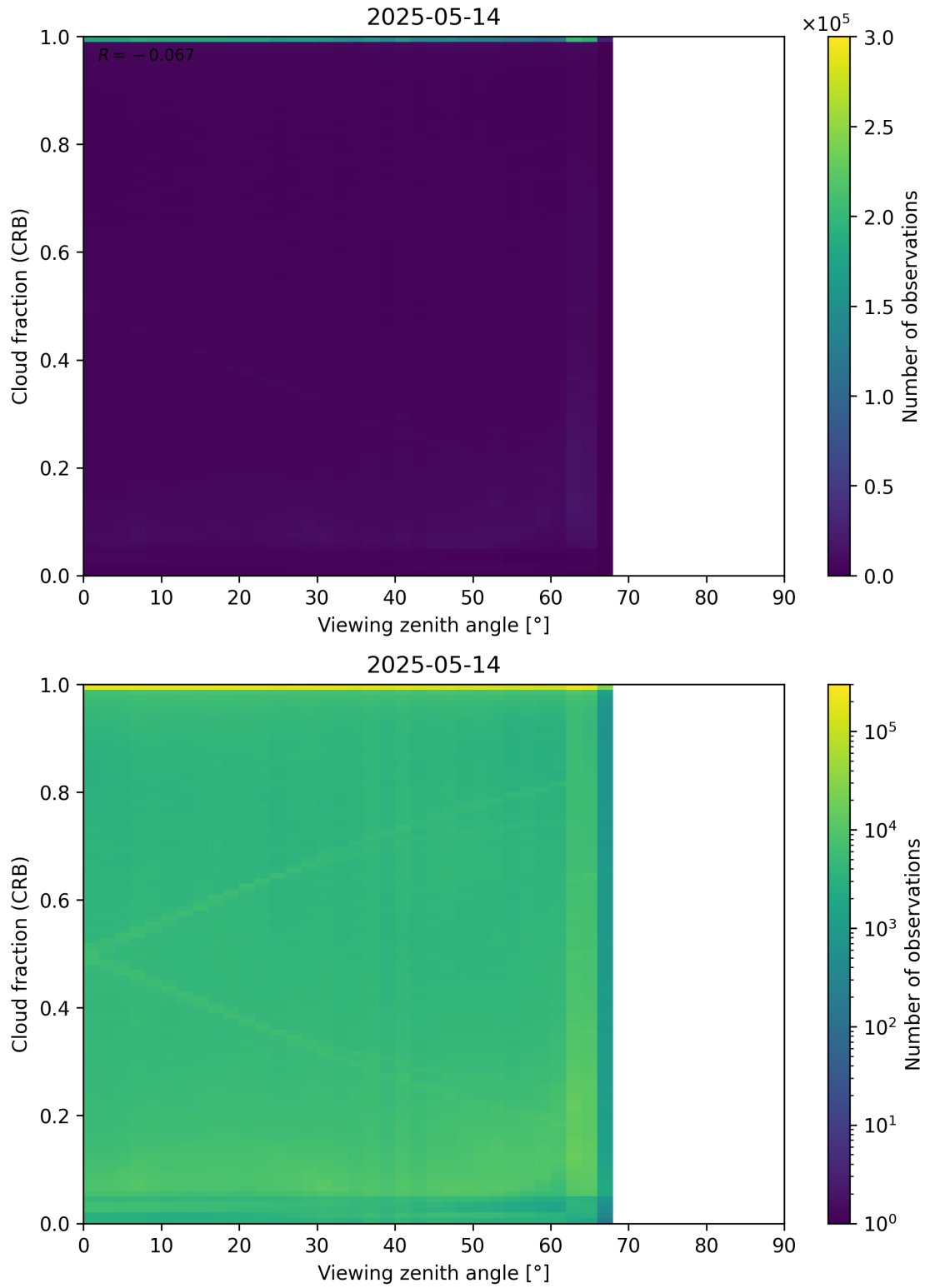
Figure 109: Scatter density plot of “Viewing zenith angle” against “Cloud fraction (CRB)” for 2025-05-13 to 2025-05-15.
