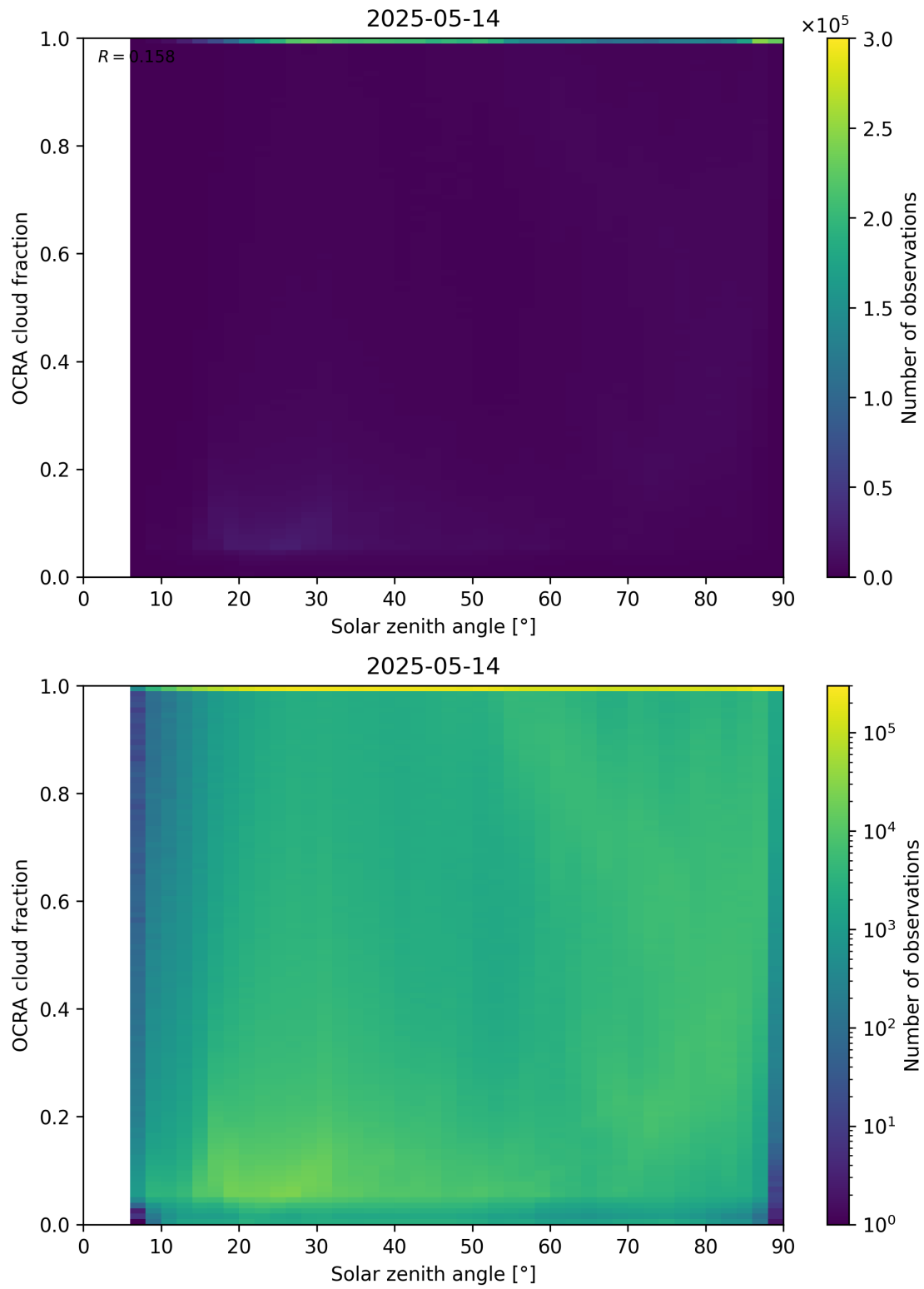
Figure 100: Scatter density plot of “Solar zenith angle” against “OCRA cloud fraction” for 2025-05-13 to 2025-05-15.
