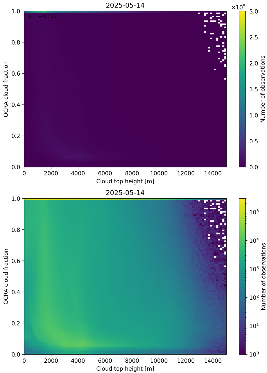
Figure 87: Scatter density plot of “Cloud top height” against “OCRA cloud fraction” for 2025-05-13 to 2025-05-15.
