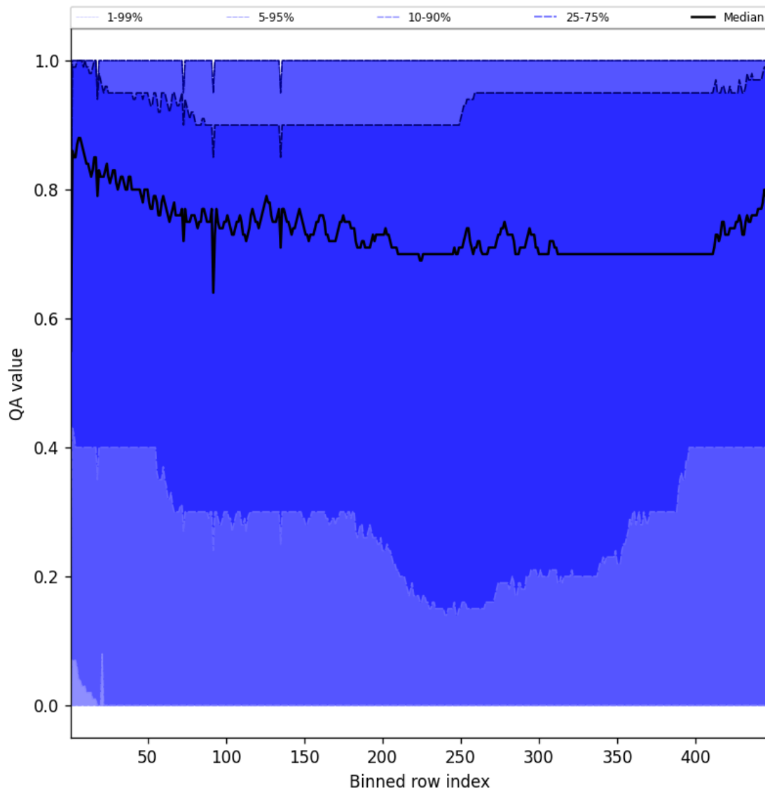
Figure 54: Along track statistics of “QA value” for 2025-05-13 to 2025-05-15
