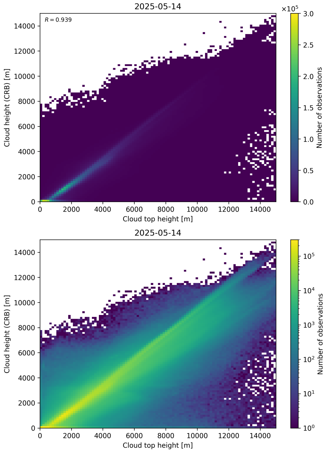
Figure 89: Scatter density plot of “Cloud top height” against “Cloud height (CRB)” for 2025-05-13 to 2025-05-15.
