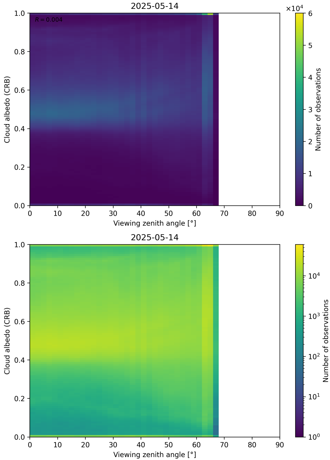
Figure 106: Scatter density plot of “Viewing zenith angle” against “Cloud albedo (CRB)” for 2025-05-13 to 2025-05-15.
