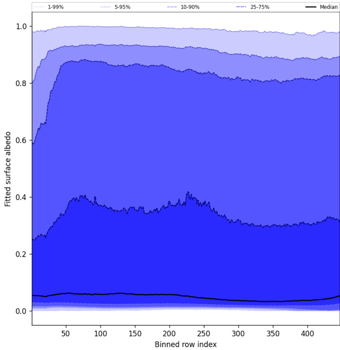
Figure 61: Along track statistics of “Fitted surface albedo” for 2025-05-13 to 2025-05-15
