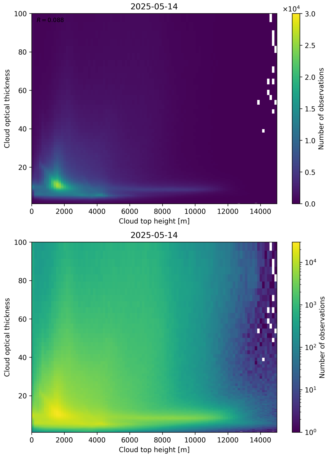
Figure 90: Scatter density plot of “Cloud top height” against “Cloud optical thickness” for 2025-05-13 to 2025-05-15.
