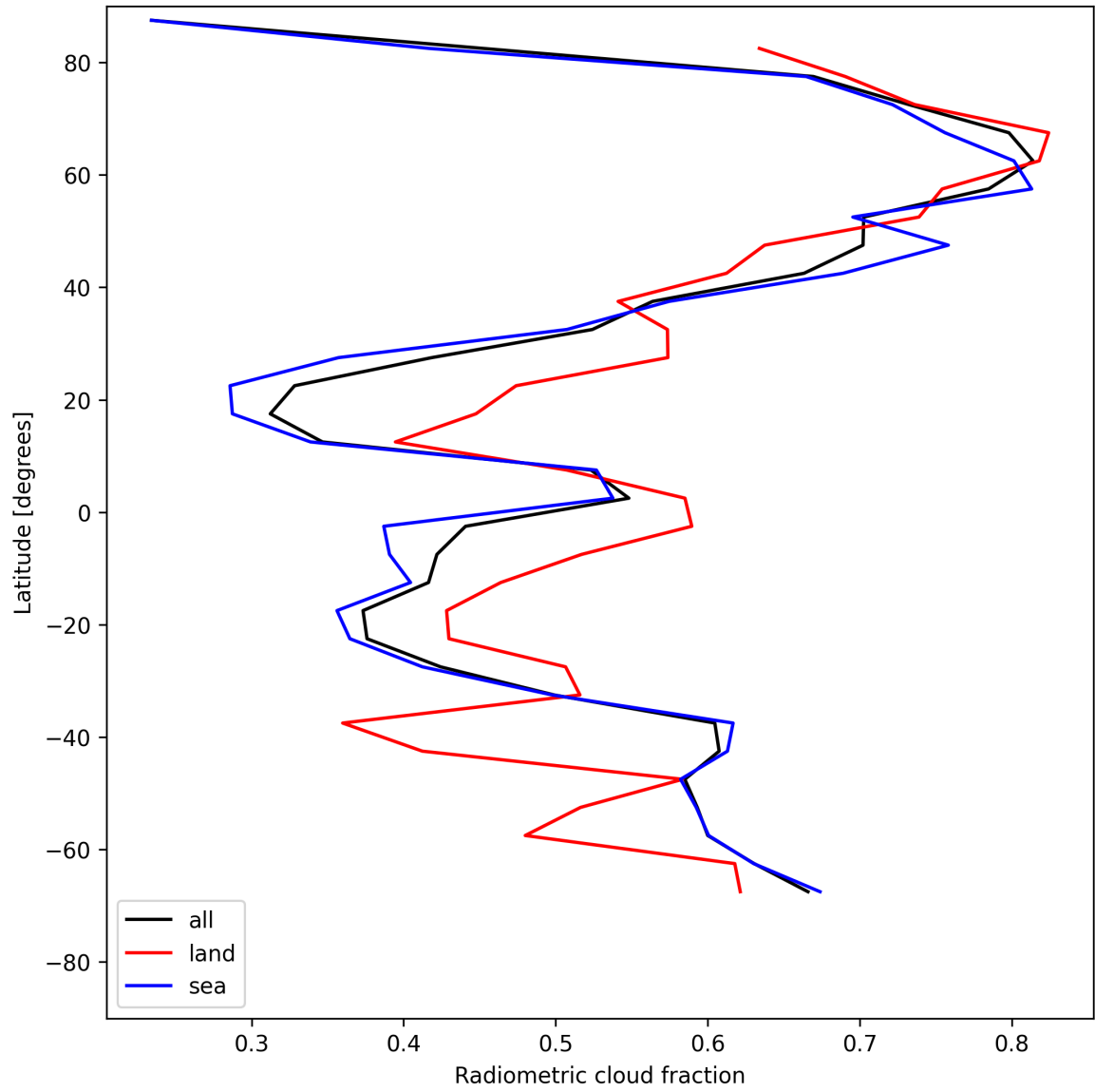
Figure 23: Zonal average of “Radiometric cloud fraction” for 2025-05-13 to 2025-05-15.
