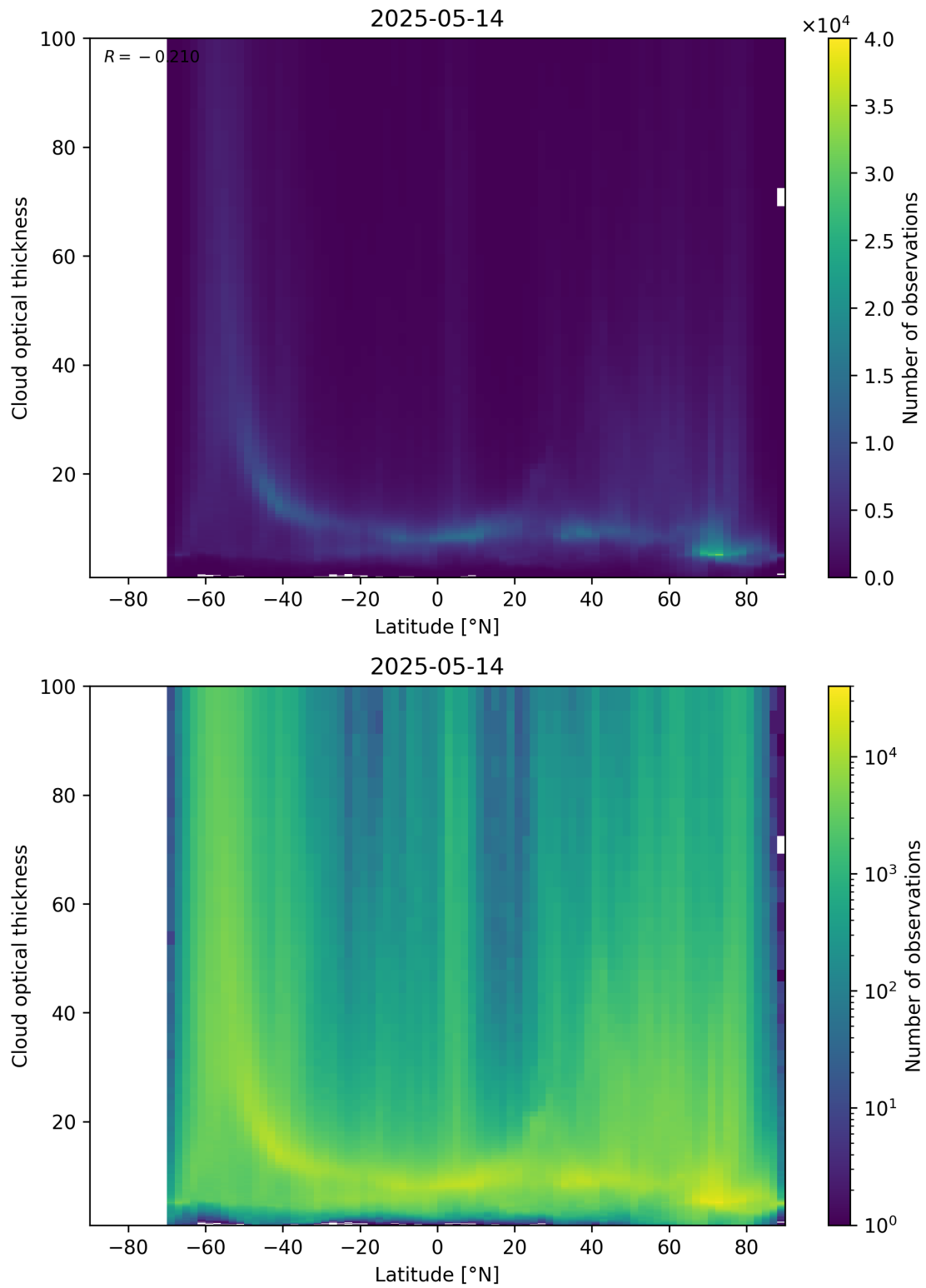
Figure 96: Scatter density plot of “Latitude” against “Cloud optical thickness” for 2025-05-13 to 2025-05-15.
