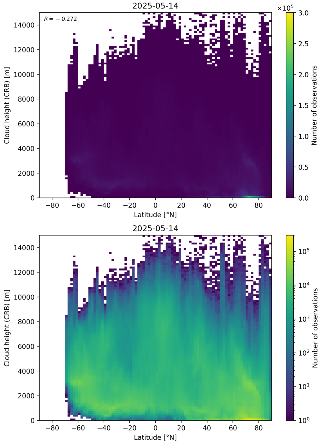
Figure 95: Scatter density plot of “Latitude” against “Cloud height (CRB)” for 2025-05-13 to 2025-05-15.
