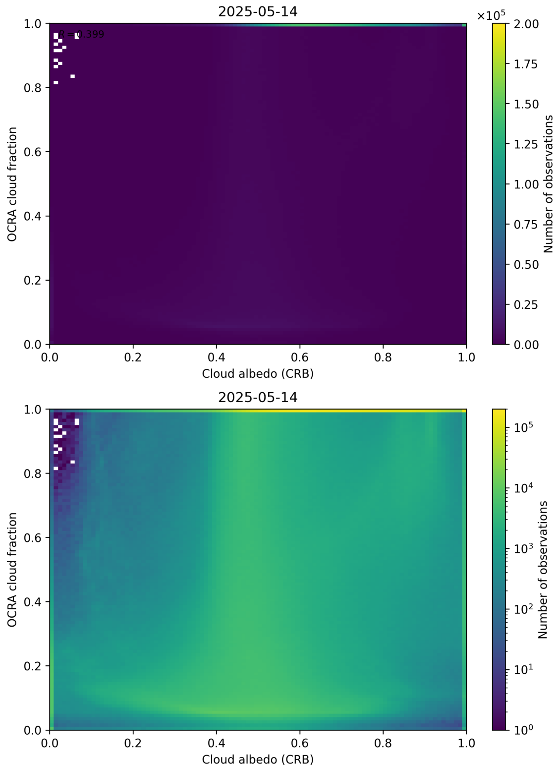
Figure 70: Scatter density plot of “Cloud albedo (CRB)” against “OCRA cloud fraction” for 2025-05-13 to 2025-05-15.
