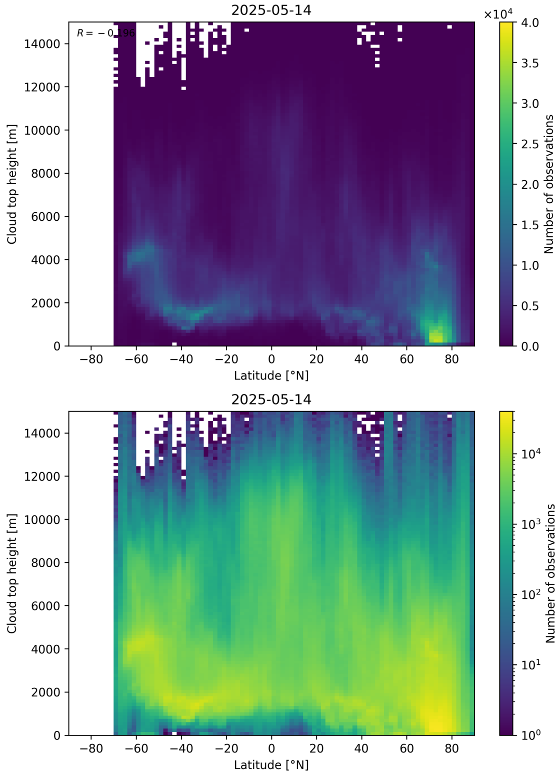
Figure 97: Scatter density plot of “Latitude” against “Cloud top height” for 2025-05-13 to 2025-05-15.
