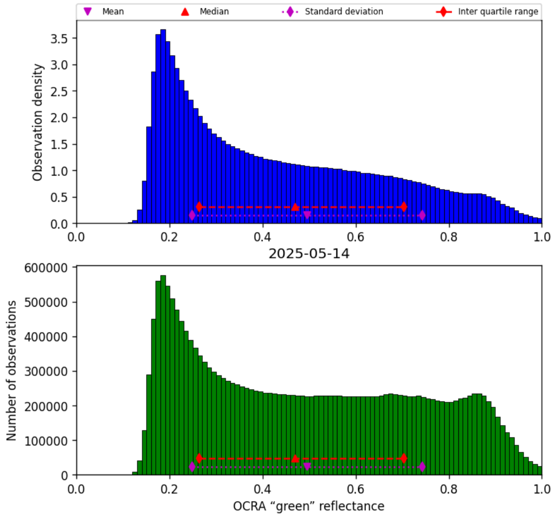
Figure 52: Histogram of “OCRA “green” reflectance” for 2025-05-13 to 2025-05-15
