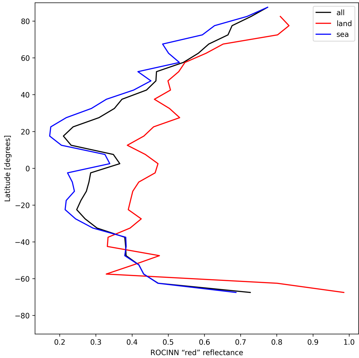
Figure 37: Zonal average of “ROCINN “red” reflectance” for 2025-05-13 to 2025-05-15.
