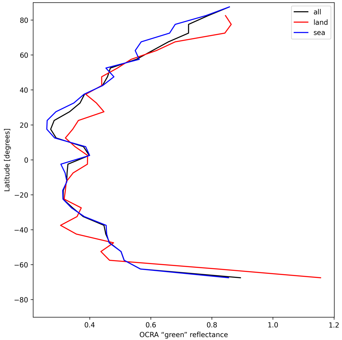
Figure 36: Zonal average of “OCRA “green” reflectance” for 2025-05-13 to 2025-05-15.
