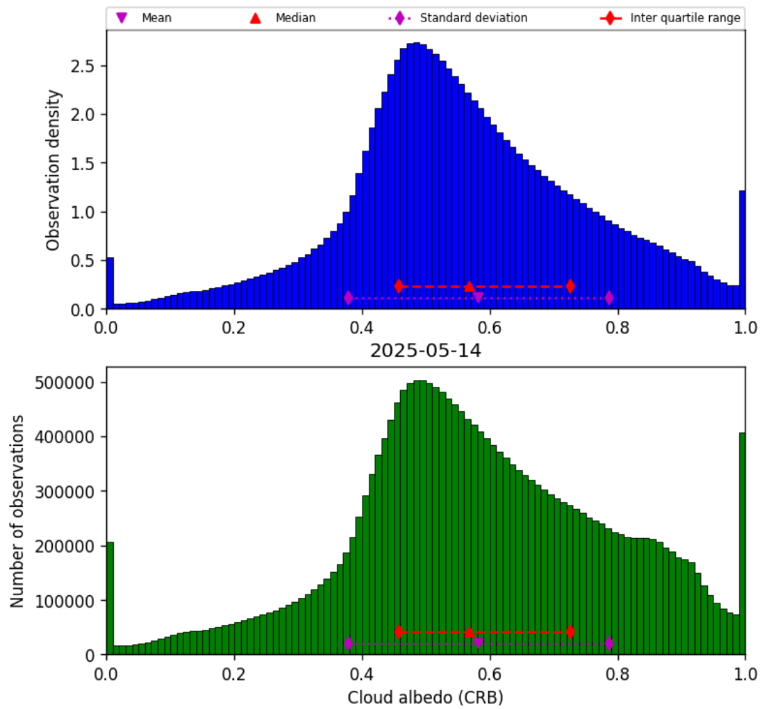
Figure 44: Histogram of “Cloud albedo (CRB)” for 2025-05-13 to 2025-05-15
