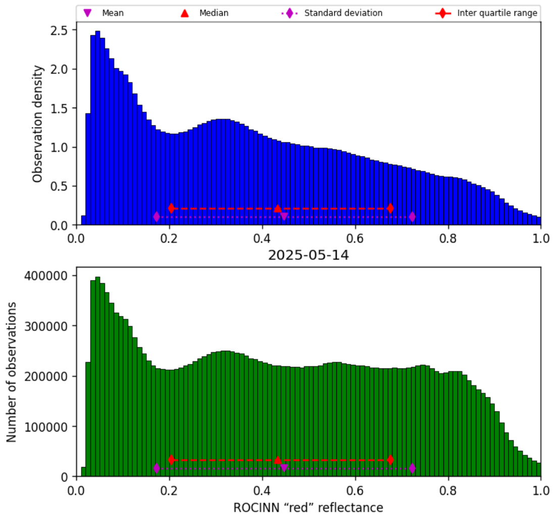
Figure 53: Histogram of “ROCINN “red” reflectance” for 2025-05-13 to 2025-05-15
