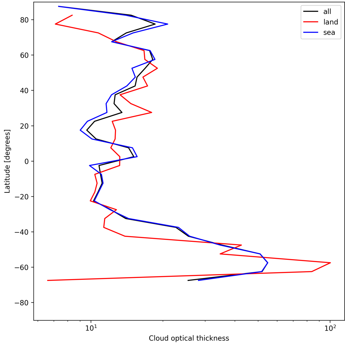
Figure 25: Zonal average of “Cloud optical thickness” for 2025-05-13 to 2025-05-15.
