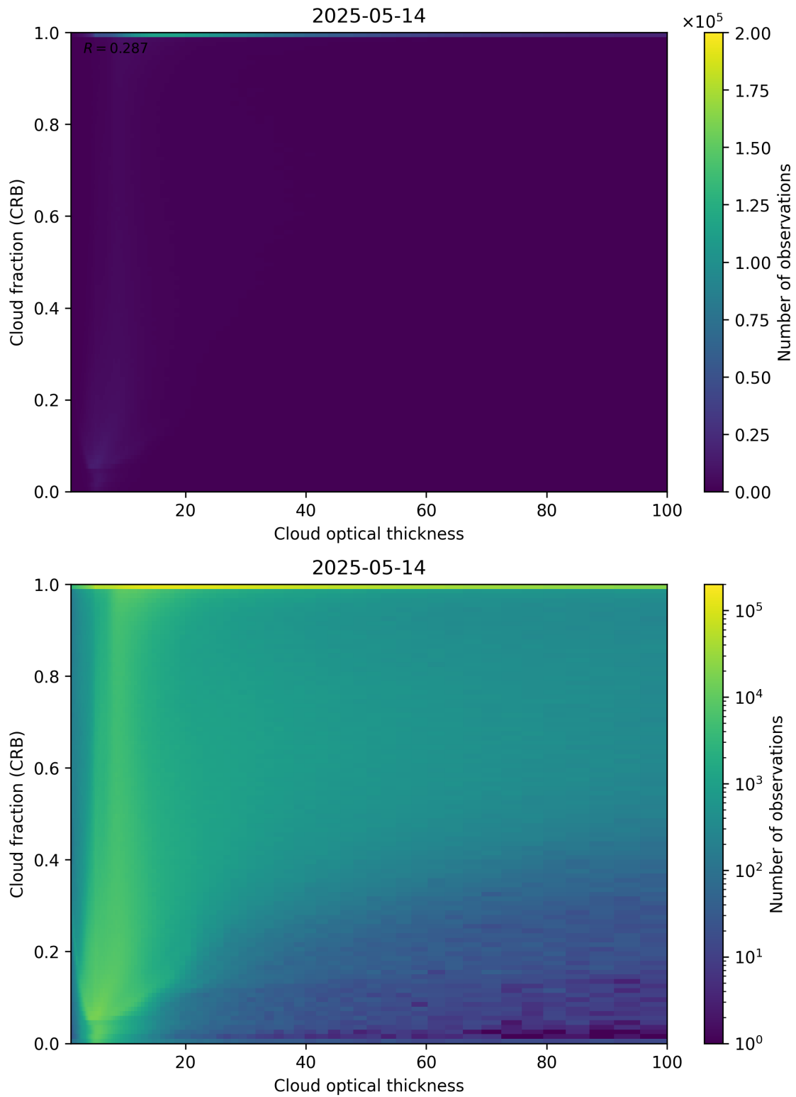
Figure 84: Scatter density plot of “Cloud optical thickness” against “Cloud fraction (CRB)” for 2025-05-13 to 2025-05-15.
