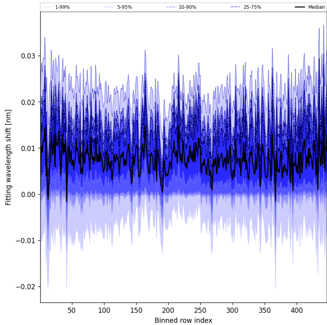
Figure 65: Along track statistics of “Fitting wavelength shift” for 2025-05-13 to 2025-05-15
