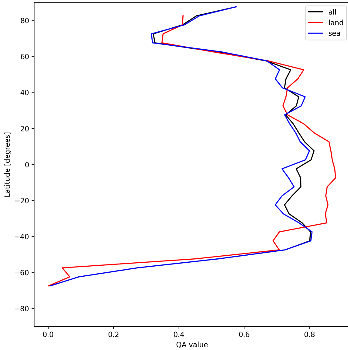
Figure 22: Zonal average of “QA value” for 2025-05-13 to 2025-05-15.
