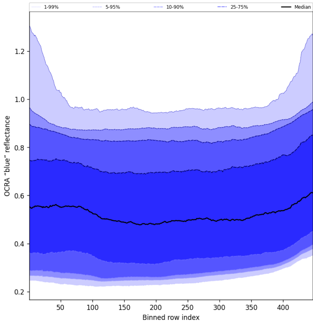
Figure 67: Along track statistics of “OCRA “blue” reflectance” for 2025-05-13 to 2025-05-15
