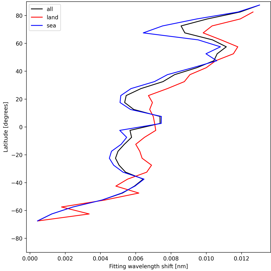
Figure 33: Zonal average of “Fitting wavelength shift” for 2025-05-13 to 2025-05-15.
