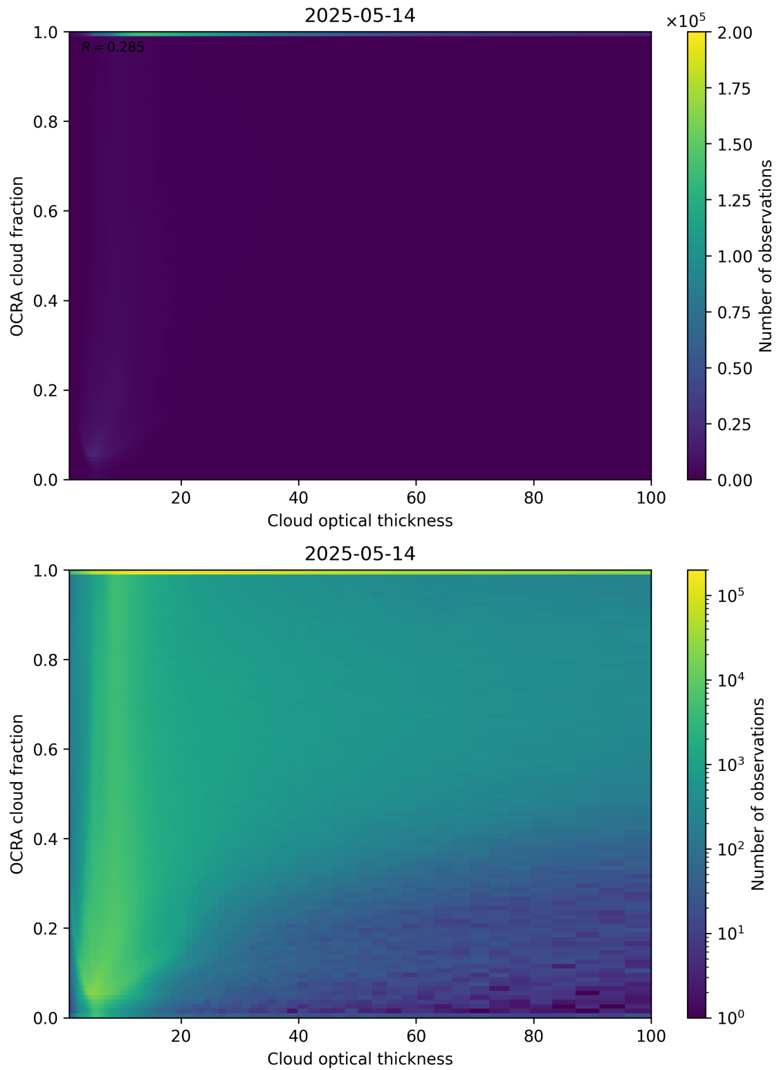
Figure 83: Scatter density plot of “Cloud optical thickness” against “OCRA cloud fraction” for 2025-05-13 to 2025-05-15.
