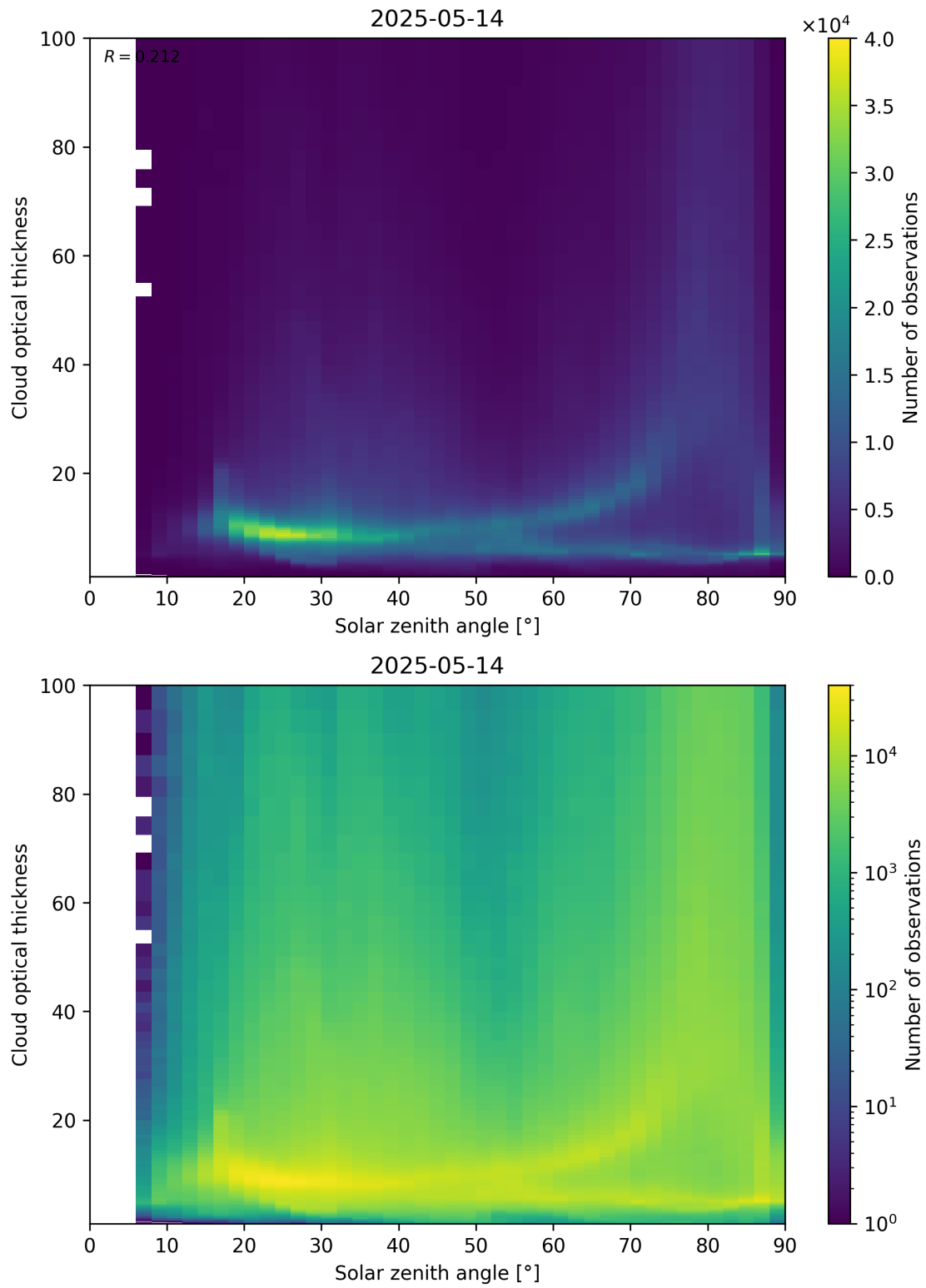
Figure 103: Scatter density plot of “Solar zenith angle” against “Cloud optical thickness” for 2025-05-13 to 2025-05-15.
