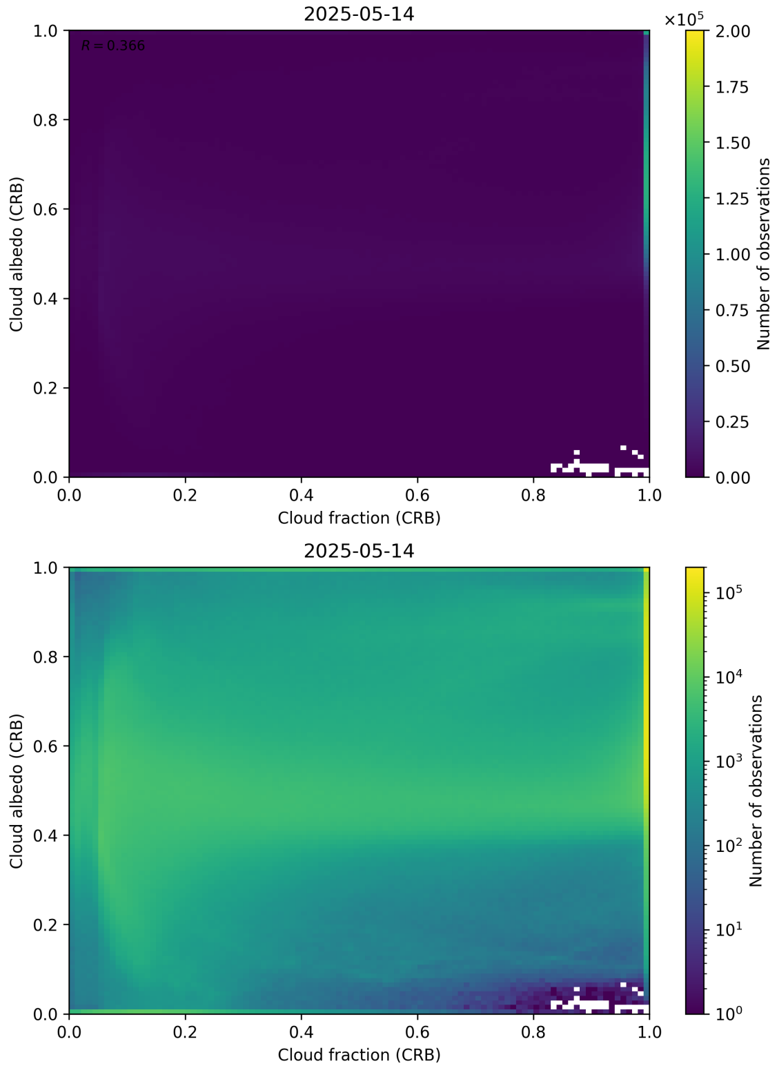
Figure 77: Scatter density plot of “Cloud fraction (CRB)” against “Cloud albedo (CRB)” for 2025-05-13 to 2025-05-15.
