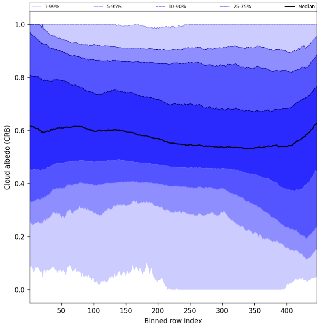
Figure 60: Along track statistics of “Cloud albedo (CRB)” for 2025-05-13 to 2025-05-15
