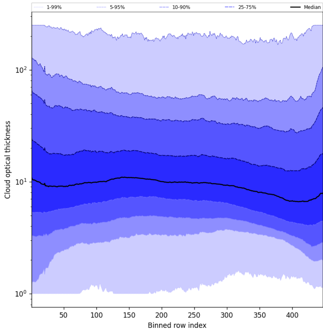
Figure 57: Along track statistics of “Cloud optical thickness” for 2025-05-13 to 2025-05-15
