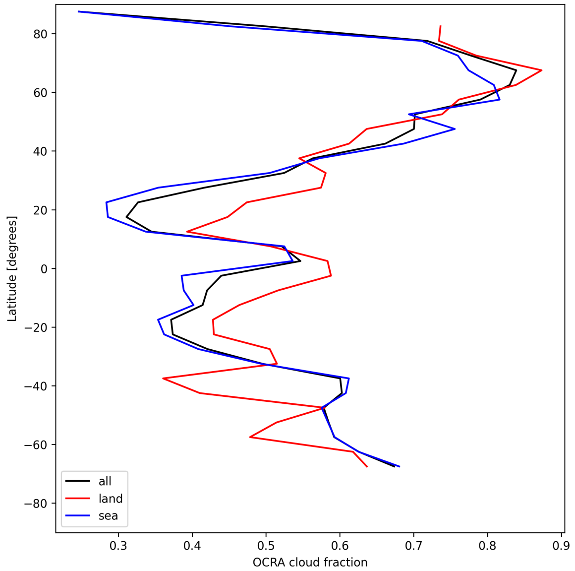
Figure 34: Zonal average of “OCRA cloud fraction” for 2025-05-13 to 2025-05-15.
