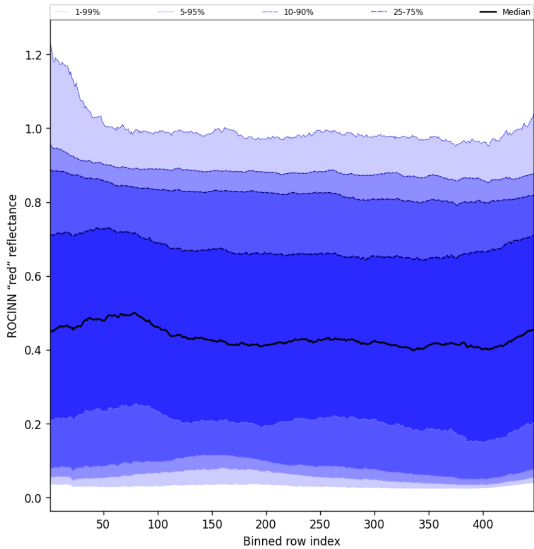
Figure 69: Along track statistics of “ROCINN “red” reflectance” for 2025-05-13 to 2025-05-15
