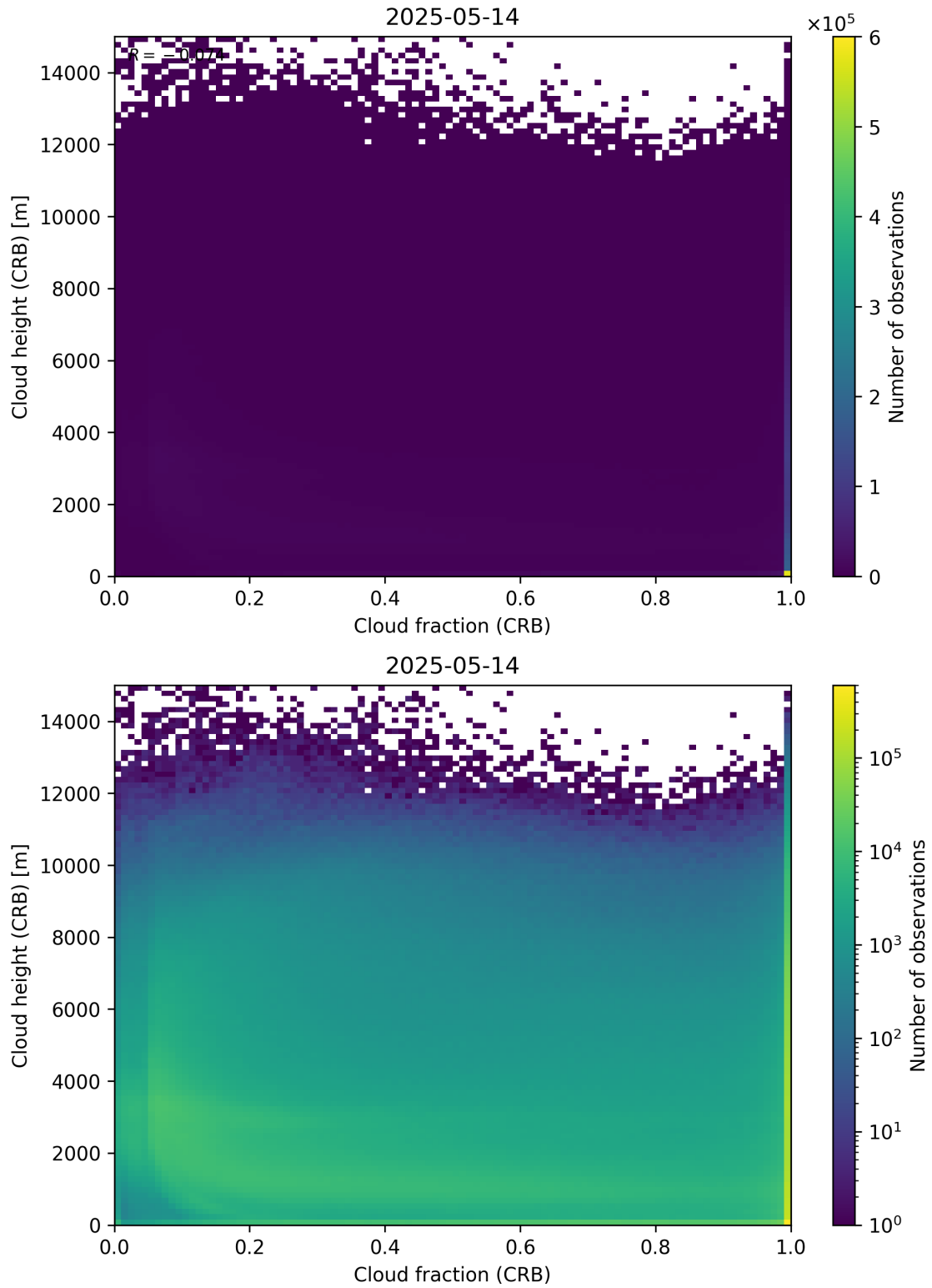
Figure 79: Scatter density plot of “Cloud fraction (CRB)” against “Cloud height (CRB)” for 2025-05-13 to 2025-05-15.
