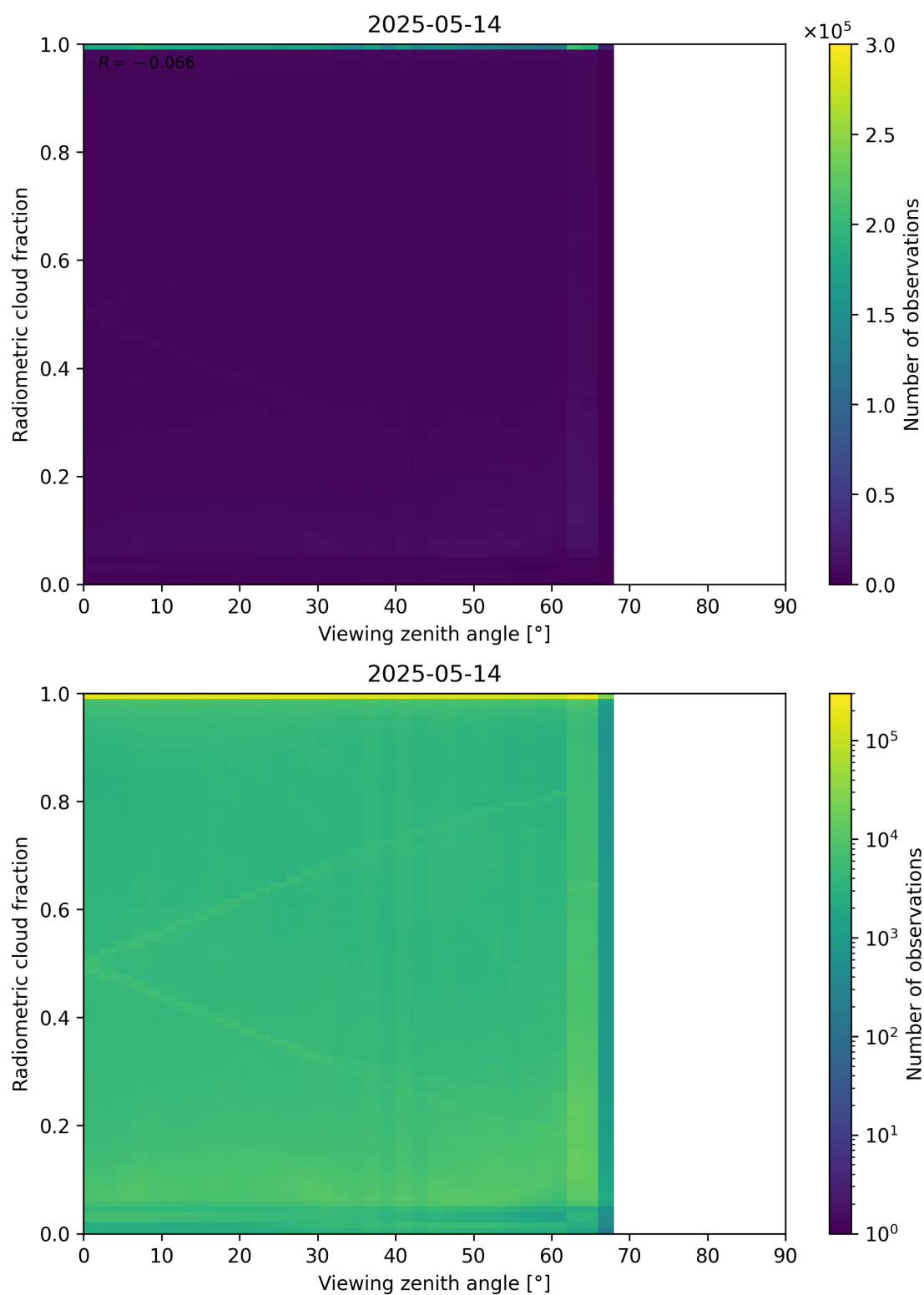
Figure 107: Scatter density plot of “Viewing zenith angle” against “Radiometric cloud fraction” for 2025-05-13 to 2025-05-15.
