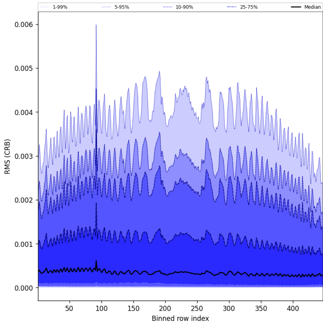
Figure 64: Along track statistics of “RMS (CRB)” for 2025-05-13 to 2025-05-15
