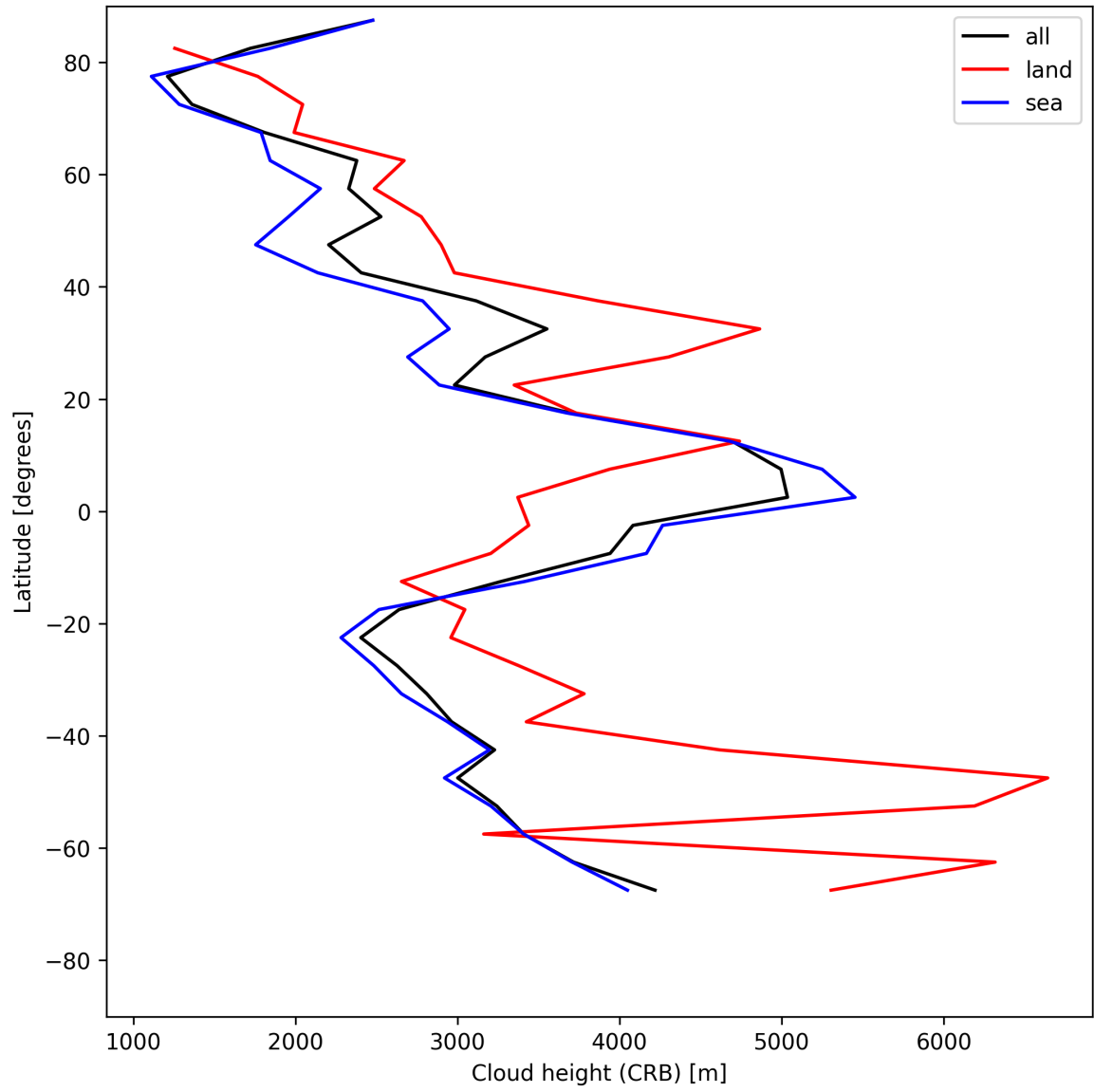
Figure 27: Zonal average of “Cloud height (CRB)” for 2025-05-13 to 2025-05-15.
