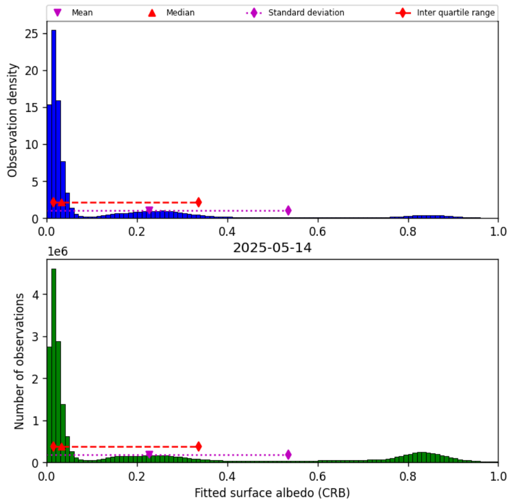
Figure 46: Histogram of “Fitted surface albedo (CRB)” for 2025-05-13 to 2025-05-15
