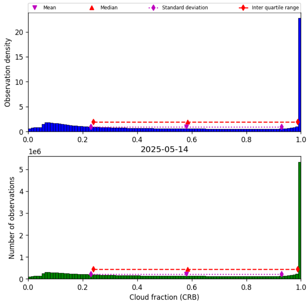
Figure 42: Histogram of “Cloud fraction (CRB)” for 2025-05-13 to 2025-05-15
