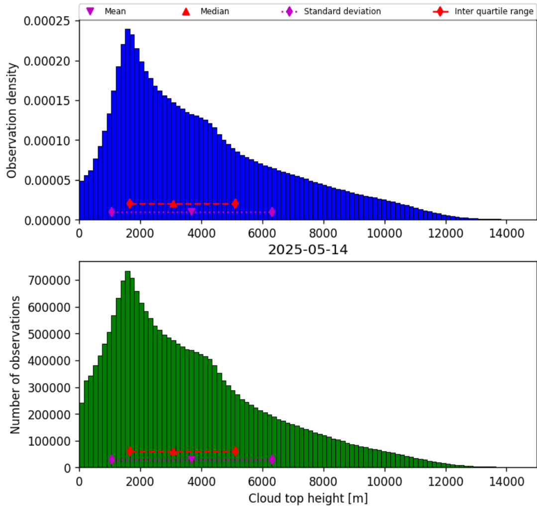
Figure 40: Histogram of “Cloud top height” for 2025-05-13 to 2025-05-15
