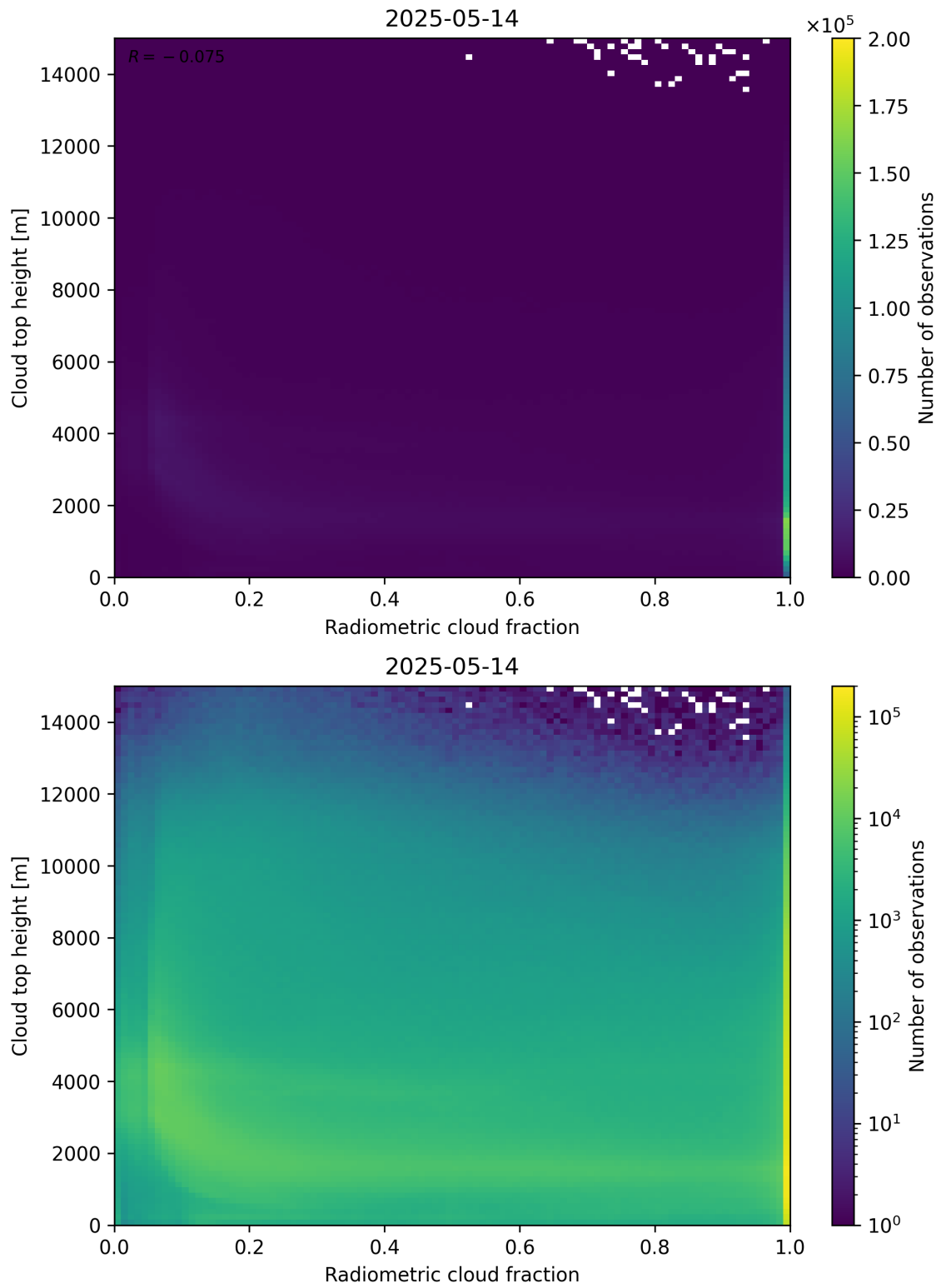
Figure 76: Scatter density plot of “Radiometric cloud fraction” against “Cloud top height” for 2025-05-13 to 2025-05-15.
