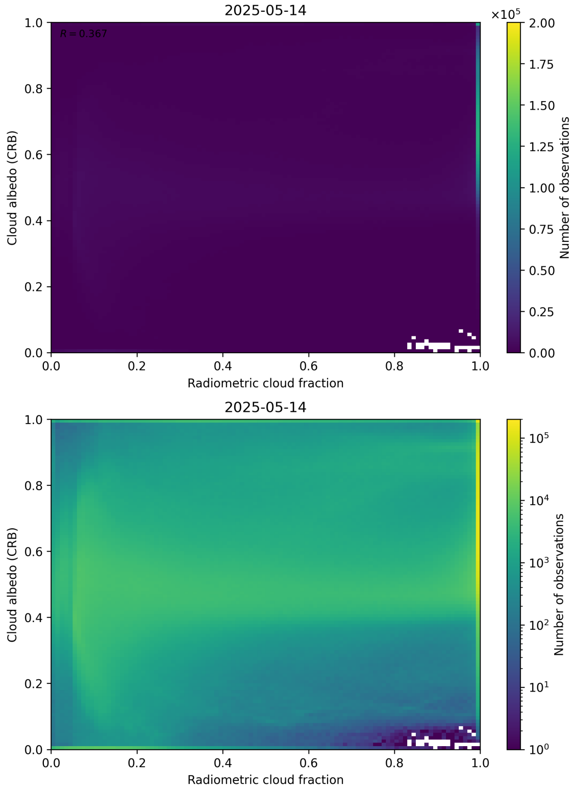
Figure 71: Scatter density plot of “Radiometric cloud fraction” against “Cloud albedo (CRB)” for 2025-05-13 to 2025-05-15.
