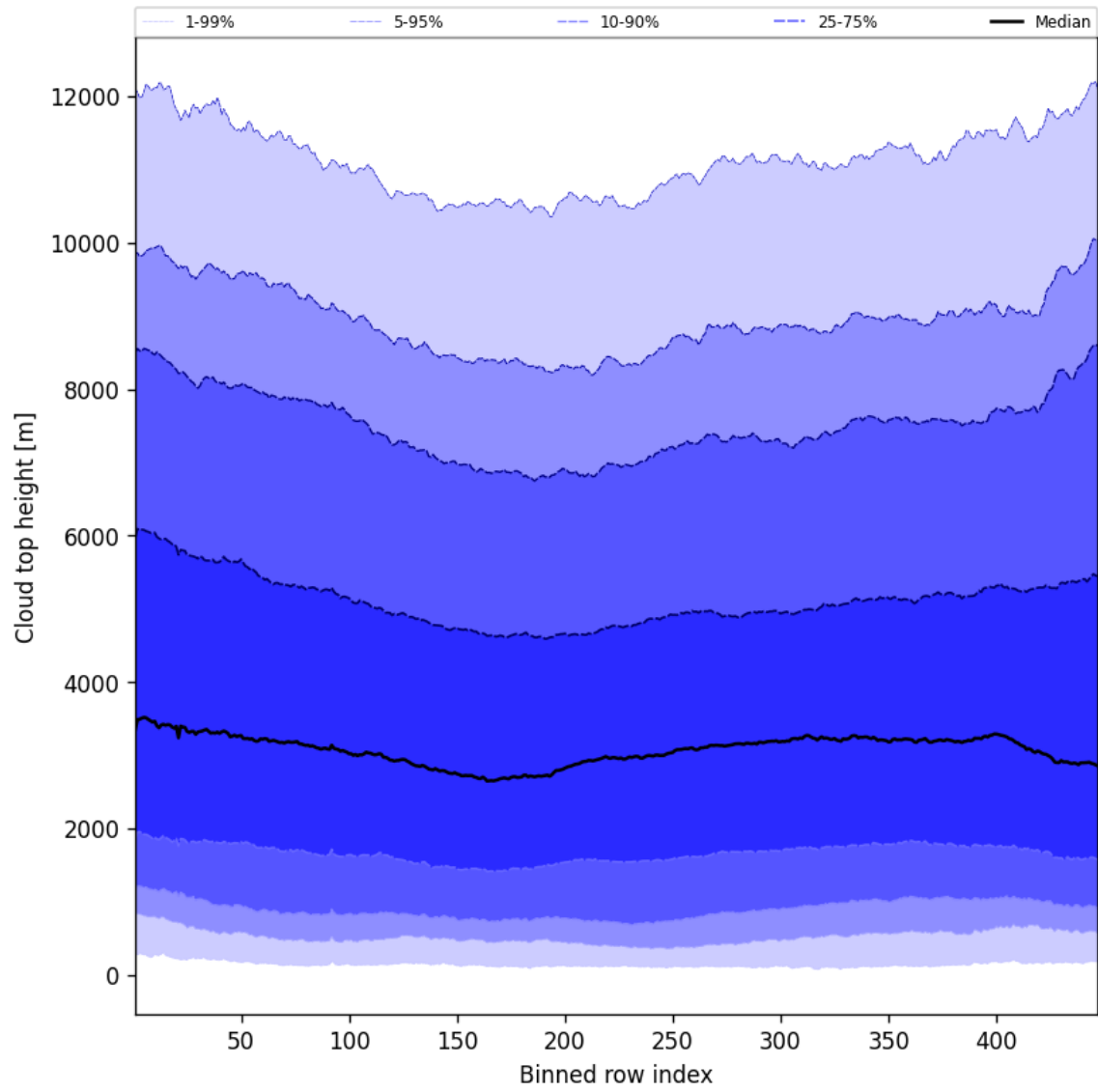
Figure 56: Along track statistics of “Cloud top height” for 2025-05-13 to 2025-05-15
