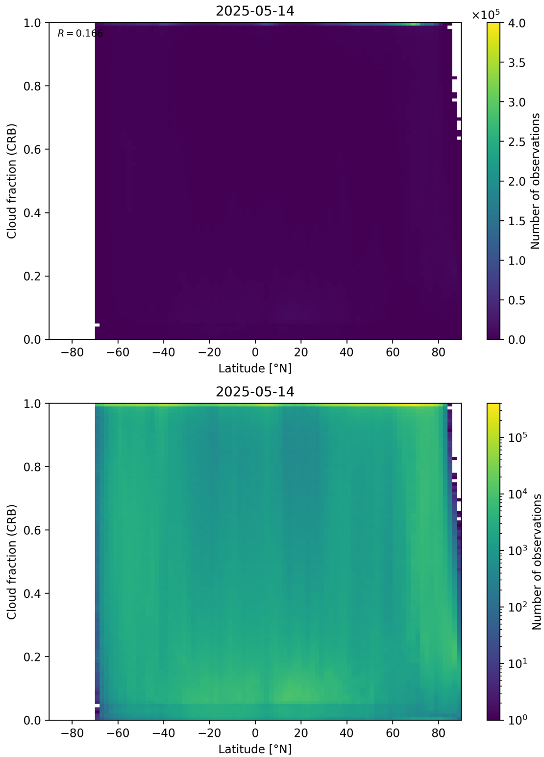
Figure 94: Scatter density plot of “Latitude” against “Cloud fraction (CRB)” for 2025-05-13 to 2025-05-15.
