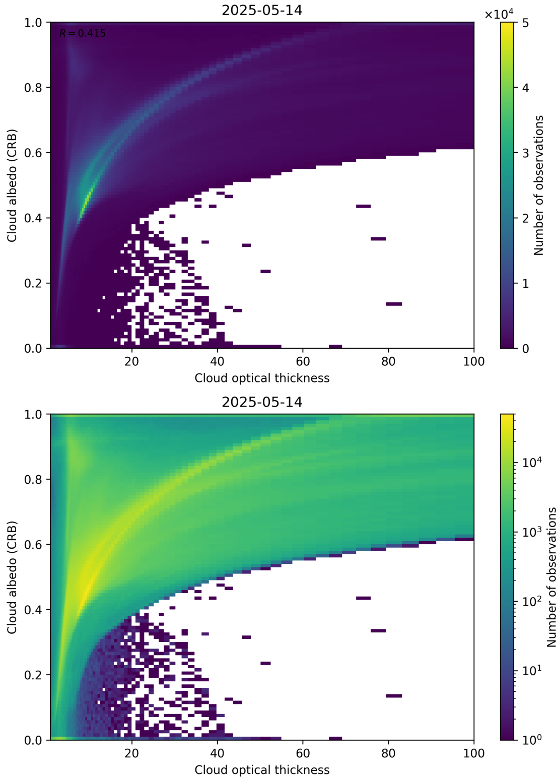
Figure 82: Scatter density plot of “Cloud optical thickness” against “Cloud albedo (CRB)” for 2025-05-13 to 2025-05-15.
