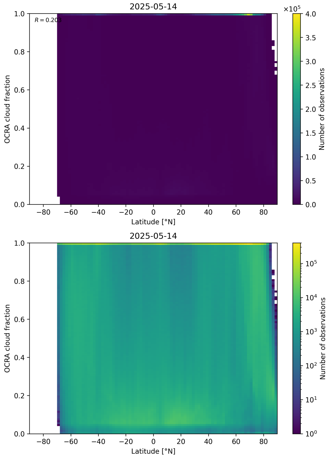
Figure 93: Scatter density plot of “Latitude” against “OCRA cloud fraction” for 2025-05-13 to 2025-05-15.
