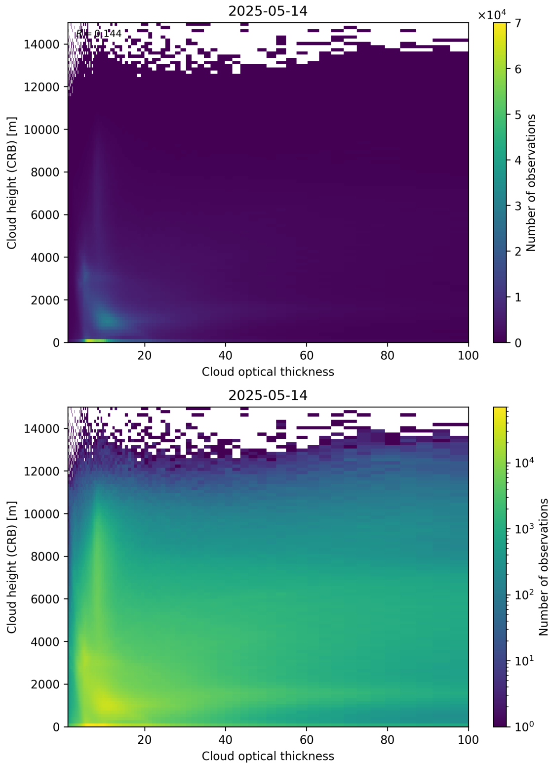
Figure 85: Scatter density plot of “Cloud optical thickness” against “Cloud height (CRB)” for 2025-05-13 to 2025-05-15.
