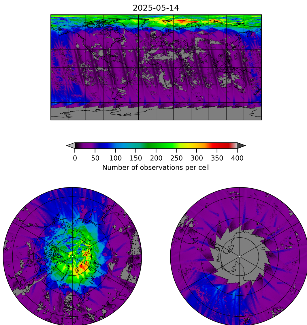
Figure 21: Map of the number of observations for 2025-05-13 to 2025-05-15
