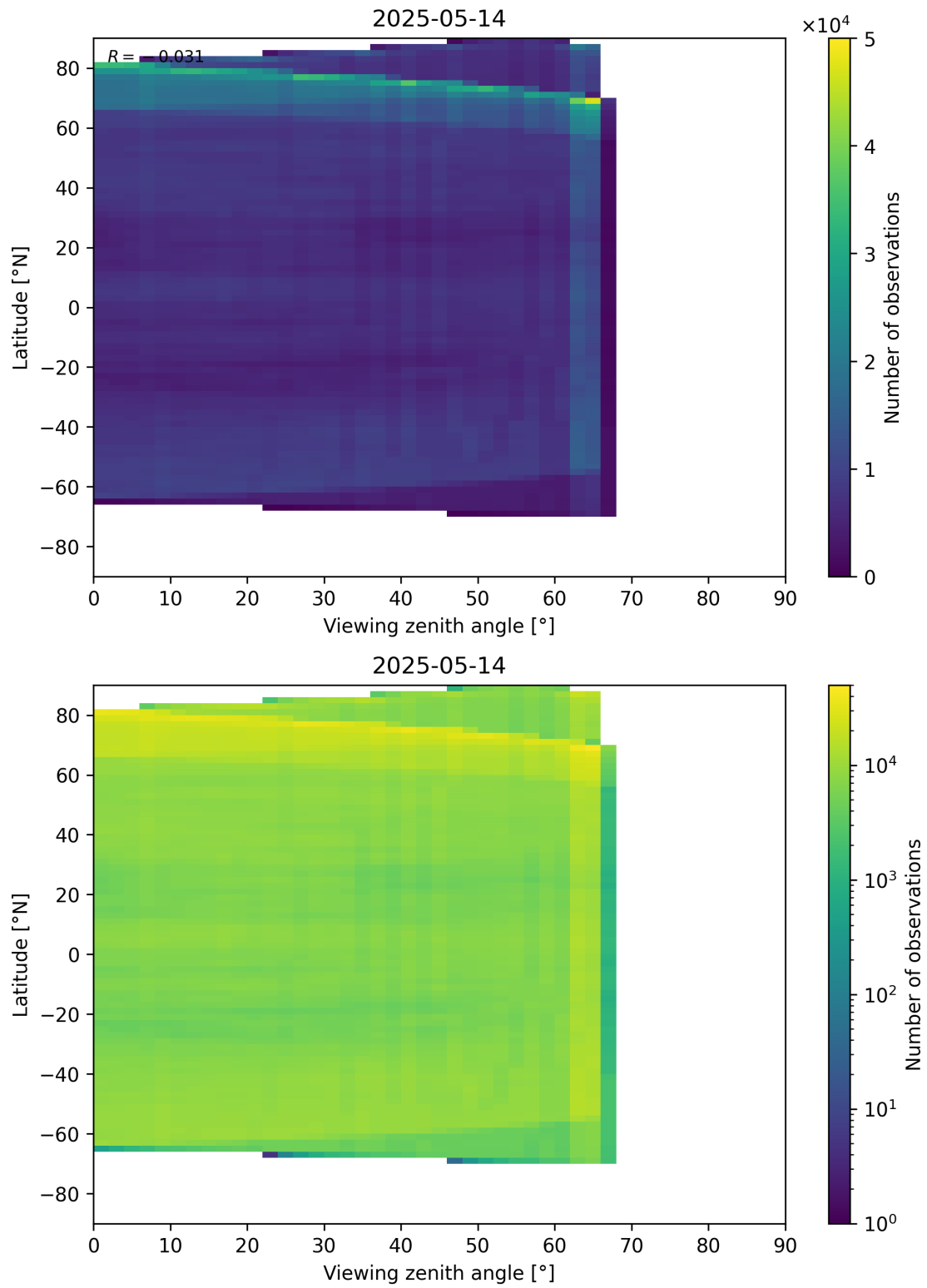
Figure 113: Scatter density plot of “Viewing zenith angle” against “Latitude” for 2025-05-13 to 2025-05-15.
