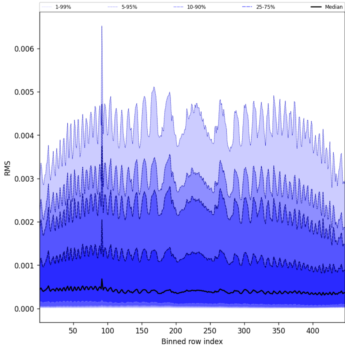
Figure 63: Along track statistics of “RMS” for 2025-05-13 to 2025-05-15
