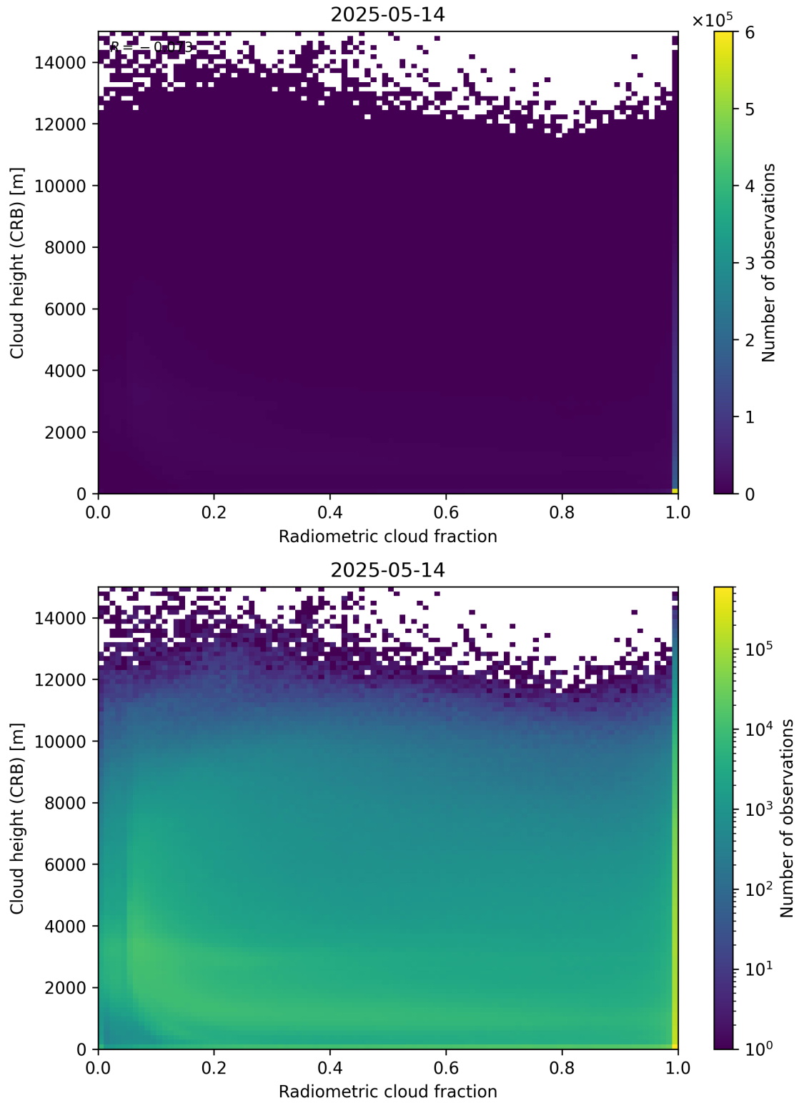
Figure 74: Scatter density plot of “Radiometric cloud fraction” against “Cloud height (CRB)” for 2025-05-13 to 2025-05-15.
