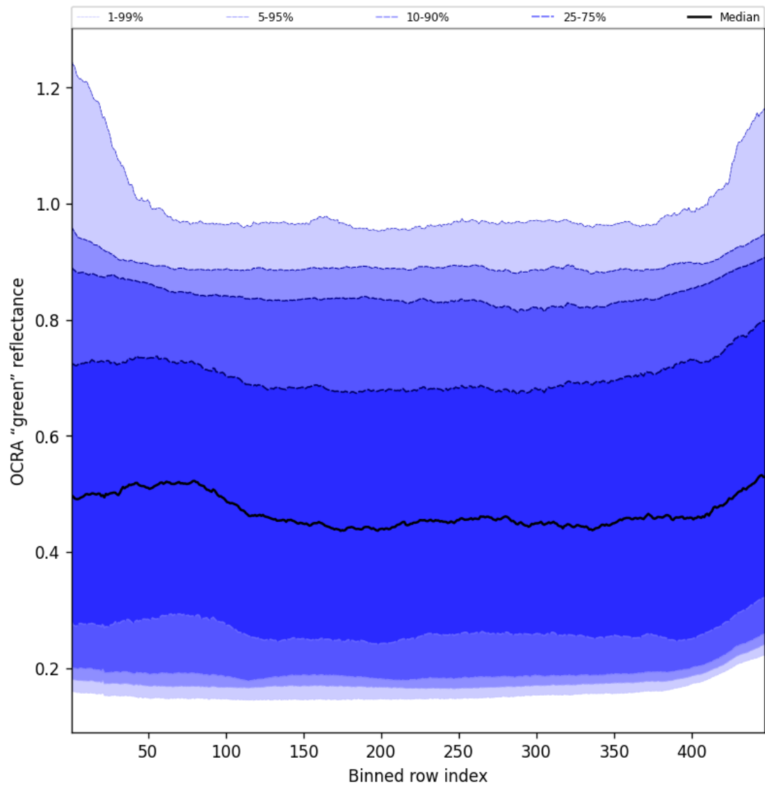
Figure 68: Along track statistics of “OCRA “green” reflectance” for 2025-05-13 to 2025-05-15
