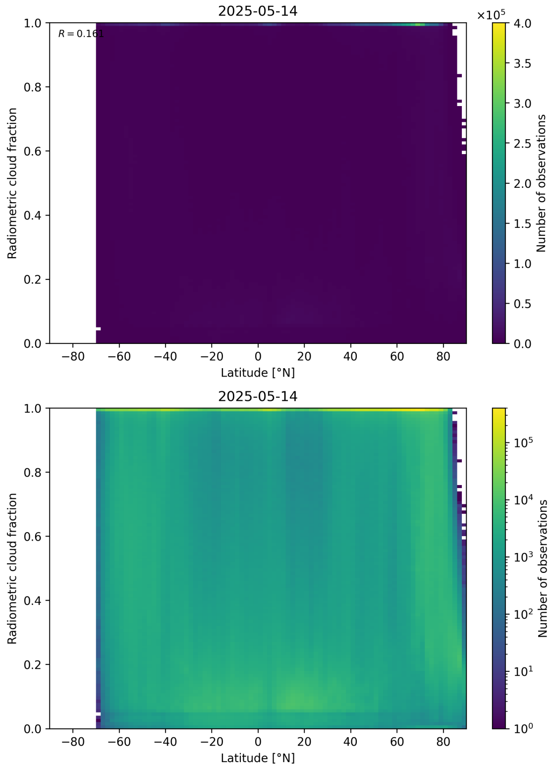
Figure 92: Scatter density plot of “Latitude” against “Radiometric cloud fraction” for 2025-05-13 to 2025-05-15.
