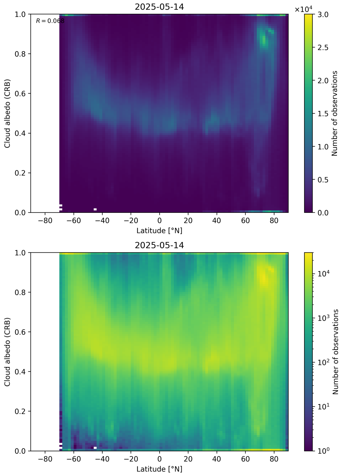
Figure 91: Scatter density plot of “Latitude” against “Cloud albedo (CRB)” for 2025-05-13 to 2025-05-15.
