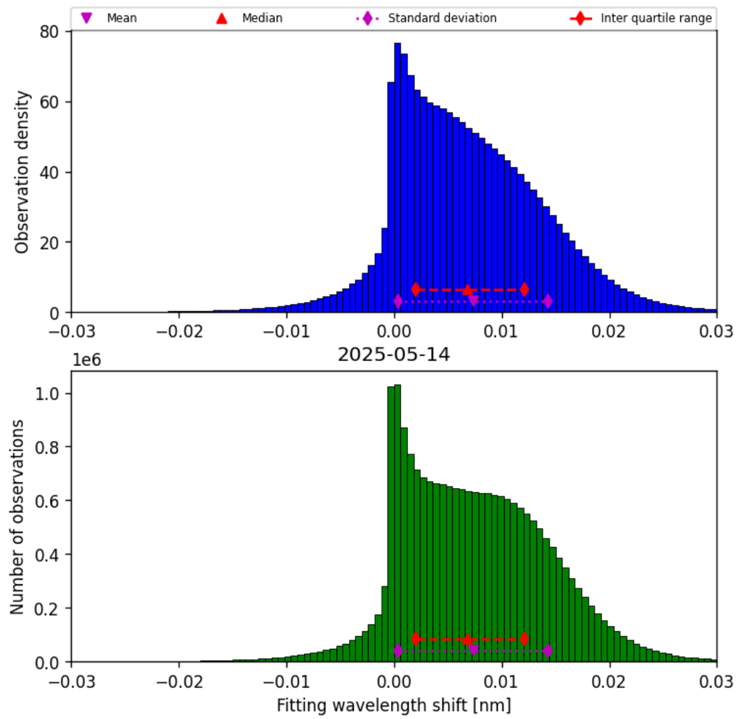
Figure 49: Histogram of “Fitting wavelength shift” for 2025-05-13 to 2025-05-15
