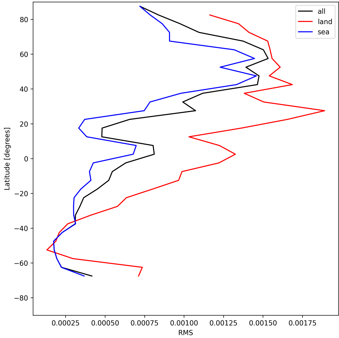
Figure 31: Zonal average of “RMS” for 2025-05-13 to 2025-05-15.
