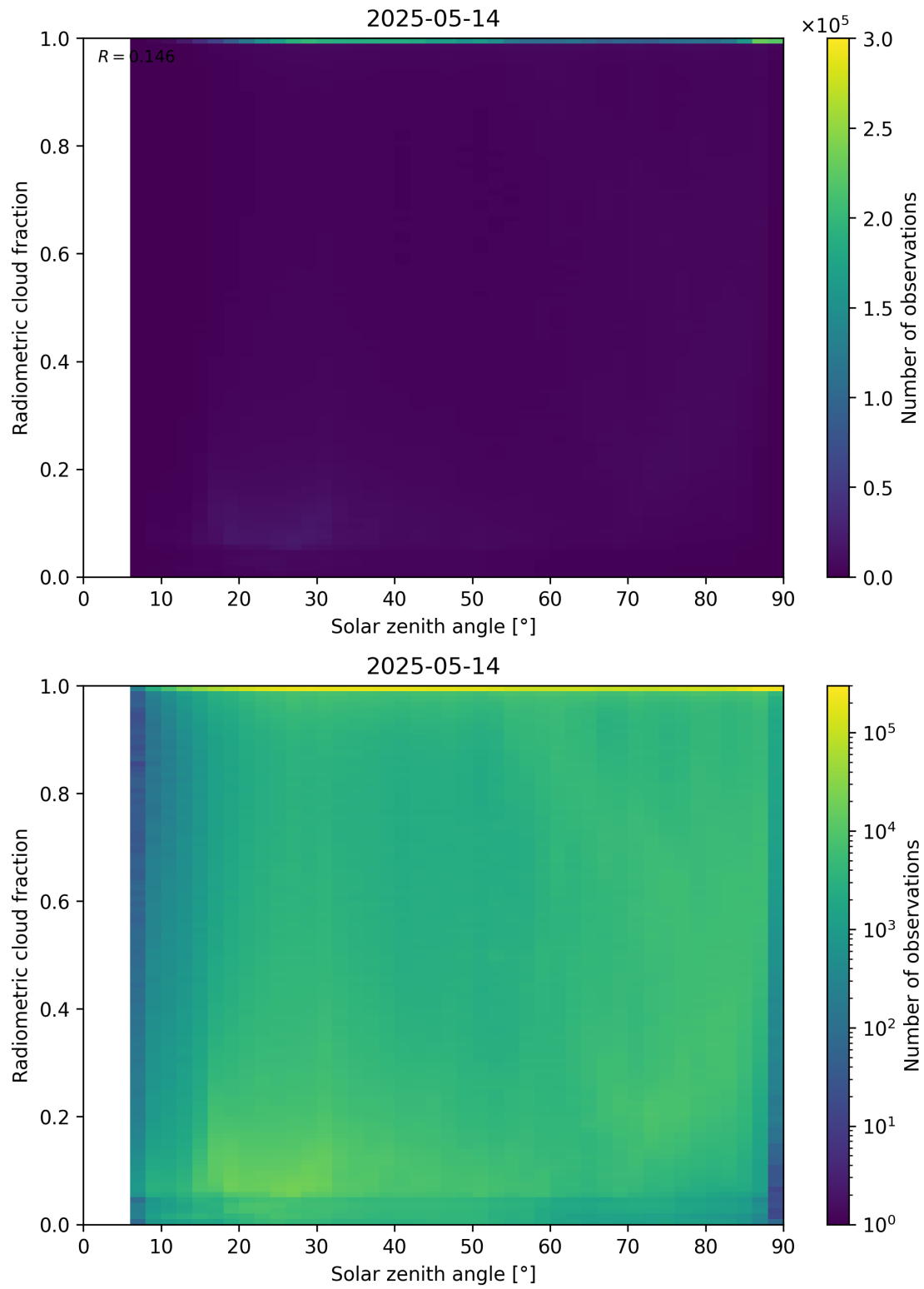
Figure 99: Scatter density plot of “Solar zenith angle” against “Radiometric cloud fraction” for 2025-05-13 to 2025-05-15.
