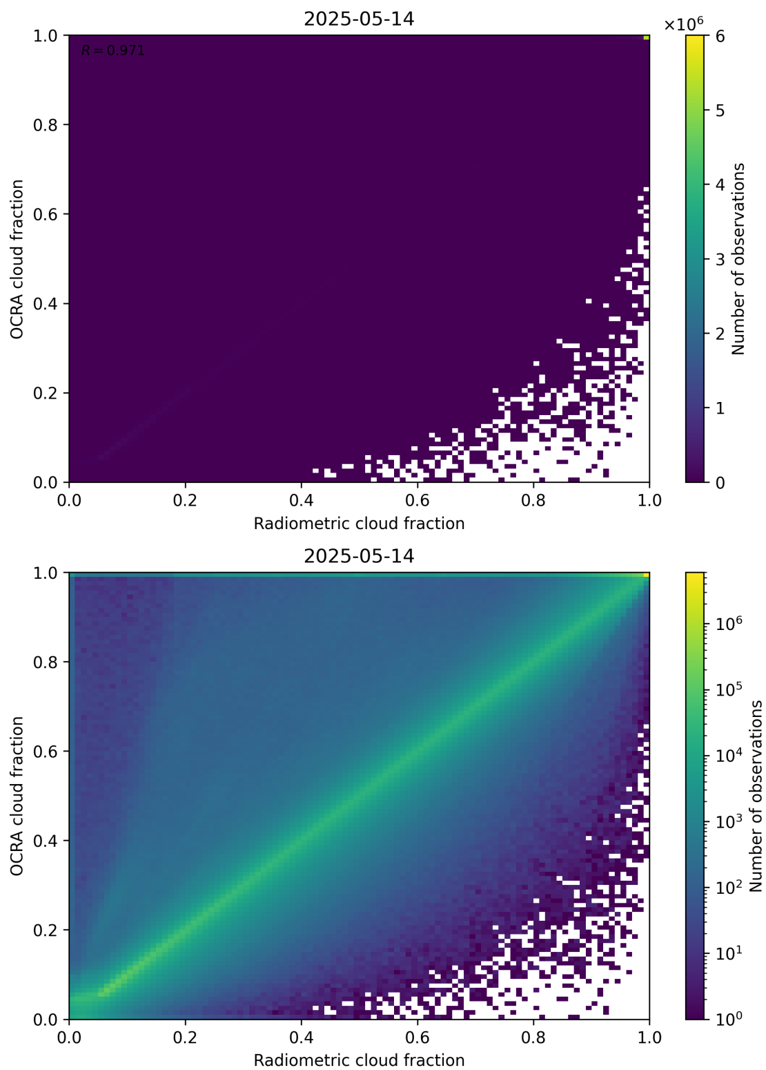
Figure 72: Scatter density plot of “Radiometric cloud fraction” against “OCRA cloud fraction” for 2025-05-13 to 2025-05-15.
