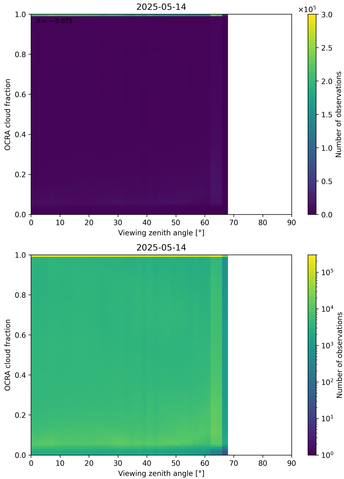
Figure 108: Scatter density plot of “Viewing zenith angle” against “OCRA cloud fraction” for 2025-05-13 to 2025-05-15.
