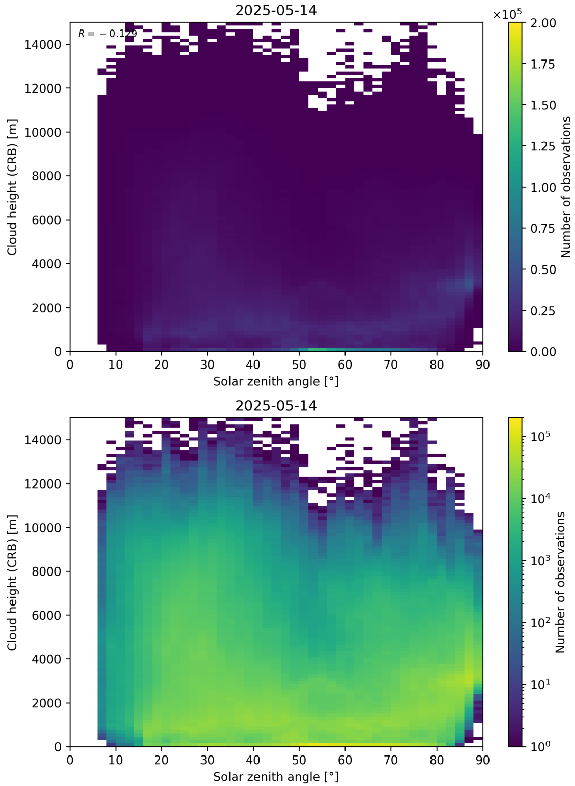
Figure 102: Scatter density plot of “Solar zenith angle” against “Cloud height (CRB)” for 2025-05-13 to 2025-05-15.
