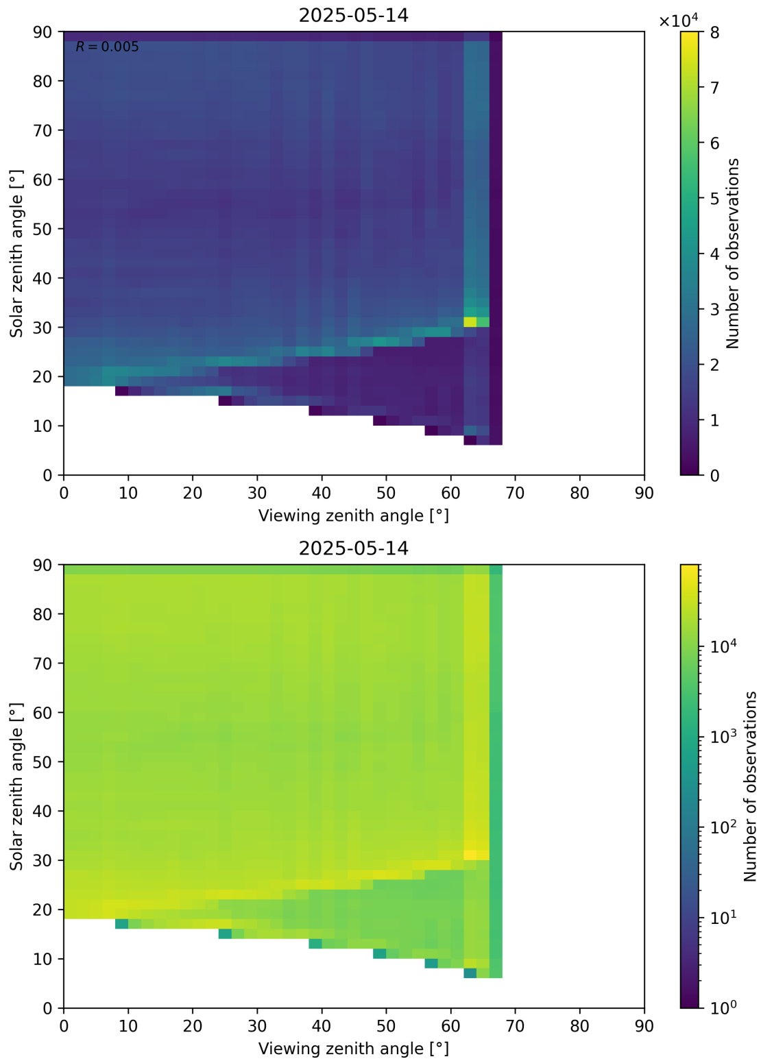
Figure 114: Scatter density plot of “Viewing zenith angle” against “Solar zenith angle” for 2025-05-13 to 2025-05-15.
