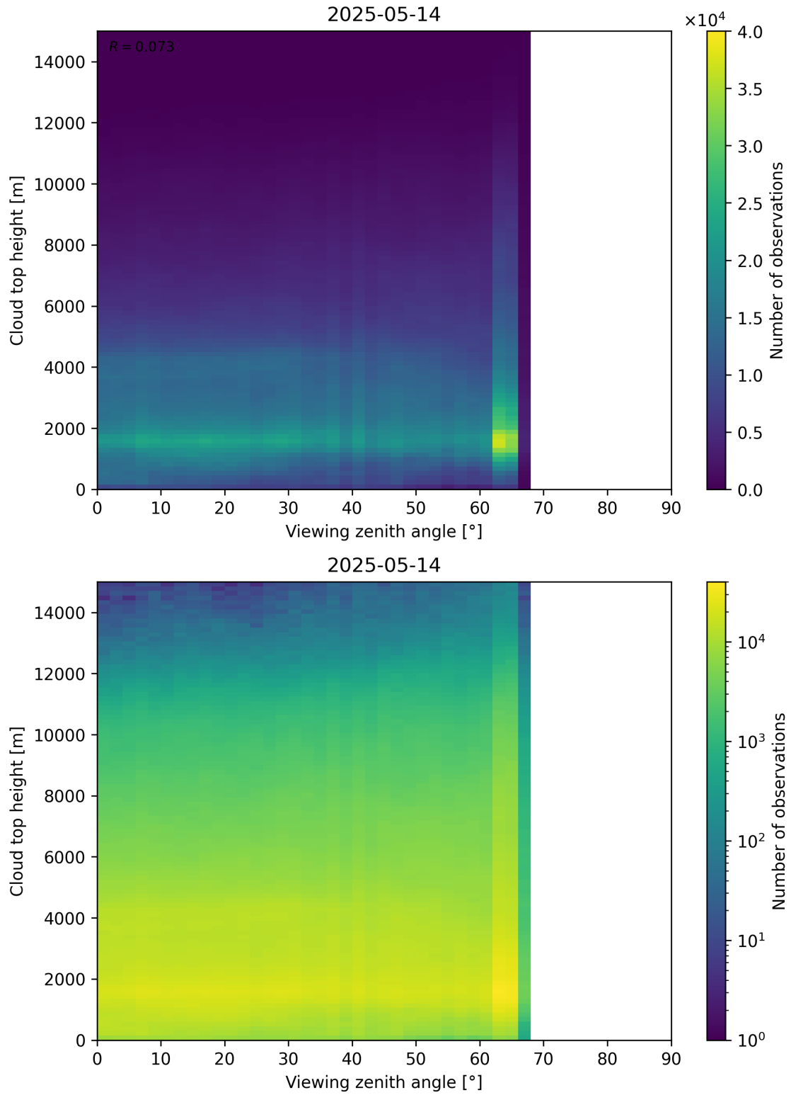
Figure 112: Scatter density plot of “Viewing zenith angle” against “Cloud top height” for 2025-05-13 to 2025-05-15.
