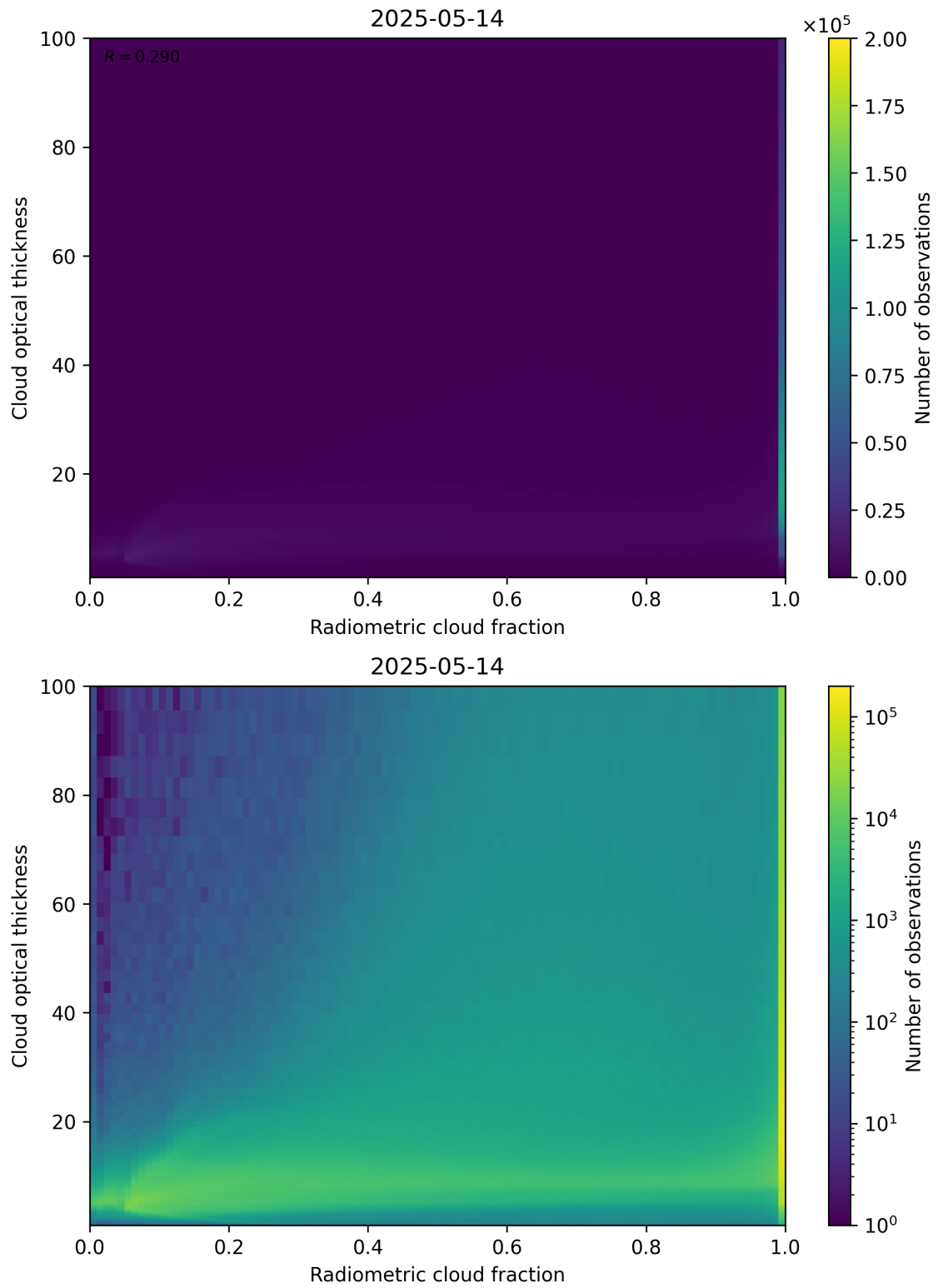
Figure 75: Scatter density plot of “Radiometric cloud fraction” against “Cloud optical thickness” for 2025-05-13 to 2025-05-15.
