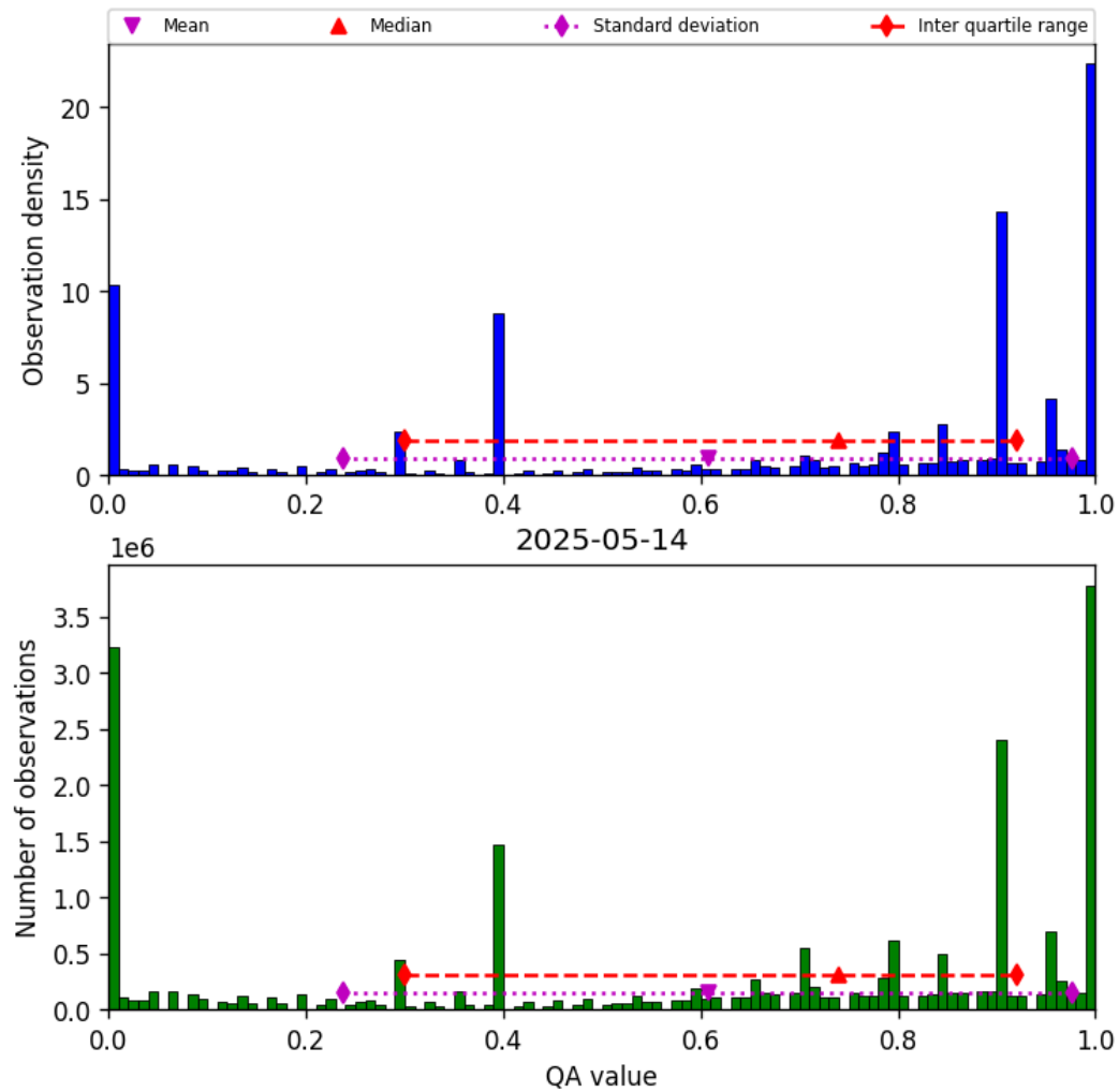
Figure 38: Histogram of “QA value” for 2025-05-13 to 2025-05-15
