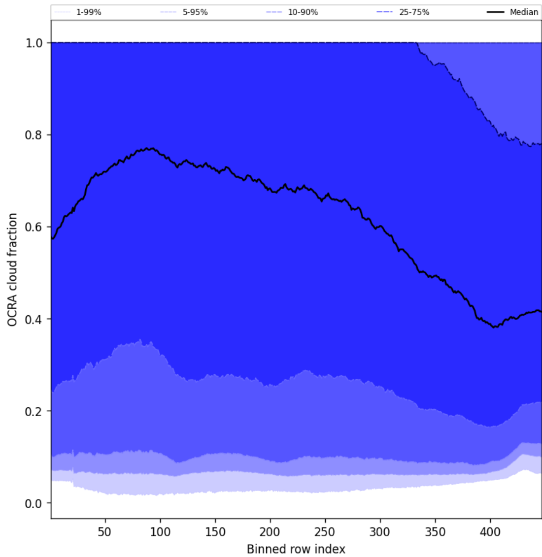
Figure 66: Along track statistics of “OCRA cloud fraction” for 2025-05-13 to 2025-05-15
