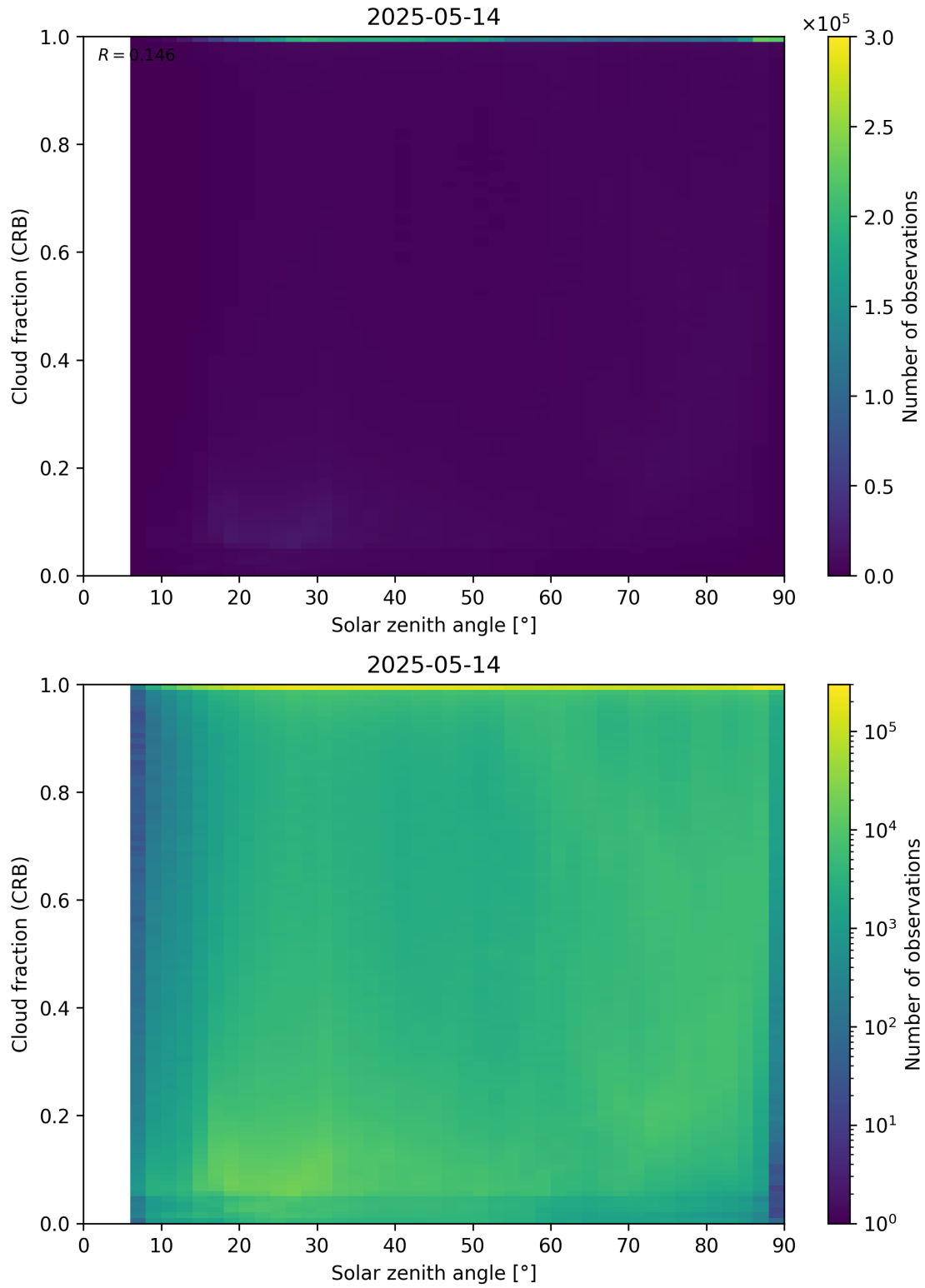
Figure 101: Scatter density plot of “Solar zenith angle” against “Cloud fraction (CRB)” for 2025-05-13 to 2025-05-15.
