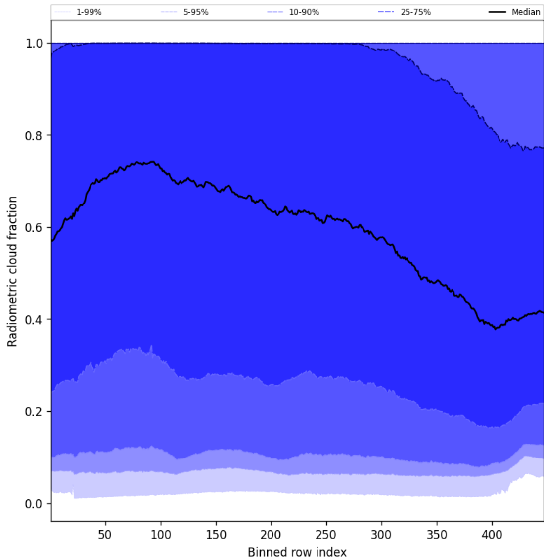
Figure 55: Along track statistics of “Radiometric cloud fraction” for 2025-05-13 to 2025-05-15
