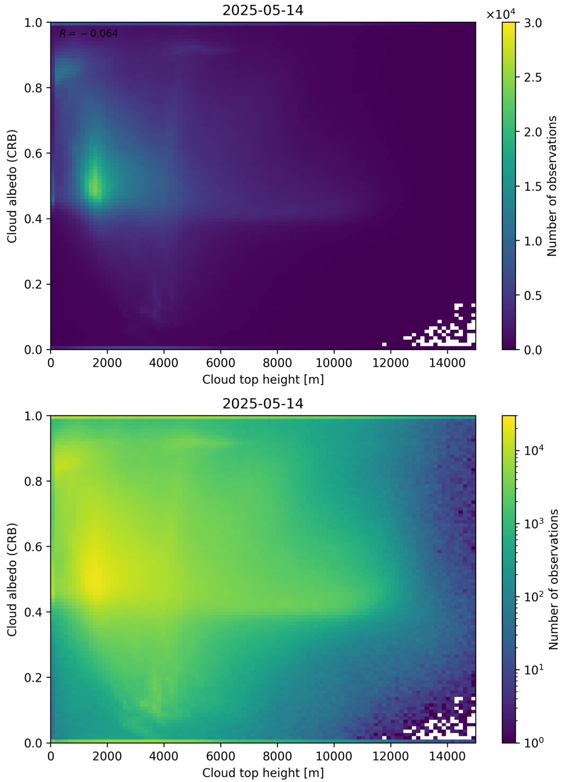
Figure 86: Scatter density plot of “Cloud top height” against “Cloud albedo (CRB)” for 2025-05-13 to 2025-05-15.
