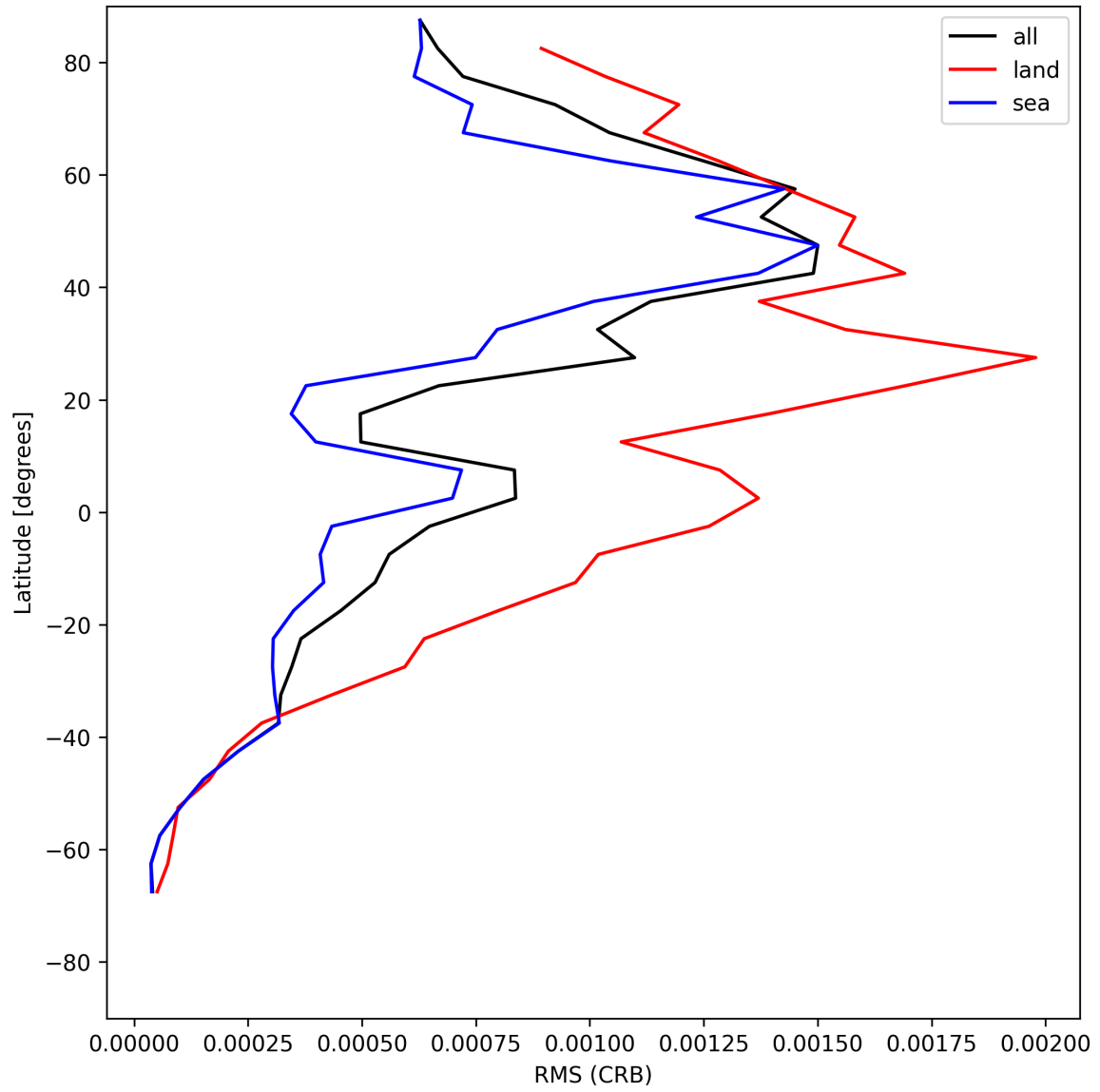
Figure 32: Zonal average of “RMS (CRB)” for 2025-05-13 to 2025-05-15.
