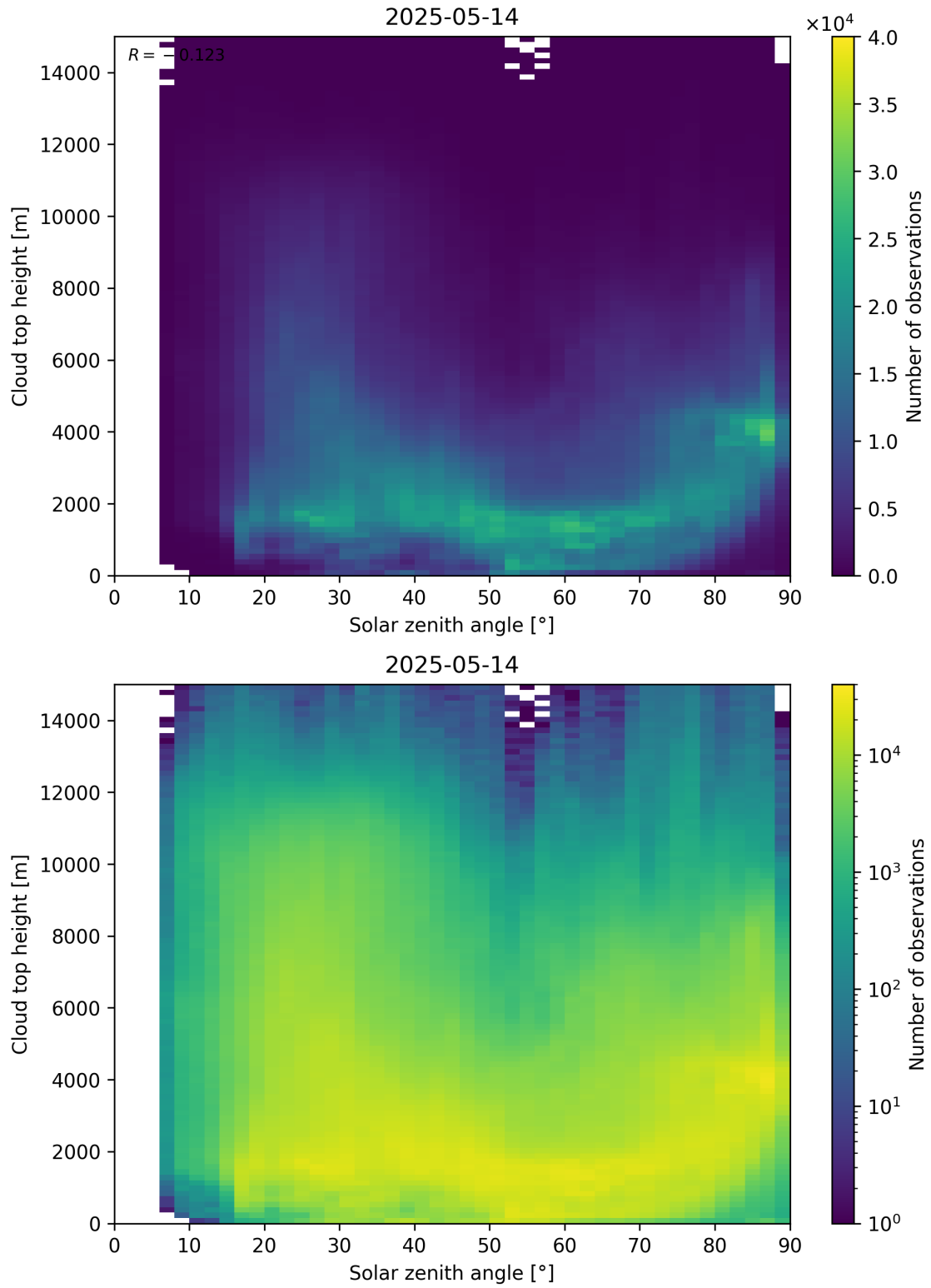
Figure 104: Scatter density plot of “Solar zenith angle” against “Cloud top height” for 2025-05-13 to 2025-05-15.
