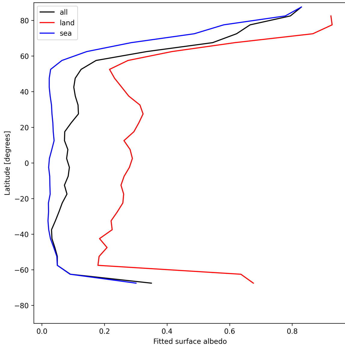
Figure 29: Zonal average of “Fitted surface albedo” for 2025-05-13 to 2025-05-15.
