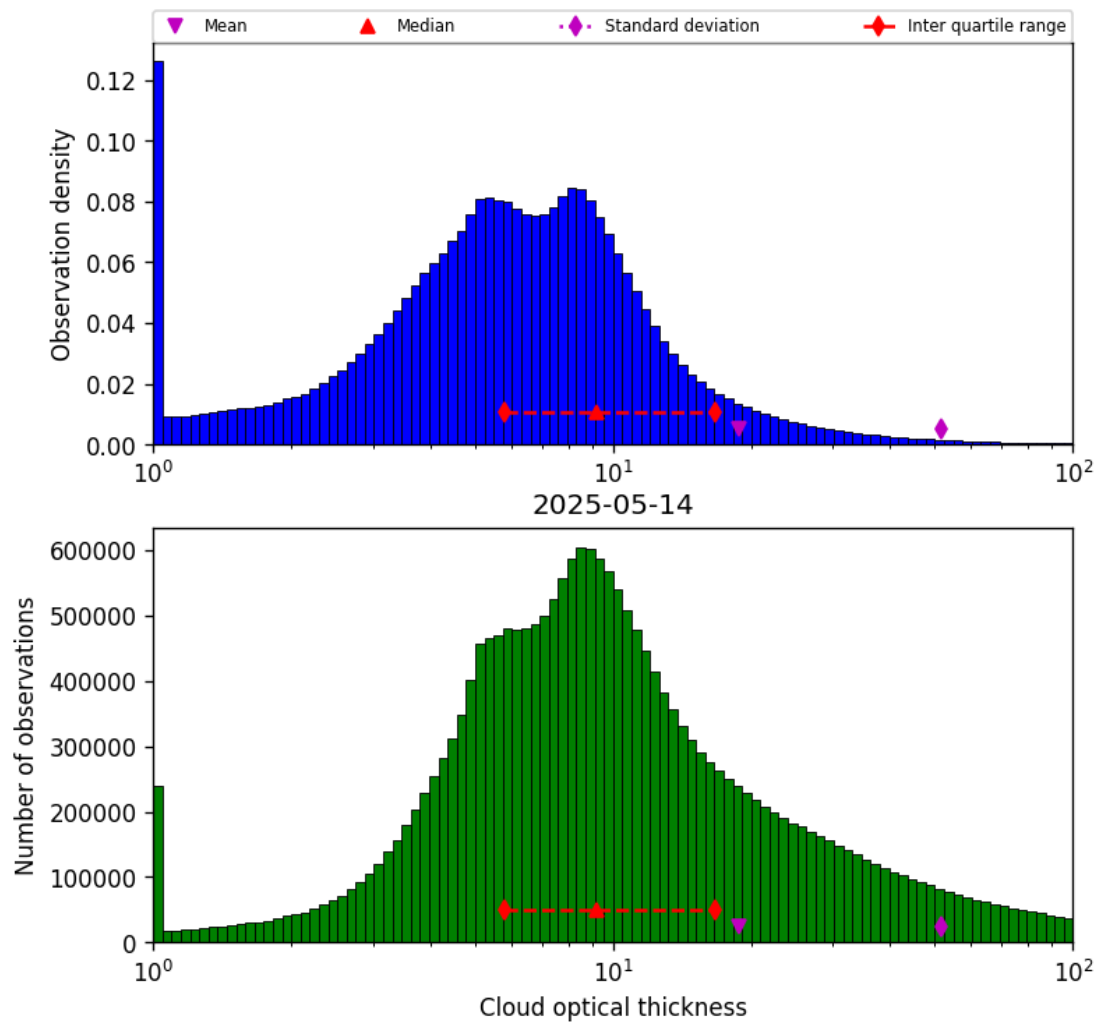
Figure 41: Histogram of “Cloud optical thickness” for 2025-05-13 to 2025-05-15
