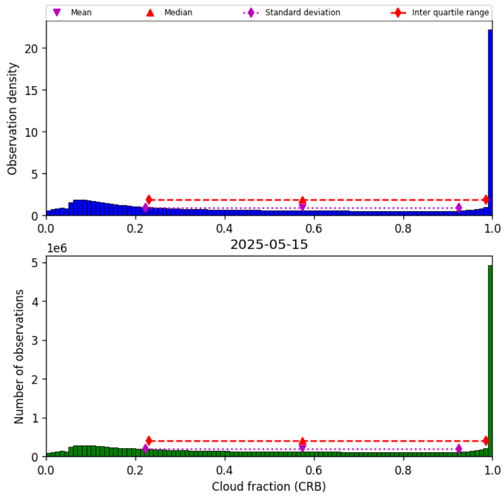
Figure 42: Histogram of “Cloud fraction (CRB)” for 2025-05-15 to 2025-05-16
