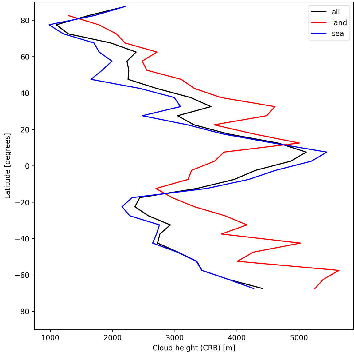
Figure 27: Zonal average of “Cloud height (CRB)” for 2025-05-15 to 2025-05-16.
