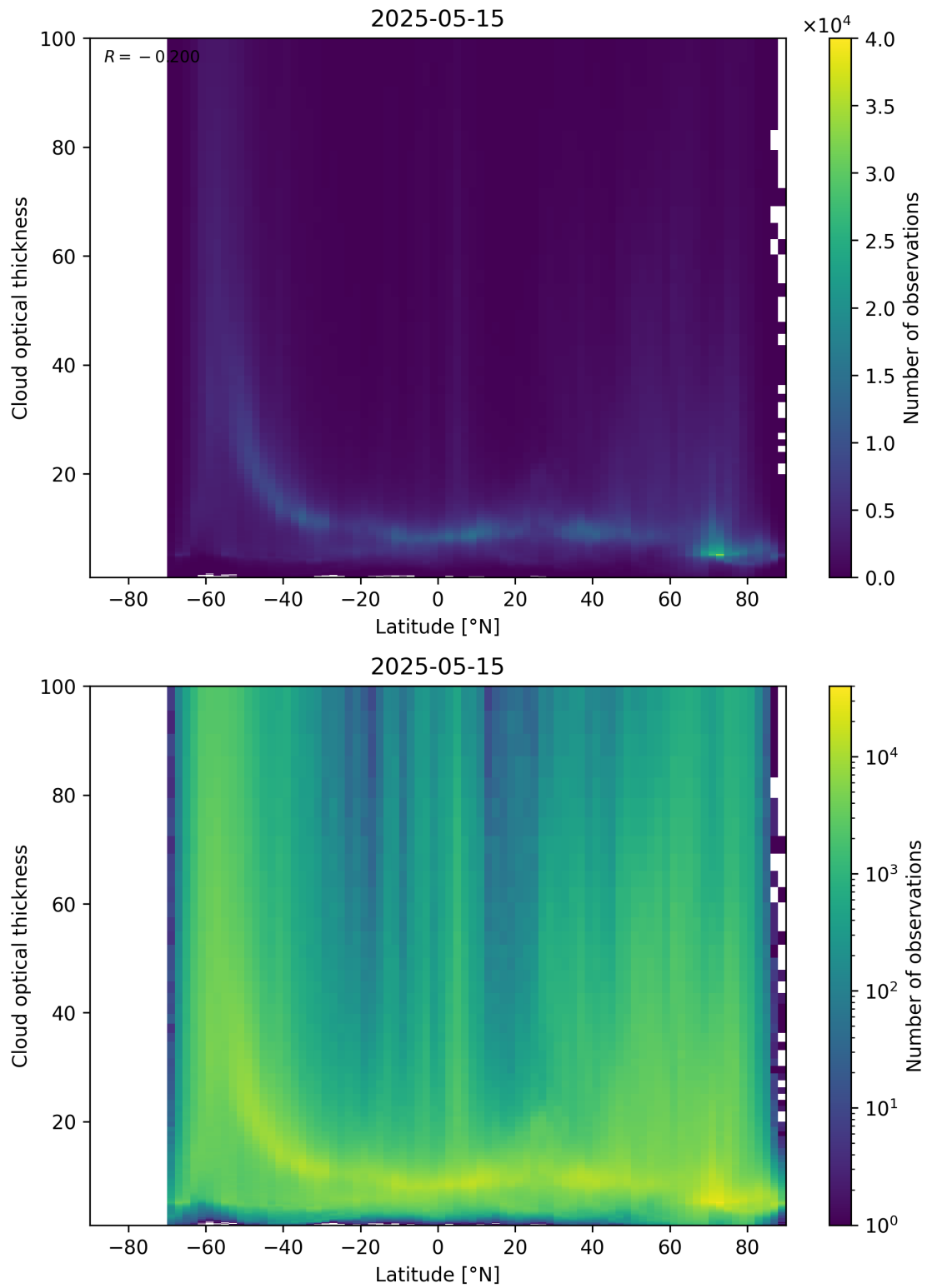
Figure 96: Scatter density plot of “Latitude” against “Cloud optical thickness” for 2025-05-15 to 2025-05-16.
