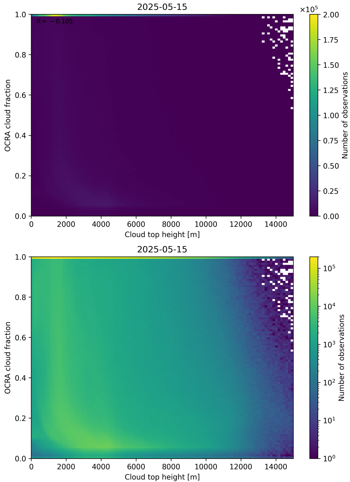
Figure 87: Scatter density plot of “Cloud top height” against “OCRA cloud fraction” for 2025-05-15 to 2025-05-16.
