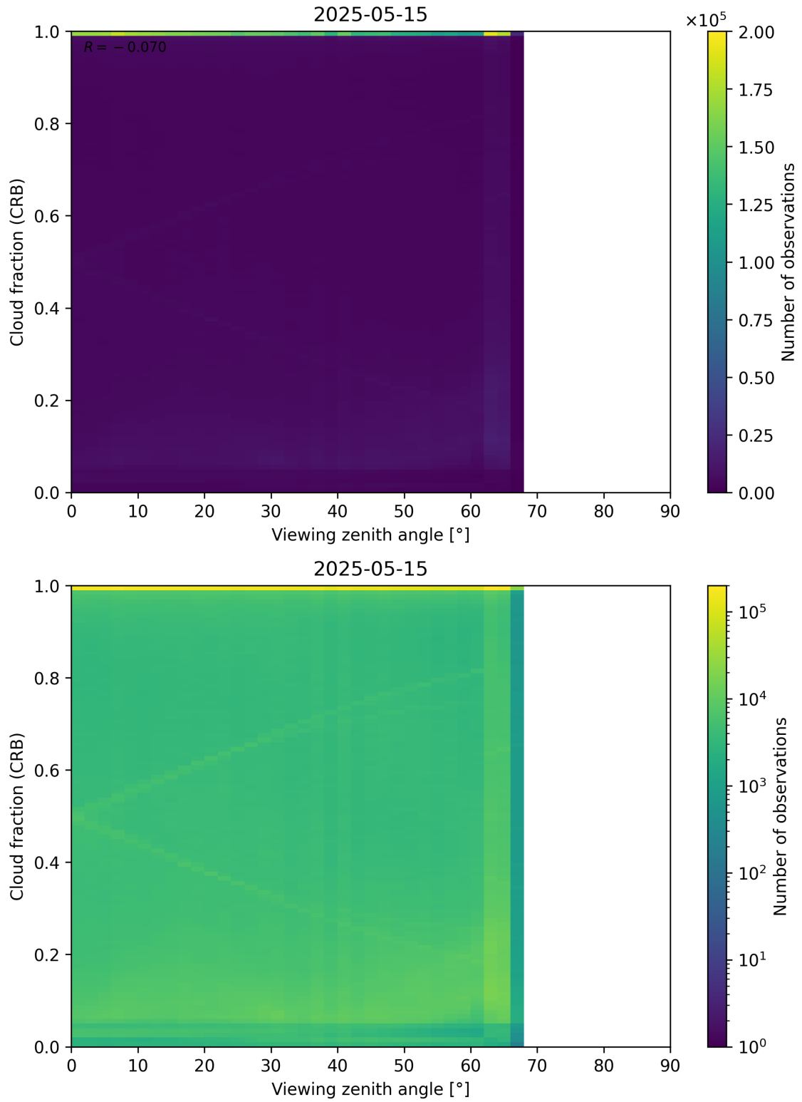
Figure 109: Scatter density plot of “Viewing zenith angle” against “Cloud fraction (CRB)” for 2025-05-15 to 2025-05-16.
