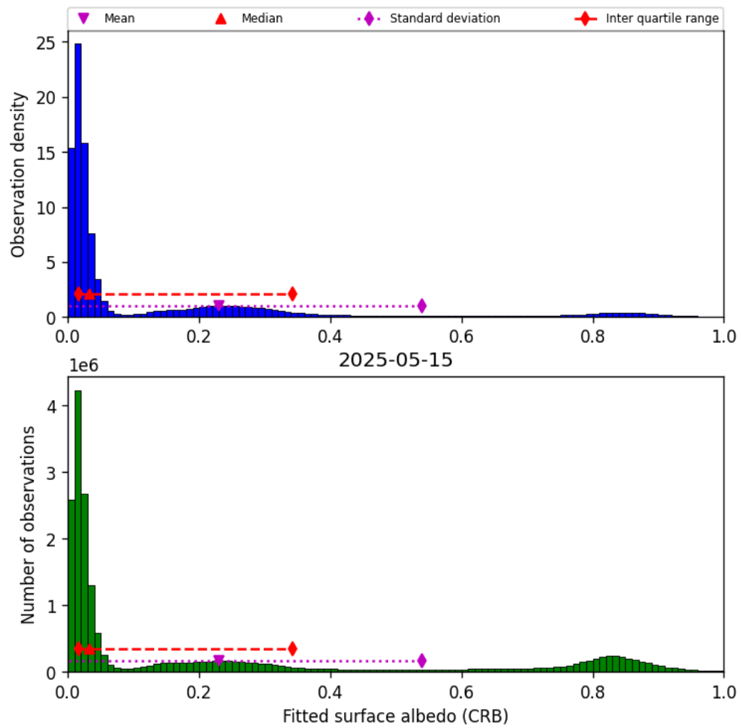
Figure 46: Histogram of “Fitted surface albedo (CRB)” for 2025-05-15 to 2025-05-16
