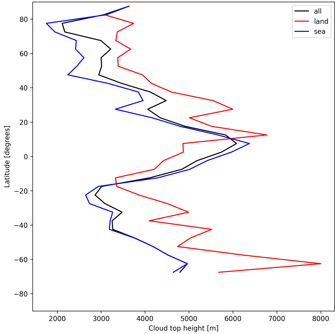
Figure 24: Zonal average of “Cloud top height” for 2025-05-15 to 2025-05-16.
