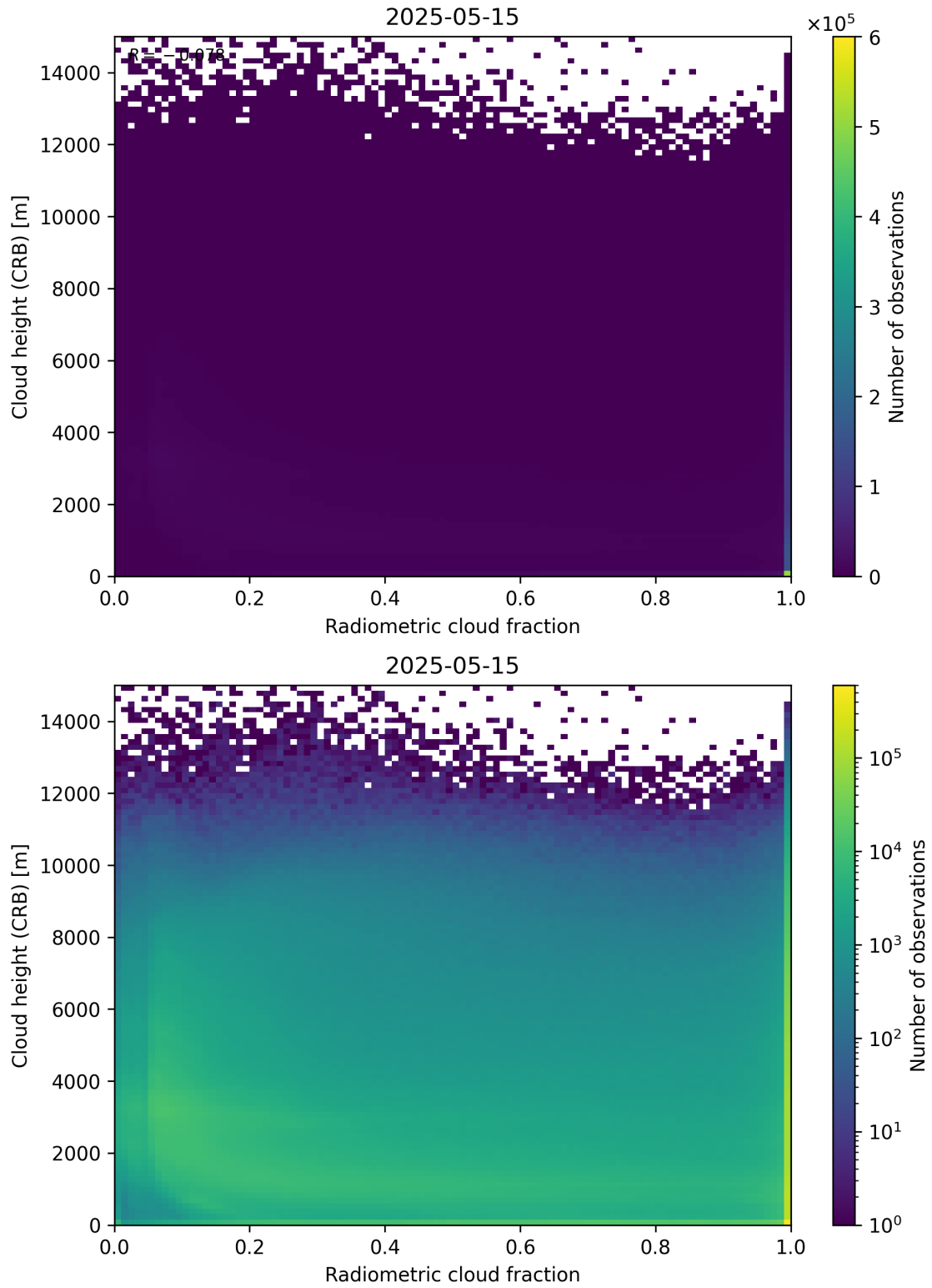
Figure 74: Scatter density plot of “Radiometric cloud fraction” against “Cloud height (CRB)” for 2025-05-15 to 2025-05-16.
