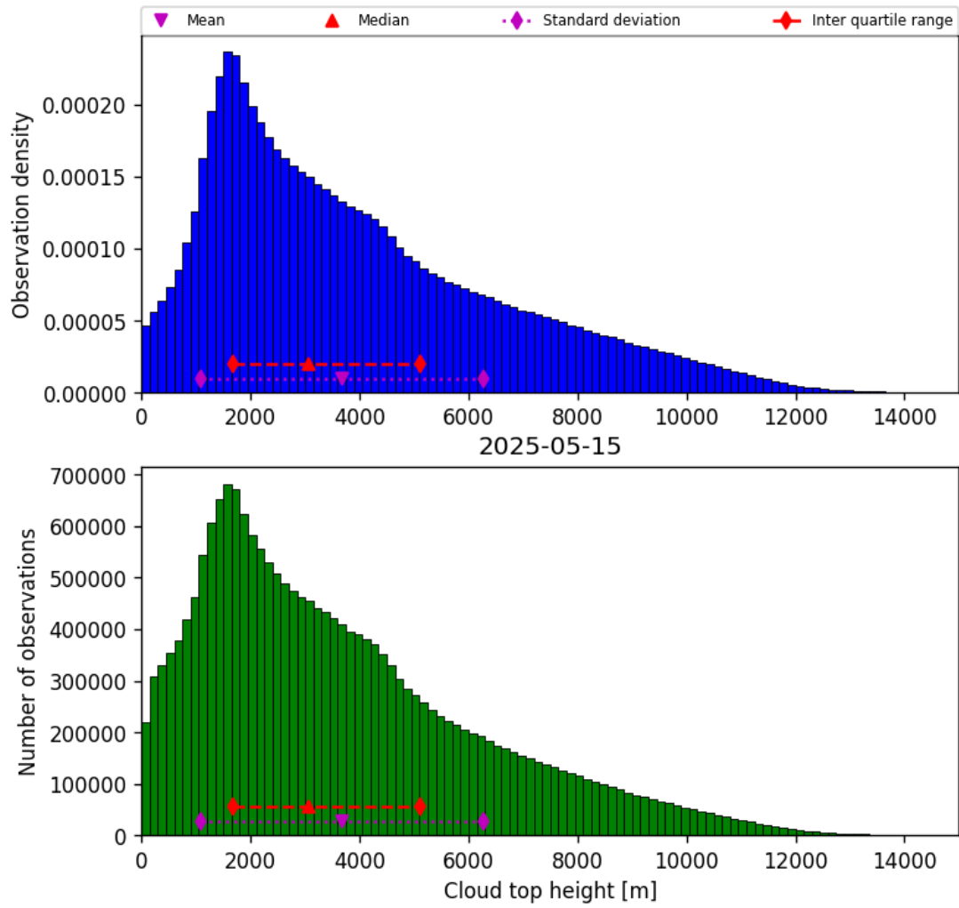
Figure 40: Histogram of “Cloud top height” for 2025-05-15 to 2025-05-16
