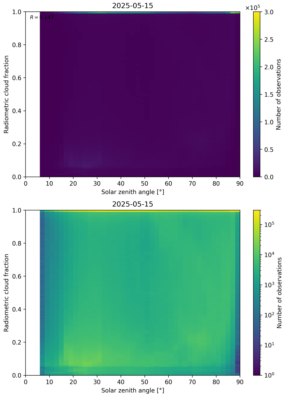
Figure 99: Scatter density plot of “Solar zenith angle” against “Radiometric cloud fraction” for 2025-05-15 to 2025-05-16.
