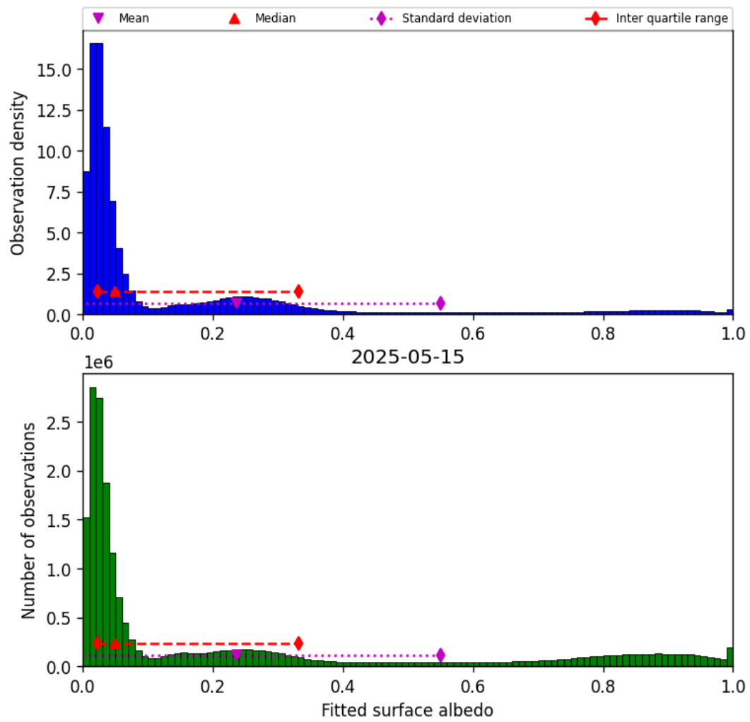
Figure 45: Histogram of “Fitted surface albedo” for 2025-05-15 to 2025-05-16
