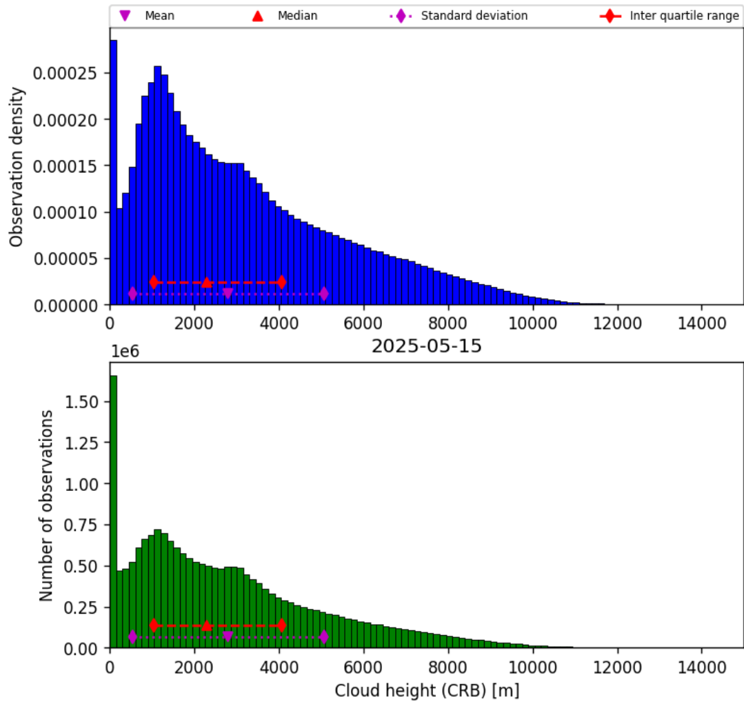
Figure 43: Histogram of “Cloud height (CRB)” for 2025-05-15 to 2025-05-16
