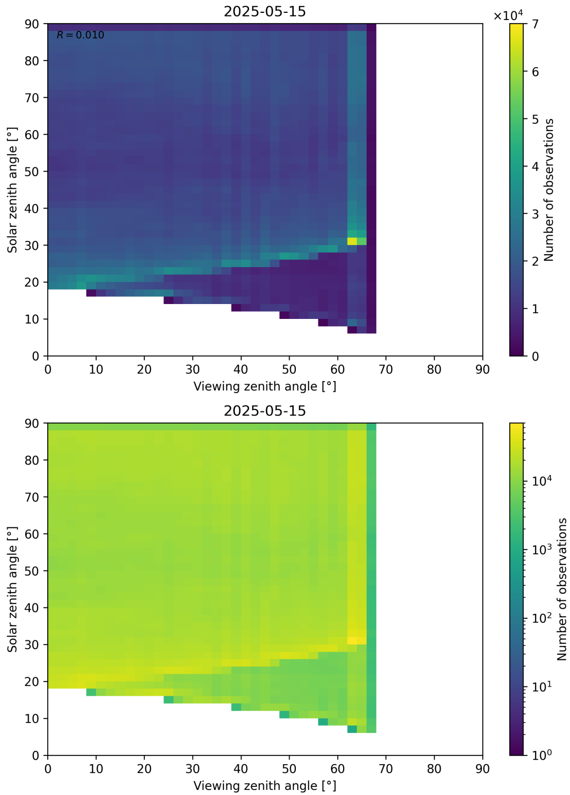
Figure 114: Scatter density plot of “Viewing zenith angle” against “Solar zenith angle” for 2025-05-15 to 2025-05-16.
