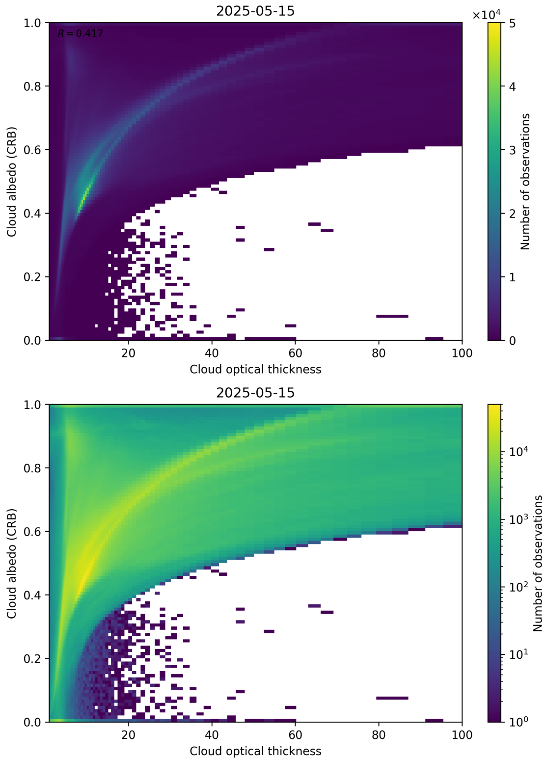
Figure 82: Scatter density plot of “Cloud optical thickness” against “Cloud albedo (CRB)” for 2025-05-15 to 2025-05-16.
