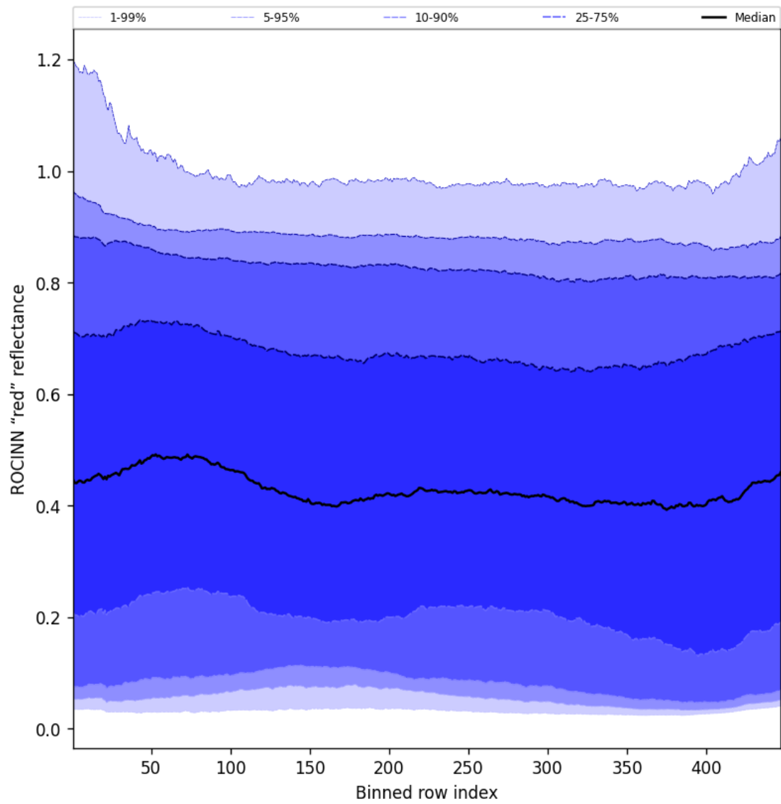
Figure 69: Along track statistics of "ROCINN "red" reflectance" for 2025-05-15 to 2025-05-16
