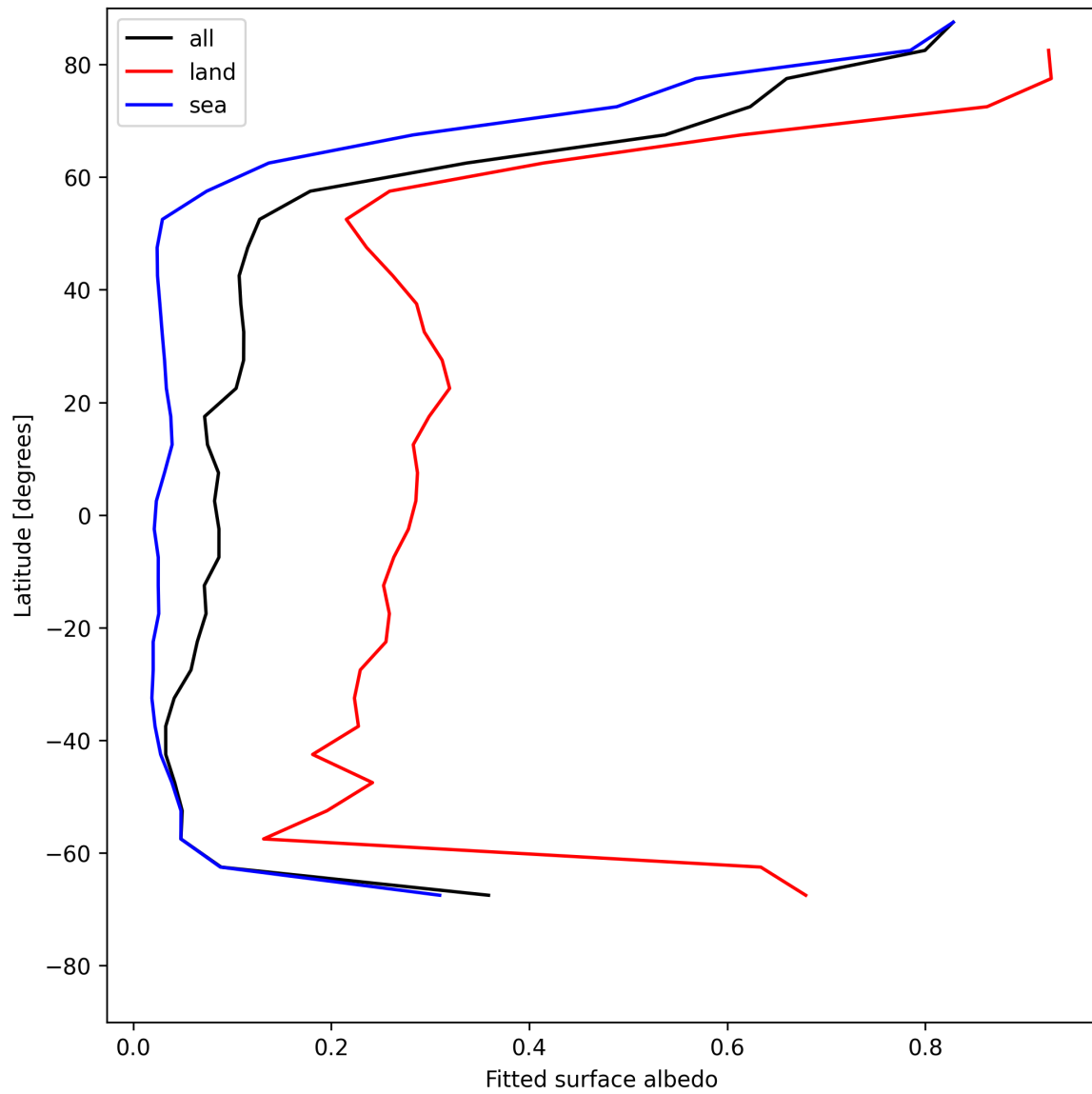
Figure 29: Zonal average of “Fitted surface albedo” for 2025-05-15 to 2025-05-16.
