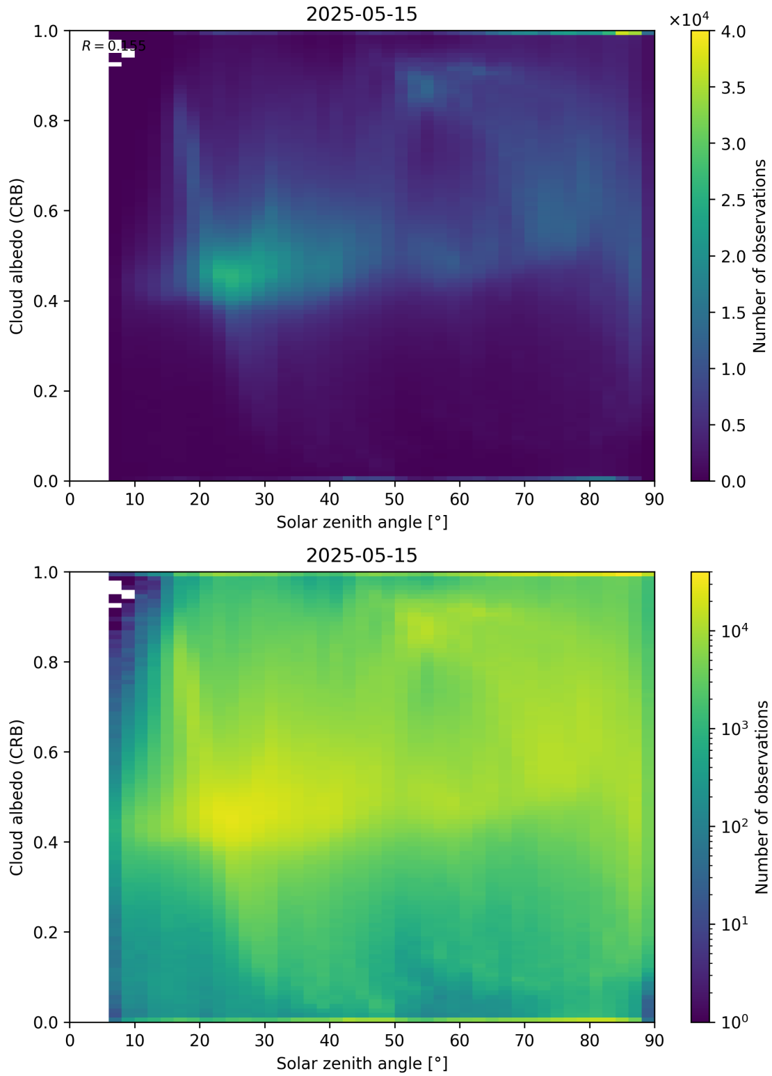
Figure 98: Scatter density plot of “Solar zenith angle” against “Cloud albedo (CRB)” for 2025-05-15 to 2025-05-16.
