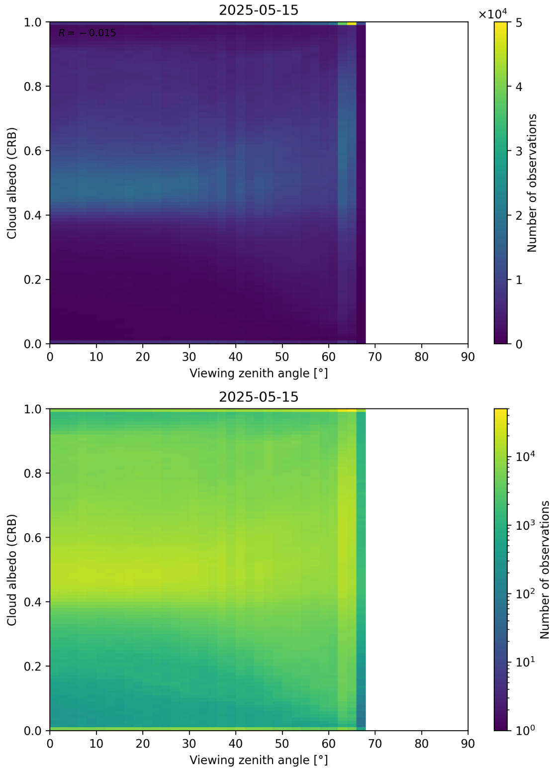
Figure 106: Scatter density plot of “Viewing zenith angle” against “Cloud albedo (CRB)” for 2025-05-15 to 2025-05-16.
