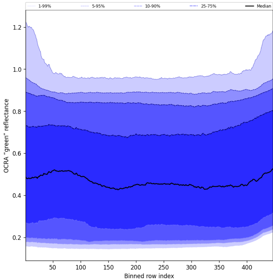
Figure 68: Along track statistics of "OCRA "green" reflectance" for 2025-05-15 to 2025-05-16
