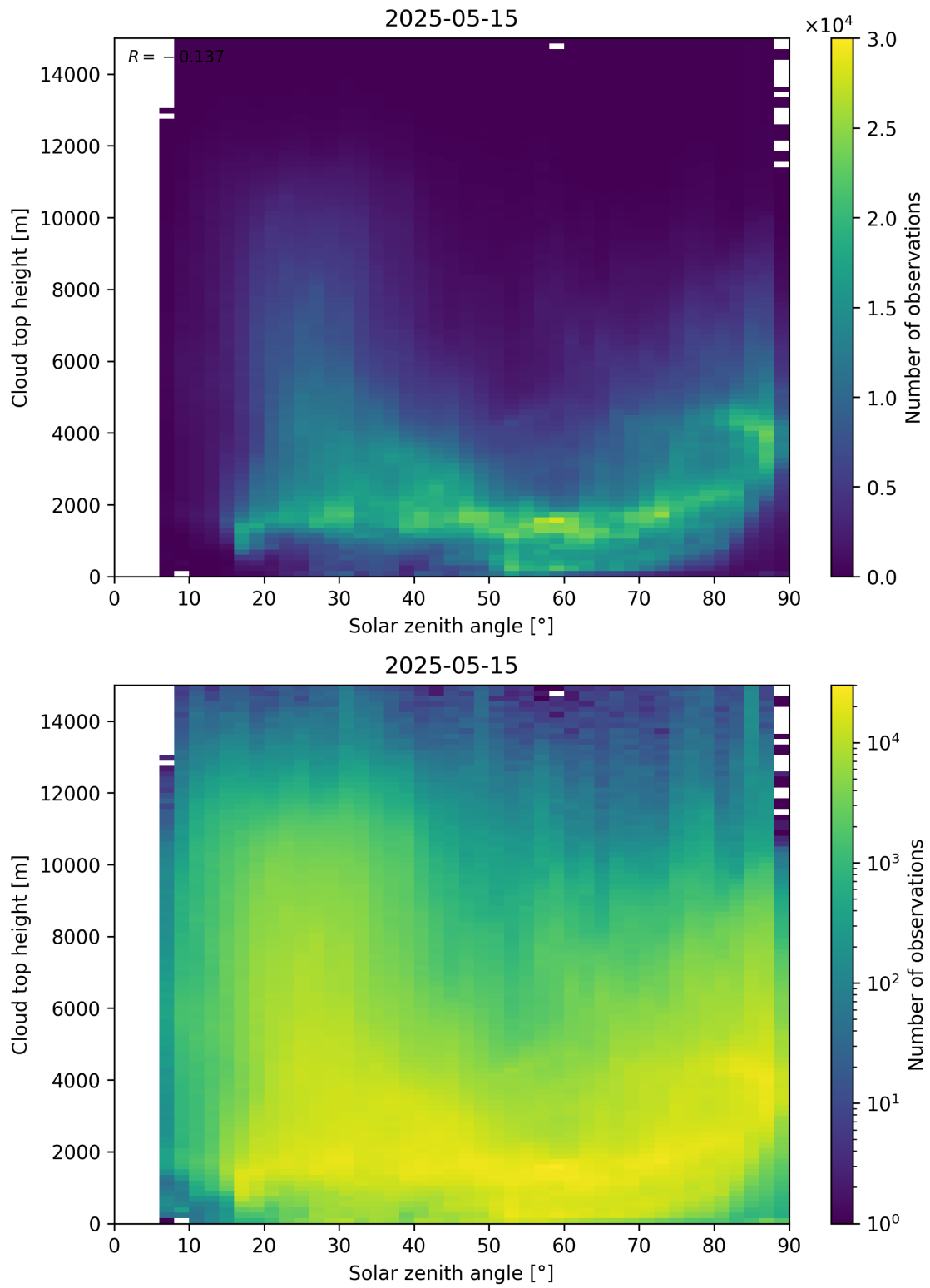
Figure 104: Scatter density plot of “Solar zenith angle” against “Cloud top height” for 2025-05-15 to 2025-05-16.
