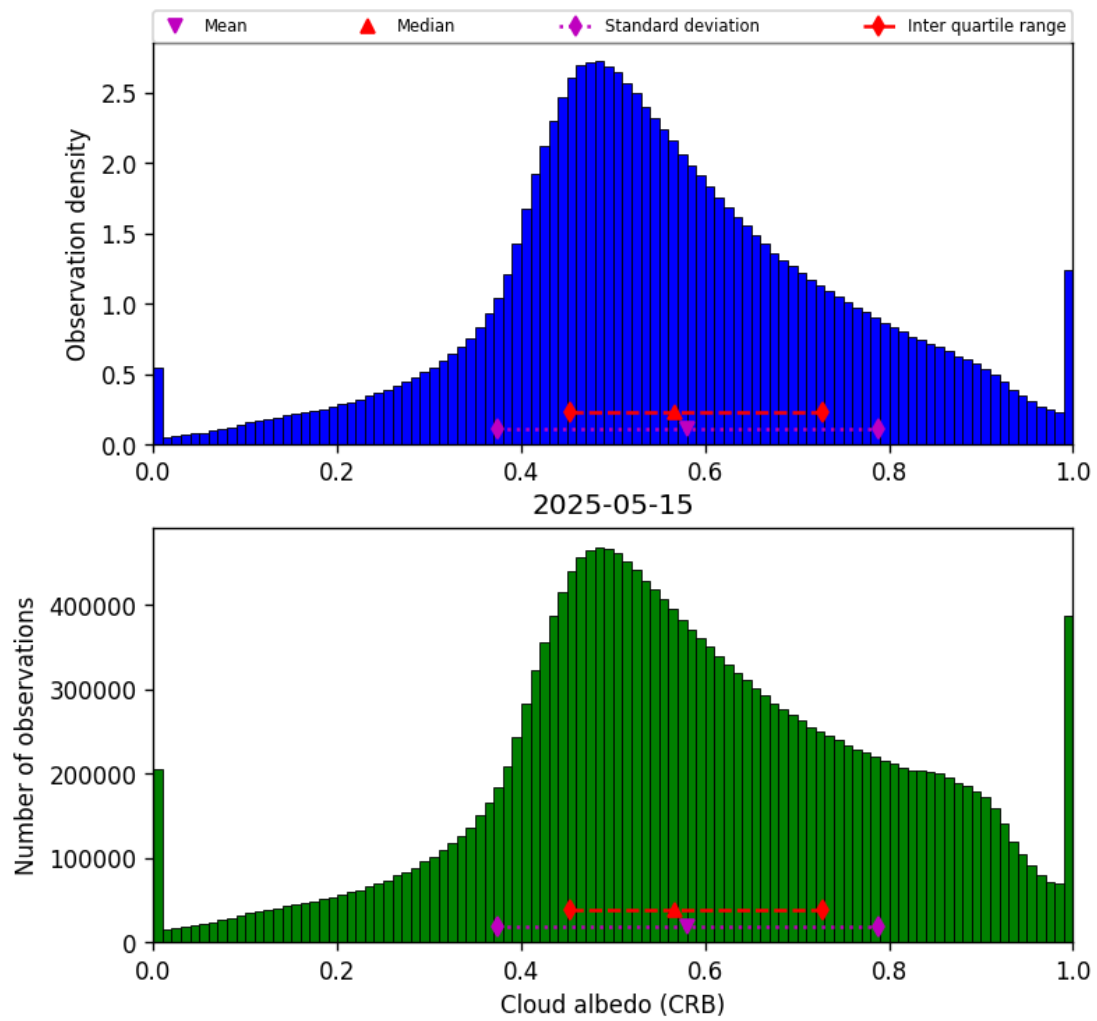
Figure 44: Histogram of “Cloud albedo (CRB)” for 2025-05-15 to 2025-05-16
