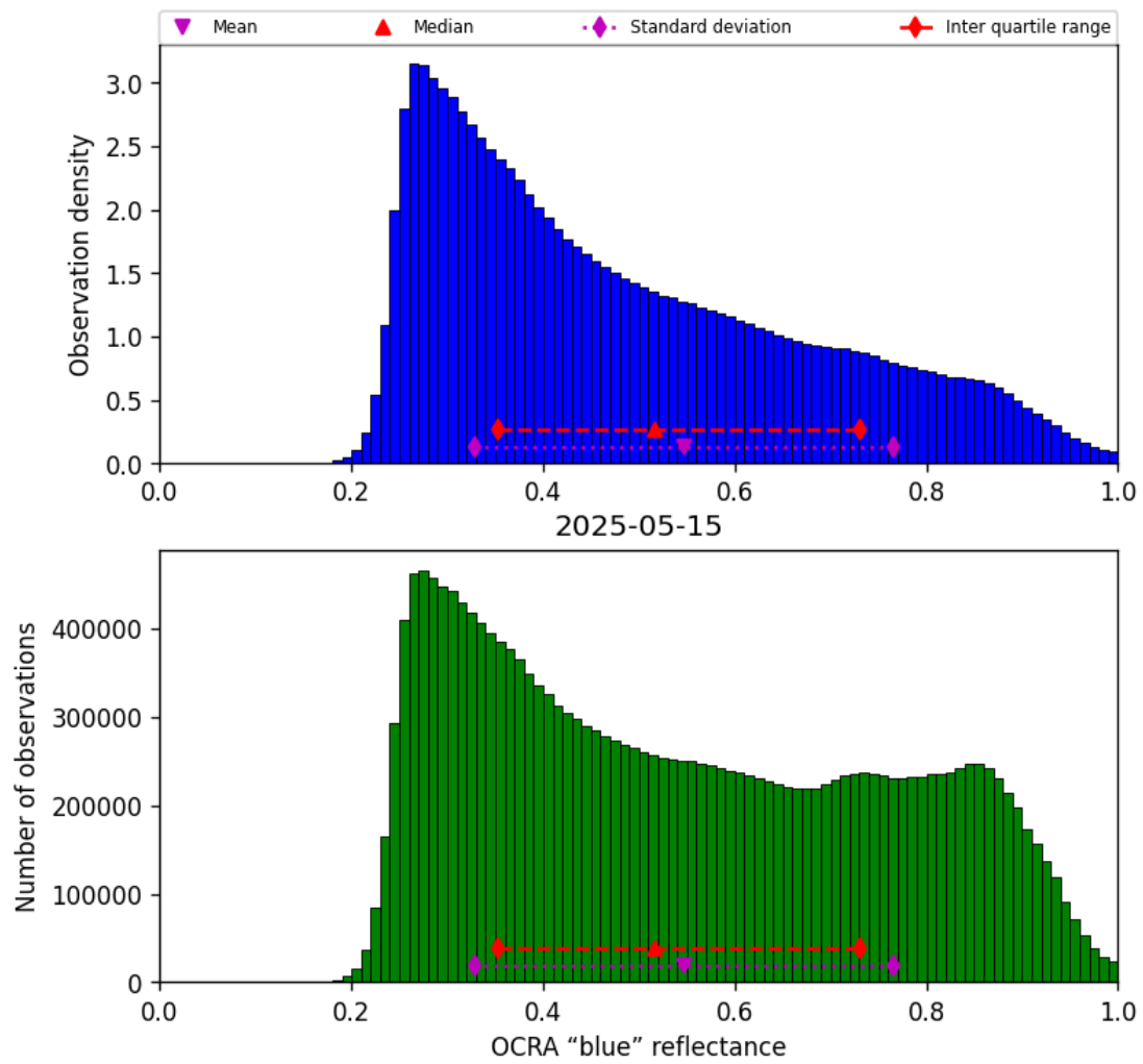
Figure 51: Histogram of “OCRA “blue” reflectance” for 2025-05-15 to 2025-05-16
