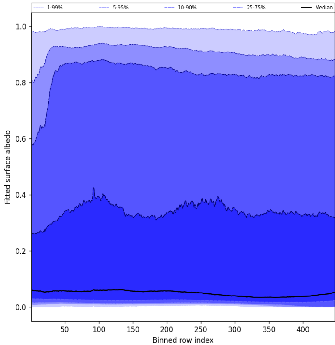
Figure 61: Along track statistics of “Fitted surface albedo” for 2025-05-15 to 2025-05-16
