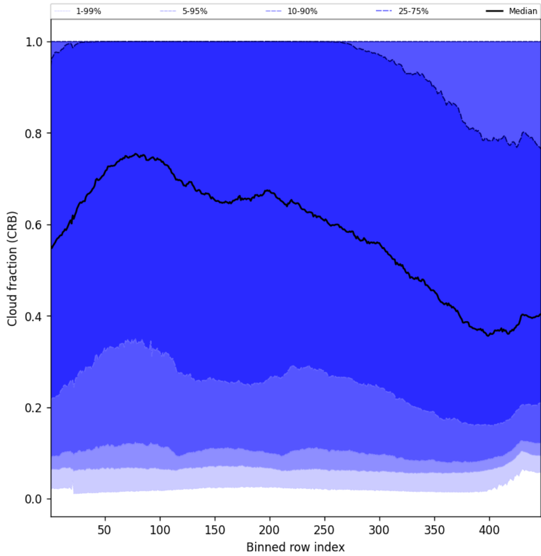
Figure 58: Along track statistics of “Cloud fraction (CRB)” for 2025-05-15 to 2025-05-16
