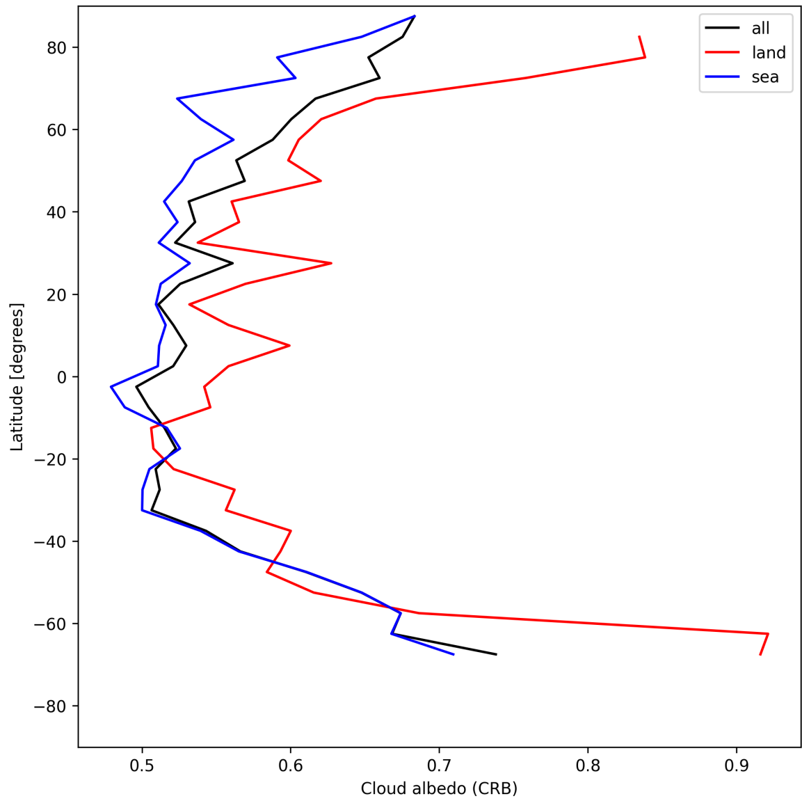
Figure 28: Zonal average of “Cloud albedo (CRB)” for 2025-05-15 to 2025-05-16.
