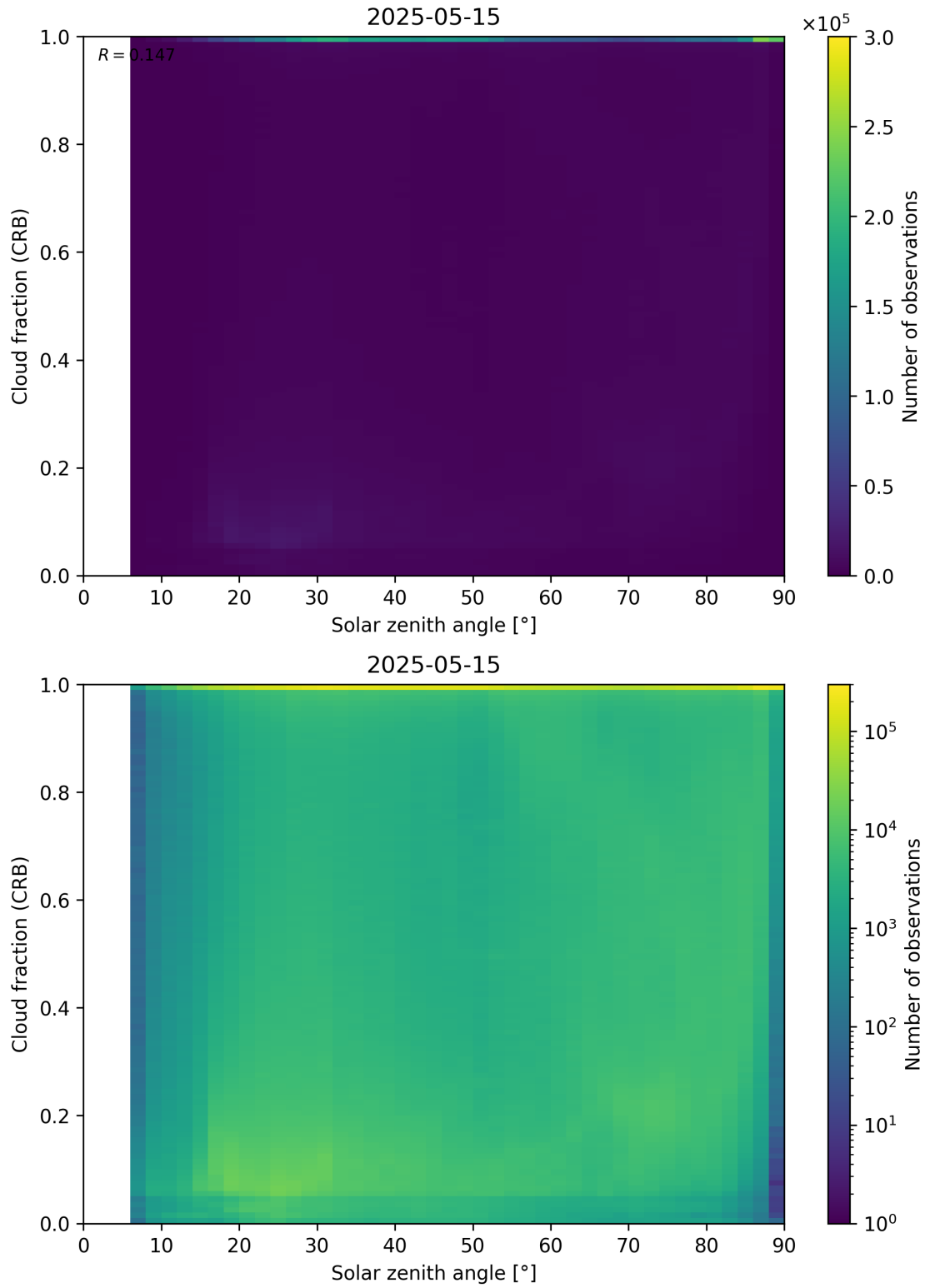
Figure 101: Scatter density plot of “Solar zenith angle” against “Cloud fraction (CRB)” for 2025-05-15 to 2025-05-16.
