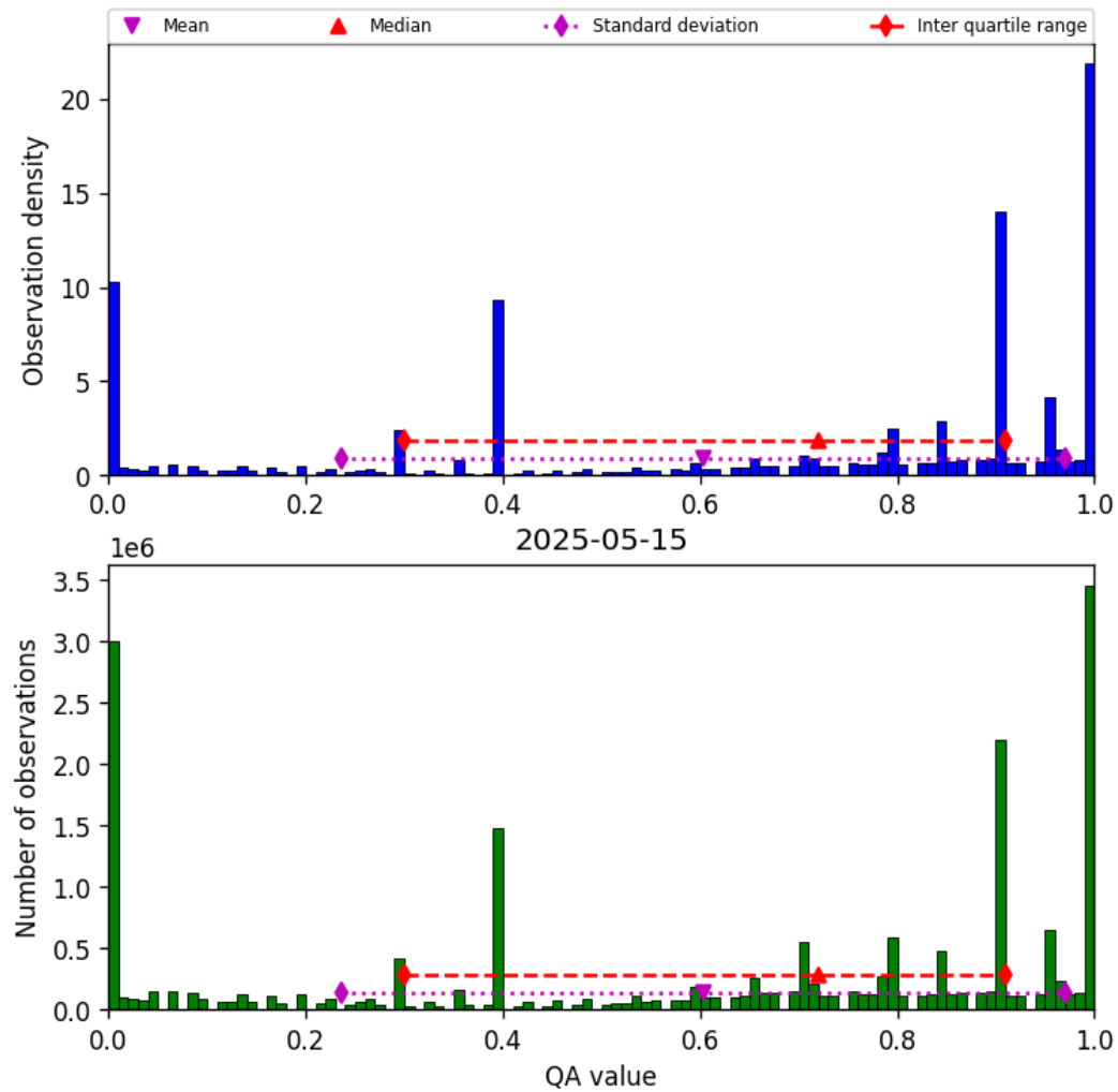
Figure 38: Histogram of “QA value” for 2025-05-15 to 2025-05-16
