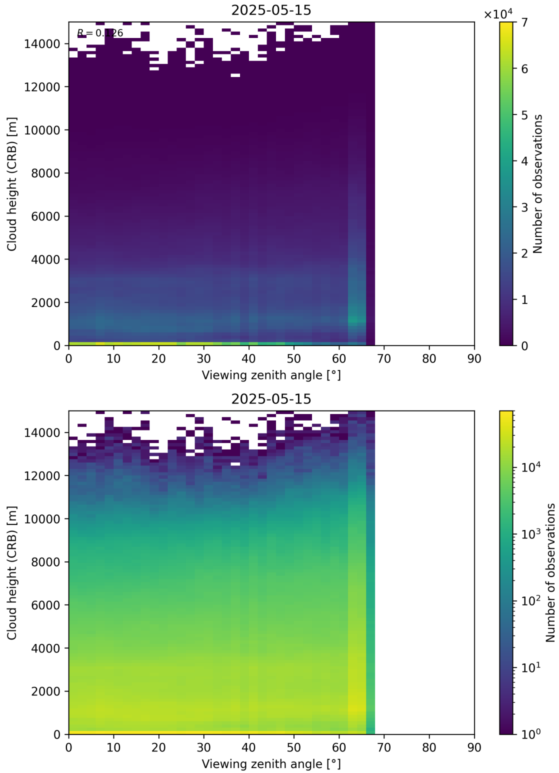
Figure 110: Scatter density plot of “Viewing zenith angle” against “Cloud height (CRB)” for 2025-05-15 to 2025-05-16.
