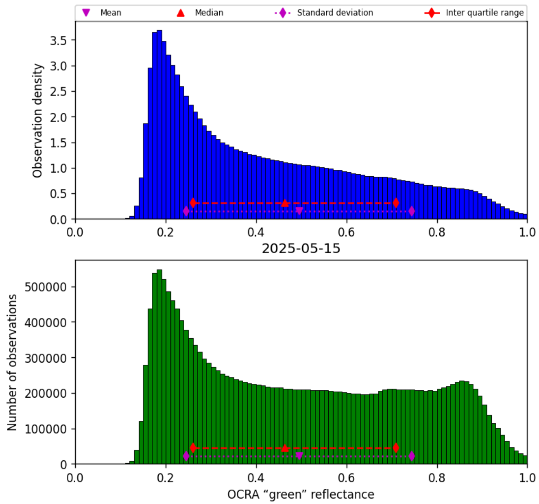
Figure 52: Histogram of “OCRA “green” reflectance” for 2025-05-15 to 2025-05-16
