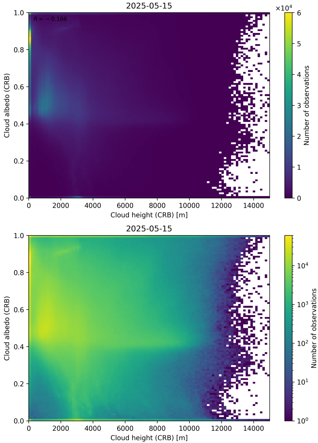
Figure 80: Scatter density plot of “Cloud height (CRB)” against “Cloud albedo (CRB)” for 2025-05-15 to 2025-05-16.
