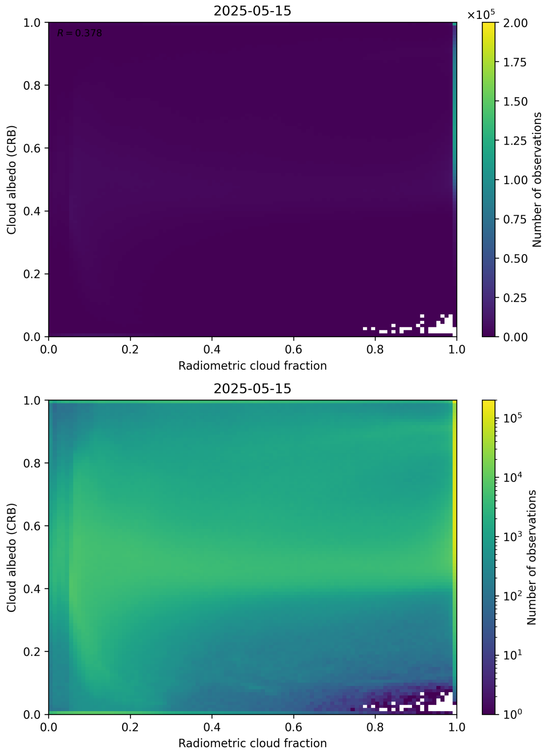
Figure 71: Scatter density plot of “Radiometric cloud fraction” against “Cloud albedo (CRB)” for 2025-05-15 to 2025-05-16.
