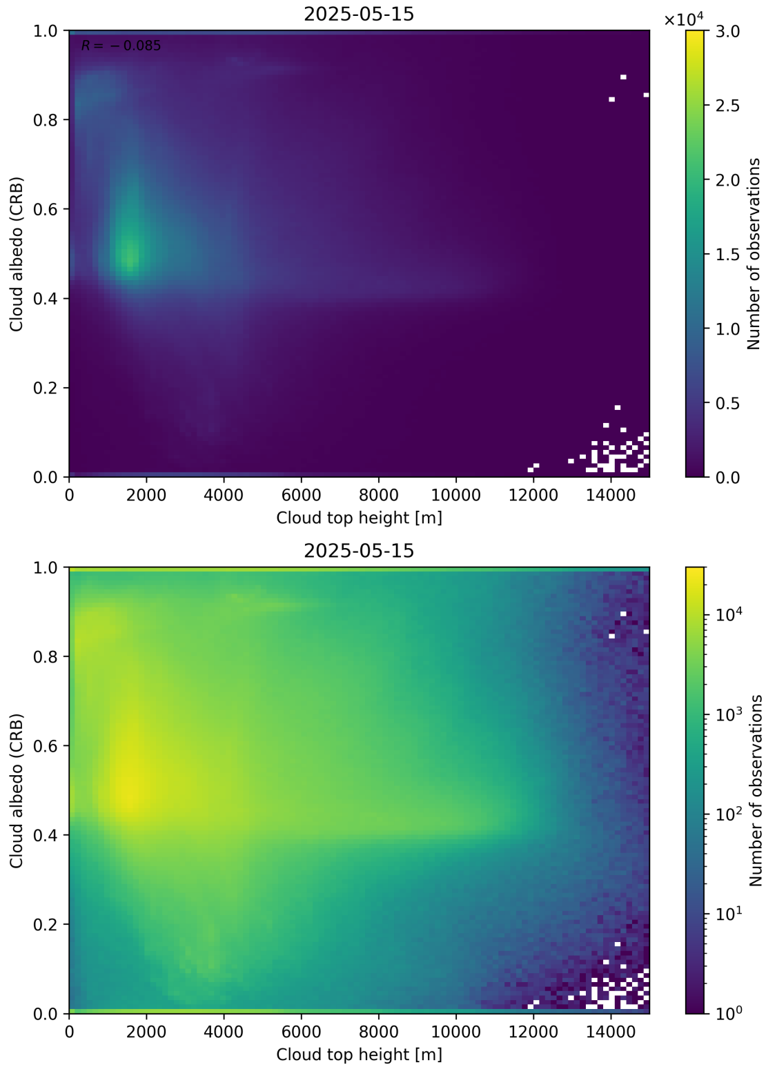
Figure 86: Scatter density plot of “Cloud top height” against “Cloud albedo (CRB)” for 2025-05-15 to 2025-05-16.
