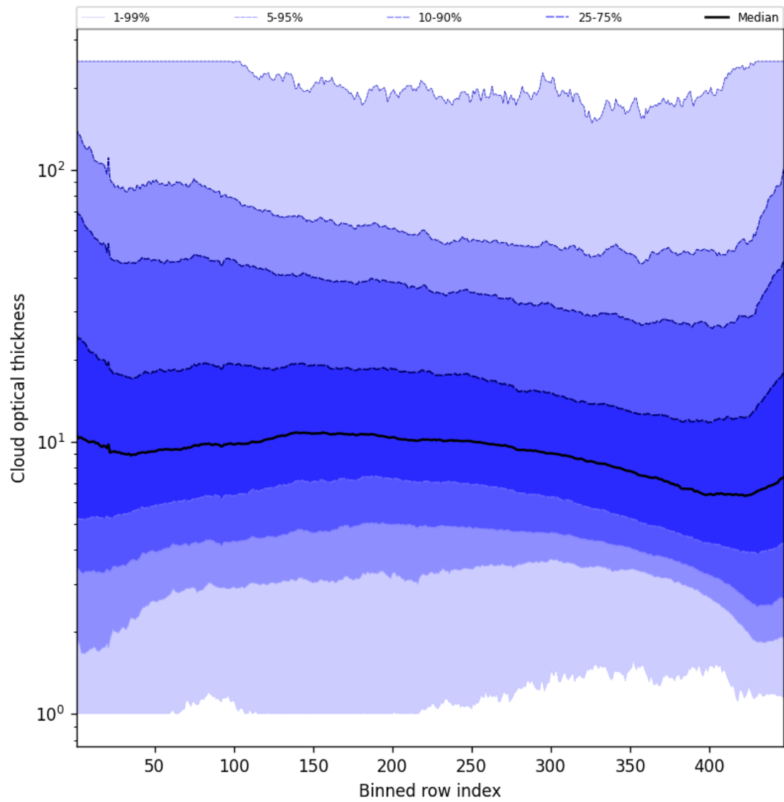
Figure 57: Along track statistics of “Cloud optical thickness” for 2025-05-15 to 2025-05-16
