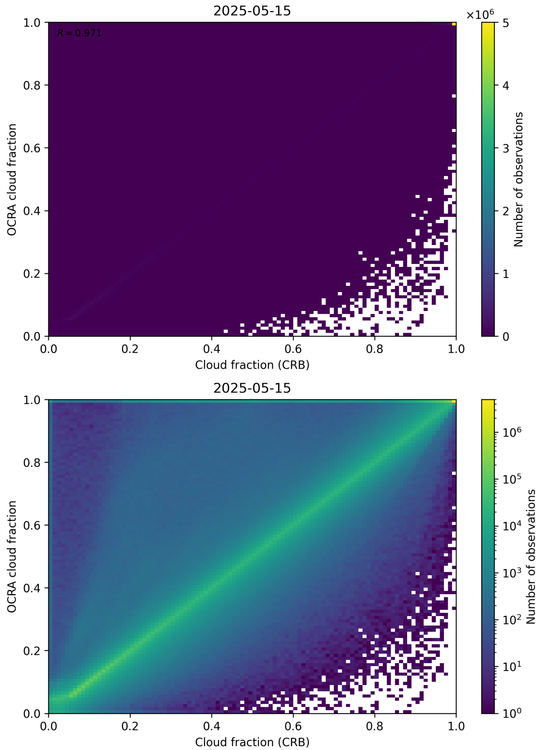
Figure 78: Scatter density plot of “Cloud fraction (CRB)” against “OCRA cloud fraction” for 2025-05-15 to 2025-05-16.
