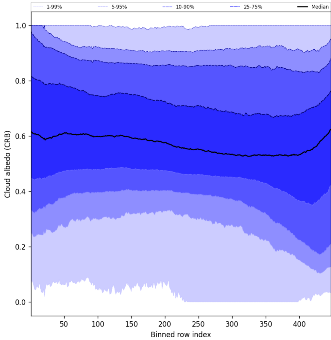
Figure 60: Along track statistics of “Cloud albedo (CRB)” for 2025-05-15 to 2025-05-16
