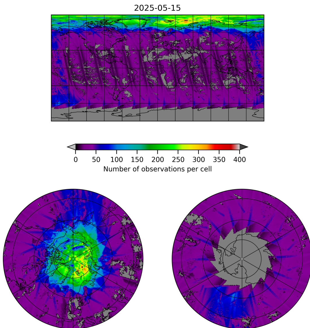
Figure 21: Map of the number of observations for 2025-05-15 to 2025-05-16
