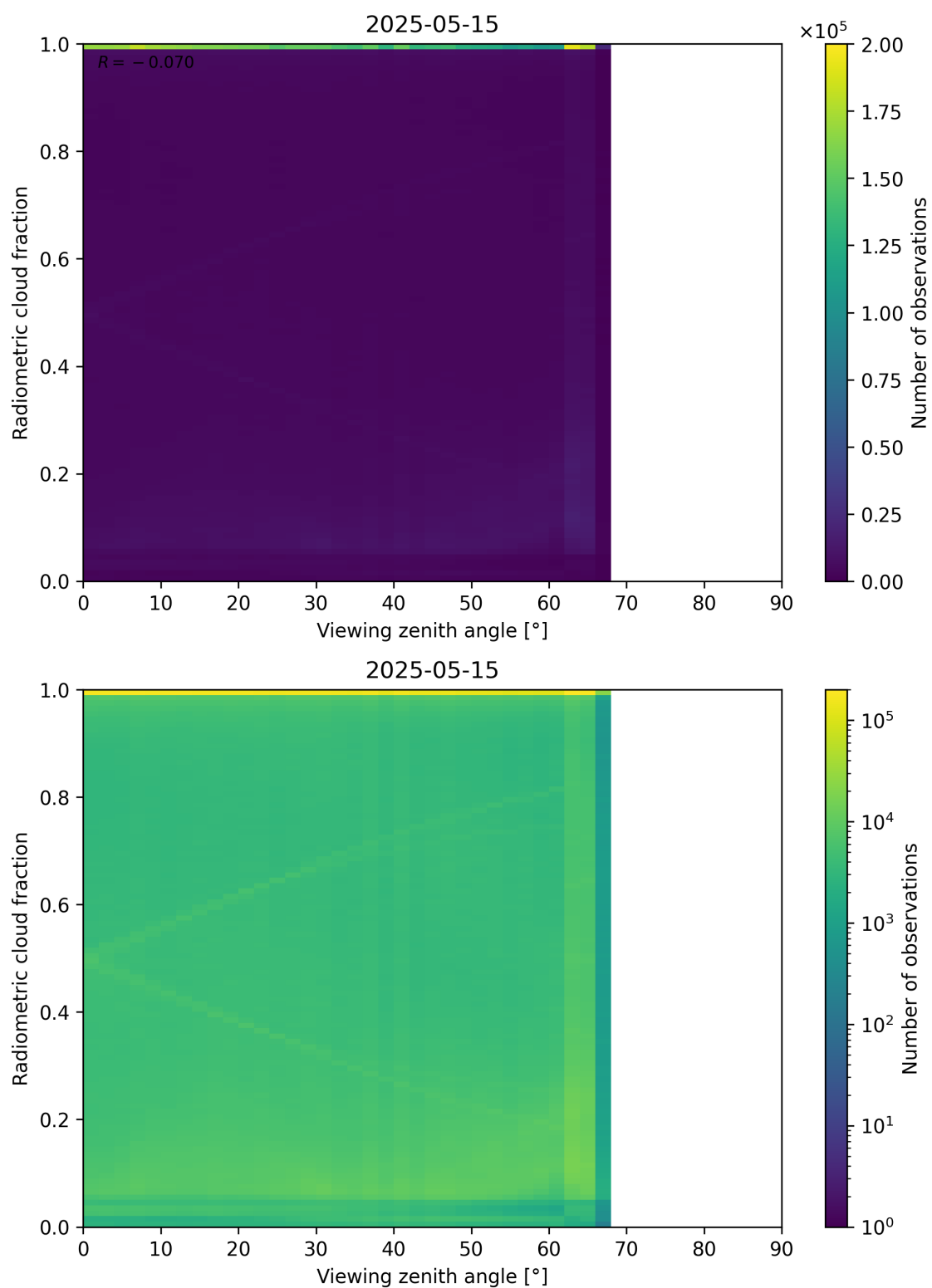
Figure 107: Scatter density plot of “Viewing zenith angle” against “Radiometric cloud fraction” for 2025-05-15 to 2025-05-16.
