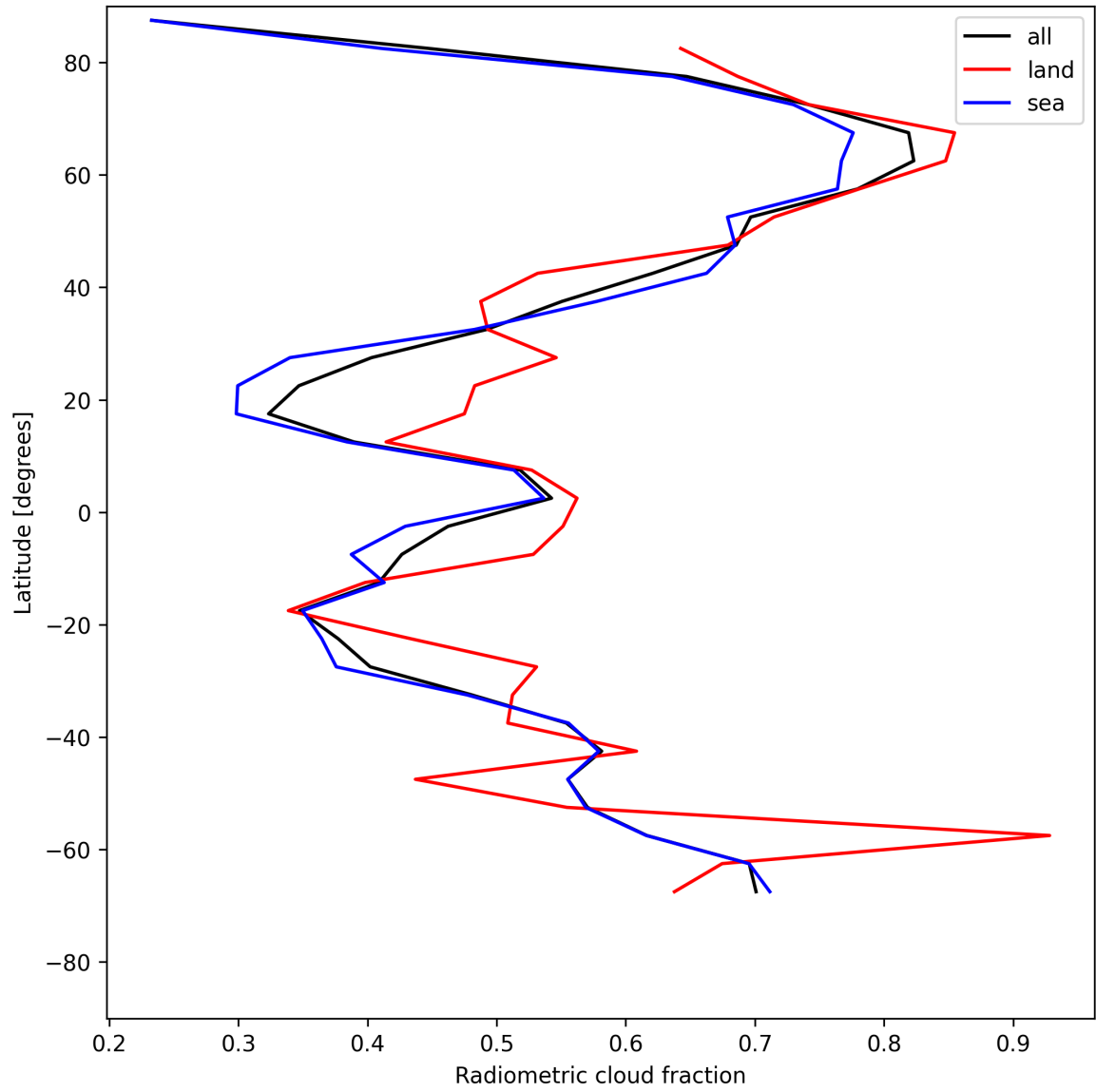
Figure 23: Zonal average of “Radiometric cloud fraction” for 2025-05-15 to 2025-05-16.
