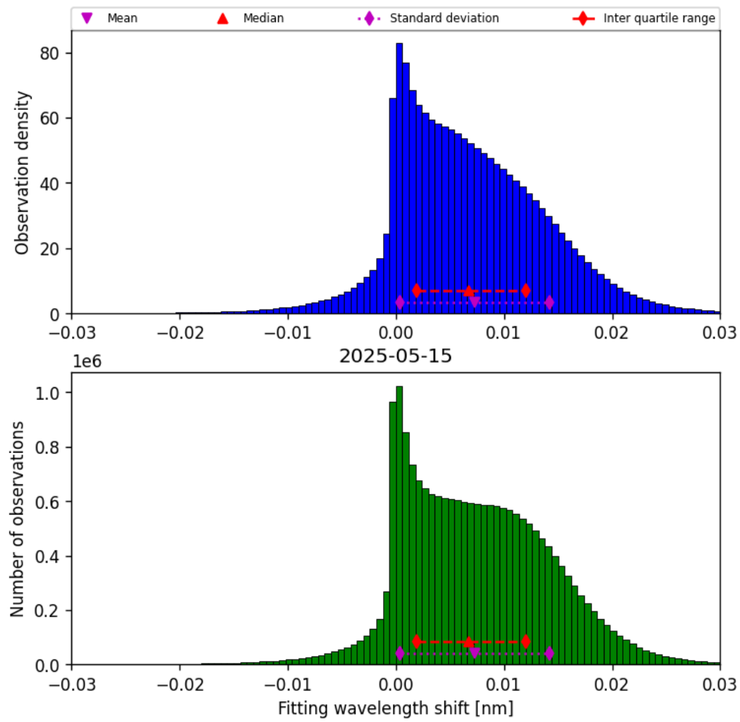
Figure 49: Histogram of “Fitting wavelength shift” for 2025-05-15 to 2025-05-16
