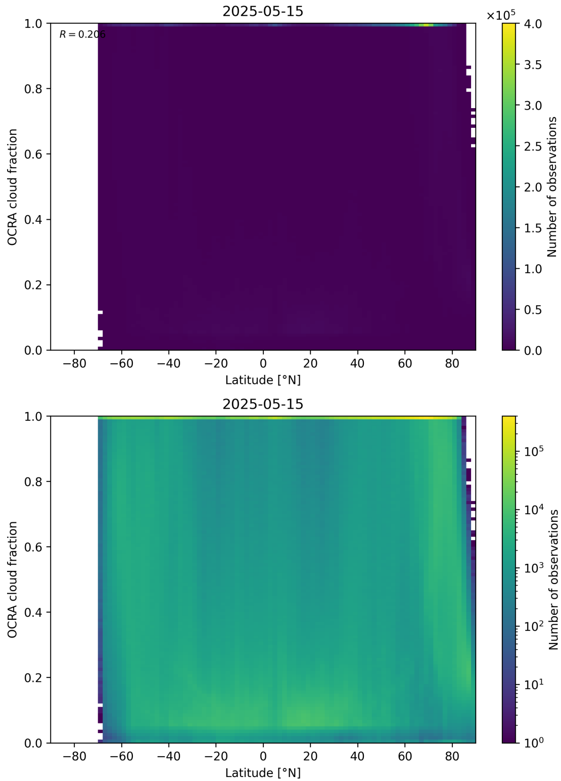
Figure 93: Scatter density plot of “Latitude” against “OCRA cloud fraction” for 2025-05-15 to 2025-05-16.
