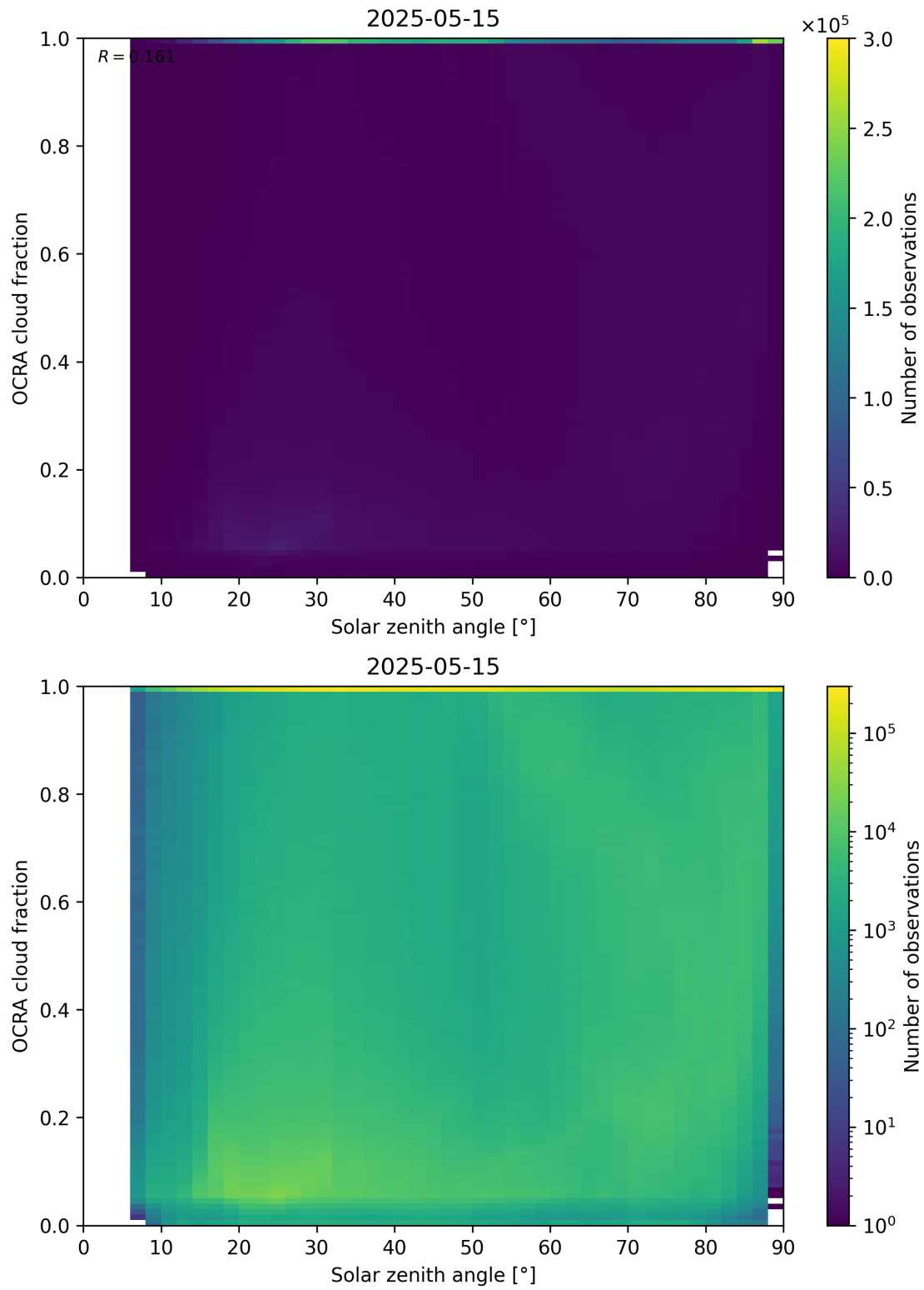
Figure 100: Scatter density plot of “Solar zenith angle” against “OCRA cloud fraction” for 2025-05-15 to 2025-05-16.
