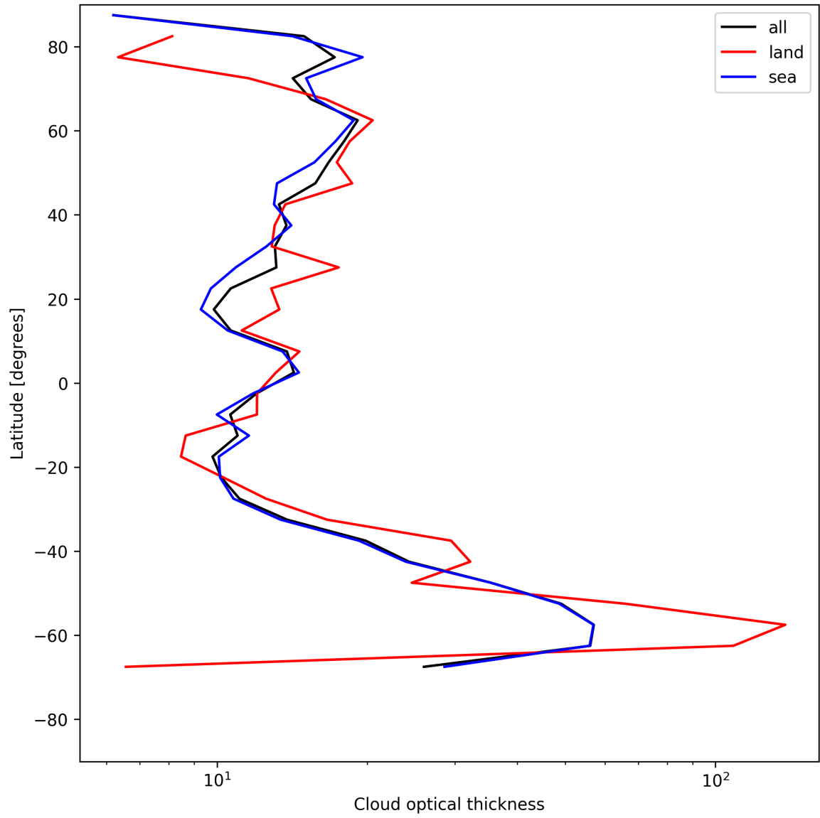
Figure 25: Zonal average of “Cloud optical thickness” for 2025-05-15 to 2025-05-16.
