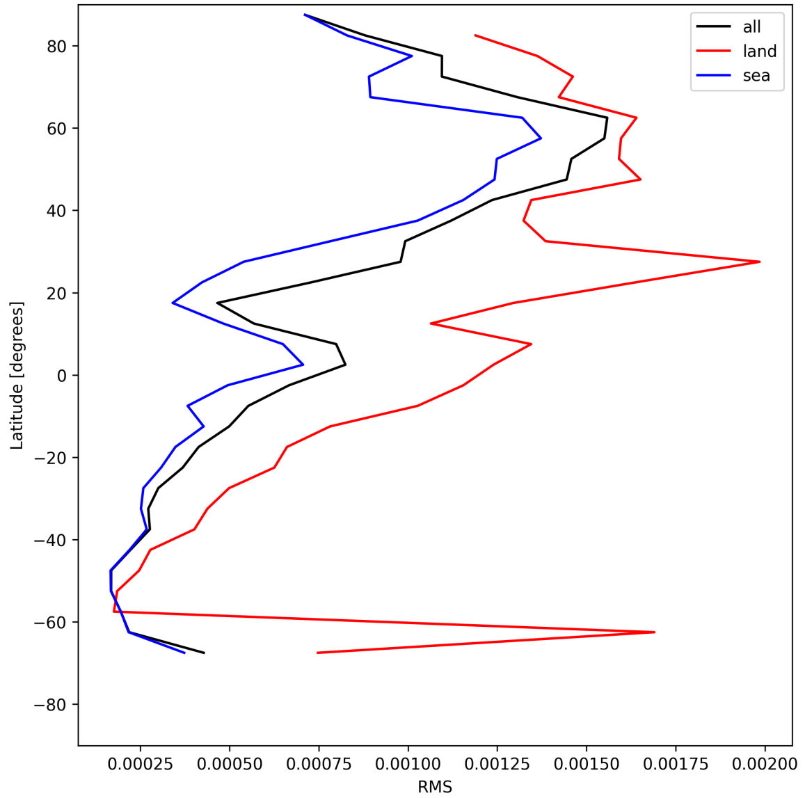
Figure 31: Zonal average of “RMS” for 2025-05-15 to 2025-05-16.
