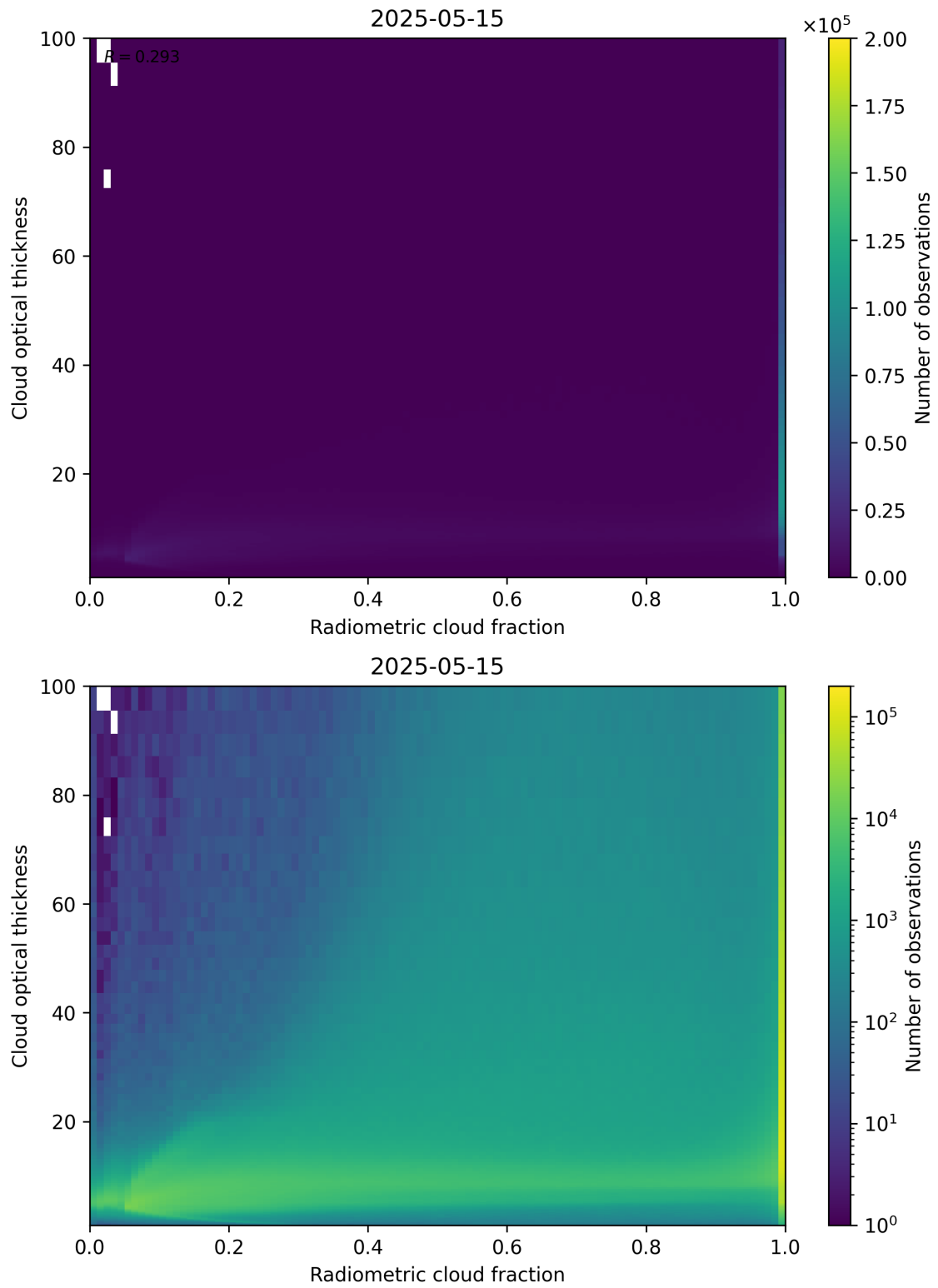
Figure 75: Scatter density plot of “Radiometric cloud fraction” against “Cloud optical thickness” for 2025-05-15 to 2025-05-16.
