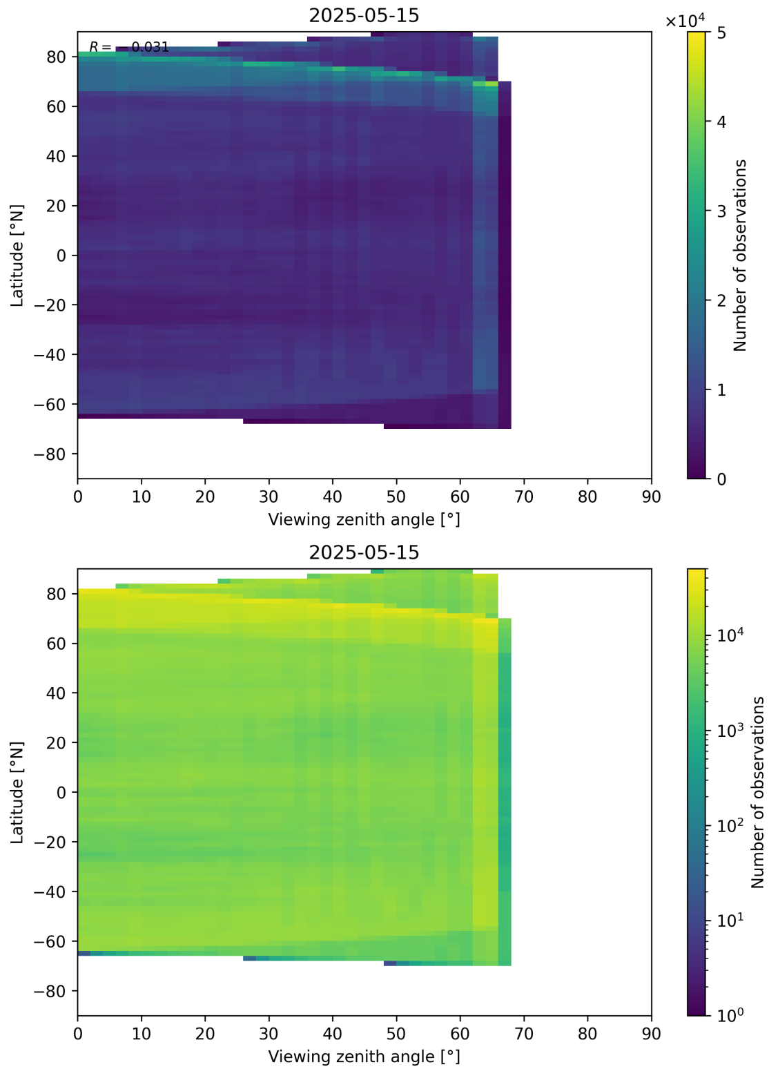
Figure 113: Scatter density plot of “Viewing zenith angle” against “Latitude” for 2025-05-15 to 2025-05-16.
