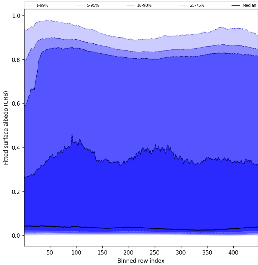
Figure 62: Along track statistics of “Fitted surface albedo (CRB)” for 2025-05-15 to 2025-05-16
