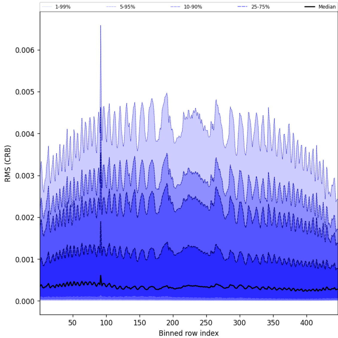
Figure 64: Along track statistics of “RMS (CRB)” for 2025-05-15 to 2025-05-16
