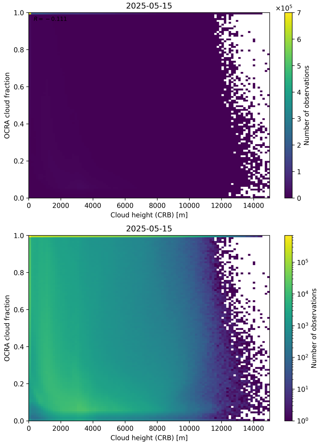
Figure 81: Scatter density plot of “Cloud height (CRB)” against “OCRA cloud fraction” for 2025-05-15 to 2025-05-16.
