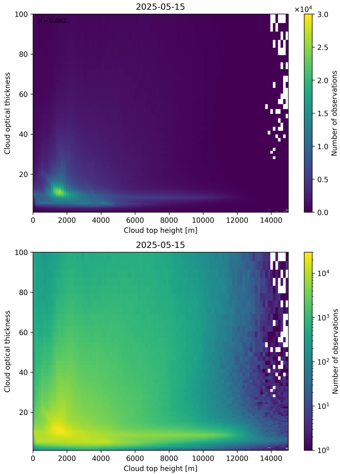
Figure 90: Scatter density plot of “Cloud top height” against “Cloud optical thickness” for 2025-05-15 to 2025-05-16.
