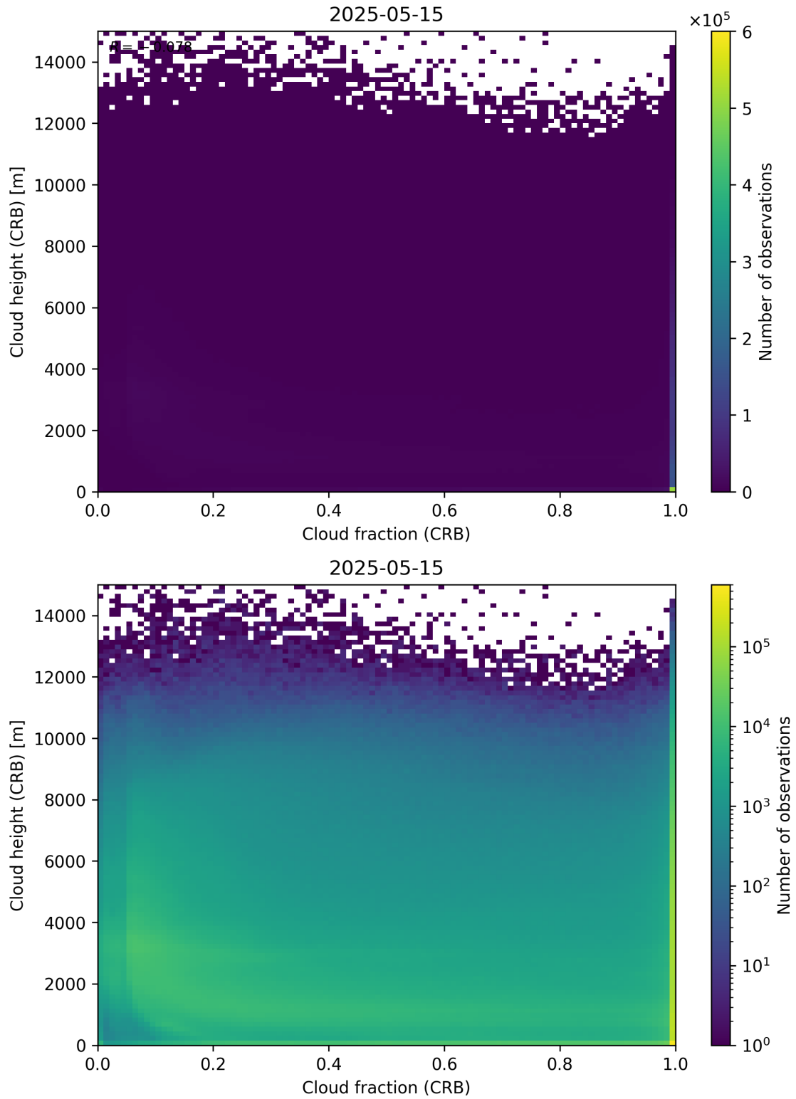
Figure 79: Scatter density plot of “Cloud fraction (CRB)” against “Cloud height (CRB)” for 2025-05-15 to 2025-05-16.
