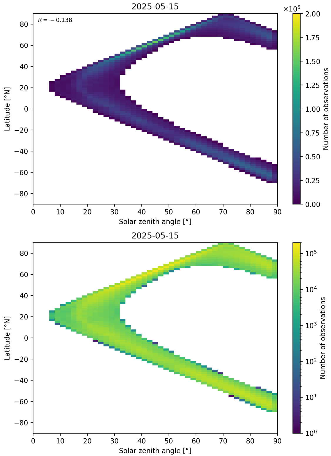
Figure 105: Scatter density plot of “Solar zenith angle” against “Latitude” for 2025-05-15 to 2025-05-16.
