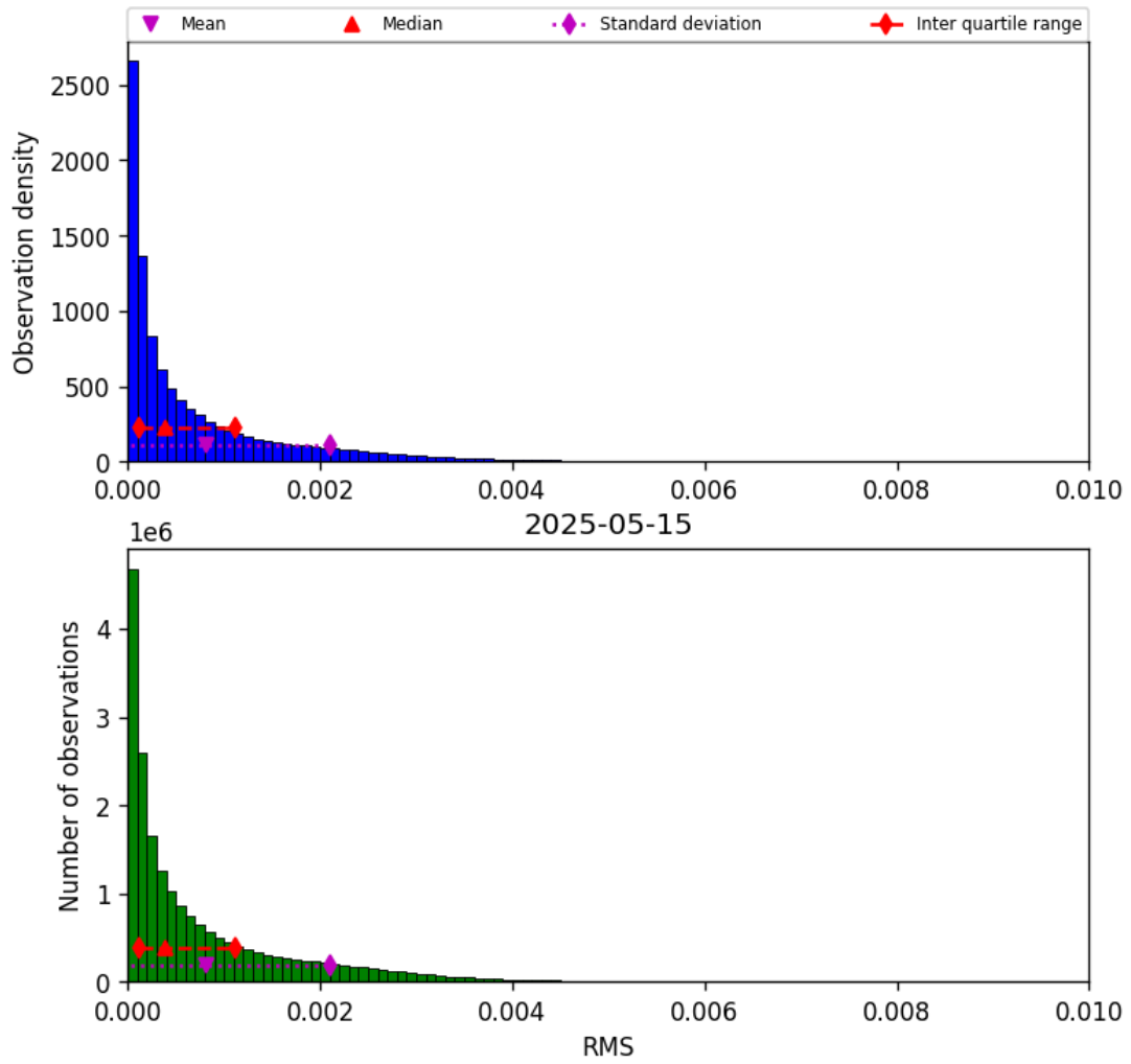
Figure 47: Histogram of “RMS” for 2025-05-15 to 2025-05-16
