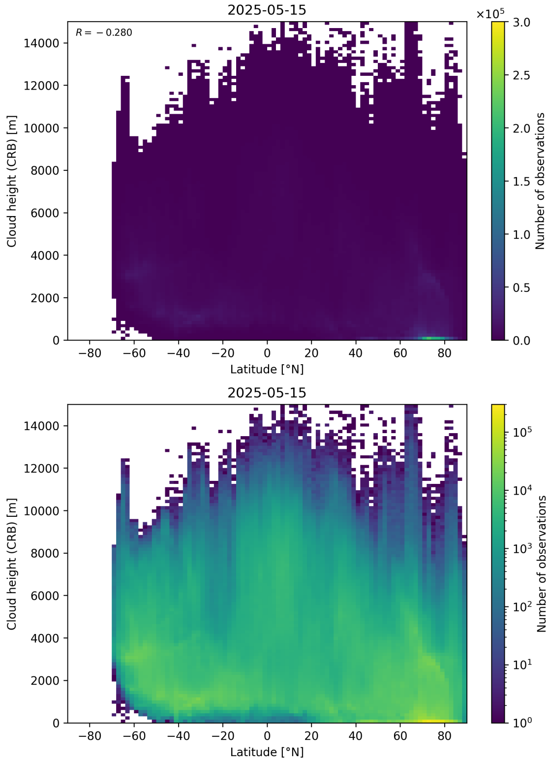
Figure 95: Scatter density plot of “Latitude” against “Cloud height (CRB)” for 2025-05-15 to 2025-05-16.
