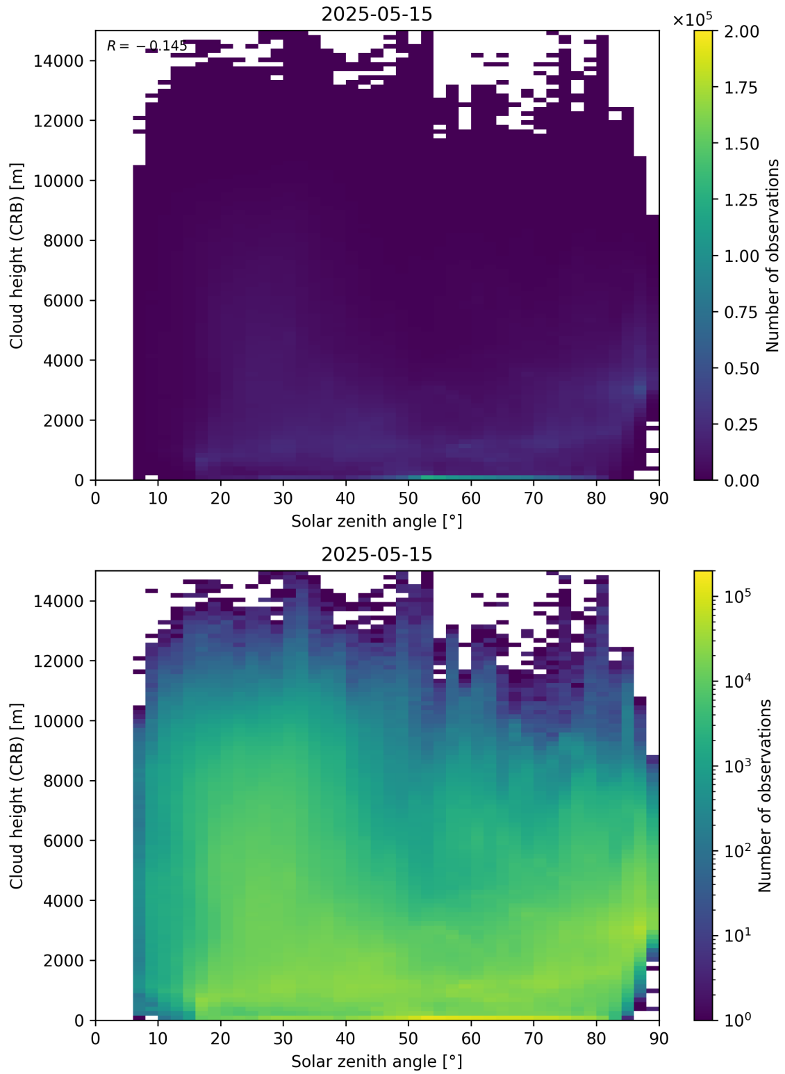
Figure 102: Scatter density plot of “Solar zenith angle” against “Cloud height (CRB)” for 2025-05-15 to 2025-05-16.
