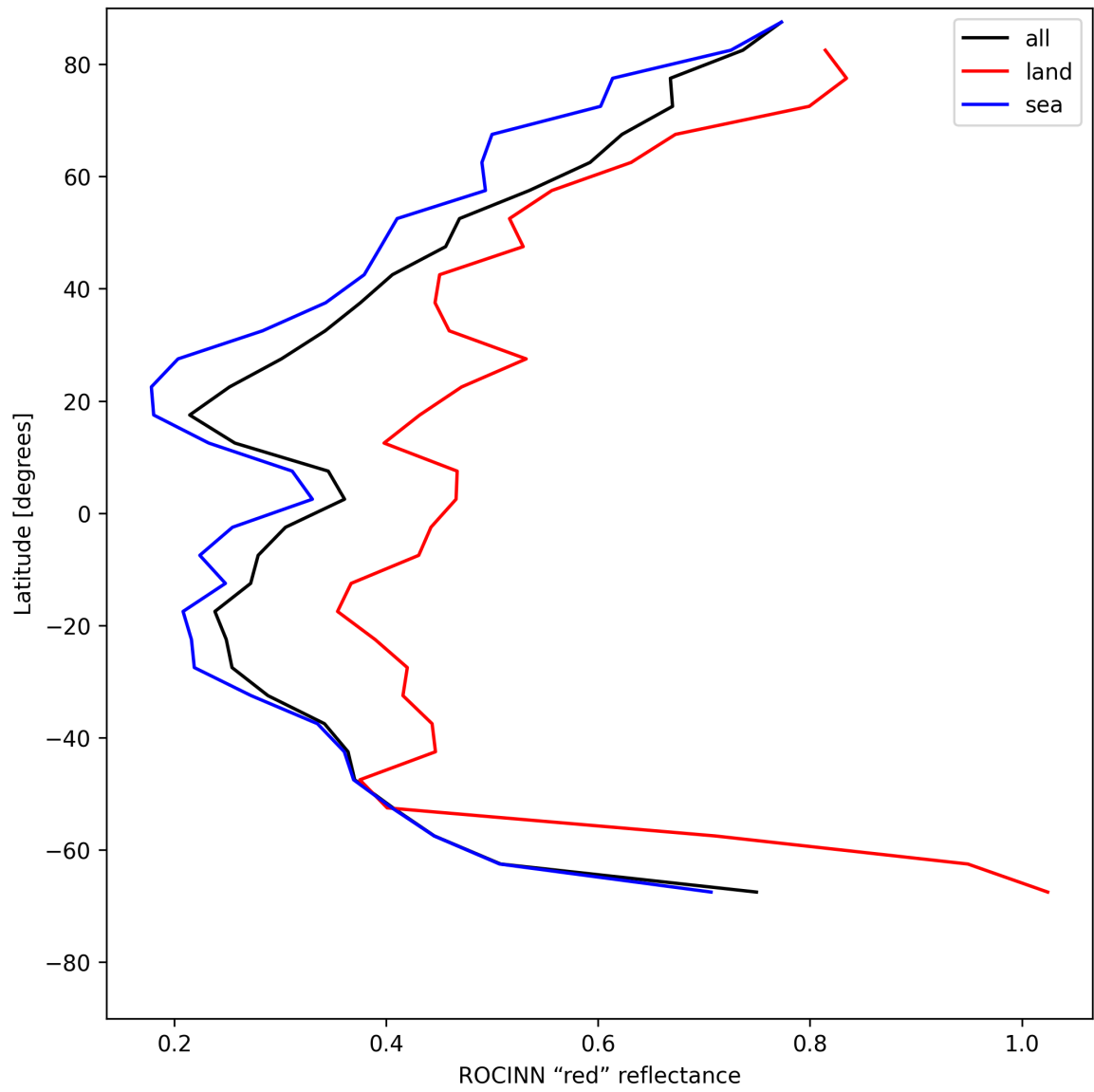
Figure 37: Zonal average of “ROCINN “red” reflectance” for 2025-05-15 to 2025-05-16.
