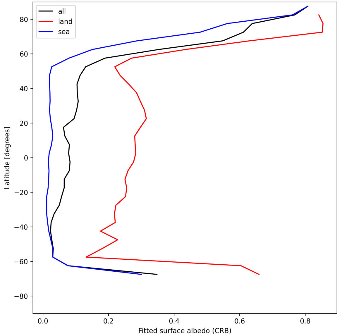
Figure 30: Zonal average of “Fitted surface albedo (CRB)” for 2025-05-15 to 2025-05-16.
