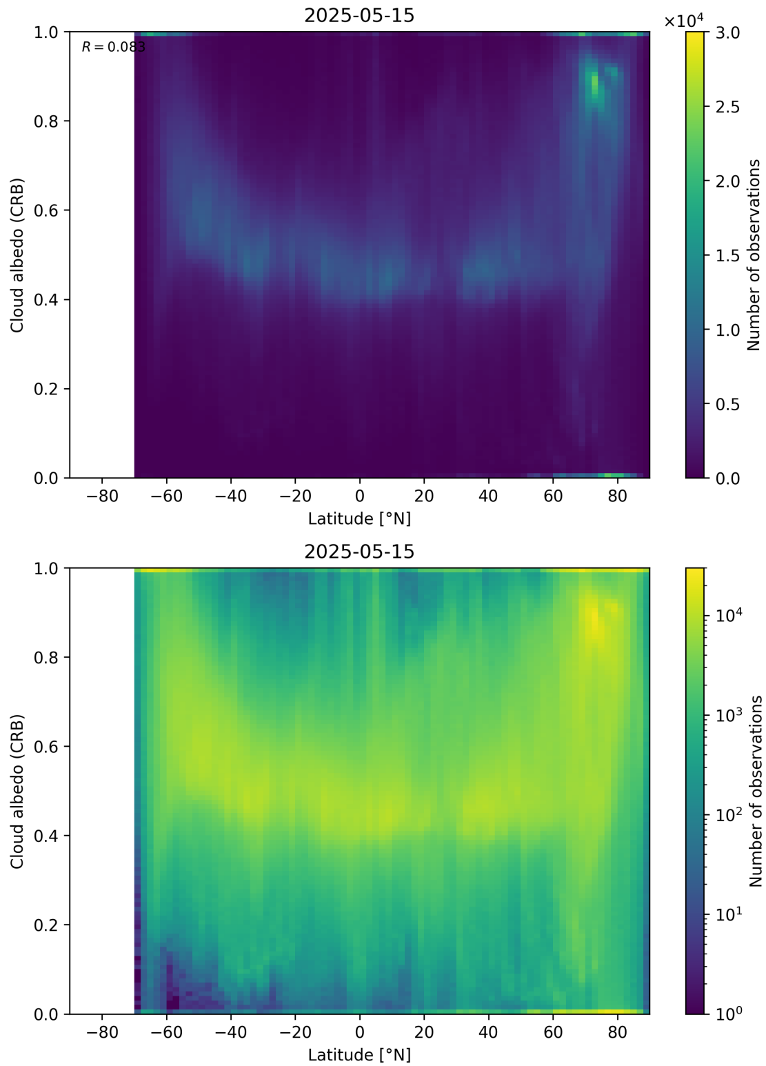
Figure 91: Scatter density plot of “Latitude” against “Cloud albedo (CRB)” for 2025-05-15 to 2025-05-16.
