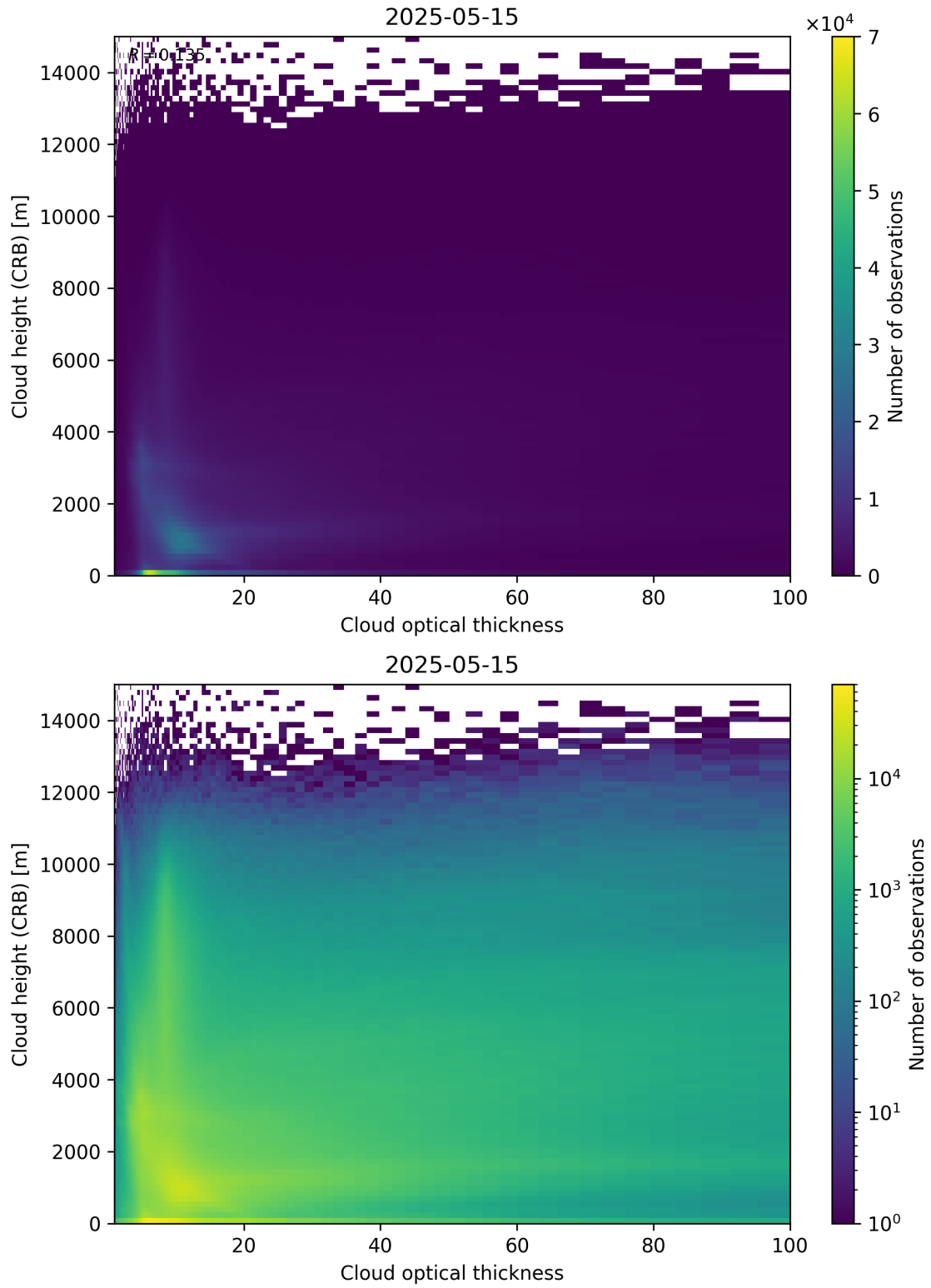
Figure 85: Scatter density plot of “Cloud optical thickness” against “Cloud height (CRB)” for 2025-05-15 to 2025-05-16.
