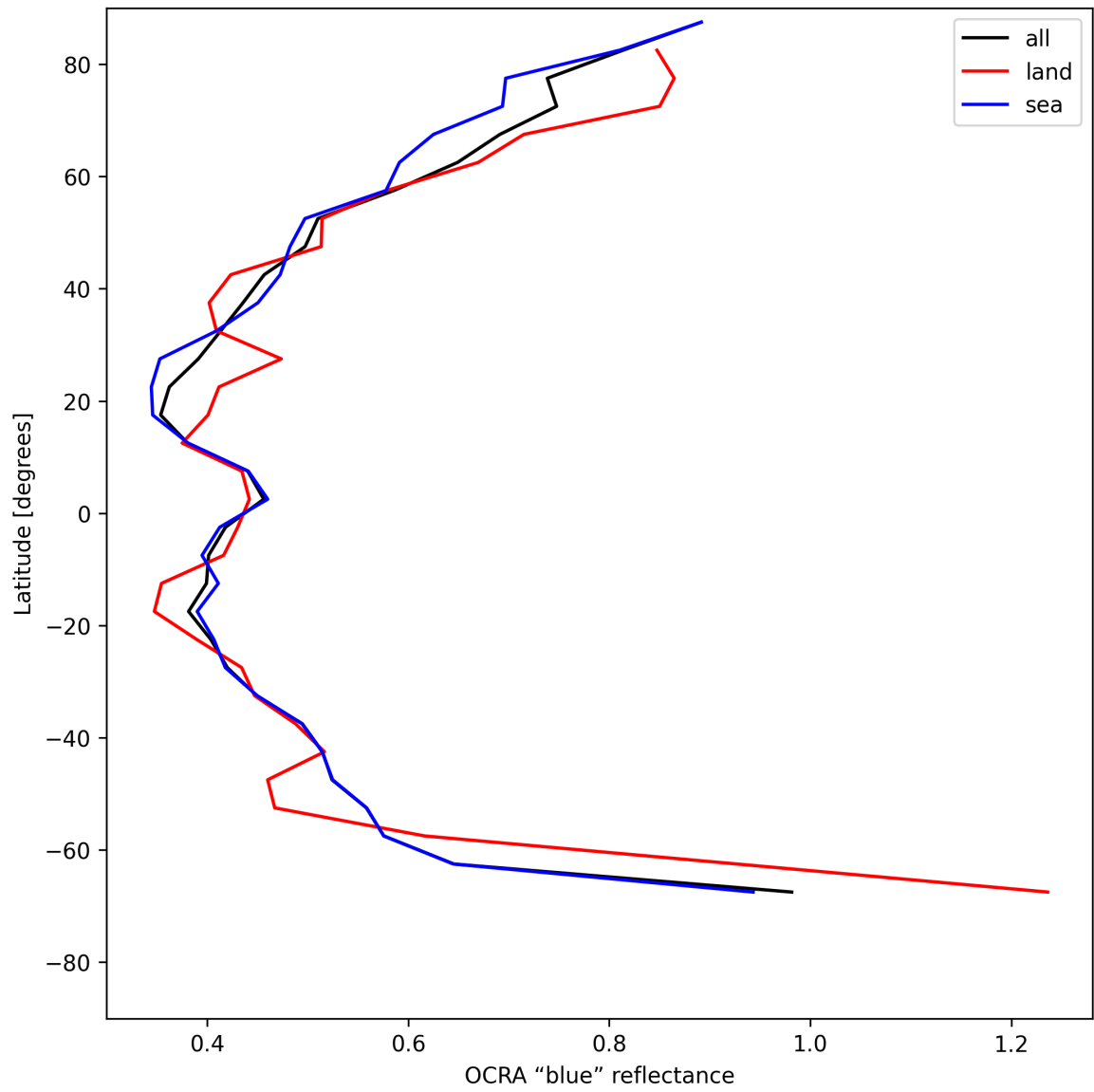
Figure 35: Zonal average of "OCRA "blue" reflectance" for 2025-05-15 to 2025-05-16.
