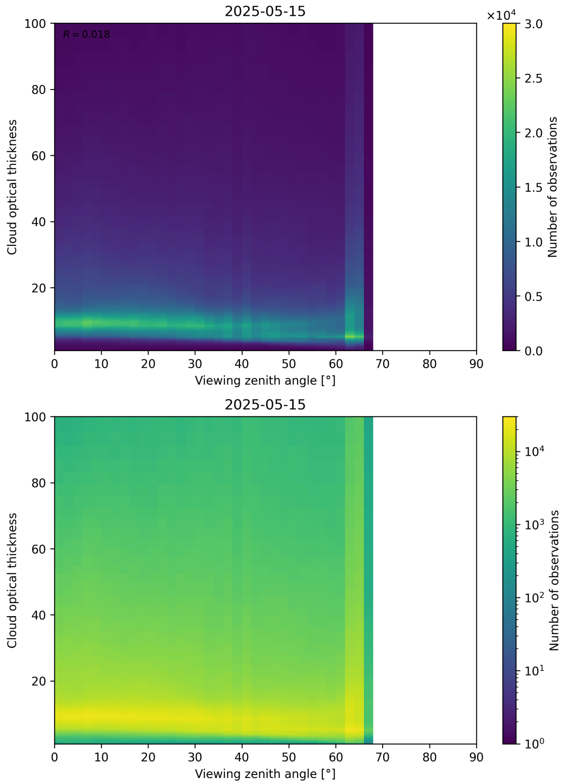
Figure 111: Scatter density plot of “Viewing zenith angle” against “Cloud optical thickness” for 2025-05-15 to 2025-05-16.
