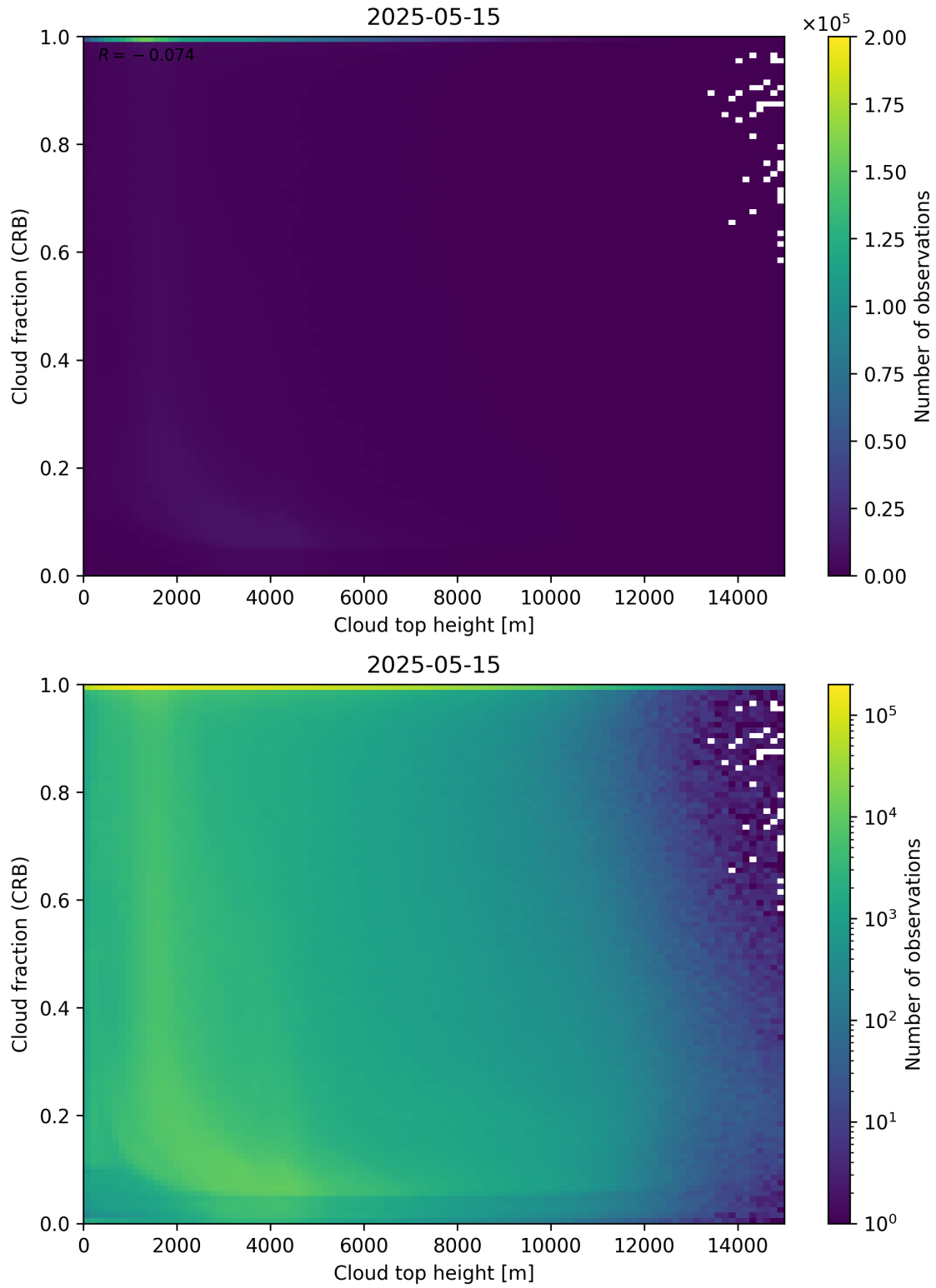
Figure 88: Scatter density plot of “Cloud top height” against “Cloud fraction (CRB)” for 2025-05-15 to 2025-05-16.
