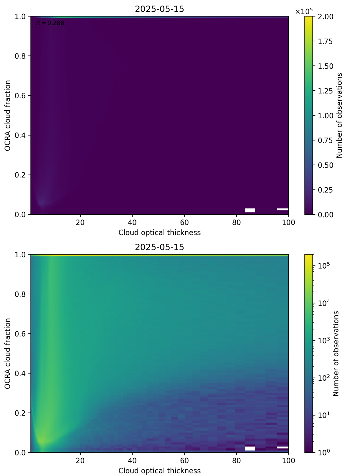
Figure 83: Scatter density plot of “Cloud optical thickness” against “OCRA cloud fraction” for 2025-05-15 to 2025-05-16.
