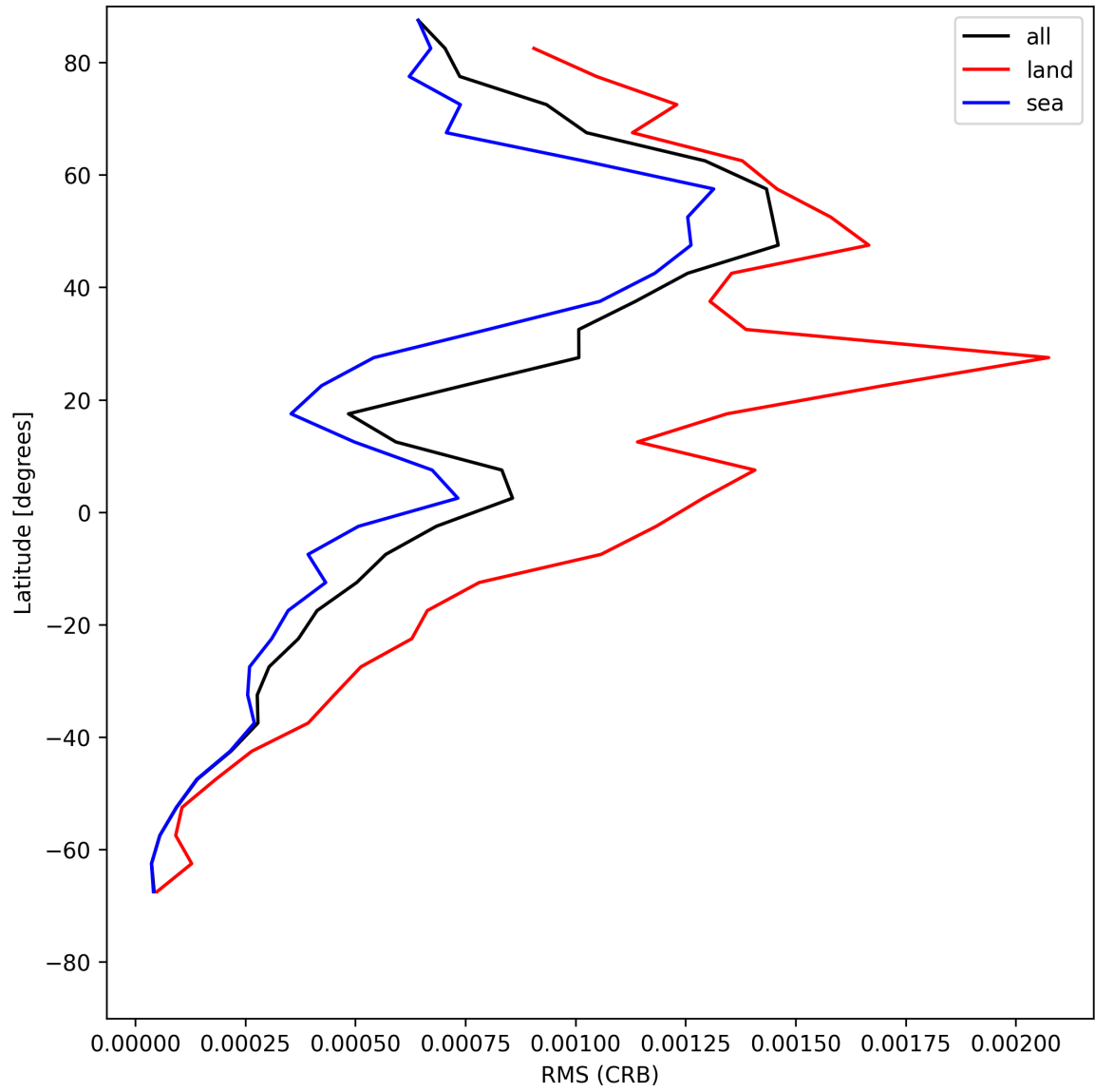
Figure 32: Zonal average of “RMS (CRB)” for 2025-05-15 to 2025-05-16.
