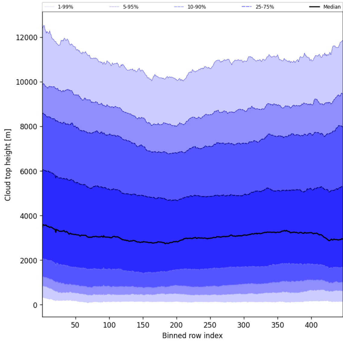
Figure 56: Along track statistics of “Cloud top height” for 2025-05-15 to 2025-05-16
