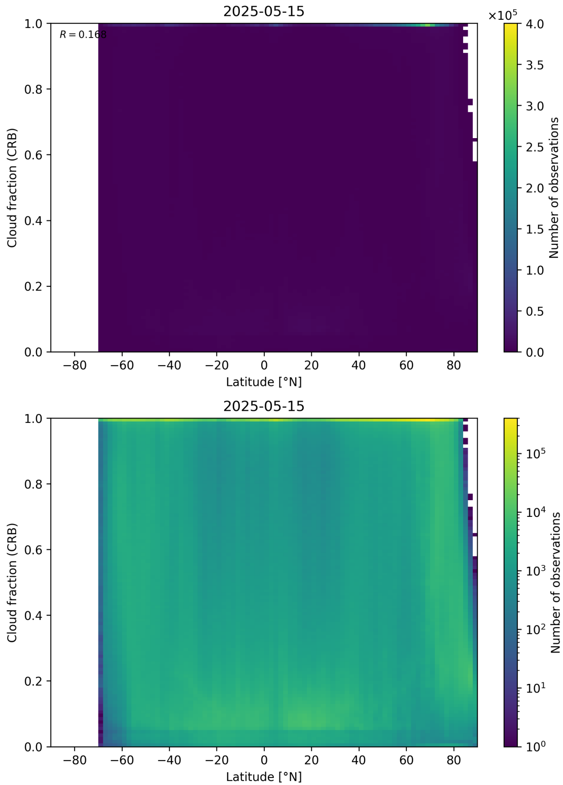
Figure 94: Scatter density plot of “Latitude” against “Cloud fraction (CRB)” for 2025-05-15 to 2025-05-16.
