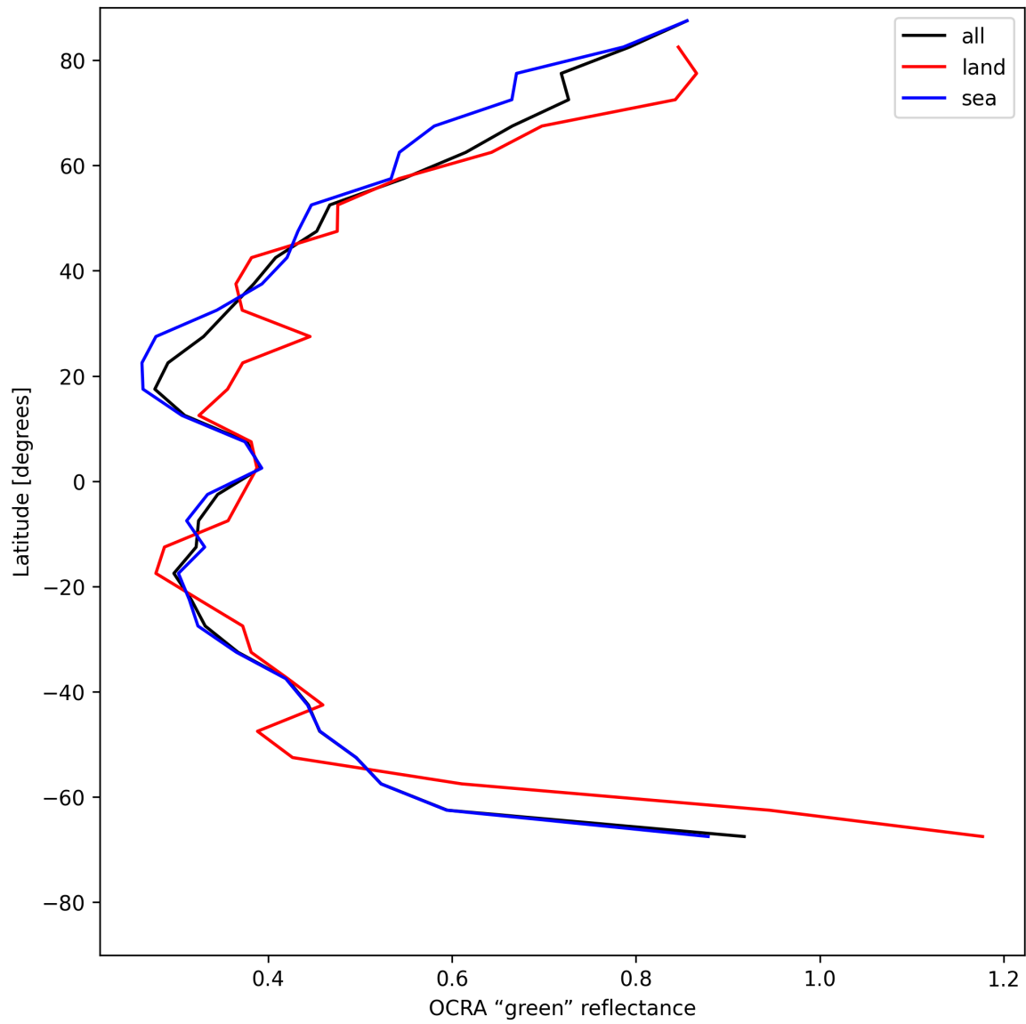
Figure 36: Zonal average of “OCRA “green” reflectance” for 2025-05-15 to 2025-05-16.
