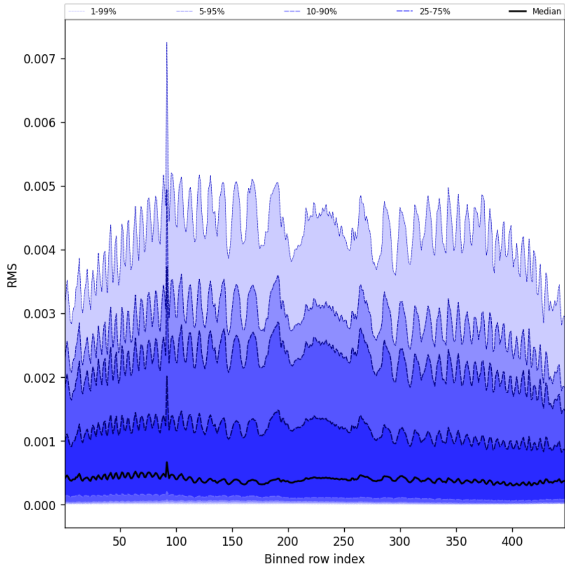
Figure 63: Along track statistics of “RMS” for 2025-05-15 to 2025-05-16
