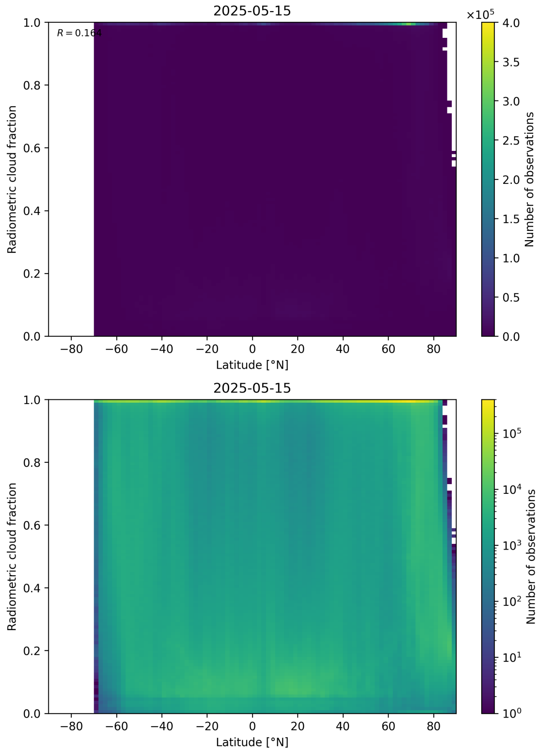
Figure 92: Scatter density plot of “Latitude” against “Radiometric cloud fraction” for 2025-05-15 to 2025-05-16.
