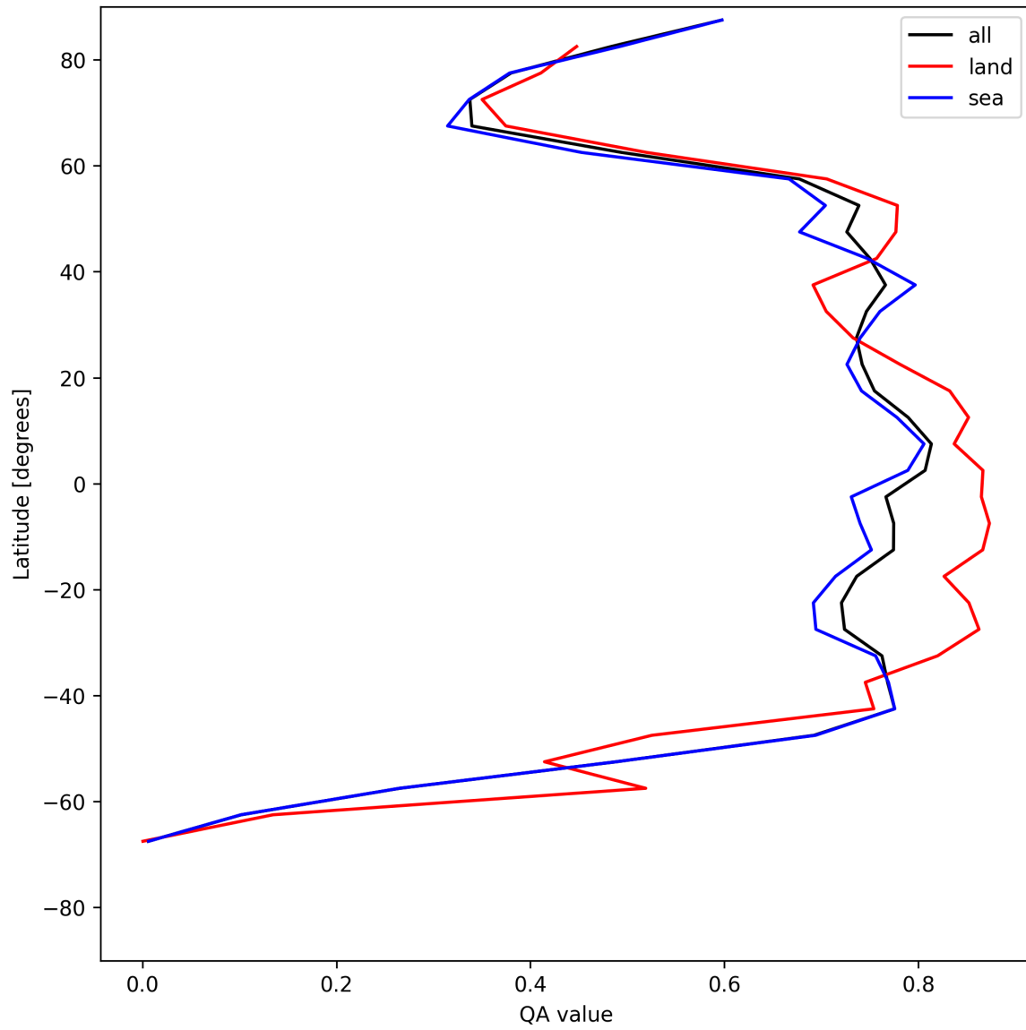
Figure 22: Zonal average of “QA value” for 2025-05-15 to 2025-05-16.
