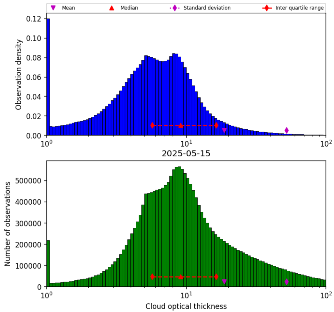
Figure 41: Histogram of “Cloud optical thickness” for 2025-05-15 to 2025-05-16
