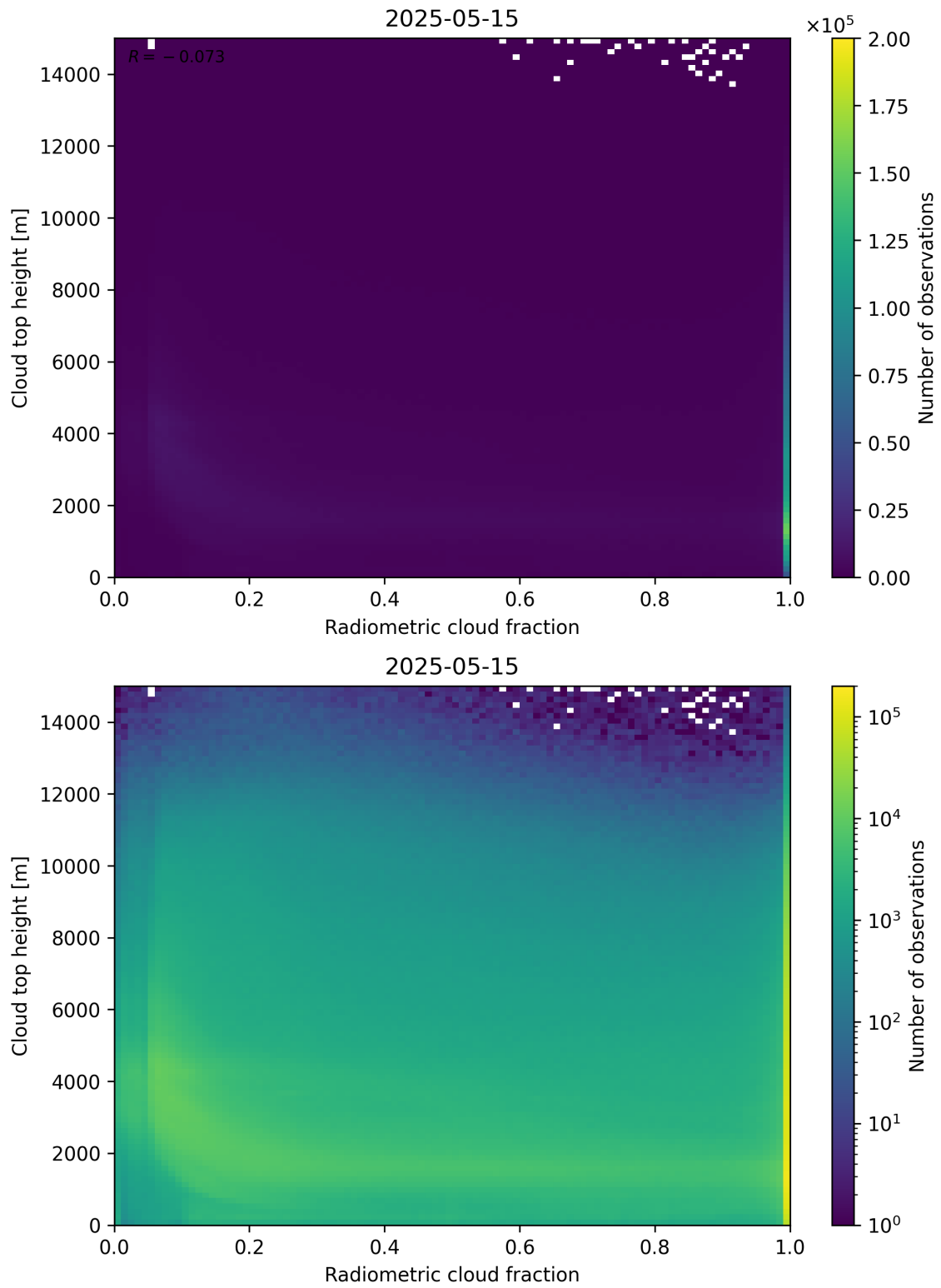
Figure 76: Scatter density plot of “Radiometric cloud fraction” against “Cloud top height” for 2025-05-15 to 2025-05-16.
