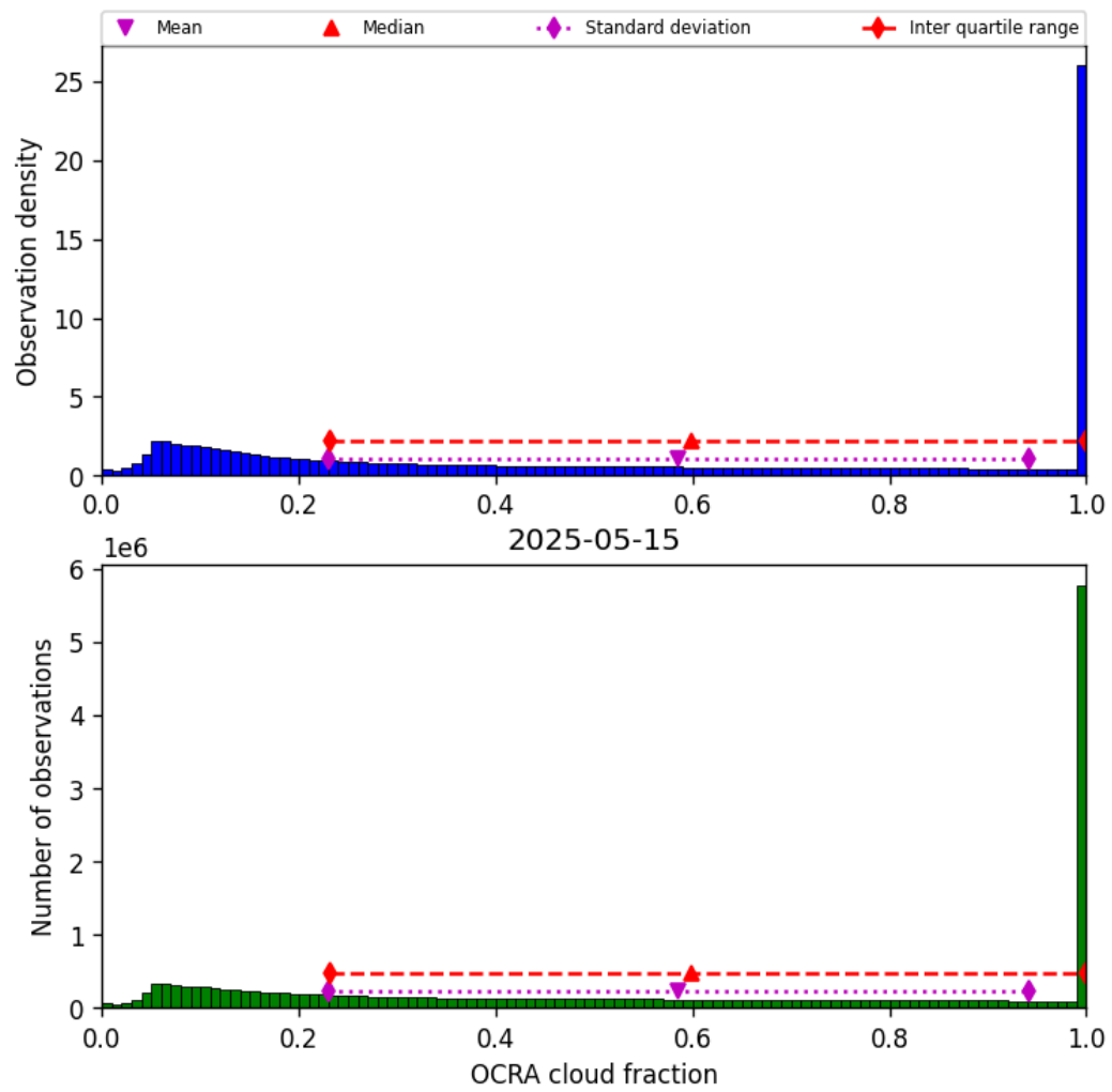
Figure 50: Histogram of “OCRA cloud fraction” for 2025-05-15 to 2025-05-16
