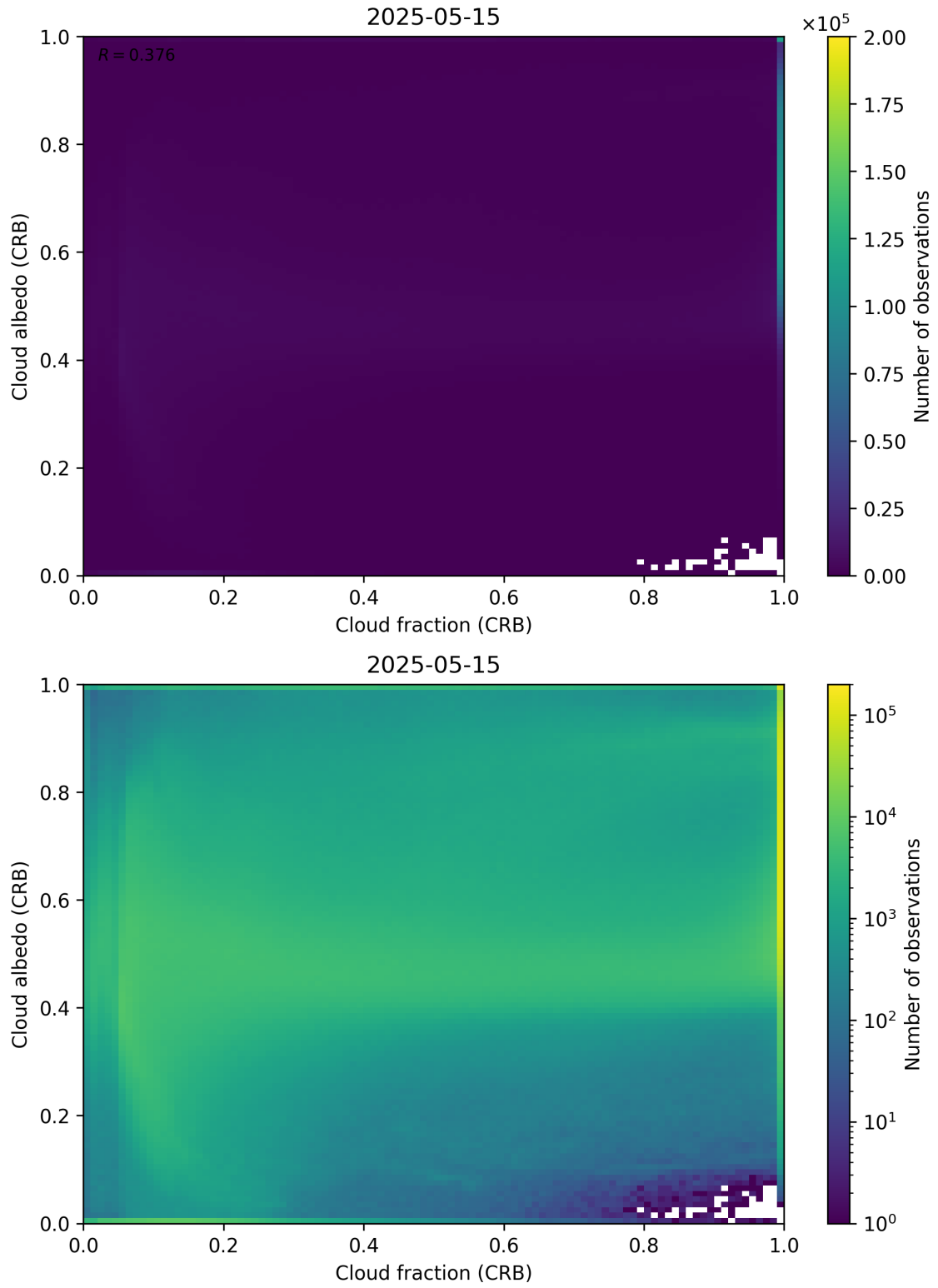
Figure 77: Scatter density plot of “Cloud fraction (CRB)” against “Cloud albedo (CRB)” for 2025-05-15 to 2025-05-16.
