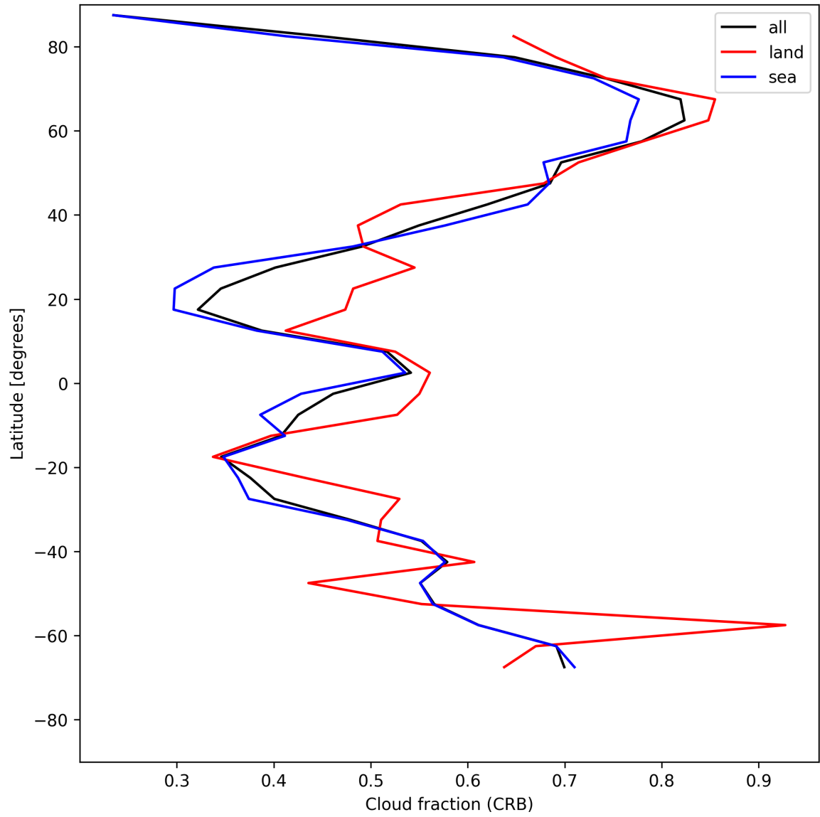
Figure 26: Zonal average of “Cloud fraction (CRB)” for 2025-05-15 to 2025-05-16.
