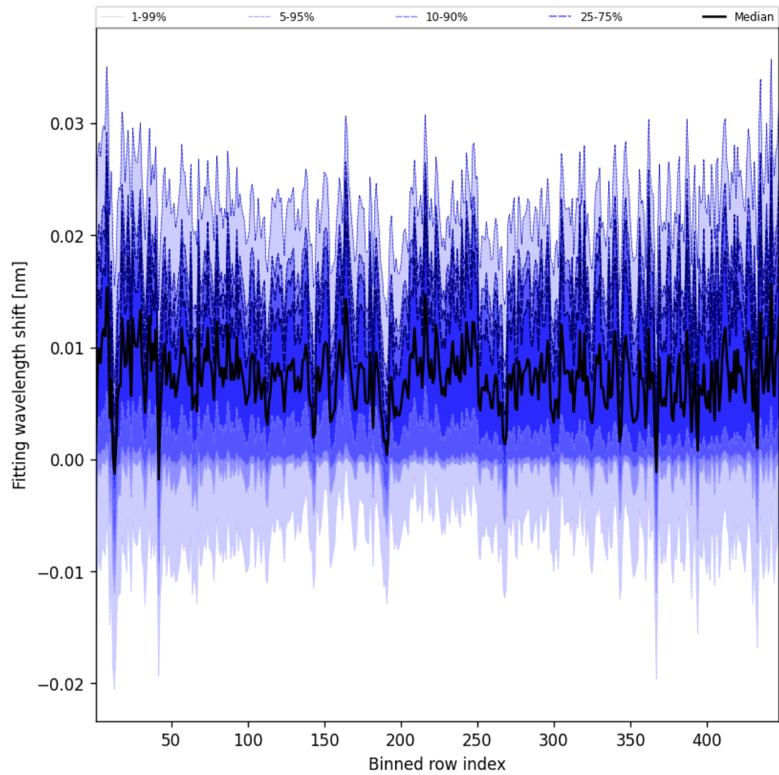
Figure 65: Along track statistics of “Fitting wavelength shift” for 2025-05-15 to 2025-05-16
