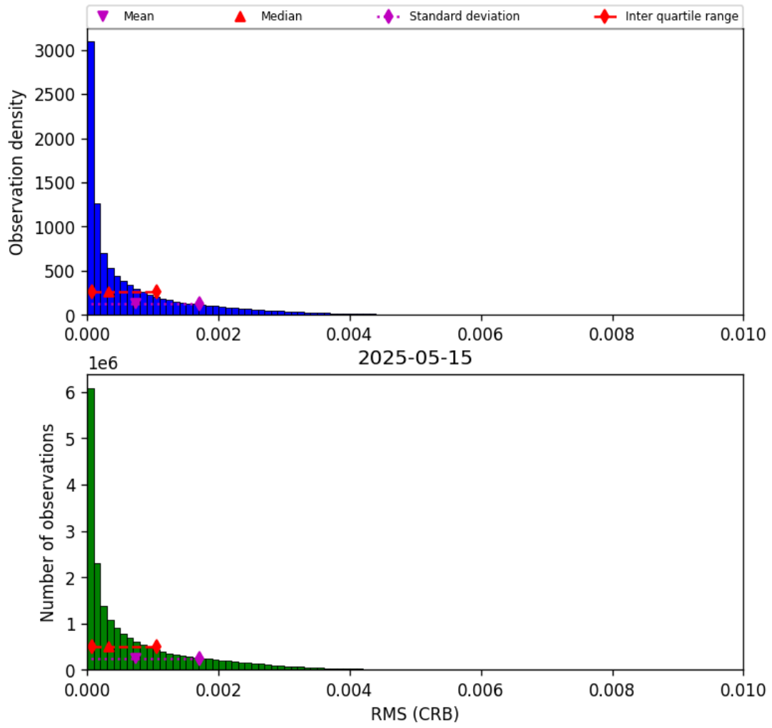
Figure 48: Histogram of “RMS (CRB)” for 2025-05-15 to 2025-05-16
