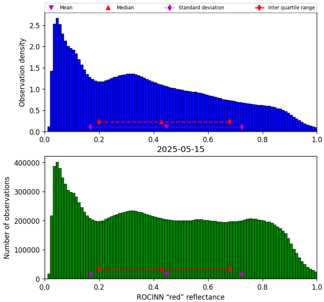
Figure 53: Histogram of “ROCINN “red” reflectance” for 2025-05-15 to 2025-05-16
