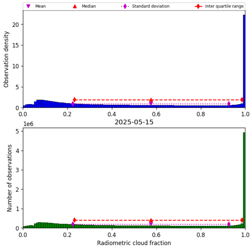
Figure 39: Histogram of “Radiometric cloud fraction” for 2025-05-15 to 2025-05-16
