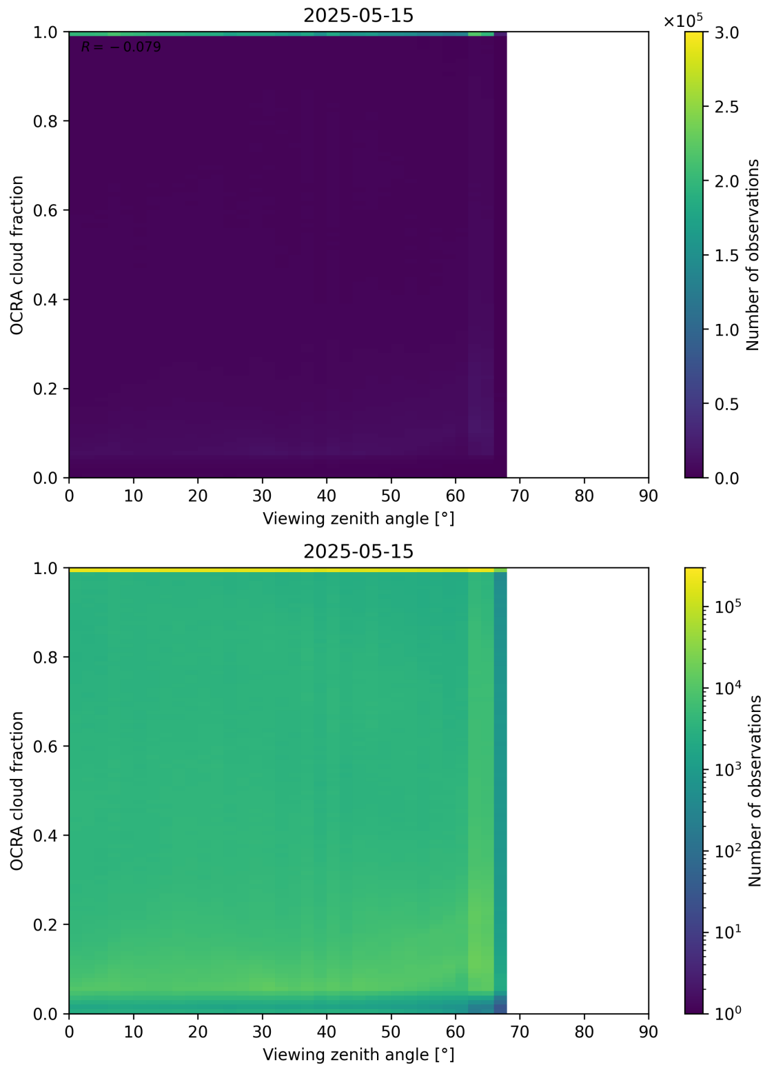
Figure 108: Scatter density plot of “Viewing zenith angle” against “OCRA cloud fraction” for 2025-05-15 to 2025-05-16.
