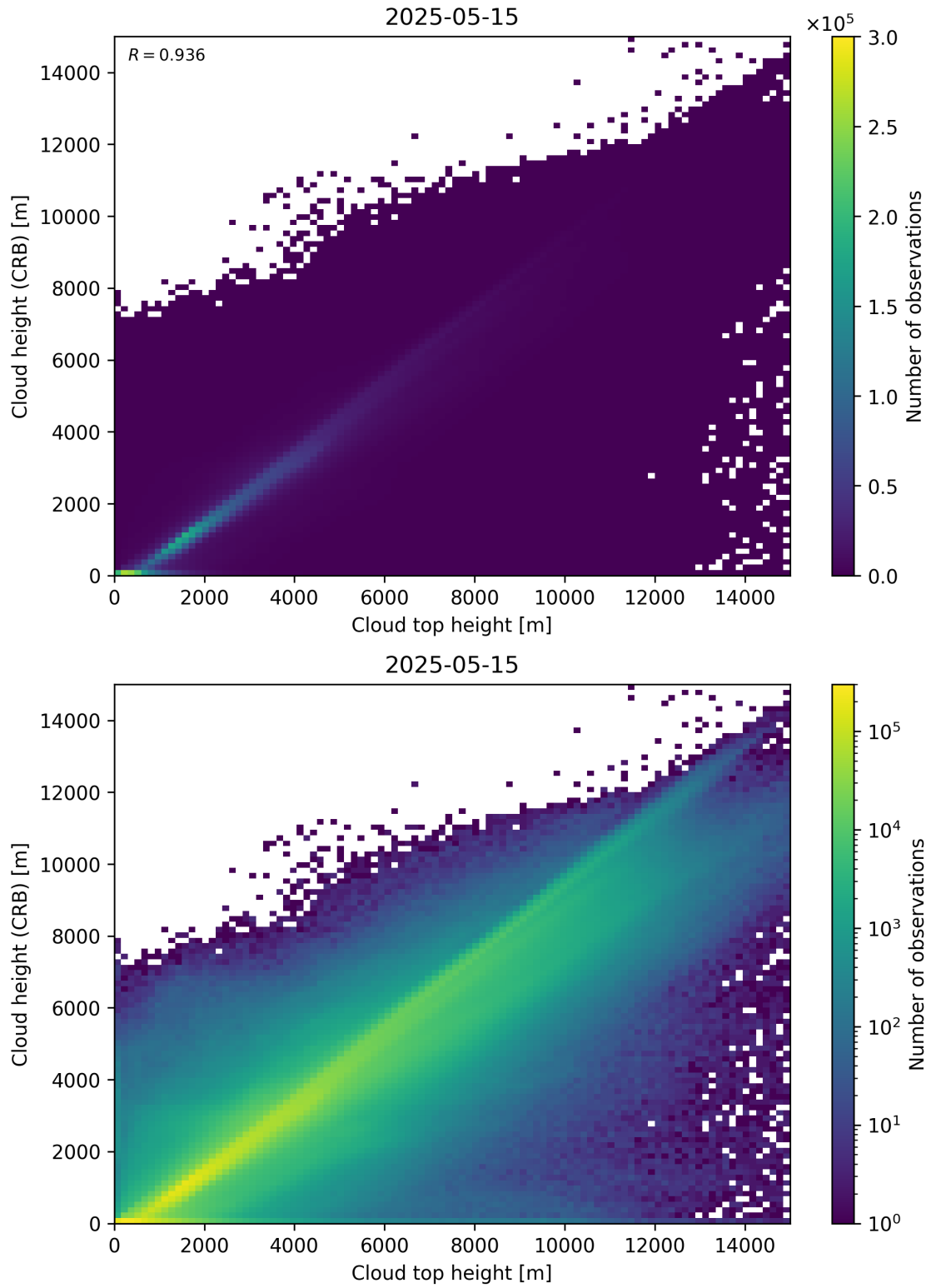
Figure 89: Scatter density plot of “Cloud top height” against “Cloud height (CRB)” for 2025-05-15 to 2025-05-16.
