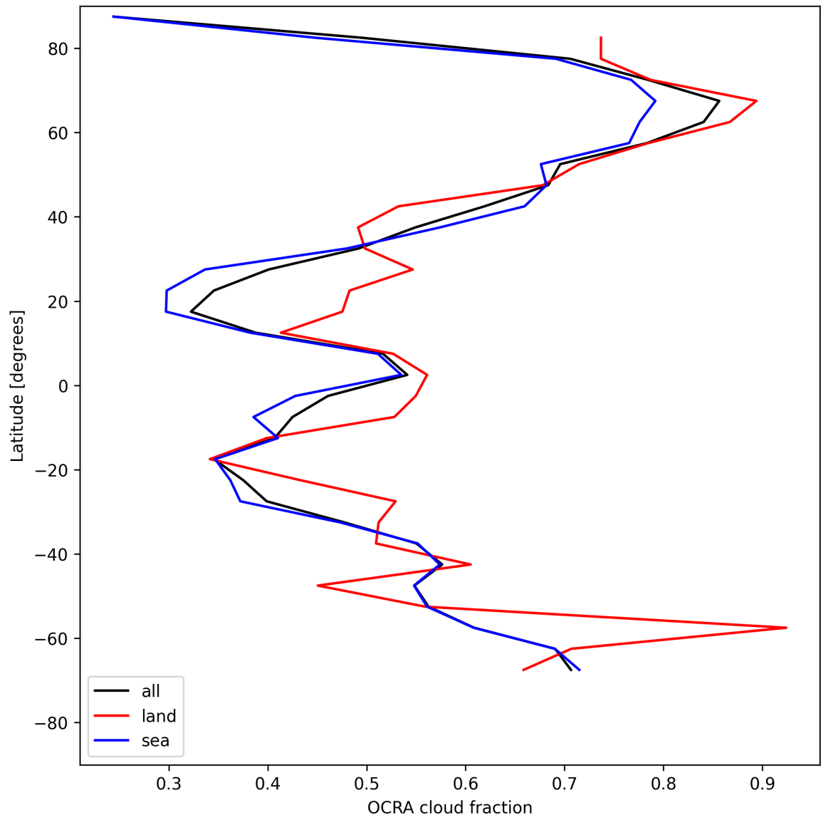
Figure 34: Zonal average of “OCRA cloud fraction” for 2025-05-15 to 2025-05-16.
