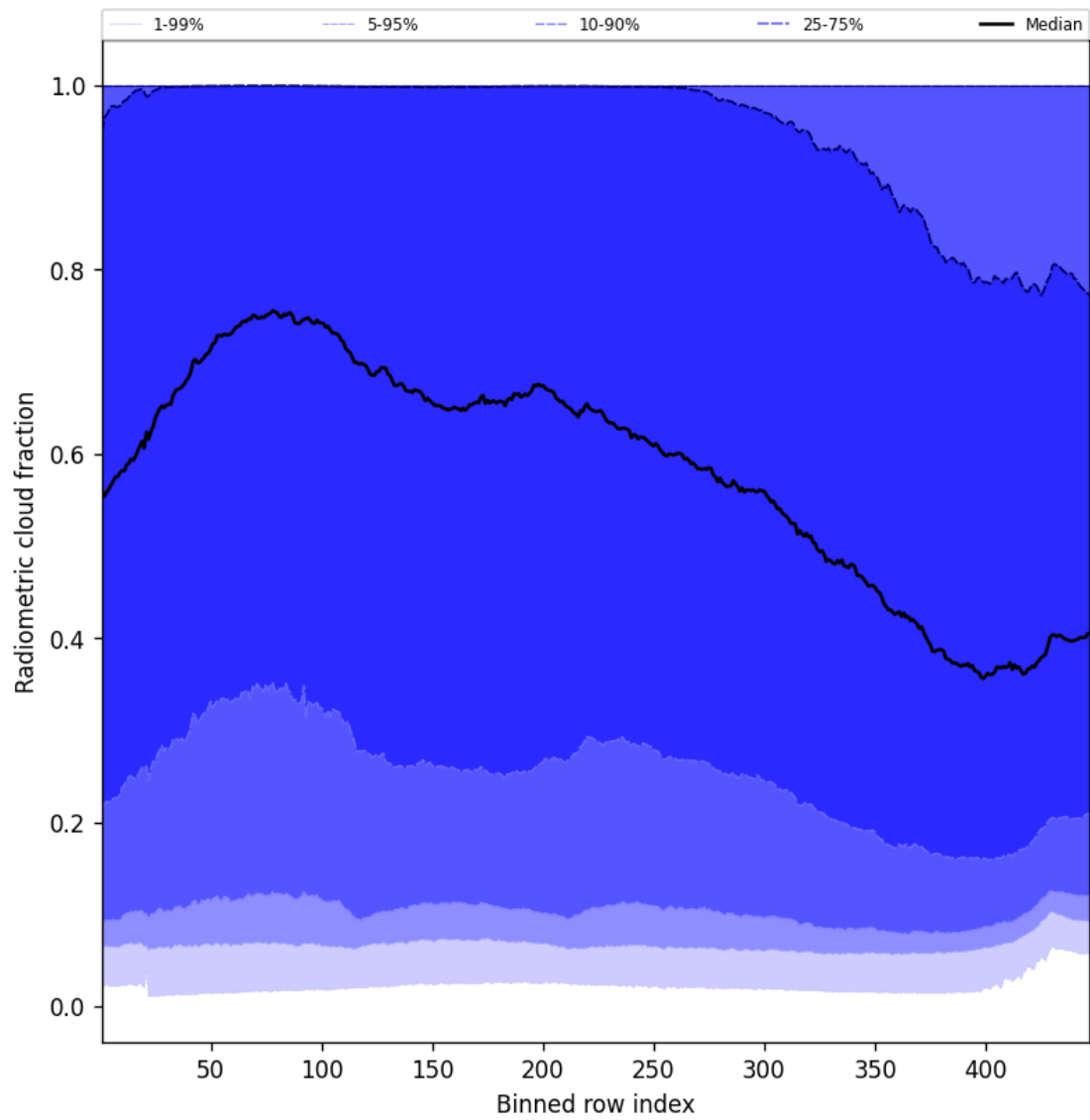
Figure 55: Along track statistics of “Radiometric cloud fraction” for 2025-05-15 to 2025-05-16
