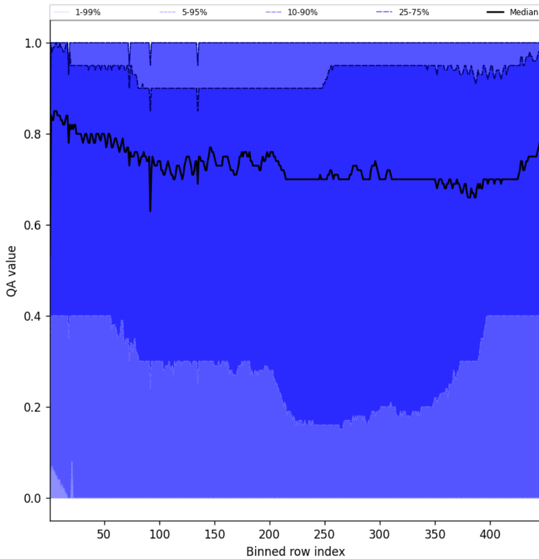
Figure 54: Along track statistics of “QA value” for 2025-05-15 to 2025-05-16
