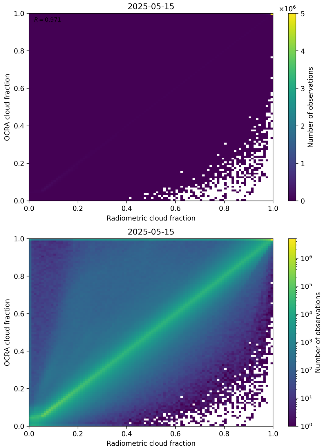
Figure 72: Scatter density plot of “Radiometric cloud fraction” against “OCRA cloud fraction” for 2025-05-15 to 2025-05-16.
