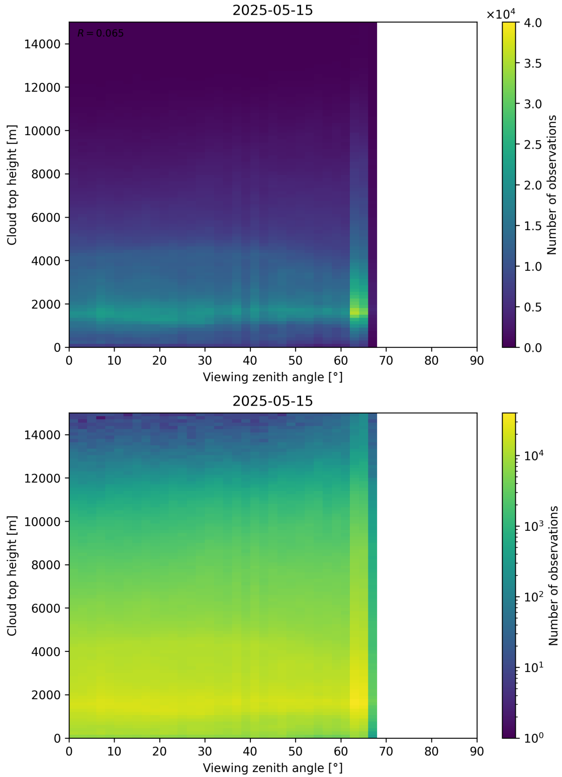
Figure 112: Scatter density plot of “Viewing zenith angle” against “Cloud top height” for 2025-05-15 to 2025-05-16.
