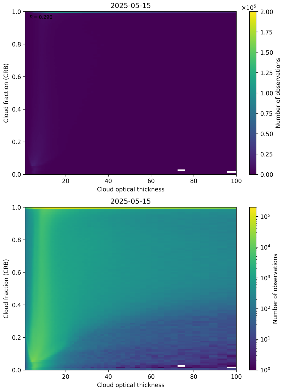
Figure 84: Scatter density plot of “Cloud optical thickness” against “Cloud fraction (CRB)” for 2025-05-15 to 2025-05-16.
