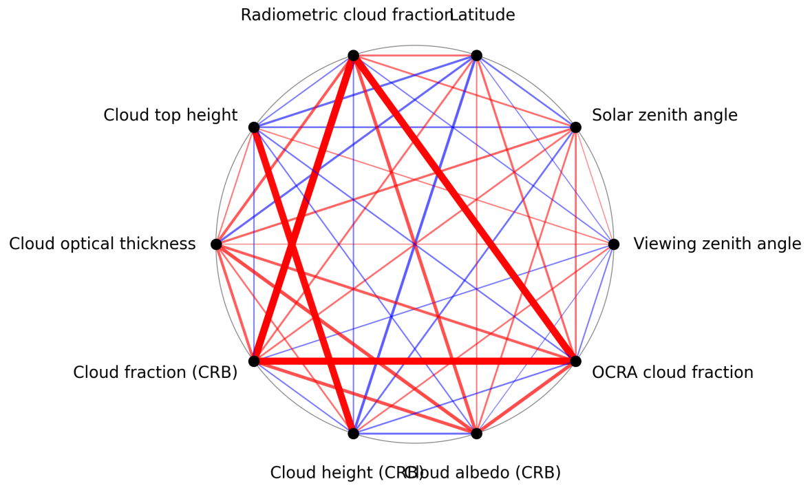
Figure 1: Map of correlation graph for 2025-05-15 to 2025-05-16.
