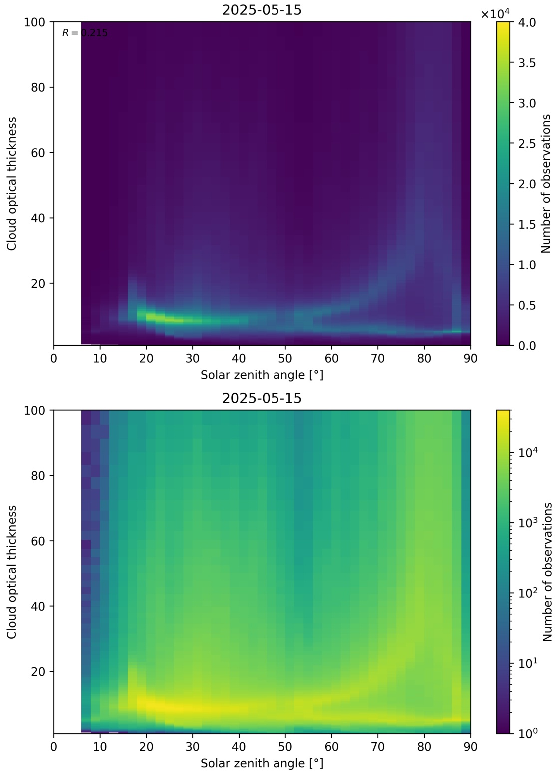
Figure 103: Scatter density plot of “Solar zenith angle” against “Cloud optical thickness” for 2025-05-15 to 2025-05-16.
