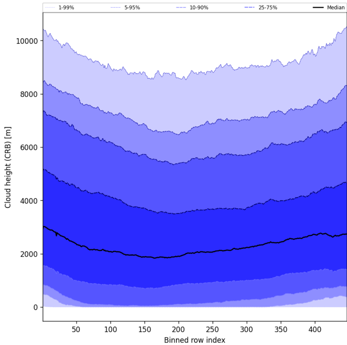
Figure 59: Along track statistics of “Cloud height (CRB)” for 2025-05-15 to 2025-05-16
