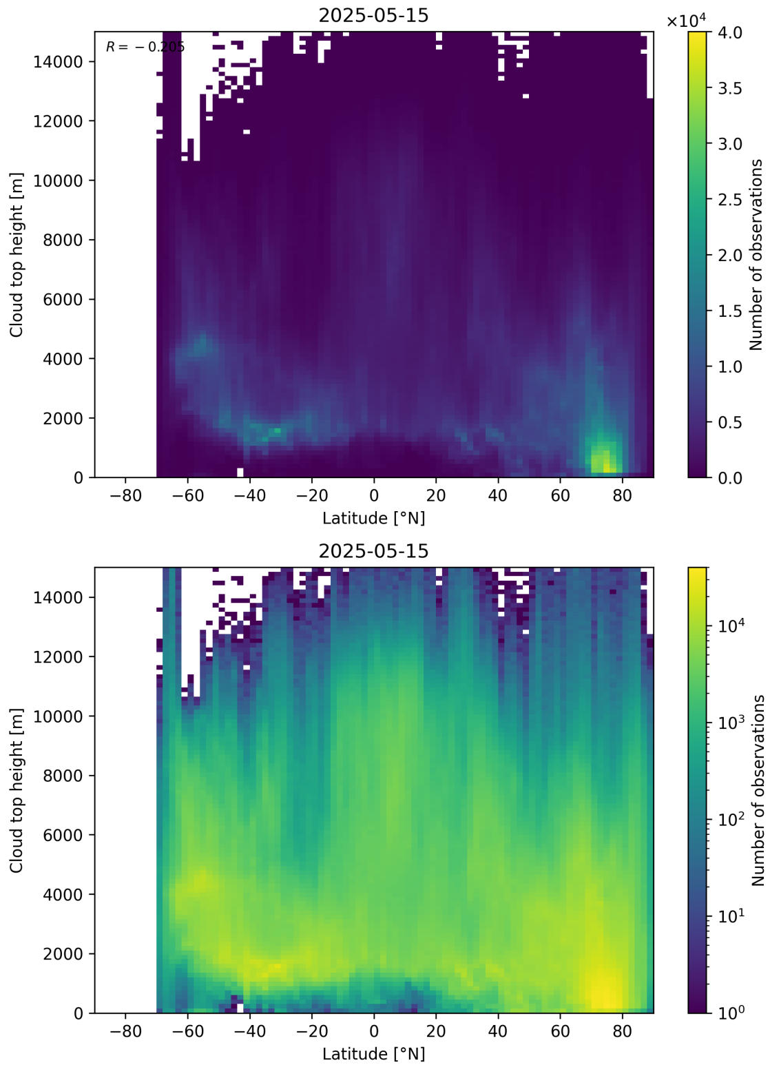
Figure 97: Scatter density plot of “Latitude” against “Cloud top height” for 2025-05-15 to 2025-05-16.
