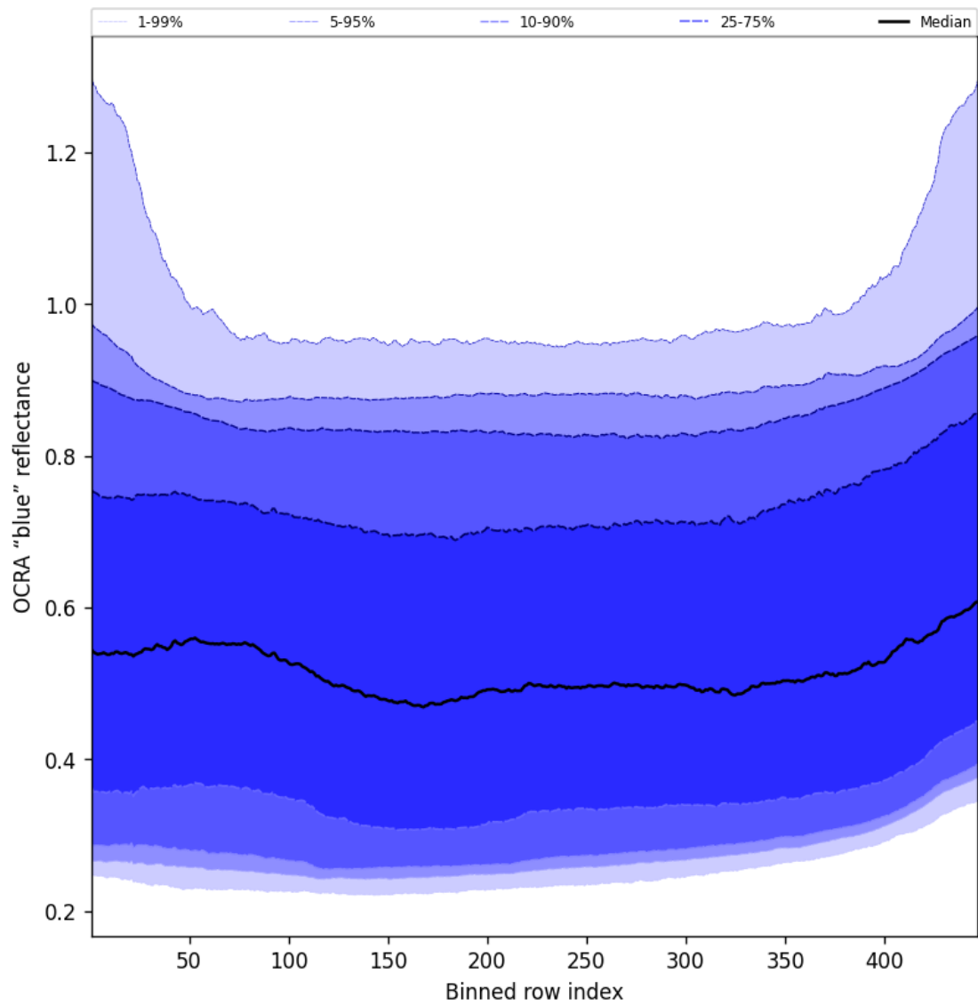
Figure 67: Along track statistics of “OCRA “blue” reflectance” for 2025-05-15 to 2025-05-16
