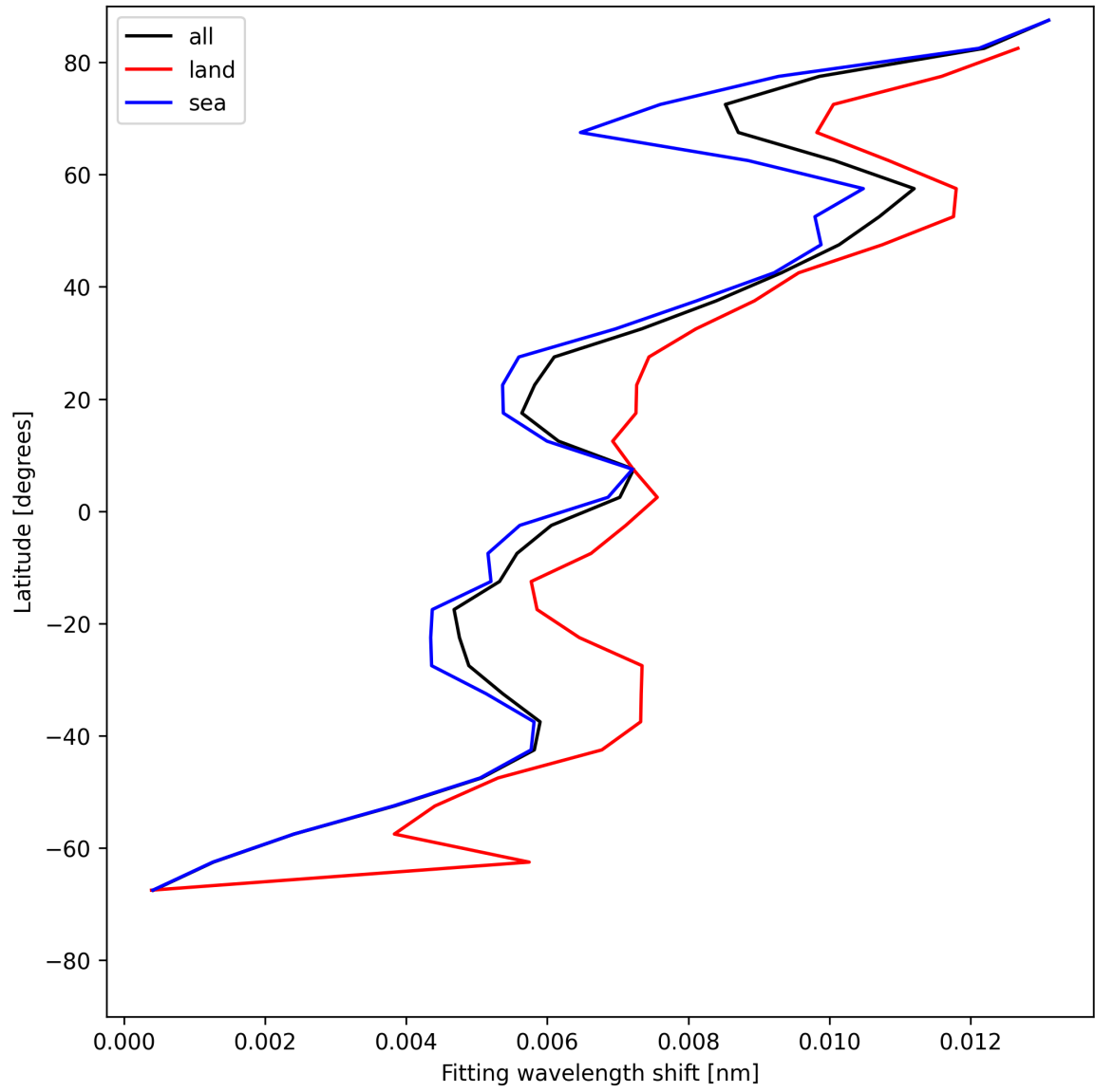
Figure 33: Zonal average of “Fitting wavelength shift” for 2025-05-15 to 2025-05-16.
