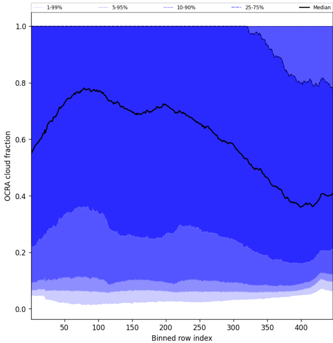
Figure 66: Along track statistics of “OCRA cloud fraction” for 2025-05-15 to 2025-05-16
