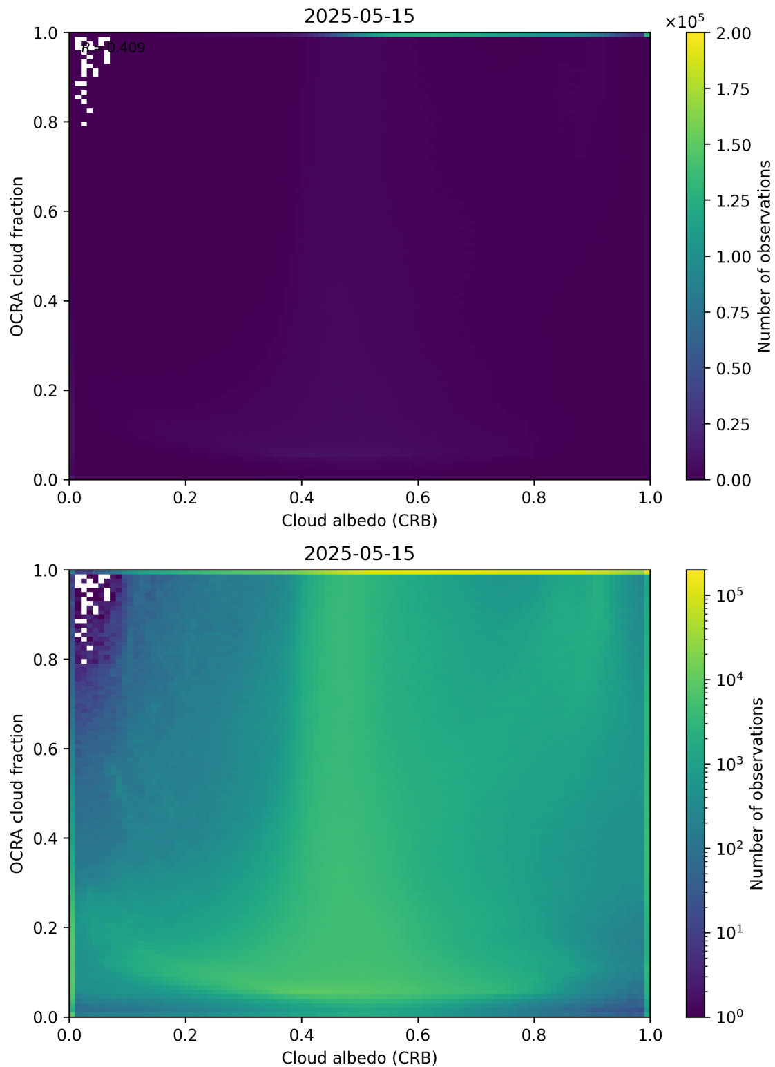
Figure 70: Scatter density plot of “Cloud albedo (CRB)” against “OCRA cloud fraction” for 2025-05-15 to 2025-05-16.
