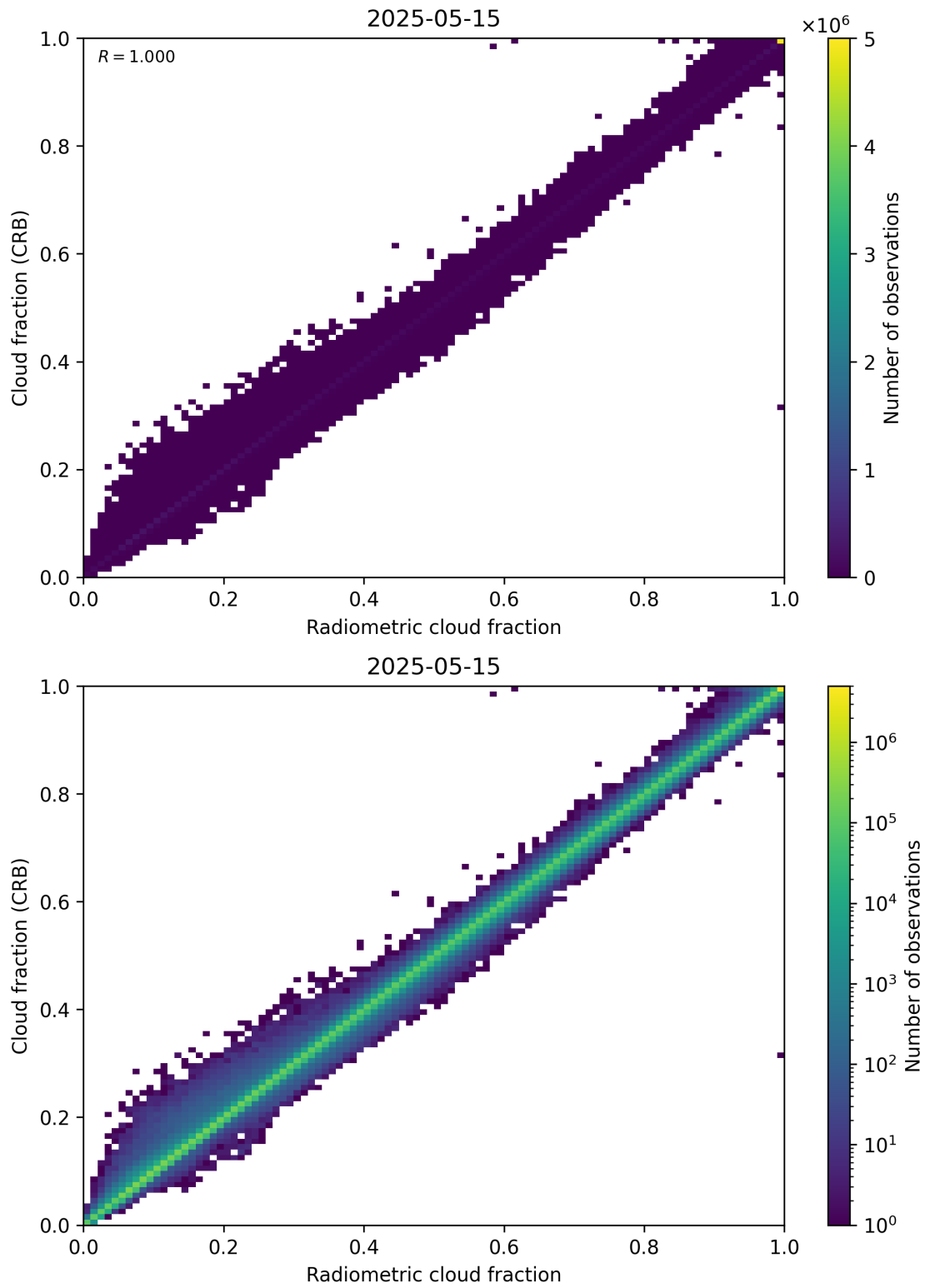
Figure 73: Scatter density plot of “Radiometric cloud fraction” against “Cloud fraction (CRB)” for 2025-05-15 to 2025-05-16.
