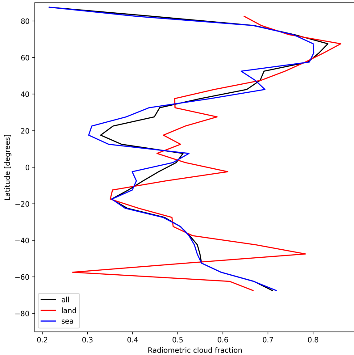
Figure 23: Zonal average of “Radiometric cloud fraction” for 2025-05-15 to 2025-05-17.
