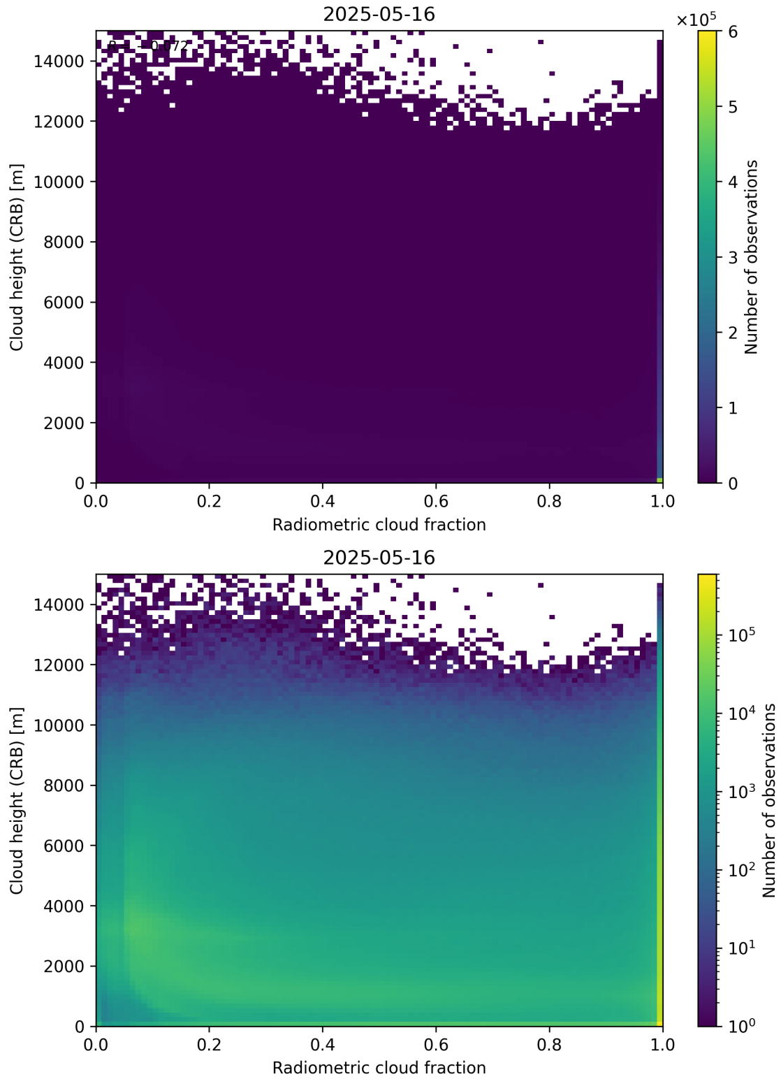
Figure 74: Scatter density plot of “Radiometric cloud fraction” against “Cloud height (CRB)” for 2025-05-15 to 2025-05-17.
