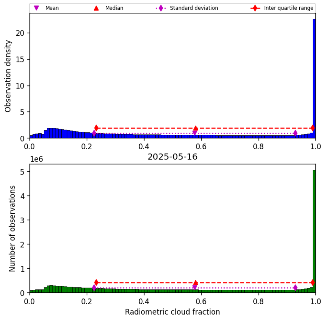
Figure 39: Histogram of “Radiometric cloud fraction” for 2025-05-15 to 2025-05-17
