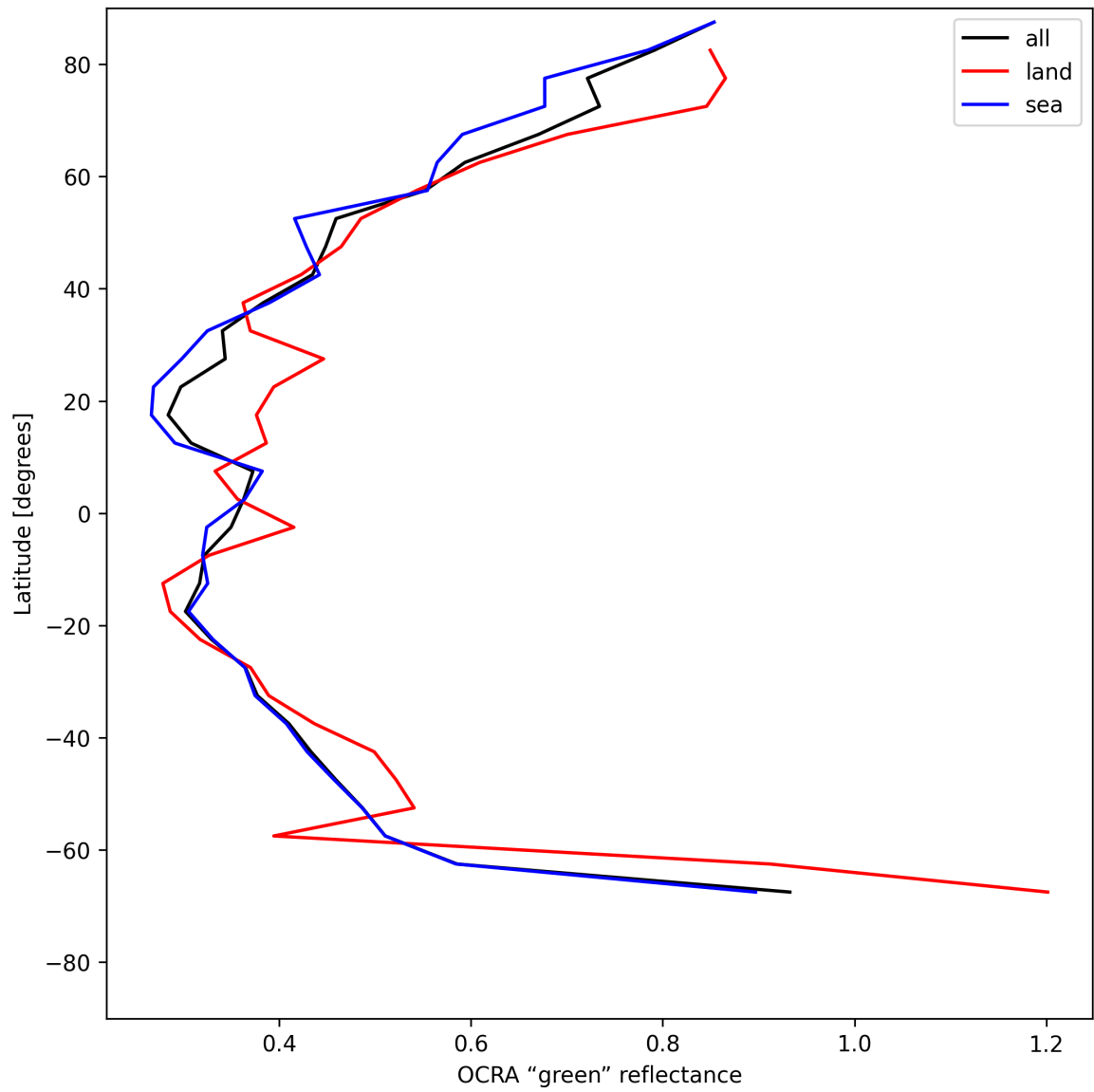
Figure 36: Zonal average of “OCRA “green” reflectance” for 2025-05-15 to 2025-05-17.
