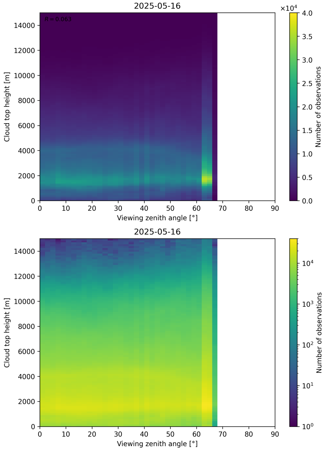
Figure 112: Scatter density plot of “Viewing zenith angle” against “Cloud top height” for 2025-05-15 to 2025-05-17.
