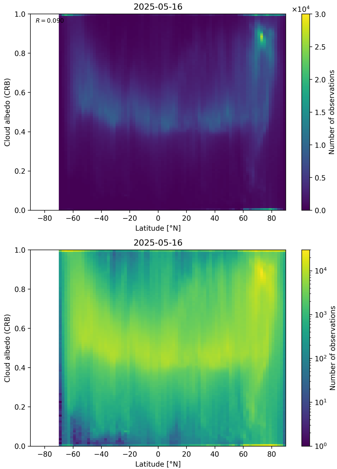
Figure 91: Scatter density plot of “Latitude” against “Cloud albedo (CRB)” for 2025-05-15 to 2025-05-17.
