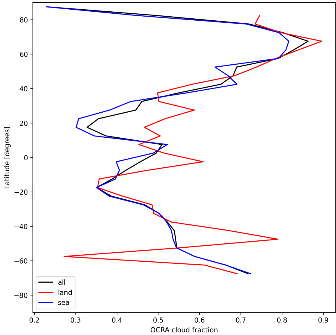
Figure 34: Zonal average of “OCRA cloud fraction” for 2025-05-15 to 2025-05-17.
