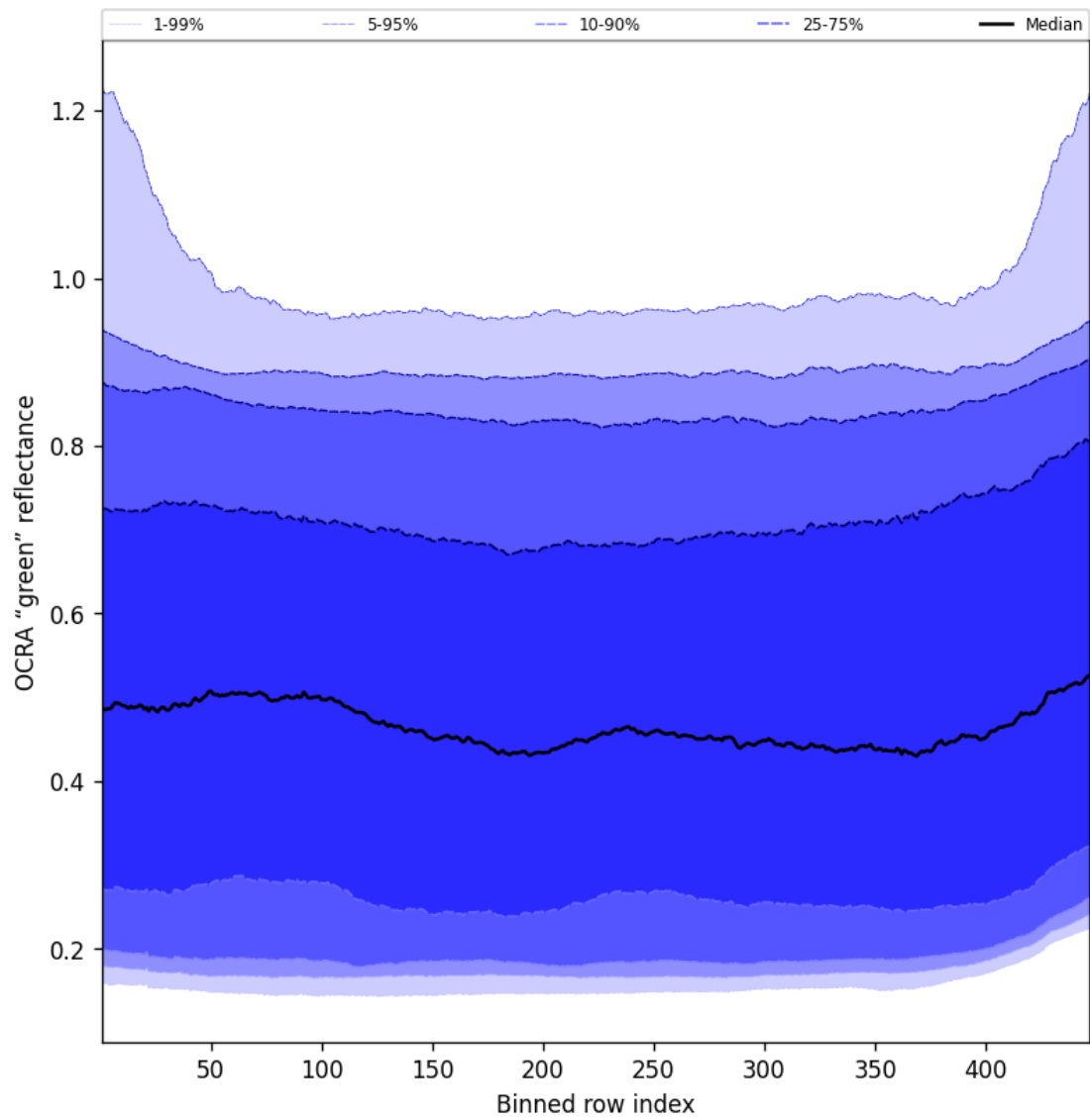
Figure 68: Along track statistics of "OCRA "green" reflectance" for 2025-05-15 to 2025-05-17
