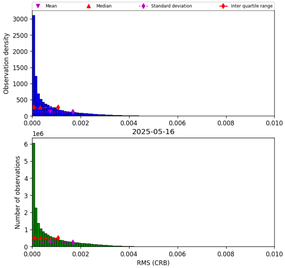
Figure 48: Histogram of “RMS (CRB)” for 2025-05-15 to 2025-05-17
