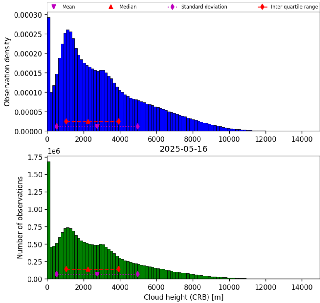
Figure 43: Histogram of “Cloud height (CRB)” for 2025-05-15 to 2025-05-17
