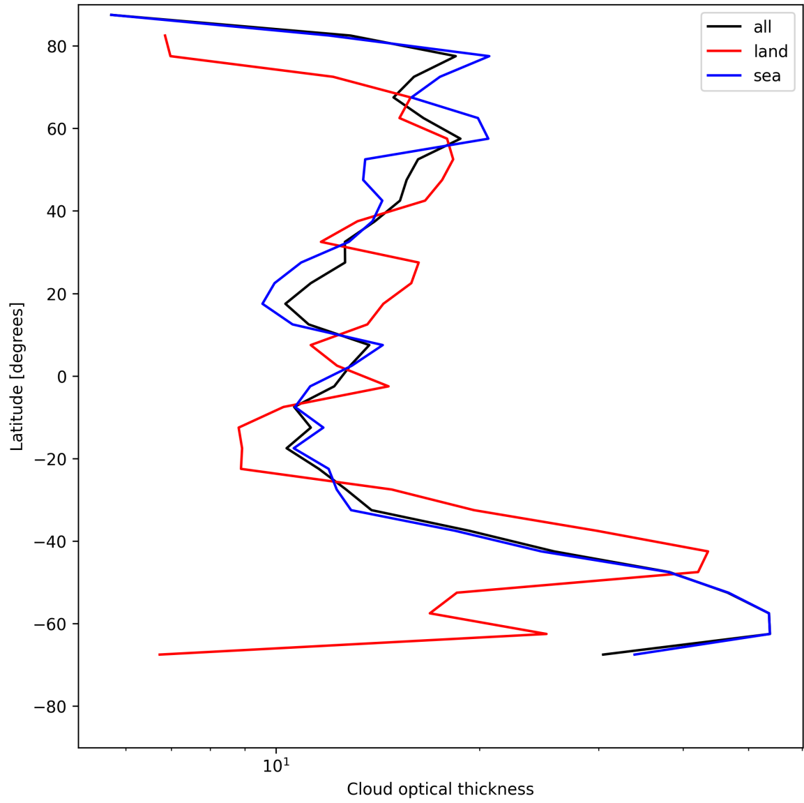
Figure 25: Zonal average of “Cloud optical thickness” for 2025-05-15 to 2025-05-17.
