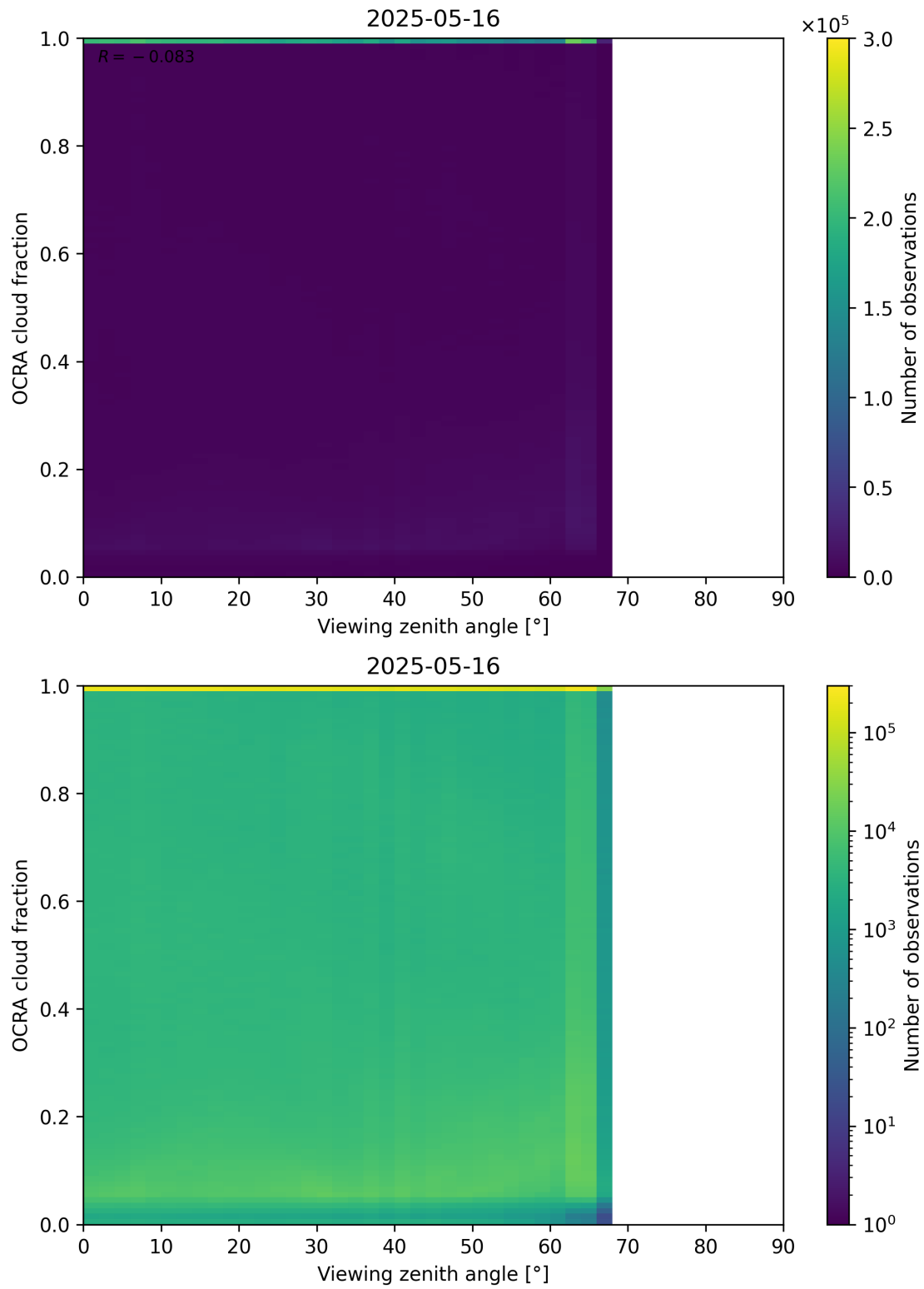
Figure 108: Scatter density plot of “Viewing zenith angle” against “OCRA cloud fraction” for 2025-05-15 to 2025-05-17.
