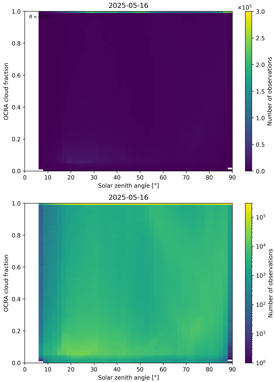
Figure 100: Scatter density plot of “Solar zenith angle” against “OCRA cloud fraction” for 2025-05-15 to 2025-05-17.
