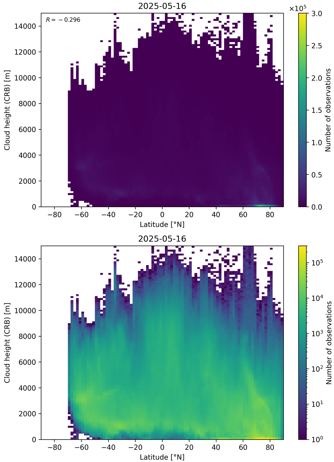
Figure 95: Scatter density plot of “Latitude” against “Cloud height (CRB)” for 2025-05-15 to 2025-05-17.
