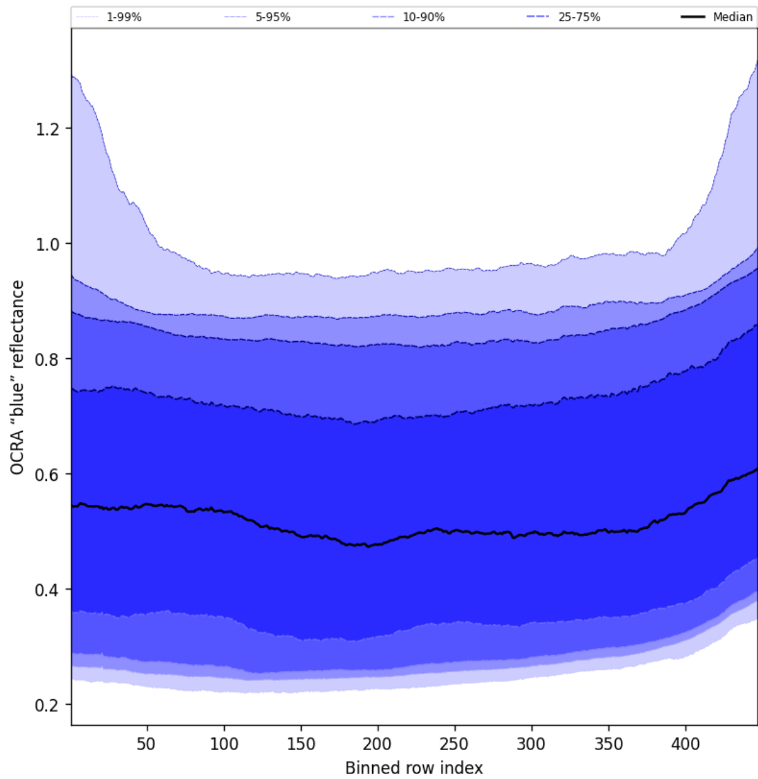
Figure 67: Along track statistics of “OCRA “blue” reflectance” for 2025-05-15 to 2025-05-17
