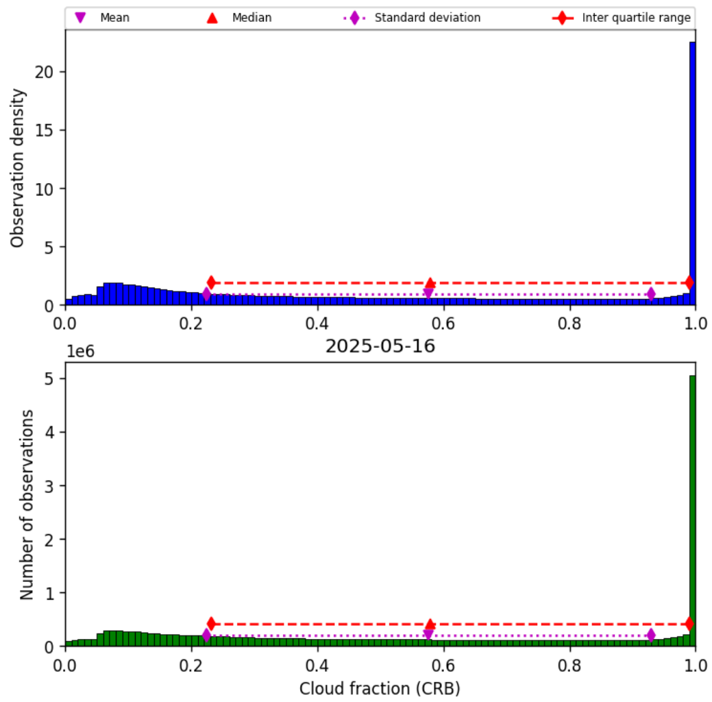
Figure 42: Histogram of “Cloud fraction (CRB)” for 2025-05-15 to 2025-05-17
