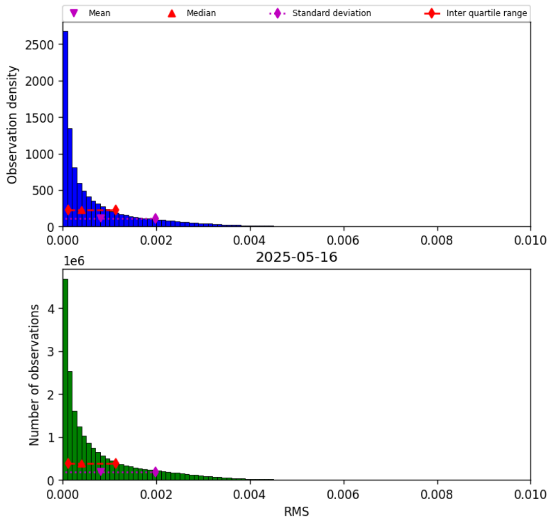
Figure 47: Histogram of “RMS” for 2025-05-15 to 2025-05-17
