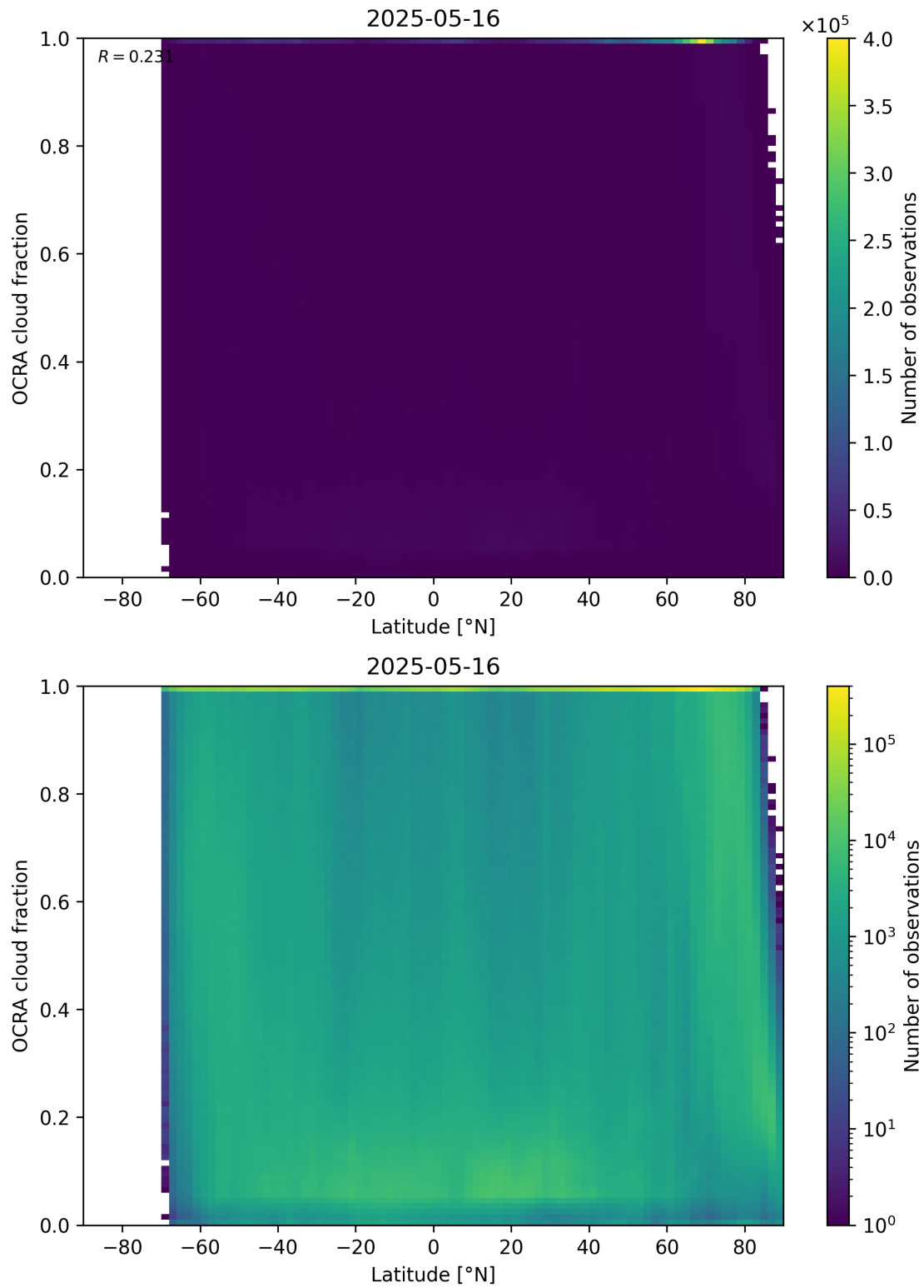
Figure 93: Scatter density plot of “Latitude” against “OCRA cloud fraction” for 2025-05-15 to 2025-05-17.
