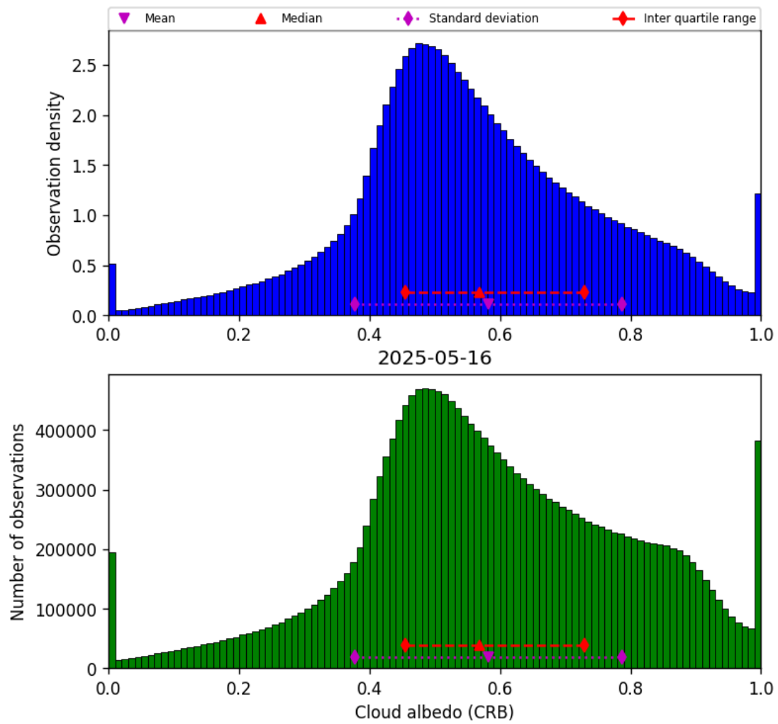
Figure 44: Histogram of “Cloud albedo (CRB)” for 2025-05-15 to 2025-05-17
