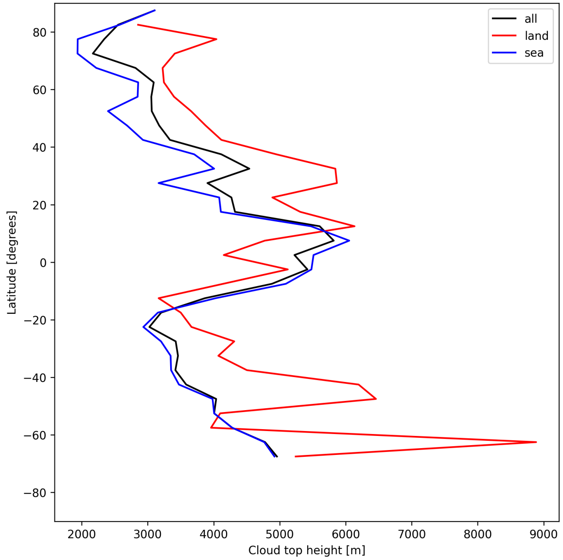
Figure 24: Zonal average of “Cloud top height” for 2025-05-15 to 2025-05-17.
