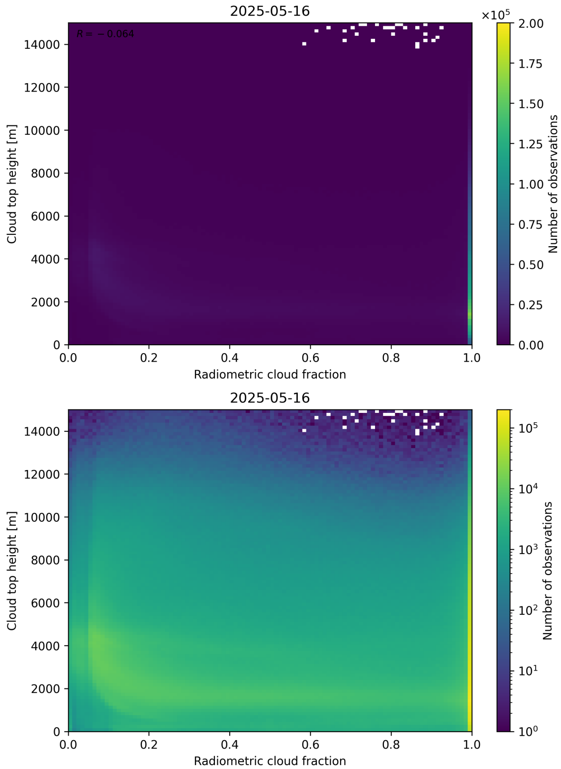
Figure 76: Scatter density plot of “Radiometric cloud fraction” against “Cloud top height” for 2025-05-15 to 2025-05-17.
