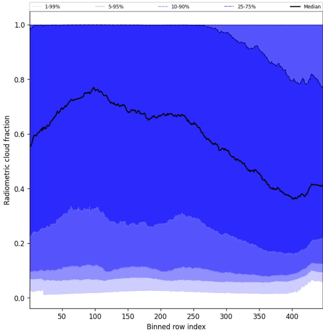
Figure 55: Along track statistics of “Radiometric cloud fraction” for 2025-05-15 to 2025-05-17
