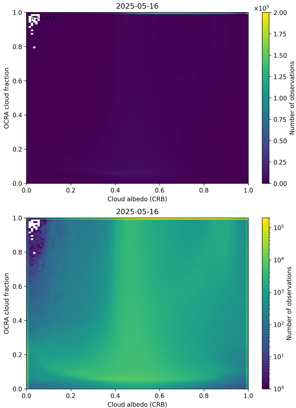
Figure 70: Scatter density plot of “Cloud albedo (CRB)” against “OCRA cloud fraction” for 2025-05-15 to 2025-05-17.
