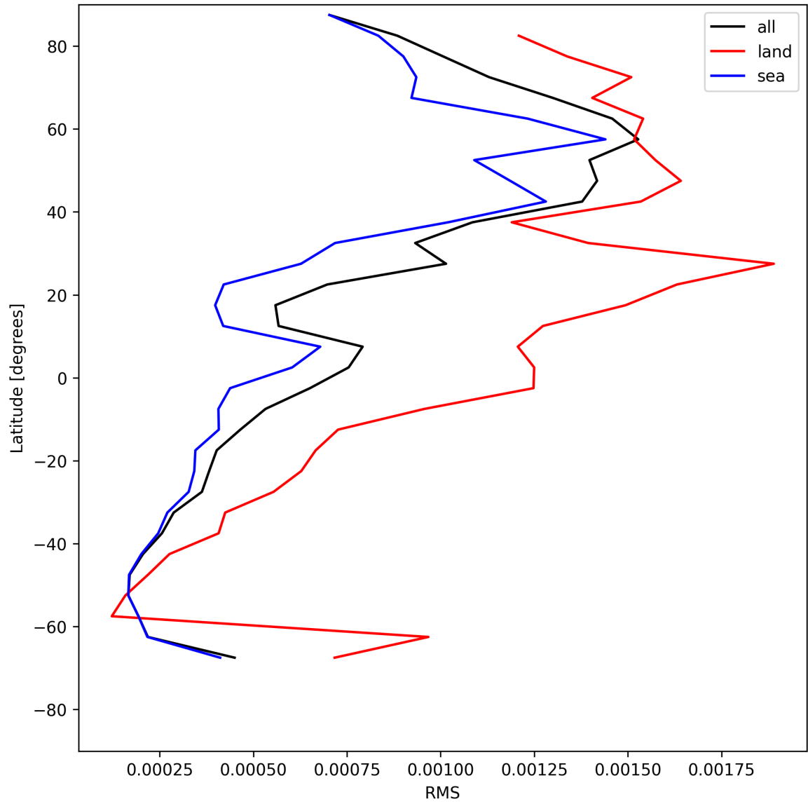
Figure 31: Zonal average of “RMS” for 2025-05-15 to 2025-05-17.
