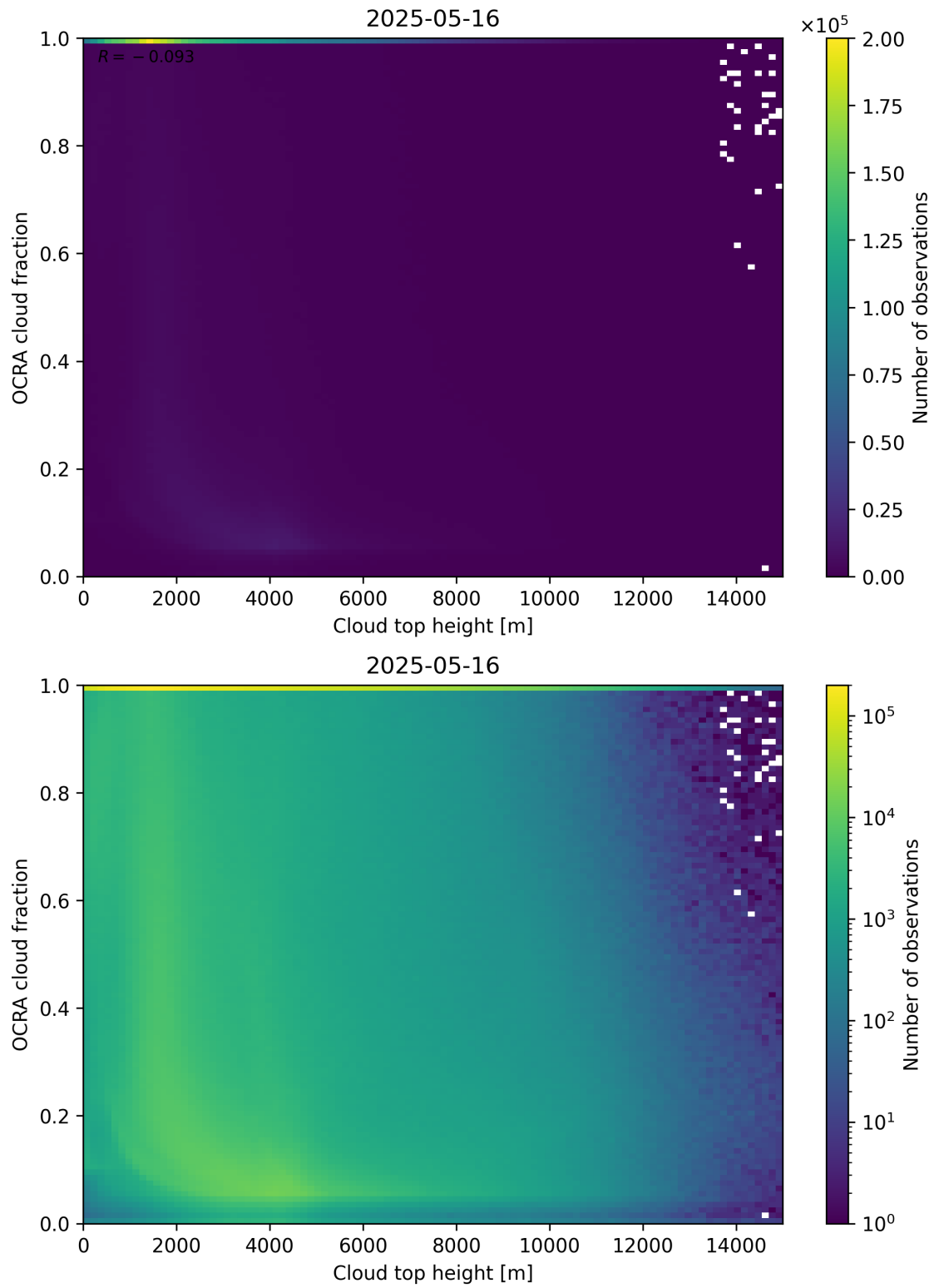
Figure 87: Scatter density plot of “Cloud top height” against “OCRA cloud fraction” for 2025-05-15 to 2025-05-17.
