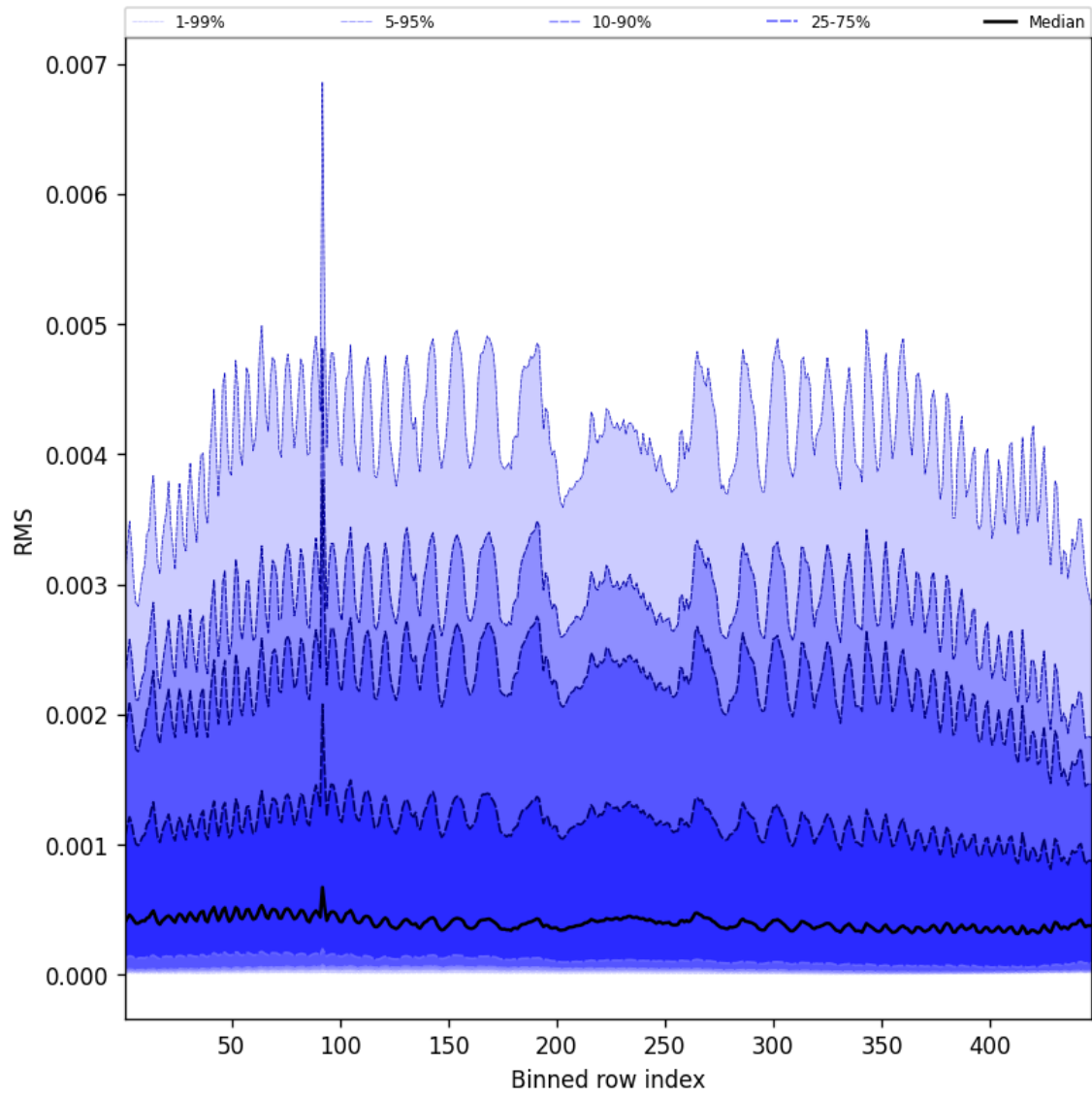
Figure 63: Along track statistics of “RMS” for 2025-05-15 to 2025-05-17
