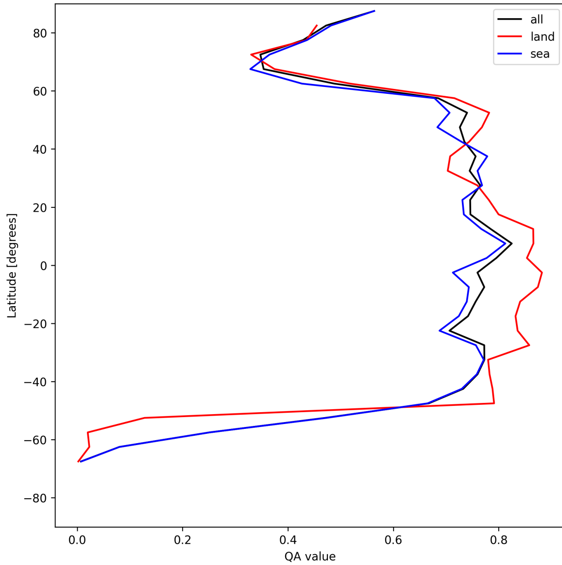
Figure 22: Zonal average of “QA value” for 2025-05-15 to 2025-05-17.
