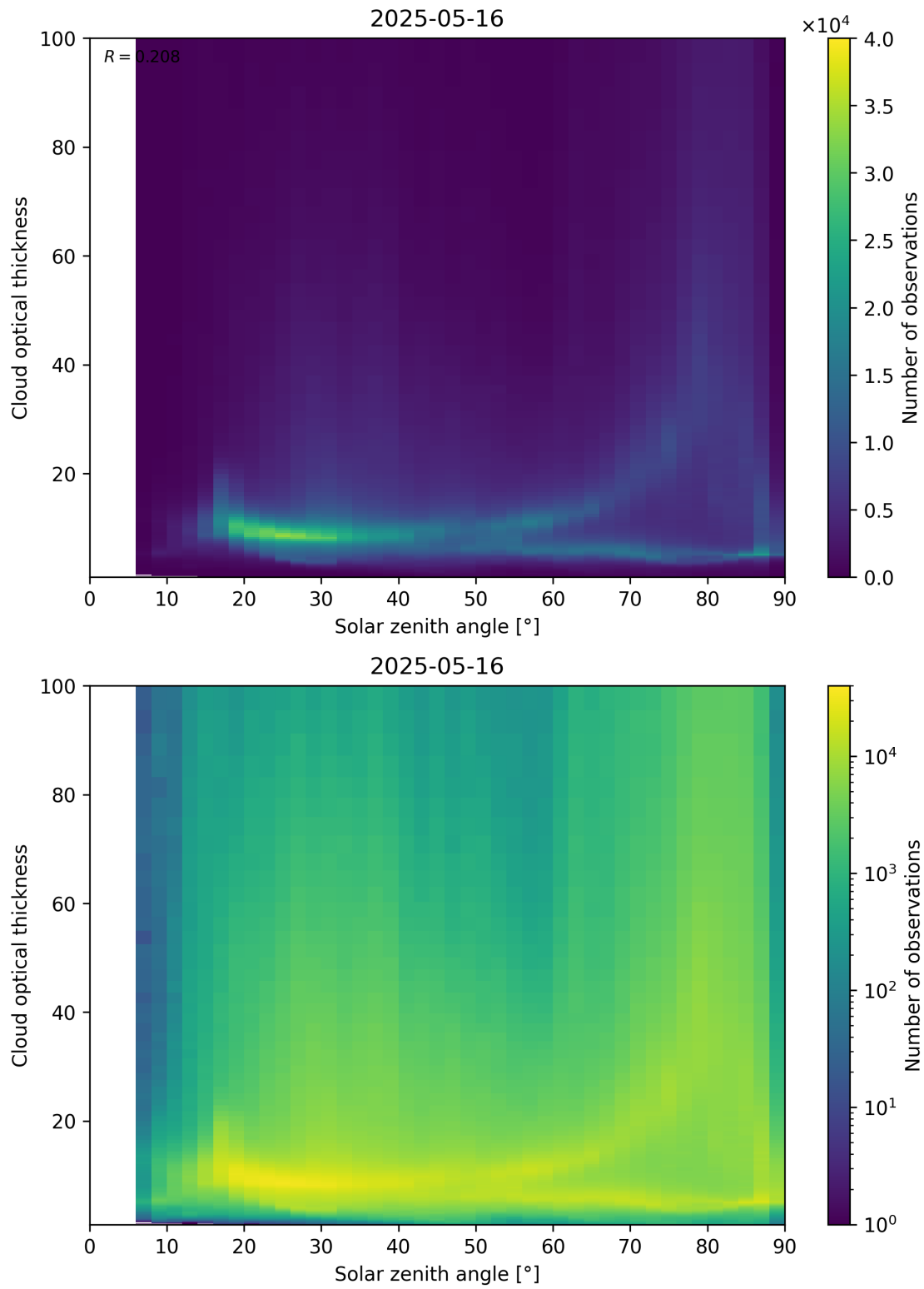
Figure 103: Scatter density plot of “Solar zenith angle” against “Cloud optical thickness” for 2025-05-15 to 2025-05-17.
