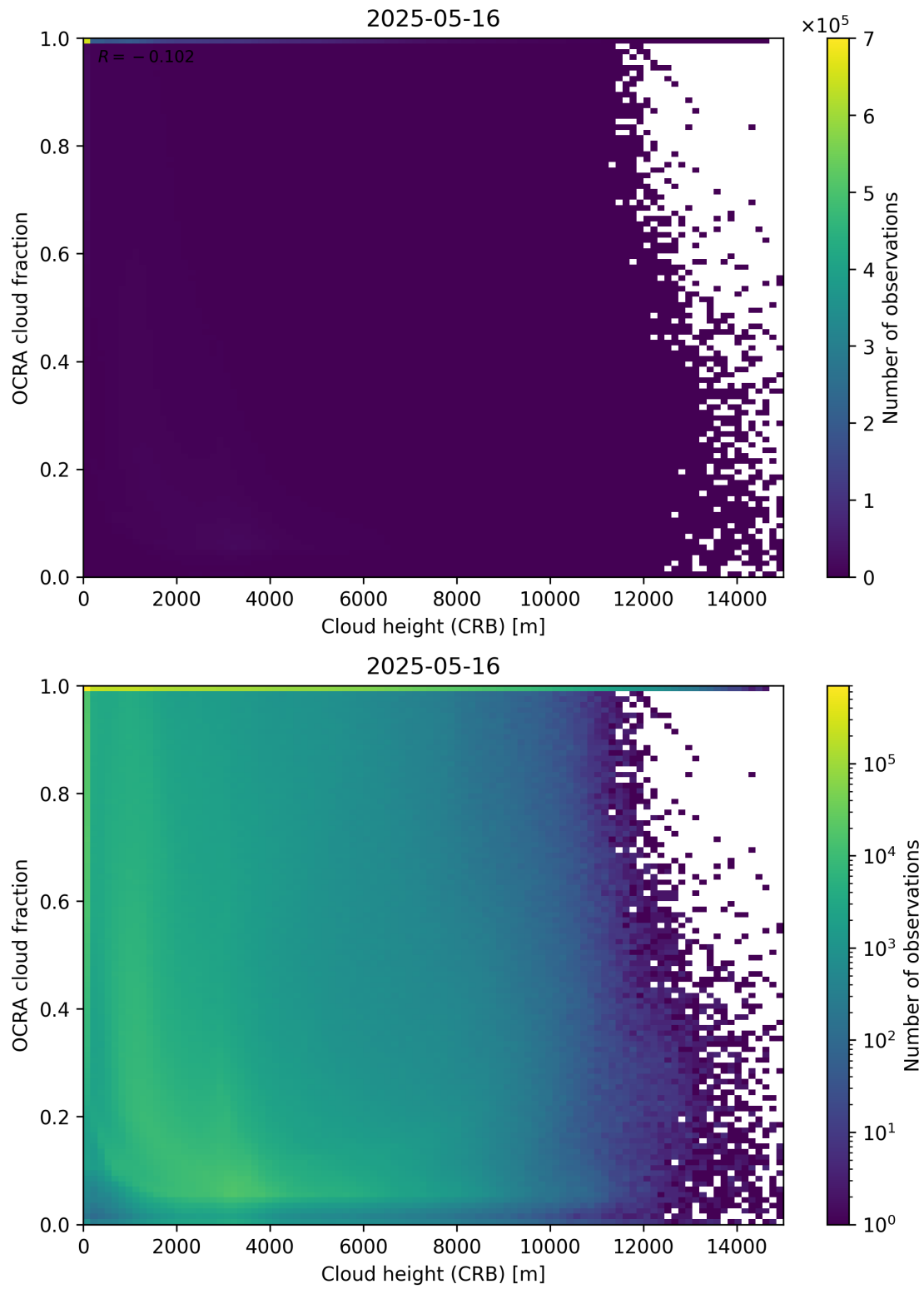
Figure 81: Scatter density plot of “Cloud height (CRB)” against “OCRA cloud fraction” for 2025-05-15 to 2025-05-17.
