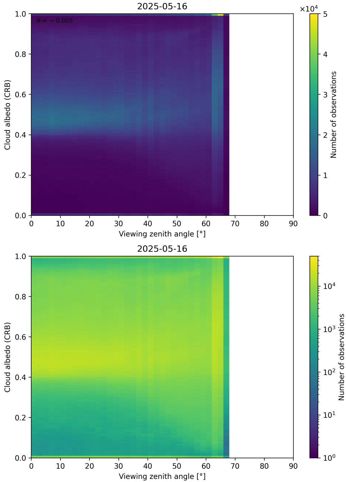
Figure 106: Scatter density plot of “Viewing zenith angle” against “Cloud albedo (CRB)” for 2025-05-15 to 2025-05-17.
