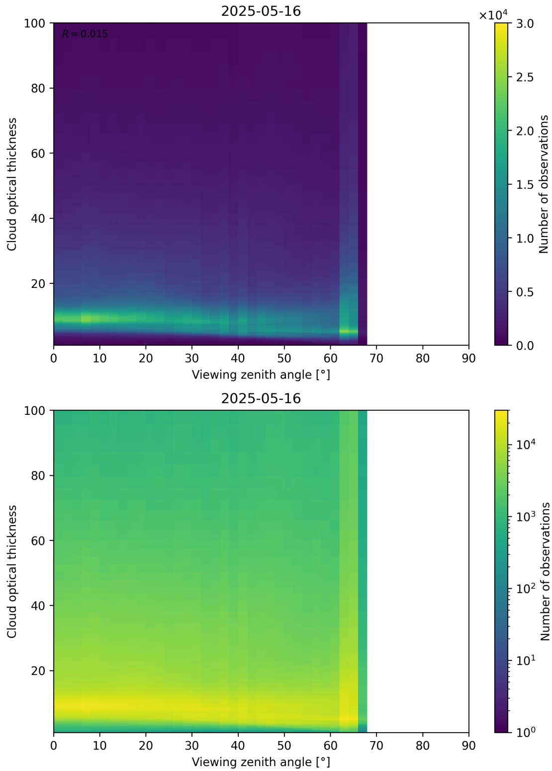
Figure 111: Scatter density plot of “Viewing zenith angle” against “Cloud optical thickness” for 2025-05-15 to 2025-05-17.
