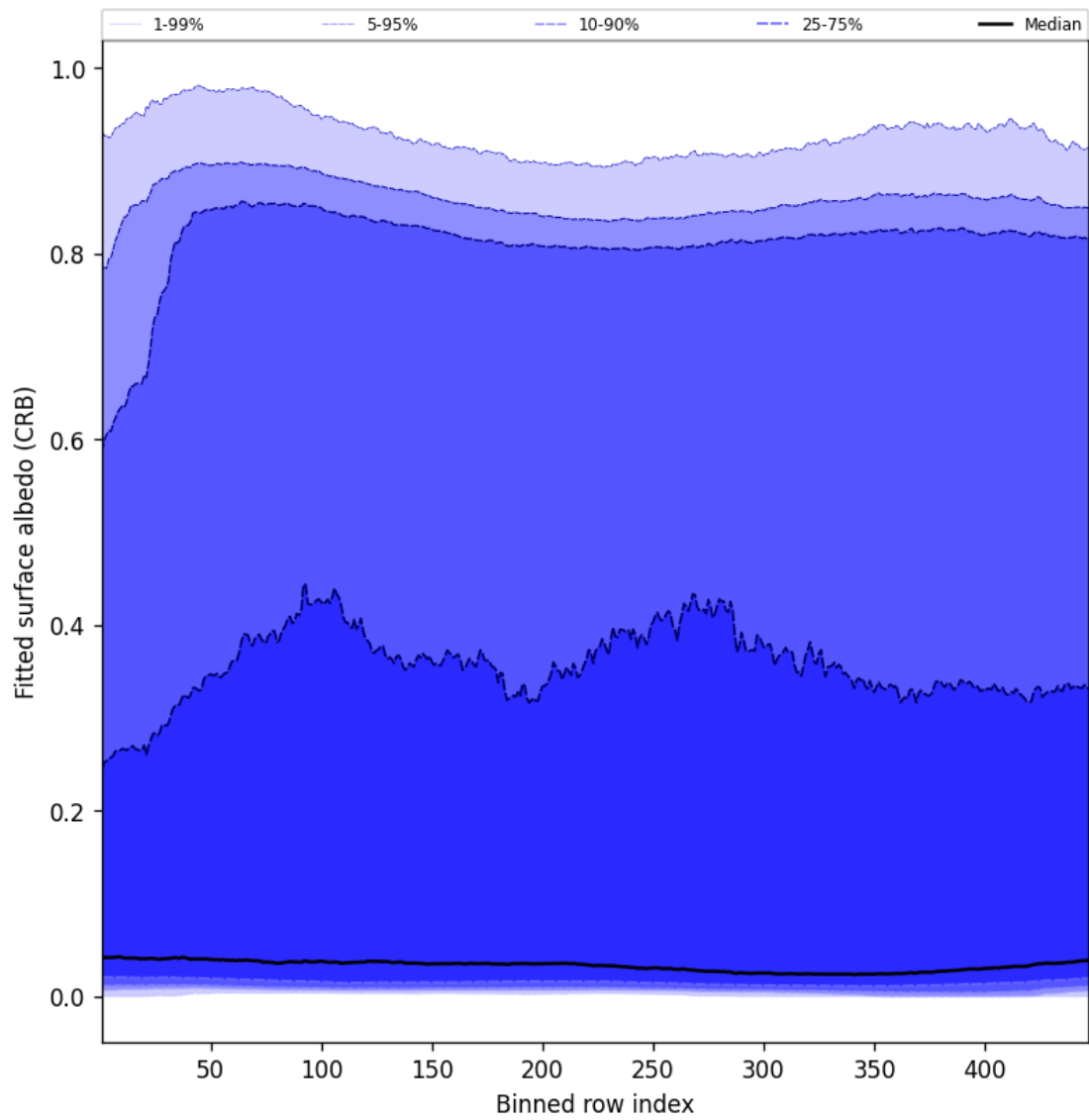
Figure 62: Along track statistics of “Fitted surface albedo (CRB)” for 2025-05-15 to 2025-05-17
