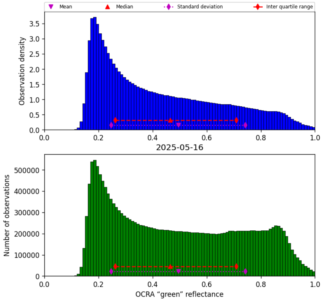
Figure 52: Histogram of “OCRA “green” reflectance” for 2025-05-15 to 2025-05-17
