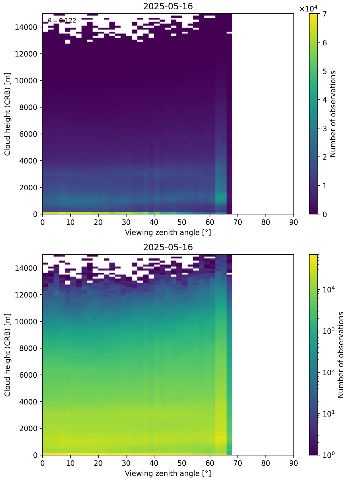
Figure 110: Scatter density plot of “Viewing zenith angle” against “Cloud height (CRB)” for 2025-05-15 to 2025-05-17.
