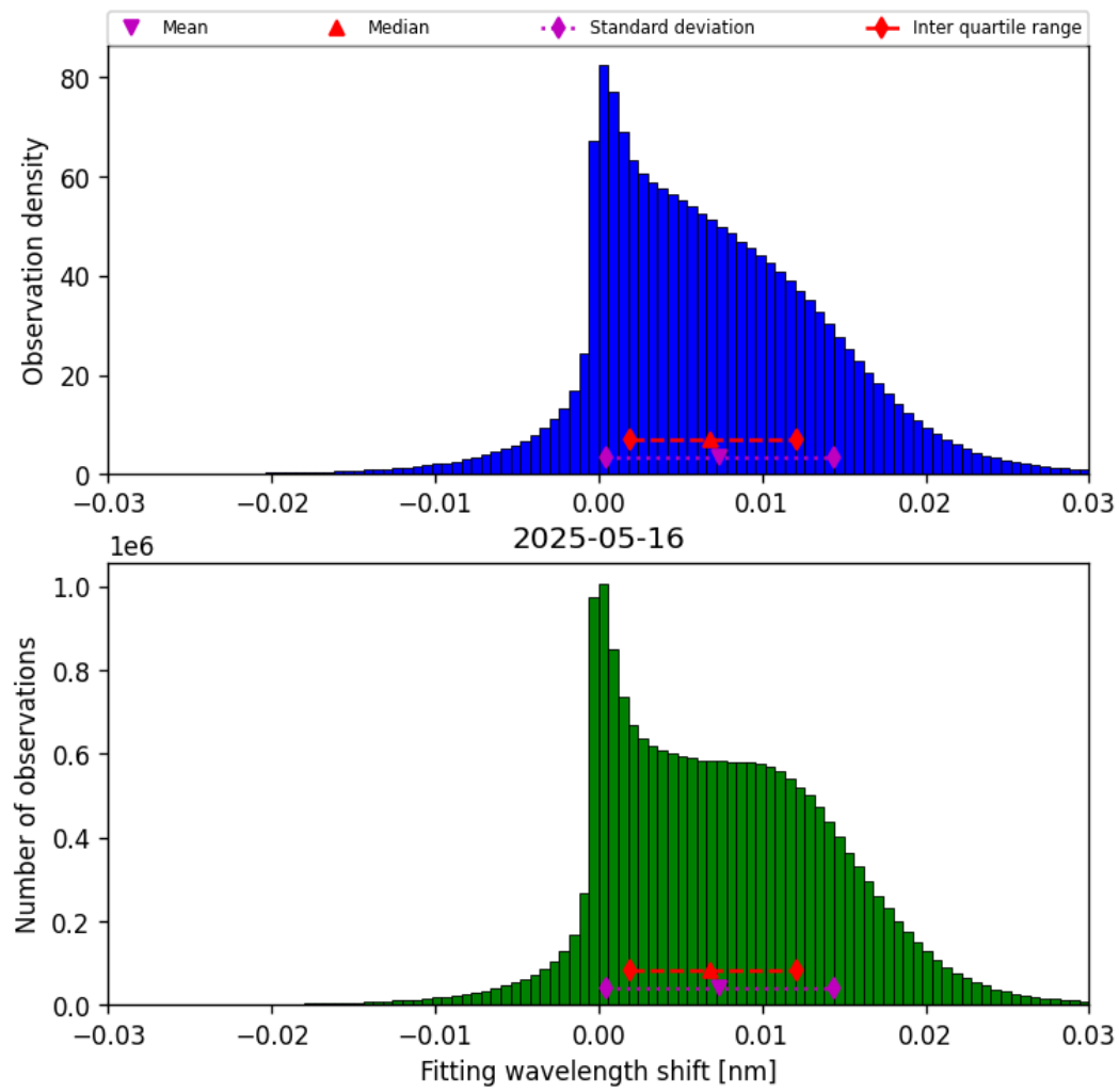
Figure 49: Histogram of “Fitting wavelength shift” for 2025-05-15 to 2025-05-17
