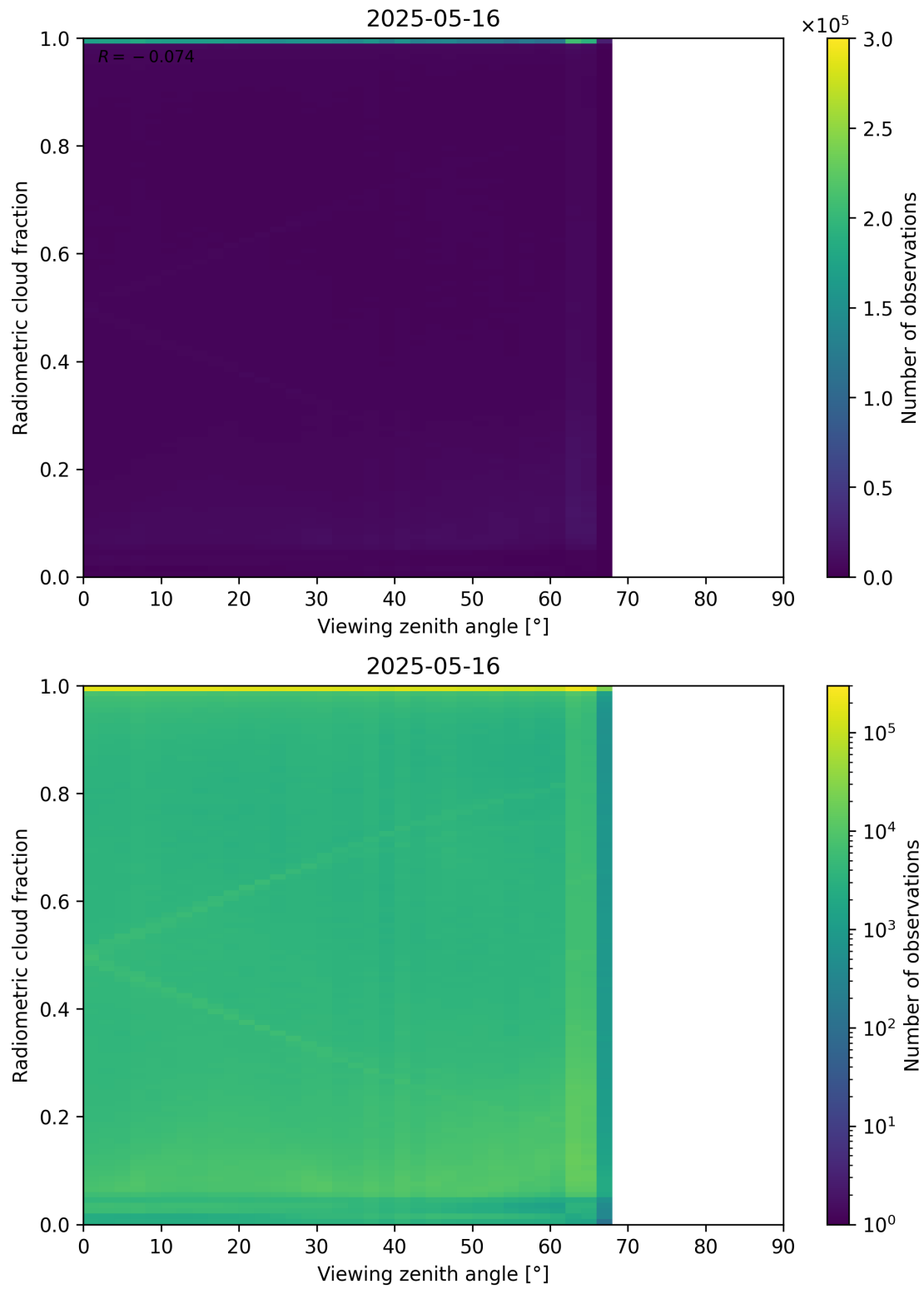
Figure 107: Scatter density plot of “Viewing zenith angle” against “Radiometric cloud fraction” for 2025-05-15 to 2025-05-17.
