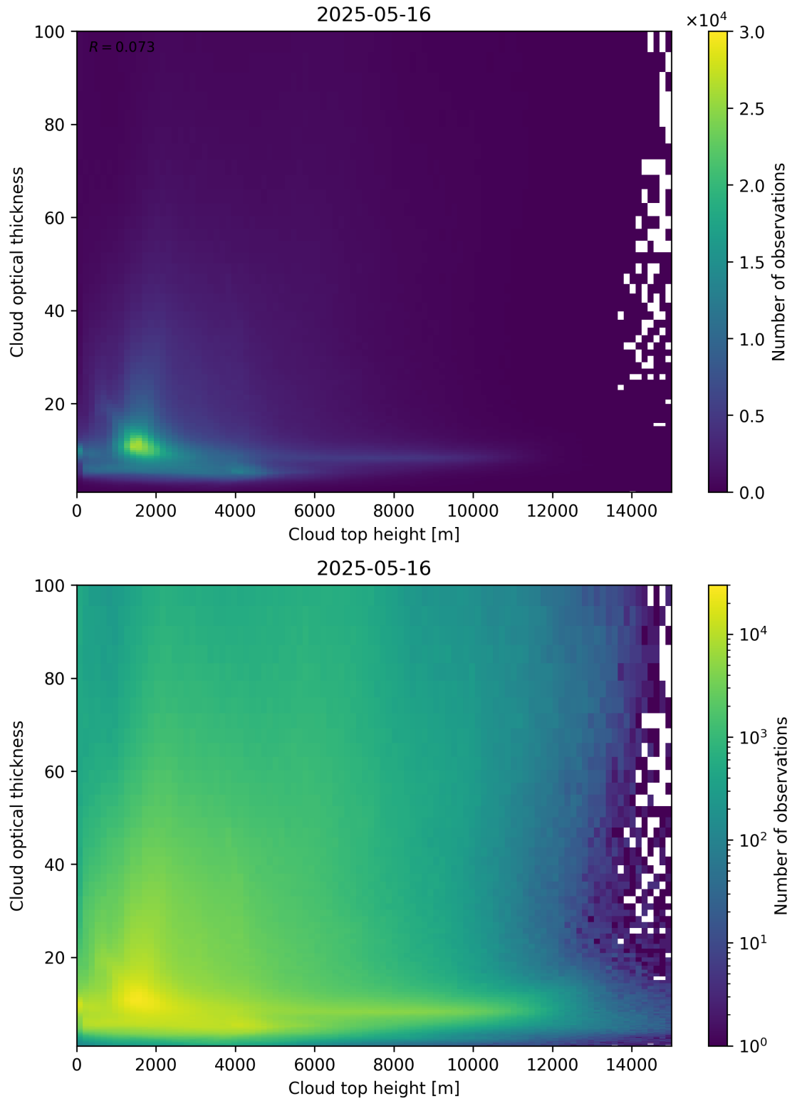
Figure 90: Scatter density plot of “Cloud top height” against “Cloud optical thickness” for 2025-05-15 to 2025-05-17.
