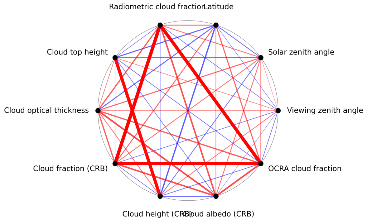
Figure 1: Map of correlation graph for 2025-05-15 to 2025-05-17.
