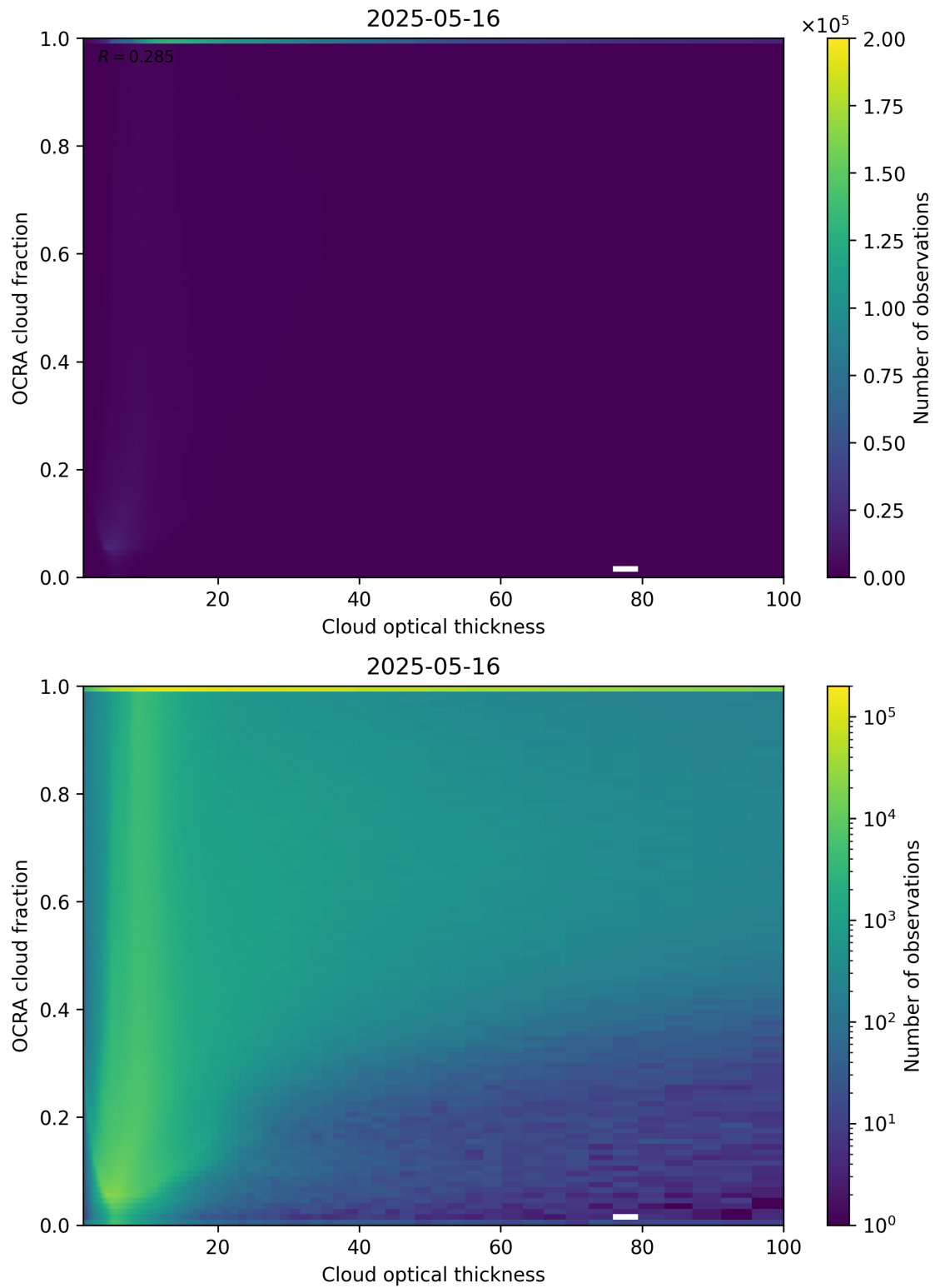
Figure 83: Scatter density plot of “Cloud optical thickness” against “OCRA cloud fraction” for 2025-05-15 to 2025-05-17.
