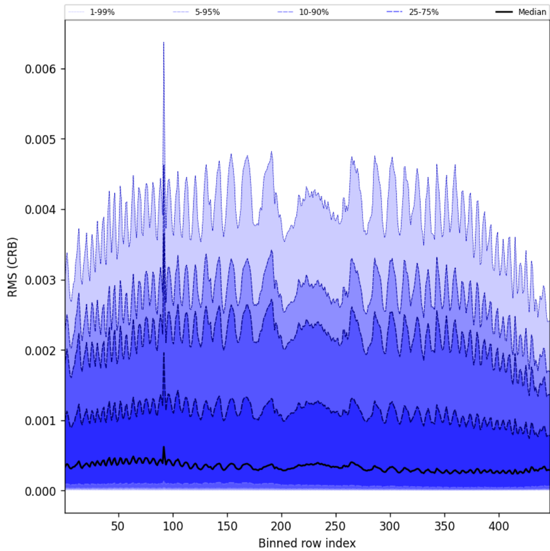
Figure 64: Along track statistics of “RMS (CRB)” for 2025-05-15 to 2025-05-17
