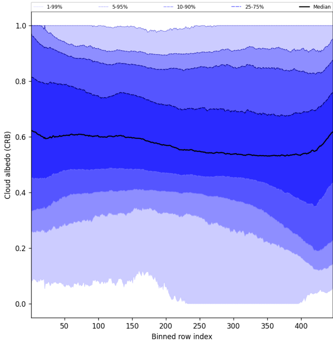
Figure 60: Along track statistics of “Cloud albedo (CRB)” for 2025-05-15 to 2025-05-17
