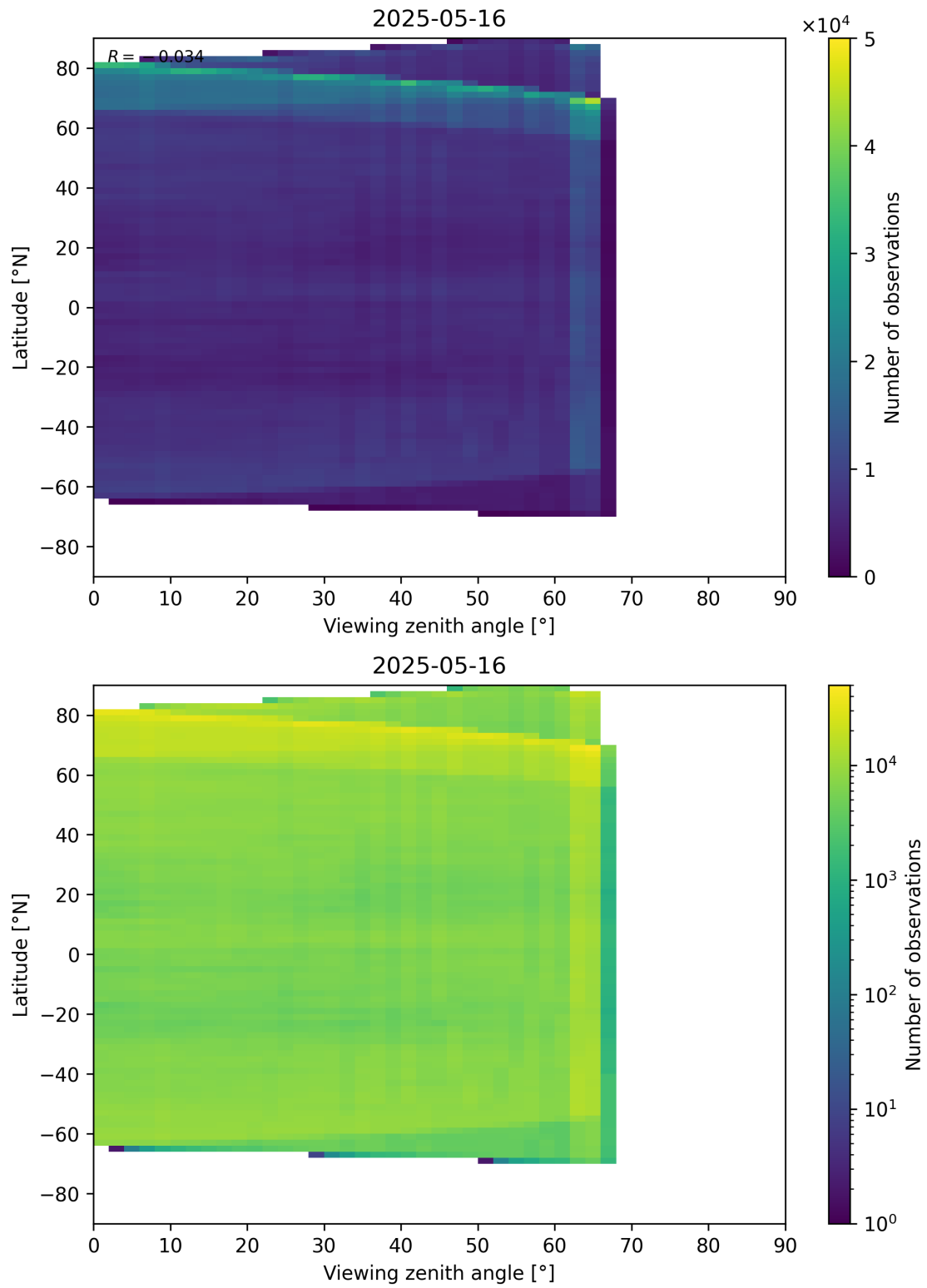
Figure 113: Scatter density plot of “Viewing zenith angle” against “Latitude” for 2025-05-15 to 2025-05-17.
