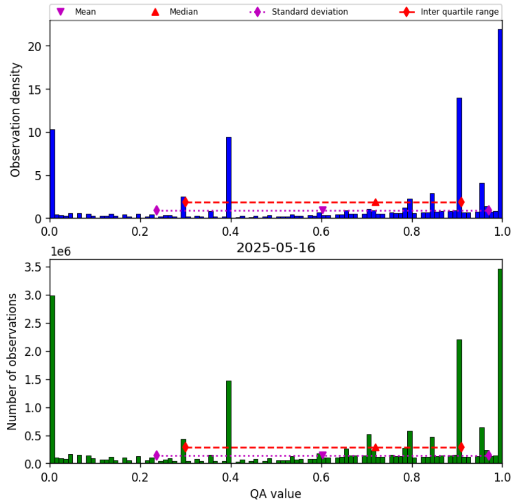
Figure 38: Histogram of “QA value” for 2025-05-15 to 2025-05-17
