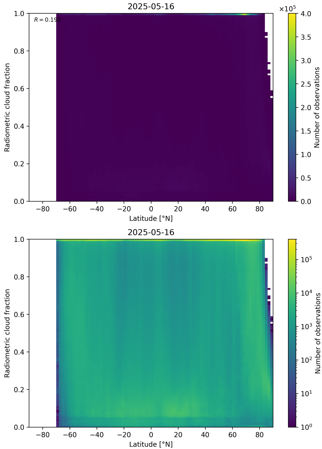
Figure 92: Scatter density plot of “Latitude” against “Radiometric cloud fraction” for 2025-05-15 to 2025-05-17.
