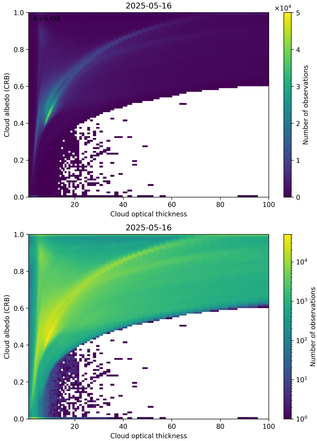
Figure 82: Scatter density plot of “Cloud optical thickness” against “Cloud albedo (CRB)” for 2025-05-15 to 2025-05-17.
