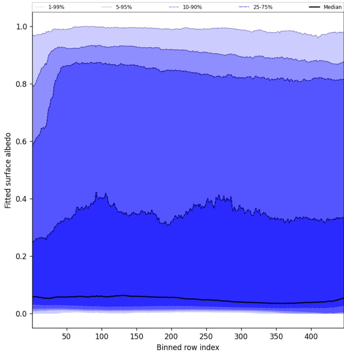
Figure 61: Along track statistics of “Fitted surface albedo” for 2025-05-15 to 2025-05-17
