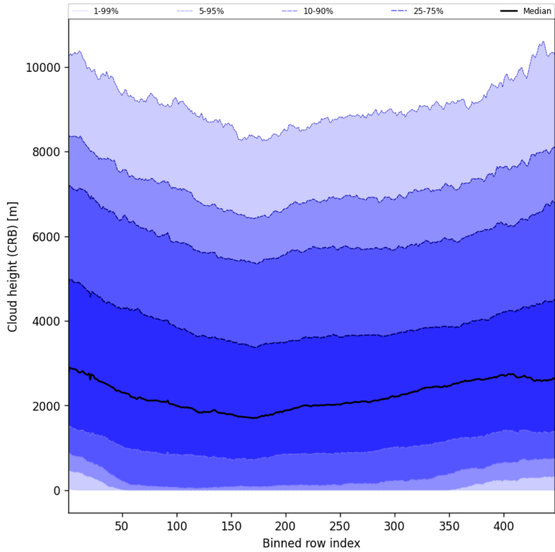
Figure 59: Along track statistics of “Cloud height (CRB)” for 2025-05-15 to 2025-05-17
