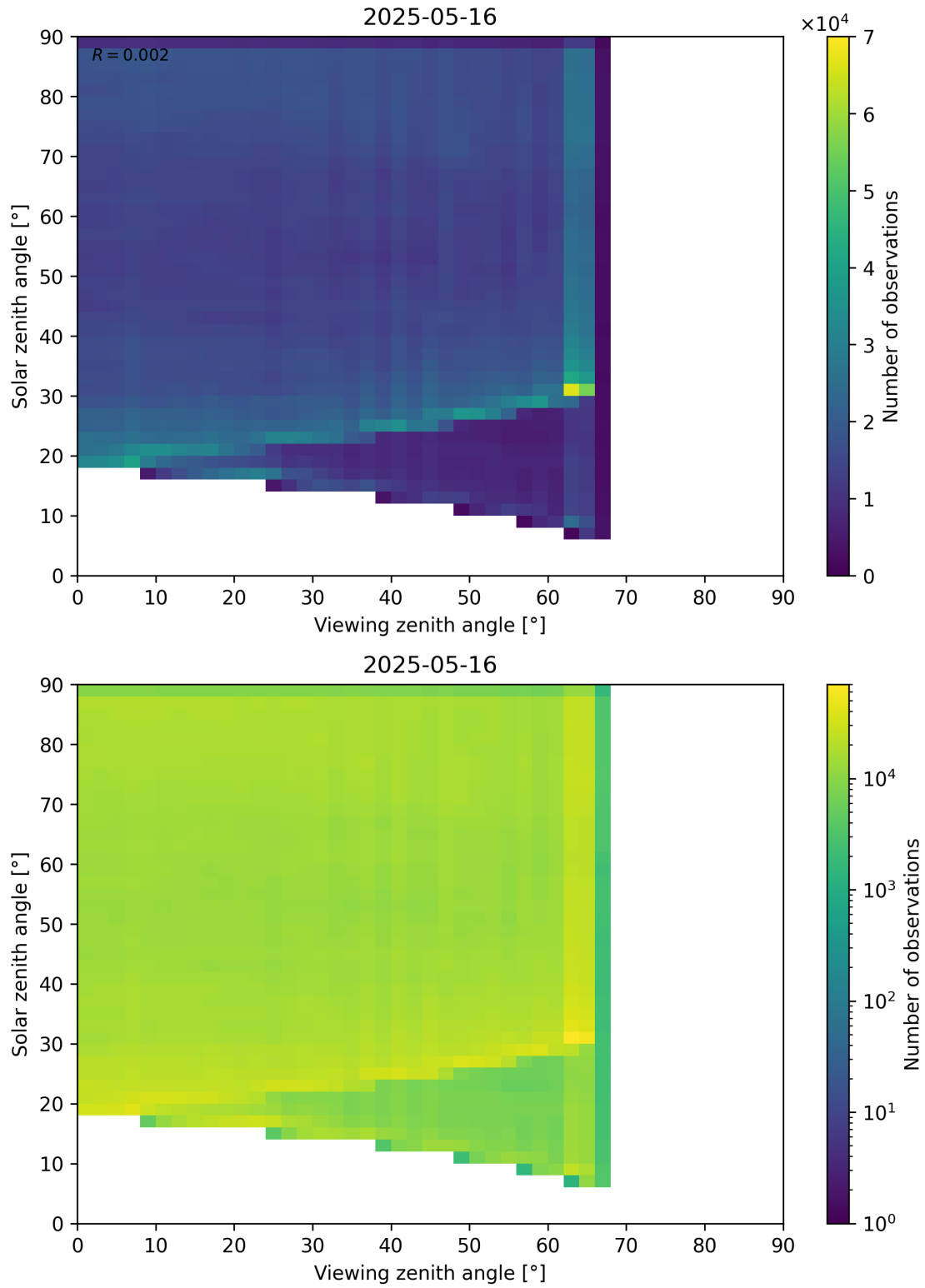
Figure 114: Scatter density plot of “Viewing zenith angle” against “Solar zenith angle” for 2025-05-15 to 2025-05-17.
