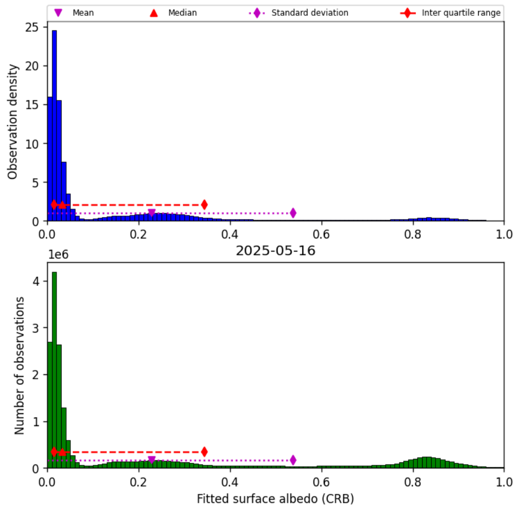
Figure 46: Histogram of “Fitted surface albedo (CRB)” for 2025-05-15 to 2025-05-17
