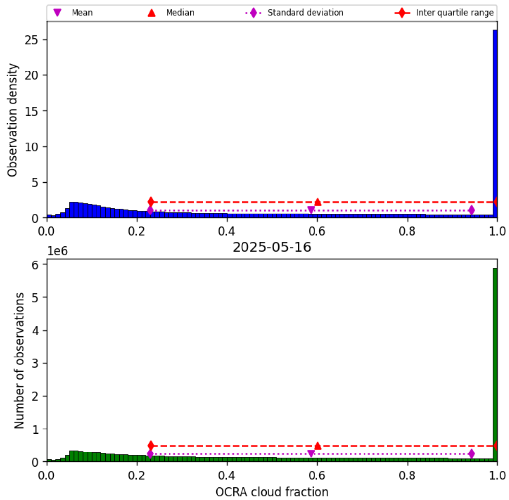
Figure 50: Histogram of “OCRA cloud fraction” for 2025-05-15 to 2025-05-17
