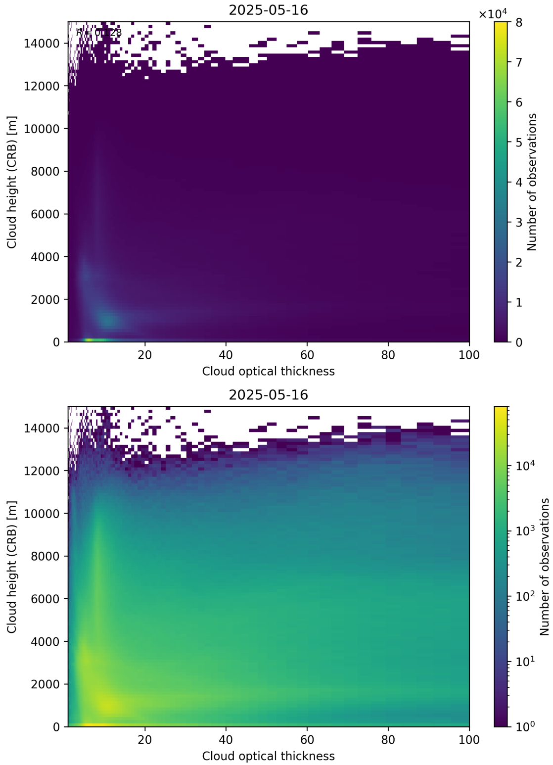
Figure 85: Scatter density plot of “Cloud optical thickness” against “Cloud height (CRB)” for 2025-05-15 to 2025-05-17.
