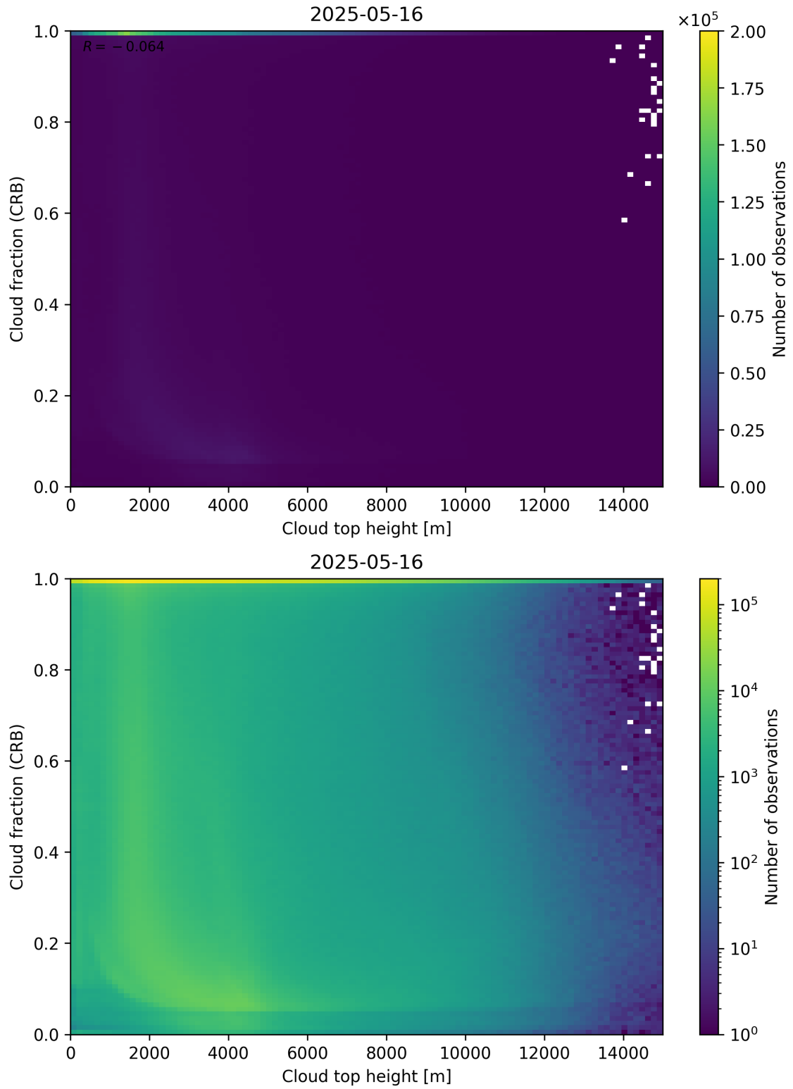
Figure 88: Scatter density plot of “Cloud top height” against “Cloud fraction (CRB)” for 2025-05-15 to 2025-05-17.
