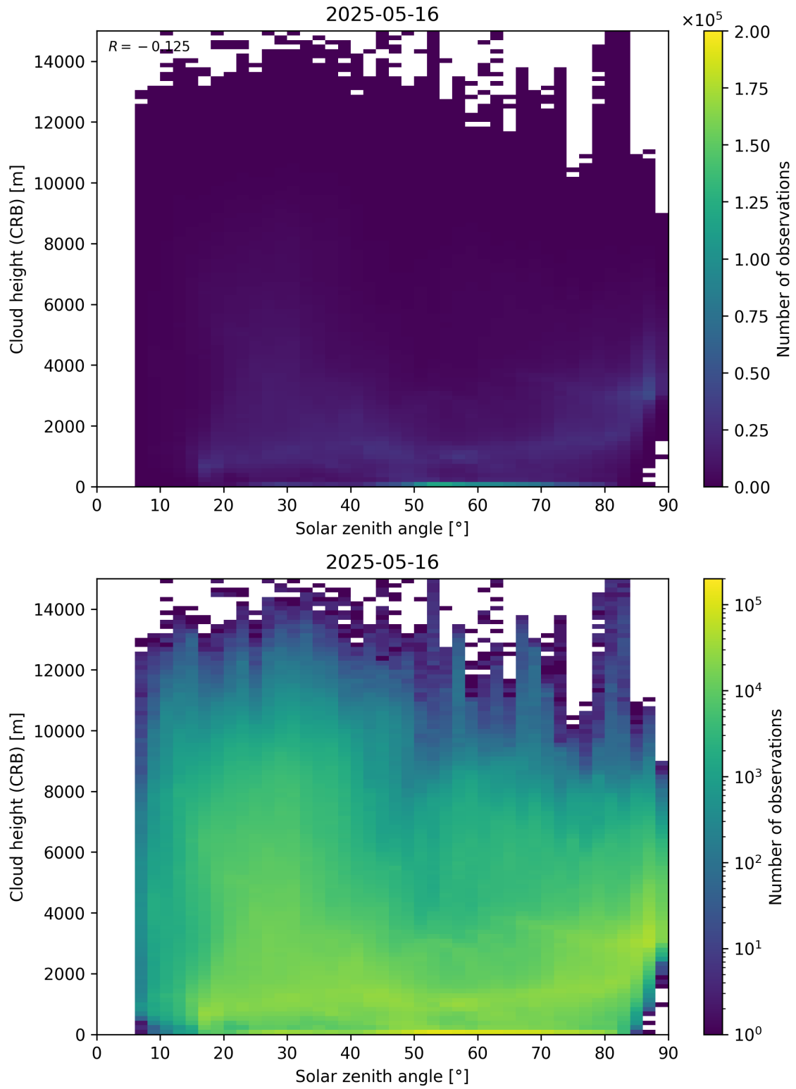
Figure 102: Scatter density plot of “Solar zenith angle” against “Cloud height (CRB)” for 2025-05-15 to 2025-05-17.
