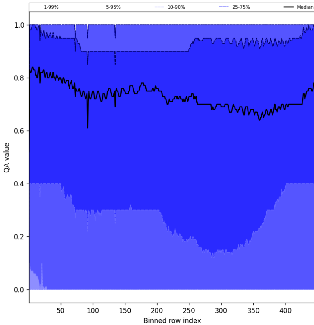
Figure 54: Along track statistics of “QA value” for 2025-05-15 to 2025-05-17
