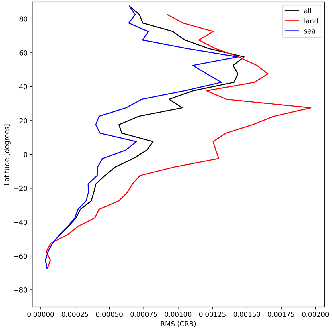
Figure 32: Zonal average of “RMS (CRB)” for 2025-05-15 to 2025-05-17.
