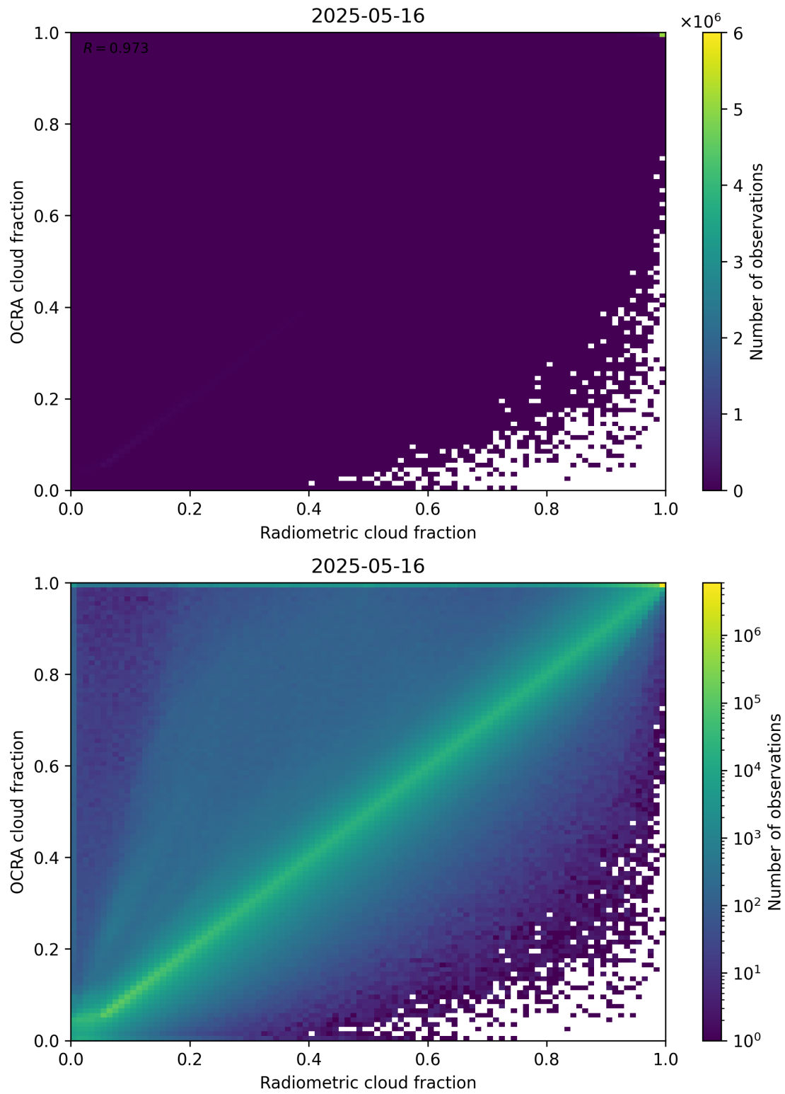
Figure 72: Scatter density plot of “Radiometric cloud fraction” against “OCRA cloud fraction” for 2025-05-15 to 2025-05-17.
