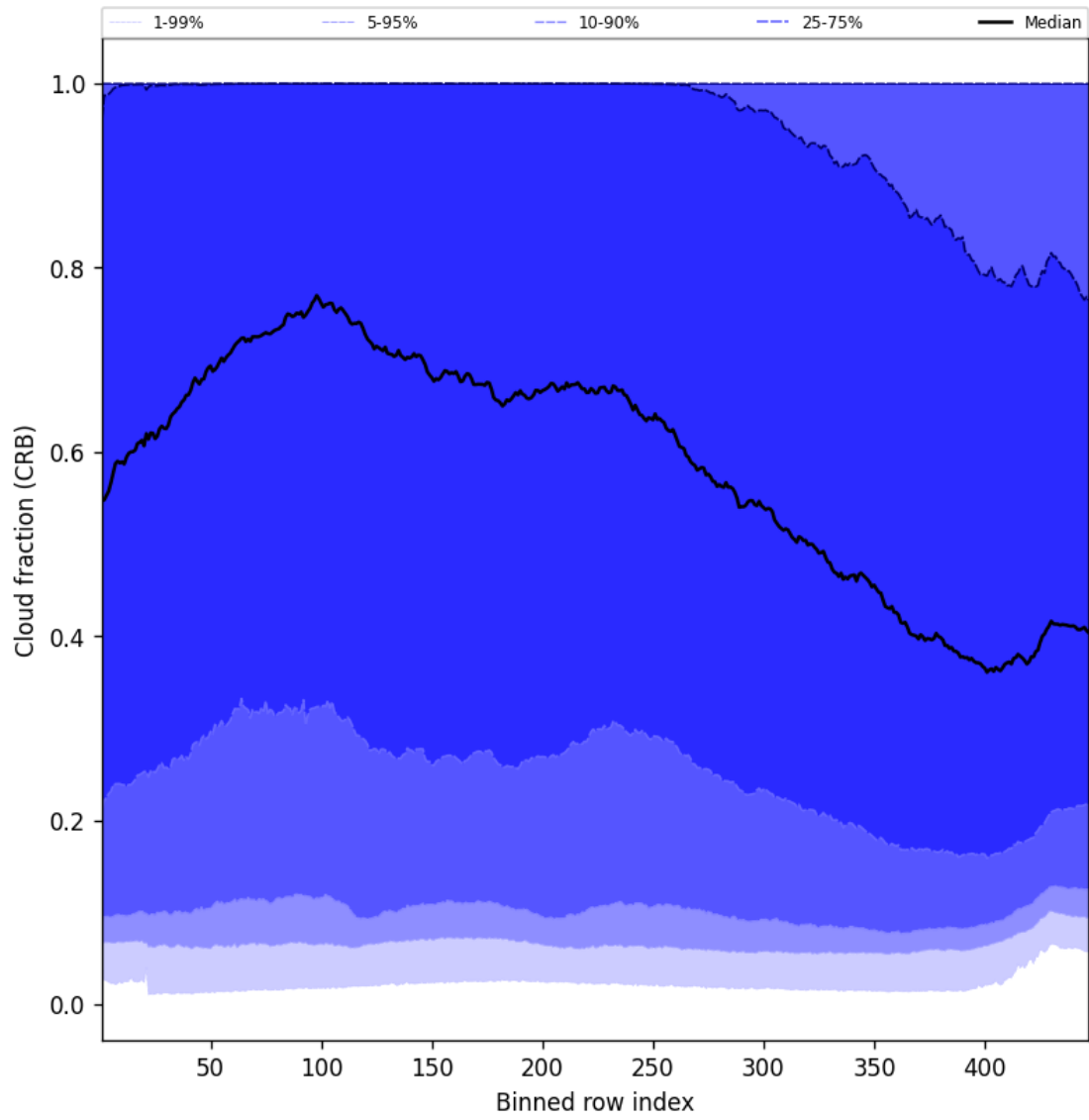
Figure 58: Along track statistics of “Cloud fraction (CRB)” for 2025-05-15 to 2025-05-17
