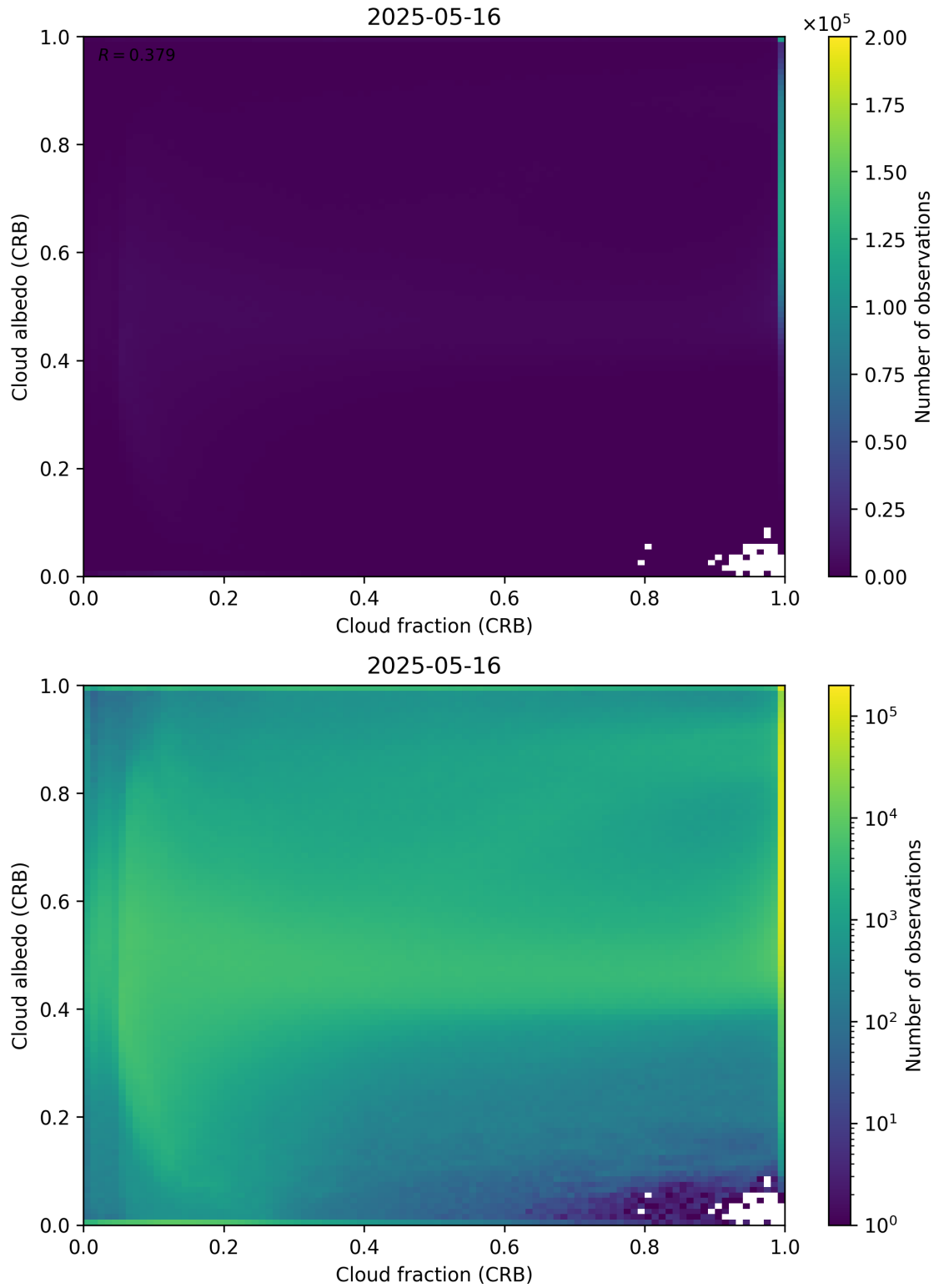
Figure 77: Scatter density plot of “Cloud fraction (CRB)” against “Cloud albedo (CRB)” for 2025-05-15 to 2025-05-17.
