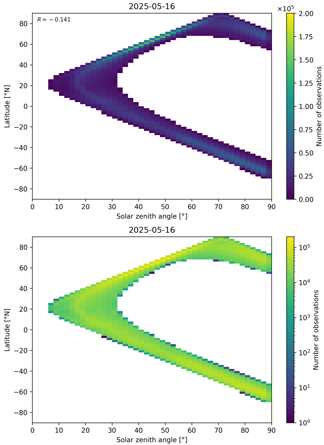
Figure 105: Scatter density plot of “Solar zenith angle” against “Latitude” for 2025-05-15 to 2025-05-17.
