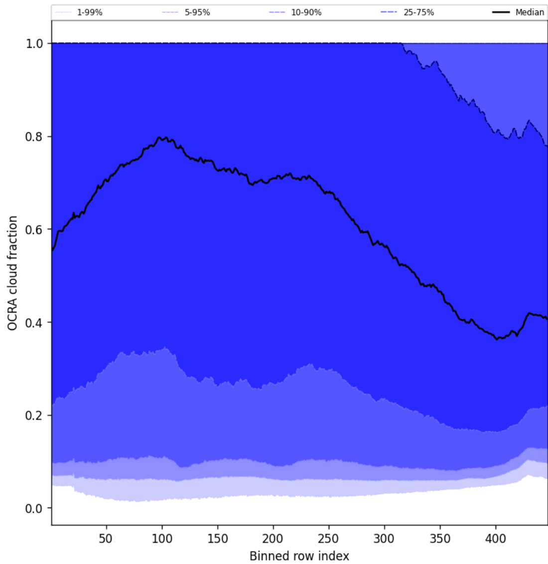
Figure 66: Along track statistics of “OCRA cloud fraction” for 2025-05-15 to 2025-05-17
