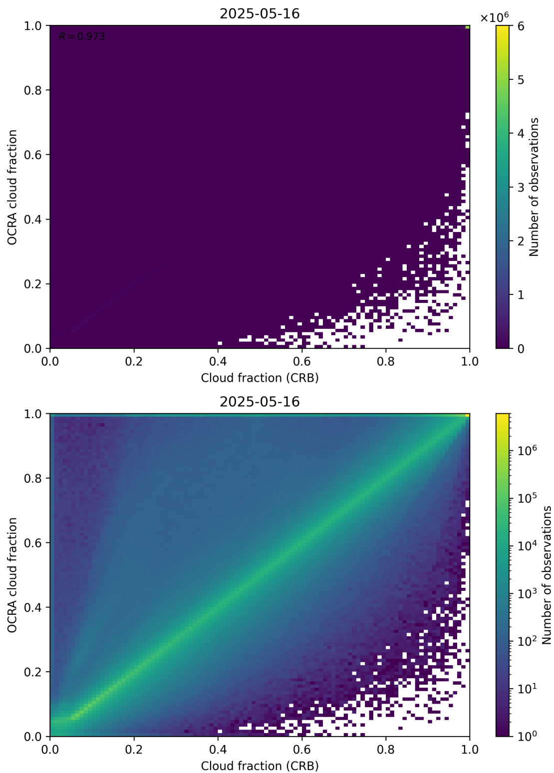
Figure 78: Scatter density plot of “Cloud fraction (CRB)” against “OCRA cloud fraction” for 2025-05-15 to 2025-05-17.
