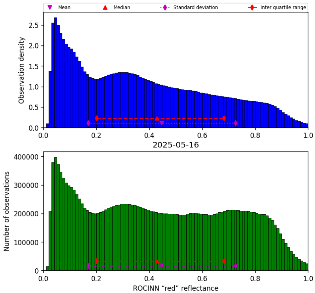
Figure 53: Histogram of “ROCINN “red” reflectance” for 2025-05-15 to 2025-05-17
