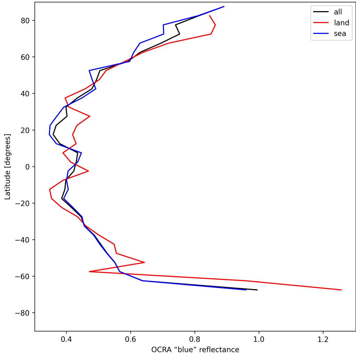
Figure 35: Zonal average of “OCRA “blue” reflectance” for 2025-05-15 to 2025-05-17.
