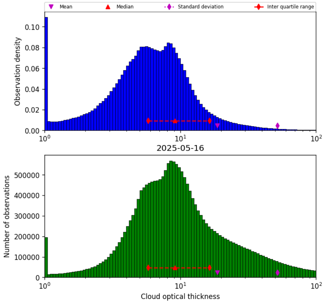
Figure 41: Histogram of “Cloud optical thickness” for 2025-05-15 to 2025-05-17
