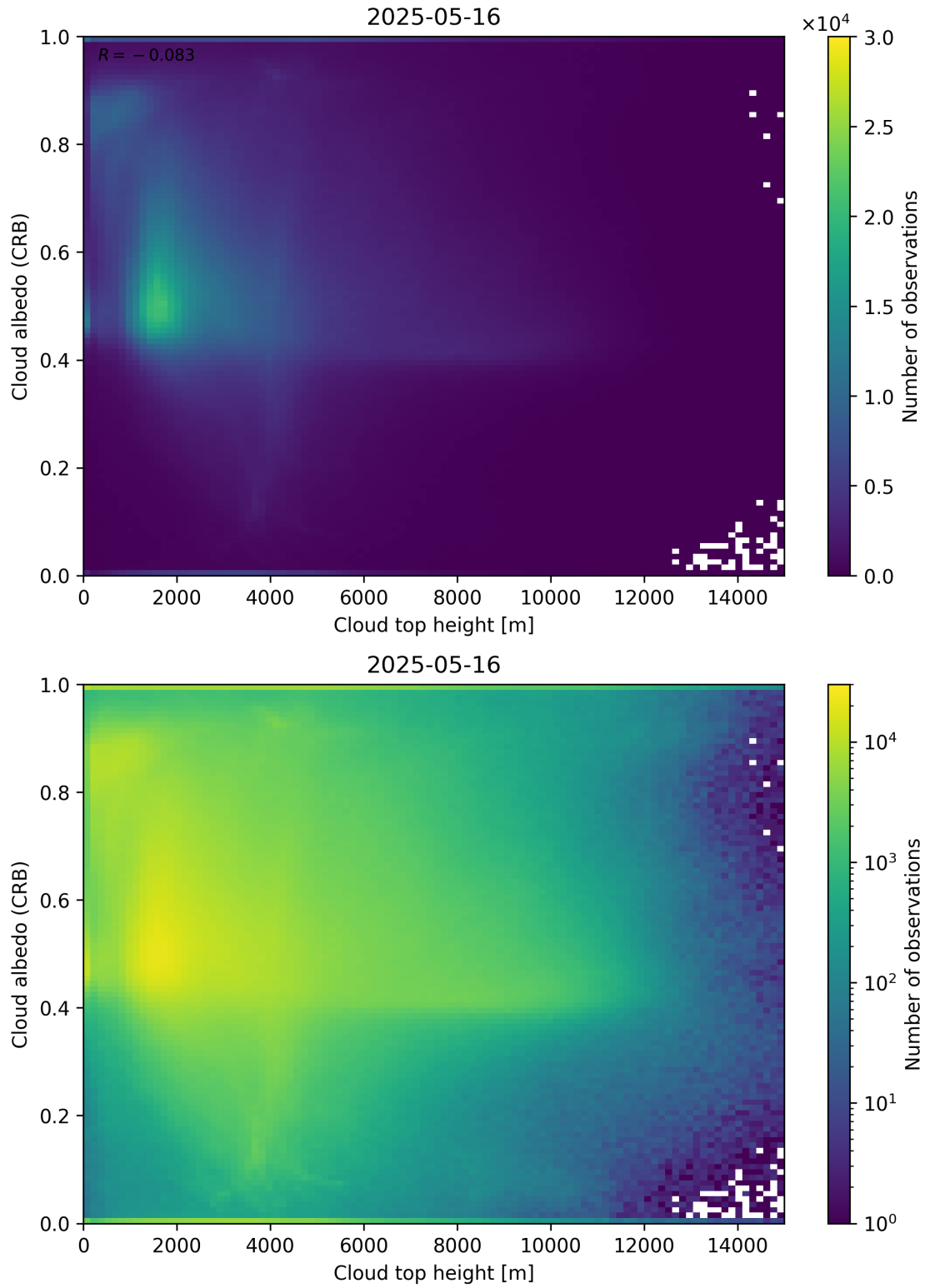
Figure 86: Scatter density plot of “Cloud top height” against “Cloud albedo (CRB)” for 2025-05-15 to 2025-05-17.
