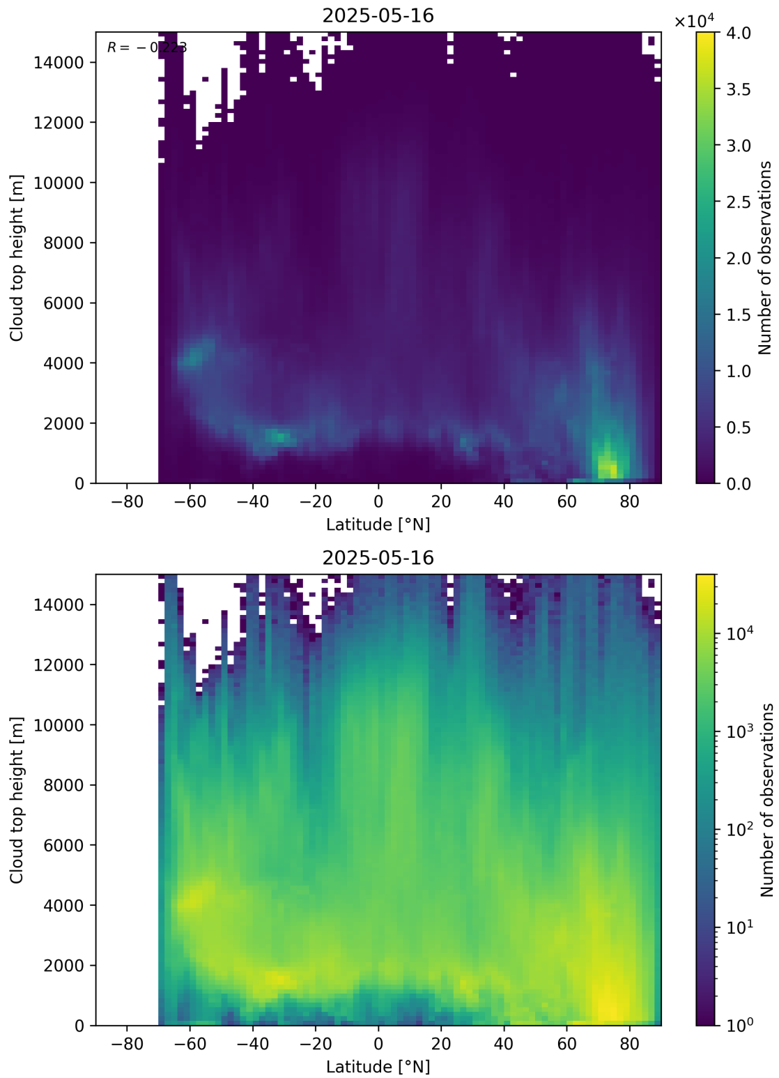
Figure 97: Scatter density plot of “Latitude” against “Cloud top height” for 2025-05-15 to 2025-05-17.
