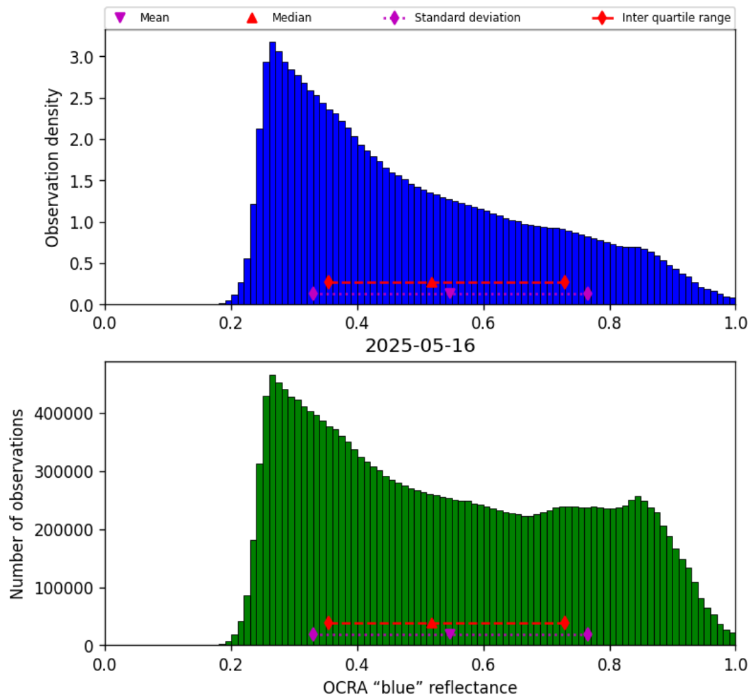
Figure 51: Histogram of “OCRA “blue” reflectance” for 2025-05-15 to 2025-05-17
