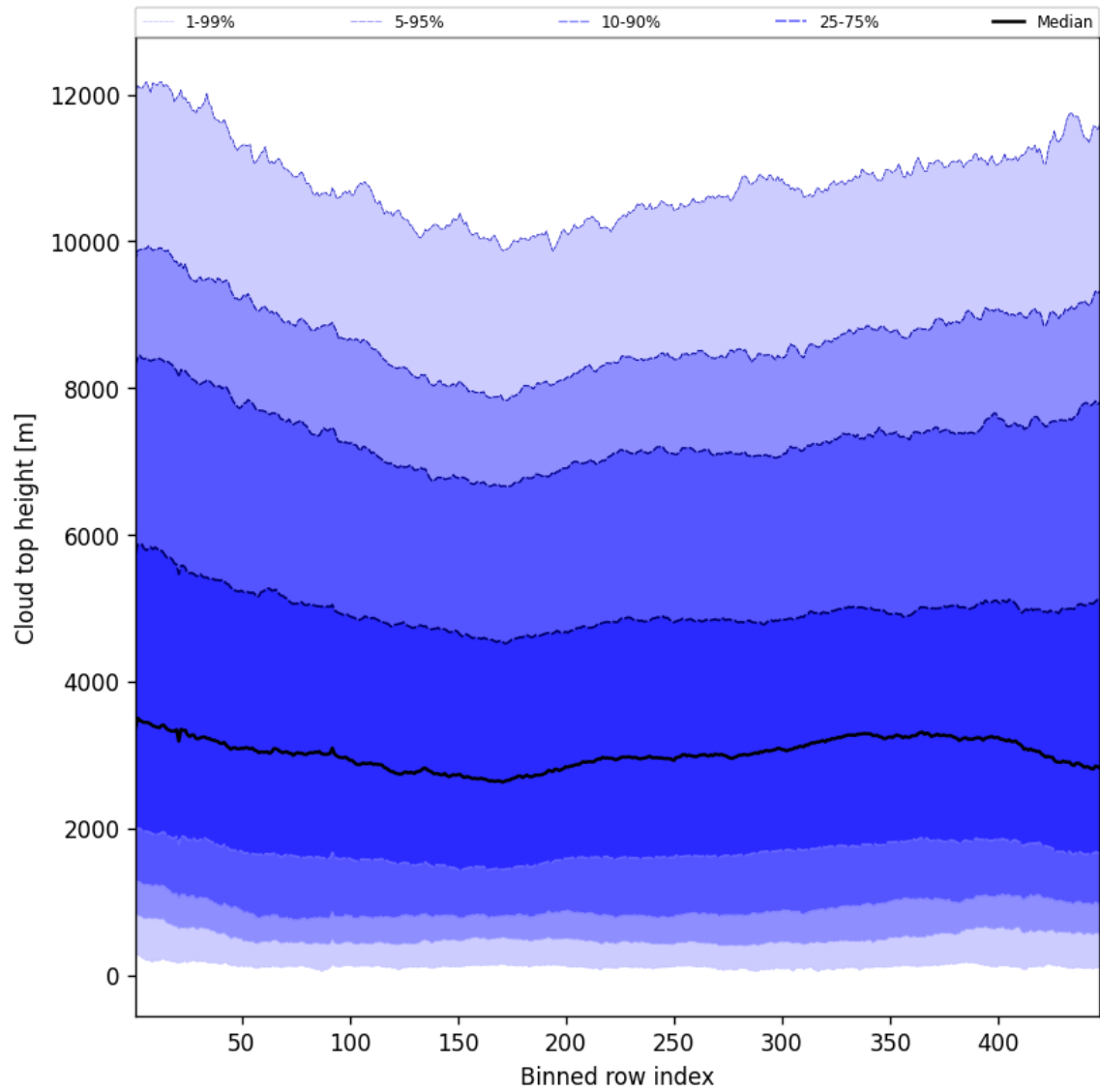
Figure 56: Along track statistics of “Cloud top height” for 2025-05-15 to 2025-05-17
