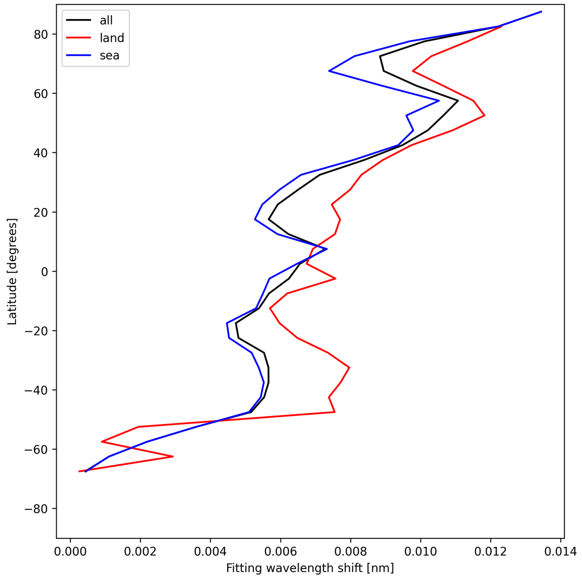
Figure 33: Zonal average of “Fitting wavelength shift” for 2025-05-15 to 2025-05-17.
