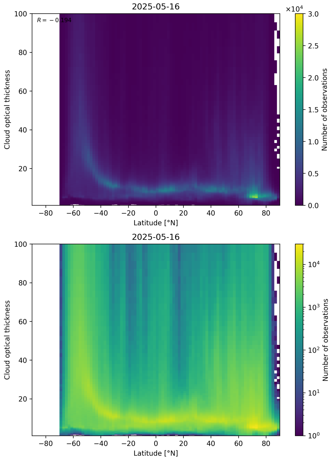
Figure 96: Scatter density plot of “Latitude” against “Cloud optical thickness” for 2025-05-15 to 2025-05-17.
