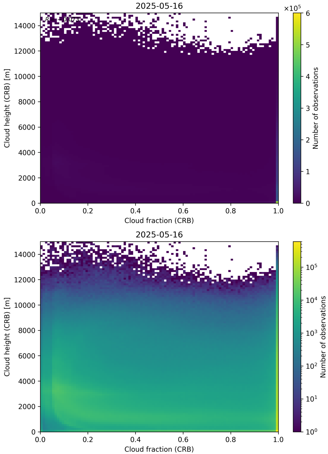
Figure 79: Scatter density plot of “Cloud fraction (CRB)” against “Cloud height (CRB)” for 2025-05-15 to 2025-05-17.
