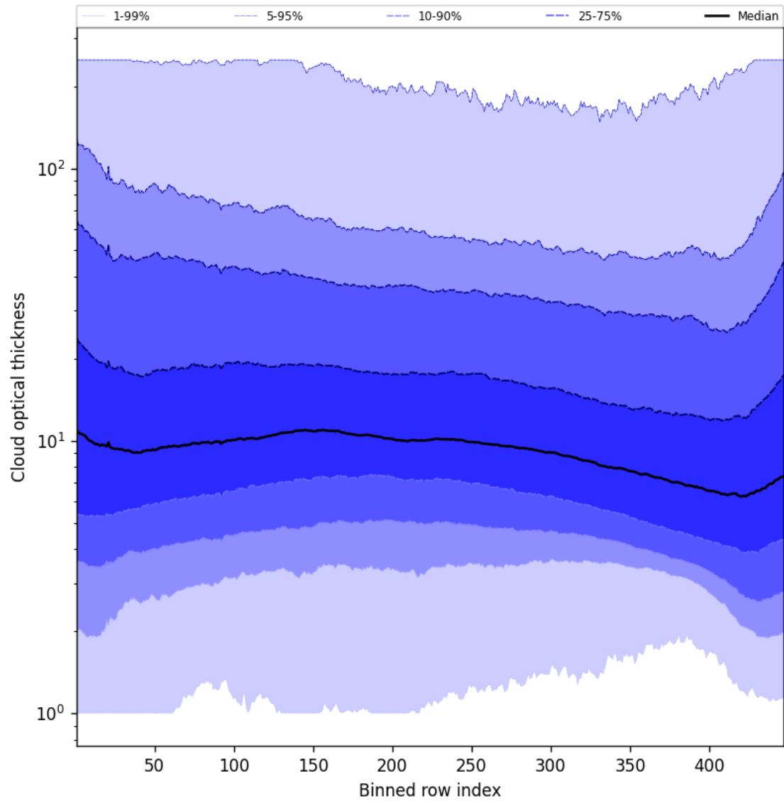
Figure 57: Along track statistics of “Cloud optical thickness” for 2025-05-15 to 2025-05-17
