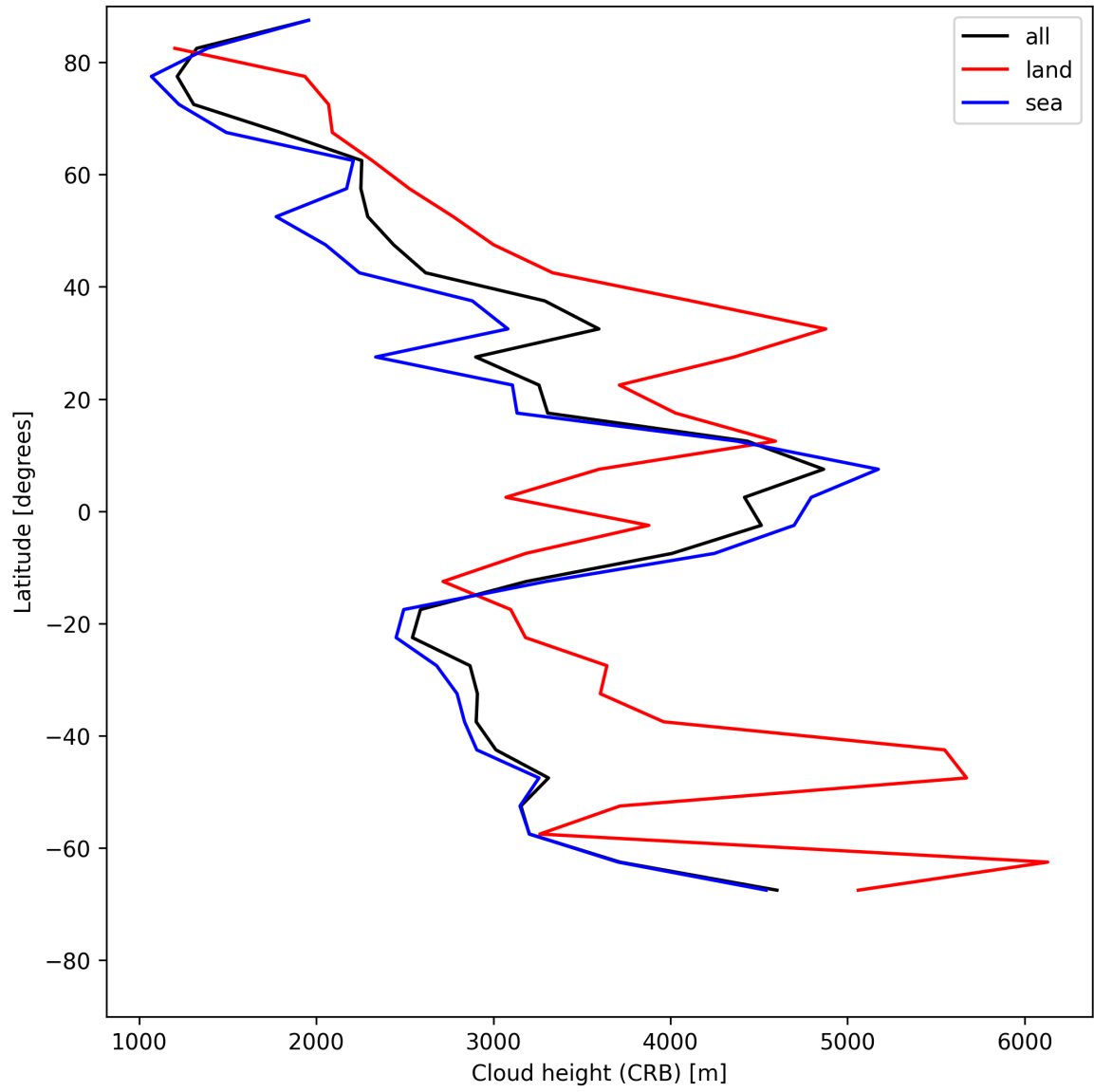
Figure 27: Zonal average of “Cloud height (CRB)” for 2025-05-15 to 2025-05-17.
