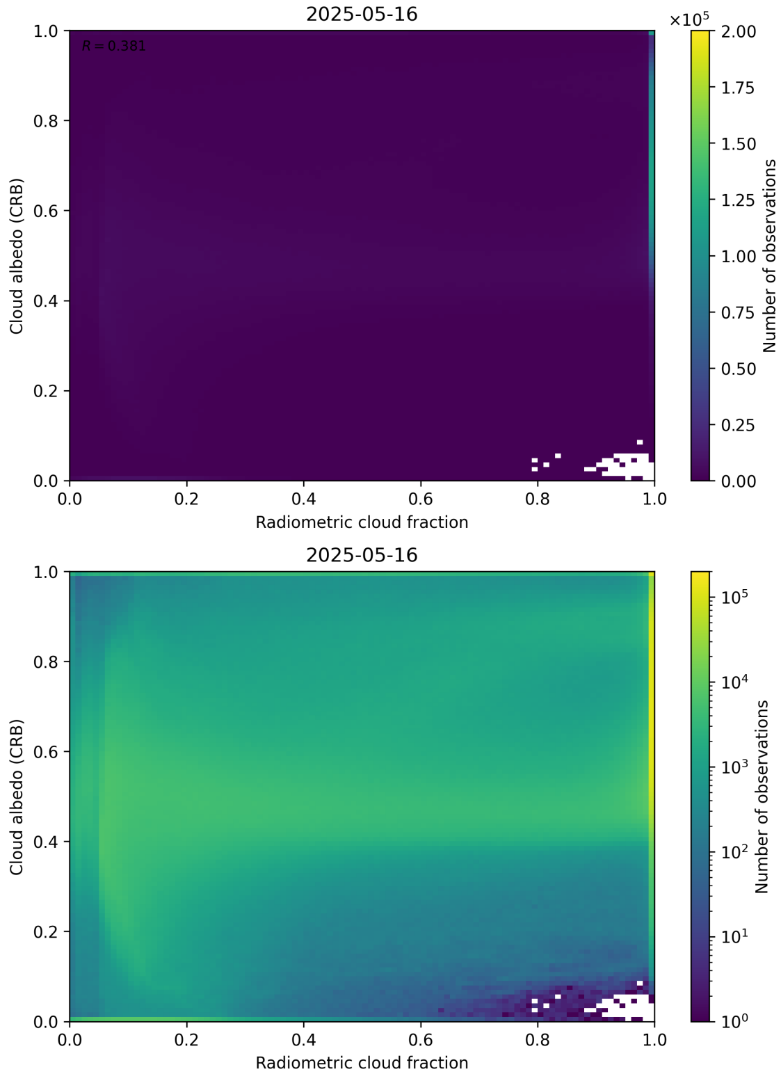
Figure 71: Scatter density plot of “Radiometric cloud fraction” against “Cloud albedo (CRB)” for 2025-05-15 to 2025-05-17.
