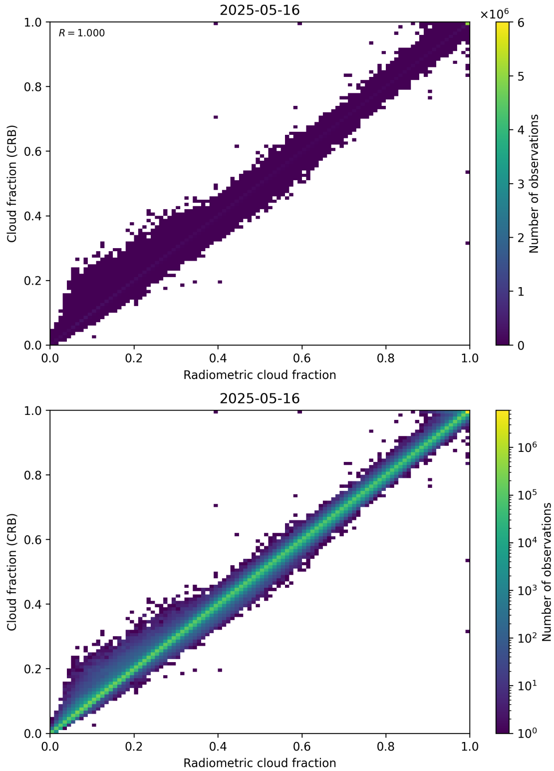
Figure 73: Scatter density plot of “Radiometric cloud fraction” against “Cloud fraction (CRB)” for 2025-05-15 to 2025-05-17.
