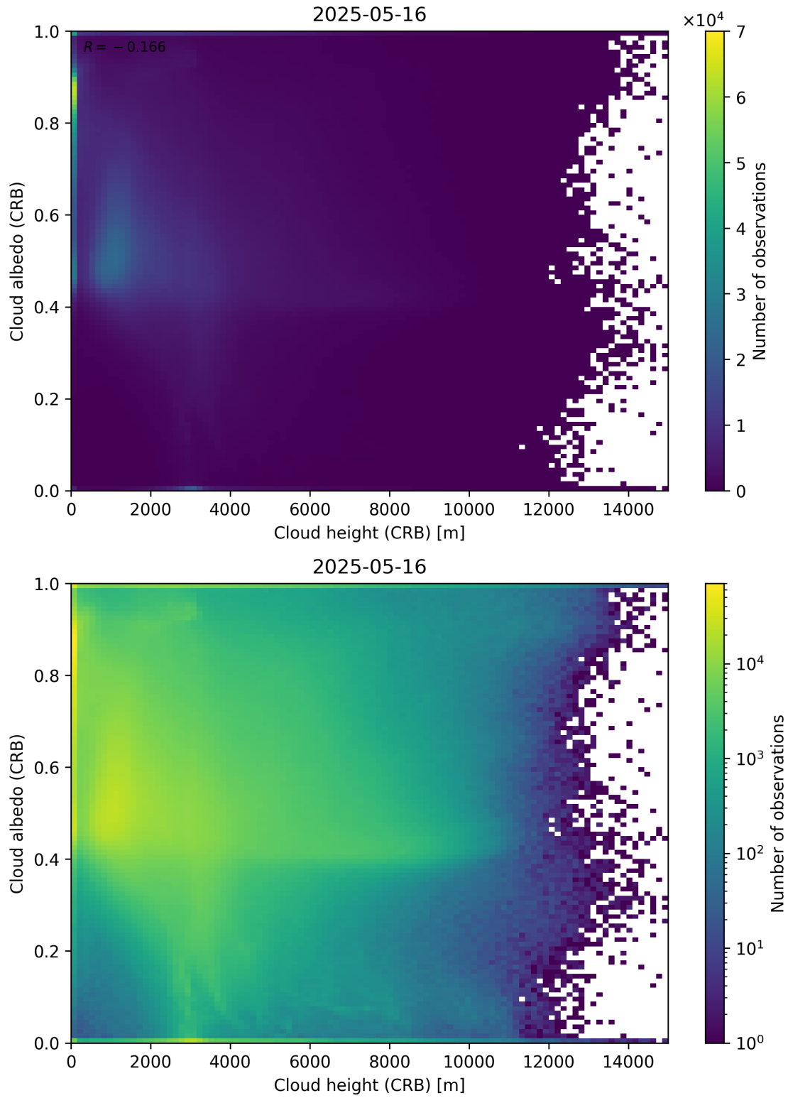
Figure 80: Scatter density plot of “Cloud height (CRB)” against “Cloud albedo (CRB)” for 2025-05-15 to 2025-05-17.
