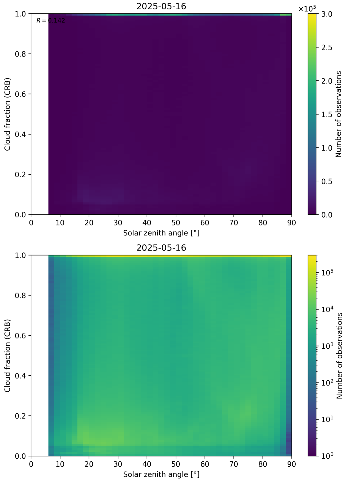
Figure 101: Scatter density plot of “Solar zenith angle” against “Cloud fraction (CRB)” for 2025-05-15 to 2025-05-17.
