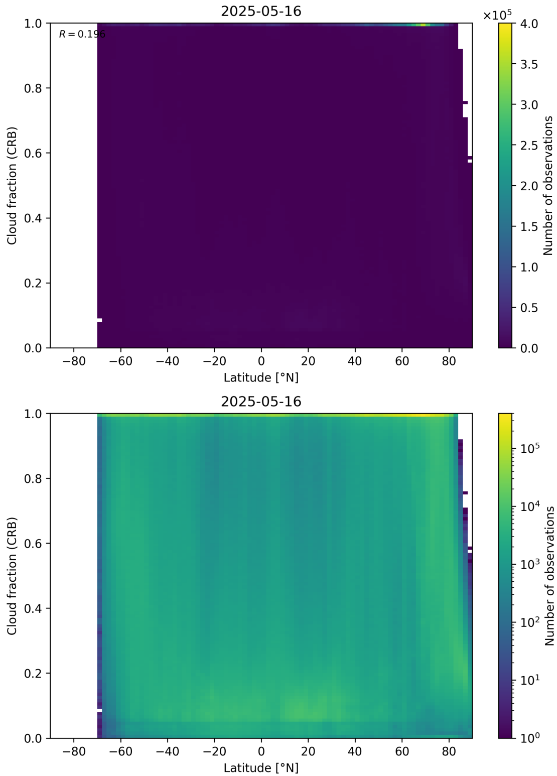
Figure 94: Scatter density plot of “Latitude” against “Cloud fraction (CRB)” for 2025-05-15 to 2025-05-17.
