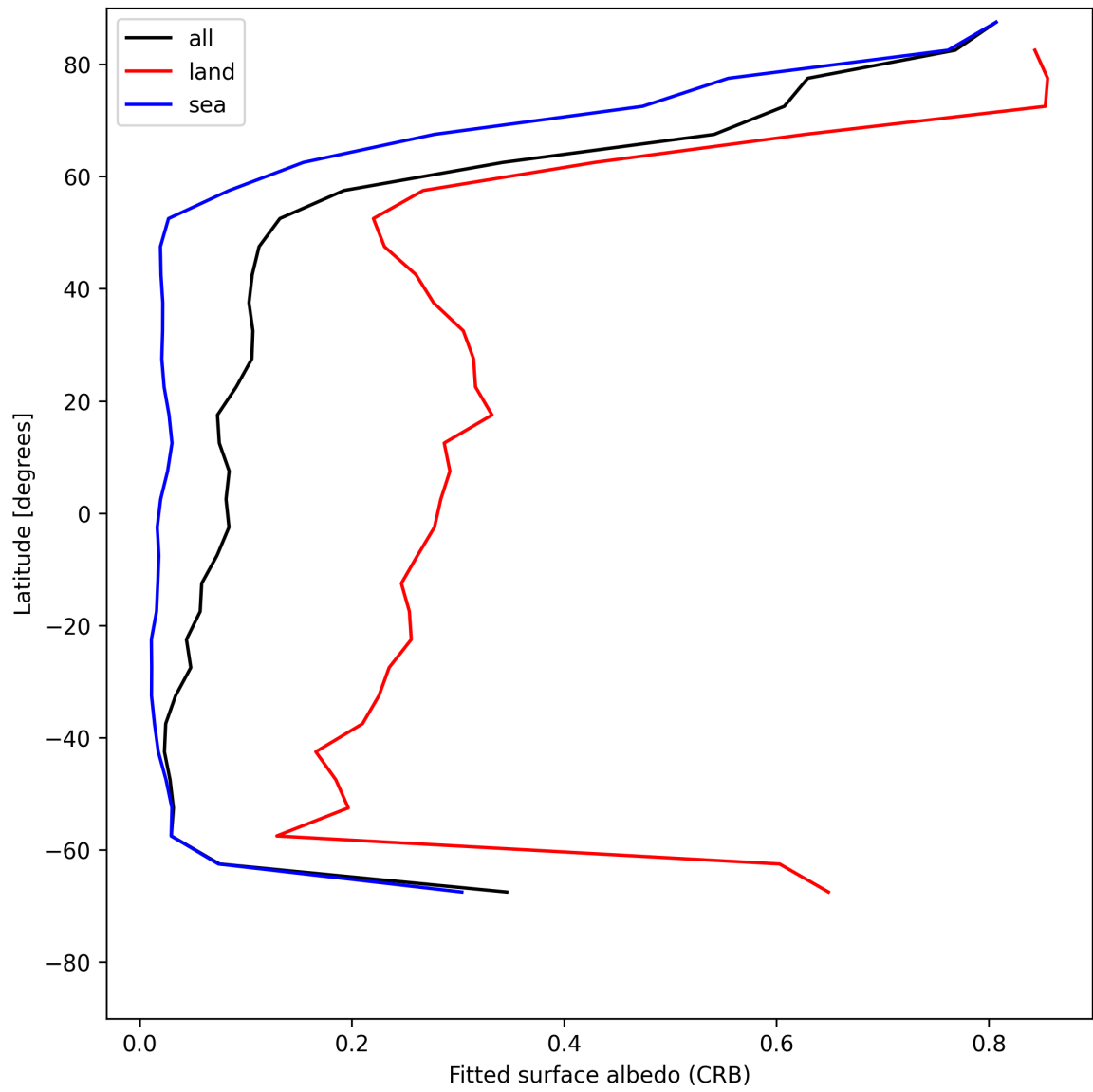
Figure 30: Zonal average of “Fitted surface albedo (CRB)” for 2025-05-15 to 2025-05-17.
