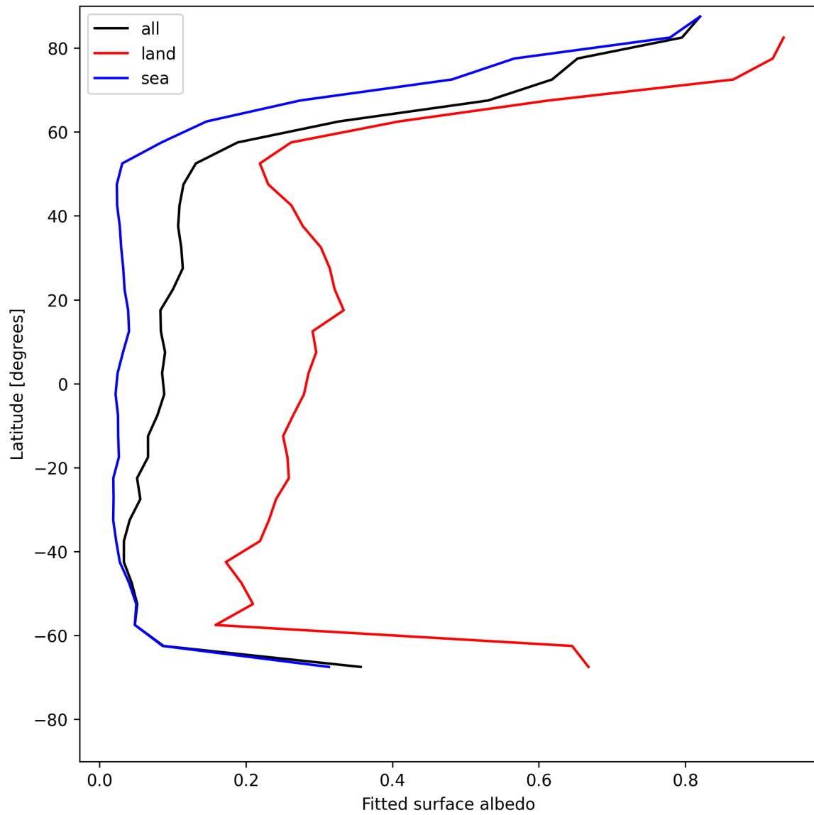
Figure 29: Zonal average of “Fitted surface albedo” for 2025-05-15 to 2025-05-17.
