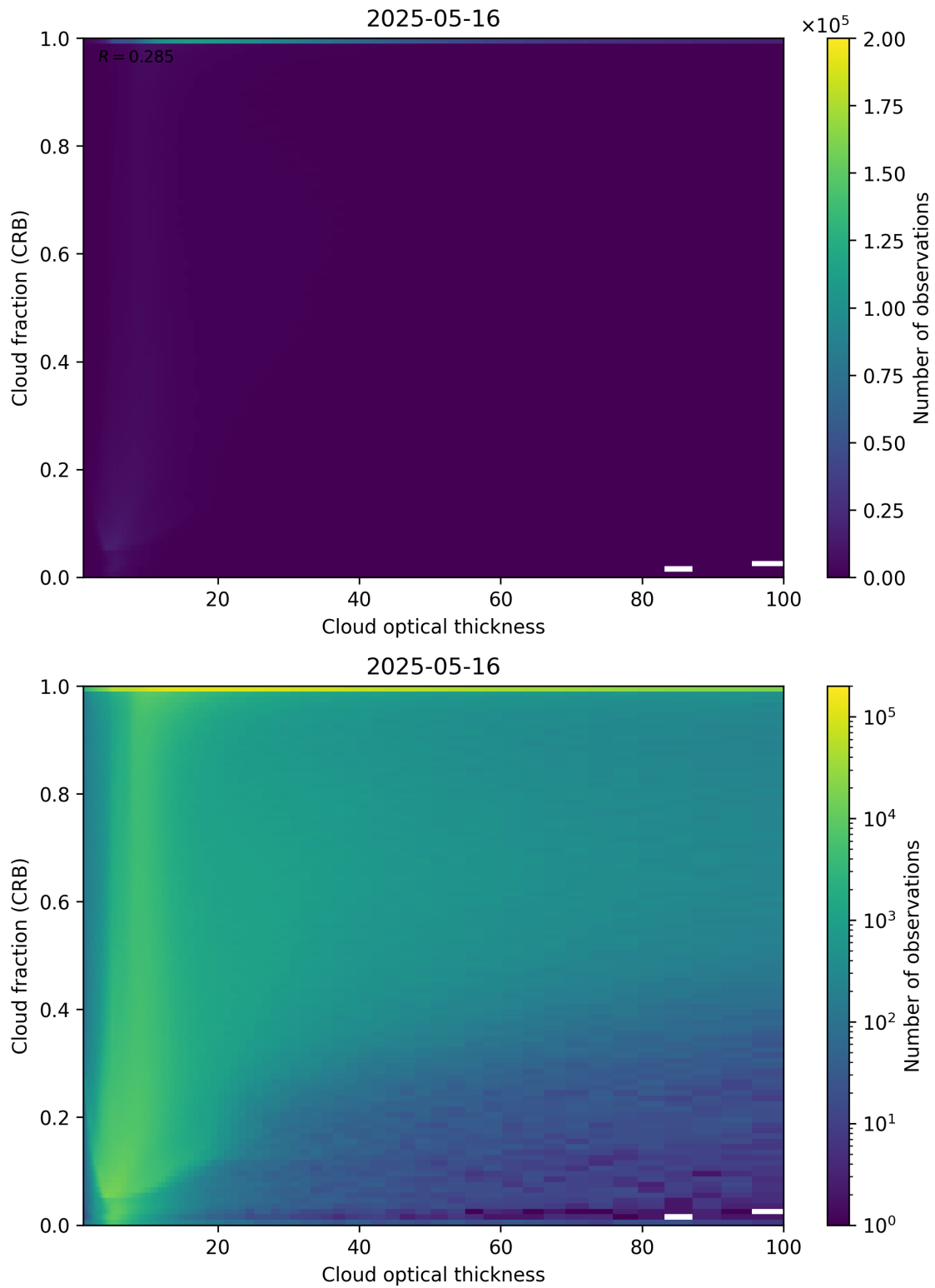
Figure 84: Scatter density plot of “Cloud optical thickness” against “Cloud fraction (CRB)” for 2025-05-15 to 2025-05-17.
