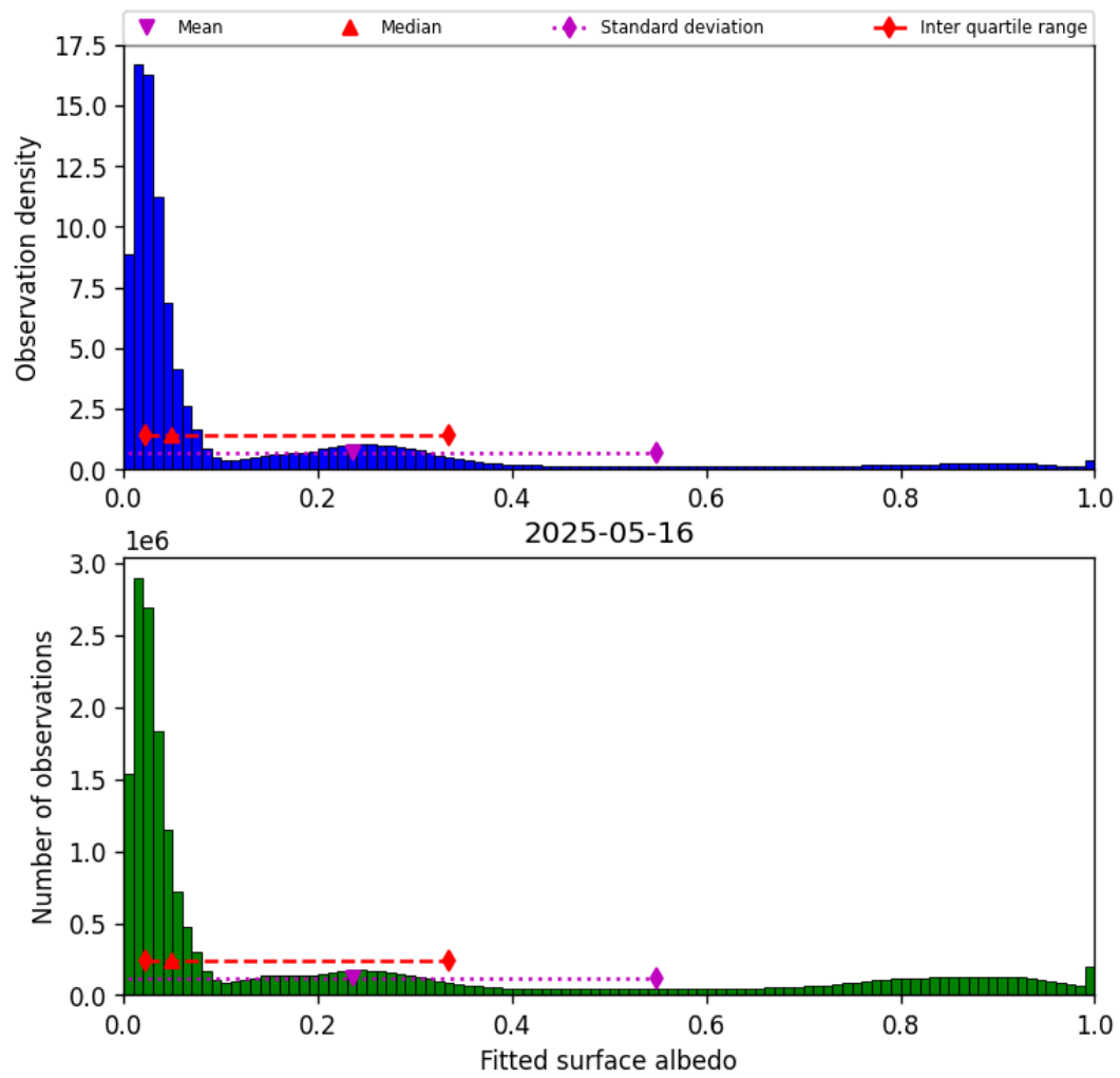
Figure 45: Histogram of “Fitted surface albedo” for 2025-05-15 to 2025-05-17
