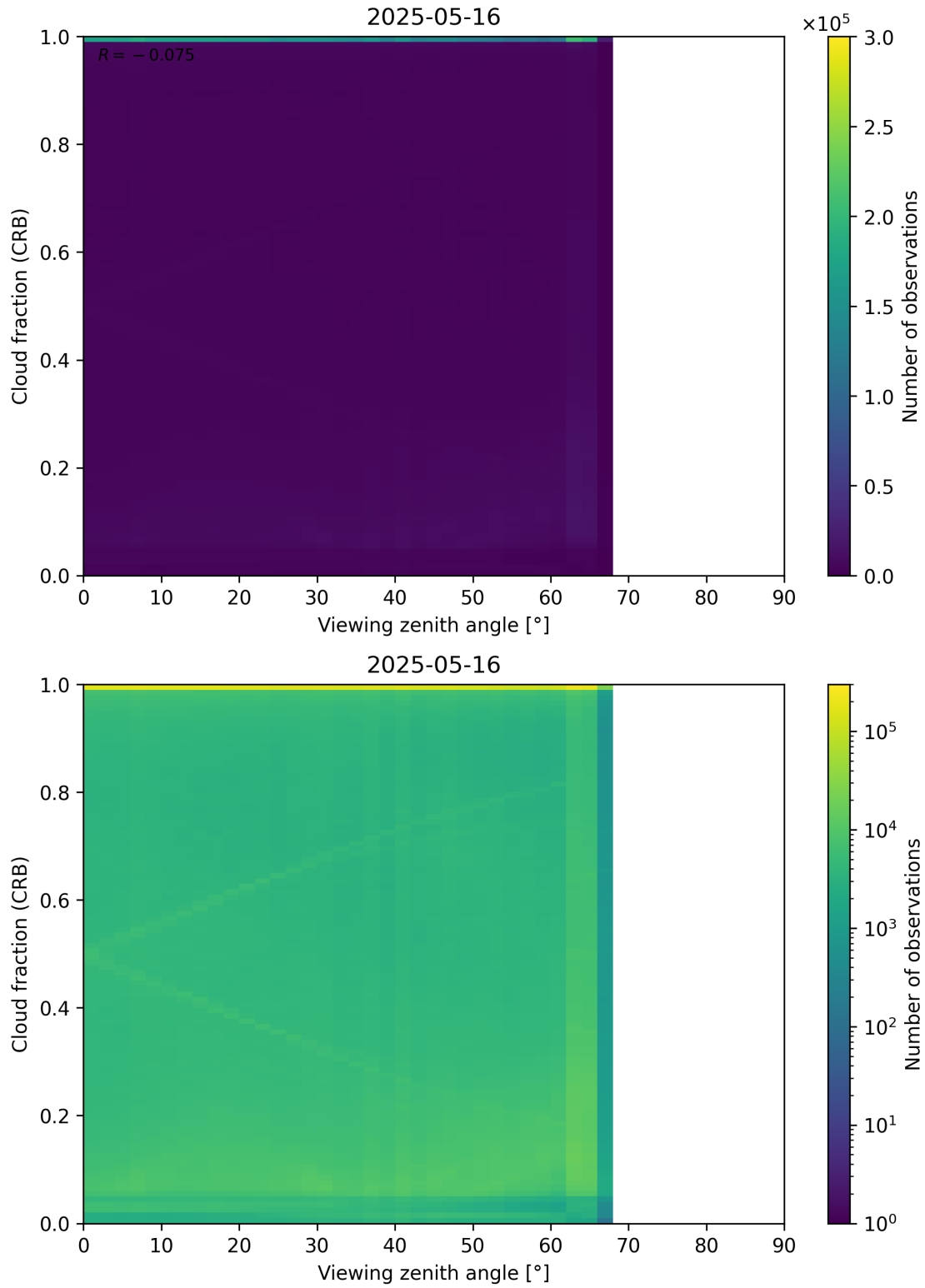
Figure 109: Scatter density plot of “Viewing zenith angle” against “Cloud fraction (CRB)” for 2025-05-15 to 2025-05-17.
