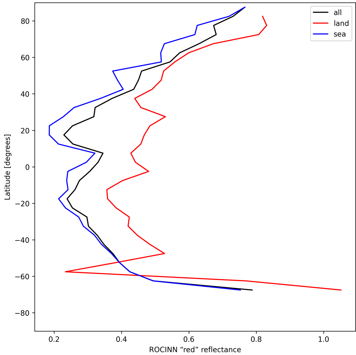
Figure 37: Zonal average of "ROCINN "red" reflectance" for 2025-05-15 to 2025-05-17.
