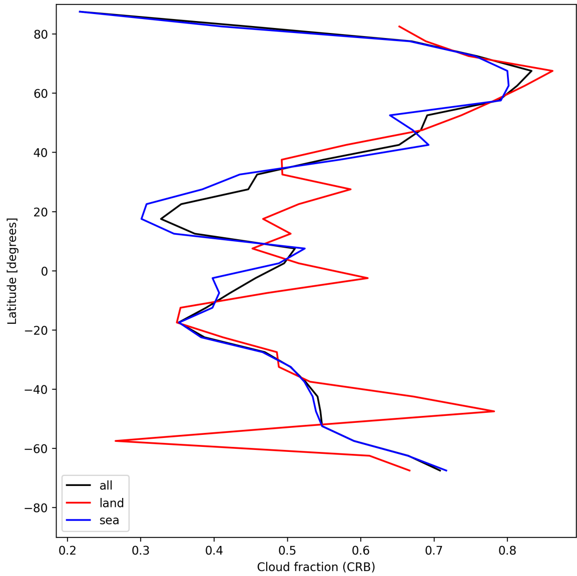
Figure 26: Zonal average of “Cloud fraction (CRB)” for 2025-05-15 to 2025-05-17.
