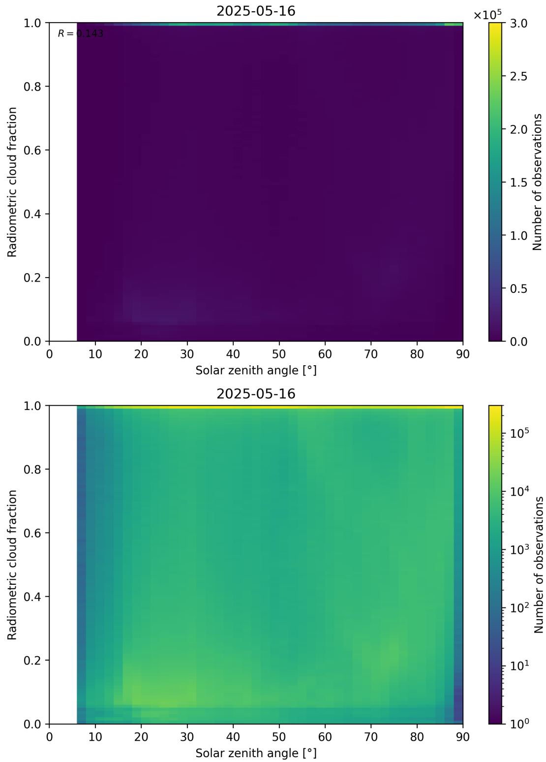
Figure 99: Scatter density plot of “Solar zenith angle” against “Radiometric cloud fraction” for 2025-05-15 to 2025-05-17.
