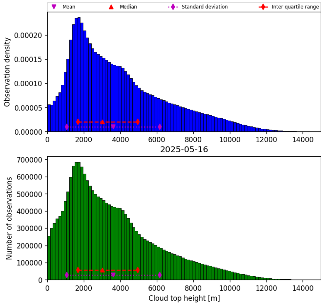
Figure 40: Histogram of “Cloud top height” for 2025-05-15 to 2025-05-17
