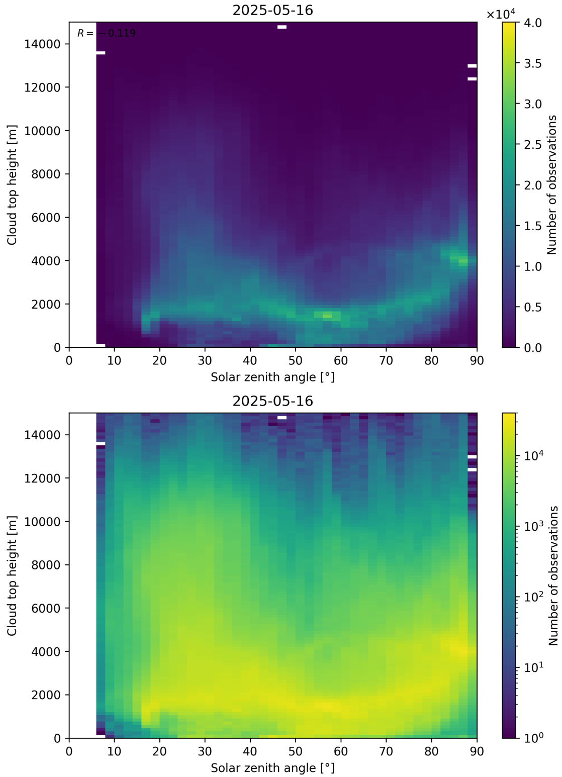
Figure 104: Scatter density plot of “Solar zenith angle” against “Cloud top height” for 2025-05-15 to 2025-05-17.
