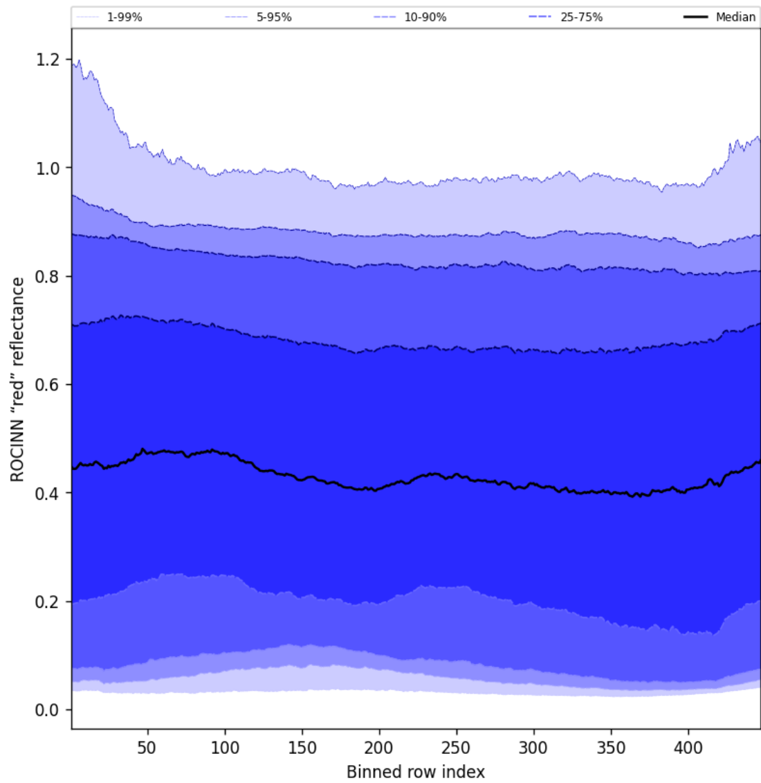
Figure 69: Along track statistics of "ROCINN "red" reflectance" for 2025-05-15 to 2025-05-17
