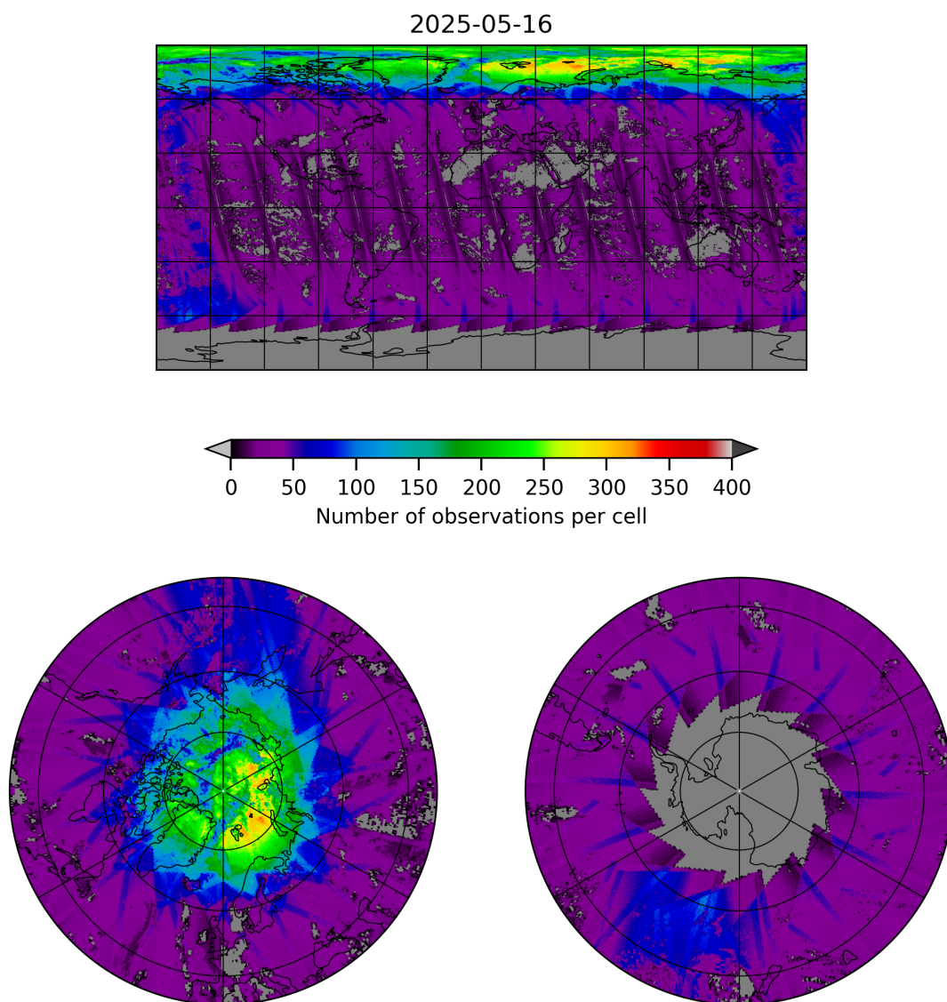
Figure 21: Map of the number of observations for 2025-05-15 to 2025-05-17
