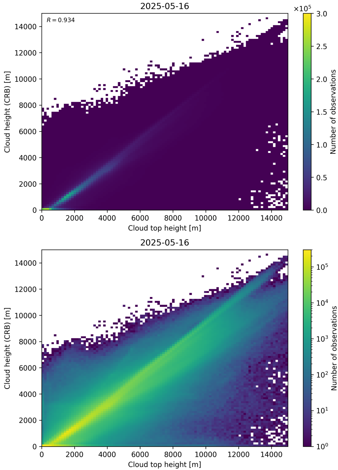
Figure 89: Scatter density plot of “Cloud top height” against “Cloud height (CRB)” for 2025-05-15 to 2025-05-17.
