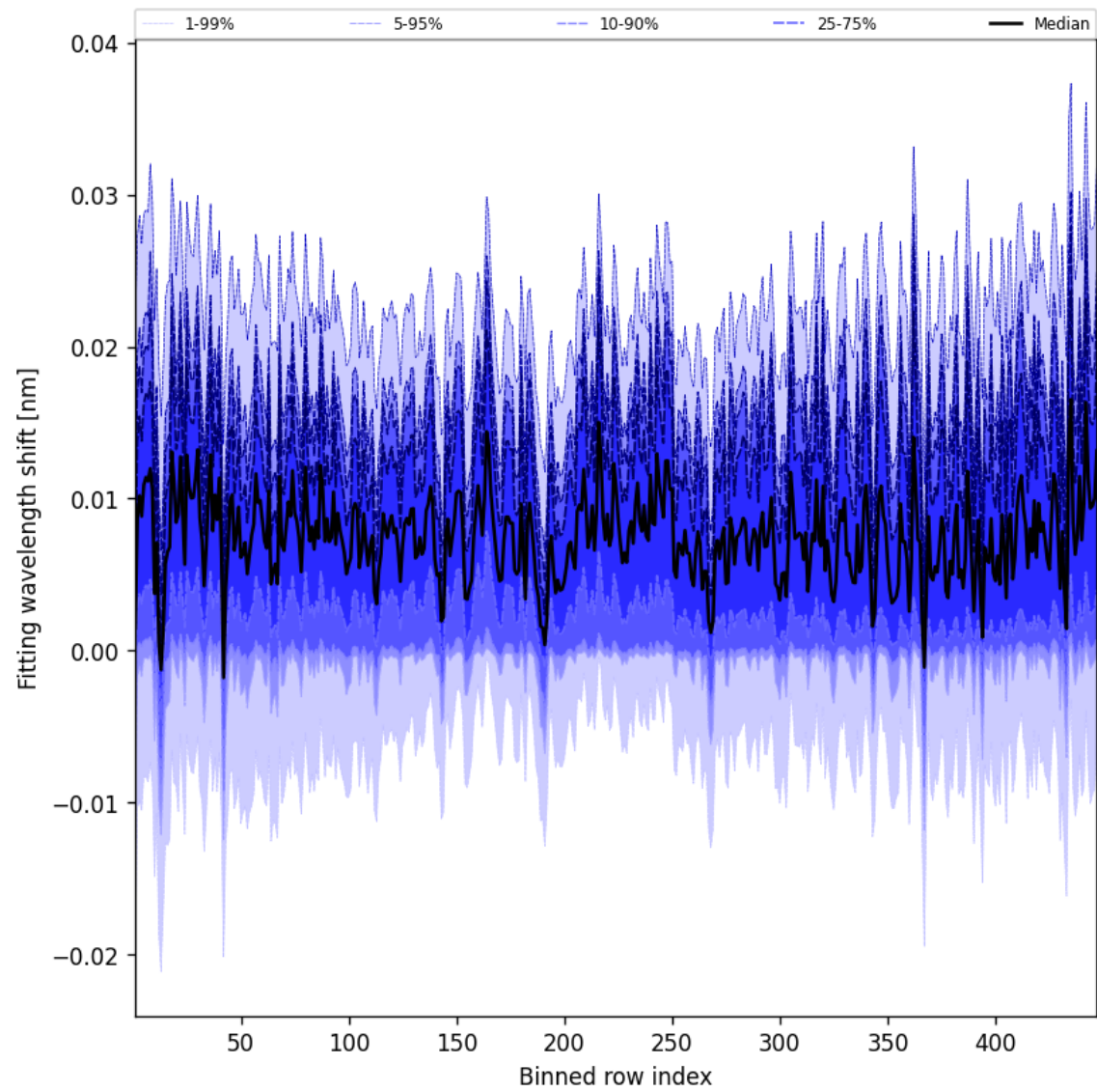
Figure 65: Along track statistics of “Fitting wavelength shift” for 2025-05-15 to 2025-05-17
