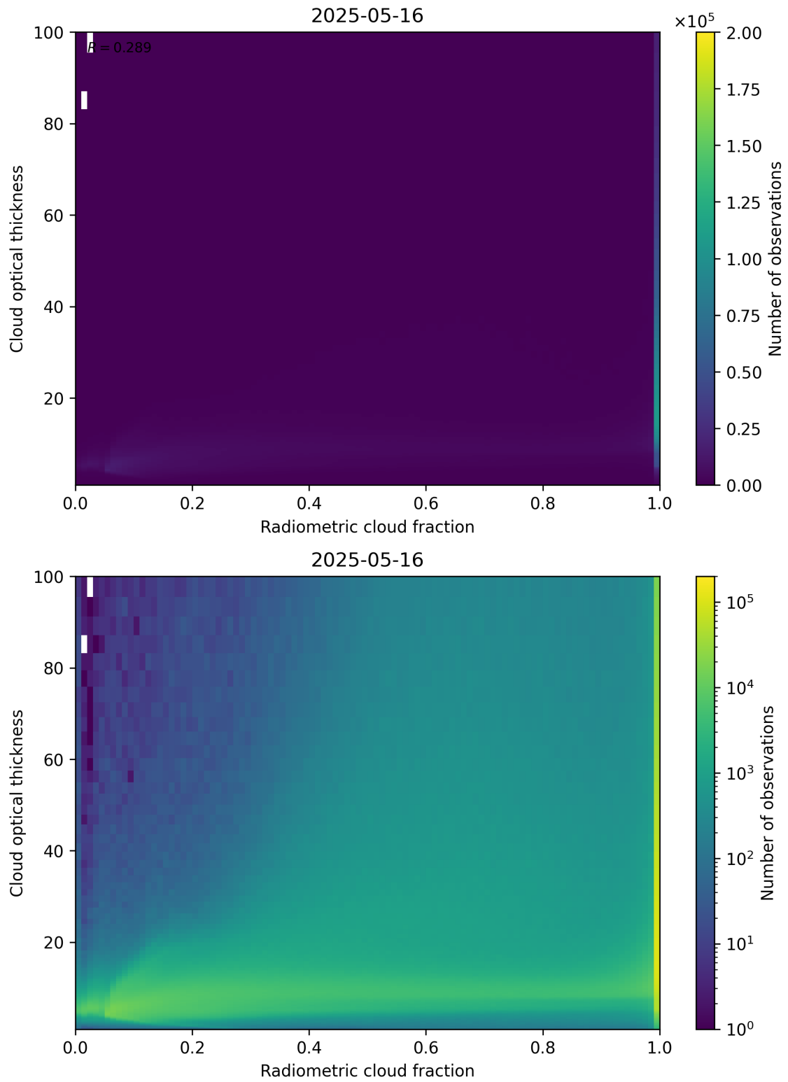
Figure 75: Scatter density plot of “Radiometric cloud fraction” against “Cloud optical thickness” for 2025-05-15 to 2025-05-17.
