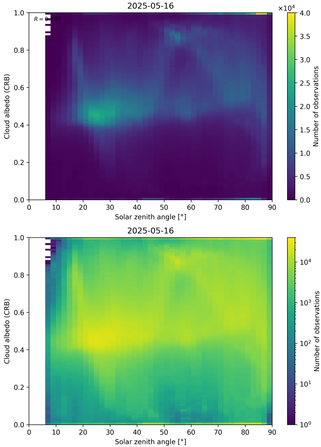
Figure 98: Scatter density plot of “Solar zenith angle” against “Cloud albedo (CRB)” for 2025-05-15 to 2025-05-17.
