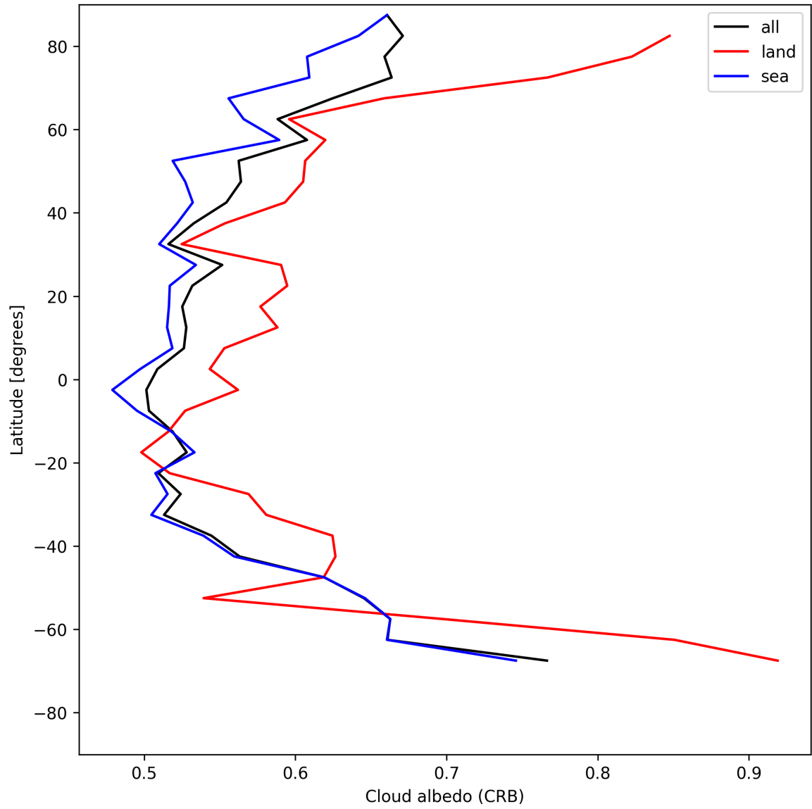
Figure 28: Zonal average of “Cloud albedo (CRB)” for 2025-05-15 to 2025-05-17.
