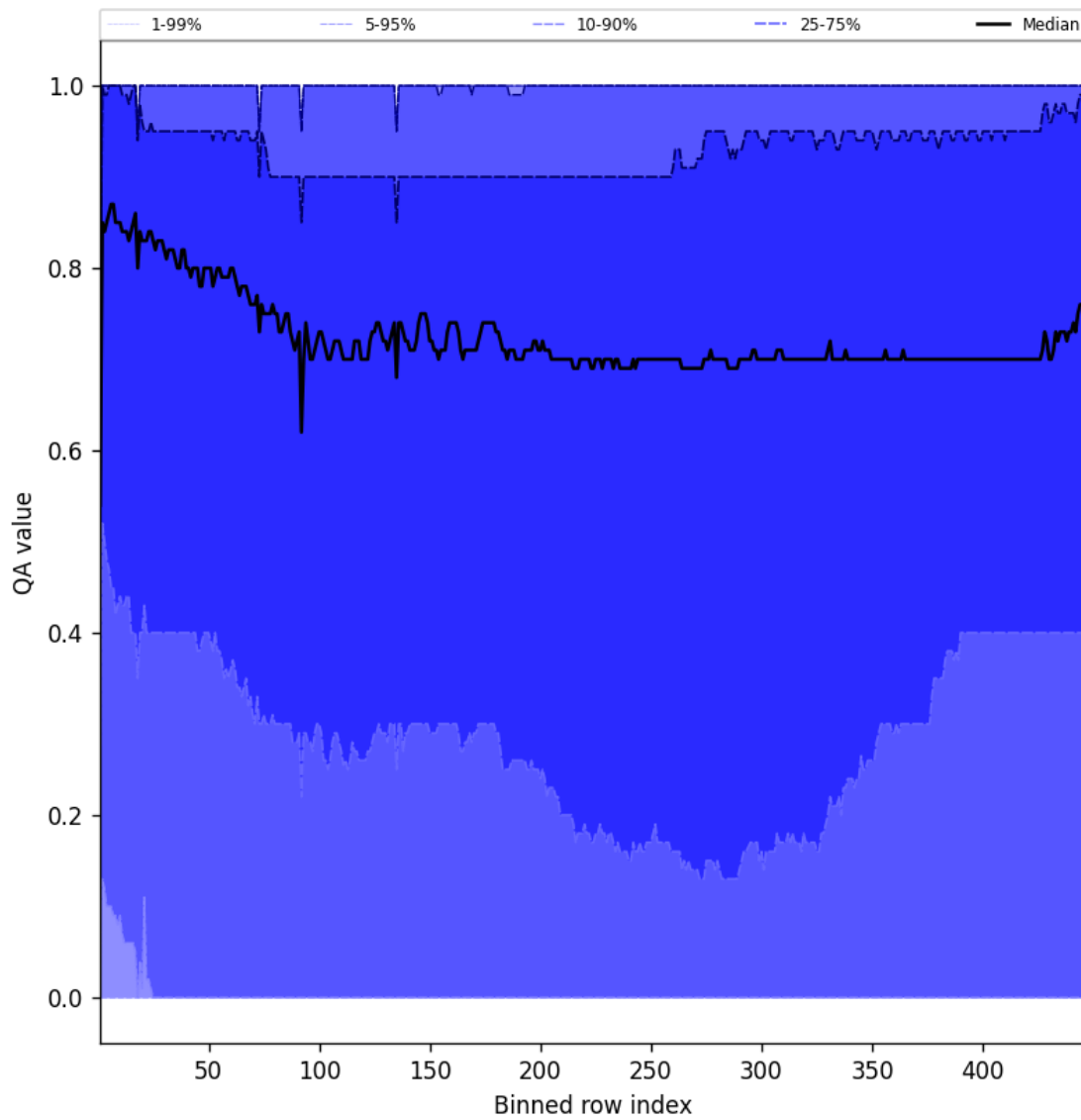
Figure 54: Along track statistics of “QA value” for 2025-05-16 to 2025-05-18
