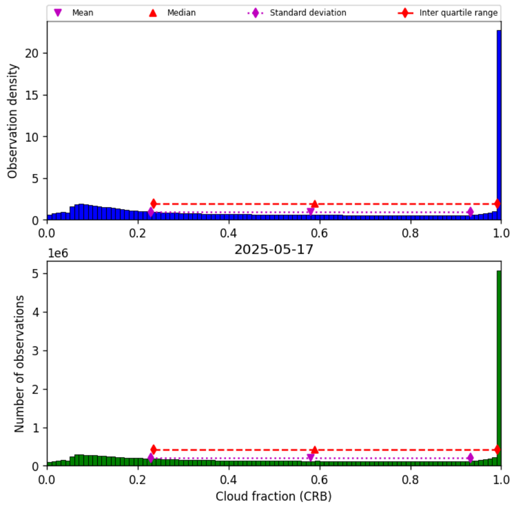
Figure 42: Histogram of “Cloud fraction (CRB)” for 2025-05-16 to 2025-05-18
