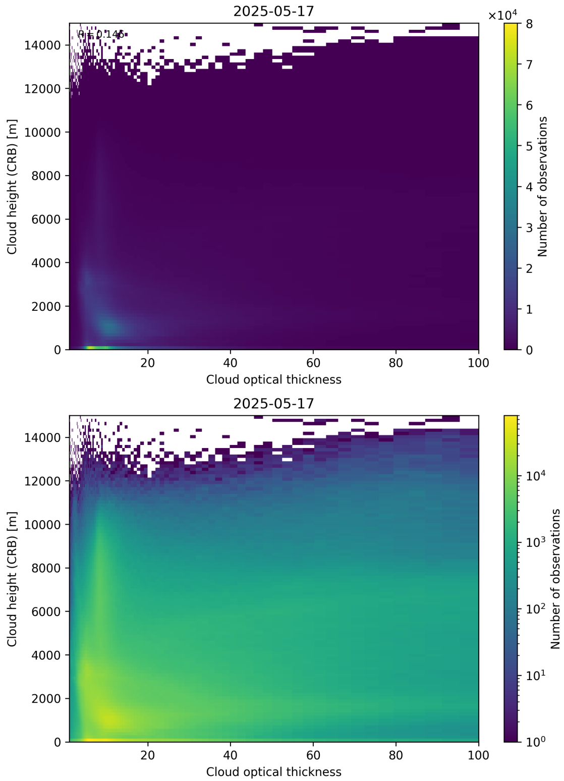
Figure 85: Scatter density plot of “Cloud optical thickness” against “Cloud height (CRB)” for 2025-05-16 to 2025-05-18.
