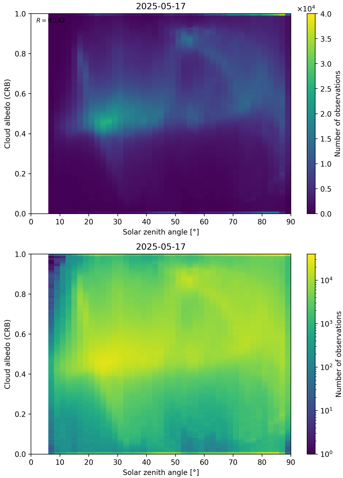
Figure 98: Scatter density plot of “Solar zenith angle” against “Cloud albedo (CRB)” for 2025-05-16 to 2025-05-18.
