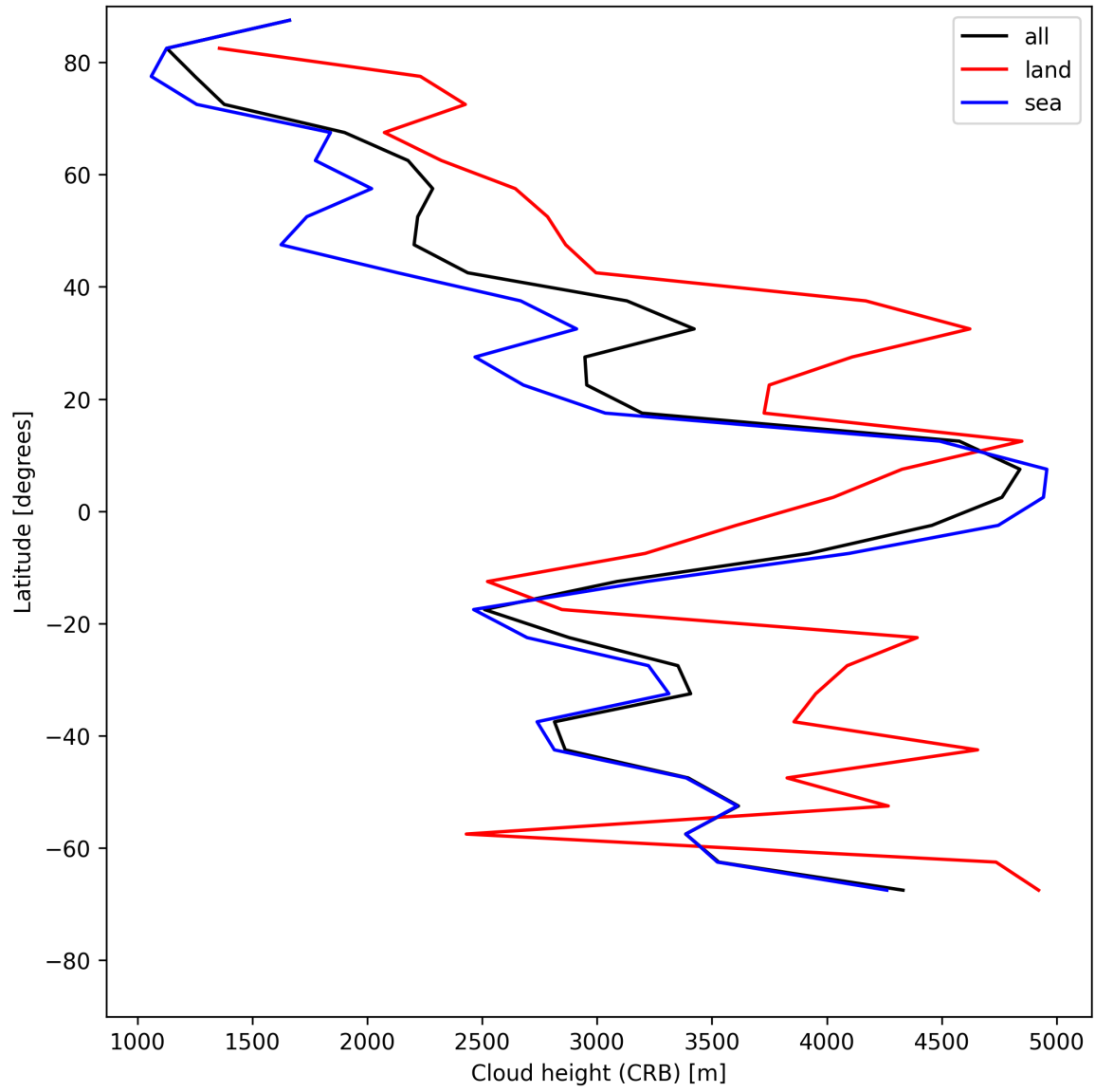
Figure 27: Zonal average of “Cloud height (CRB)” for 2025-05-16 to 2025-05-18.
