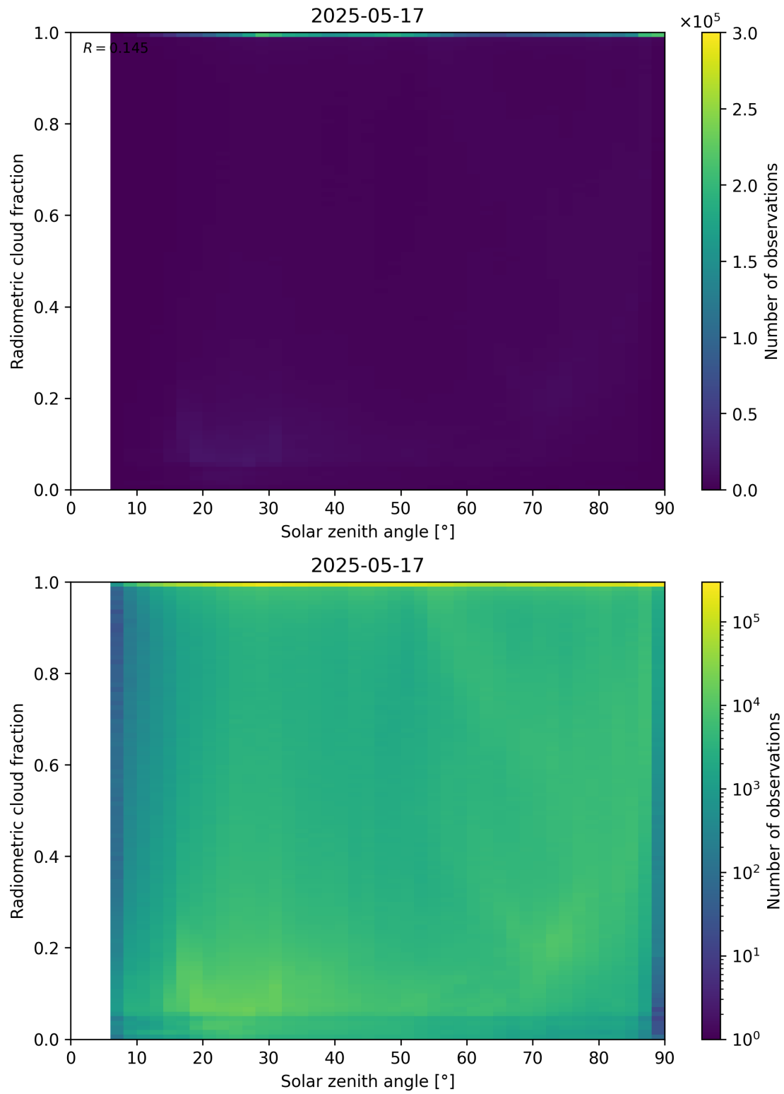
Figure 99: Scatter density plot of “Solar zenith angle” against “Radiometric cloud fraction” for 2025-05-16 to 2025-05-18.
