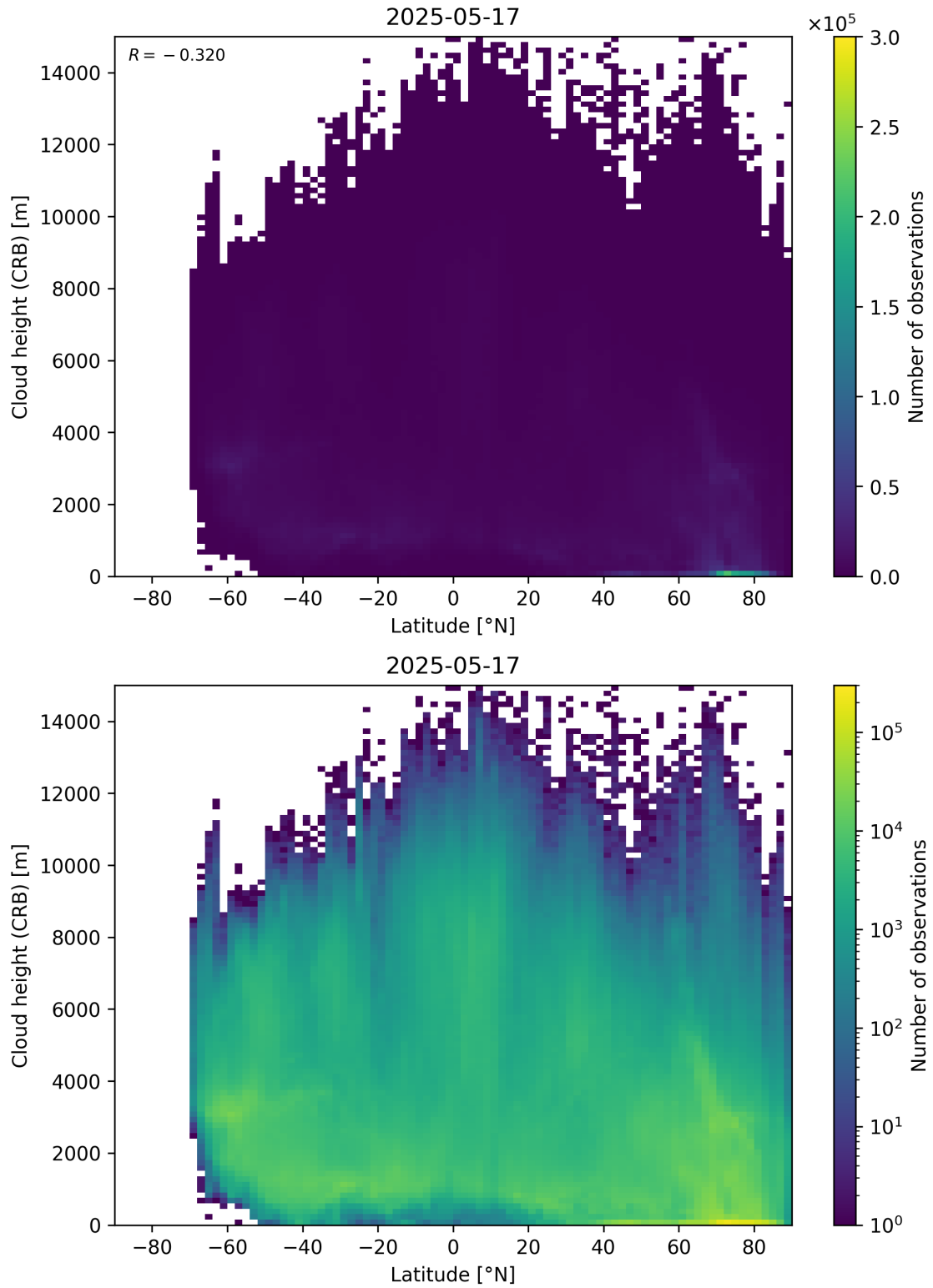
Figure 95: Scatter density plot of “Latitude” against “Cloud height (CRB)” for 2025-05-16 to 2025-05-18.
