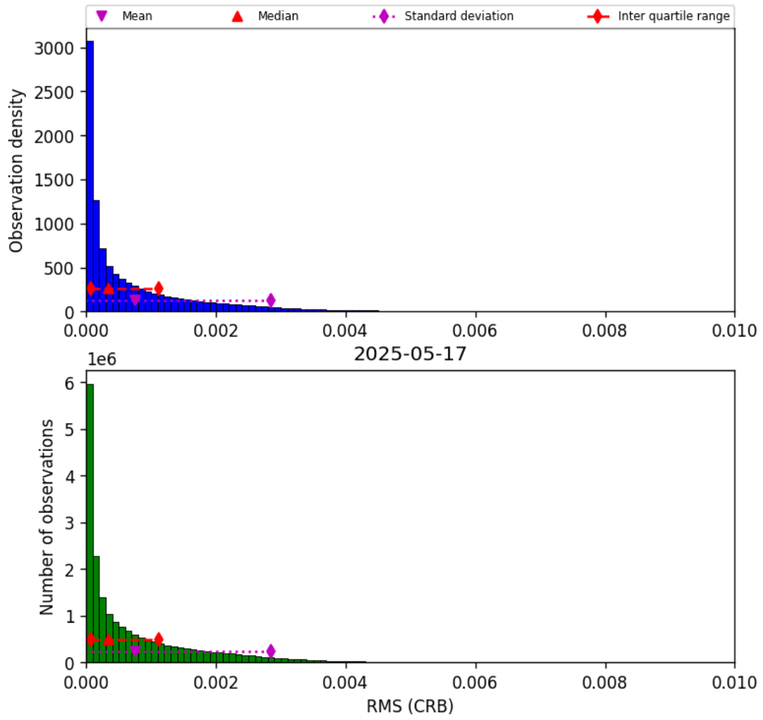
Figure 48: Histogram of “RMS (CRB)” for 2025-05-16 to 2025-05-18
