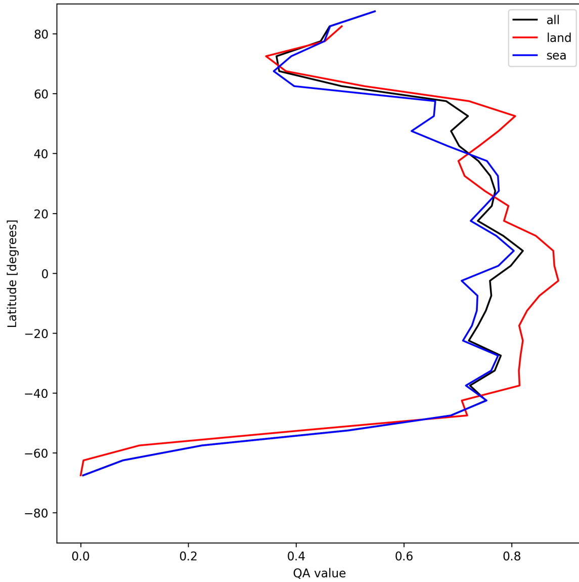
Figure 22: Zonal average of “QA value” for 2025-05-16 to 2025-05-18.
