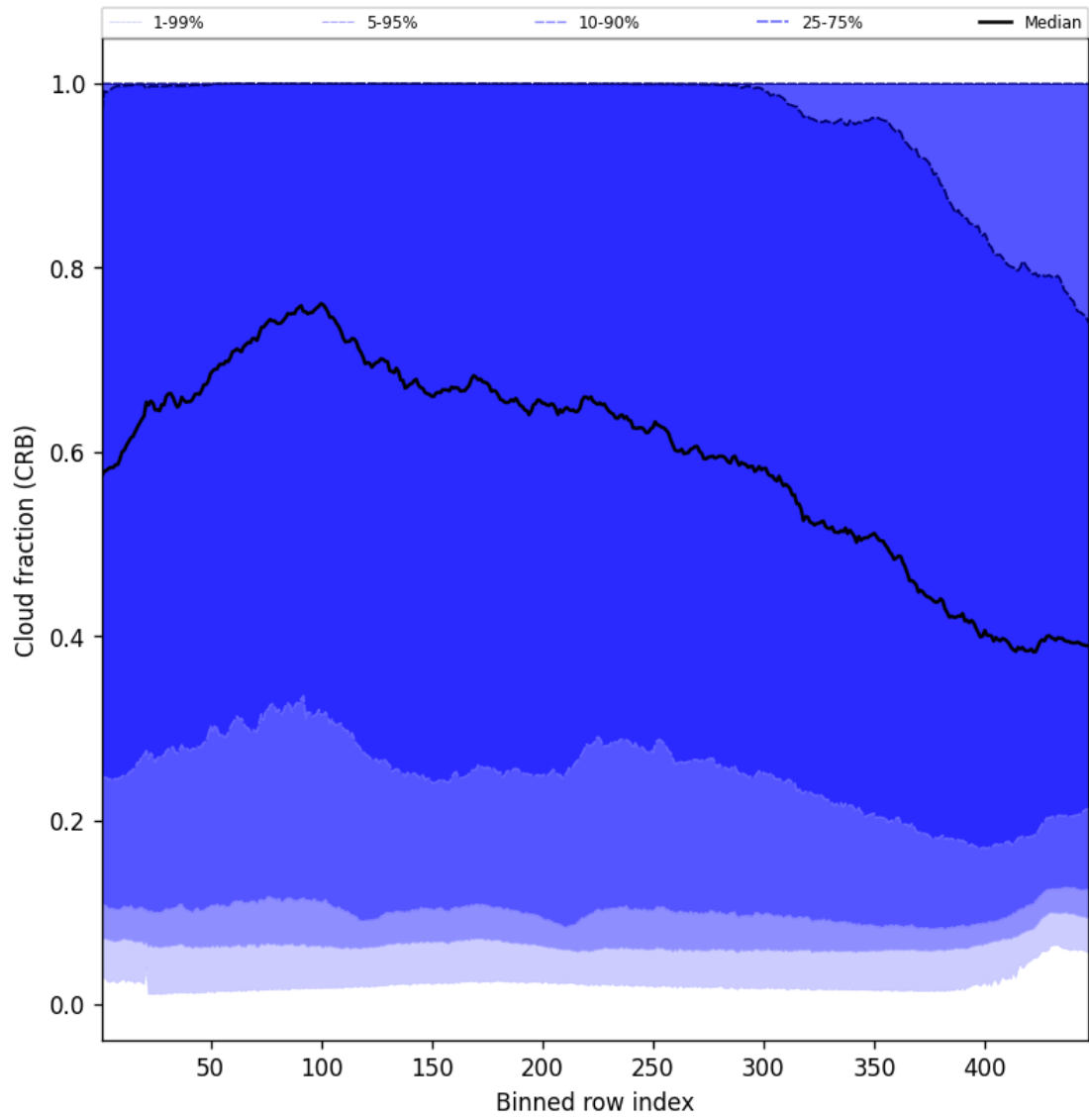
Figure 58: Along track statistics of “Cloud fraction (CRB)” for 2025-05-16 to 2025-05-18
