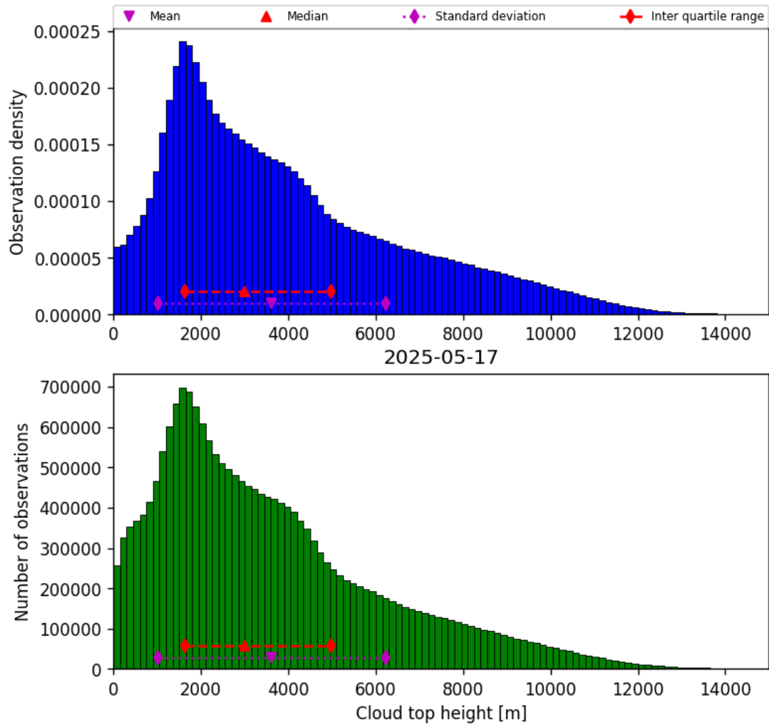
Figure 40: Histogram of “Cloud top height” for 2025-05-16 to 2025-05-18
