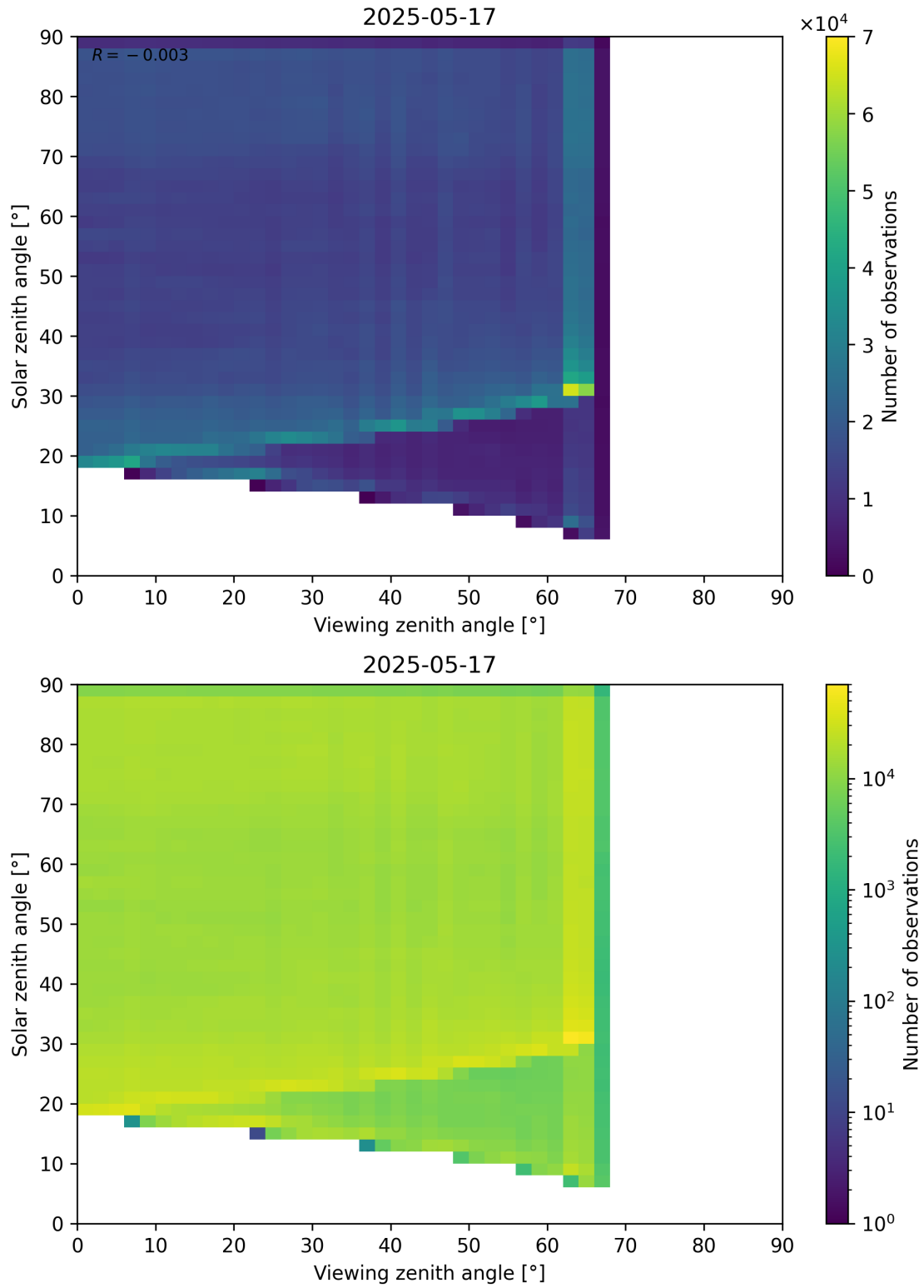
Figure 114: Scatter density plot of “Viewing zenith angle” against “Solar zenith angle” for 2025-05-16 to 2025-05-18.
