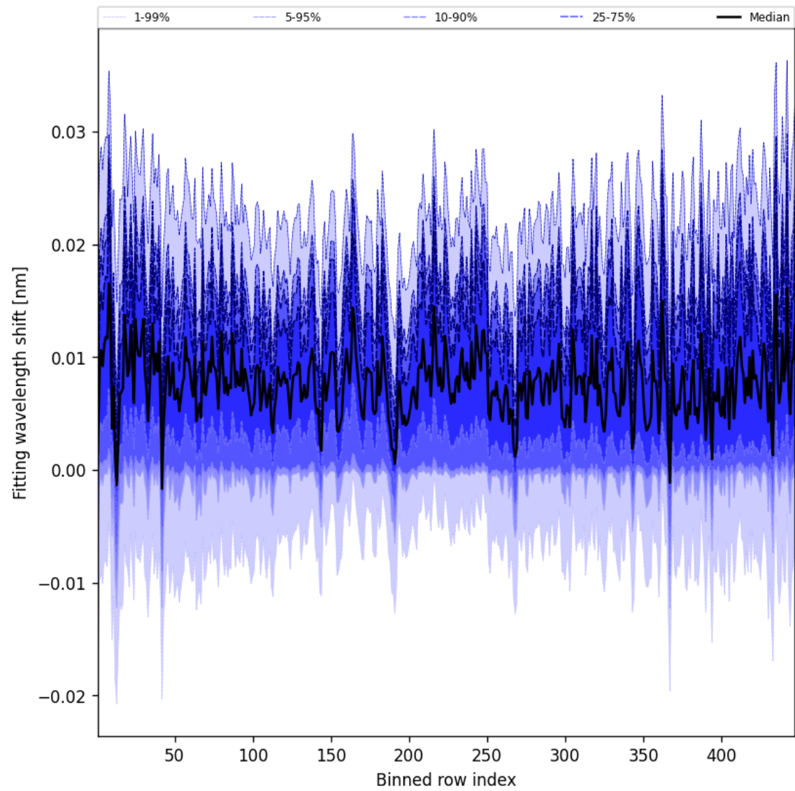
Figure 65: Along track statistics of “Fitting wavelength shift” for 2025-05-16 to 2025-05-18
