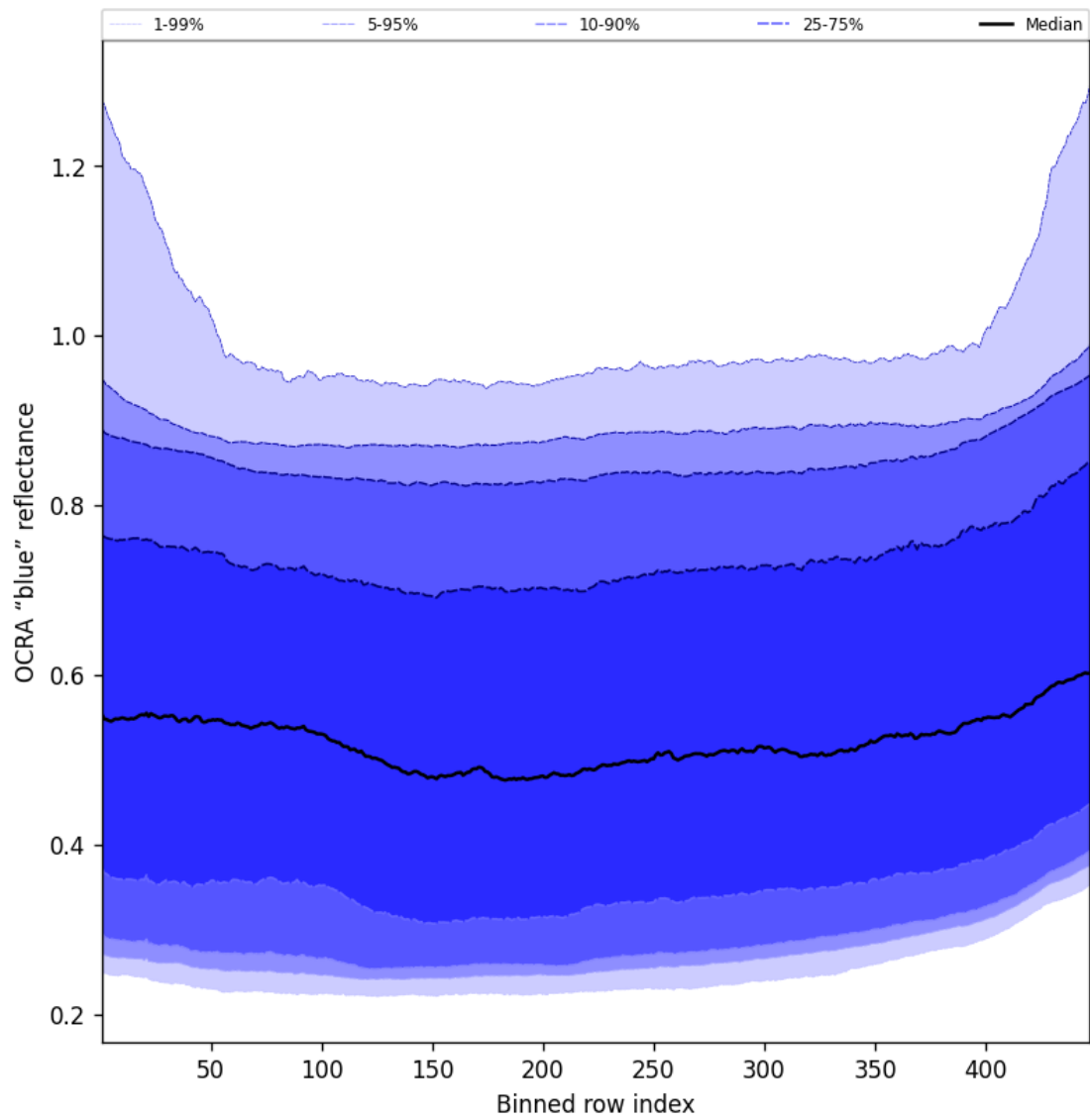
Figure 67: Along track statistics of “OCRA “blue” reflectance” for 2025-05-16 to 2025-05-18
