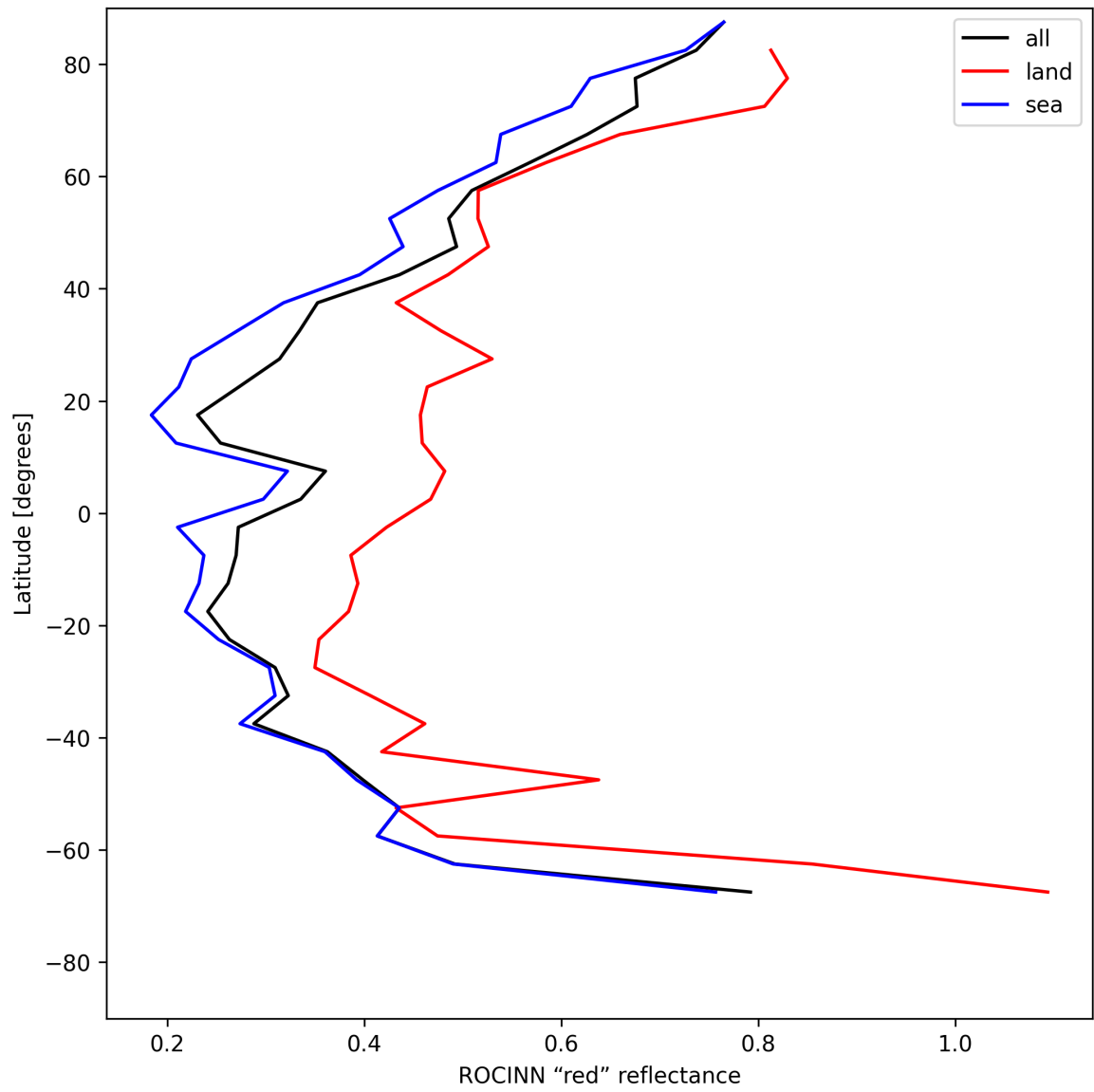
Figure 37: Zonal average of “ROCINN “red” reflectance” for 2025-05-16 to 2025-05-18.
