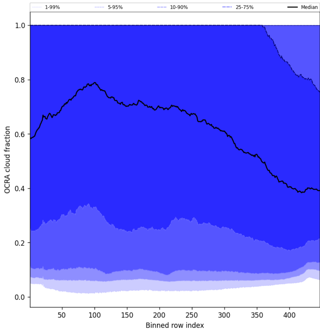
Figure 66: Along track statistics of “OCRA cloud fraction” for 2025-05-16 to 2025-05-18
