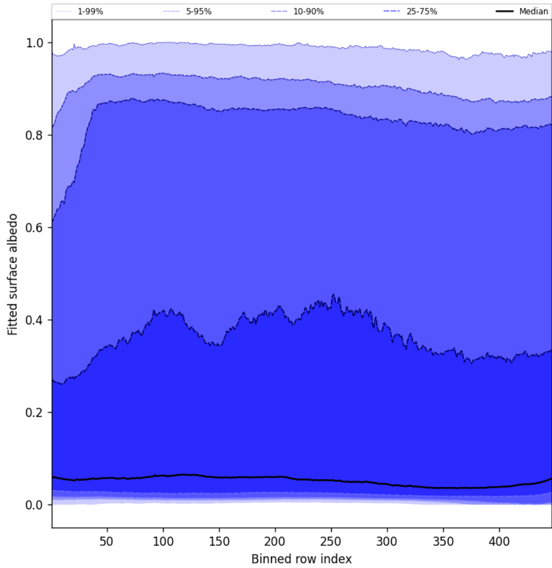
Figure 61: Along track statistics of “Fitted surface albedo” for 2025-05-16 to 2025-05-18
