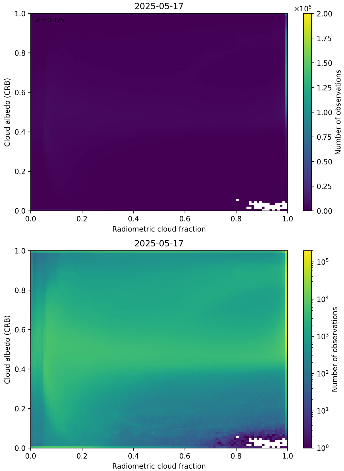
Figure 71: Scatter density plot of “Radiometric cloud fraction” against “Cloud albedo (CRB)” for 2025-05-16 to 2025-05-18.
