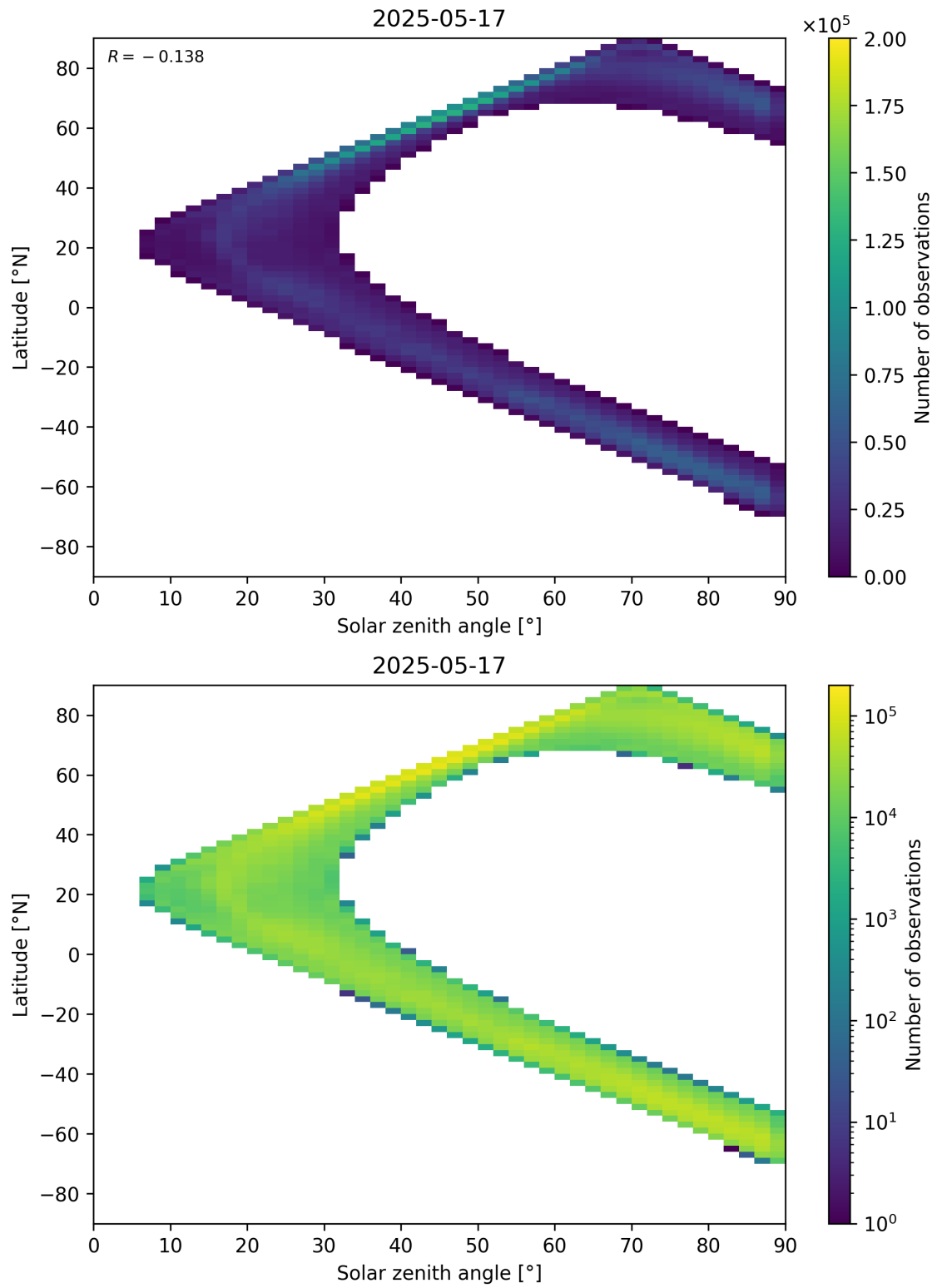
Figure 105: Scatter density plot of “Solar zenith angle” against “Latitude” for 2025-05-16 to 2025-05-18.
