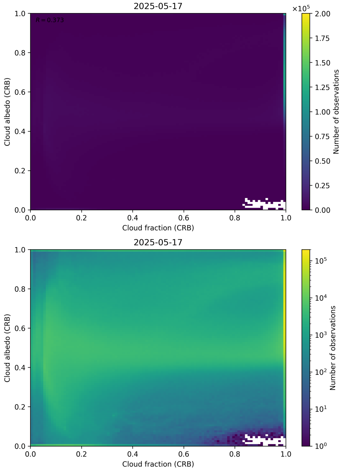
Figure 77: Scatter density plot of “Cloud fraction (CRB)” against “Cloud albedo (CRB)” for 2025-05-16 to 2025-05-18.
