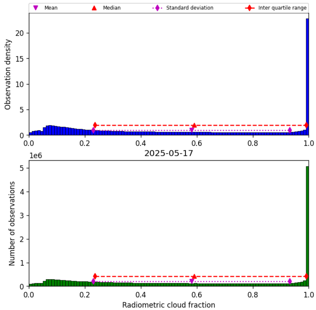
Figure 39: Histogram of “Radiometric cloud fraction” for 2025-05-16 to 2025-05-18
