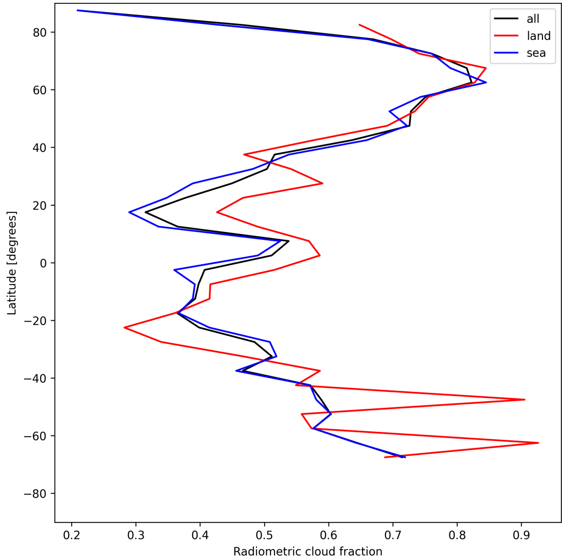
Figure 23: Zonal average of “Radiometric cloud fraction” for 2025-05-16 to 2025-05-18.
