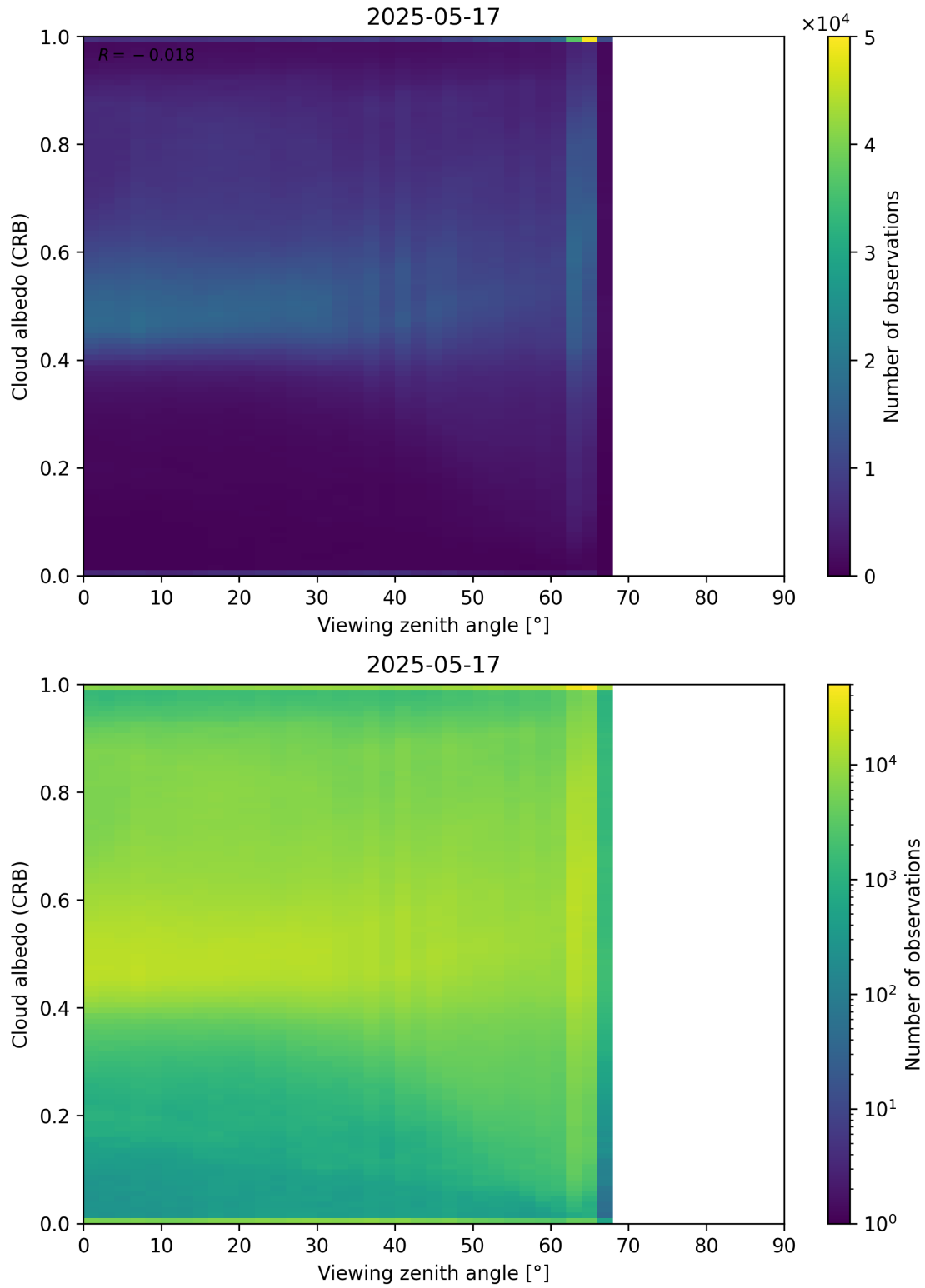
Figure 106: Scatter density plot of “Viewing zenith angle” against “Cloud albedo (CRB)” for 2025-05-16 to 2025-05-18.
