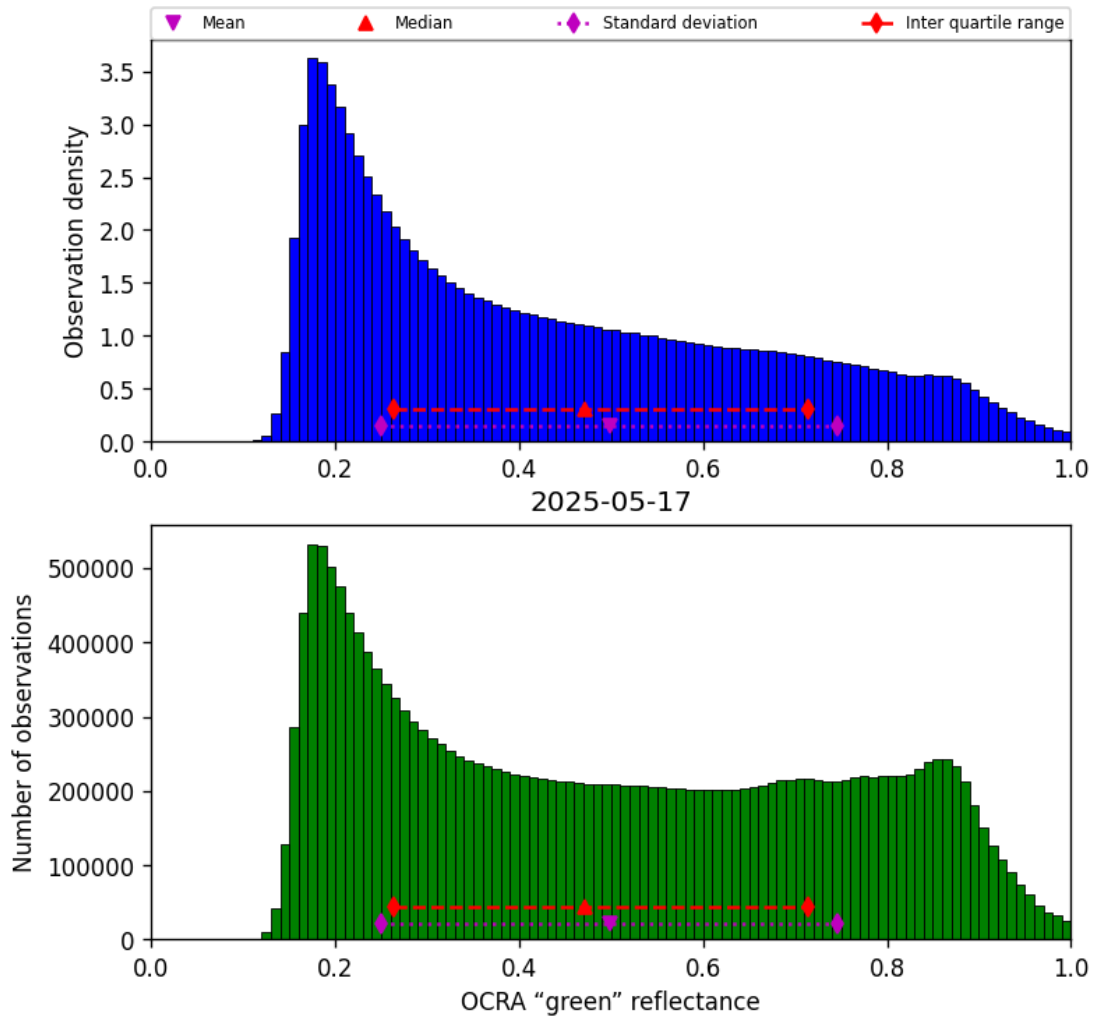
Figure 52: Histogram of “OCRA “green” reflectance” for 2025-05-16 to 2025-05-18
