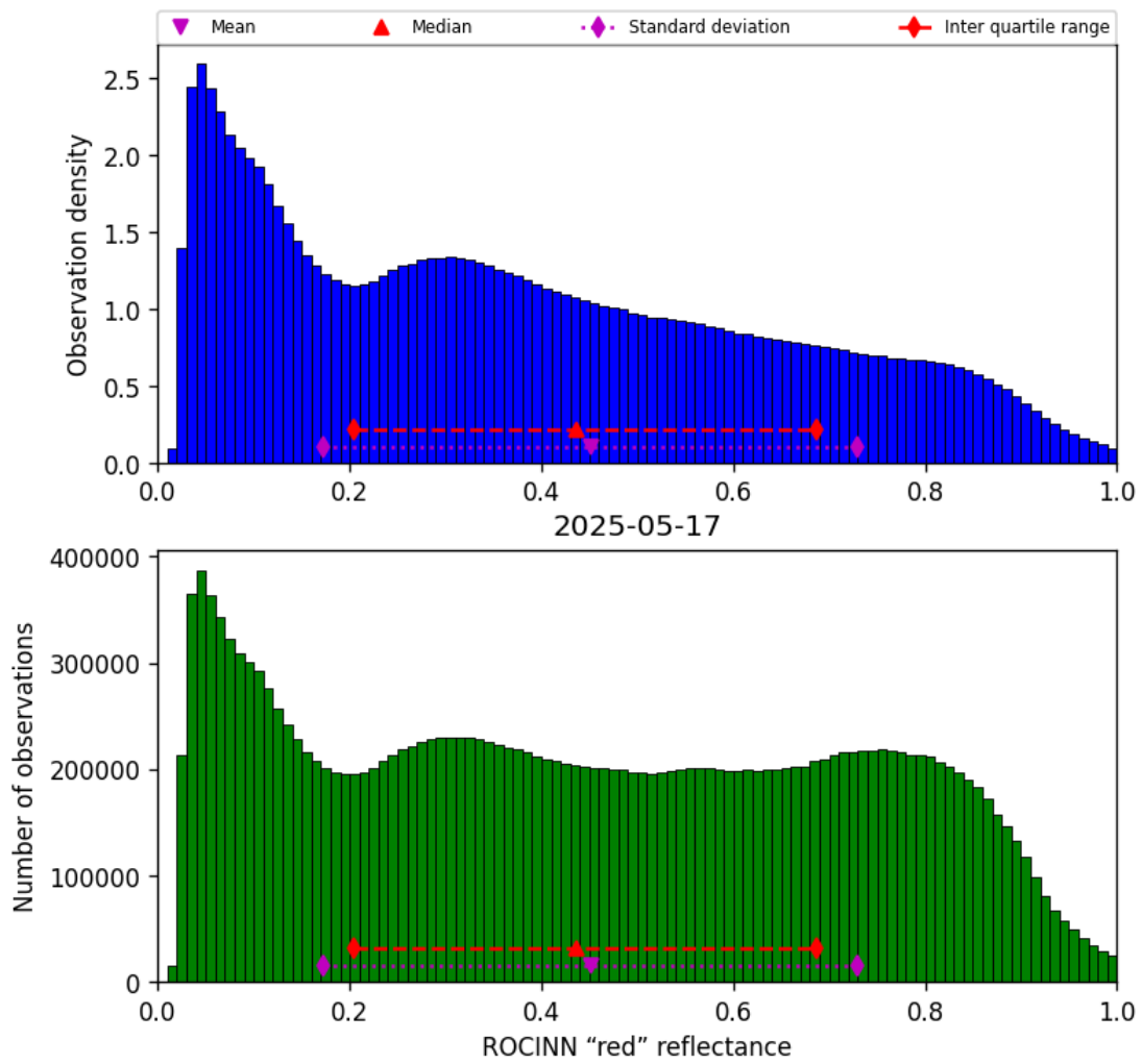
Figure 53: Histogram of “ROCINN “red” reflectance” for 2025-05-16 to 2025-05-18
