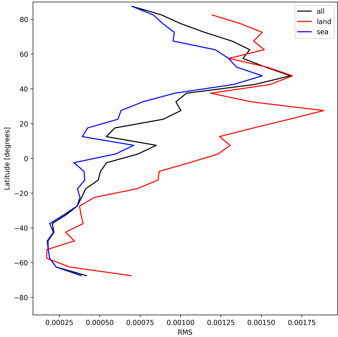
Figure 31: Zonal average of “RMS” for 2025-05-16 to 2025-05-18.
