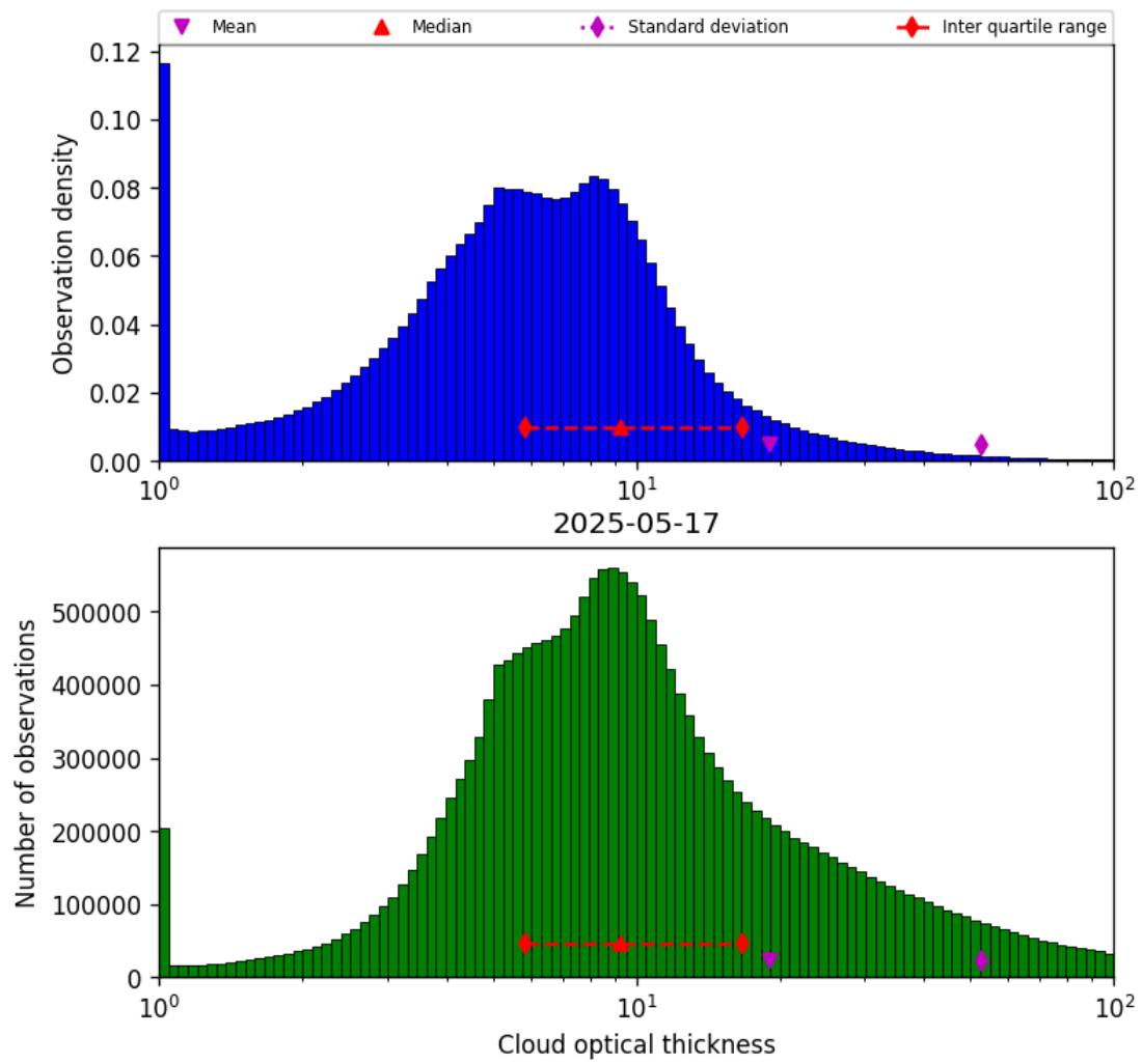
Figure 41: Histogram of “Cloud optical thickness” for 2025-05-16 to 2025-05-18
