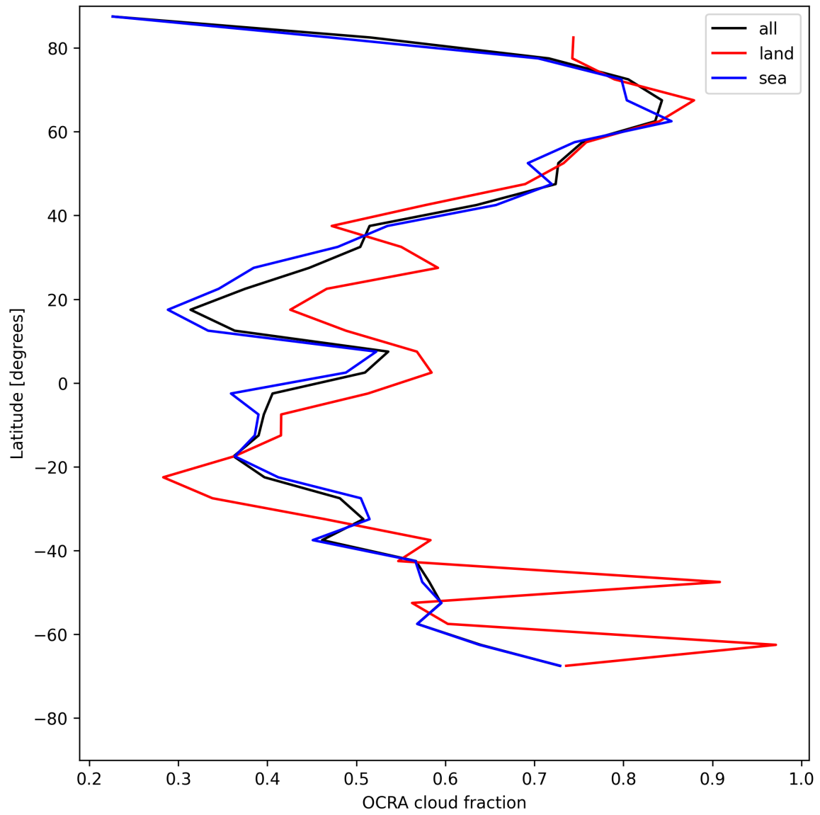
Figure 34: Zonal average of “OCRA cloud fraction” for 2025-05-16 to 2025-05-18.
