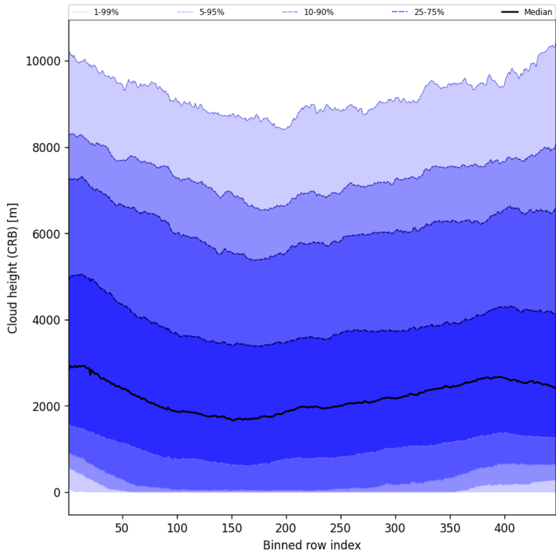
Figure 59: Along track statistics of “Cloud height (CRB)” for 2025-05-16 to 2025-05-18
