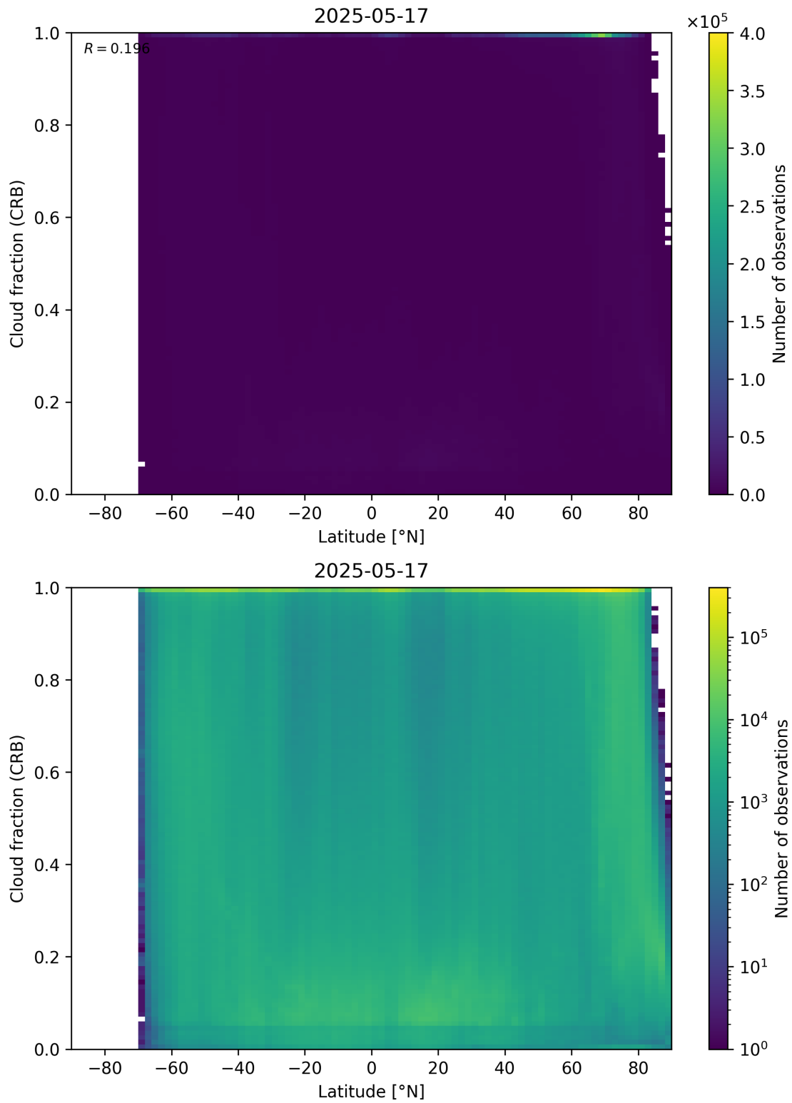
Figure 94: Scatter density plot of “Latitude” against “Cloud fraction (CRB)” for 2025-05-16 to 2025-05-18.
