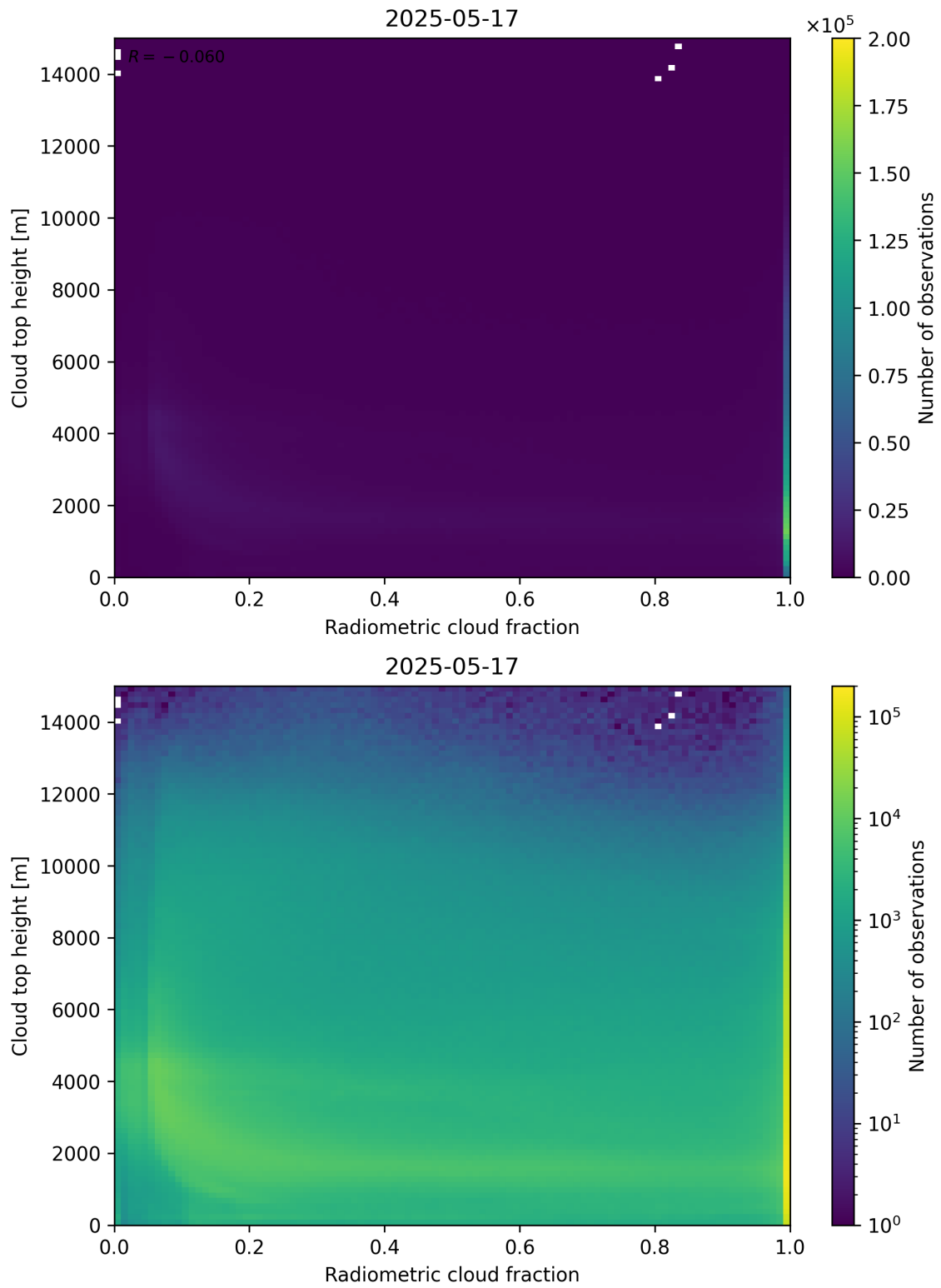
Figure 76: Scatter density plot of “Radiometric cloud fraction” against “Cloud top height” for 2025-05-16 to 2025-05-18.
