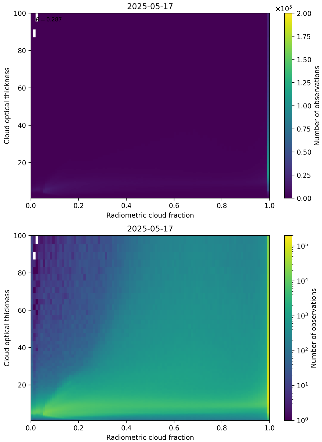
Figure 75: Scatter density plot of “Radiometric cloud fraction” against “Cloud optical thickness” for 2025-05-16 to 2025-05-18.
