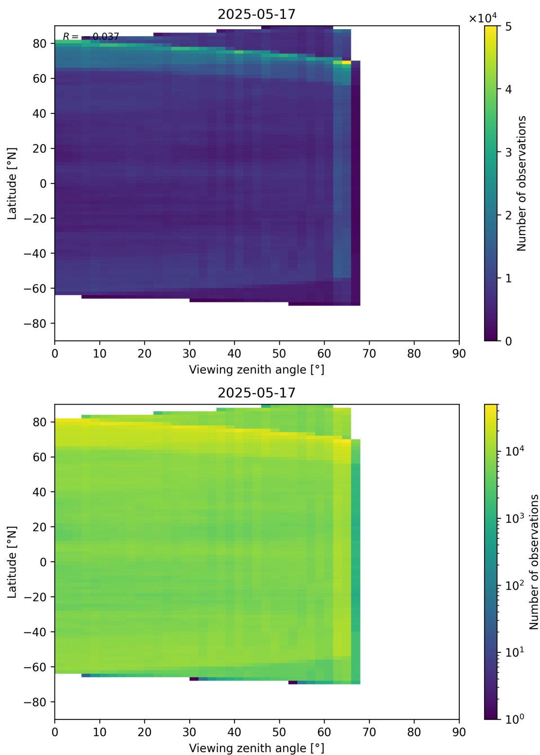
Figure 113: Scatter density plot of “Viewing zenith angle” against “Latitude” for 2025-05-16 to 2025-05-18.
