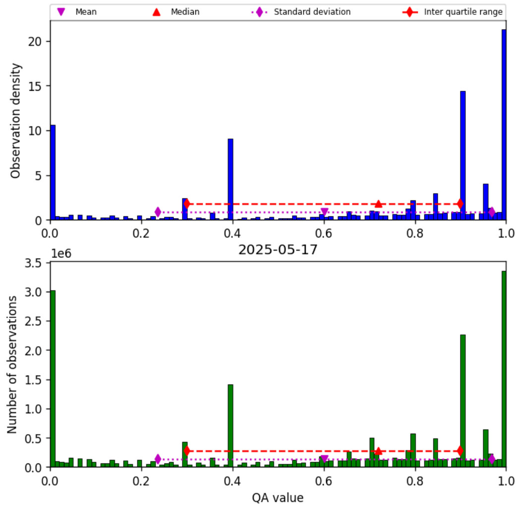
Figure 38: Histogram of “QA value” for 2025-05-16 to 2025-05-18
