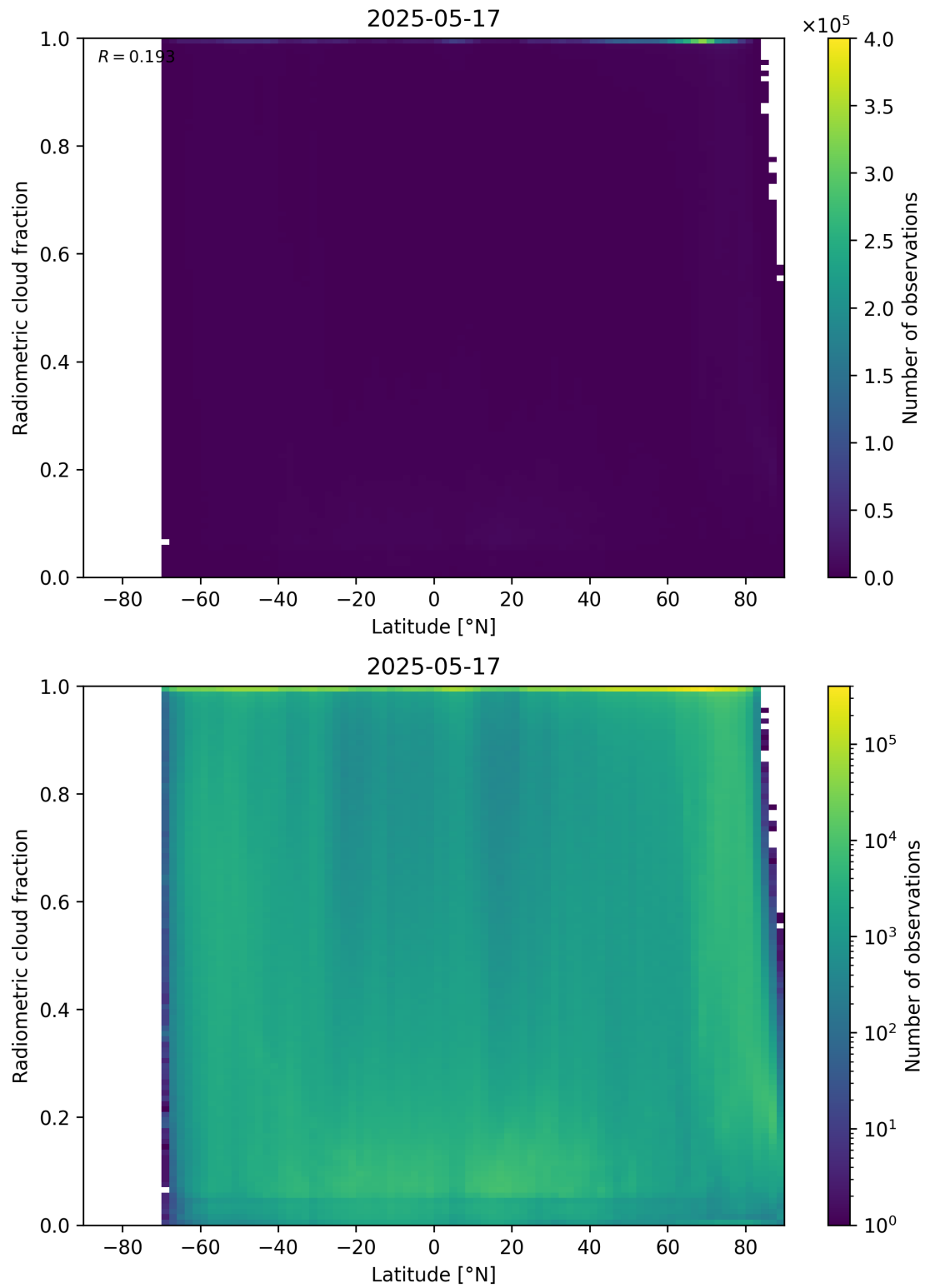
Figure 92: Scatter density plot of “Latitude” against “Radiometric cloud fraction” for 2025-05-16 to 2025-05-18.
