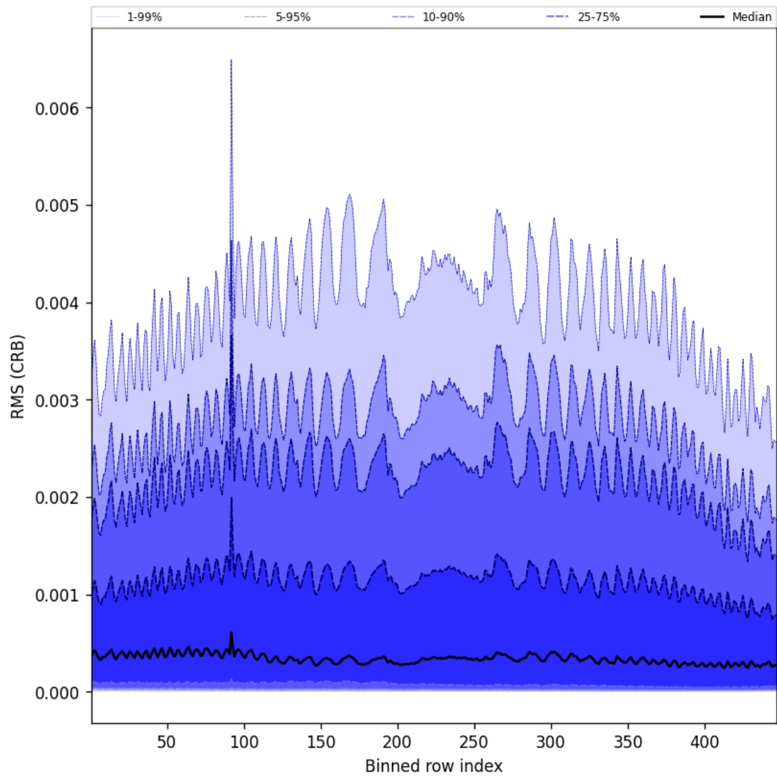
Figure 64: Along track statistics of “RMS (CRB)” for 2025-05-16 to 2025-05-18
