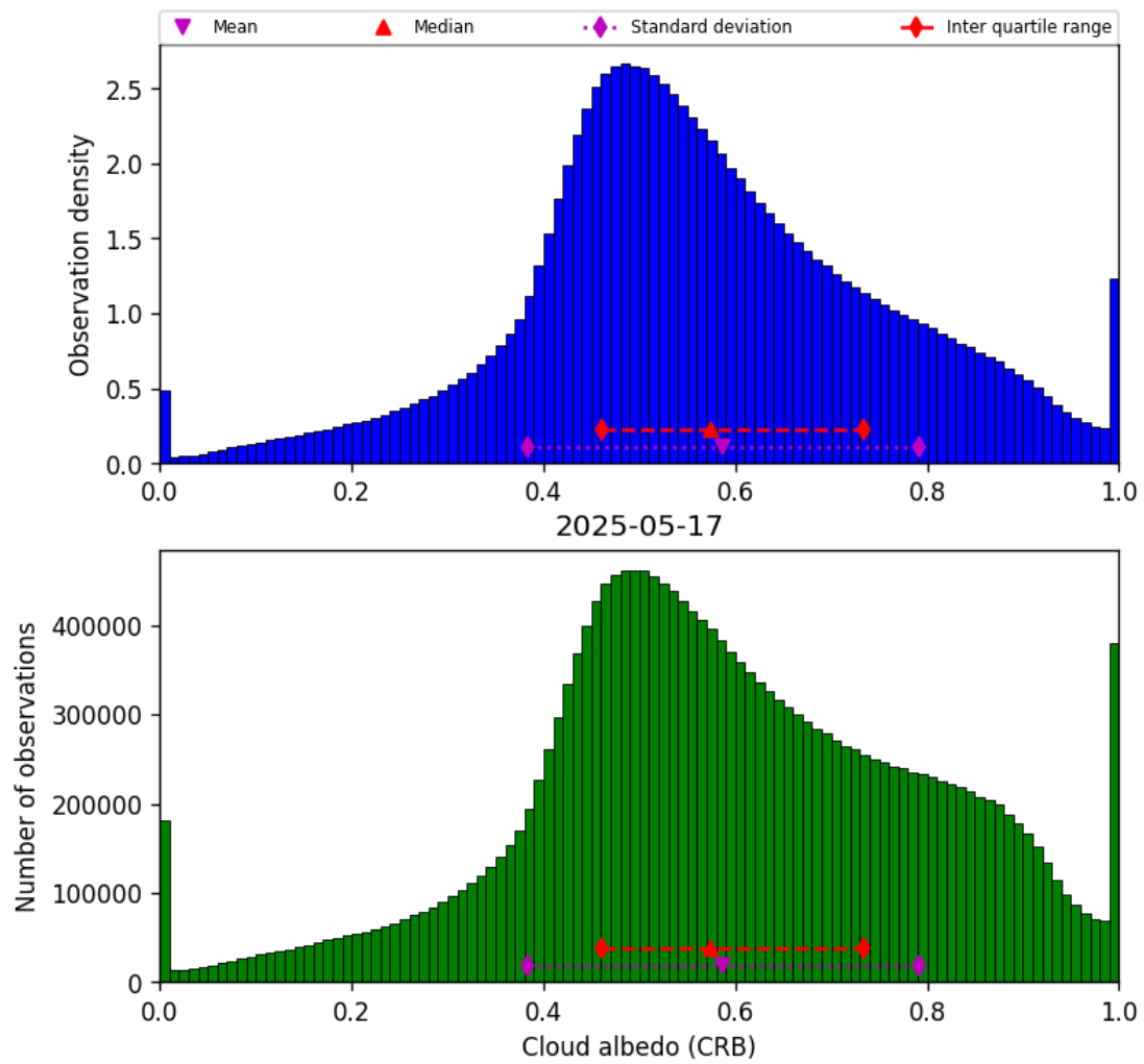
Figure 44: Histogram of “Cloud albedo (CRB)” for 2025-05-16 to 2025-05-18
