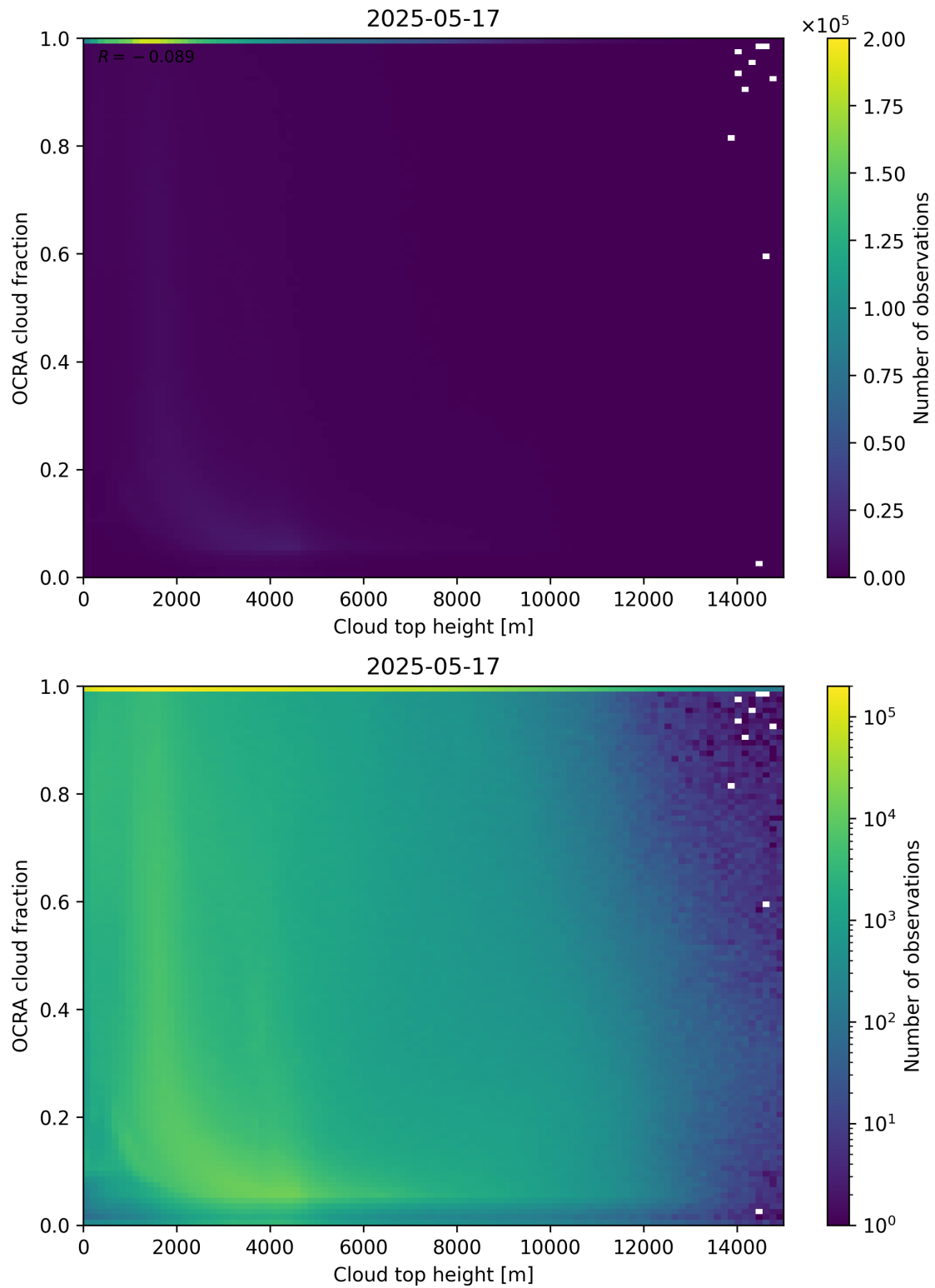
Figure 87: Scatter density plot of “Cloud top height” against “OCRA cloud fraction” for 2025-05-16 to 2025-05-18.
