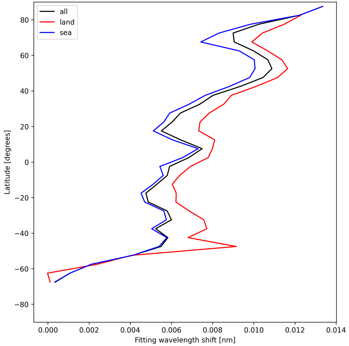
Figure 33: Zonal average of “Fitting wavelength shift” for 2025-05-16 to 2025-05-18.
