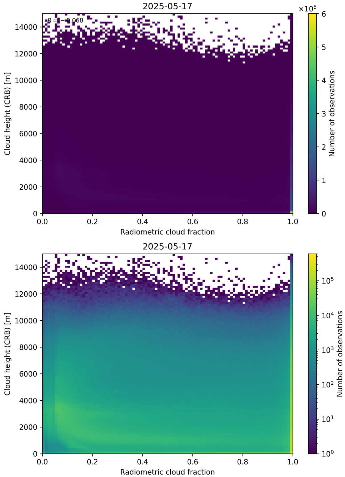
Figure 74: Scatter density plot of “Radiometric cloud fraction” against “Cloud height (CRB)” for 2025-05-16 to 2025-05-18.
