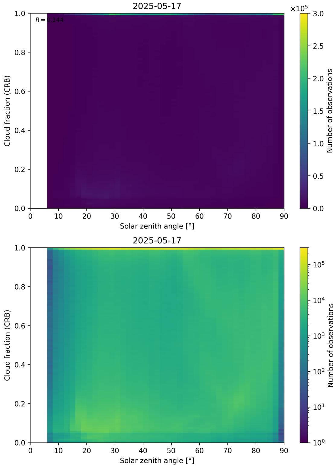
Figure 101: Scatter density plot of “Solar zenith angle” against “Cloud fraction (CRB)” for 2025-05-16 to 2025-05-18.
