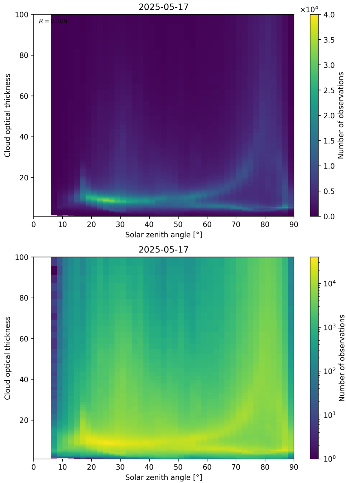
Figure 103: Scatter density plot of “Solar zenith angle” against “Cloud optical thickness” for 2025-05-16 to 2025-05-18.
