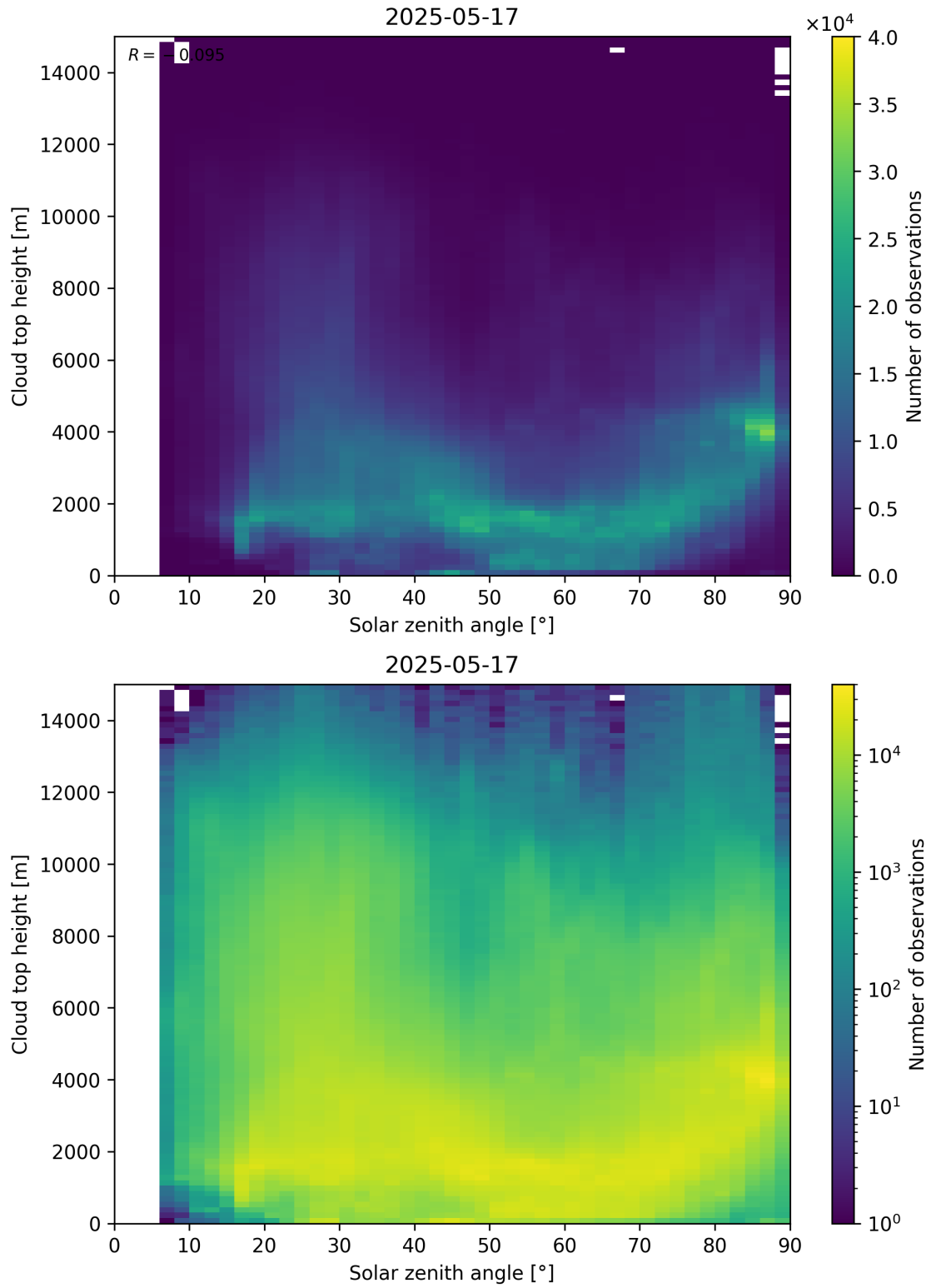
Figure 104: Scatter density plot of “Solar zenith angle” against “Cloud top height” for 2025-05-16 to 2025-05-18.
