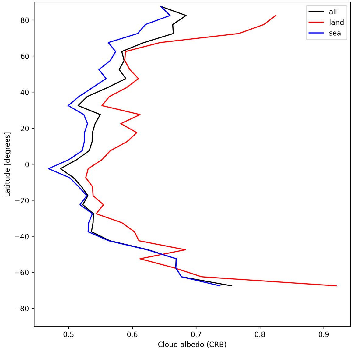
Figure 28: Zonal average of “Cloud albedo (CRB)” for 2025-05-16 to 2025-05-18.
