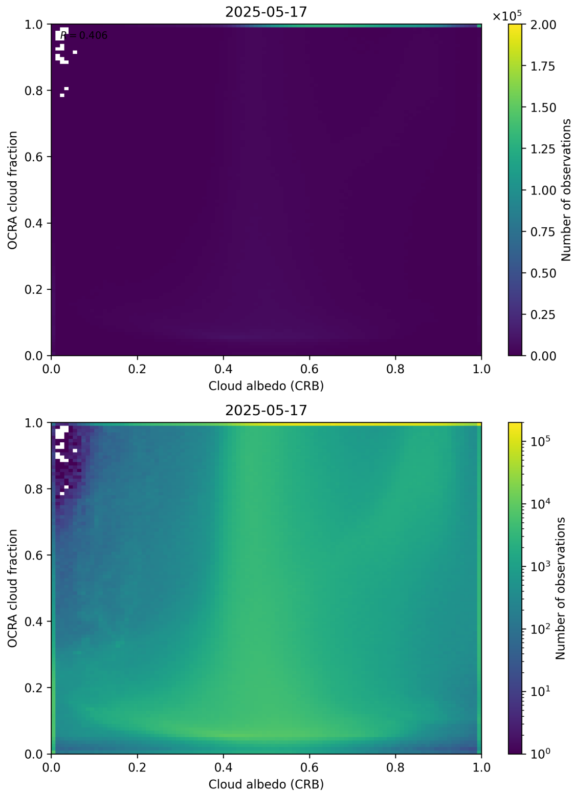
Figure 70: Scatter density plot of “Cloud albedo (CRB)” against “OCRA cloud fraction” for 2025-05-16 to 2025-05-18.
