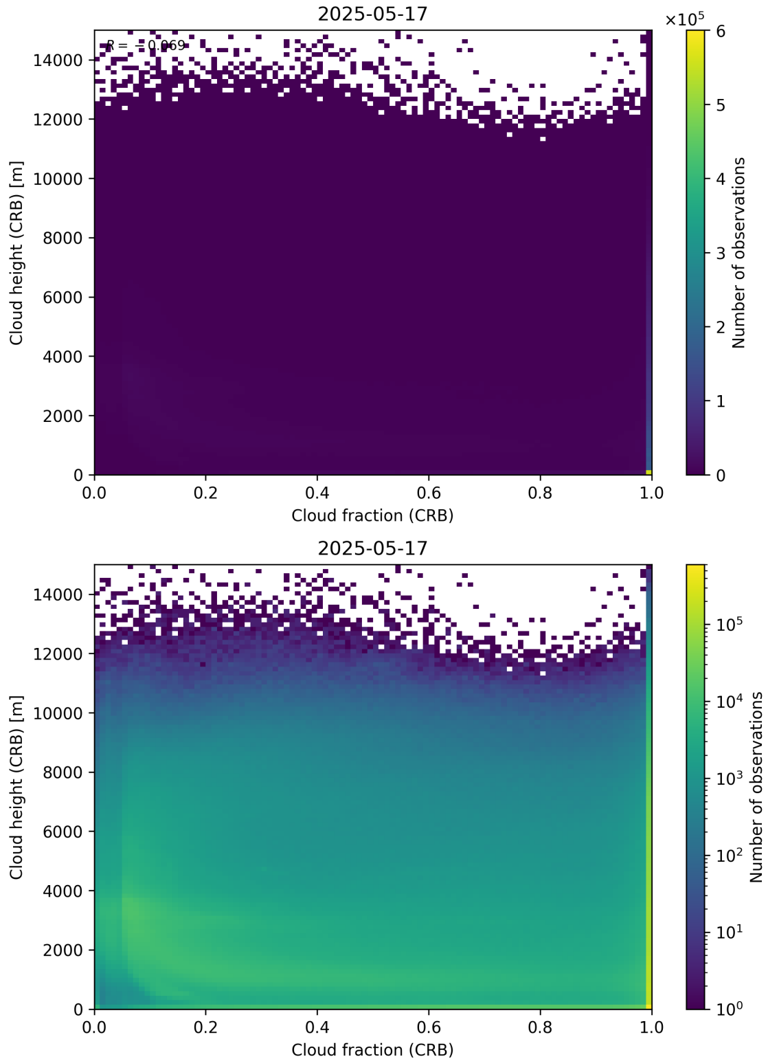
Figure 79: Scatter density plot of “Cloud fraction (CRB)” against “Cloud height (CRB)” for 2025-05-16 to 2025-05-18.
