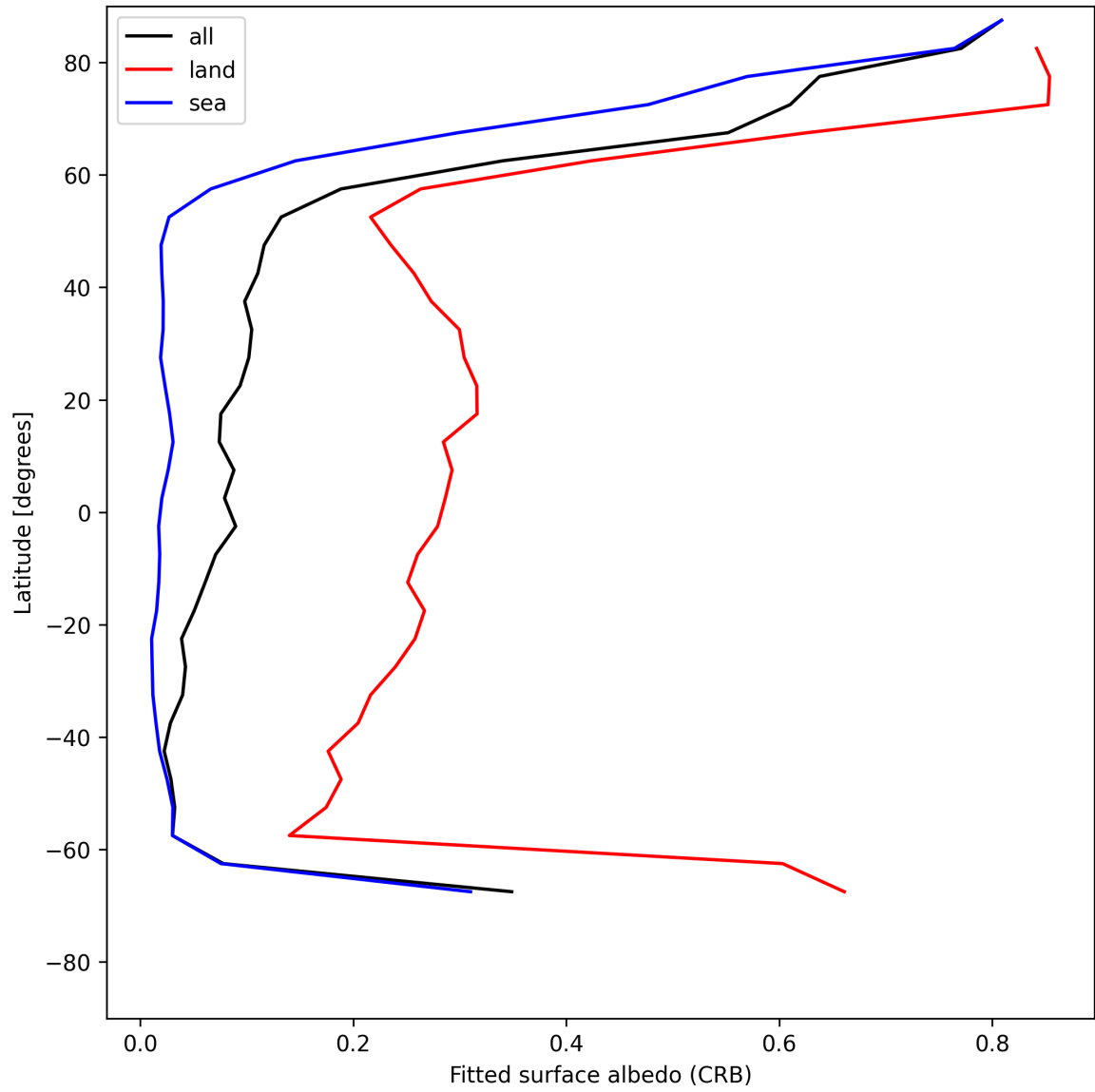
Figure 30: Zonal average of “Fitted surface albedo (CRB)” for 2025-05-16 to 2025-05-18.
