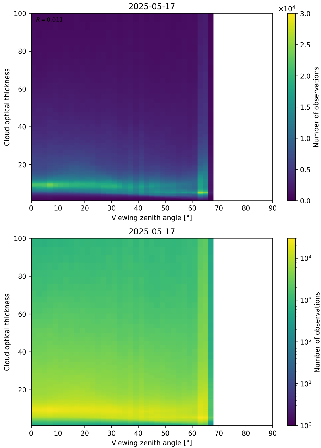
Figure 111: Scatter density plot of “Viewing zenith angle” against “Cloud optical thickness” for 2025-05-16 to 2025-05-18.
