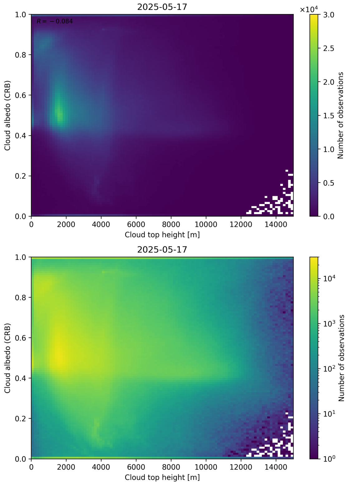
Figure 86: Scatter density plot of “Cloud top height” against “Cloud albedo (CRB)” for 2025-05-16 to 2025-05-18.
