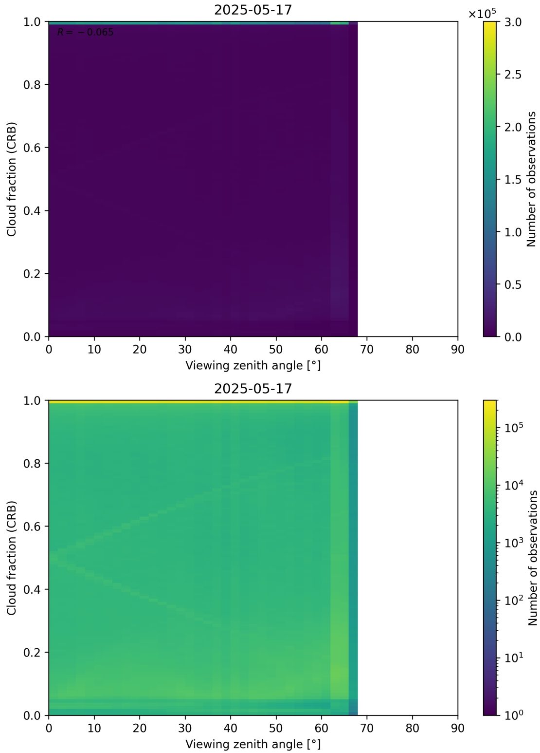
Figure 109: Scatter density plot of “Viewing zenith angle” against “Cloud fraction (CRB)” for 2025-05-16 to 2025-05-18.
