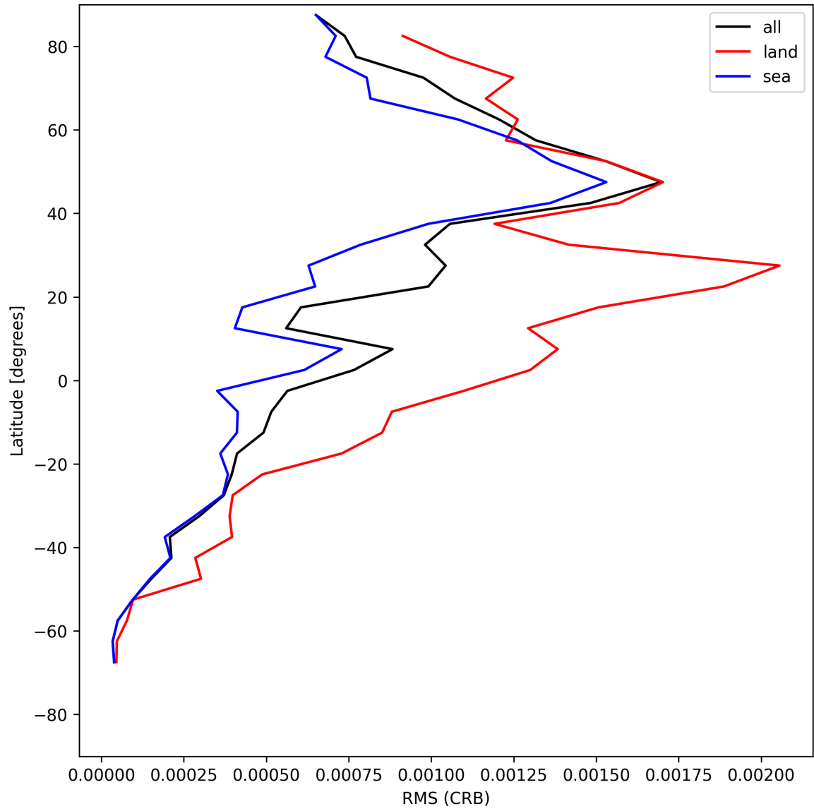
Figure 32: Zonal average of “RMS (CRB)” for 2025-05-16 to 2025-05-18.
