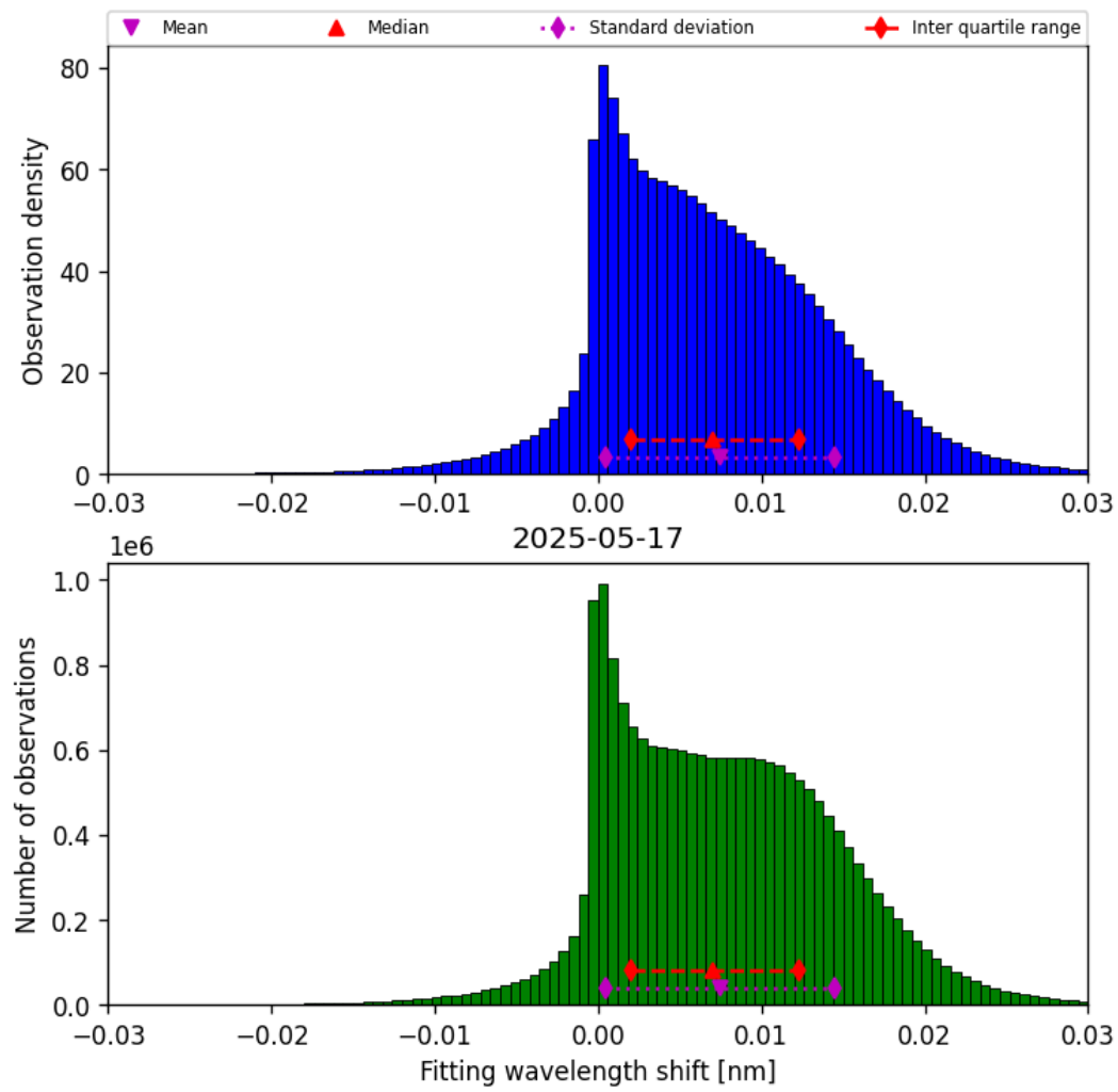
Figure 49: Histogram of “Fitting wavelength shift” for 2025-05-16 to 2025-05-18
