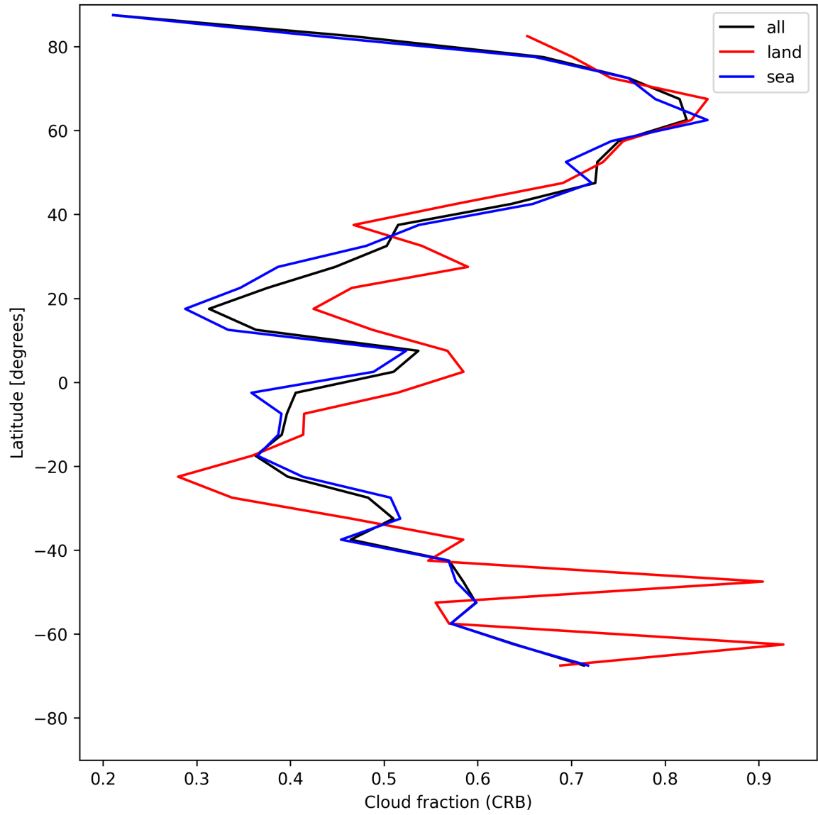
Figure 26: Zonal average of “Cloud fraction (CRB)” for 2025-05-16 to 2025-05-18.
