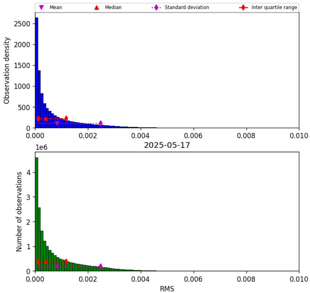
Figure 47: Histogram of “RMS” for 2025-05-16 to 2025-05-18
