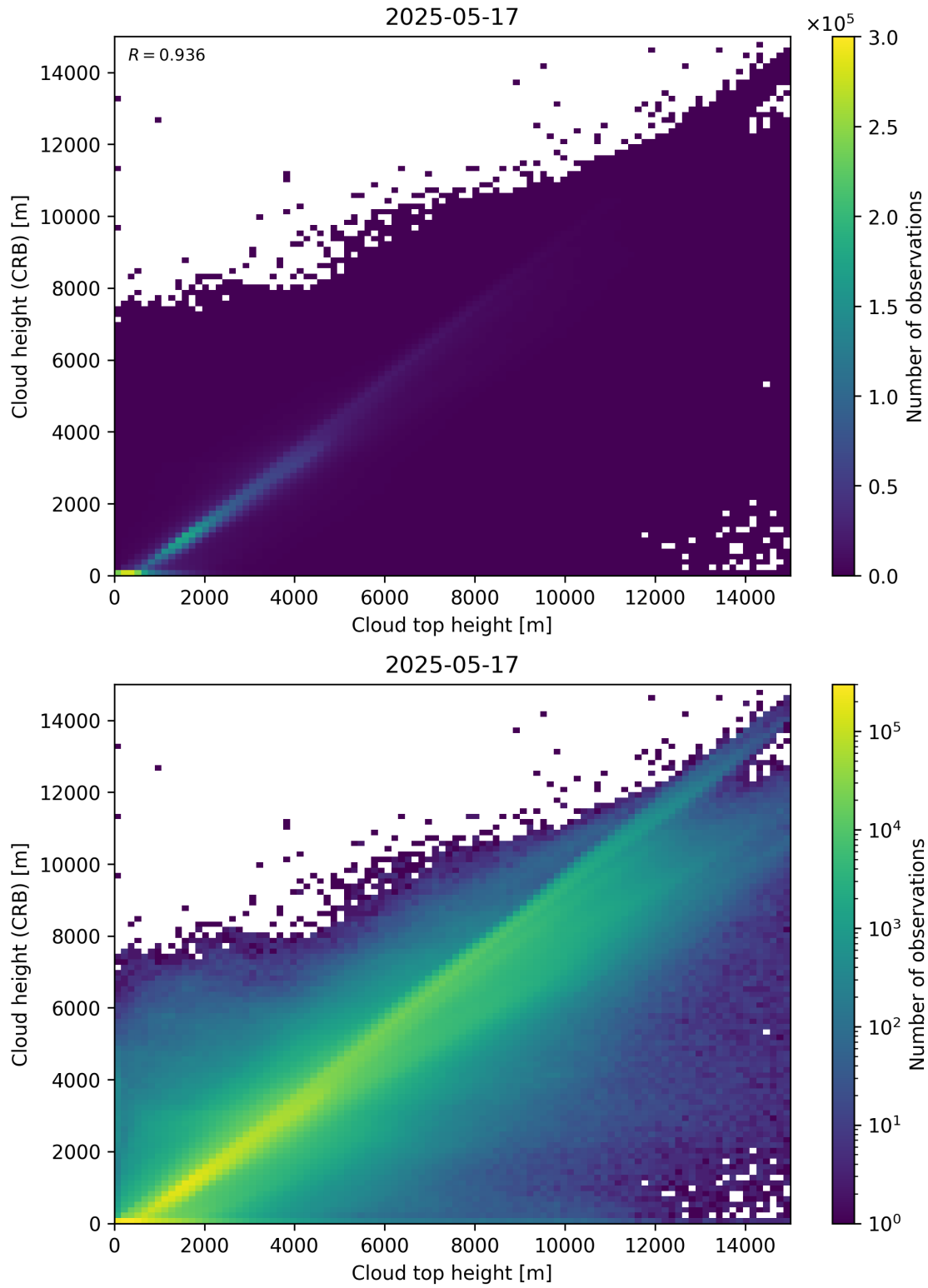
Figure 89: Scatter density plot of “Cloud top height” against “Cloud height (CRB)” for 2025-05-16 to 2025-05-18.
