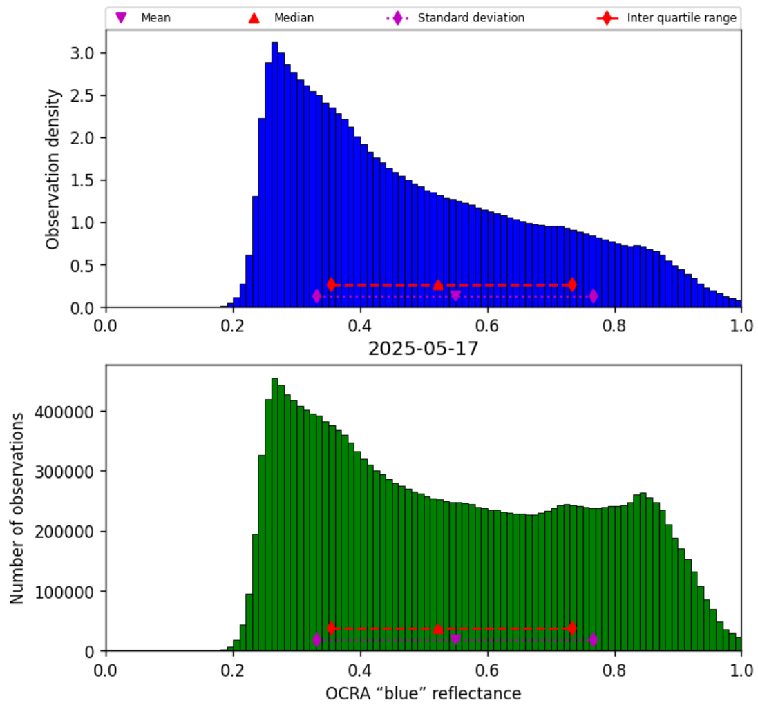
Figure 51: Histogram of “OCRA “blue” reflectance” for 2025-05-16 to 2025-05-18
