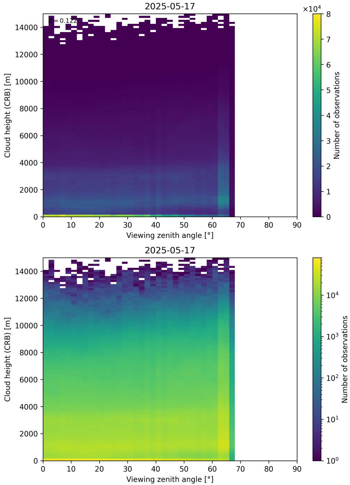
Figure 110: Scatter density plot of “Viewing zenith angle” against “Cloud height (CRB)” for 2025-05-16 to 2025-05-18.
