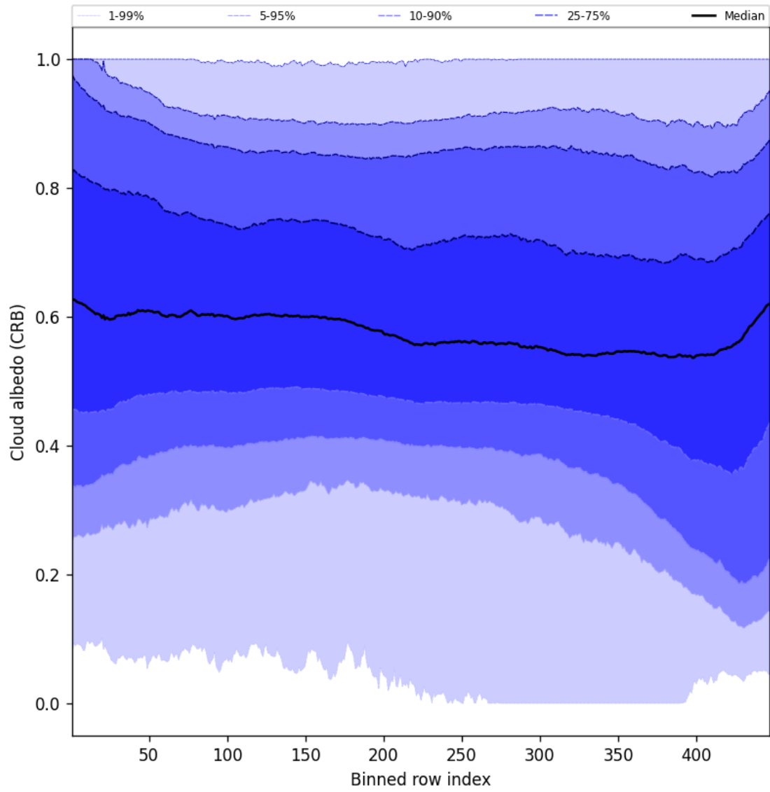
Figure 60: Along track statistics of “Cloud albedo (CRB)” for 2025-05-16 to 2025-05-18
