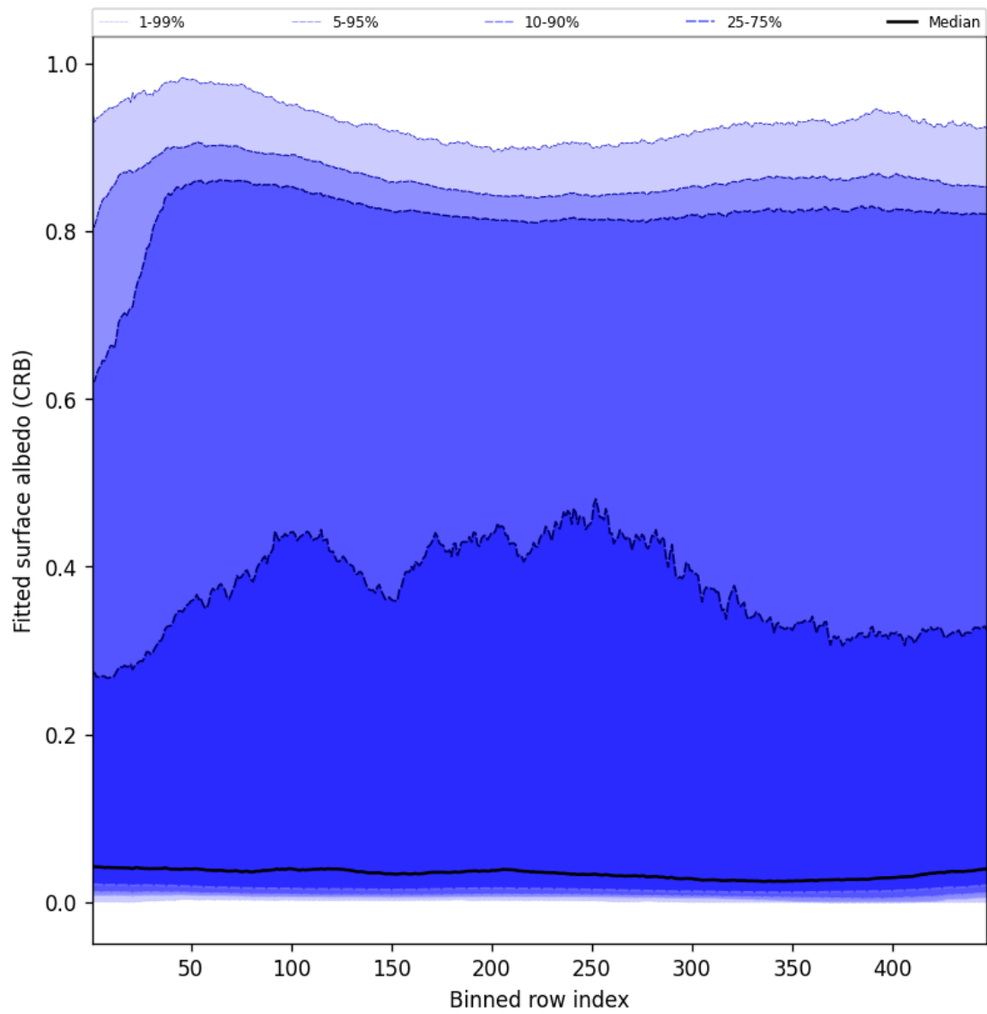
Figure 62: Along track statistics of “Fitted surface albedo (CRB)” for 2025-05-16 to 2025-05-18
