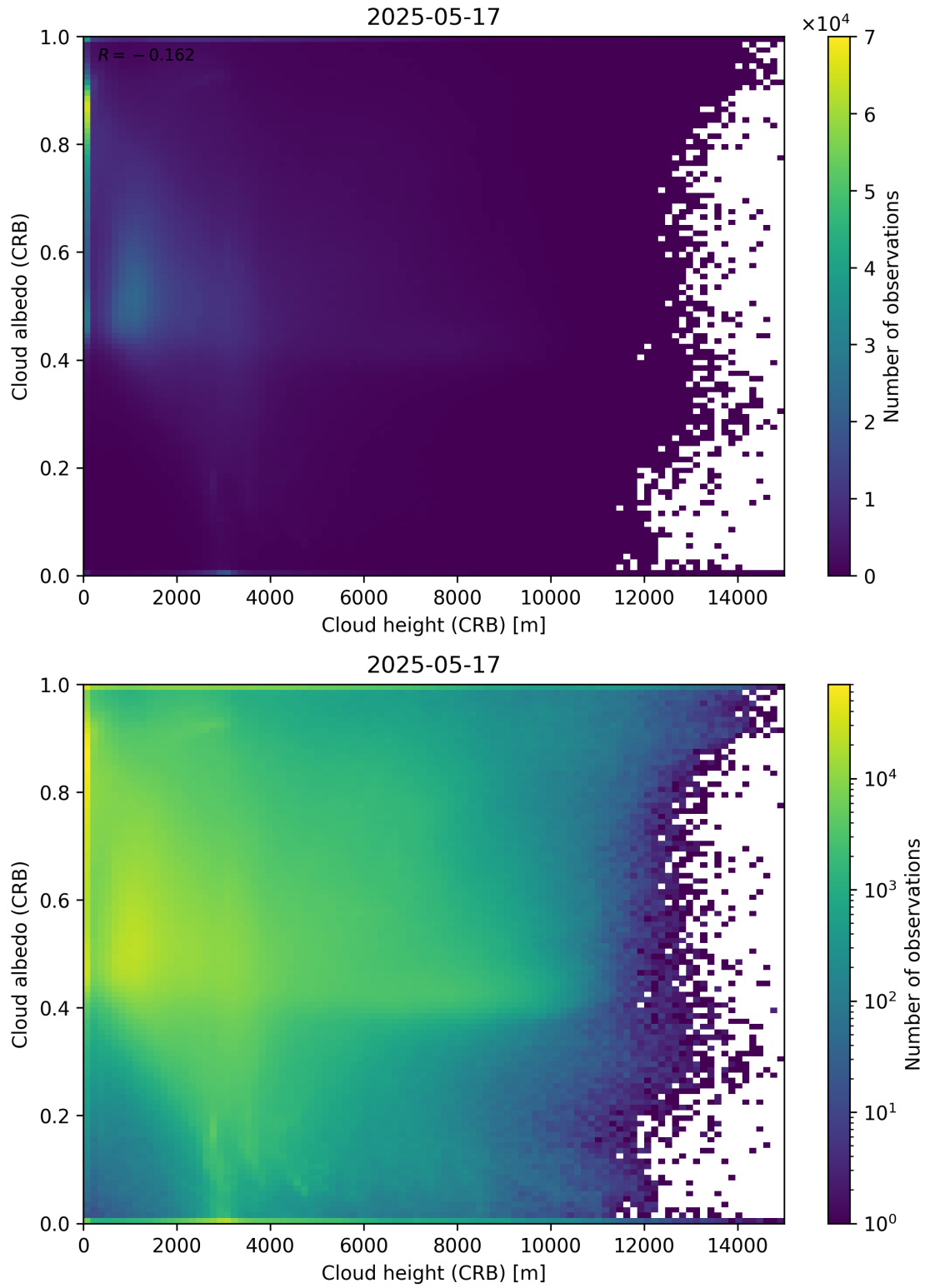
Figure 80: Scatter density plot of “Cloud height (CRB)” against “Cloud albedo (CRB)” for 2025-05-16 to 2025-05-18.
