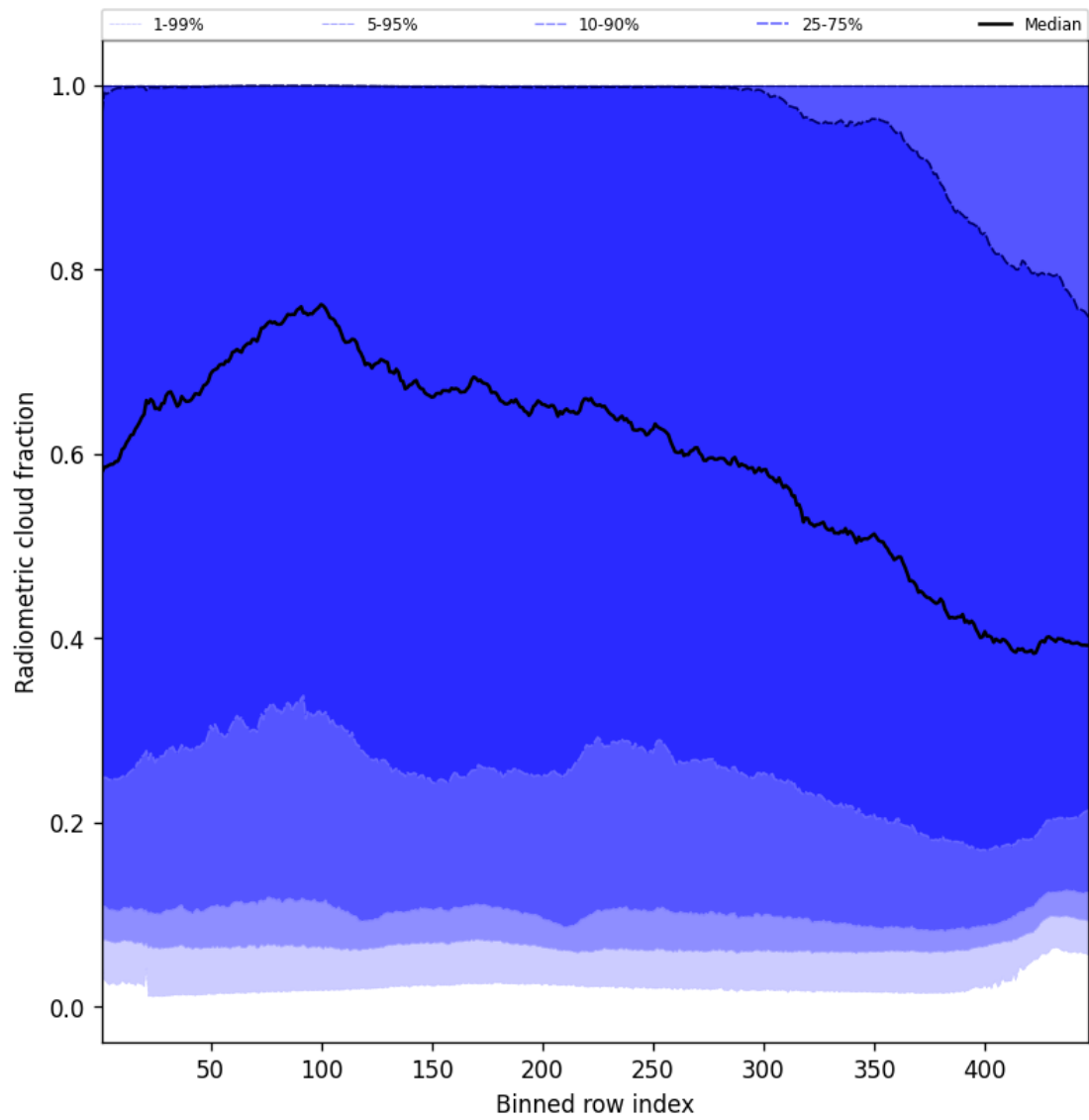
Figure 55: Along track statistics of “Radiometric cloud fraction” for 2025-05-16 to 2025-05-18
