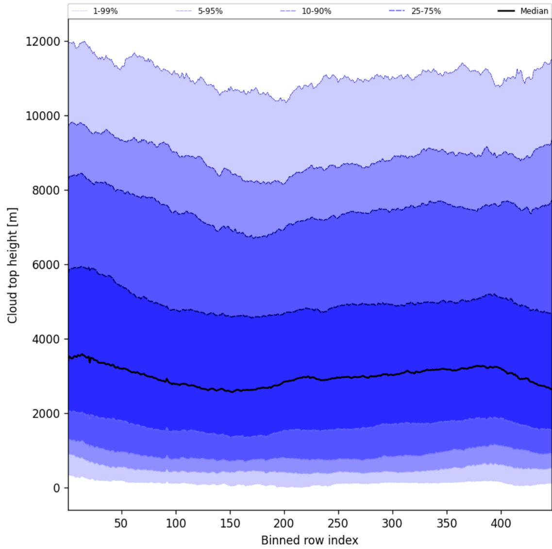
Figure 56: Along track statistics of “Cloud top height” for 2025-05-16 to 2025-05-18
