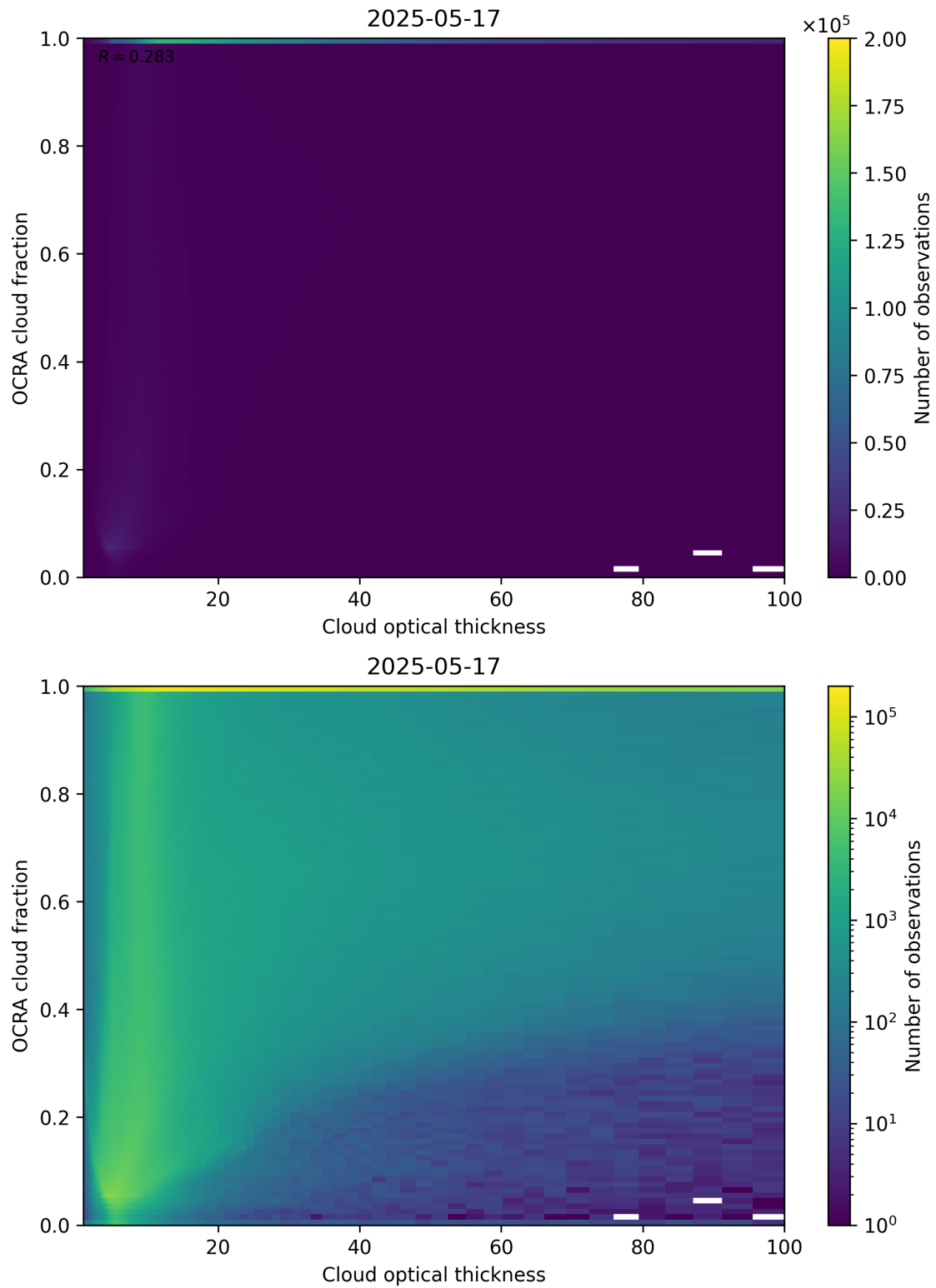
Figure 83: Scatter density plot of “Cloud optical thickness” against “OCRA cloud fraction” for 2025-05-16 to 2025-05-18.
