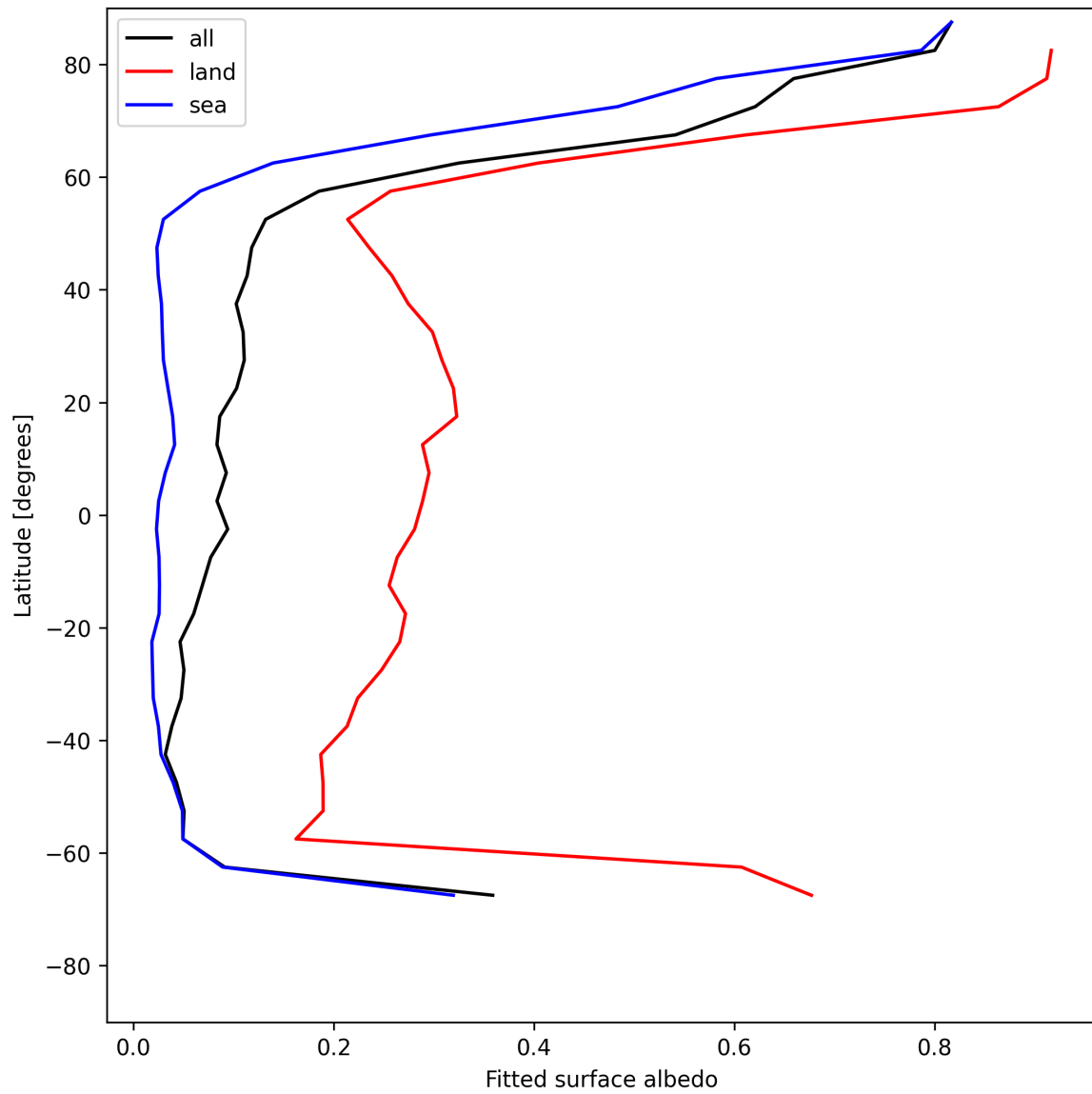
Figure 29: Zonal average of “Fitted surface albedo” for 2025-05-16 to 2025-05-18.
