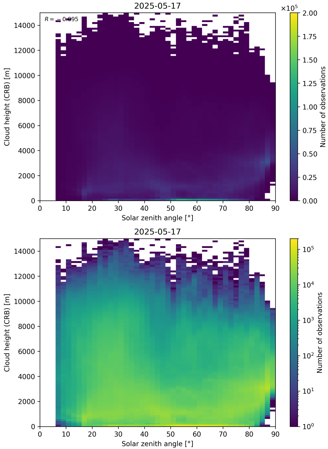
Figure 102: Scatter density plot of “Solar zenith angle” against “Cloud height (CRB)” for 2025-05-16 to 2025-05-18.
