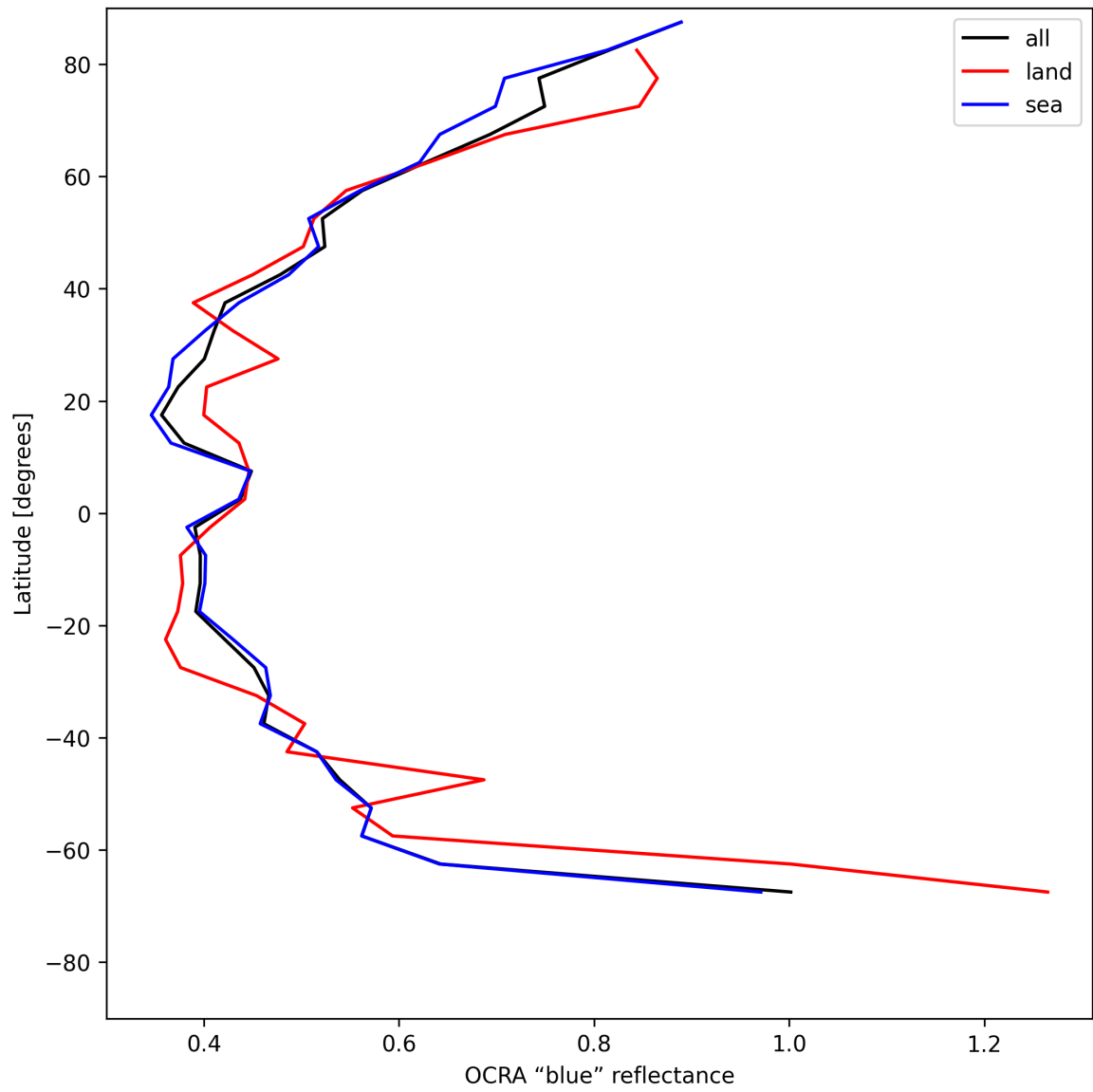
Figure 35: Zonal average of “OCRA “blue” reflectance” for 2025-05-16 to 2025-05-18.
