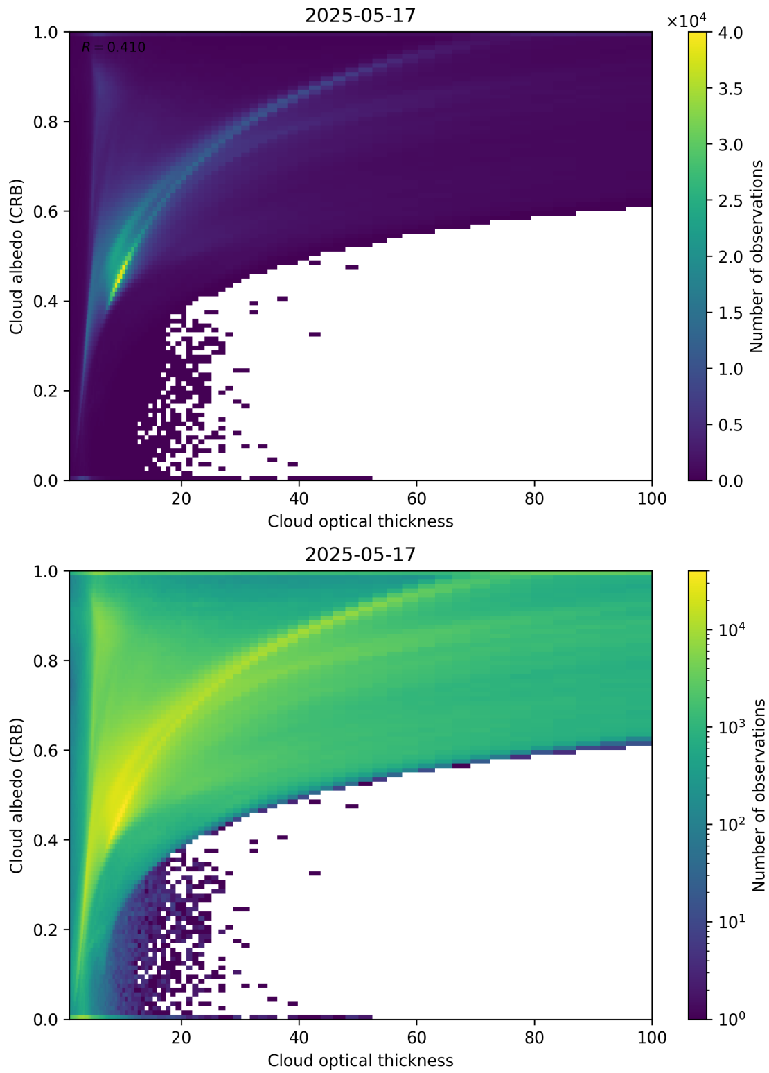
Figure 82: Scatter density plot of “Cloud optical thickness” against “Cloud albedo (CRB)” for 2025-05-16 to 2025-05-18.
