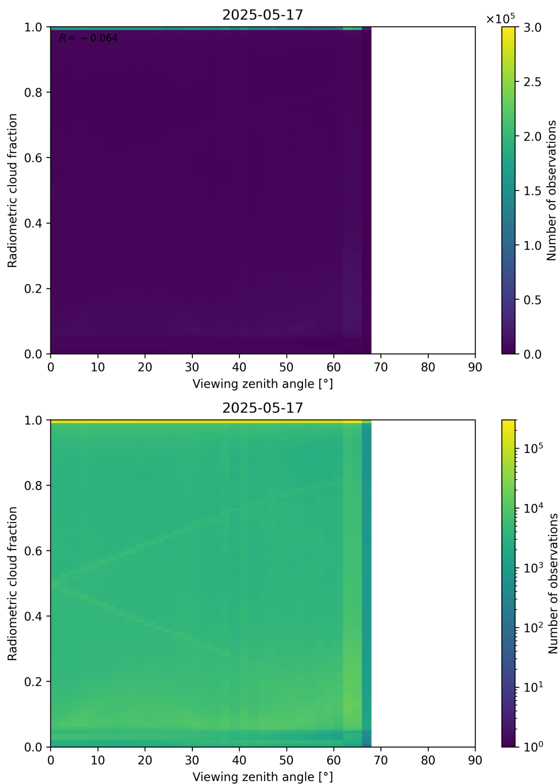
Figure 107: Scatter density plot of “Viewing zenith angle” against “Radiometric cloud fraction” for 2025-05-16 to 2025-05-18.
