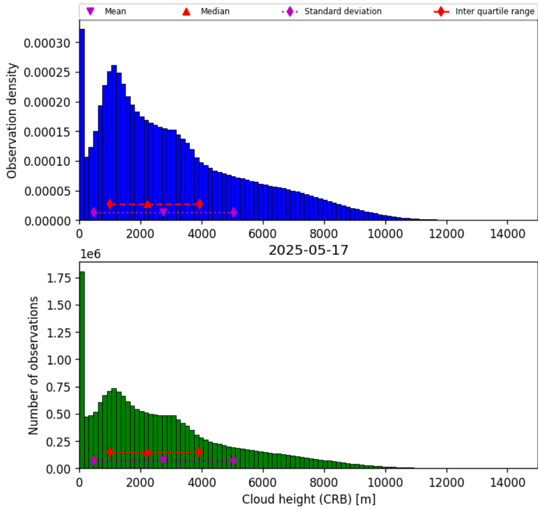
Figure 43: Histogram of “Cloud height (CRB)” for 2025-05-16 to 2025-05-18
