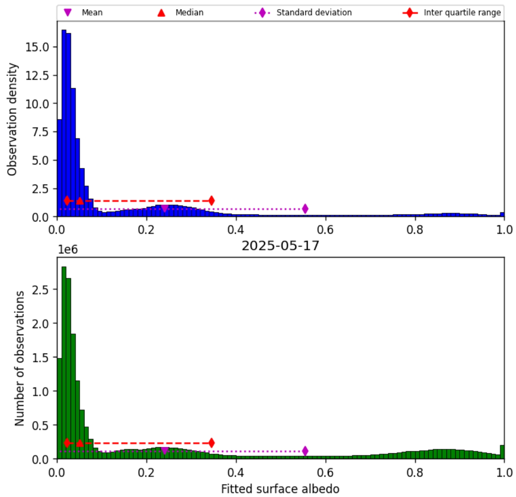
Figure 45: Histogram of “Fitted surface albedo” for 2025-05-16 to 2025-05-18
