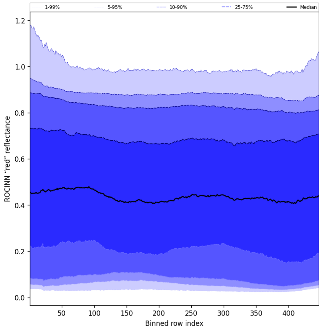
Figure 69: Along track statistics of “ROCINN “red” reflectance” for 2025-05-16 to 2025-05-18
