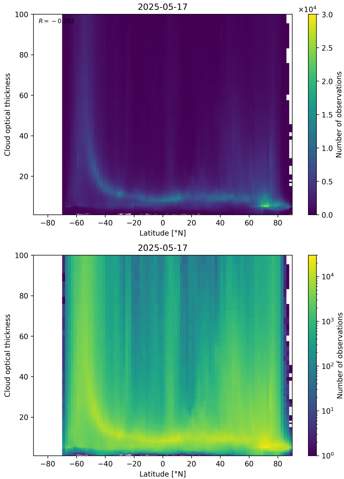
Figure 96: Scatter density plot of “Latitude” against “Cloud optical thickness” for 2025-05-16 to 2025-05-18.
