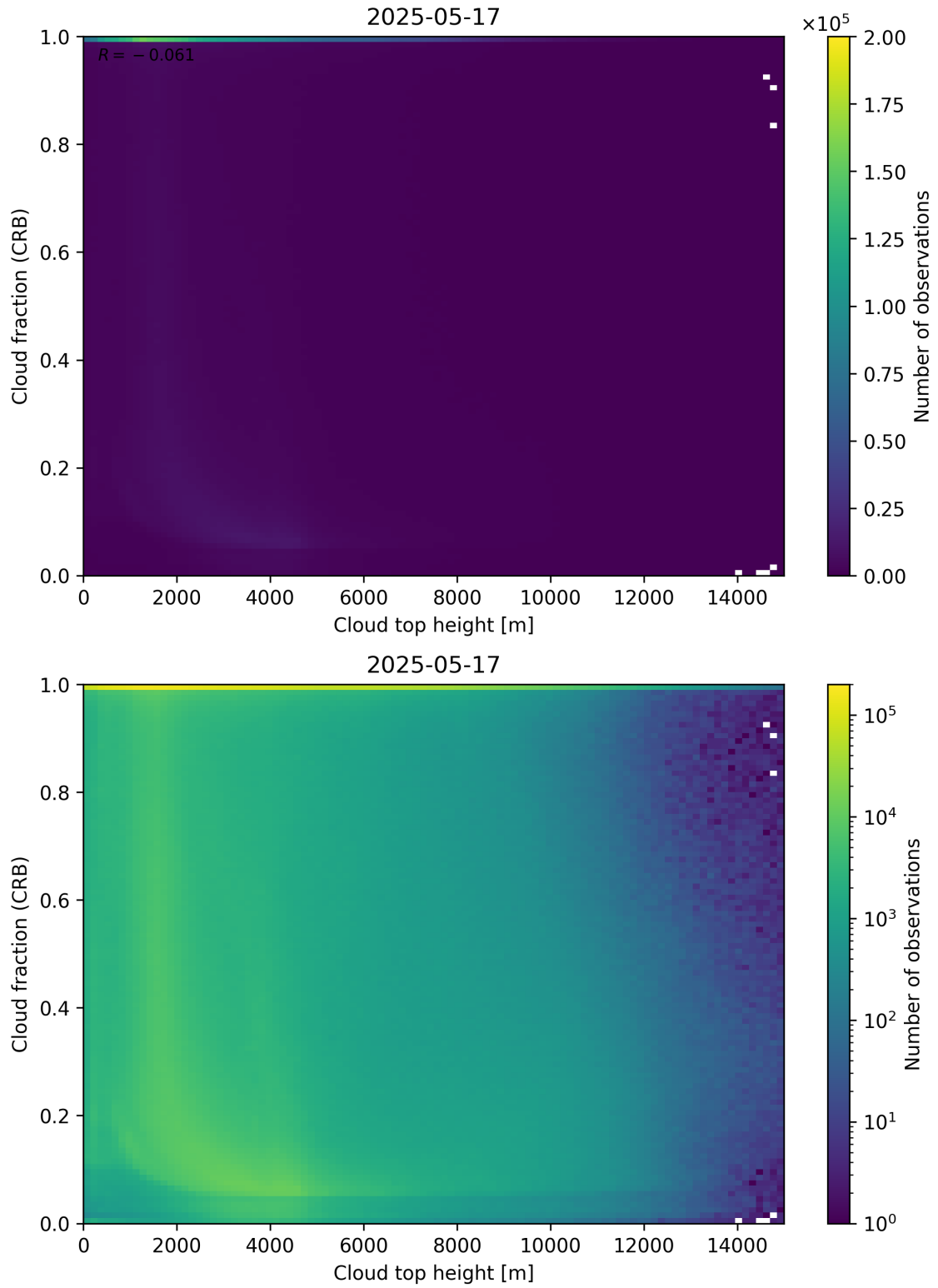
Figure 88: Scatter density plot of “Cloud top height” against “Cloud fraction (CRB)” for 2025-05-16 to 2025-05-18.
