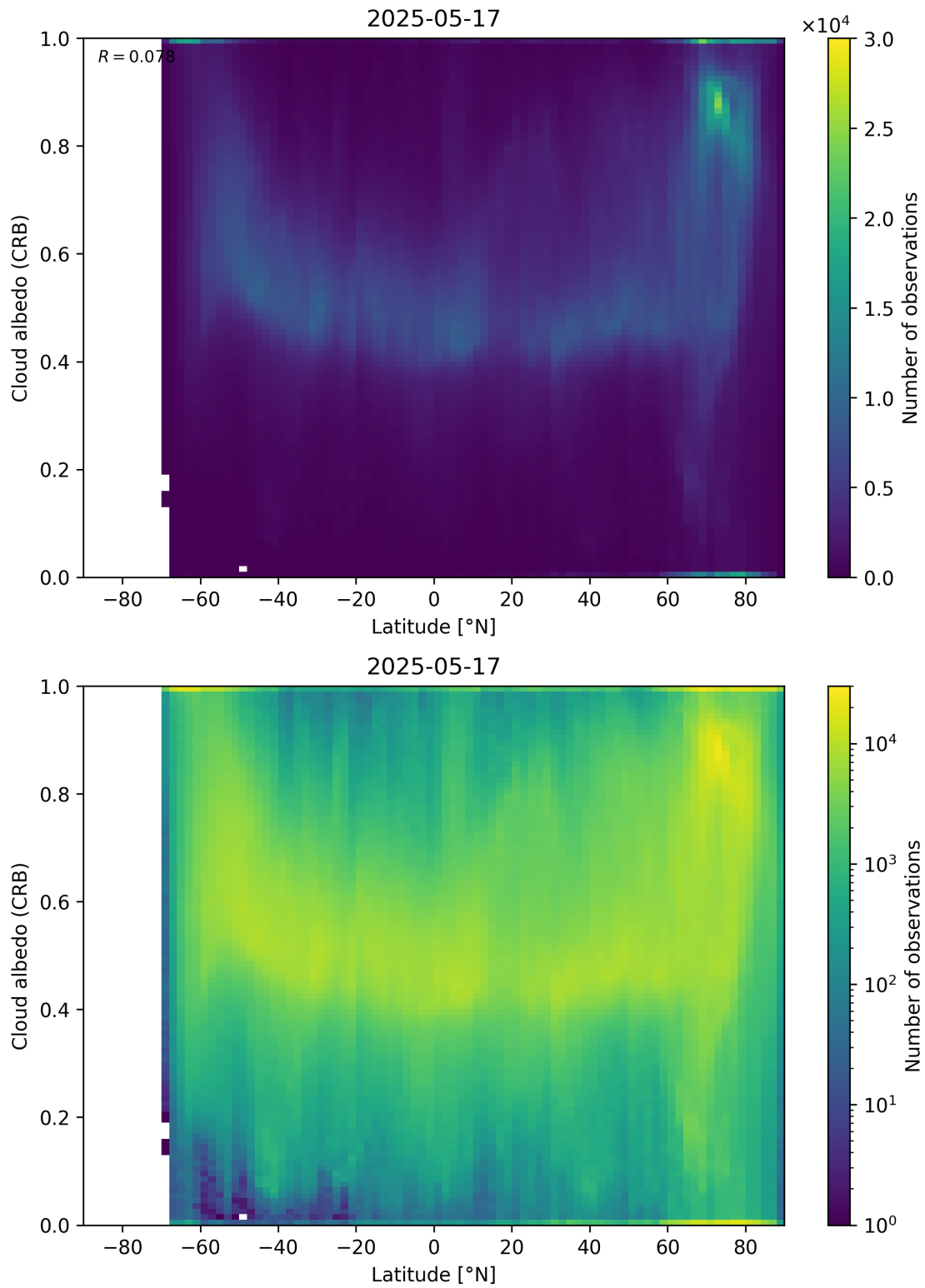
Figure 91: Scatter density plot of “Latitude” against “Cloud albedo (CRB)” for 2025-05-16 to 2025-05-18.
