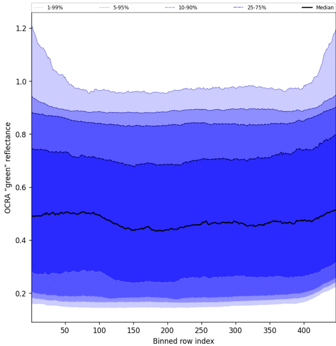
Figure 68: Along track statistics of "OCRA "green" reflectance" for 2025-05-16 to 2025-05-18
