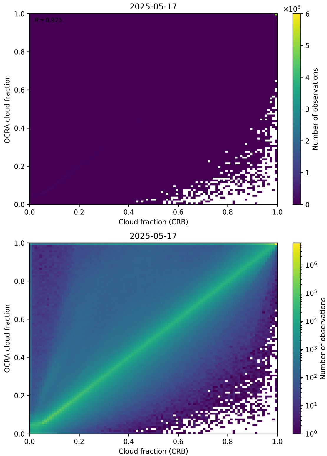
Figure 78: Scatter density plot of “Cloud fraction (CRB)” against “OCRA cloud fraction” for 2025-05-16 to 2025-05-18.
