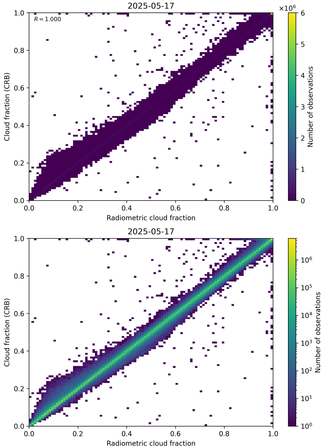
Figure 73: Scatter density plot of “Radiometric cloud fraction” against “Cloud fraction (CRB)” for 2025-05-16 to 2025-05-18.
