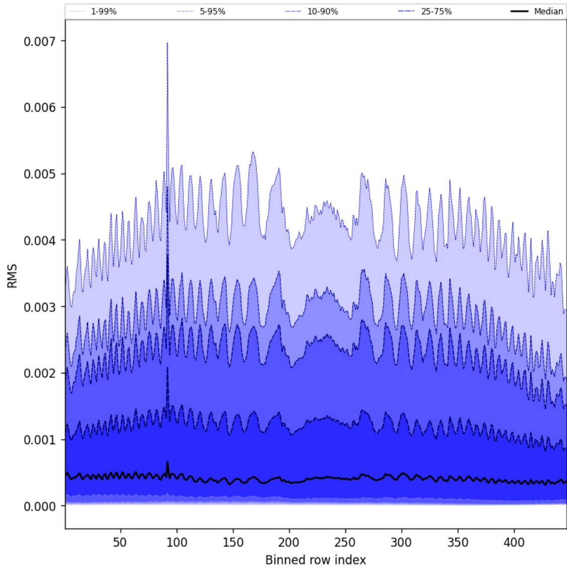
Figure 63: Along track statistics of “RMS” for 2025-05-16 to 2025-05-18
