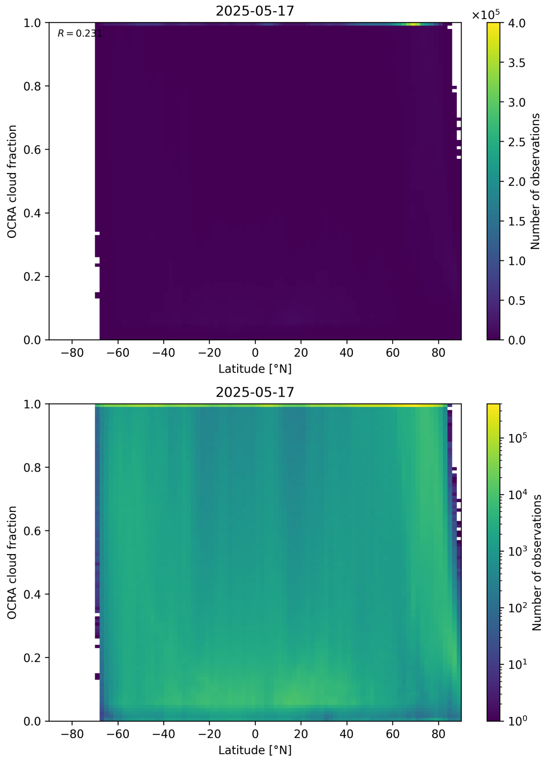
Figure 93: Scatter density plot of “Latitude” against “OCRA cloud fraction” for 2025-05-16 to 2025-05-18.
