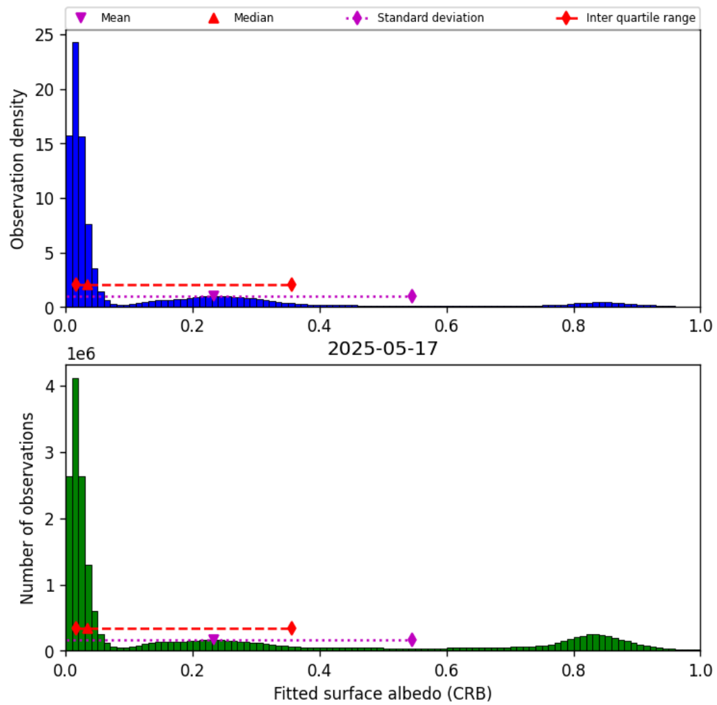
Figure 46: Histogram of “Fitted surface albedo (CRB)” for 2025-05-16 to 2025-05-18
