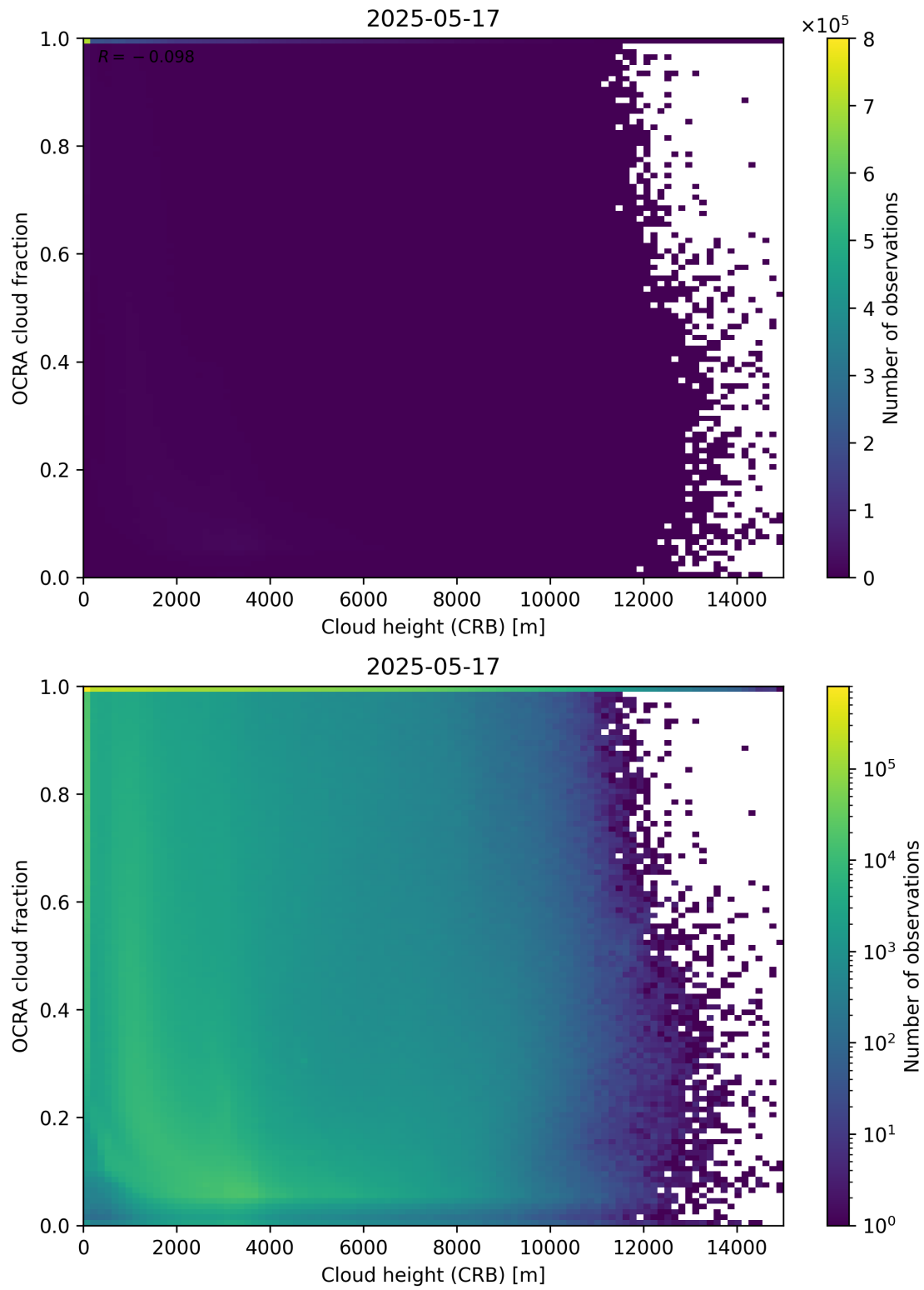
Figure 81: Scatter density plot of “Cloud height (CRB)” against “OCRA cloud fraction” for 2025-05-16 to 2025-05-18.
