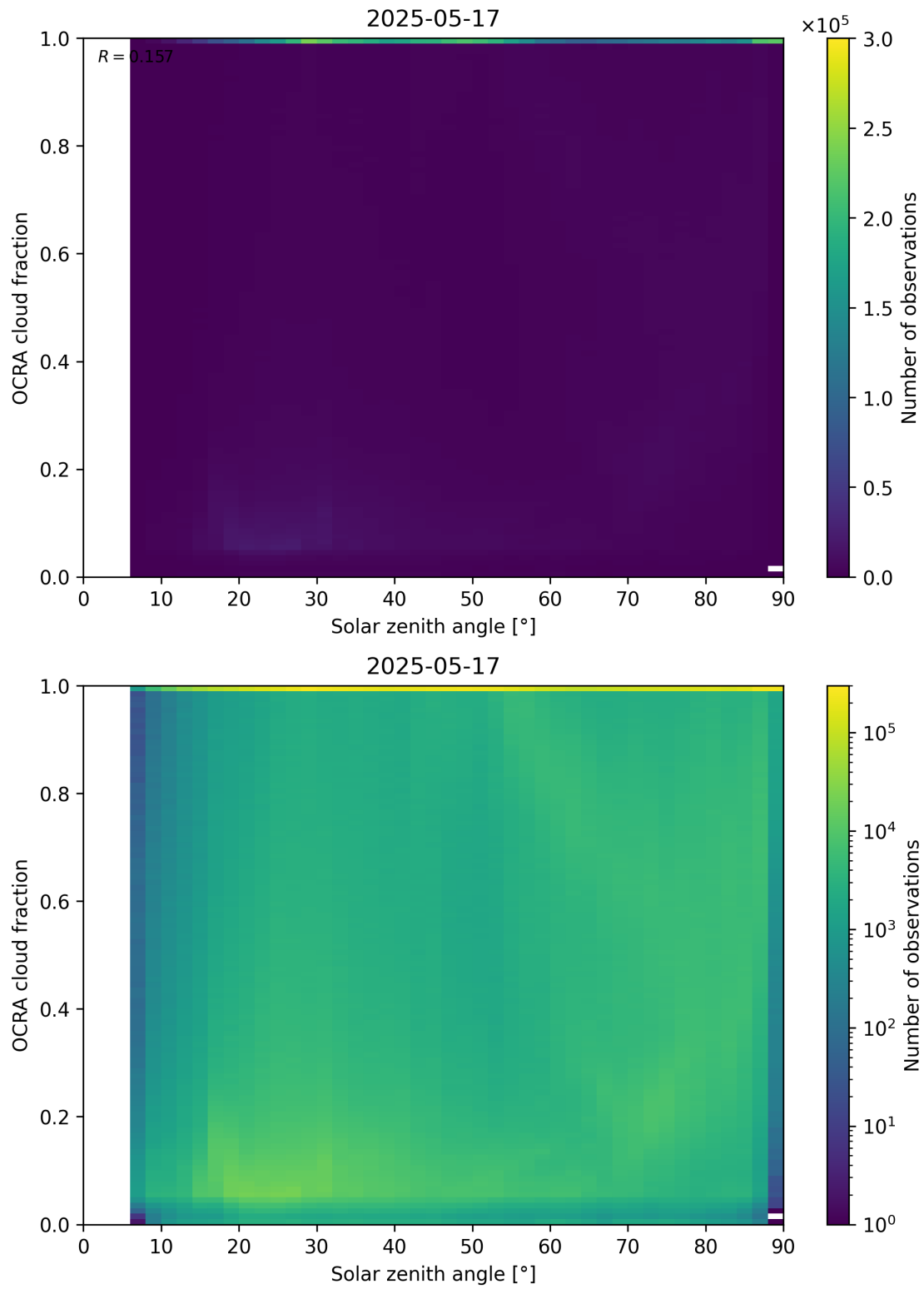
Figure 100: Scatter density plot of “Solar zenith angle” against “OCRA cloud fraction” for 2025-05-16 to 2025-05-18.
