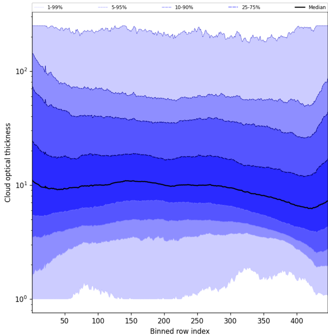
Figure 57: Along track statistics of “Cloud optical thickness” for 2025-05-16 to 2025-05-18
