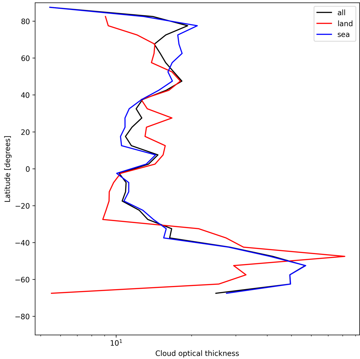
Figure 25: Zonal average of “Cloud optical thickness” for 2025-05-16 to 2025-05-18.
