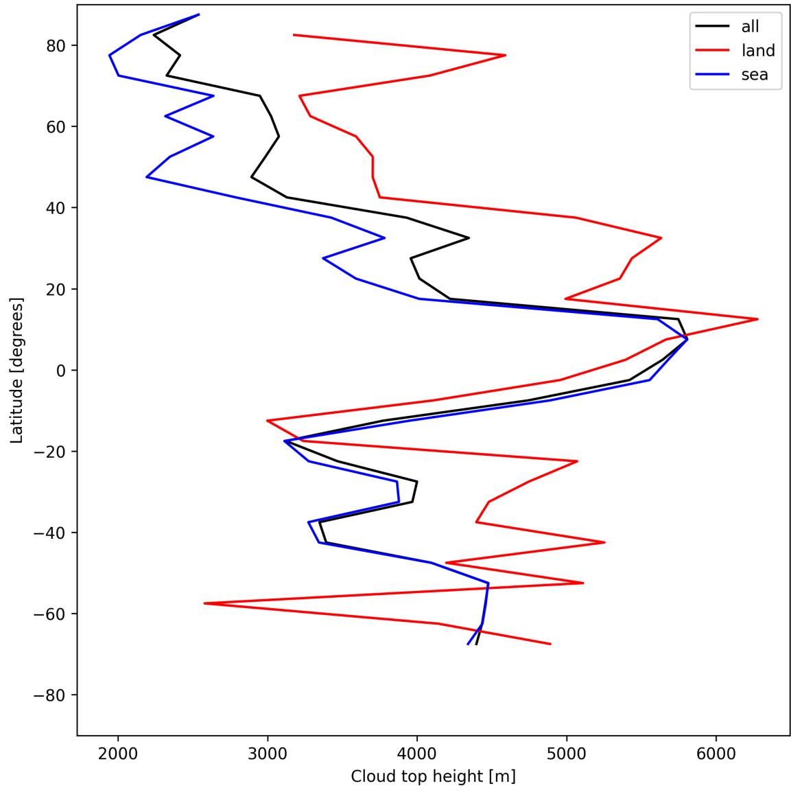
Figure 24: Zonal average of “Cloud top height” for 2025-05-16 to 2025-05-18.
