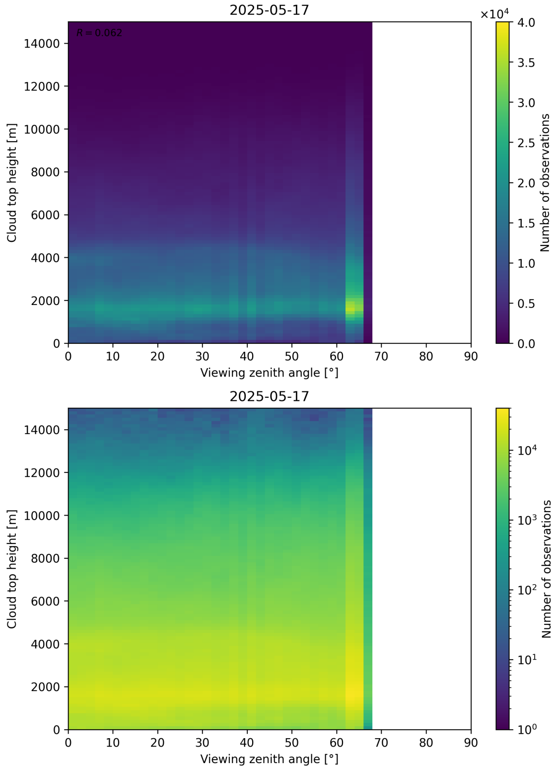
Figure 112: Scatter density plot of “Viewing zenith angle” against “Cloud top height” for 2025-05-16 to 2025-05-18.
