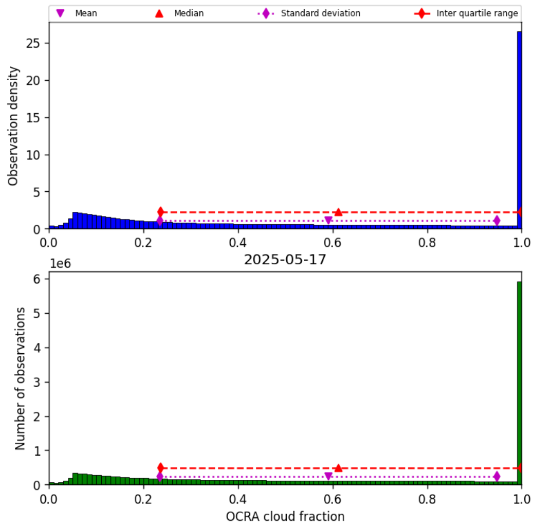
Figure 50: Histogram of “OCRA cloud fraction” for 2025-05-16 to 2025-05-18
