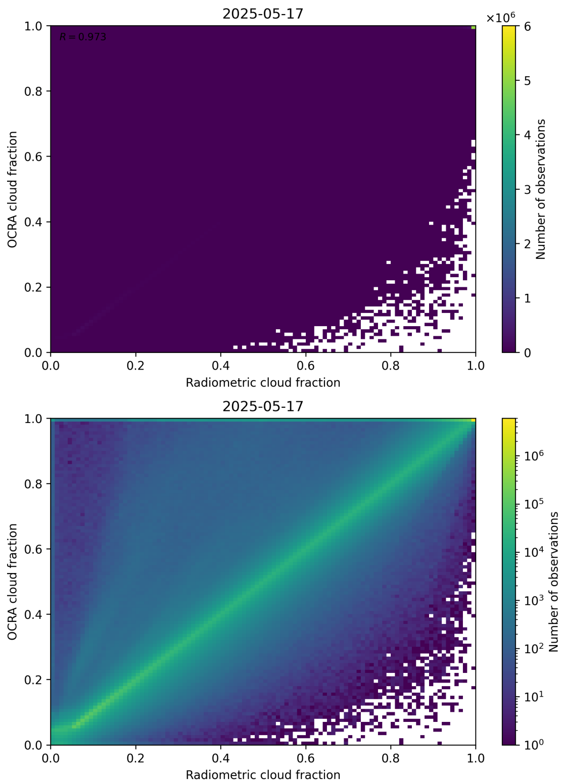
Figure 72: Scatter density plot of “Radiometric cloud fraction” against “OCRA cloud fraction” for 2025-05-16 to 2025-05-18.
