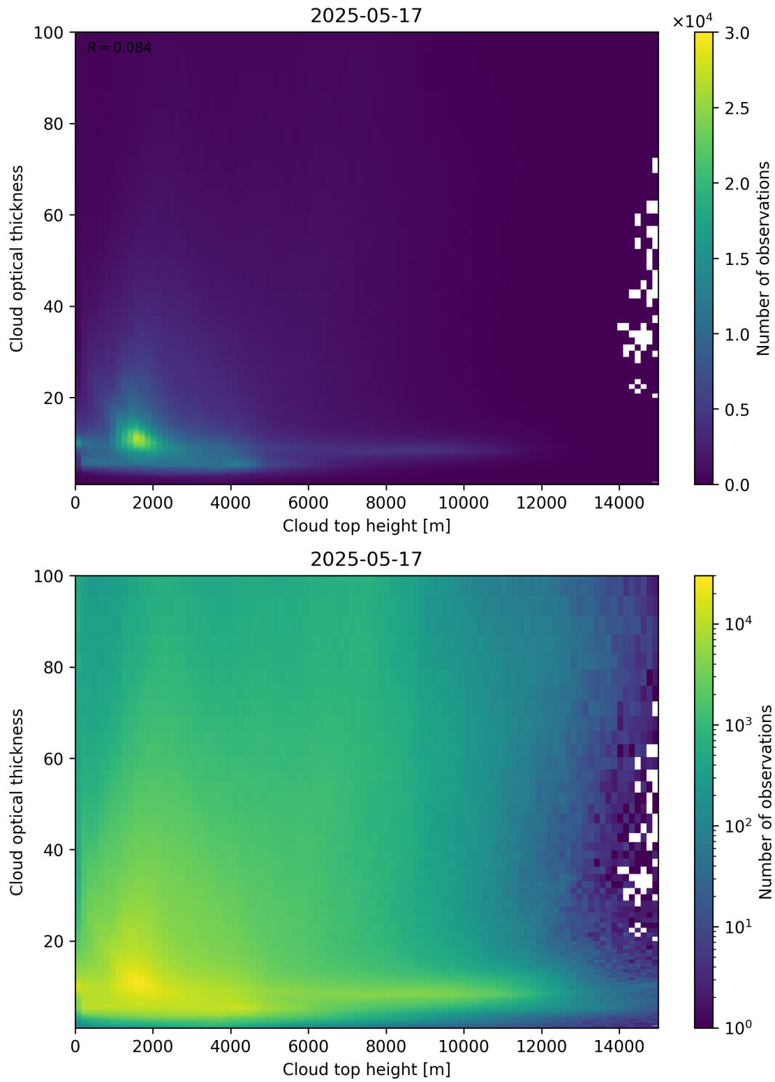
Figure 90: Scatter density plot of “Cloud top height” against “Cloud optical thickness” for 2025-05-16 to 2025-05-18.
