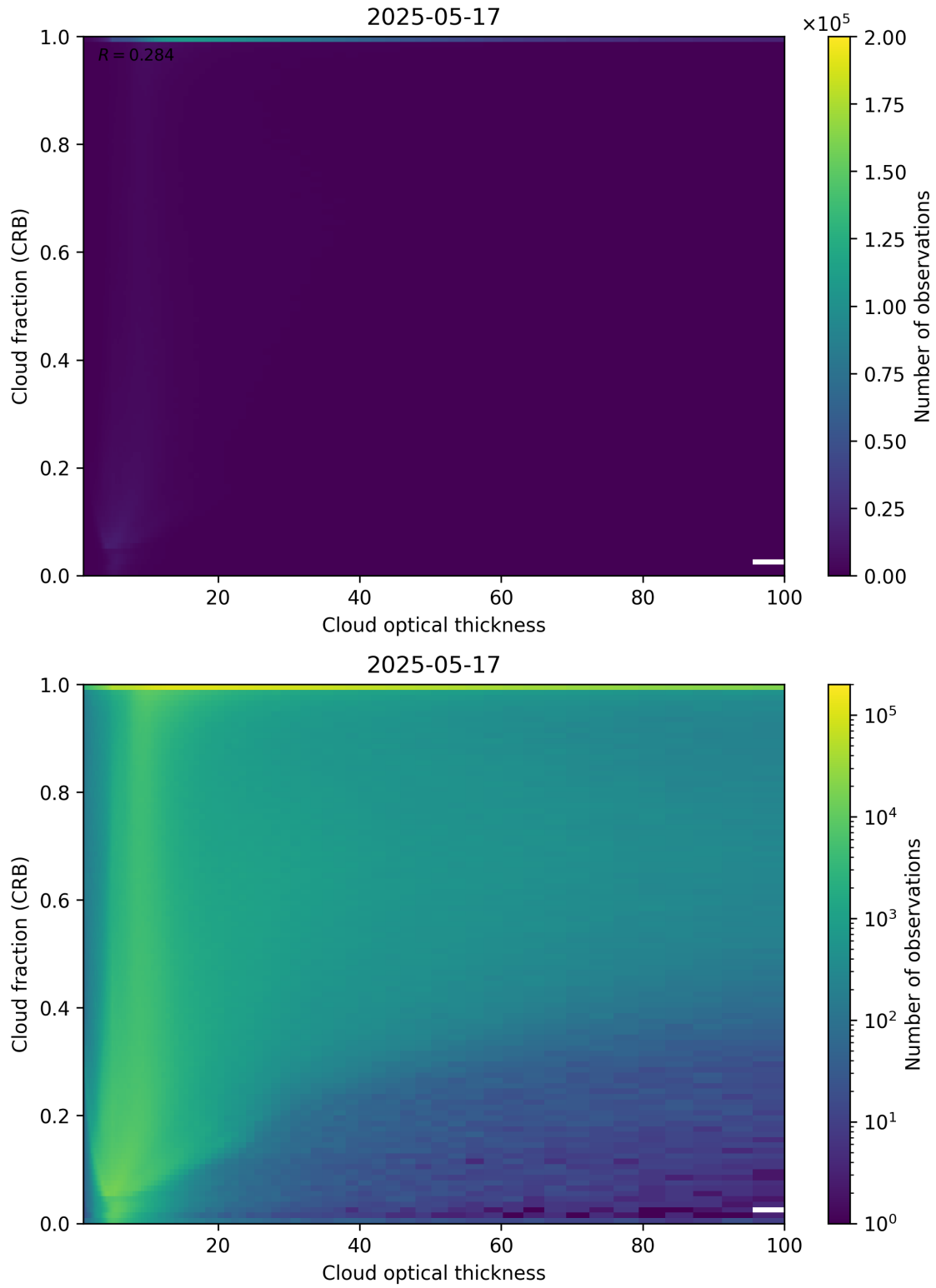
Figure 84: Scatter density plot of “Cloud optical thickness” against “Cloud fraction (CRB)” for 2025-05-16 to 2025-05-18.
