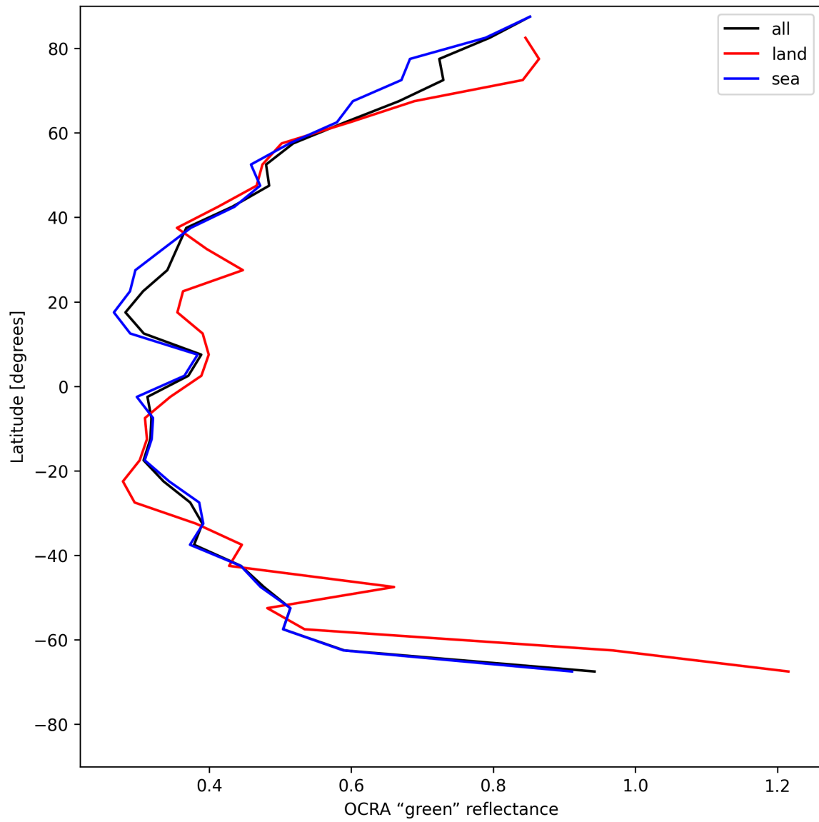
Figure 36: Zonal average of “OCRA “green” reflectance” for 2025-05-16 to 2025-05-18.
