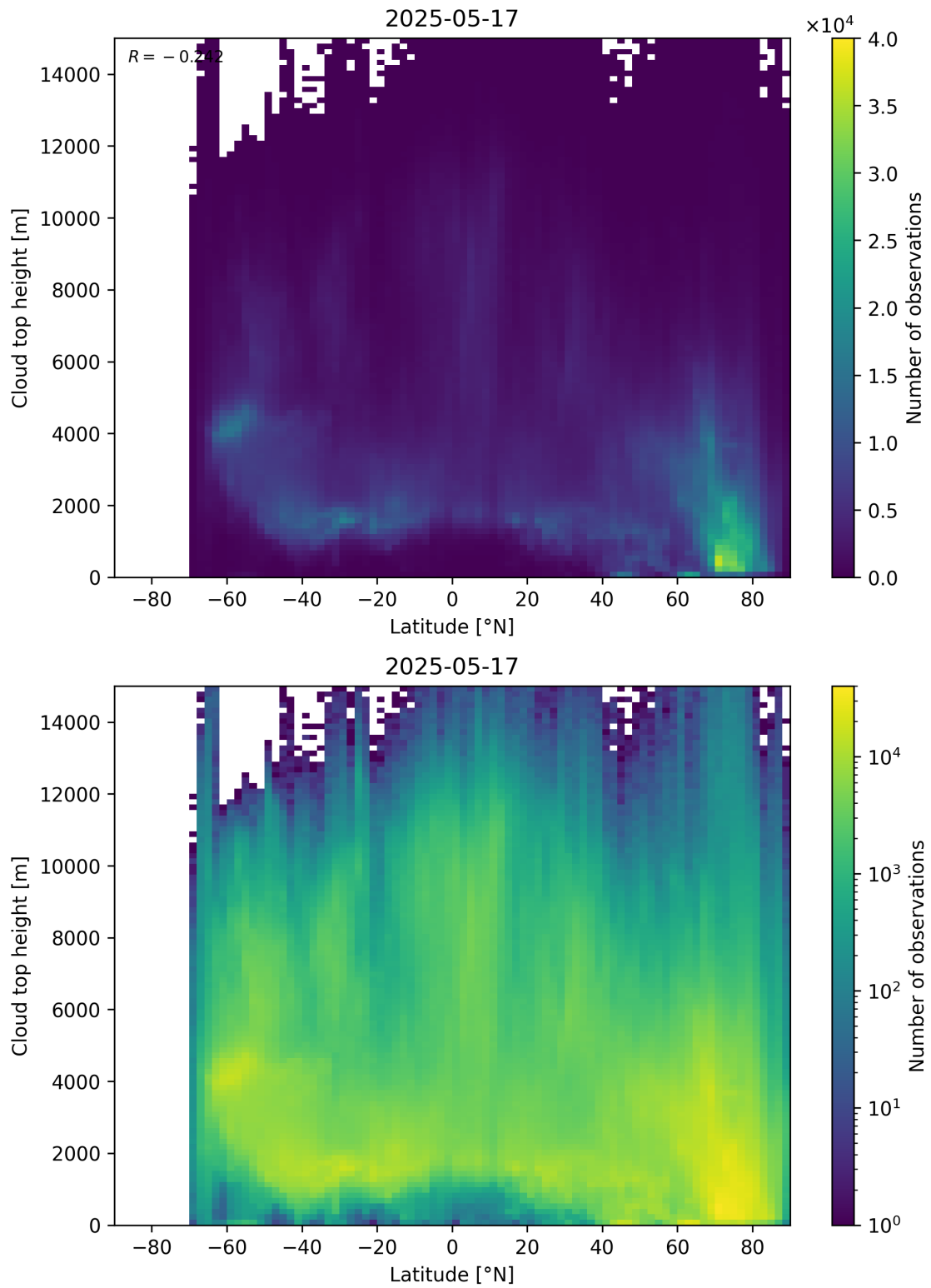
Figure 97: Scatter density plot of “Latitude” against “Cloud top height” for 2025-05-16 to 2025-05-18.
