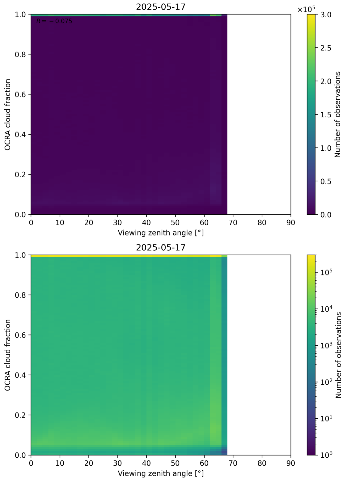
Figure 108: Scatter density plot of “Viewing zenith angle” against “OCRA cloud fraction” for 2025-05-16 to 2025-05-18.
