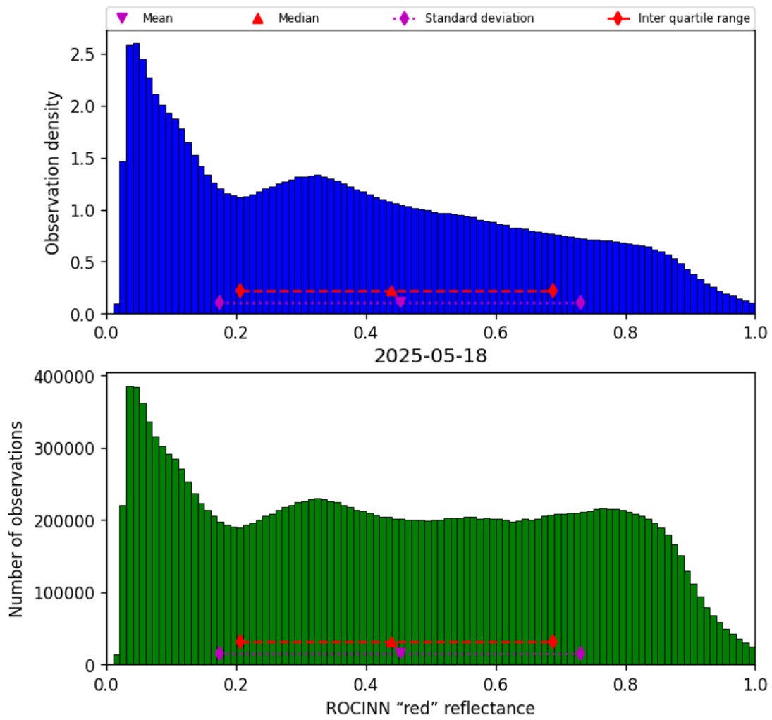
Figure 53: Histogram of “ROCINN “red” reflectance” for 2025-05-17 to 2025-05-19
