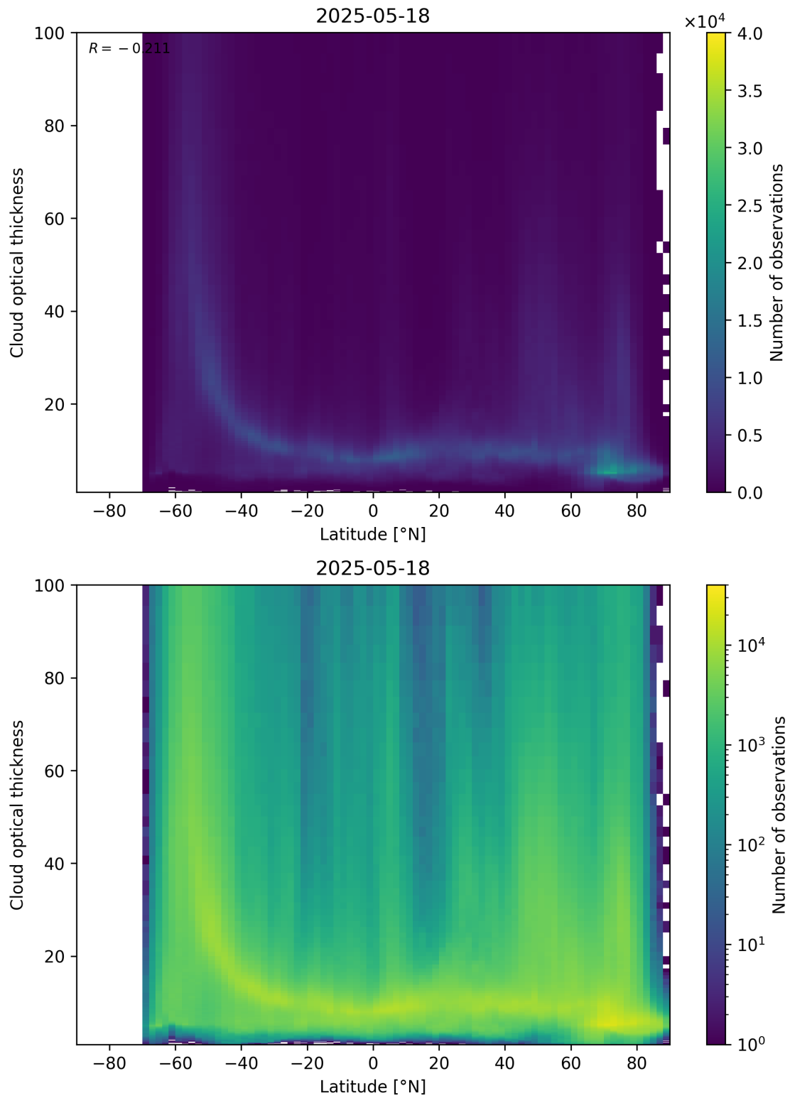
Figure 96: Scatter density plot of “Latitude” against “Cloud optical thickness” for 2025-05-17 to 2025-05-19.
