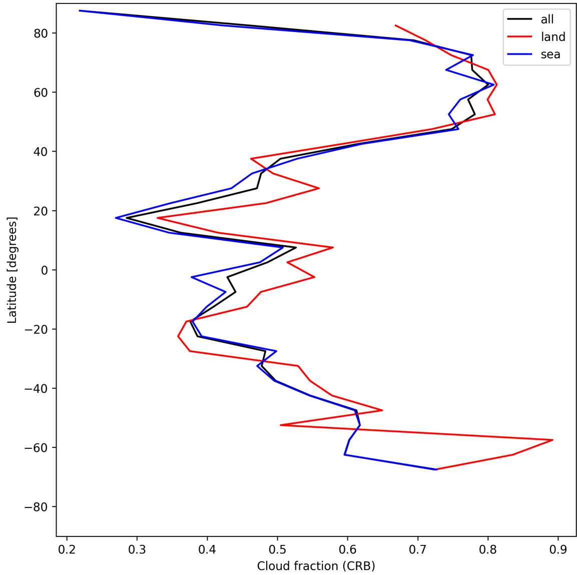
Figure 26: Zonal average of “Cloud fraction (CRB)” for 2025-05-17 to 2025-05-19.
