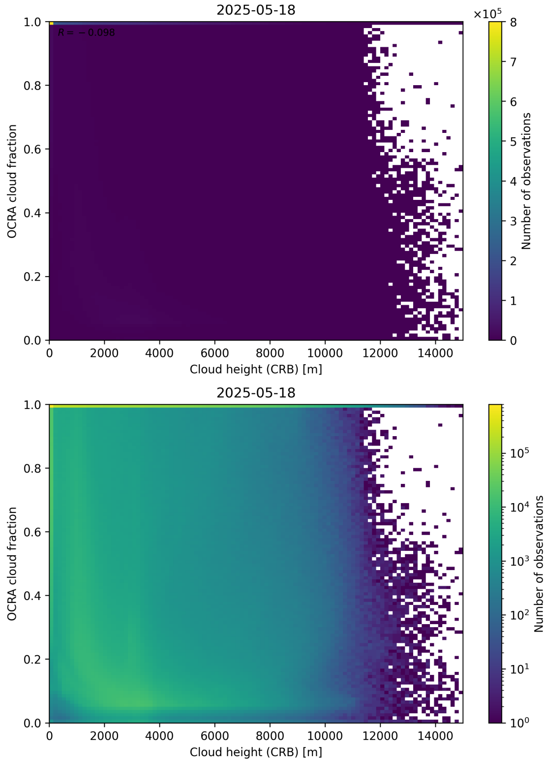
Figure 81: Scatter density plot of “Cloud height (CRB)” against “OCRA cloud fraction” for 2025-05-17 to 2025-05-19.
