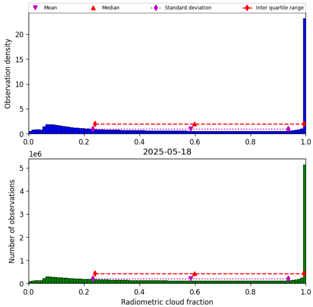
Figure 39: Histogram of “Radiometric cloud fraction” for 2025-05-17 to 2025-05-19
