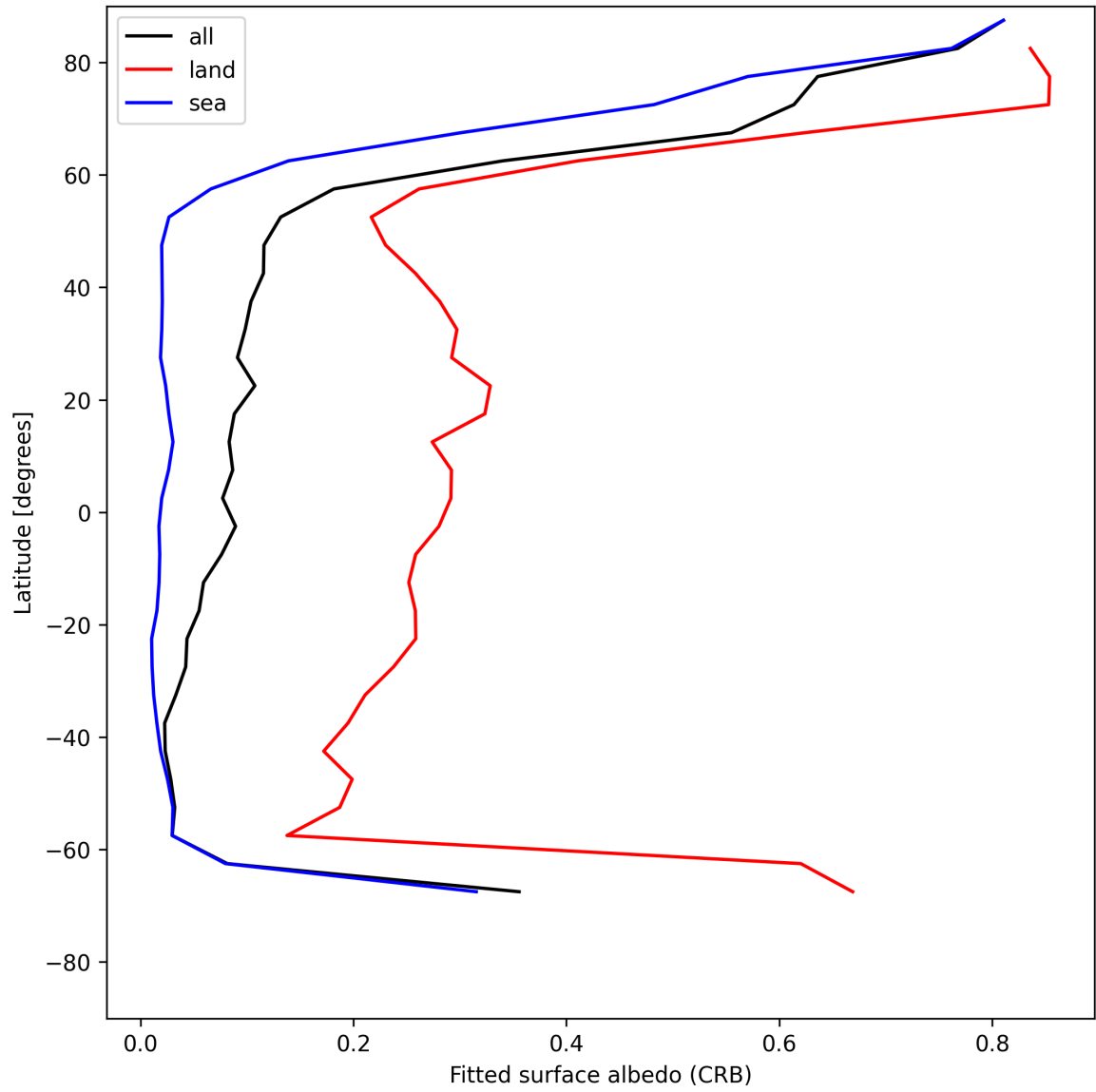
Figure 30: Zonal average of “Fitted surface albedo (CRB)” for 2025-05-17 to 2025-05-19.
