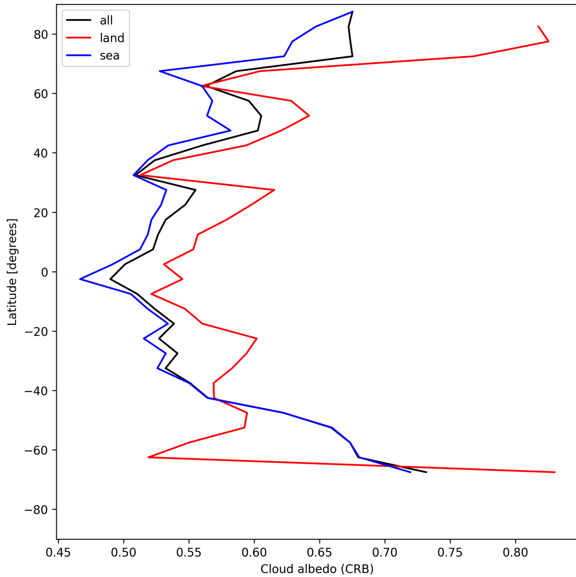
Figure 28: Zonal average of “Cloud albedo (CRB)” for 2025-05-17 to 2025-05-19.
