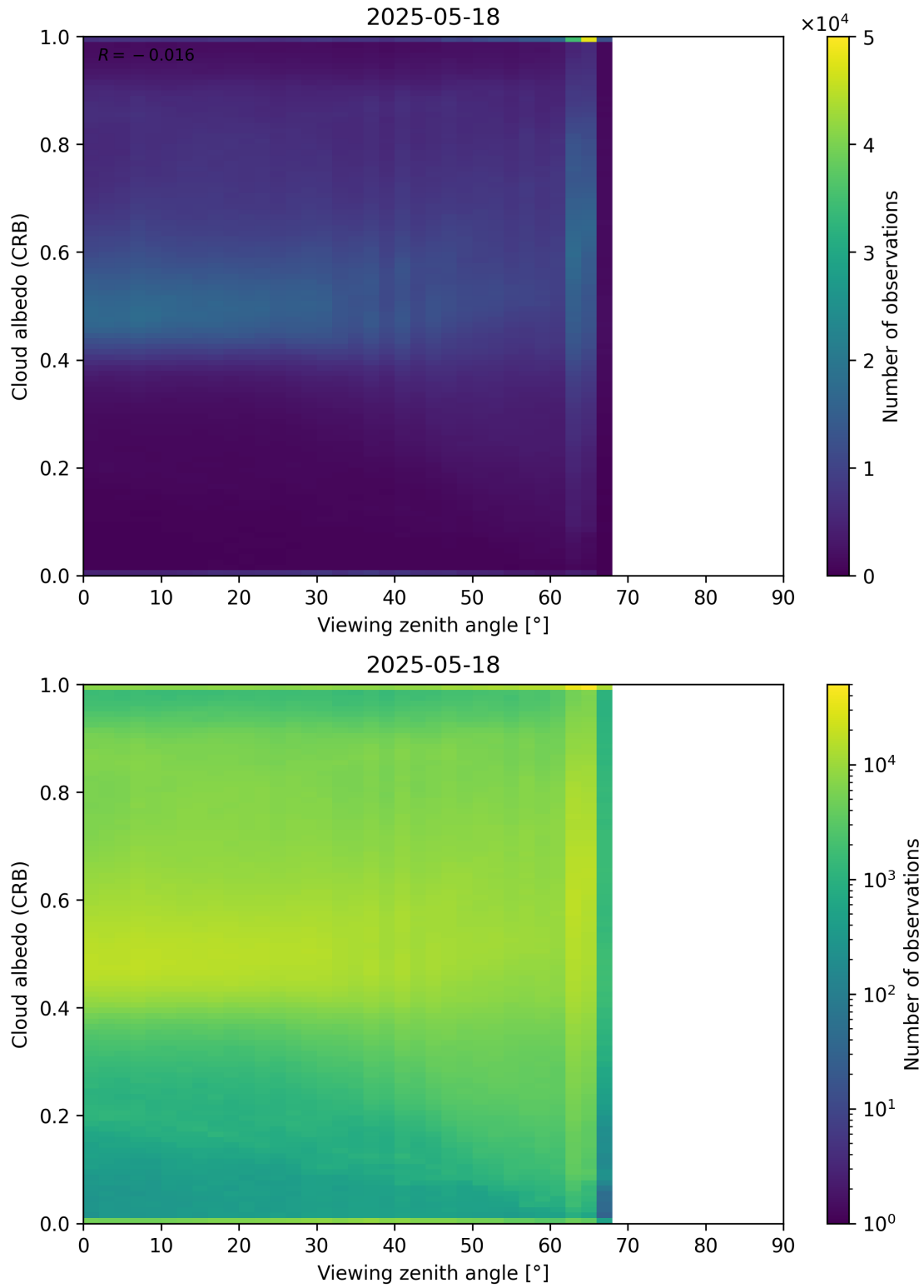
Figure 106: Scatter density plot of “Viewing zenith angle” against “Cloud albedo (CRB)” for 2025-05-17 to 2025-05-19.
