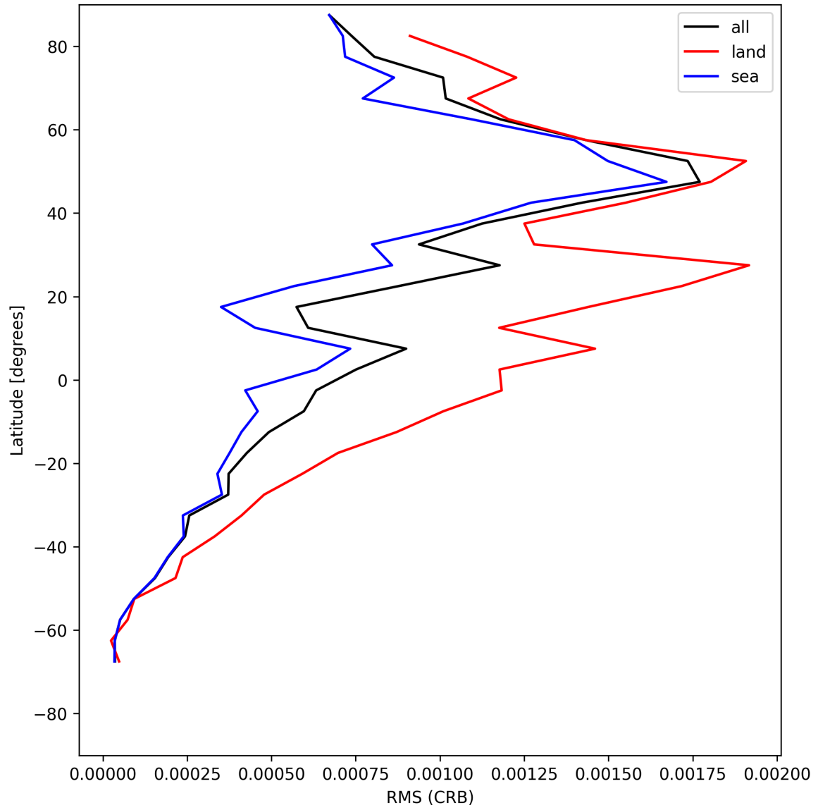
Figure 32: Zonal average of “RMS (CRB)” for 2025-05-17 to 2025-05-19.
