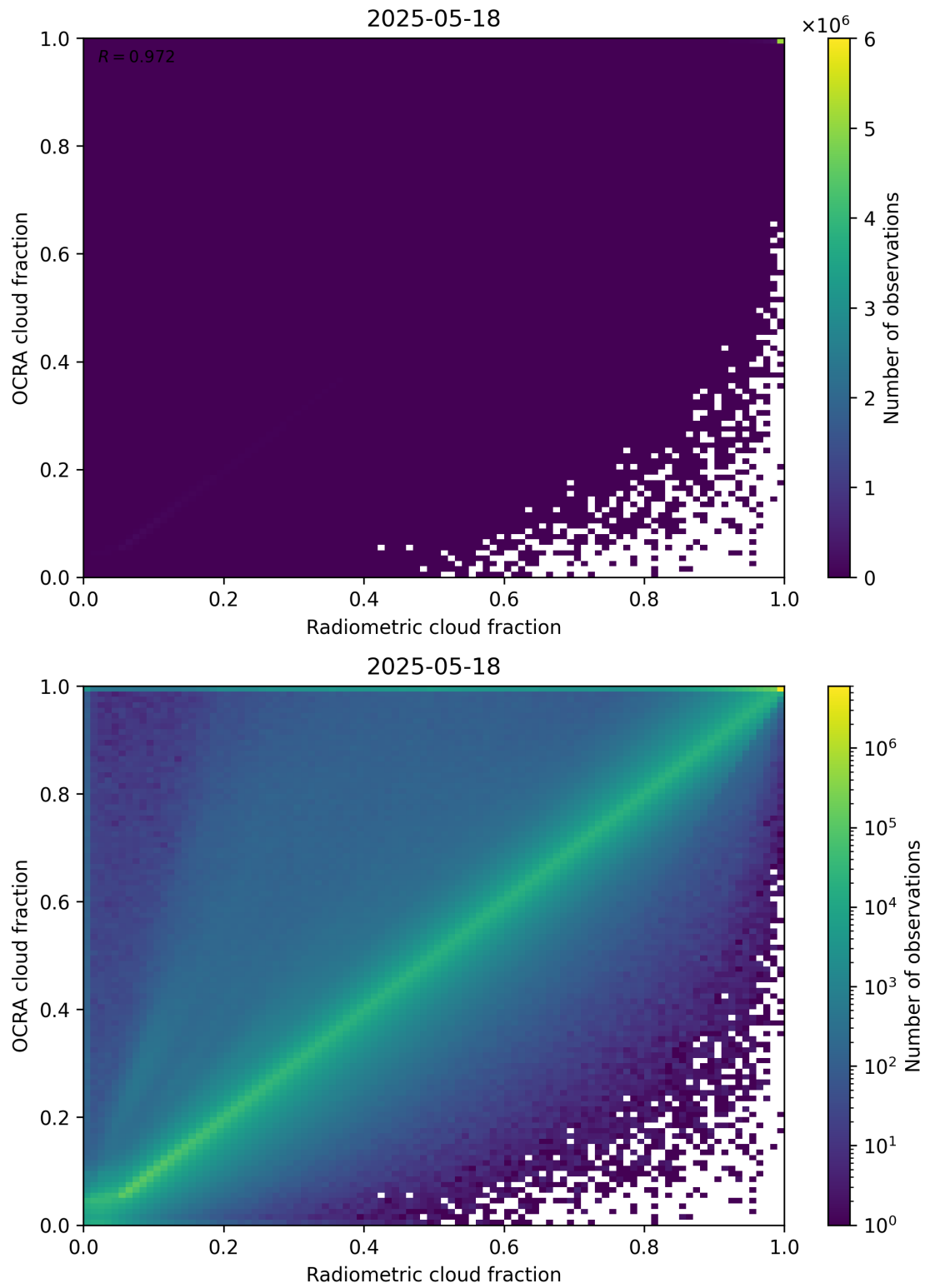
Figure 72: Scatter density plot of “Radiometric cloud fraction” against “OCRA cloud fraction” for 2025-05-17 to 2025-05-19.
