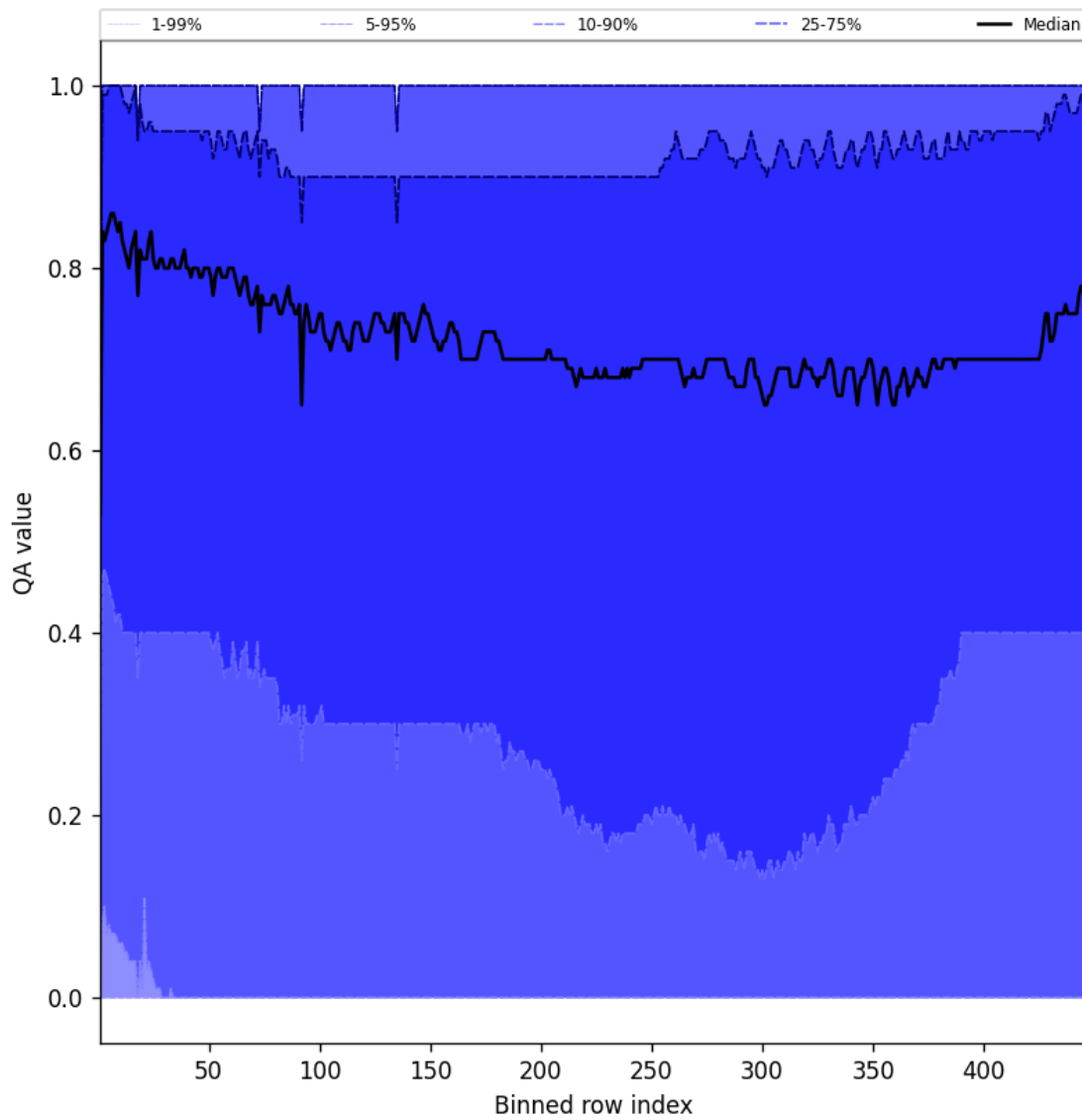
Figure 54: Along track statistics of “QA value” for 2025-05-17 to 2025-05-19
