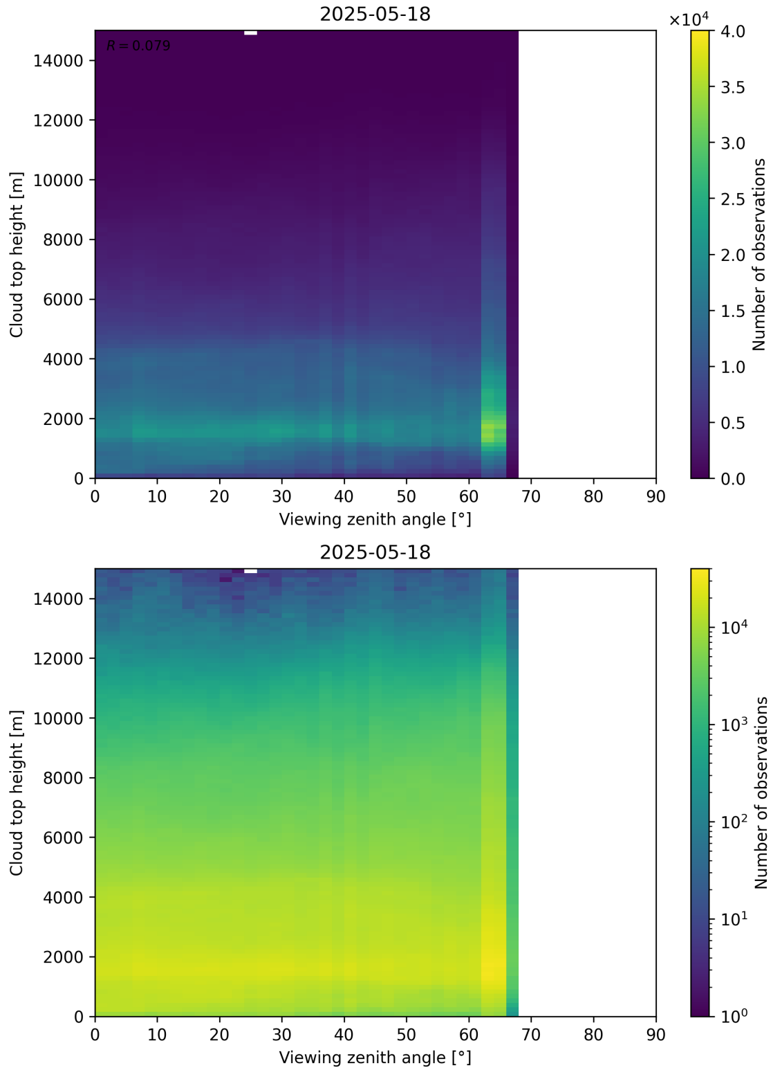
Figure 112: Scatter density plot of “Viewing zenith angle” against “Cloud top height” for 2025-05-17 to 2025-05-19.
