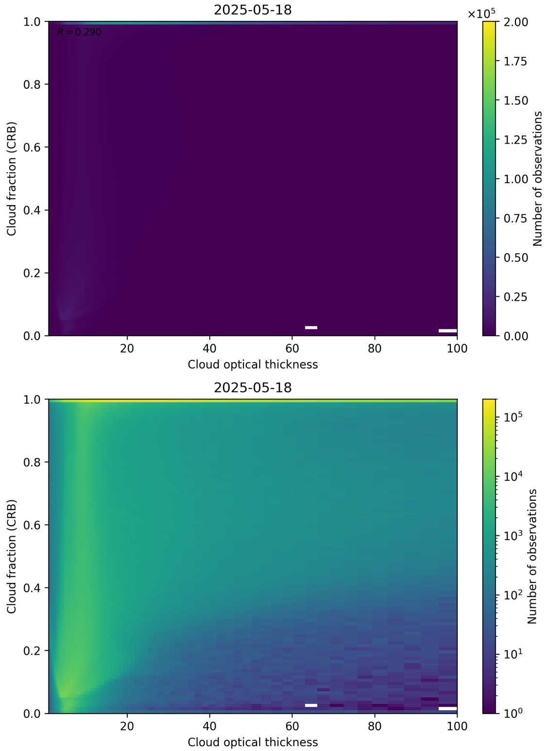
Figure 84: Scatter density plot of “Cloud optical thickness” against “Cloud fraction (CRB)” for 2025-05-17 to 2025-05-19.
