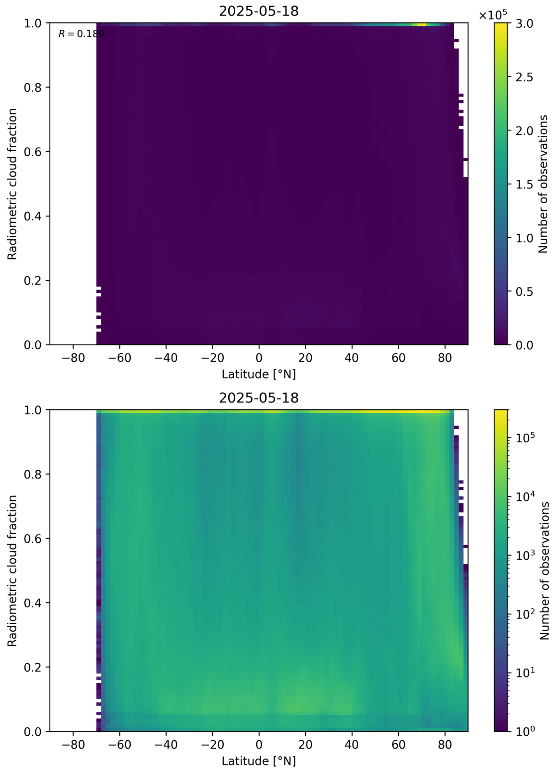
Figure 92: Scatter density plot of “Latitude” against “Radiometric cloud fraction” for 2025-05-17 to 2025-05-19.
