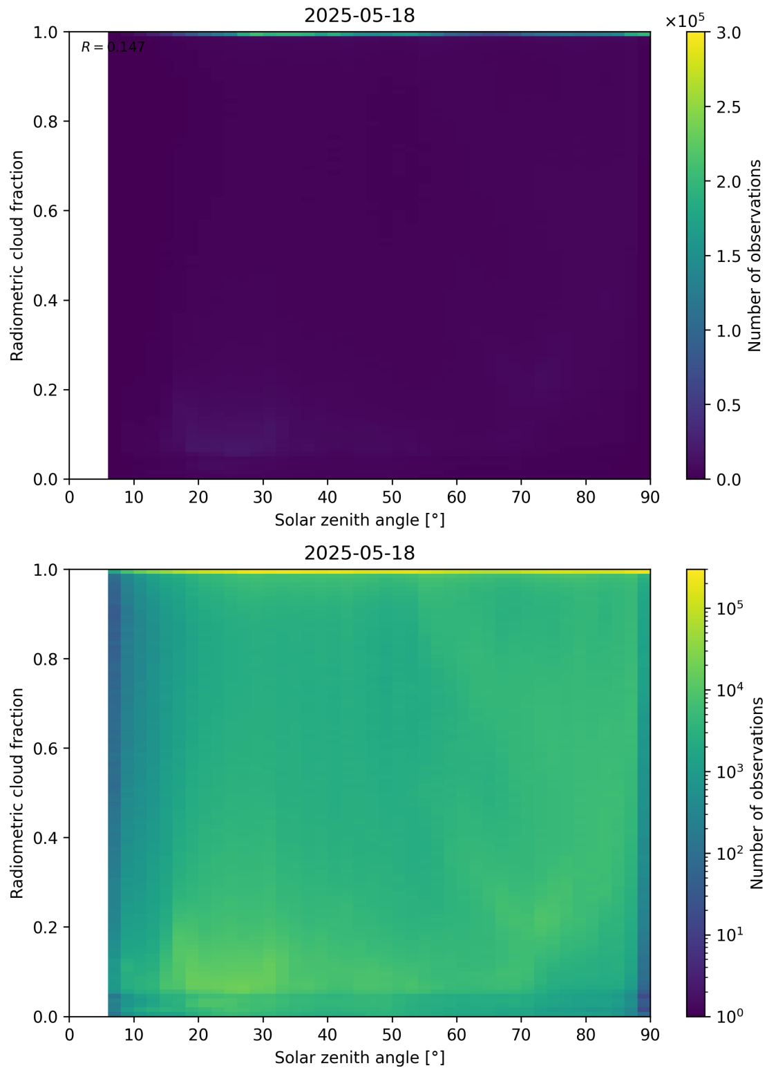
Figure 99: Scatter density plot of “Solar zenith angle” against “Radiometric cloud fraction” for 2025-05-17 to 2025-05-19.
