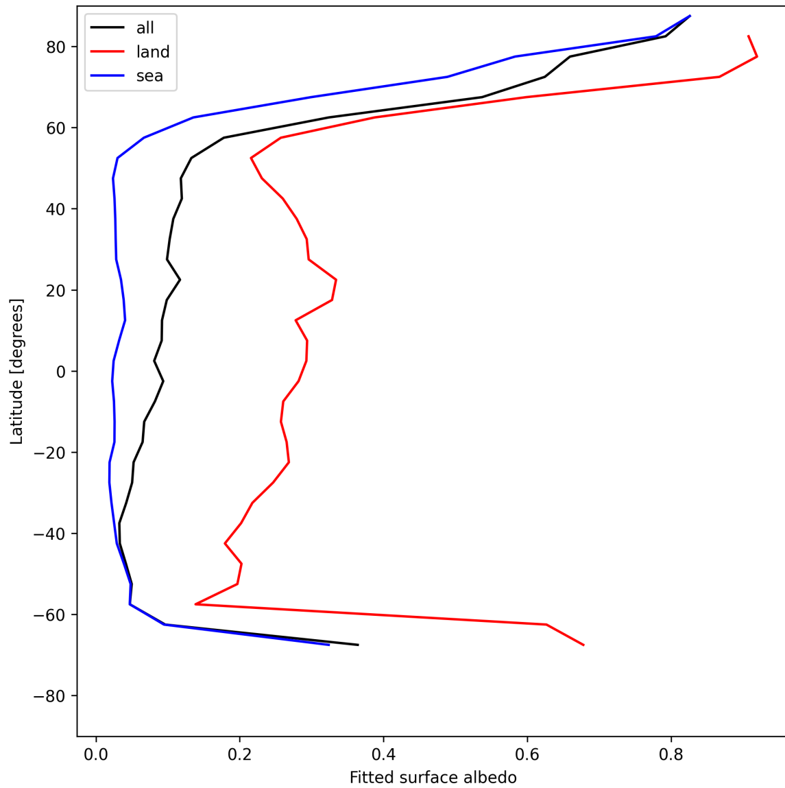
Figure 29: Zonal average of “Fitted surface albedo” for 2025-05-17 to 2025-05-19.
