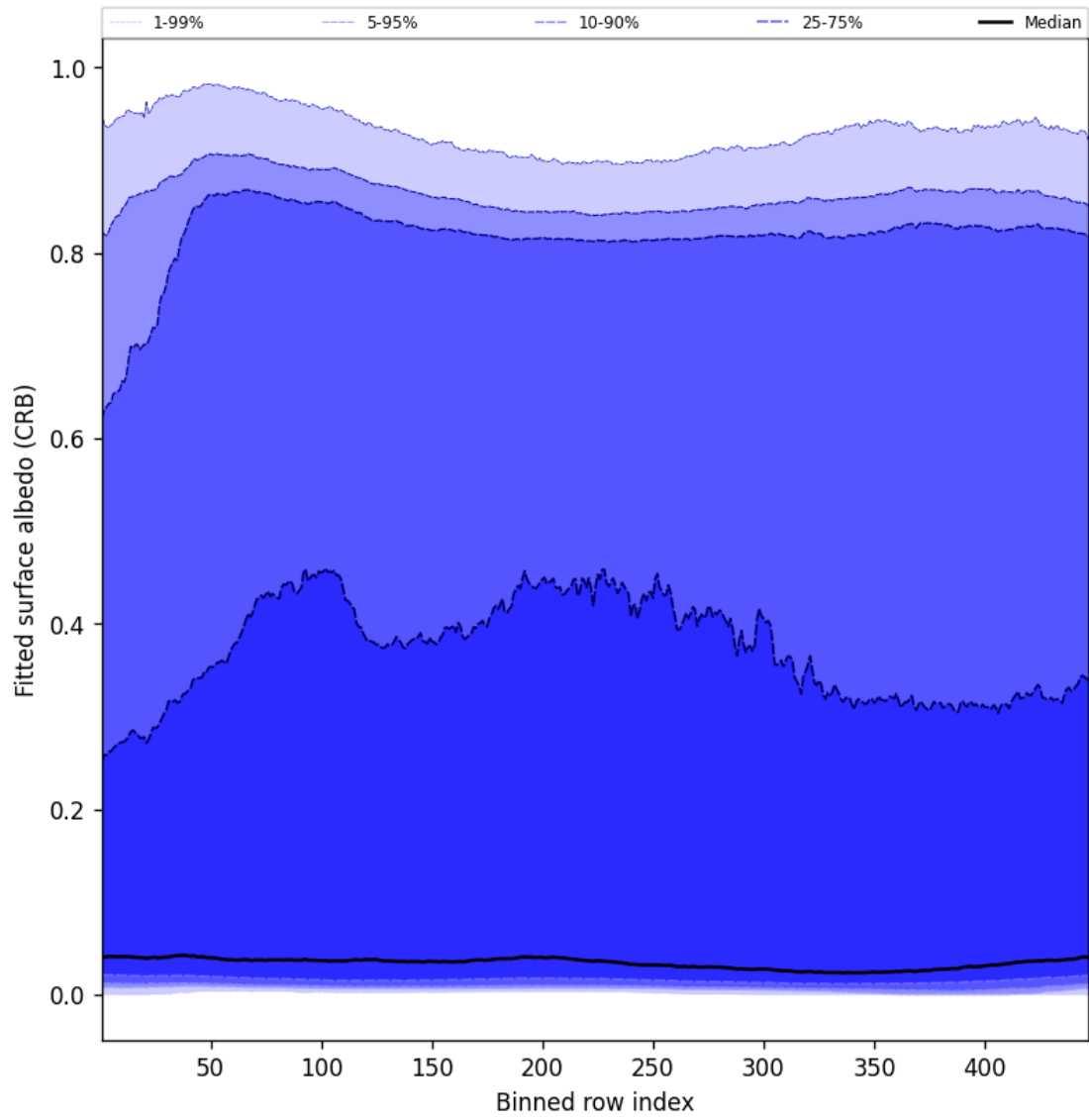
Figure 62: Along track statistics of “Fitted surface albedo (CRB)” for 2025-05-17 to 2025-05-19
