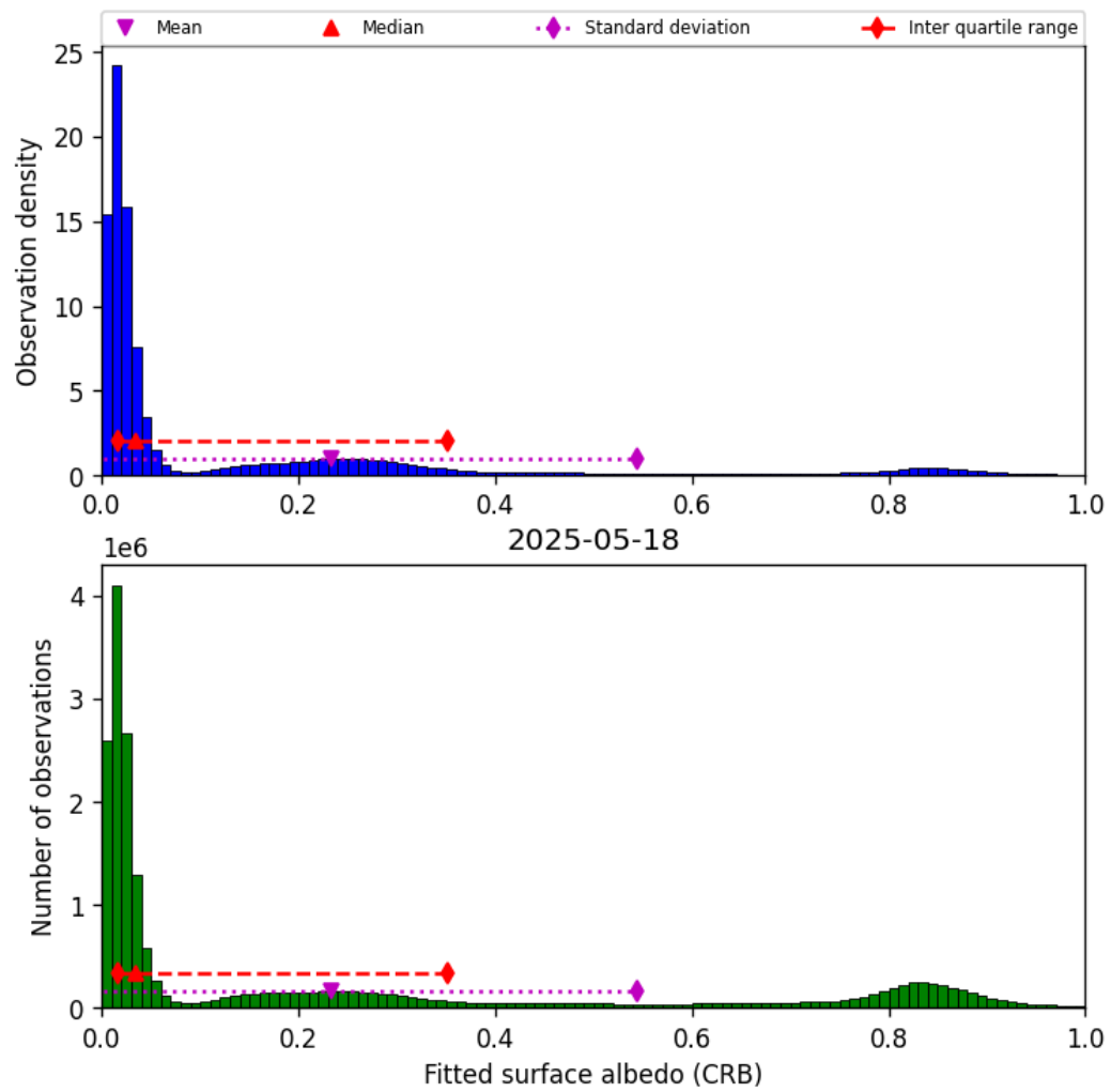
Figure 46: Histogram of “Fitted surface albedo (CRB)” for 2025-05-17 to 2025-05-19
