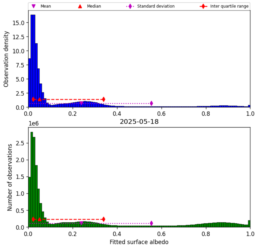
Figure 45: Histogram of “Fitted surface albedo” for 2025-05-17 to 2025-05-19
