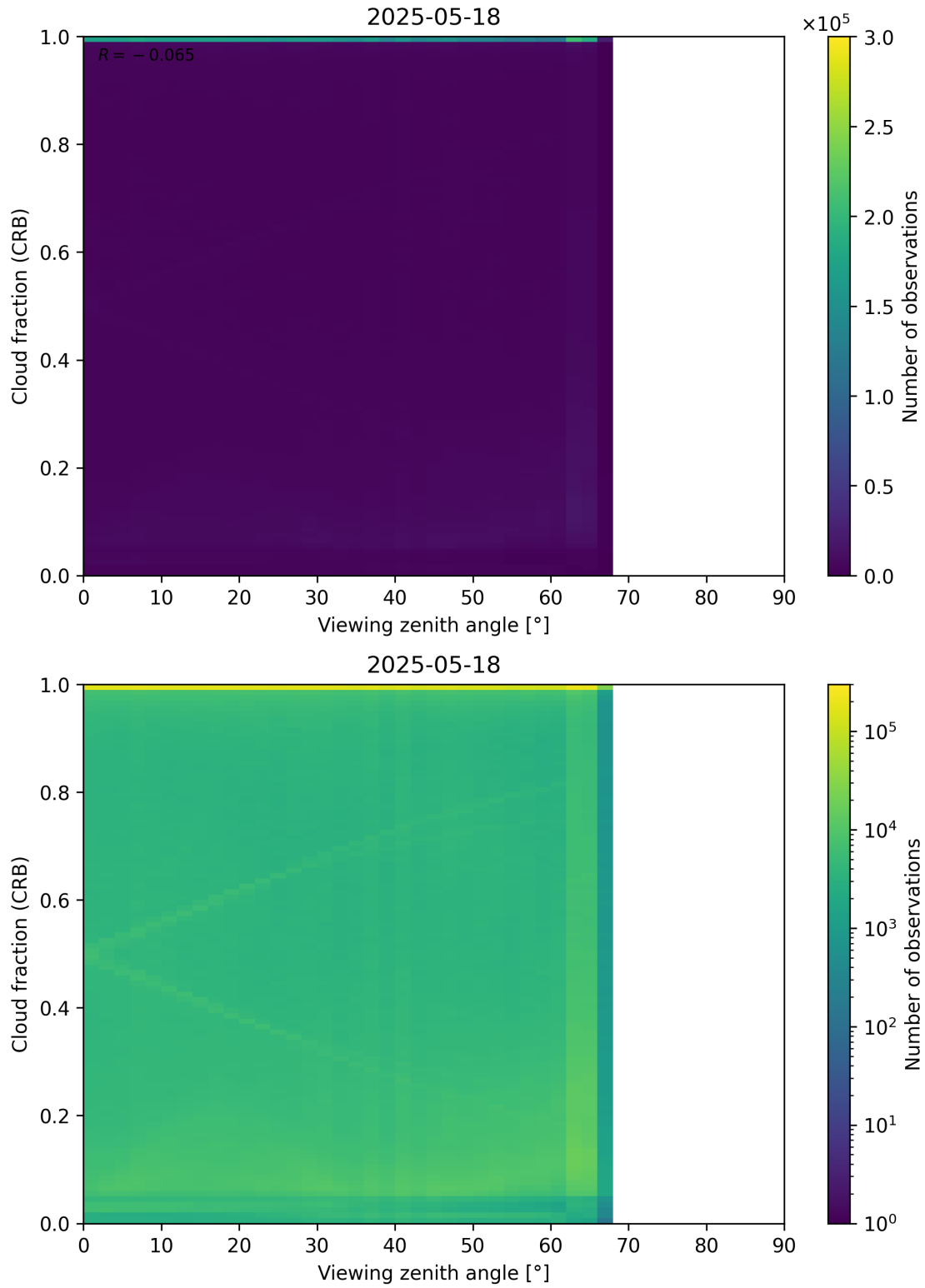
Figure 109: Scatter density plot of “Viewing zenith angle” against “Cloud fraction (CRB)” for 2025-05-17 to 2025-05-19.
