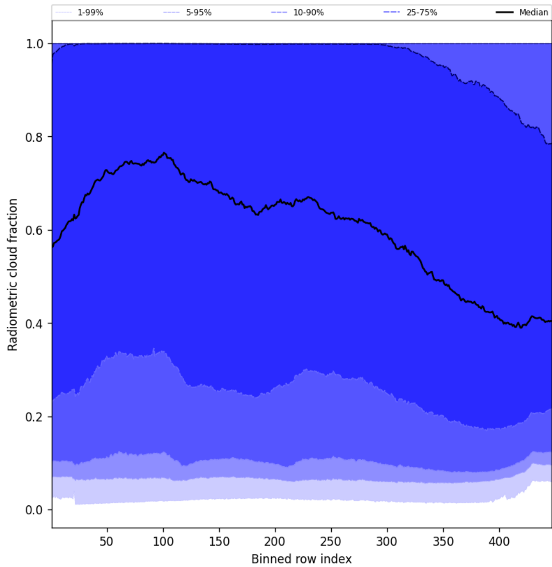
Figure 55: Along track statistics of “Radiometric cloud fraction” for 2025-05-17 to 2025-05-19
