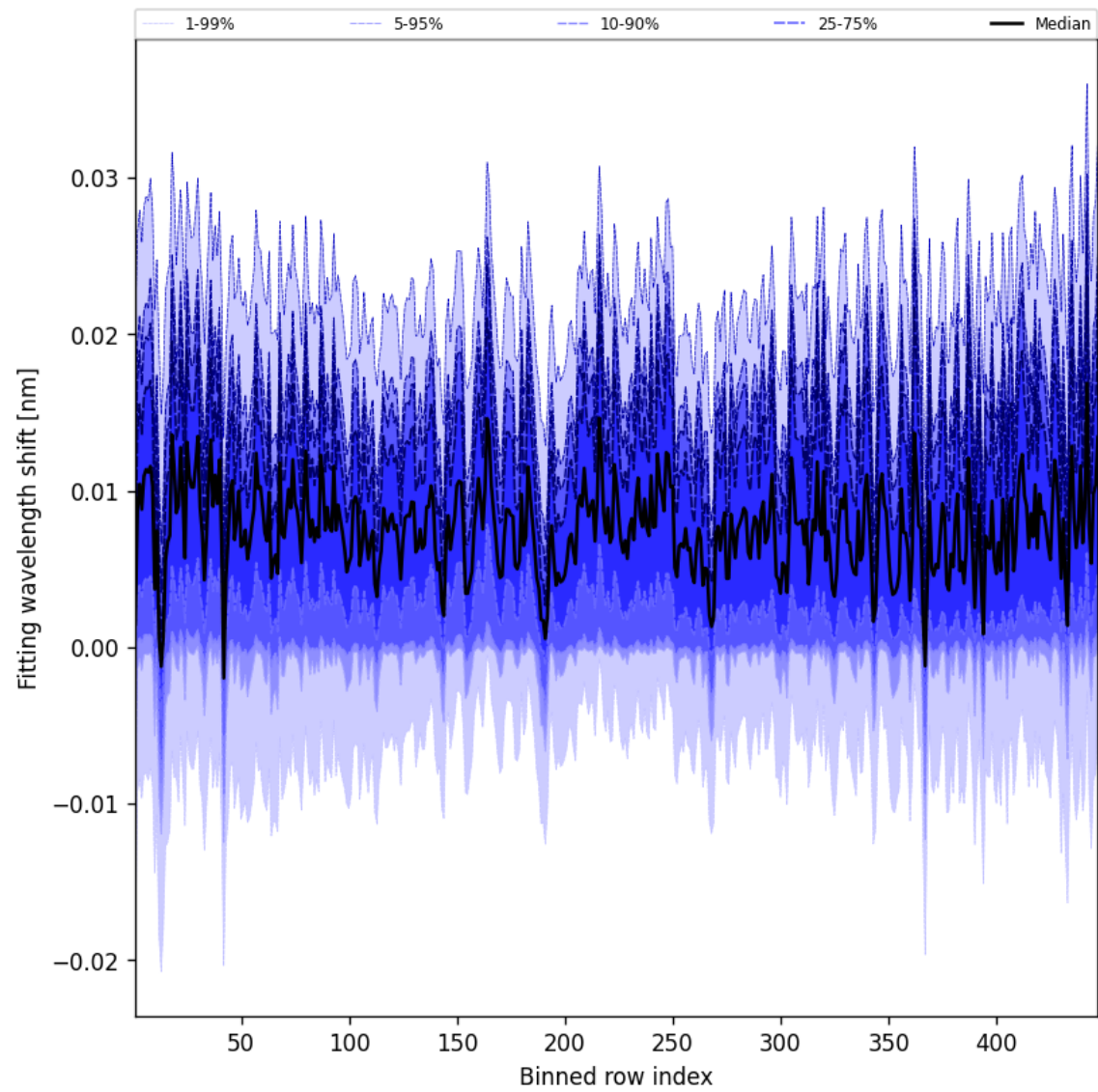
Figure 65: Along track statistics of “Fitting wavelength shift” for 2025-05-17 to 2025-05-19
