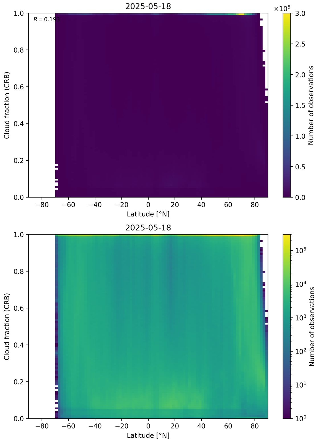
Figure 94: Scatter density plot of “Latitude” against “Cloud fraction (CRB)” for 2025-05-17 to 2025-05-19.
