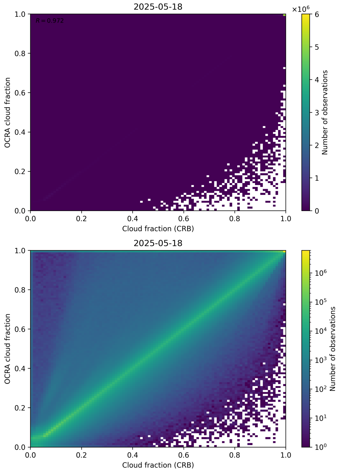
Figure 78: Scatter density plot of “Cloud fraction (CRB)” against “OCRA cloud fraction” for 2025-05-17 to 2025-05-19.
