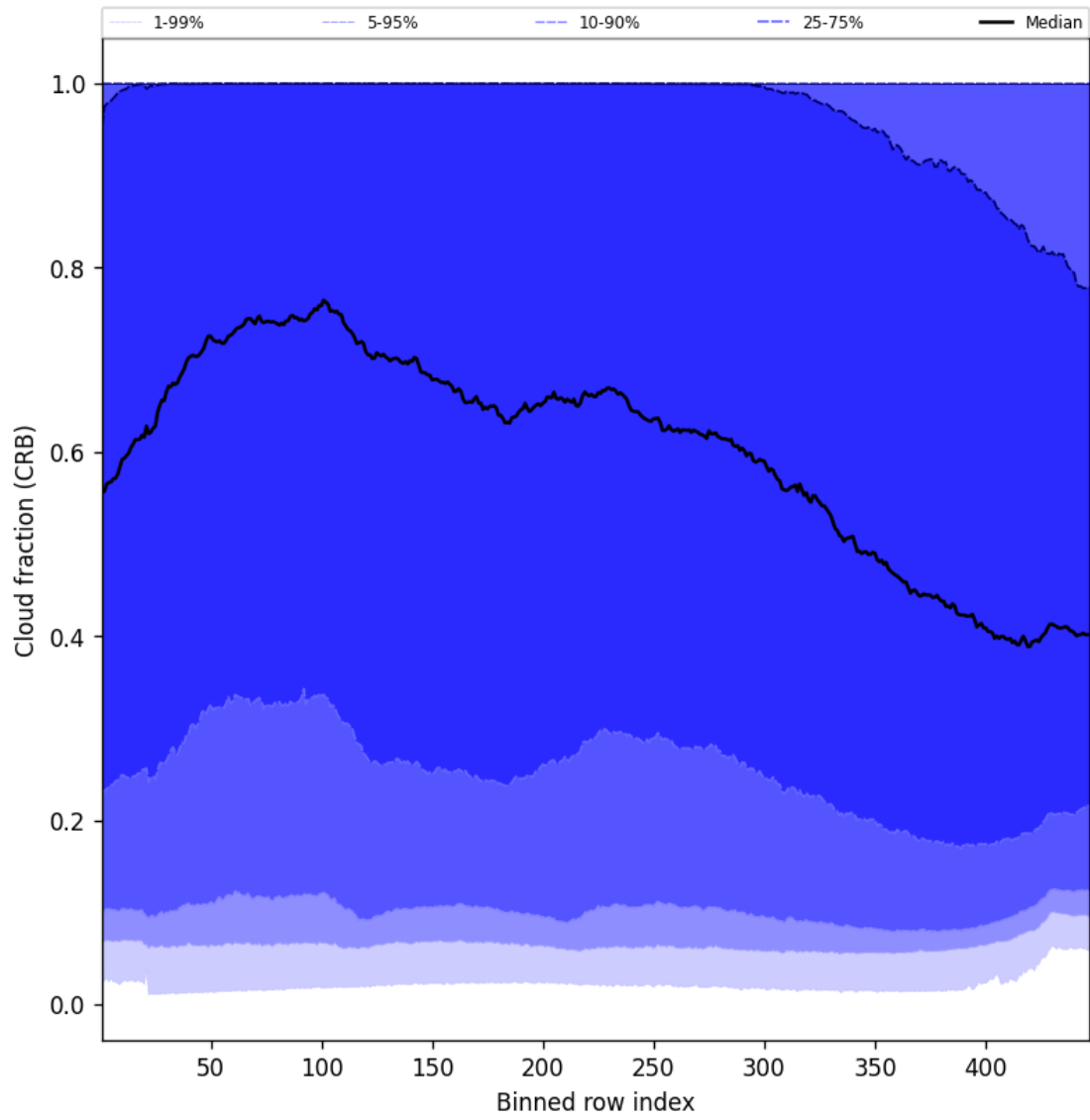
Figure 58: Along track statistics of “Cloud fraction (CRB)” for 2025-05-17 to 2025-05-19
