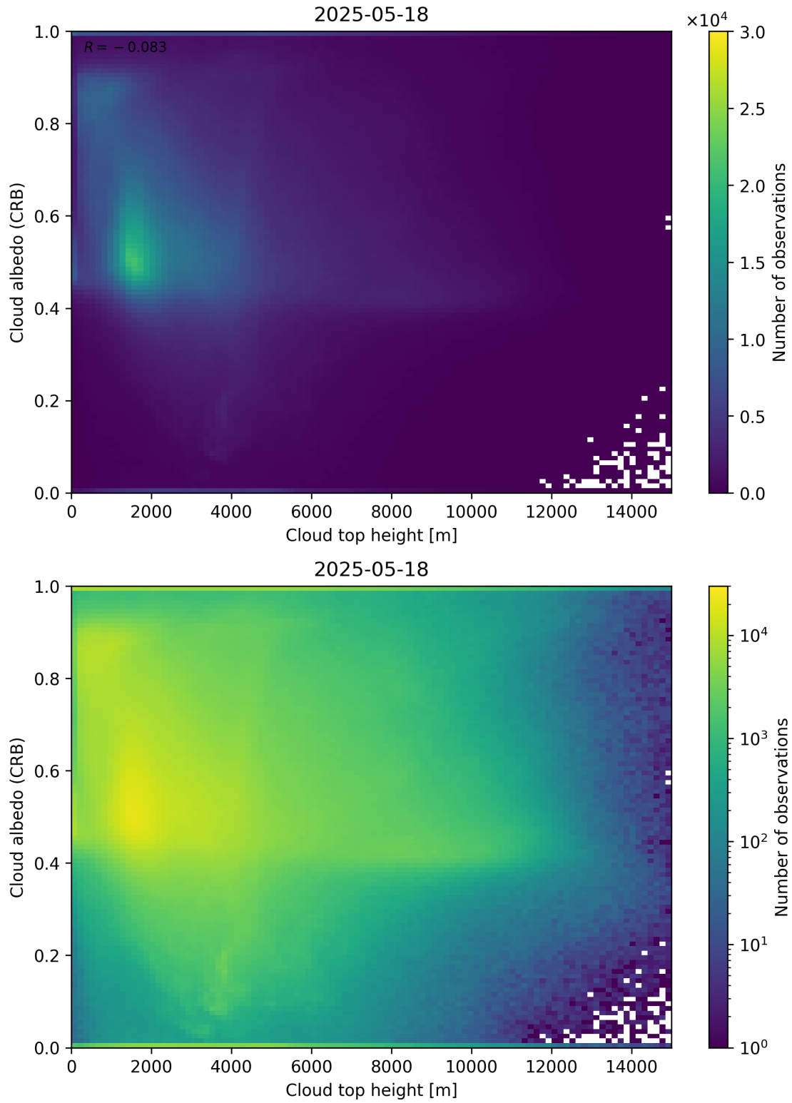
Figure 86: Scatter density plot of “Cloud top height” against “Cloud albedo (CRB)” for 2025-05-17 to 2025-05-19.
