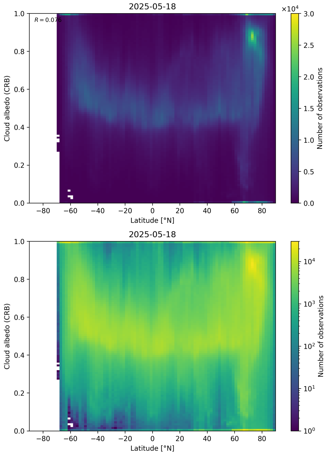
Figure 91: Scatter density plot of “Latitude” against “Cloud albedo (CRB)” for 2025-05-17 to 2025-05-19.
