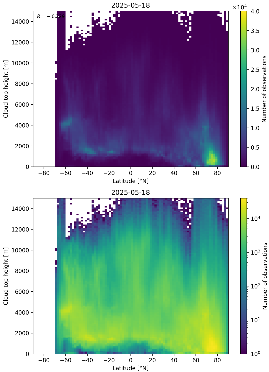
Figure 97: Scatter density plot of “Latitude” against “Cloud top height” for 2025-05-17 to 2025-05-19.
