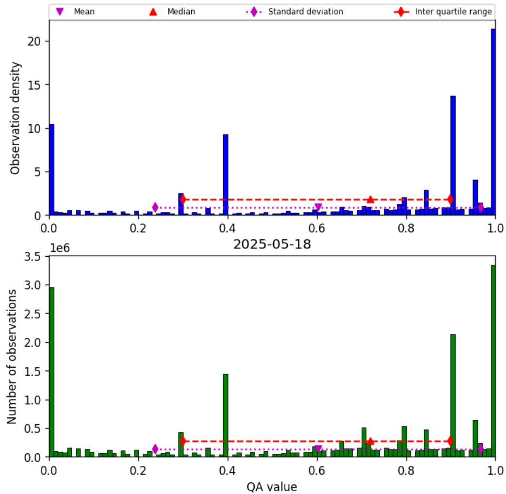
Figure 38: Histogram of “QA value” for 2025-05-17 to 2025-05-19
