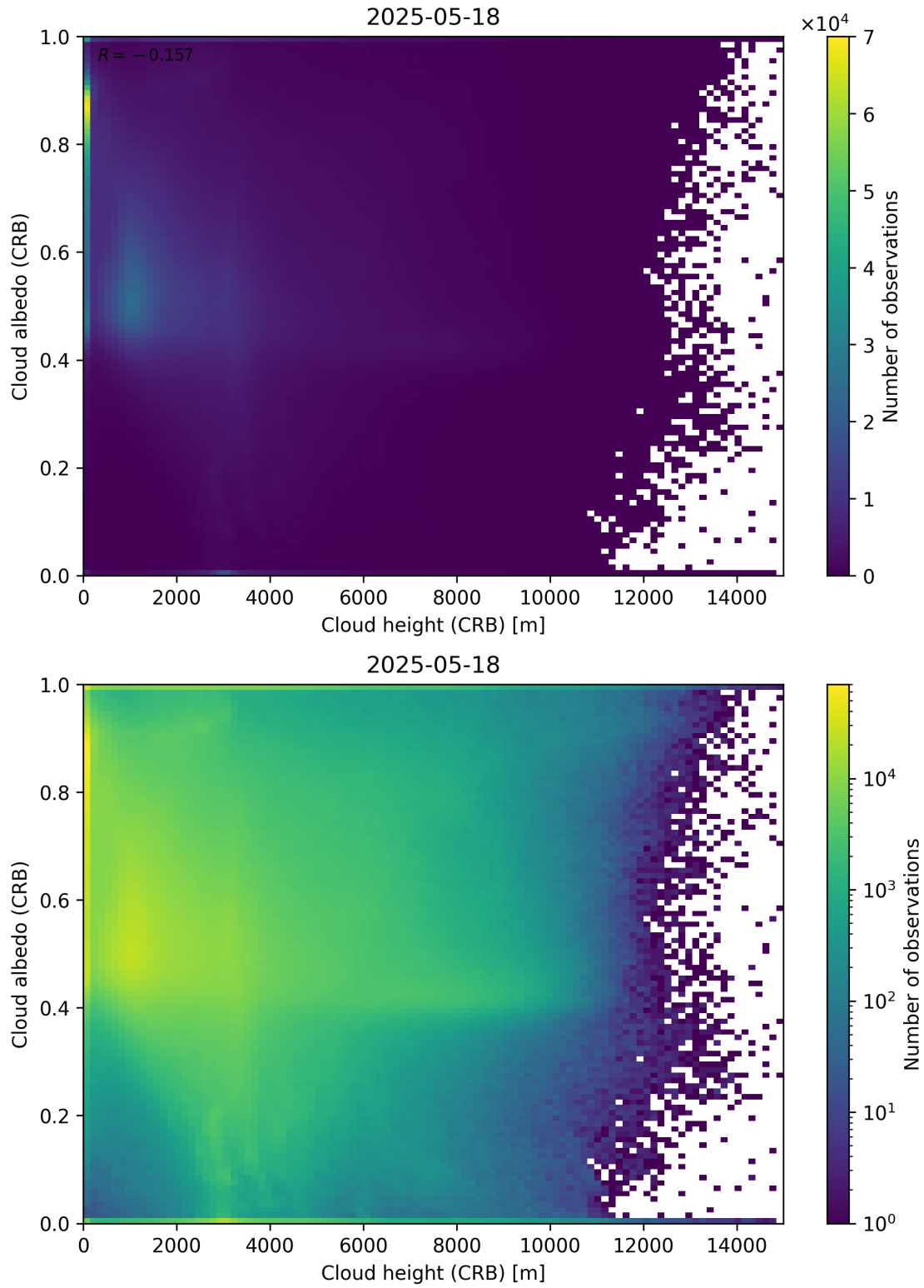
Figure 80: Scatter density plot of “Cloud height (CRB)” against “Cloud albedo (CRB)” for 2025-05-17 to 2025-05-19.
