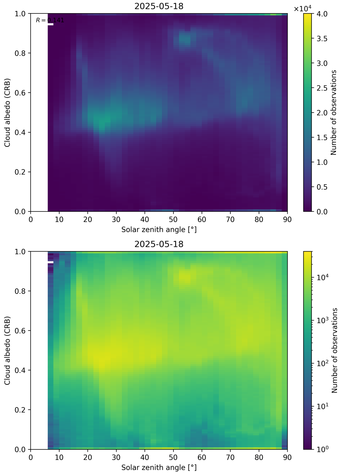
Figure 98: Scatter density plot of “Solar zenith angle” against “Cloud albedo (CRB)” for 2025-05-17 to 2025-05-19.
