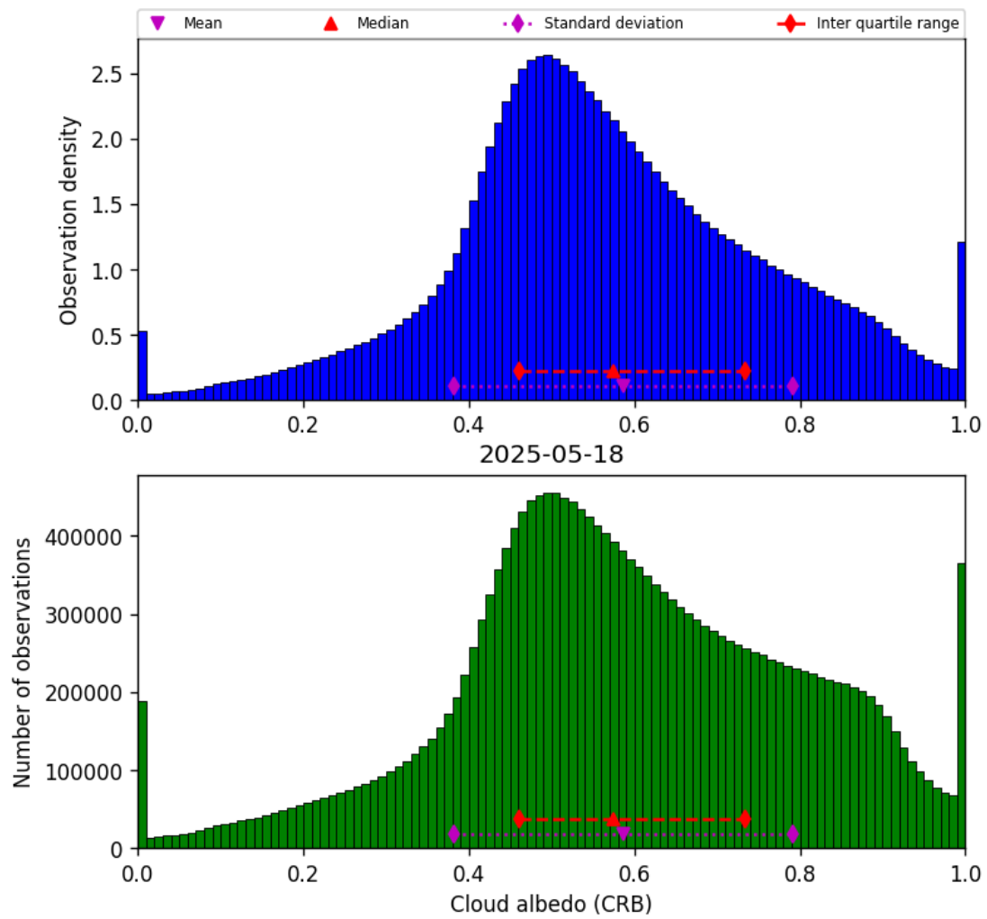
Figure 44: Histogram of “Cloud albedo (CRB)” for 2025-05-17 to 2025-05-19
