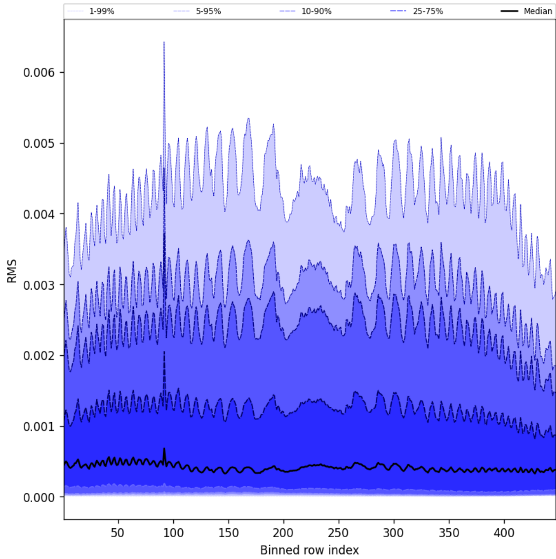
Figure 63: Along track statistics of “RMS” for 2025-05-17 to 2025-05-19
