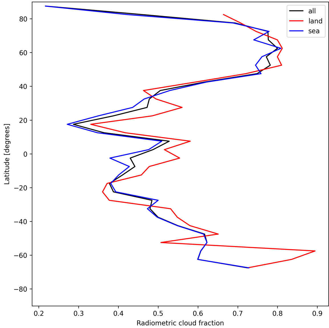
Figure 23: Zonal average of “Radiometric cloud fraction” for 2025-05-17 to 2025-05-19.
