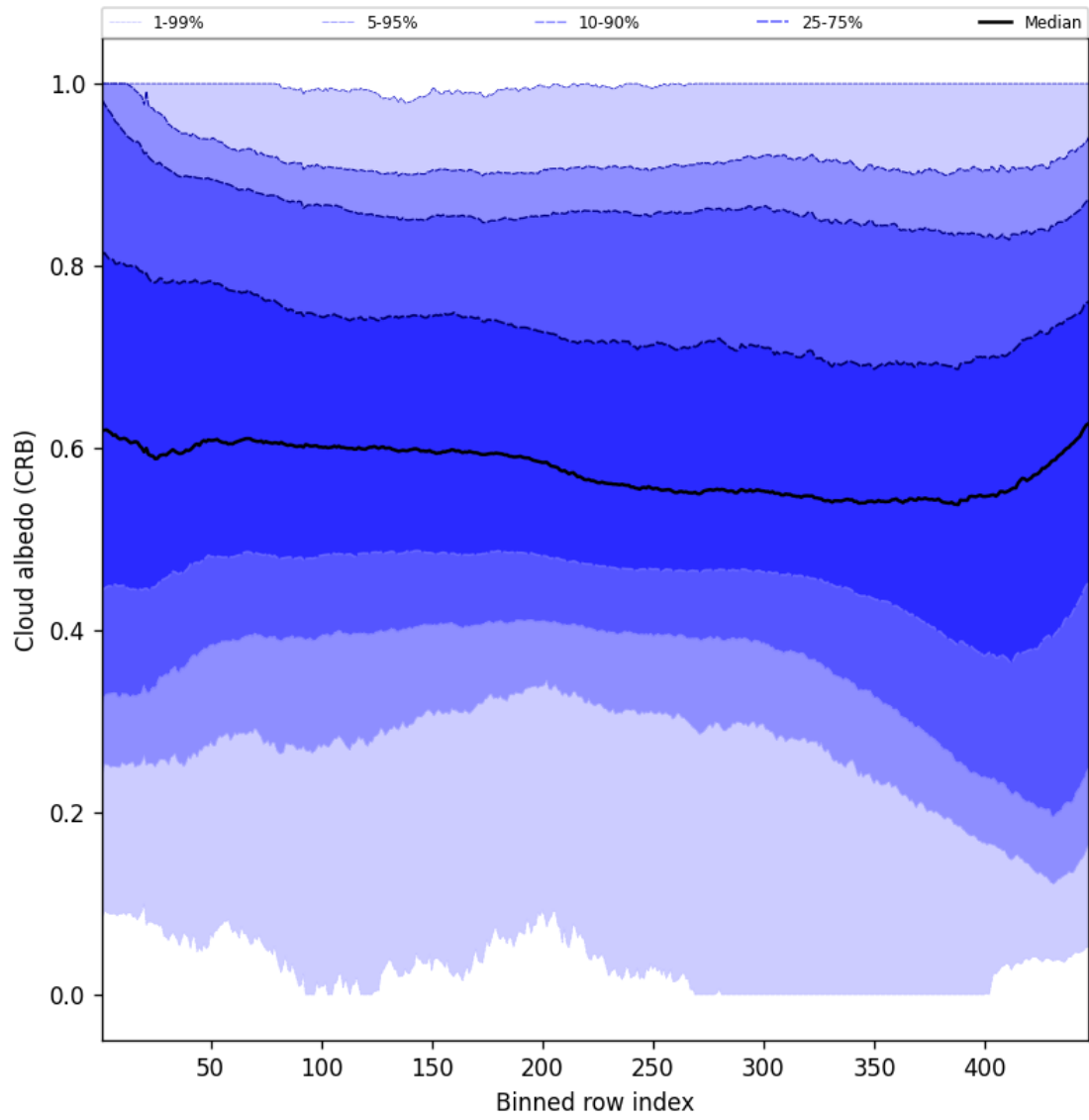
Figure 60: Along track statistics of “Cloud albedo (CRB)” for 2025-05-17 to 2025-05-19
