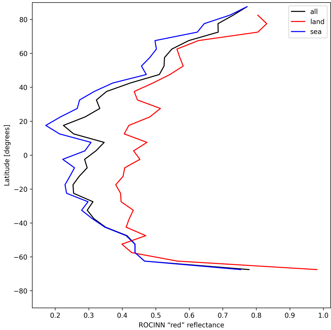
Figure 37: Zonal average of "ROCINN "red" reflectance" for 2025-05-17 to 2025-05-19.
