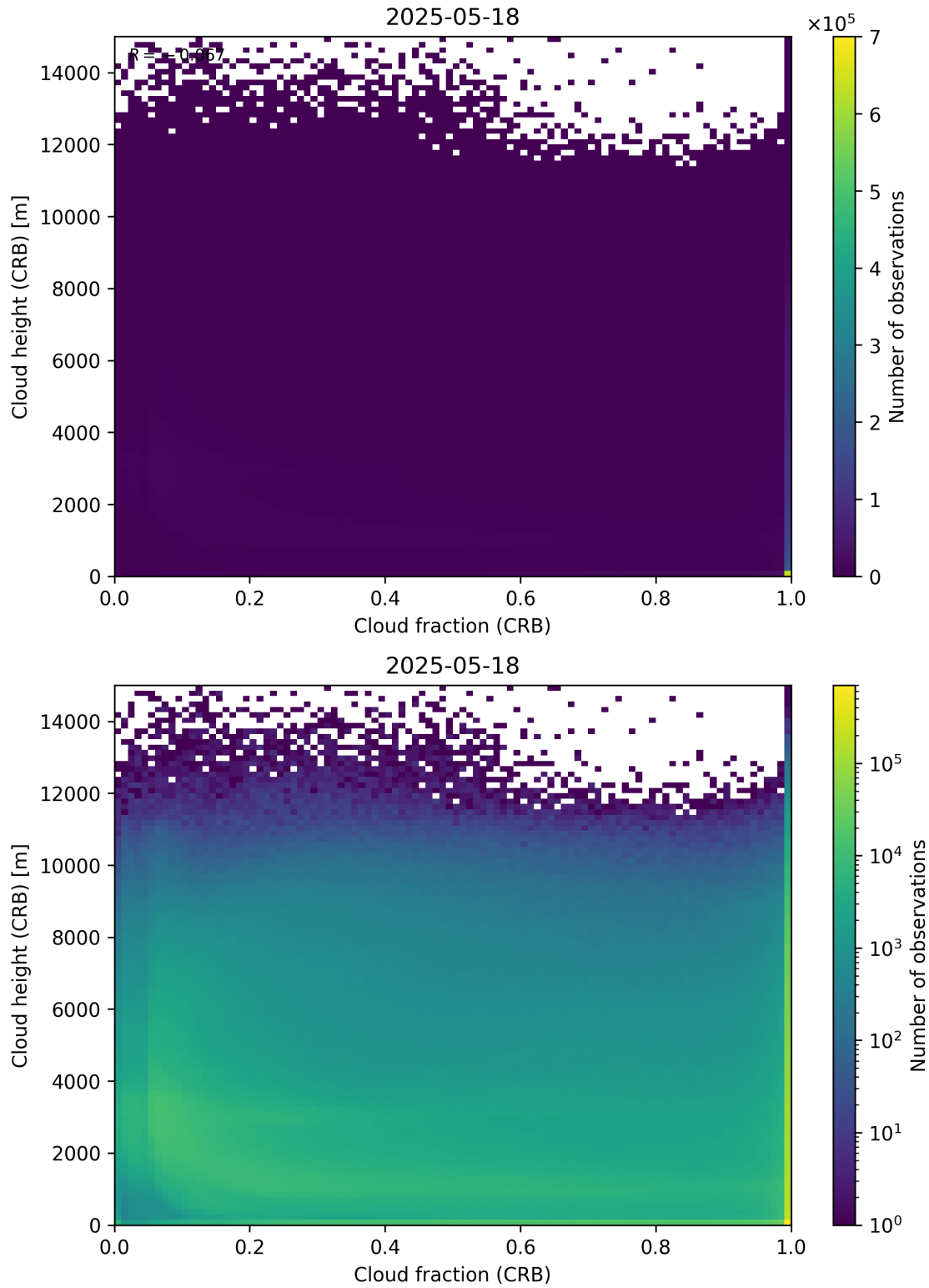
Figure 79: Scatter density plot of “Cloud fraction (CRB)” against “Cloud height (CRB)” for 2025-05-17 to 2025-05-19.
