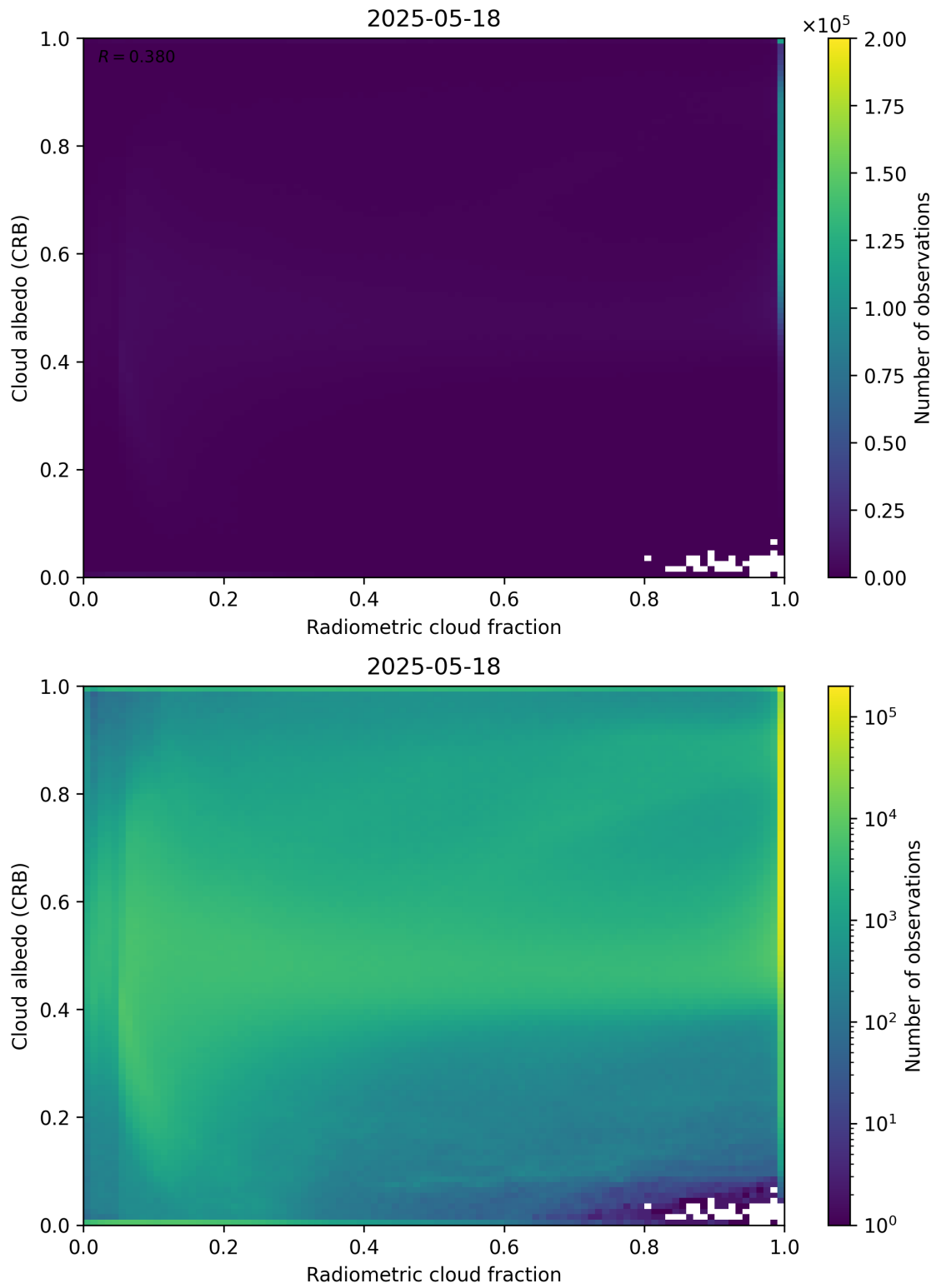
Figure 71: Scatter density plot of “Radiometric cloud fraction” against “Cloud albedo (CRB)” for 2025-05-17 to 2025-05-19.
