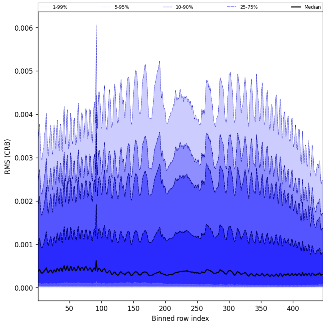
Figure 64: Along track statistics of “RMS (CRB)” for 2025-05-17 to 2025-05-19
