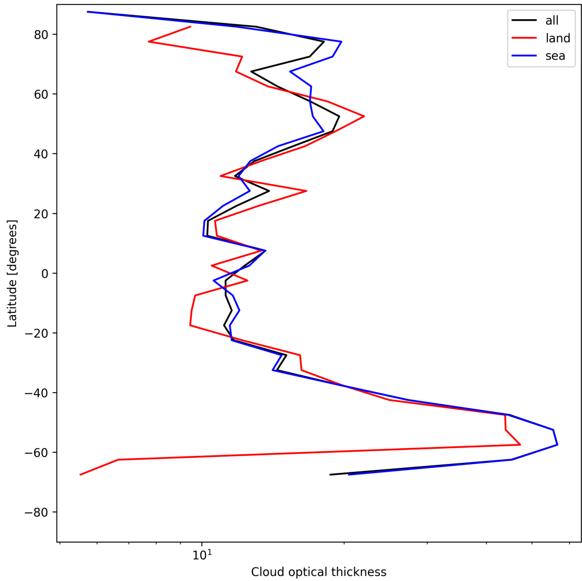
Figure 25: Zonal average of “Cloud optical thickness” for 2025-05-17 to 2025-05-19.
