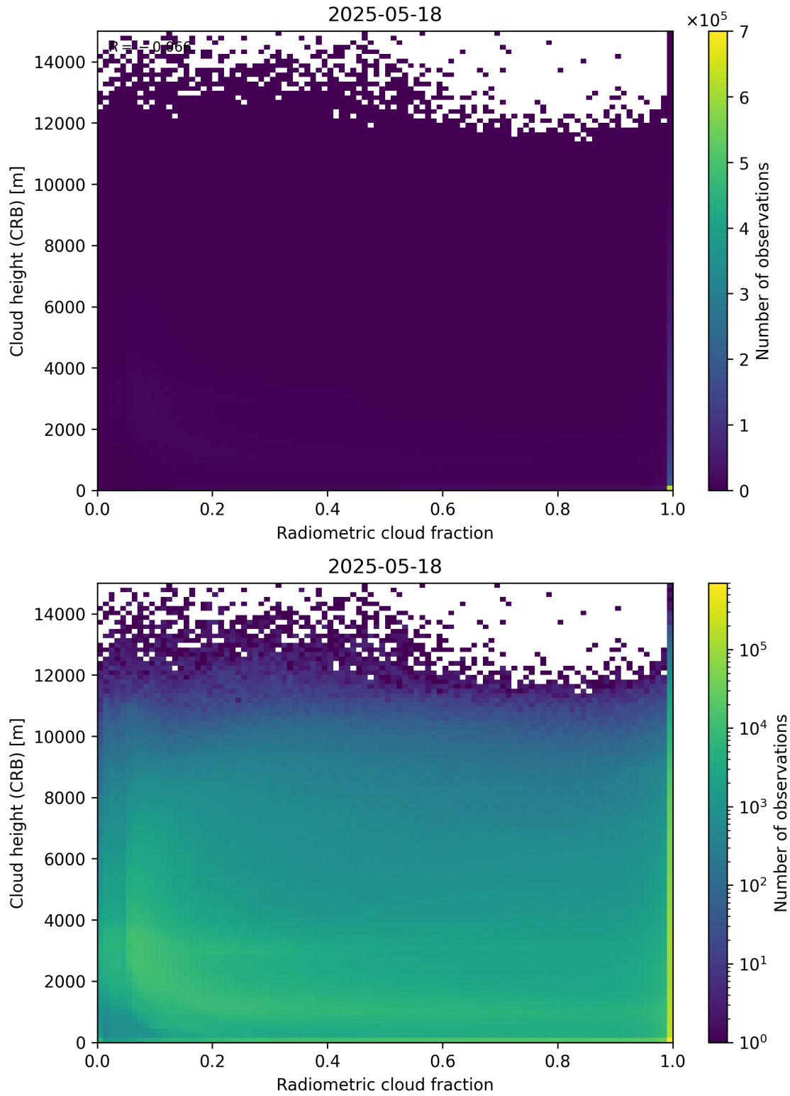
Figure 74: Scatter density plot of “Radiometric cloud fraction” against “Cloud height (CRB)” for 2025-05-17 to 2025-05-19.
