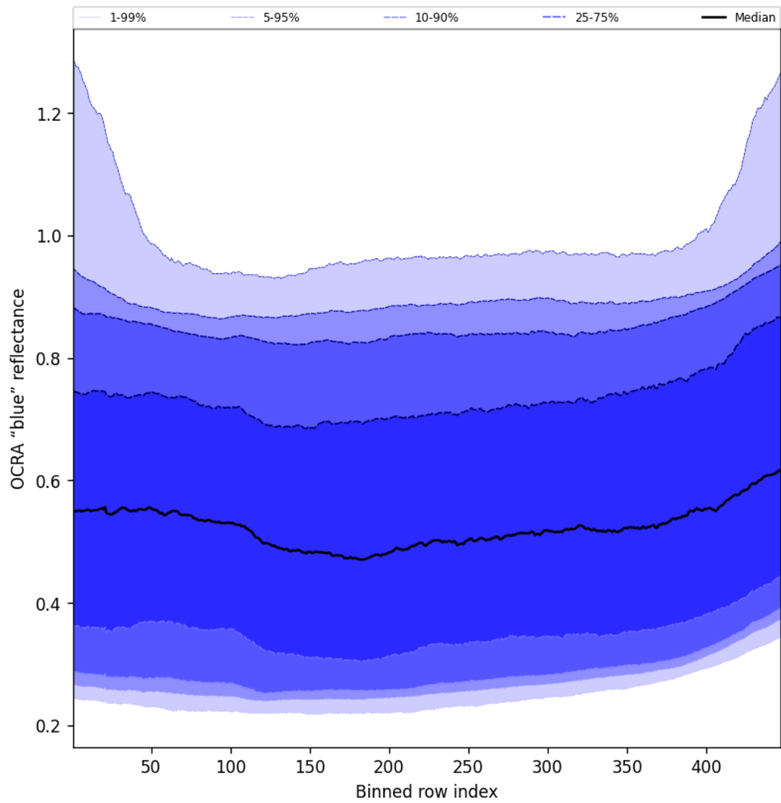
Figure 67: Along track statistics of “OCRA “blue” reflectance” for 2025-05-17 to 2025-05-19
