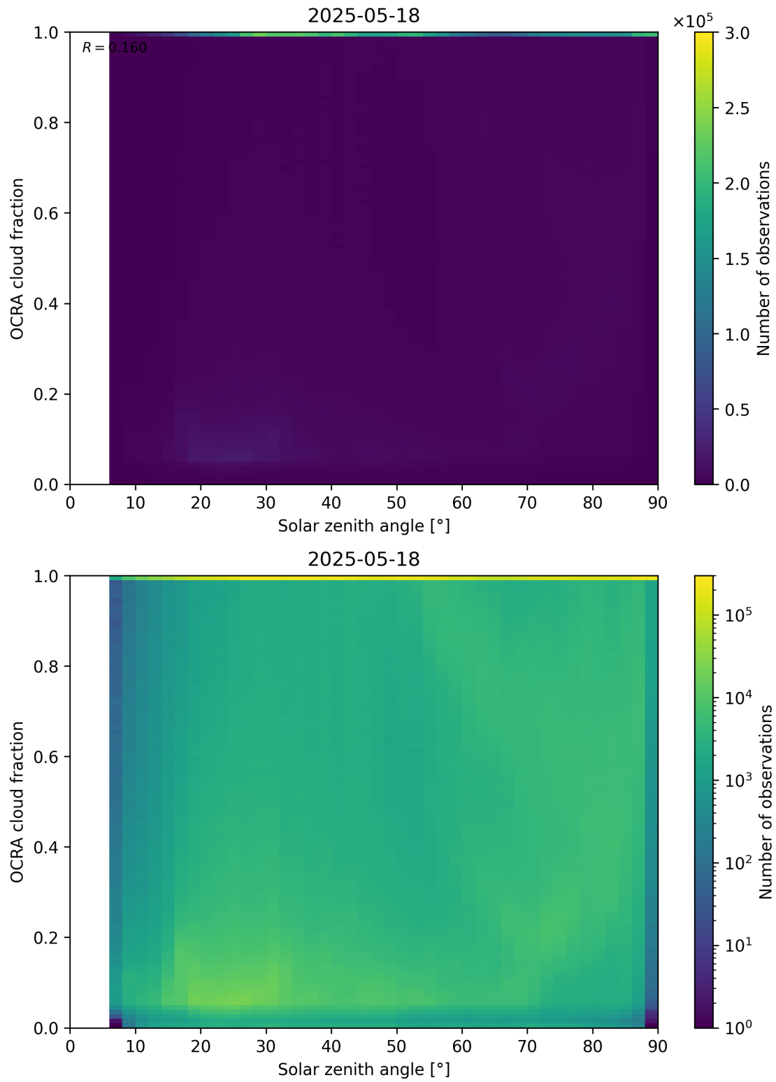
Figure 100: Scatter density plot of “Solar zenith angle” against “OCRA cloud fraction” for 2025-05-17 to 2025-05-19.
