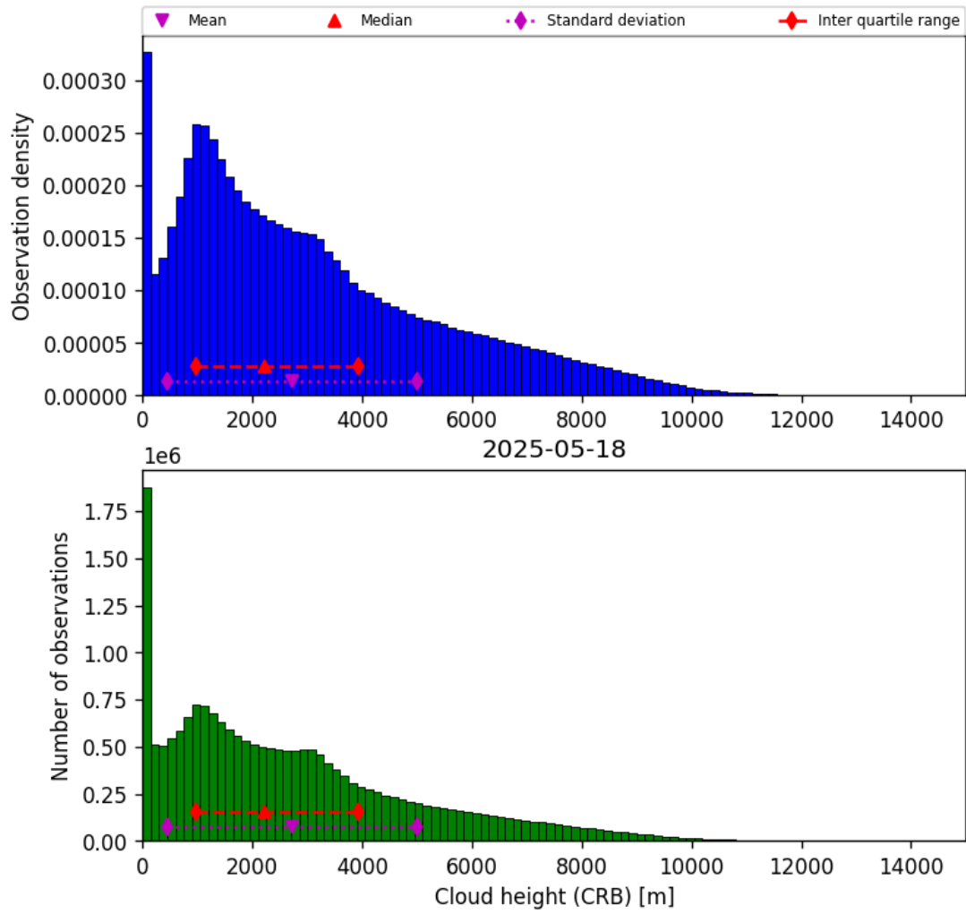
Figure 43: Histogram of “Cloud height (CRB)” for 2025-05-17 to 2025-05-19
