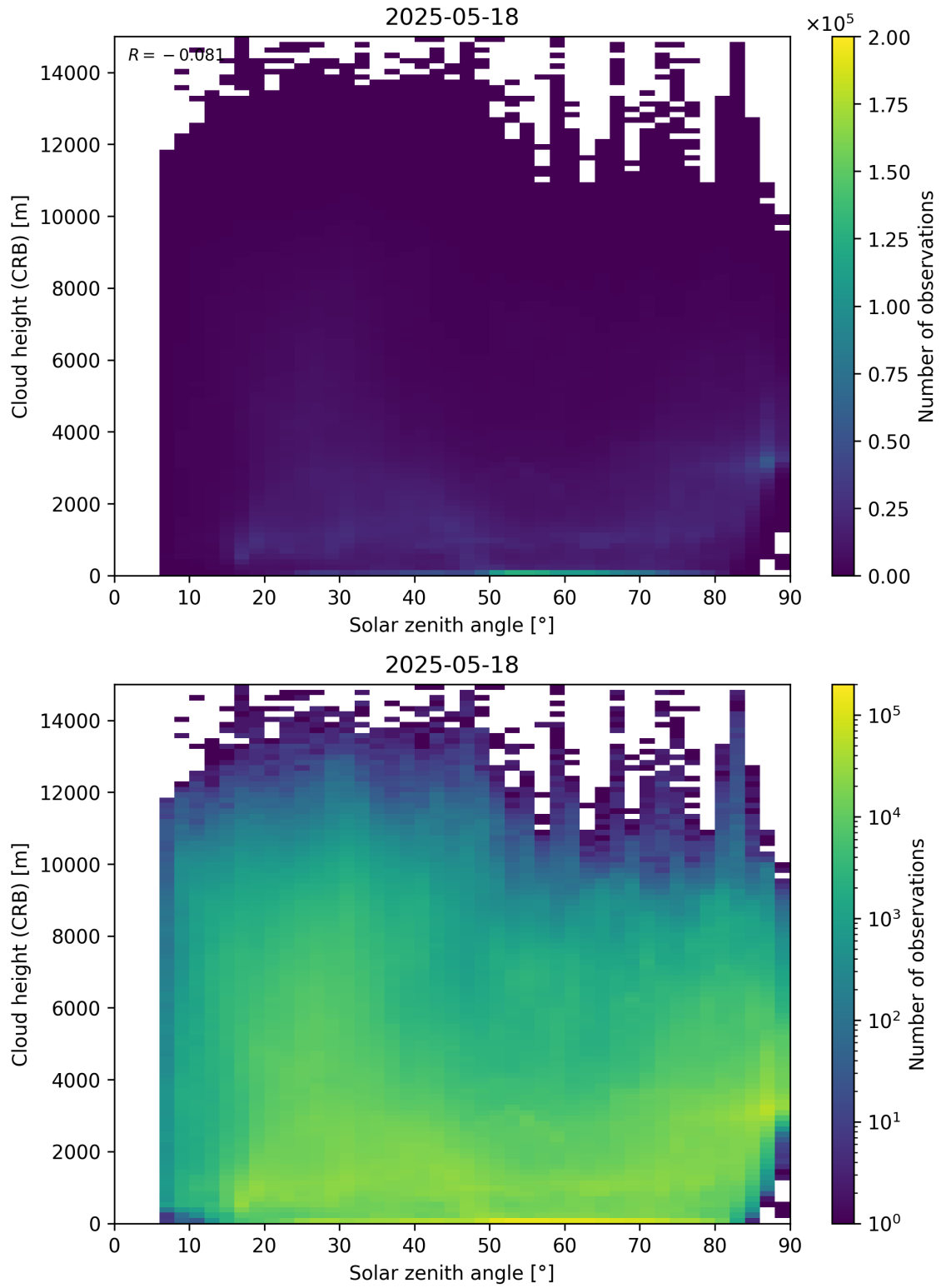
Figure 102: Scatter density plot of “Solar zenith angle” against “Cloud height (CRB)” for 2025-05-17 to 2025-05-19.
