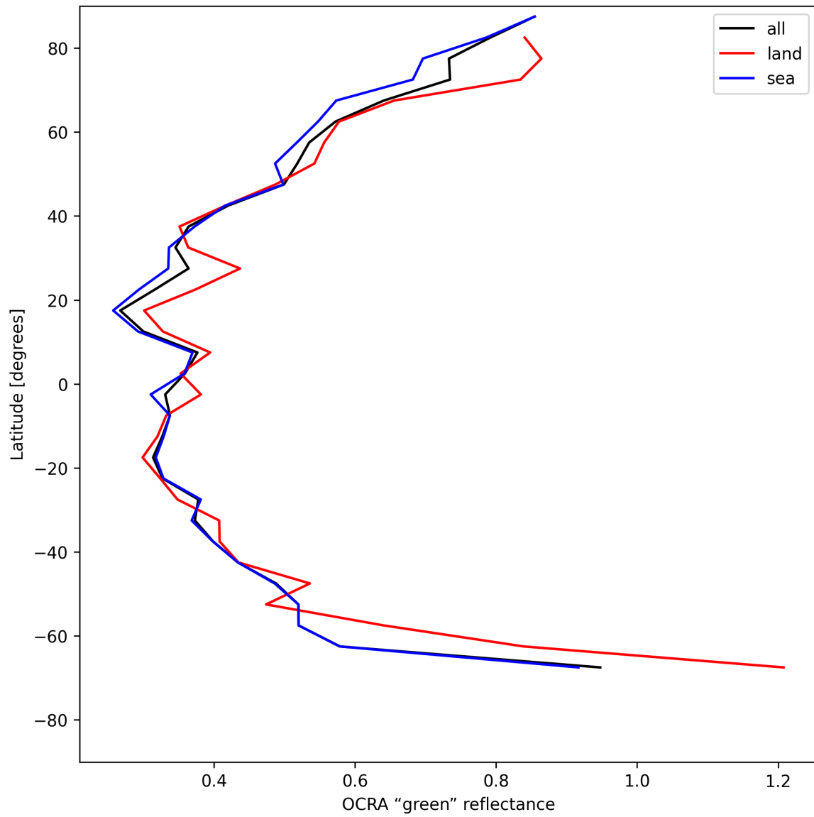
Figure 36: Zonal average of “OCRA “green” reflectance” for 2025-05-17 to 2025-05-19.
