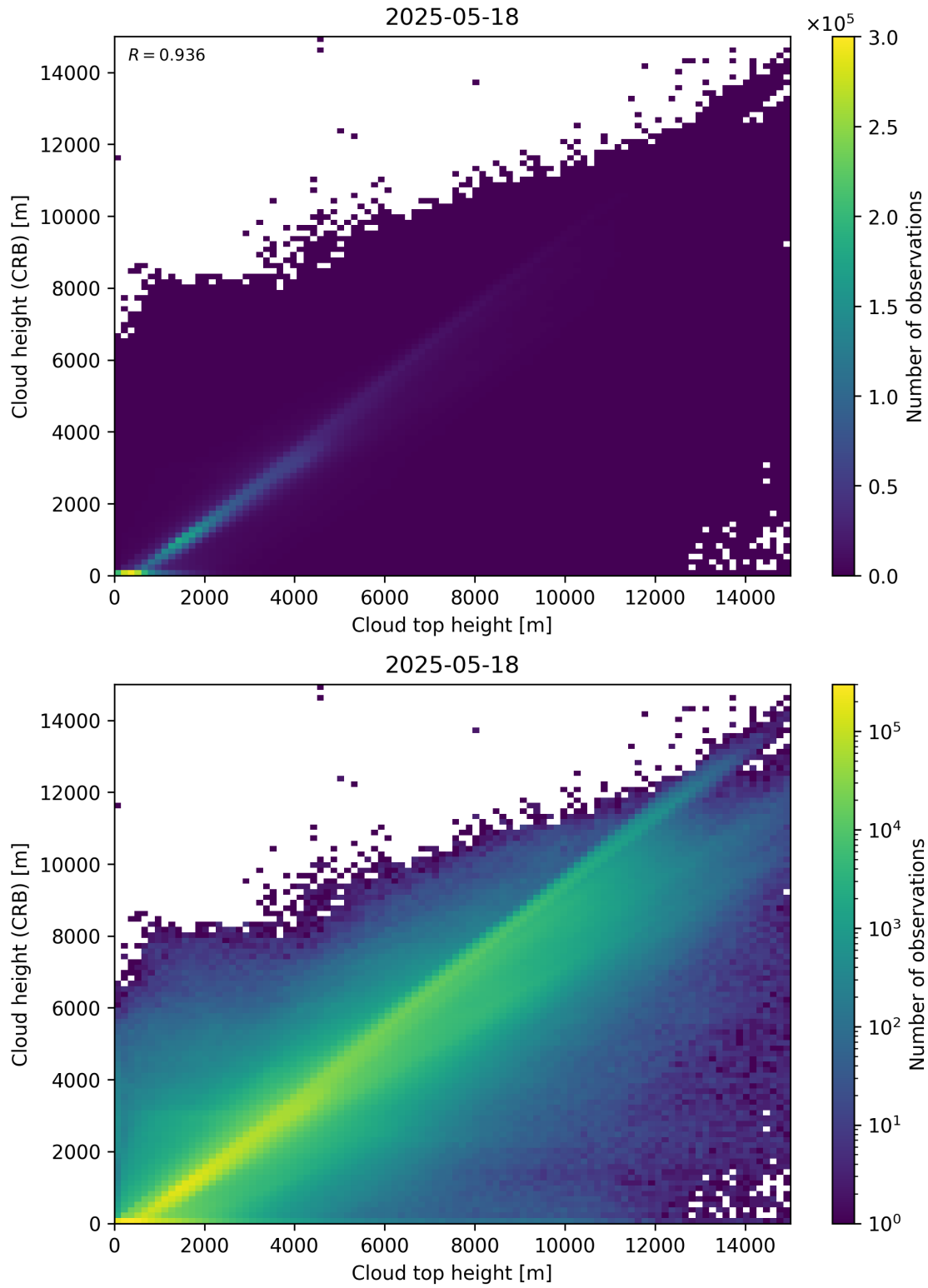
Figure 89: Scatter density plot of “Cloud top height” against “Cloud height (CRB)” for 2025-05-17 to 2025-05-19.
