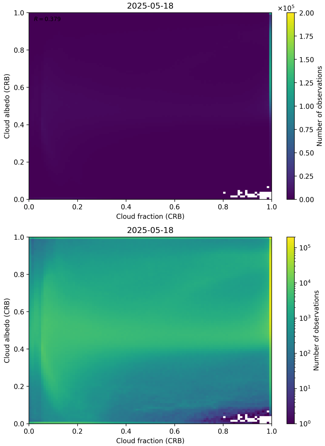
Figure 77: Scatter density plot of “Cloud fraction (CRB)” against “Cloud albedo (CRB)” for 2025-05-17 to 2025-05-19.
