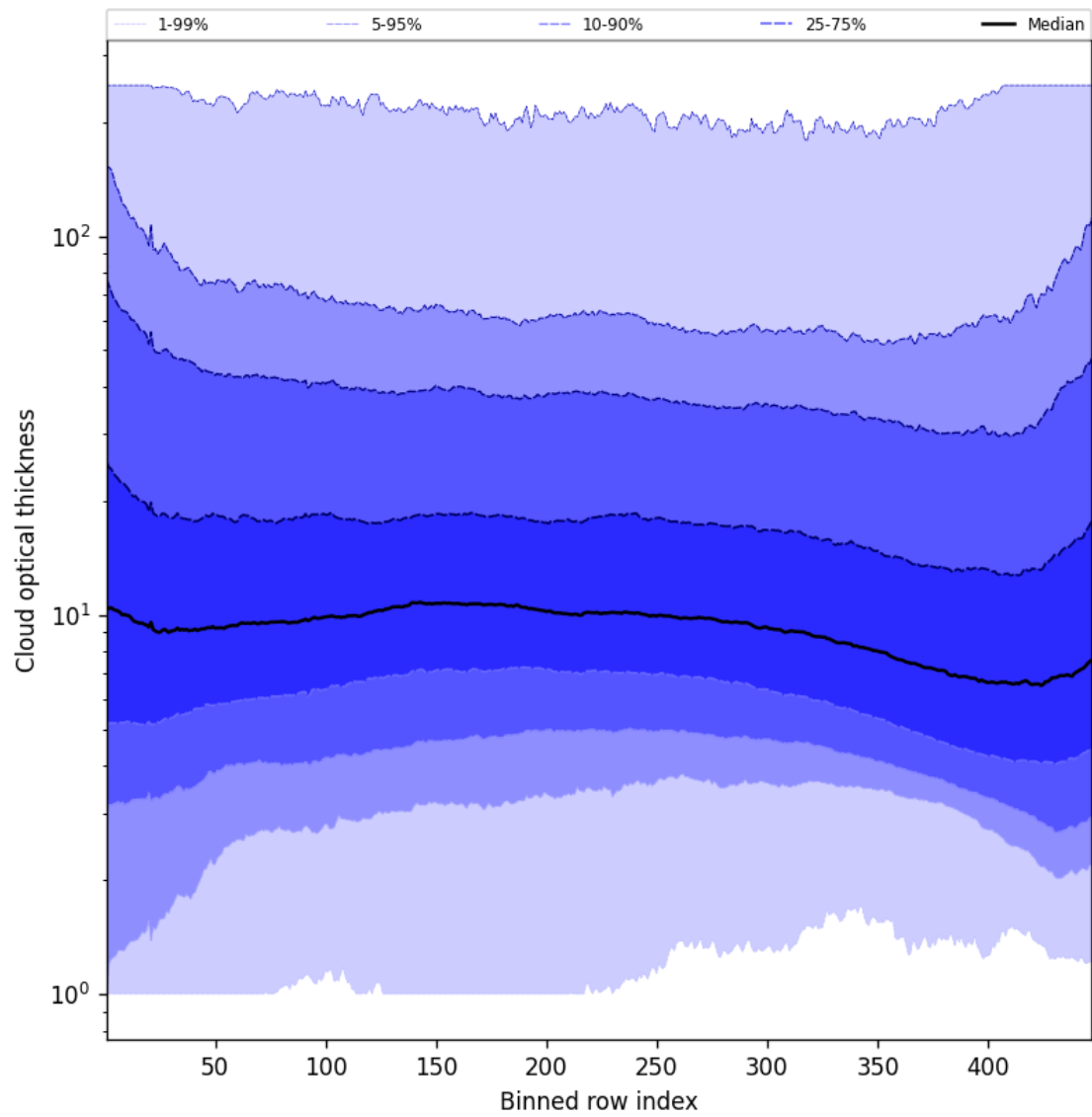
Figure 57: Along track statistics of “Cloud optical thickness” for 2025-05-17 to 2025-05-19
