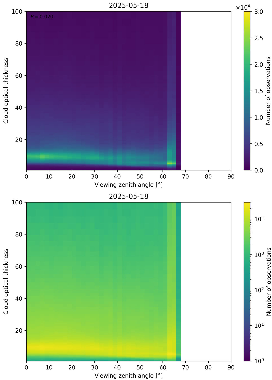
Figure 111: Scatter density plot of “Viewing zenith angle” against “Cloud optical thickness” for 2025-05-17 to 2025-05-19.
