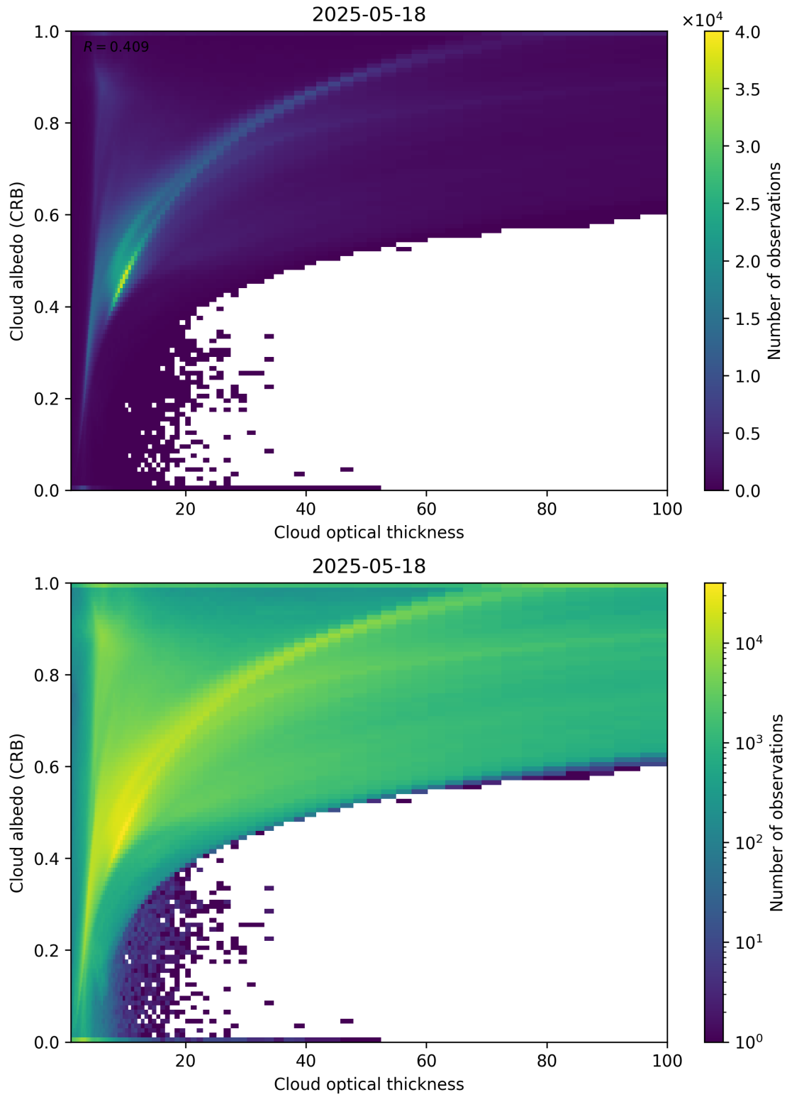
Figure 82: Scatter density plot of “Cloud optical thickness” against “Cloud albedo (CRB)” for 2025-05-17 to 2025-05-19.
