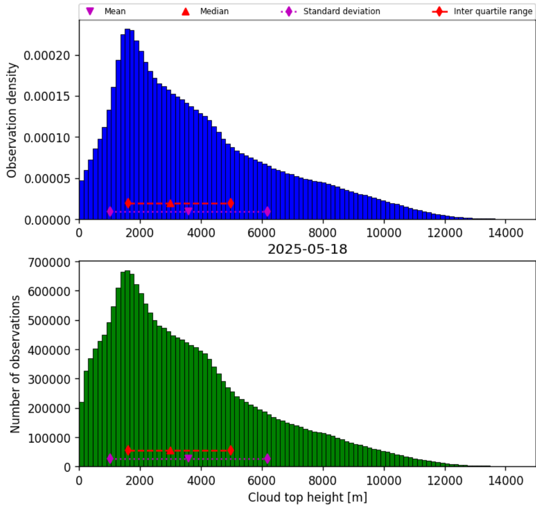
Figure 40: Histogram of “Cloud top height” for 2025-05-17 to 2025-05-19
