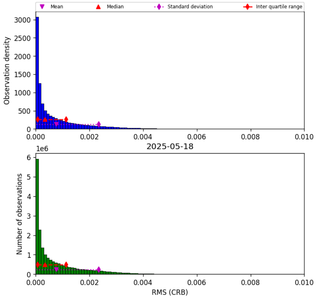
Figure 48: Histogram of “RMS (CRB)” for 2025-05-17 to 2025-05-19
