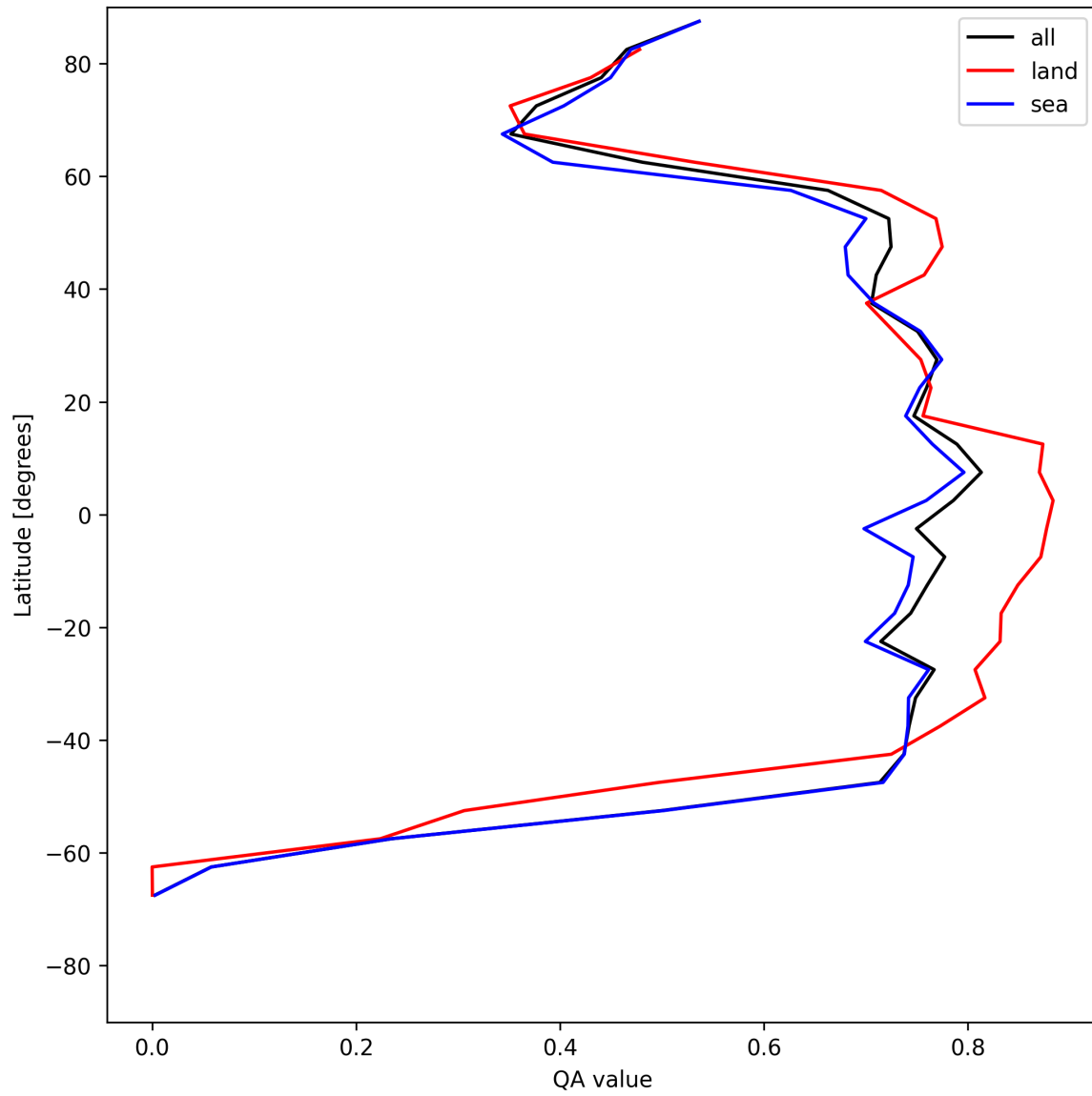
Figure 22: Zonal average of “QA value” for 2025-05-17 to 2025-05-19.
