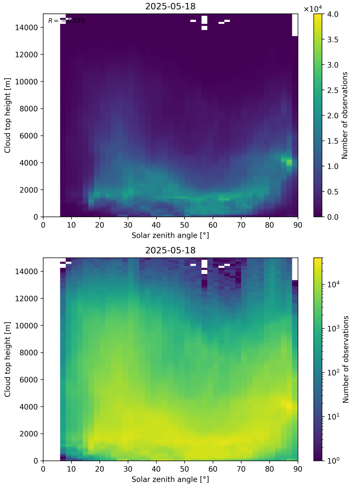
Figure 104: Scatter density plot of “Solar zenith angle” against “Cloud top height” for 2025-05-17 to 2025-05-19.
