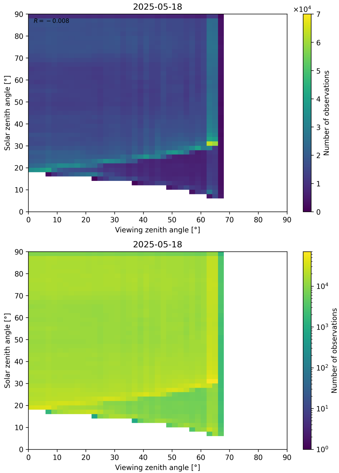
Figure 114: Scatter density plot of “Viewing zenith angle” against “Solar zenith angle” for 2025-05-17 to 2025-05-19.
