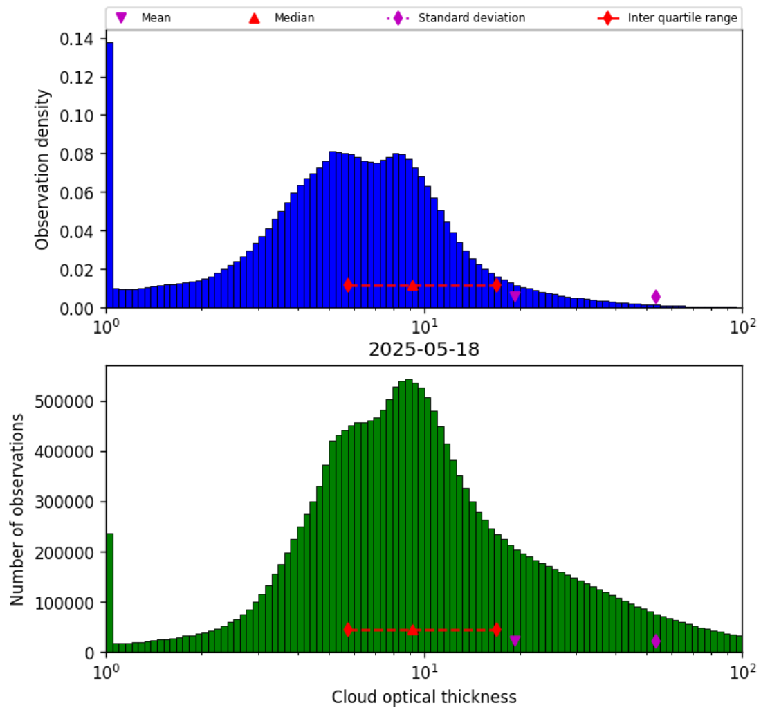
Figure 41: Histogram of “Cloud optical thickness” for 2025-05-17 to 2025-05-19
