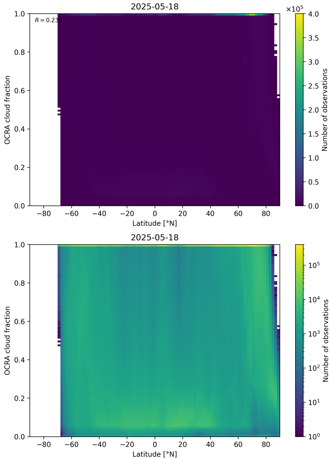
Figure 93: Scatter density plot of “Latitude” against “OCRA cloud fraction” for 2025-05-17 to 2025-05-19.
