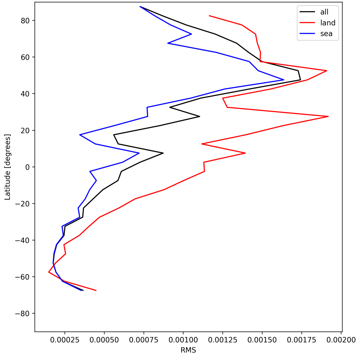
Figure 31: Zonal average of “RMS” for 2025-05-17 to 2025-05-19.
