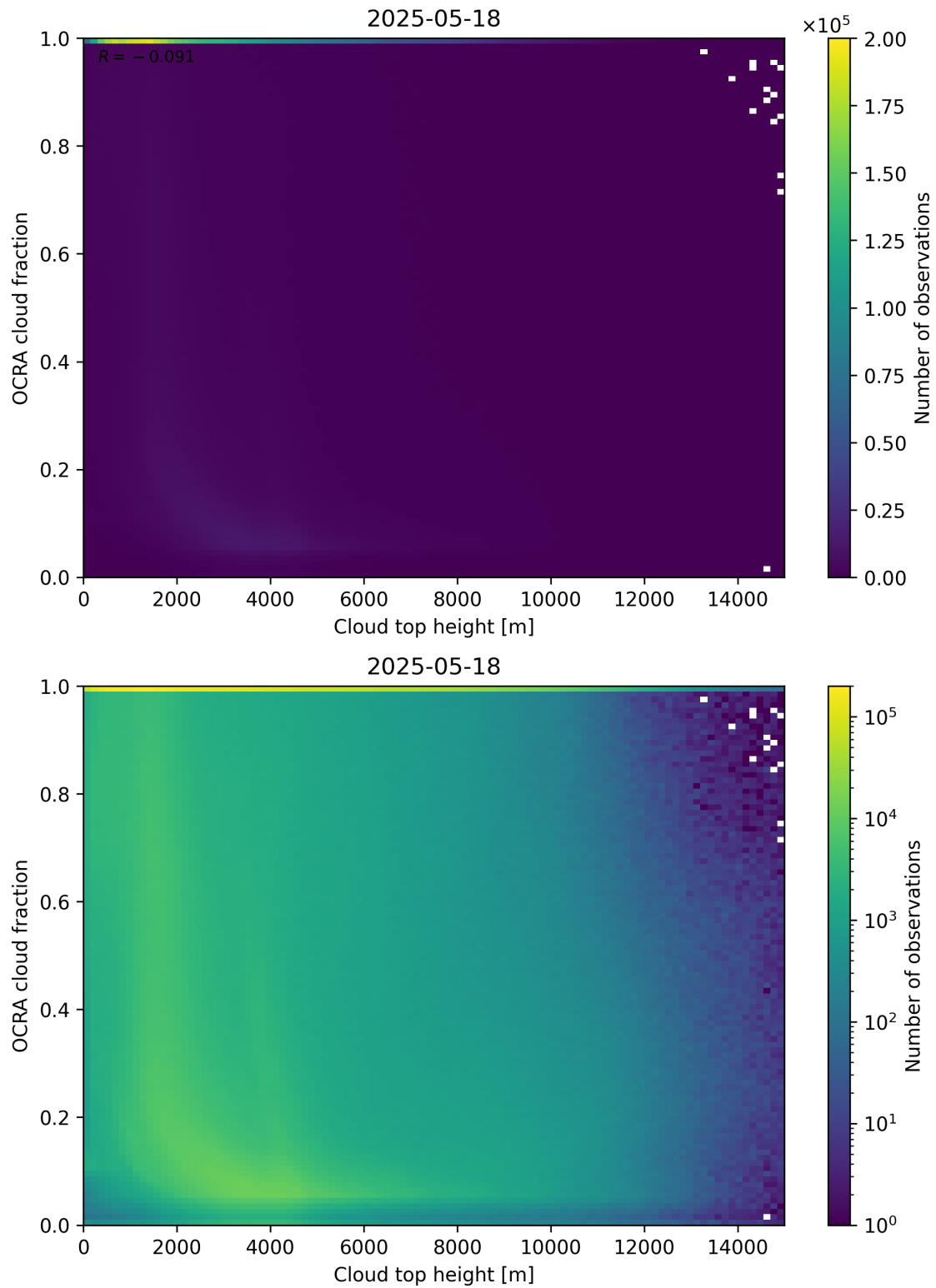
Figure 87: Scatter density plot of “Cloud top height” against “OCRA cloud fraction” for 2025-05-17 to 2025-05-19.
