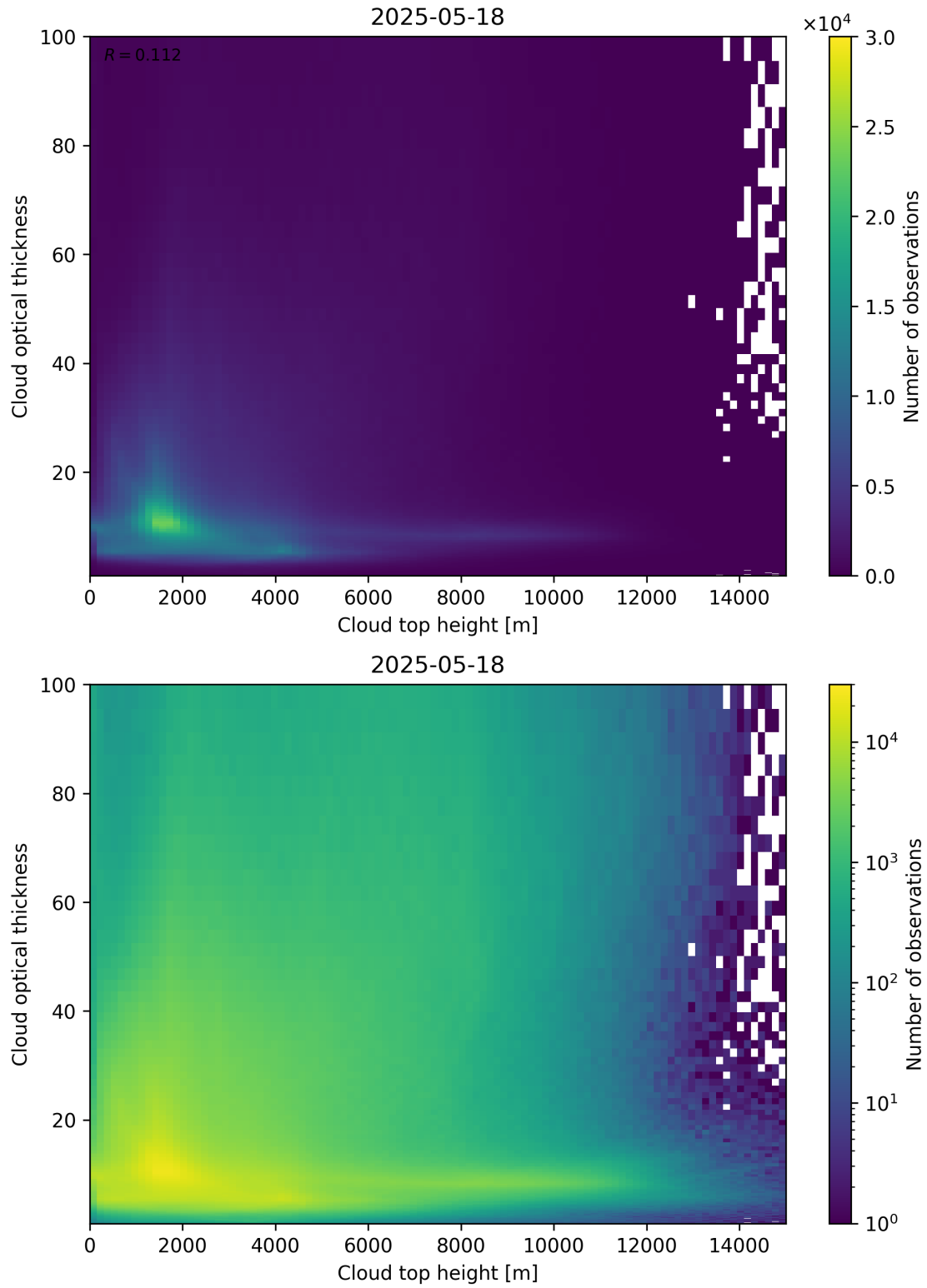
Figure 90: Scatter density plot of “Cloud top height” against “Cloud optical thickness” for 2025-05-17 to 2025-05-19.
