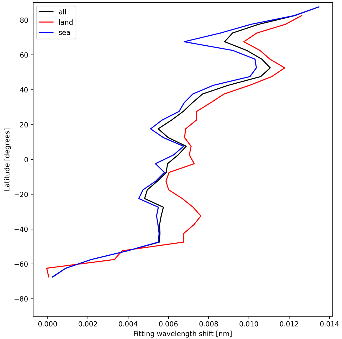
Figure 33: Zonal average of “Fitting wavelength shift” for 2025-05-17 to 2025-05-19.
