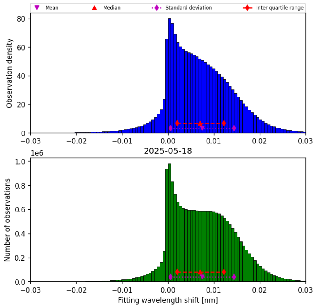
Figure 49: Histogram of “Fitting wavelength shift” for 2025-05-17 to 2025-05-19
