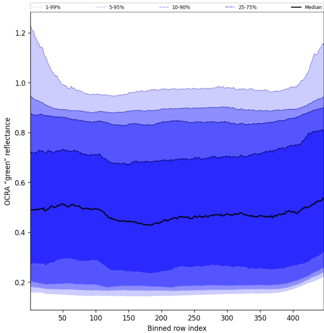
Figure 68: Along track statistics of “OCRA “green” reflectance” for 2025-05-17 to 2025-05-19
