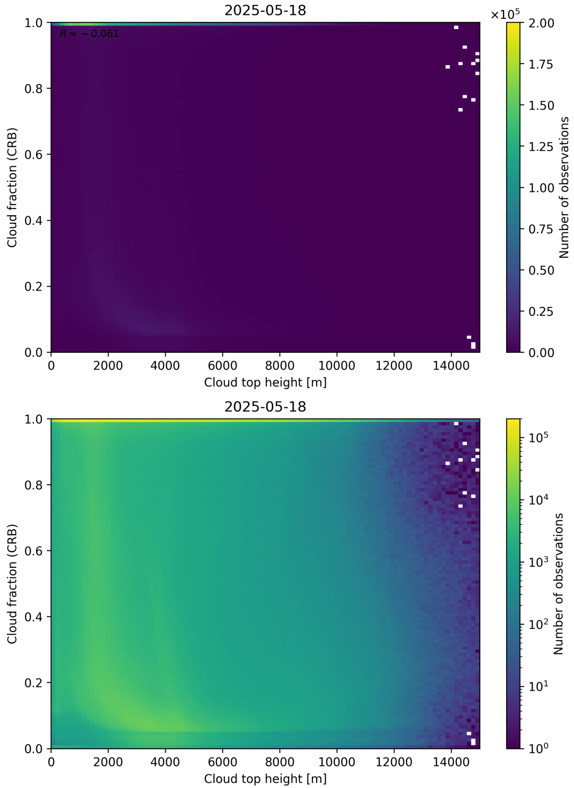
Figure 88: Scatter density plot of “Cloud top height” against “Cloud fraction (CRB)” for 2025-05-17 to 2025-05-19.
