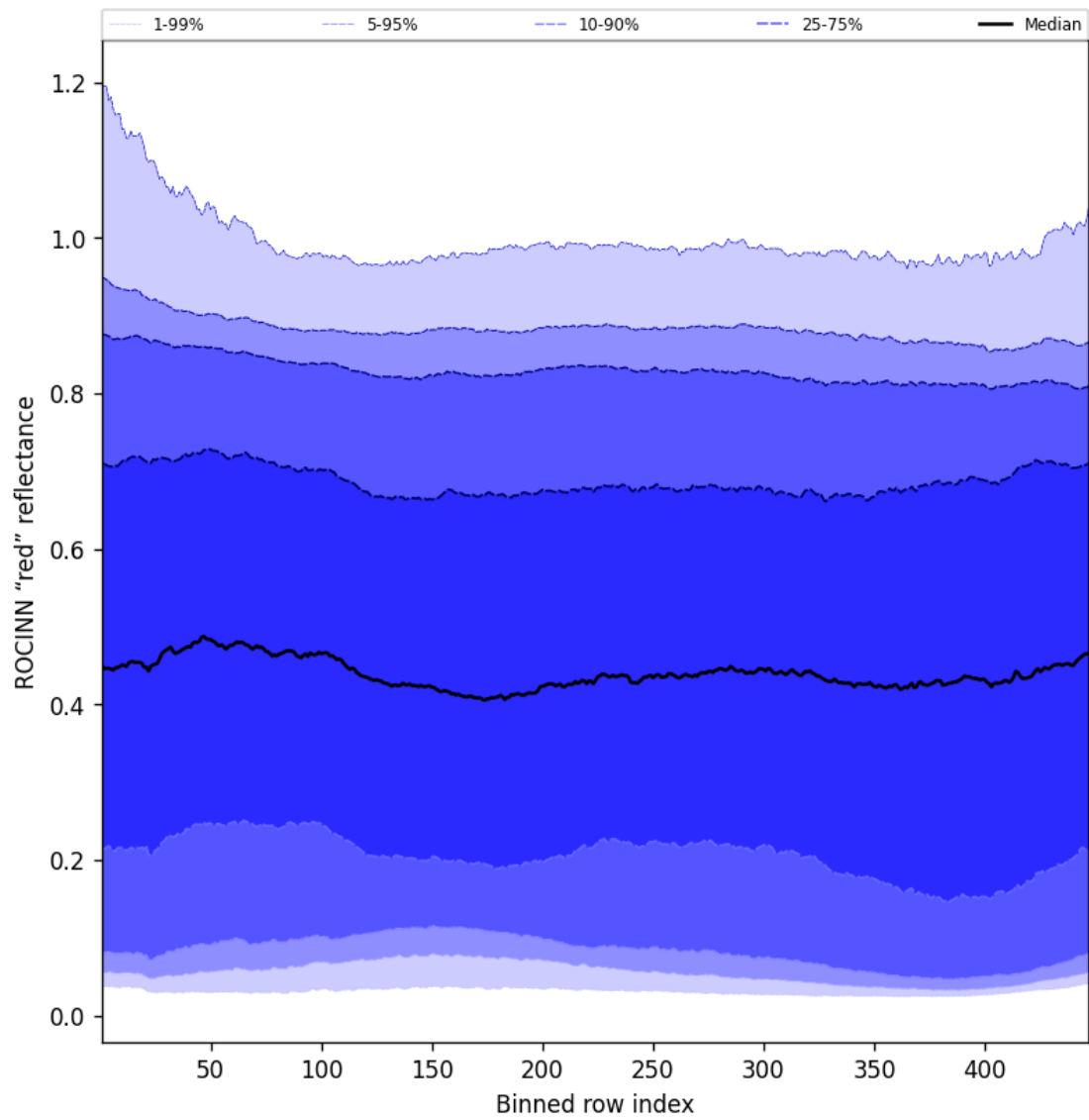
Figure 69: Along track statistics of “ROCINN “red” reflectance” for 2025-05-17 to 2025-05-19
