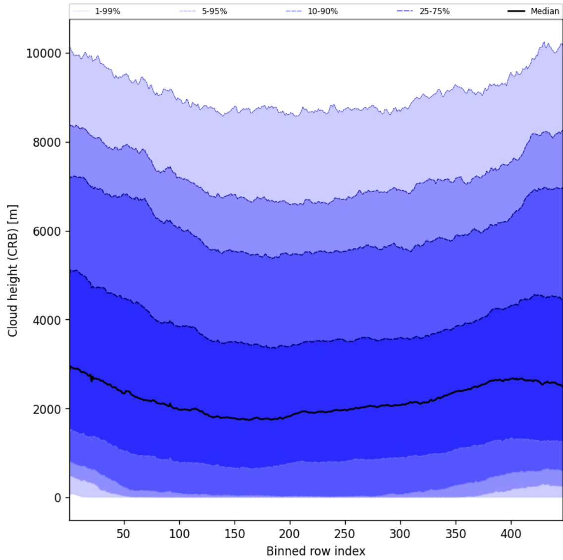
Figure 59: Along track statistics of “Cloud height (CRB)” for 2025-05-17 to 2025-05-19
