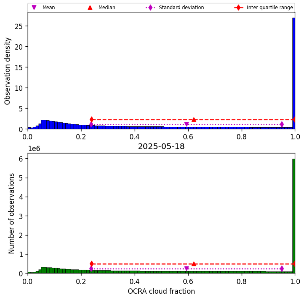
Figure 50: Histogram of “OCRA cloud fraction” for 2025-05-17 to 2025-05-19
