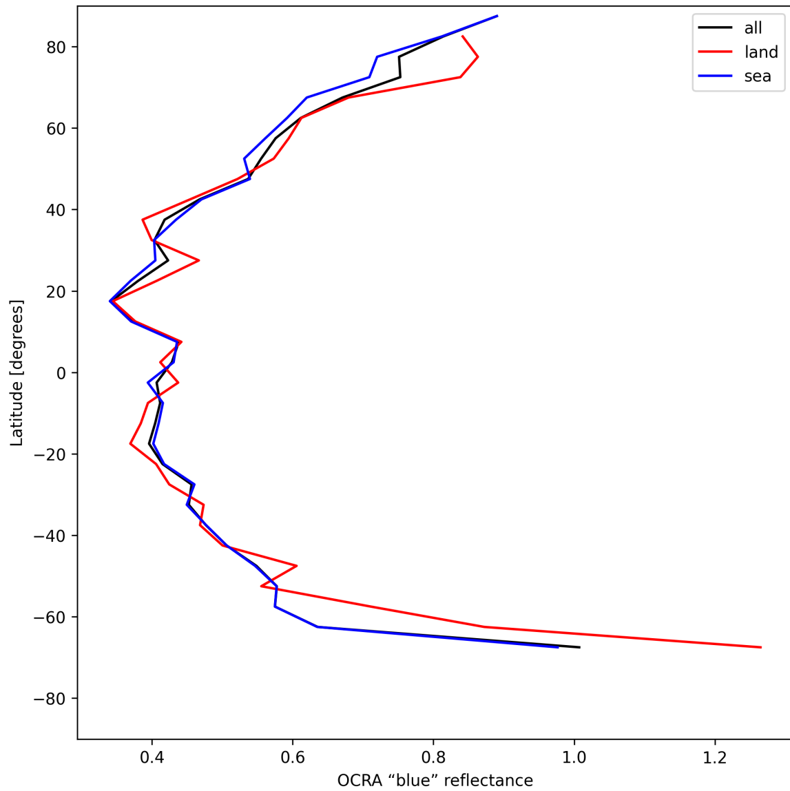
Figure 35: Zonal average of “OCRA “blue” reflectance” for 2025-05-17 to 2025-05-19.
