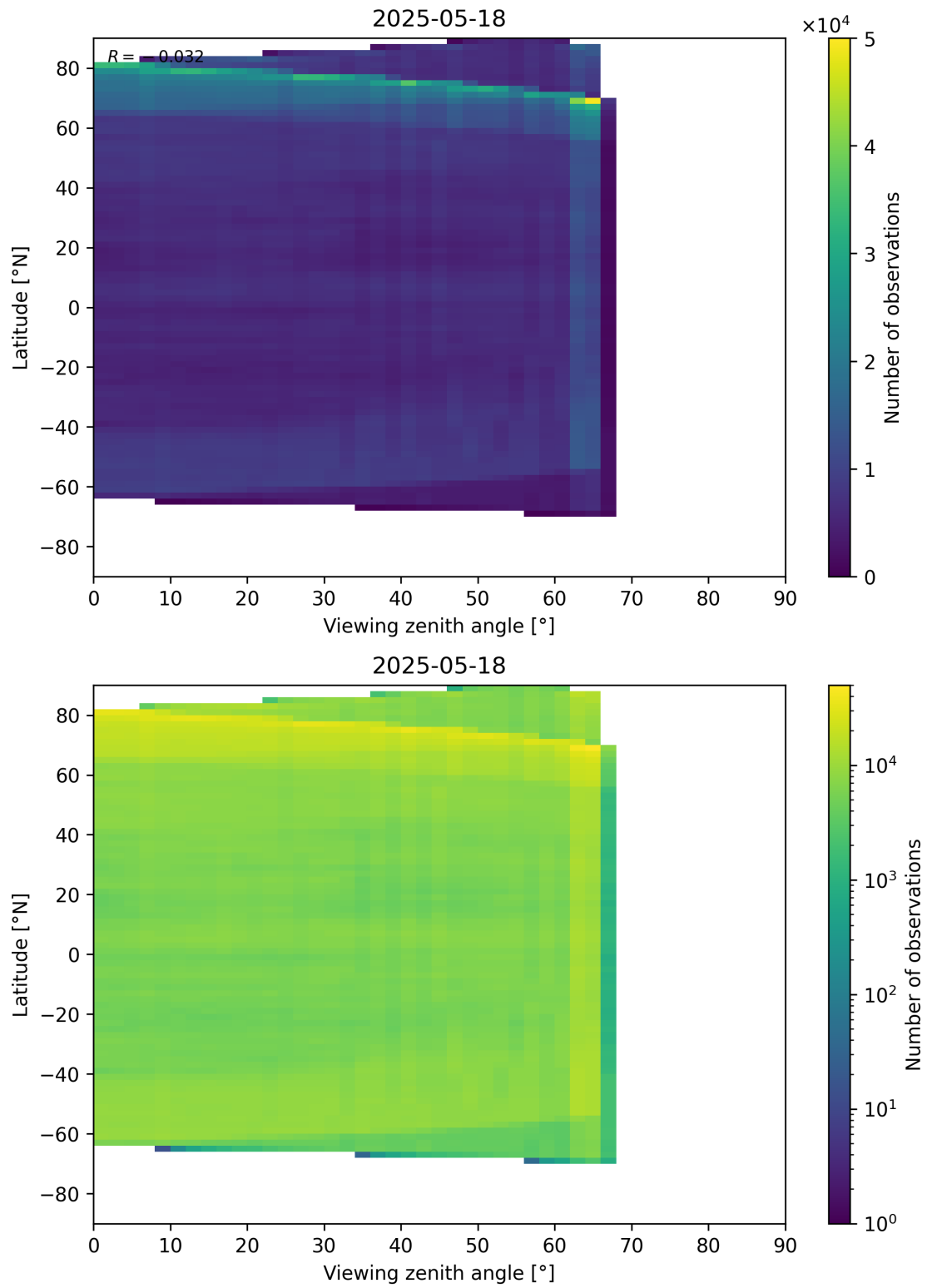
Figure 113: Scatter density plot of “Viewing zenith angle” against “Latitude” for 2025-05-17 to 2025-05-19.
