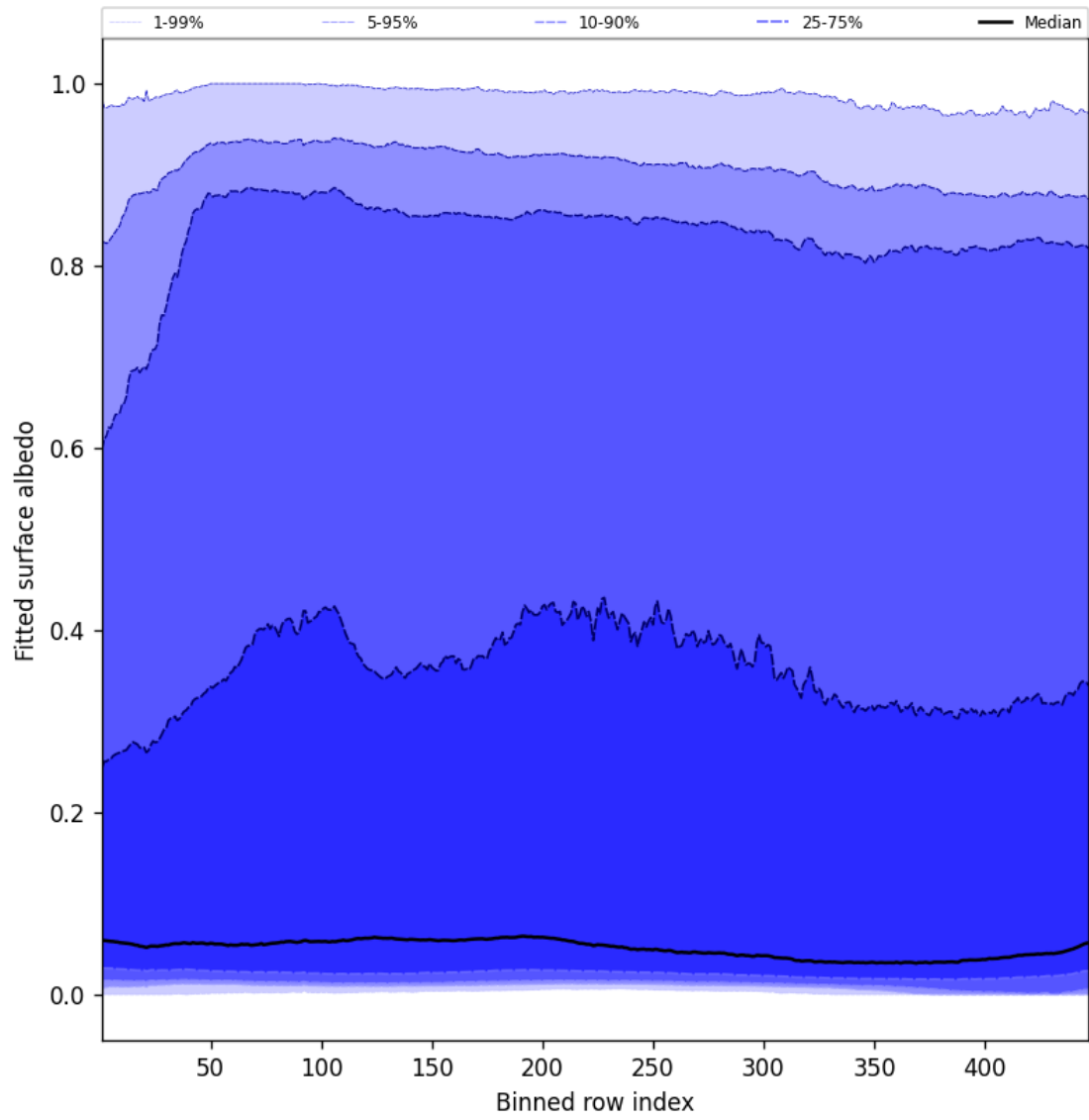
Figure 61: Along track statistics of “Fitted surface albedo” for 2025-05-17 to 2025-05-19
