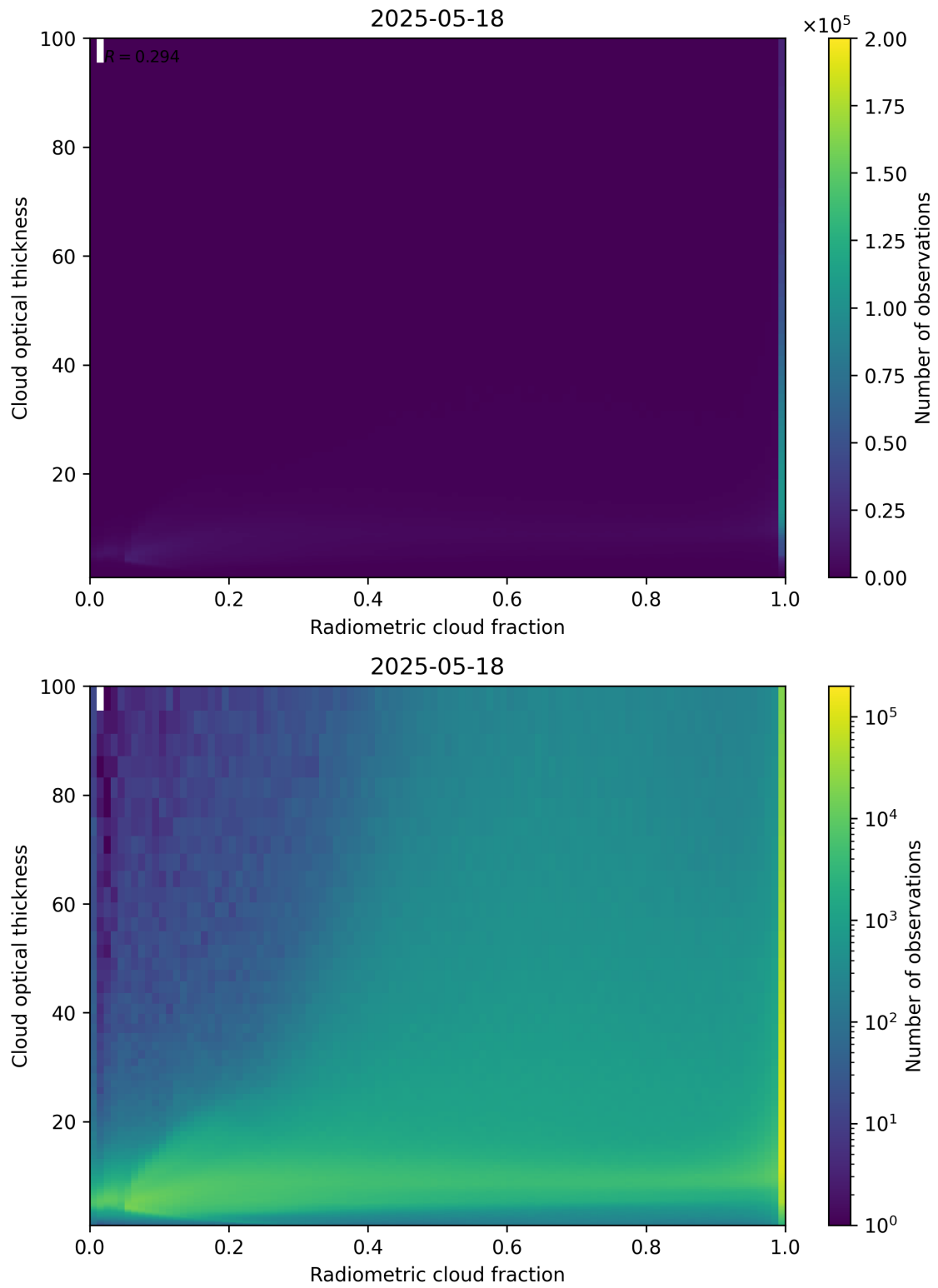
Figure 75: Scatter density plot of “Radiometric cloud fraction” against “Cloud optical thickness” for 2025-05-17 to 2025-05-19.
