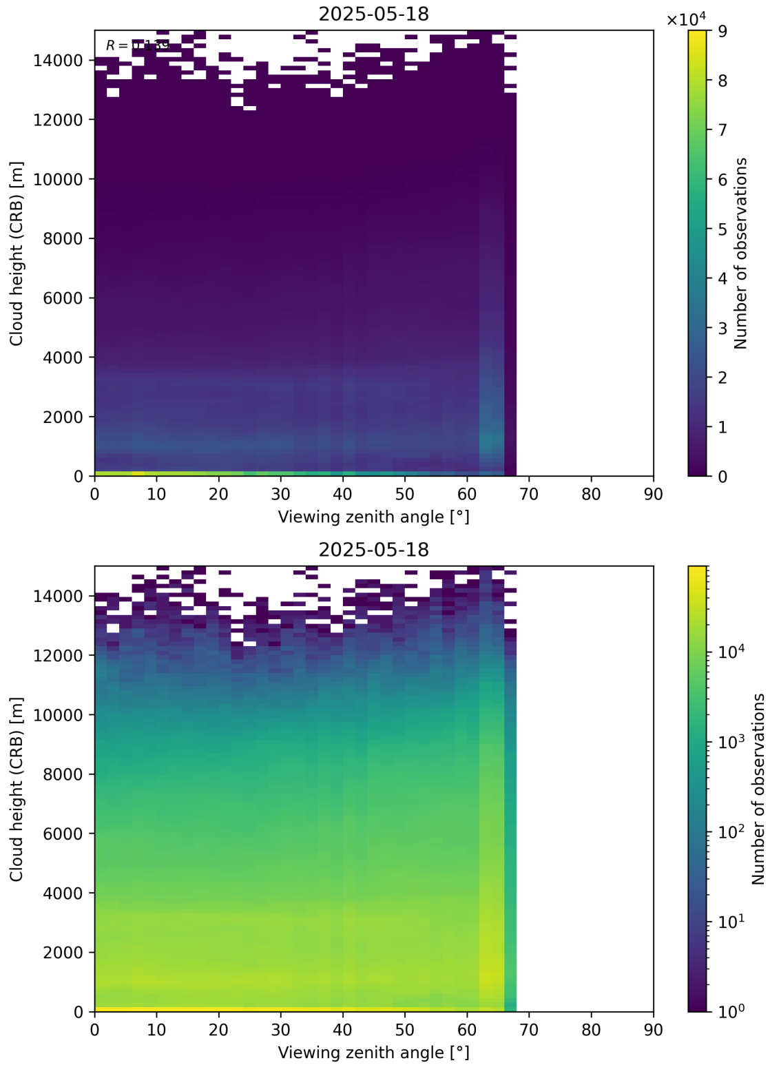
Figure 110: Scatter density plot of “Viewing zenith angle” against “Cloud height (CRB)” for 2025-05-17 to 2025-05-19.
