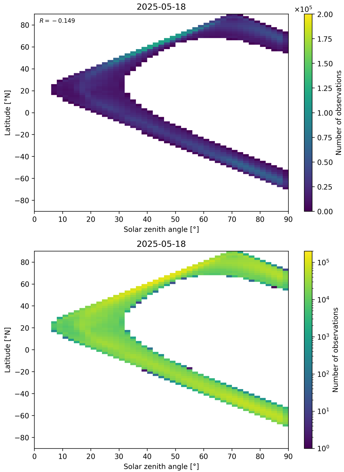
Figure 105: Scatter density plot of “Solar zenith angle” against “Latitude” for 2025-05-17 to 2025-05-19.
