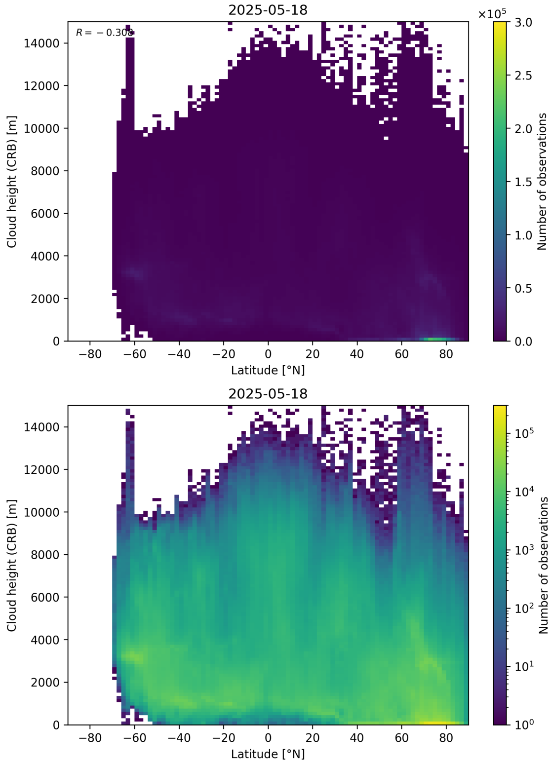
Figure 95: Scatter density plot of “Latitude” against “Cloud height (CRB)” for 2025-05-17 to 2025-05-19.
