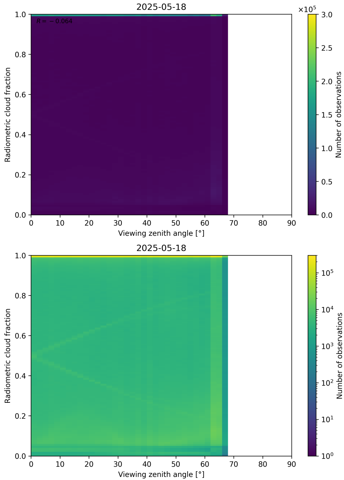
Figure 107: Scatter density plot of “Viewing zenith angle” against “Radiometric cloud fraction” for 2025-05-17 to 2025-05-19.
