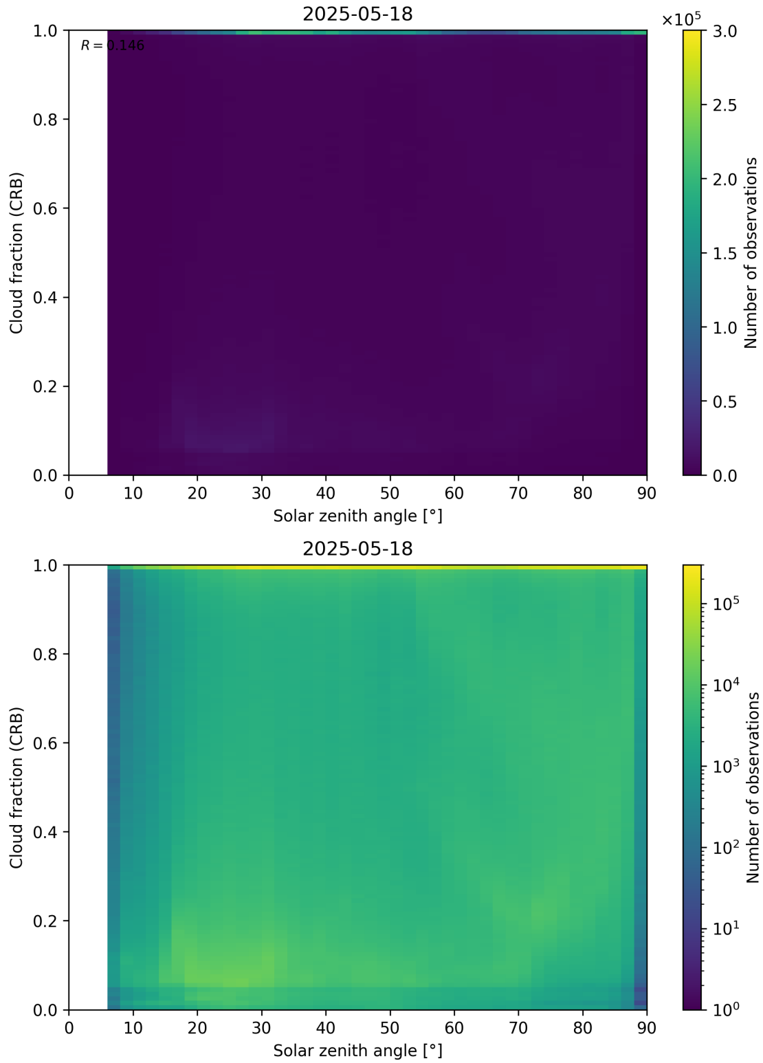
Figure 101: Scatter density plot of “Solar zenith angle” against “Cloud fraction (CRB)” for 2025-05-17 to 2025-05-19.
