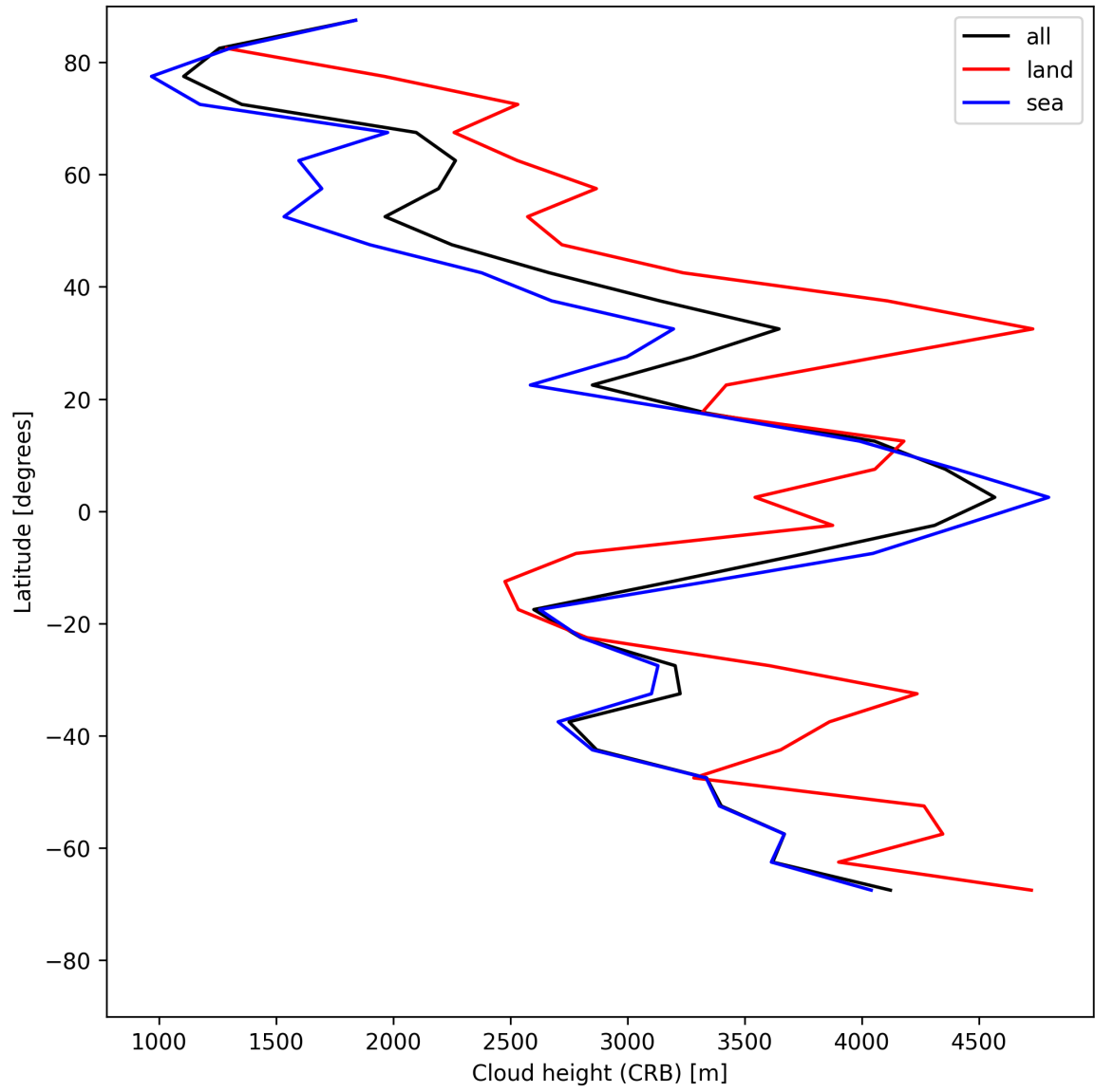
Figure 27: Zonal average of “Cloud height (CRB)” for 2025-05-17 to 2025-05-19.
