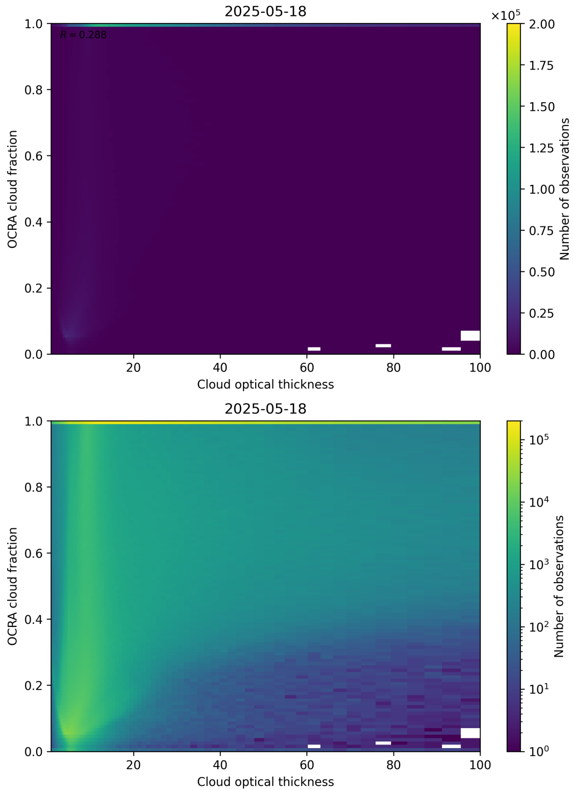
Figure 83: Scatter density plot of “Cloud optical thickness” against “OCRA cloud fraction” for 2025-05-17 to 2025-05-19.
