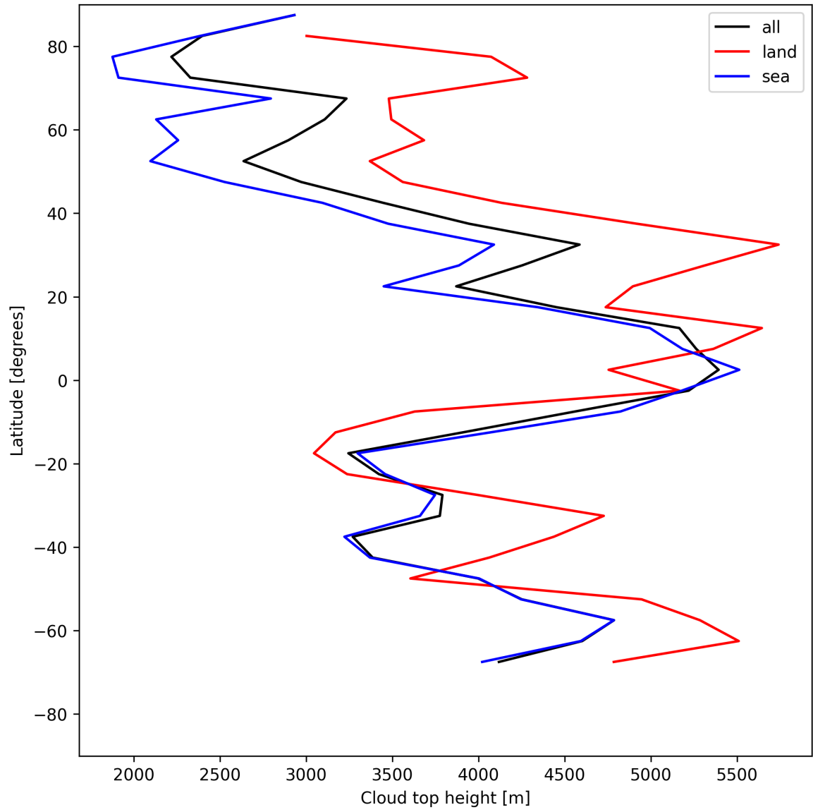
Figure 24: Zonal average of “Cloud top height” for 2025-05-17 to 2025-05-19.
