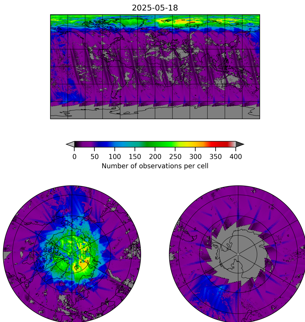
Figure 21: Map of the number of observations for 2025-05-17 to 2025-05-19
