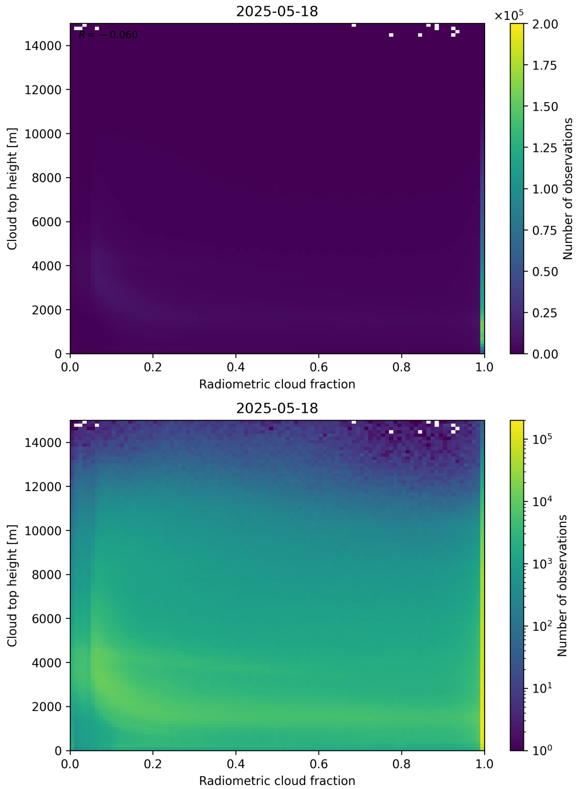
Figure 76: Scatter density plot of “Radiometric cloud fraction” against “Cloud top height” for 2025-05-17 to 2025-05-19.
