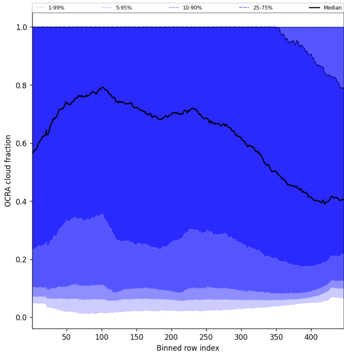
Figure 66: Along track statistics of “OCRA cloud fraction” for 2025-05-17 to 2025-05-19
