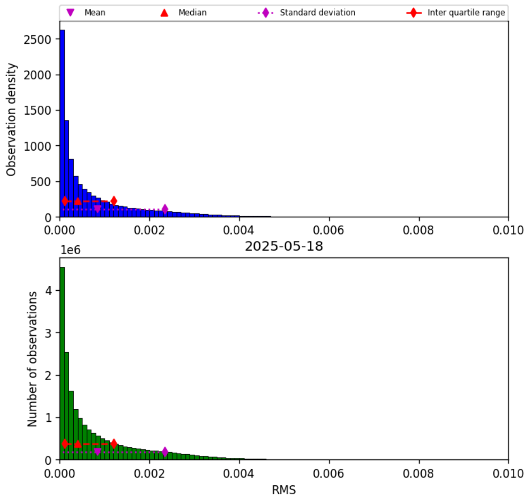
Figure 47: Histogram of “RMS” for 2025-05-17 to 2025-05-19
