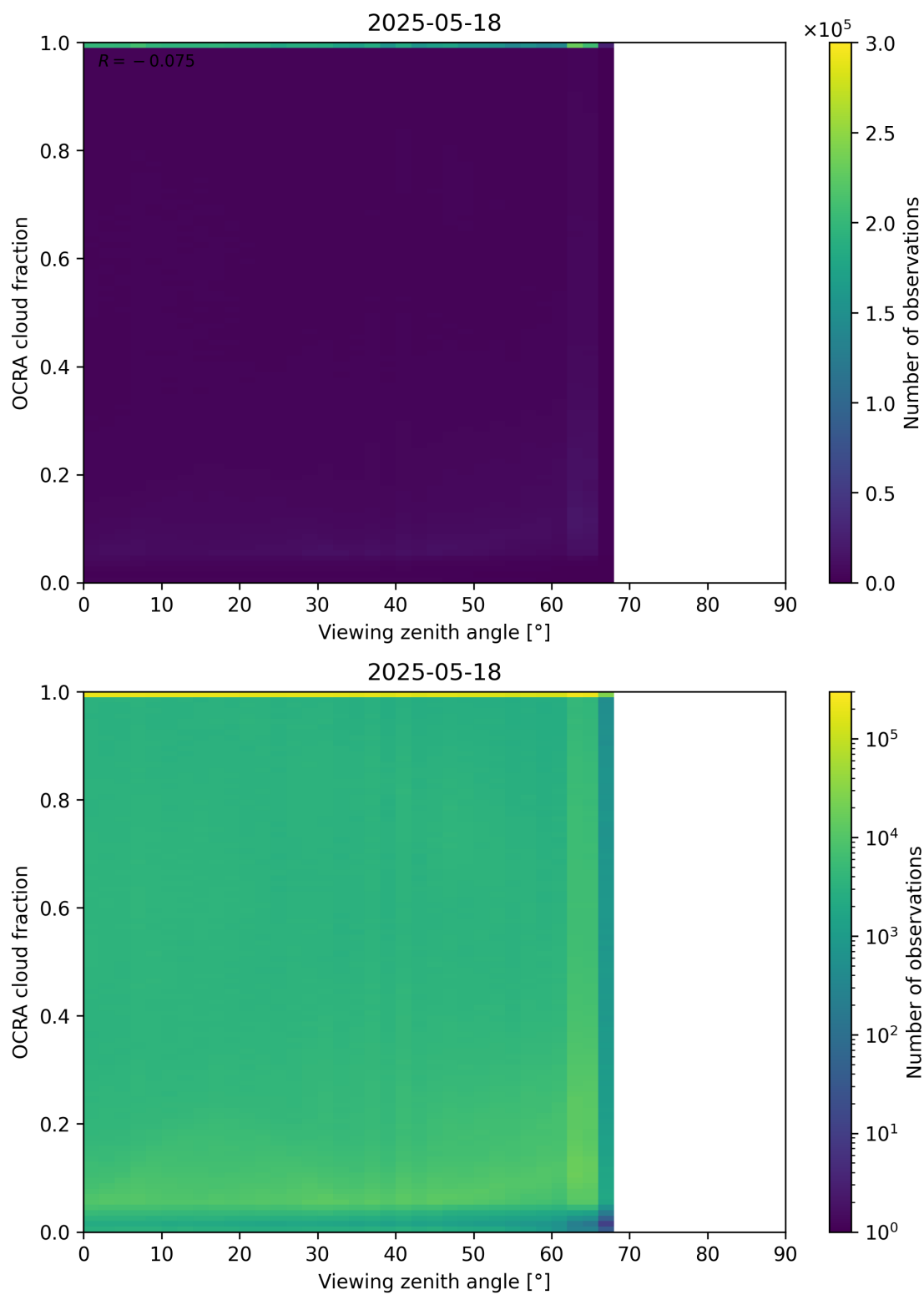
Figure 108: Scatter density plot of “Viewing zenith angle” against “OCRA cloud fraction” for 2025-05-17 to 2025-05-19.
