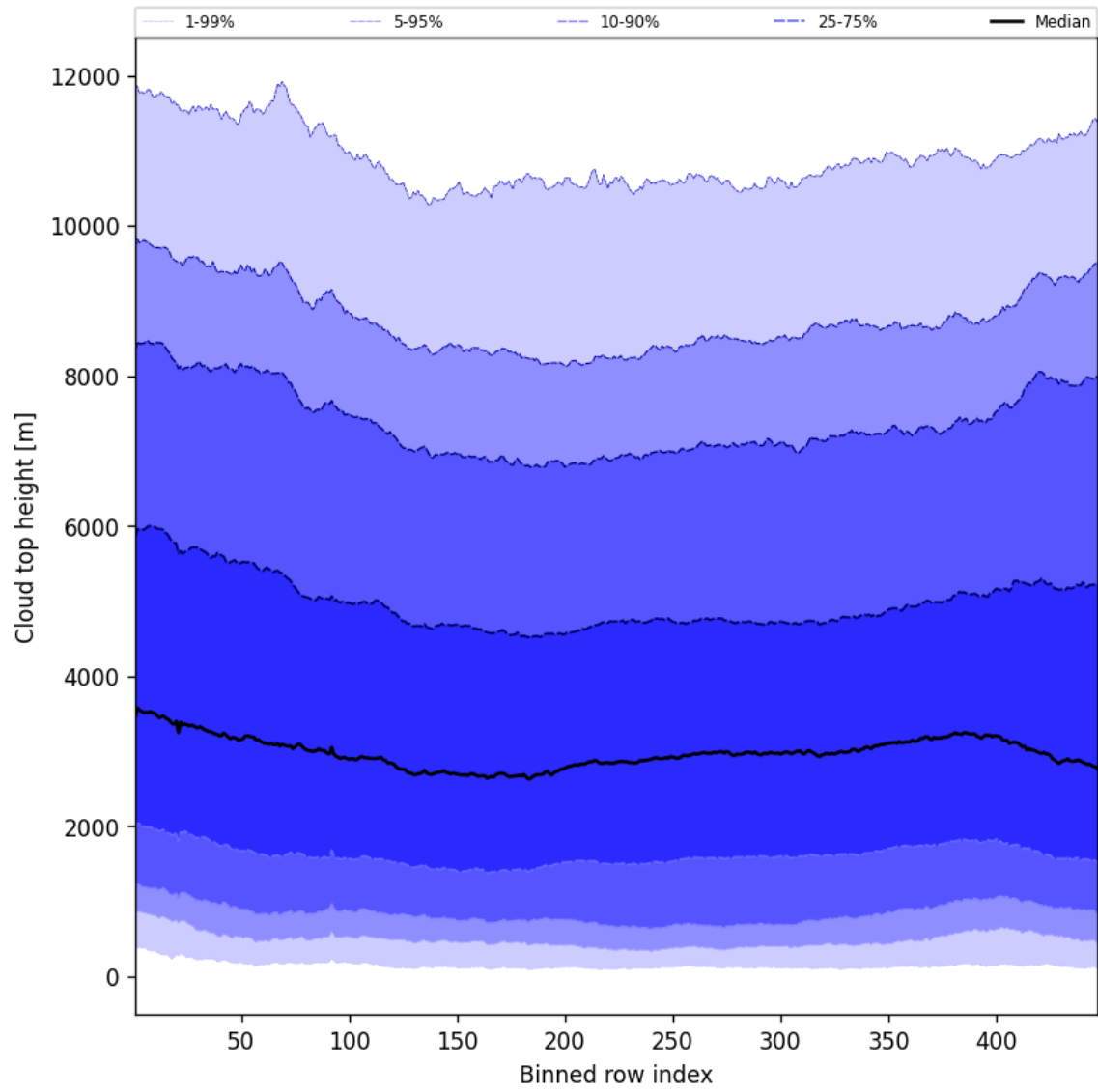
Figure 56: Along track statistics of “Cloud top height” for 2025-05-17 to 2025-05-19
