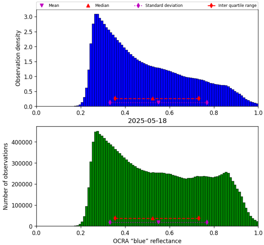
Figure 51: Histogram of “OCRA “blue” reflectance” for 2025-05-17 to 2025-05-19
