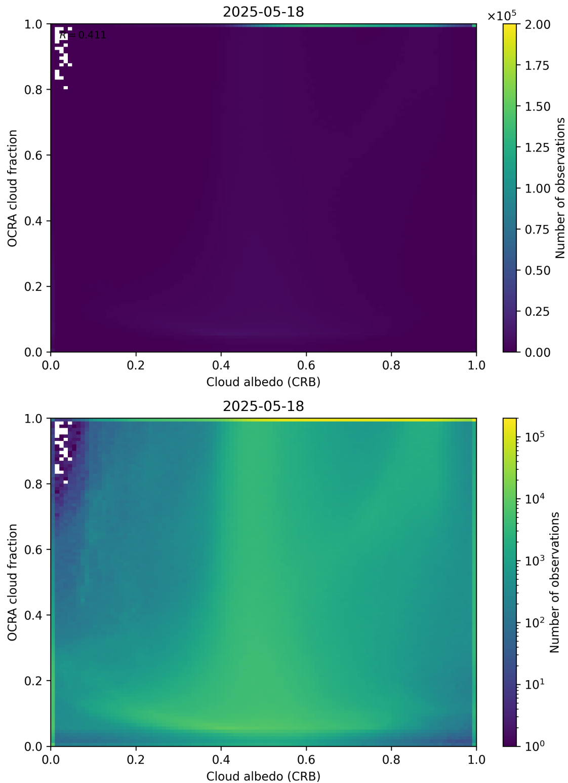
Figure 70: Scatter density plot of “Cloud albedo (CRB)” against “OCRA cloud fraction” for 2025-05-17 to 2025-05-19.
