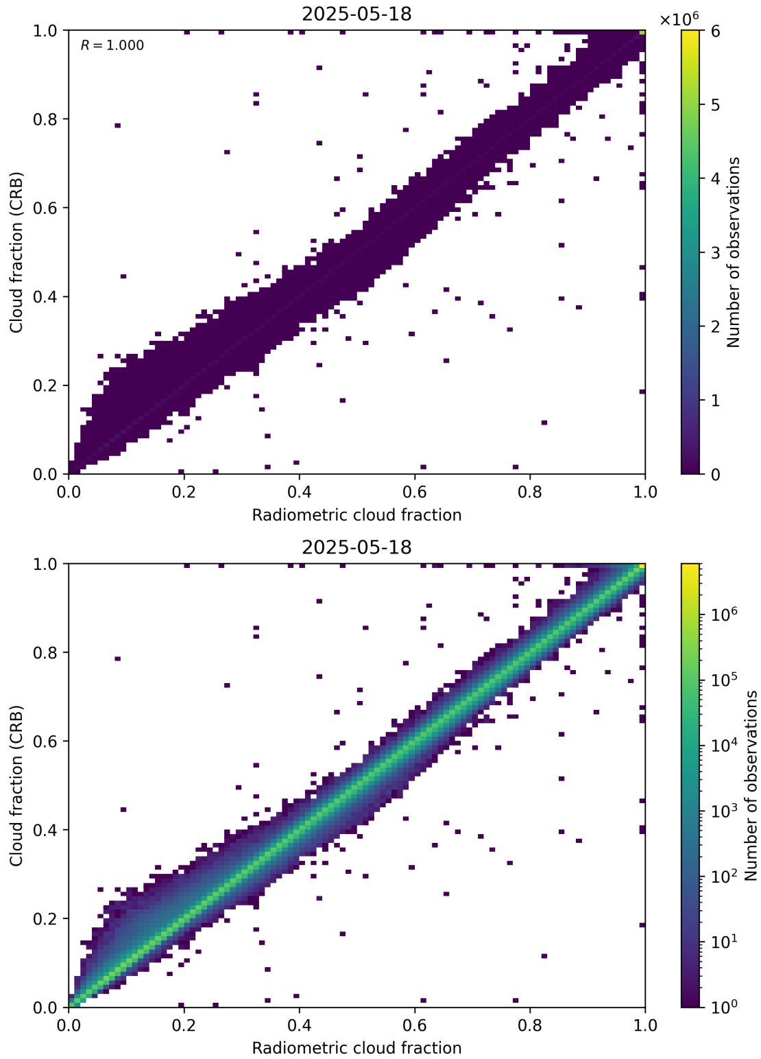
Figure 73: Scatter density plot of “Radiometric cloud fraction” against “Cloud fraction (CRB)” for 2025-05-17 to 2025-05-19.
