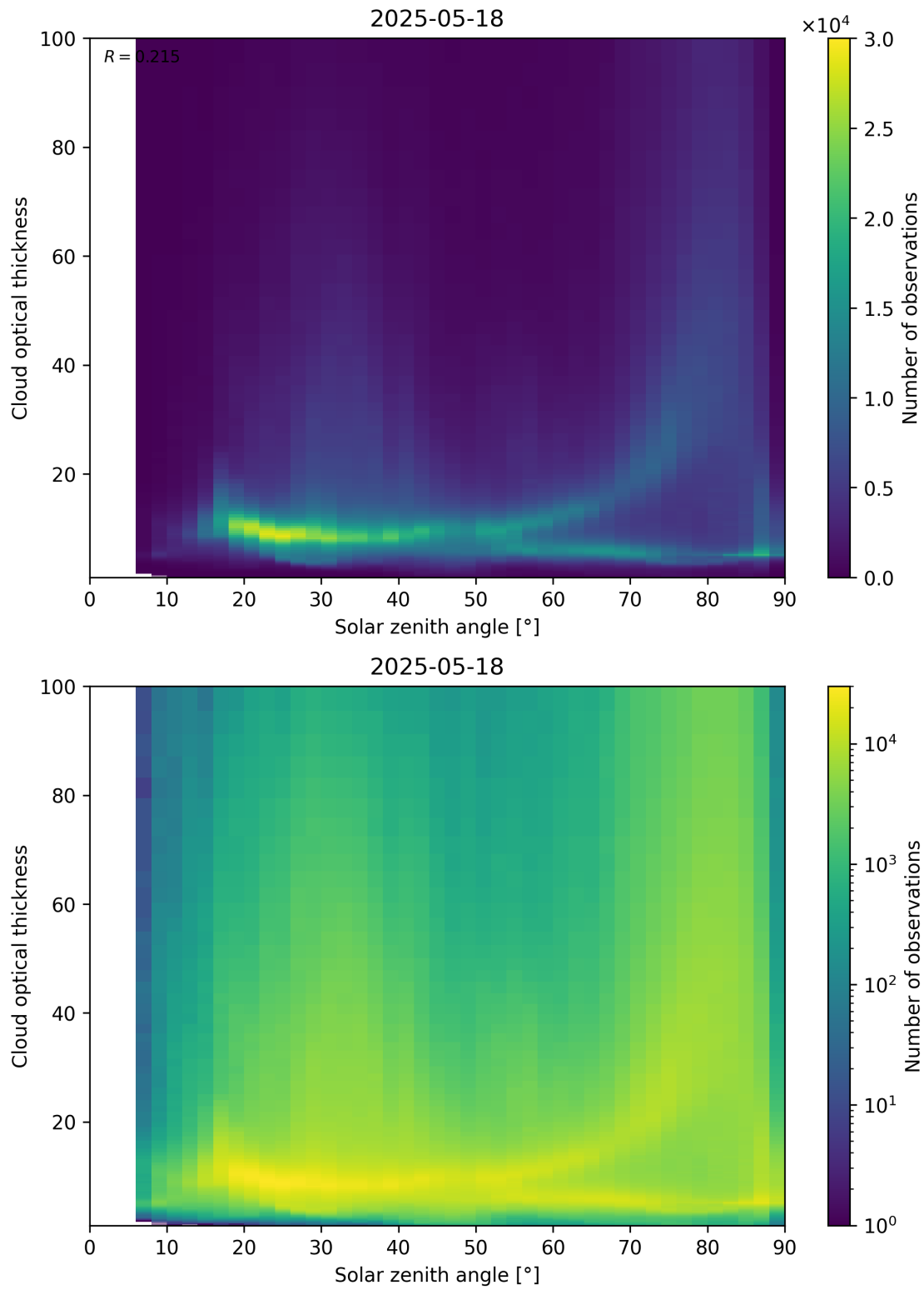
Figure 103: Scatter density plot of “Solar zenith angle” against “Cloud optical thickness” for 2025-05-17 to 2025-05-19.
