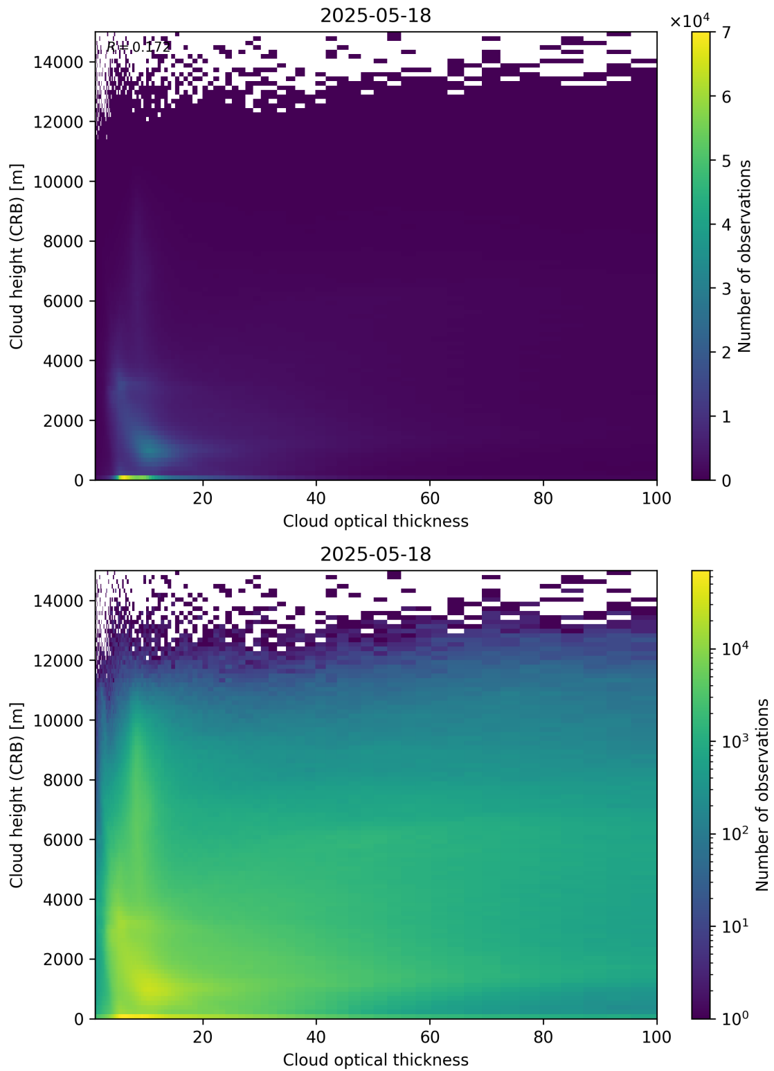
Figure 85: Scatter density plot of “Cloud optical thickness” against “Cloud height (CRB)” for 2025-05-17 to 2025-05-19.
