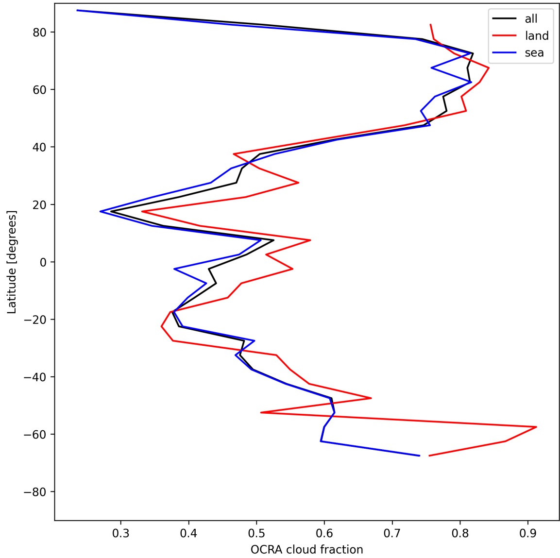
Figure 34: Zonal average of “OCRA cloud fraction” for 2025-05-17 to 2025-05-19.
