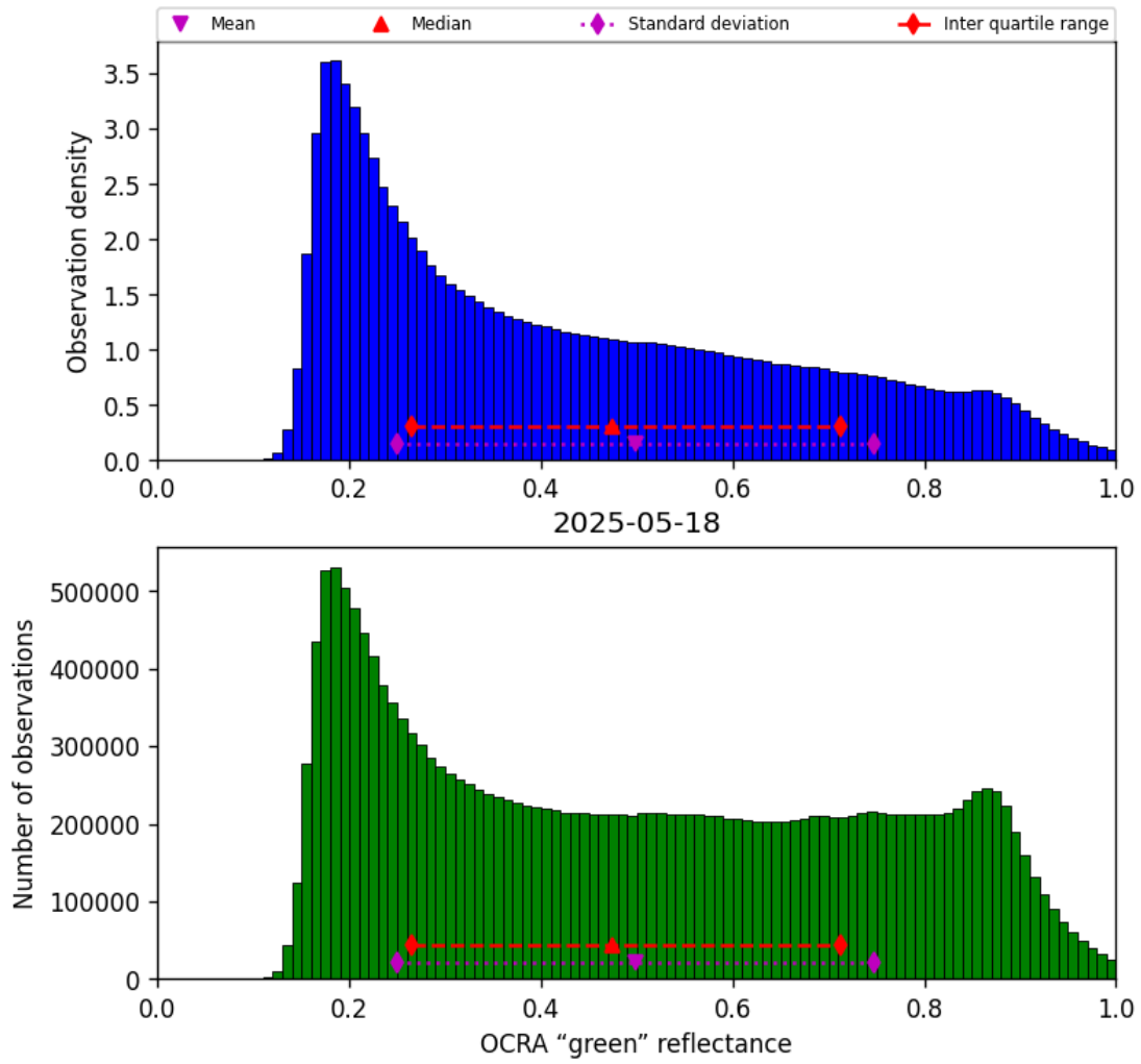
Figure 52: Histogram of “OCRA “green” reflectance” for 2025-05-17 to 2025-05-19
