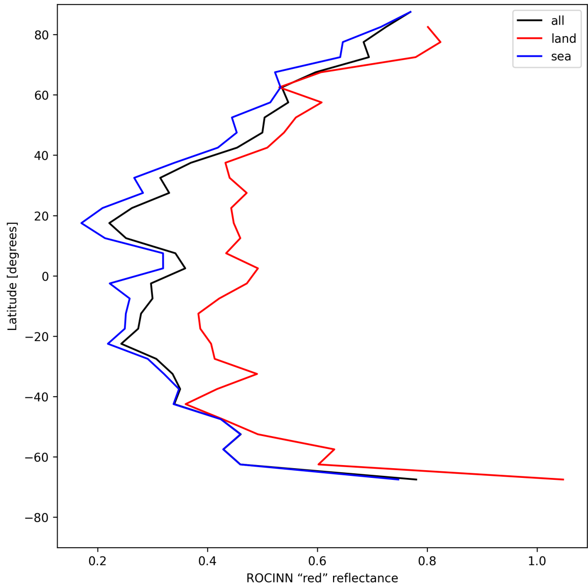
Figure 37: Zonal average of "ROCINN "red" reflectance" for 2025-05-18 to 2025-05-20.
