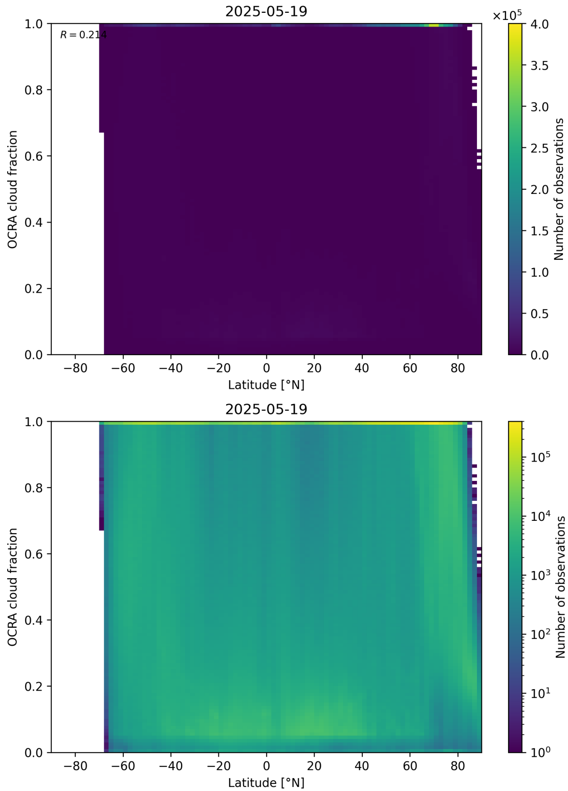
Figure 93: Scatter density plot of “Latitude” against “OCRA cloud fraction” for 2025-05-18 to 2025-05-20.
