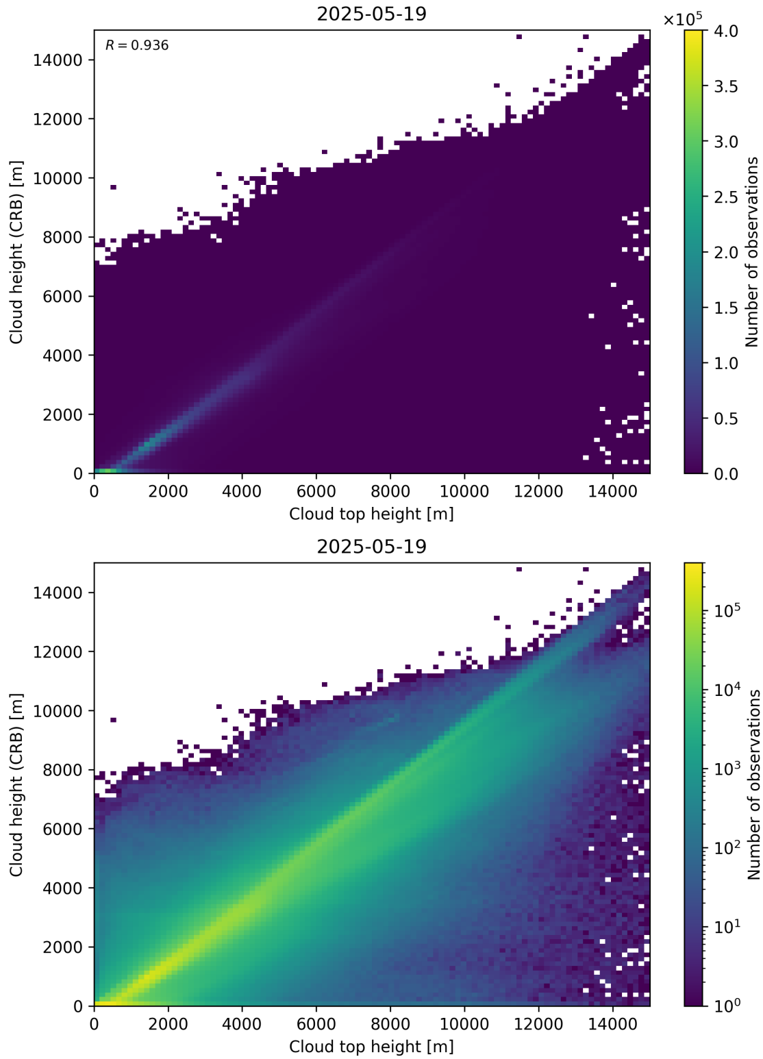
Figure 89: Scatter density plot of “Cloud top height” against “Cloud height (CRB)” for 2025-05-18 to 2025-05-20.
