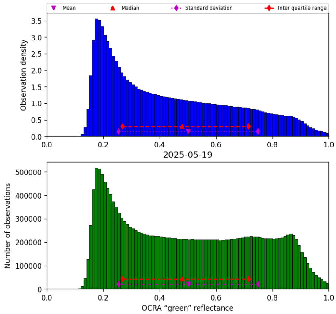
Figure 52: Histogram of “OCRA “green” reflectance” for 2025-05-18 to 2025-05-20
