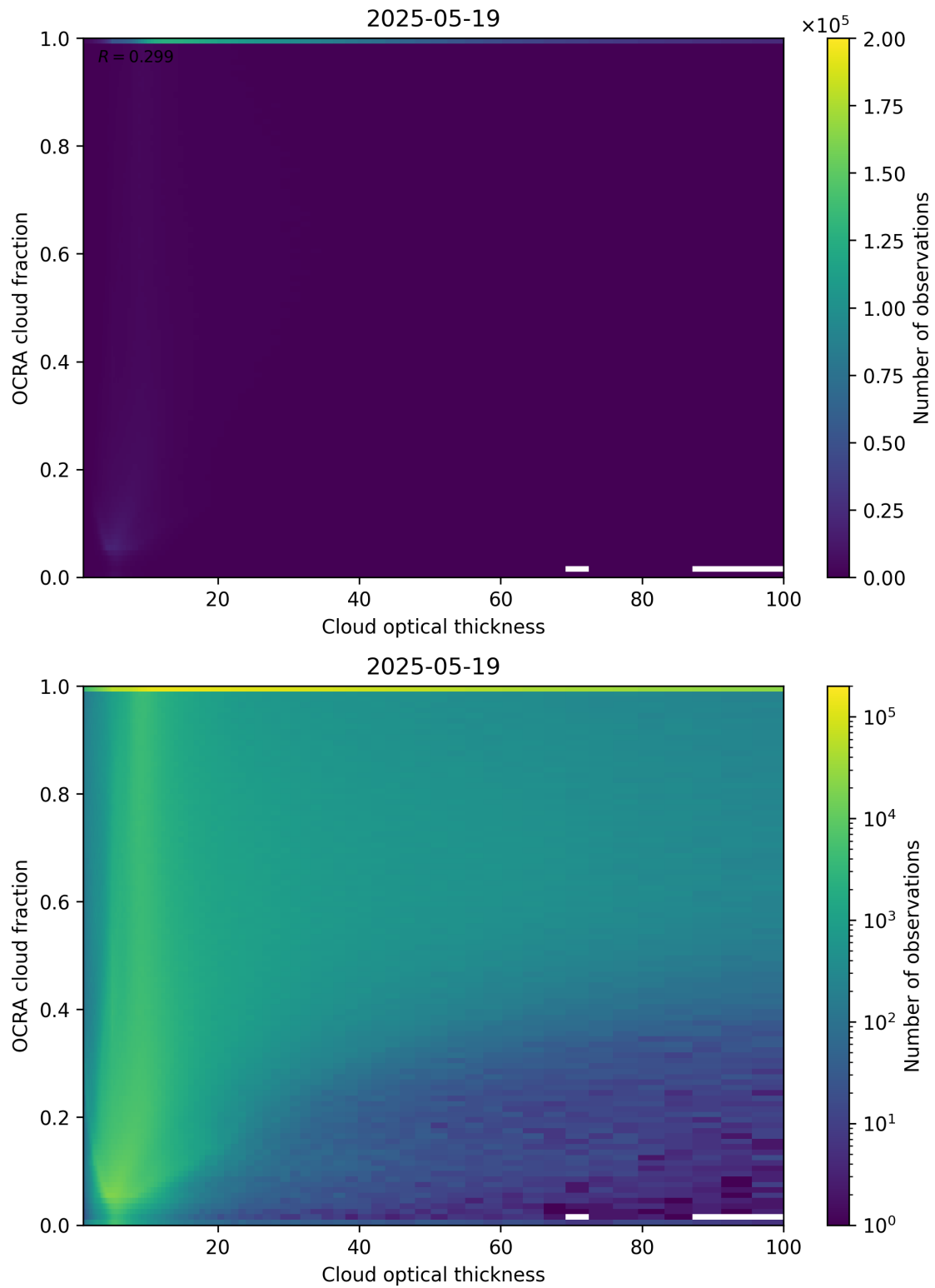
Figure 83: Scatter density plot of “Cloud optical thickness” against “OCRA cloud fraction” for 2025-05-18 to 2025-05-20.
