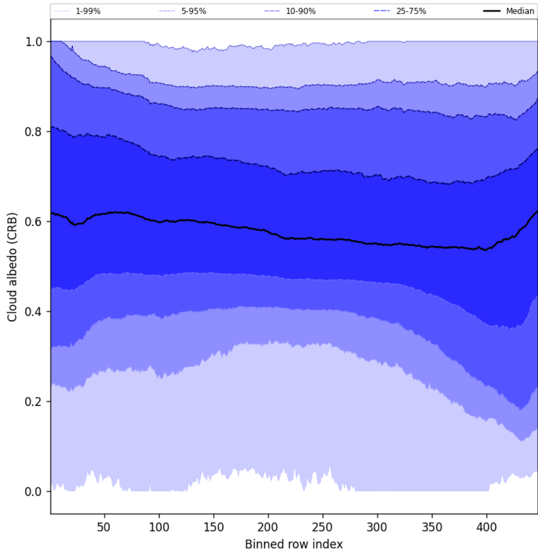
Figure 60: Along track statistics of “Cloud albedo (CRB)” for 2025-05-18 to 2025-05-20
