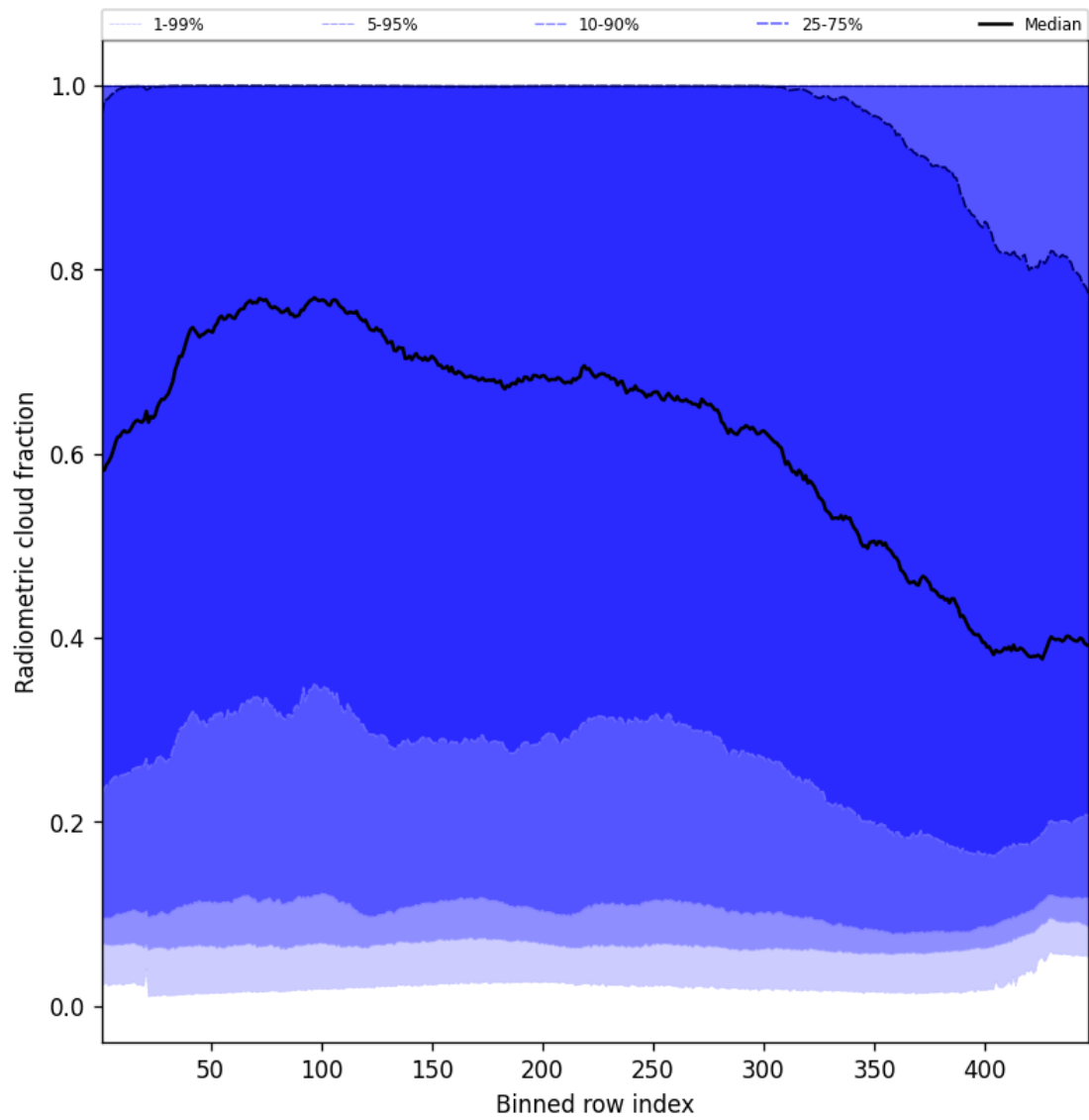
Figure 55: Along track statistics of “Radiometric cloud fraction” for 2025-05-18 to 2025-05-20
