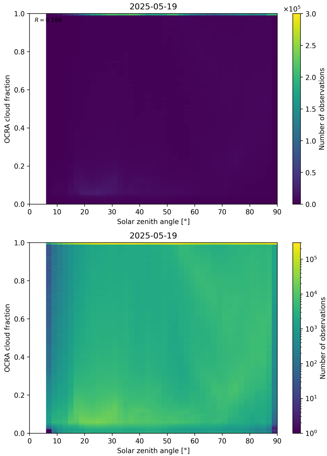
Figure 100: Scatter density plot of “Solar zenith angle” against “OCRA cloud fraction” for 2025-05-18 to 2025-05-20.
