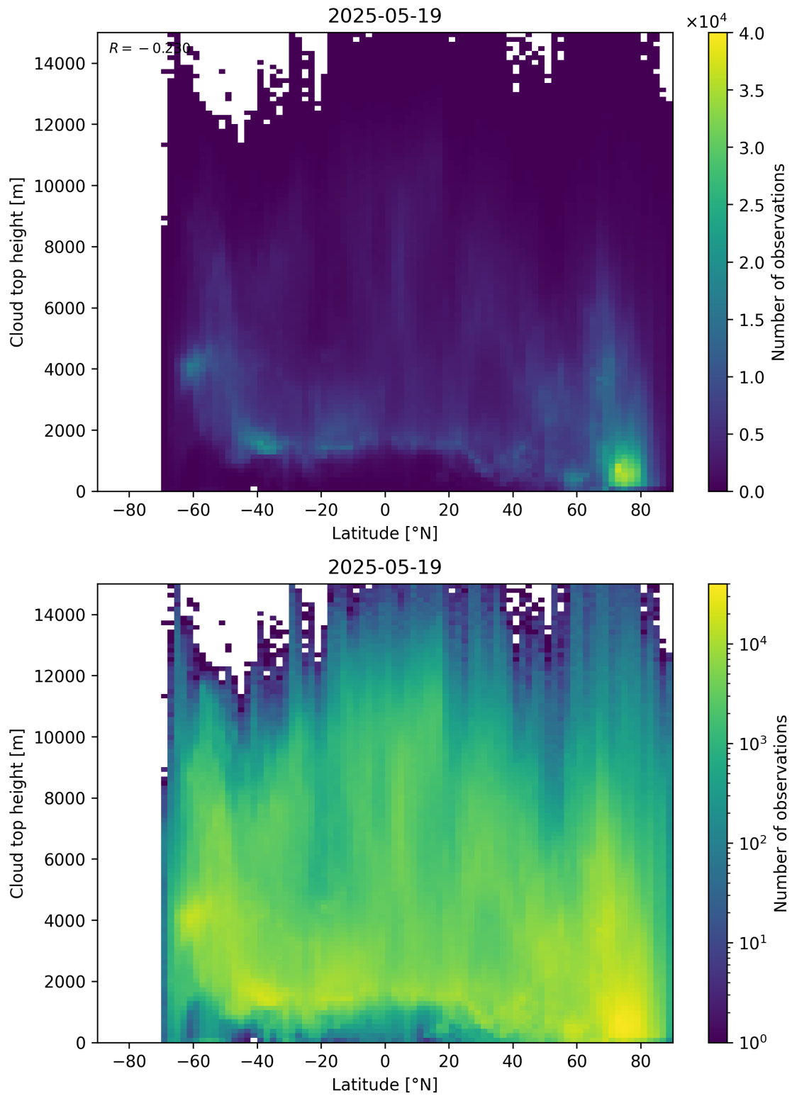
Figure 97: Scatter density plot of “Latitude” against “Cloud top height” for 2025-05-18 to 2025-05-20.
