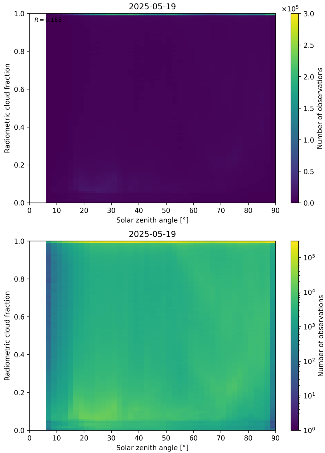
Figure 99: Scatter density plot of “Solar zenith angle” against “Radiometric cloud fraction” for 2025-05-18 to 2025-05-20.
