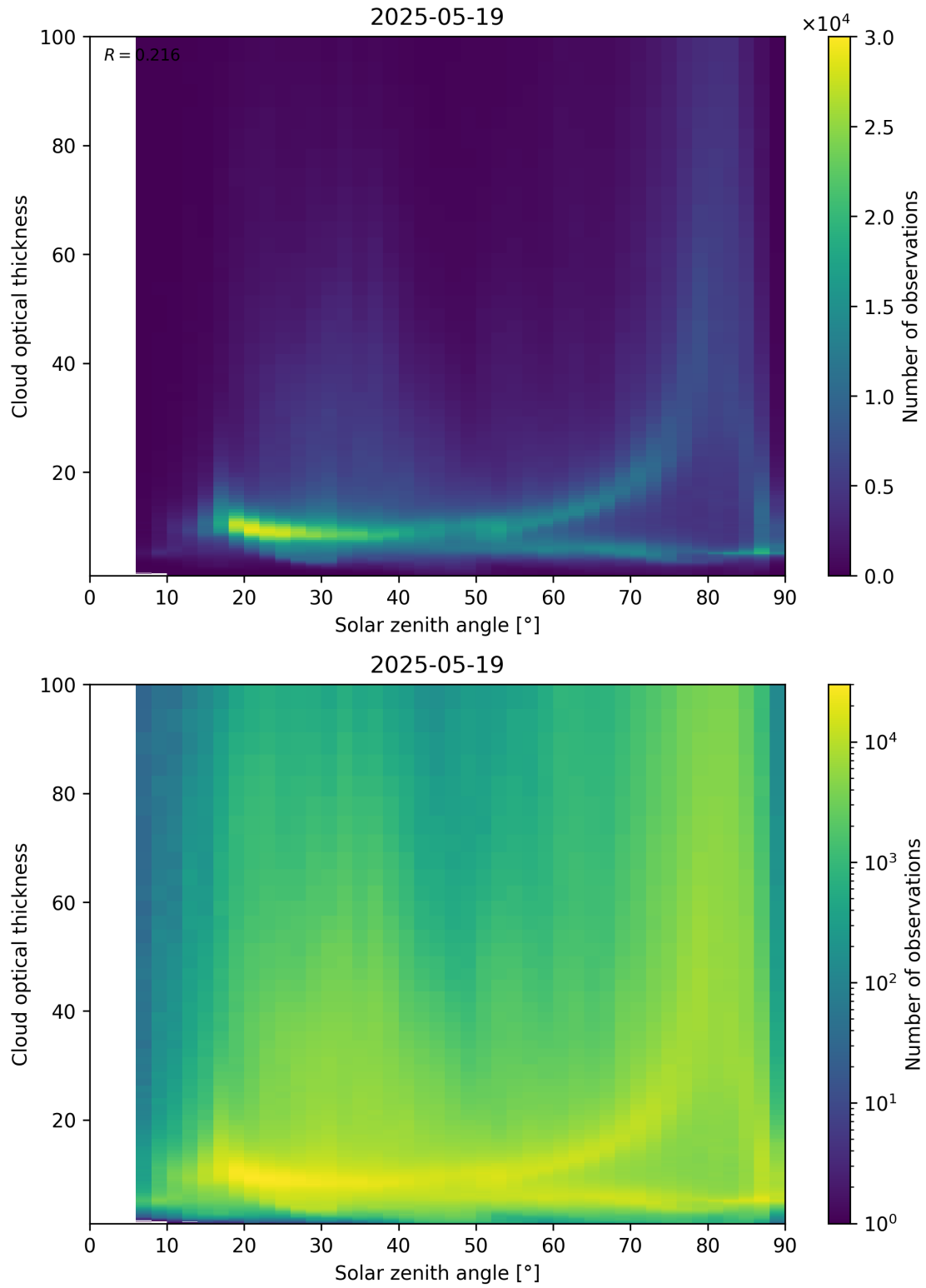
Figure 103: Scatter density plot of “Solar zenith angle” against “Cloud optical thickness” for 2025-05-18 to 2025-05-20.
