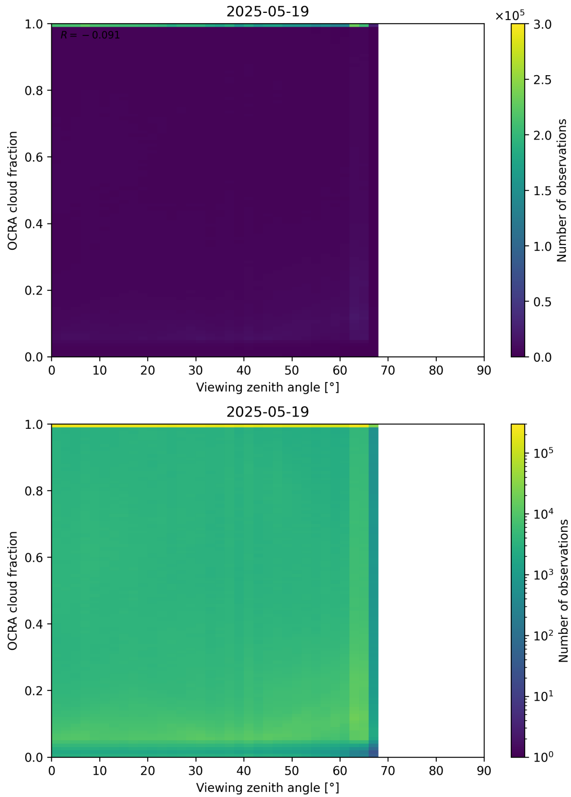
Figure 108: Scatter density plot of “Viewing zenith angle” against “OCRA cloud fraction” for 2025-05-18 to 2025-05-20.
