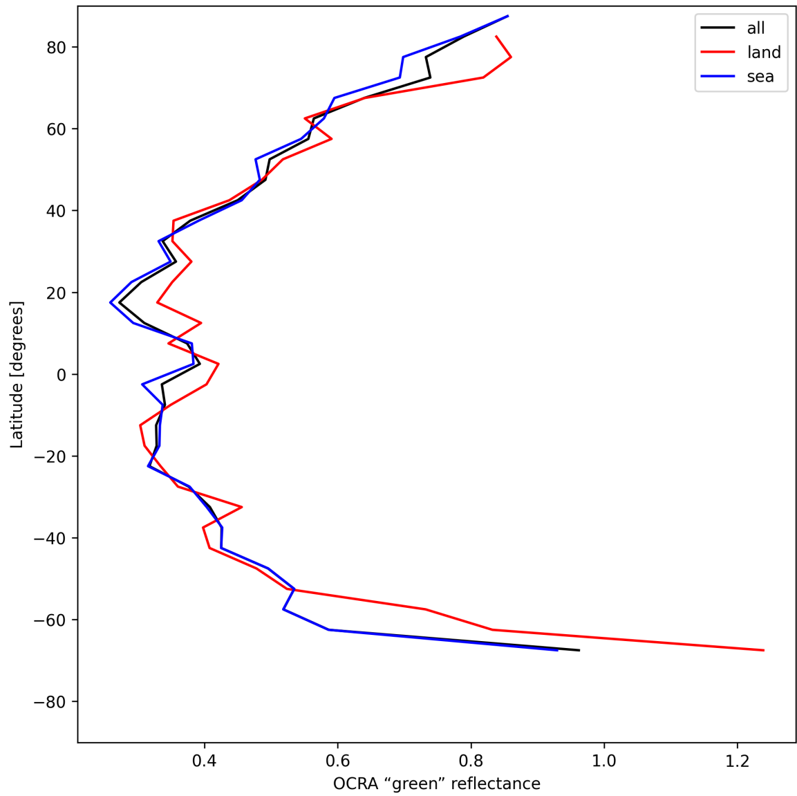
Figure 36: Zonal average of “OCRA “green” reflectance” for 2025-05-18 to 2025-05-20.
