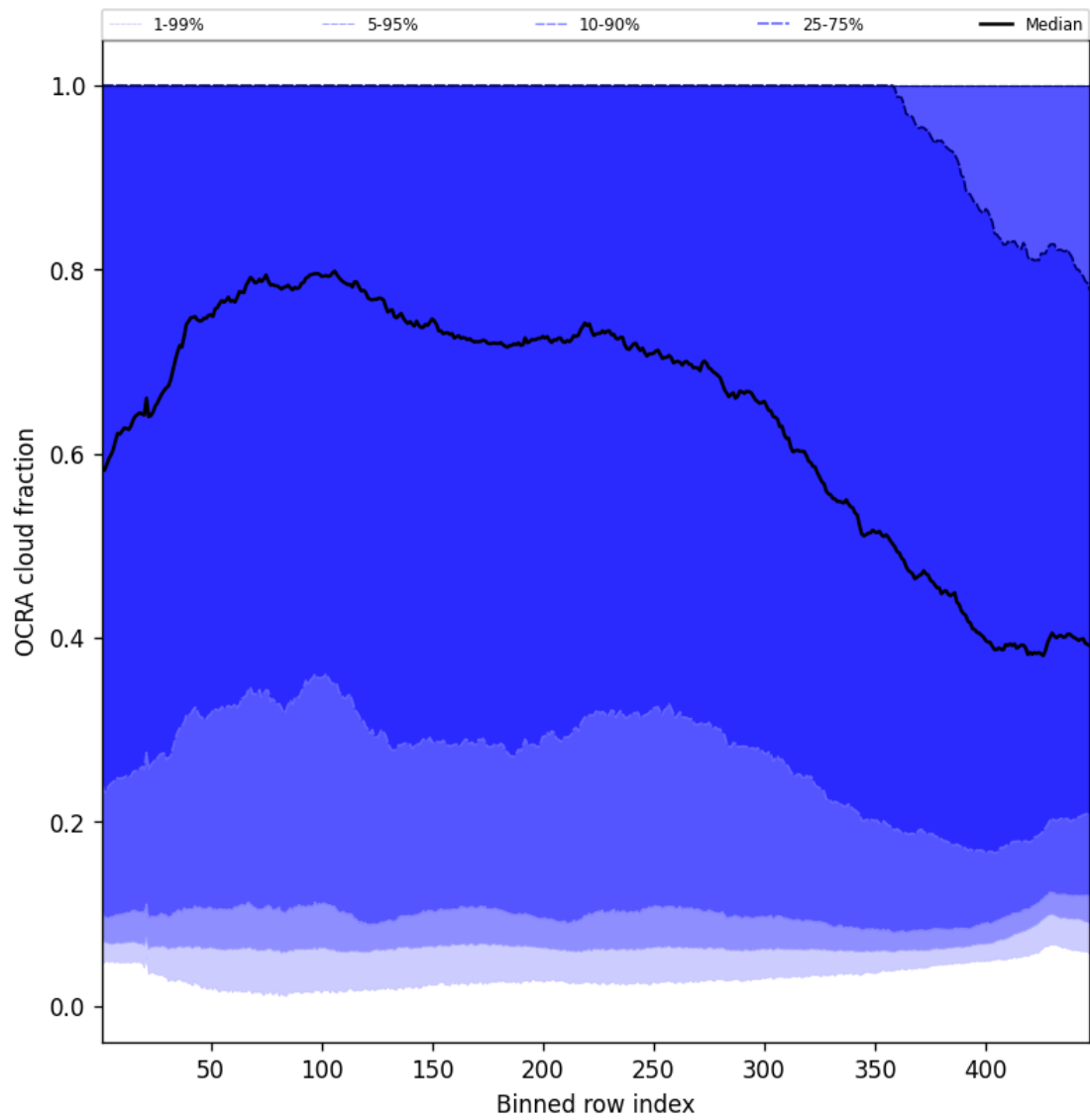
Figure 66: Along track statistics of “OCRA cloud fraction” for 2025-05-18 to 2025-05-20
