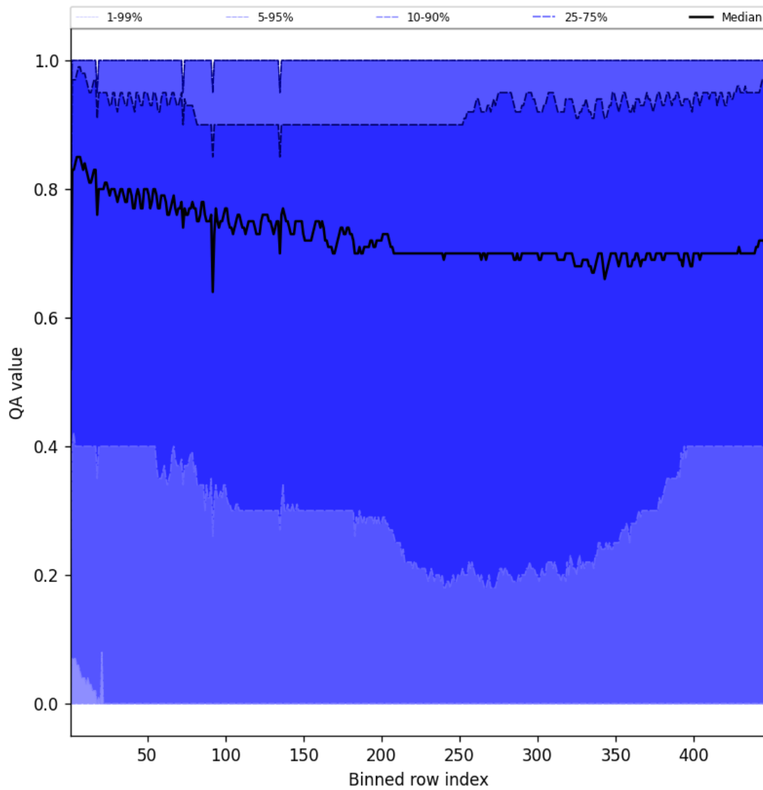
Figure 54: Along track statistics of “QA value” for 2025-05-18 to 2025-05-20
