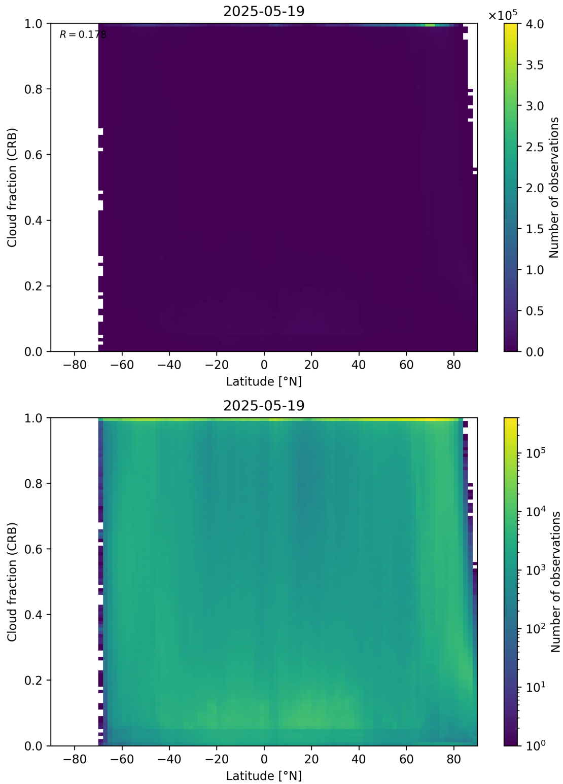
Figure 94: Scatter density plot of “Latitude” against “Cloud fraction (CRB)” for 2025-05-18 to 2025-05-20.
