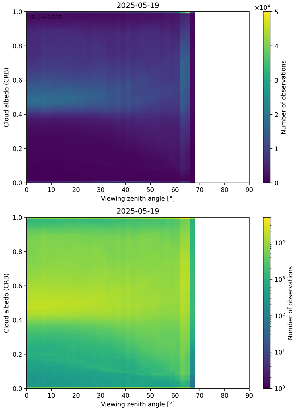
Figure 106: Scatter density plot of “Viewing zenith angle” against “Cloud albedo (CRB)” for 2025-05-18 to 2025-05-20.
