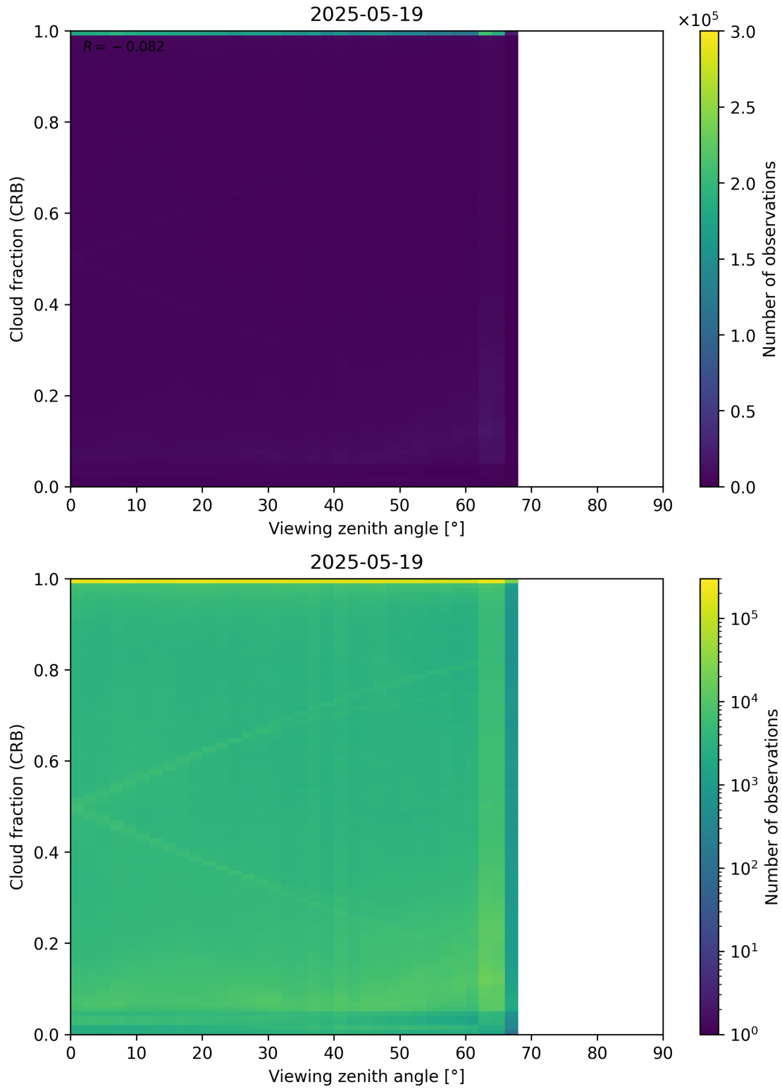
Figure 109: Scatter density plot of “Viewing zenith angle” against “Cloud fraction (CRB)” for 2025-05-18 to 2025-05-20.
