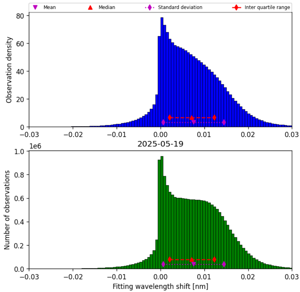
Figure 49: Histogram of “Fitting wavelength shift” for 2025-05-18 to 2025-05-20
