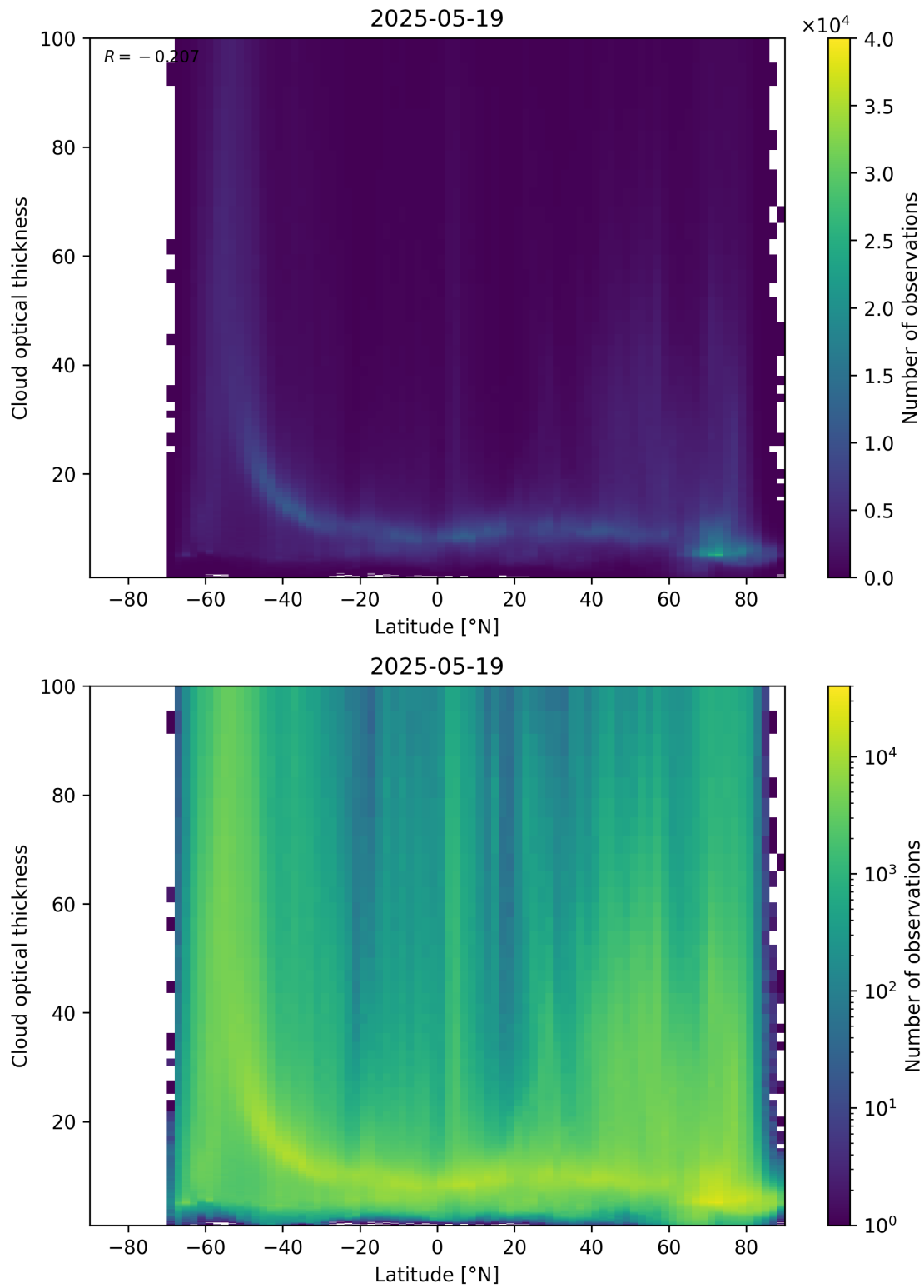
Figure 96: Scatter density plot of “Latitude” against “Cloud optical thickness” for 2025-05-18 to 2025-05-20.
