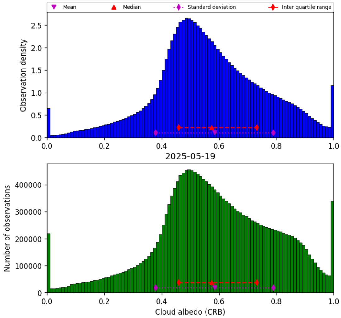
Figure 44: Histogram of “Cloud albedo (CRB)” for 2025-05-18 to 2025-05-20
