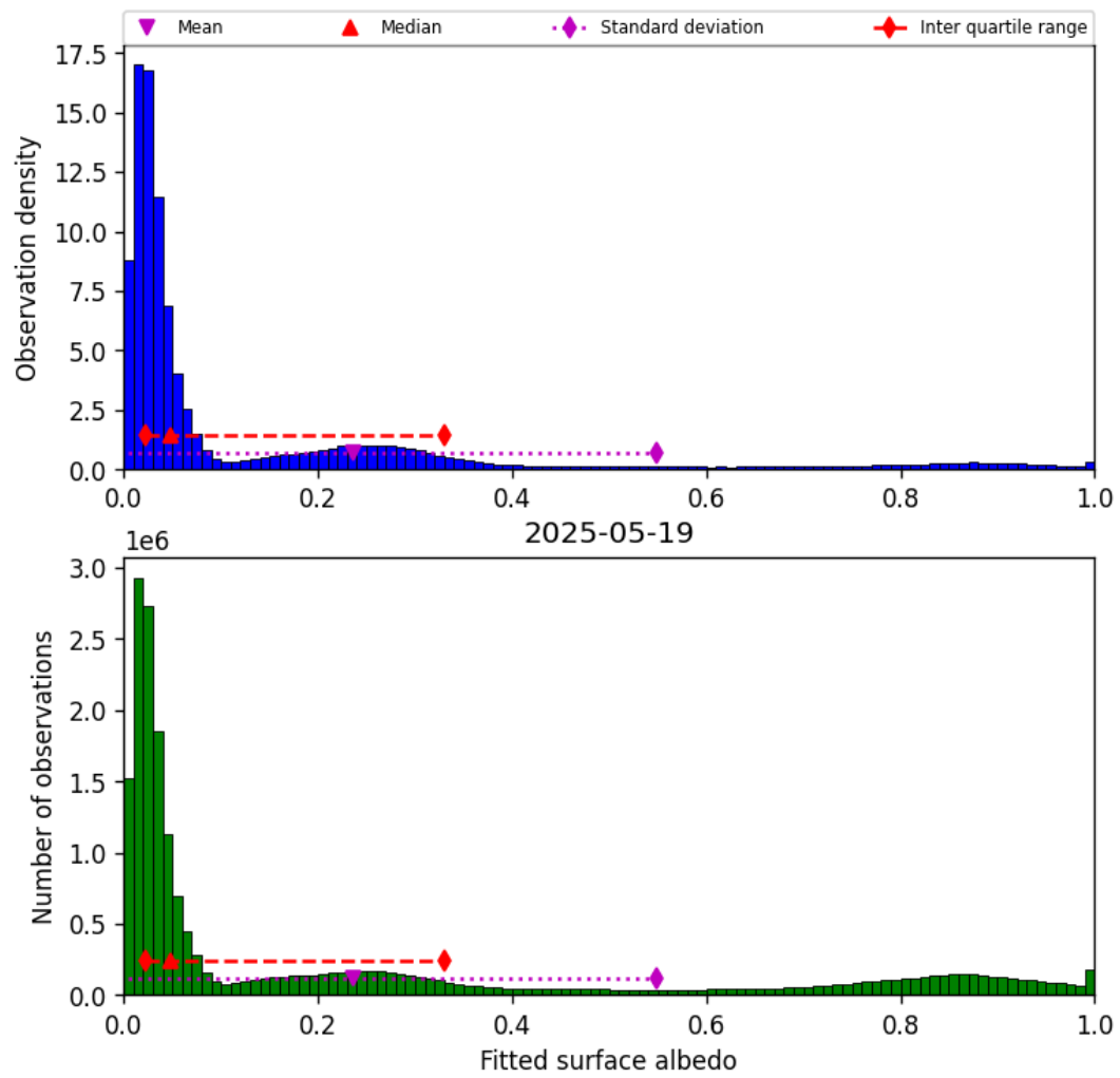
Figure 45: Histogram of “Fitted surface albedo” for 2025-05-18 to 2025-05-20
