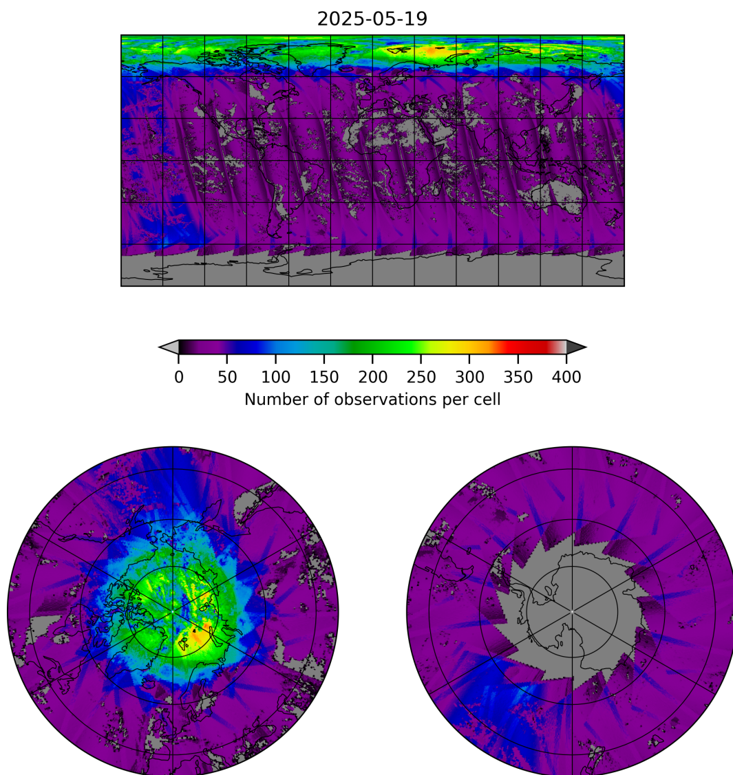
Figure 21: Map of the number of observations for 2025-05-18 to 2025-05-20
