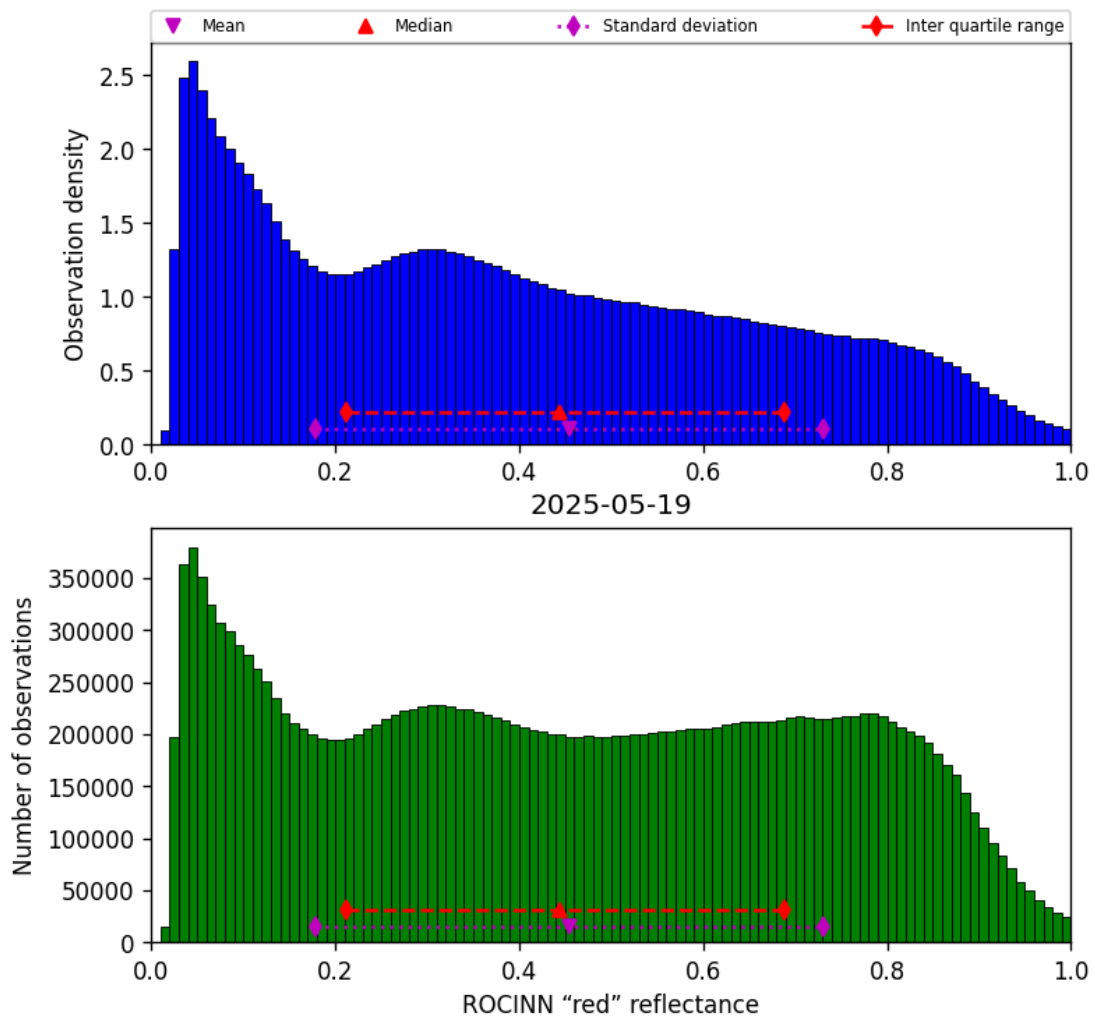
Figure 53: Histogram of “ROCINN “red” reflectance” for 2025-05-18 to 2025-05-20
