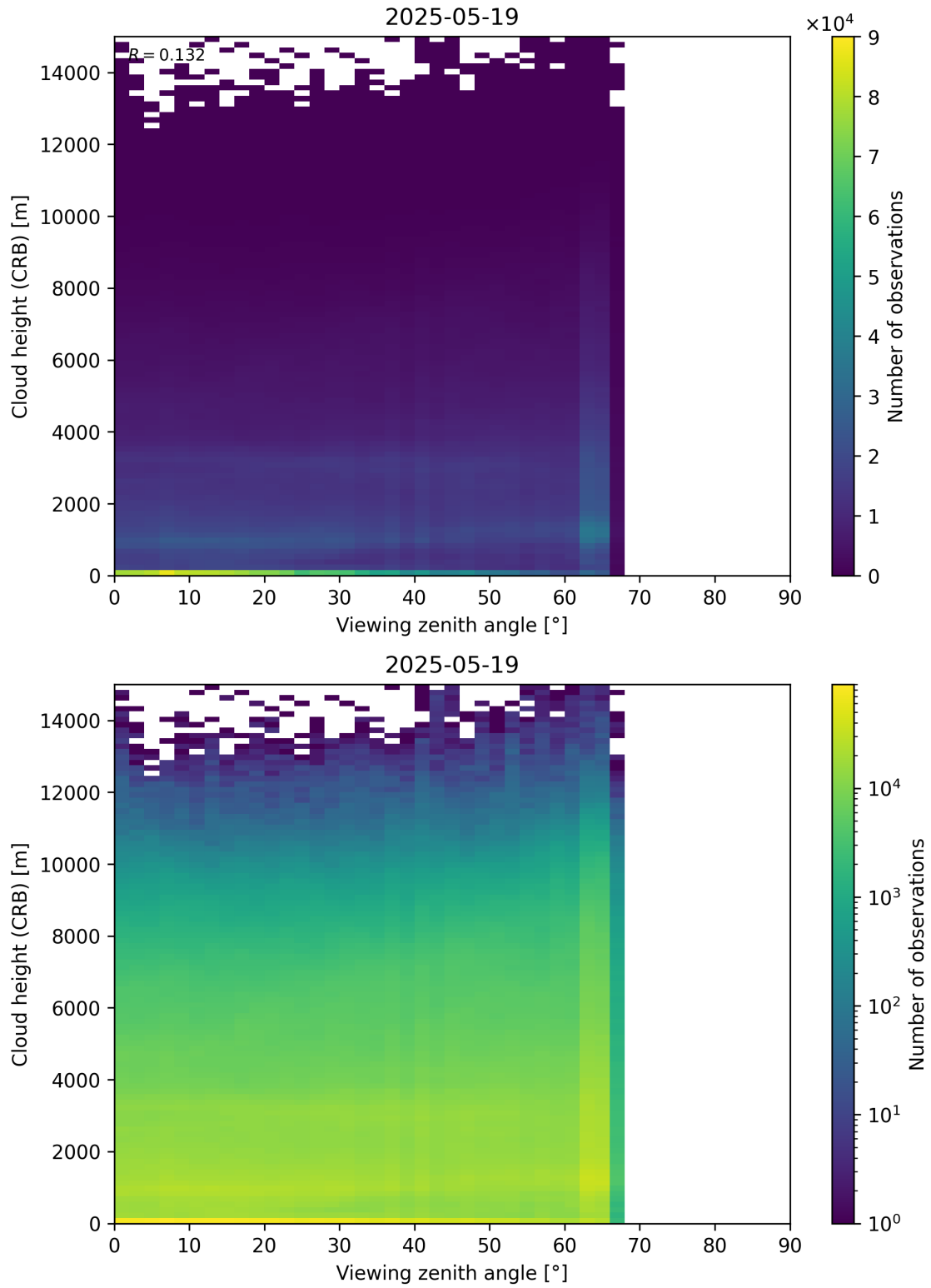
Figure 110: Scatter density plot of “Viewing zenith angle” against “Cloud height (CRB)” for 2025-05-18 to 2025-05-20.
