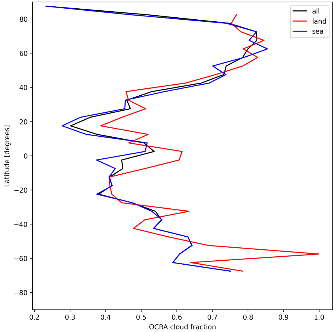
Figure 34: Zonal average of “OCRA cloud fraction” for 2025-05-18 to 2025-05-20.
