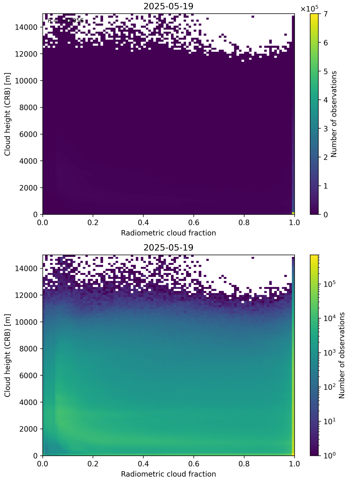
Figure 74: Scatter density plot of “Radiometric cloud fraction” against “Cloud height (CRB)” for 2025-05-18 to 2025-05-20.
