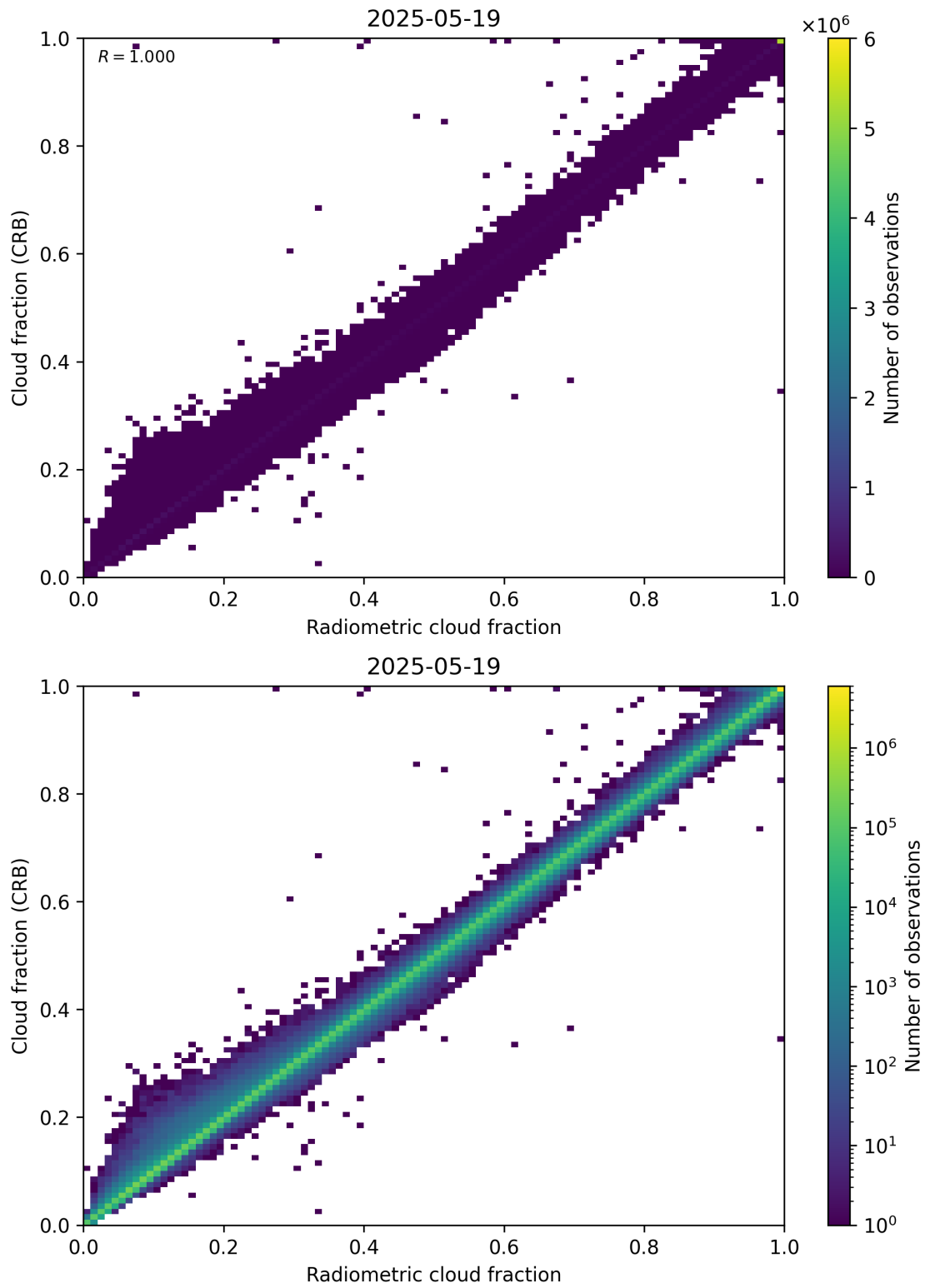
Figure 73: Scatter density plot of “Radiometric cloud fraction” against “Cloud fraction (CRB)” for 2025-05-18 to 2025-05-20.
