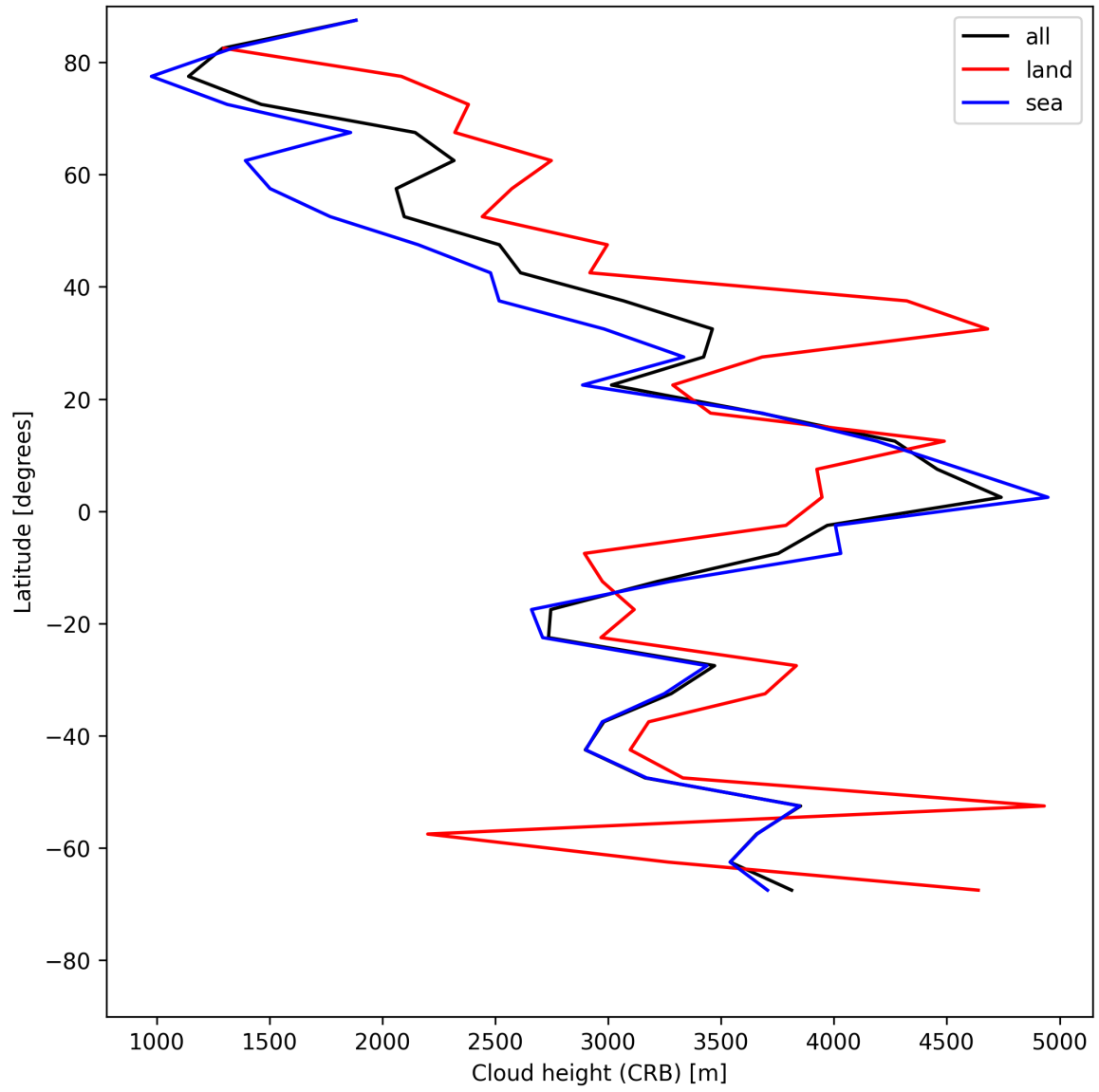
Figure 27: Zonal average of “Cloud height (CRB)” for 2025-05-18 to 2025-05-20.
