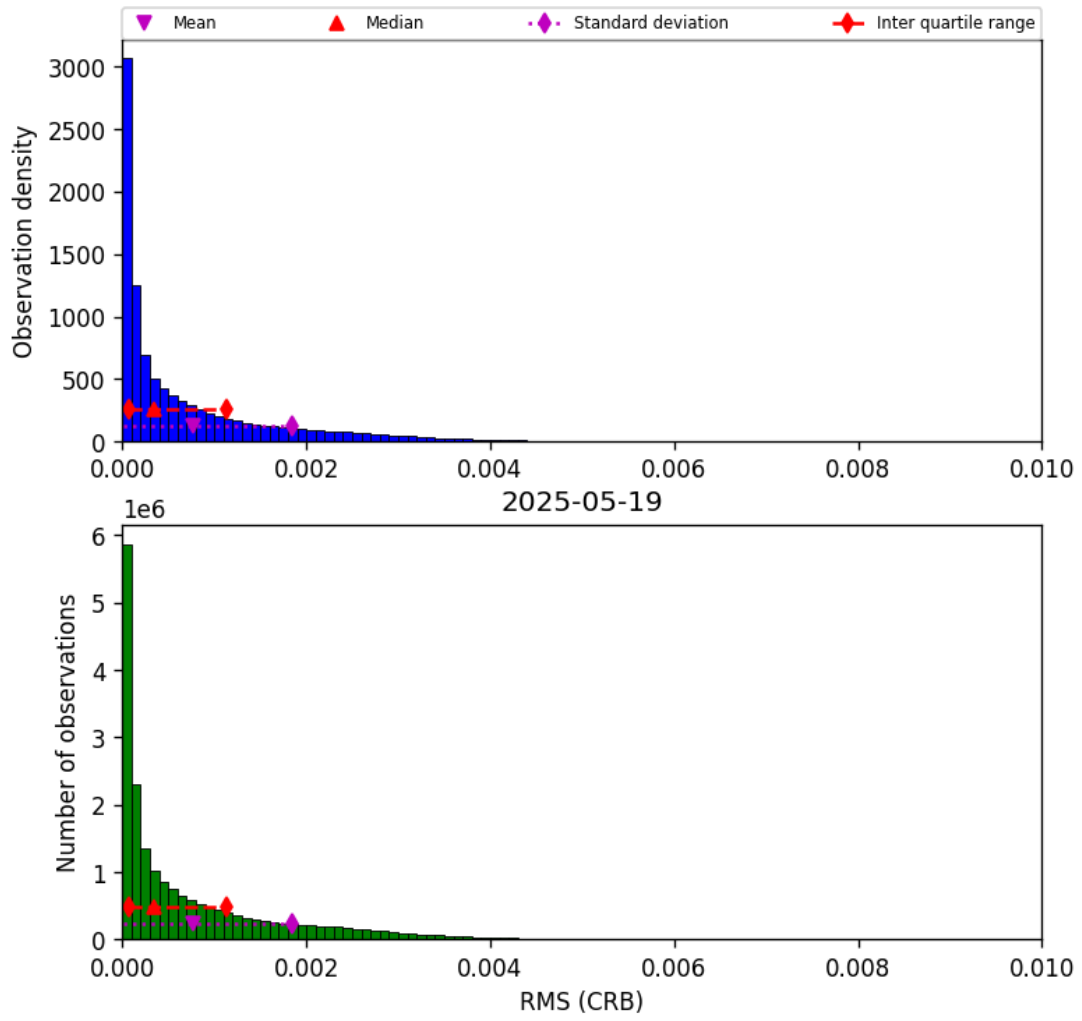
Figure 48: Histogram of “RMS (CRB)” for 2025-05-18 to 2025-05-20
