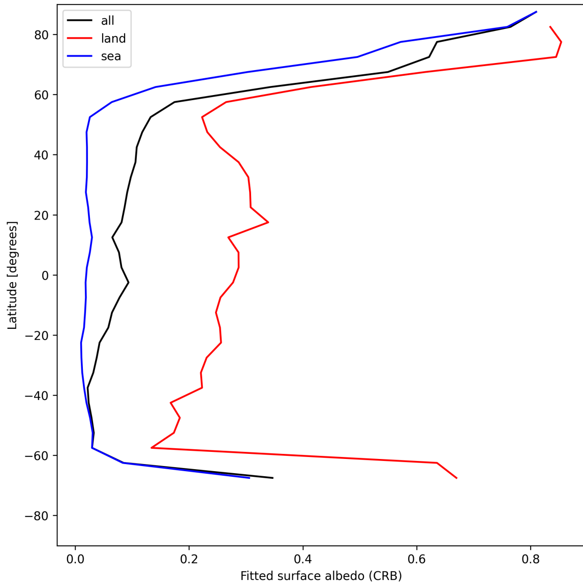
Figure 30: Zonal average of “Fitted surface albedo (CRB)” for 2025-05-18 to 2025-05-20.
