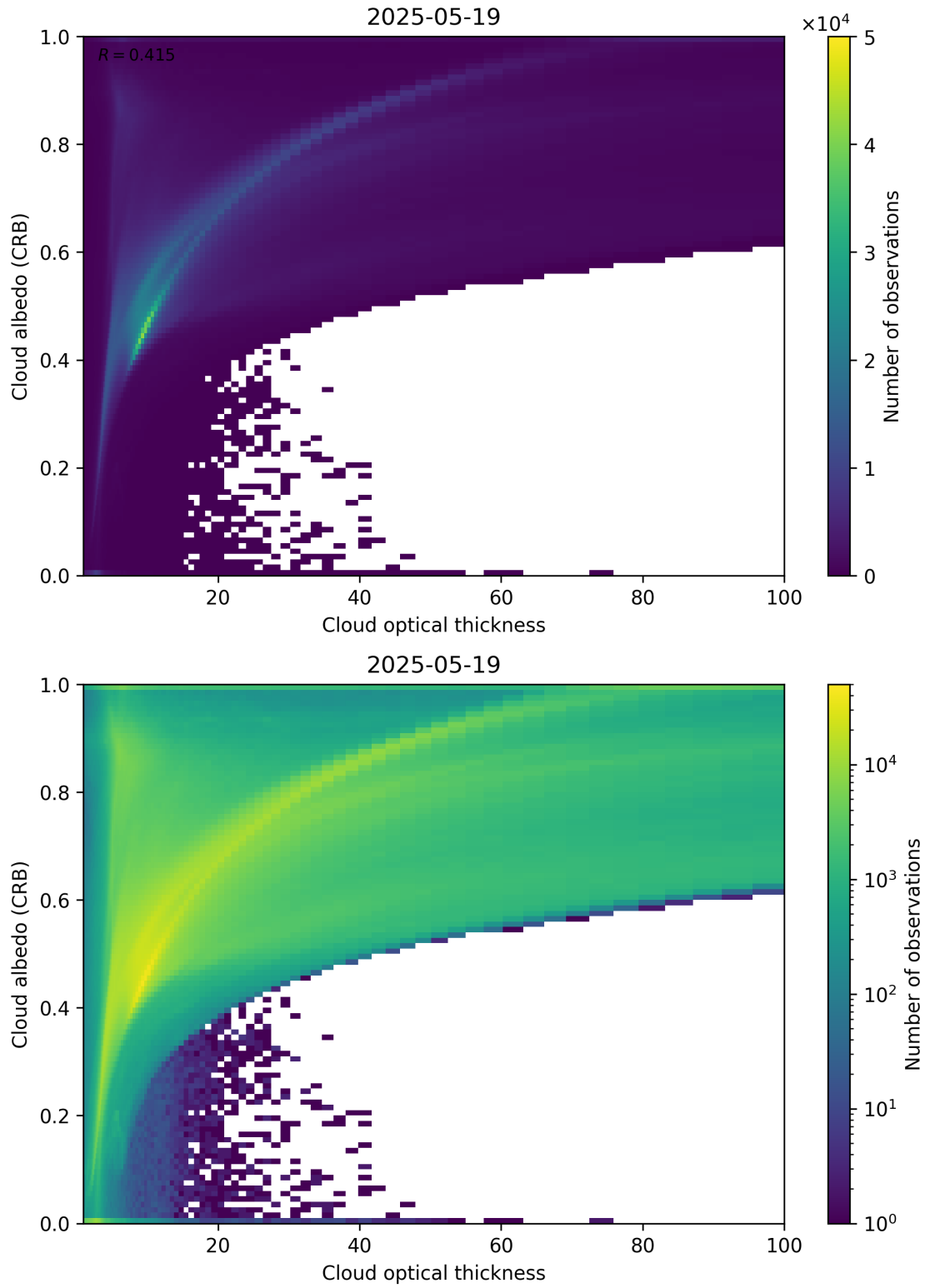
Figure 82: Scatter density plot of “Cloud optical thickness” against “Cloud albedo (CRB)” for 2025-05-18 to 2025-05-20.
