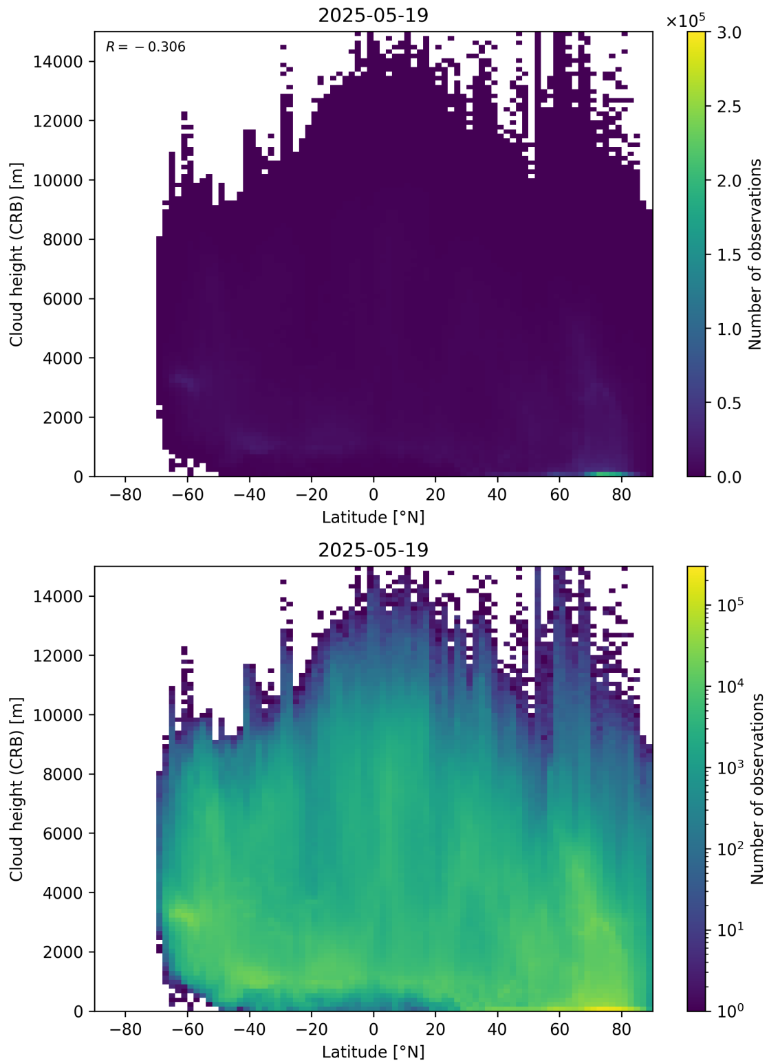
Figure 95: Scatter density plot of “Latitude” against “Cloud height (CRB)” for 2025-05-18 to 2025-05-20.
