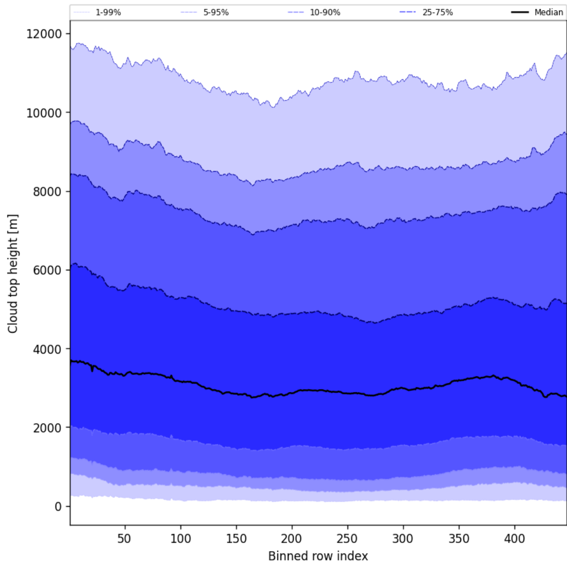
Figure 56: Along track statistics of “Cloud top height” for 2025-05-18 to 2025-05-20
