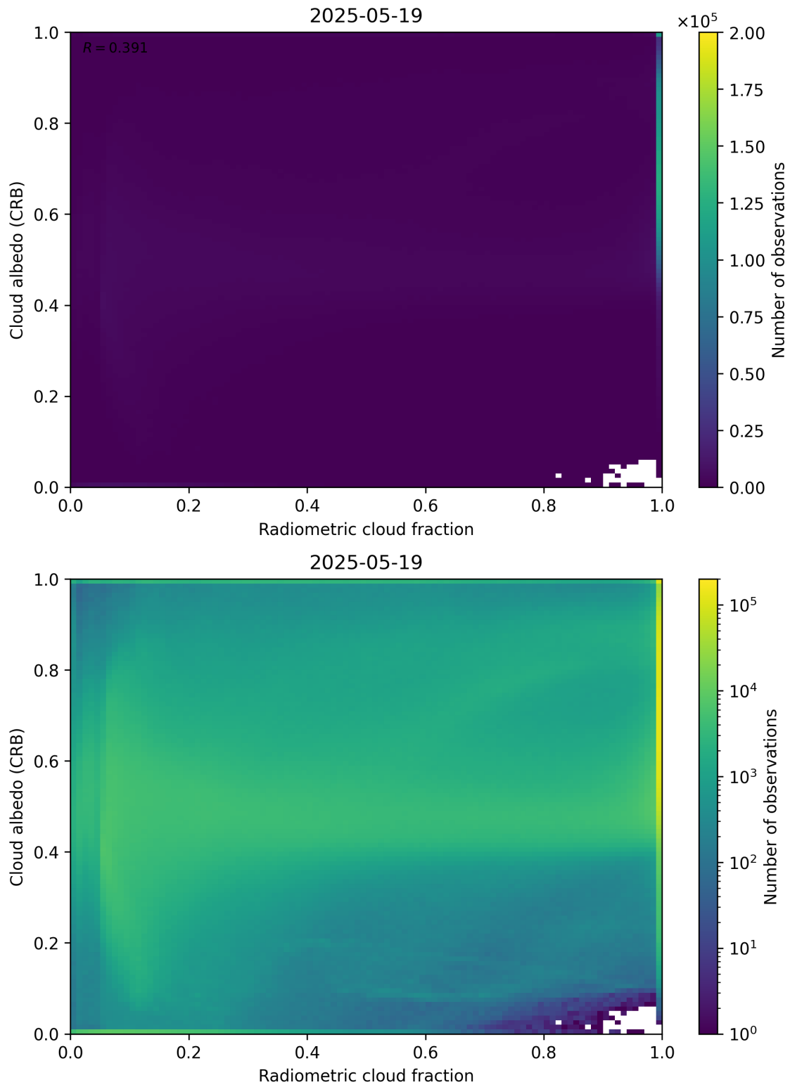
Figure 71: Scatter density plot of “Radiometric cloud fraction” against “Cloud albedo (CRB)” for 2025-05-18 to 2025-05-20.
