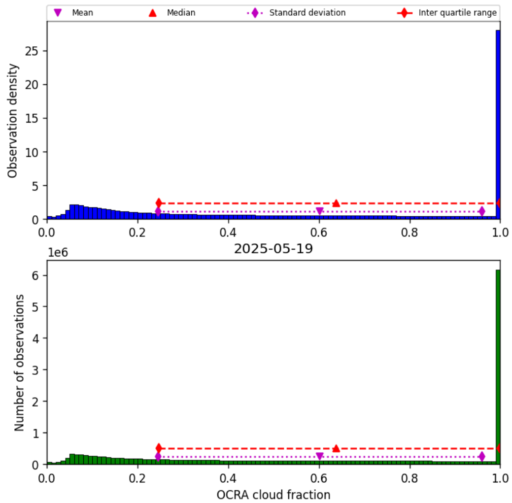
Figure 50: Histogram of “OCRA cloud fraction” for 2025-05-18 to 2025-05-20
