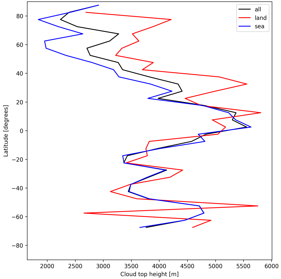
Figure 24: Zonal average of “Cloud top height” for 2025-05-18 to 2025-05-20.
