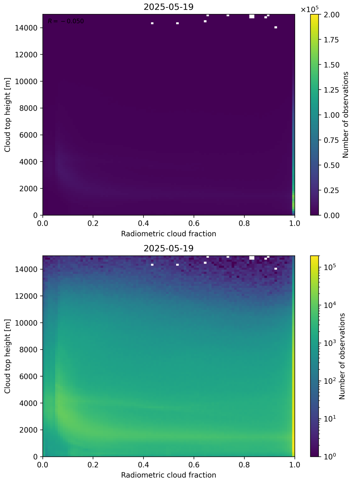
Figure 76: Scatter density plot of “Radiometric cloud fraction” against “Cloud top height” for 2025-05-18 to 2025-05-20.
