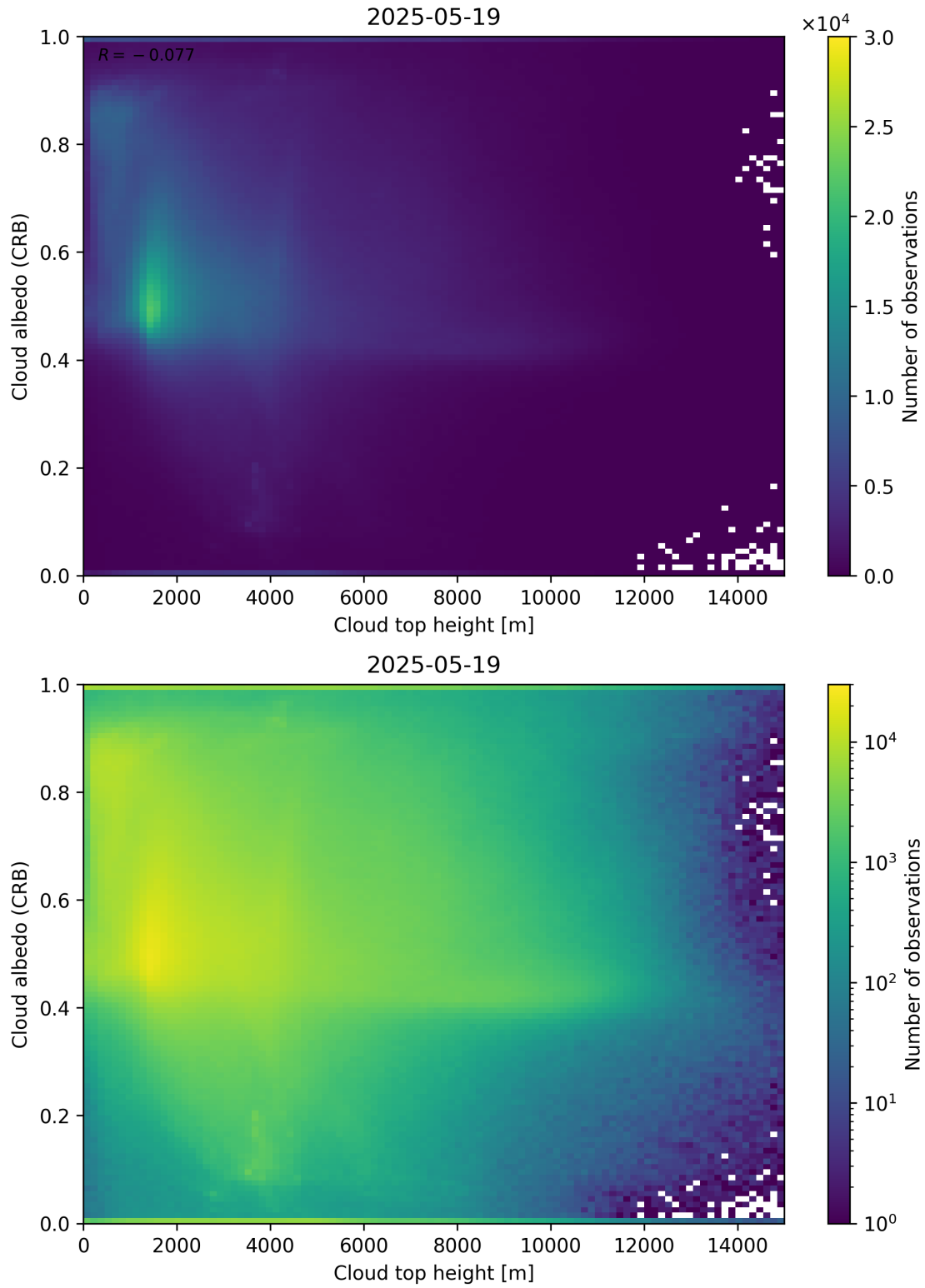
Figure 86: Scatter density plot of “Cloud top height” against “Cloud albedo (CRB)” for 2025-05-18 to 2025-05-20.
