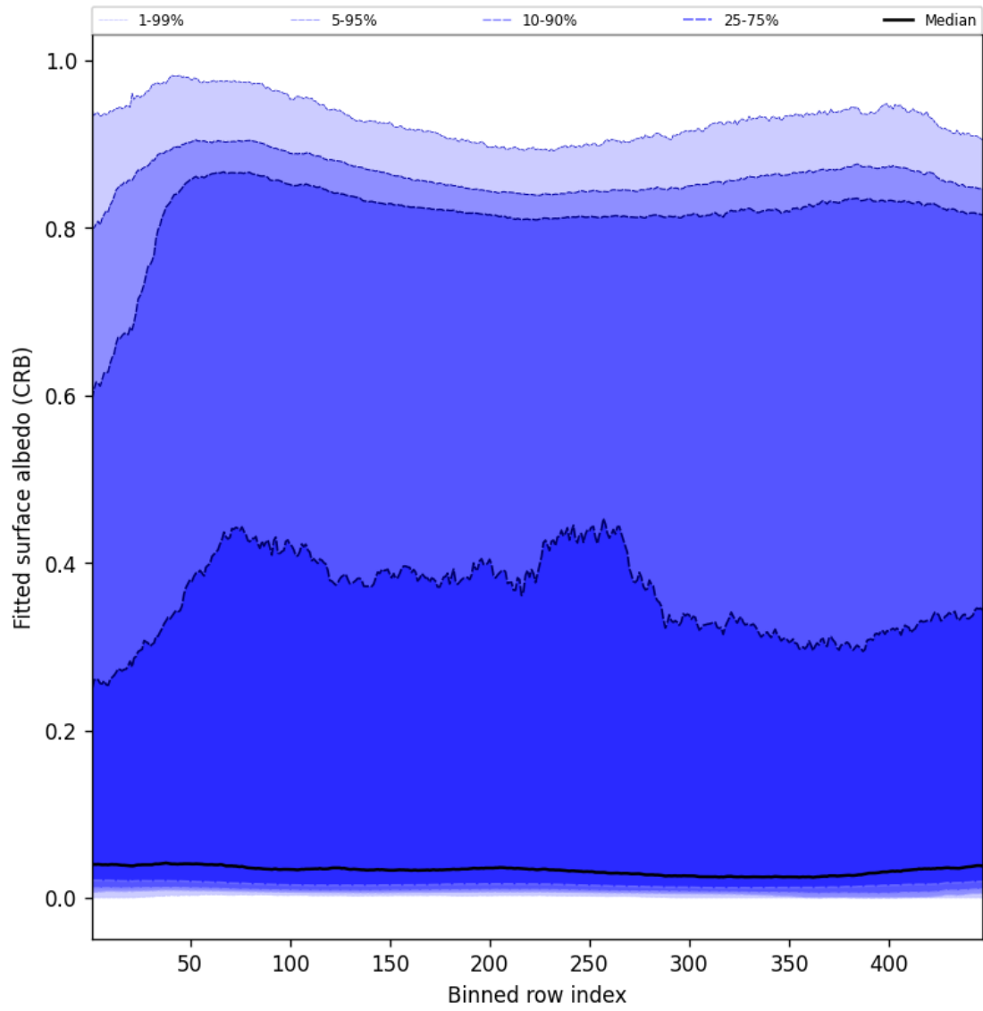
Figure 62: Along track statistics of “Fitted surface albedo (CRB)” for 2025-05-18 to 2025-05-20
