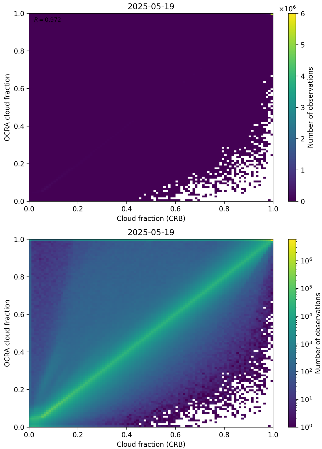
Figure 78: Scatter density plot of “Cloud fraction (CRB)” against “OCRA cloud fraction” for 2025-05-18 to 2025-05-20.
