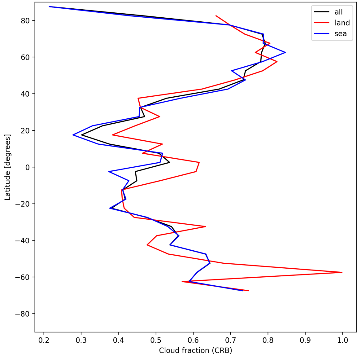
Figure 26: Zonal average of “Cloud fraction (CRB)” for 2025-05-18 to 2025-05-20.
