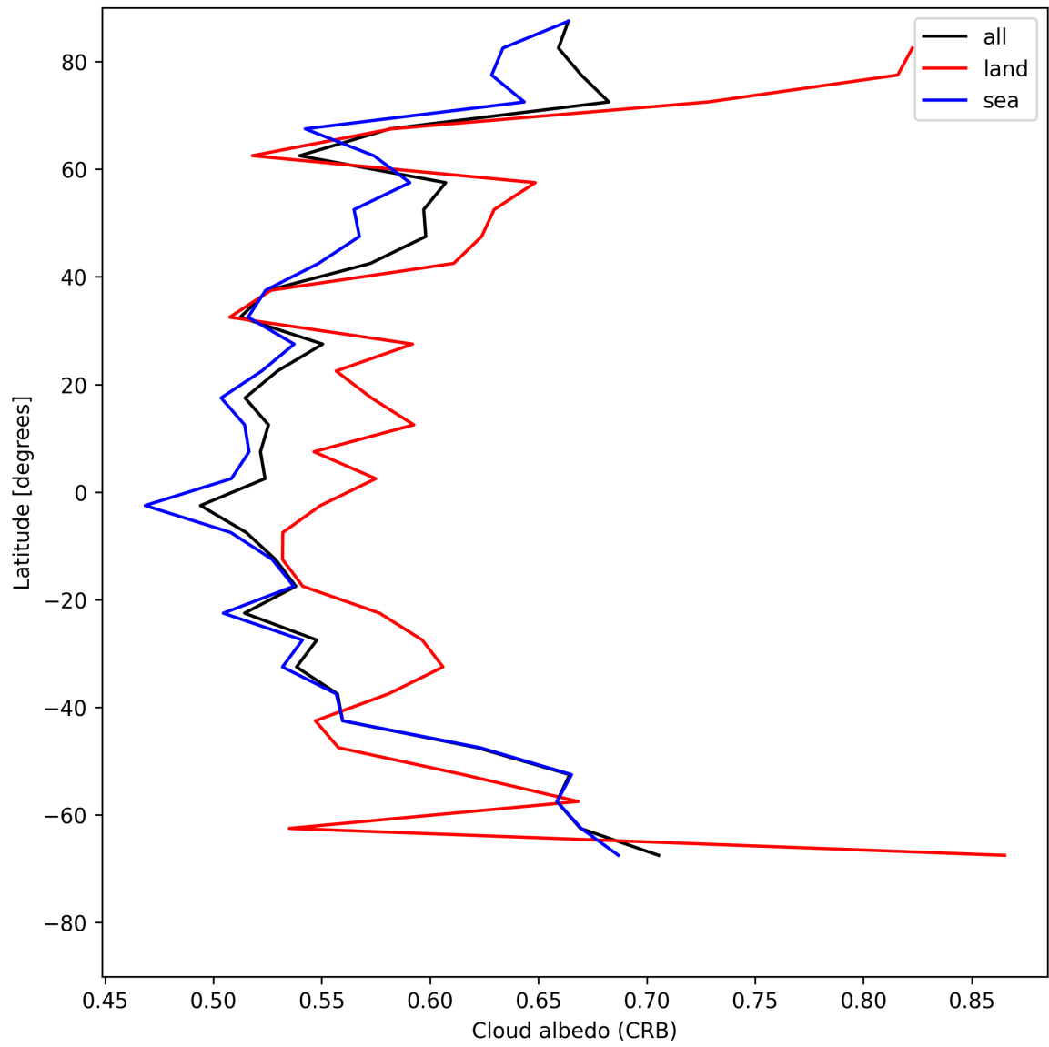
Figure 28: Zonal average of “Cloud albedo (CRB)” for 2025-05-18 to 2025-05-20.
