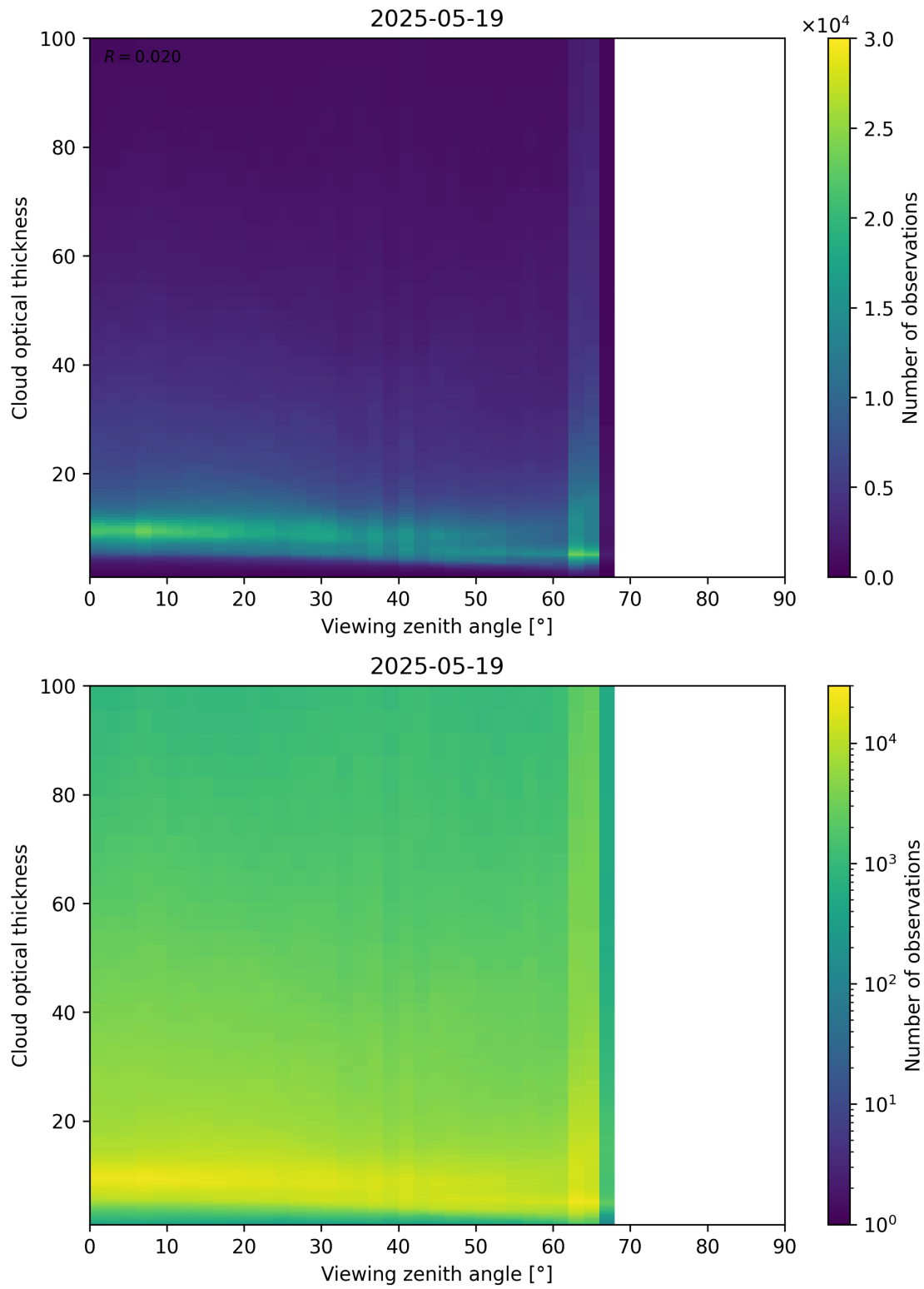
Figure 111: Scatter density plot of “Viewing zenith angle” against “Cloud optical thickness” for 2025-05-18 to 2025-05-20.
