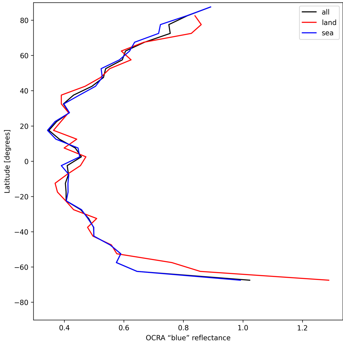
Figure 35: Zonal average of “OCRA “blue” reflectance” for 2025-05-18 to 2025-05-20.
