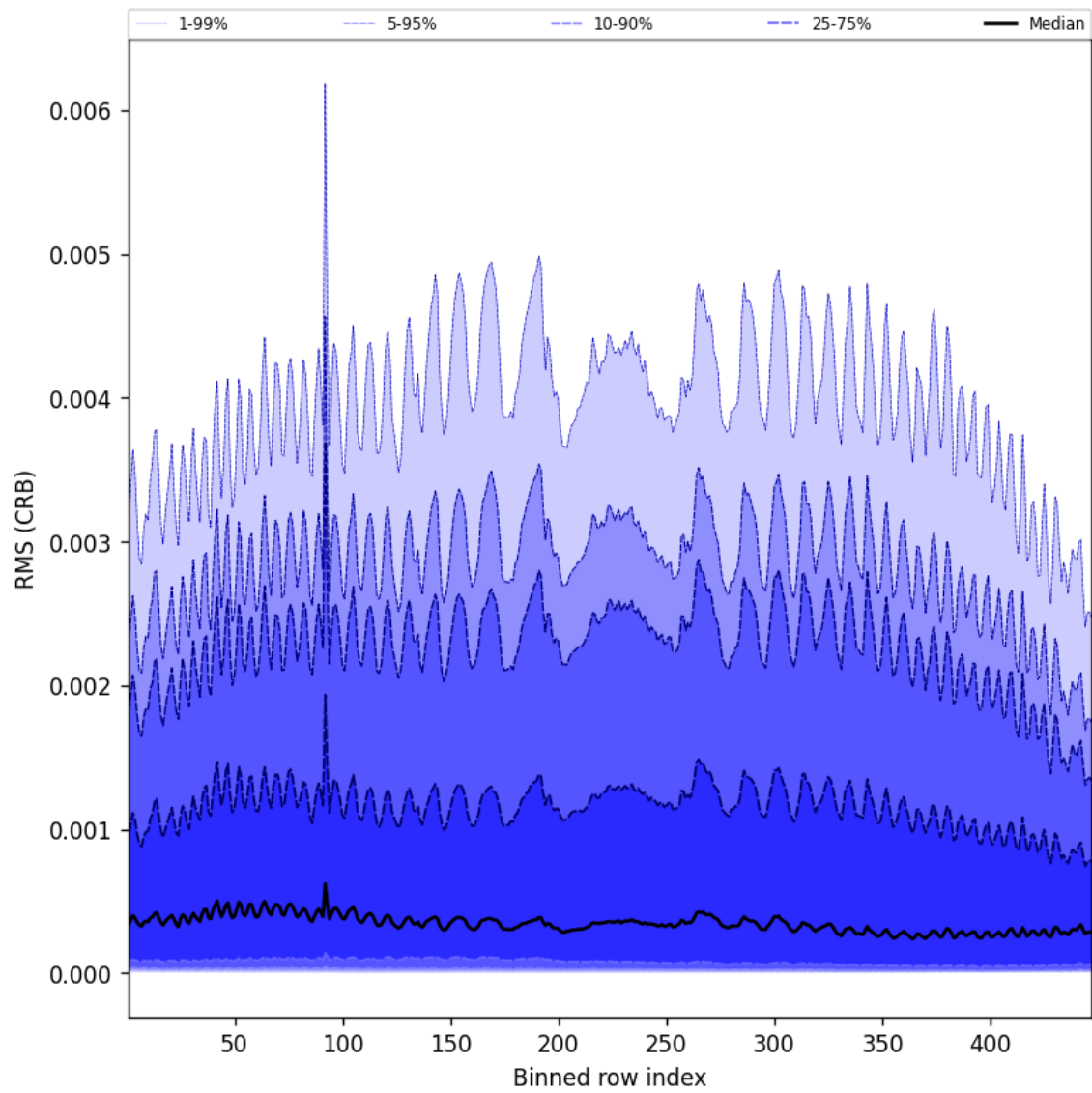
Figure 64: Along track statistics of “RMS (CRB)” for 2025-05-18 to 2025-05-20
