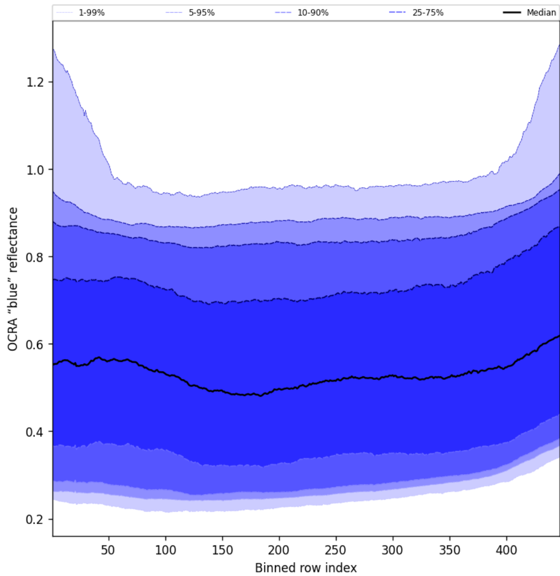
Figure 67: Along track statistics of "OCRA "blue" reflectance" for 2025-05-18 to 2025-05-20
