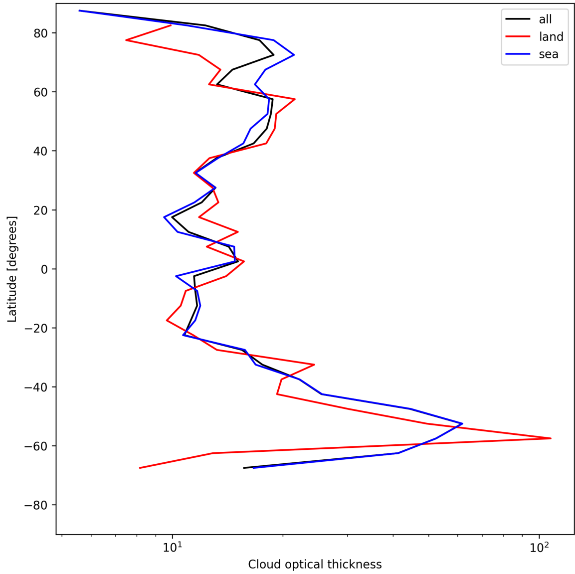
Figure 25: Zonal average of “Cloud optical thickness” for 2025-05-18 to 2025-05-20.
