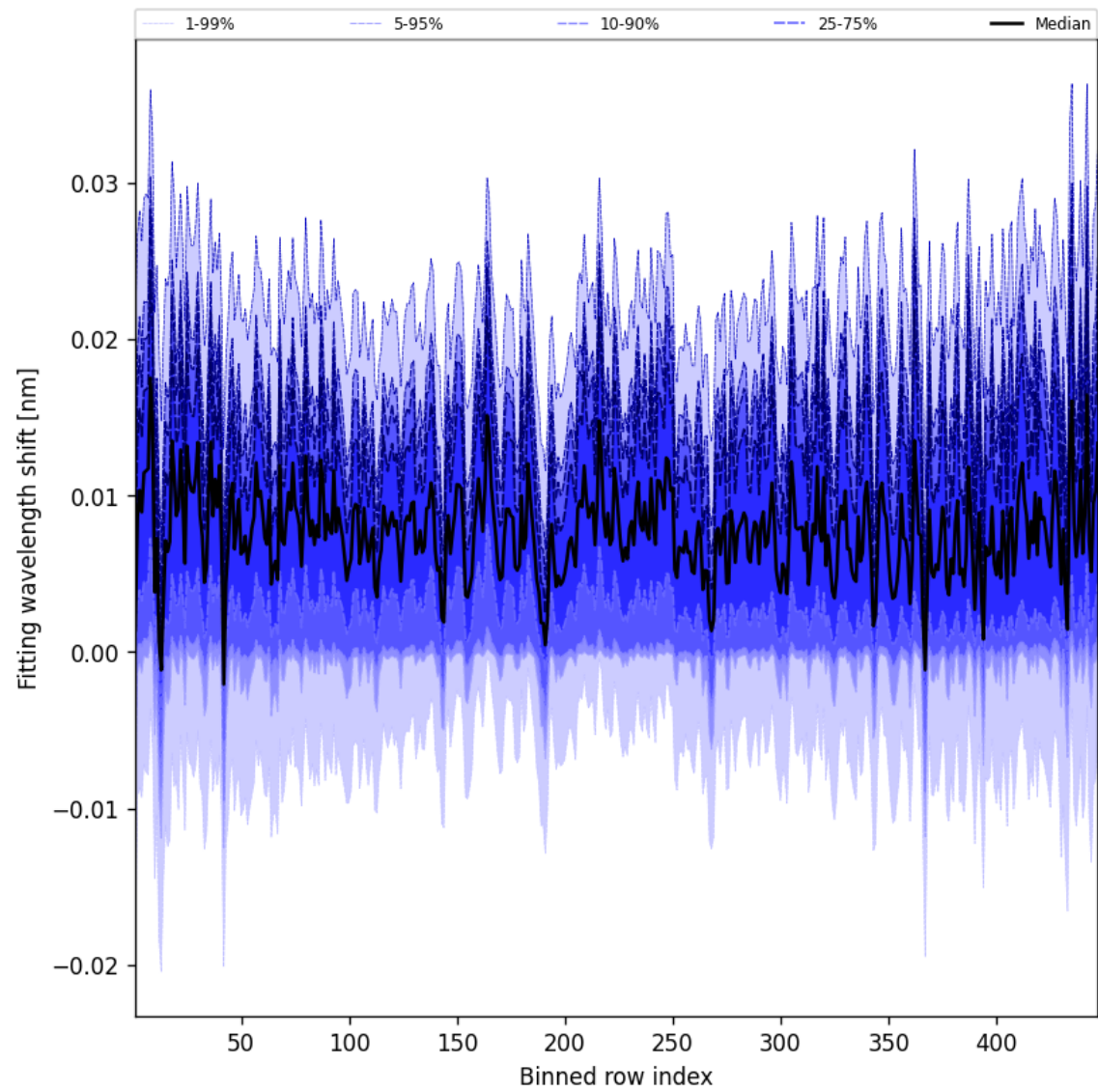
Figure 65: Along track statistics of “Fitting wavelength shift” for 2025-05-18 to 2025-05-20
