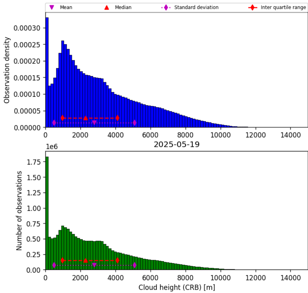
Figure 43: Histogram of “Cloud height (CRB)” for 2025-05-18 to 2025-05-20
