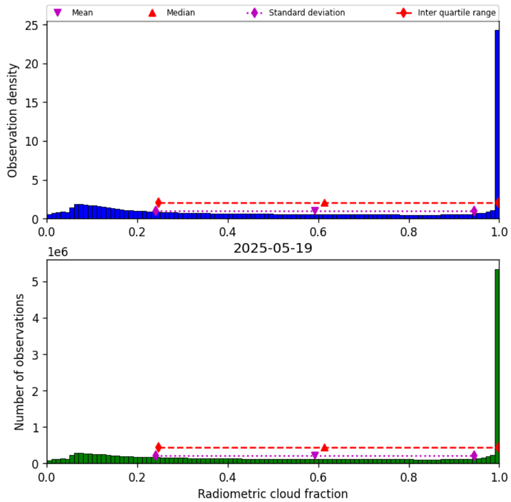
Figure 39: Histogram of “Radiometric cloud fraction” for 2025-05-18 to 2025-05-20
