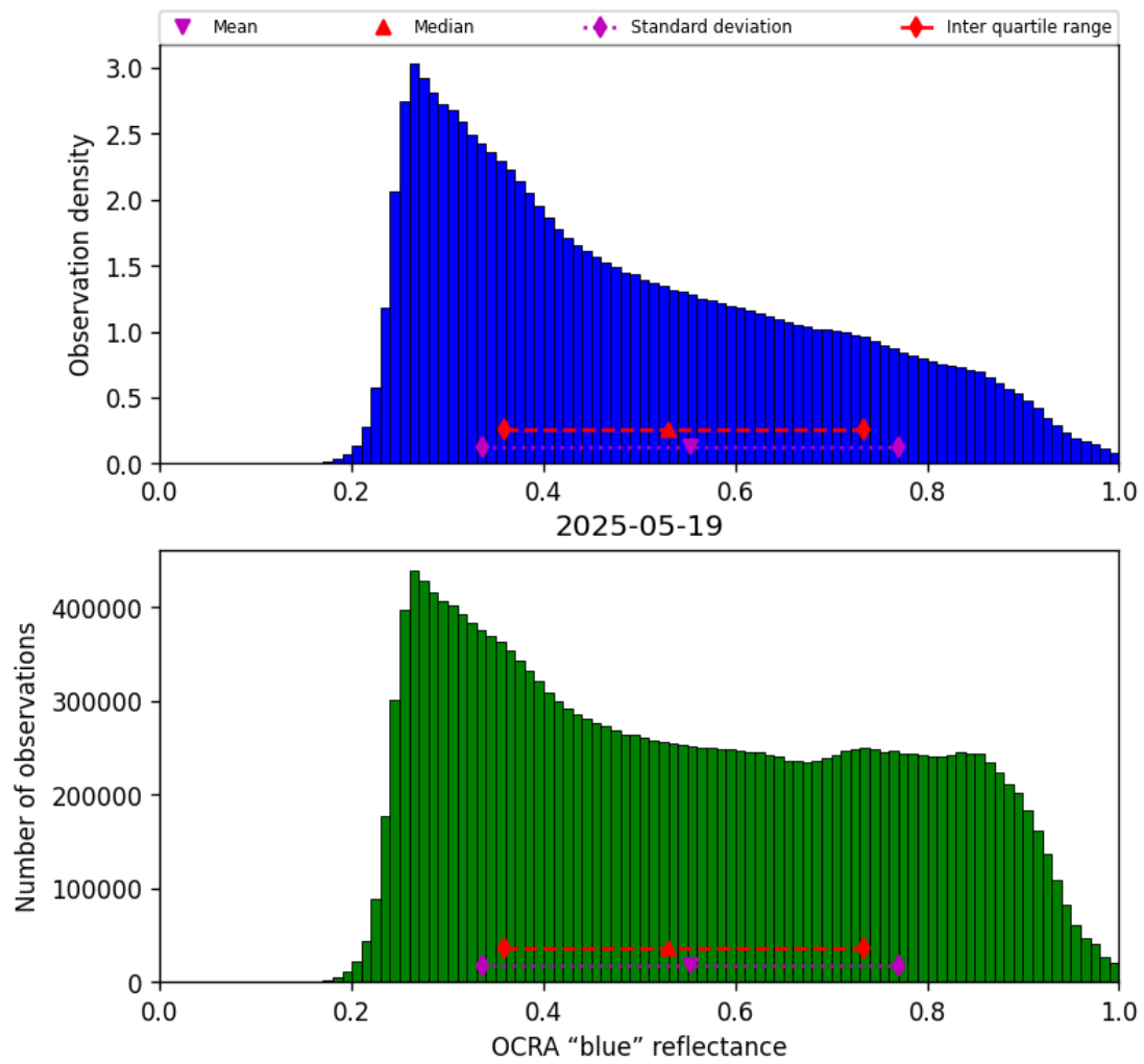
Figure 51: Histogram of “OCRA “blue” reflectance” for 2025-05-18 to 2025-05-20
