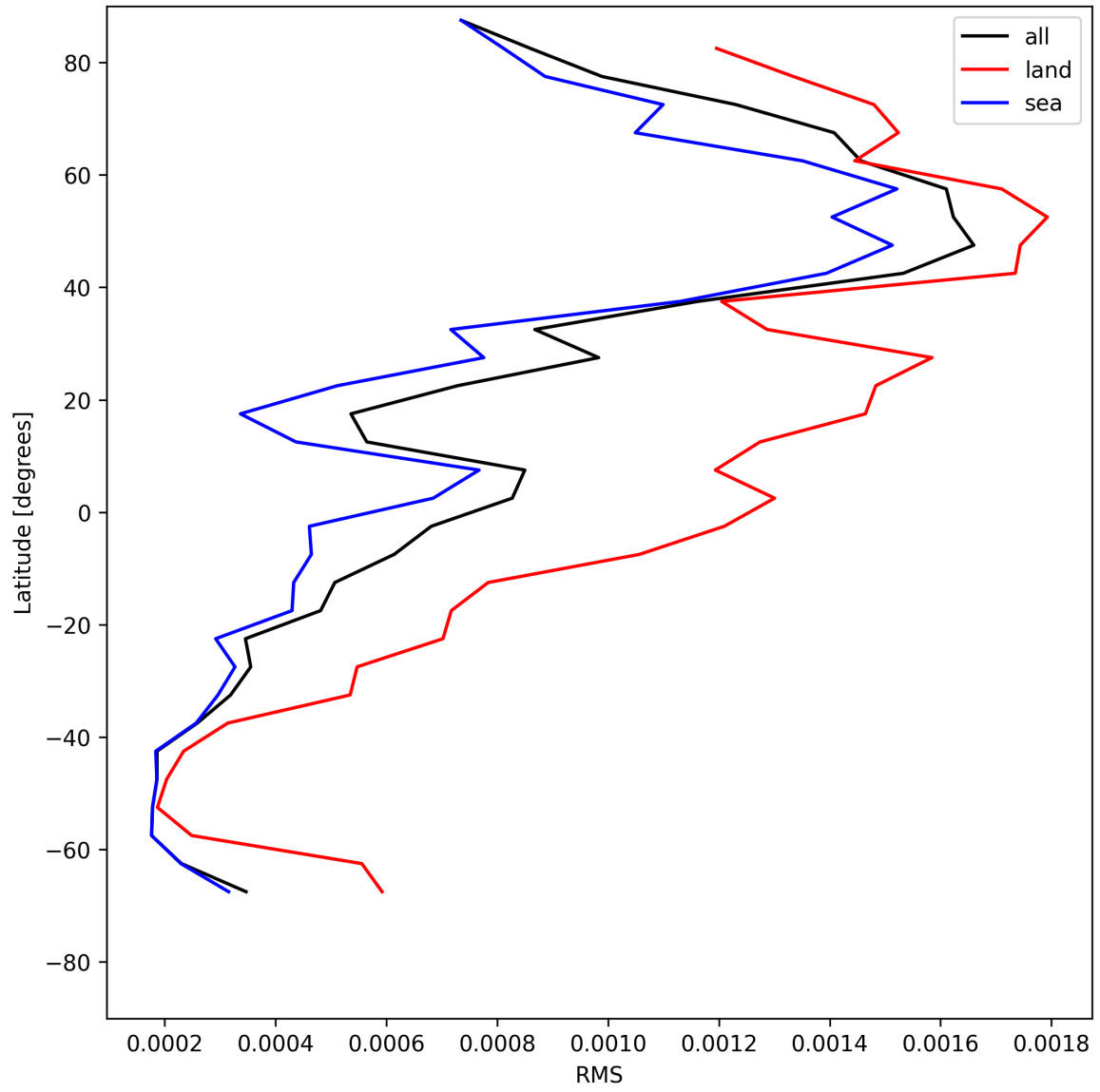
Figure 31: Zonal average of “RMS” for 2025-05-18 to 2025-05-20.
