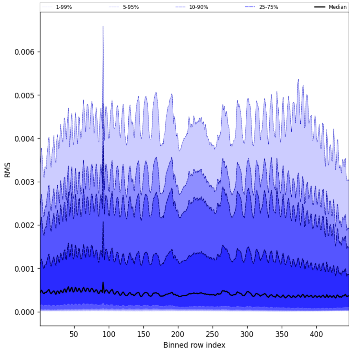
Figure 63: Along track statistics of “RMS” for 2025-05-18 to 2025-05-20
