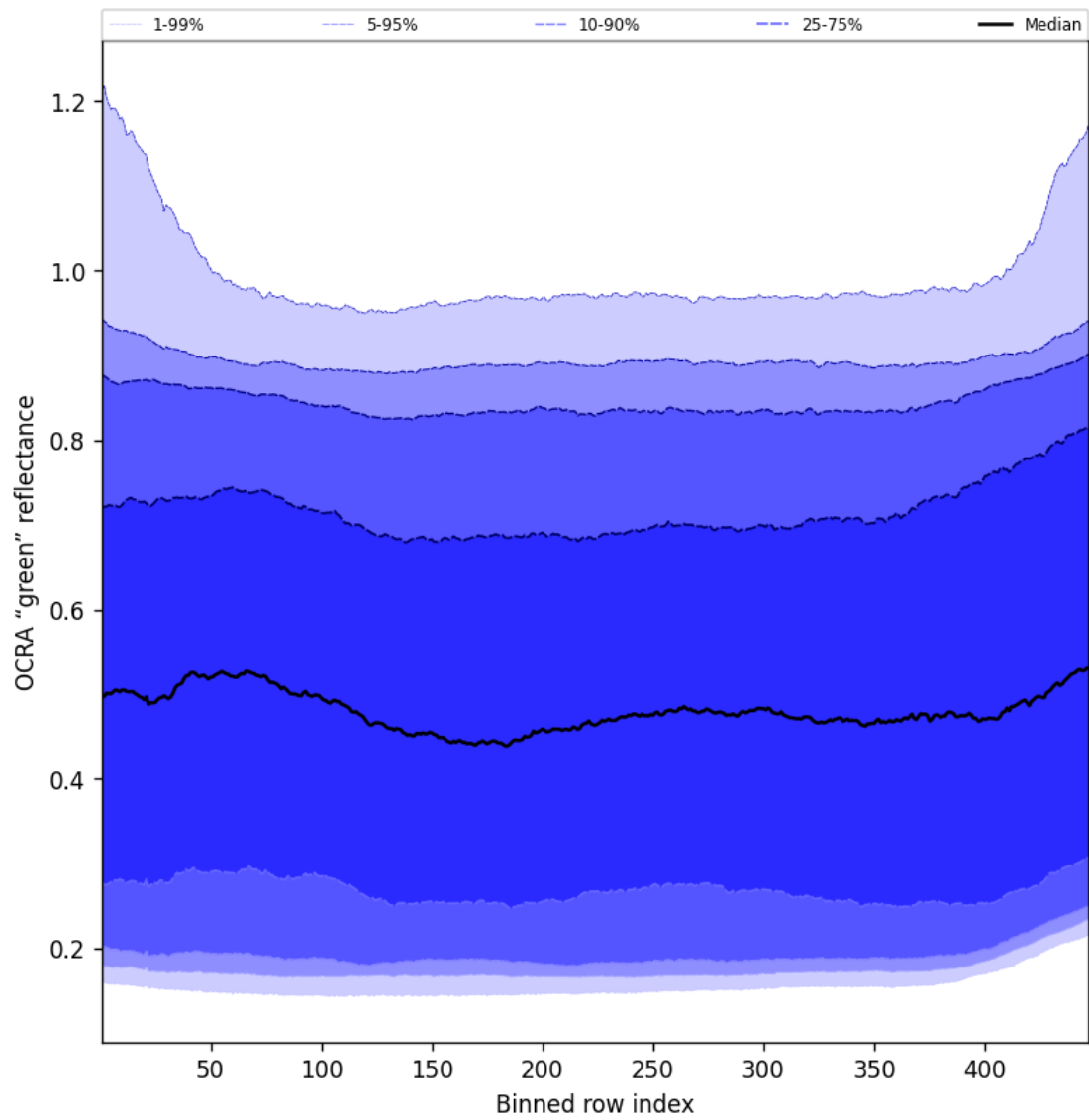
Figure 68: Along track statistics of "OCRA "green" reflectance" for 2025-05-18 to 2025-05-20
