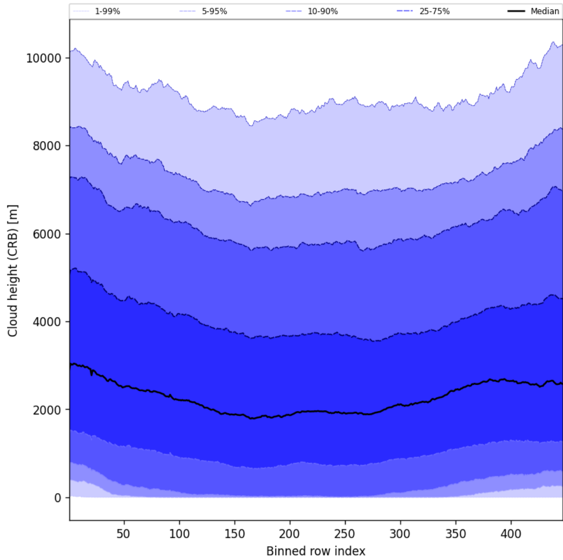
Figure 59: Along track statistics of “Cloud height (CRB)” for 2025-05-18 to 2025-05-20
