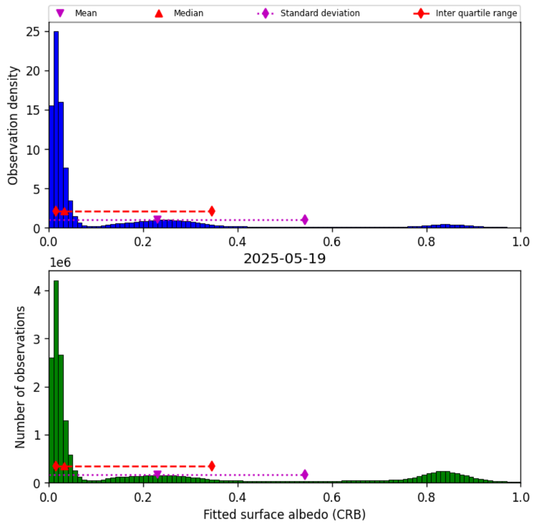
Figure 46: Histogram of “Fitted surface albedo (CRB)” for 2025-05-18 to 2025-05-20
