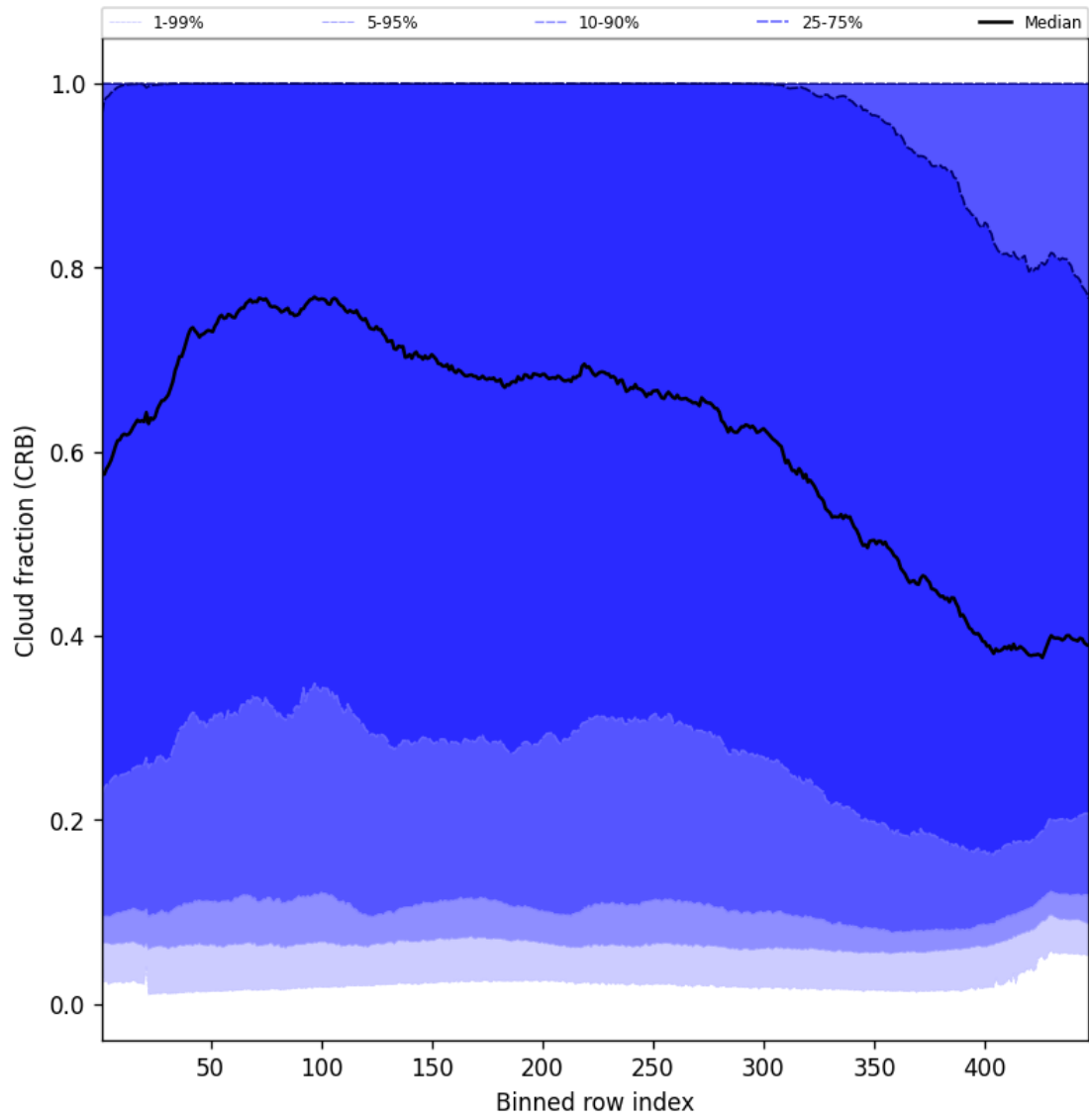
Figure 58: Along track statistics of “Cloud fraction (CRB)” for 2025-05-18 to 2025-05-20
