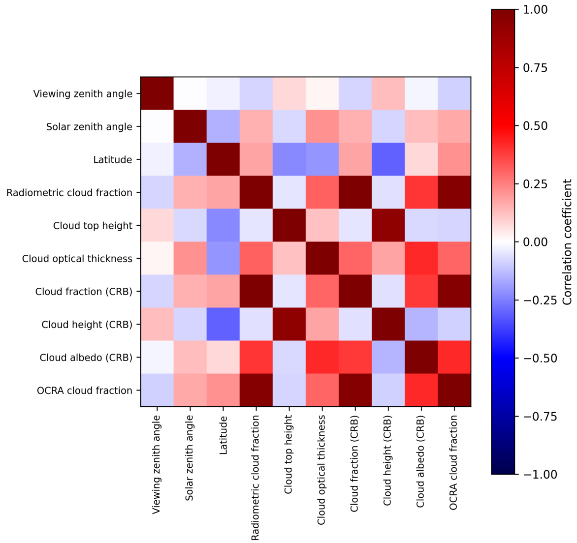
Figure 2: Map of correlation matrix for 2025-05-18 to 2025-05-20.
