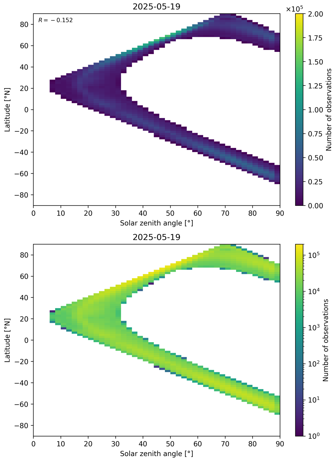
Figure 105: Scatter density plot of “Solar zenith angle” against “Latitude” for 2025-05-18 to 2025-05-20.
