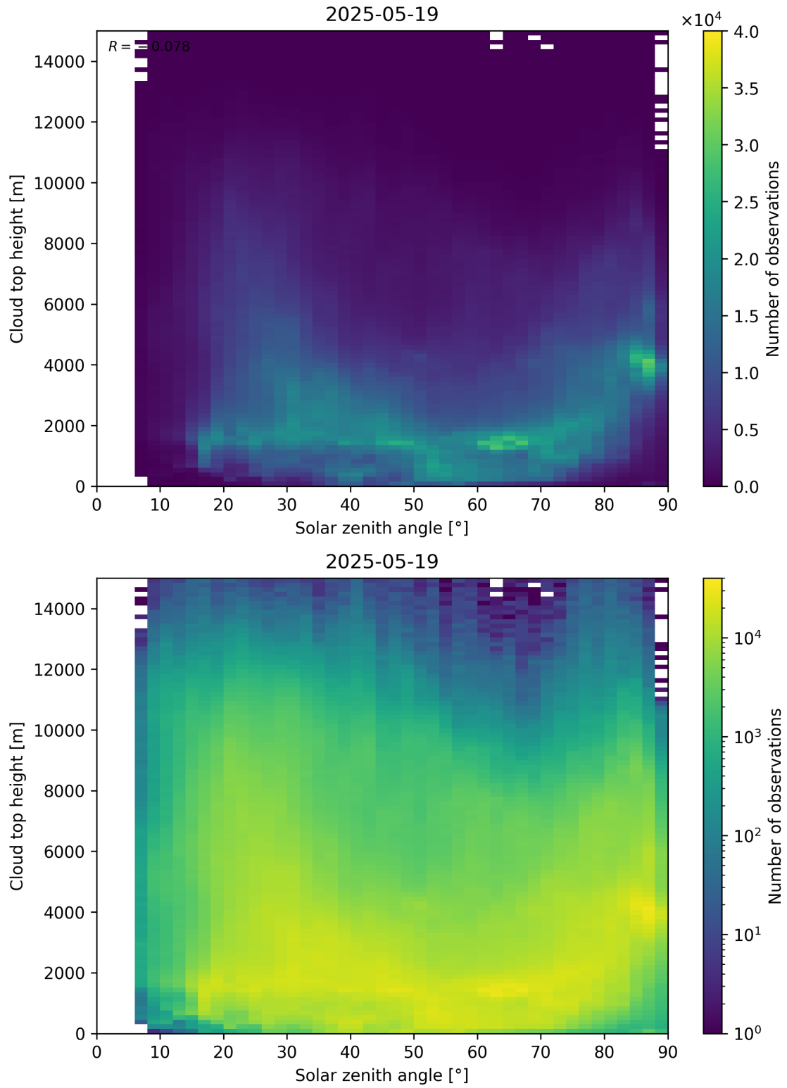
Figure 104: Scatter density plot of “Solar zenith angle” against “Cloud top height” for 2025-05-18 to 2025-05-20.
