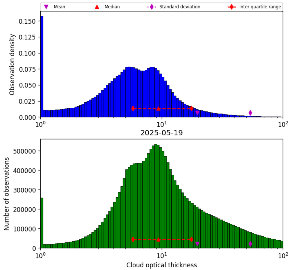
Figure 41: Histogram of “Cloud optical thickness” for 2025-05-18 to 2025-05-20
