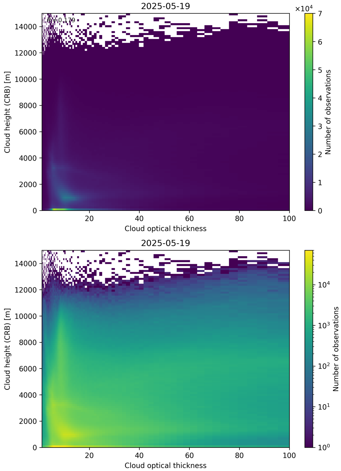
Figure 85: Scatter density plot of “Cloud optical thickness” against “Cloud height (CRB)” for 2025-05-18 to 2025-05-20.
