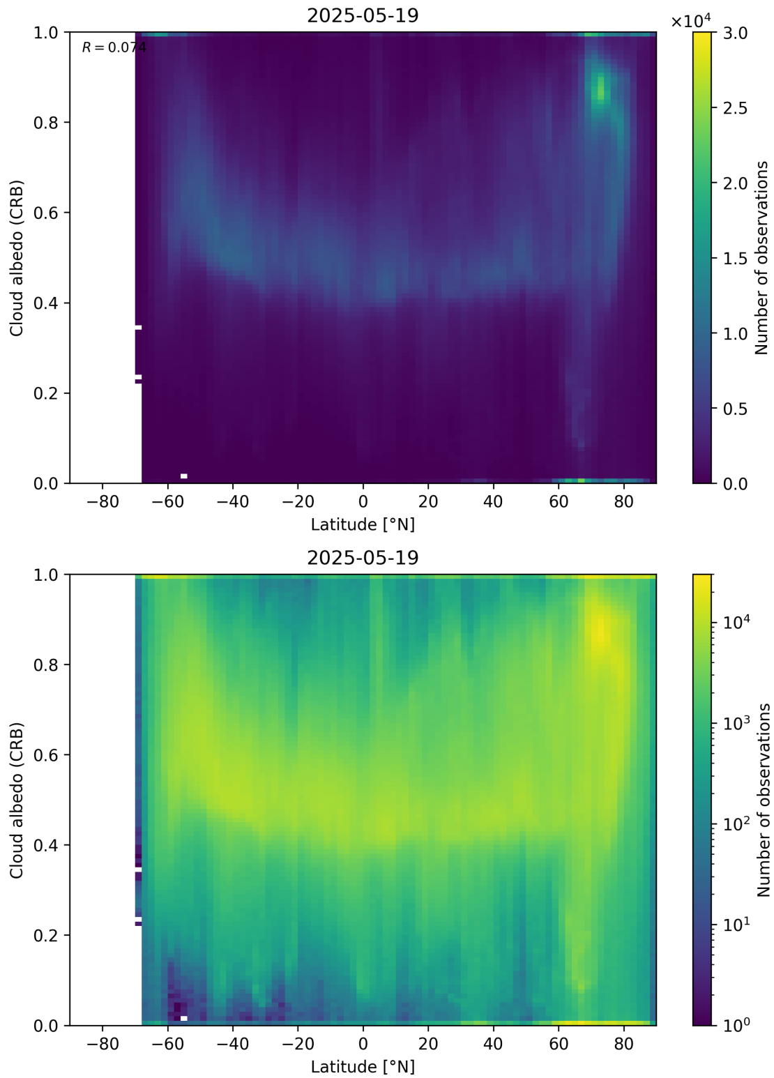
Figure 91: Scatter density plot of “Latitude” against “Cloud albedo (CRB)” for 2025-05-18 to 2025-05-20.
