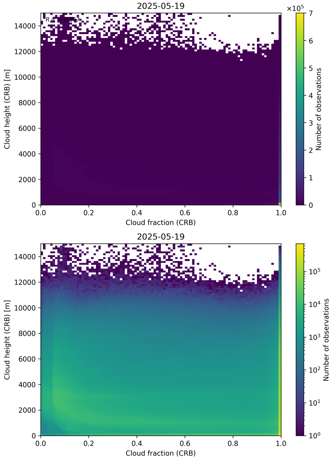
Figure 79: Scatter density plot of “Cloud fraction (CRB)” against “Cloud height (CRB)” for 2025-05-18 to 2025-05-20.
