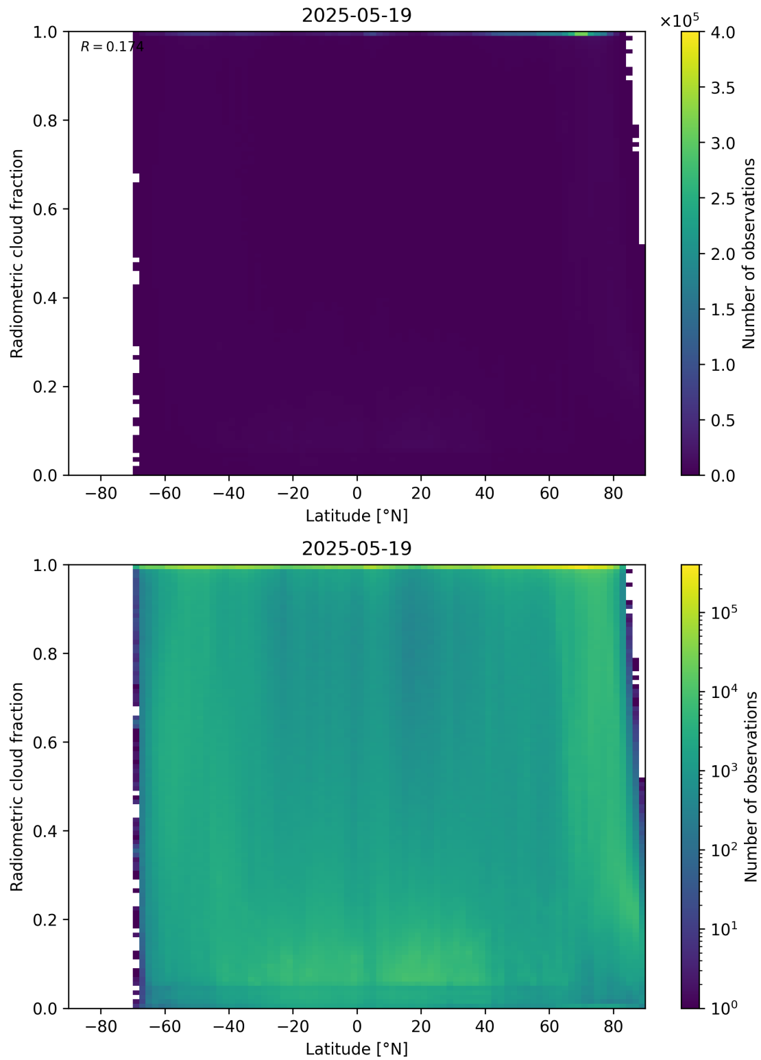
Figure 92: Scatter density plot of “Latitude” against “Radiometric cloud fraction” for 2025-05-18 to 2025-05-20.
