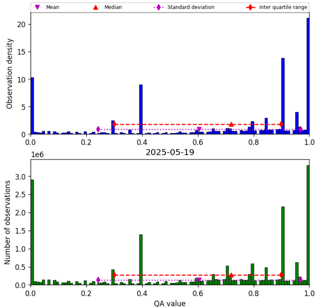
Figure 38: Histogram of “QA value” for 2025-05-18 to 2025-05-20
