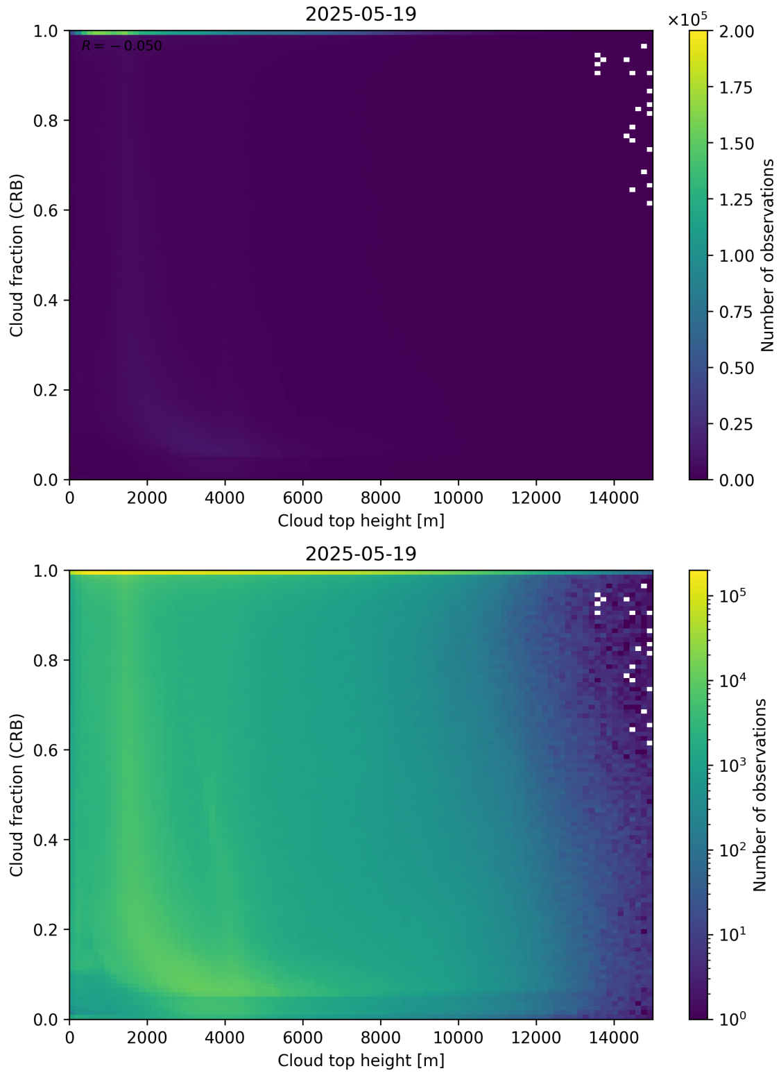
Figure 88: Scatter density plot of “Cloud top height” against “Cloud fraction (CRB)” for 2025-05-18 to 2025-05-20.
