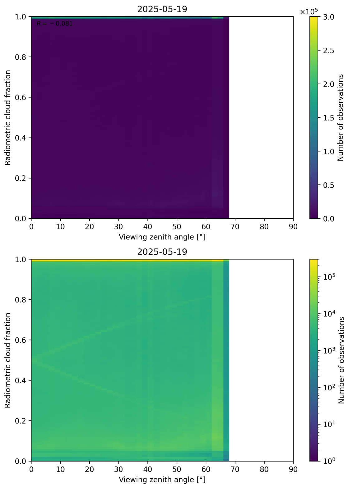
Figure 107: Scatter density plot of “Viewing zenith angle” against “Radiometric cloud fraction” for 2025-05-18 to 2025-05-20.
