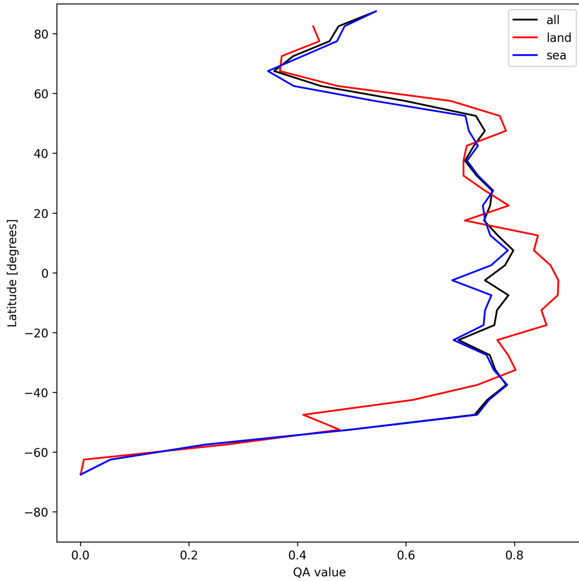
Figure 22: Zonal average of “QA value” for 2025-05-18 to 2025-05-20.
