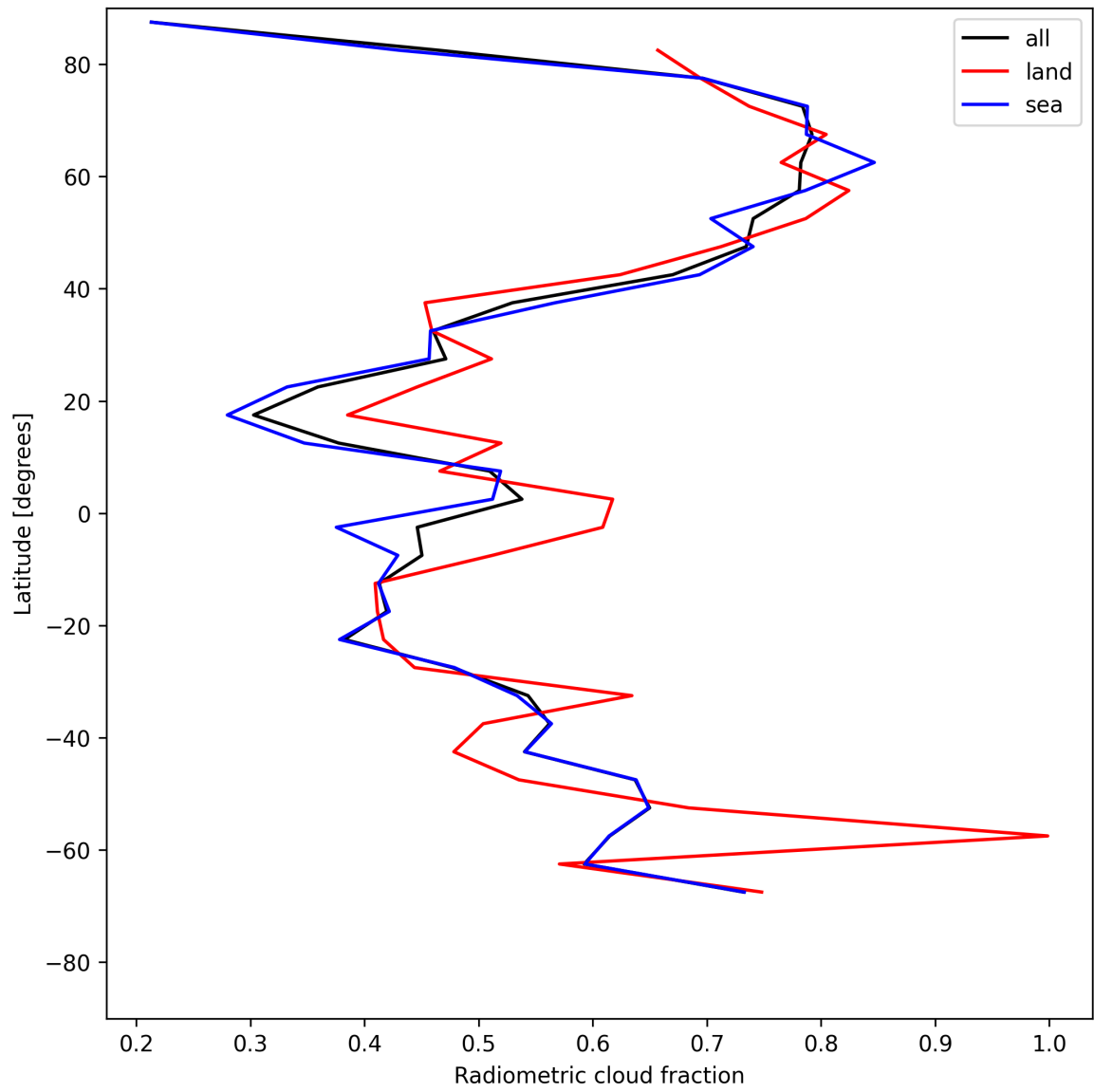
Figure 23: Zonal average of “Radiometric cloud fraction” for 2025-05-18 to 2025-05-20.
