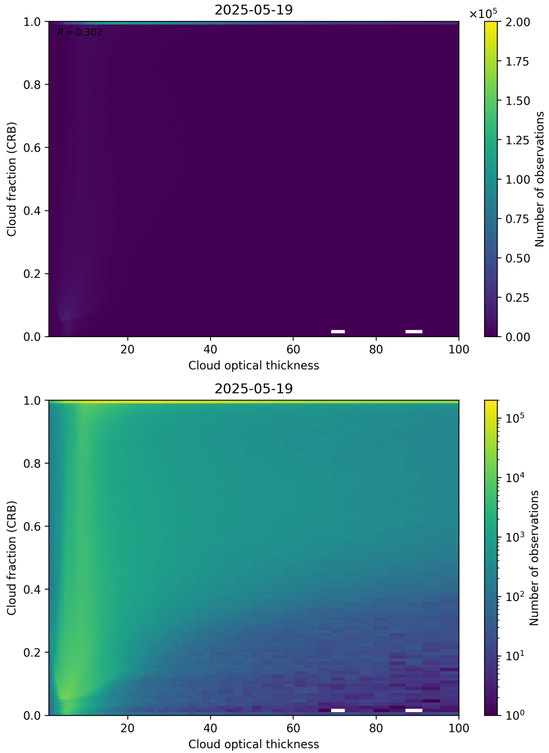
Figure 84: Scatter density plot of “Cloud optical thickness” against “Cloud fraction (CRB)” for 2025-05-18 to 2025-05-20.
