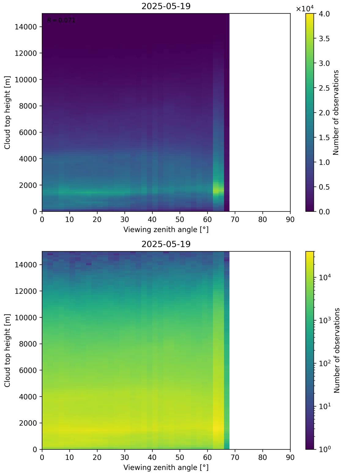
Figure 112: Scatter density plot of “Viewing zenith angle” against “Cloud top height” for 2025-05-18 to 2025-05-20.
