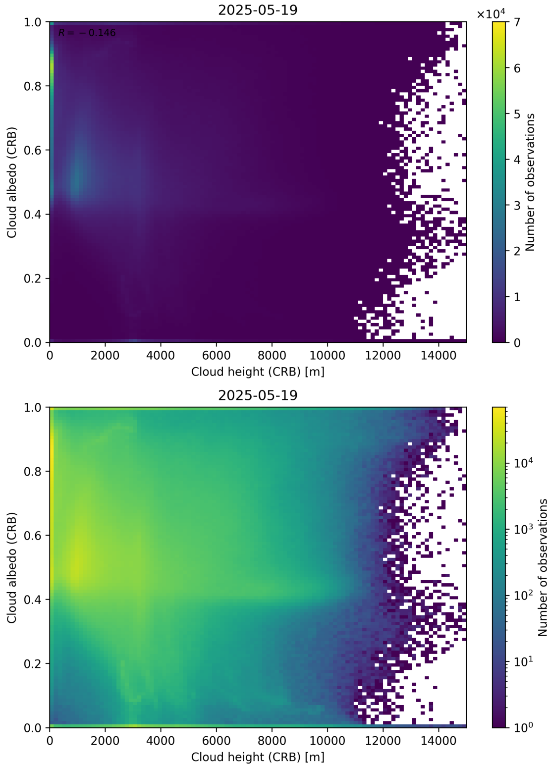
Figure 80: Scatter density plot of “Cloud height (CRB)” against “Cloud albedo (CRB)” for 2025-05-18 to 2025-05-20.
