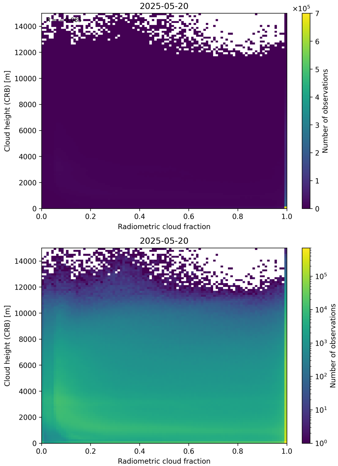
Figure 74: Scatter density plot of “Radiometric cloud fraction” against “Cloud height (CRB)” for 2025-05-19 to 2025-05-21.
