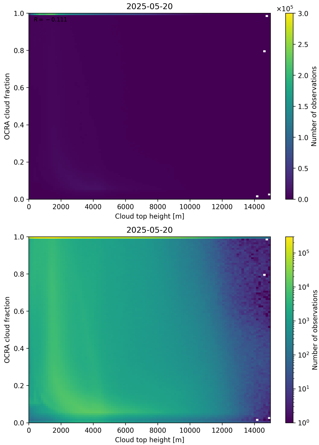
Figure 87: Scatter density plot of “Cloud top height” against “OCRA cloud fraction” for 2025-05-19 to 2025-05-21.
