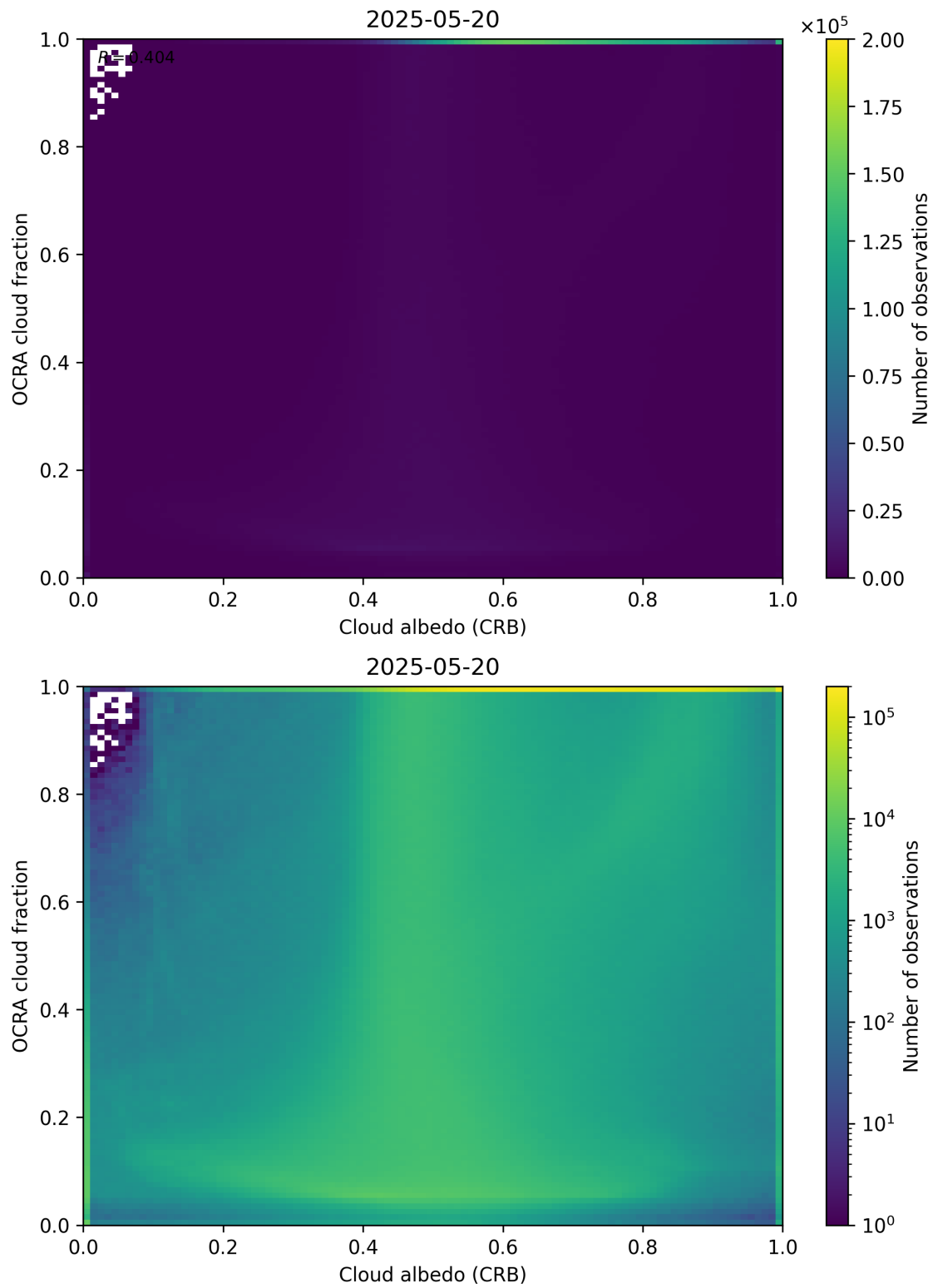
Figure 70: Scatter density plot of “Cloud albedo (CRB)” against “OCRA cloud fraction” for 2025-05-19 to 2025-05-21.
