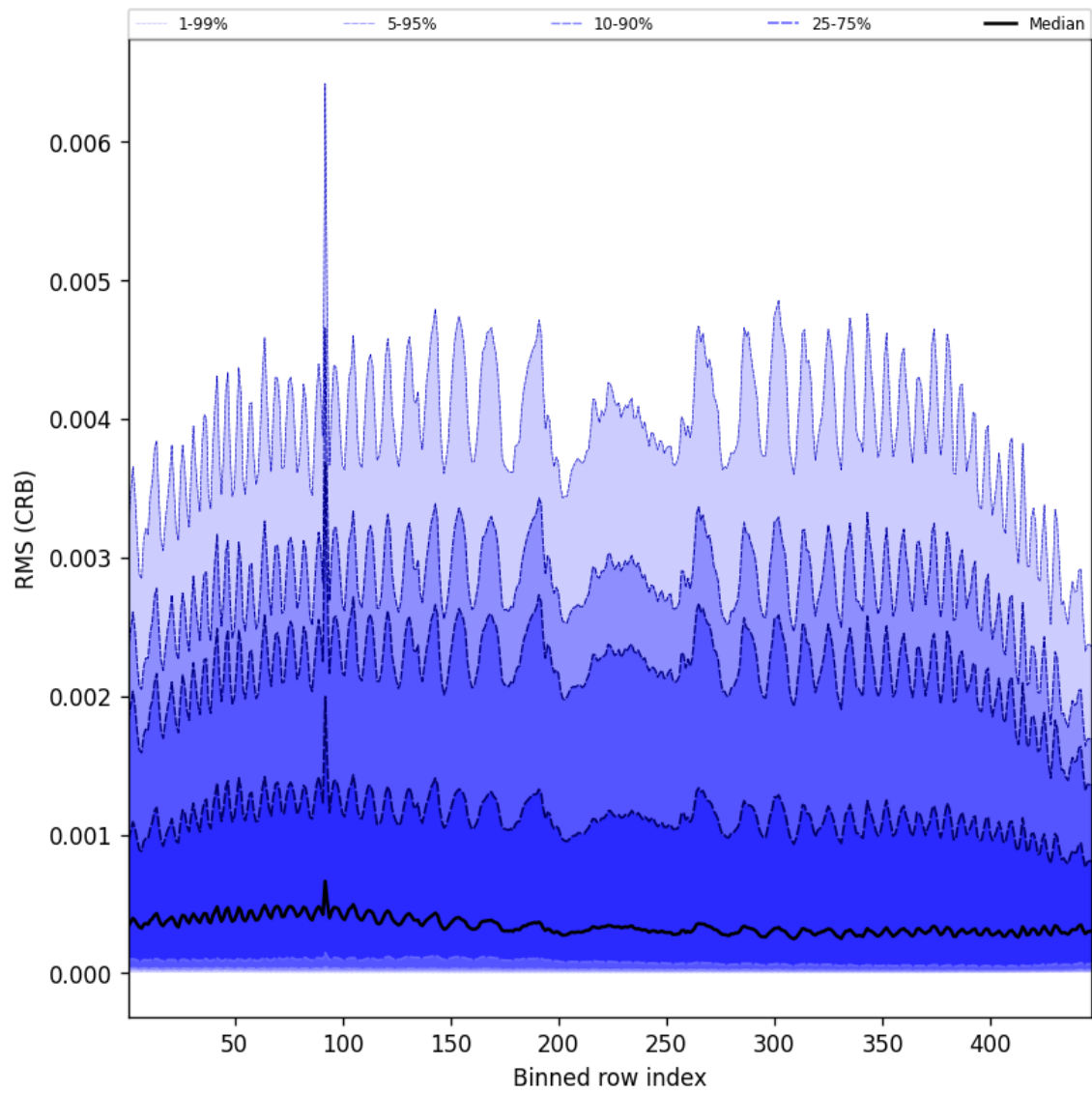
Figure 64: Along track statistics of “RMS (CRB)” for 2025-05-19 to 2025-05-21
