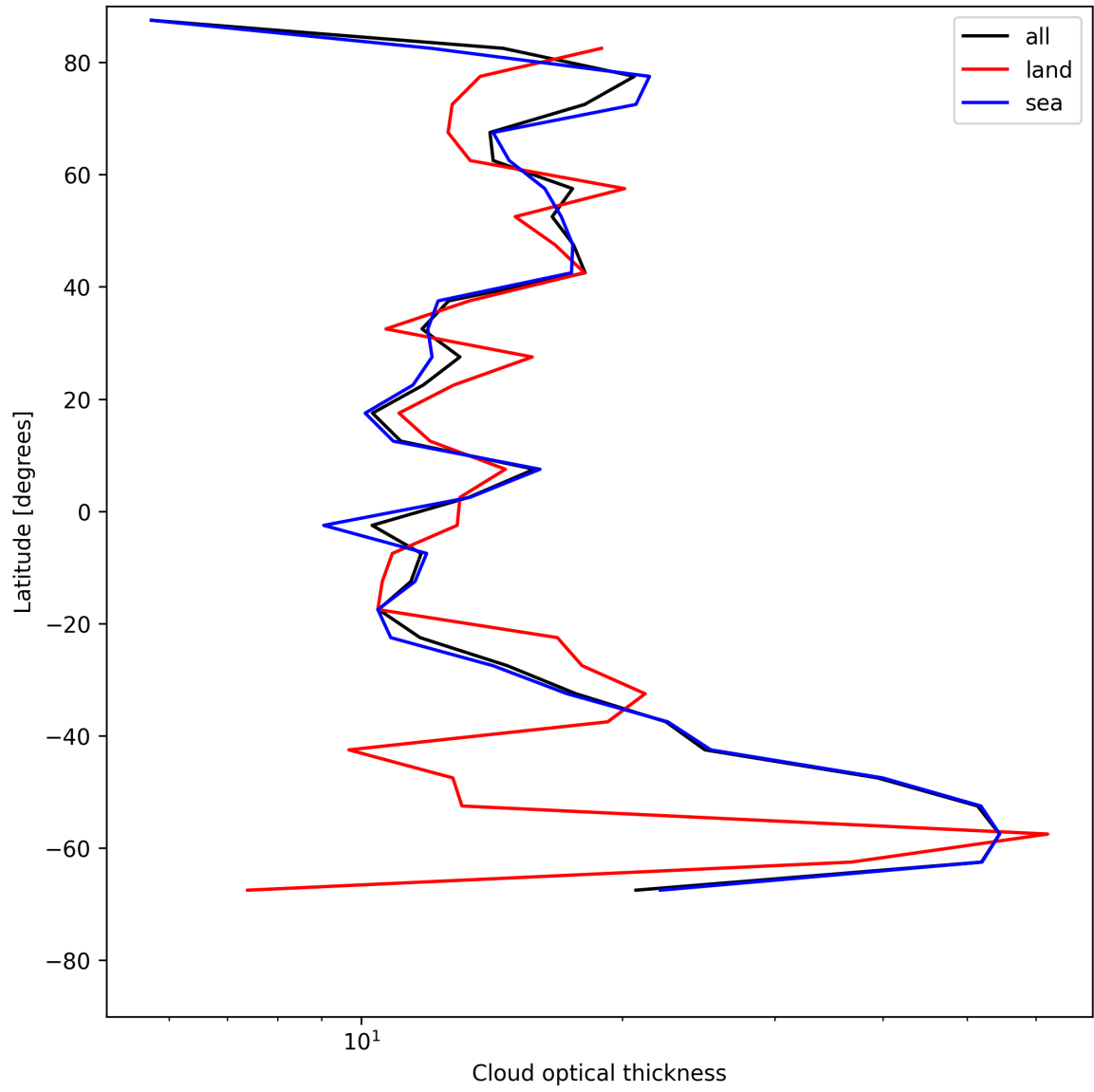
Figure 25: Zonal average of “Cloud optical thickness” for 2025-05-19 to 2025-05-21.
