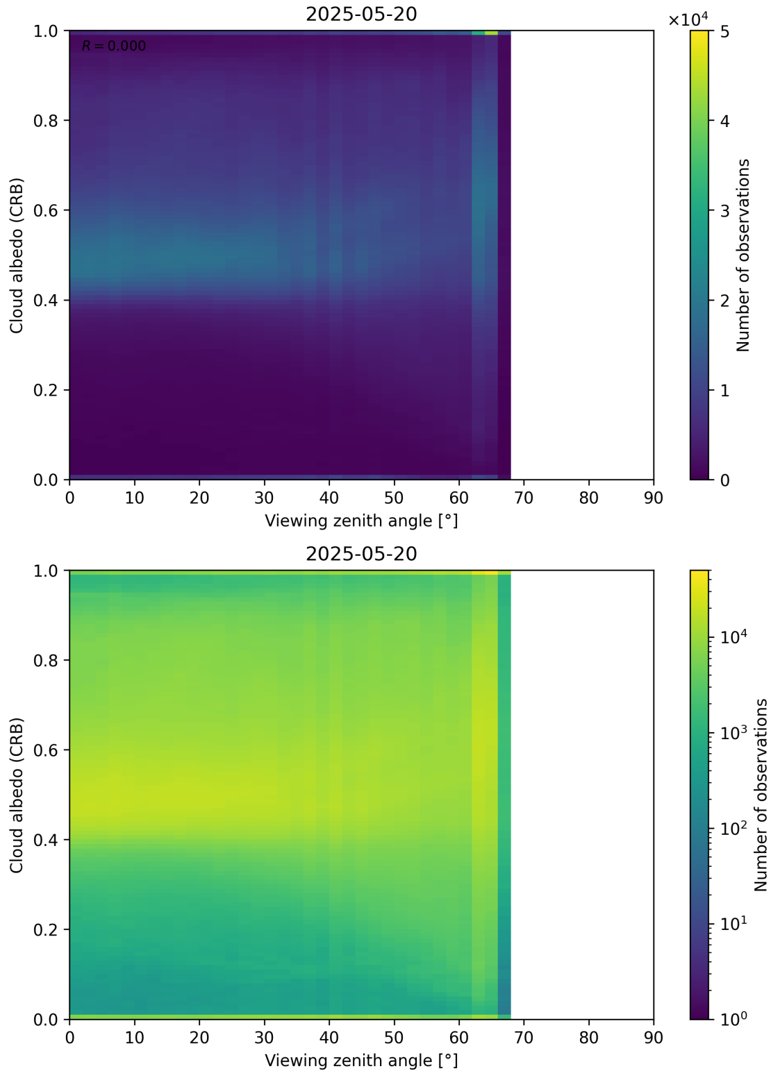
Figure 106: Scatter density plot of “Viewing zenith angle” against “Cloud albedo (CRB)” for 2025-05-19 to 2025-05-21.
