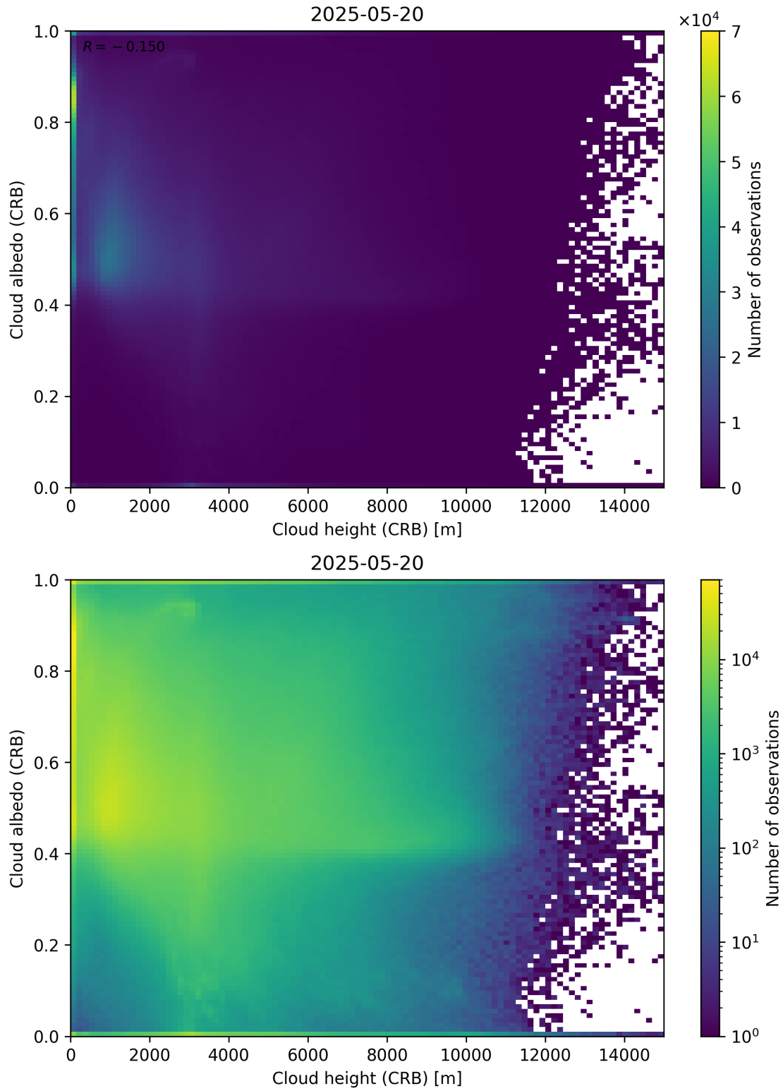
Figure 80: Scatter density plot of “Cloud height (CRB)” against “Cloud albedo (CRB)” for 2025-05-19 to 2025-05-21.
