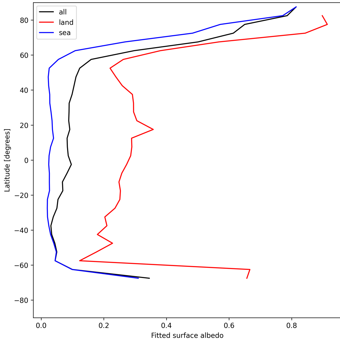
Figure 29: Zonal average of “Fitted surface albedo” for 2025-05-19 to 2025-05-21.
