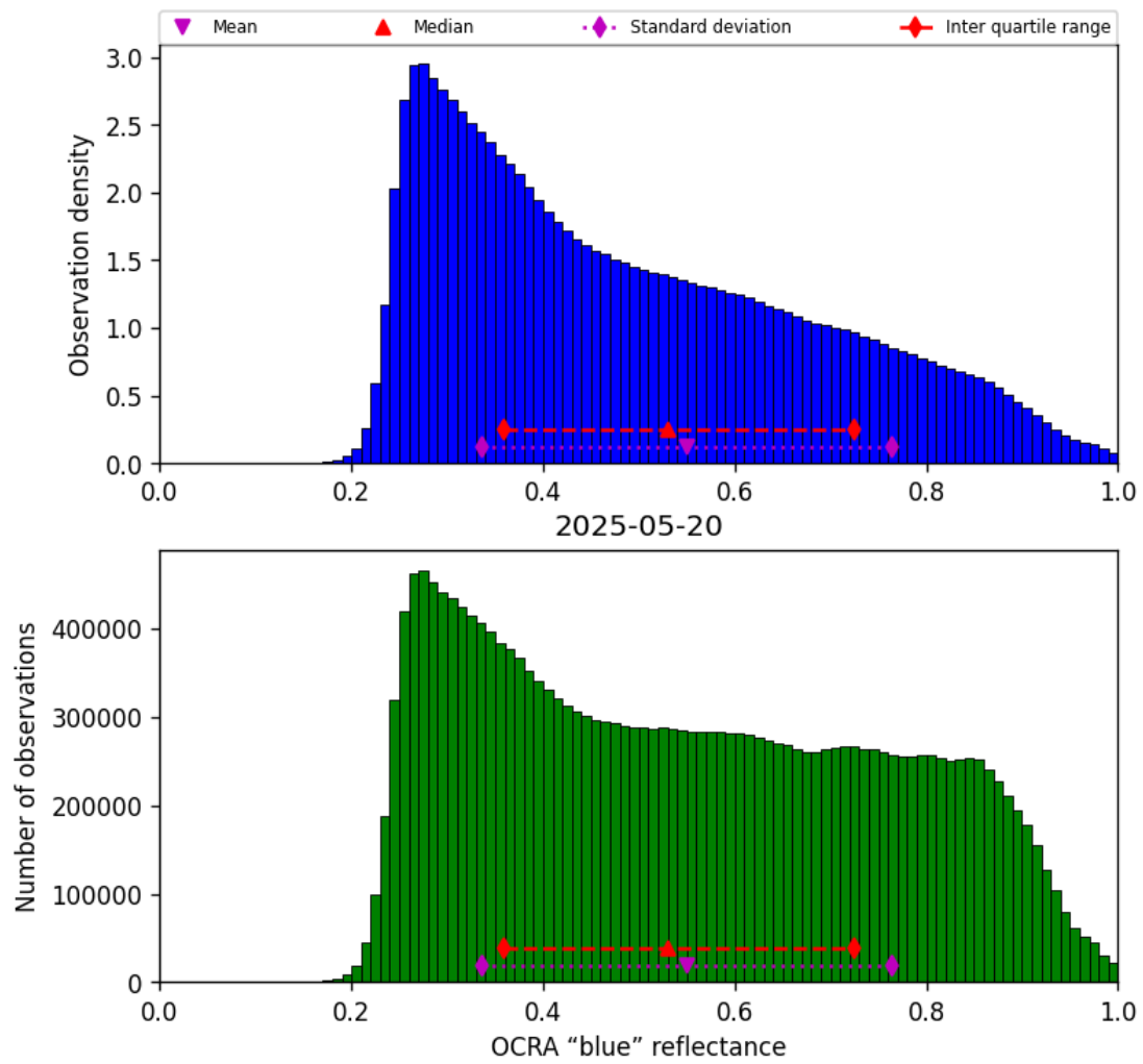
Figure 51: Histogram of “OCRA “blue” reflectance” for 2025-05-19 to 2025-05-21
