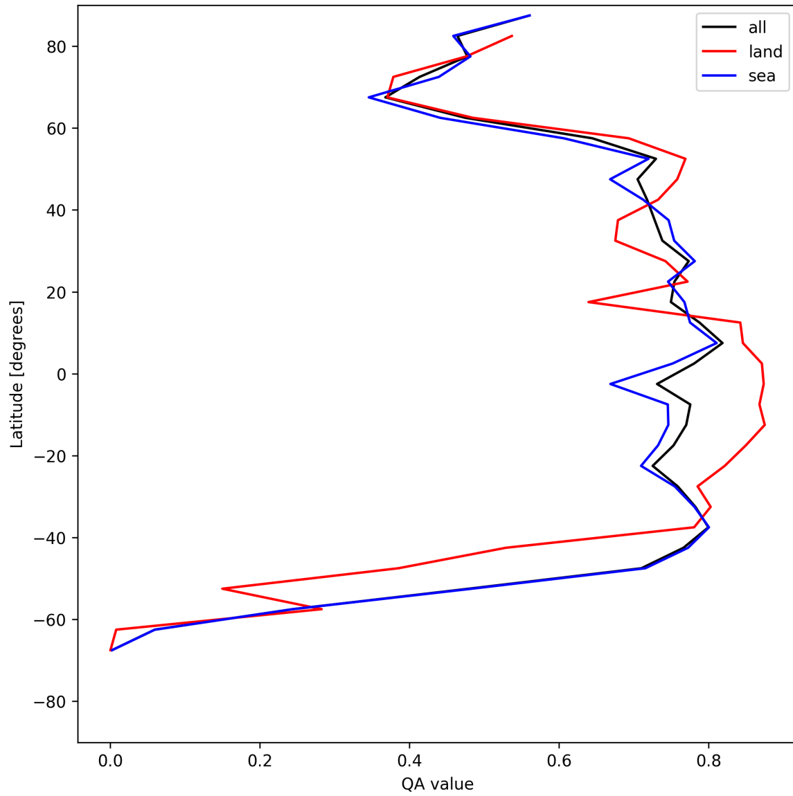
Figure 22: Zonal average of “QA value” for 2025-05-19 to 2025-05-21.
