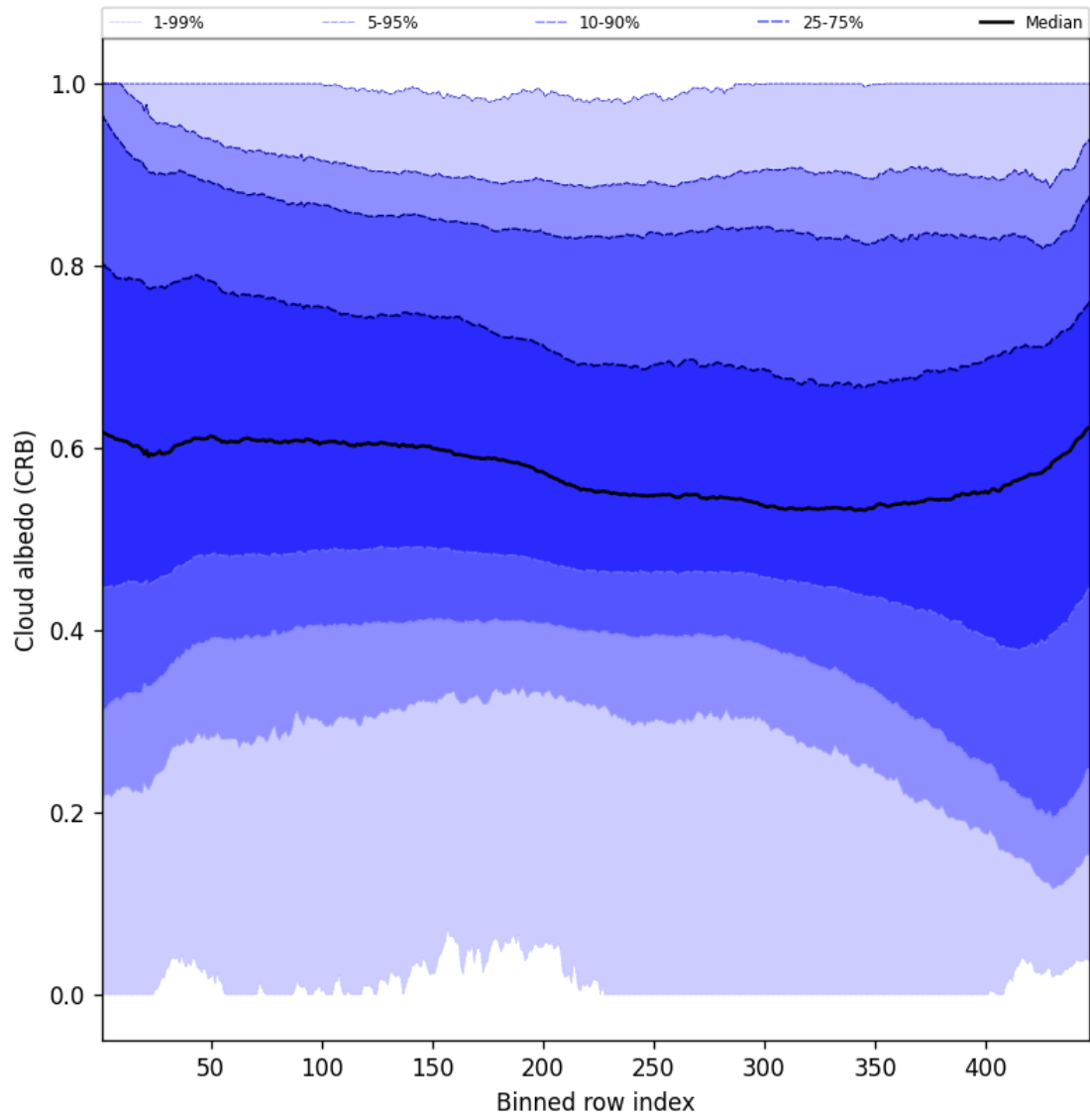
Figure 60: Along track statistics of “Cloud albedo (CRB)” for 2025-05-19 to 2025-05-21
