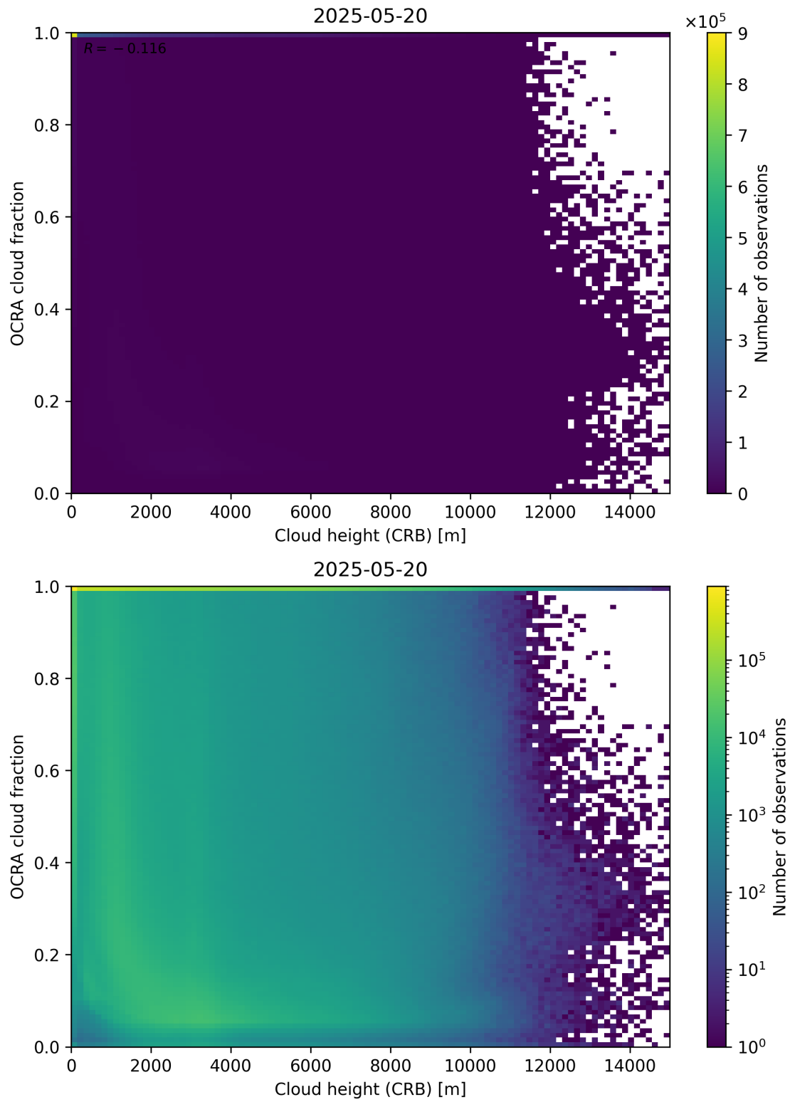
Figure 81: Scatter density plot of “Cloud height (CRB)” against “OCRA cloud fraction” for 2025-05-19 to 2025-05-21.
