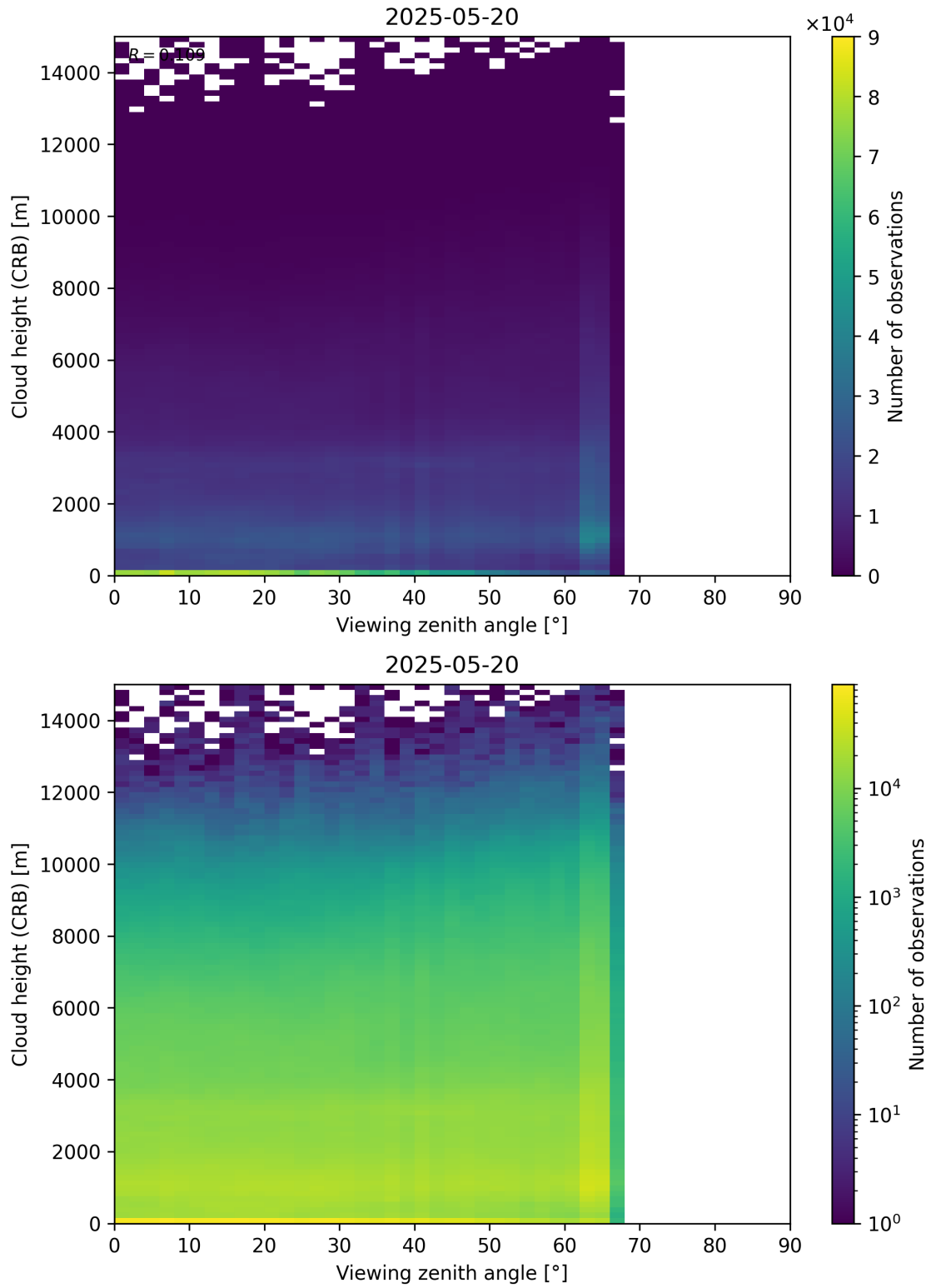
Figure 110: Scatter density plot of “Viewing zenith angle” against “Cloud height (CRB)” for 2025-05-19 to 2025-05-21.
