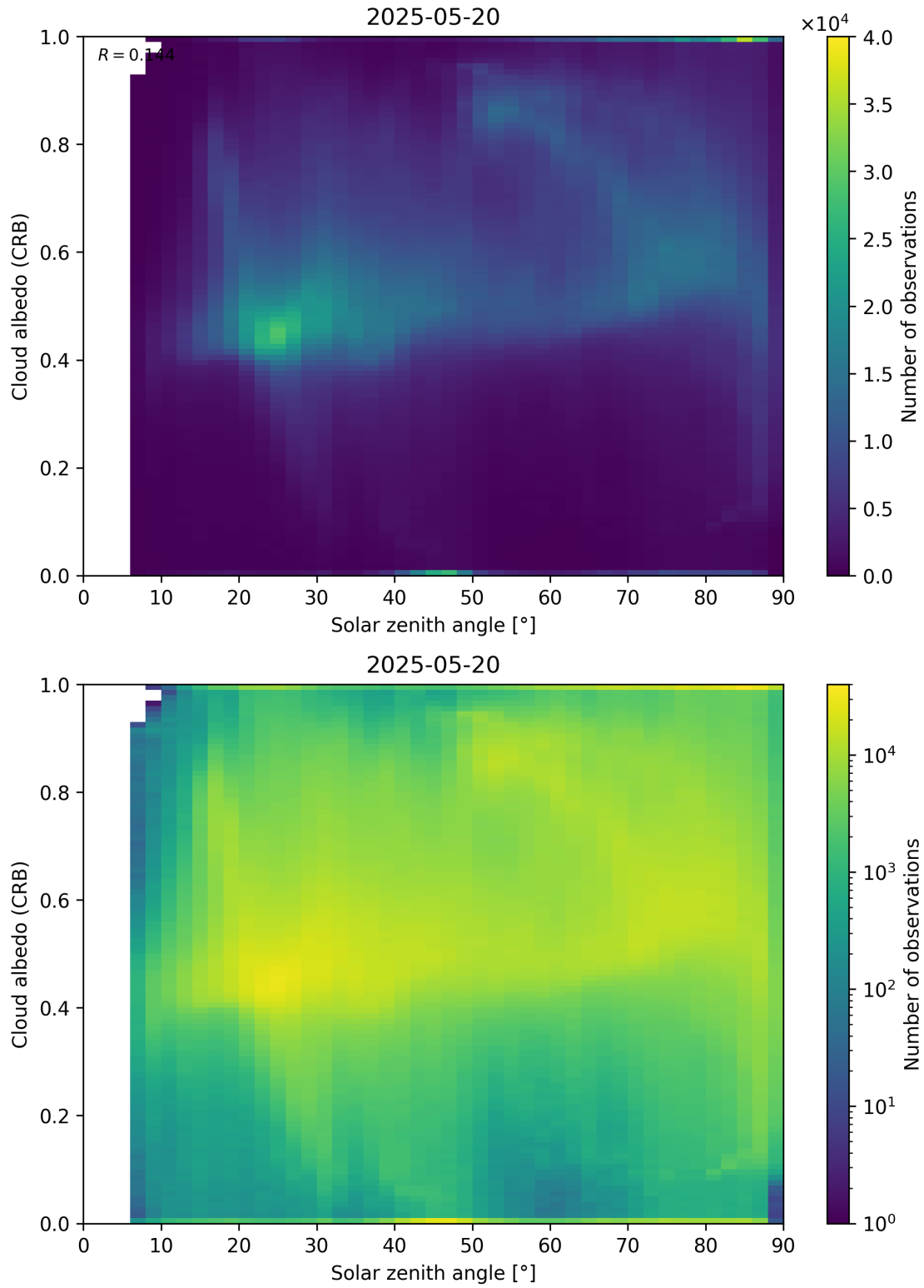
Figure 98: Scatter density plot of “Solar zenith angle” against “Cloud albedo (CRB)” for 2025-05-19 to 2025-05-21.
