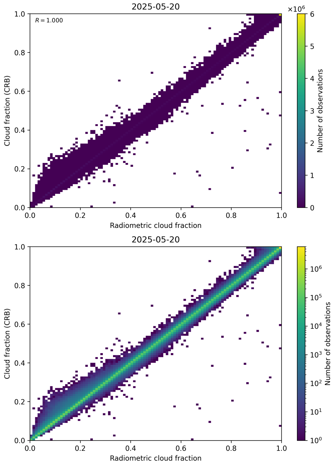
Figure 73: Scatter density plot of “Radiometric cloud fraction” against “Cloud fraction (CRB)” for 2025-05-19 to 2025-05-21.
