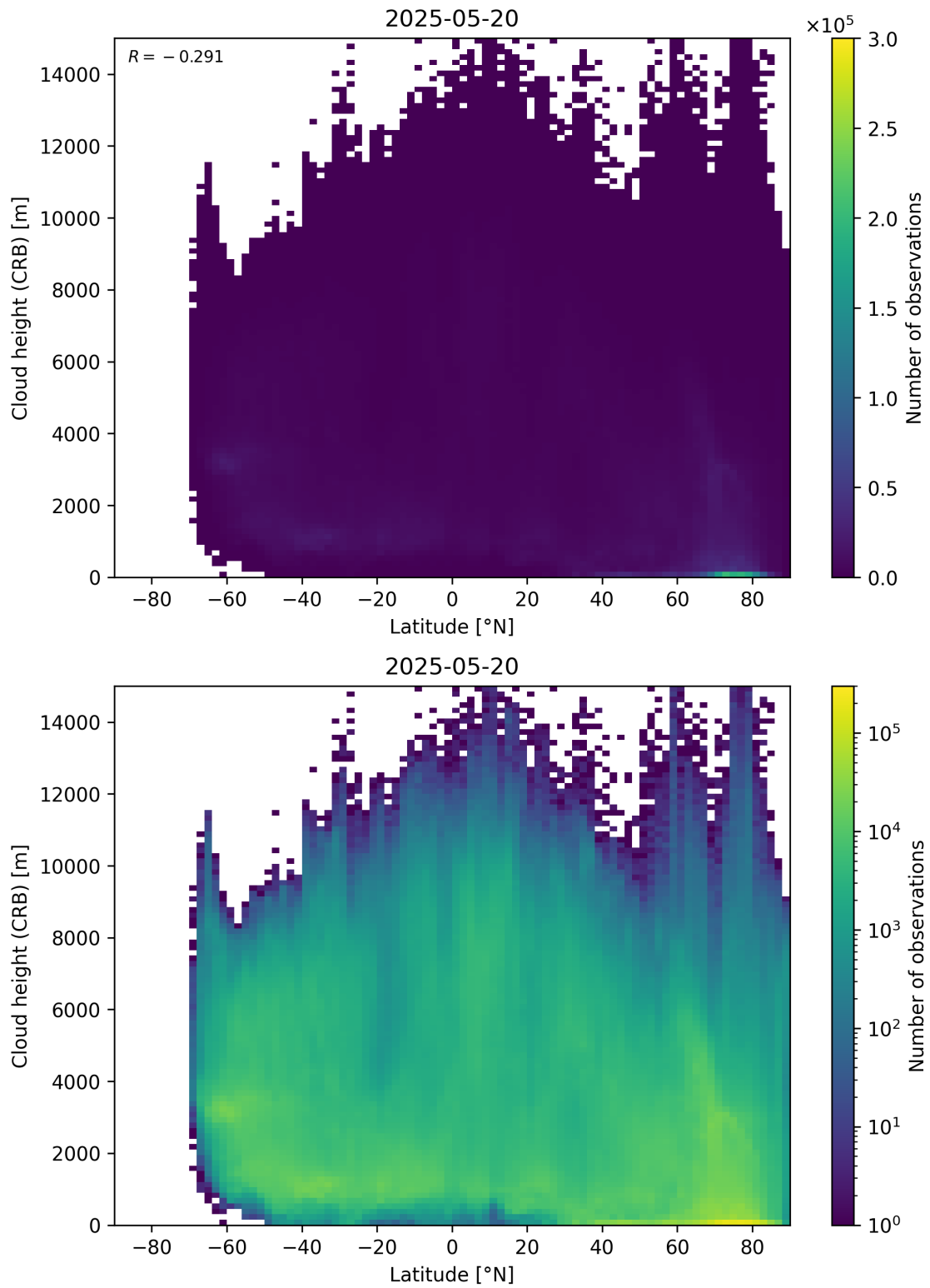
Figure 95: Scatter density plot of “Latitude” against “Cloud height (CRB)” for 2025-05-19 to 2025-05-21.
