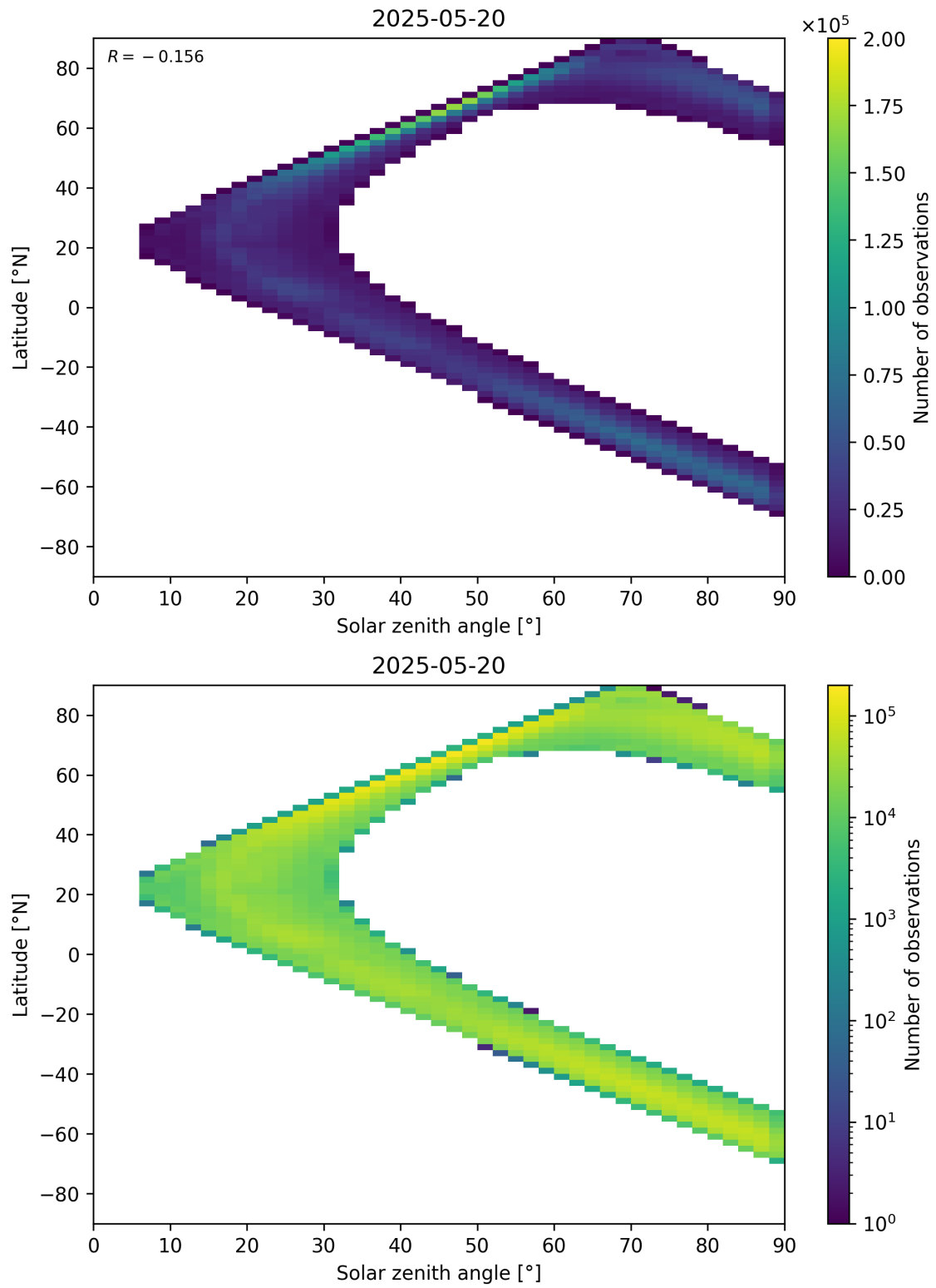
Figure 105: Scatter density plot of “Solar zenith angle” against “Latitude” for 2025-05-19 to 2025-05-21.
