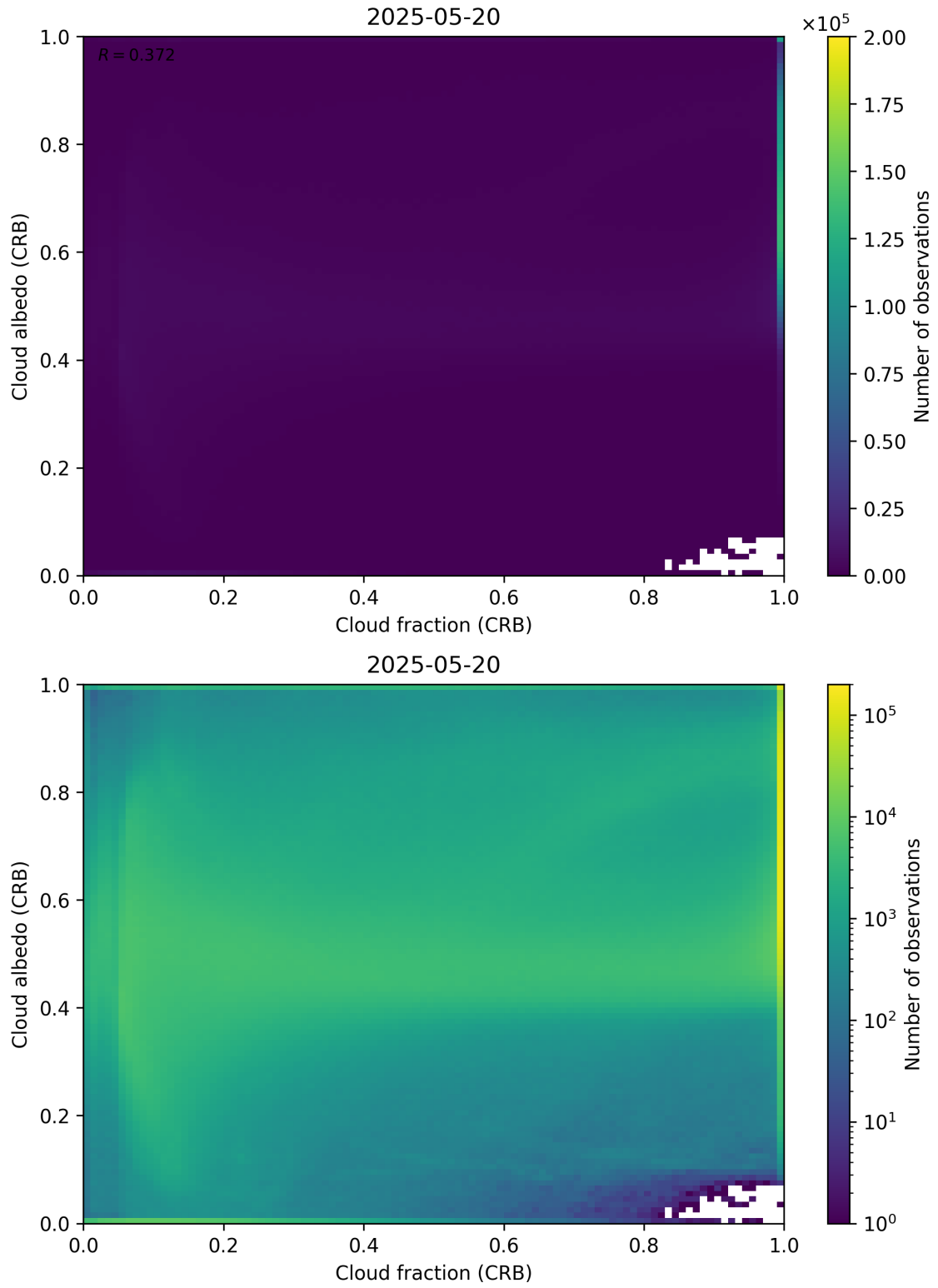
Figure 77: Scatter density plot of “Cloud fraction (CRB)” against “Cloud albedo (CRB)” for 2025-05-19 to 2025-05-21.
