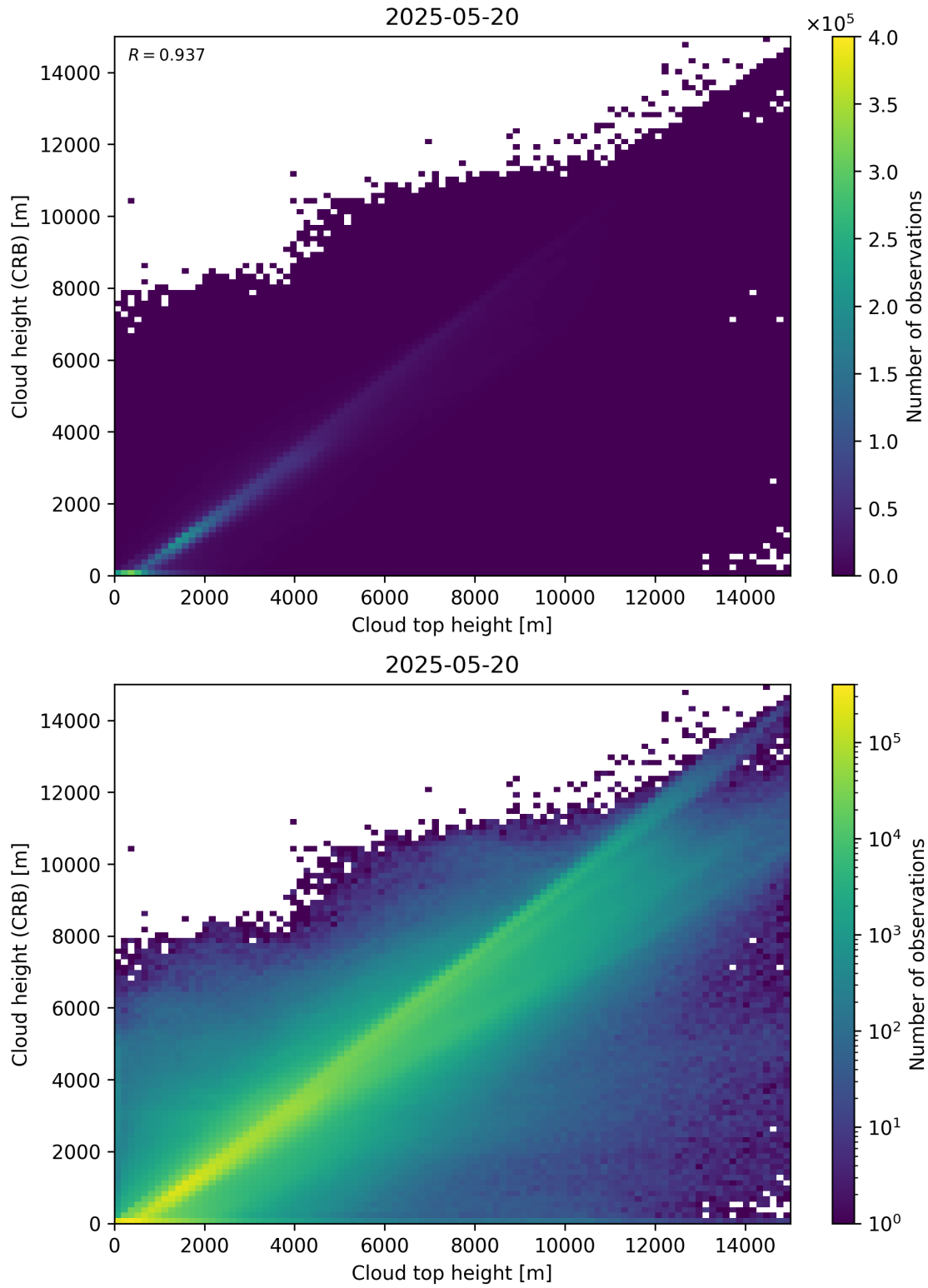
Figure 89: Scatter density plot of “Cloud top height” against “Cloud height (CRB)” for 2025-05-19 to 2025-05-21.
