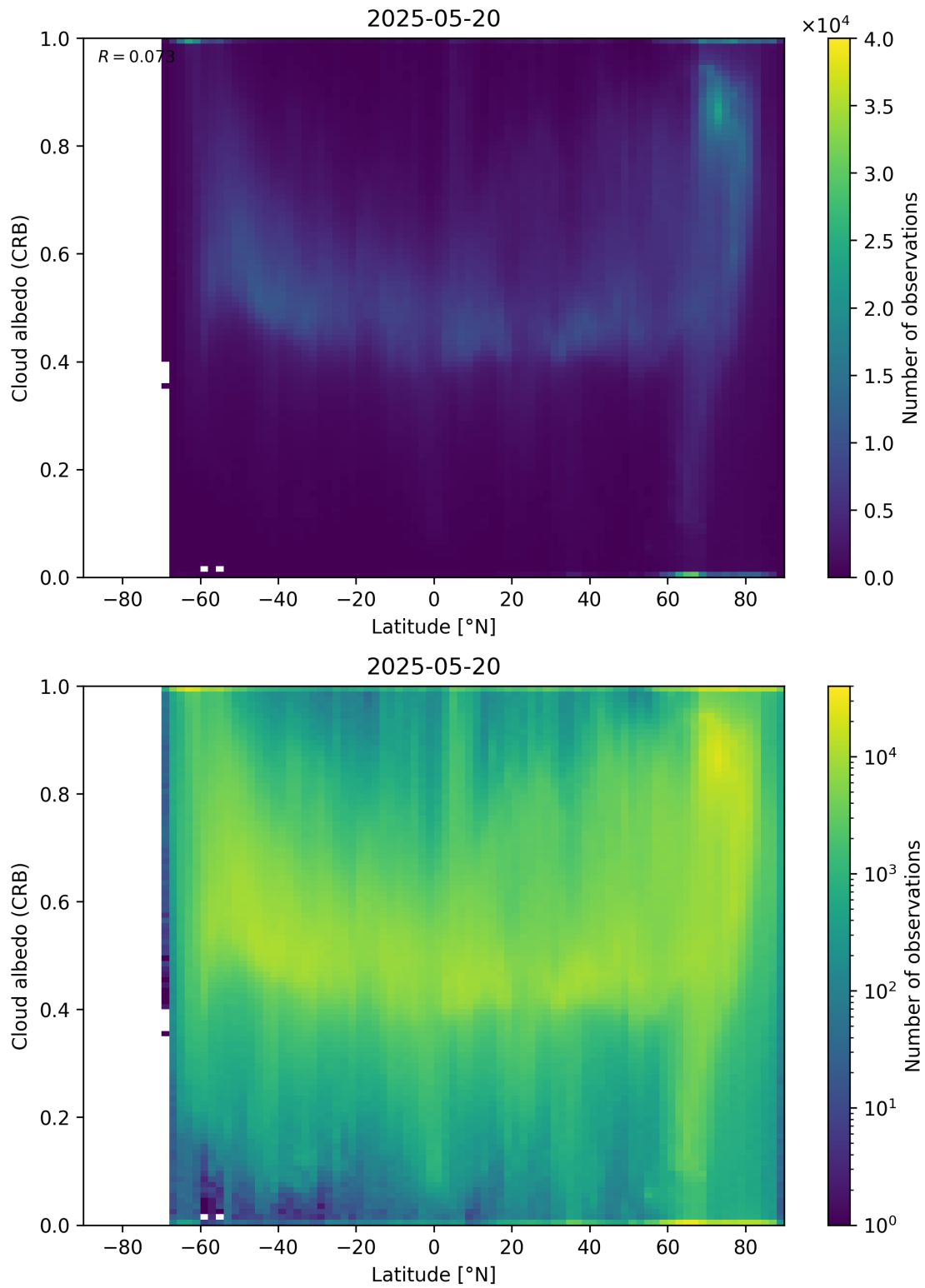
Figure 91: Scatter density plot of “Latitude” against “Cloud albedo (CRB)” for 2025-05-19 to 2025-05-21.
