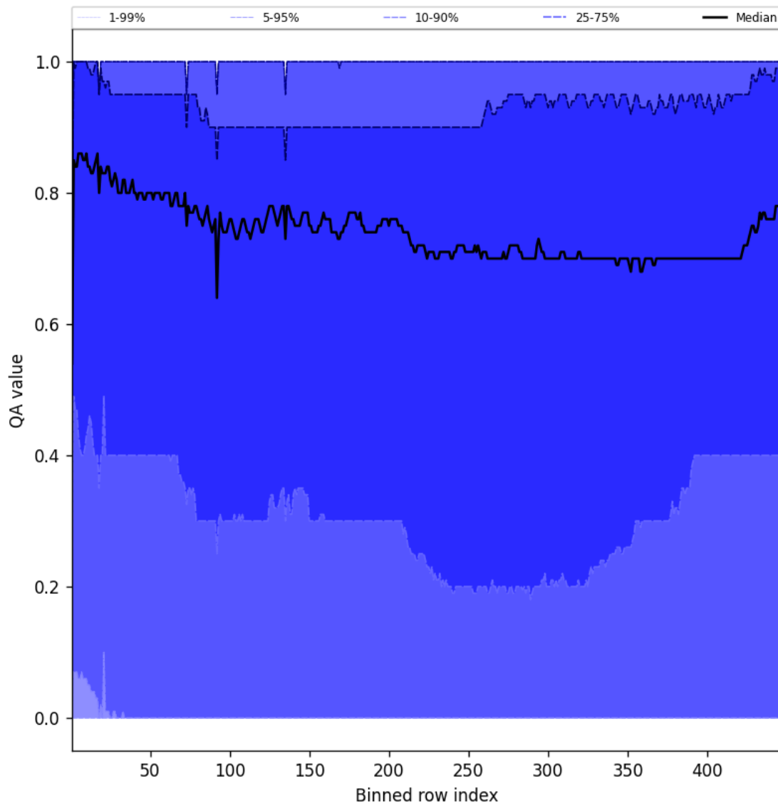
Figure 54: Along track statistics of “QA value” for 2025-05-19 to 2025-05-21
