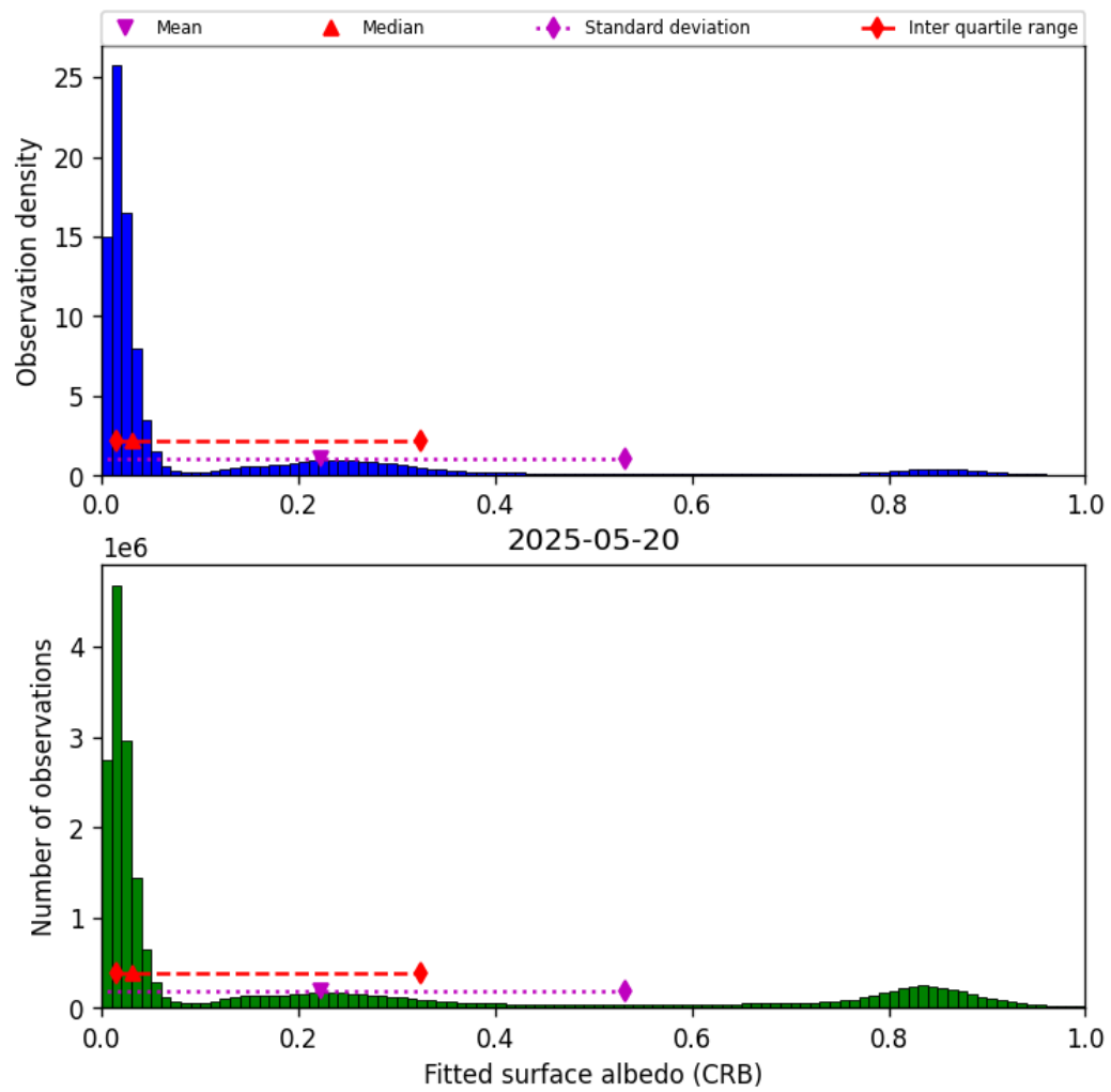
Figure 46: Histogram of “Fitted surface albedo (CRB)” for 2025-05-19 to 2025-05-21
