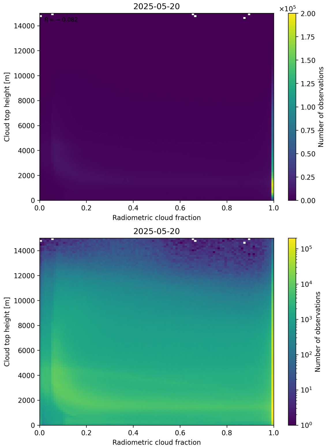
Figure 76: Scatter density plot of “Radiometric cloud fraction” against “Cloud top height” for 2025-05-19 to 2025-05-21.
