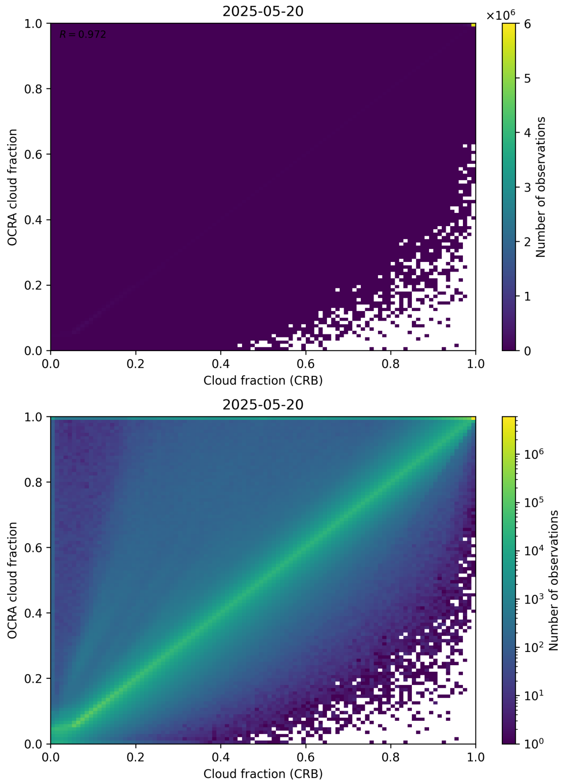
Figure 78: Scatter density plot of “Cloud fraction (CRB)” against “OCRA cloud fraction” for 2025-05-19 to 2025-05-21.
