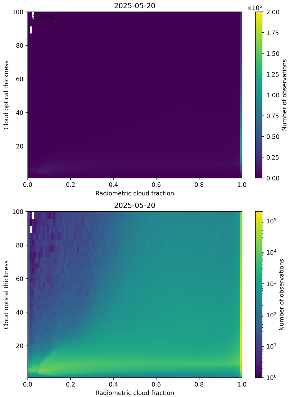
Figure 75: Scatter density plot of “Radiometric cloud fraction” against “Cloud optical thickness” for 2025-05-19 to 2025-05-21.
