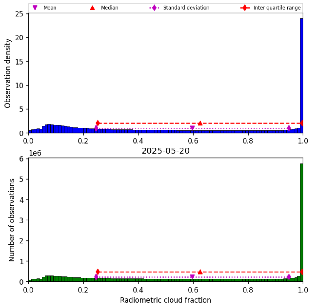
Figure 39: Histogram of “Radiometric cloud fraction” for 2025-05-19 to 2025-05-21
