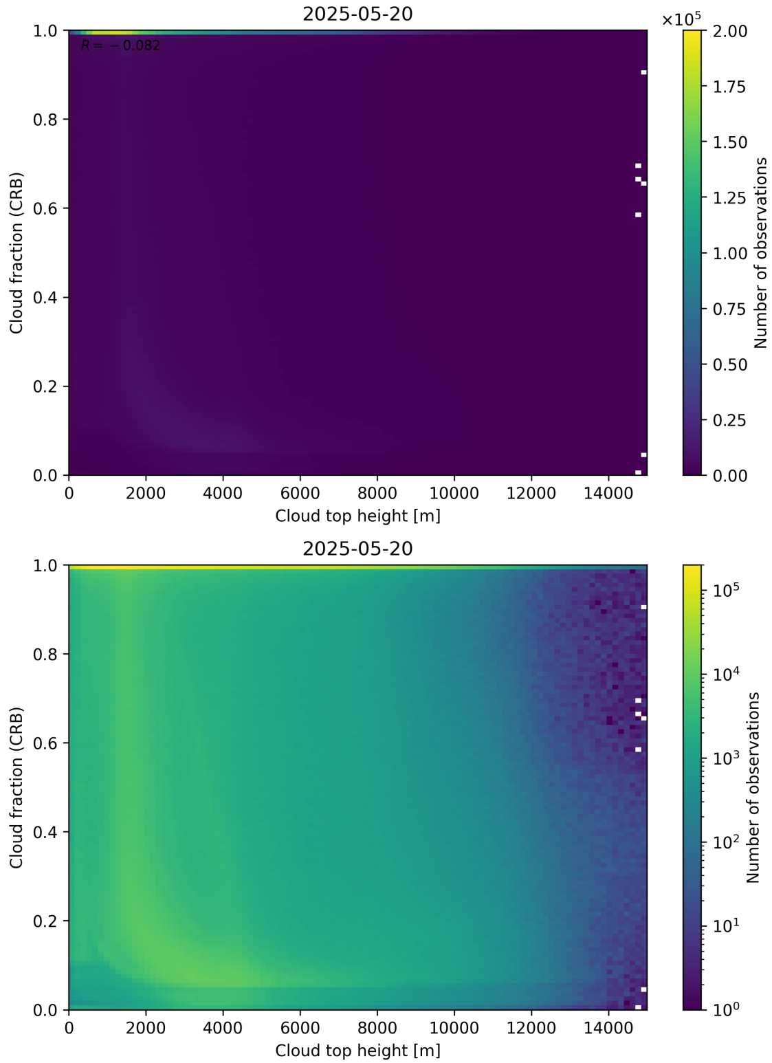
Figure 88: Scatter density plot of “Cloud top height” against “Cloud fraction (CRB)” for 2025-05-19 to 2025-05-21.
