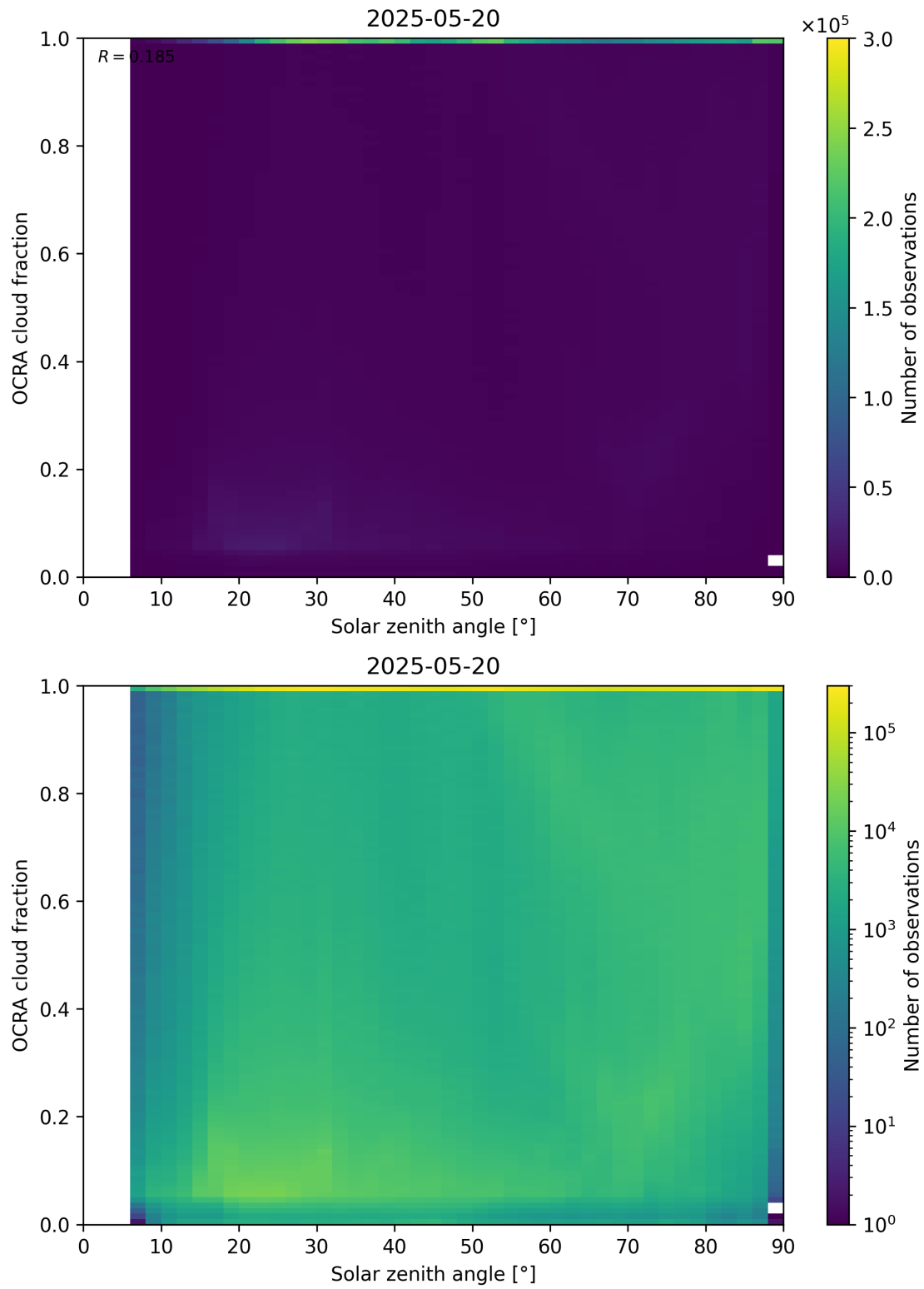
Figure 100: Scatter density plot of “Solar zenith angle” against “OCRA cloud fraction” for 2025-05-19 to 2025-05-21.
