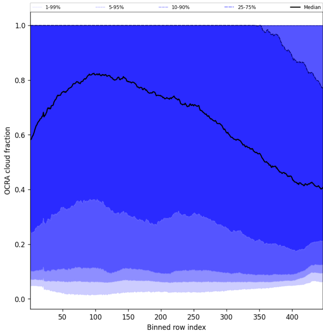
Figure 66: Along track statistics of “OCRA cloud fraction” for 2025-05-19 to 2025-05-21
