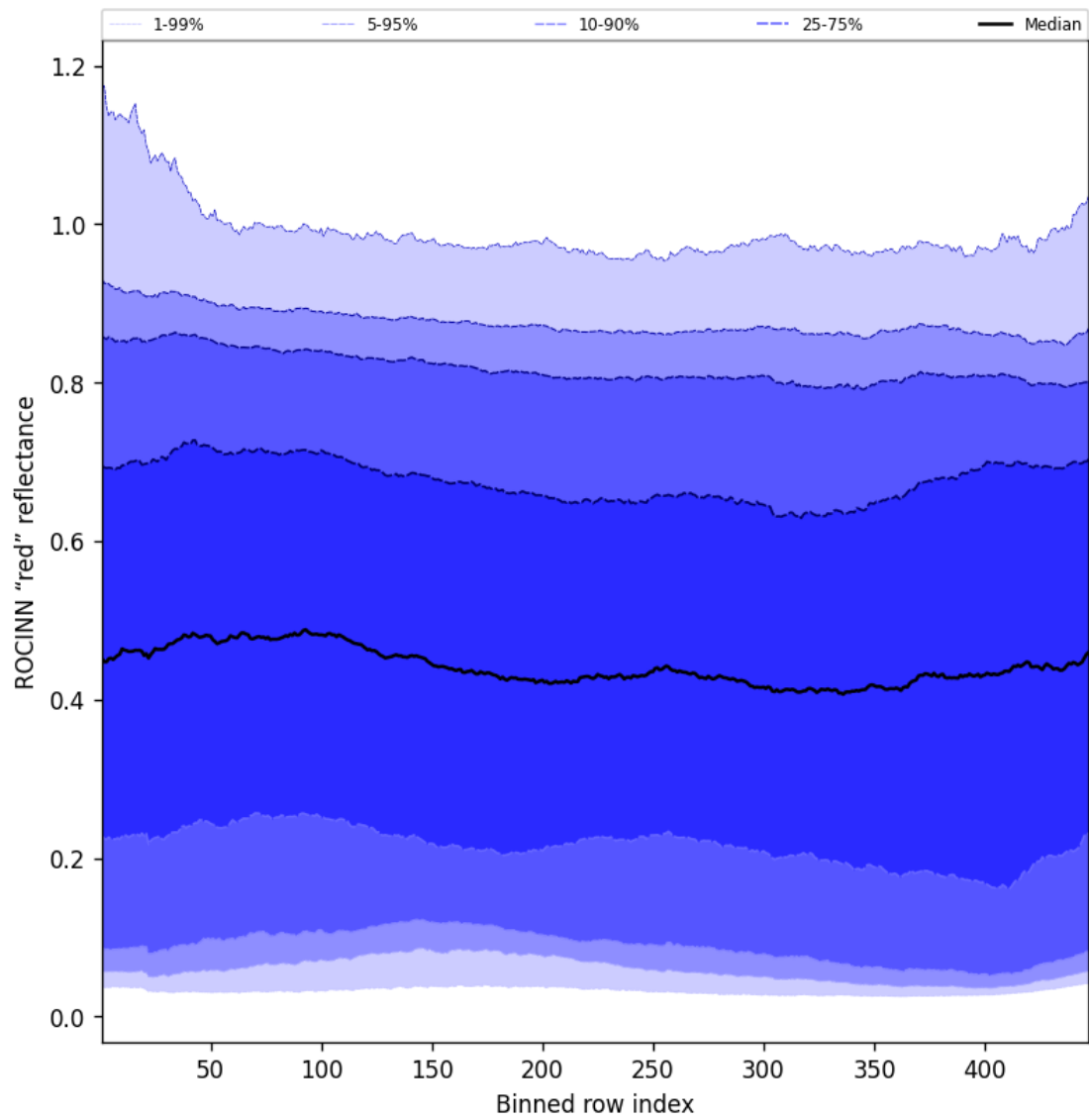
Figure 69: Along track statistics of “ROCINN “red” reflectance” for 2025-05-19 to 2025-05-21
