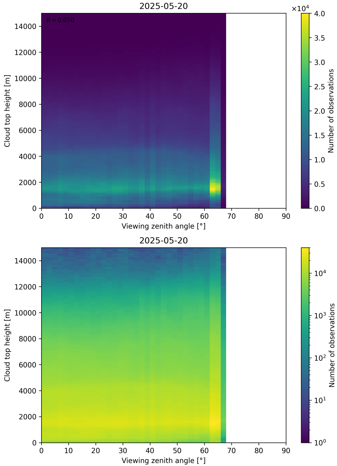
Figure 112: Scatter density plot of “Viewing zenith angle” against “Cloud top height” for 2025-05-19 to 2025-05-21.
