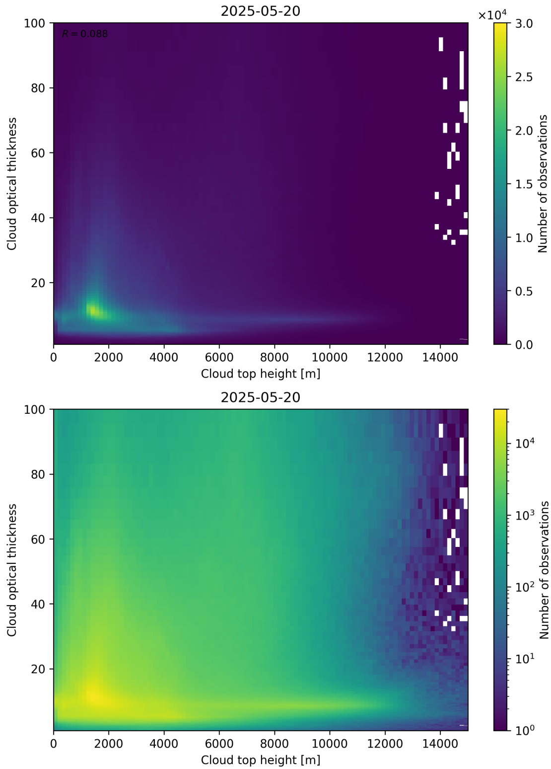
Figure 90: Scatter density plot of “Cloud top height” against “Cloud optical thickness” for 2025-05-19 to 2025-05-21.
