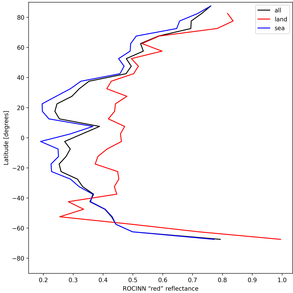
Figure 37: Zonal average of “ROCINN “red” reflectance” for 2025-05-19 to 2025-05-21.
