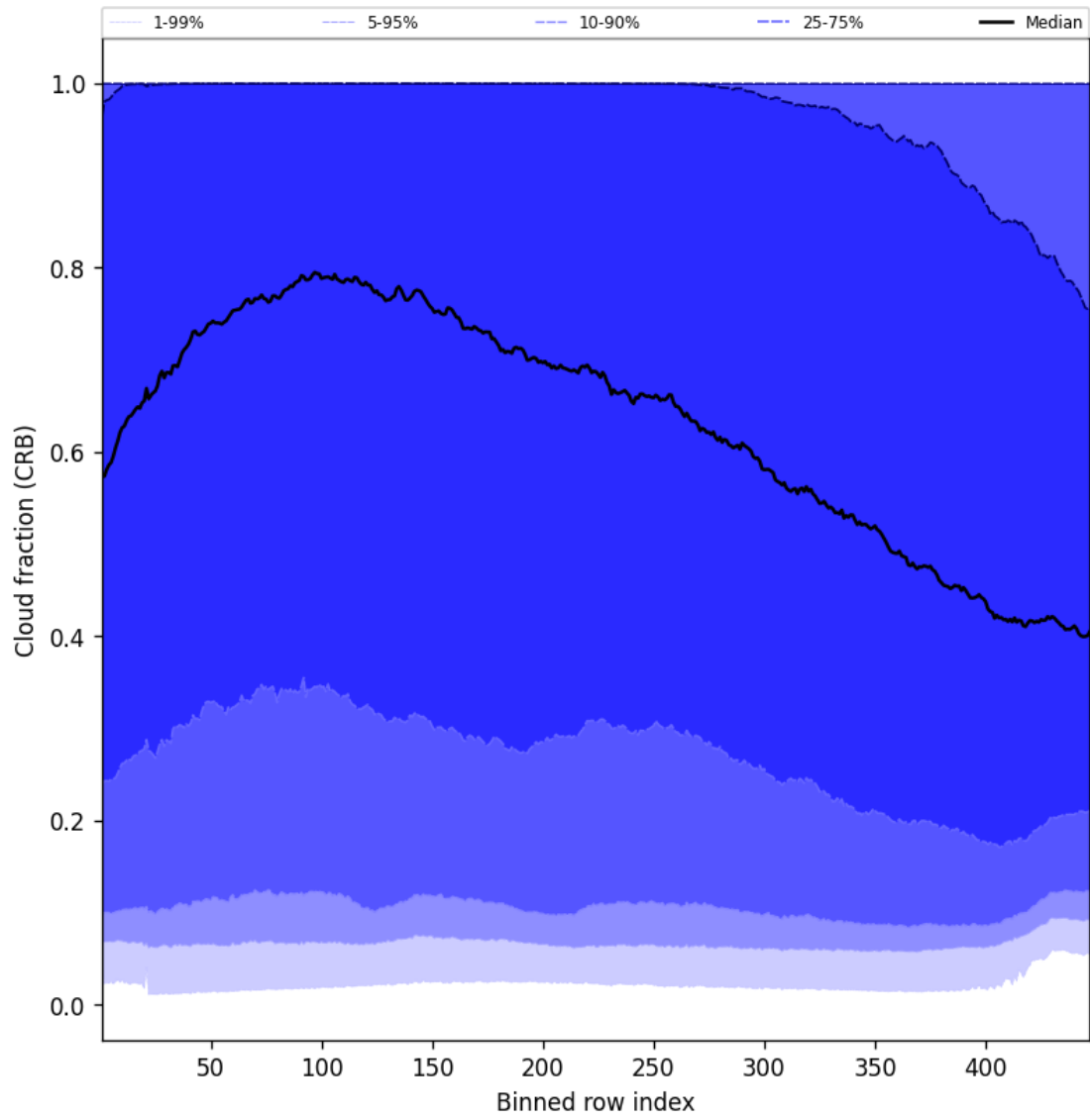
Figure 58: Along track statistics of “Cloud fraction (CRB)” for 2025-05-19 to 2025-05-21
