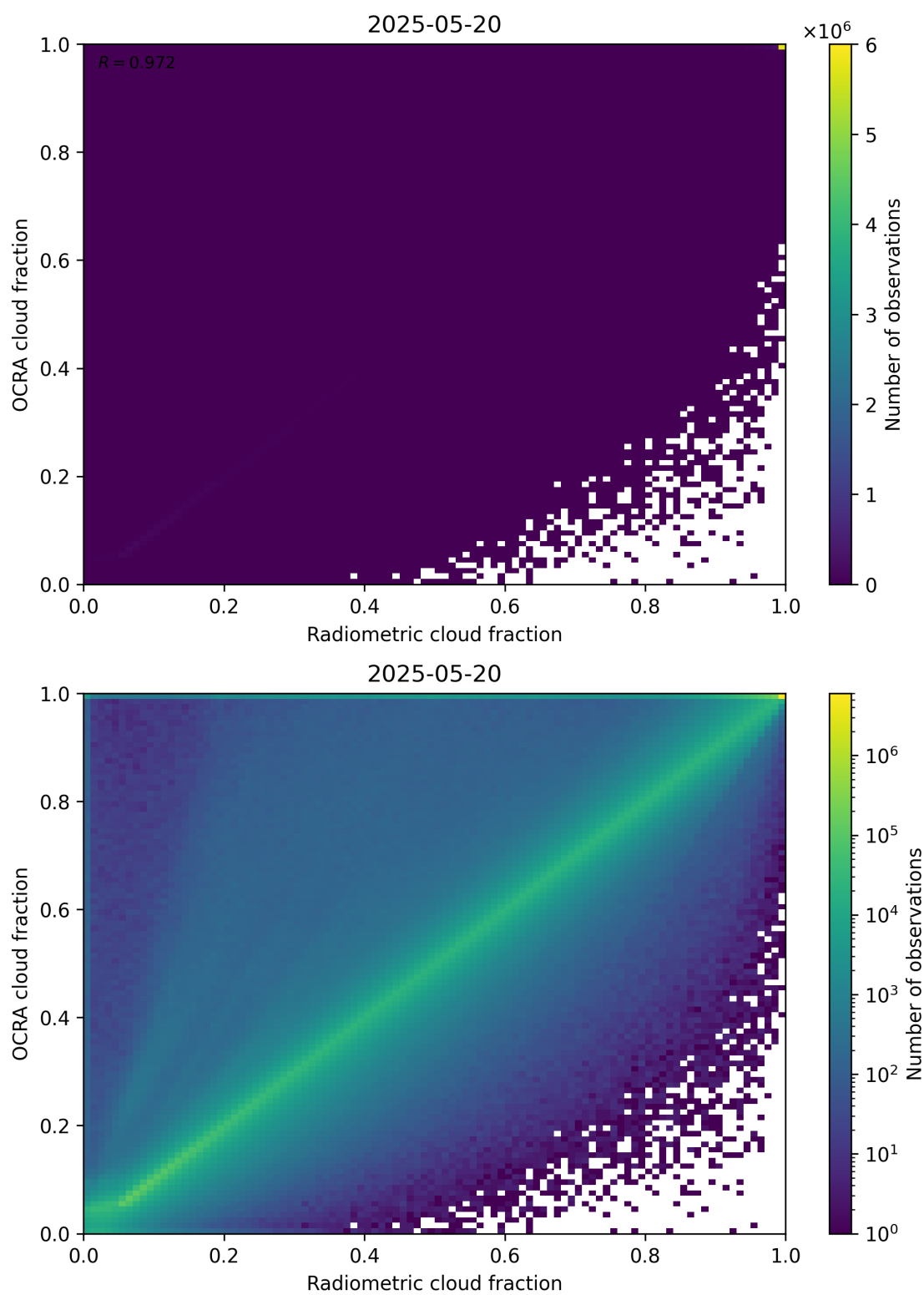
Figure 72: Scatter density plot of “Radiometric cloud fraction” against “OCRA cloud fraction” for 2025-05-19 to 2025-05-21.
