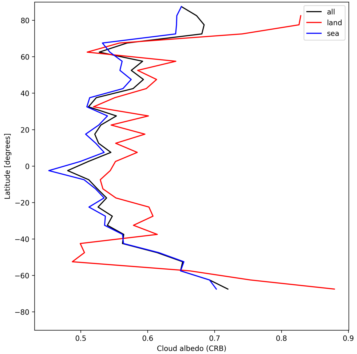
Figure 28: Zonal average of “Cloud albedo (CRB)” for 2025-05-19 to 2025-05-21.
