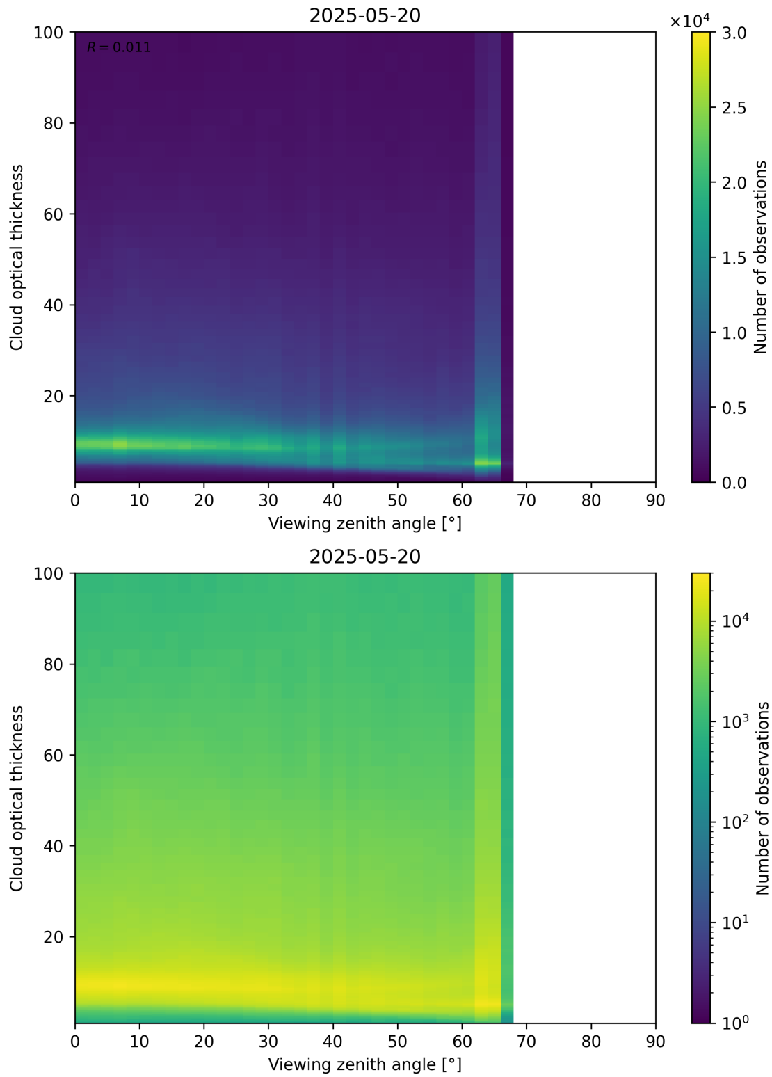
Figure 111: Scatter density plot of “Viewing zenith angle” against “Cloud optical thickness” for 2025-05-19 to 2025-05-21.
