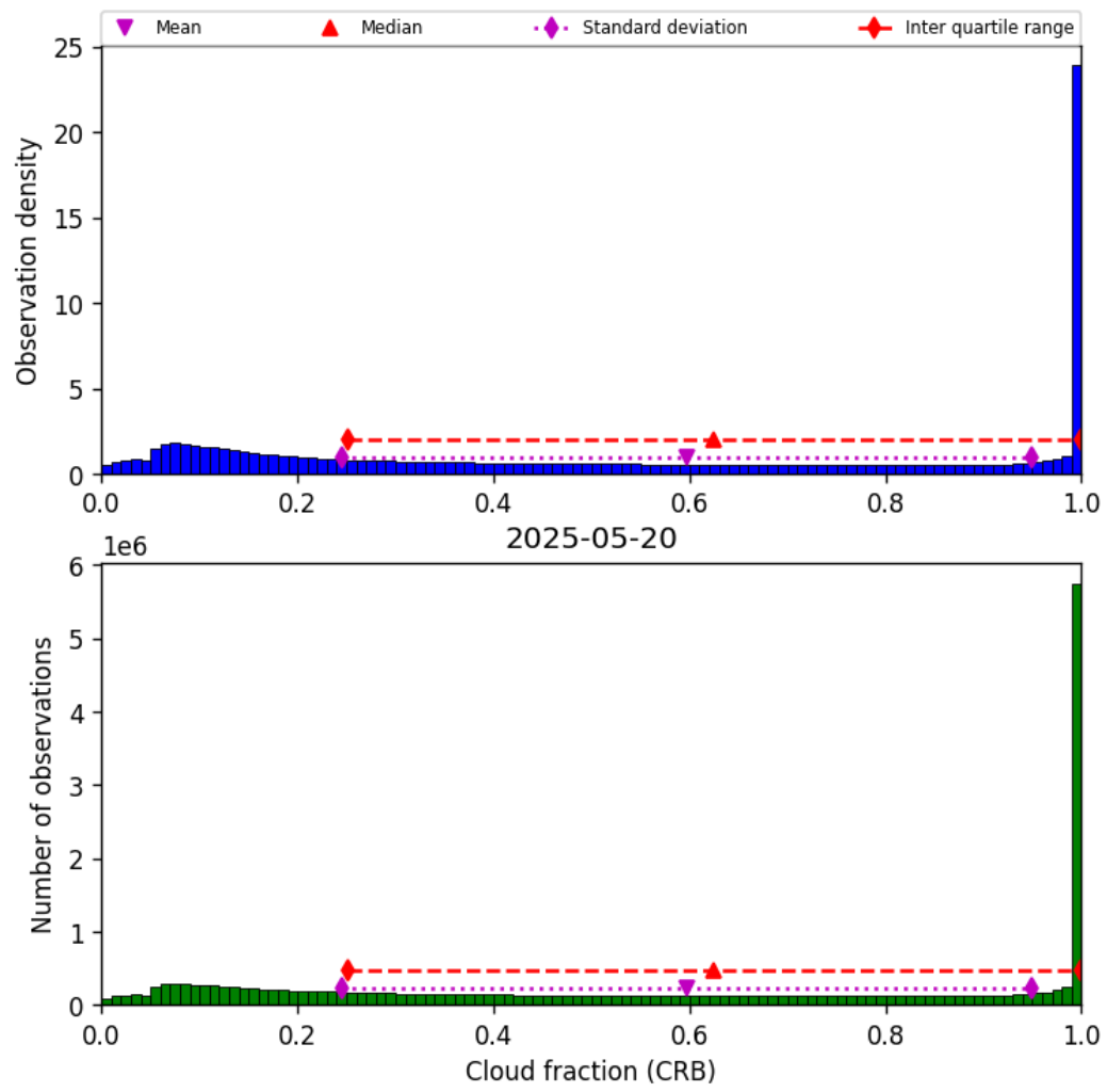
Figure 42: Histogram of “Cloud fraction (CRB)” for 2025-05-19 to 2025-05-21
