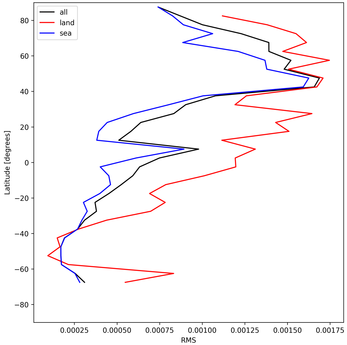
Figure 31: Zonal average of “RMS” for 2025-05-19 to 2025-05-21.
