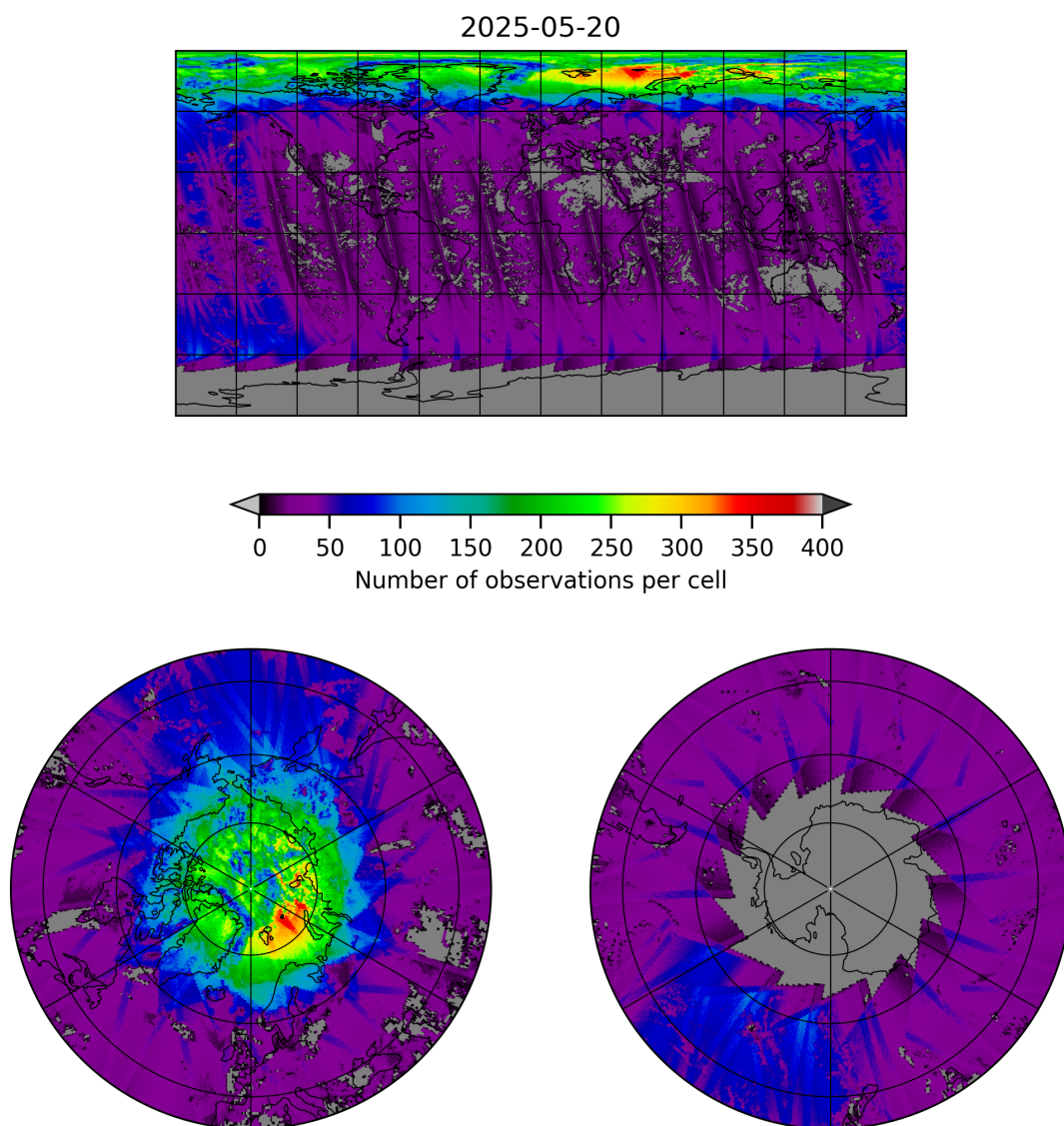
Figure 21: Map of the number of observations for 2025-05-19 to 2025-05-21
