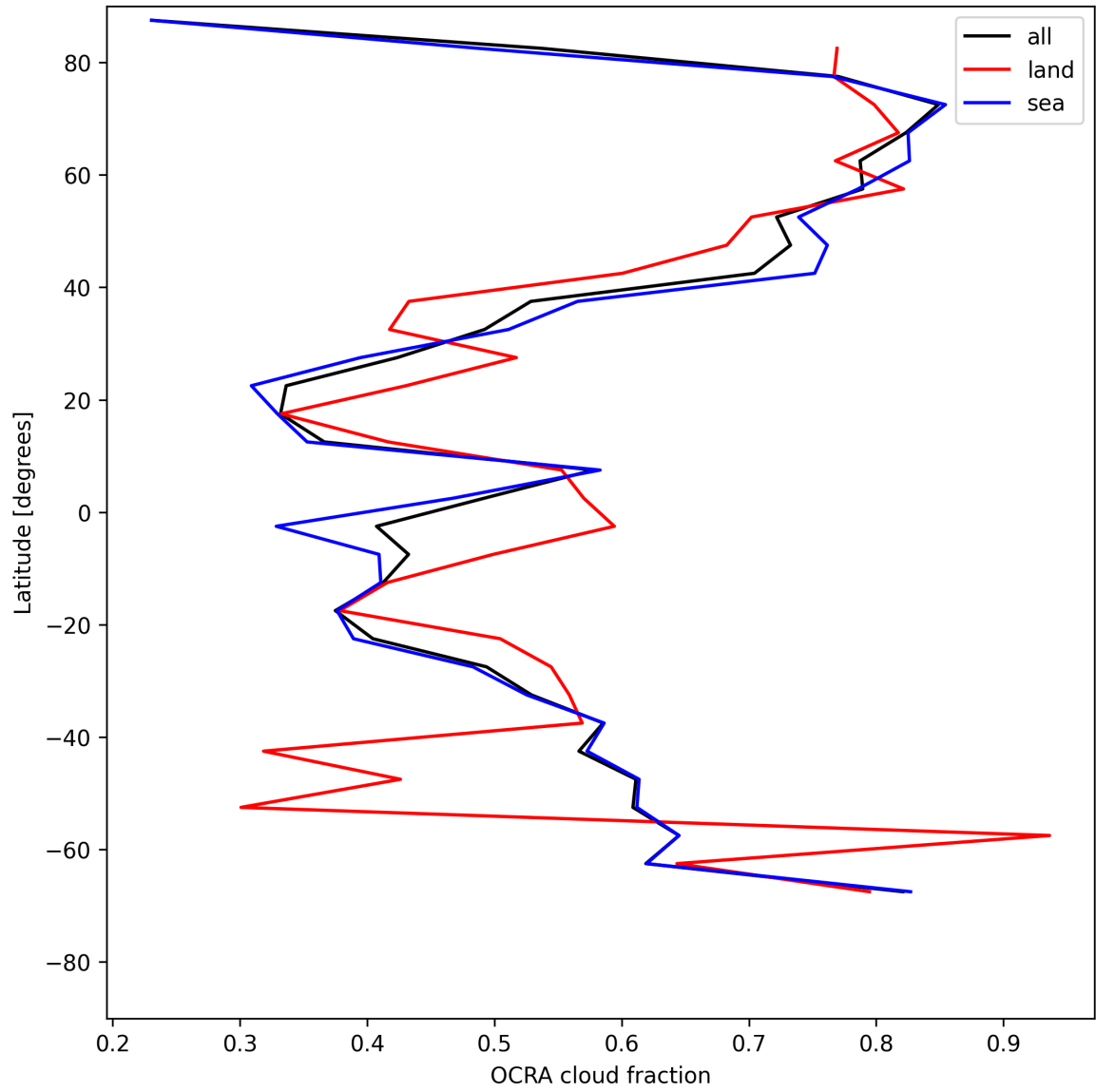
Figure 34: Zonal average of “OCRA cloud fraction” for 2025-05-19 to 2025-05-21.
