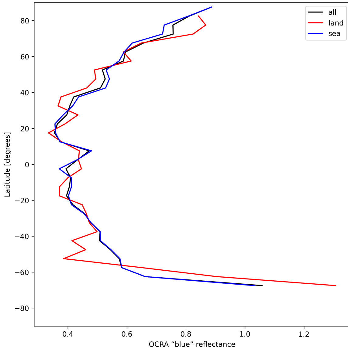
Figure 35: Zonal average of “OCRA “blue” reflectance” for 2025-05-19 to 2025-05-21.
