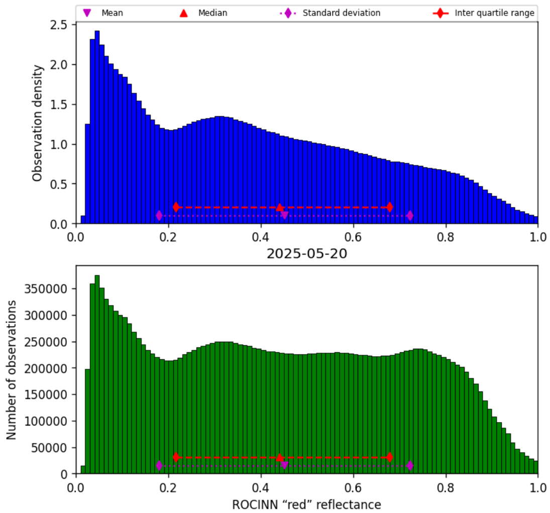
Figure 53: Histogram of “ROCINN “red” reflectance” for 2025-05-19 to 2025-05-21
