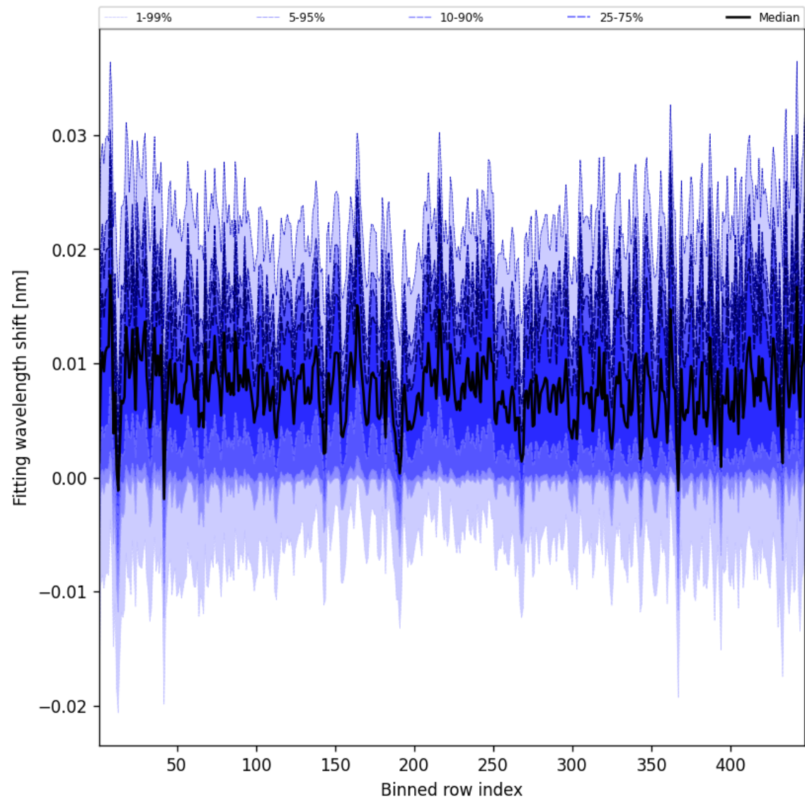
Figure 65: Along track statistics of “Fitting wavelength shift” for 2025-05-19 to 2025-05-21
