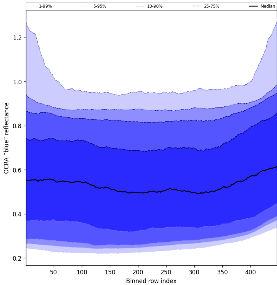
Figure 67: Along track statistics of “OCRA “blue” reflectance” for 2025-05-19 to 2025-05-21
