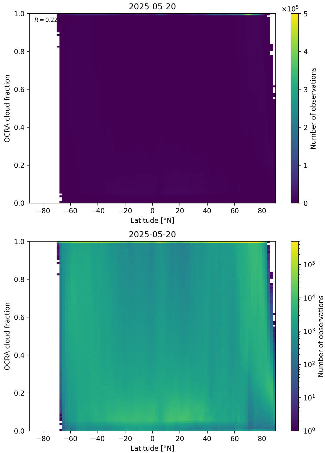
Figure 93: Scatter density plot of “Latitude” against “OCRA cloud fraction” for 2025-05-19 to 2025-05-21.
