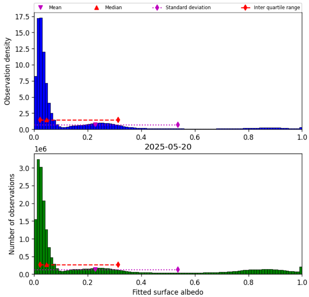
Figure 45: Histogram of “Fitted surface albedo” for 2025-05-19 to 2025-05-21
