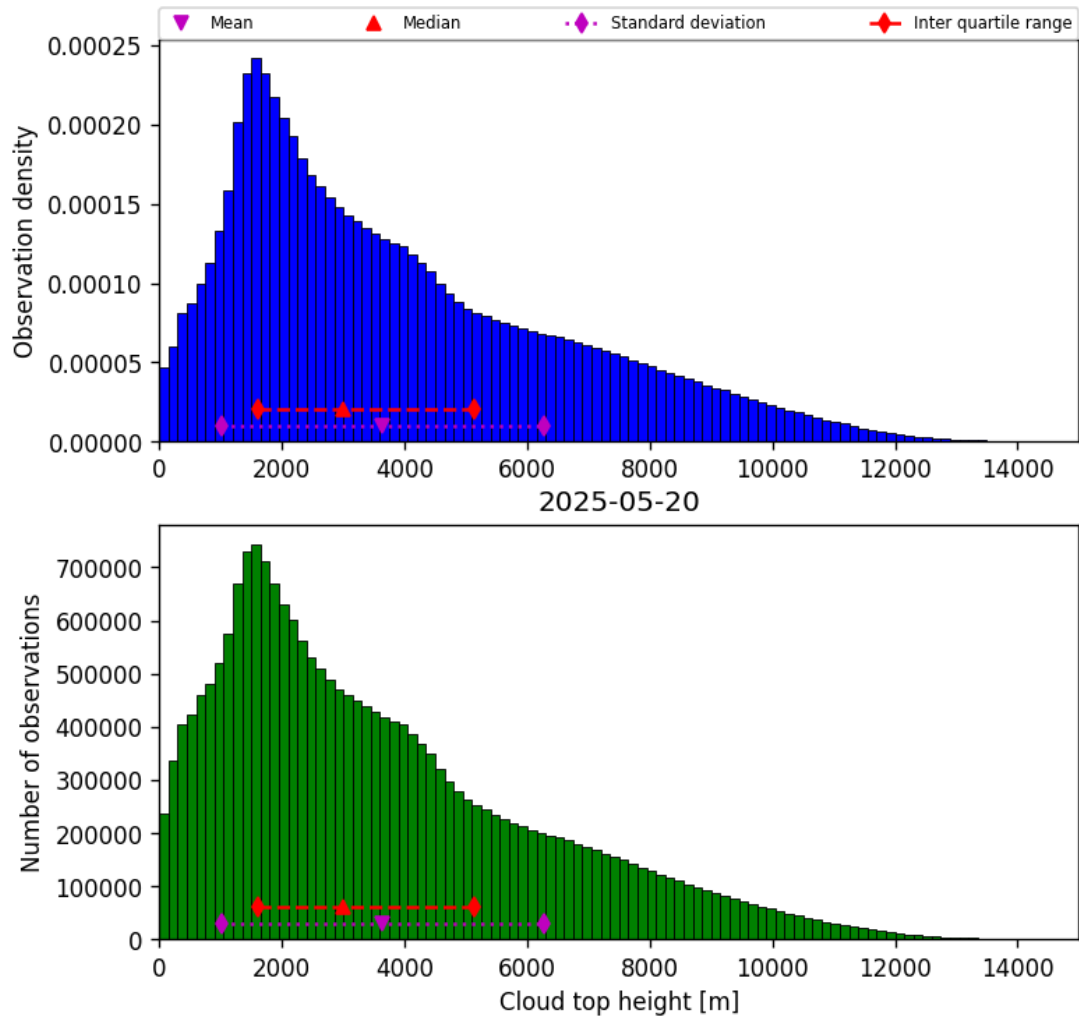
Figure 40: Histogram of “Cloud top height” for 2025-05-19 to 2025-05-21
