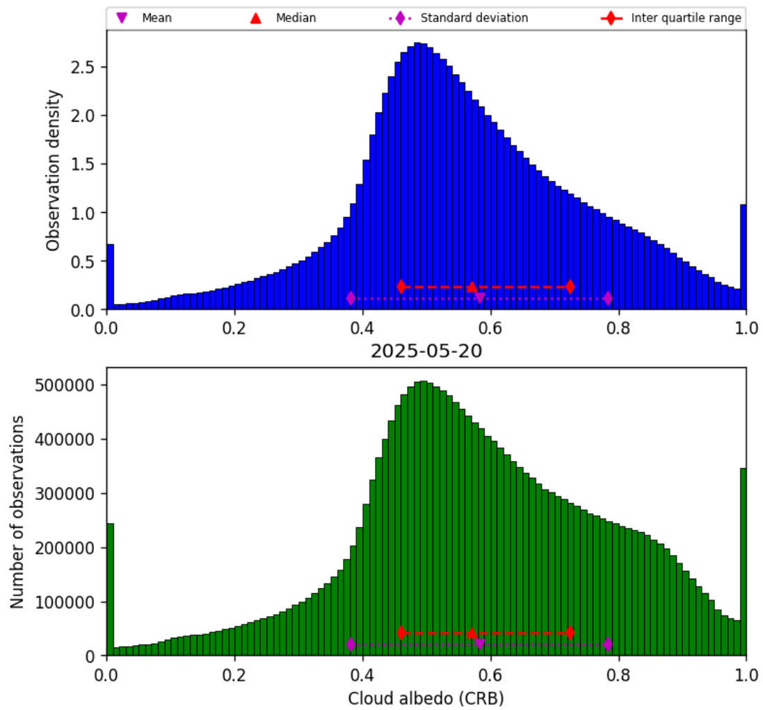
Figure 44: Histogram of “Cloud albedo (CRB)” for 2025-05-19 to 2025-05-21
