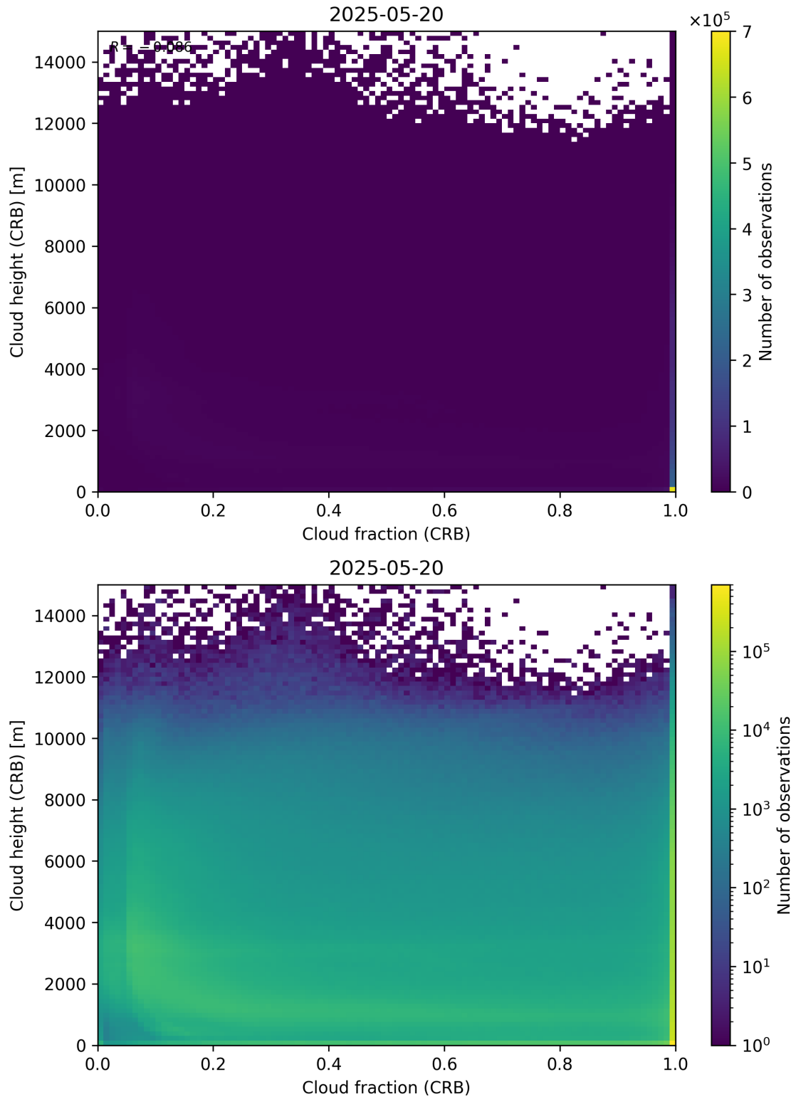
Figure 79: Scatter density plot of “Cloud fraction (CRB)” against “Cloud height (CRB)” for 2025-05-19 to 2025-05-21.
