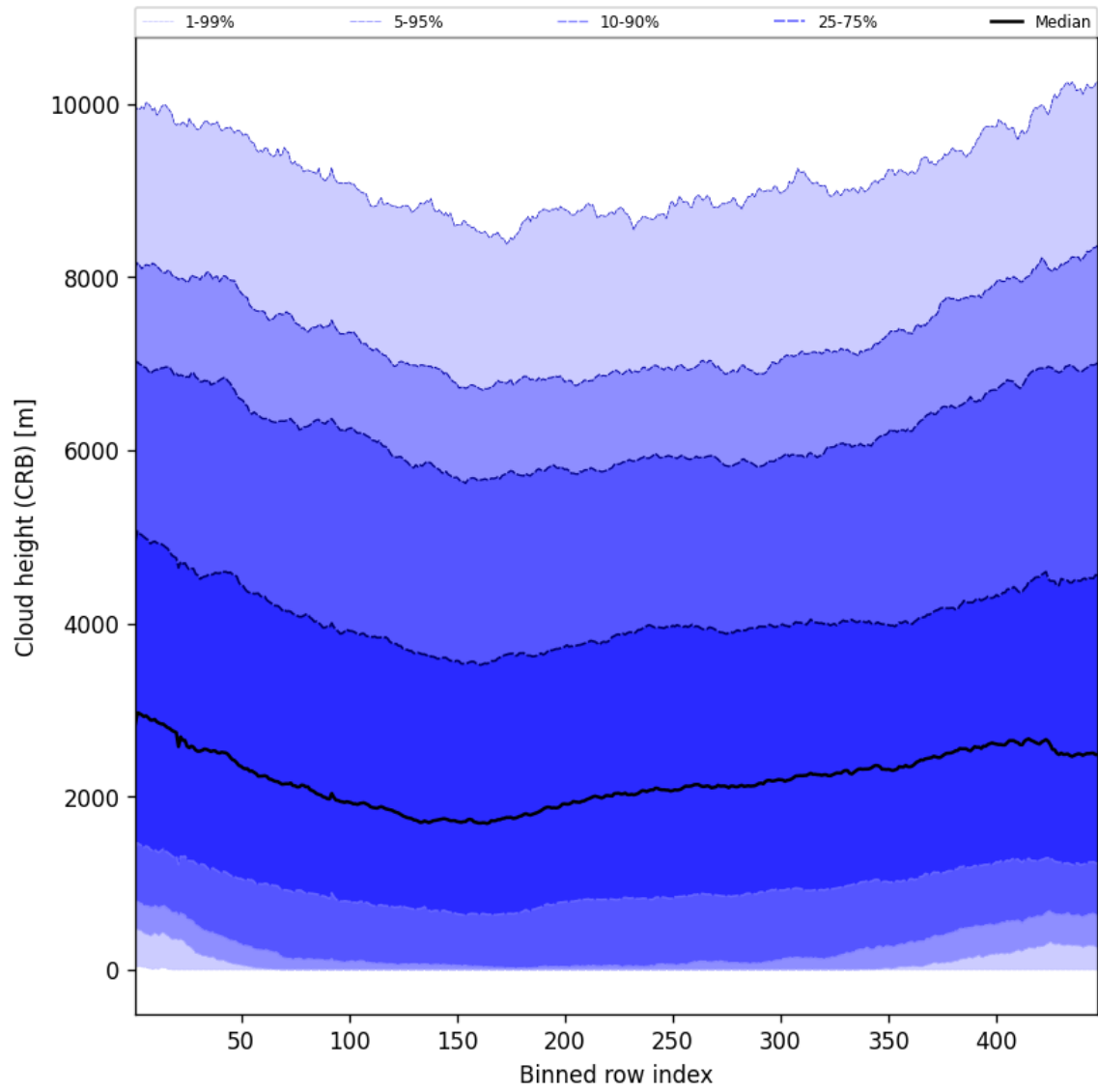
Figure 59: Along track statistics of “Cloud height (CRB)” for 2025-05-19 to 2025-05-21
