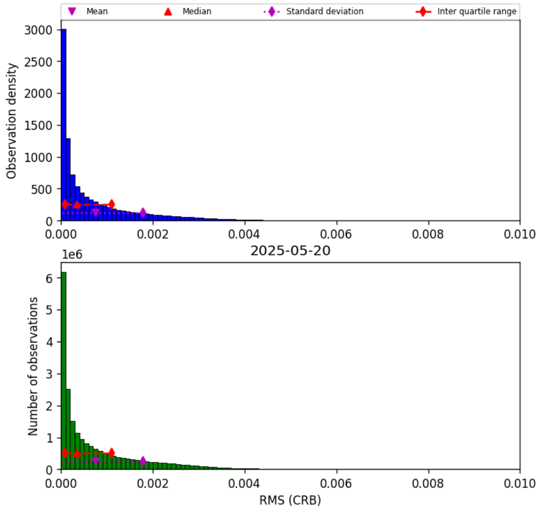
Figure 48: Histogram of “RMS (CRB)” for 2025-05-19 to 2025-05-21
