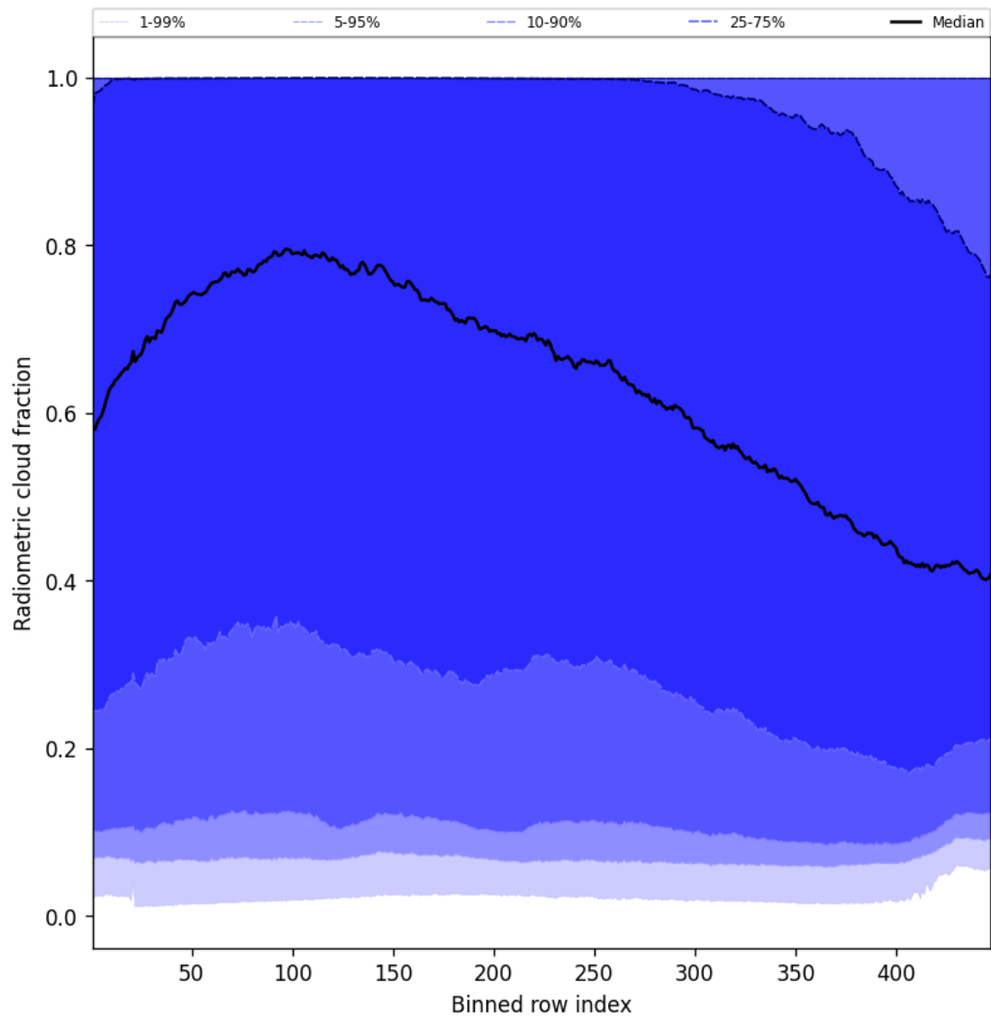
Figure 55: Along track statistics of “Radiometric cloud fraction” for 2025-05-19 to 2025-05-21
