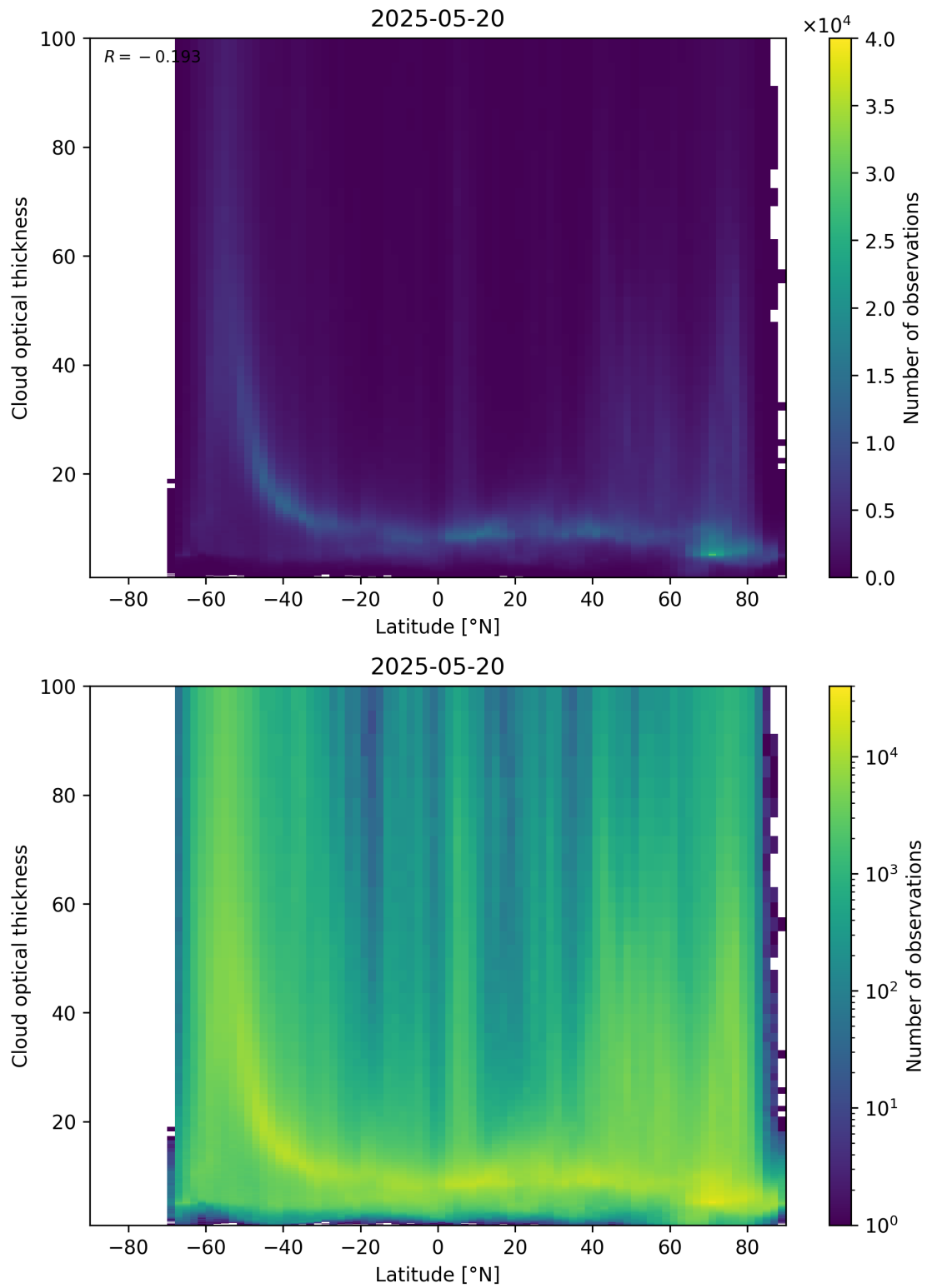
Figure 96: Scatter density plot of “Latitude” against “Cloud optical thickness” for 2025-05-19 to 2025-05-21.
