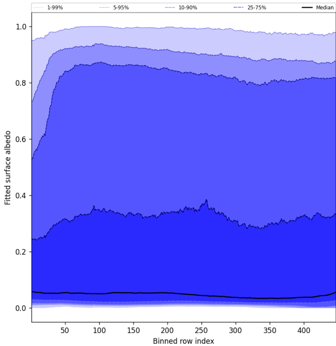
Figure 61: Along track statistics of “Fitted surface albedo” for 2025-05-19 to 2025-05-21
