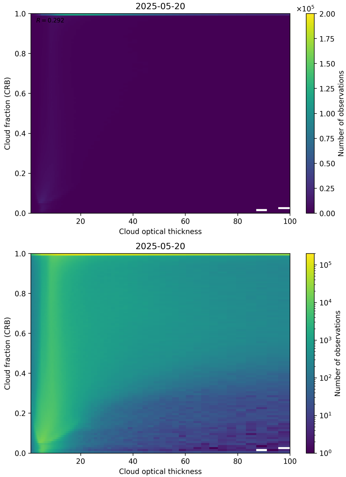
Figure 84: Scatter density plot of “Cloud optical thickness” against “Cloud fraction (CRB)” for 2025-05-19 to 2025-05-21.
