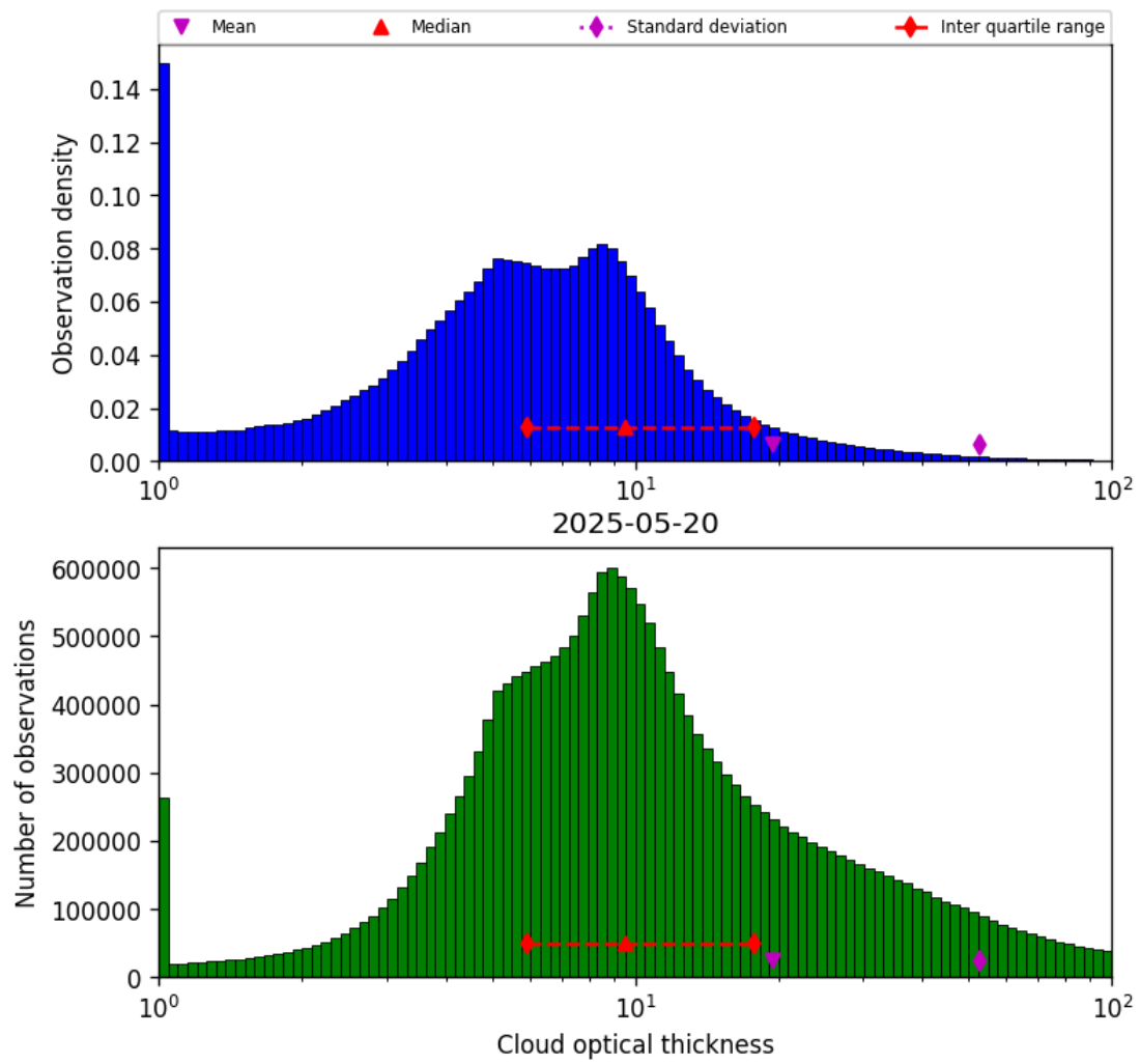
Figure 41: Histogram of “Cloud optical thickness” for 2025-05-19 to 2025-05-21
