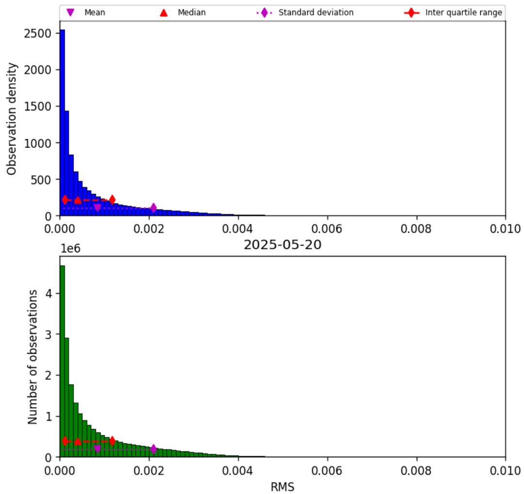
Figure 47: Histogram of “RMS” for 2025-05-19 to 2025-05-21
