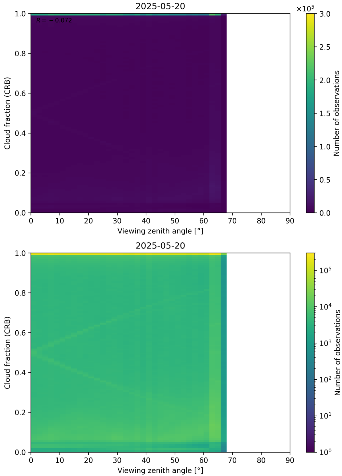
Figure 109: Scatter density plot of “Viewing zenith angle” against “Cloud fraction (CRB)” for 2025-05-19 to 2025-05-21.
