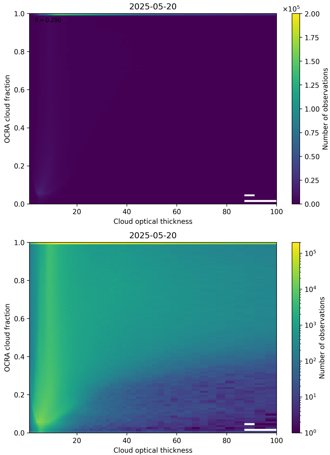
Figure 83: Scatter density plot of “Cloud optical thickness” against “OCRA cloud fraction” for 2025-05-19 to 2025-05-21.
