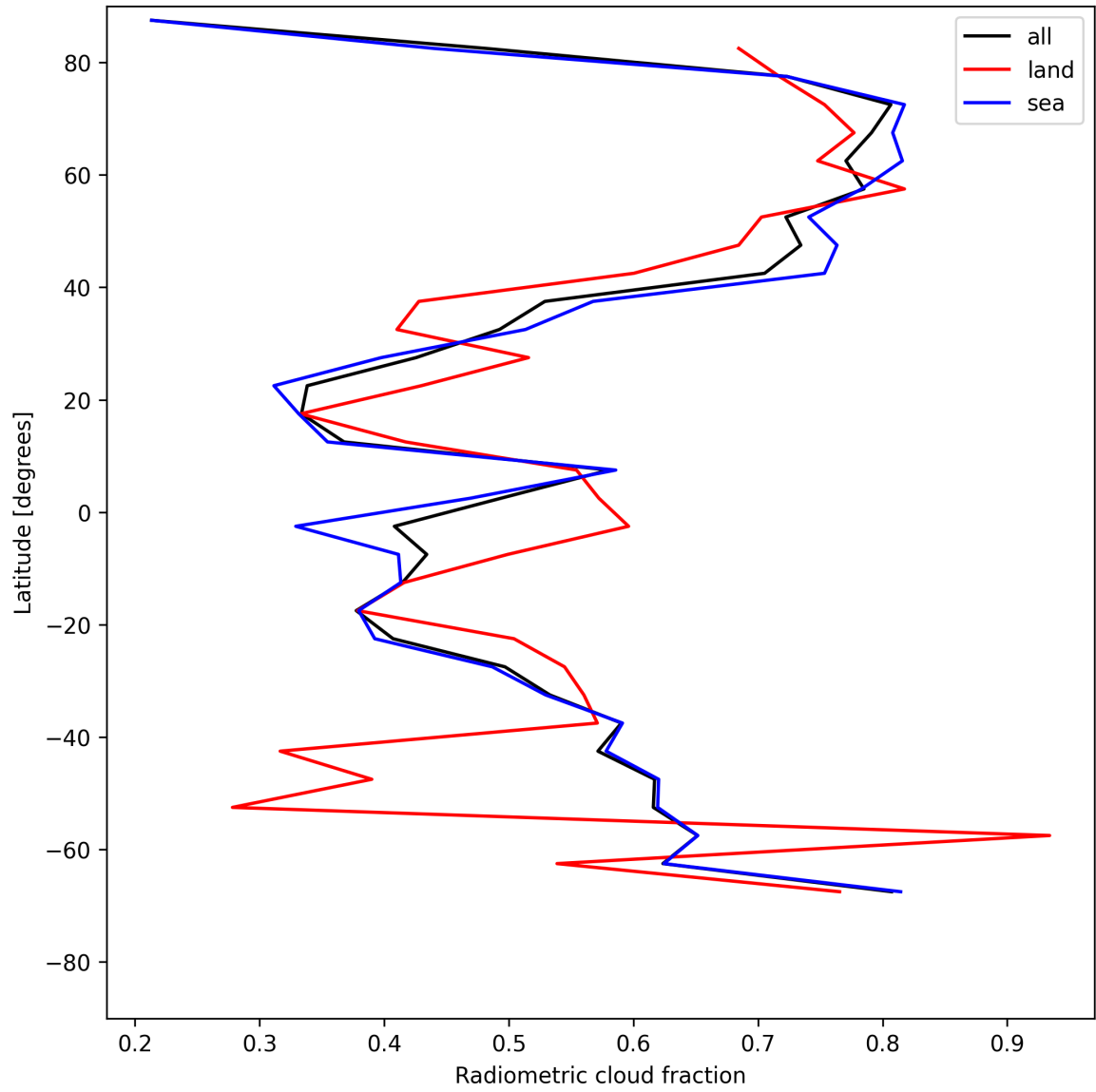
Figure 23: Zonal average of “Radiometric cloud fraction” for 2025-05-19 to 2025-05-21.
