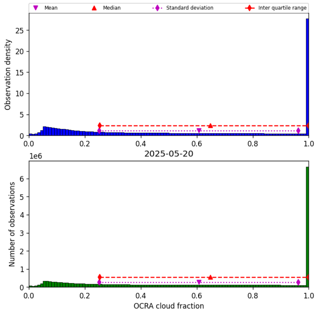
Figure 50: Histogram of “OCRA cloud fraction” for 2025-05-19 to 2025-05-21
