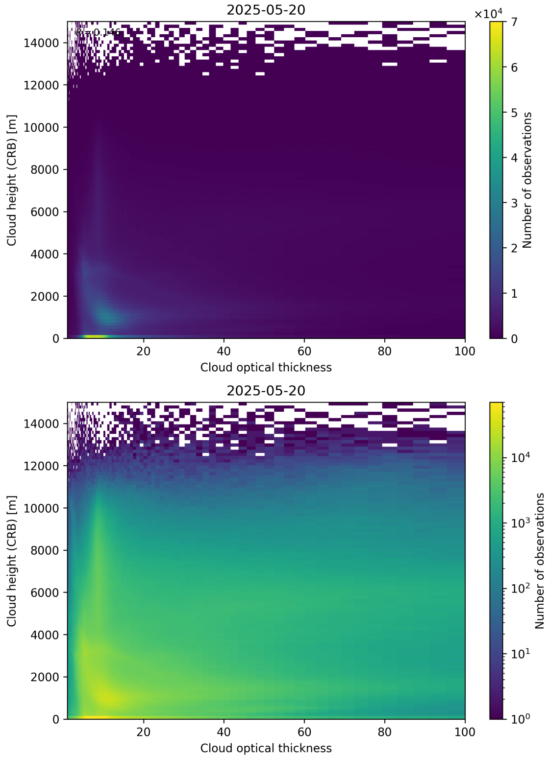
Figure 85: Scatter density plot of “Cloud optical thickness” against “Cloud height (CRB)” for 2025-05-19 to 2025-05-21.
