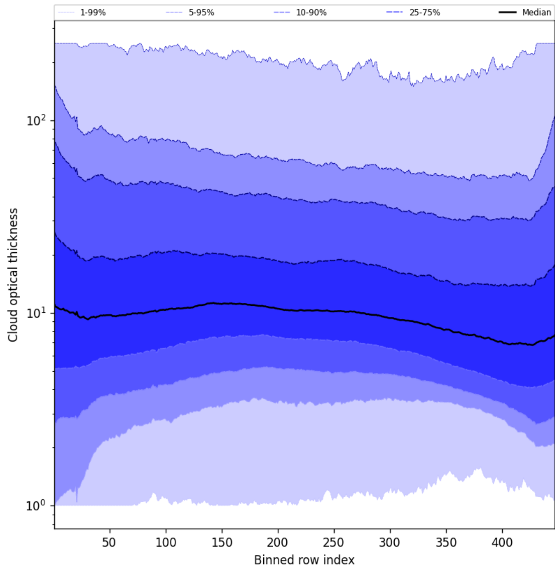
Figure 57: Along track statistics of “Cloud optical thickness” for 2025-05-19 to 2025-05-21
