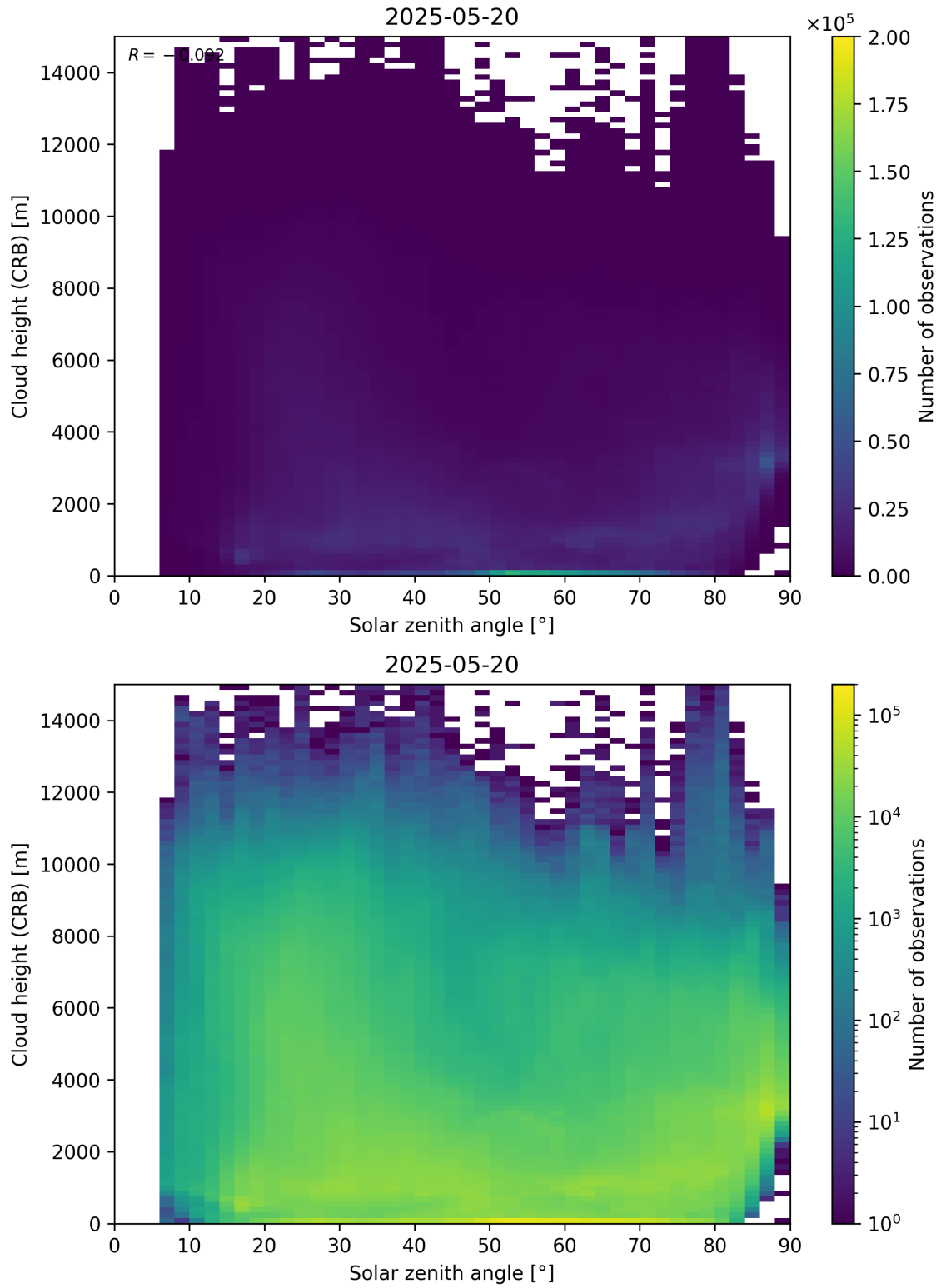
Figure 102: Scatter density plot of “Solar zenith angle” against “Cloud height (CRB)” for 2025-05-19 to 2025-05-21.
