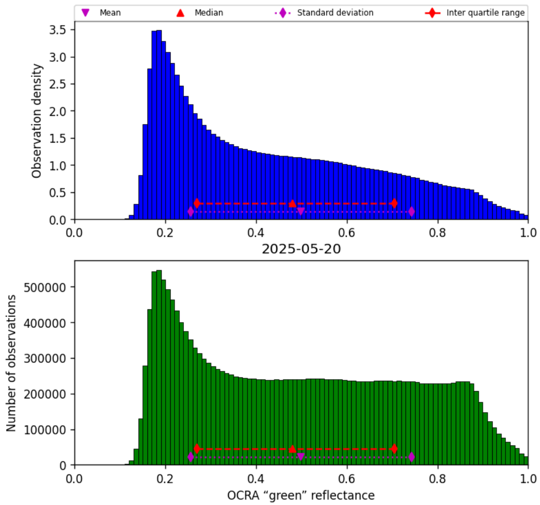
Figure 52: Histogram of “OCRA “green” reflectance” for 2025-05-19 to 2025-05-21
