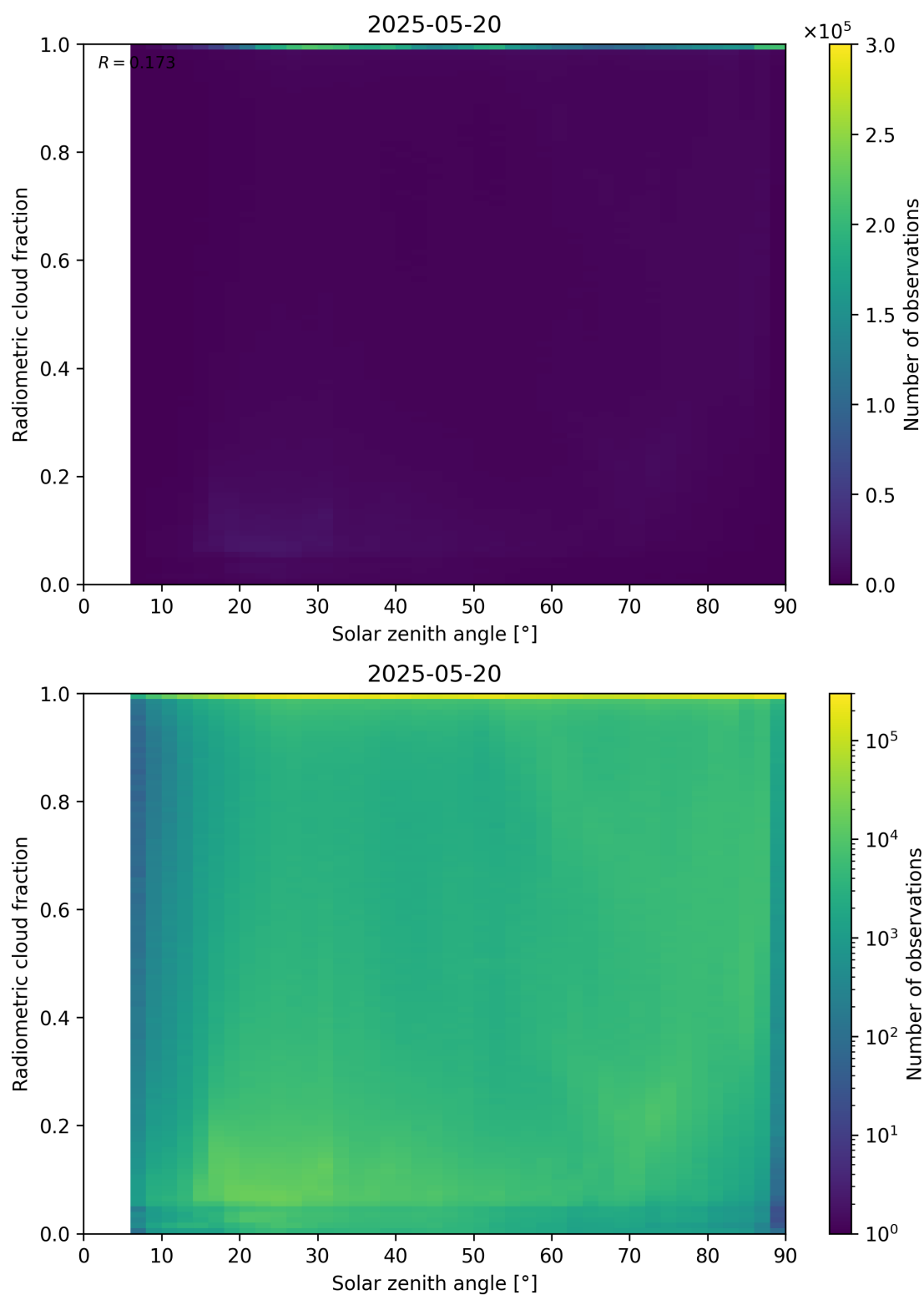
Figure 99: Scatter density plot of “Solar zenith angle” against “Radiometric cloud fraction” for 2025-05-19 to 2025-05-21.
