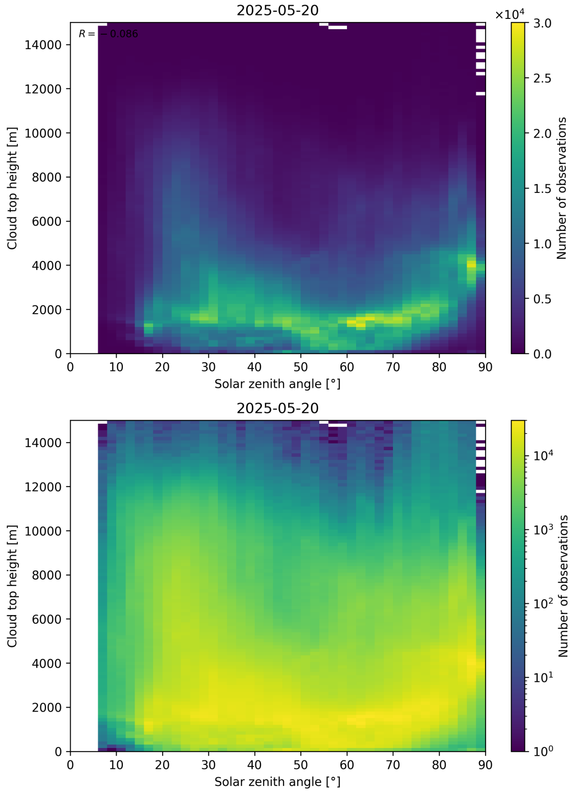
Figure 104: Scatter density plot of “Solar zenith angle” against “Cloud top height” for 2025-05-19 to 2025-05-21.
