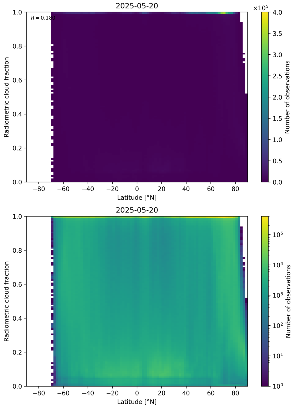
Figure 92: Scatter density plot of “Latitude” against “Radiometric cloud fraction” for 2025-05-19 to 2025-05-21.
