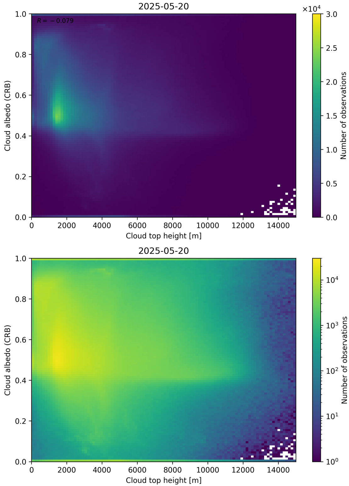
Figure 86: Scatter density plot of “Cloud top height” against “Cloud albedo (CRB)” for 2025-05-19 to 2025-05-21.
