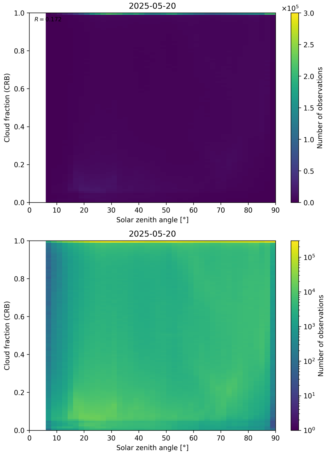
Figure 101: Scatter density plot of “Solar zenith angle” against “Cloud fraction (CRB)” for 2025-05-19 to 2025-05-21.
