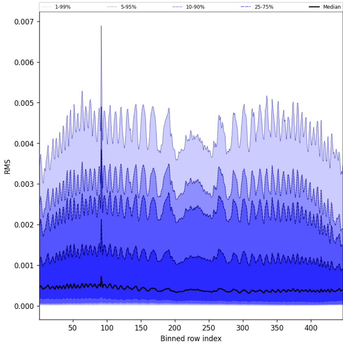
Figure 63: Along track statistics of “RMS” for 2025-05-19 to 2025-05-21
