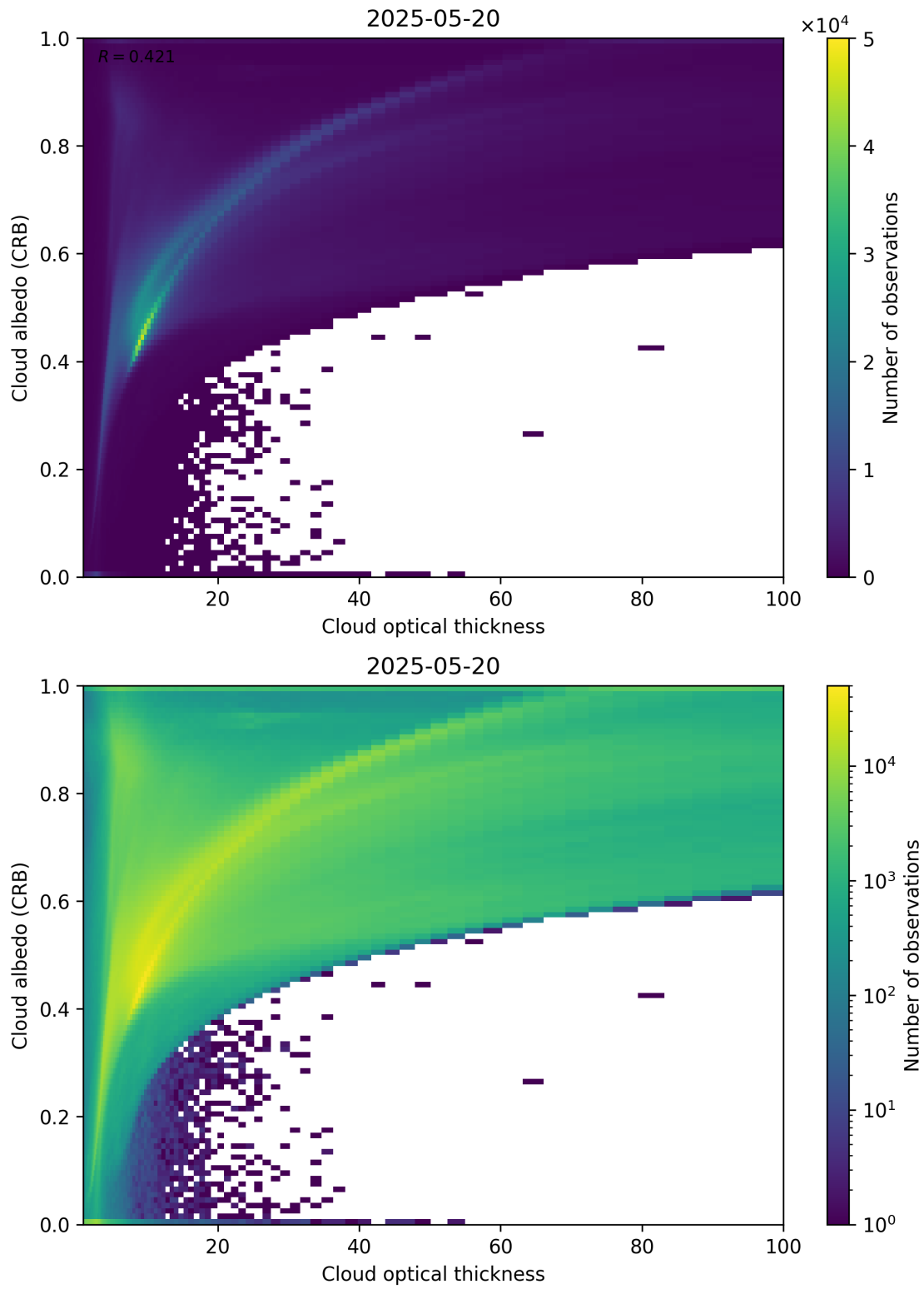
Figure 82: Scatter density plot of “Cloud optical thickness” against “Cloud albedo (CRB)” for 2025-05-19 to 2025-05-21.
