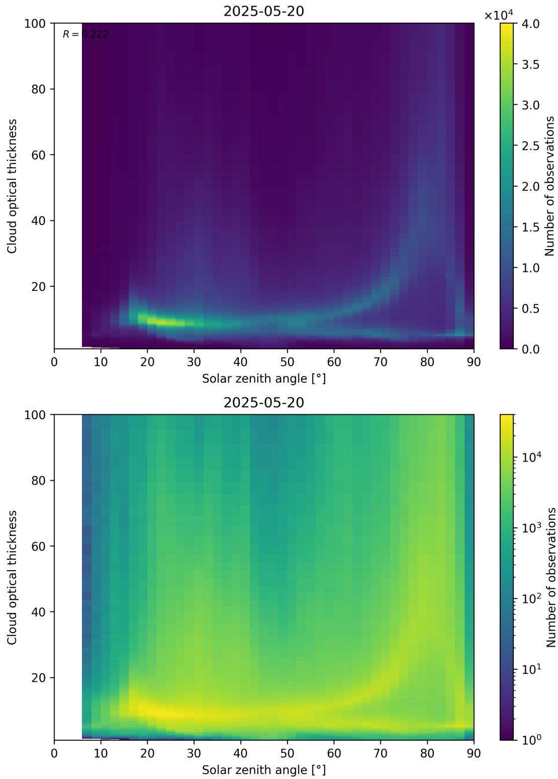
Figure 103: Scatter density plot of “Solar zenith angle” against “Cloud optical thickness” for 2025-05-19 to 2025-05-21.
