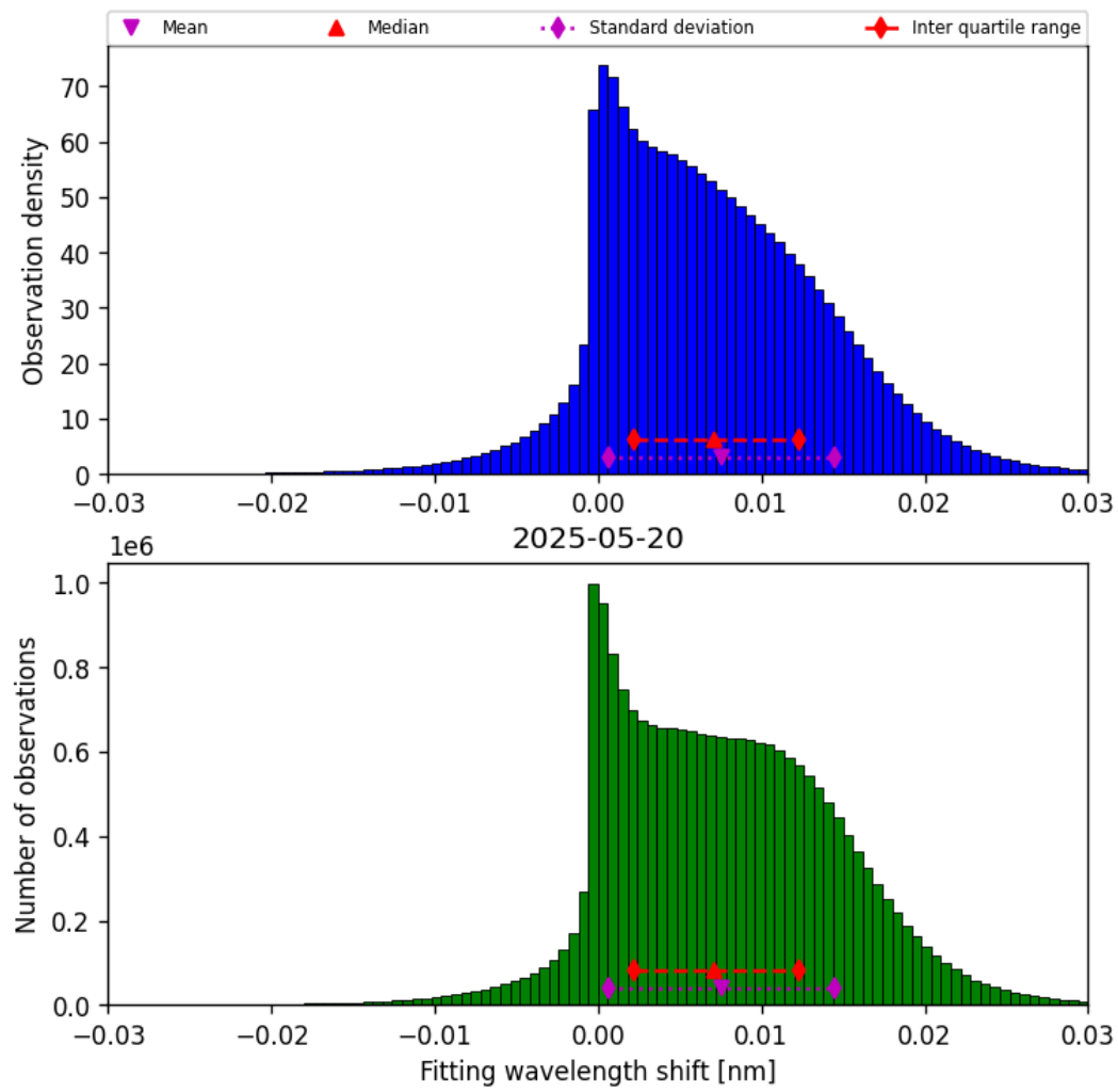
Figure 49: Histogram of “Fitting wavelength shift” for 2025-05-19 to 2025-05-21
