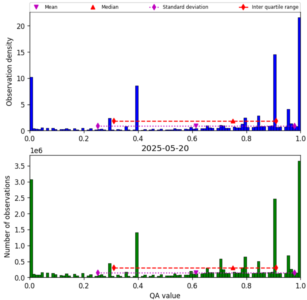
Figure 38: Histogram of “QA value” for 2025-05-19 to 2025-05-21
