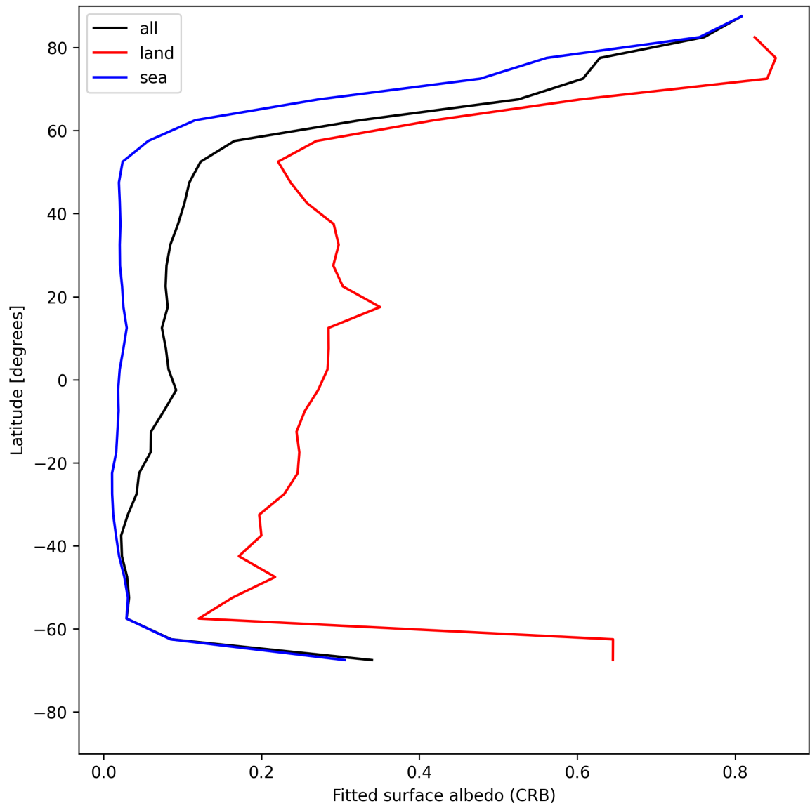
Figure 30: Zonal average of “Fitted surface albedo (CRB)” for 2025-05-19 to 2025-05-21.
