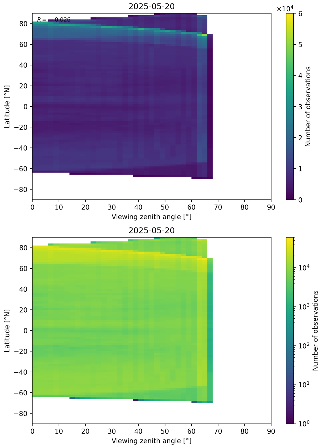
Figure 113: Scatter density plot of “Viewing zenith angle” against “Latitude” for 2025-05-19 to 2025-05-21.
