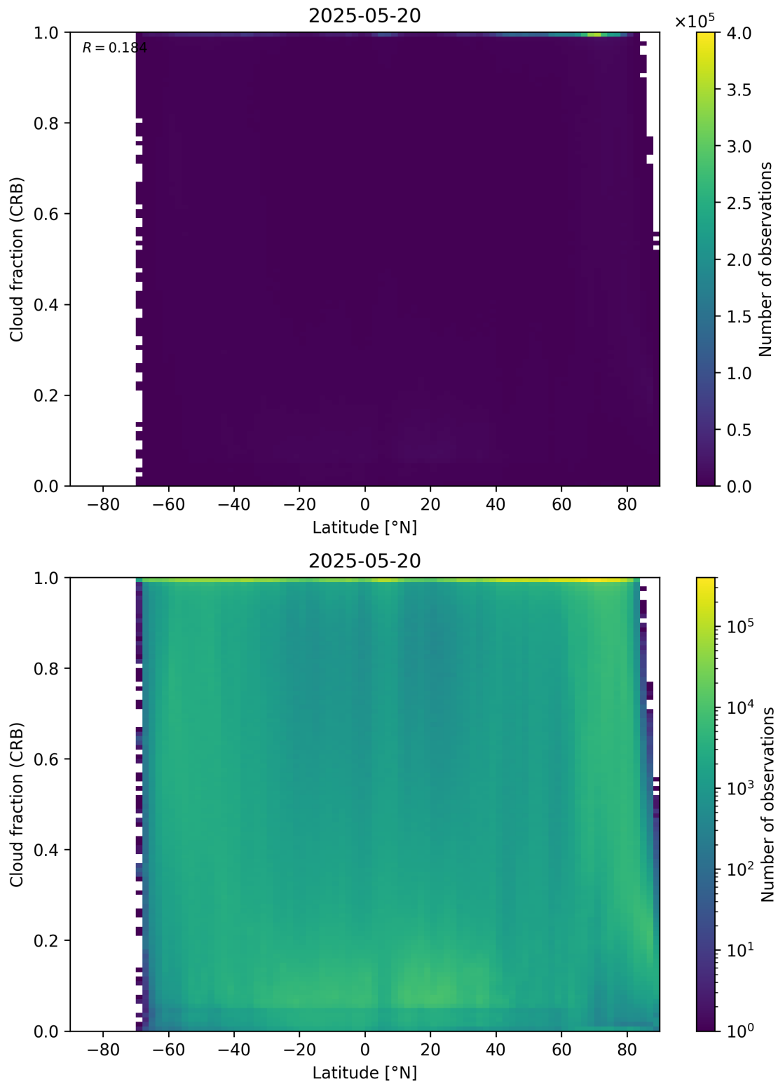
Figure 94: Scatter density plot of “Latitude” against “Cloud fraction (CRB)” for 2025-05-19 to 2025-05-21.
