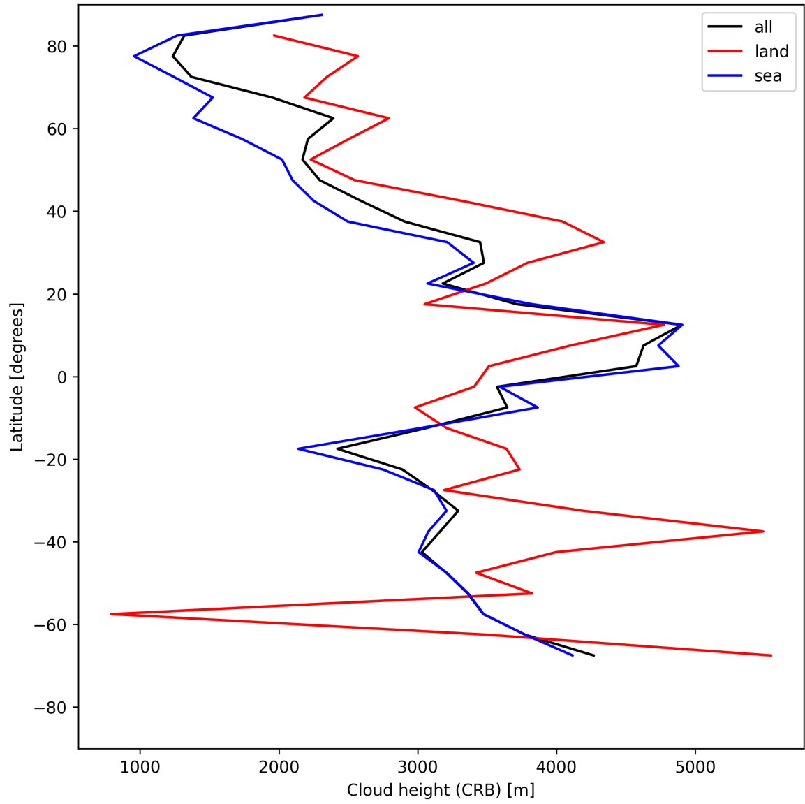
Figure 27: Zonal average of “Cloud height (CRB)” for 2025-05-19 to 2025-05-21.
