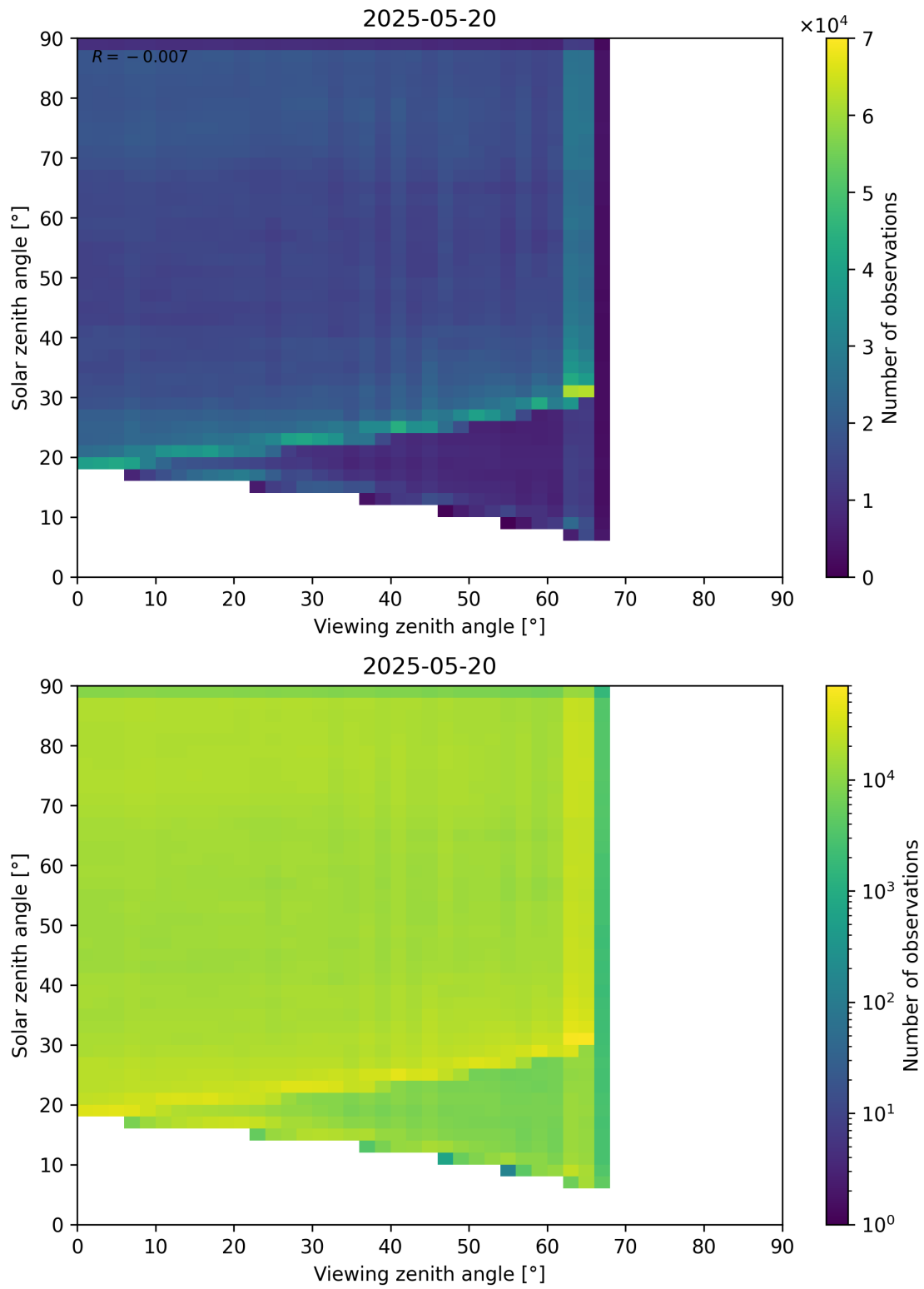
Figure 114: Scatter density plot of “Viewing zenith angle” against “Solar zenith angle” for 2025-05-19 to 2025-05-21.
