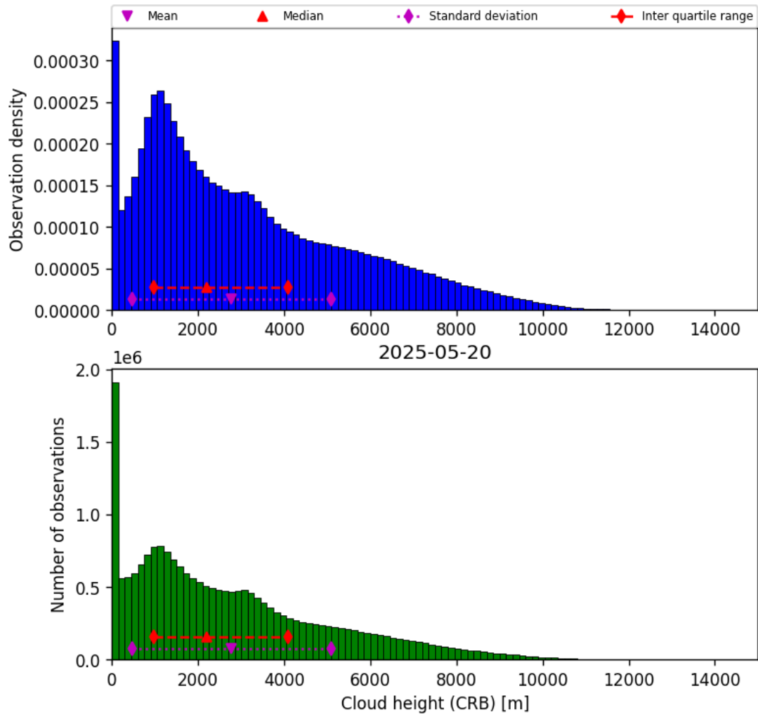
Figure 43: Histogram of “Cloud height (CRB)” for 2025-05-19 to 2025-05-21
