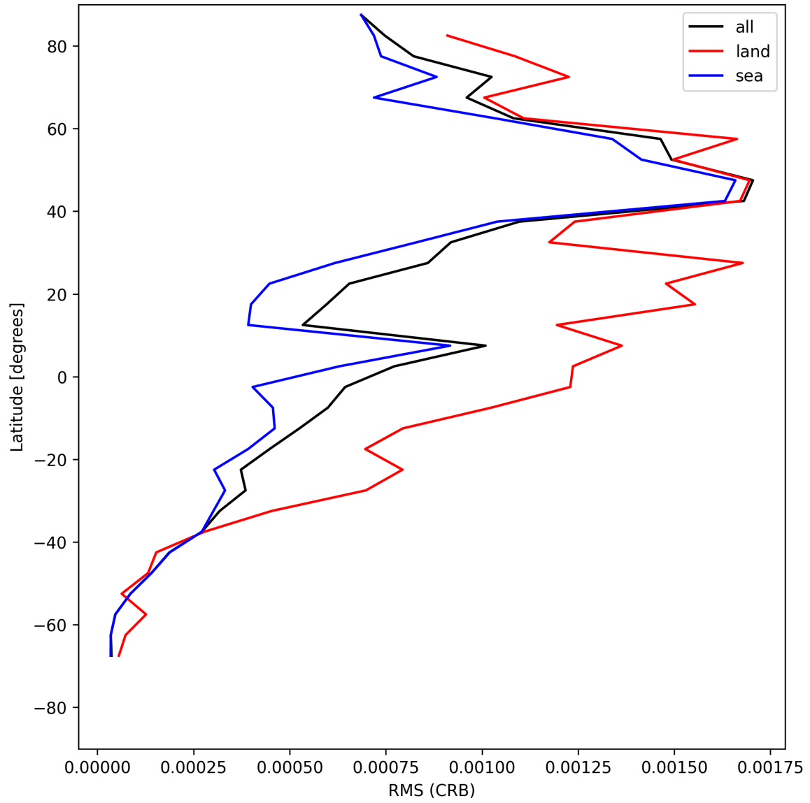
Figure 32: Zonal average of “RMS (CRB)” for 2025-05-19 to 2025-05-21.
