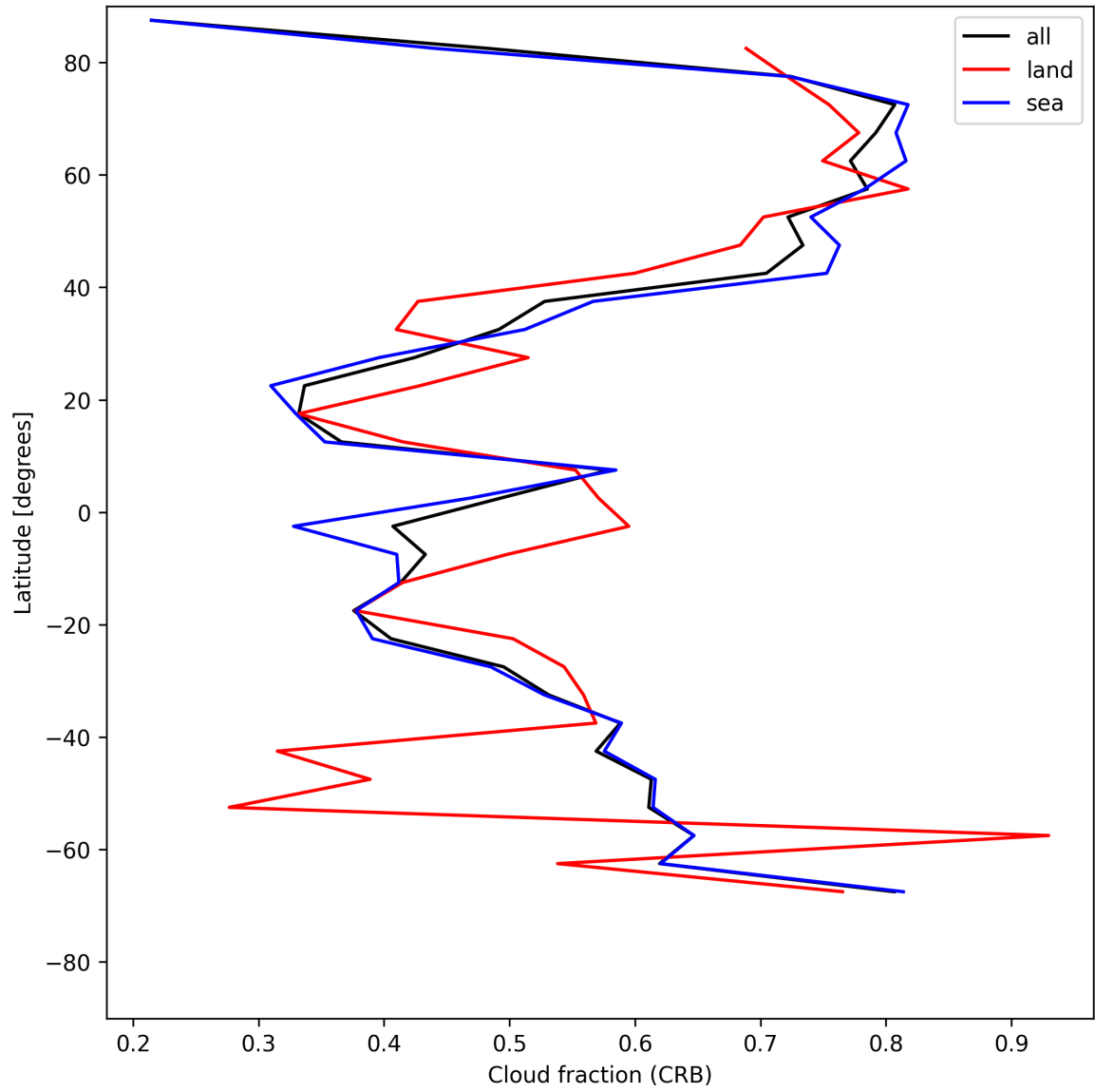
Figure 26: Zonal average of “Cloud fraction (CRB)” for 2025-05-19 to 2025-05-21.
