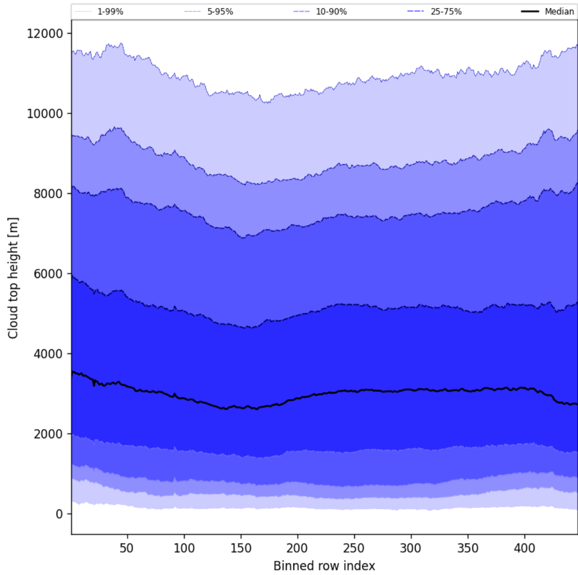
Figure 56: Along track statistics of “Cloud top height” for 2025-05-19 to 2025-05-21
