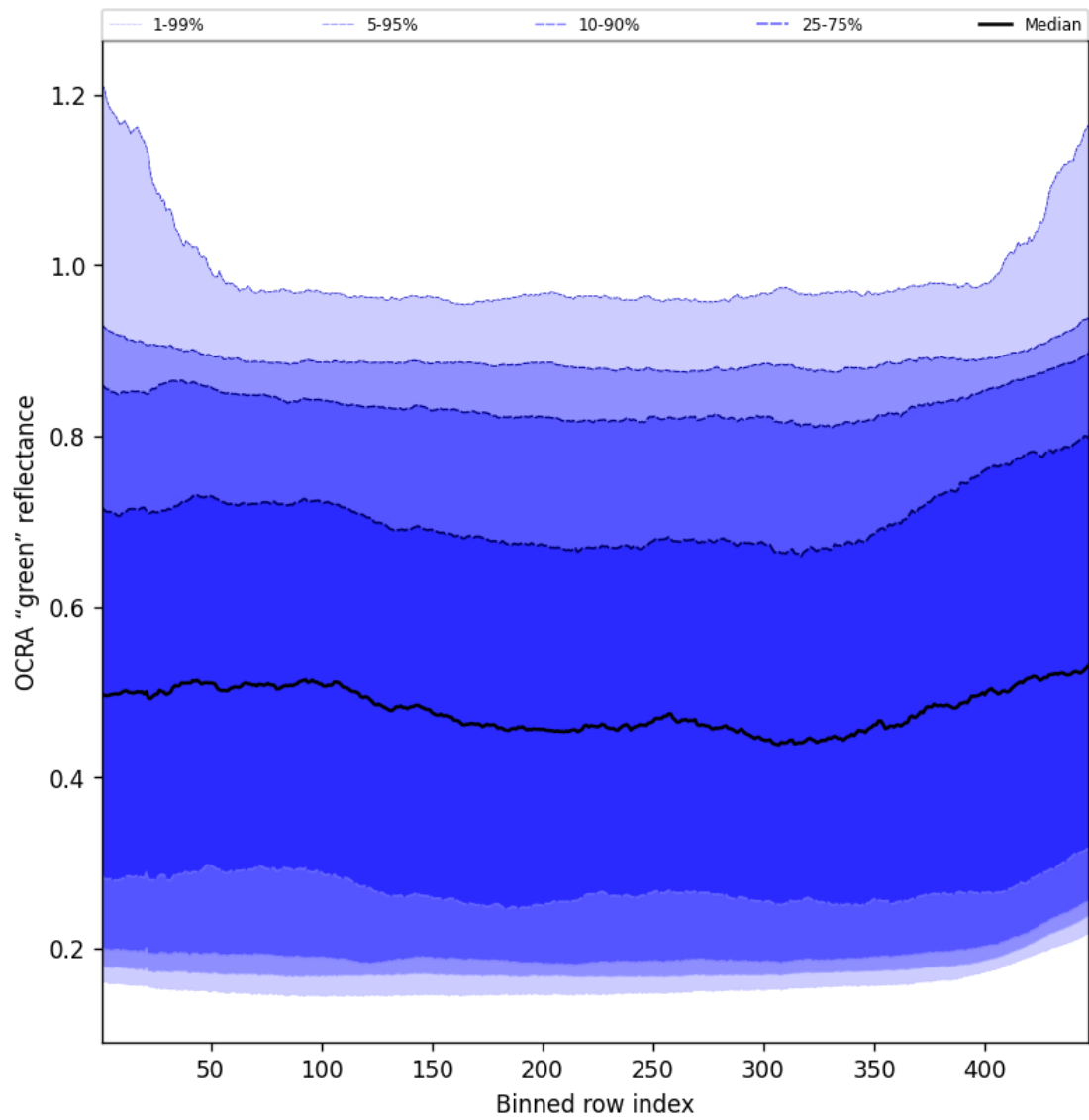
Figure 68: Along track statistics of “OCRA “green” reflectance” for 2025-05-19 to 2025-05-21
