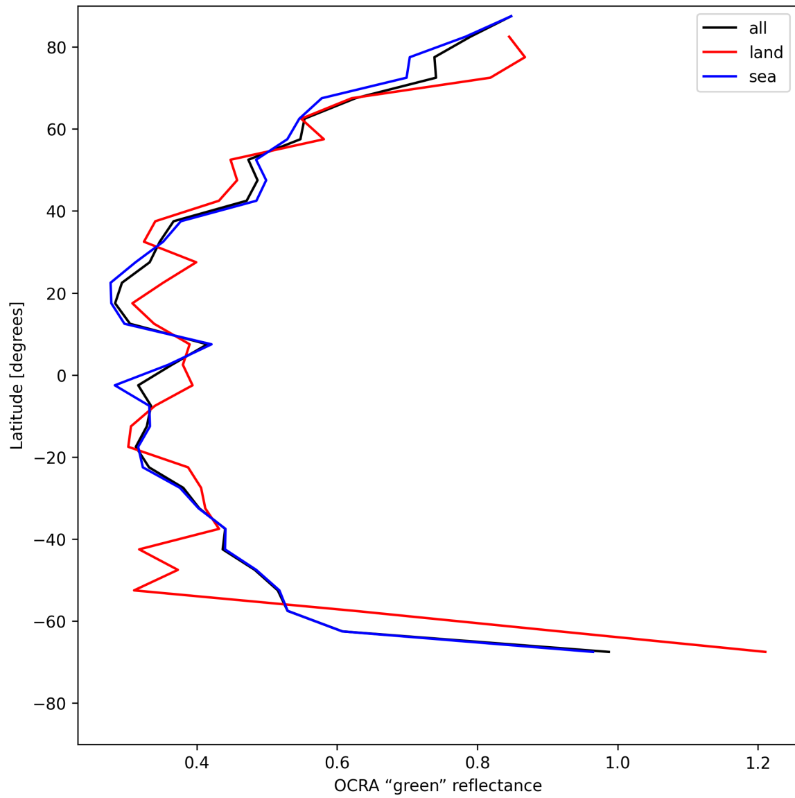
Figure 36: Zonal average of “OCRA “green” reflectance” for 2025-05-19 to 2025-05-21.
