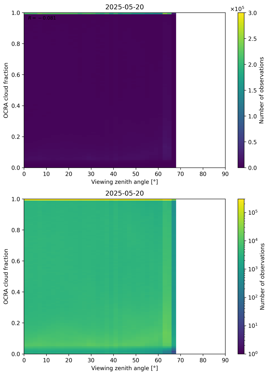
Figure 108: Scatter density plot of “Viewing zenith angle” against “OCRA cloud fraction” for 2025-05-19 to 2025-05-21.
