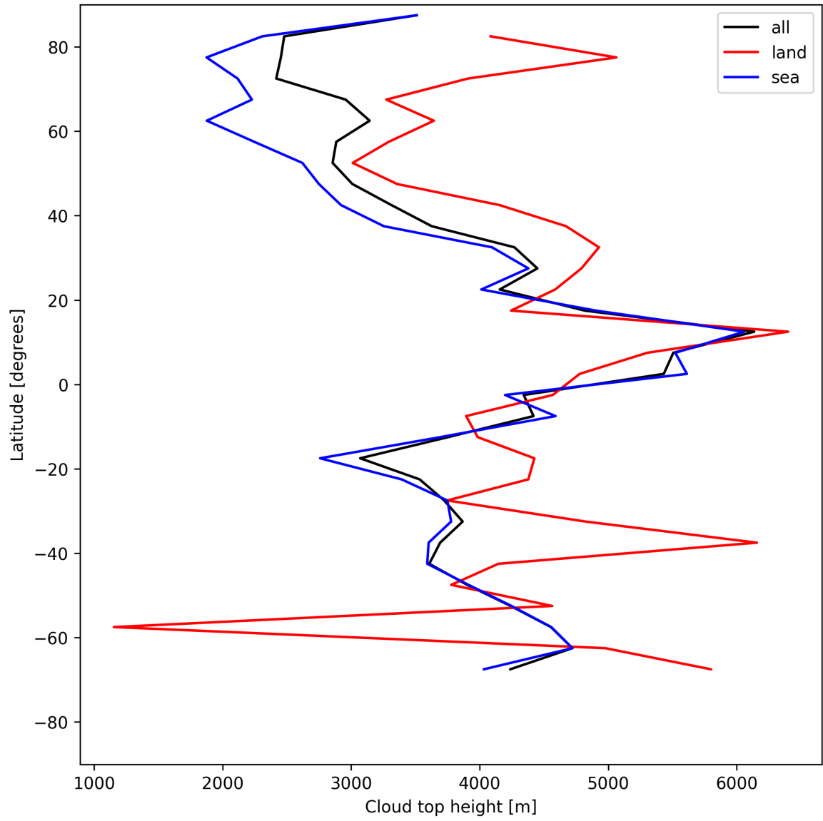
Figure 24: Zonal average of “Cloud top height” for 2025-05-19 to 2025-05-21.
