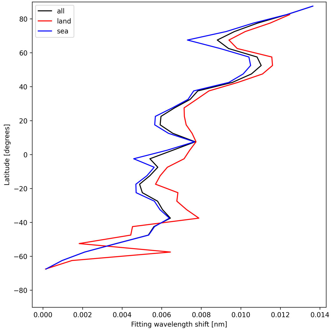
Figure 33: Zonal average of “Fitting wavelength shift” for 2025-05-19 to 2025-05-21.
