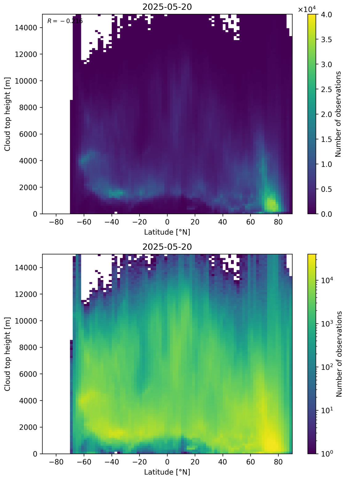
Figure 97: Scatter density plot of “Latitude” against “Cloud top height” for 2025-05-19 to 2025-05-21.
