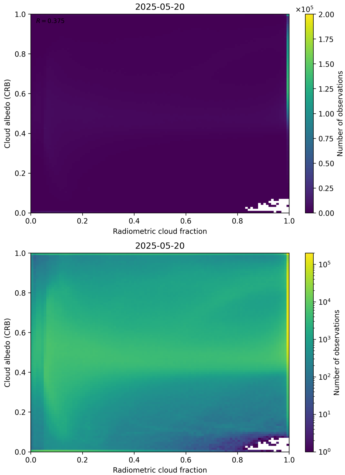
Figure 71: Scatter density plot of “Radiometric cloud fraction” against “Cloud albedo (CRB)” for 2025-05-19 to 2025-05-21.
