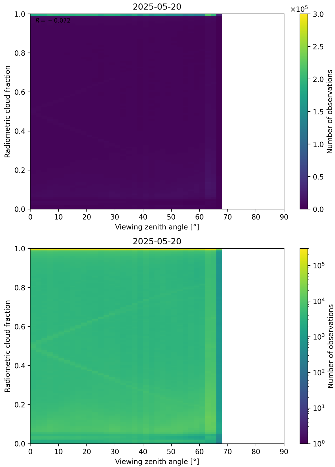
Figure 107: Scatter density plot of “Viewing zenith angle” against “Radiometric cloud fraction” for 2025-05-19 to 2025-05-21.
