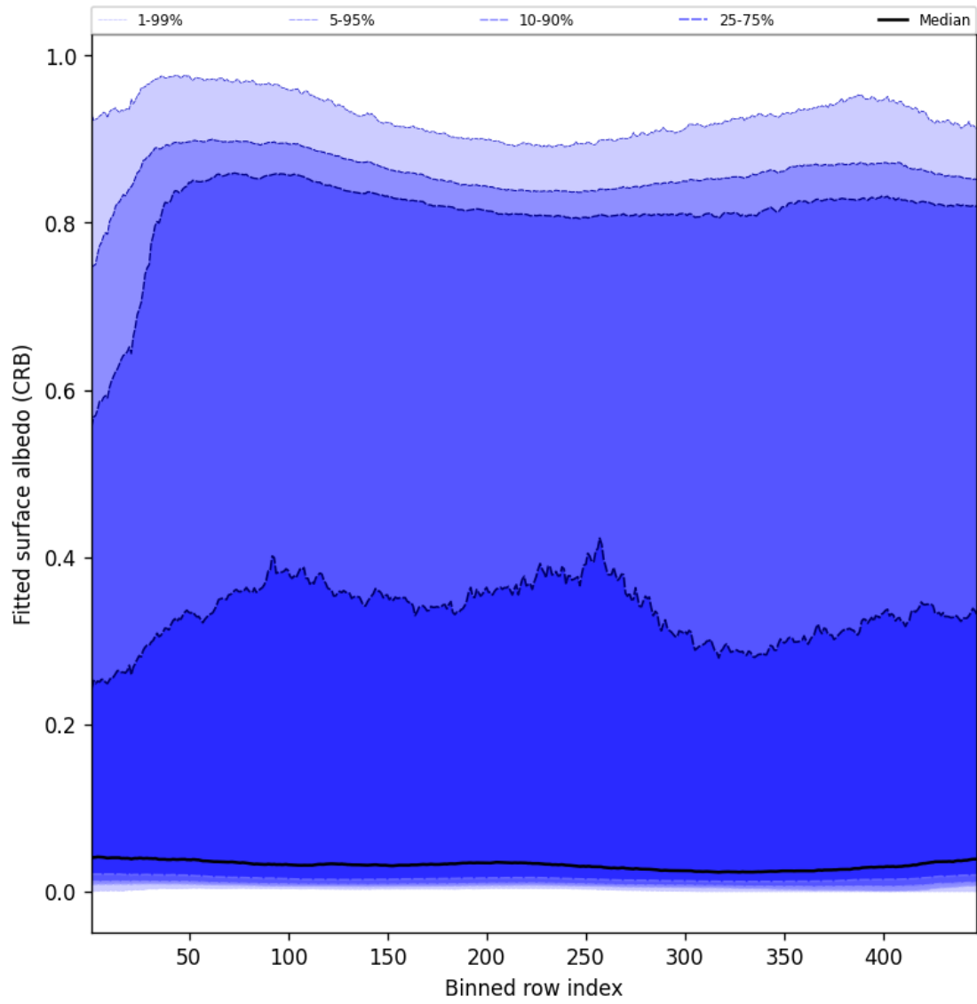
Figure 62: Along track statistics of “Fitted surface albedo (CRB)” for 2025-05-19 to 2025-05-21
