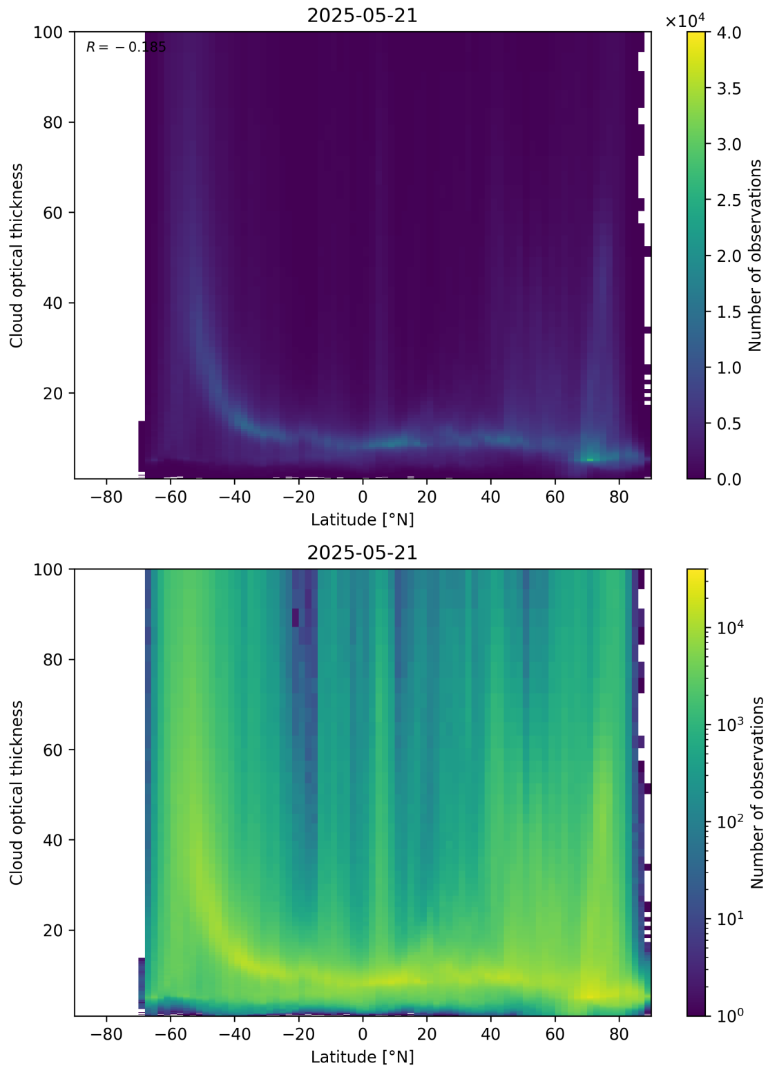
Figure 96: Scatter density plot of “Latitude” against “Cloud optical thickness” for 2025-05-21 to 2025-05-22.
