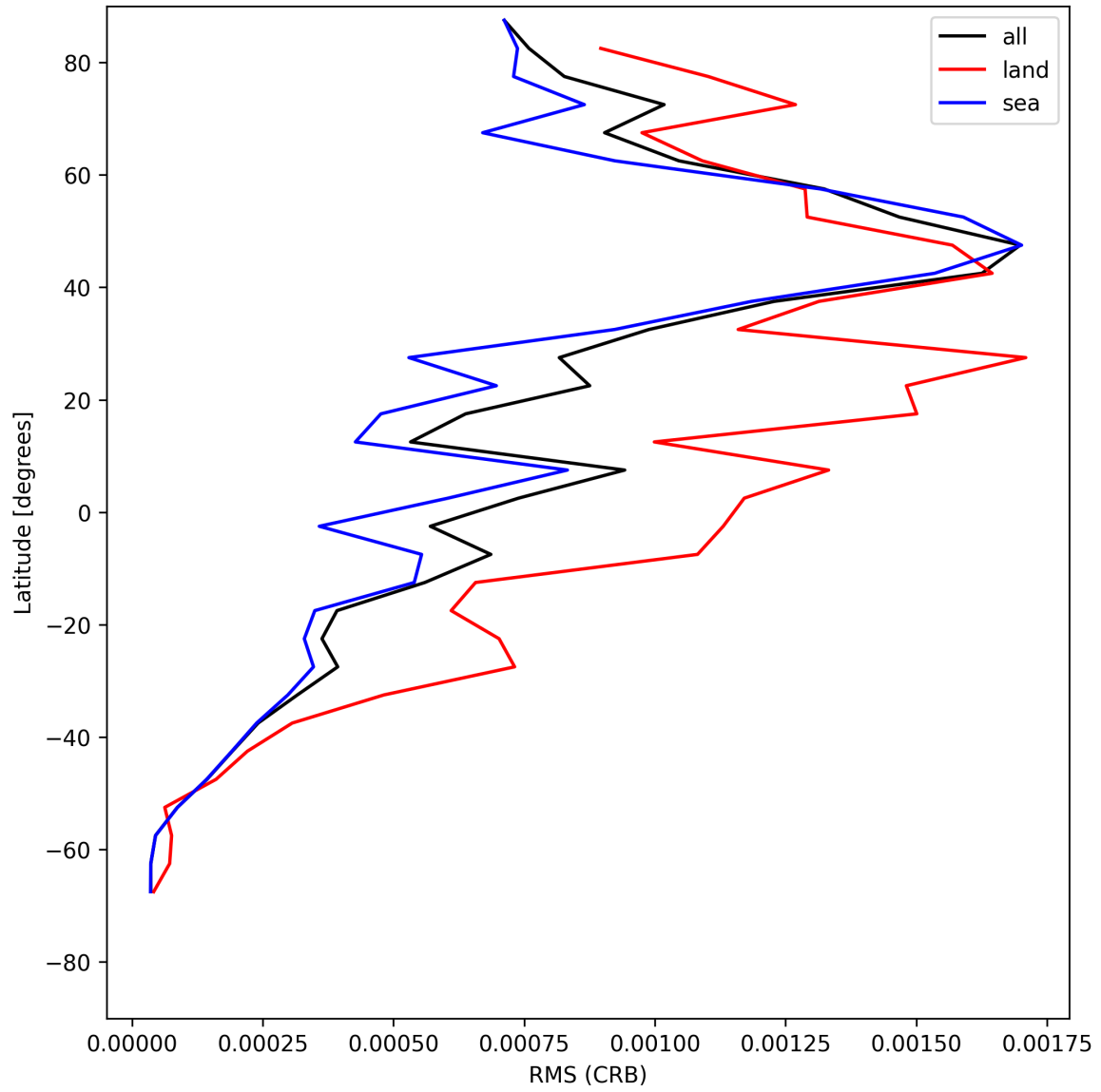
Figure 32: Zonal average of “RMS (CRB)” for 2025-05-21 to 2025-05-22.
