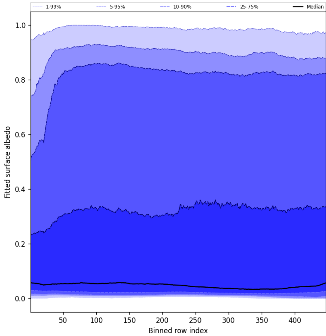
Figure 61: Along track statistics of “Fitted surface albedo” for 2025-05-21 to 2025-05-22
