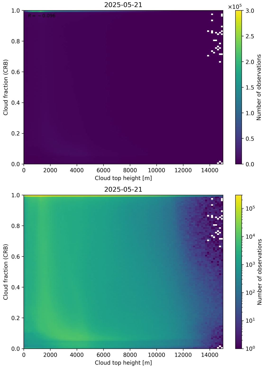
Figure 88: Scatter density plot of “Cloud top height” against “Cloud fraction (CRB)” for 2025-05-21 to 2025-05-22.
