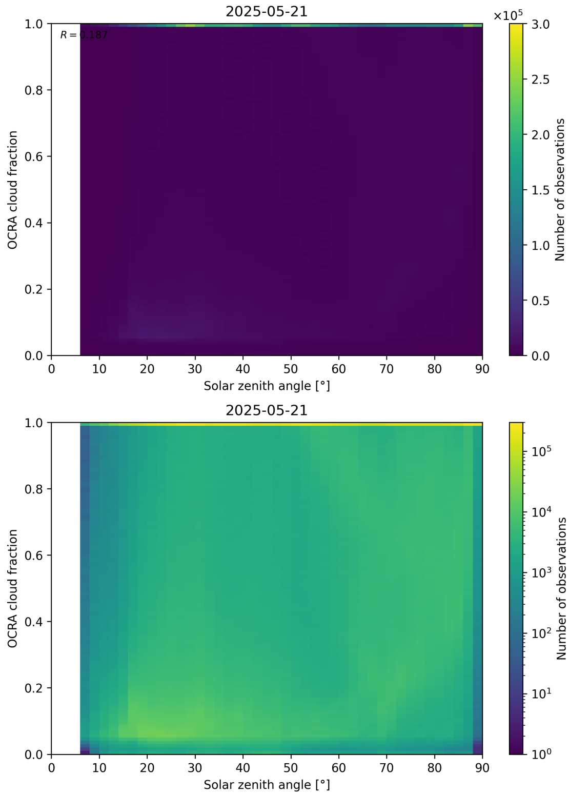
Figure 100: Scatter density plot of “Solar zenith angle” against “OCRA cloud fraction” for 2025-05-21 to 2025-05-22.
