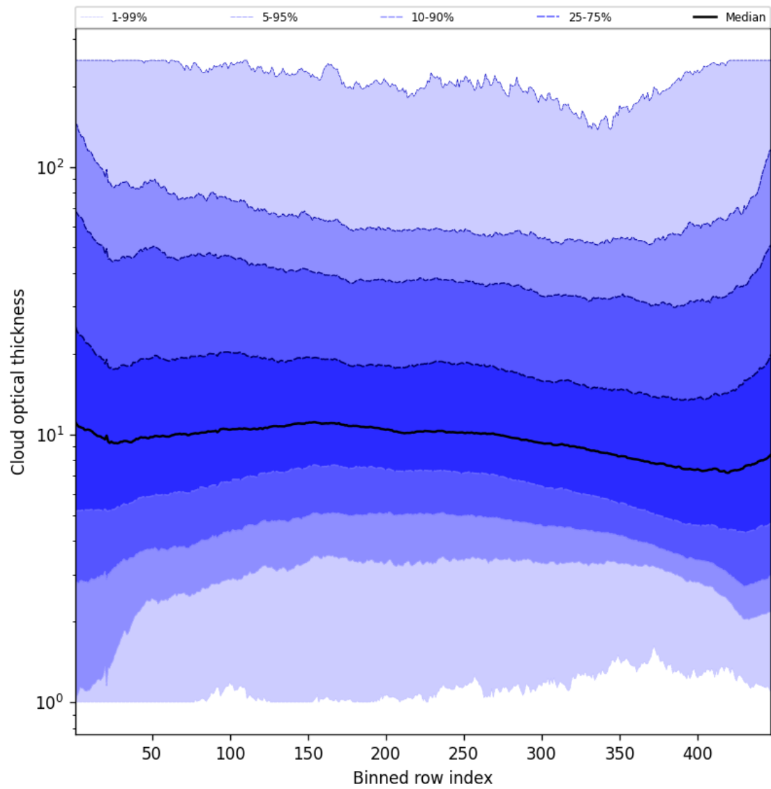
Figure 57: Along track statistics of “Cloud optical thickness” for 2025-05-21 to 2025-05-22
