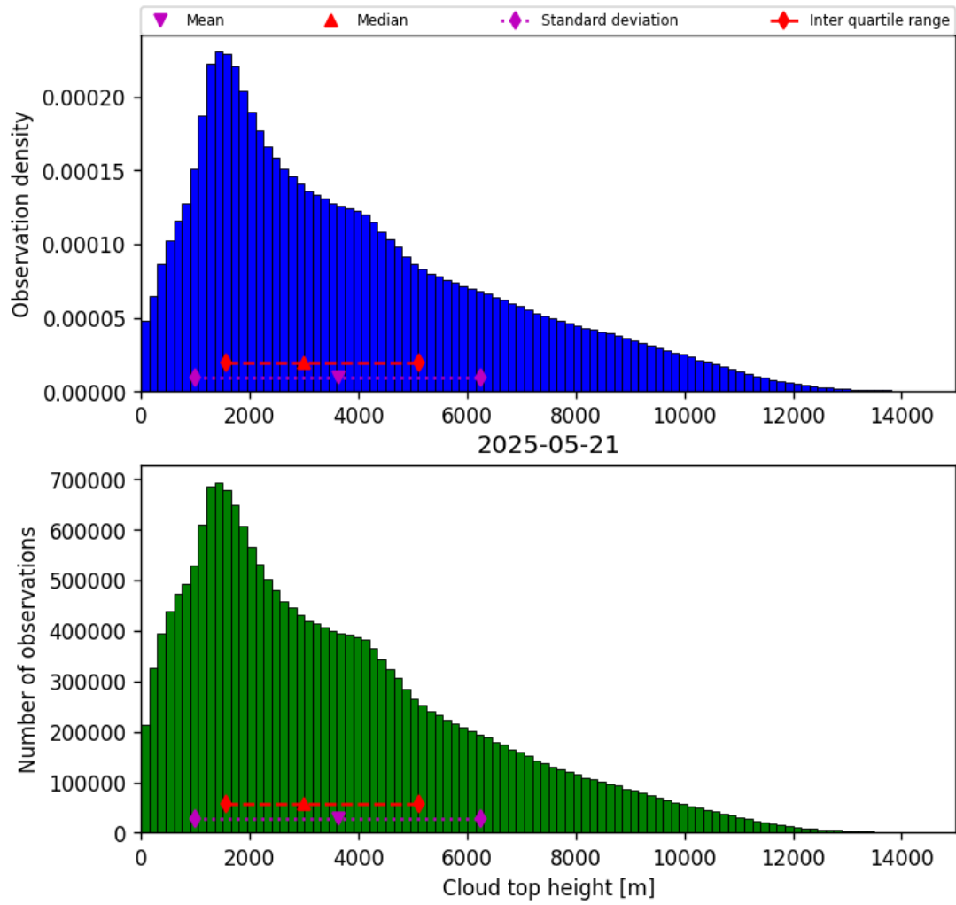
Figure 40: Histogram of “Cloud top height” for 2025-05-21 to 2025-05-22
