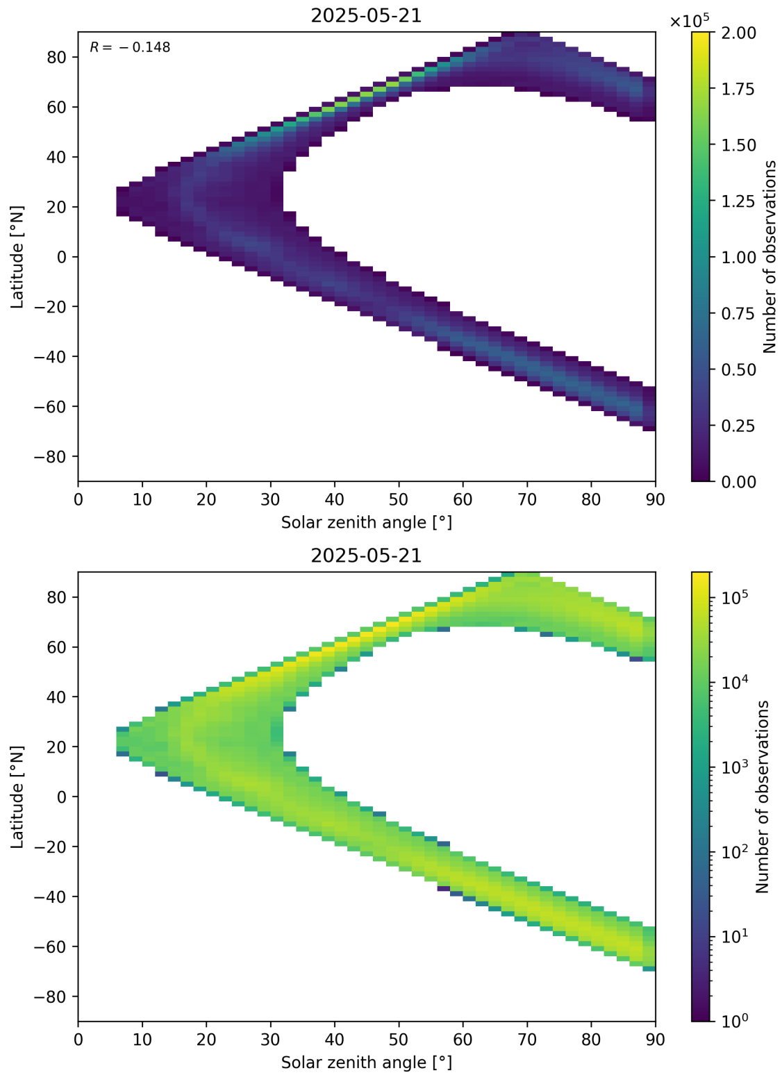
Figure 105: Scatter density plot of “Solar zenith angle” against “Latitude” for 2025-05-21 to 2025-05-22.
