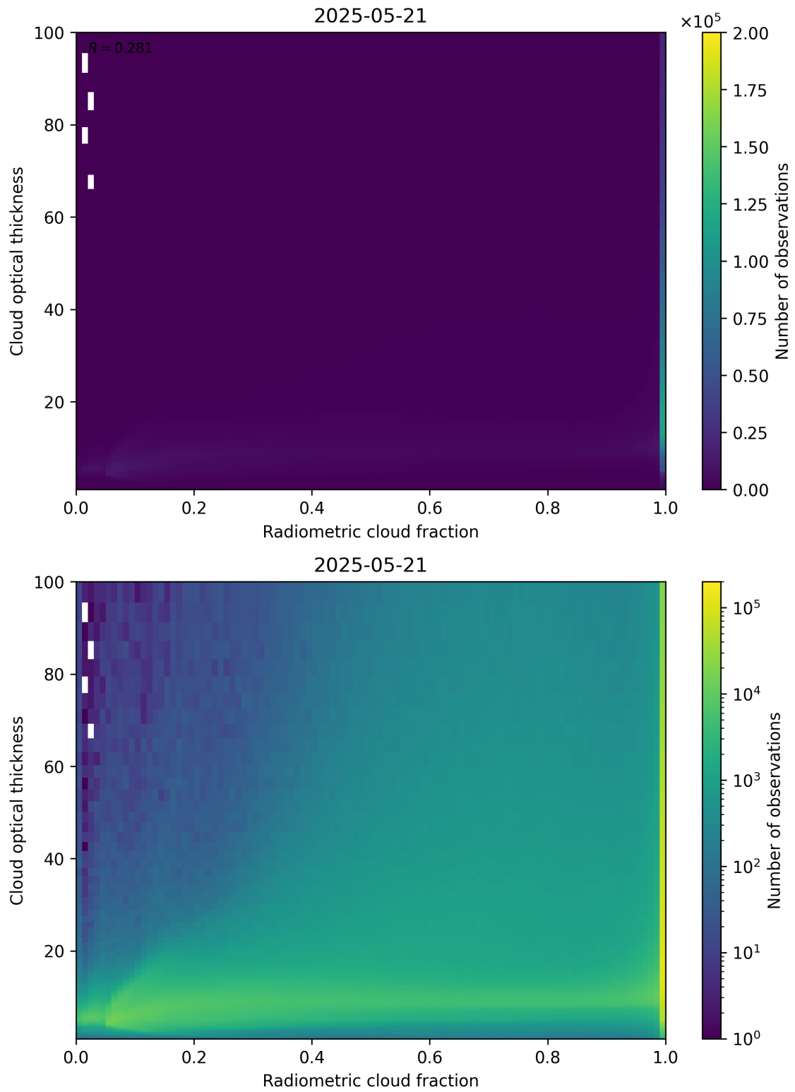
Figure 75: Scatter density plot of “Radiometric cloud fraction” against “Cloud optical thickness” for 2025-05-21 to 2025-05-22.
