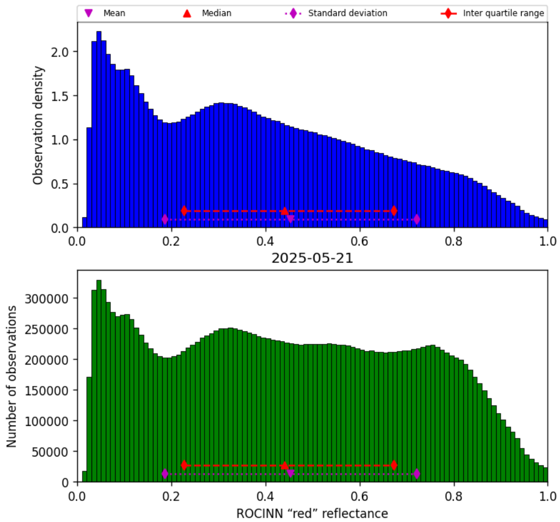
Figure 53: Histogram of “ROCINN “red” reflectance” for 2025-05-21 to 2025-05-22
