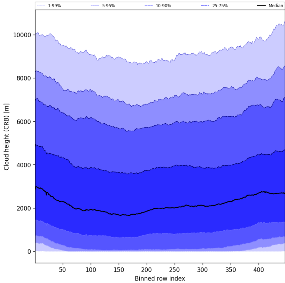
Figure 59: Along track statistics of “Cloud height (CRB)” for 2025-05-21 to 2025-05-22
