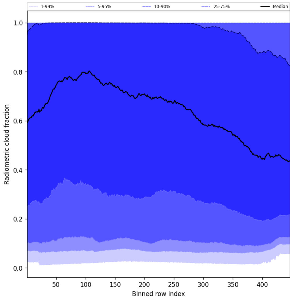
Figure 55: Along track statistics of “Radiometric cloud fraction” for 2025-05-21 to 2025-05-22
