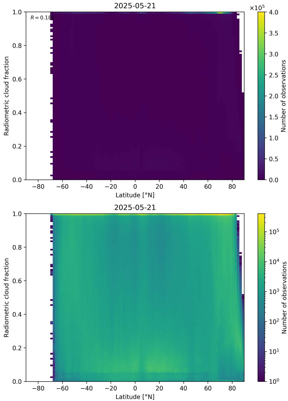
Figure 92: Scatter density plot of “Latitude” against “Radiometric cloud fraction” for 2025-05-21 to 2025-05-22.
