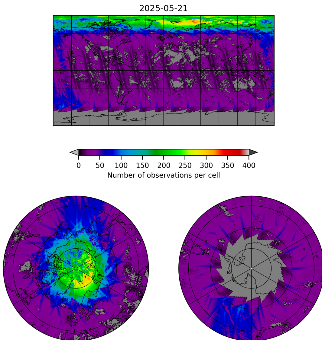
Figure 21: Map of the number of observations for 2025-05-21 to 2025-05-22
