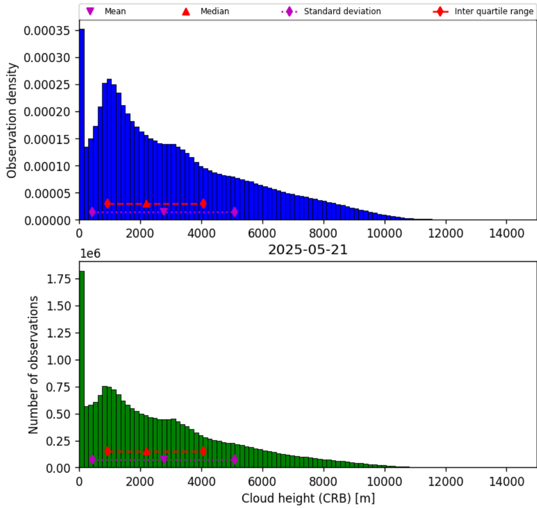
Figure 43: Histogram of “Cloud height (CRB)” for 2025-05-21 to 2025-05-22
