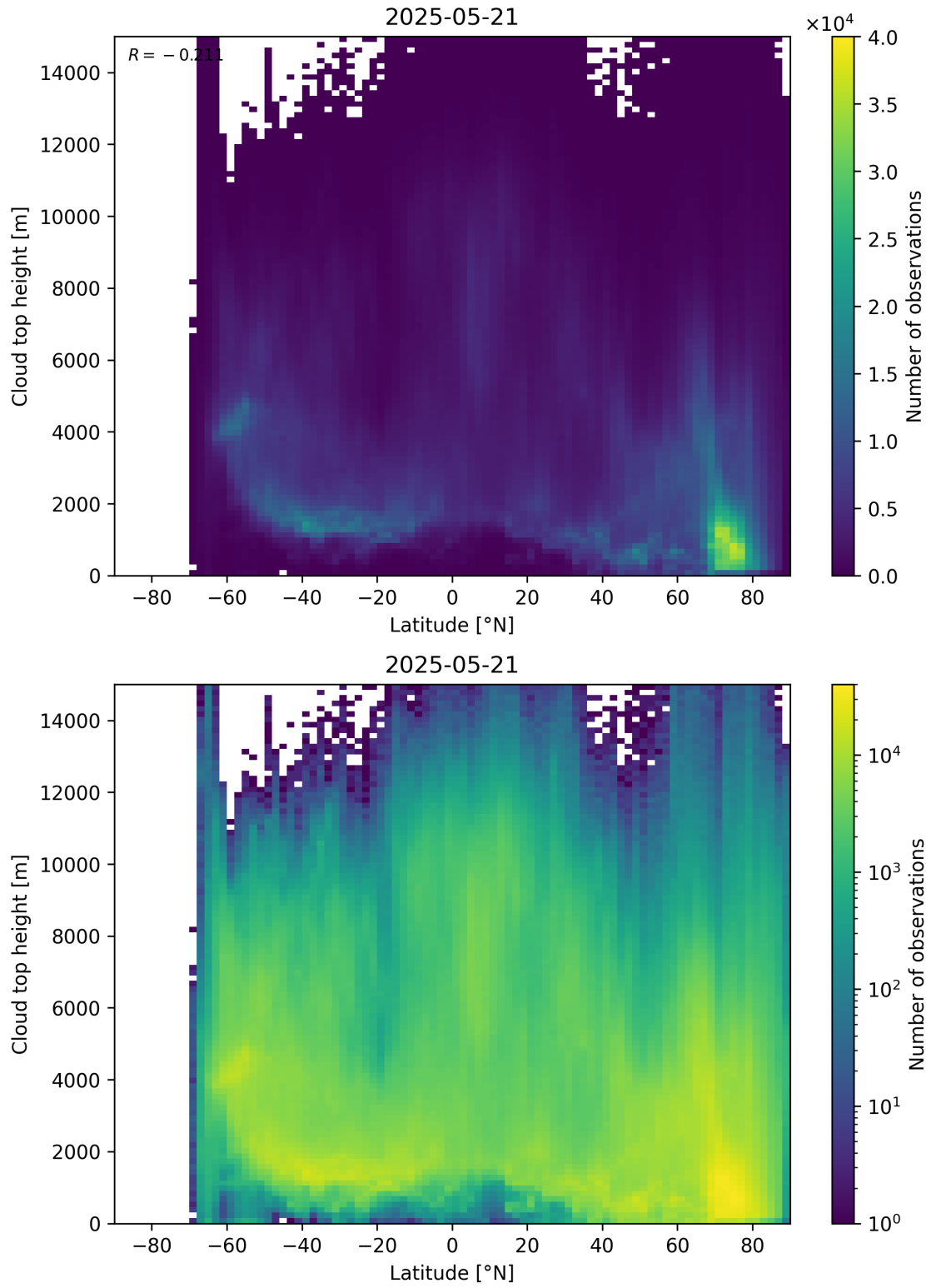
Figure 97: Scatter density plot of “Latitude” against “Cloud top height” for 2025-05-21 to 2025-05-22.
