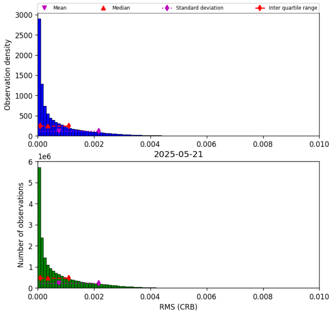
Figure 48: Histogram of “RMS (CRB)” for 2025-05-21 to 2025-05-22
