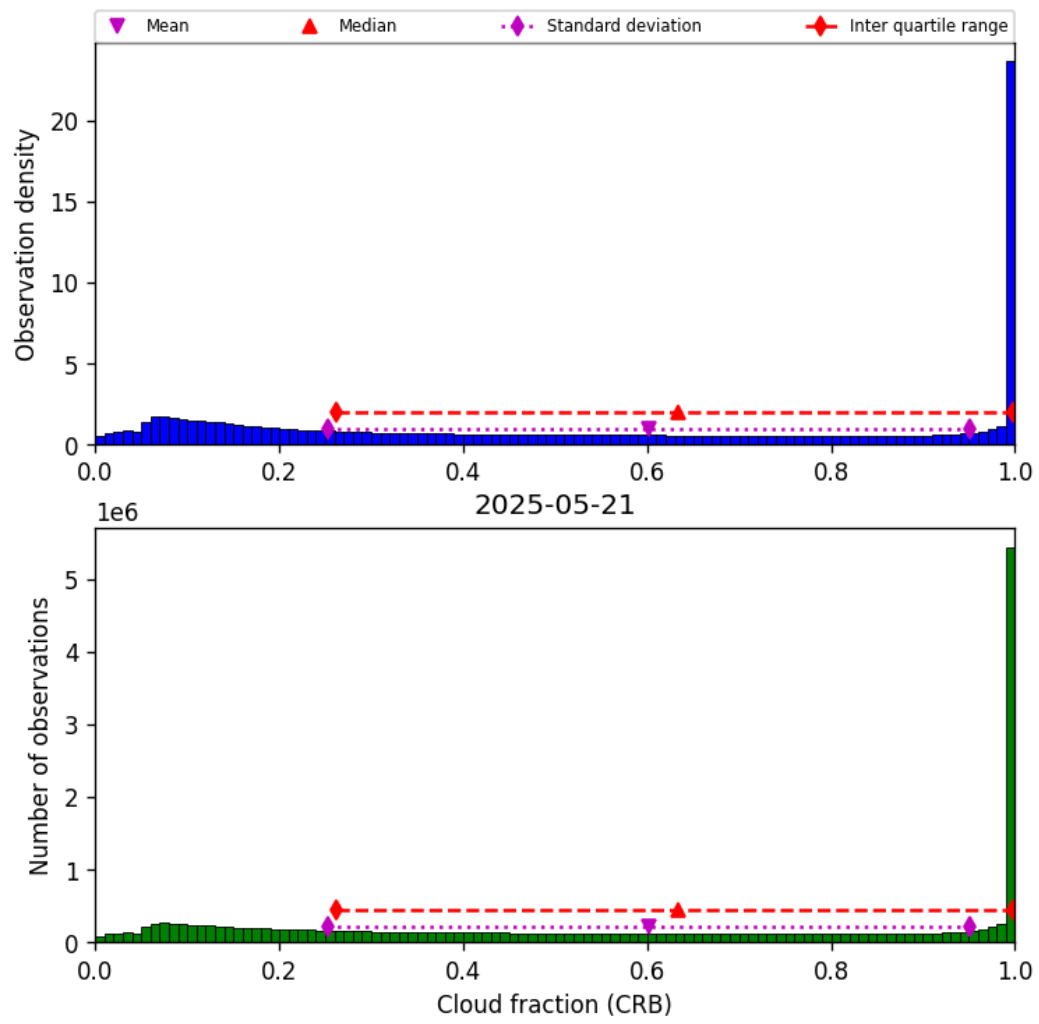
Figure 42: Histogram of “Cloud fraction (CRB)” for 2025-05-21 to 2025-05-22
