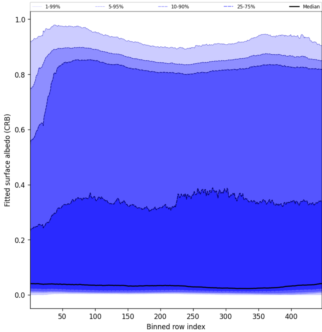
Figure 62: Along track statistics of “Fitted surface albedo (CRB)” for 2025-05-21 to 2025-05-22
