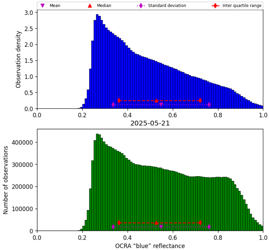
Figure 51: Histogram of “OCRA “blue” reflectance” for 2025-05-21 to 2025-05-22
