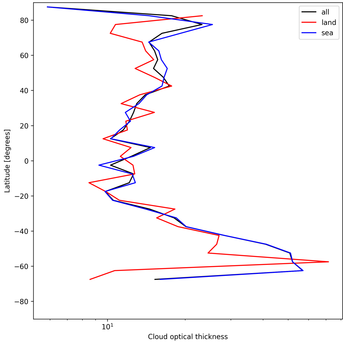
Figure 25: Zonal average of “Cloud optical thickness” for 2025-05-21 to 2025-05-22.
