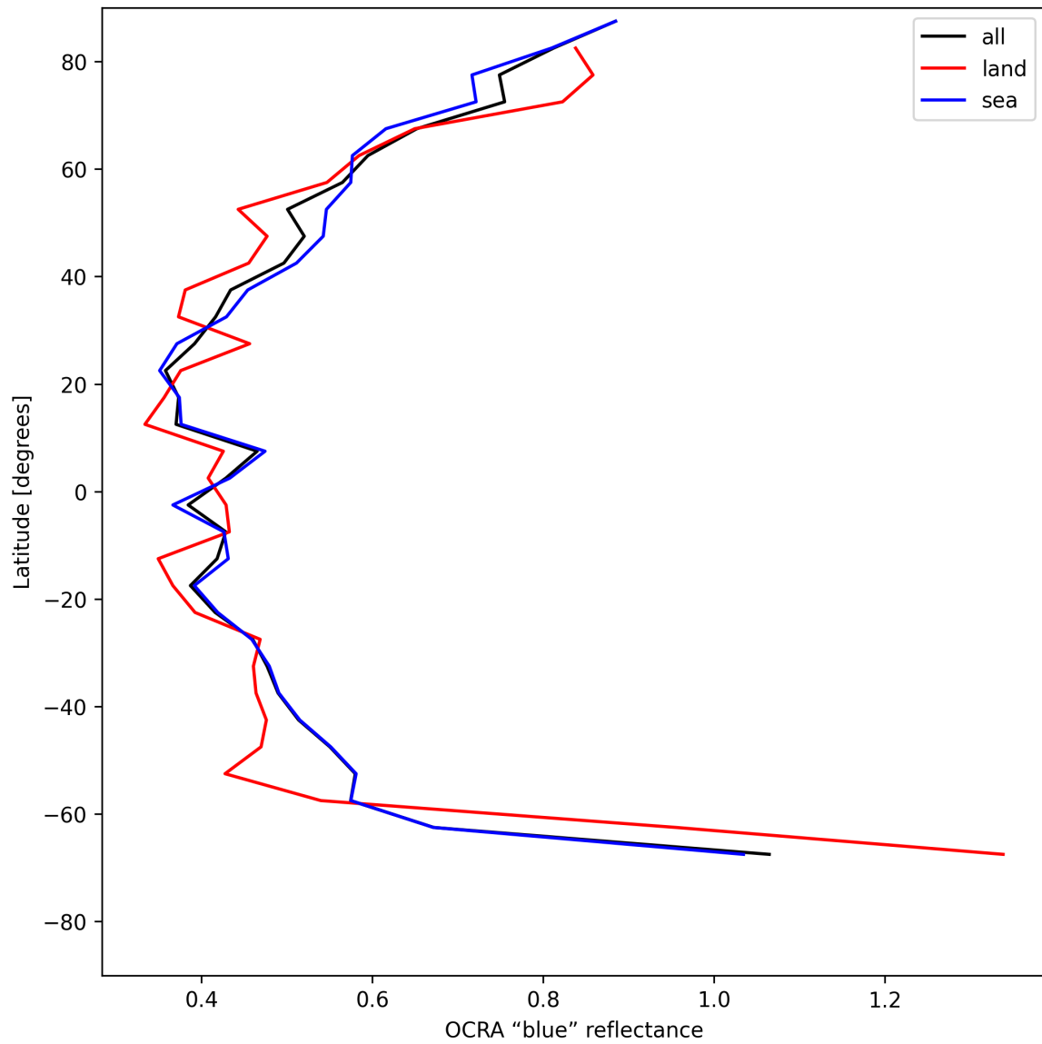
Figure 35: Zonal average of “OCRA “blue” reflectance” for 2025-05-21 to 2025-05-22.
