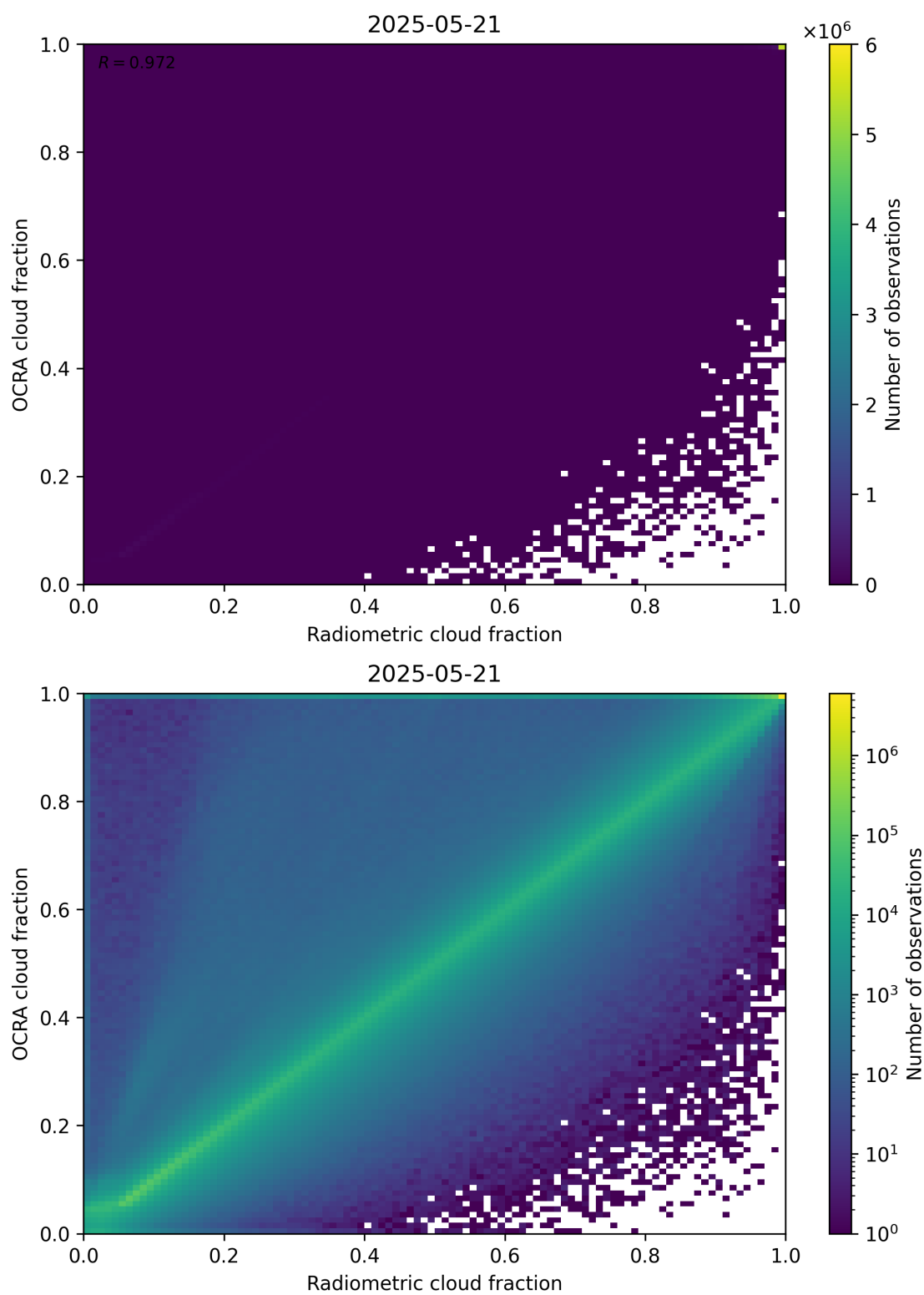
Figure 72: Scatter density plot of “Radiometric cloud fraction” against “OCRA cloud fraction” for 2025-05-21 to 2025-05-22.
