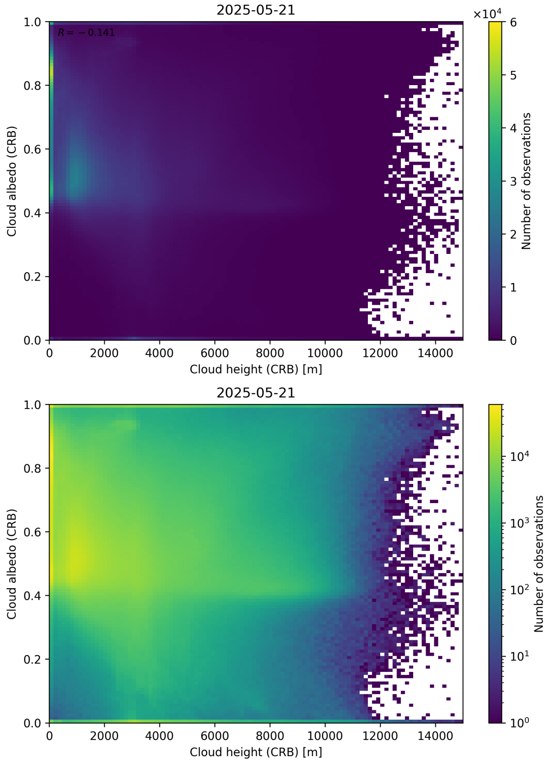
Figure 80: Scatter density plot of “Cloud height (CRB)” against “Cloud albedo (CRB)” for 2025-05-21 to 2025-05-22.
