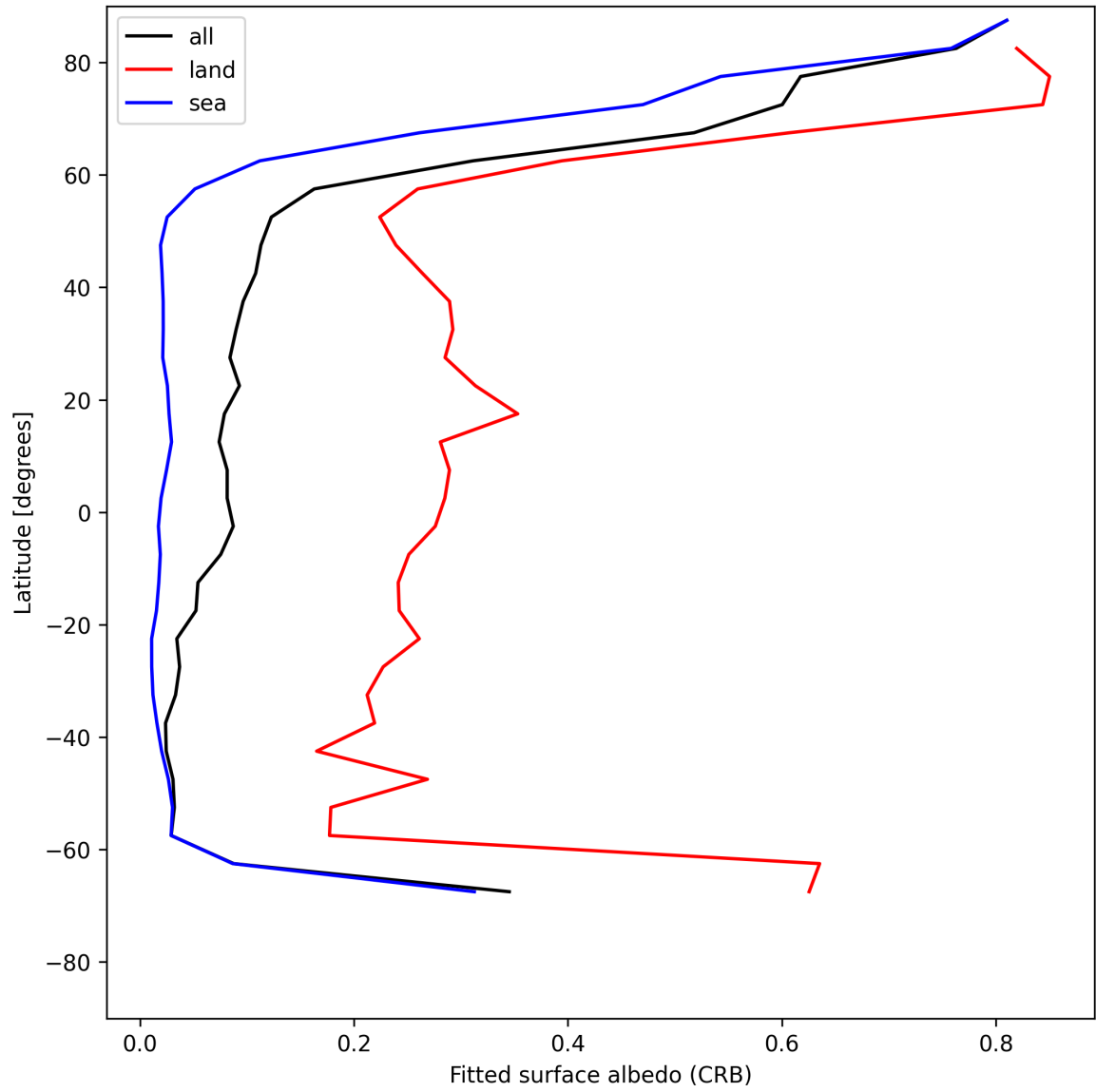
Figure 30: Zonal average of “Fitted surface albedo (CRB)” for 2025-05-21 to 2025-05-22.
