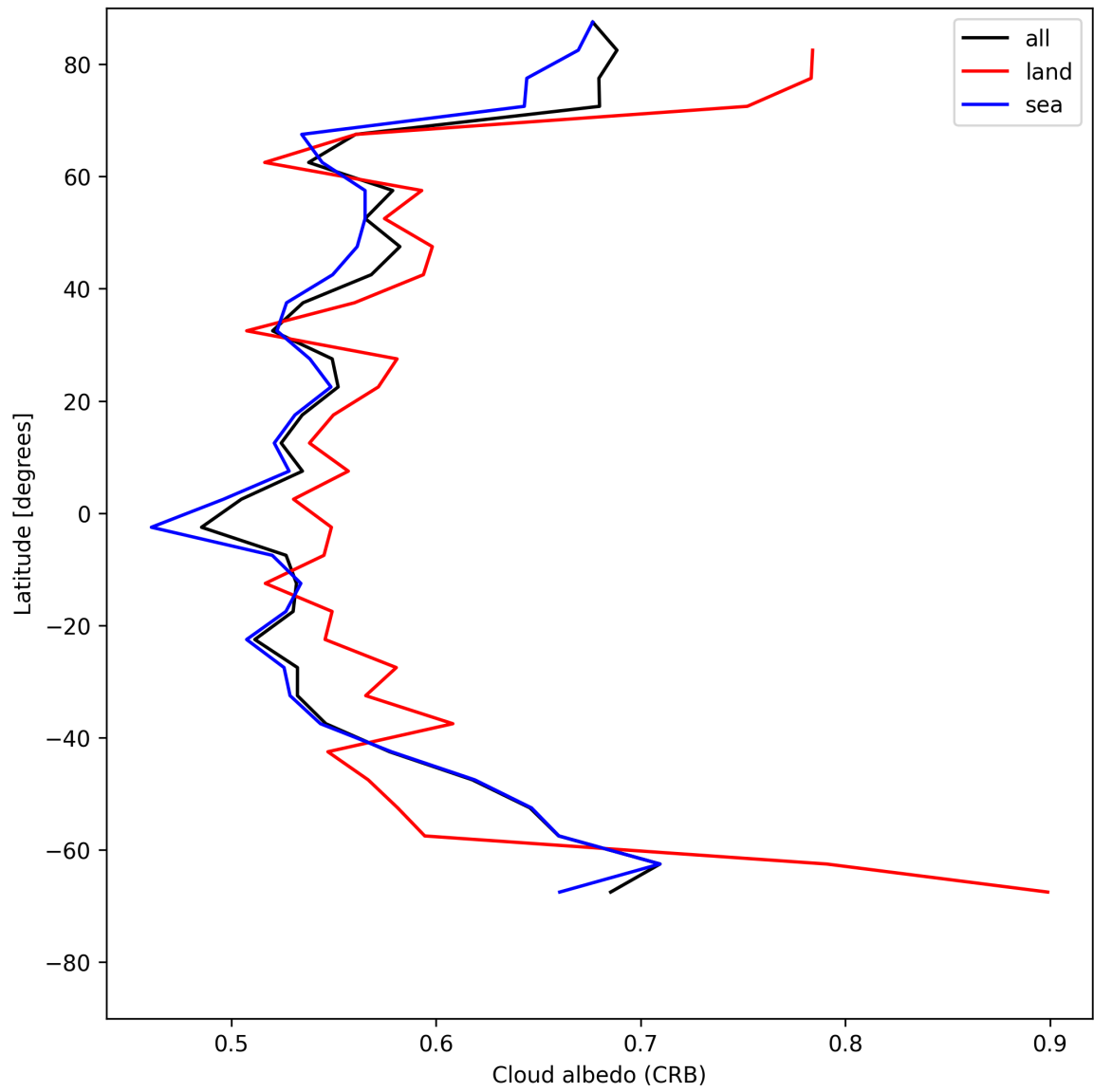
Figure 28: Zonal average of “Cloud albedo (CRB)” for 2025-05-21 to 2025-05-22.
