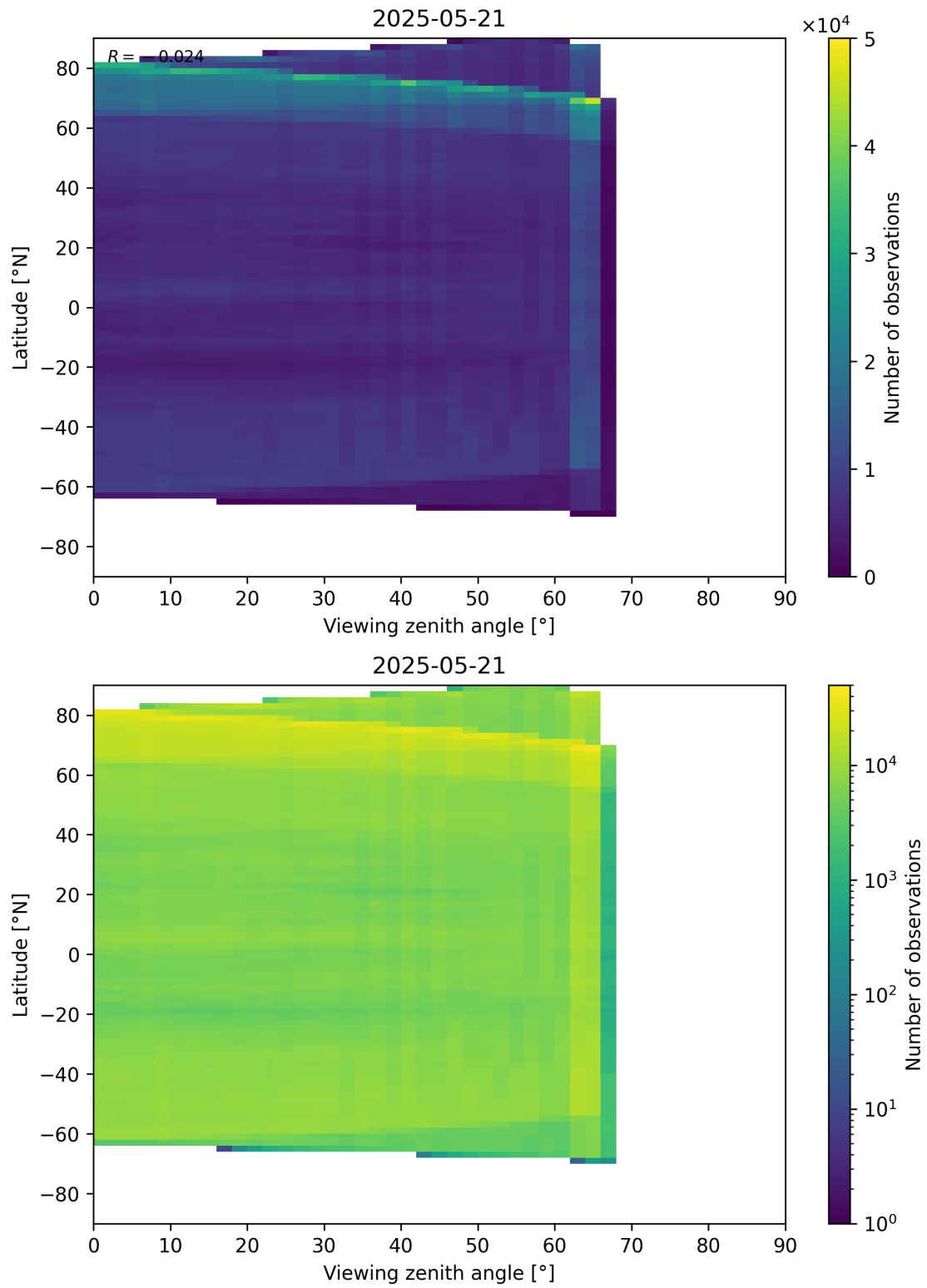
Figure 113: Scatter density plot of “Viewing zenith angle” against “Latitude” for 2025-05-21 to 2025-05-22.
