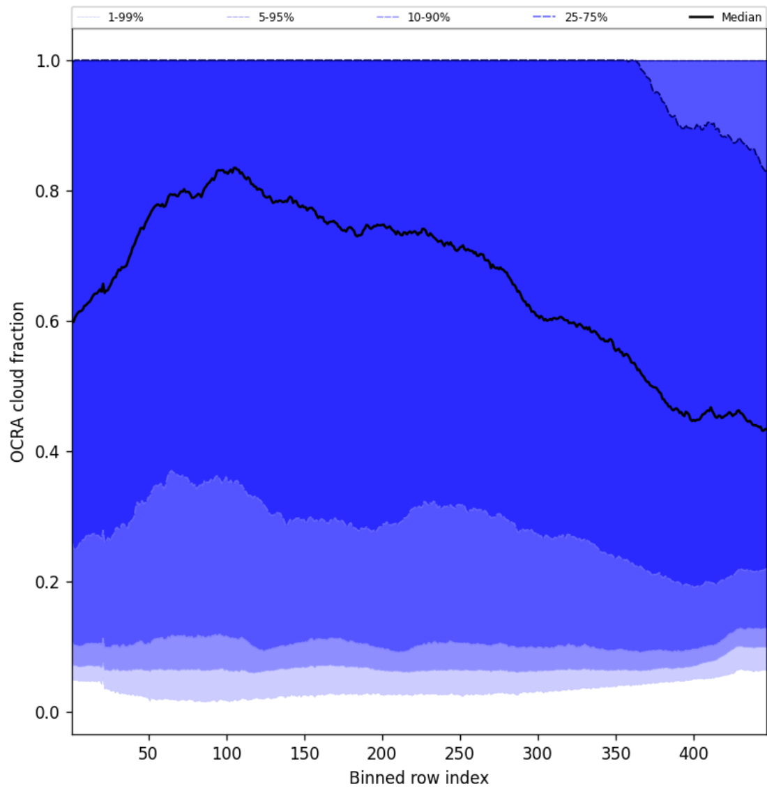
Figure 66: Along track statistics of “OCRA cloud fraction” for 2025-05-21 to 2025-05-22
