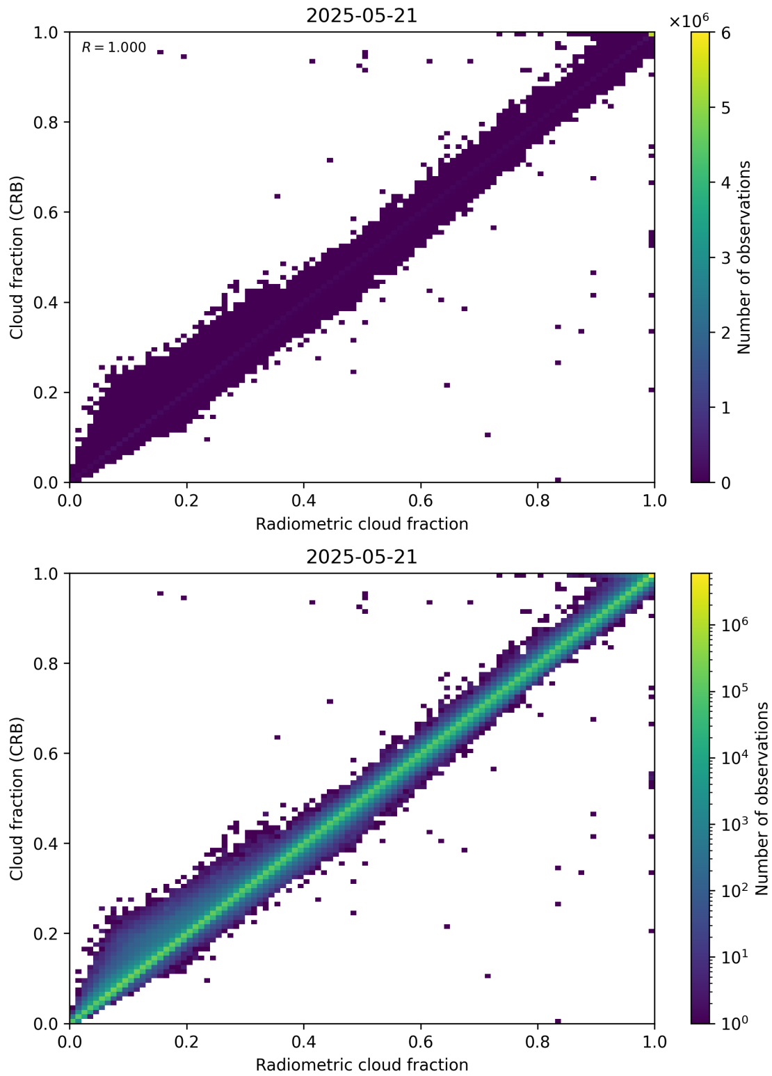
Figure 73: Scatter density plot of “Radiometric cloud fraction” against “Cloud fraction (CRB)” for 2025-05-21 to 2025-05-22.
