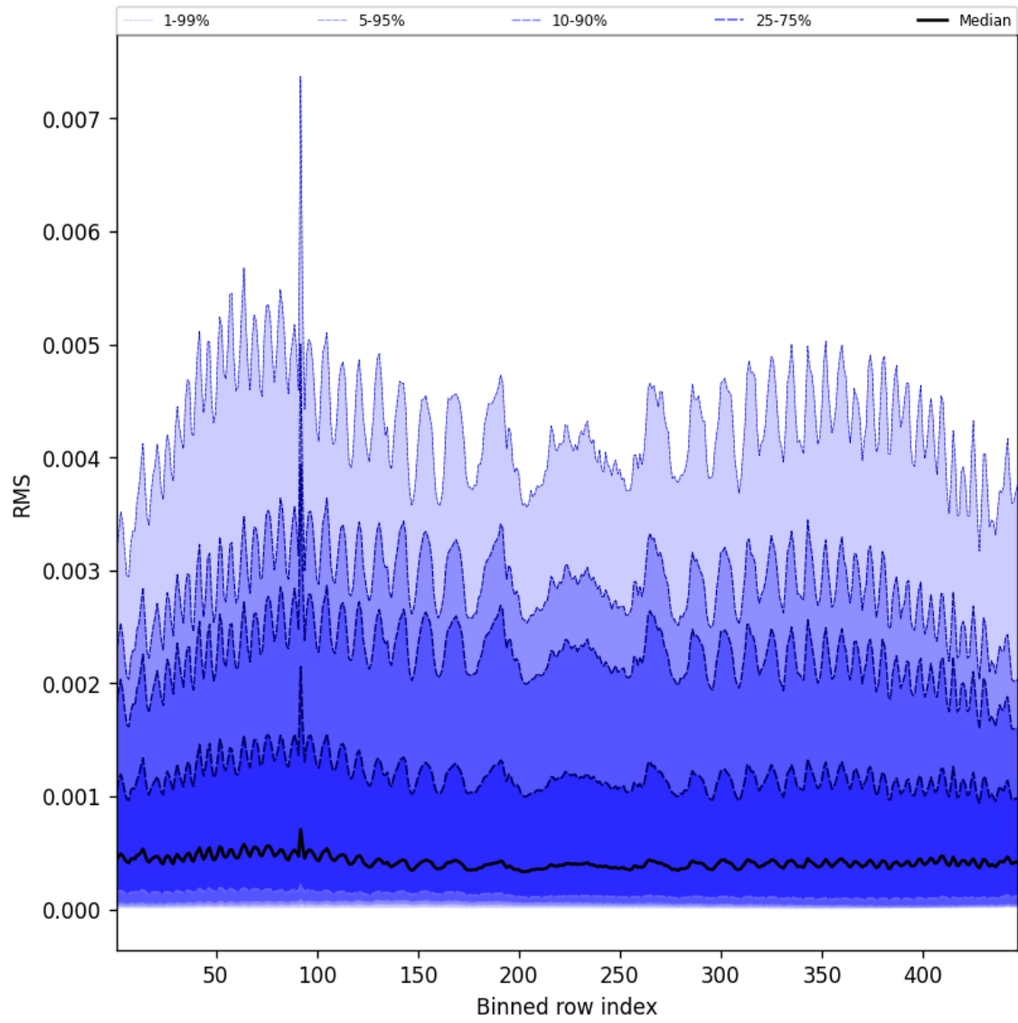
Figure 63: Along track statistics of “RMS” for 2025-05-21 to 2025-05-22
