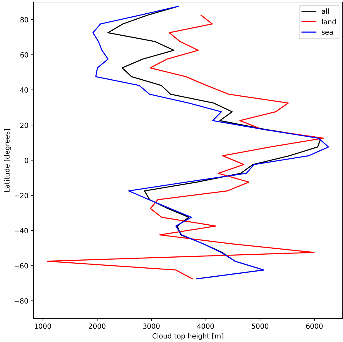
Figure 24: Zonal average of “Cloud top height” for 2025-05-21 to 2025-05-22.
