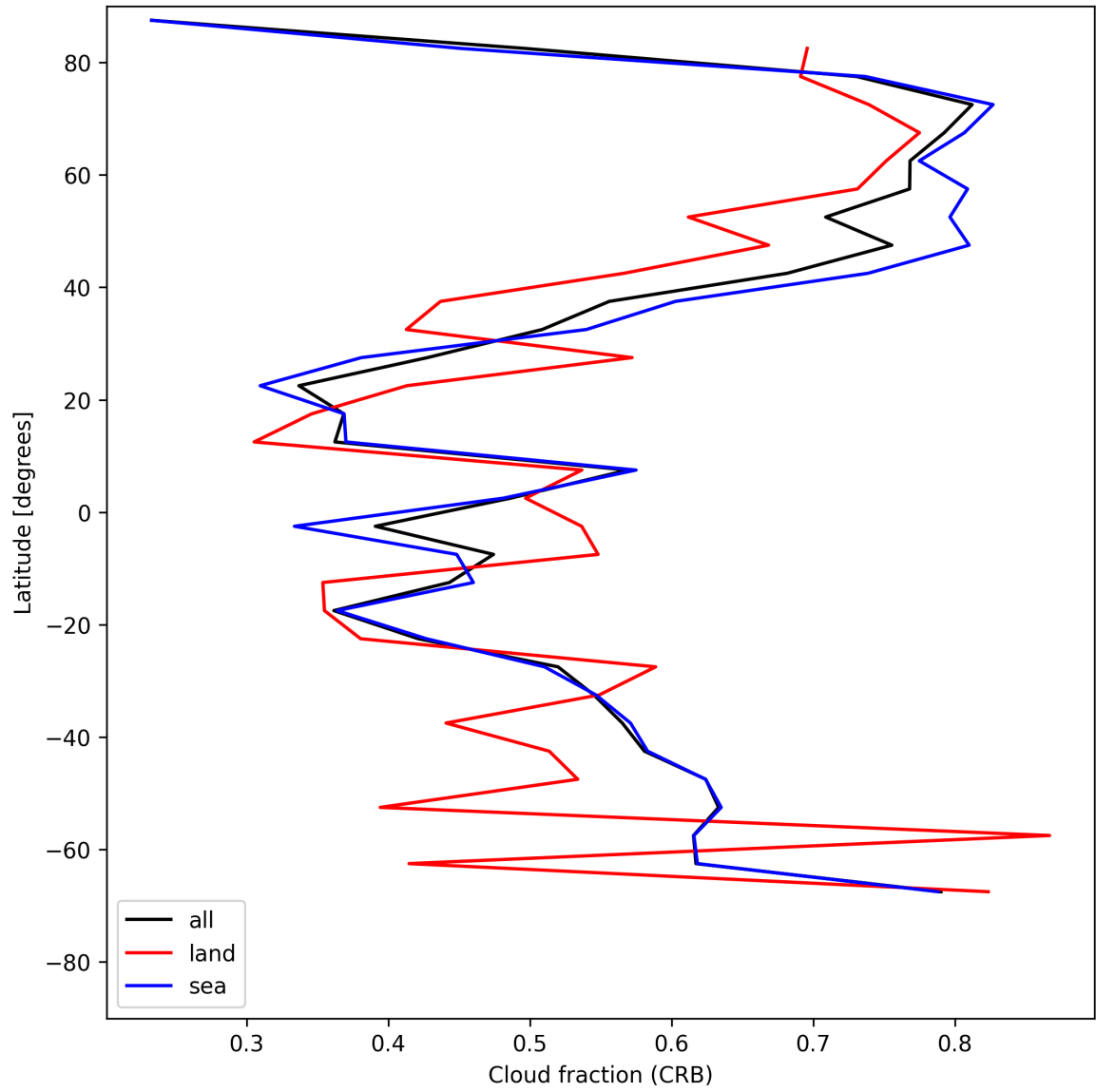
Figure 26: Zonal average of “Cloud fraction (CRB)” for 2025-05-21 to 2025-05-22.
