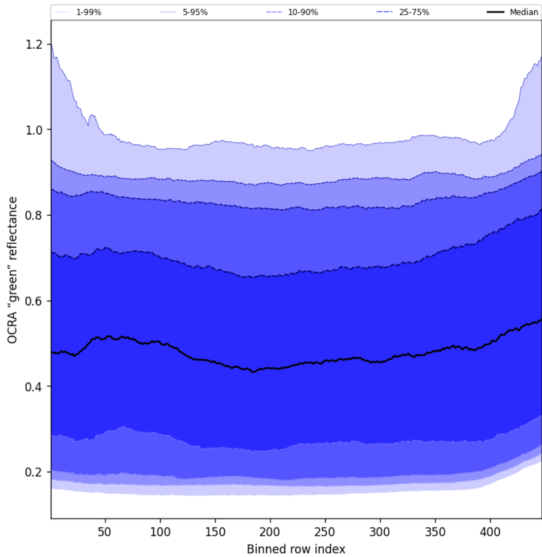
Figure 68: Along track statistics of "OCRA "green" reflectance" for 2025-05-21 to 2025-05-22
