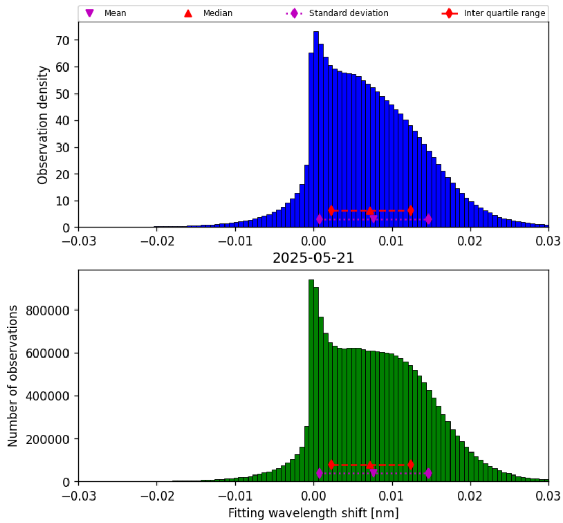
Figure 49: Histogram of “Fitting wavelength shift” for 2025-05-21 to 2025-05-22
