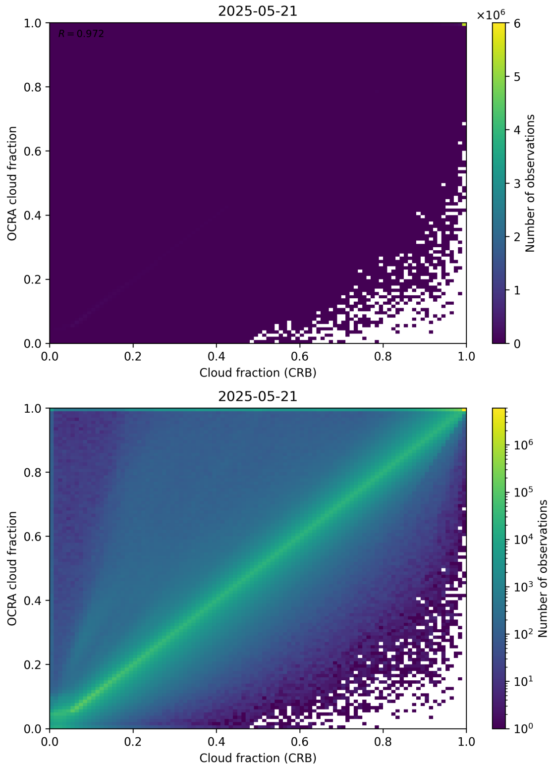
Figure 78: Scatter density plot of “Cloud fraction (CRB)” against “OCRA cloud fraction” for 2025-05-21 to 2025-05-22.
