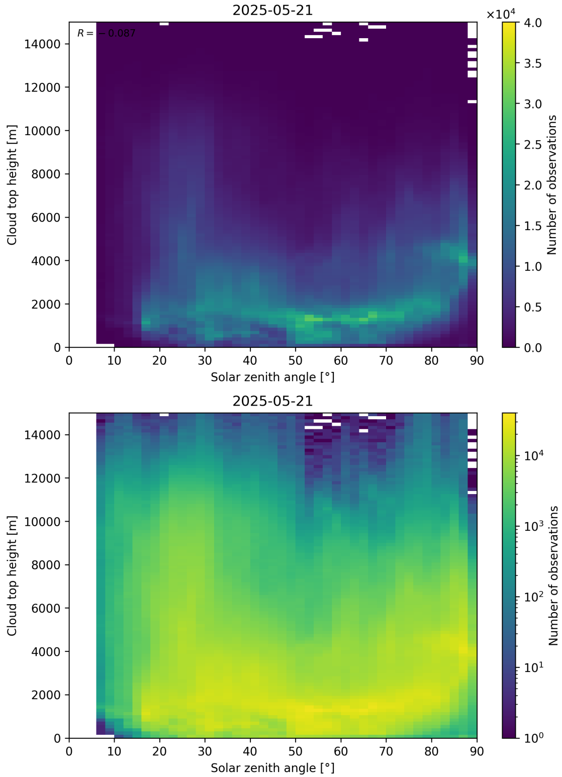
Figure 104: Scatter density plot of “Solar zenith angle” against “Cloud top height” for 2025-05-21 to 2025-05-22.
