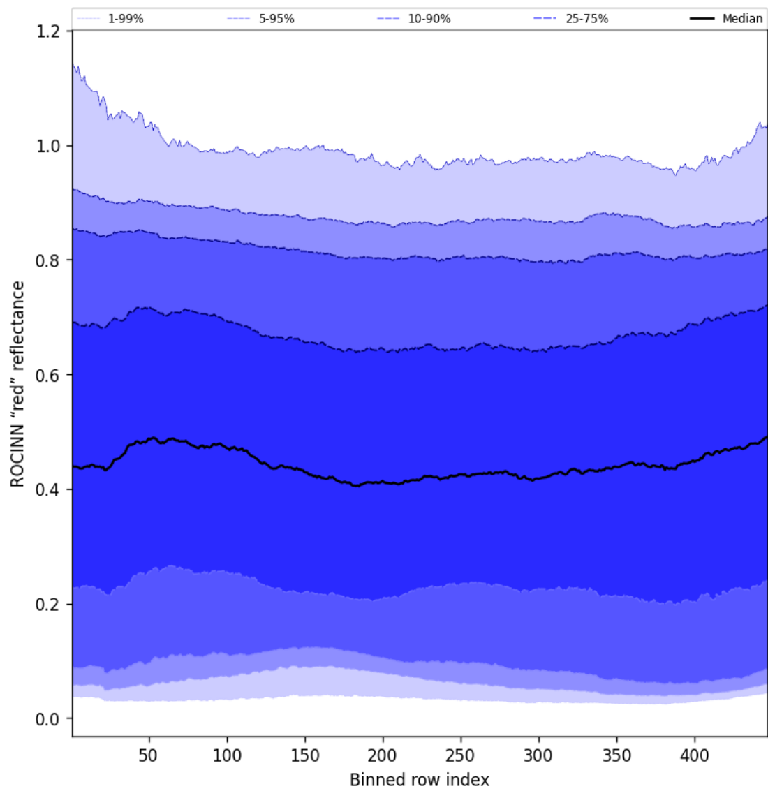
Figure 69: Along track statistics of “ROCINN “red” reflectance” for 2025-05-21 to 2025-05-22
