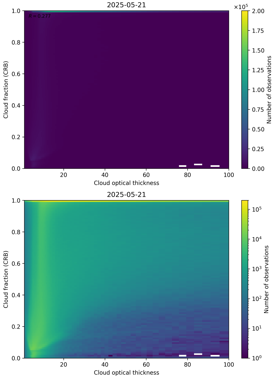
Figure 84: Scatter density plot of “Cloud optical thickness” against “Cloud fraction (CRB)” for 2025-05-21 to 2025-05-22.
