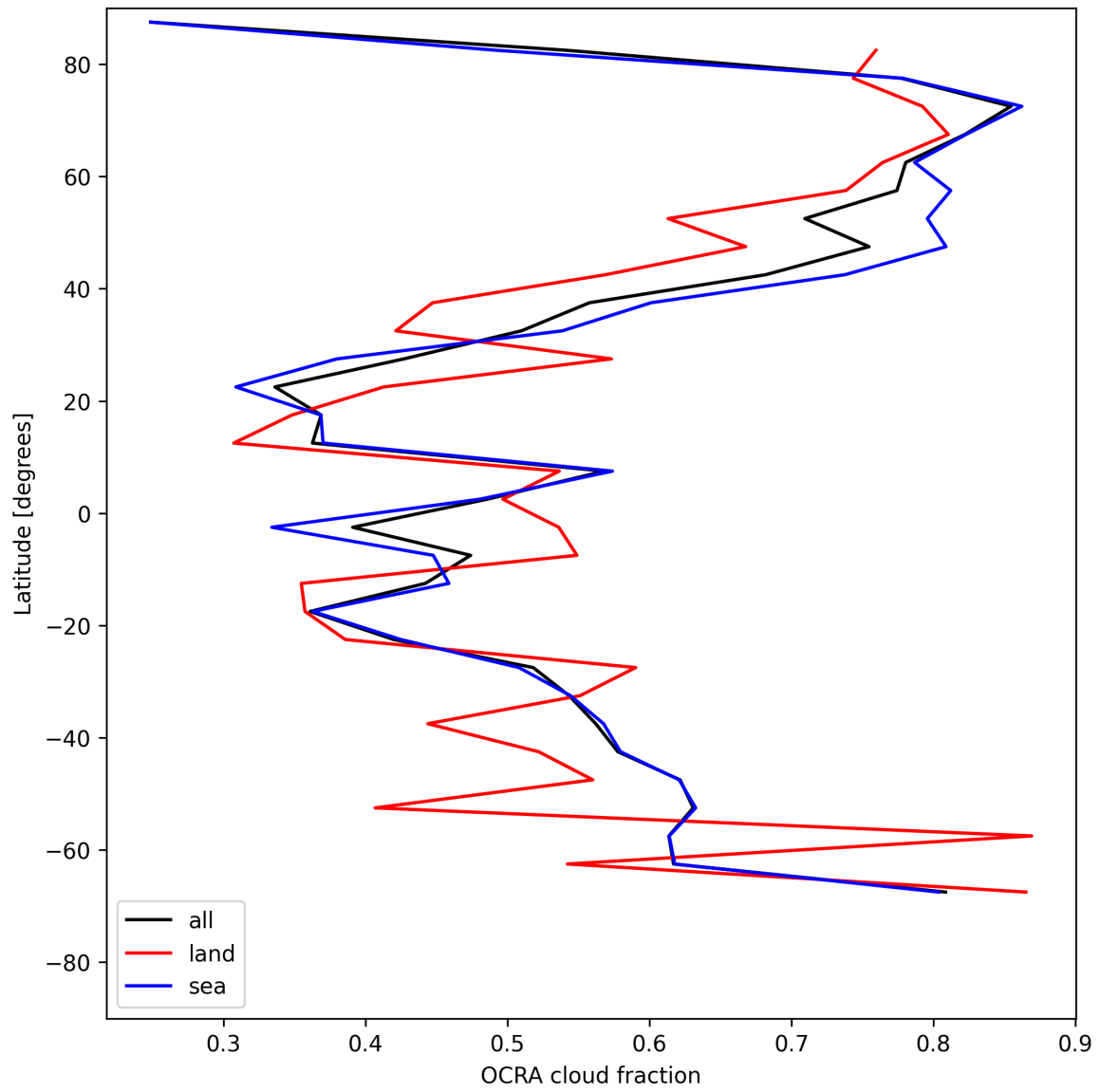
Figure 34: Zonal average of “OCRA cloud fraction” for 2025-05-21 to 2025-05-22.
