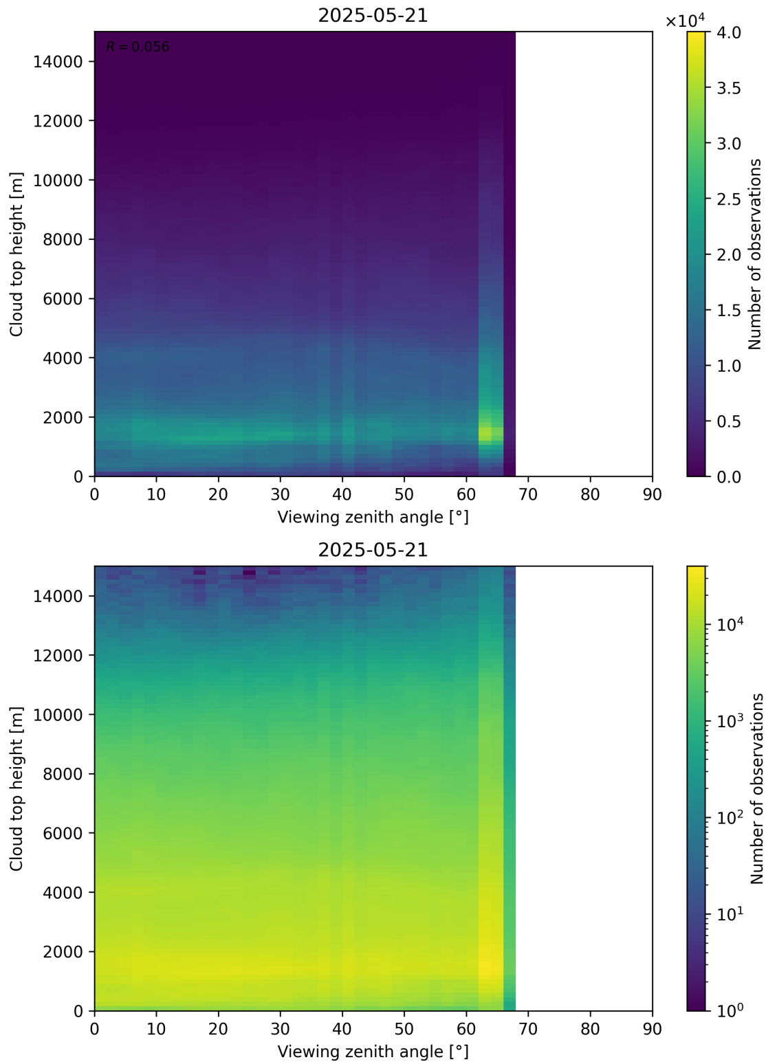
Figure 112: Scatter density plot of “Viewing zenith angle” against “Cloud top height” for 2025-05-21 to 2025-05-22.
