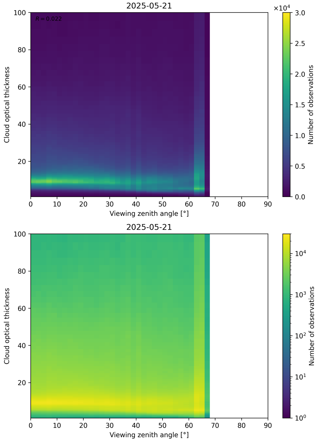
Figure 111: Scatter density plot of “Viewing zenith angle” against “Cloud optical thickness” for 2025-05-21 to 2025-05-22.
