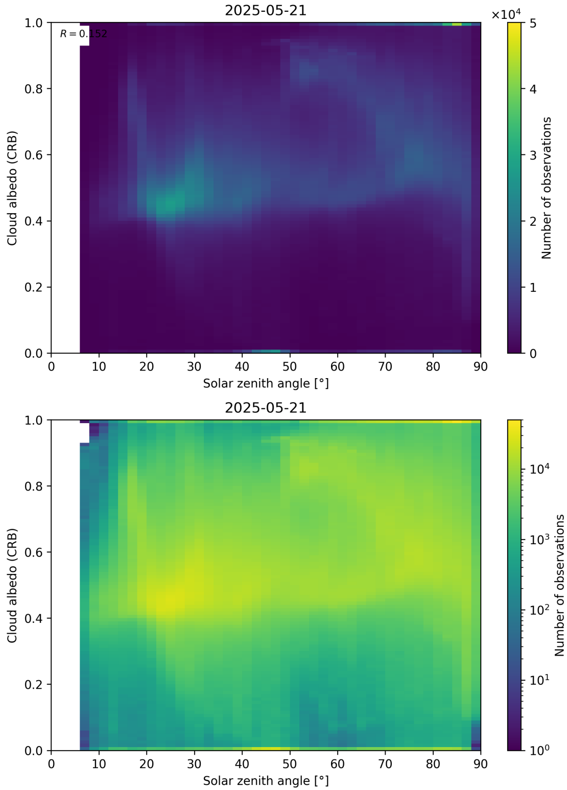
Figure 98: Scatter density plot of “Solar zenith angle” against “Cloud albedo (CRB)” for 2025-05-21 to 2025-05-22.
