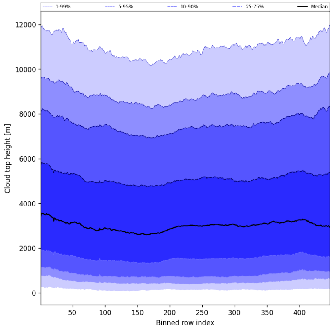
Figure 56: Along track statistics of “Cloud top height” for 2025-05-21 to 2025-05-22
