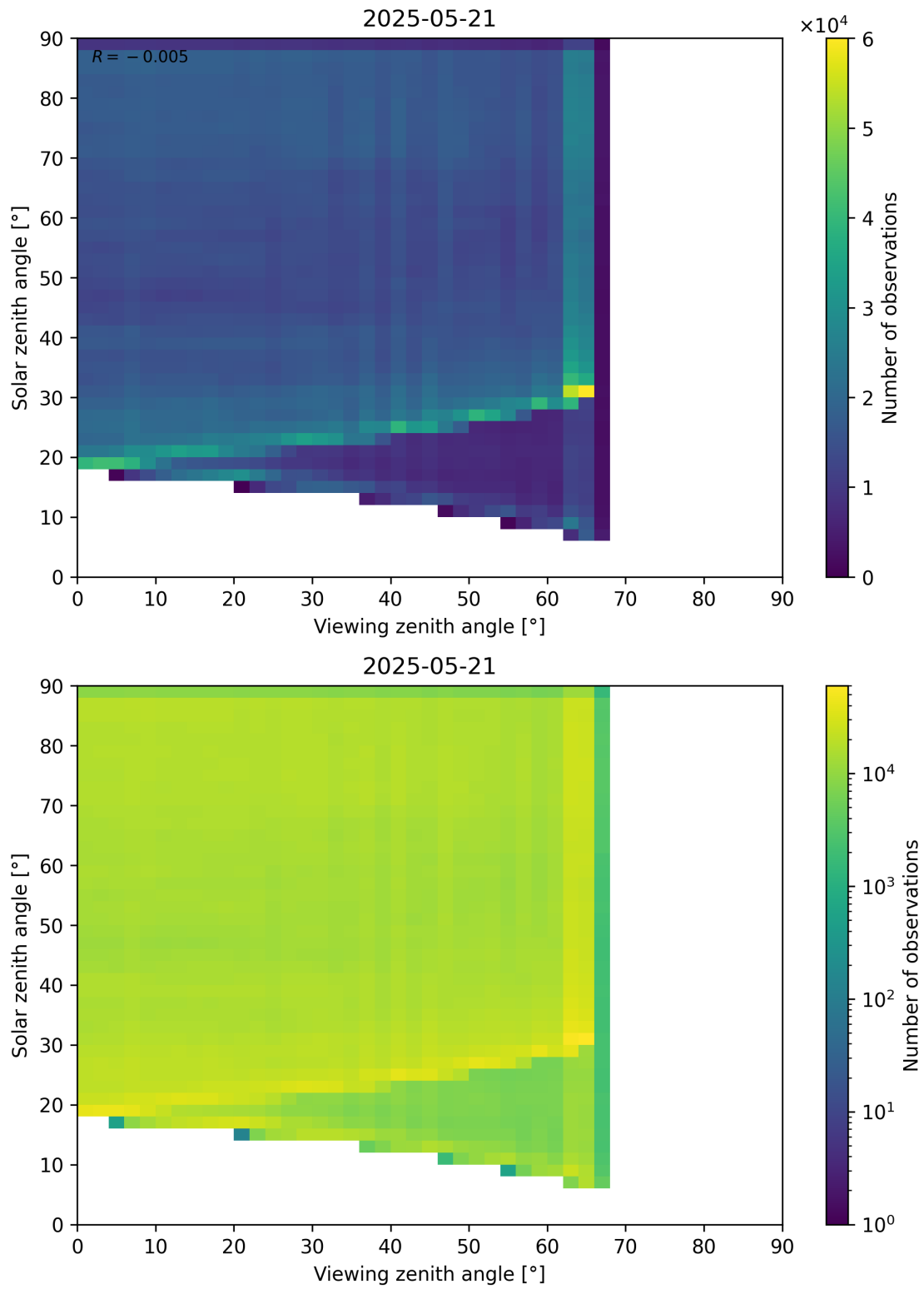
Figure 114: Scatter density plot of “Viewing zenith angle” against “Solar zenith angle” for 2025-05-21 to 2025-05-22.
