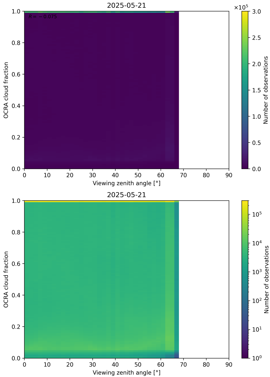
Figure 108: Scatter density plot of “Viewing zenith angle” against “OCRA cloud fraction” for 2025-05-21 to 2025-05-22.
