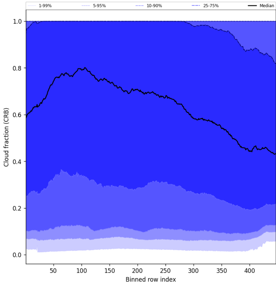
Figure 58: Along track statistics of “Cloud fraction (CRB)” for 2025-05-21 to 2025-05-22
