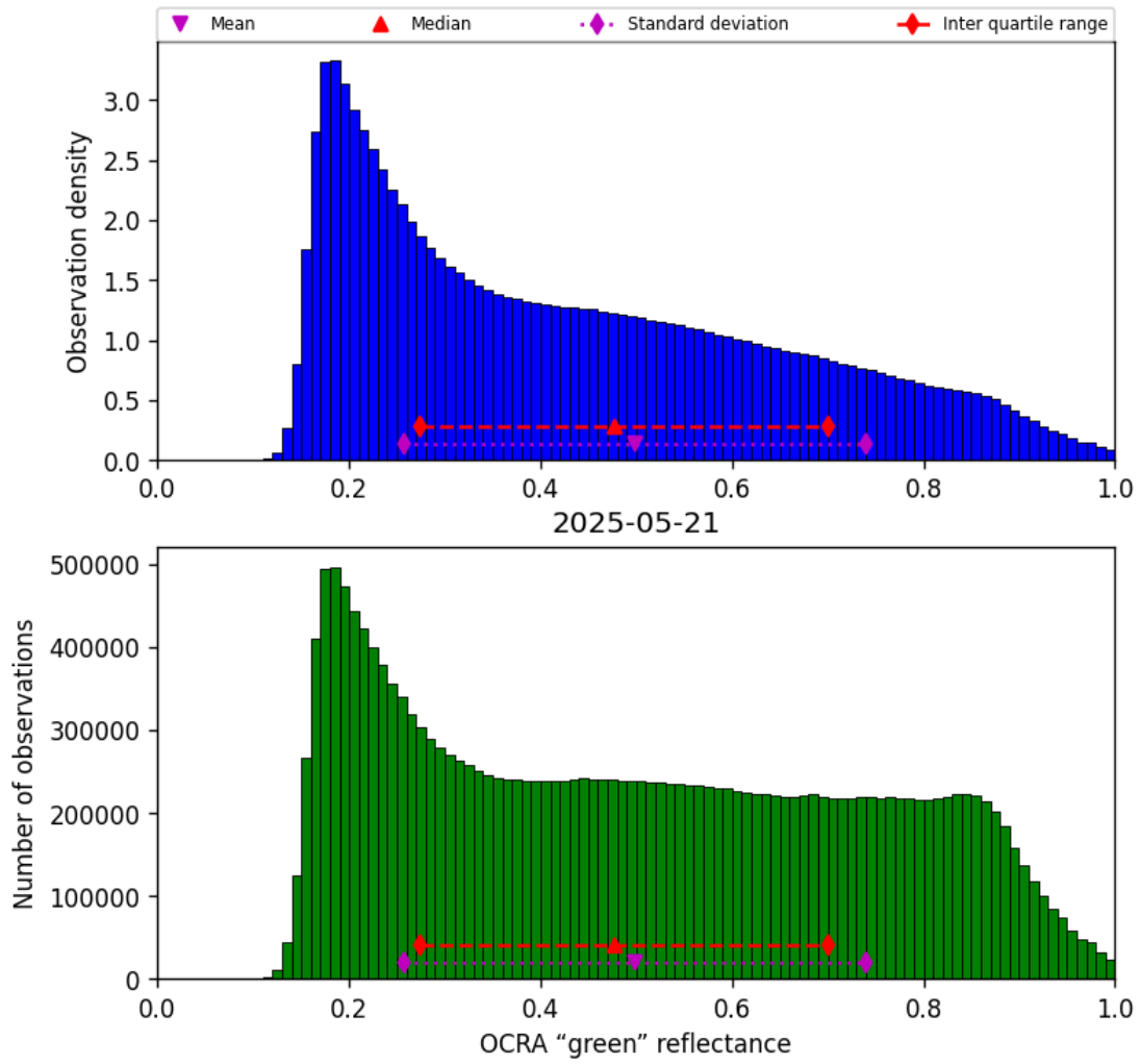
Figure 52: Histogram of “OCRA “green” reflectance” for 2025-05-21 to 2025-05-22
