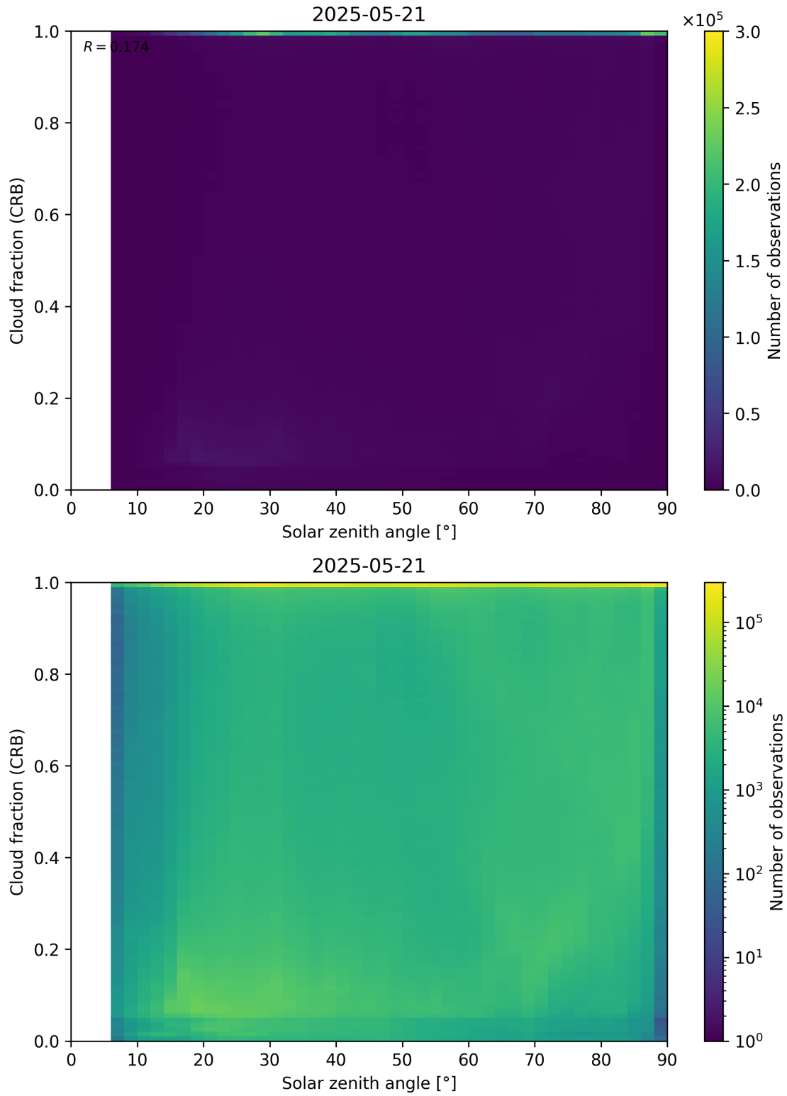
Figure 101: Scatter density plot of “Solar zenith angle” against “Cloud fraction (CRB)” for 2025-05-21 to 2025-05-22.
