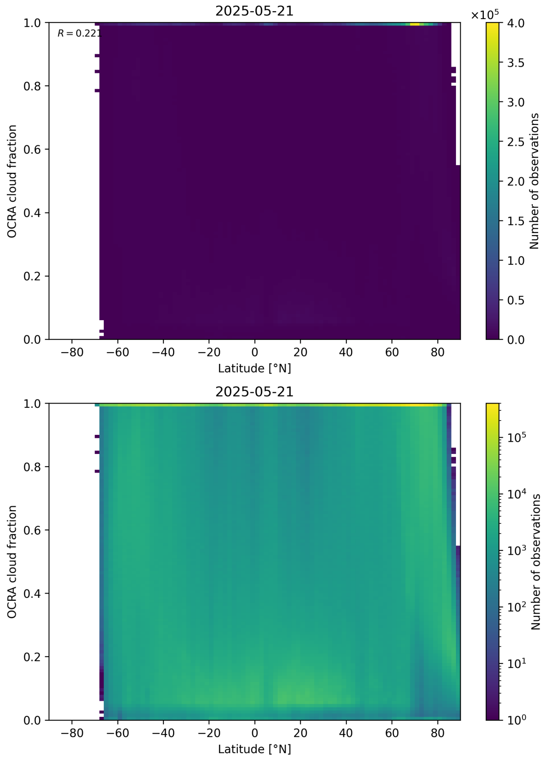
Figure 93: Scatter density plot of “Latitude” against “OCRA cloud fraction” for 2025-05-21 to 2025-05-22.
