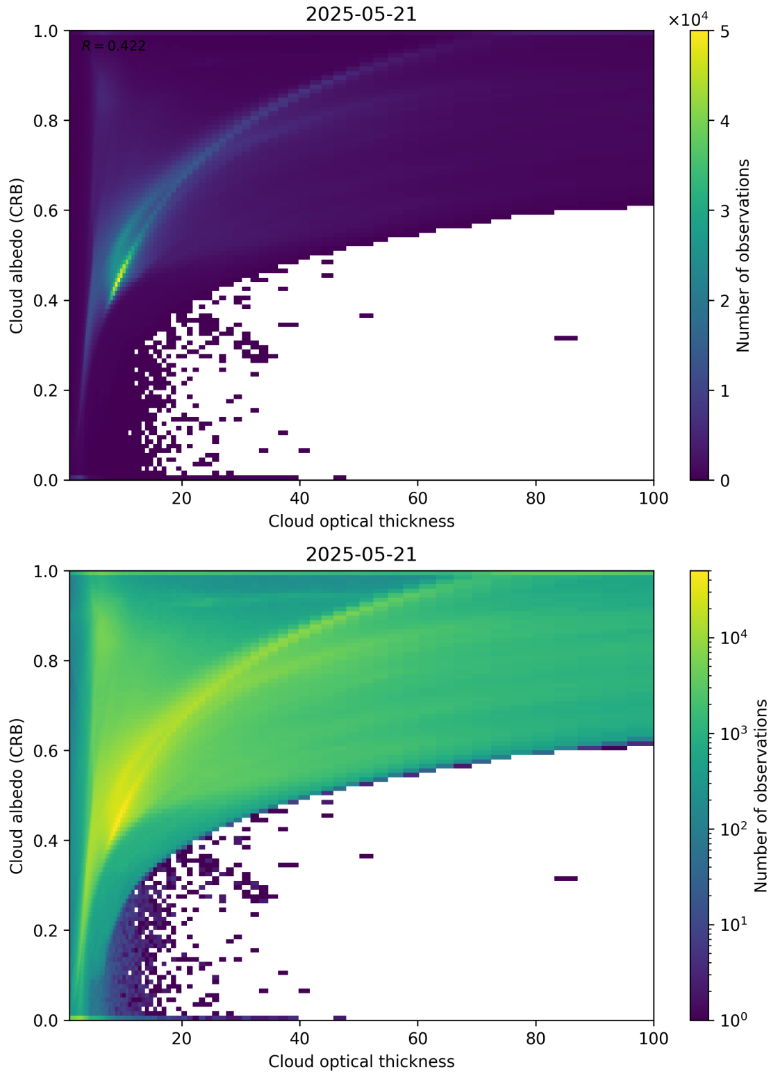
Figure 82: Scatter density plot of “Cloud optical thickness” against “Cloud albedo (CRB)” for 2025-05-21 to 2025-05-22.
