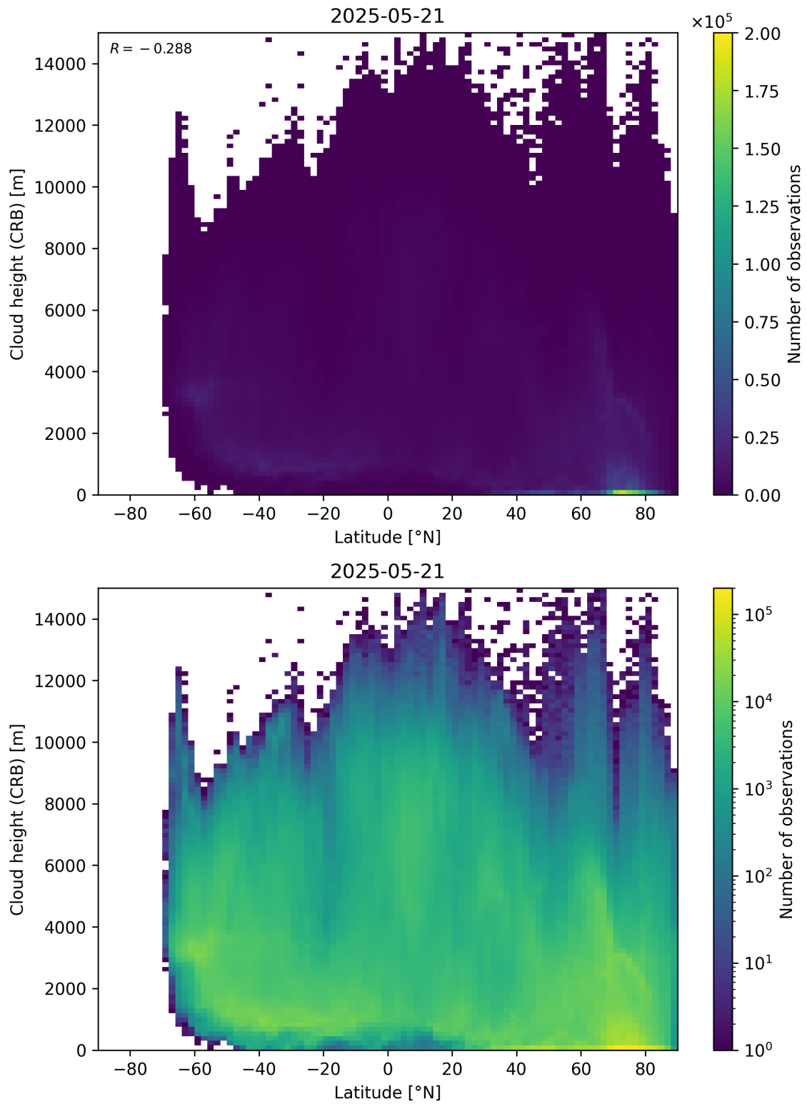
Figure 95: Scatter density plot of “Latitude” against “Cloud height (CRB)” for 2025-05-21 to 2025-05-22.
