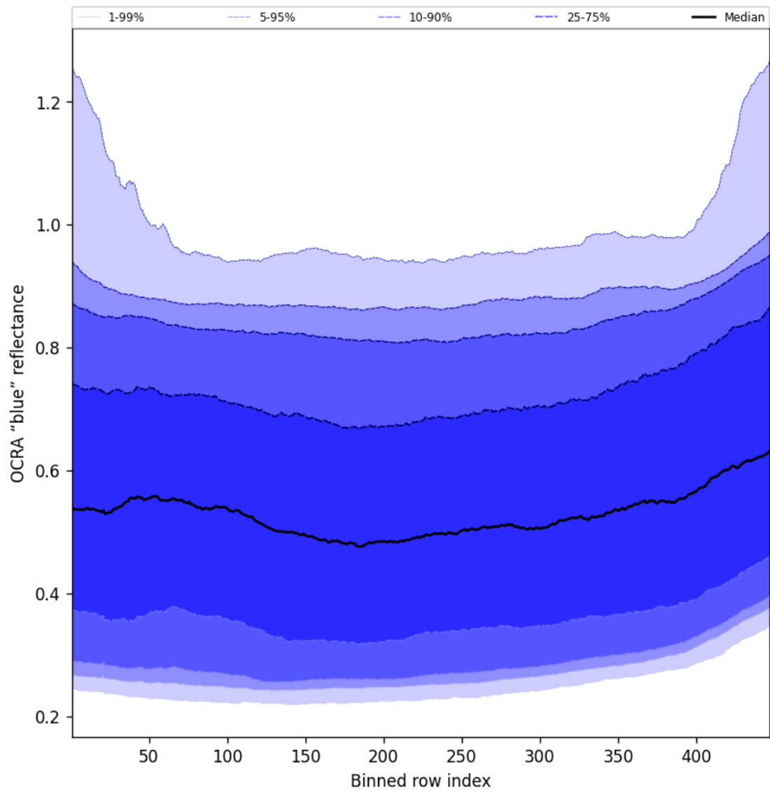
Figure 67: Along track statistics of “OCRA “blue” reflectance” for 2025-05-21 to 2025-05-22
