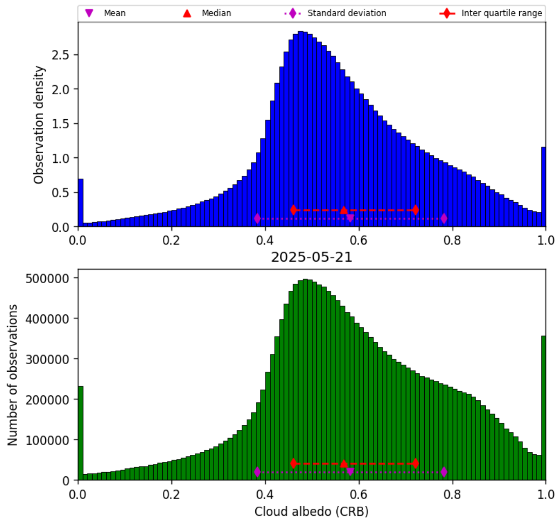
Figure 44: Histogram of “Cloud albedo (CRB)” for 2025-05-21 to 2025-05-22
