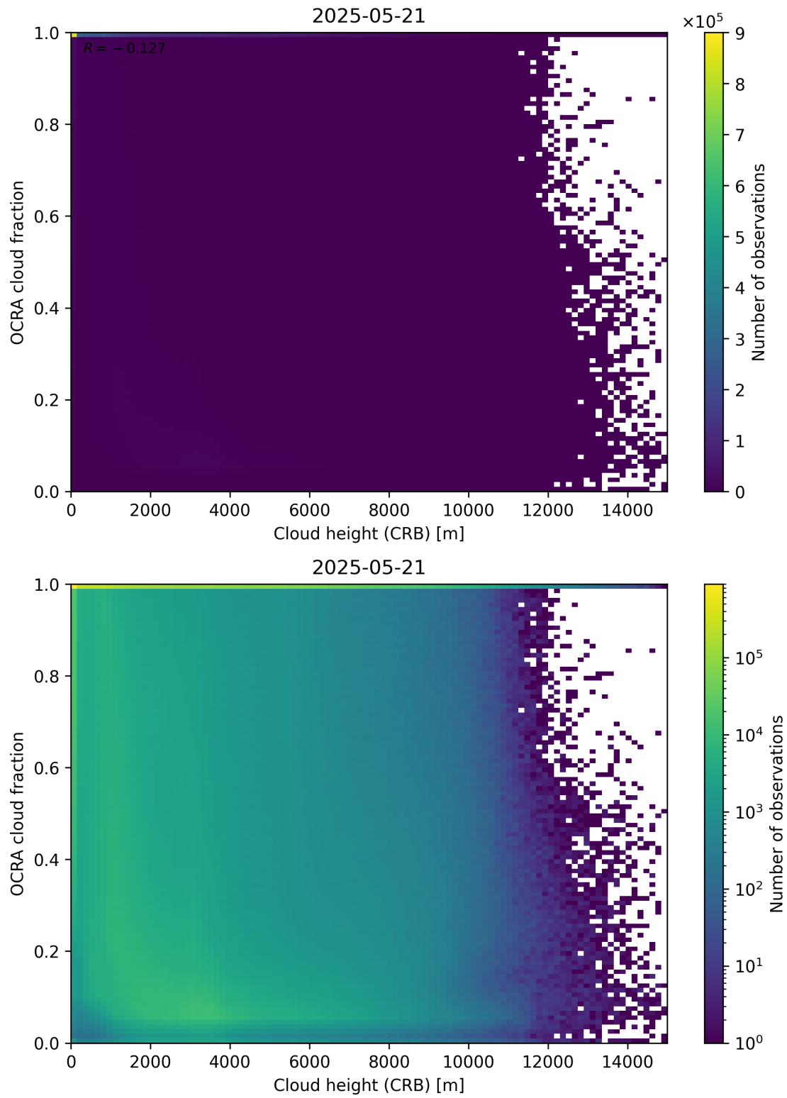
Figure 81: Scatter density plot of “Cloud height (CRB)” against “OCRA cloud fraction” for 2025-05-21 to 2025-05-22.
