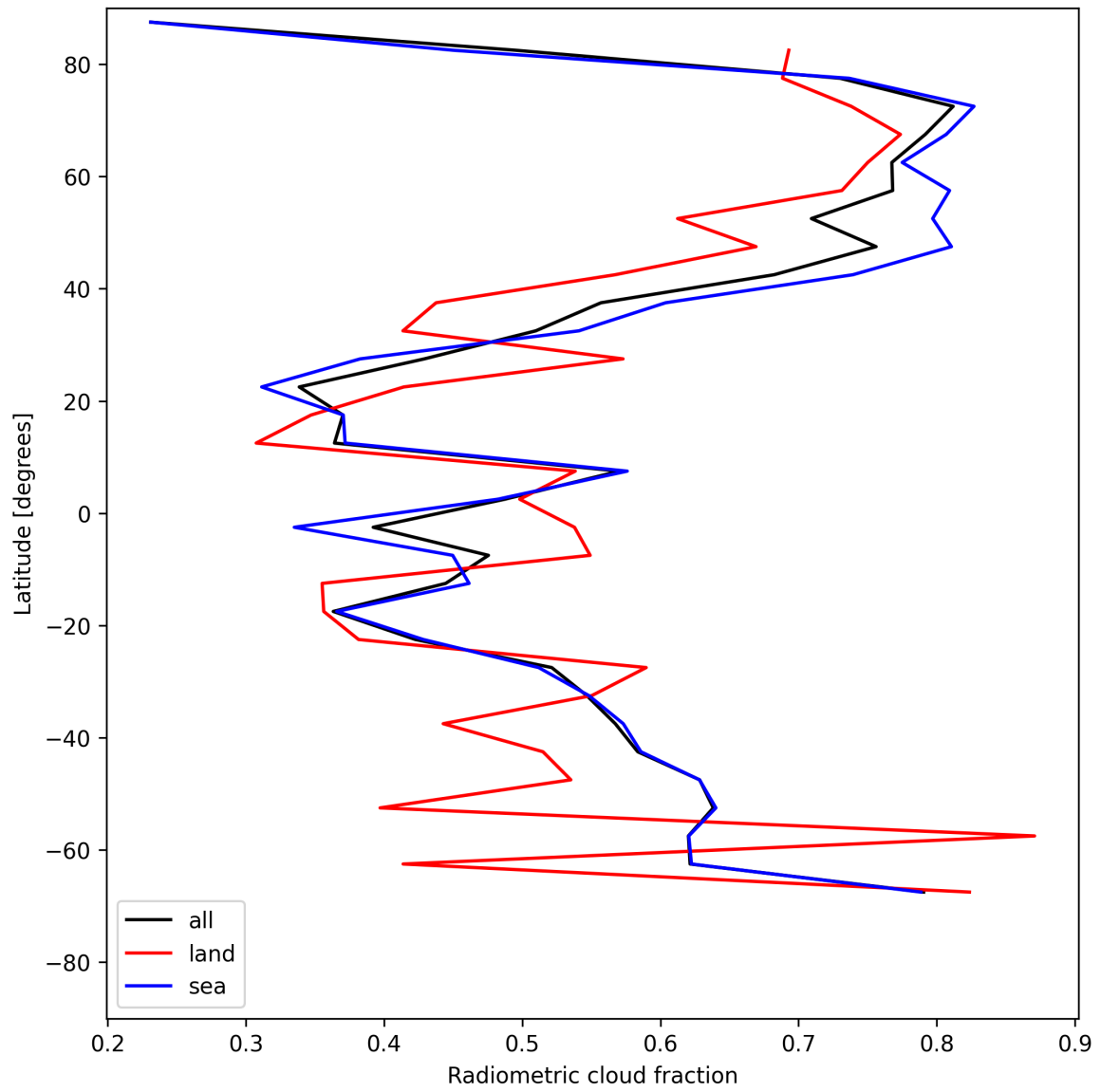
Figure 23: Zonal average of “Radiometric cloud fraction” for 2025-05-21 to 2025-05-22.
