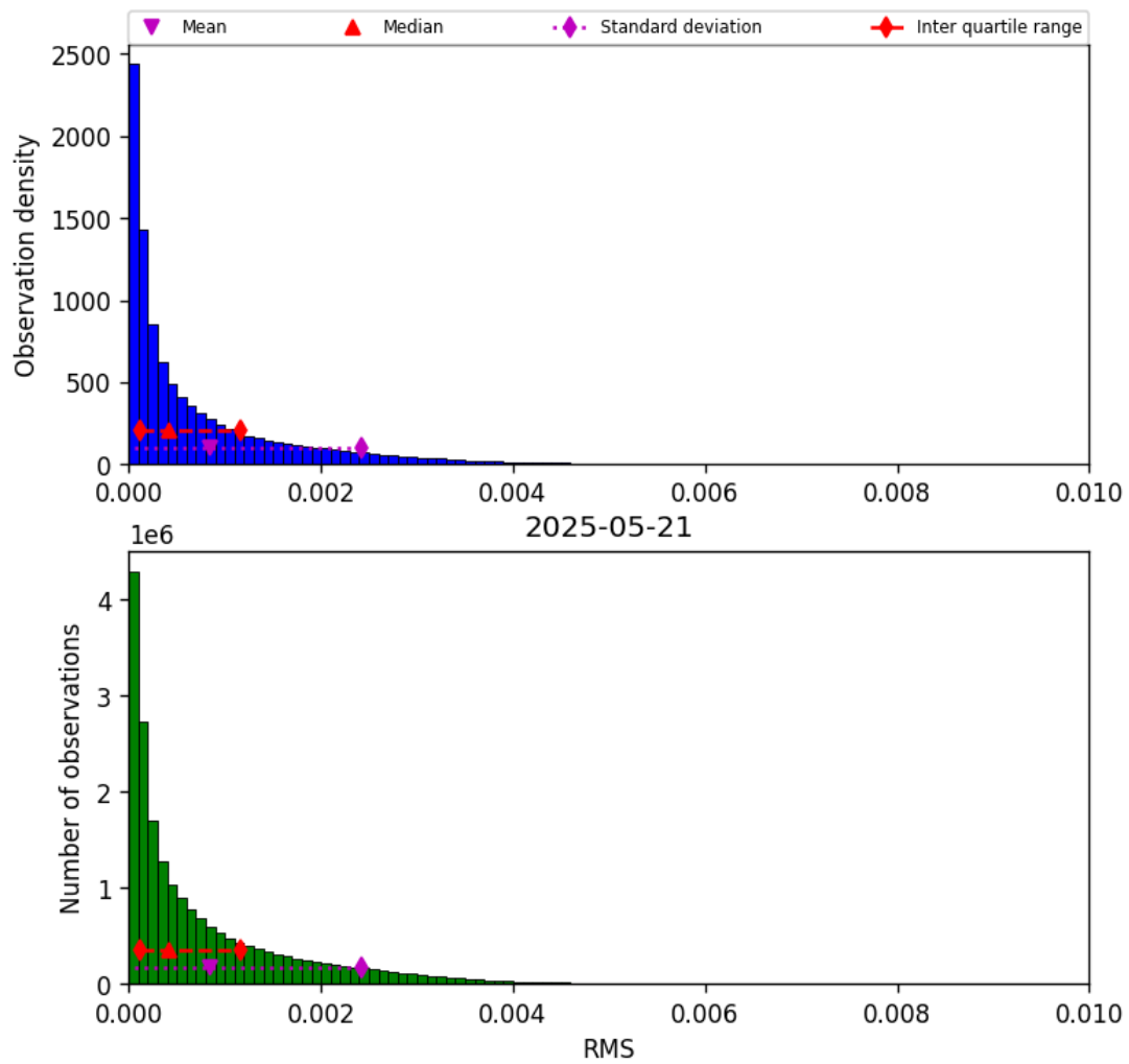
Figure 47: Histogram of “RMS” for 2025-05-21 to 2025-05-22
