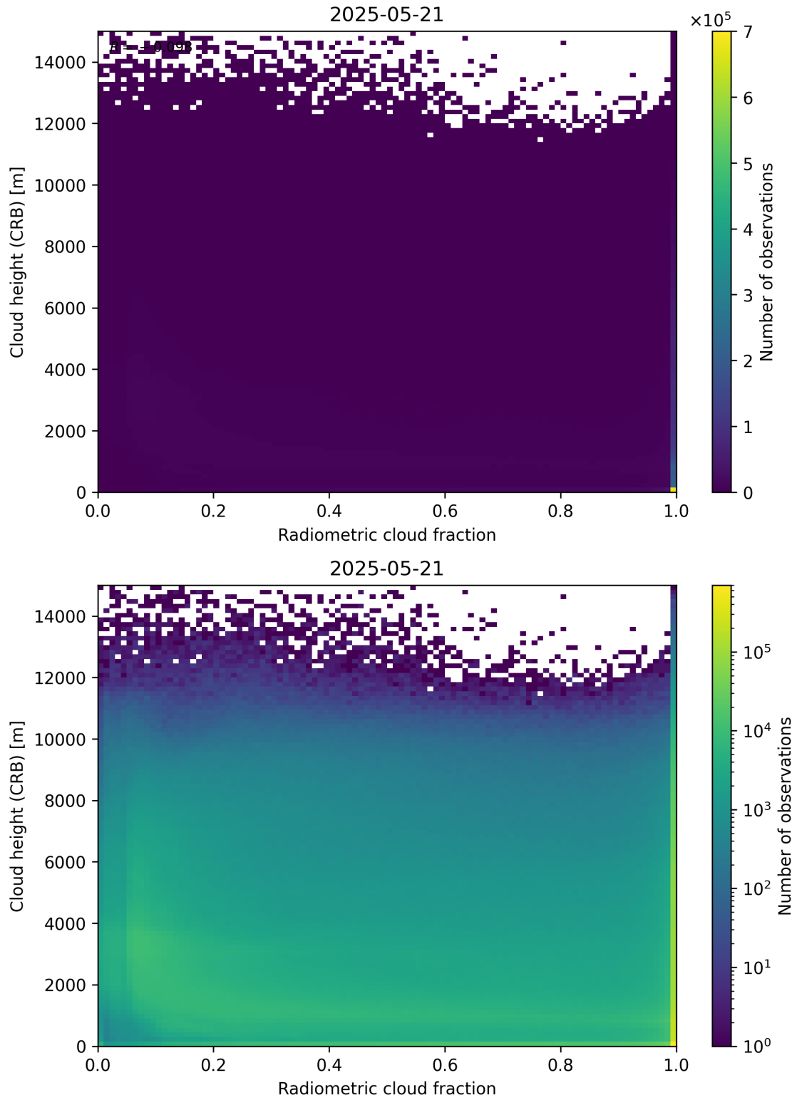
Figure 74: Scatter density plot of “Radiometric cloud fraction” against “Cloud height (CRB)” for 2025-05-21 to 2025-05-22.
