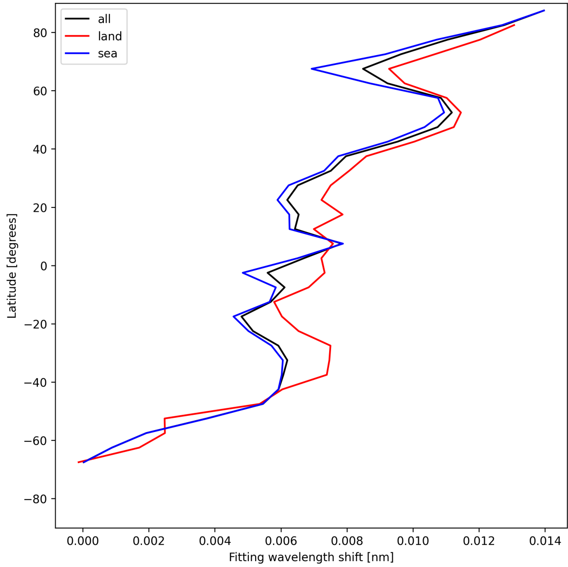
Figure 33: Zonal average of “Fitting wavelength shift” for 2025-05-21 to 2025-05-22.
