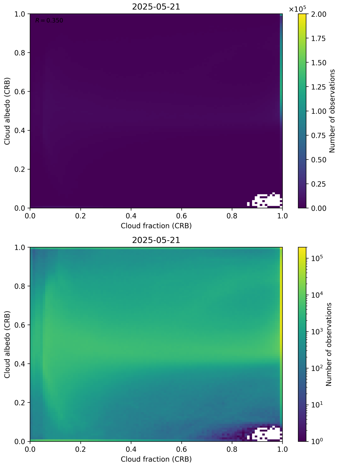
Figure 77: Scatter density plot of “Cloud fraction (CRB)” against “Cloud albedo (CRB)” for 2025-05-21 to 2025-05-22.
