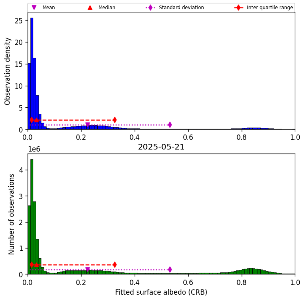
Figure 46: Histogram of “Fitted surface albedo (CRB)” for 2025-05-21 to 2025-05-22
