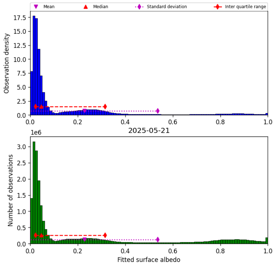
Figure 45: Histogram of “Fitted surface albedo” for 2025-05-21 to 2025-05-22
