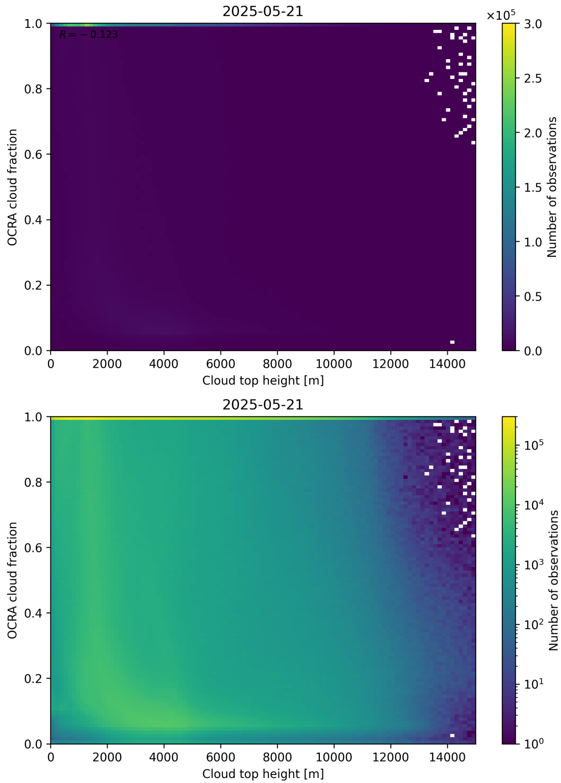
Figure 87: Scatter density plot of “Cloud top height” against “OCRA cloud fraction” for 2025-05-21 to 2025-05-22.
