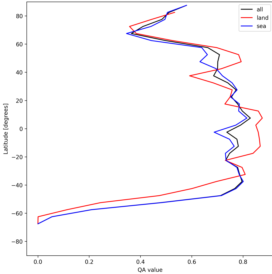
Figure 22: Zonal average of “QA value” for 2025-05-21 to 2025-05-22.
