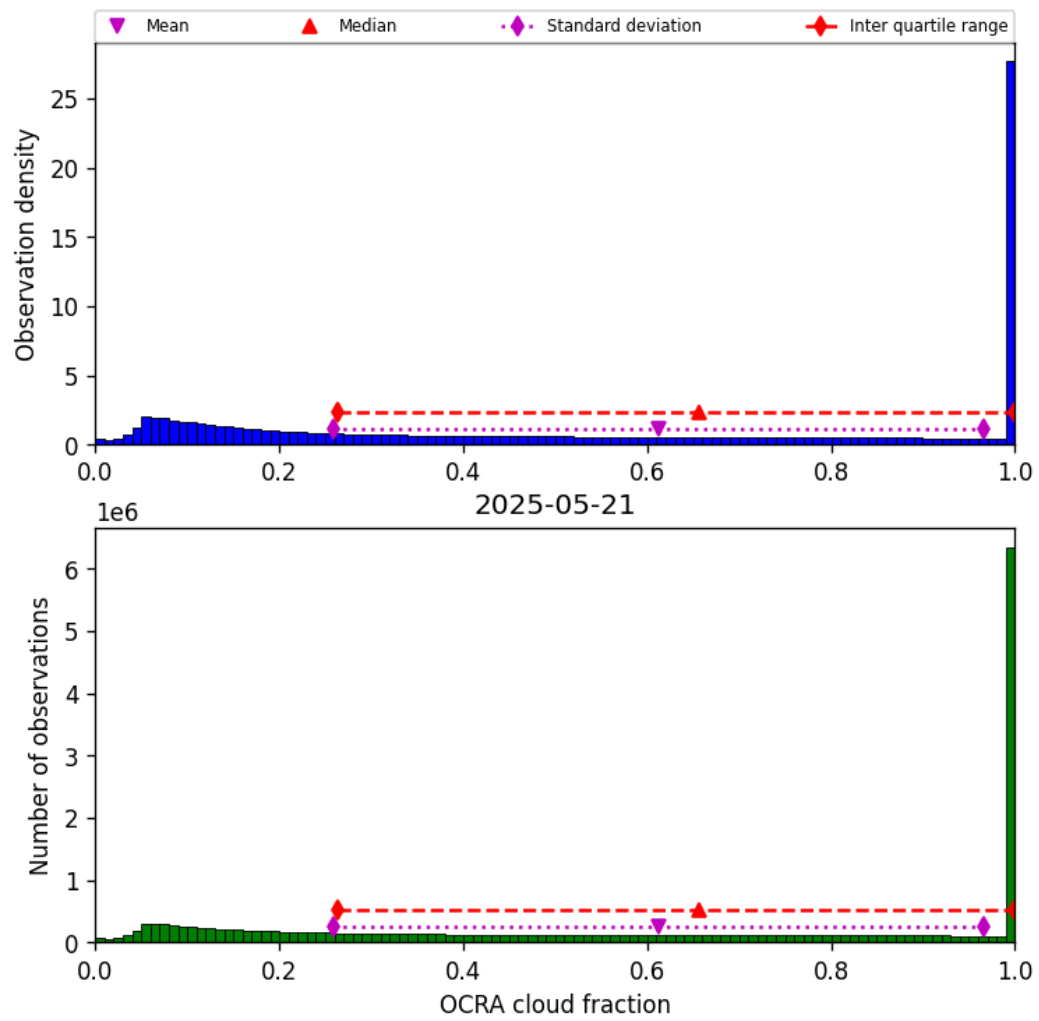
Figure 50: Histogram of “OCRA cloud fraction” for 2025-05-21 to 2025-05-22
