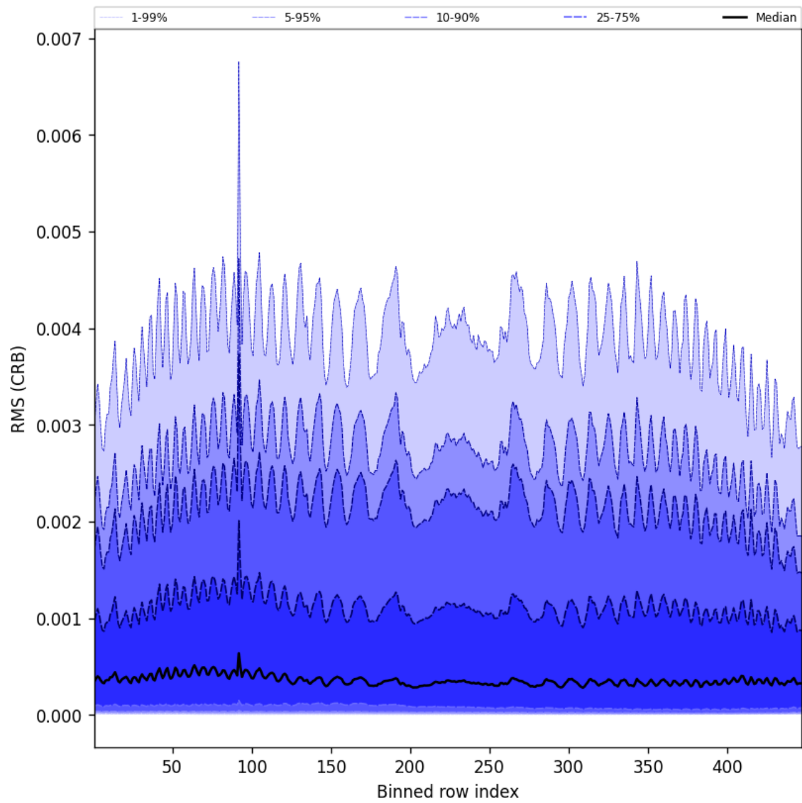
Figure 64: Along track statistics of “RMS (CRB)” for 2025-05-21 to 2025-05-22
