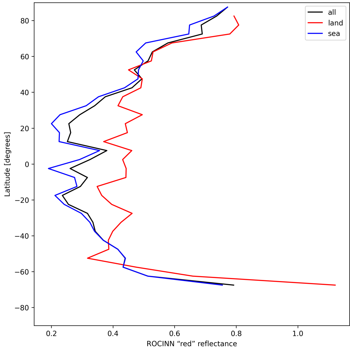
Figure 37: Zonal average of “ROCINN “red” reflectance” for 2025-05-21 to 2025-05-22.
