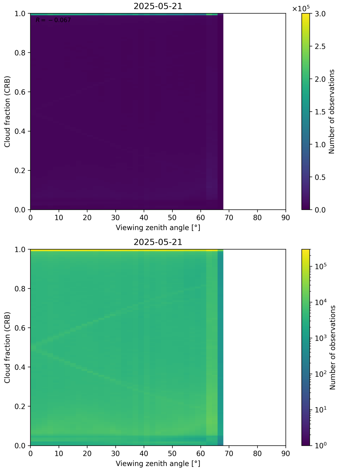
Figure 109: Scatter density plot of “Viewing zenith angle” against “Cloud fraction (CRB)” for 2025-05-21 to 2025-05-22.
