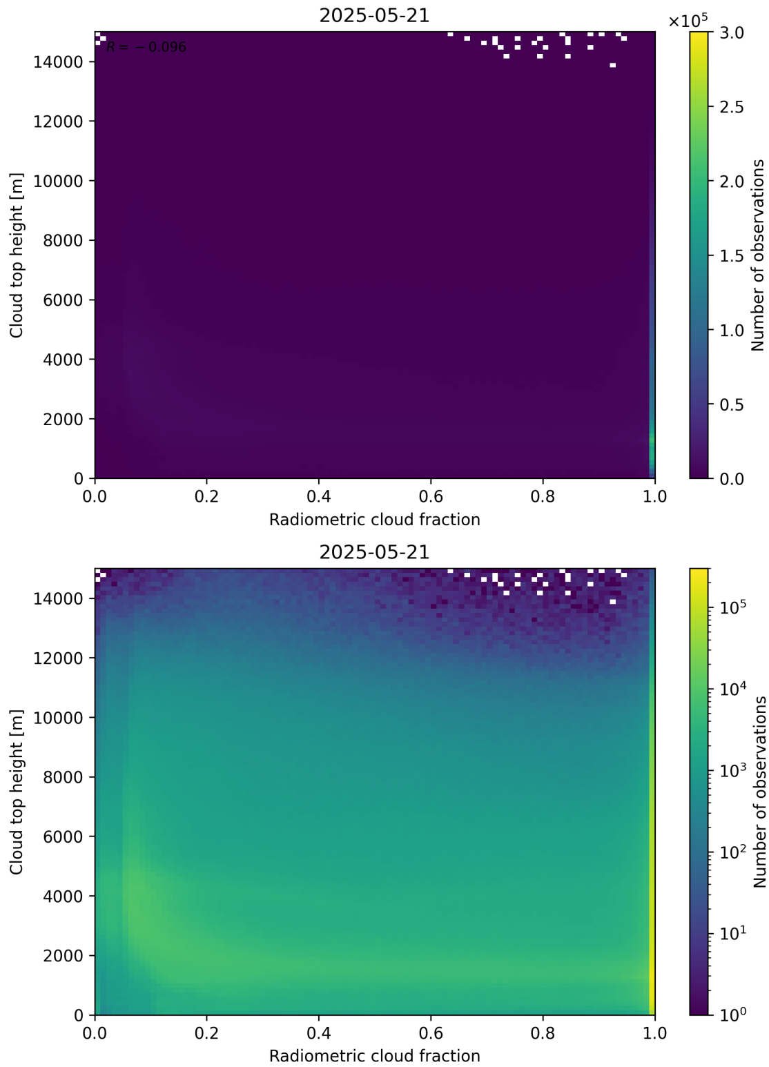
Figure 76: Scatter density plot of “Radiometric cloud fraction” against “Cloud top height” for 2025-05-21 to 2025-05-22.
