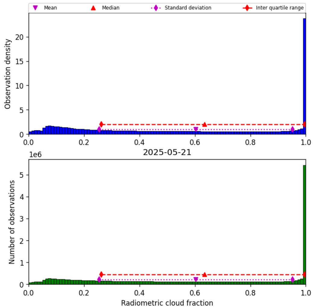
Figure 39: Histogram of “Radiometric cloud fraction” for 2025-05-21 to 2025-05-22
