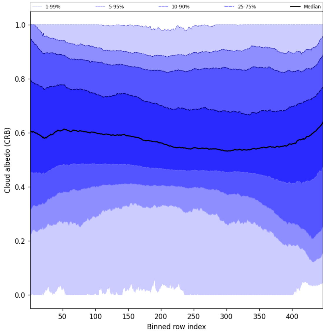
Figure 60: Along track statistics of “Cloud albedo (CRB)” for 2025-05-21 to 2025-05-22
