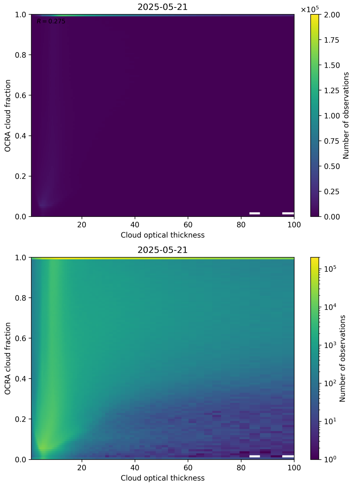
Figure 83: Scatter density plot of “Cloud optical thickness” against “OCRA cloud fraction” for 2025-05-21 to 2025-05-22.
