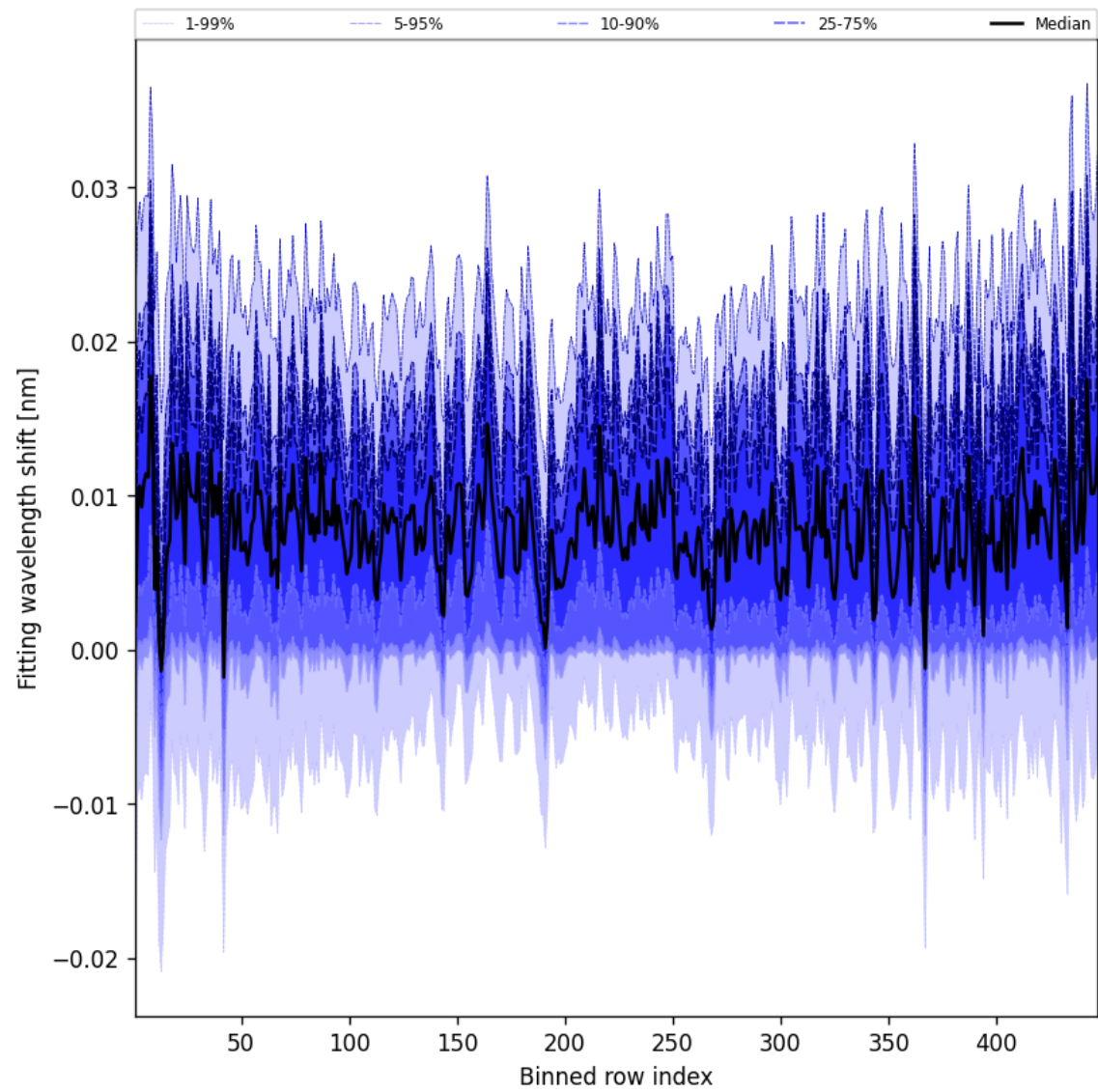
Figure 65: Along track statistics of “Fitting wavelength shift” for 2025-05-21 to 2025-05-22
