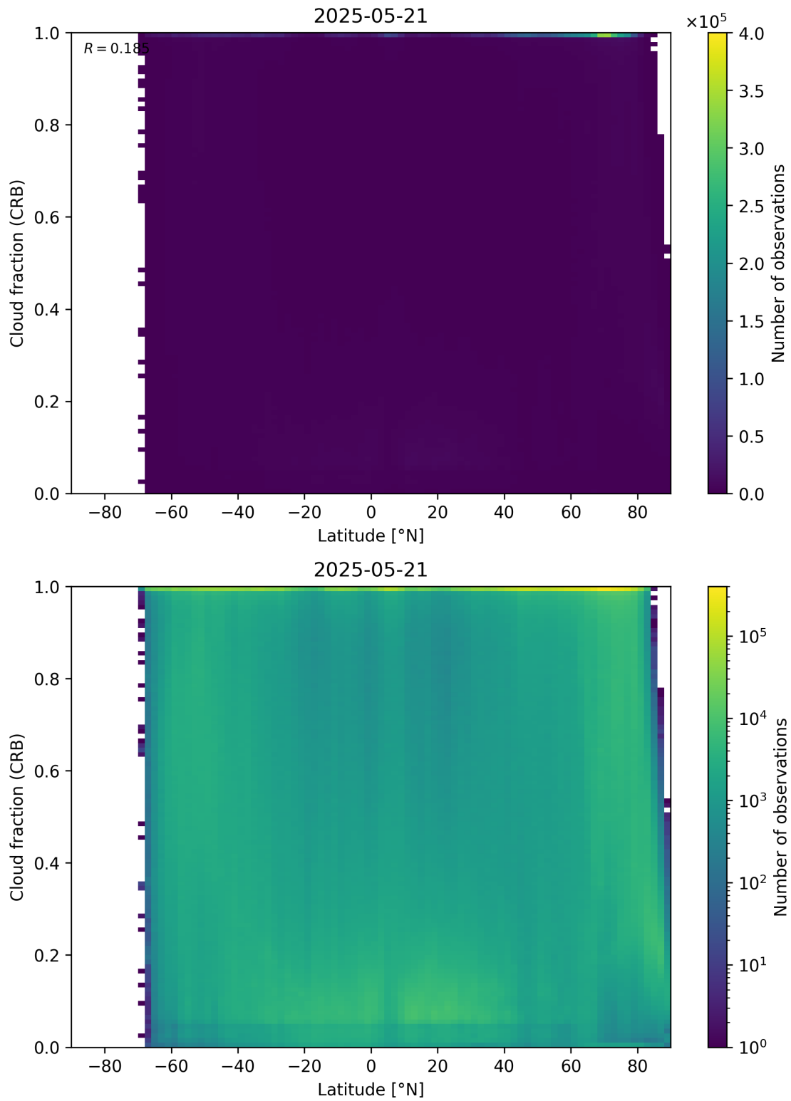
Figure 94: Scatter density plot of “Latitude” against “Cloud fraction (CRB)” for 2025-05-21 to 2025-05-22.
