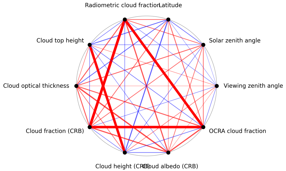
Figure 1: Map of correlation graph for 2025-05-21 to 2025-05-22.
