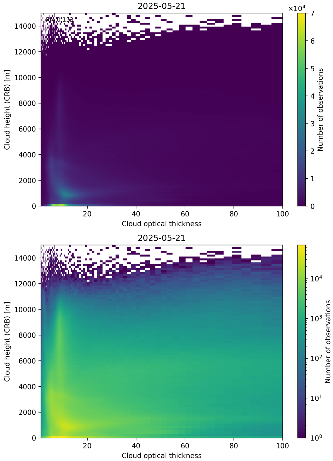
Figure 85: Scatter density plot of “Cloud optical thickness” against “Cloud height (CRB)” for 2025-05-21 to 2025-05-22.
