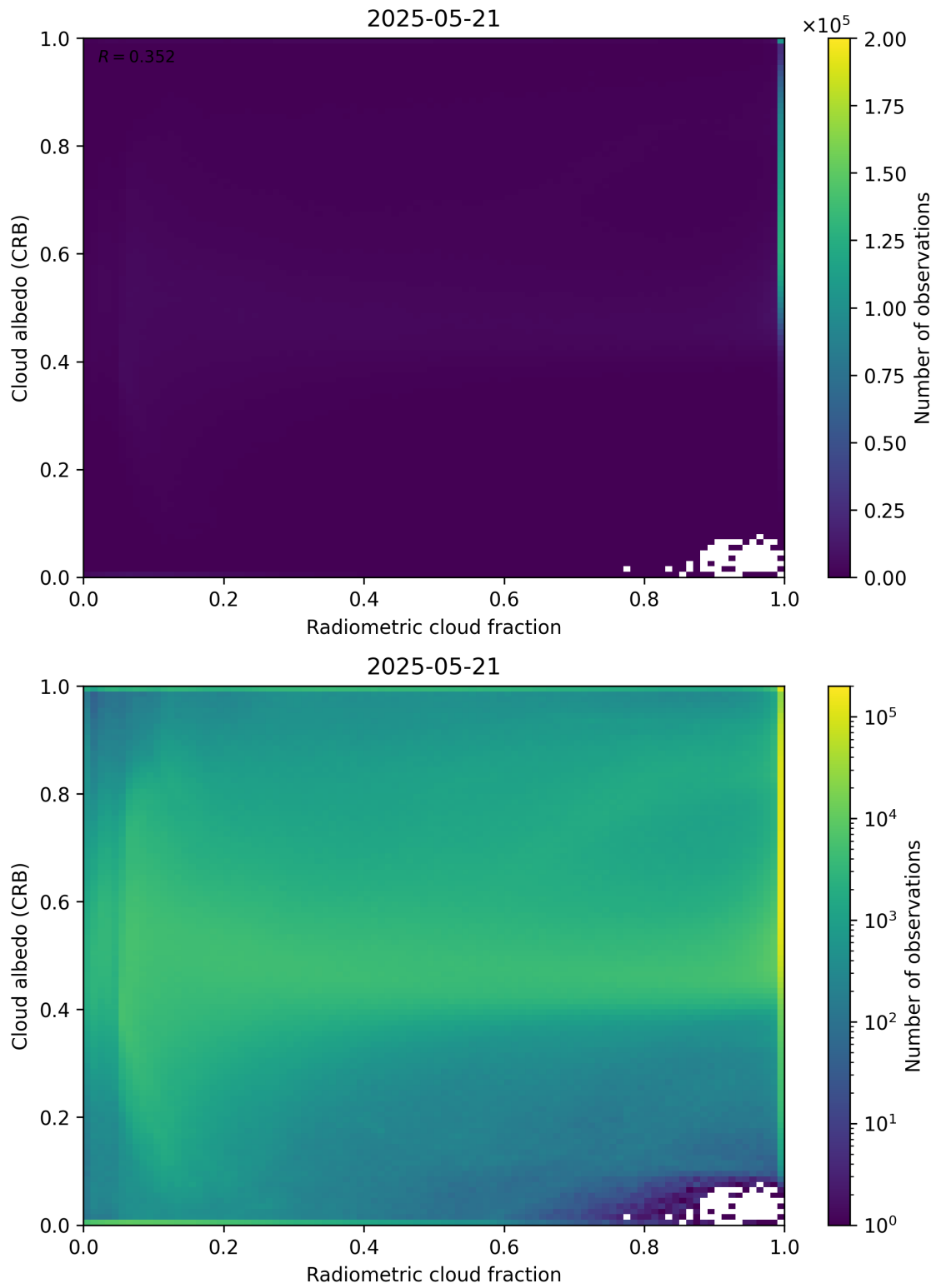
Figure 71: Scatter density plot of “Radiometric cloud fraction” against “Cloud albedo (CRB)” for 2025-05-21 to 2025-05-22.
