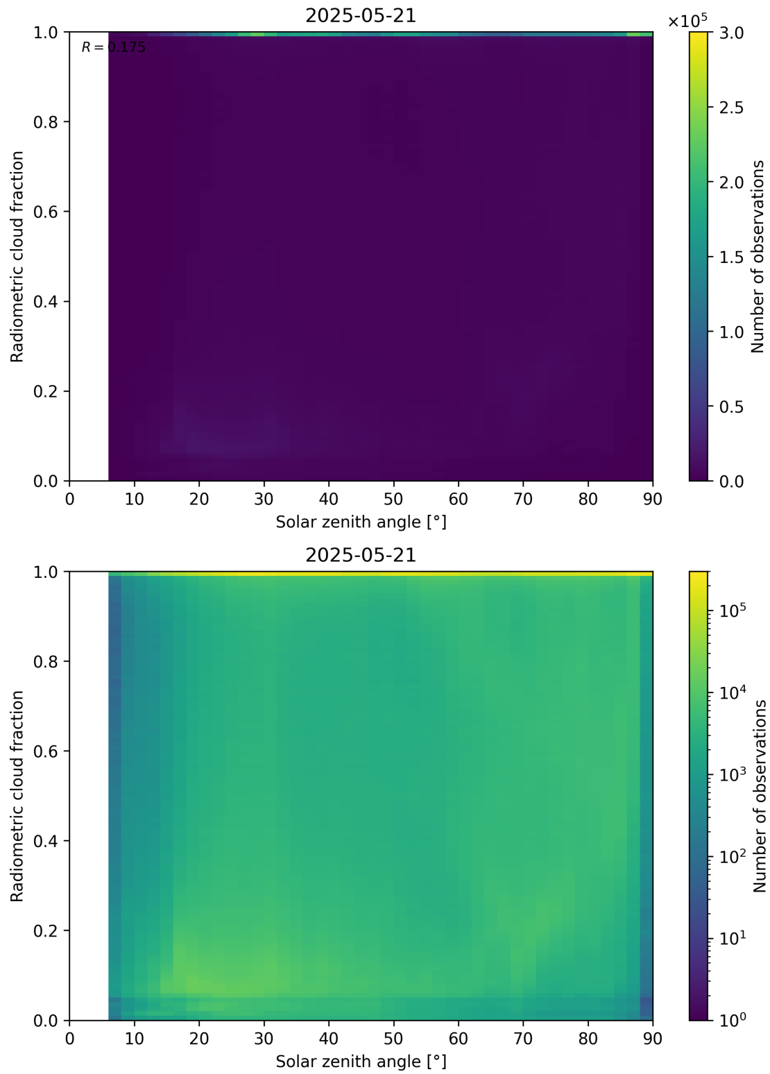
Figure 99: Scatter density plot of “Solar zenith angle” against “Radiometric cloud fraction” for 2025-05-21 to 2025-05-22.
