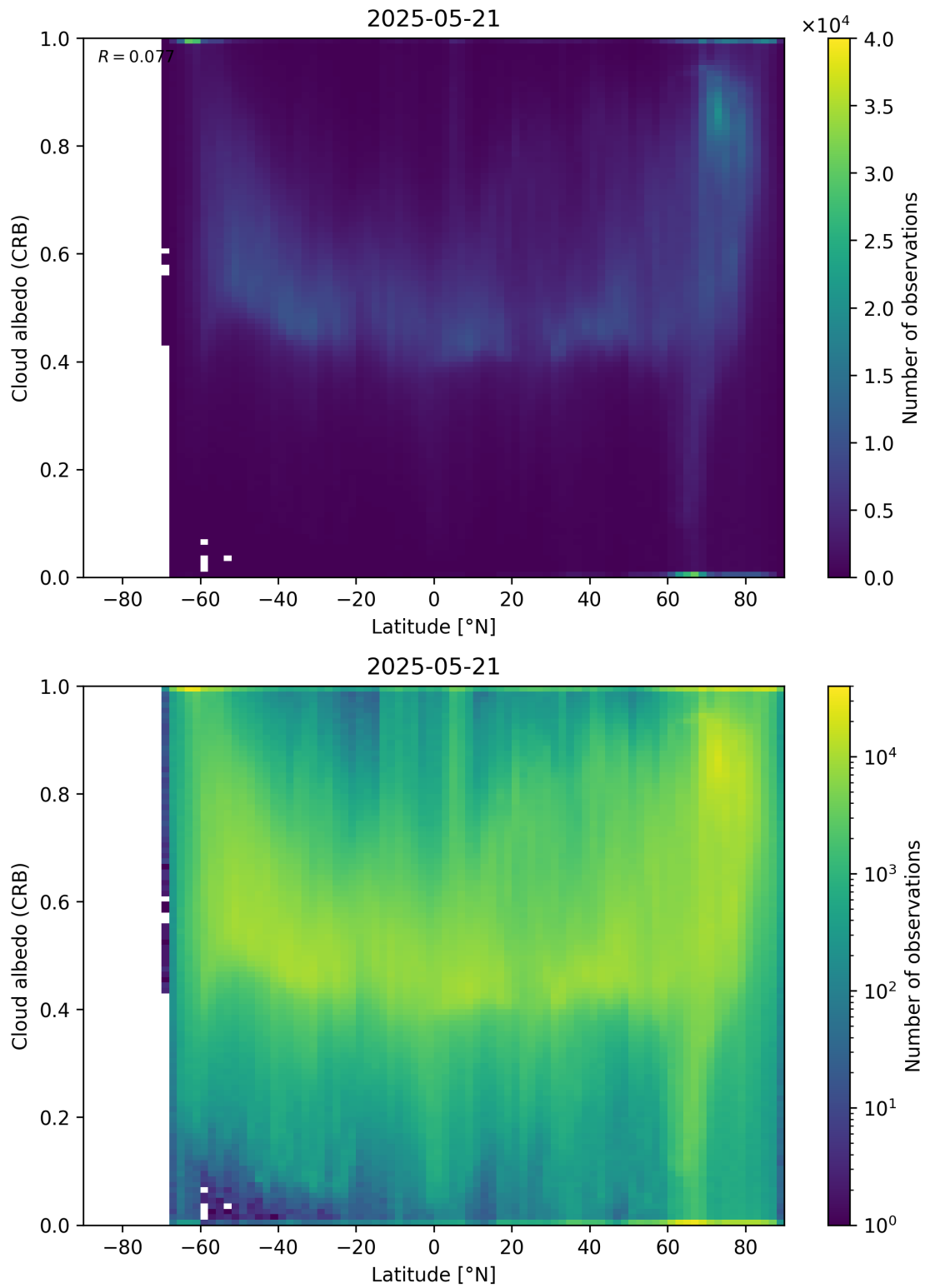
Figure 91: Scatter density plot of “Latitude” against “Cloud albedo (CRB)” for 2025-05-21 to 2025-05-22.
