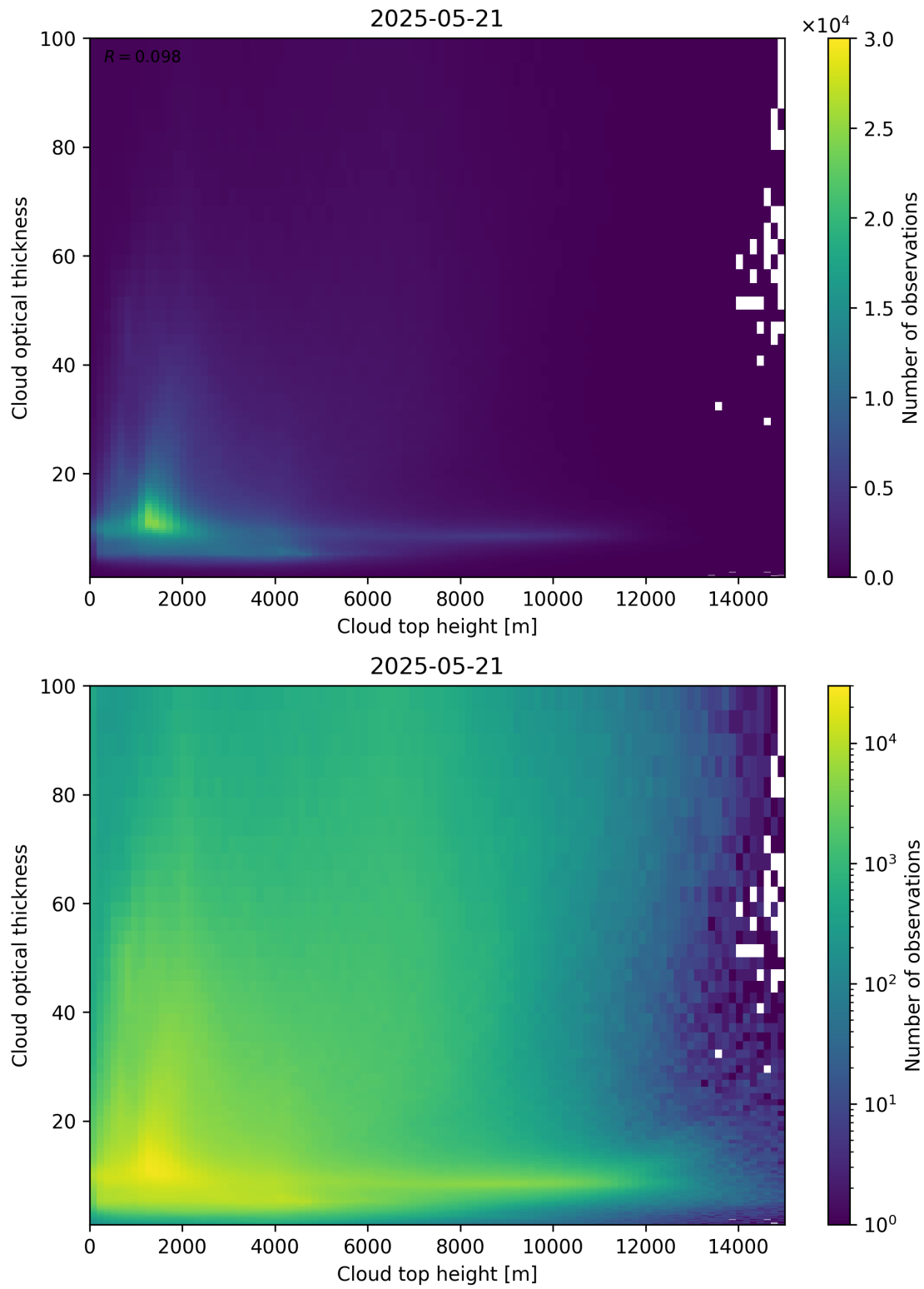
Figure 90: Scatter density plot of “Cloud top height” against “Cloud optical thickness” for 2025-05-21 to 2025-05-22.
