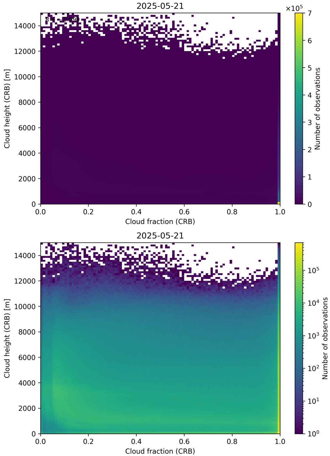
Figure 79: Scatter density plot of “Cloud fraction (CRB)” against “Cloud height (CRB)” for 2025-05-21 to 2025-05-22.
