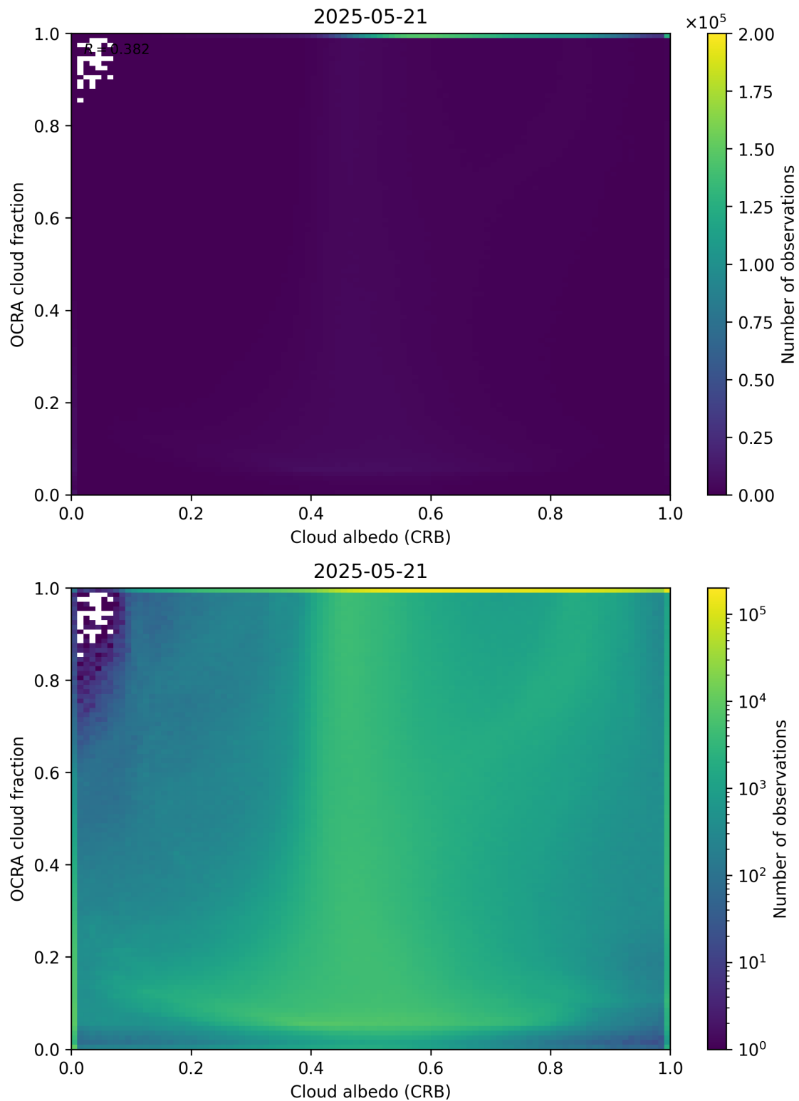
Figure 70: Scatter density plot of “Cloud albedo (CRB)” against “OCRA cloud fraction” for 2025-05-21 to 2025-05-22.
