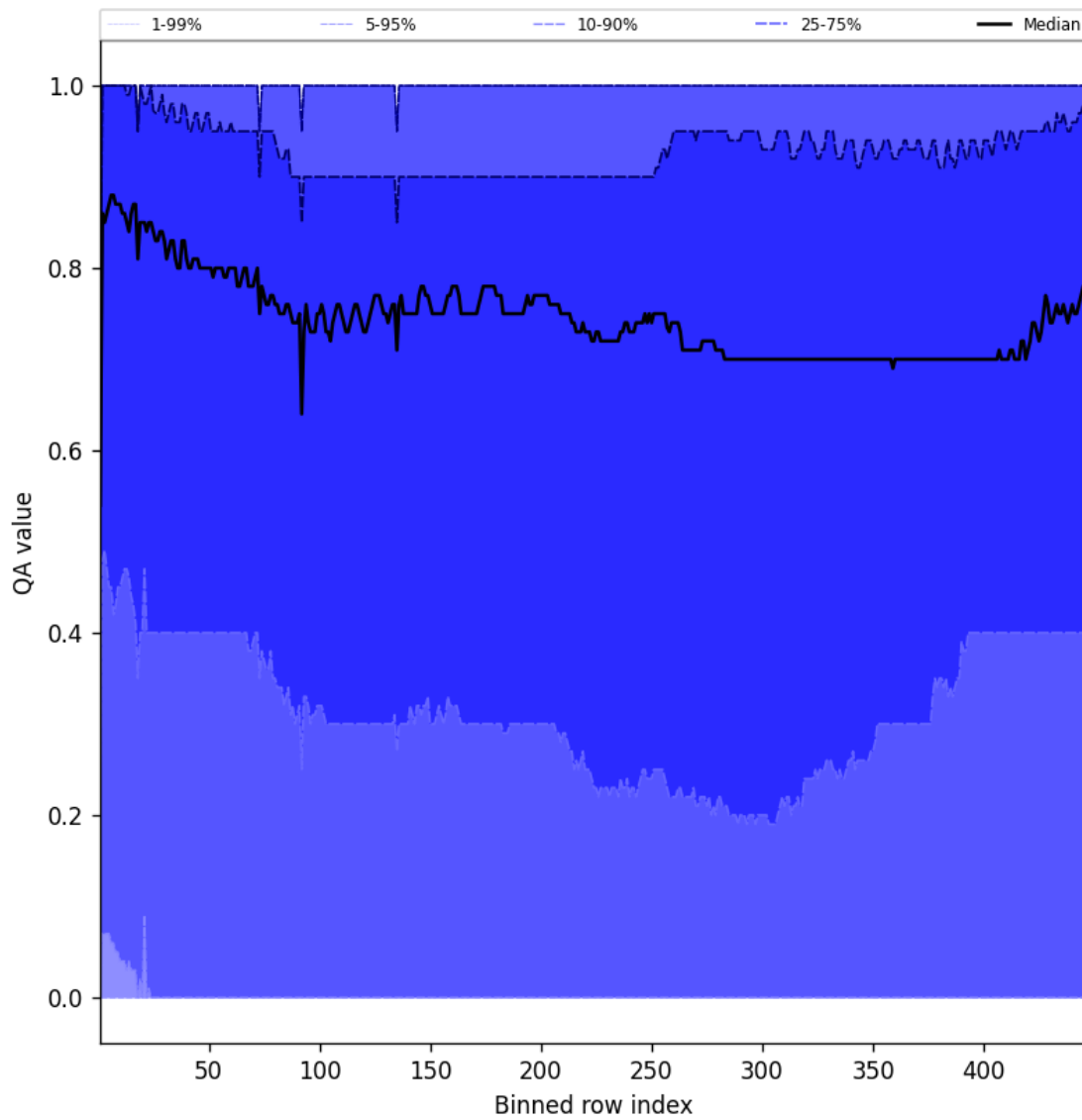
Figure 54: Along track statistics of “QA value” for 2025-05-21 to 2025-05-22
