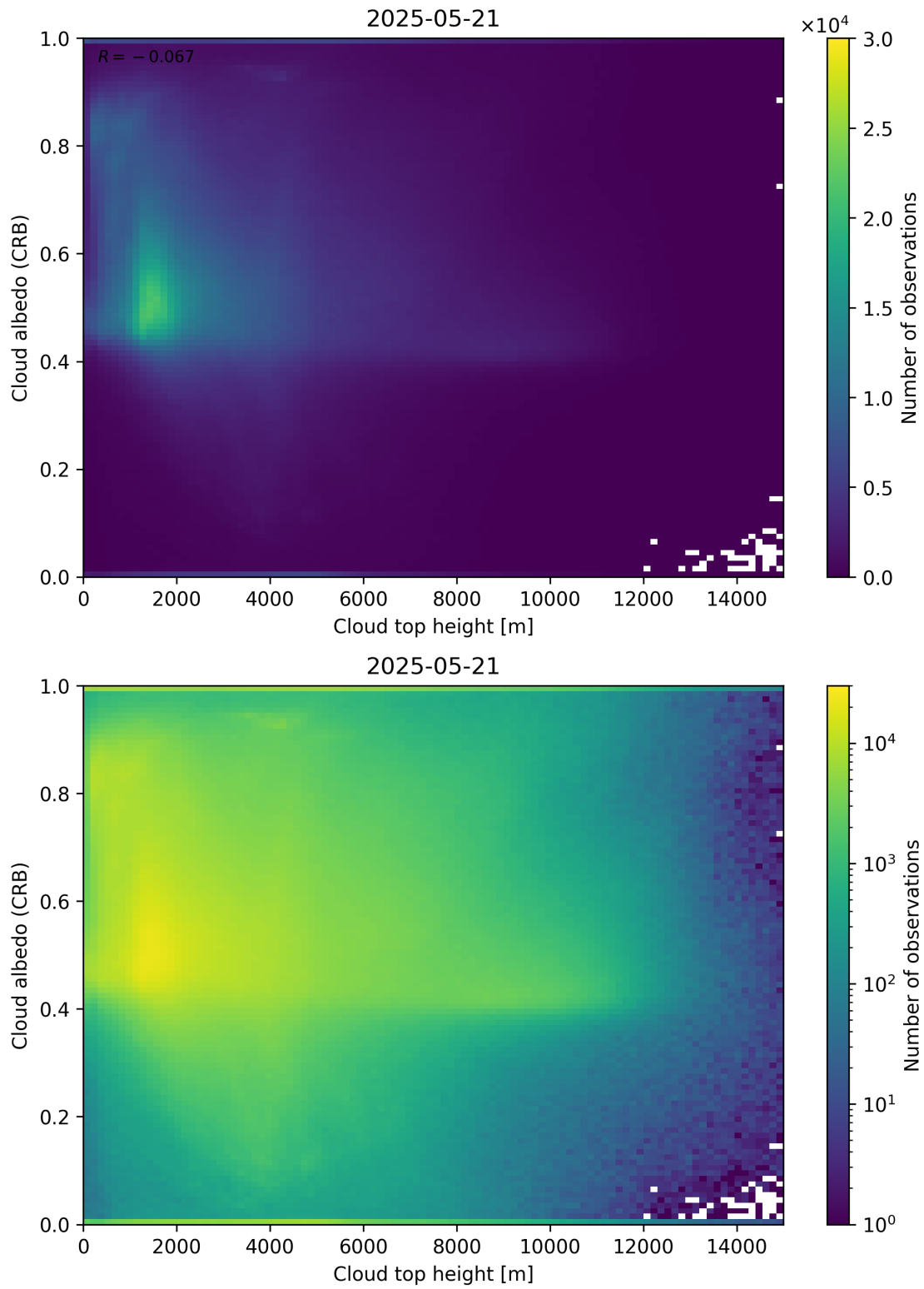
Figure 86: Scatter density plot of “Cloud top height” against “Cloud albedo (CRB)” for 2025-05-21 to 2025-05-22.
