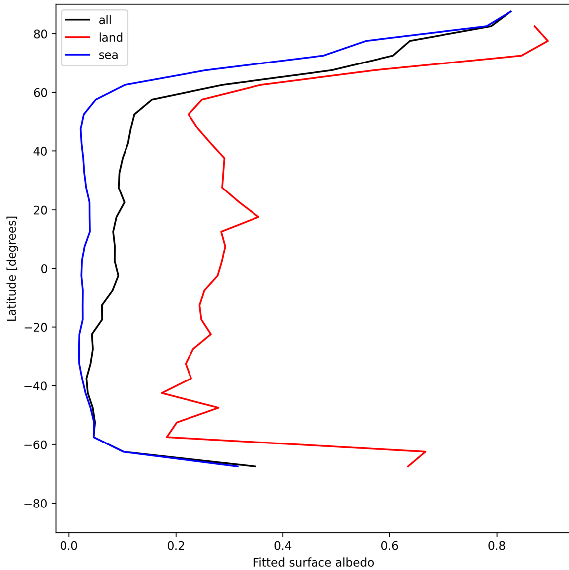
Figure 29: Zonal average of “Fitted surface albedo” for 2025-05-21 to 2025-05-22.
