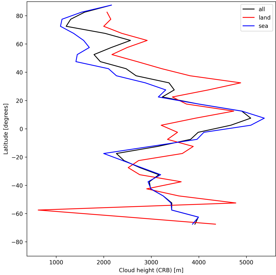
Figure 27: Zonal average of “Cloud height (CRB)” for 2025-05-21 to 2025-05-22.
