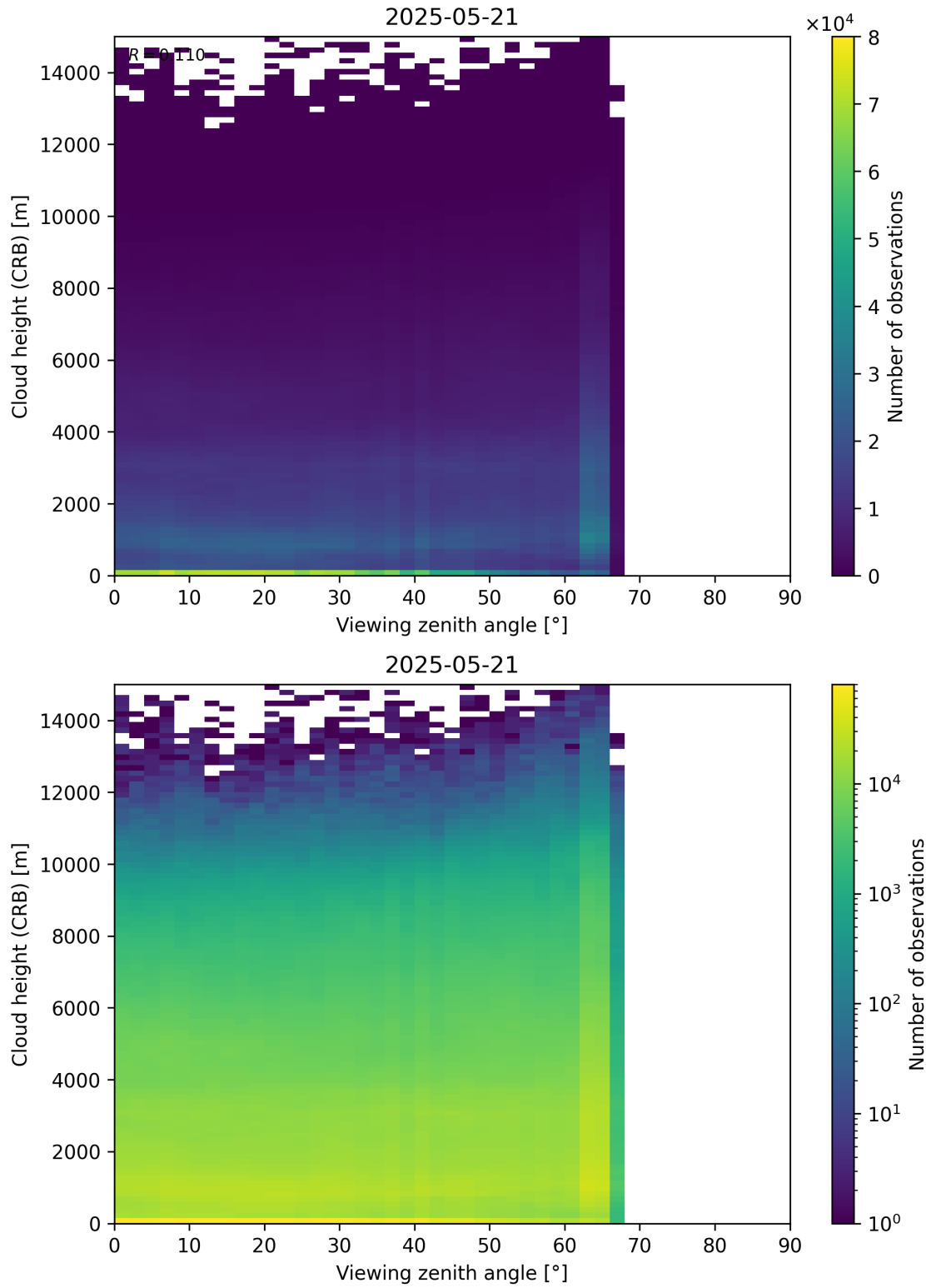
Figure 110: Scatter density plot of “Viewing zenith angle” against “Cloud height (CRB)” for 2025-05-21 to 2025-05-22.
