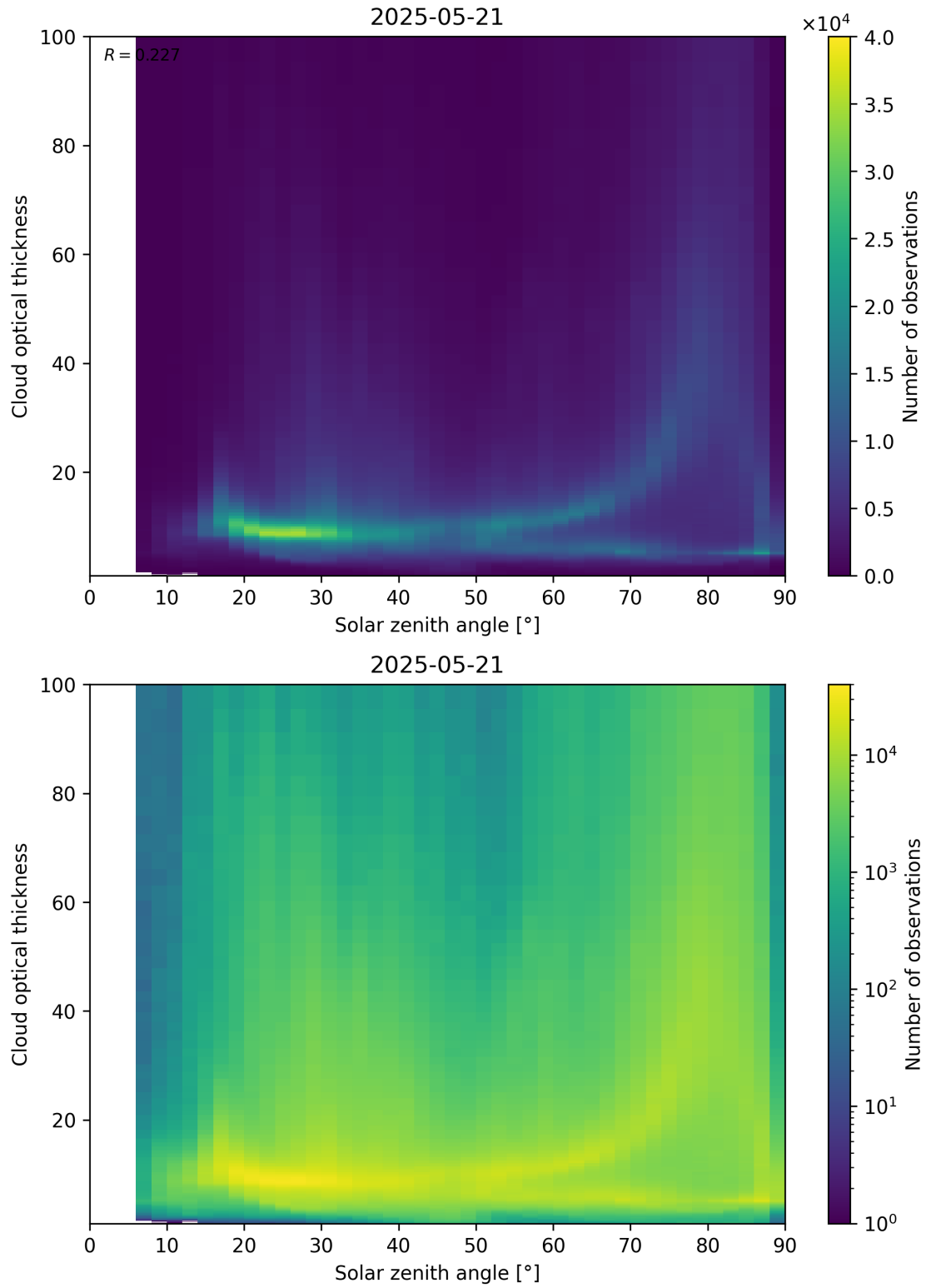
Figure 103: Scatter density plot of “Solar zenith angle” against “Cloud optical thickness” for 2025-05-21 to 2025-05-22.
