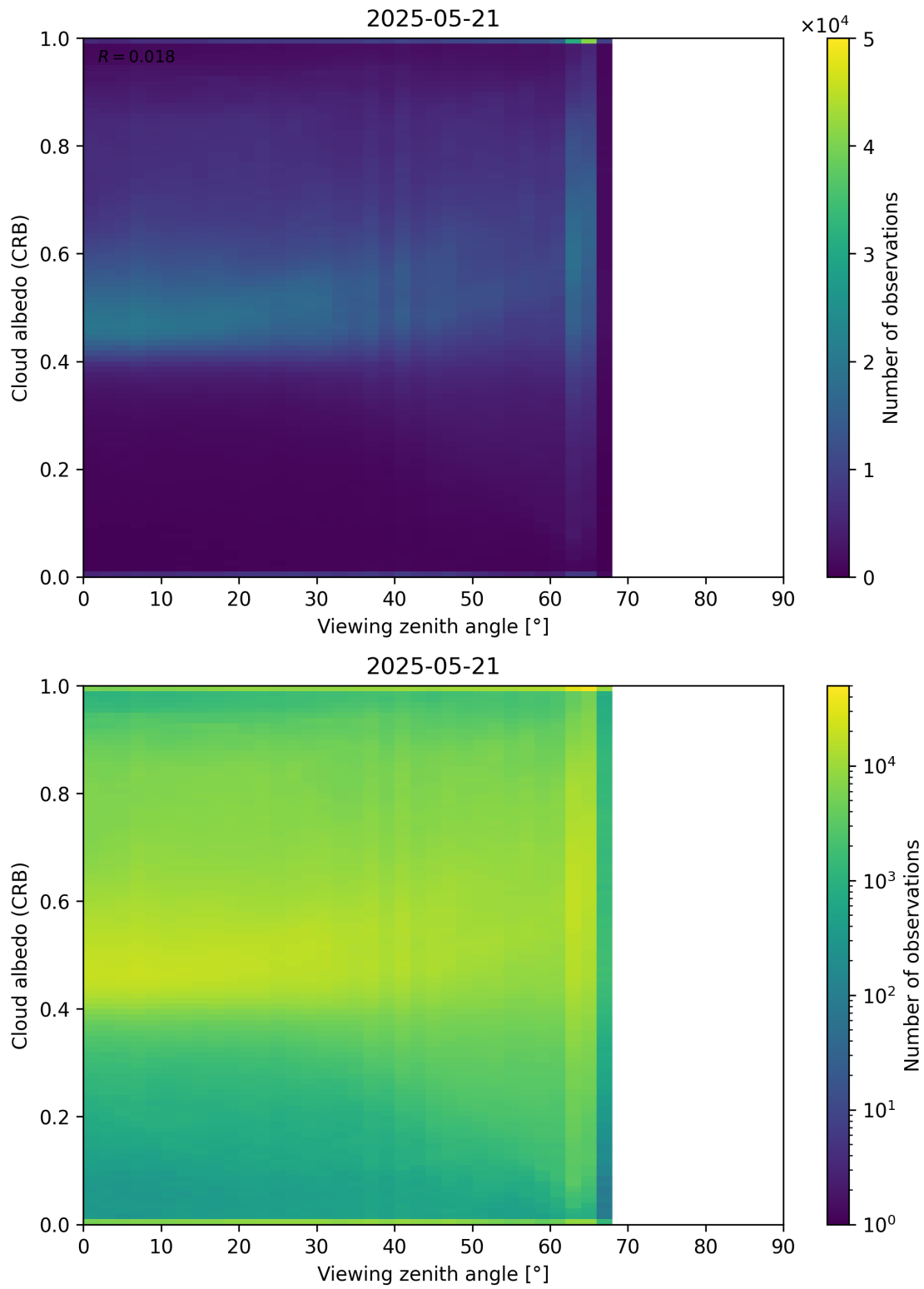
Figure 106: Scatter density plot of “Viewing zenith angle” against “Cloud albedo (CRB)” for 2025-05-21 to 2025-05-22.
