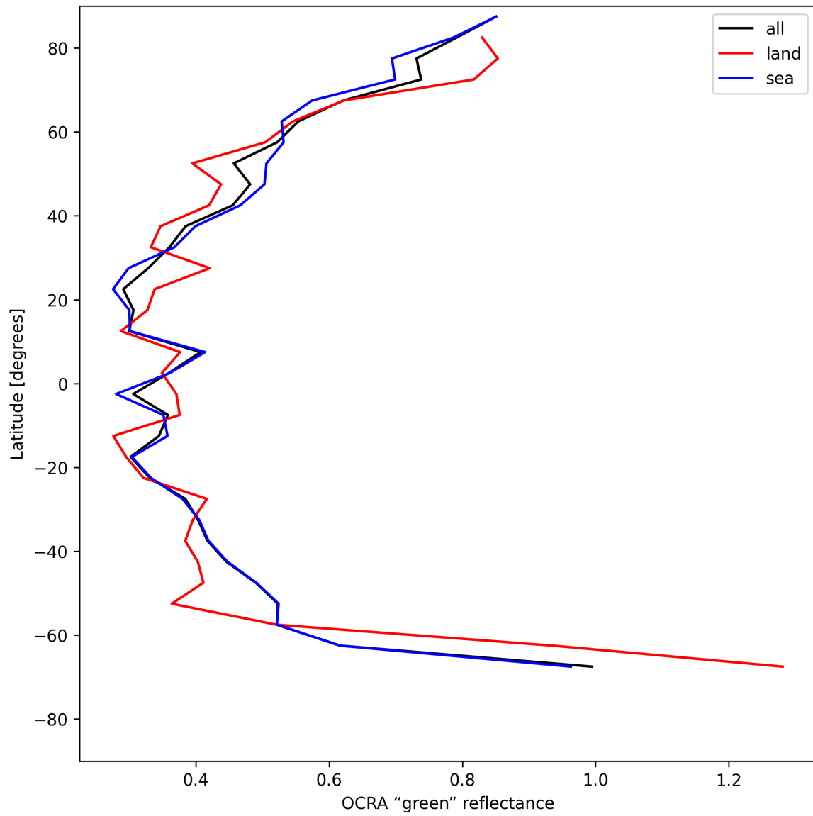
Figure 36: Zonal average of “OCRA “green” reflectance” for 2025-05-21 to 2025-05-22.
