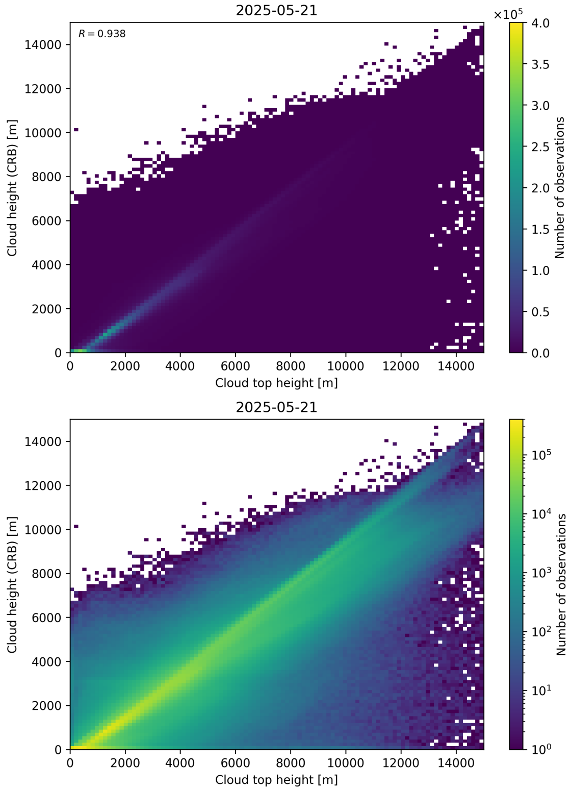
Figure 89: Scatter density plot of “Cloud top height” against “Cloud height (CRB)” for 2025-05-21 to 2025-05-22.
