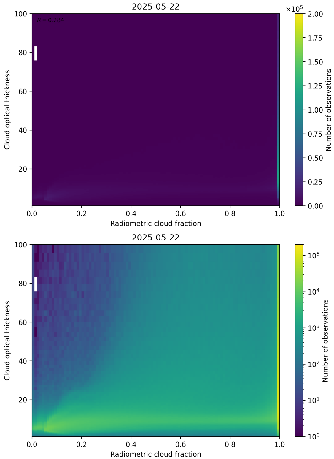
Figure 75: Scatter density plot of “Radiometric cloud fraction” against “Cloud optical thickness” for 2025-05-21 to 2025-05-23.
