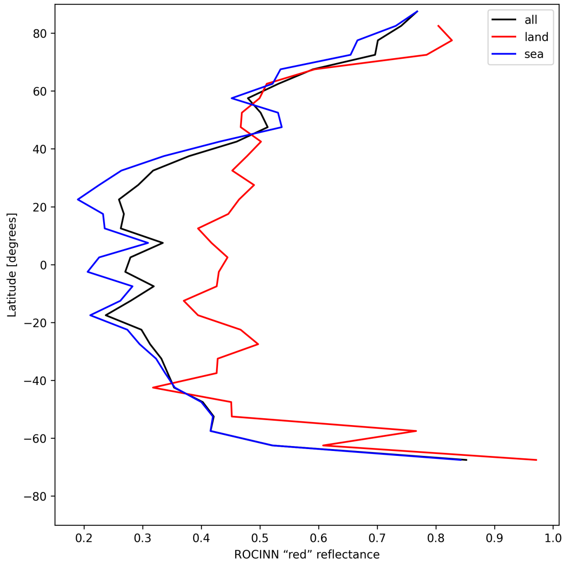
Figure 37: Zonal average of “ROCINN “red” reflectance” for 2025-05-21 to 2025-05-23.
