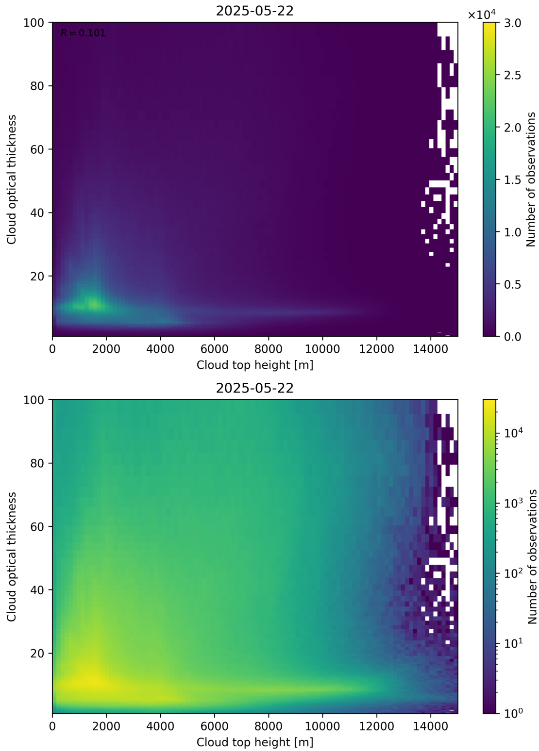
Figure 90: Scatter density plot of “Cloud top height” against “Cloud optical thickness” for 2025-05-21 to 2025-05-23.
