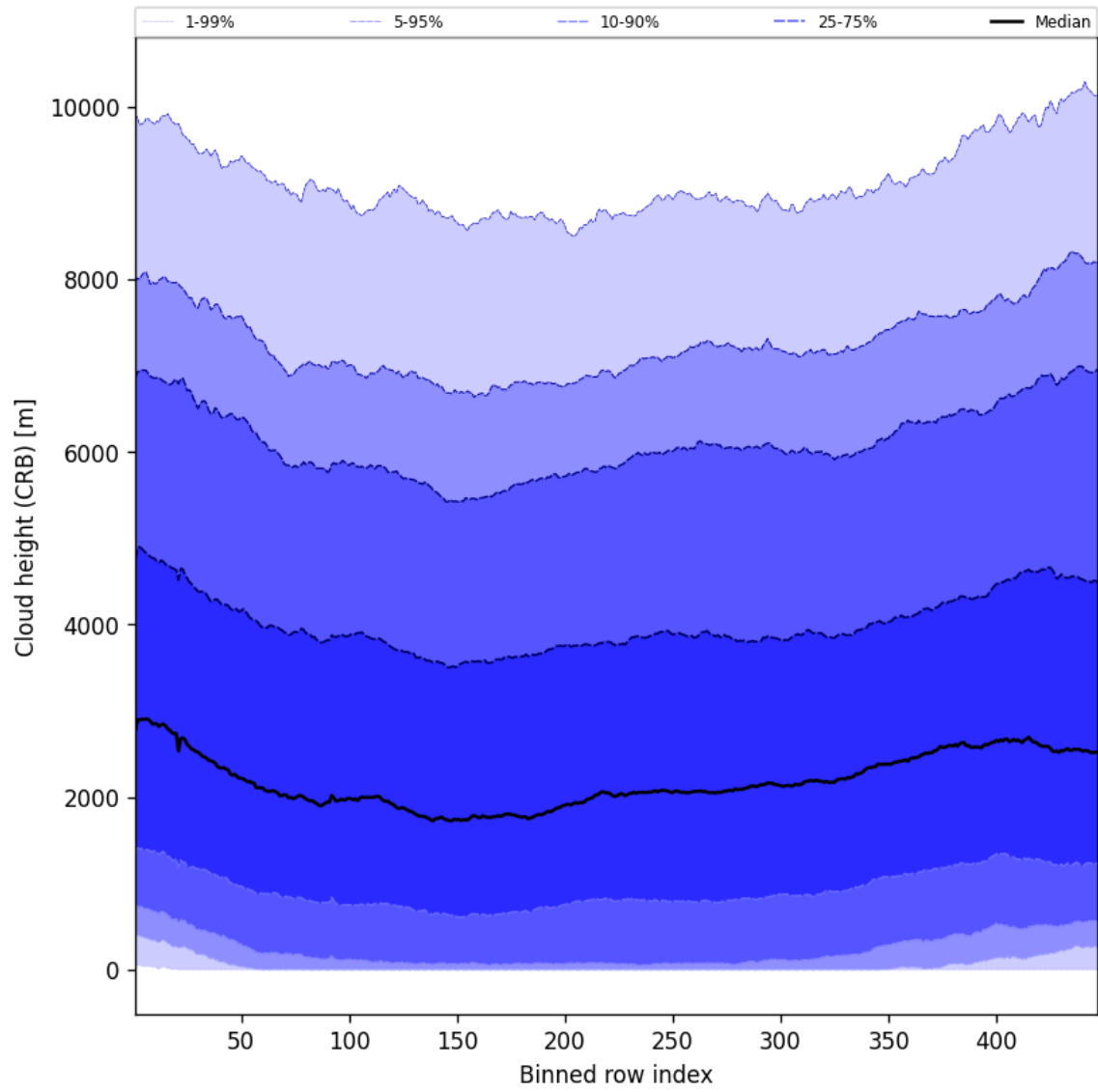
Figure 59: Along track statistics of “Cloud height (CRB)” for 2025-05-21 to 2025-05-23
