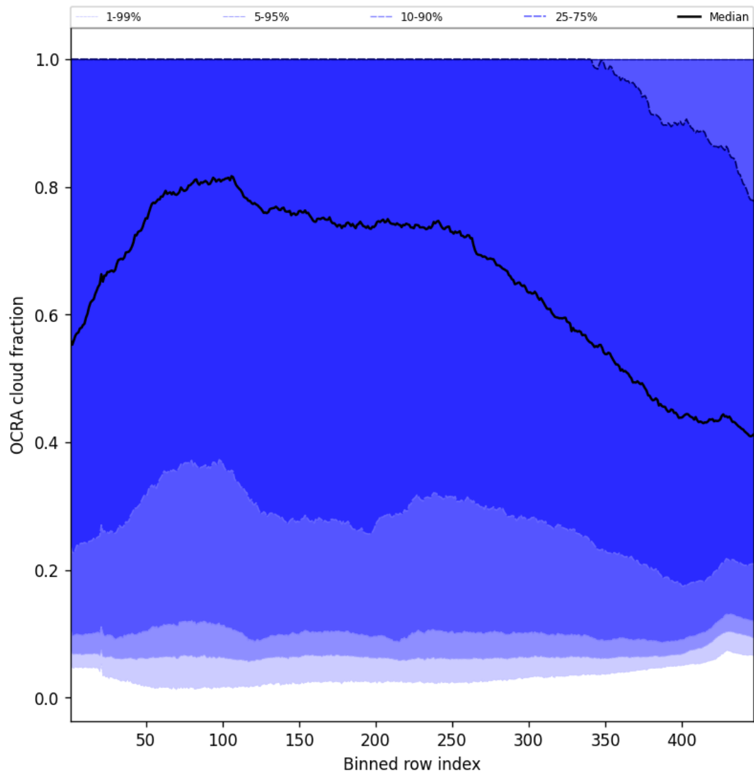
Figure 66: Along track statistics of “OCRA cloud fraction” for 2025-05-21 to 2025-05-23
