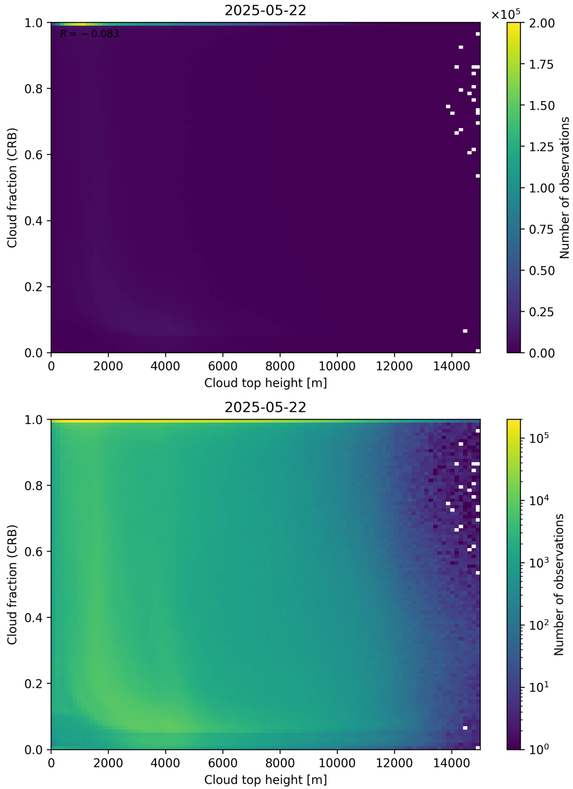
Figure 88: Scatter density plot of “Cloud top height” against “Cloud fraction (CRB)” for 2025-05-21 to 2025-05-23.
