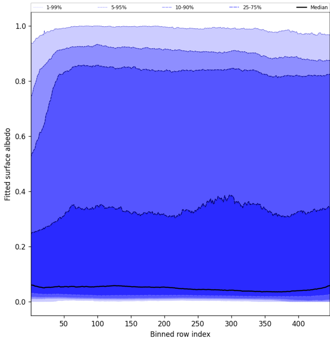
Figure 61: Along track statistics of “Fitted surface albedo” for 2025-05-21 to 2025-05-23
