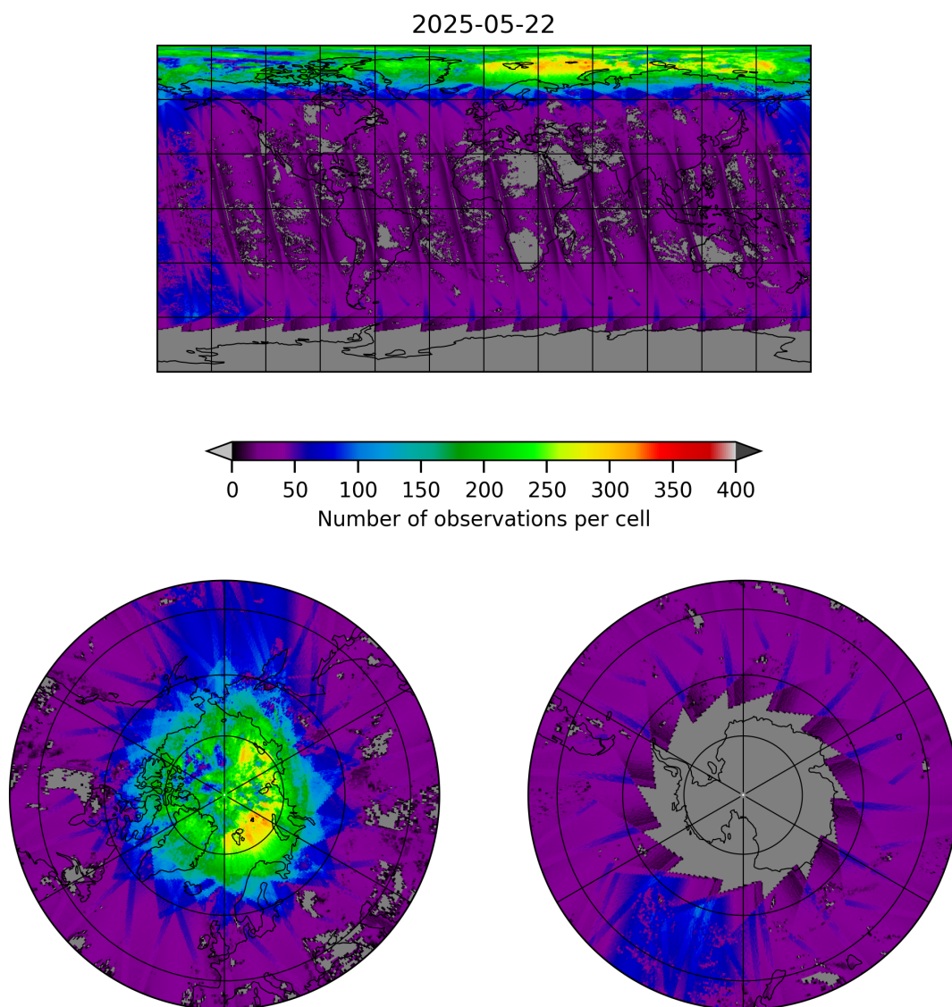
Figure 21: Map of the number of observations for 2025-05-21 to 2025-05-23
