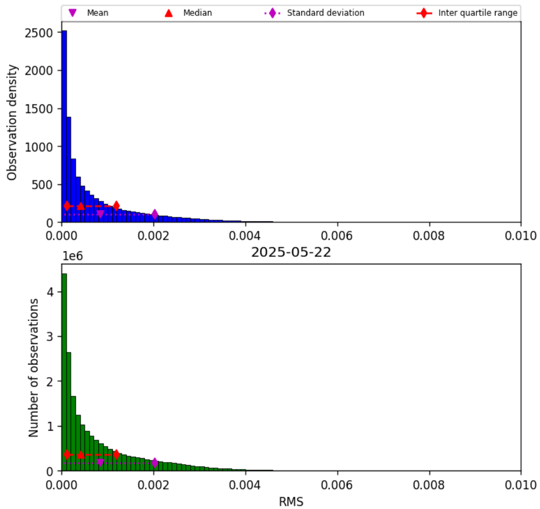
Figure 47: Histogram of “RMS” for 2025-05-21 to 2025-05-23
