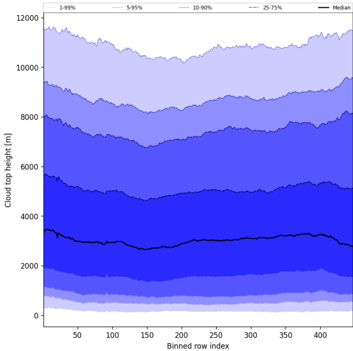
Figure 56: Along track statistics of “Cloud top height” for 2025-05-21 to 2025-05-23
