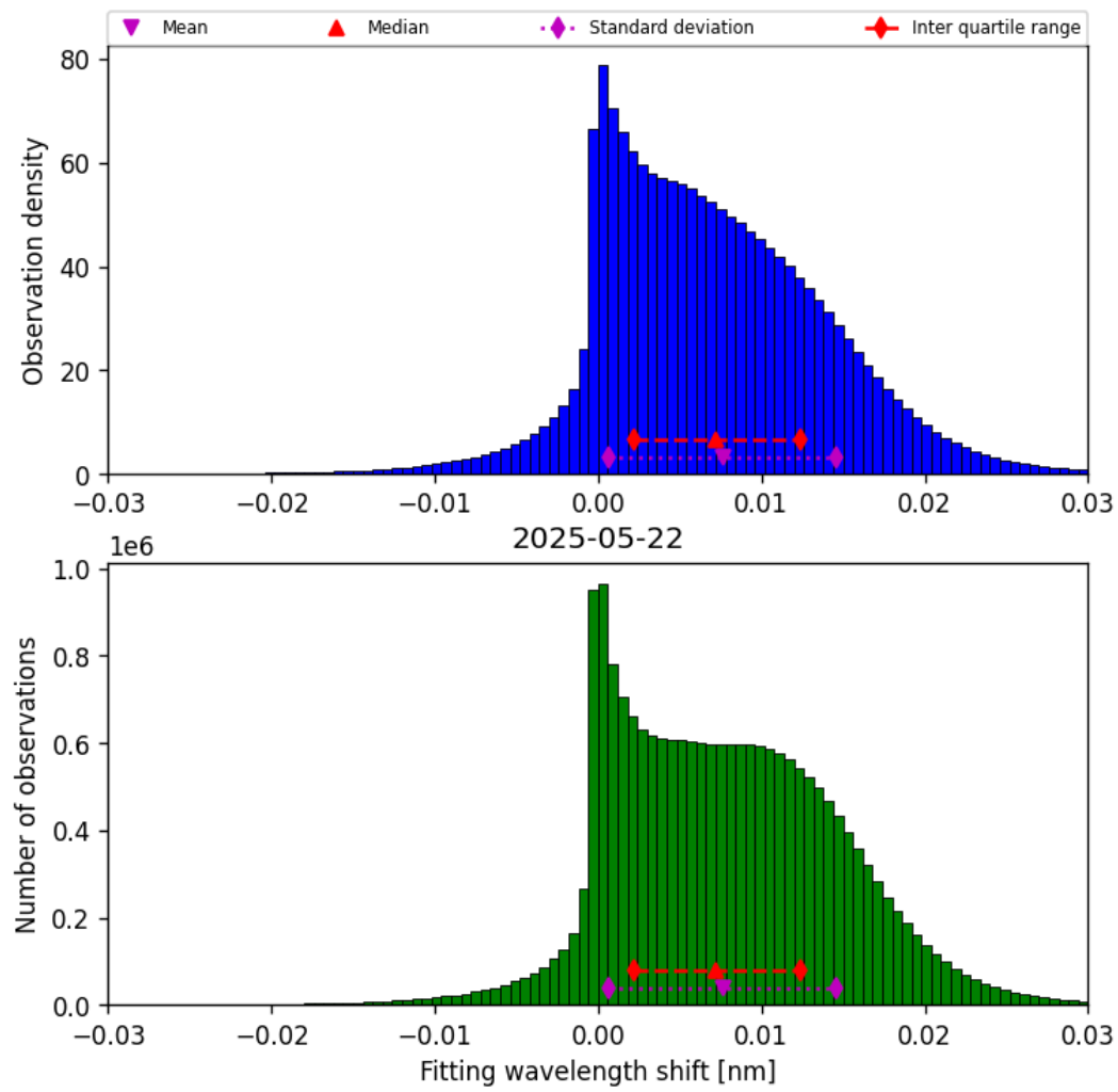
Figure 49: Histogram of “Fitting wavelength shift” for 2025-05-21 to 2025-05-23
