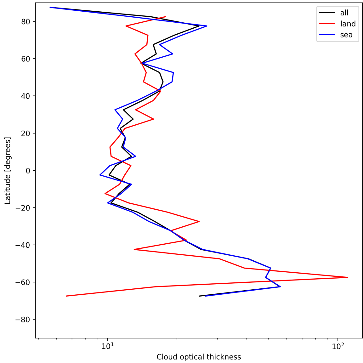
Figure 25: Zonal average of “Cloud optical thickness” for 2025-05-21 to 2025-05-23.
