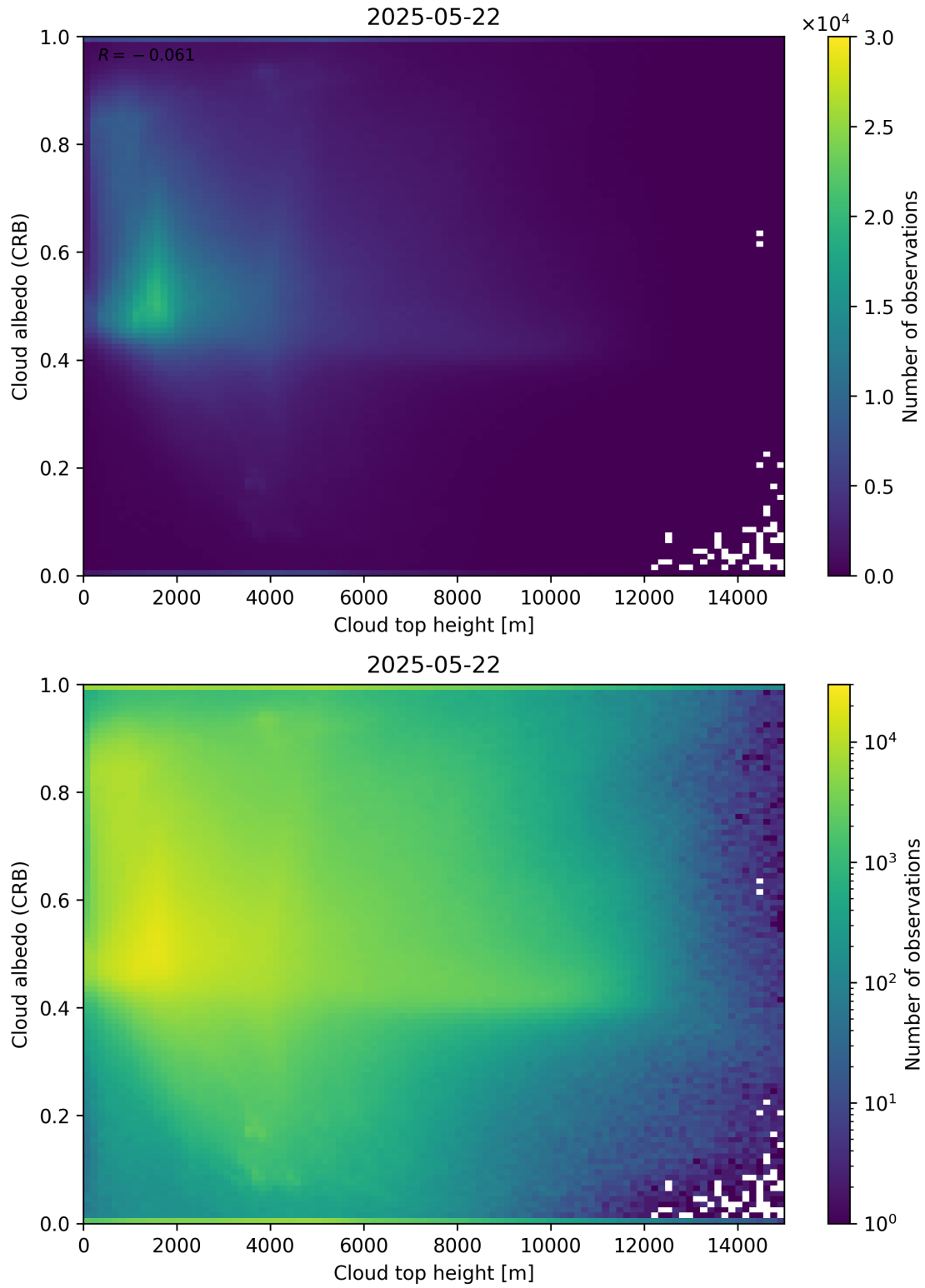
Figure 86: Scatter density plot of “Cloud top height” against “Cloud albedo (CRB)” for 2025-05-21 to 2025-05-23.
