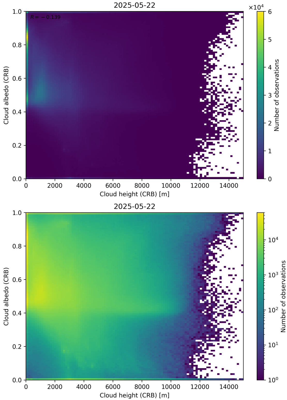
Figure 80: Scatter density plot of “Cloud height (CRB)” against “Cloud albedo (CRB)” for 2025-05-21 to 2025-05-23.
