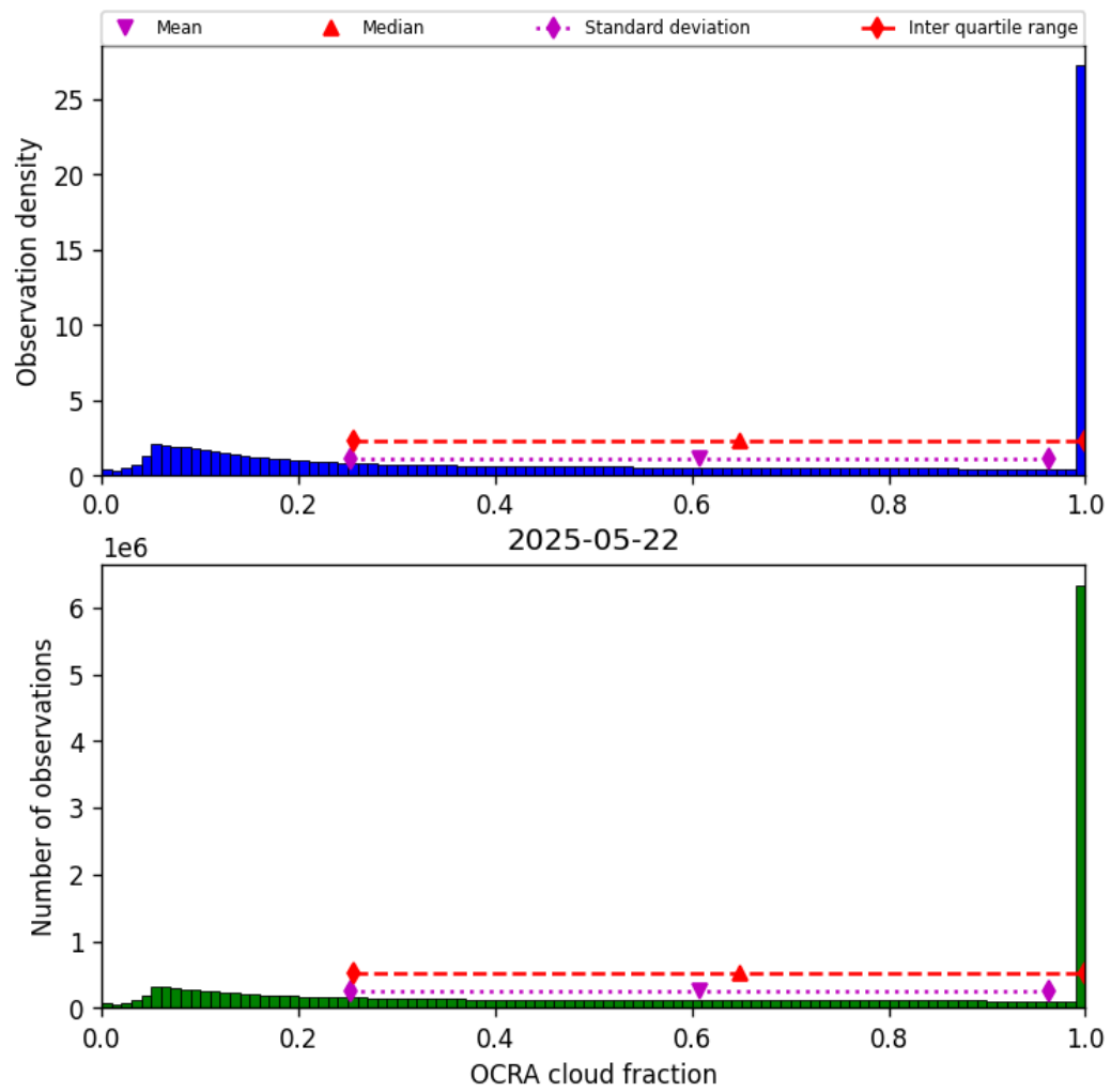
Figure 50: Histogram of “OCRA cloud fraction” for 2025-05-21 to 2025-05-23
