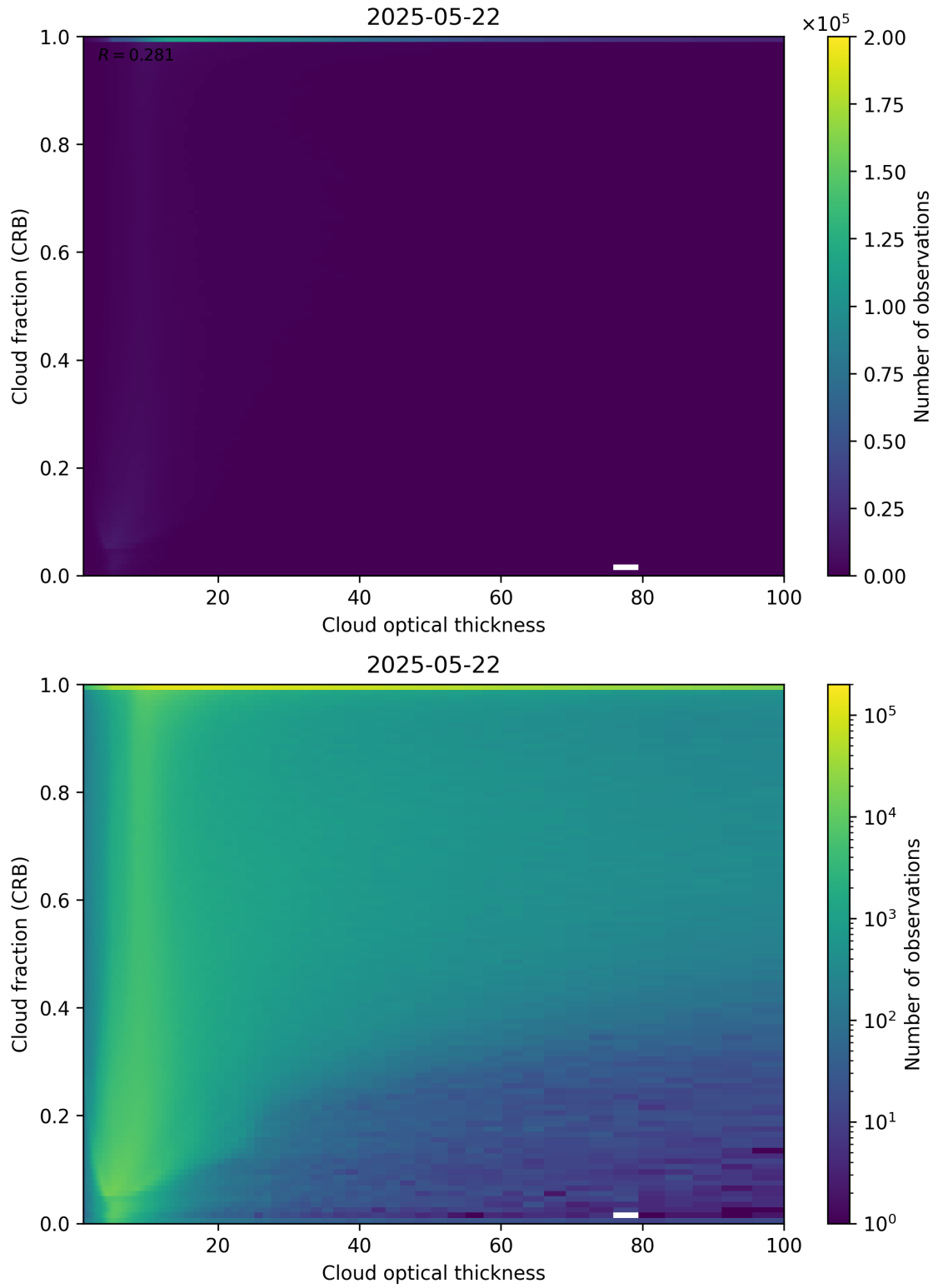
Figure 84: Scatter density plot of “Cloud optical thickness” against “Cloud fraction (CRB)” for 2025-05-21 to 2025-05-23.
