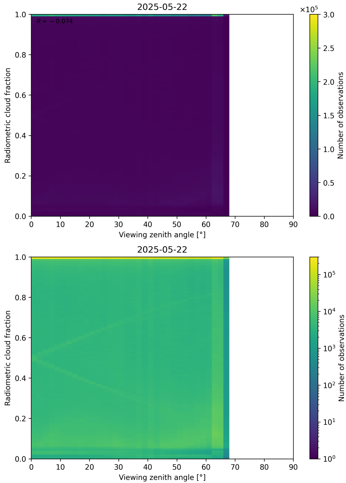
Figure 107: Scatter density plot of “Viewing zenith angle” against “Radiometric cloud fraction” for 2025-05-21 to 2025-05-23.
