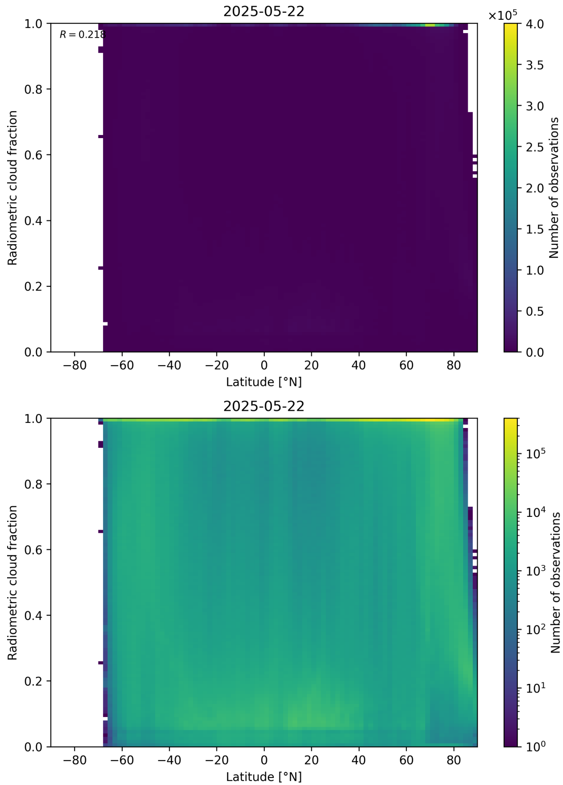
Figure 92: Scatter density plot of “Latitude” against “Radiometric cloud fraction” for 2025-05-21 to 2025-05-23.
