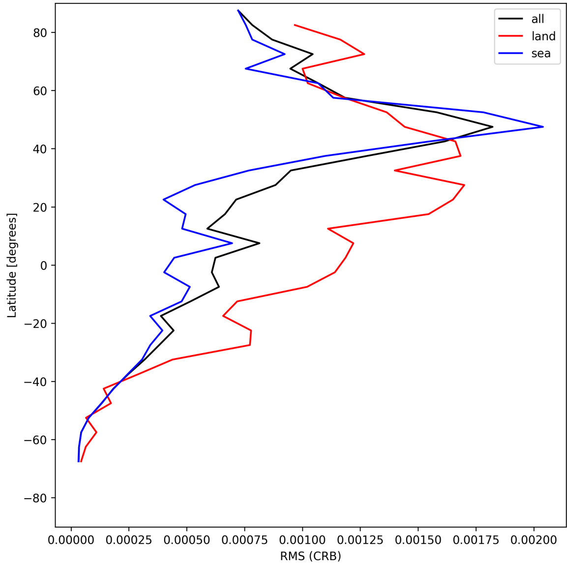
Figure 32: Zonal average of “RMS (CRB)” for 2025-05-21 to 2025-05-23.
