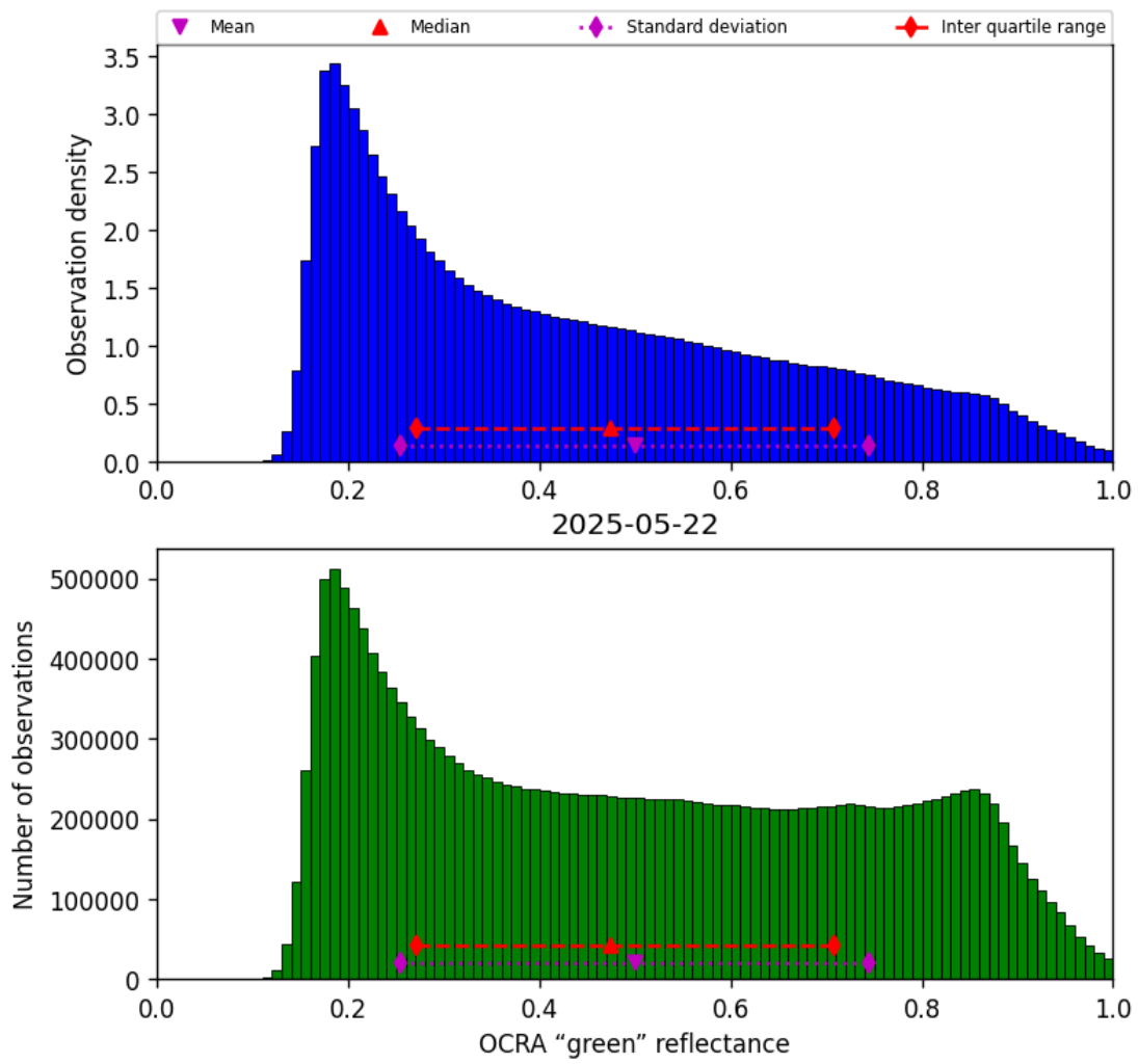
Figure 52: Histogram of “OCRA “green” reflectance” for 2025-05-21 to 2025-05-23
