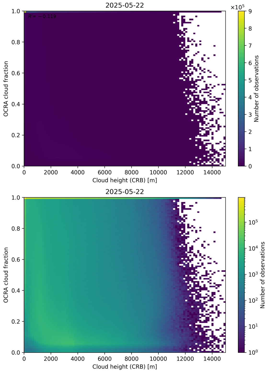
Figure 81: Scatter density plot of “Cloud height (CRB)” against “OCRA cloud fraction” for 2025-05-21 to 2025-05-23.
