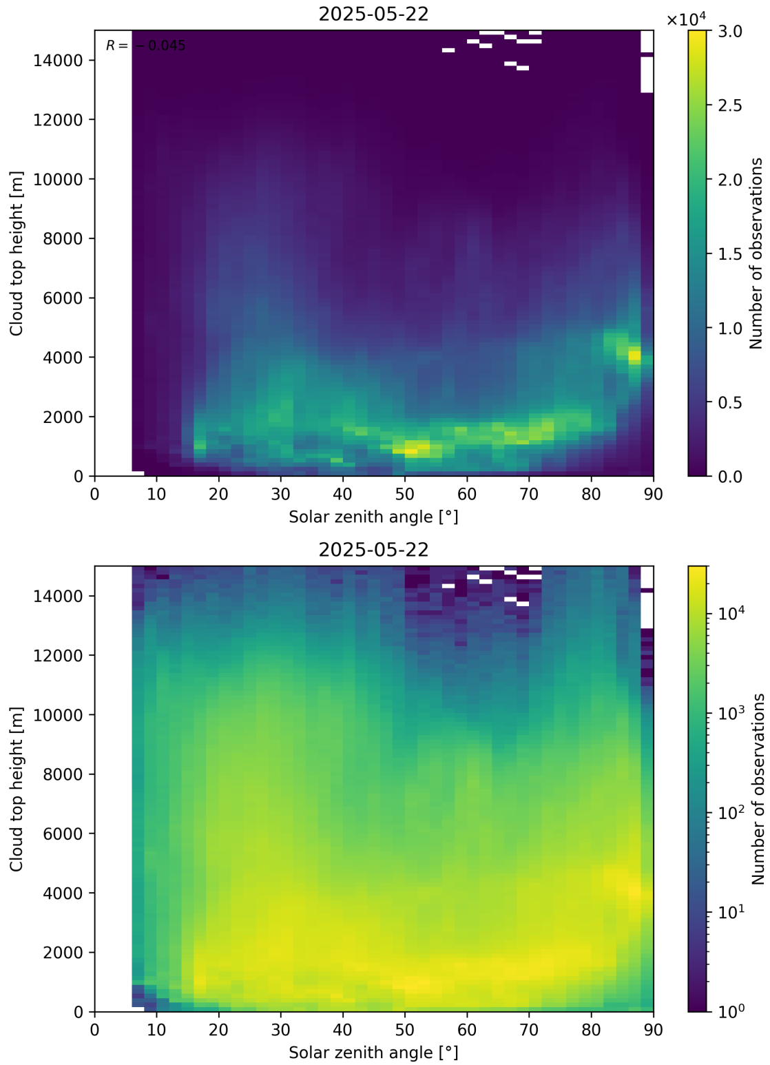
Figure 104: Scatter density plot of “Solar zenith angle” against “Cloud top height” for 2025-05-21 to 2025-05-23.
