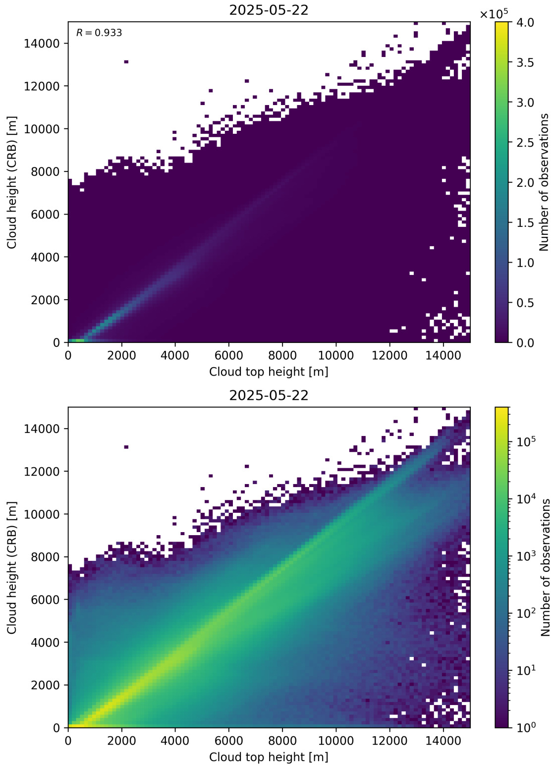
Figure 89: Scatter density plot of “Cloud top height” against “Cloud height (CRB)” for 2025-05-21 to 2025-05-23.
