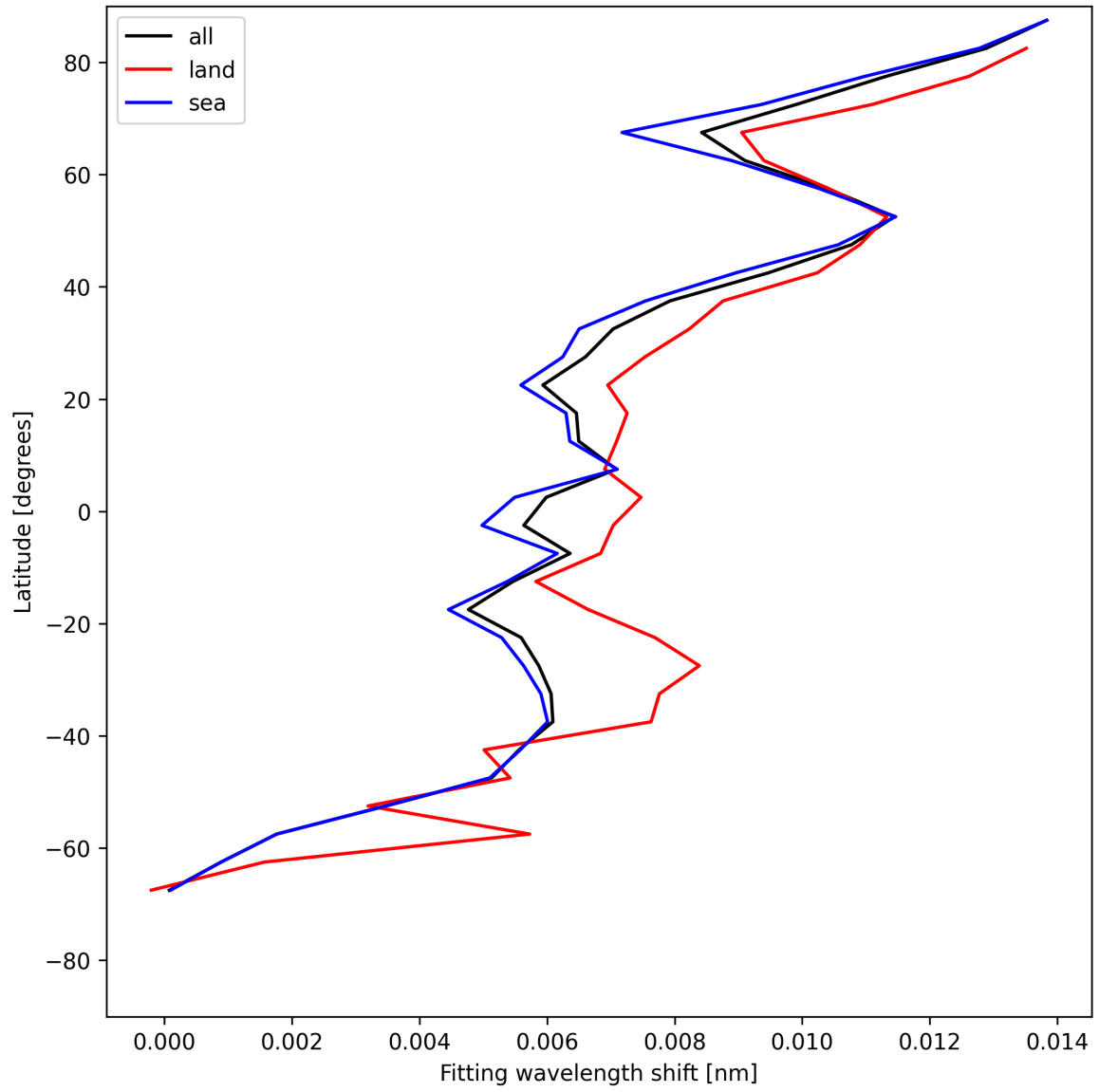
Figure 33: Zonal average of “Fitting wavelength shift” for 2025-05-21 to 2025-05-23.
