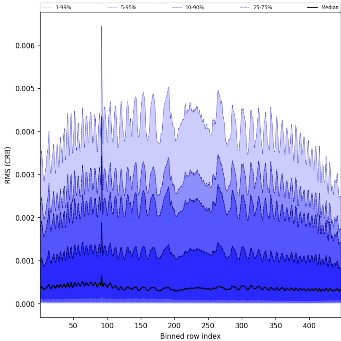
Figure 64: Along track statistics of “RMS (CRB)” for 2025-05-21 to 2025-05-23
