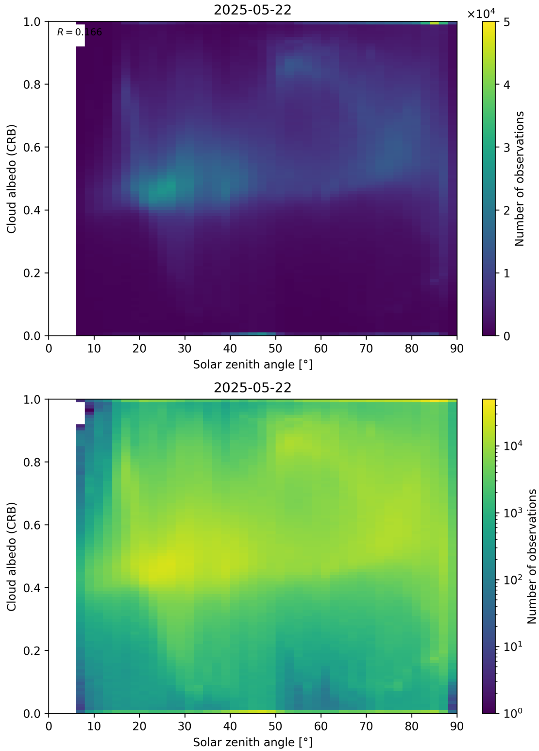
Figure 98: Scatter density plot of “Solar zenith angle” against “Cloud albedo (CRB)” for 2025-05-21 to 2025-05-23.
