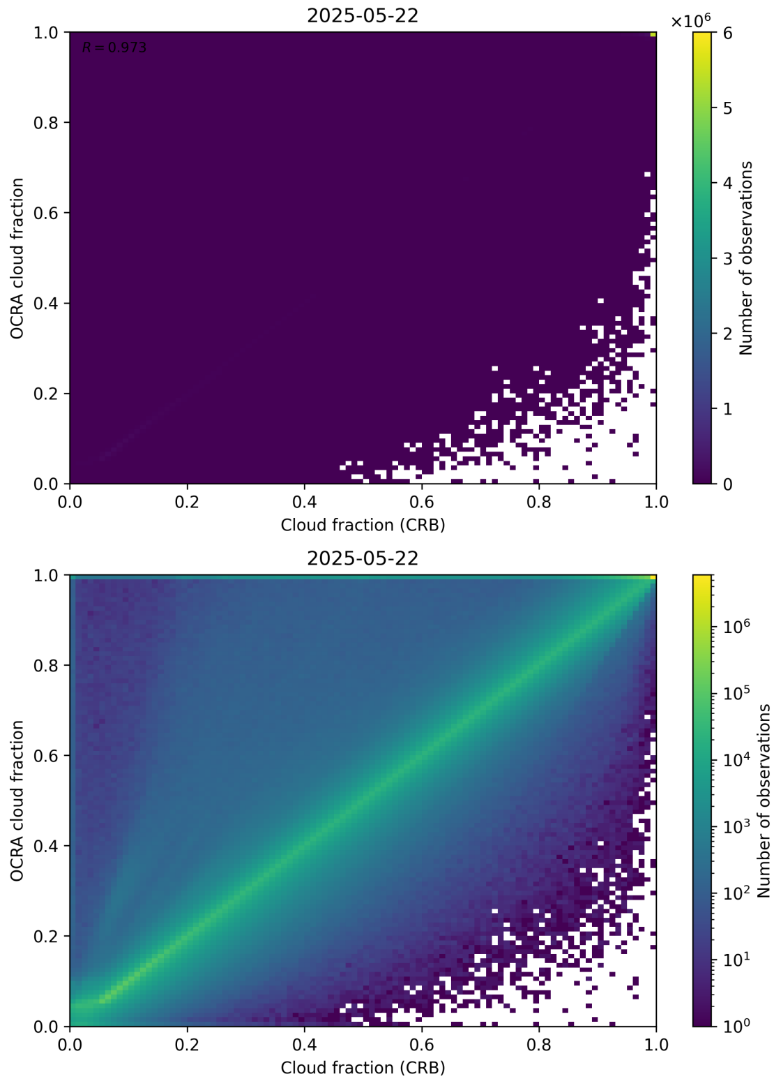
Figure 78: Scatter density plot of “Cloud fraction (CRB)” against “OCRA cloud fraction” for 2025-05-21 to 2025-05-23.
