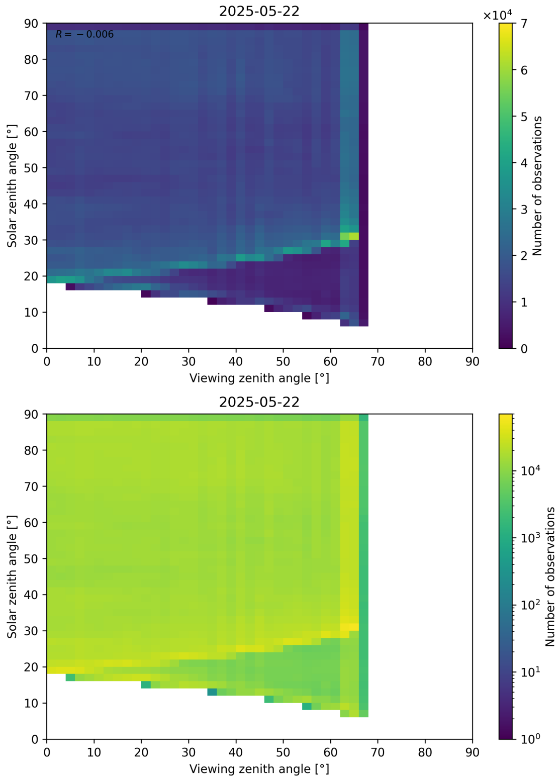
Figure 114: Scatter density plot of “Viewing zenith angle” against “Solar zenith angle” for 2025-05-21 to 2025-05-23.
