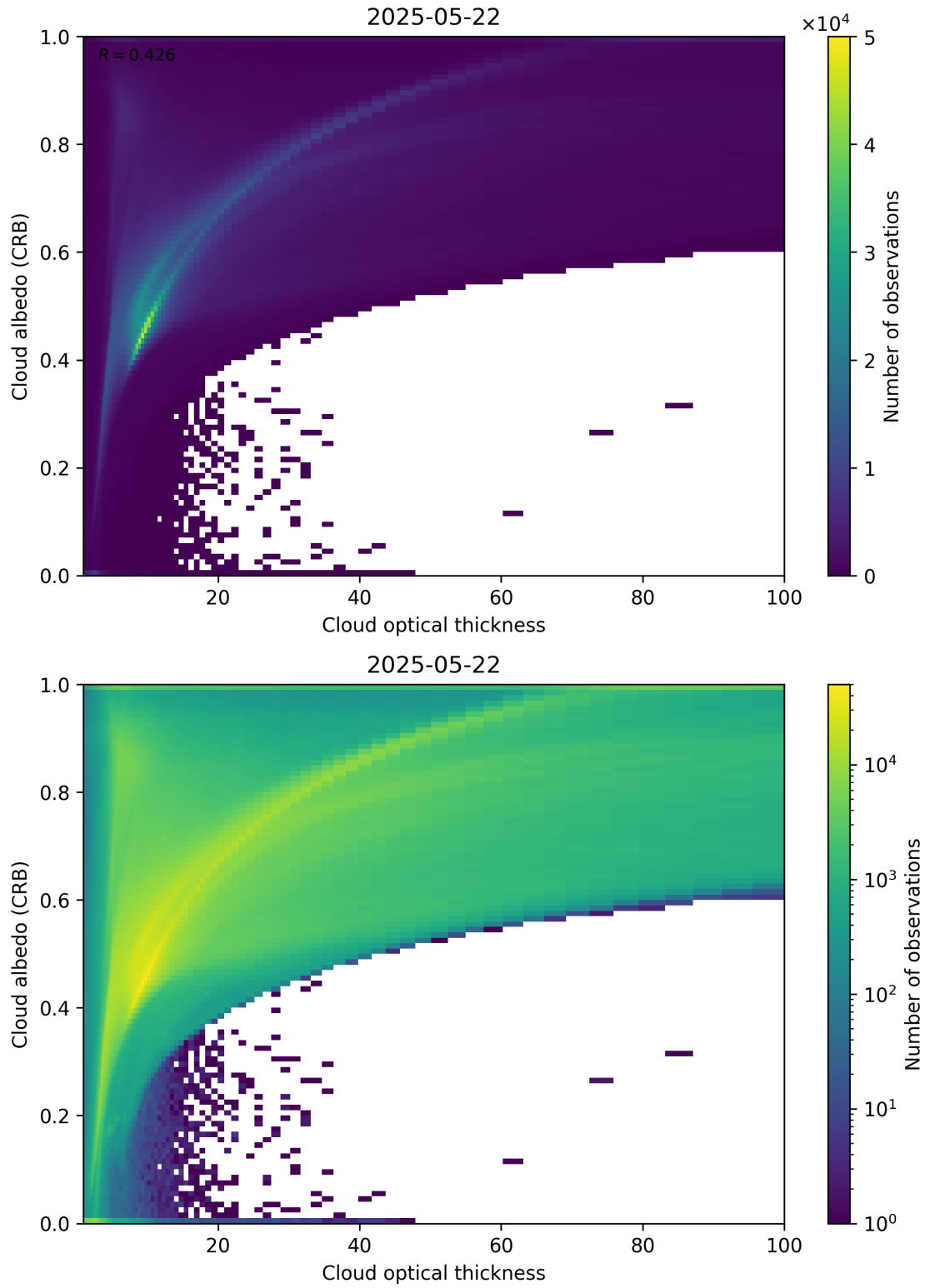
Figure 82: Scatter density plot of “Cloud optical thickness” against “Cloud albedo (CRB)” for 2025-05-21 to 2025-05-23.
