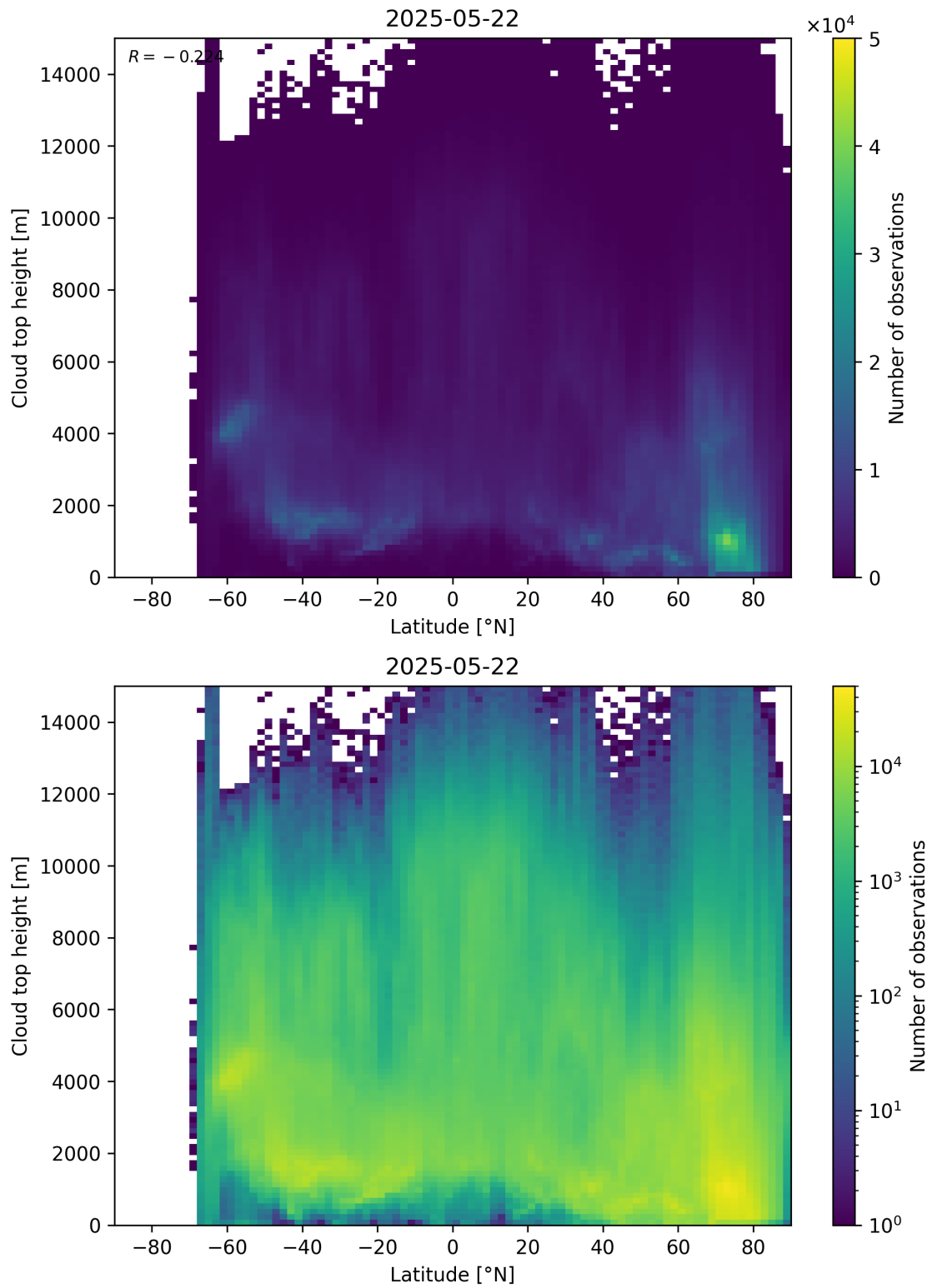
Figure 97: Scatter density plot of “Latitude” against “Cloud top height” for 2025-05-21 to 2025-05-23.
