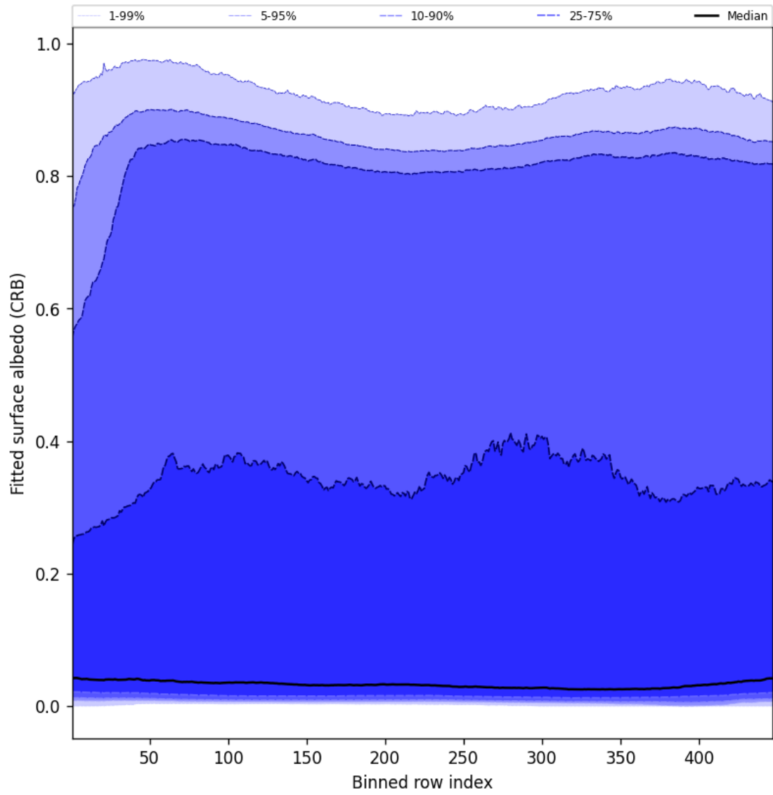
Figure 62: Along track statistics of “Fitted surface albedo (CRB)” for 2025-05-21 to 2025-05-23
