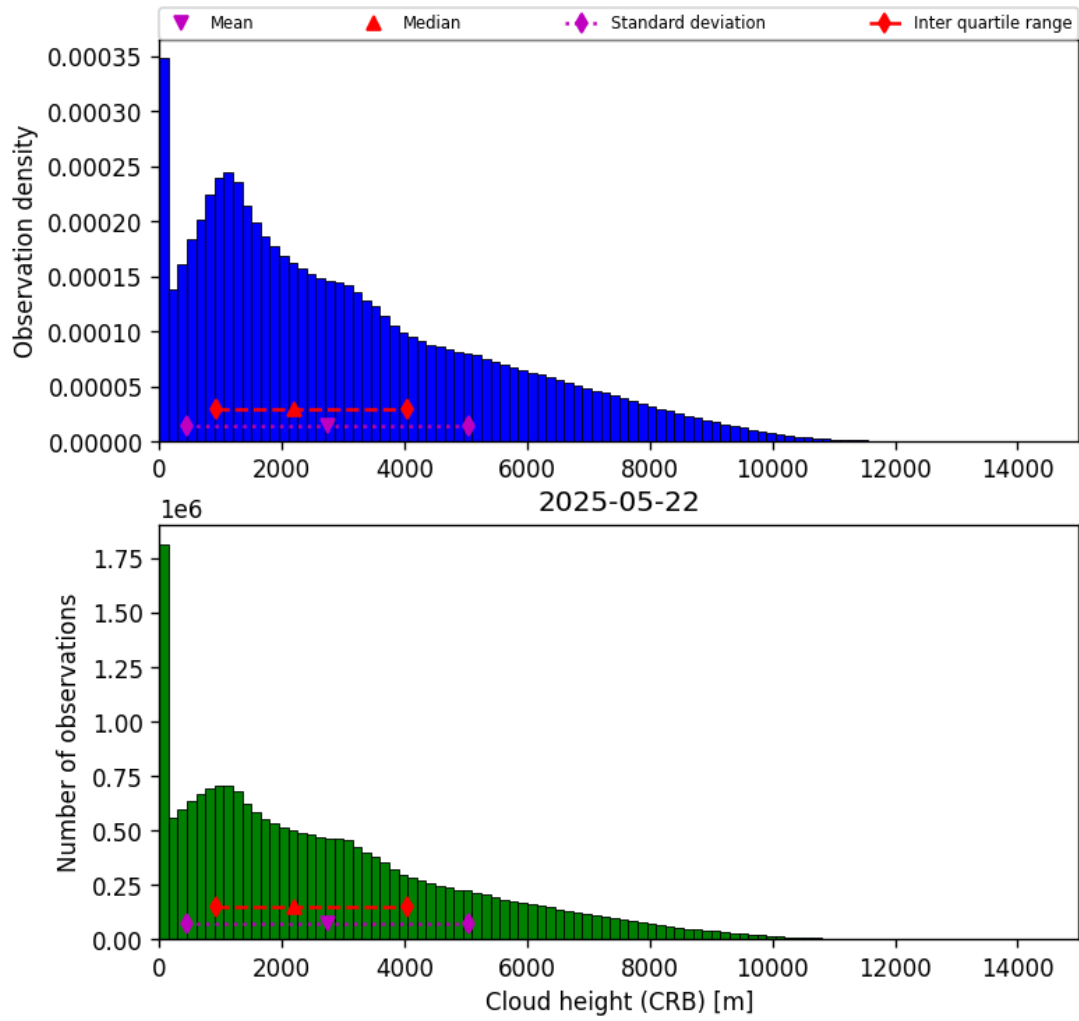
Figure 43: Histogram of “Cloud height (CRB)” for 2025-05-21 to 2025-05-23
