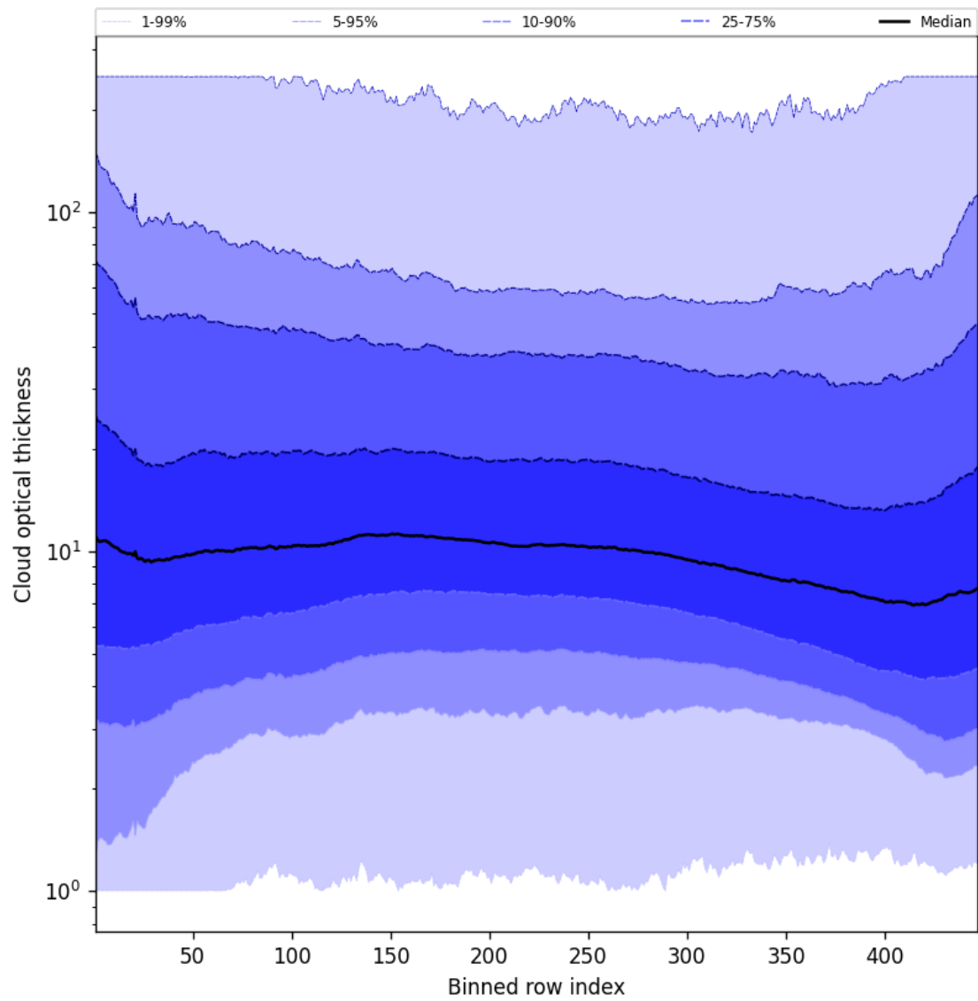
Figure 57: Along track statistics of “Cloud optical thickness” for 2025-05-21 to 2025-05-23
