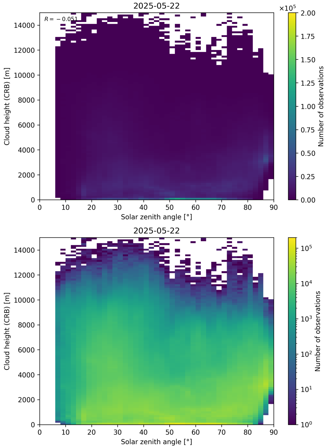
Figure 102: Scatter density plot of “Solar zenith angle” against “Cloud height (CRB)” for 2025-05-21 to 2025-05-23.
