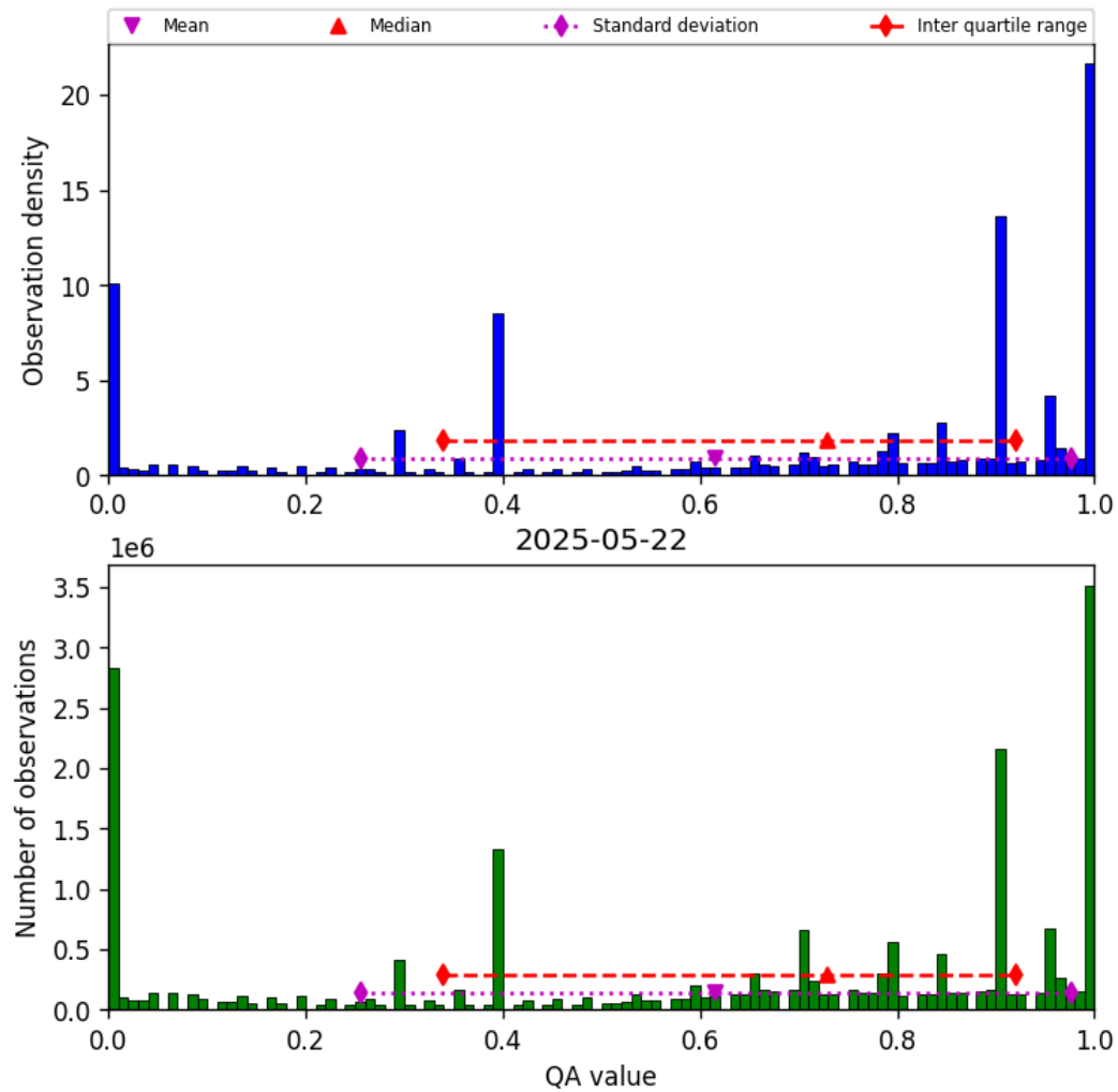
Figure 38: Histogram of “QA value” for 2025-05-21 to 2025-05-23
