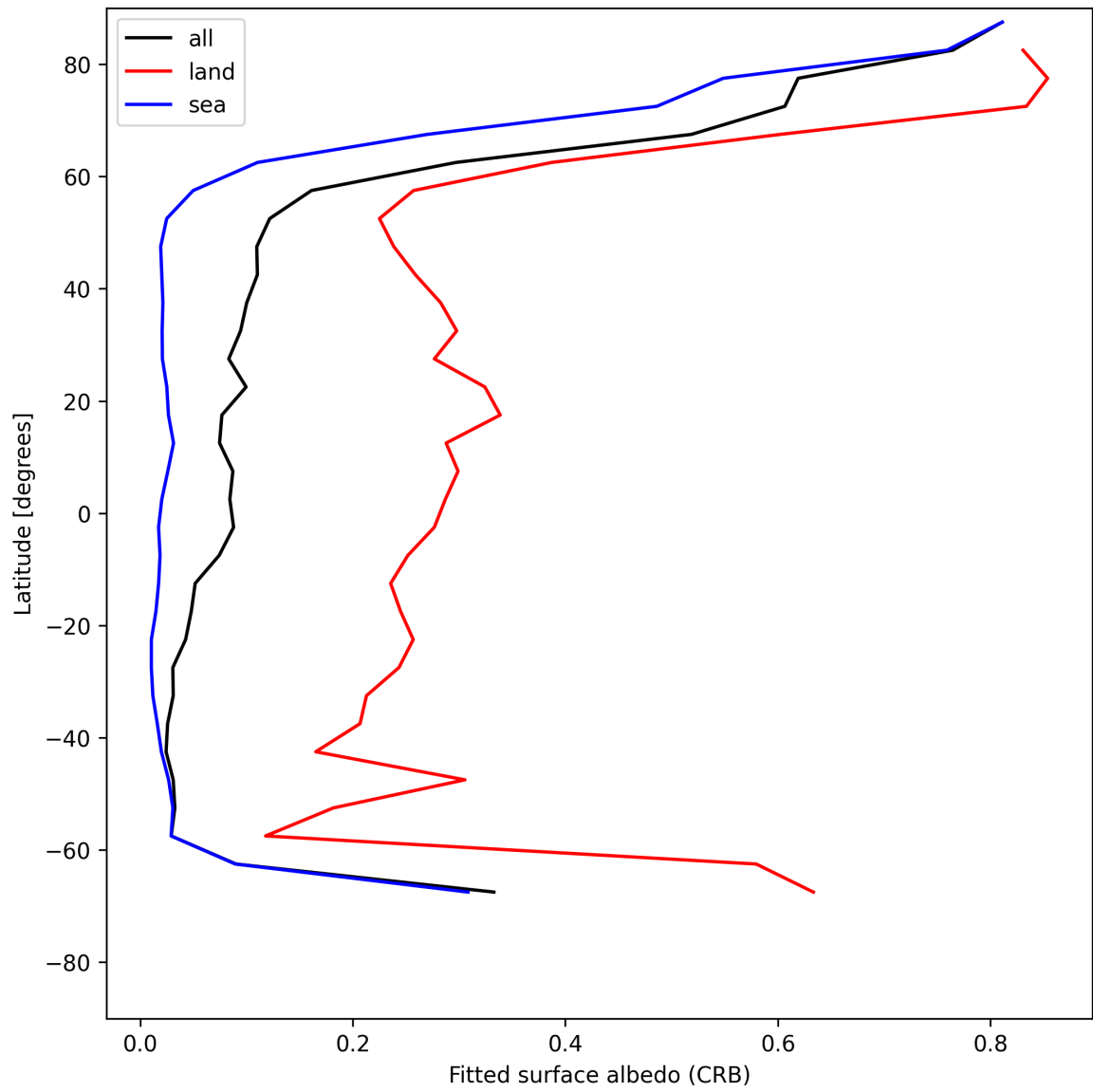
Figure 30: Zonal average of “Fitted surface albedo (CRB)” for 2025-05-21 to 2025-05-23.
