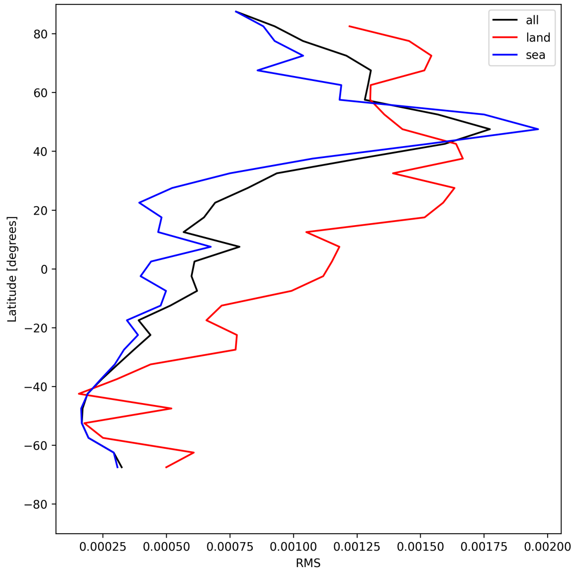
Figure 31: Zonal average of “RMS” for 2025-05-21 to 2025-05-23.
