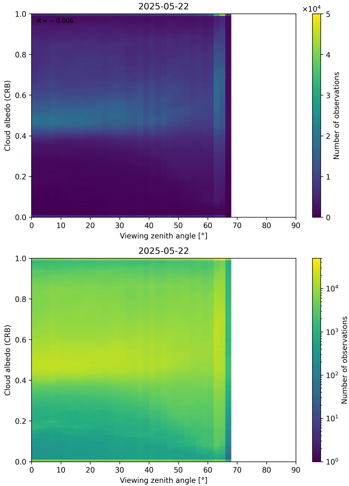
Figure 106: Scatter density plot of “Viewing zenith angle” against “Cloud albedo (CRB)” for 2025-05-21 to 2025-05-23.
