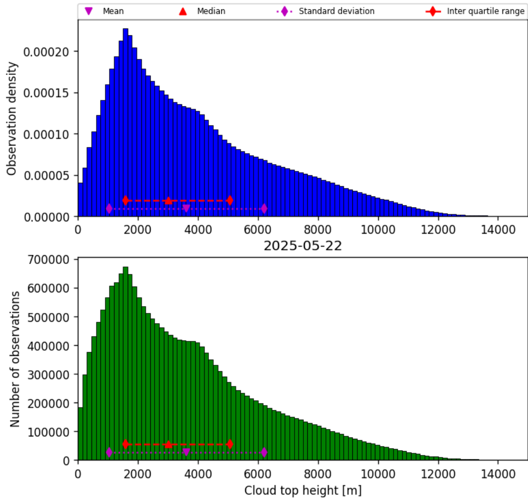
Figure 40: Histogram of “Cloud top height” for 2025-05-21 to 2025-05-23
