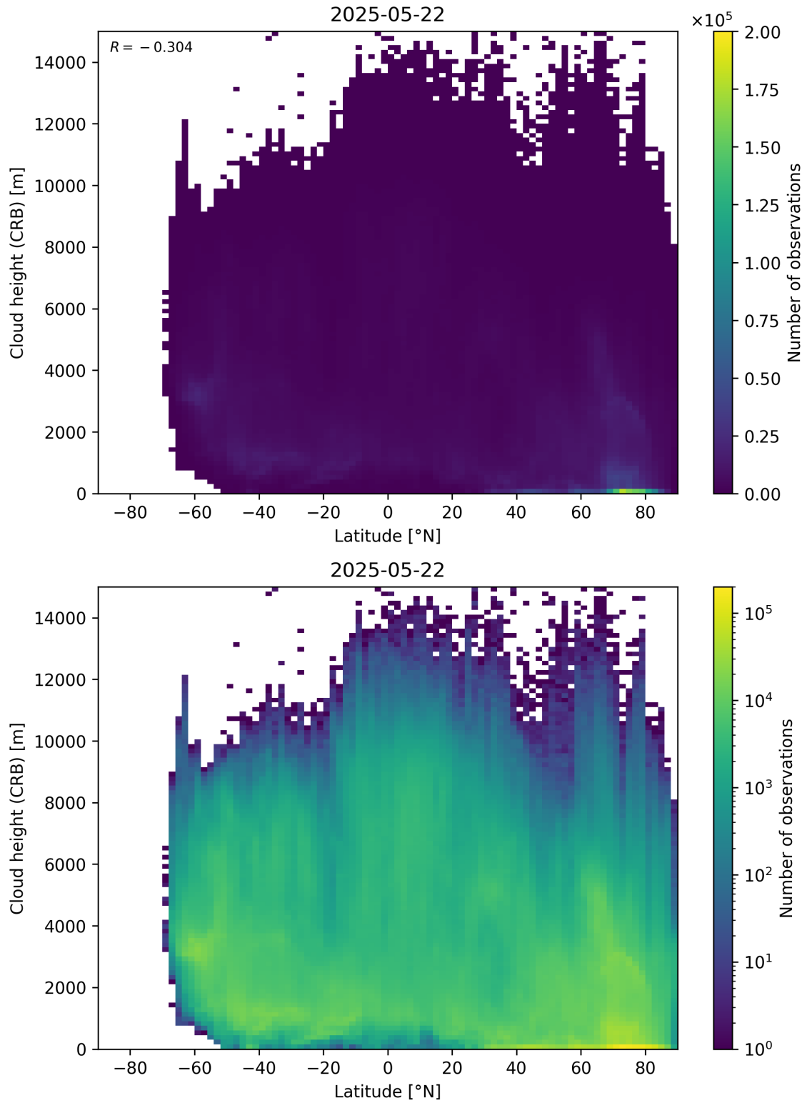
Figure 95: Scatter density plot of “Latitude” against “Cloud height (CRB)” for 2025-05-21 to 2025-05-23.
