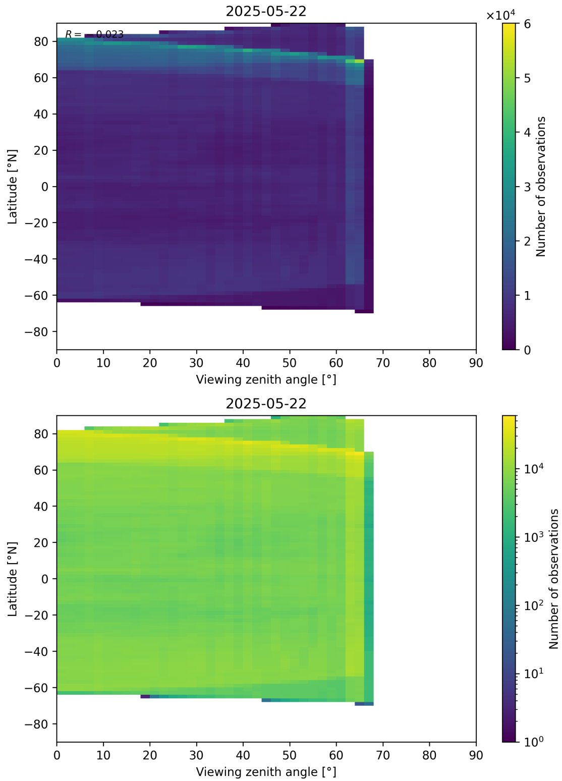
Figure 113: Scatter density plot of “Viewing zenith angle” against “Latitude” for 2025-05-21 to 2025-05-23.
