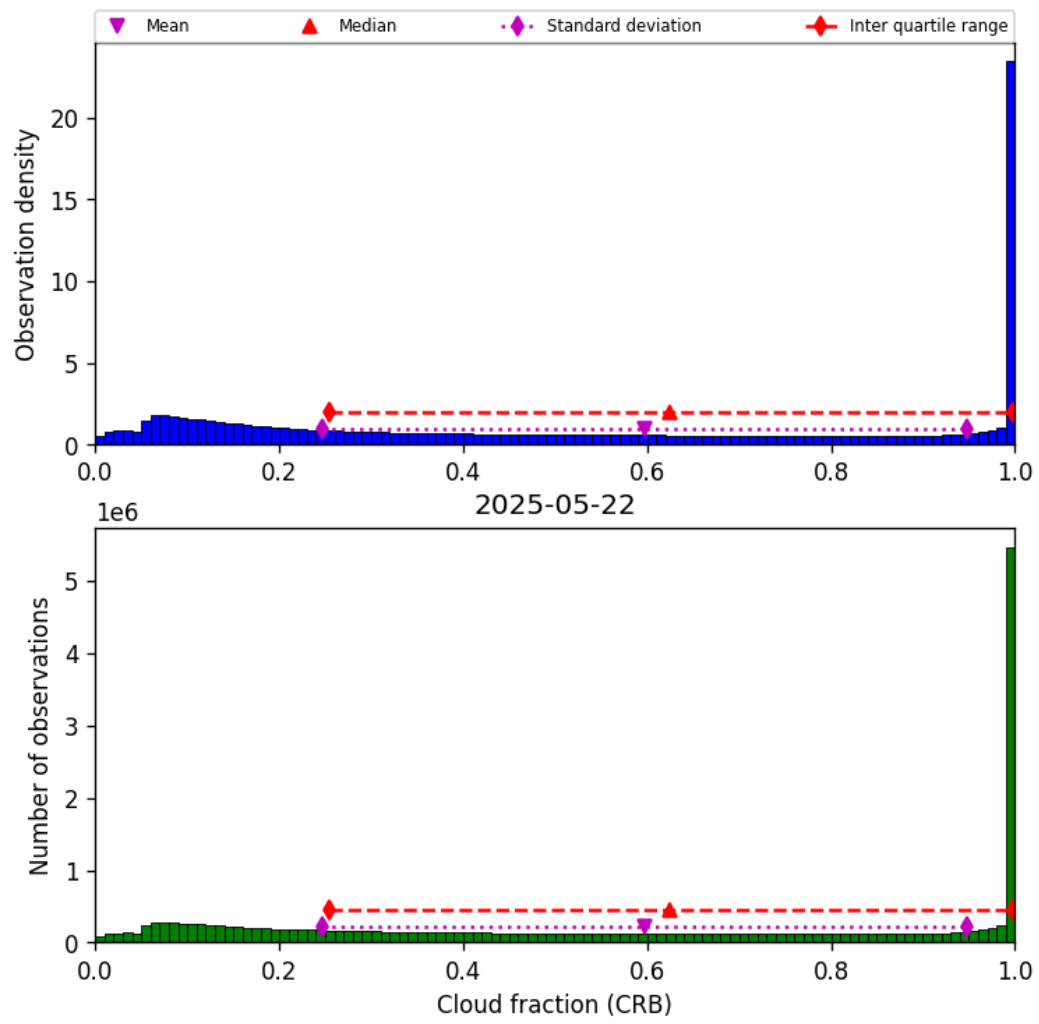
Figure 42: Histogram of “Cloud fraction (CRB)” for 2025-05-21 to 2025-05-23
