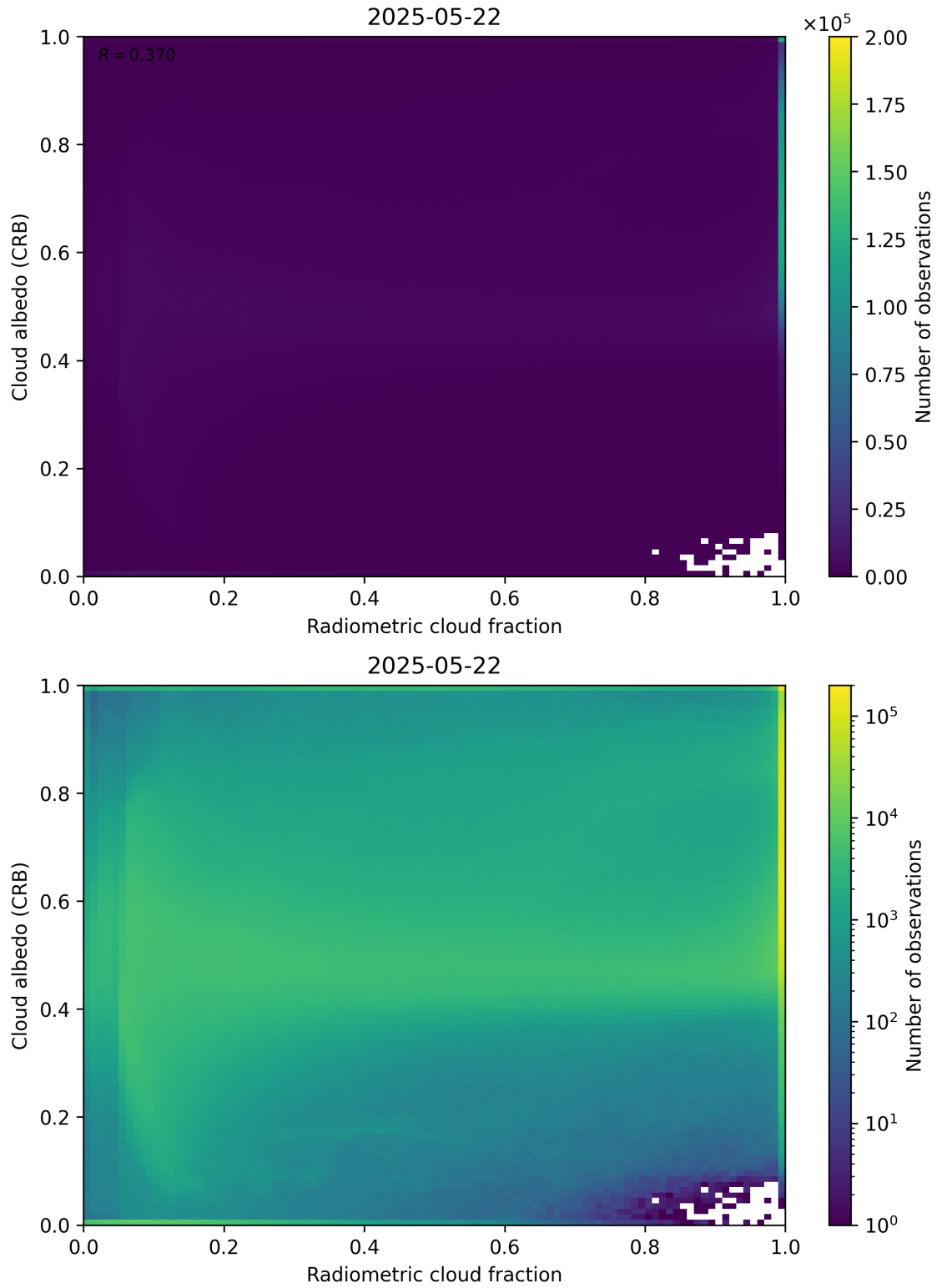
Figure 71: Scatter density plot of “Radiometric cloud fraction” against “Cloud albedo (CRB)” for 2025-05-21 to 2025-05-23.
