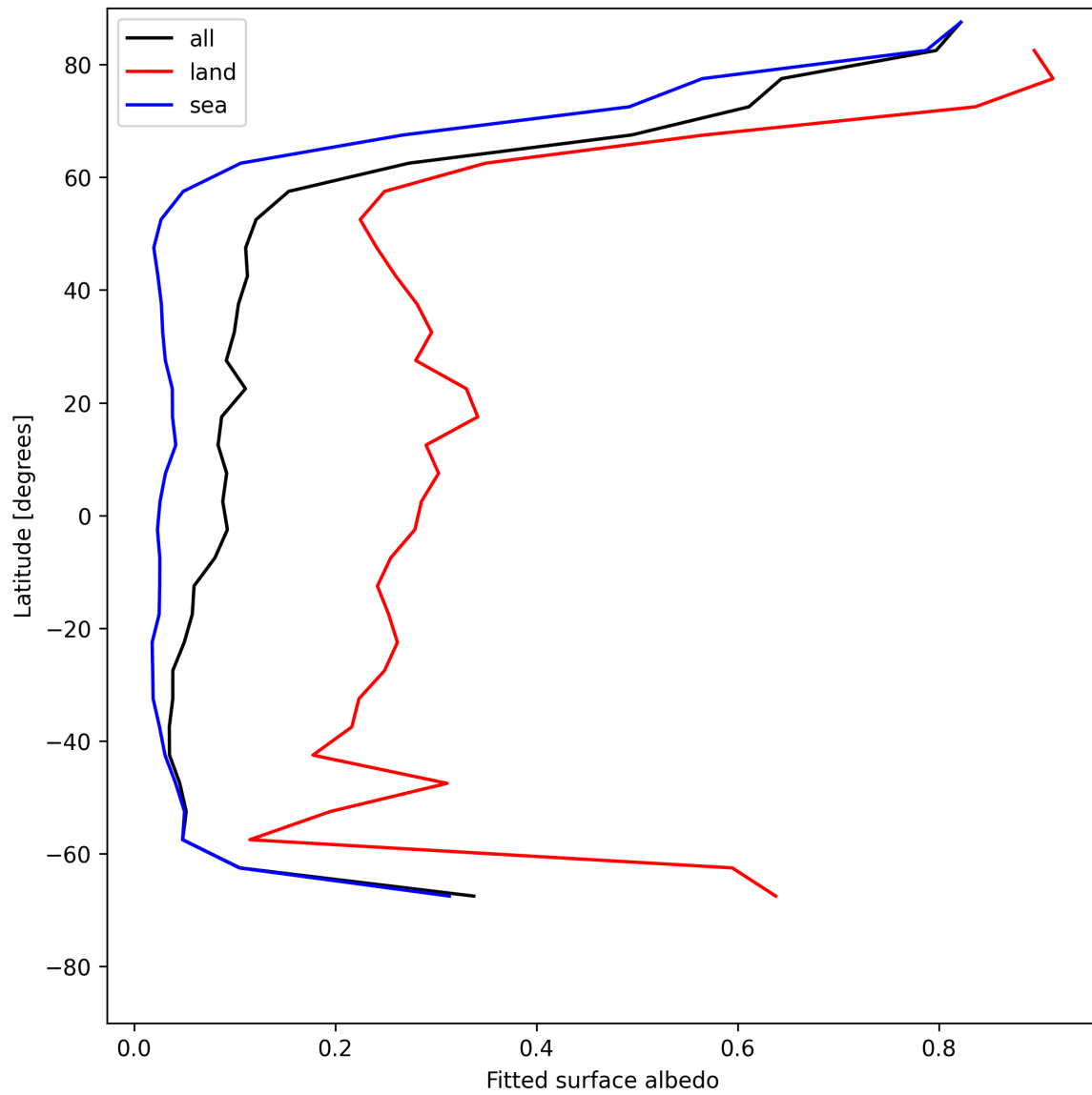
Figure 29: Zonal average of “Fitted surface albedo” for 2025-05-21 to 2025-05-23.
