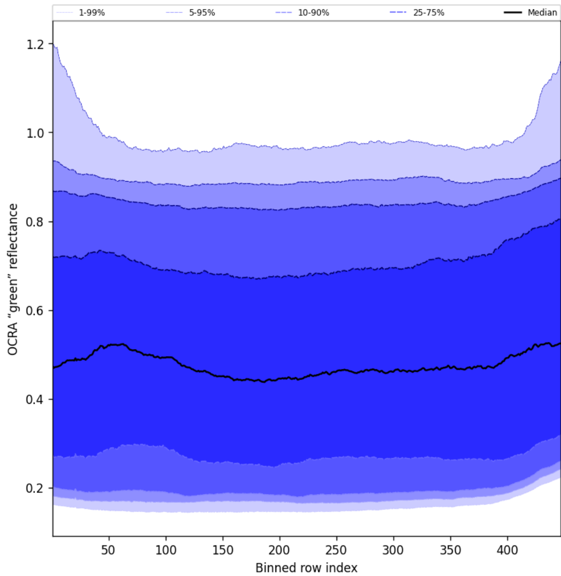
Figure 68: Along track statistics of “OCRA “green” reflectance” for 2025-05-21 to 2025-05-23
