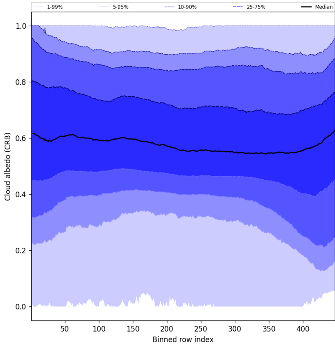
Figure 60: Along track statistics of “Cloud albedo (CRB)” for 2025-05-21 to 2025-05-23
