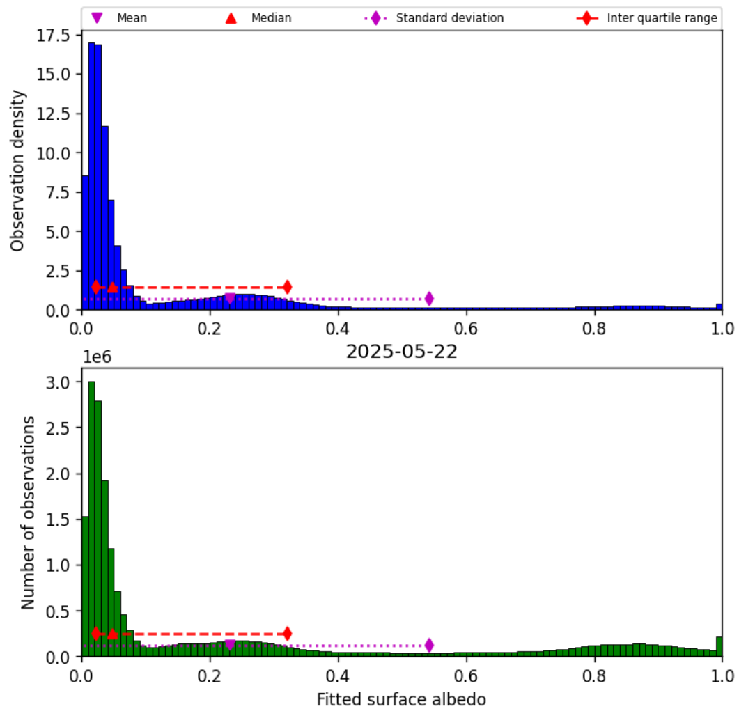
Figure 45: Histogram of “Fitted surface albedo” for 2025-05-21 to 2025-05-23
