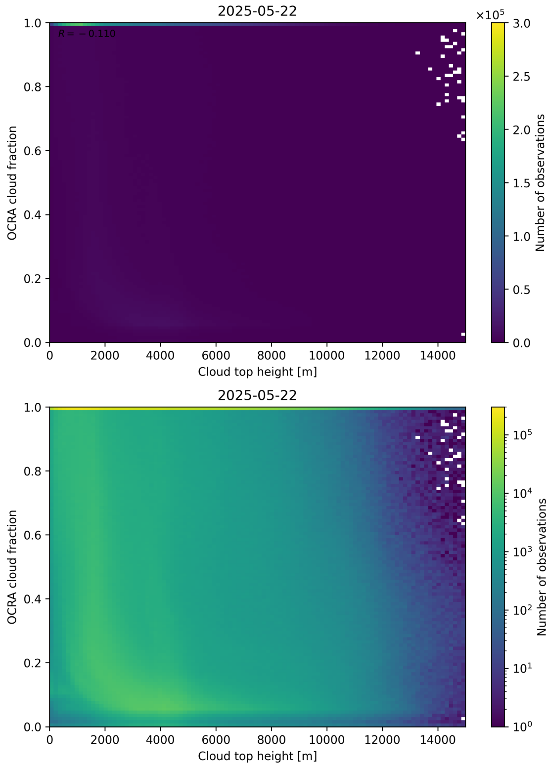
Figure 87: Scatter density plot of “Cloud top height” against “OCRA cloud fraction” for 2025-05-21 to 2025-05-23.
