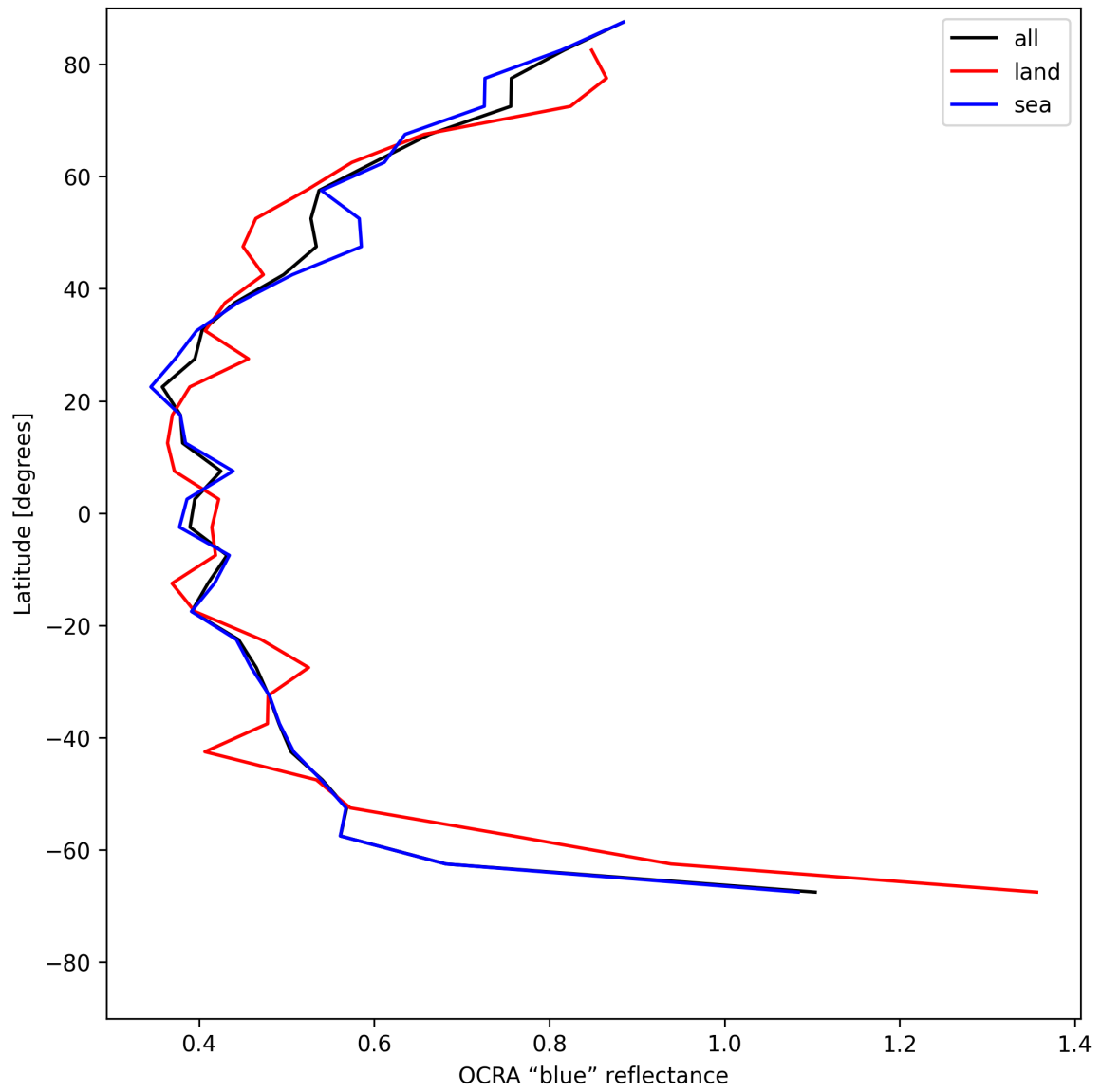
Figure 35: Zonal average of “OCRA “blue” reflectance” for 2025-05-21 to 2025-05-23.
