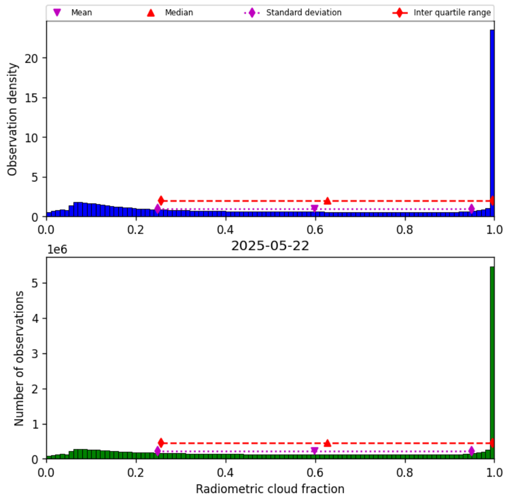
Figure 39: Histogram of “Radiometric cloud fraction” for 2025-05-21 to 2025-05-23
