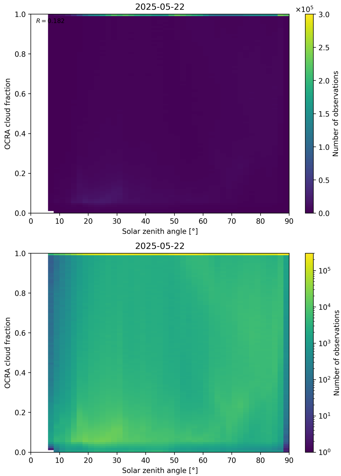
Figure 100: Scatter density plot of “Solar zenith angle” against “OCRA cloud fraction” for 2025-05-21 to 2025-05-23.
