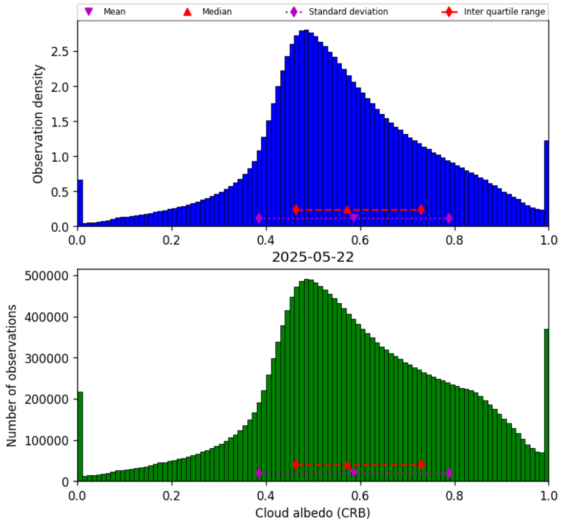
Figure 44: Histogram of “Cloud albedo (CRB)” for 2025-05-21 to 2025-05-23
