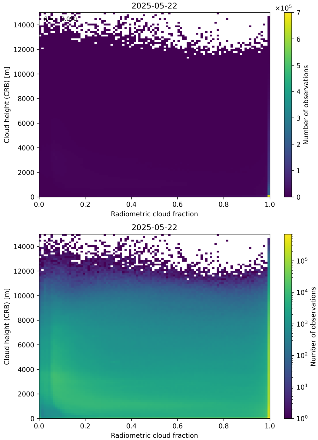
Figure 74: Scatter density plot of “Radiometric cloud fraction” against “Cloud height (CRB)” for 2025-05-21 to 2025-05-23.
