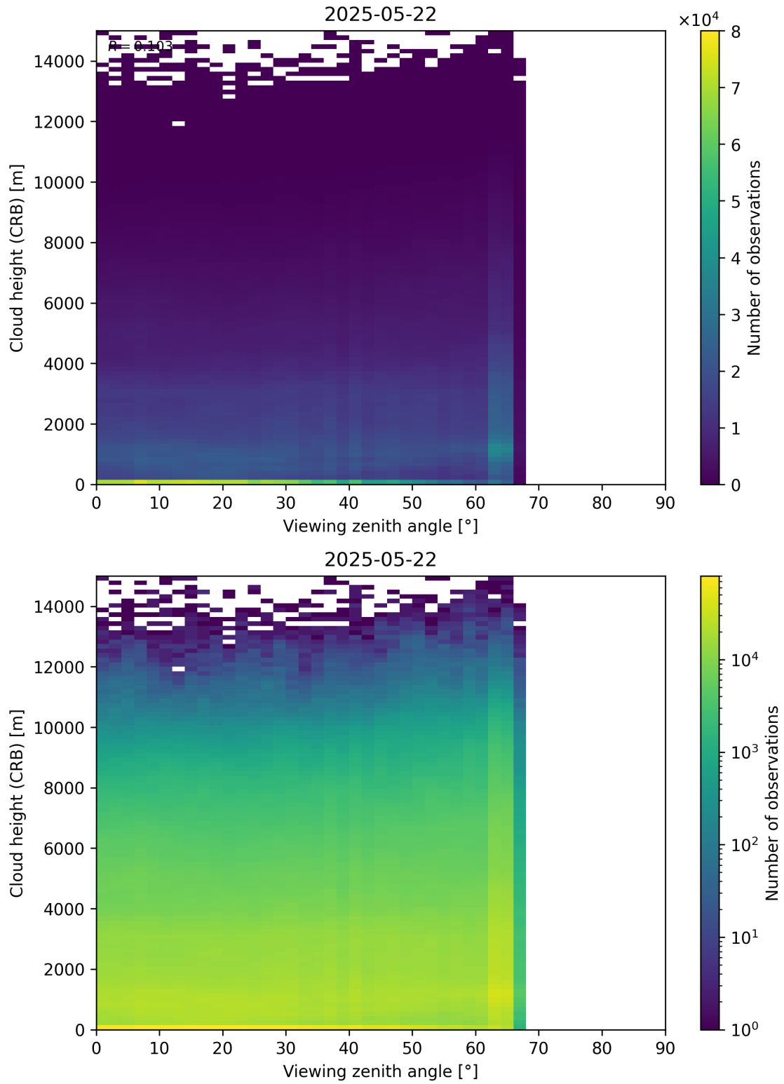
Figure 110: Scatter density plot of “Viewing zenith angle” against “Cloud height (CRB)” for 2025-05-21 to 2025-05-23.
