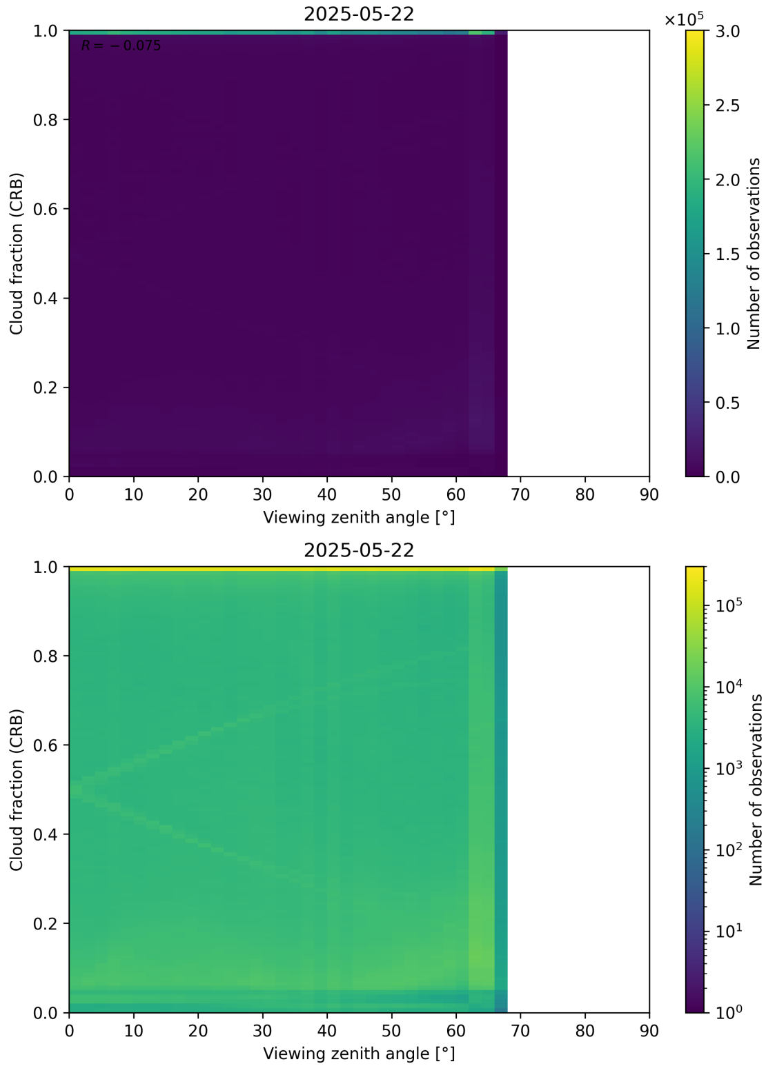
Figure 109: Scatter density plot of “Viewing zenith angle” against “Cloud fraction (CRB)” for 2025-05-21 to 2025-05-23.
