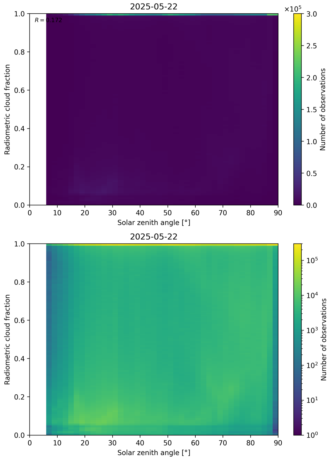
Figure 99: Scatter density plot of “Solar zenith angle” against “Radiometric cloud fraction” for 2025-05-21 to 2025-05-23.
