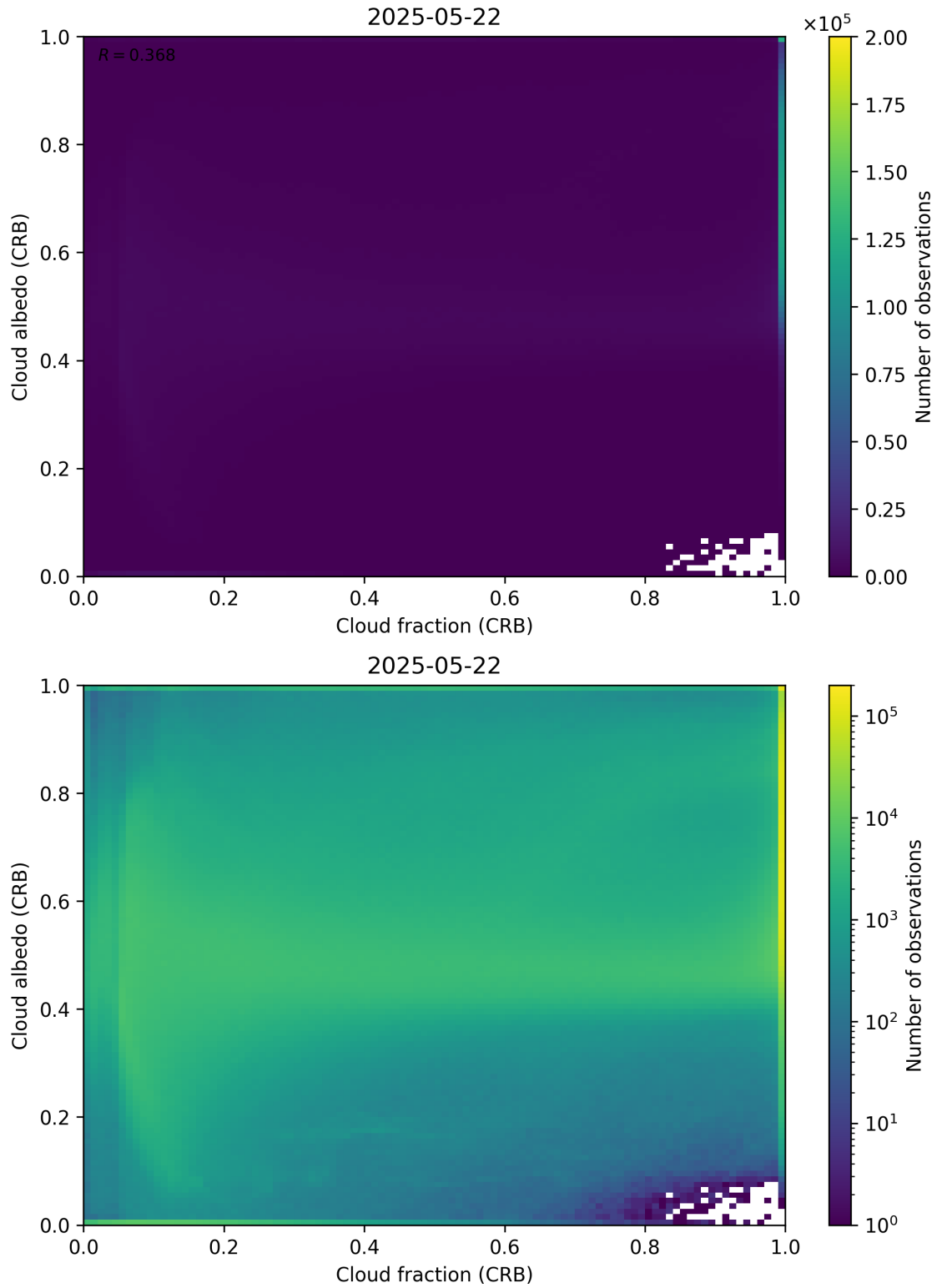
Figure 77: Scatter density plot of “Cloud fraction (CRB)” against “Cloud albedo (CRB)” for 2025-05-21 to 2025-05-23.
