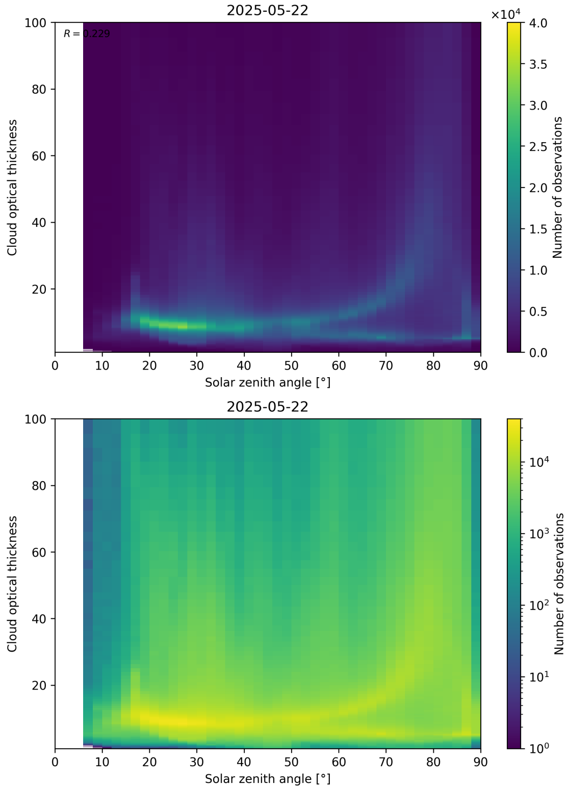
Figure 103: Scatter density plot of “Solar zenith angle” against “Cloud optical thickness” for 2025-05-21 to 2025-05-23.
