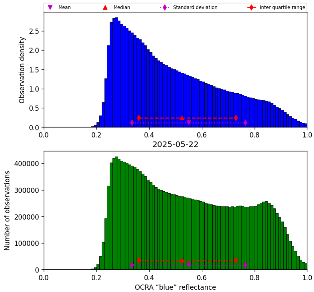
Figure 51: Histogram of “OCRA “blue” reflectance” for 2025-05-21 to 2025-05-23
