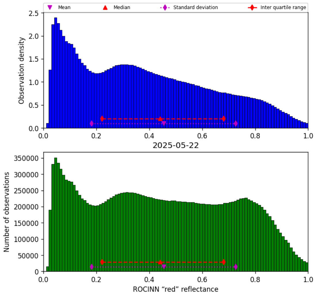
Figure 53: Histogram of “ROCINN “red” reflectance” for 2025-05-21 to 2025-05-23
