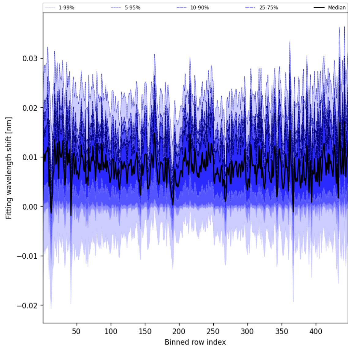
Figure 65: Along track statistics of “Fitting wavelength shift” for 2025-05-21 to 2025-05-23
