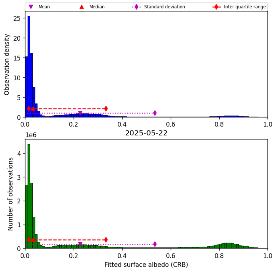
Figure 46: Histogram of “Fitted surface albedo (CRB)” for 2025-05-21 to 2025-05-23
