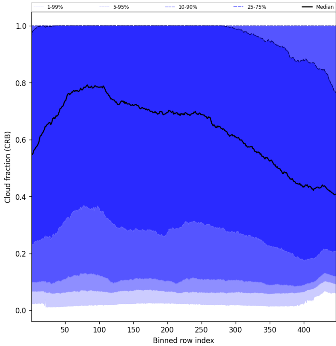
Figure 58: Along track statistics of “Cloud fraction (CRB)” for 2025-05-21 to 2025-05-23
