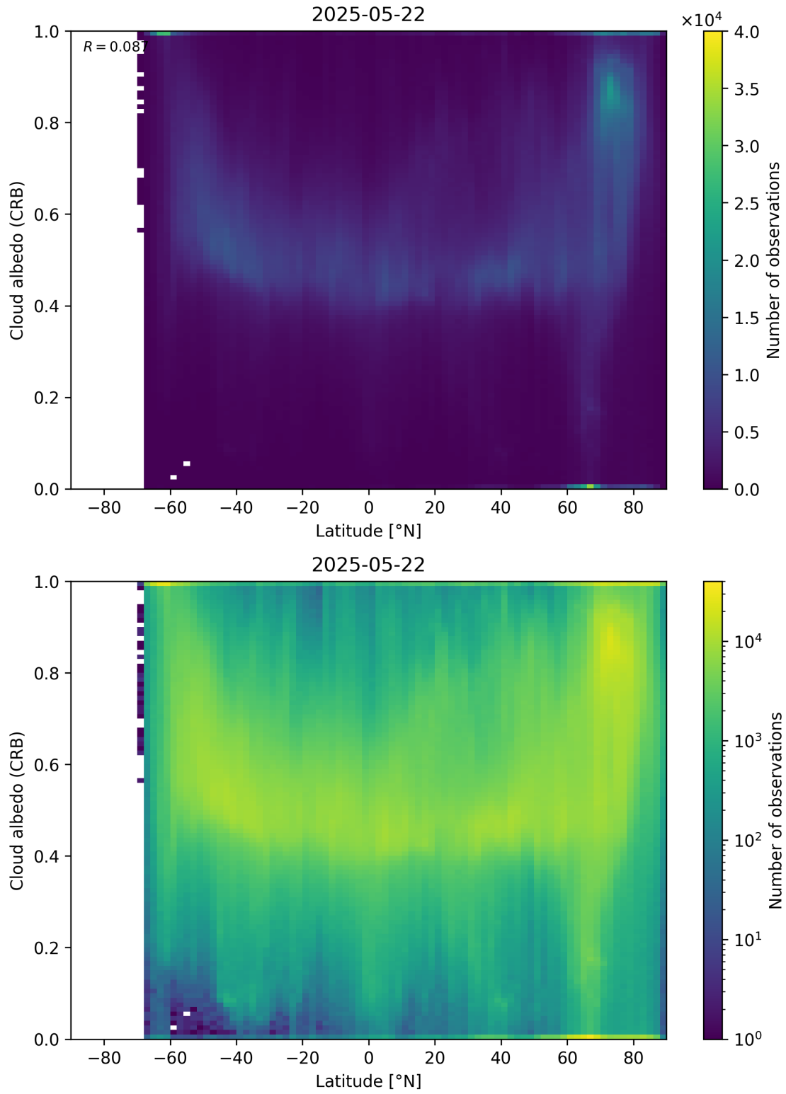
Figure 91: Scatter density plot of “Latitude” against “Cloud albedo (CRB)” for 2025-05-21 to 2025-05-23.
