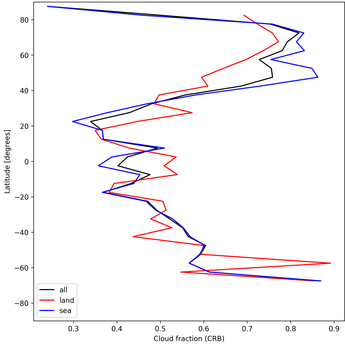
Figure 26: Zonal average of “Cloud fraction (CRB)” for 2025-05-21 to 2025-05-23.
