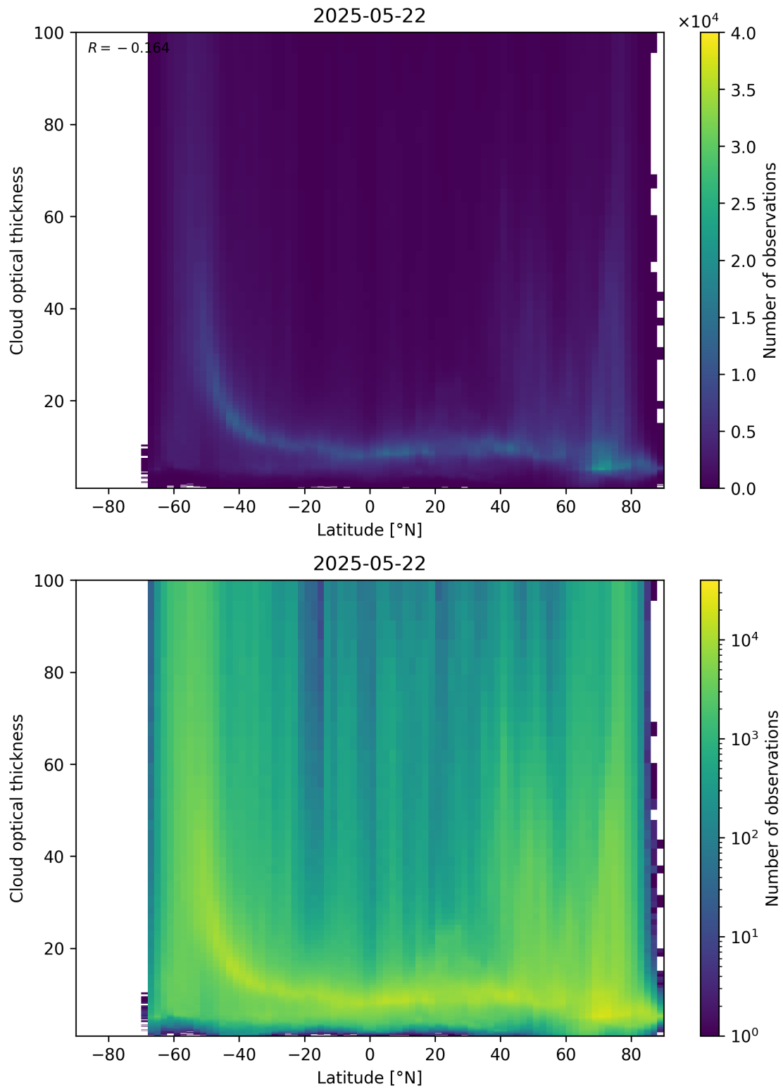
Figure 96: Scatter density plot of “Latitude” against “Cloud optical thickness” for 2025-05-21 to 2025-05-23.
