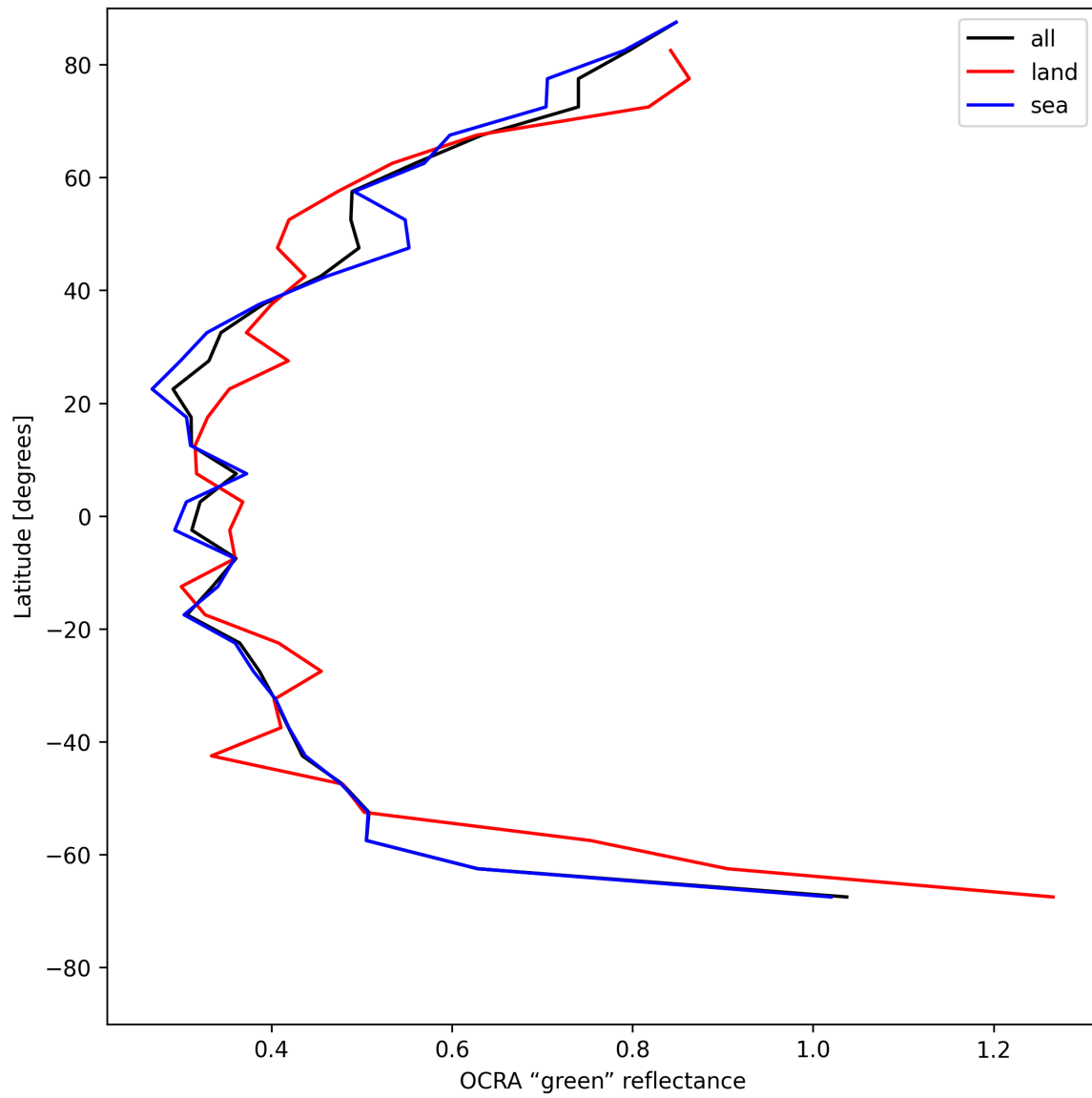
Figure 36: Zonal average of “OCRA “green” reflectance” for 2025-05-21 to 2025-05-23.
