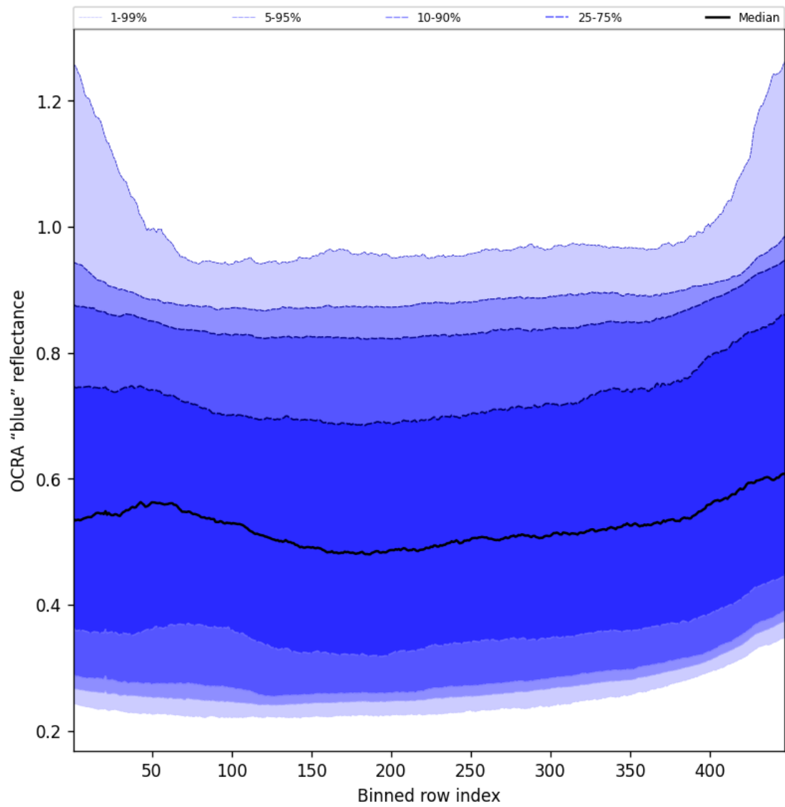
Figure 67: Along track statistics of “OCRA “blue” reflectance” for 2025-05-21 to 2025-05-23
