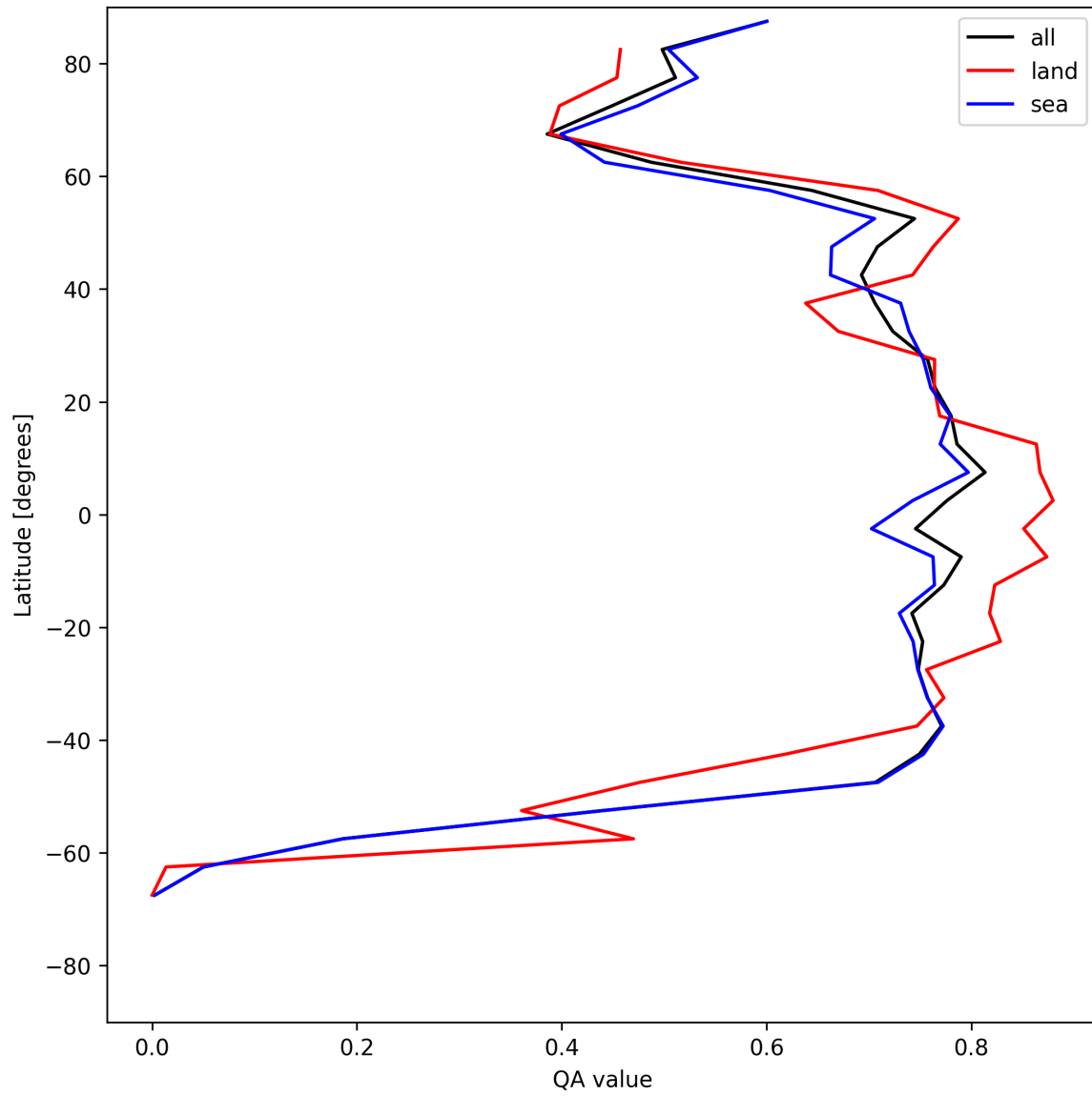
Figure 22: Zonal average of “QA value” for 2025-05-21 to 2025-05-23.
