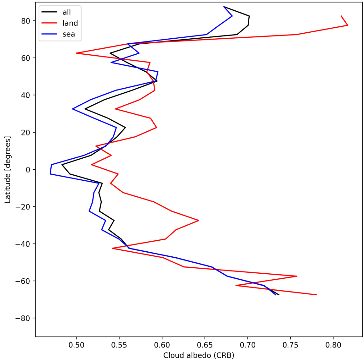
Figure 28: Zonal average of “Cloud albedo (CRB)” for 2025-05-21 to 2025-05-23.
