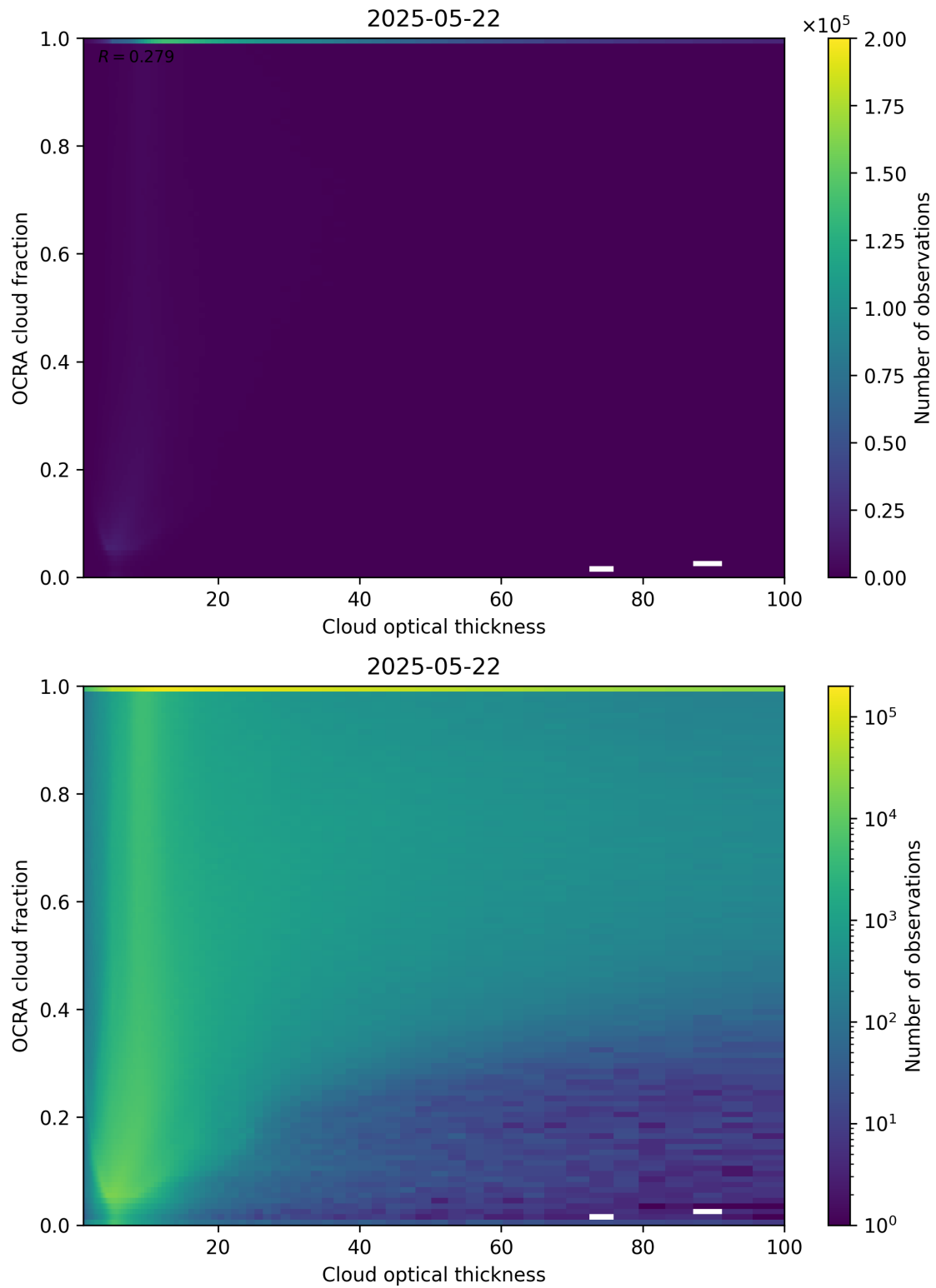
Figure 83: Scatter density plot of “Cloud optical thickness” against “OCRA cloud fraction” for 2025-05-21 to 2025-05-23.
