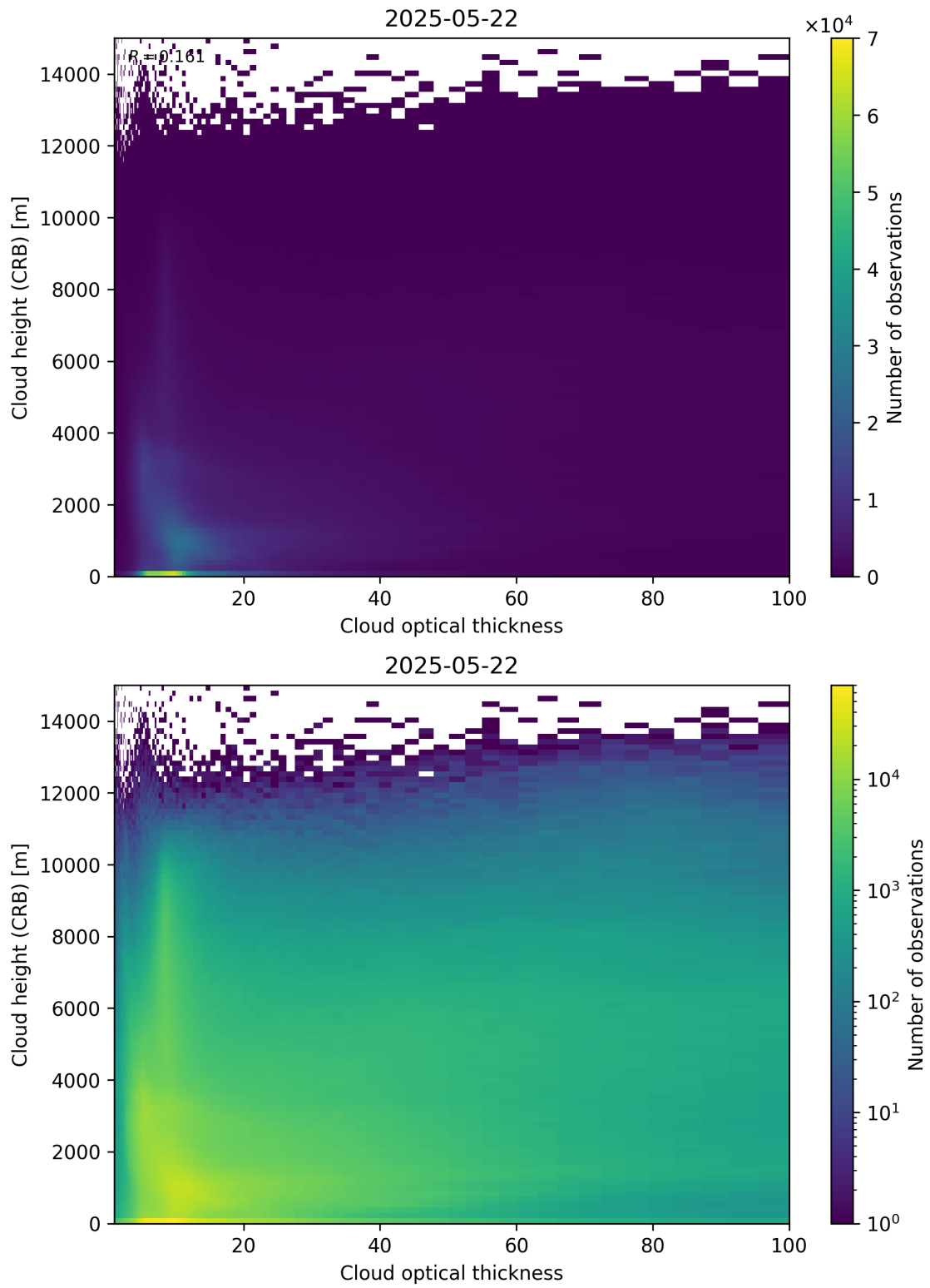
Figure 85: Scatter density plot of “Cloud optical thickness” against “Cloud height (CRB)” for 2025-05-21 to 2025-05-23.
