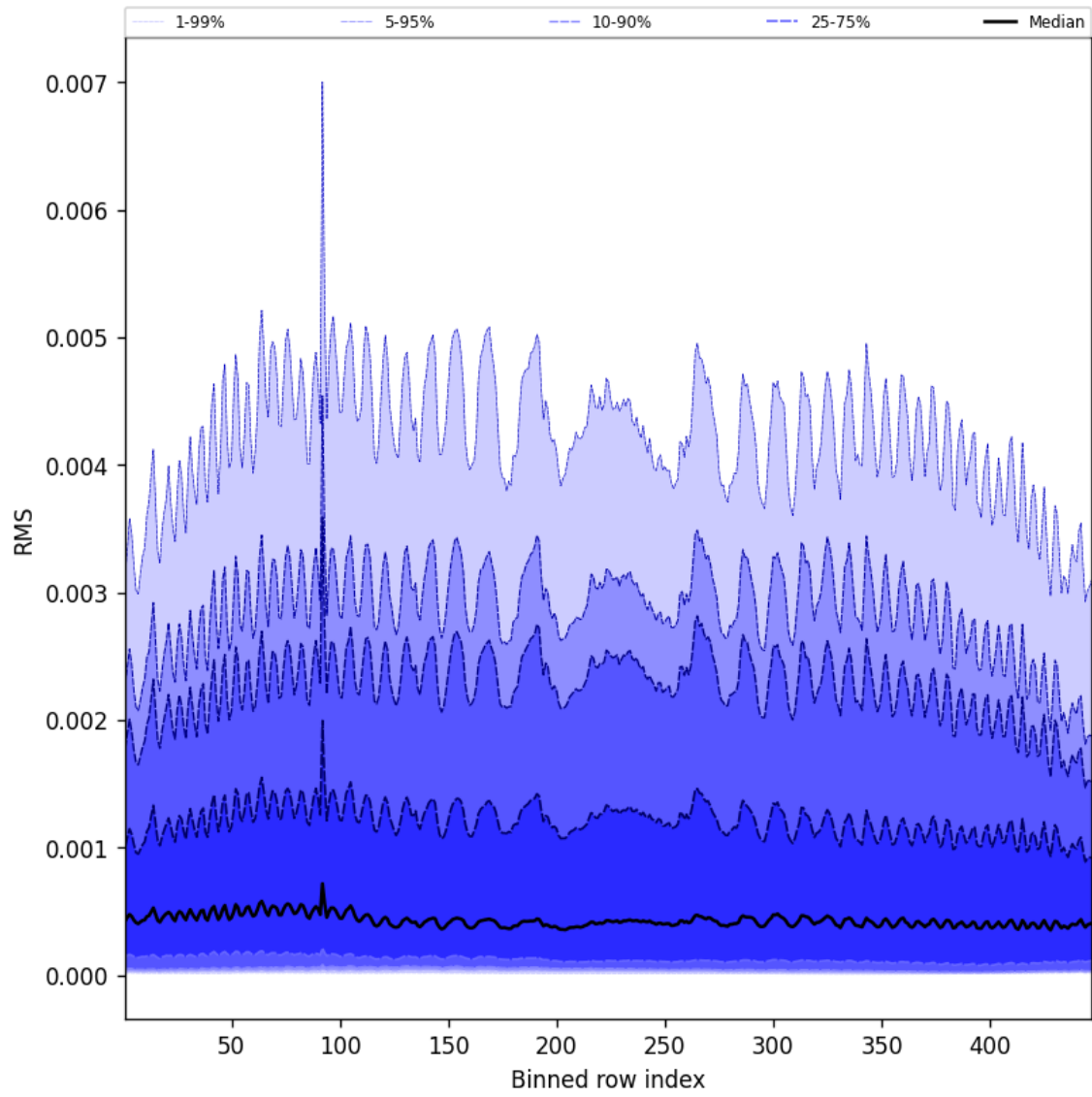
Figure 63: Along track statistics of “RMS” for 2025-05-21 to 2025-05-23
