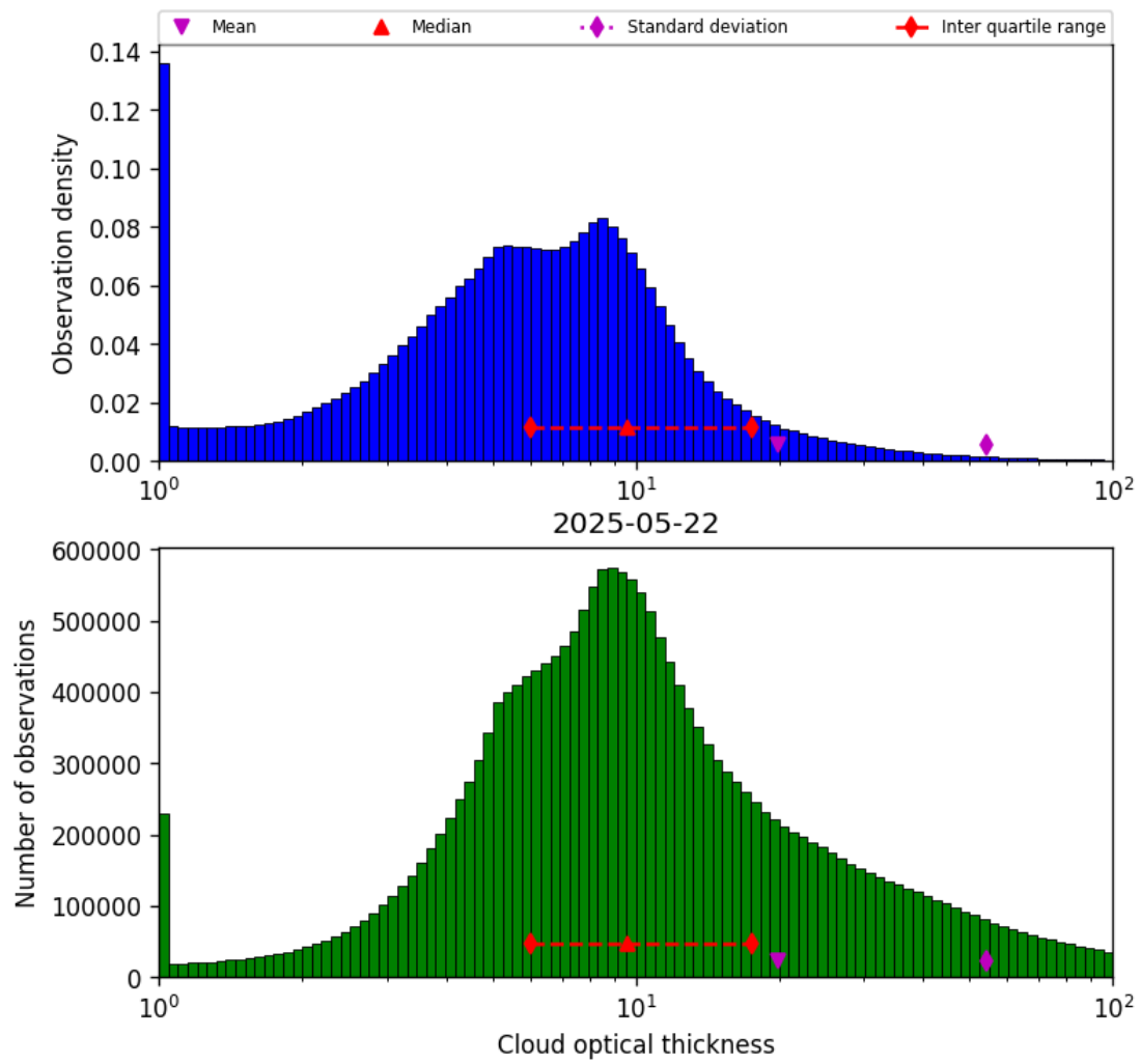
Figure 41: Histogram of “Cloud optical thickness” for 2025-05-21 to 2025-05-23
