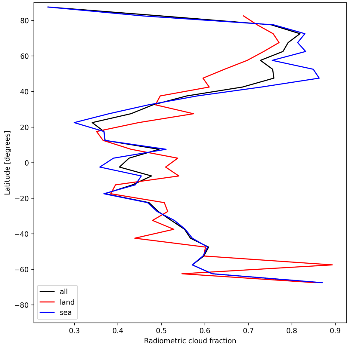
Figure 23: Zonal average of “Radiometric cloud fraction” for 2025-05-21 to 2025-05-23.
