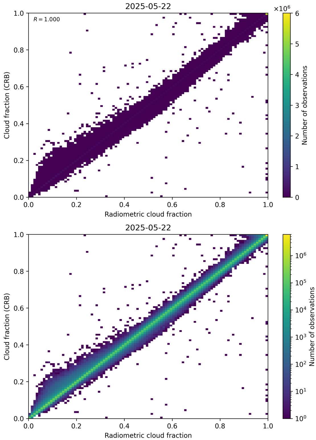
Figure 73: Scatter density plot of “Radiometric cloud fraction” against “Cloud fraction (CRB)” for 2025-05-21 to 2025-05-23.
