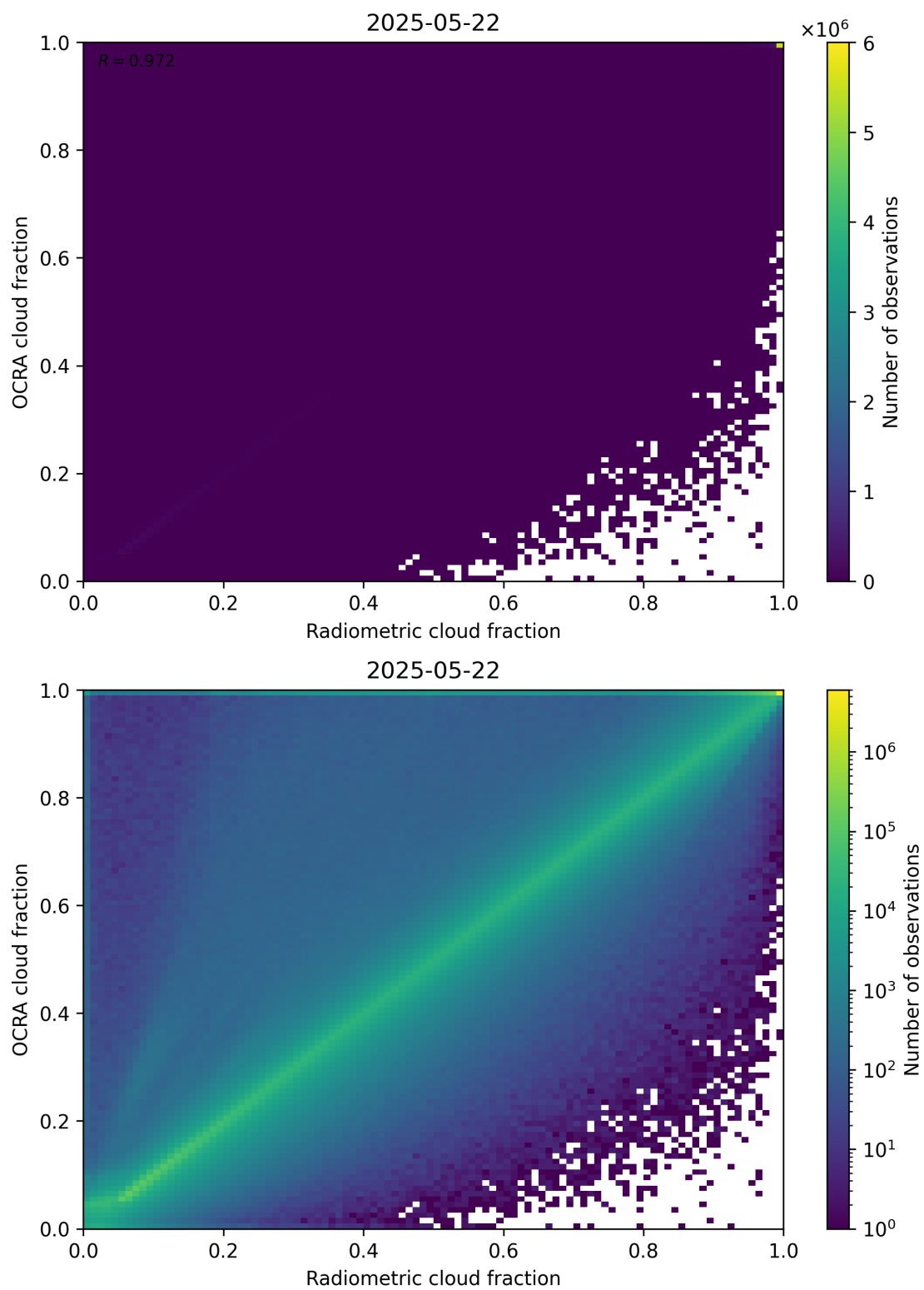
Figure 72: Scatter density plot of “Radiometric cloud fraction” against “OCRA cloud fraction” for 2025-05-21 to 2025-05-23.
