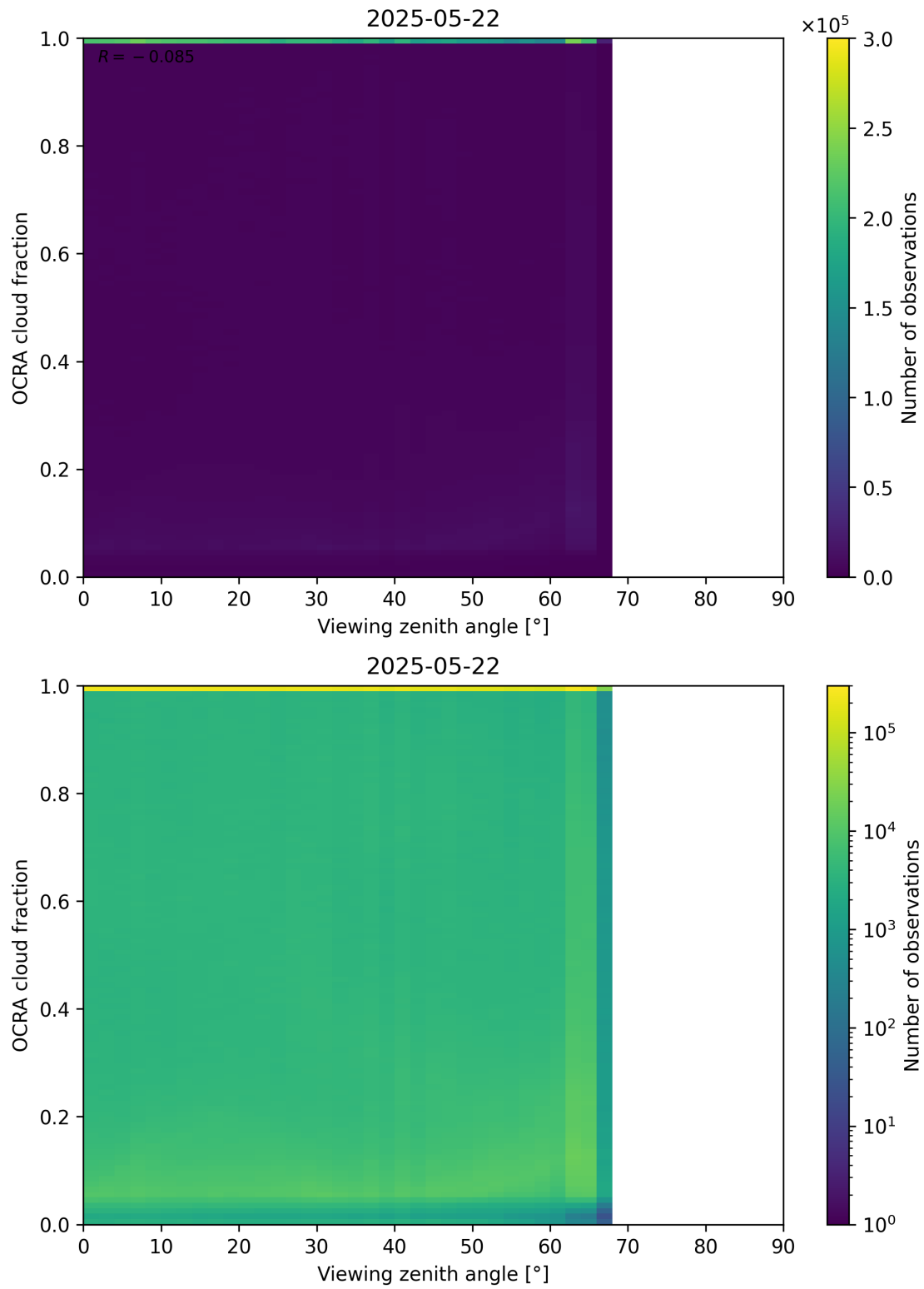
Figure 108: Scatter density plot of “Viewing zenith angle” against “OCRA cloud fraction” for 2025-05-21 to 2025-05-23.
