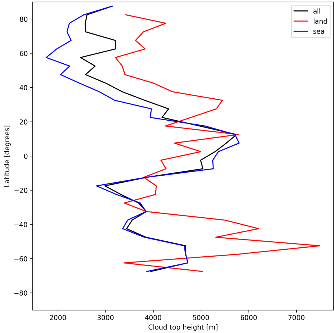
Figure 24: Zonal average of “Cloud top height” for 2025-05-21 to 2025-05-23.
