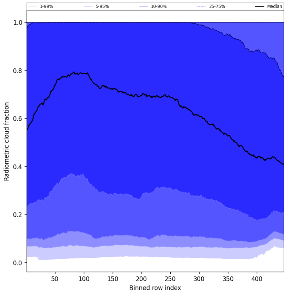
Figure 55: Along track statistics of “Radiometric cloud fraction” for 2025-05-21 to 2025-05-23
