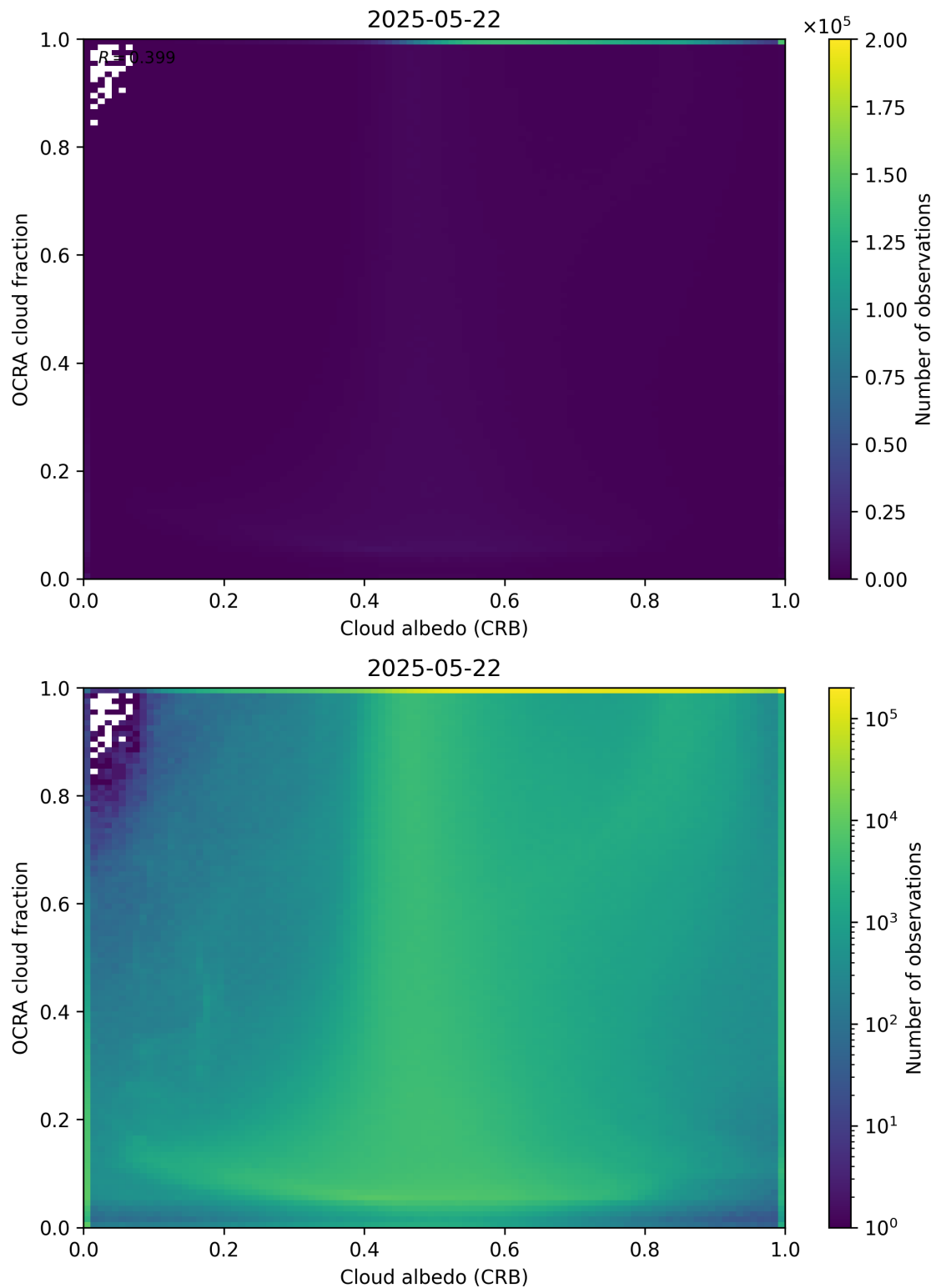
Figure 70: Scatter density plot of “Cloud albedo (CRB)” against “OCRA cloud fraction” for 2025-05-21 to 2025-05-23.
