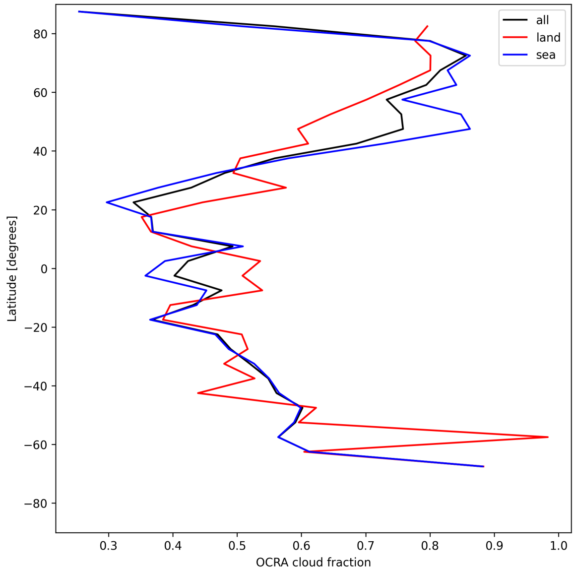
Figure 34: Zonal average of “OCRA cloud fraction” for 2025-05-21 to 2025-05-23.
