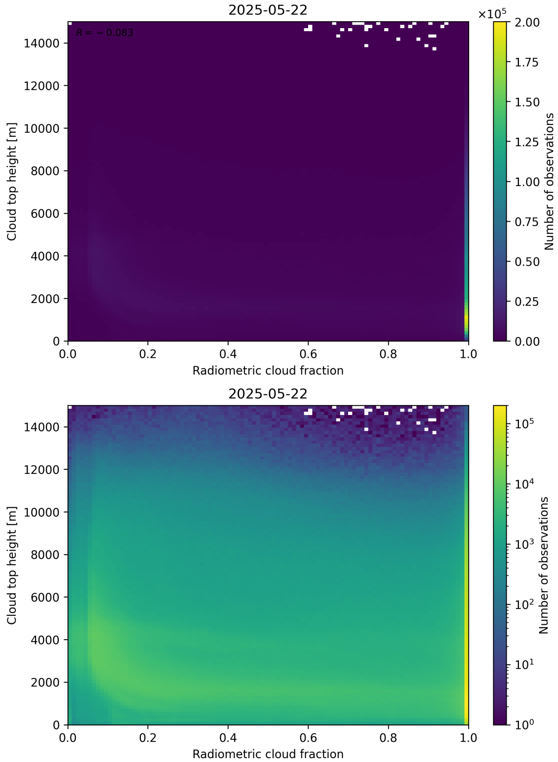
Figure 76: Scatter density plot of “Radiometric cloud fraction” against “Cloud top height” for 2025-05-21 to 2025-05-23.
