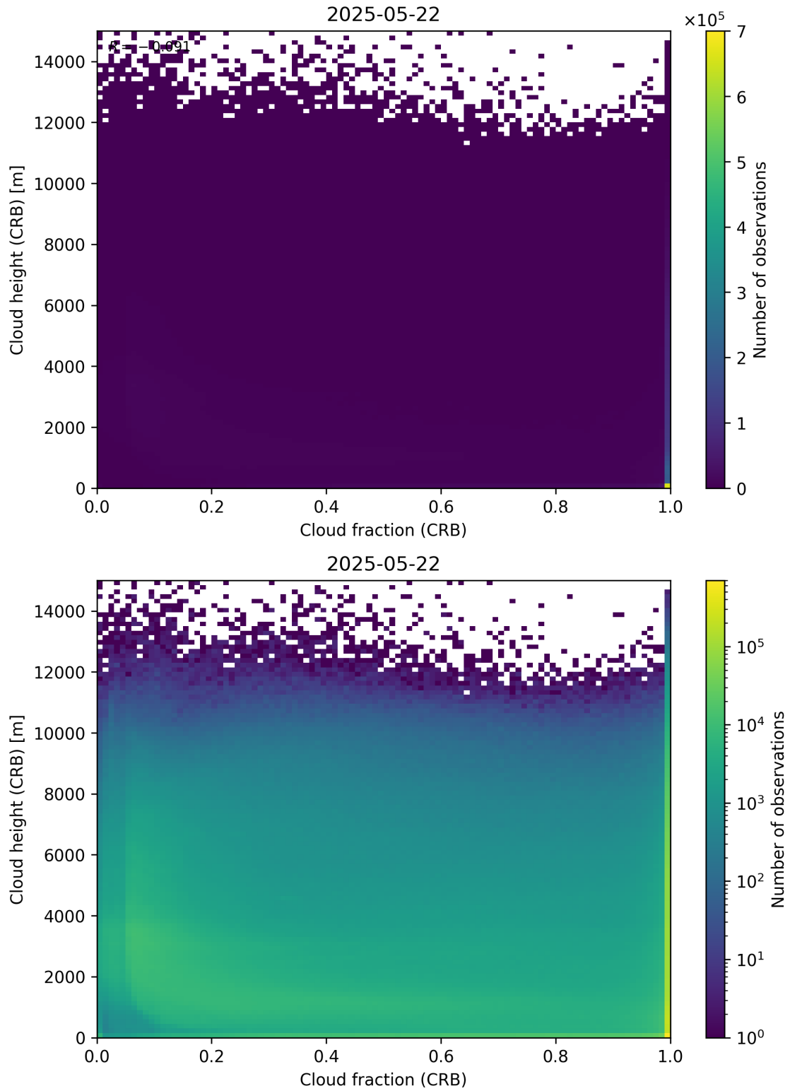
Figure 79: Scatter density plot of “Cloud fraction (CRB)” against “Cloud height (CRB)” for 2025-05-21 to 2025-05-23.
