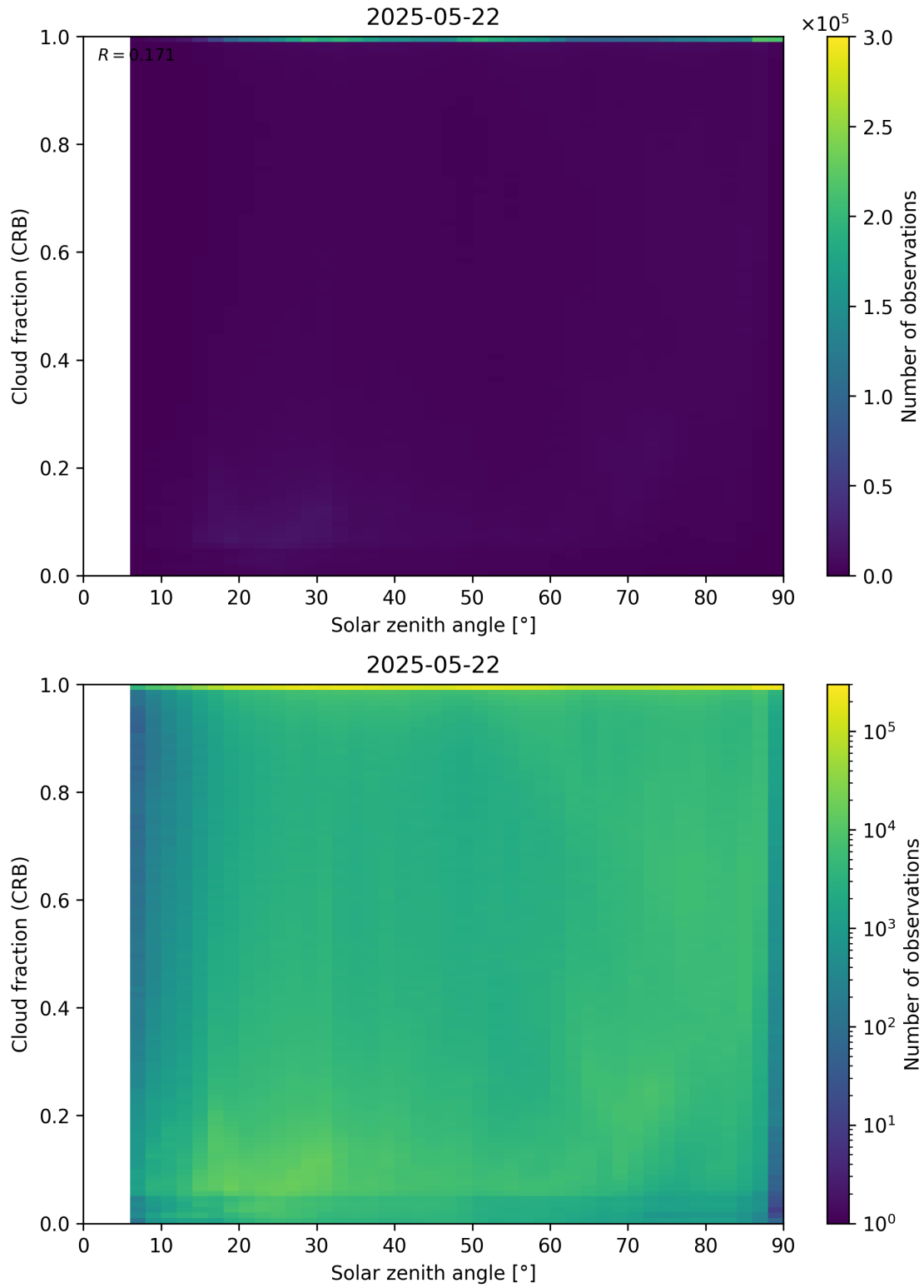
Figure 101: Scatter density plot of “Solar zenith angle” against “Cloud fraction (CRB)” for 2025-05-21 to 2025-05-23.
