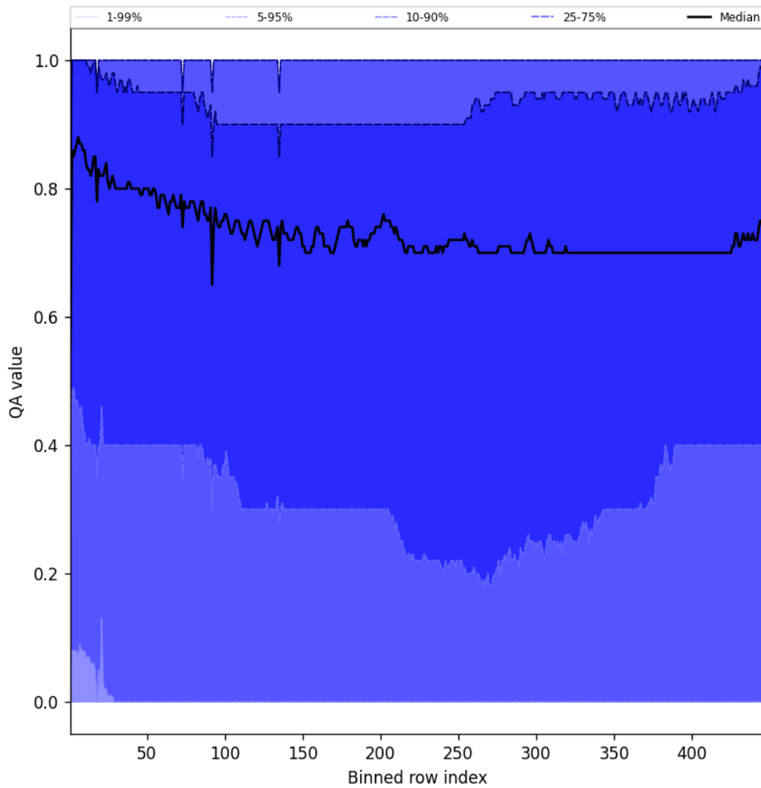
Figure 54: Along track statistics of “QA value” for 2025-05-21 to 2025-05-23
