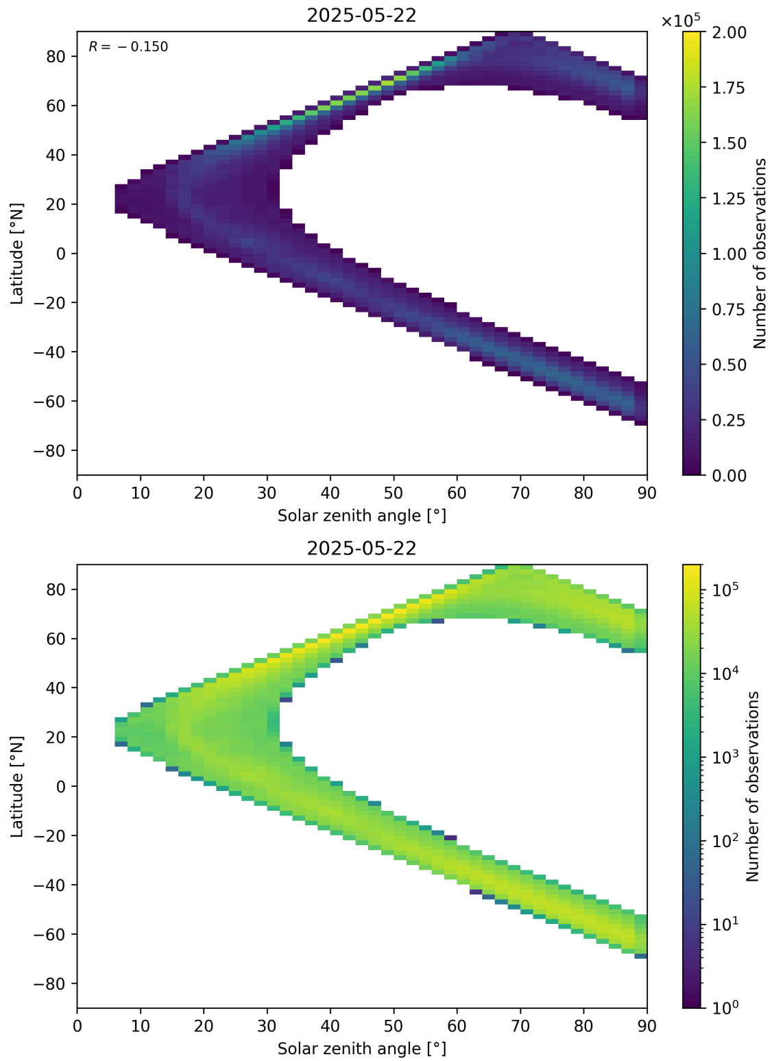
Figure 105: Scatter density plot of “Solar zenith angle” against “Latitude” for 2025-05-21 to 2025-05-23.
