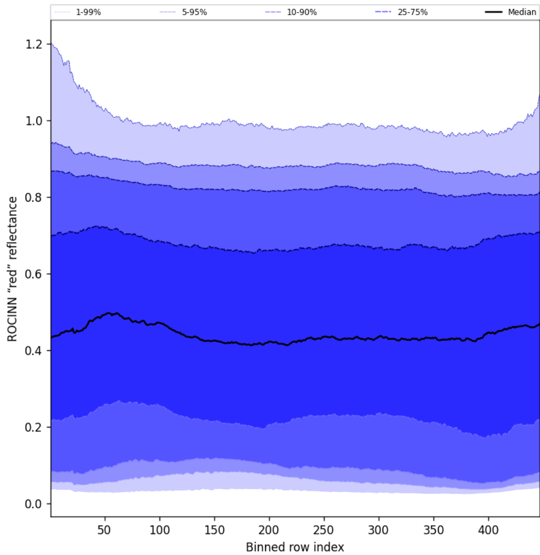
Figure 69: Along track statistics of “ROCINN “red” reflectance” for 2025-05-21 to 2025-05-23
