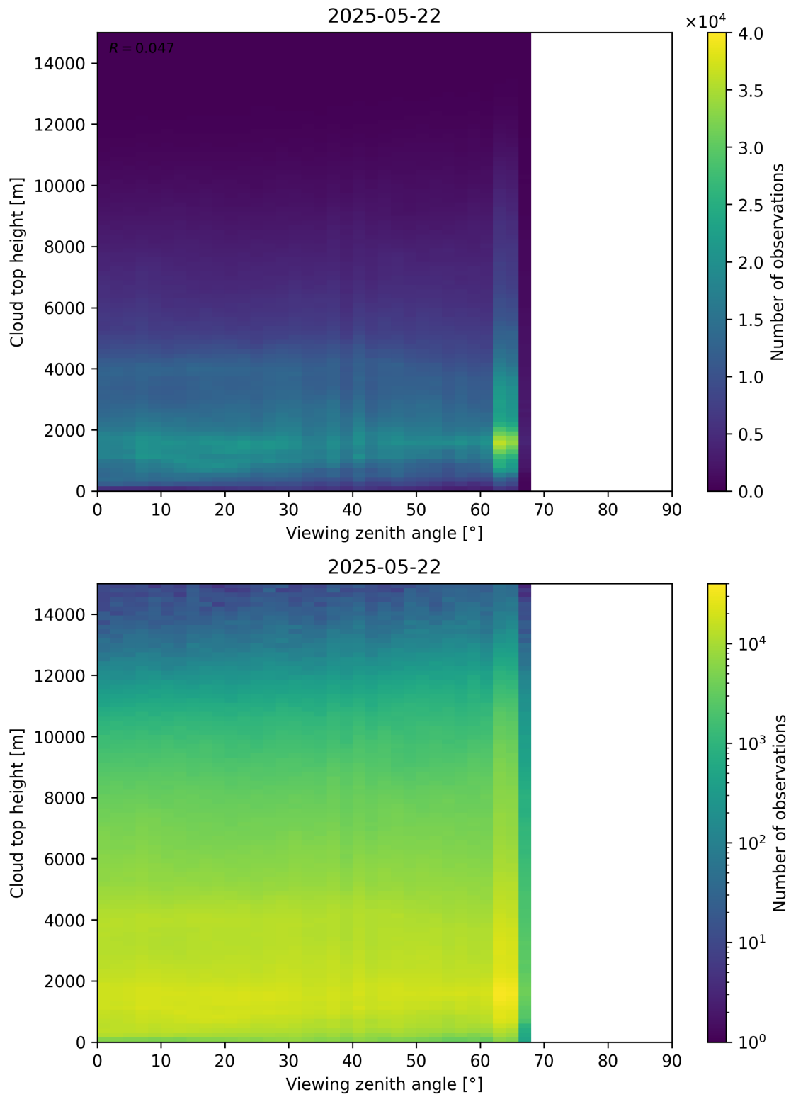
Figure 112: Scatter density plot of “Viewing zenith angle” against “Cloud top height” for 2025-05-21 to 2025-05-23.
