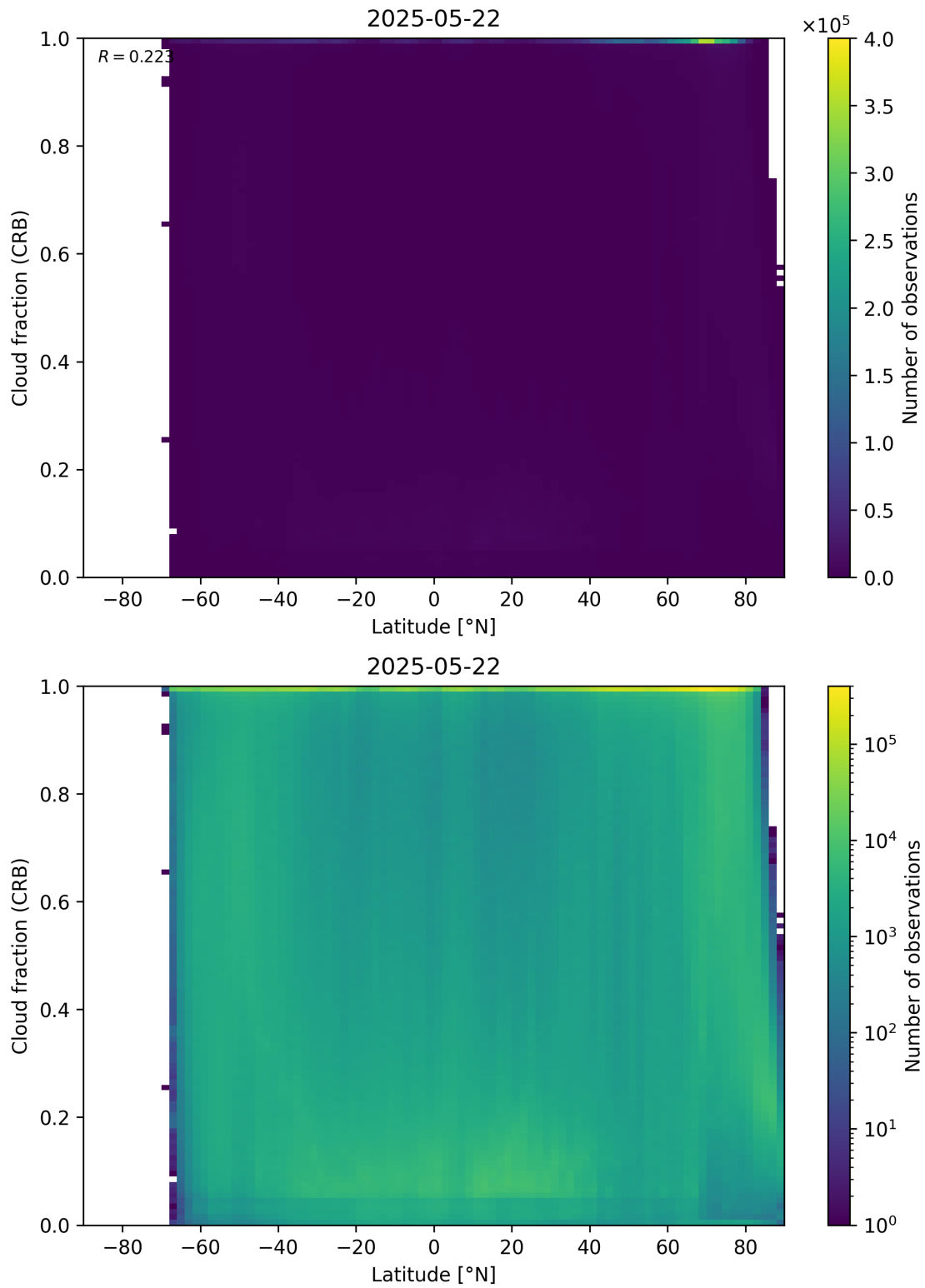
Figure 94: Scatter density plot of “Latitude” against “Cloud fraction (CRB)” for 2025-05-21 to 2025-05-23.
