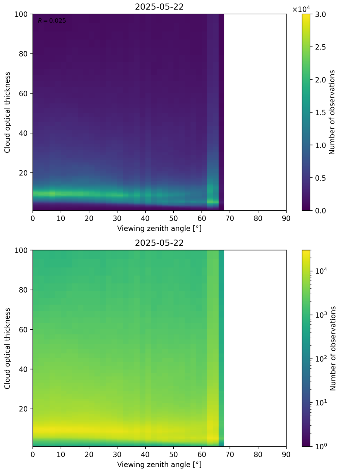
Figure 111: Scatter density plot of “Viewing zenith angle” against “Cloud optical thickness” for 2025-05-21 to 2025-05-23.
