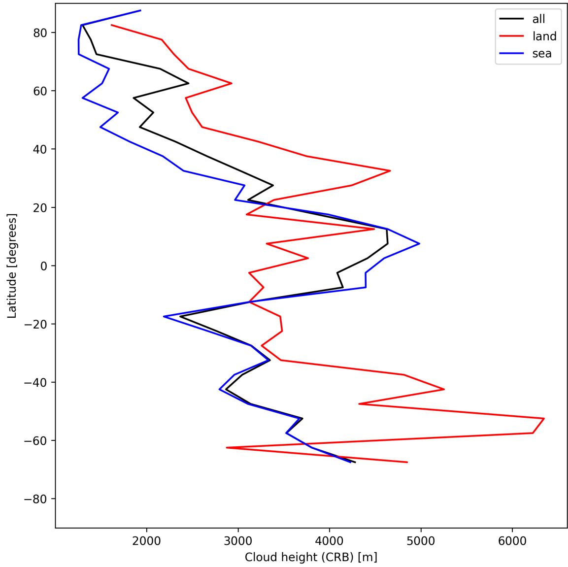
Figure 27: Zonal average of “Cloud height (CRB)” for 2025-05-21 to 2025-05-23.
