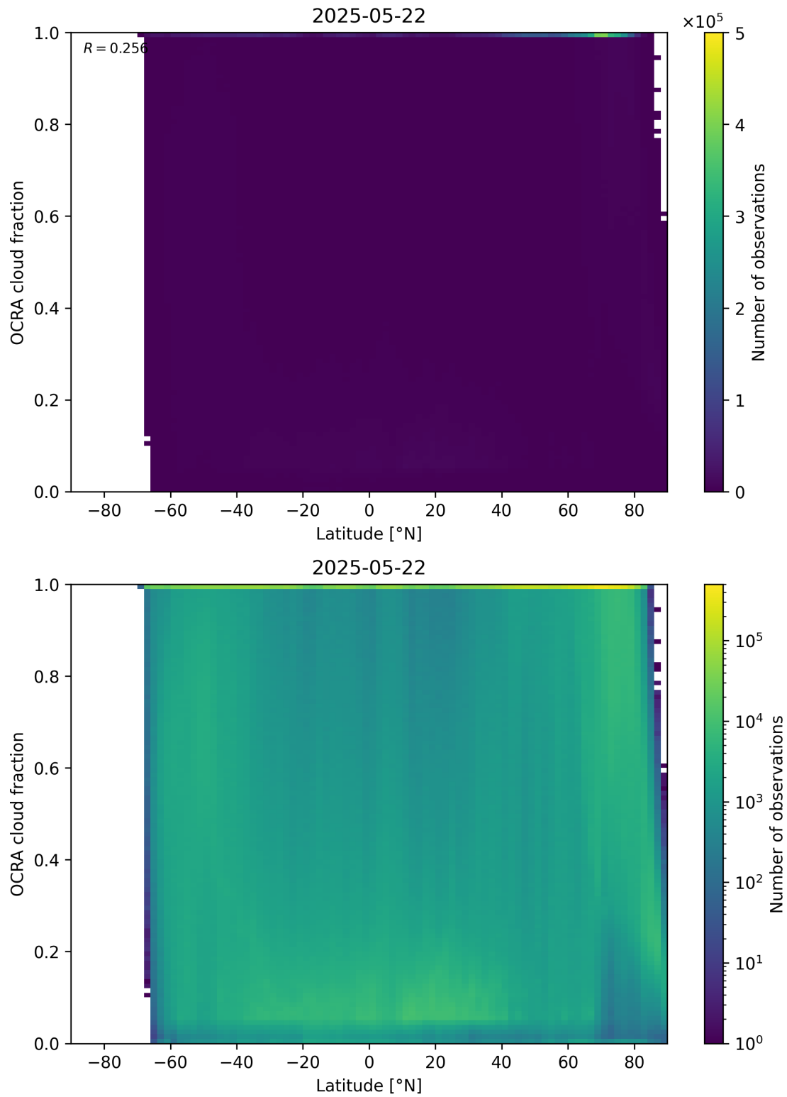
Figure 93: Scatter density plot of “Latitude” against “OCRA cloud fraction” for 2025-05-21 to 2025-05-23.
