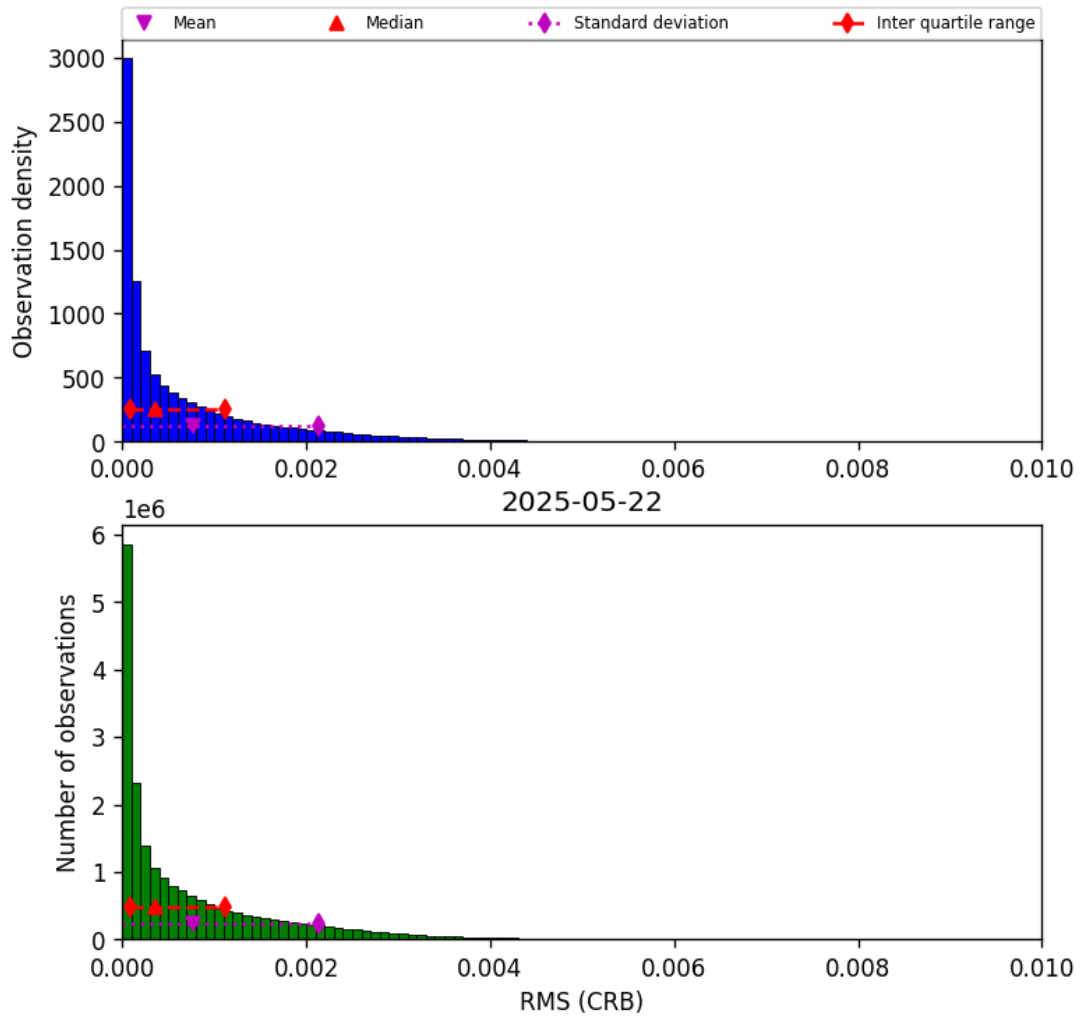
Figure 48: Histogram of “RMS (CRB)” for 2025-05-21 to 2025-05-23
