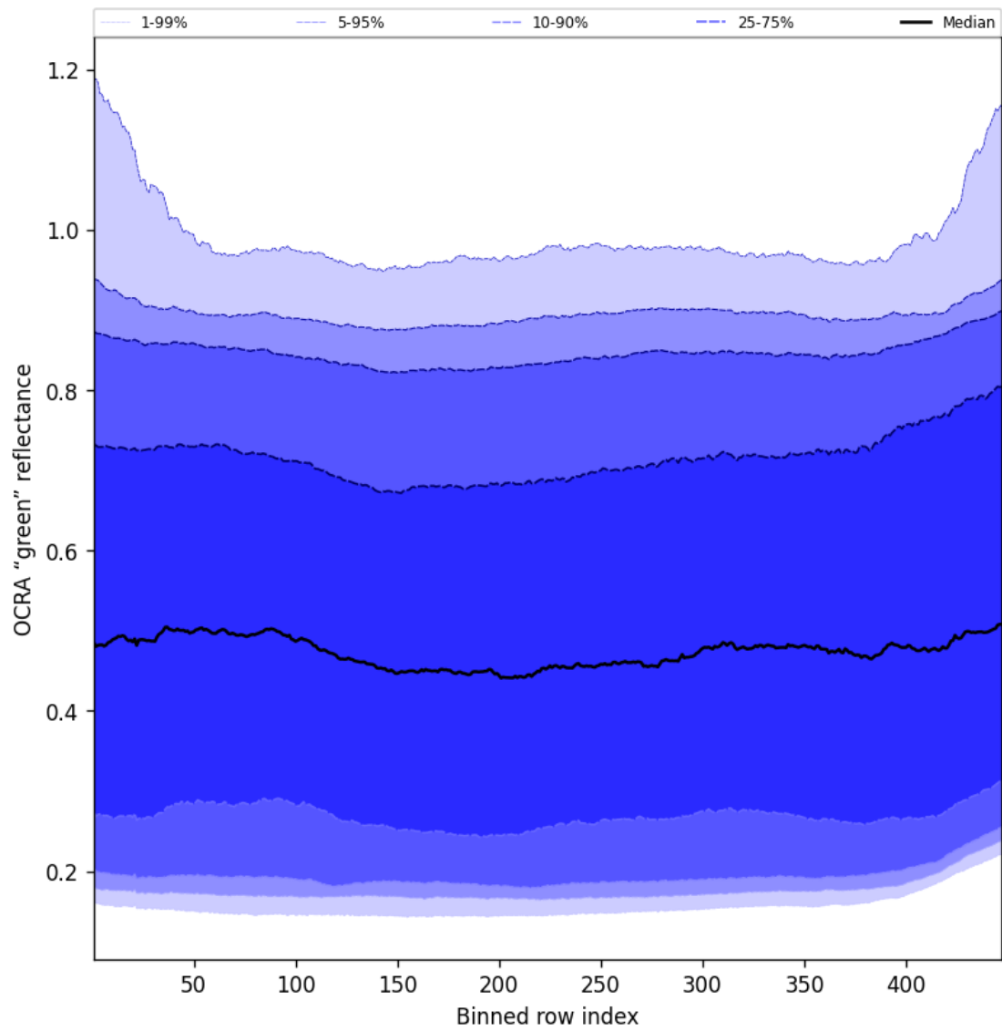
Figure 68: Along track statistics of “OCRA “green” reflectance” for 2025-05-22 to 2025-05-24
