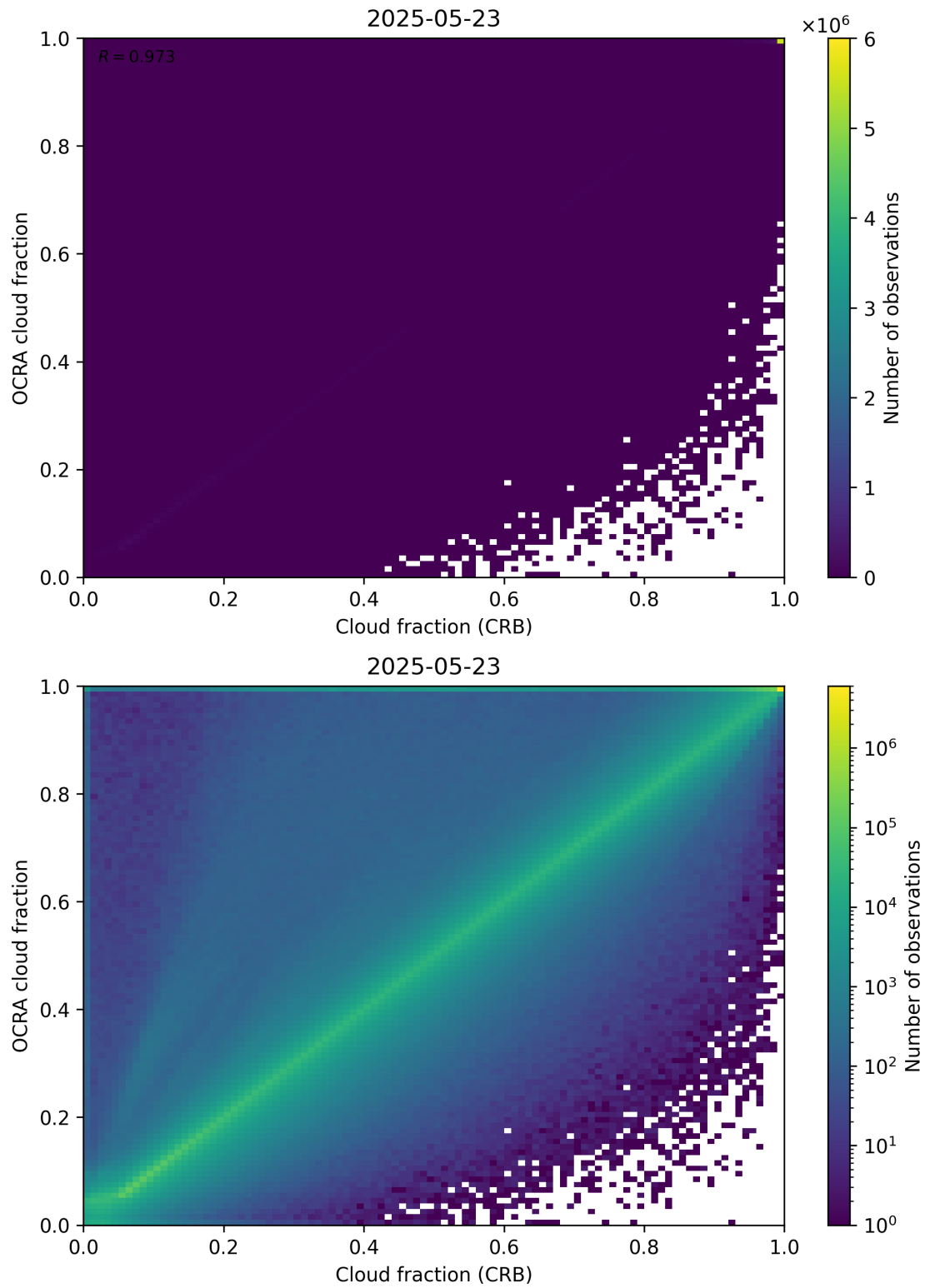
Figure 78: Scatter density plot of “Cloud fraction (CRB)” against “OCRA cloud fraction” for 2025-05-22 to 2025-05-24.
