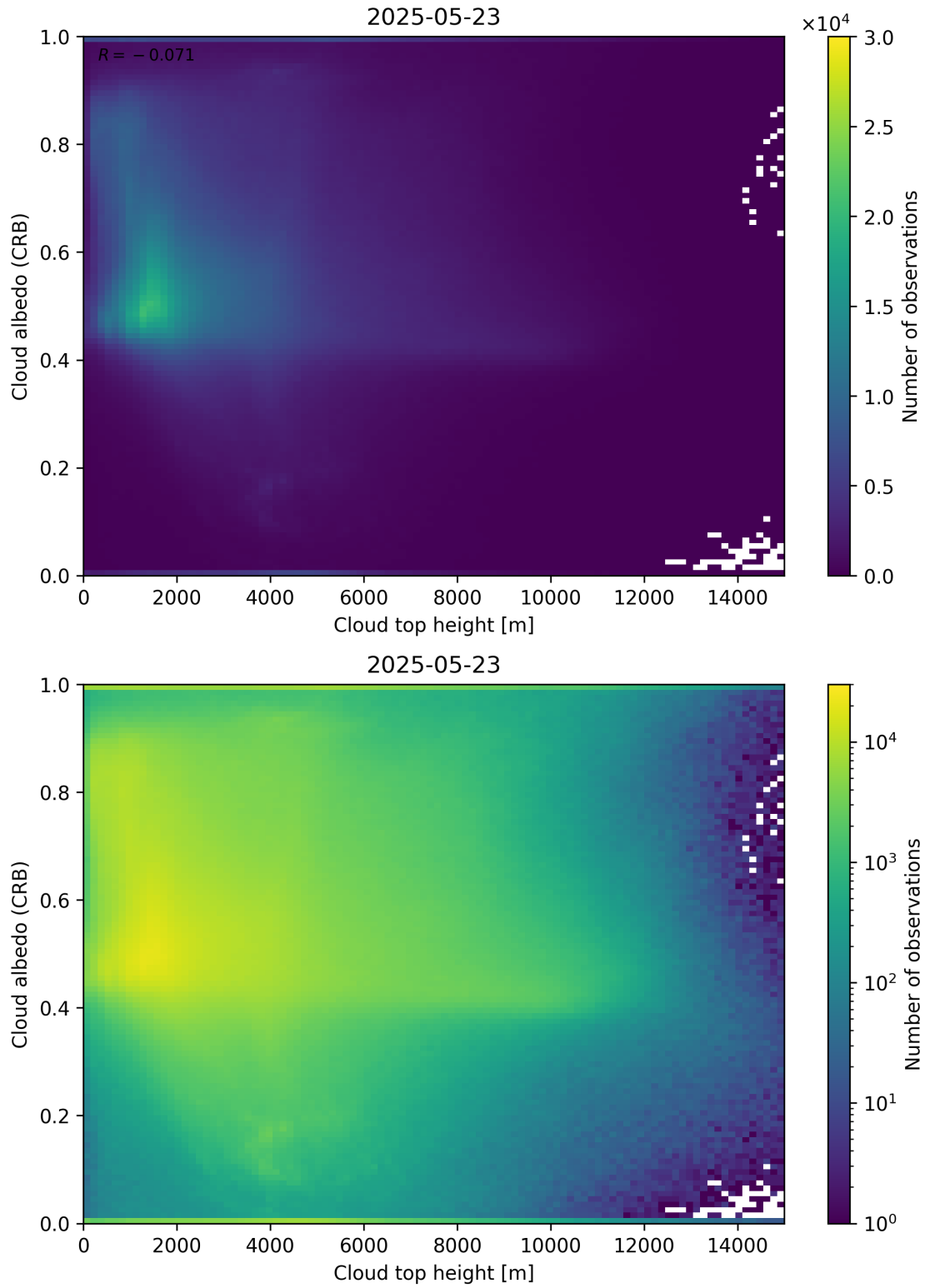
Figure 86: Scatter density plot of “Cloud top height” against “Cloud albedo (CRB)” for 2025-05-22 to 2025-05-24.
