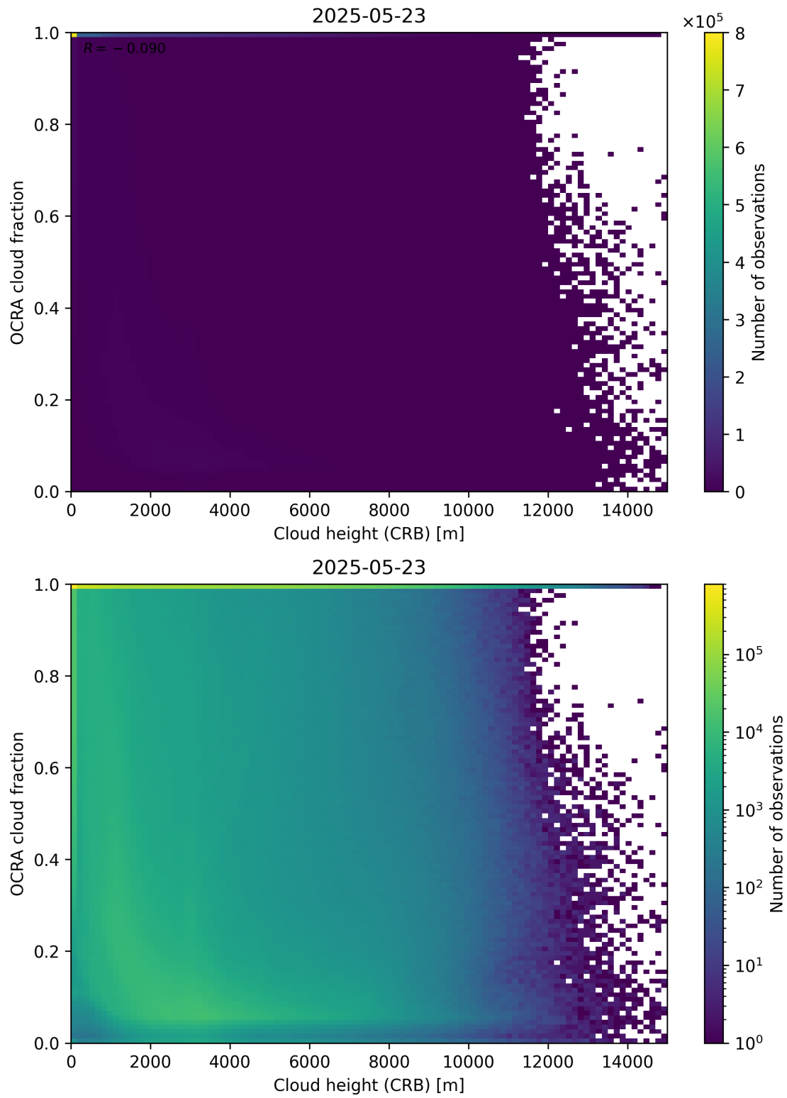
Figure 81: Scatter density plot of “Cloud height (CRB)” against “OCRA cloud fraction” for 2025-05-22 to 2025-05-24.
