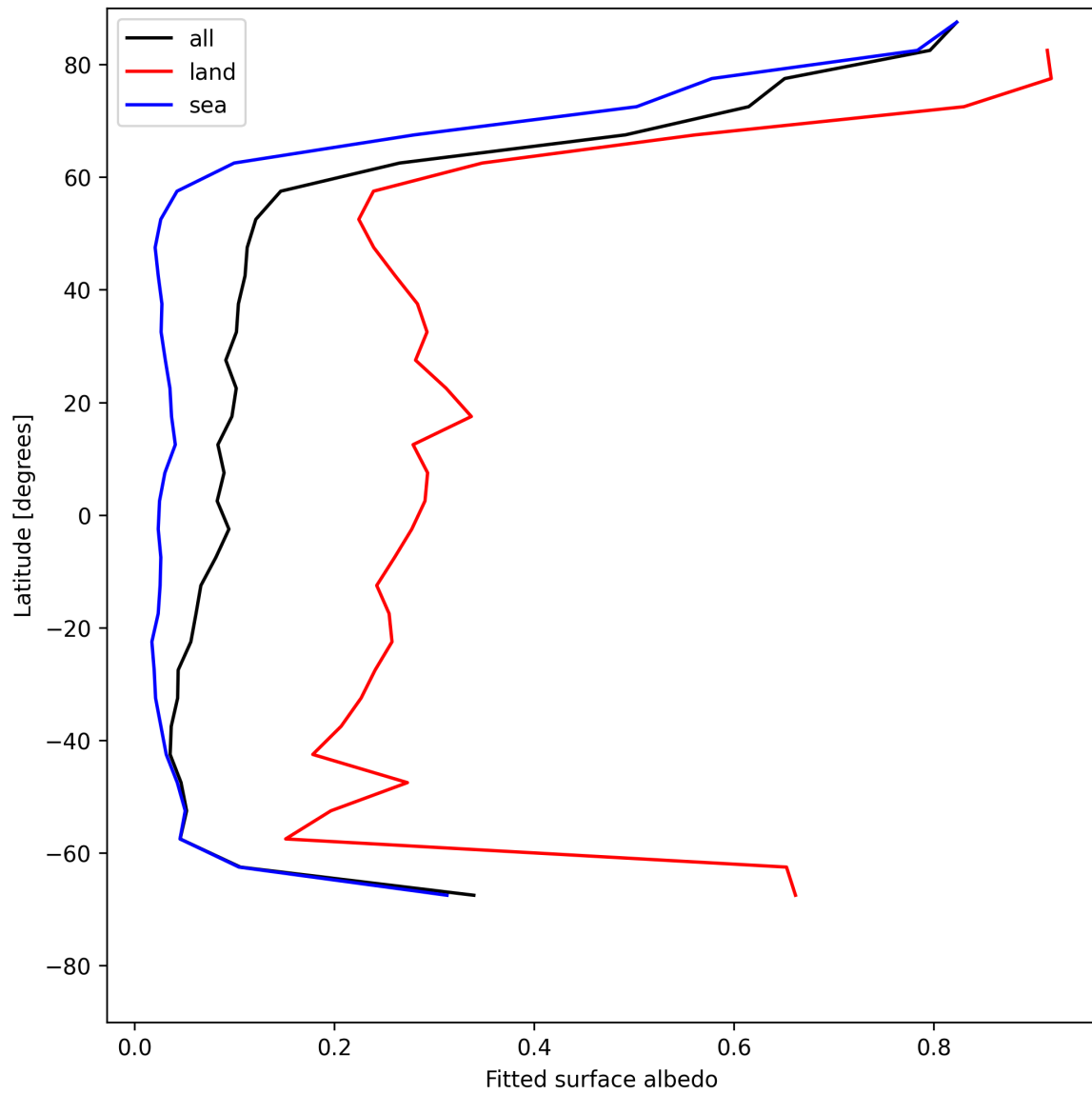
Figure 29: Zonal average of “Fitted surface albedo” for 2025-05-22 to 2025-05-24.
