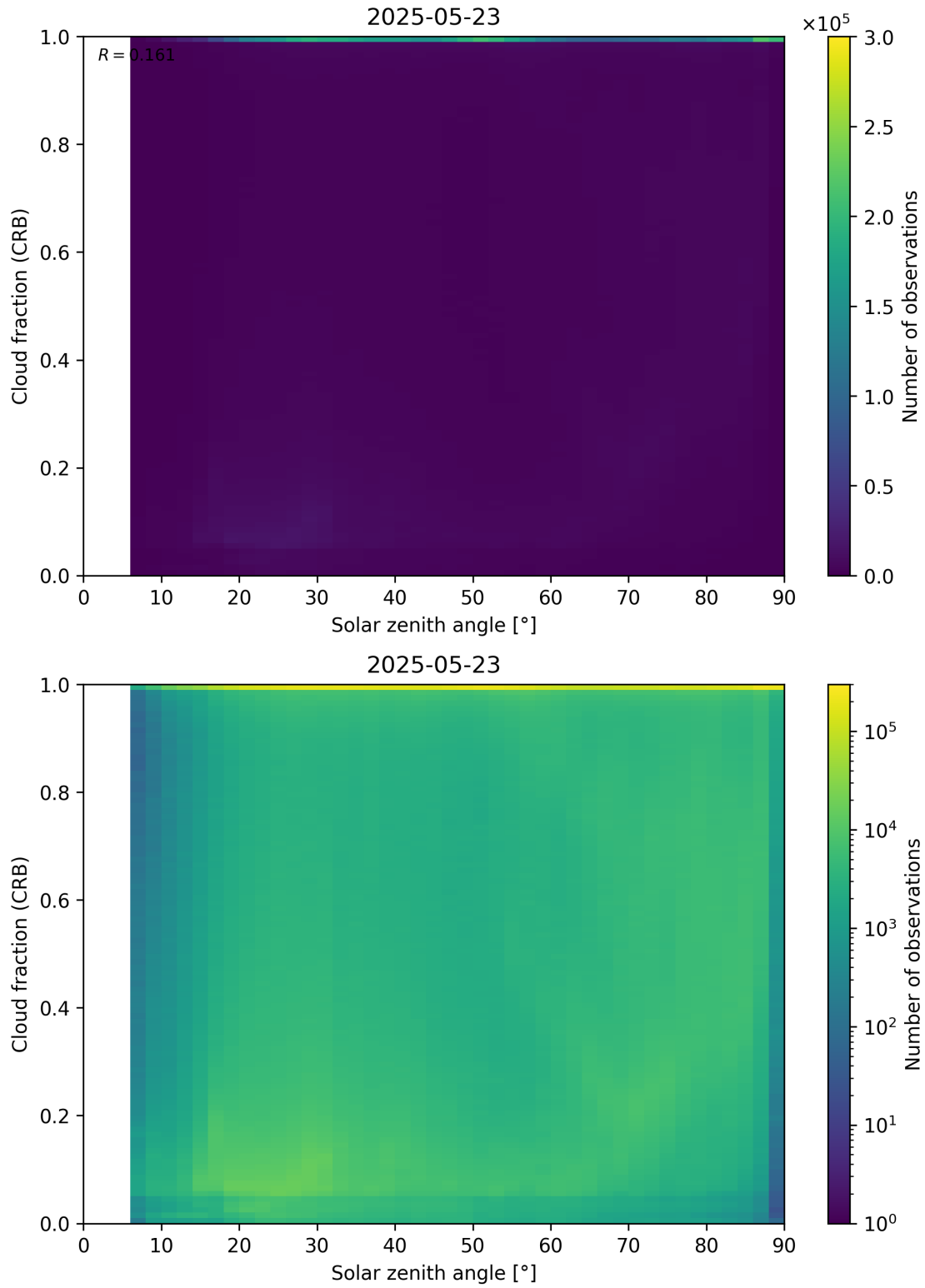
Figure 101: Scatter density plot of “Solar zenith angle” against “Cloud fraction (CRB)” for 2025-05-22 to 2025-05-24.
