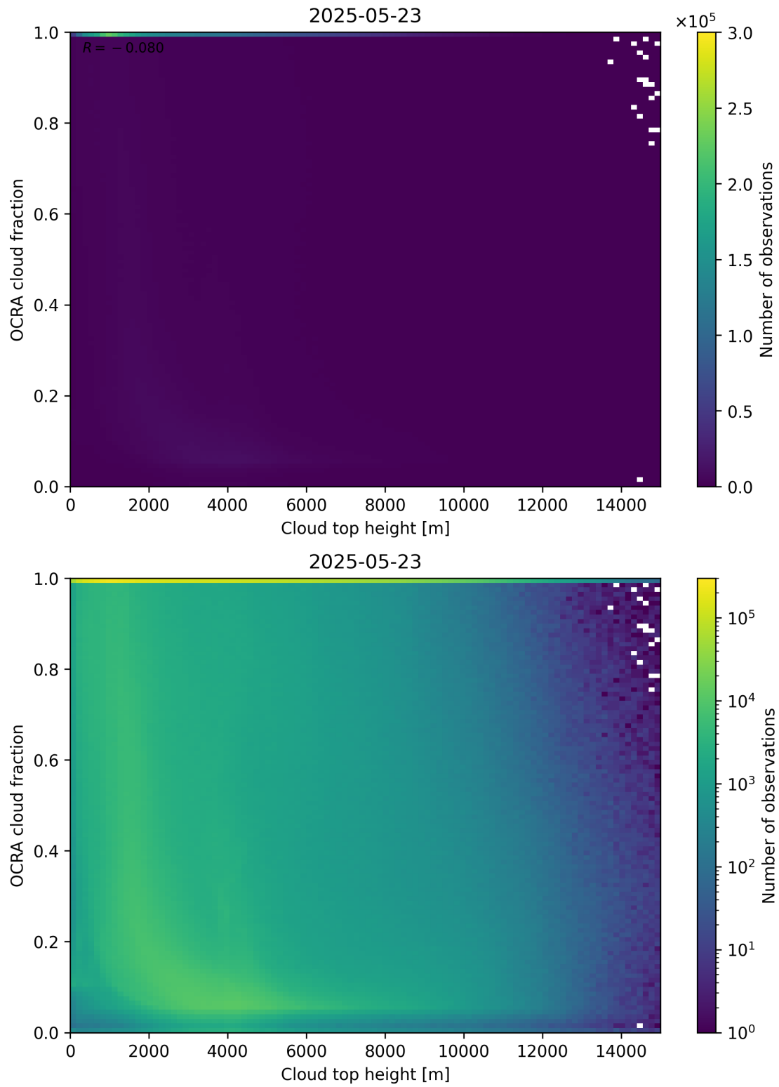
Figure 87: Scatter density plot of “Cloud top height” against “OCRA cloud fraction” for 2025-05-22 to 2025-05-24.
