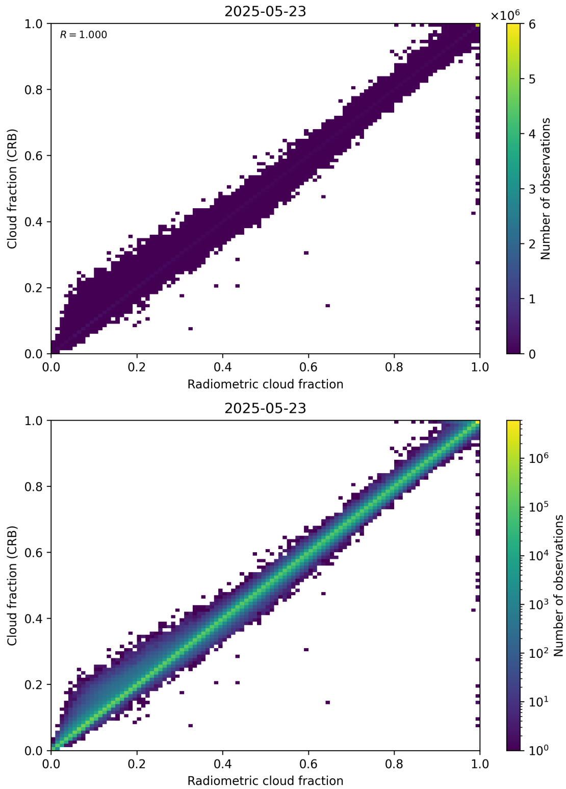
Figure 73: Scatter density plot of “Radiometric cloud fraction” against “Cloud fraction (CRB)” for 2025-05-22 to 2025-05-24.
