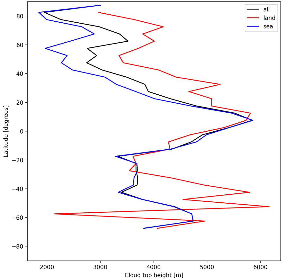
Figure 24: Zonal average of “Cloud top height” for 2025-05-22 to 2025-05-24.
