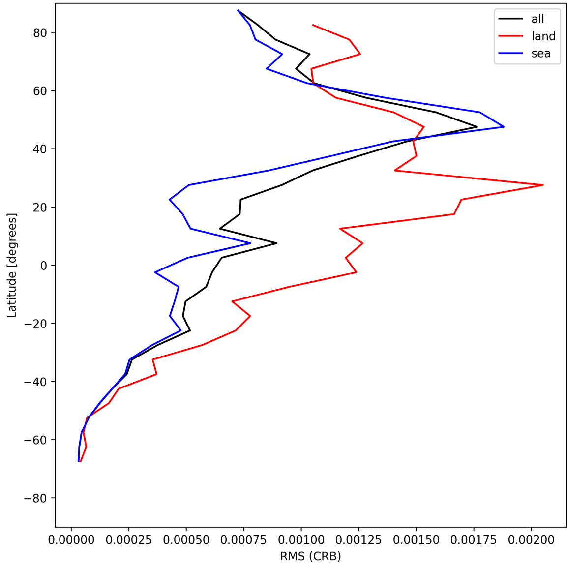
Figure 32: Zonal average of “RMS (CRB)” for 2025-05-22 to 2025-05-24.
