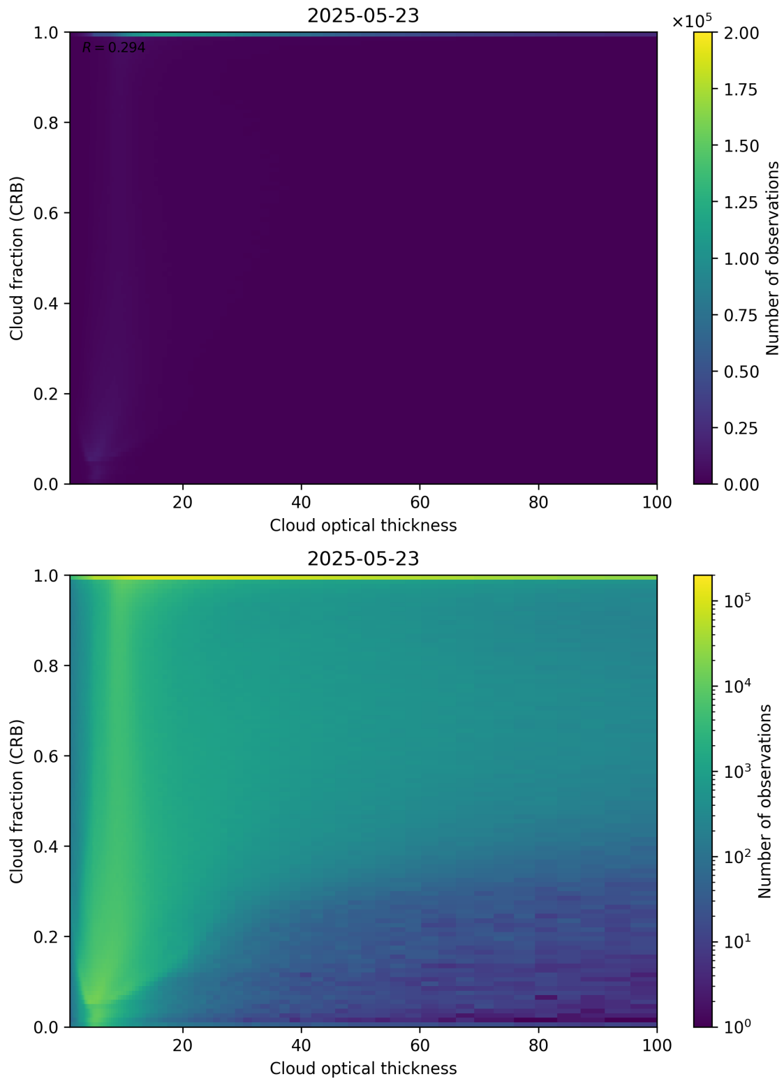
Figure 84: Scatter density plot of “Cloud optical thickness” against “Cloud fraction (CRB)” for 2025-05-22 to 2025-05-24.
