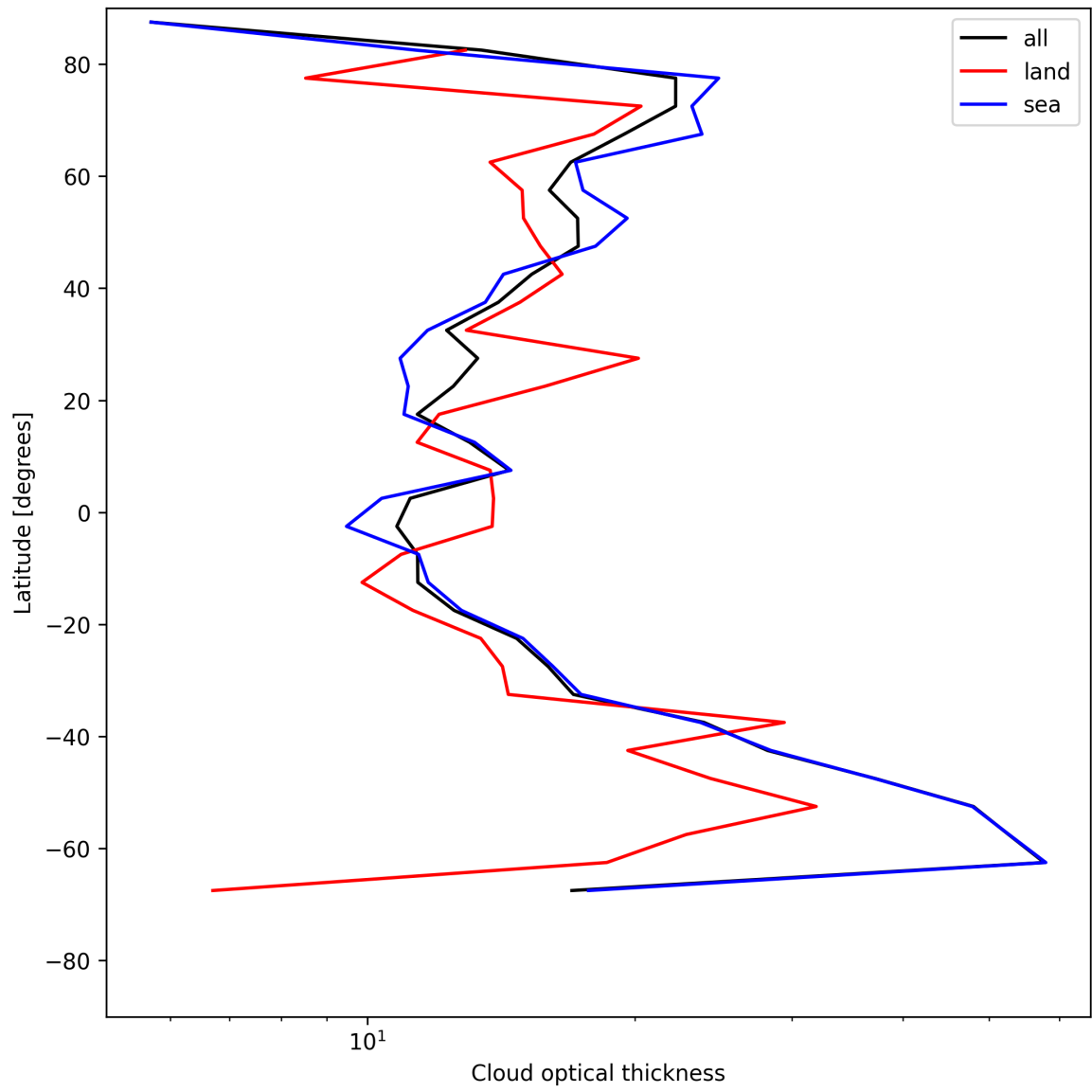
Figure 25: Zonal average of “Cloud optical thickness” for 2025-05-22 to 2025-05-24.
