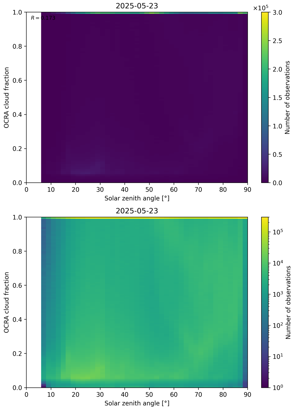
Figure 100: Scatter density plot of “Solar zenith angle” against “OCRA cloud fraction” for 2025-05-22 to 2025-05-24.
