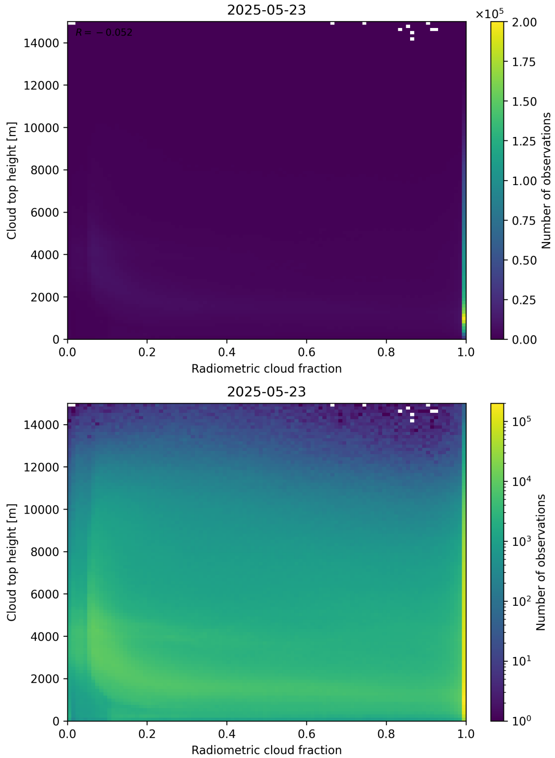
Figure 76: Scatter density plot of “Radiometric cloud fraction” against “Cloud top height” for 2025-05-22 to 2025-05-24.
