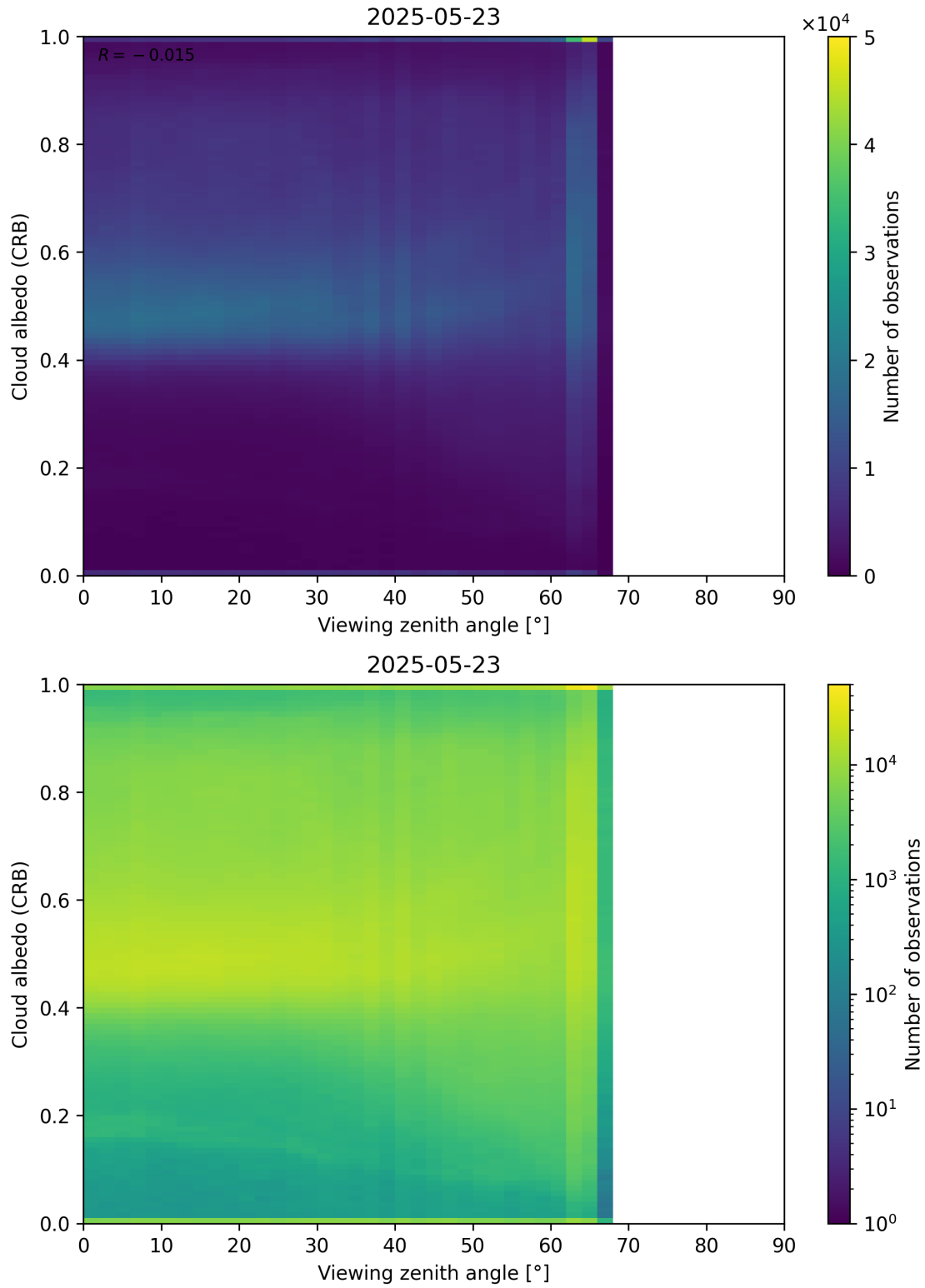
Figure 106: Scatter density plot of “Viewing zenith angle” against “Cloud albedo (CRB)” for 2025-05-22 to 2025-05-24.
