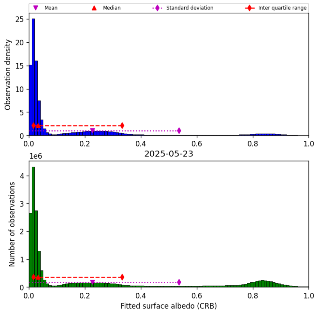
Figure 46: Histogram of “Fitted surface albedo (CRB)” for 2025-05-22 to 2025-05-24
