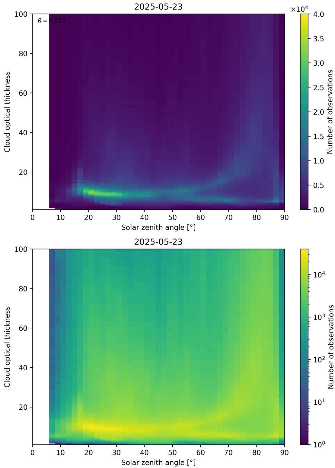
Figure 103: Scatter density plot of “Solar zenith angle” against “Cloud optical thickness” for 2025-05-22 to 2025-05-24.
