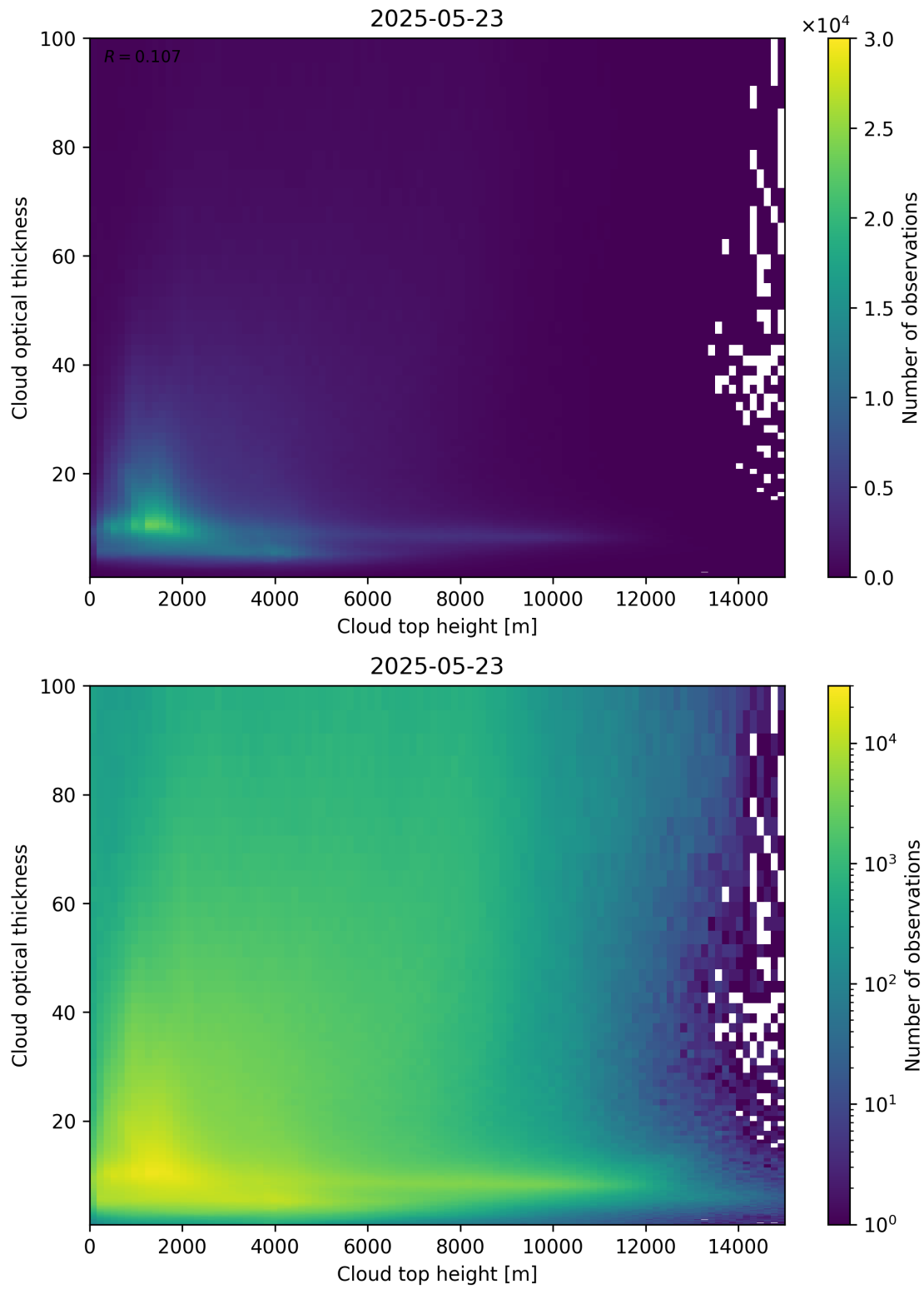
Figure 90: Scatter density plot of “Cloud top height” against “Cloud optical thickness” for 2025-05-22 to 2025-05-24.
