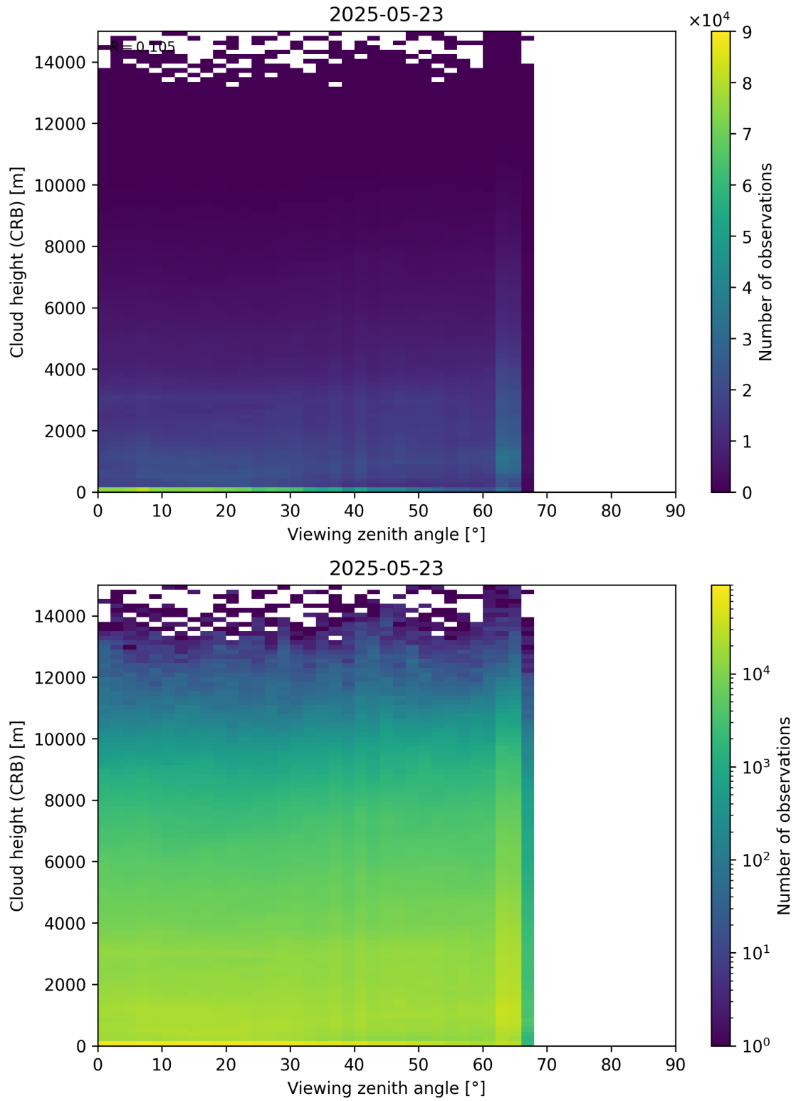
Figure 110: Scatter density plot of “Viewing zenith angle” against “Cloud height (CRB)” for 2025-05-22 to 2025-05-24.
