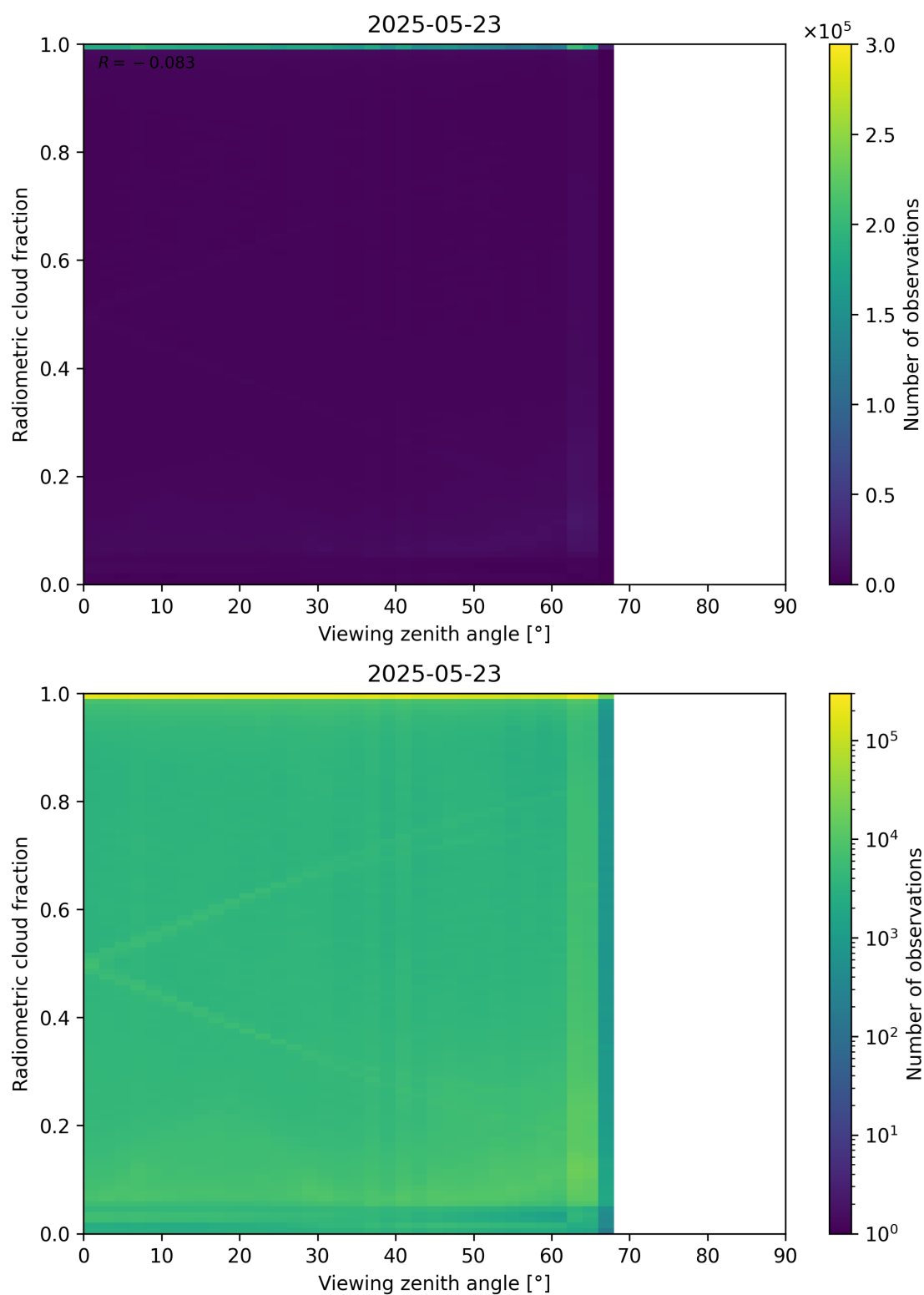
Figure 107: Scatter density plot of “Viewing zenith angle” against “Radiometric cloud fraction” for 2025-05-22 to 2025-05-24.
