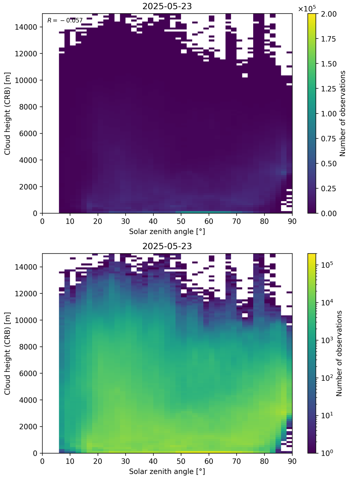
Figure 102: Scatter density plot of “Solar zenith angle” against “Cloud height (CRB)” for 2025-05-22 to 2025-05-24.
