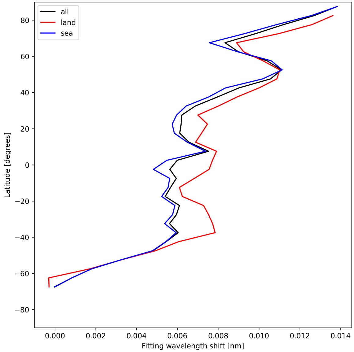
Figure 33: Zonal average of “Fitting wavelength shift” for 2025-05-22 to 2025-05-24.
