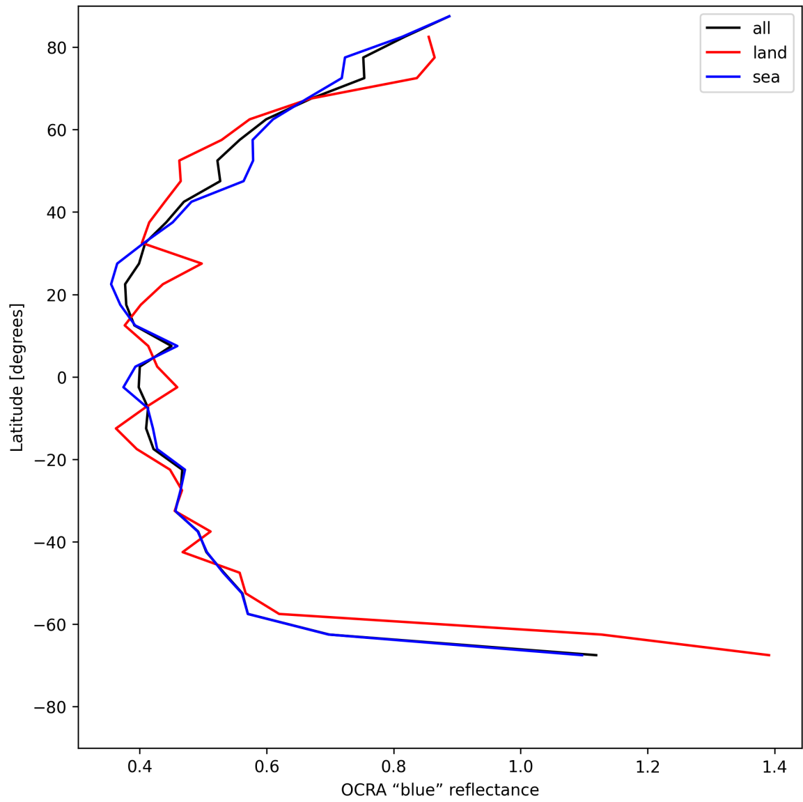
Figure 35: Zonal average of “OCRA “blue” reflectance” for 2025-05-22 to 2025-05-24.
