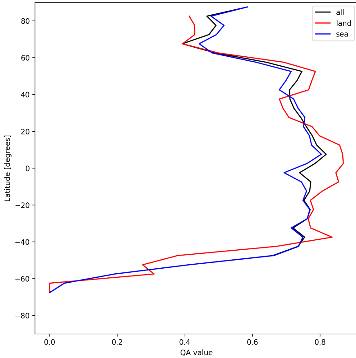
Figure 22: Zonal average of “QA value” for 2025-05-22 to 2025-05-24.
