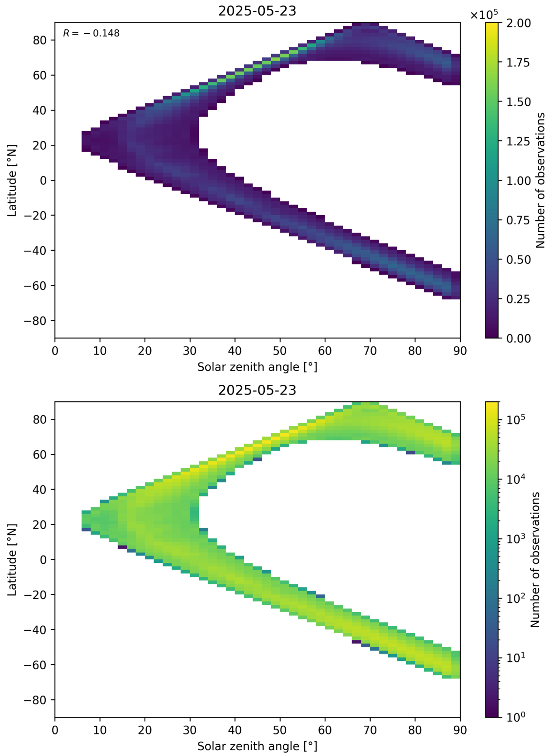
Figure 105: Scatter density plot of “Solar zenith angle” against “Latitude” for 2025-05-22 to 2025-05-24.
