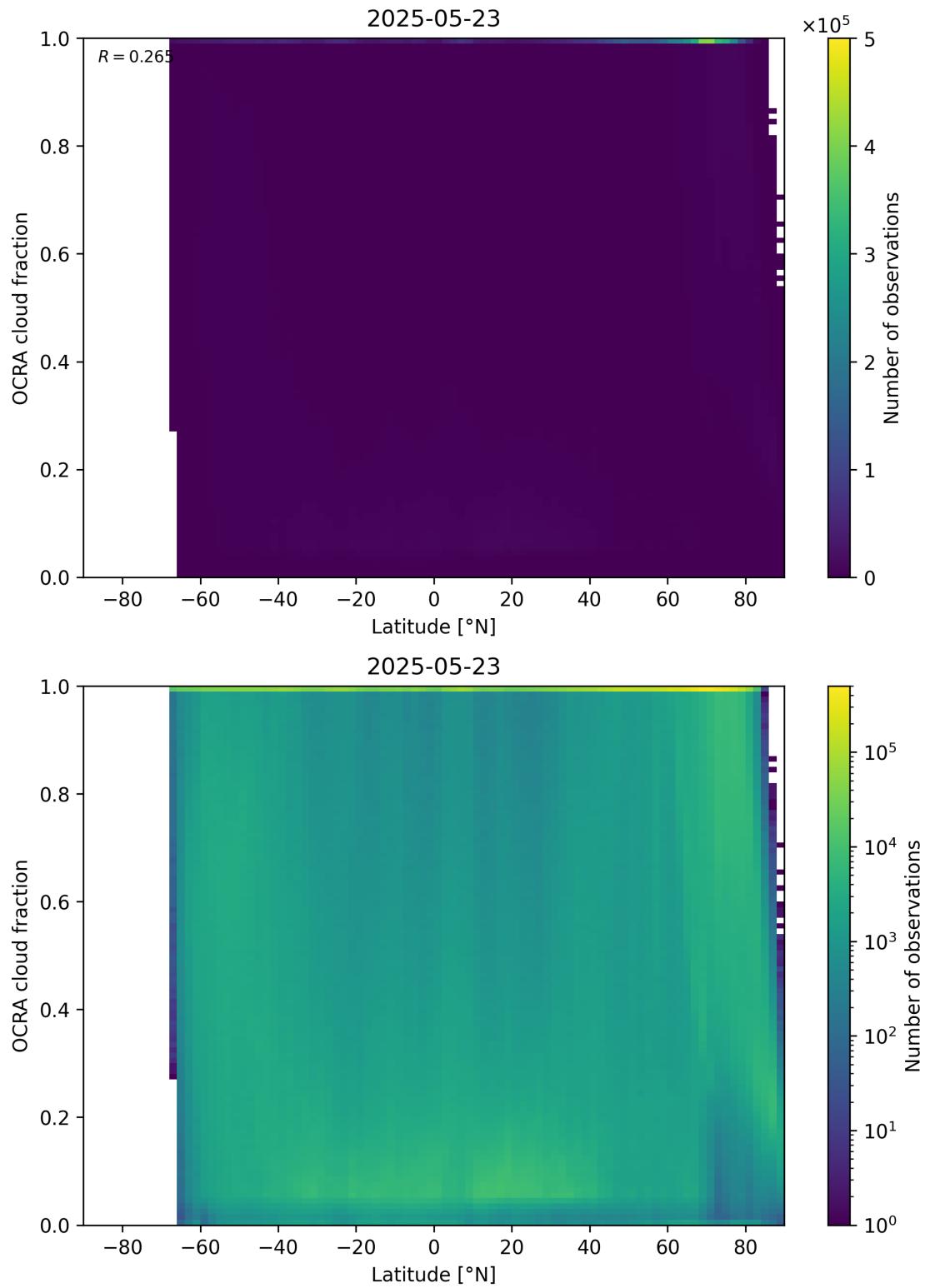
Figure 93: Scatter density plot of “Latitude” against “OCRA cloud fraction” for 2025-05-22 to 2025-05-24.
