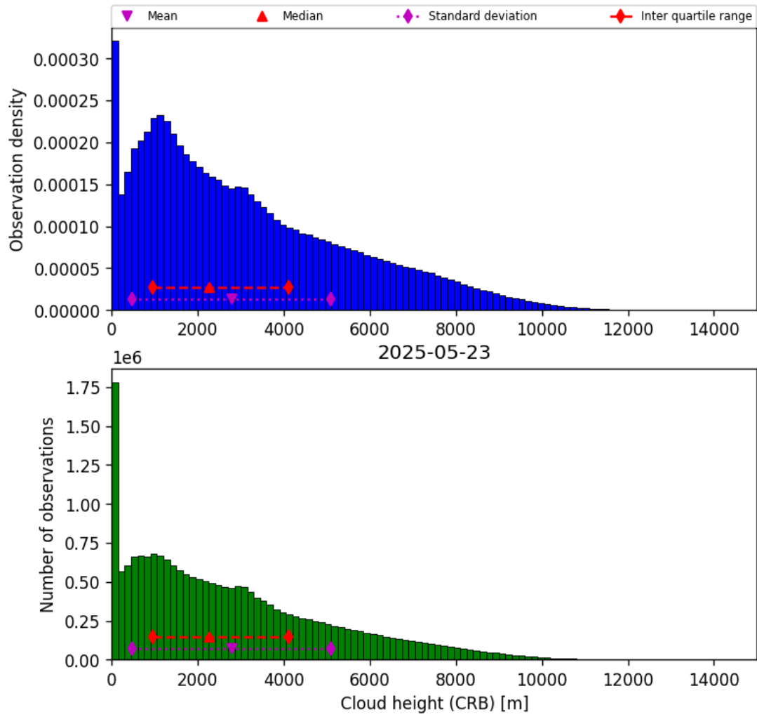
Figure 43: Histogram of “Cloud height (CRB)” for 2025-05-22 to 2025-05-24
