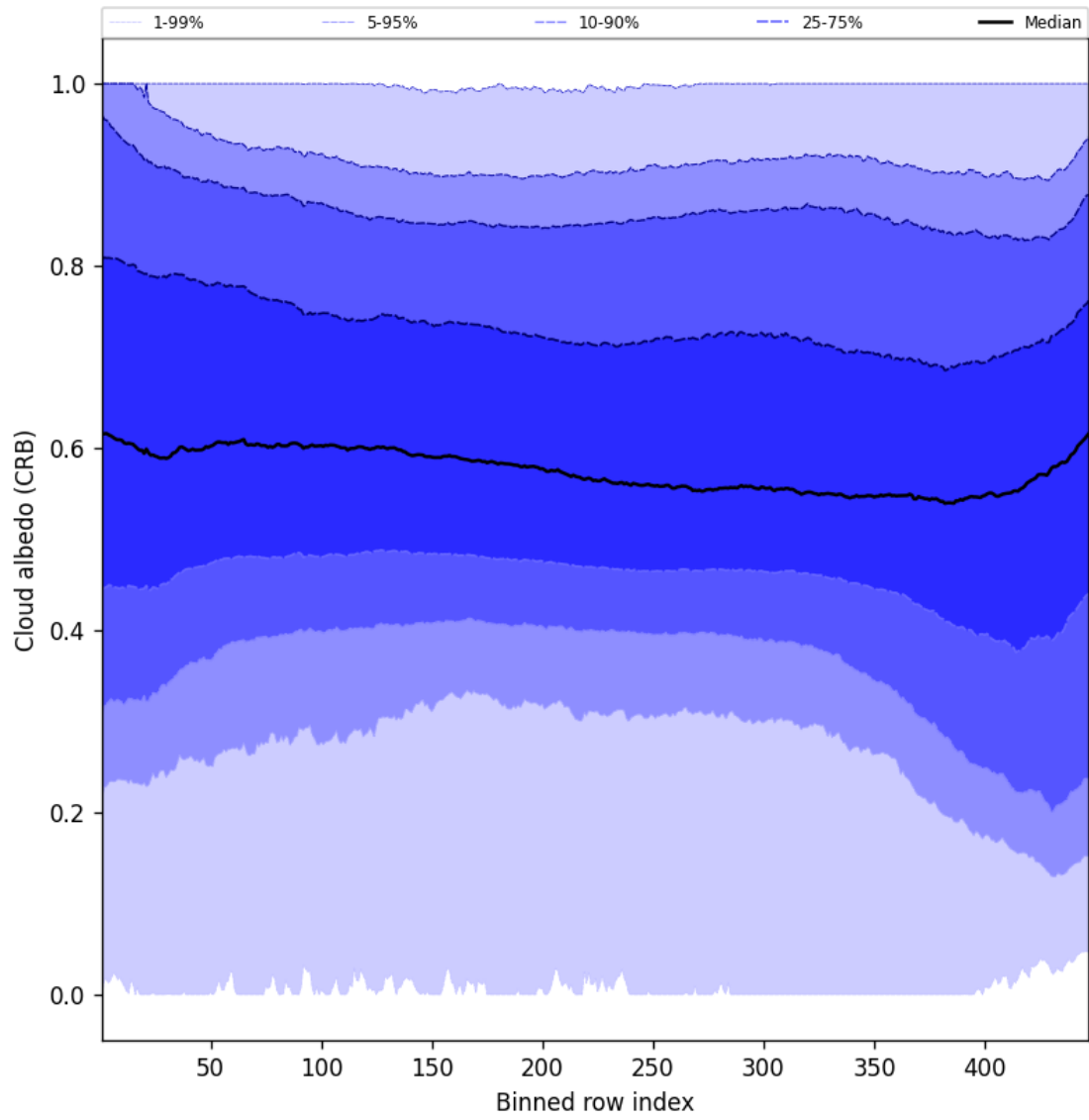
Figure 60: Along track statistics of “Cloud albedo (CRB)” for 2025-05-22 to 2025-05-24
