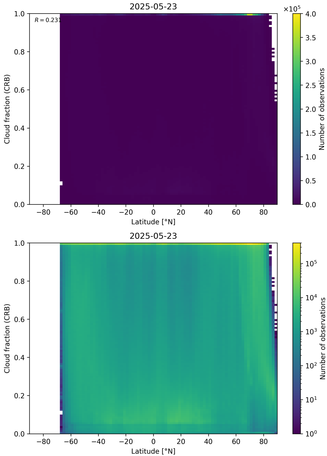
Figure 94: Scatter density plot of “Latitude” against “Cloud fraction (CRB)” for 2025-05-22 to 2025-05-24.
