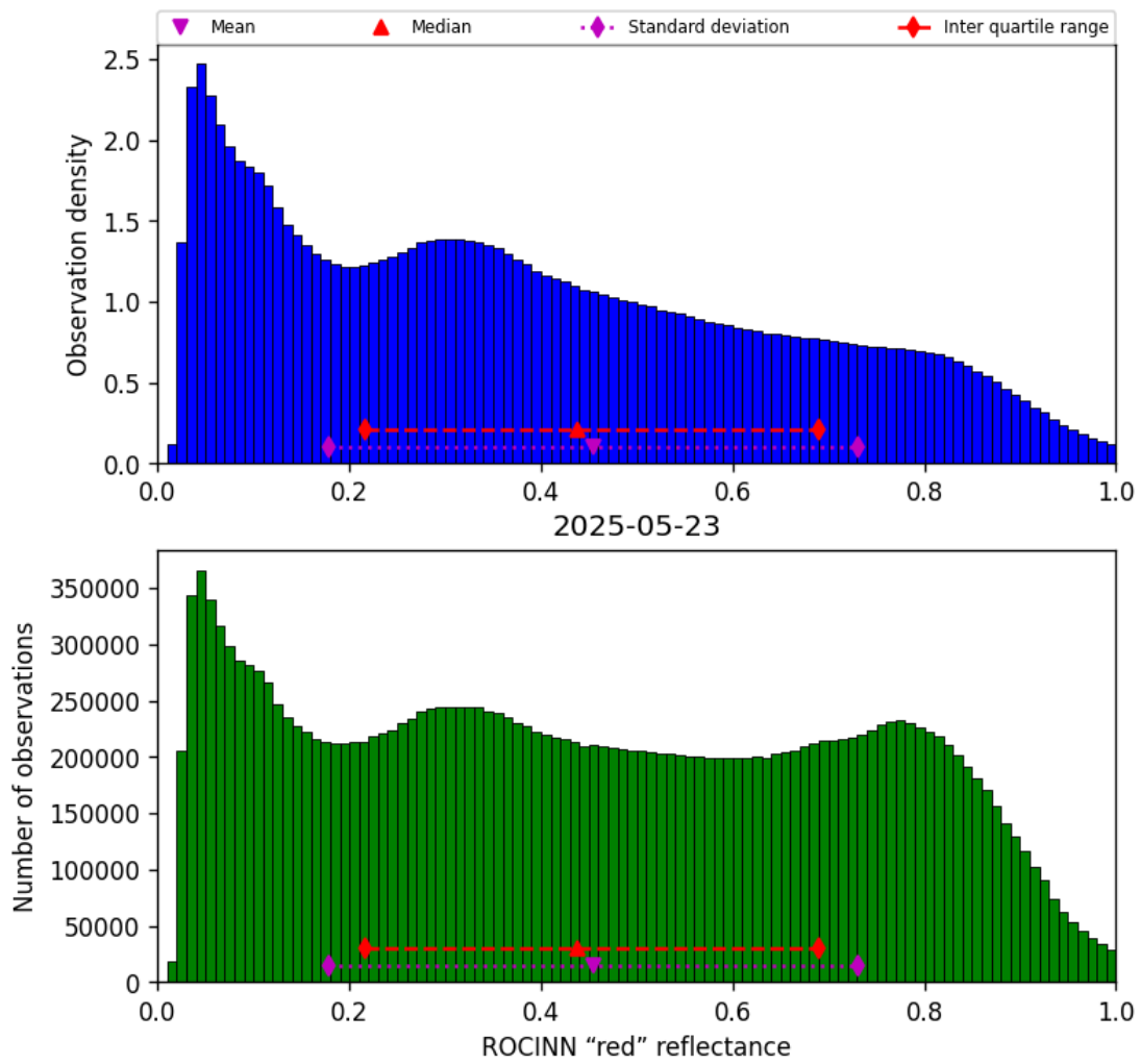
Figure 53: Histogram of “ROCINN “red” reflectance” for 2025-05-22 to 2025-05-24
