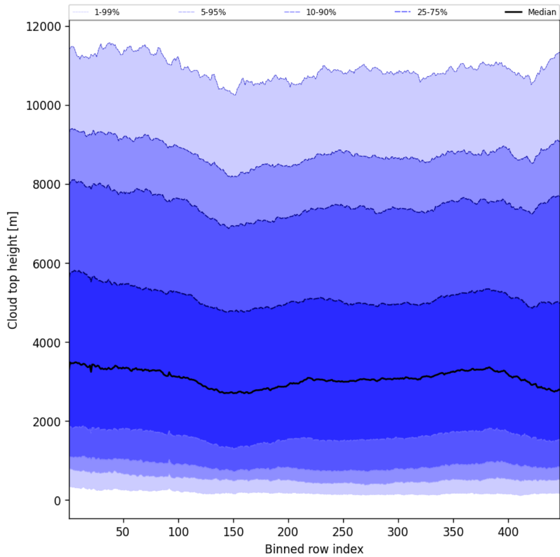
Figure 56: Along track statistics of “Cloud top height” for 2025-05-22 to 2025-05-24
