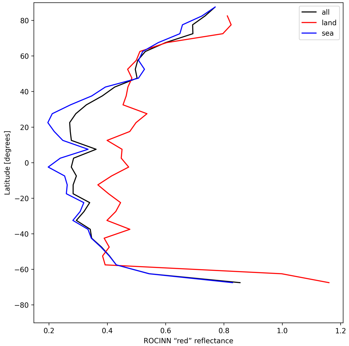
Figure 37: Zonal average of “ROCINN “red” reflectance” for 2025-05-22 to 2025-05-24.
