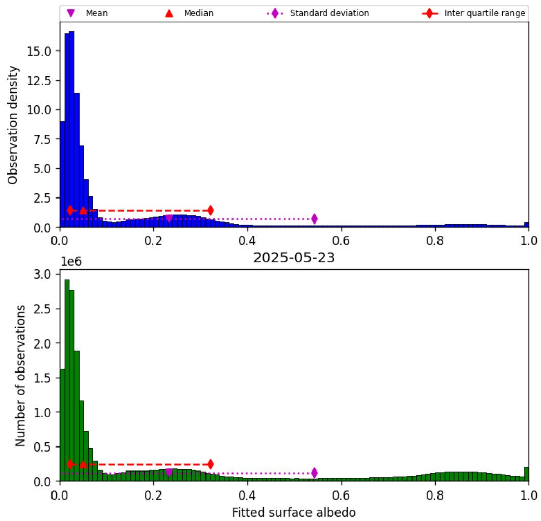
Figure 45: Histogram of “Fitted surface albedo” for 2025-05-22 to 2025-05-24
