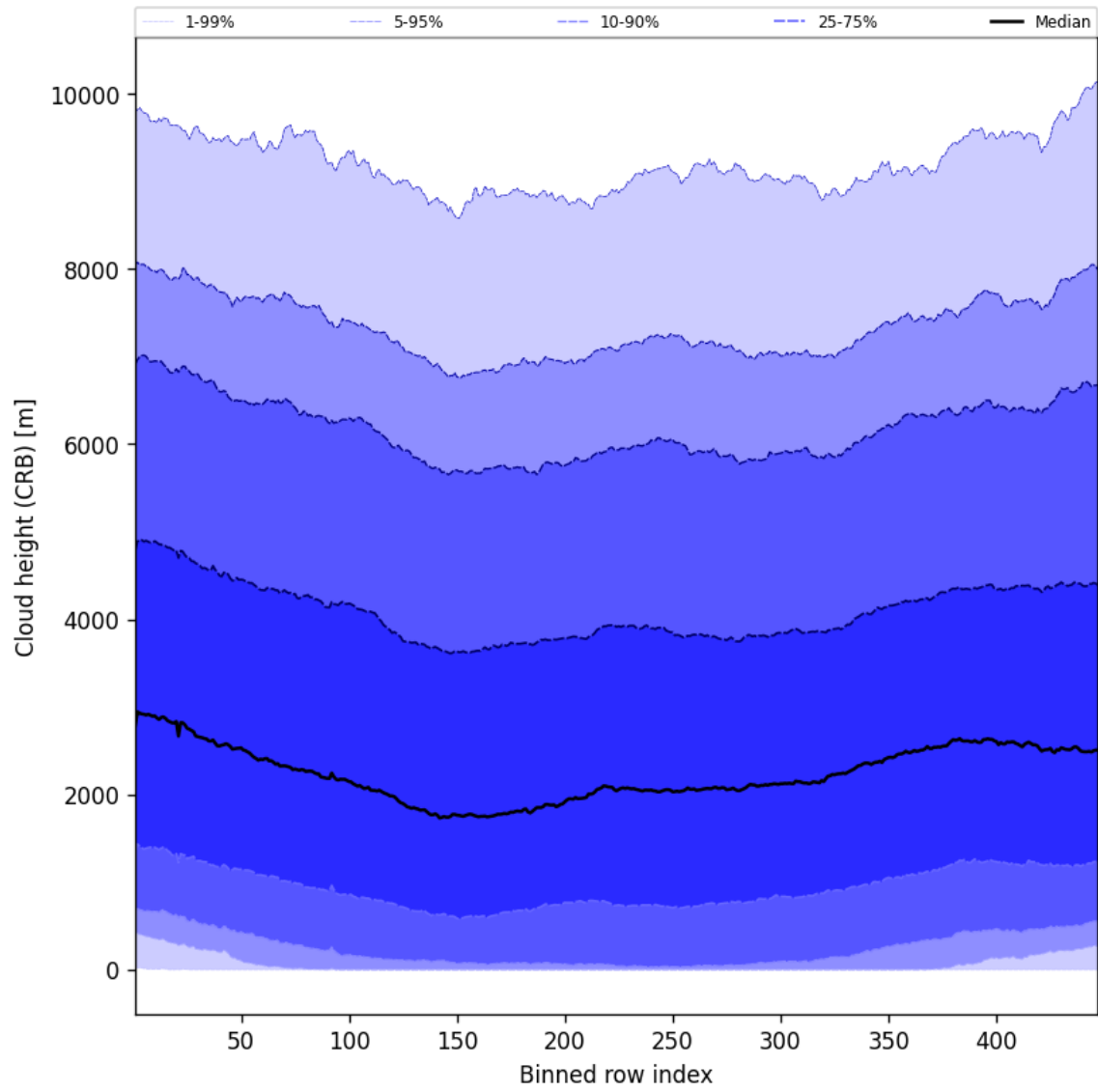
Figure 59: Along track statistics of “Cloud height (CRB)” for 2025-05-22 to 2025-05-24
