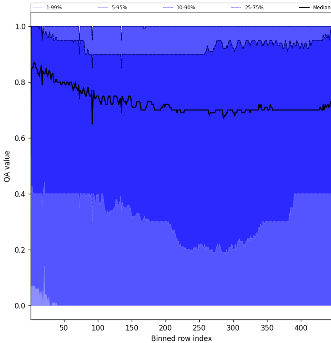
Figure 54: Along track statistics of "QA value" for 2025-05-22 to 2025-05-24
