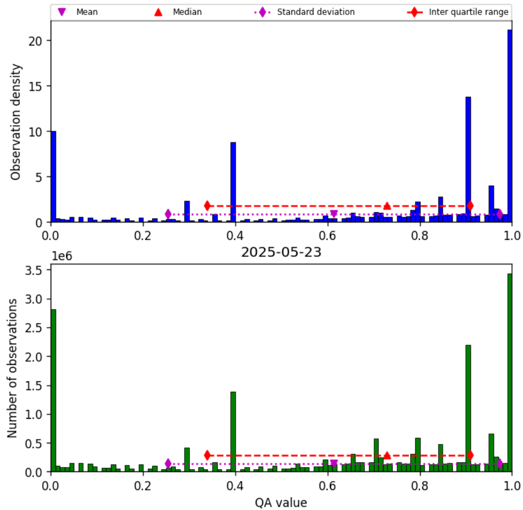
Figure 38: Histogram of “QA value” for 2025-05-22 to 2025-05-24
