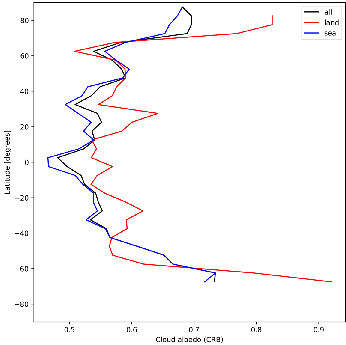
Figure 28: Zonal average of “Cloud albedo (CRB)” for 2025-05-22 to 2025-05-24.
