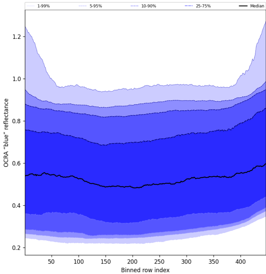
Figure 67: Along track statistics of "OCRA "blue" reflectance" for 2025-05-22 to 2025-05-24
