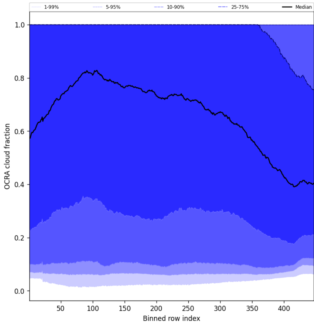
Figure 66: Along track statistics of “OCRA cloud fraction” for 2025-05-22 to 2025-05-24
