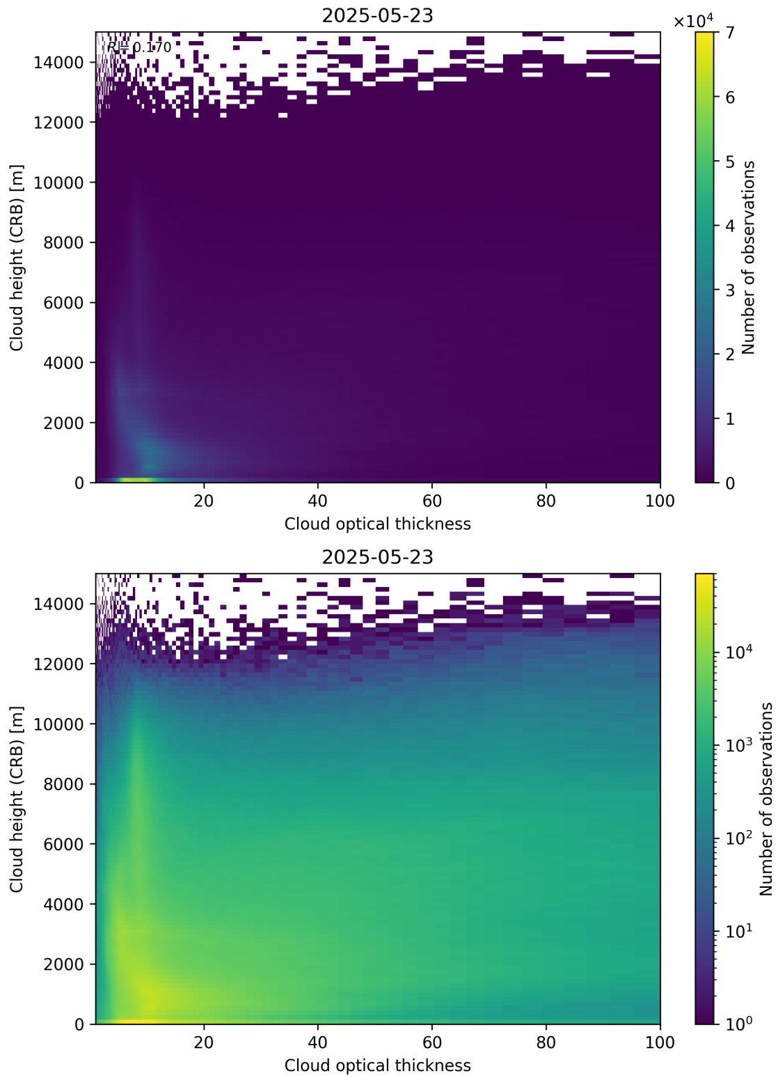
Figure 85: Scatter density plot of “Cloud optical thickness” against “Cloud height (CRB)” for 2025-05-22 to 2025-05-24.
