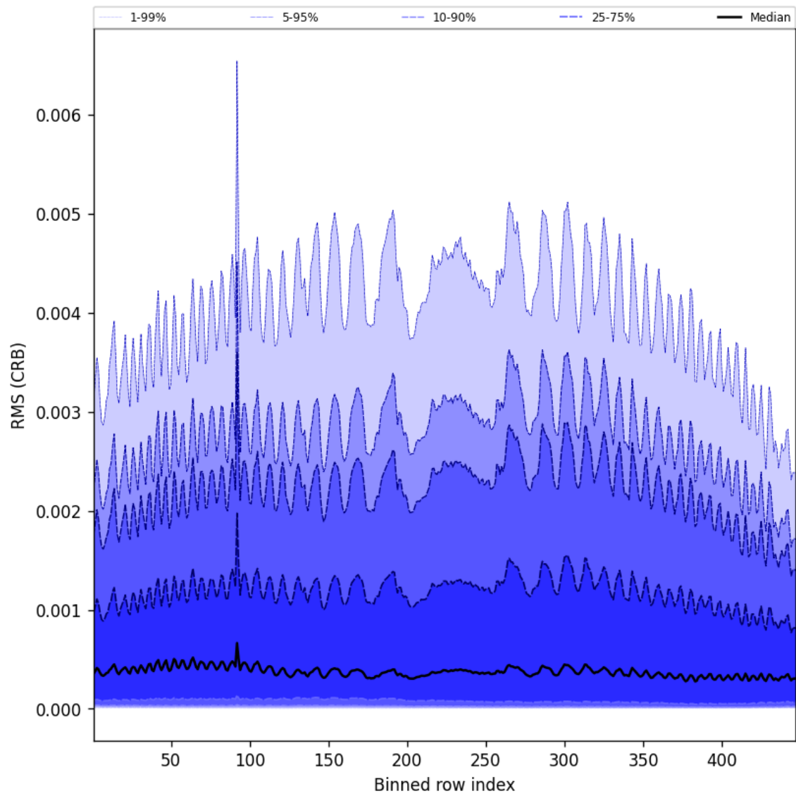
Figure 64: Along track statistics of “RMS (CRB)” for 2025-05-22 to 2025-05-24
