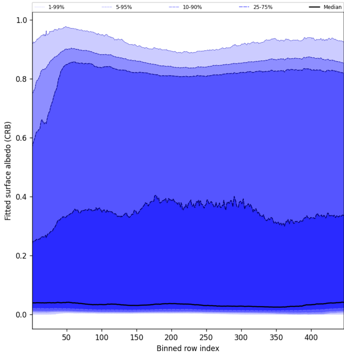
Figure 62: Along track statistics of “Fitted surface albedo (CRB)” for 2025-05-22 to 2025-05-24
