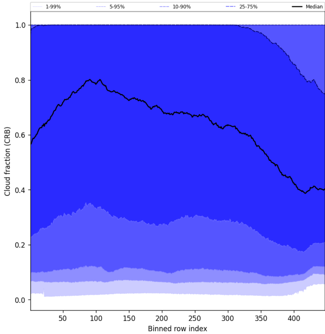
Figure 58: Along track statistics of “Cloud fraction (CRB)” for 2025-05-22 to 2025-05-24
