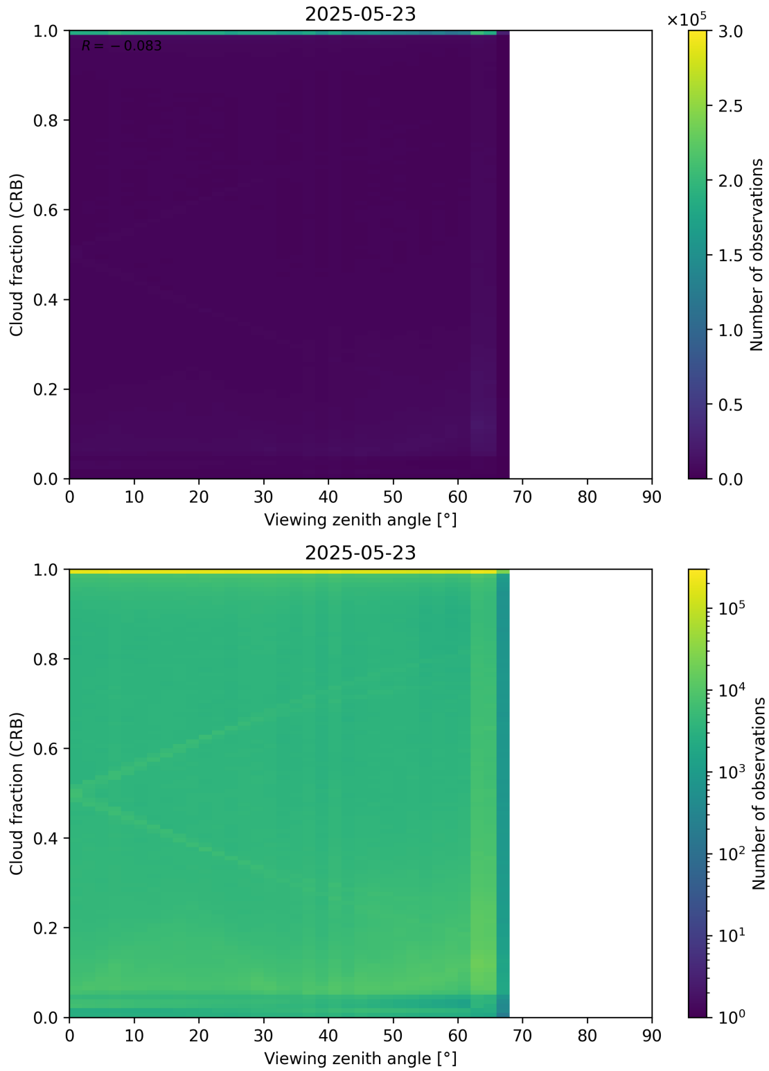
Figure 109: Scatter density plot of “Viewing zenith angle” against “Cloud fraction (CRB)” for 2025-05-22 to 2025-05-24.
