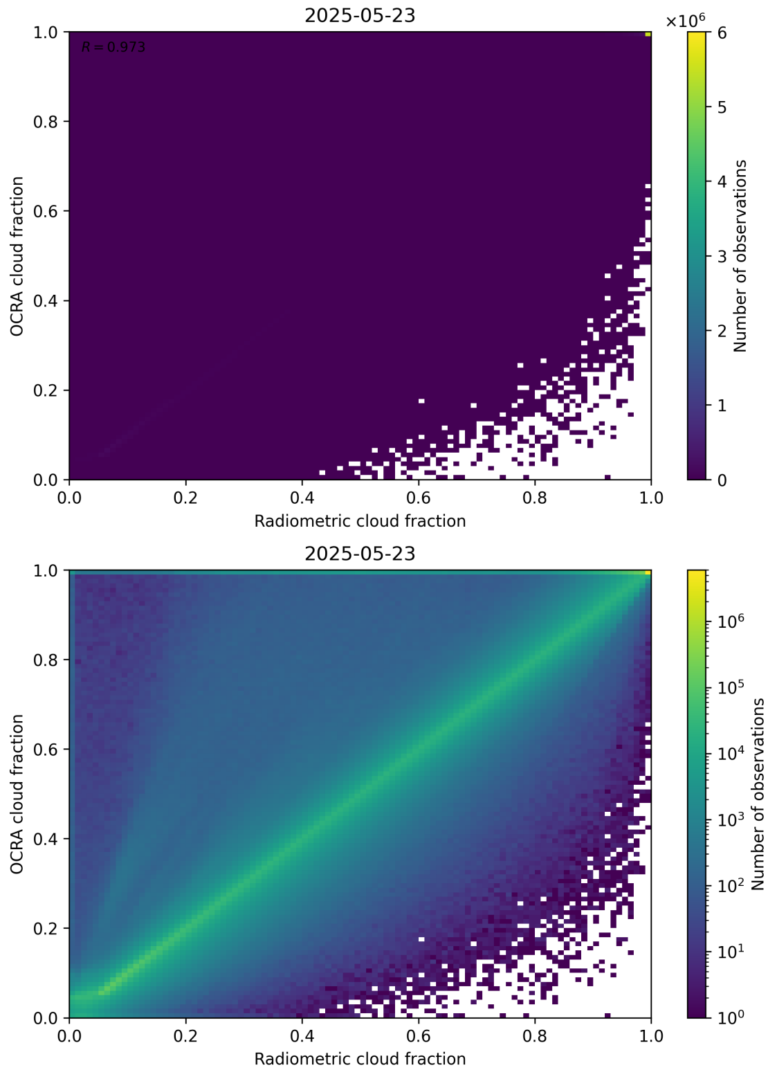
Figure 72: Scatter density plot of “Radiometric cloud fraction” against “OCRA cloud fraction” for 2025-05-22 to 2025-05-24.
