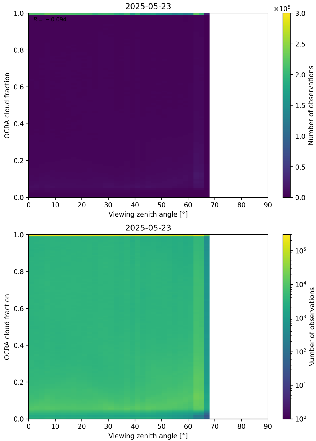
Figure 108: Scatter density plot of “Viewing zenith angle” against “OCRA cloud fraction” for 2025-05-22 to 2025-05-24.
