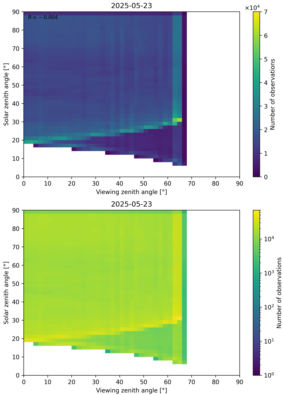
Figure 114: Scatter density plot of “Viewing zenith angle” against “Solar zenith angle” for 2025-05-22 to 2025-05-24.
