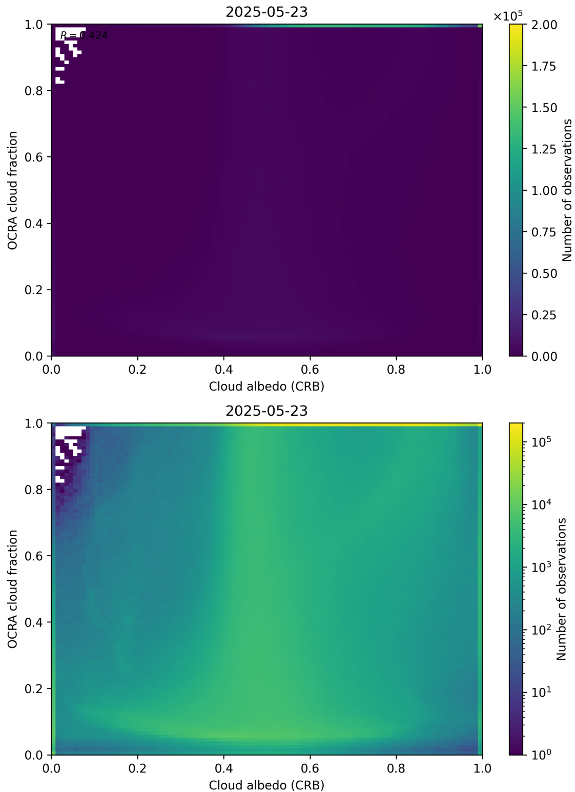
Figure 70: Scatter density plot of “Cloud albedo (CRB)” against “OCRA cloud fraction” for 2025-05-22 to 2025-05-24.
