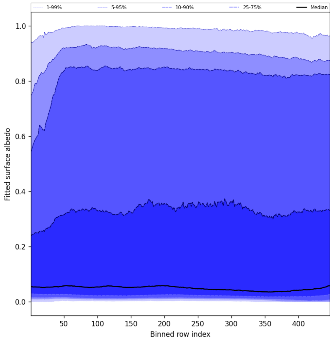
Figure 61: Along track statistics of “Fitted surface albedo” for 2025-05-22 to 2025-05-24
