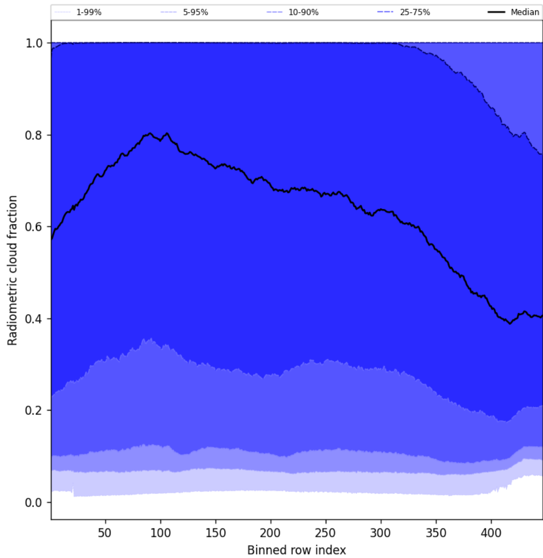
Figure 55: Along track statistics of “Radiometric cloud fraction” for 2025-05-22 to 2025-05-24
