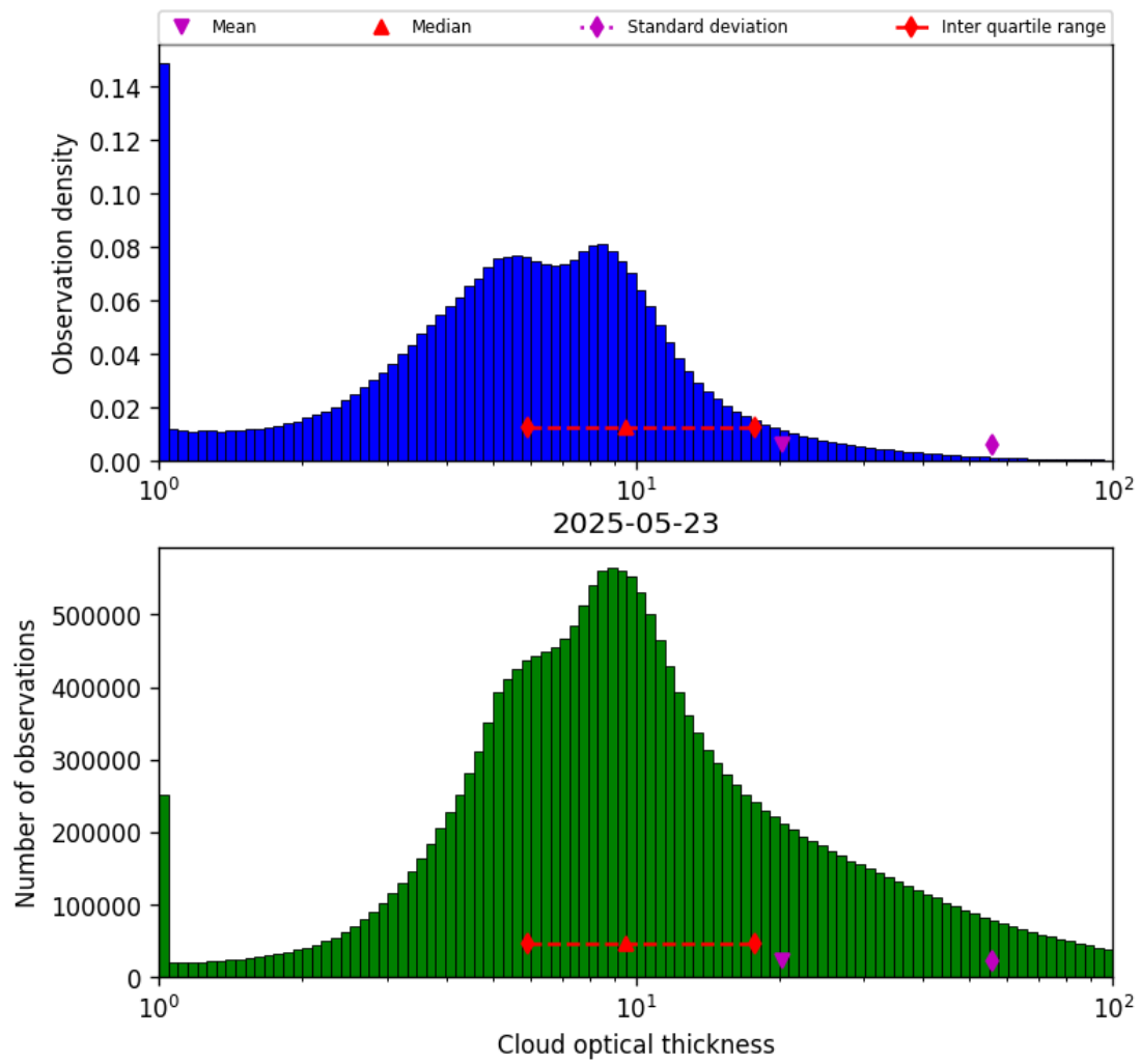
Figure 41: Histogram of “Cloud optical thickness” for 2025-05-22 to 2025-05-24
