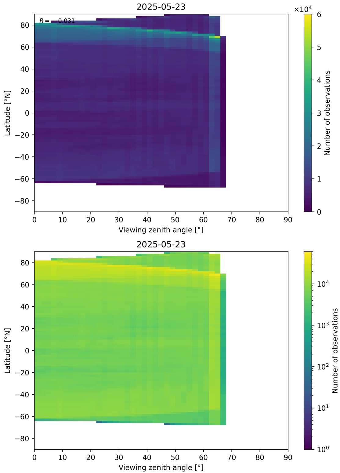
Figure 113: Scatter density plot of “Viewing zenith angle” against “Latitude” for 2025-05-22 to 2025-05-24.
