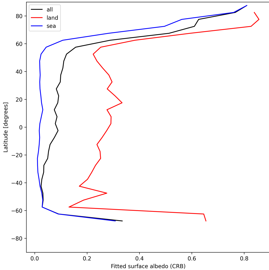
Figure 30: Zonal average of “Fitted surface albedo (CRB)” for 2025-05-22 to 2025-05-24.
