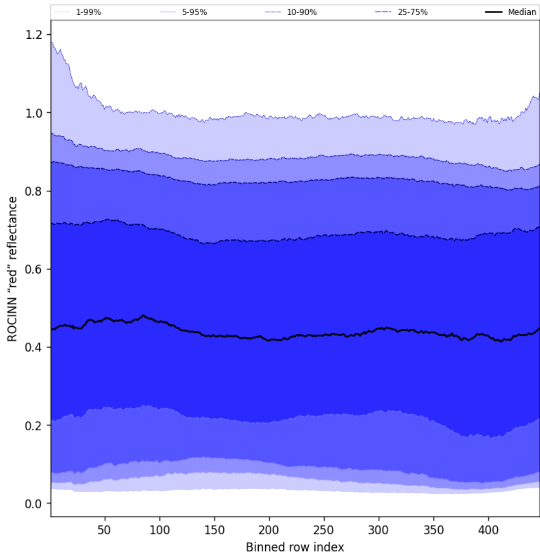
Figure 69: Along track statistics of "ROCINN "red" reflectance" for 2025-05-22 to 2025-05-24
