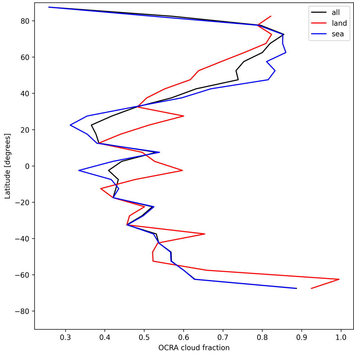
Figure 34: Zonal average of “OCRA cloud fraction” for 2025-05-22 to 2025-05-24.
