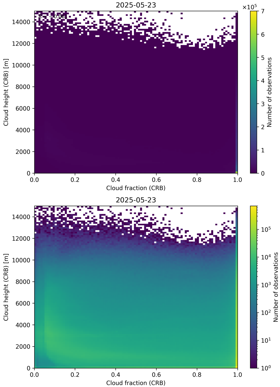
Figure 79: Scatter density plot of “Cloud fraction (CRB)” against “Cloud height (CRB)” for 2025-05-22 to 2025-05-24.
