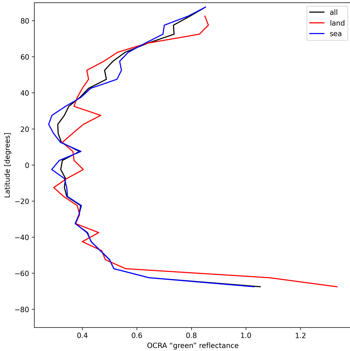
Figure 36: Zonal average of “OCRA “green” reflectance” for 2025-05-22 to 2025-05-24.
