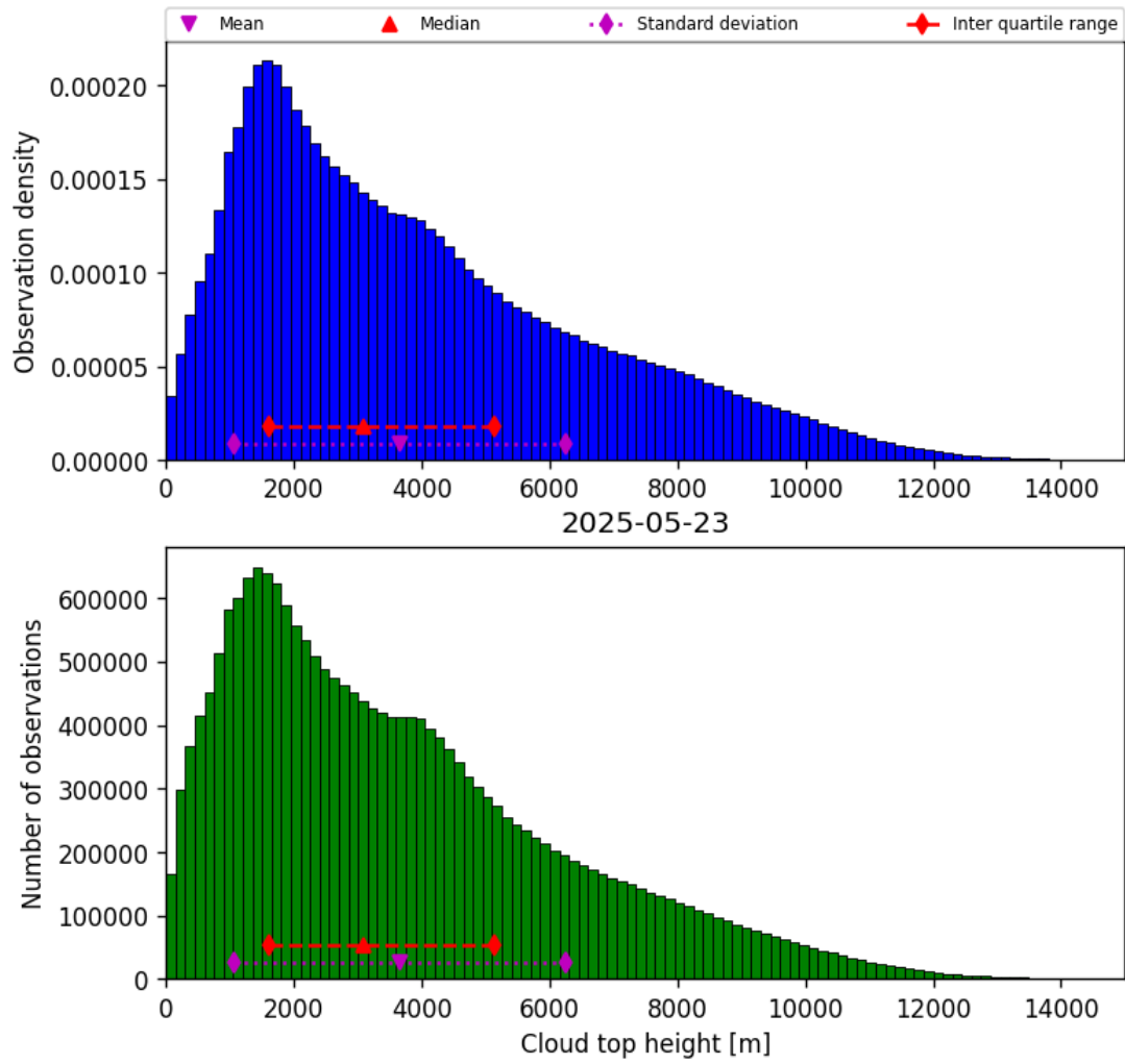
Figure 40: Histogram of “Cloud top height” for 2025-05-22 to 2025-05-24
