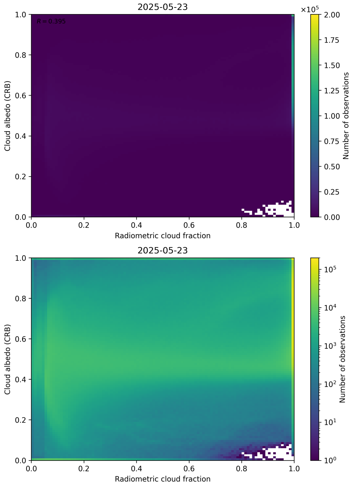
Figure 71: Scatter density plot of “Radiometric cloud fraction” against “Cloud albedo (CRB)” for 2025-05-22 to 2025-05-24.
