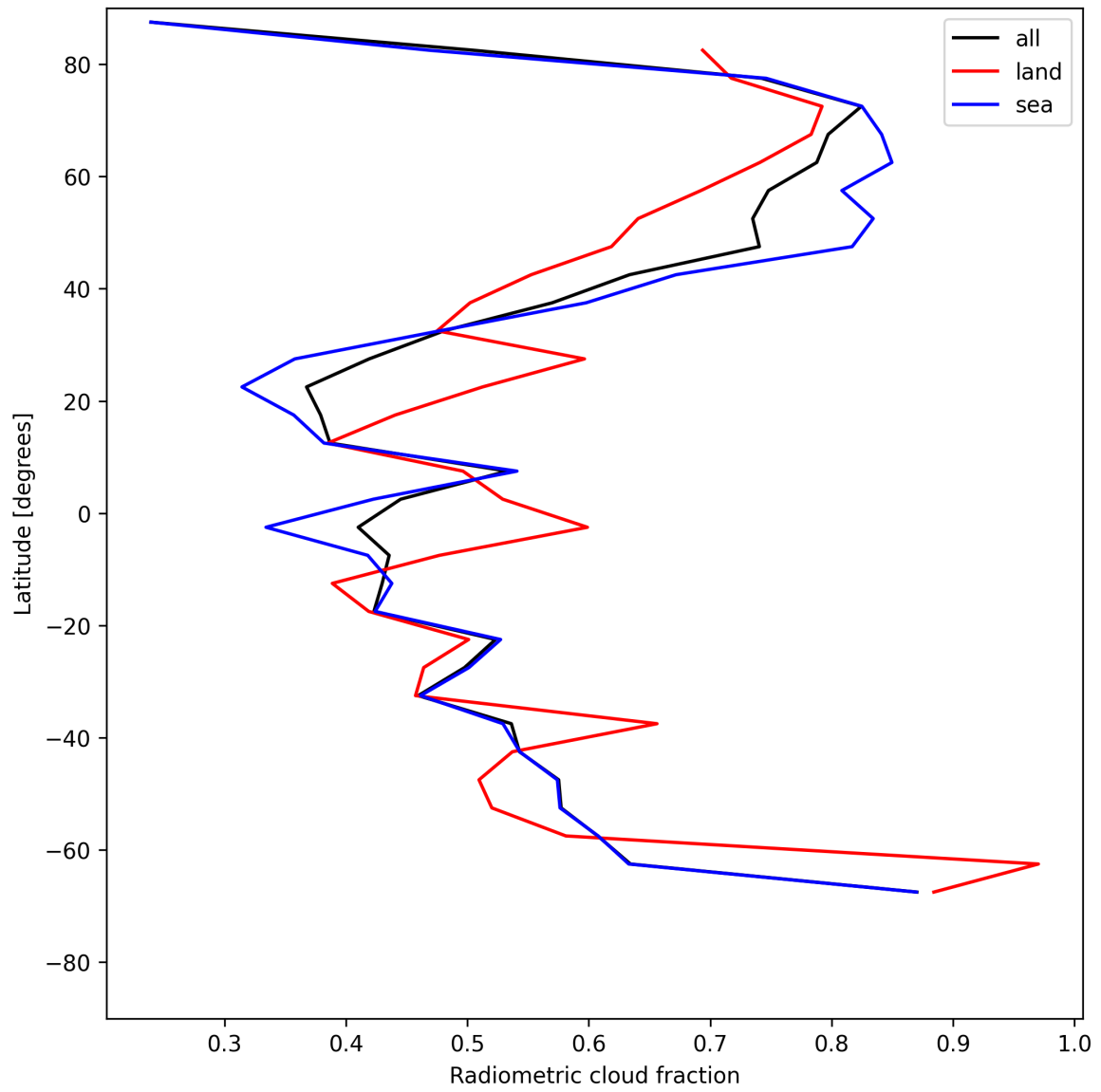
Figure 23: Zonal average of “Radiometric cloud fraction” for 2025-05-22 to 2025-05-24.
