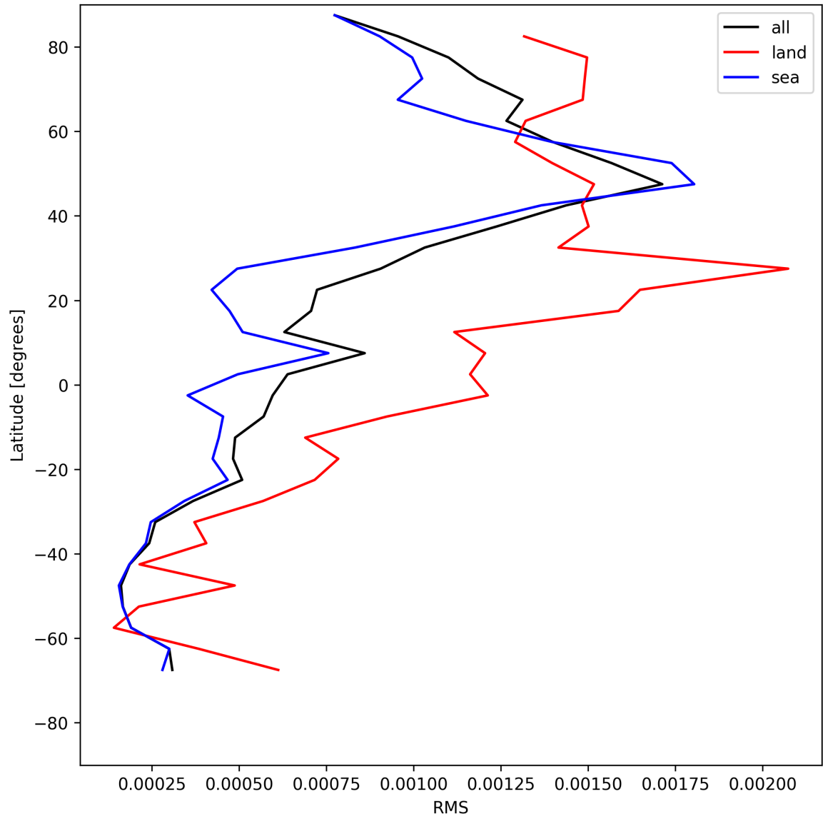
Figure 31: Zonal average of “RMS” for 2025-05-22 to 2025-05-24.
