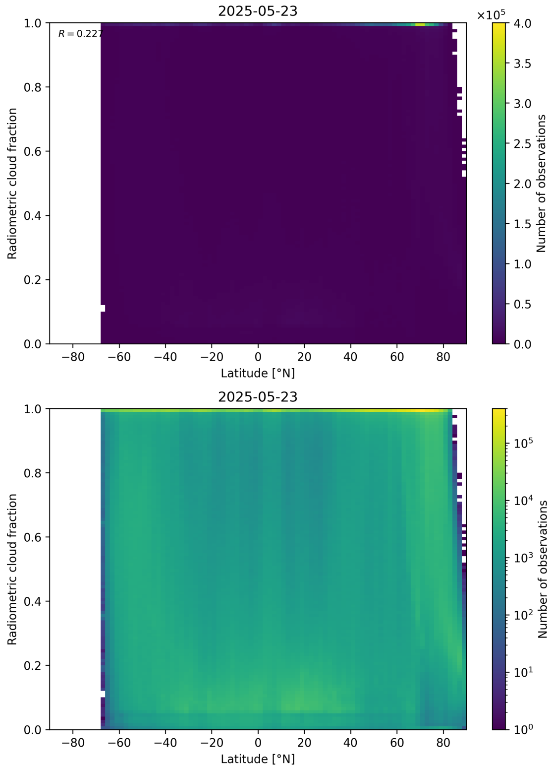
Figure 92: Scatter density plot of “Latitude” against “Radiometric cloud fraction” for 2025-05-22 to 2025-05-24.
