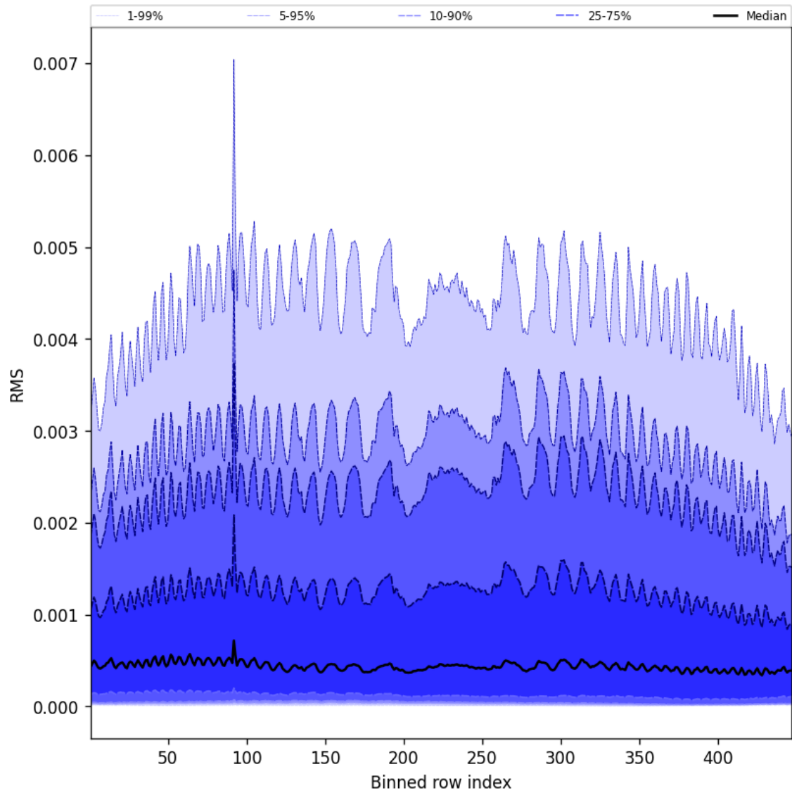
Figure 63: Along track statistics of “RMS” for 2025-05-22 to 2025-05-24
