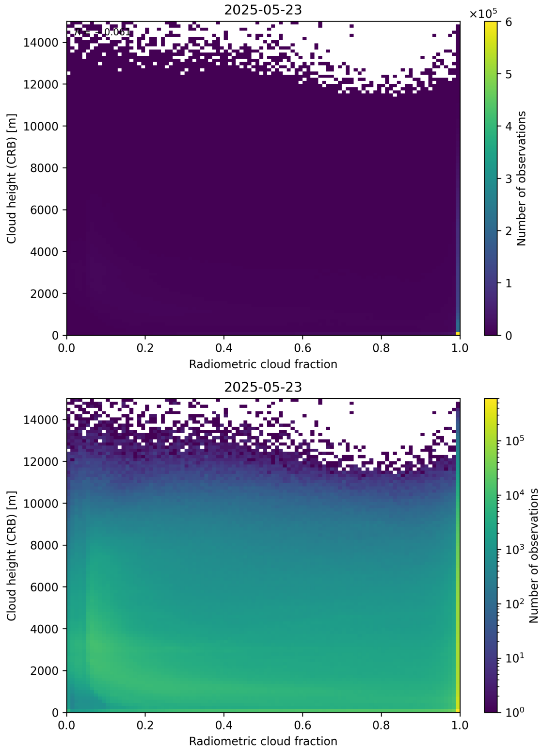
Figure 74: Scatter density plot of “Radiometric cloud fraction” against “Cloud height (CRB)” for 2025-05-22 to 2025-05-24.
