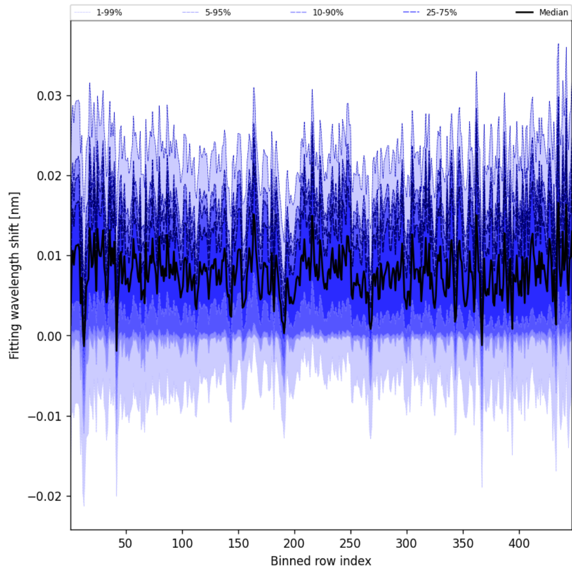
Figure 65: Along track statistics of “Fitting wavelength shift” for 2025-05-22 to 2025-05-24
