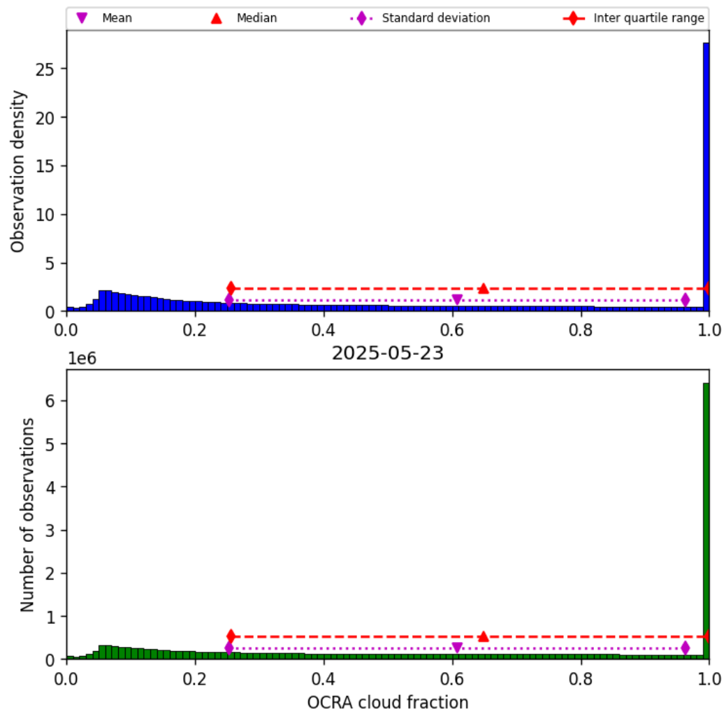
Figure 50: Histogram of “OCRA cloud fraction” for 2025-05-22 to 2025-05-24
