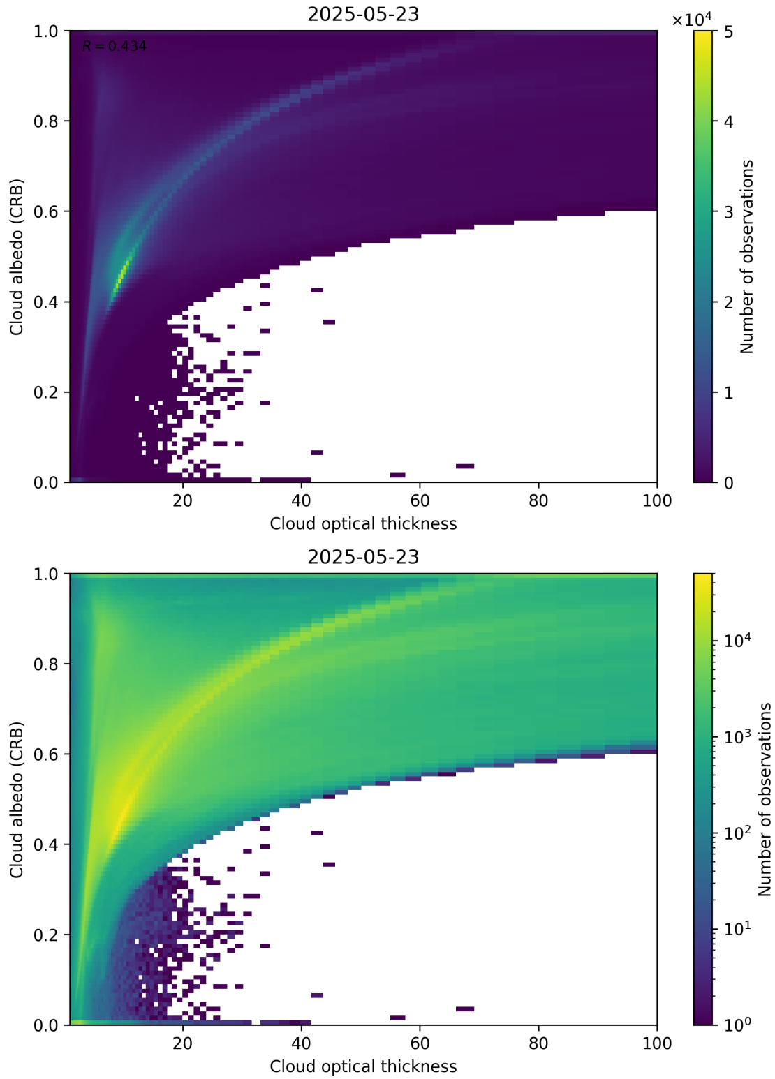
Figure 82: Scatter density plot of “Cloud optical thickness” against “Cloud albedo (CRB)” for 2025-05-22 to 2025-05-24.
