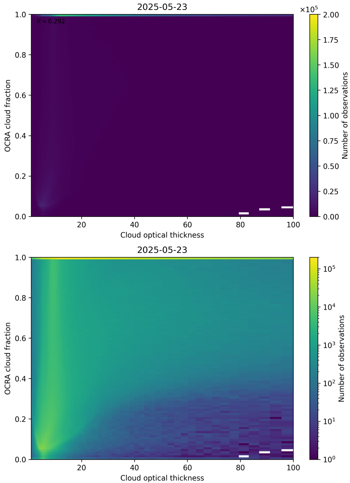
Figure 83: Scatter density plot of “Cloud optical thickness” against “OCRA cloud fraction” for 2025-05-22 to 2025-05-24.
