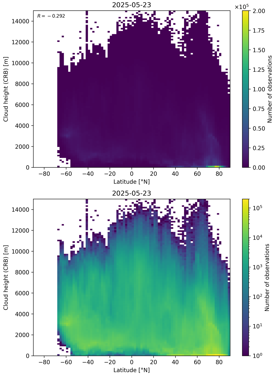
Figure 95: Scatter density plot of “Latitude” against “Cloud height (CRB)” for 2025-05-22 to 2025-05-24.
