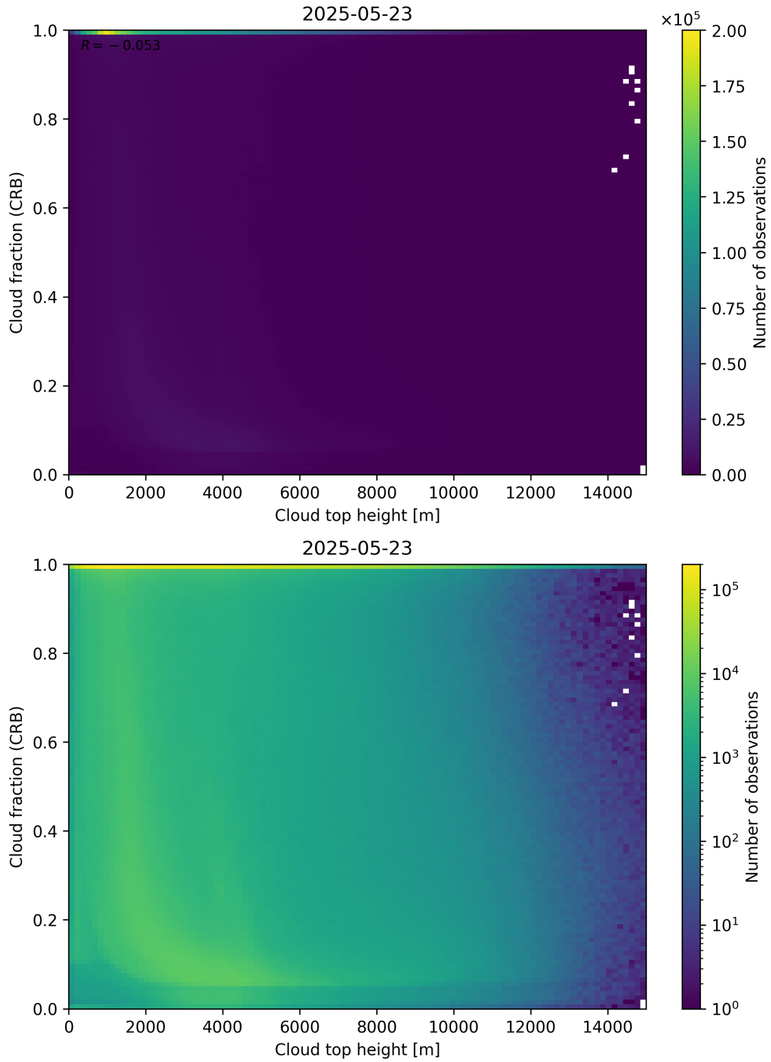
Figure 88: Scatter density plot of “Cloud top height” against “Cloud fraction (CRB)” for 2025-05-22 to 2025-05-24.
