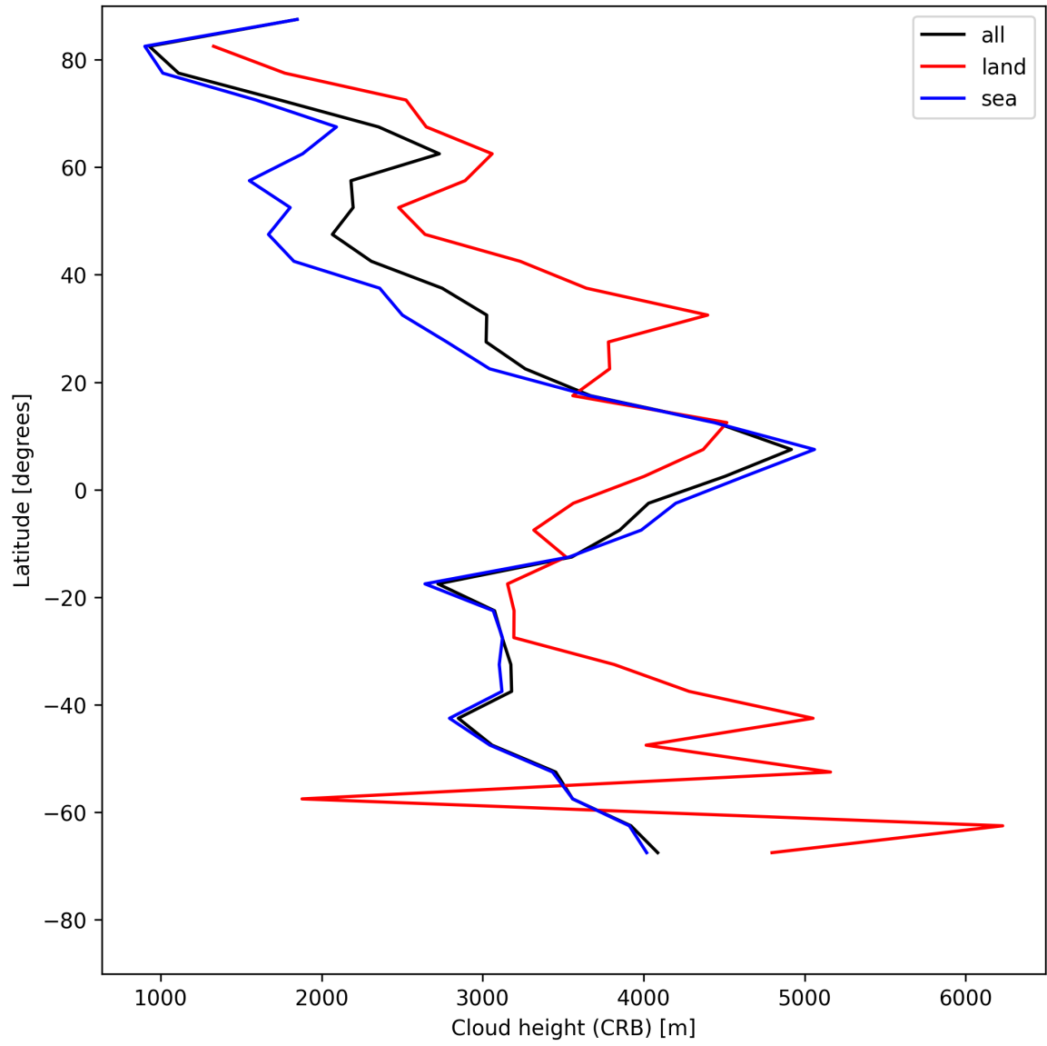
Figure 27: Zonal average of “Cloud height (CRB)” for 2025-05-22 to 2025-05-24.
