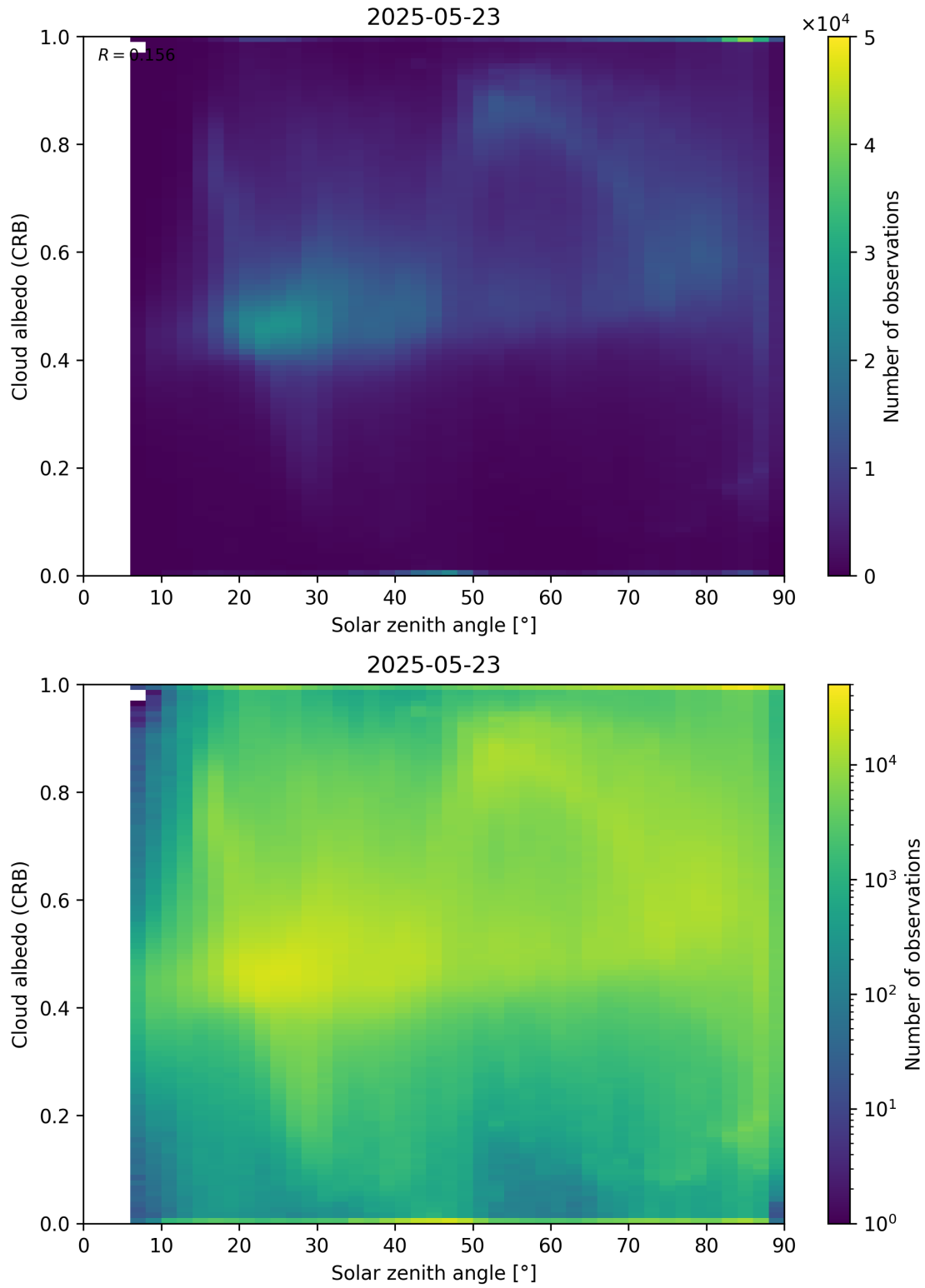
Figure 98: Scatter density plot of “Solar zenith angle” against “Cloud albedo (CRB)” for 2025-05-22 to 2025-05-24.
