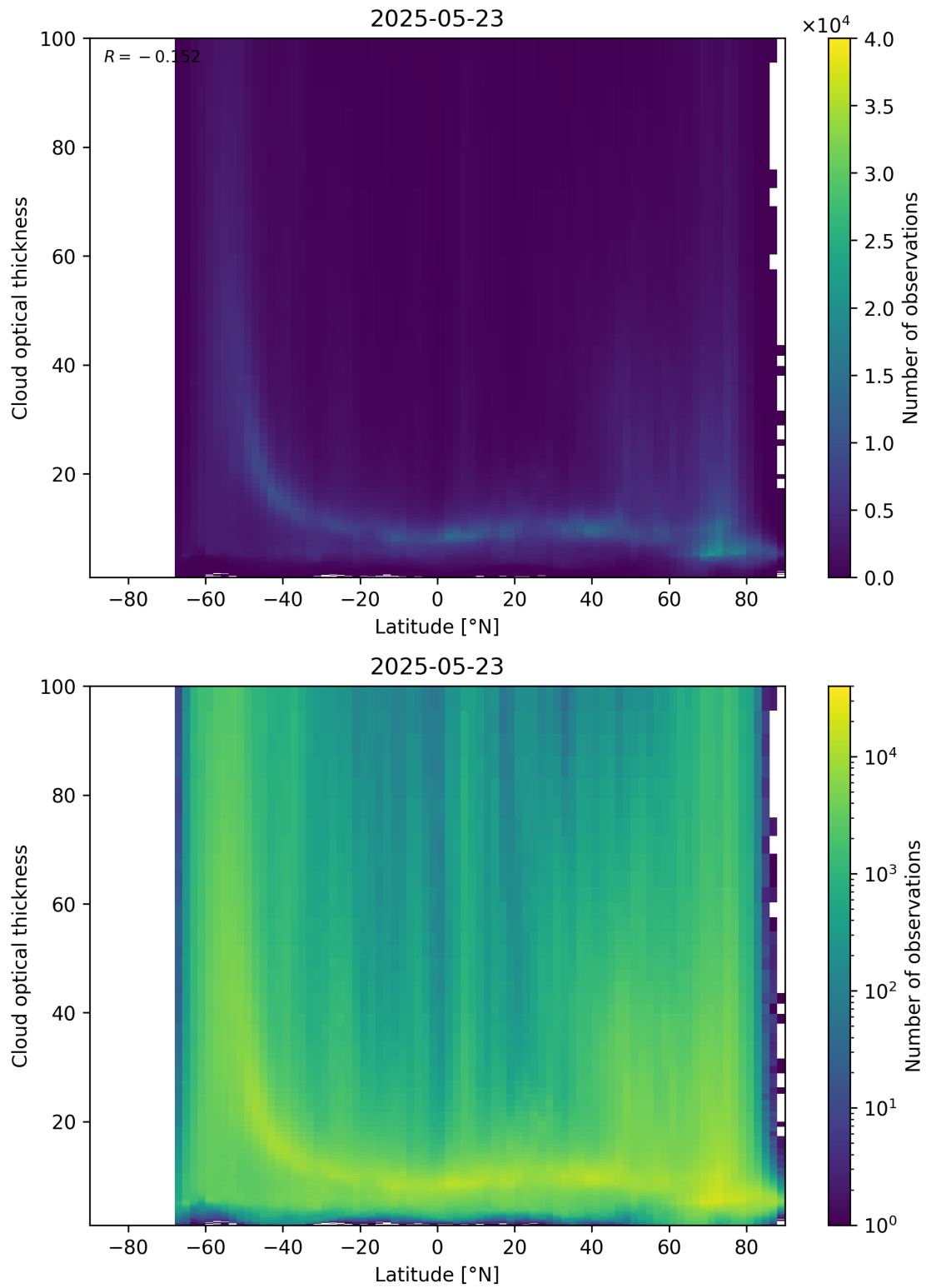
Figure 96: Scatter density plot of “Latitude” against “Cloud optical thickness” for 2025-05-22 to 2025-05-24.
