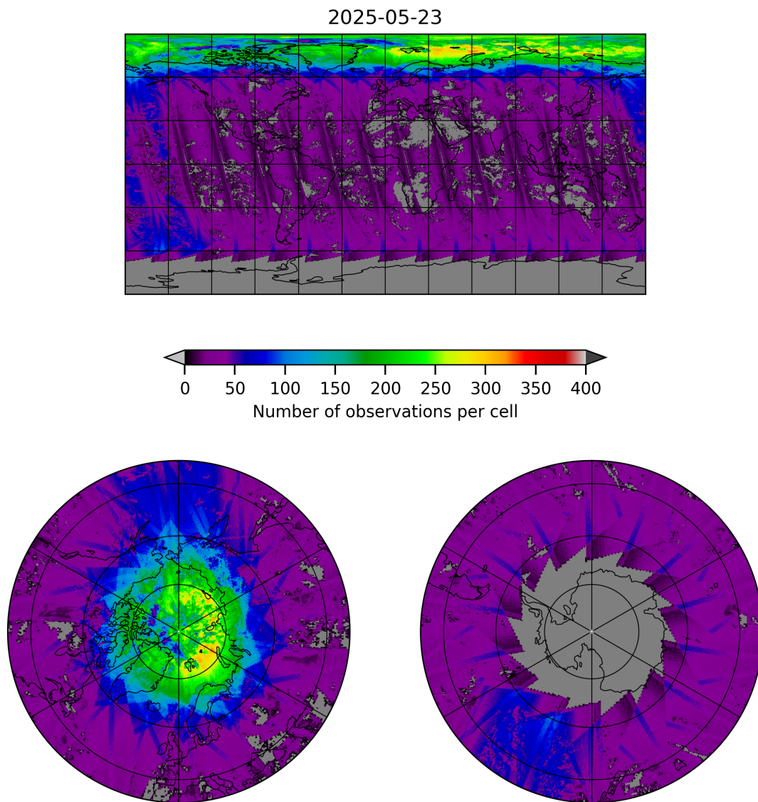
Figure 21: Map of the number of observations for 2025-05-22 to 2025-05-24
