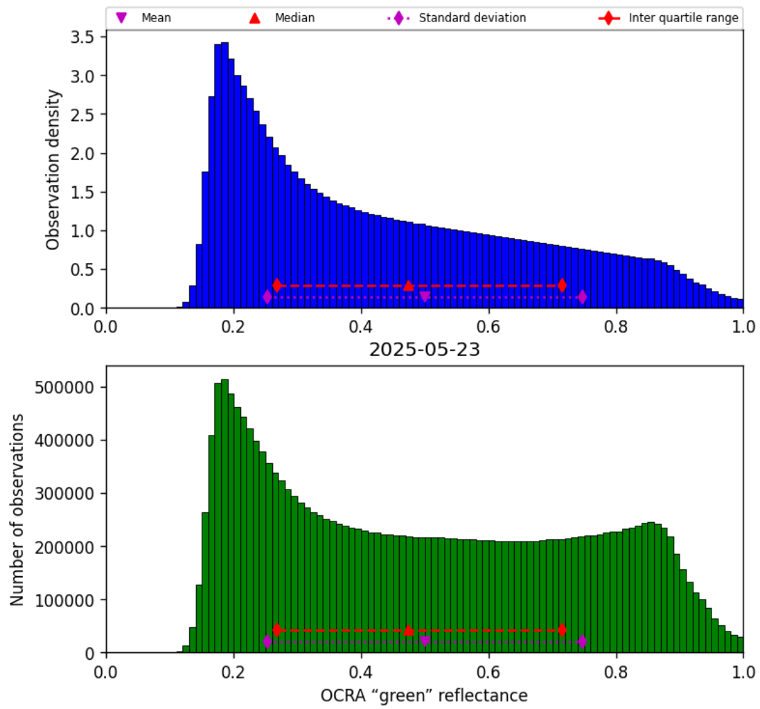
Figure 52: Histogram of “OCRA “green” reflectance” for 2025-05-22 to 2025-05-24
