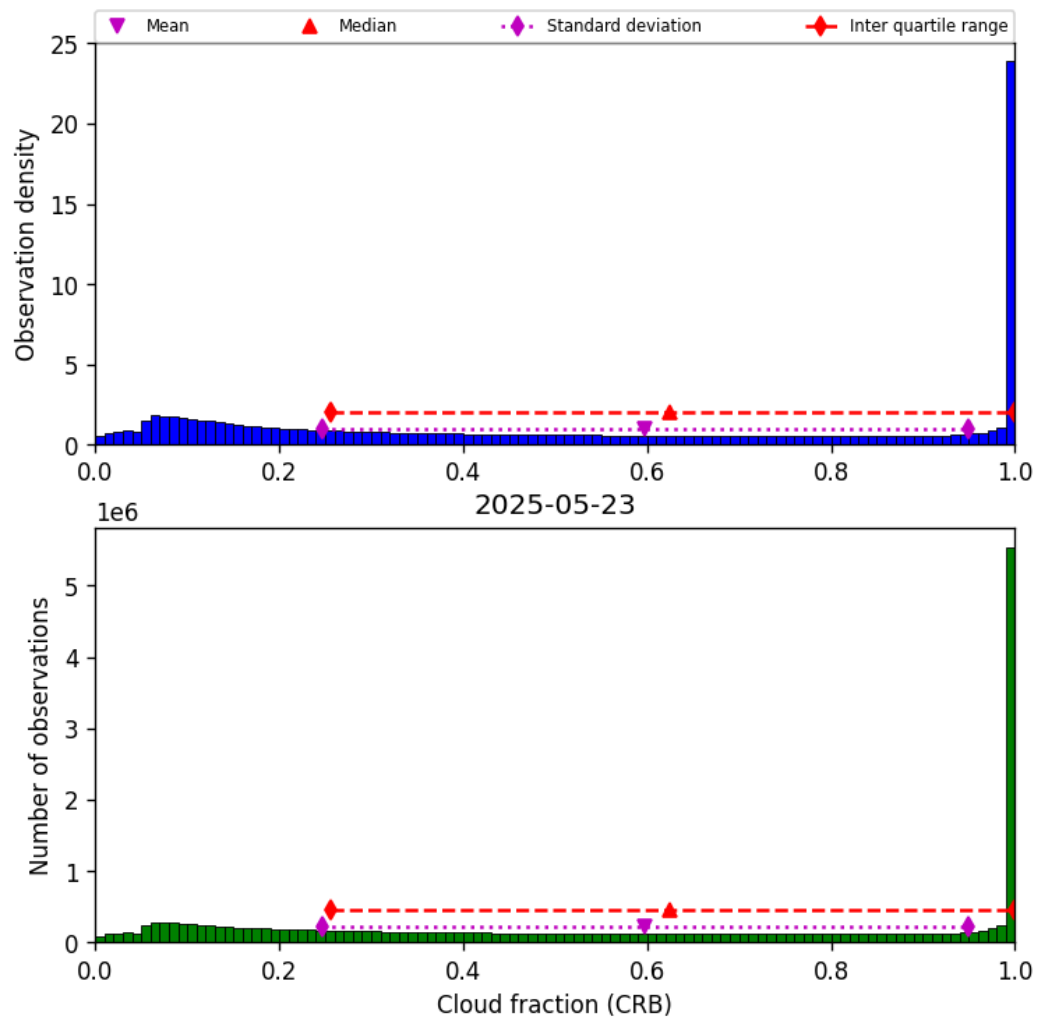
Figure 42: Histogram of “Cloud fraction (CRB)” for 2025-05-22 to 2025-05-24
