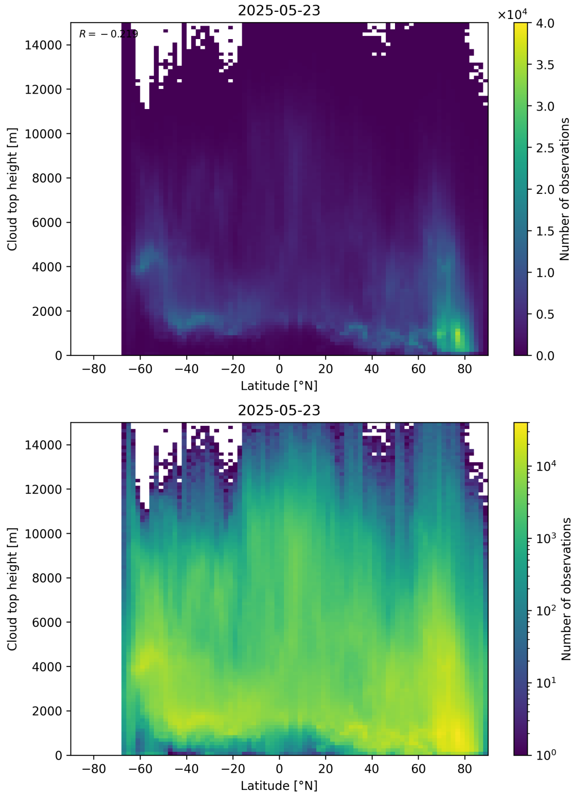
Figure 97: Scatter density plot of “Latitude” against “Cloud top height” for 2025-05-22 to 2025-05-24.
