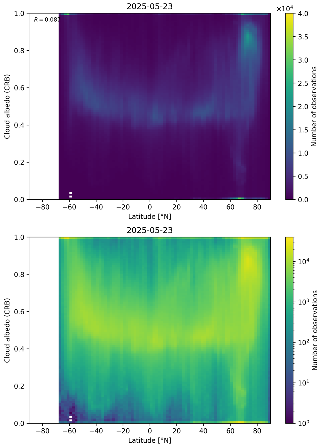
Figure 91: Scatter density plot of “Latitude” against “Cloud albedo (CRB)” for 2025-05-22 to 2025-05-24.
