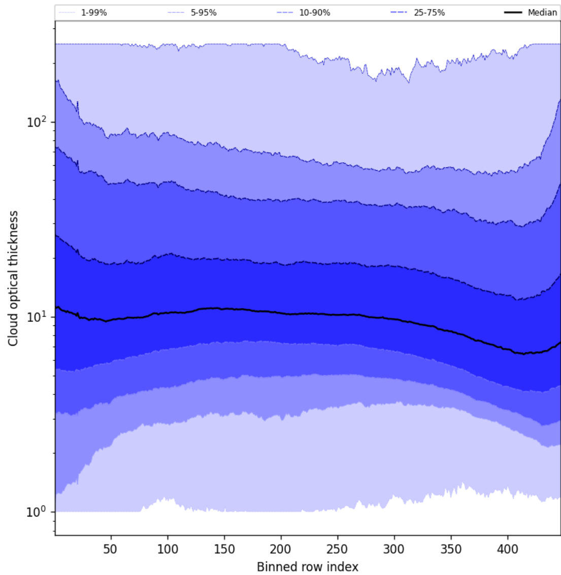
Figure 57: Along track statistics of “Cloud optical thickness” for 2025-05-22 to 2025-05-24
