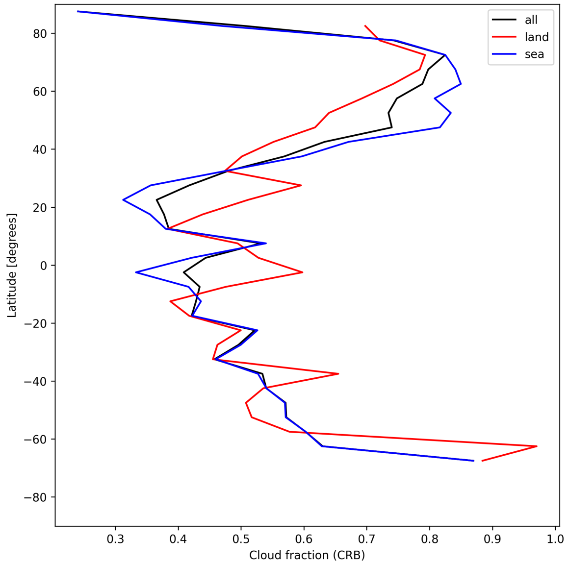
Figure 26: Zonal average of “Cloud fraction (CRB)” for 2025-05-22 to 2025-05-24.
