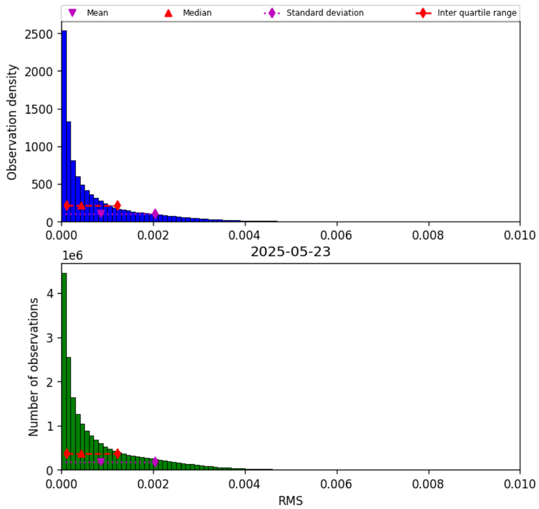
Figure 47: Histogram of “RMS” for 2025-05-22 to 2025-05-24
