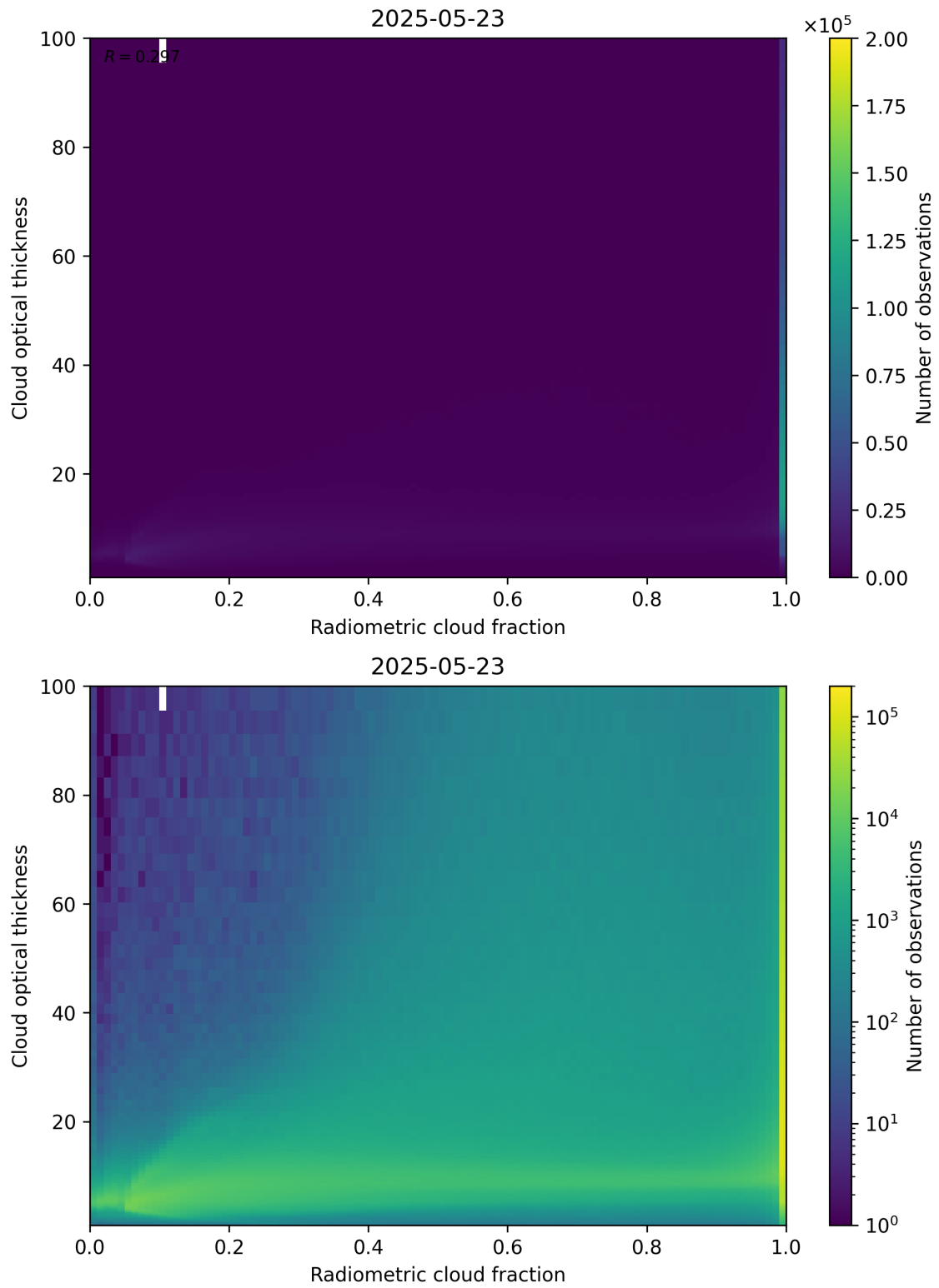
Figure 75: Scatter density plot of “Radiometric cloud fraction” against “Cloud optical thickness” for 2025-05-22 to 2025-05-24.
