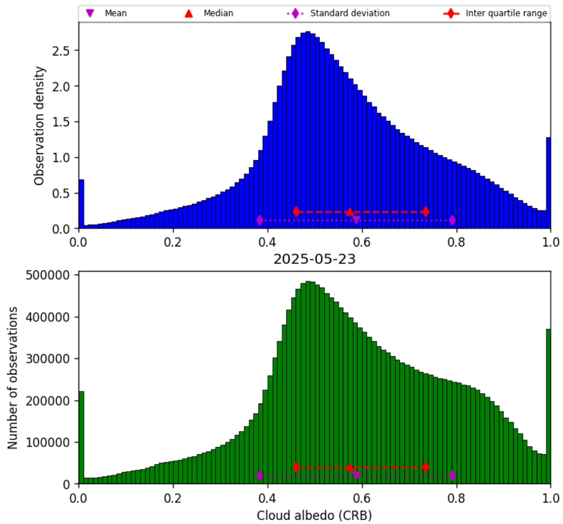
Figure 44: Histogram of “Cloud albedo (CRB)” for 2025-05-22 to 2025-05-24
