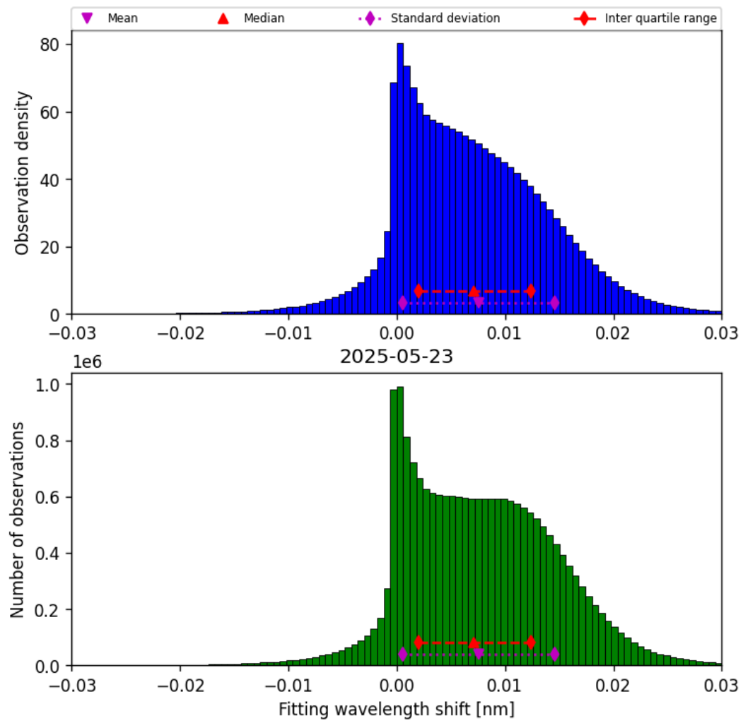
Figure 49: Histogram of “Fitting wavelength shift” for 2025-05-22 to 2025-05-24
