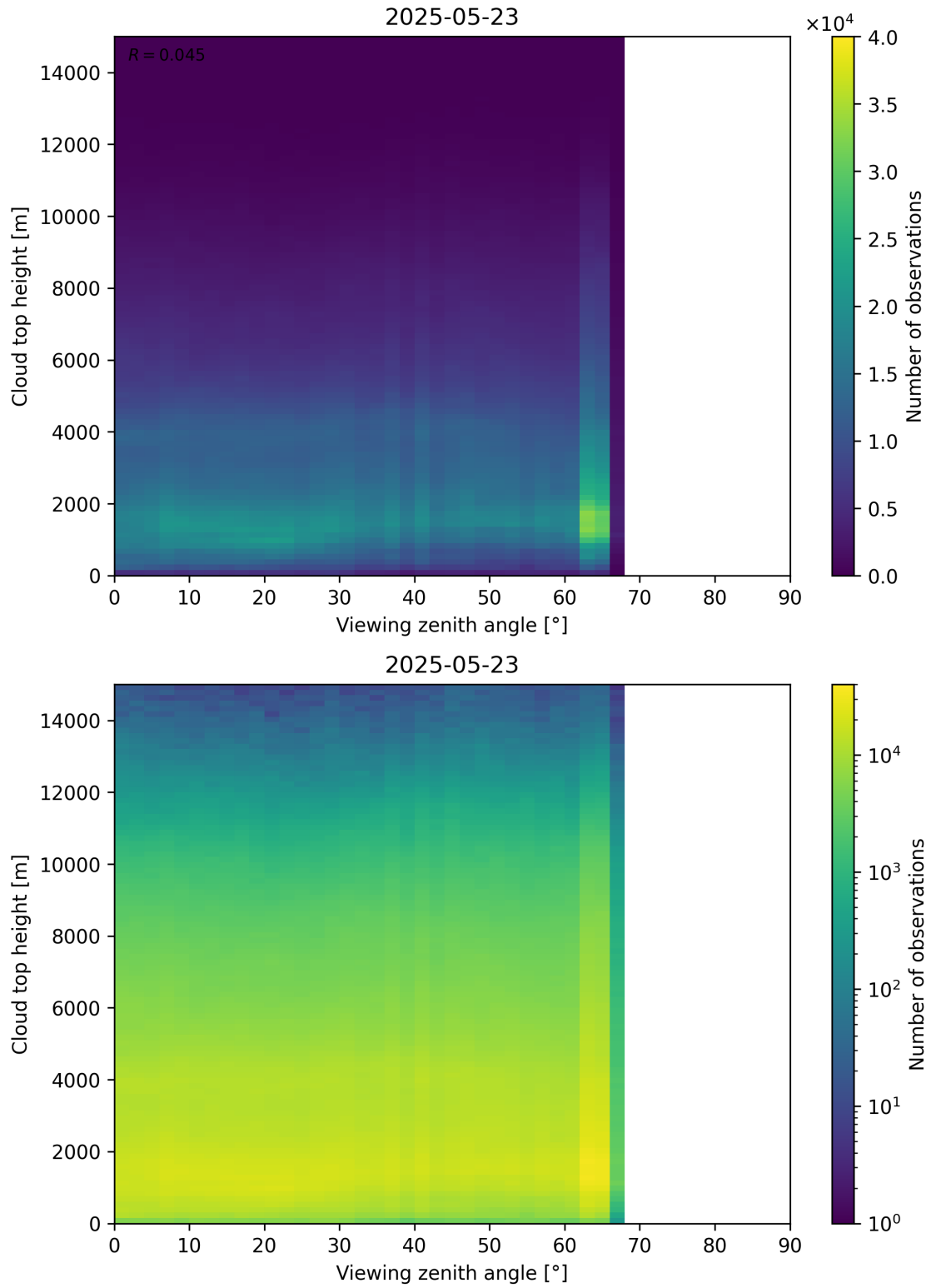
Figure 112: Scatter density plot of “Viewing zenith angle” against “Cloud top height” for 2025-05-22 to 2025-05-24.
