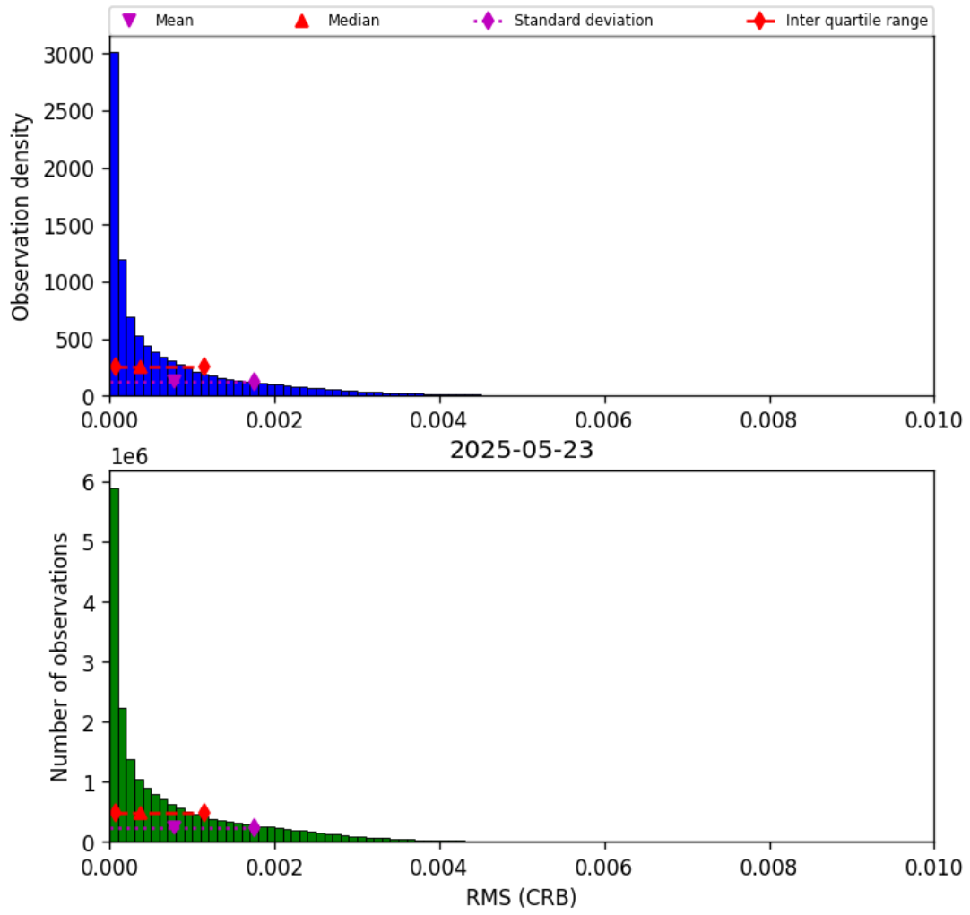
Figure 48: Histogram of “RMS (CRB)” for 2025-05-22 to 2025-05-24
