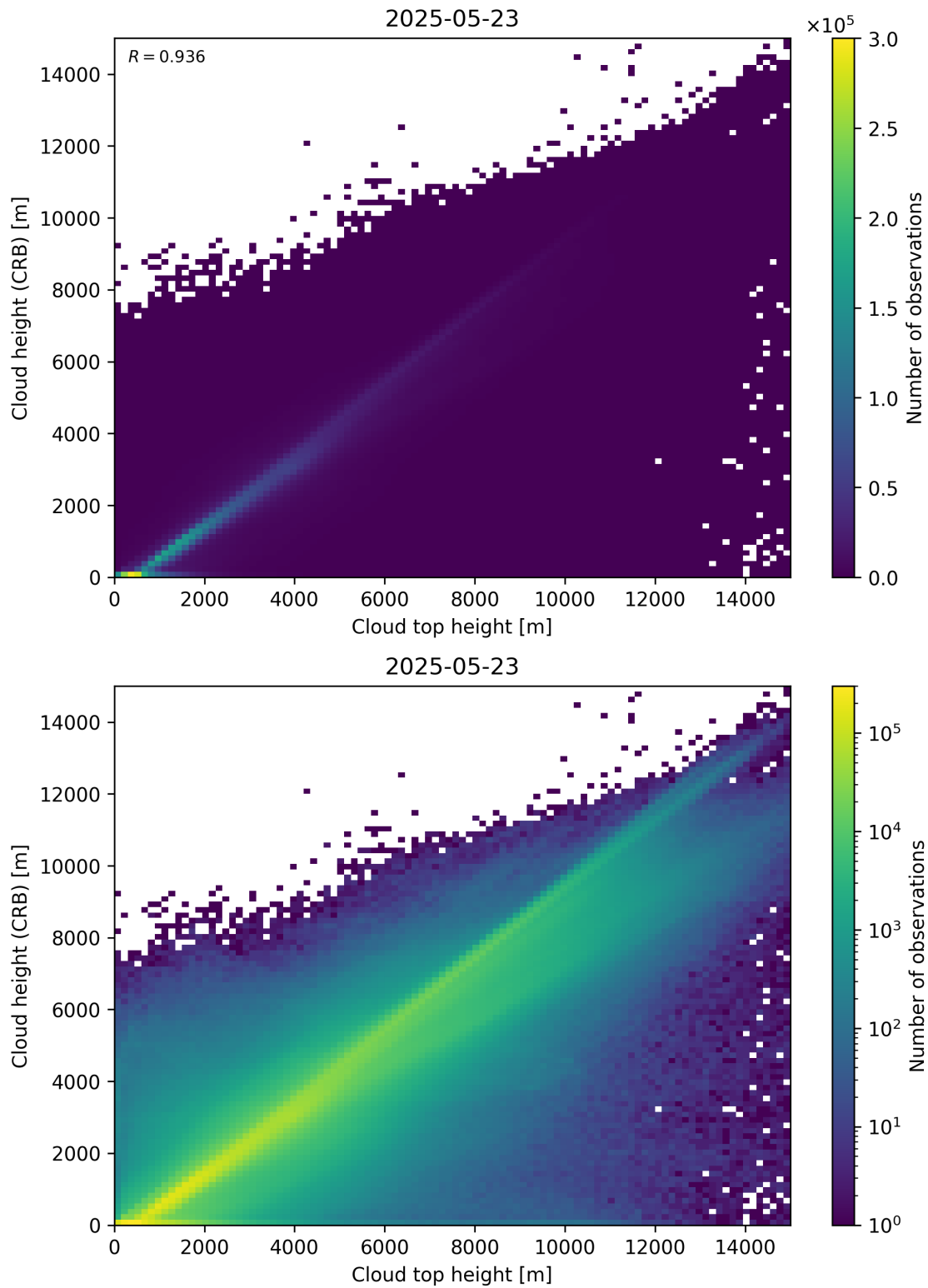
Figure 89: Scatter density plot of “Cloud top height” against “Cloud height (CRB)” for 2025-05-22 to 2025-05-24.
