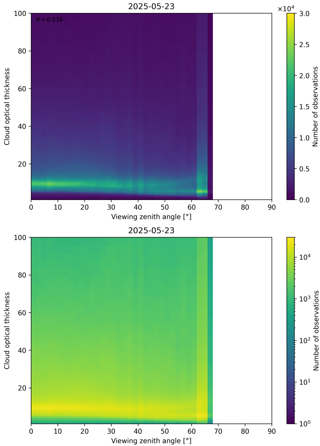
Figure 111: Scatter density plot of “Viewing zenith angle” against “Cloud optical thickness” for 2025-05-22 to 2025-05-24.
