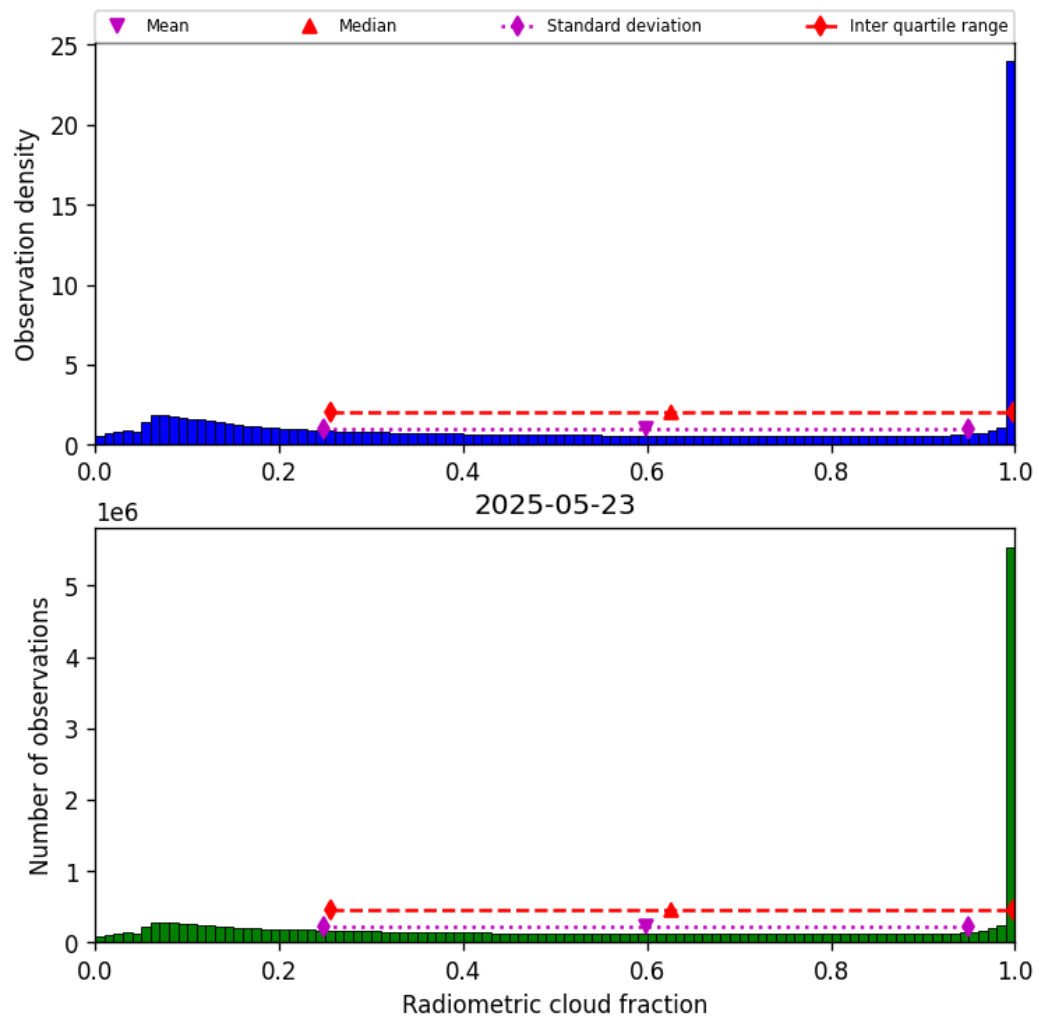
Figure 39: Histogram of “Radiometric cloud fraction” for 2025-05-22 to 2025-05-24
