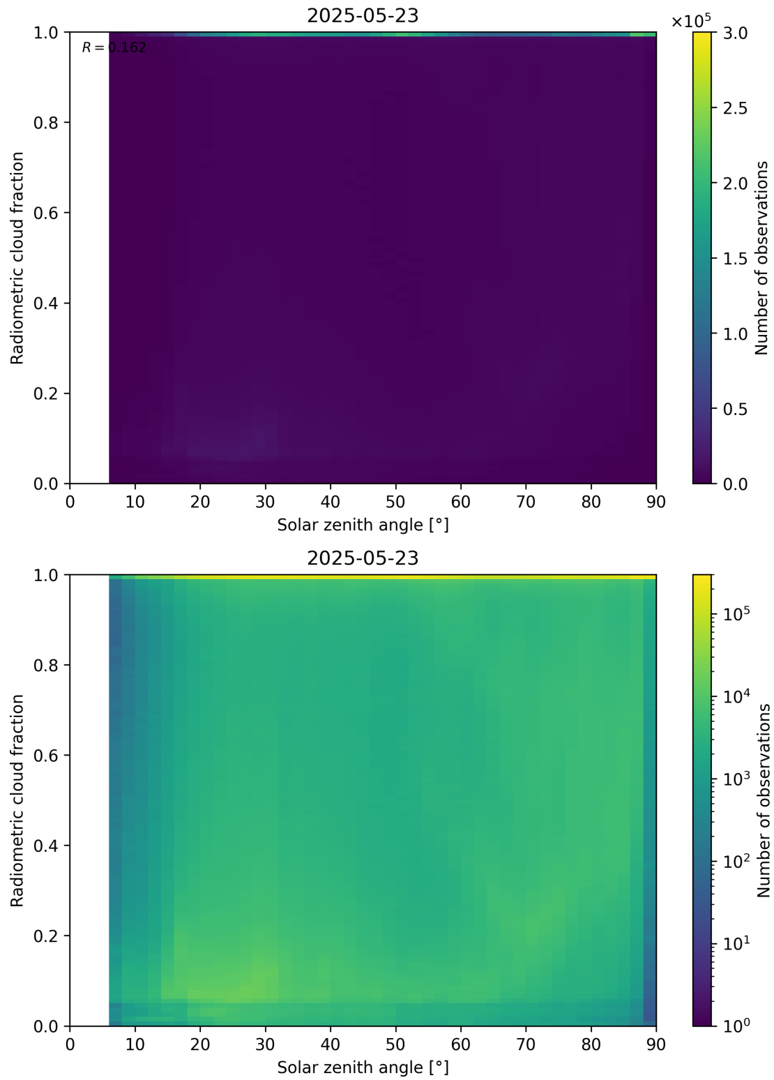
Figure 99: Scatter density plot of “Solar zenith angle” against “Radiometric cloud fraction” for 2025-05-22 to 2025-05-24.
