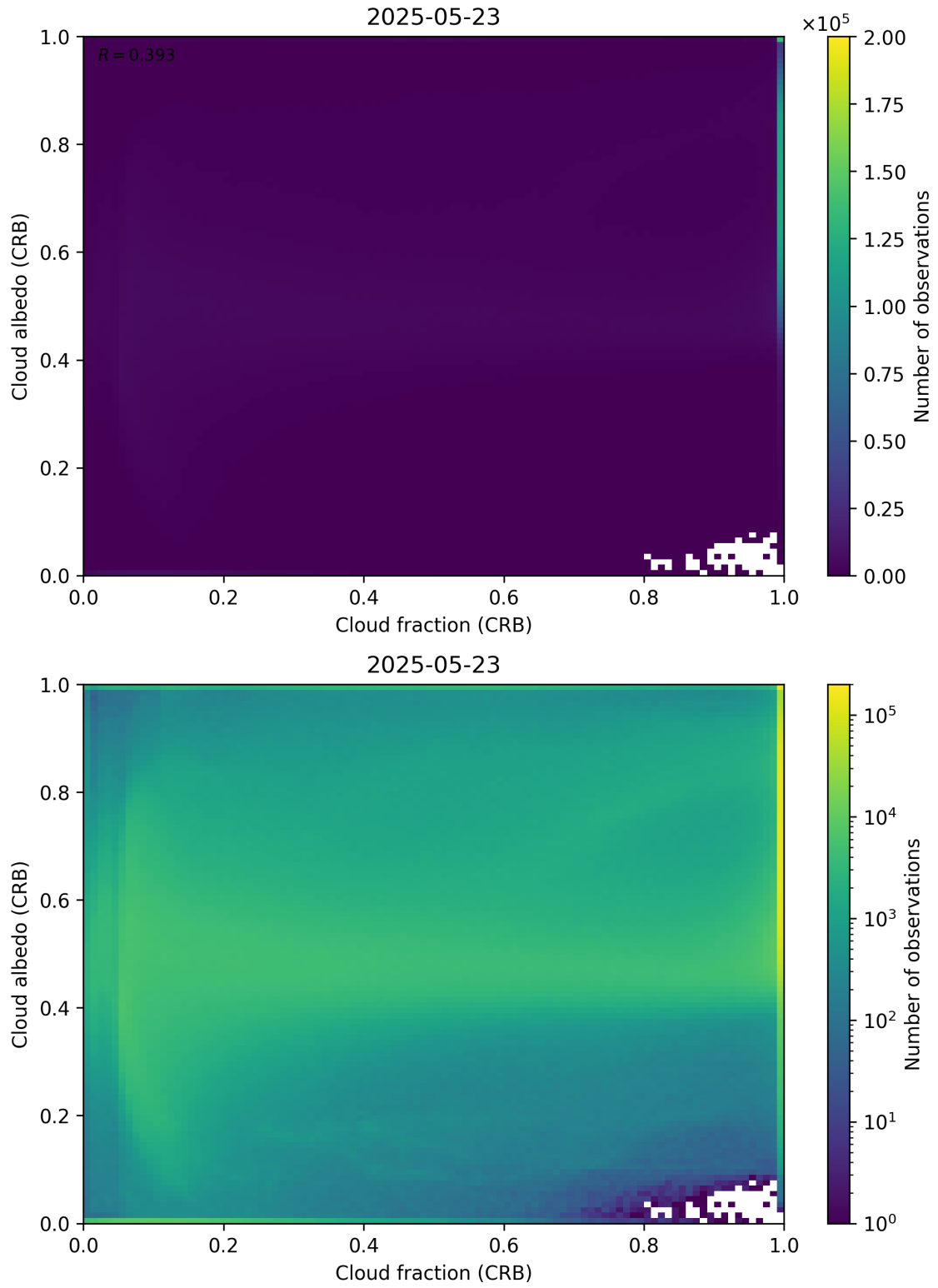
Figure 77: Scatter density plot of “Cloud fraction (CRB)” against “Cloud albedo (CRB)” for 2025-05-22 to 2025-05-24.
