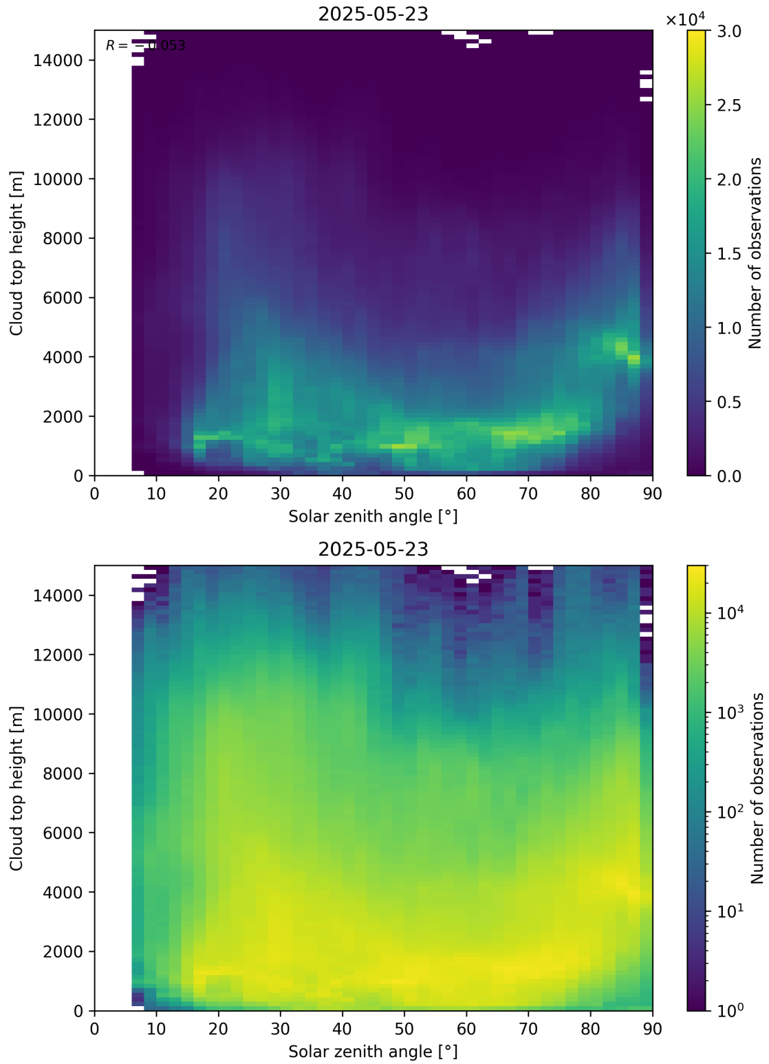
Figure 104: Scatter density plot of “Solar zenith angle” against “Cloud top height” for 2025-05-22 to 2025-05-24.
