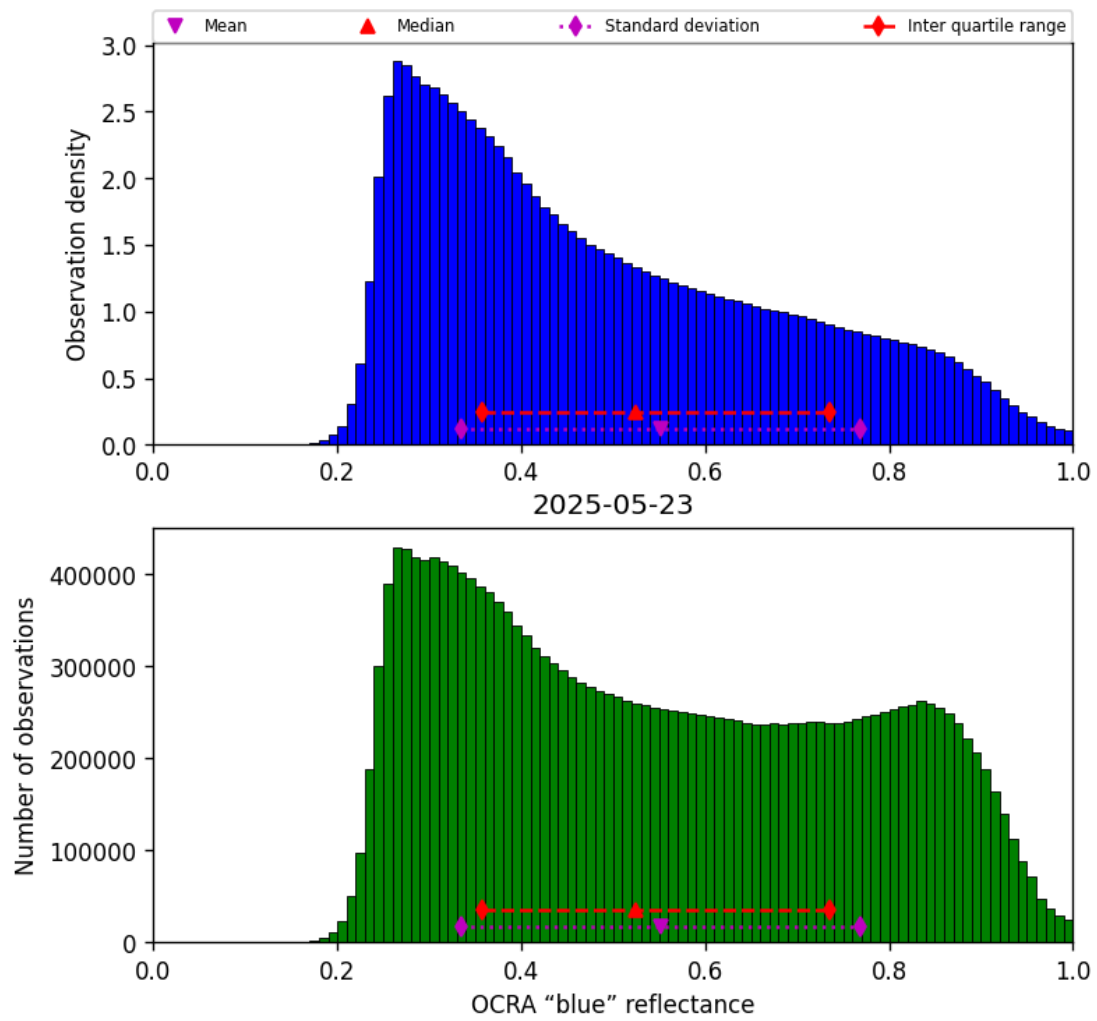
Figure 51: Histogram of “OCRA “blue” reflectance” for 2025-05-22 to 2025-05-24
