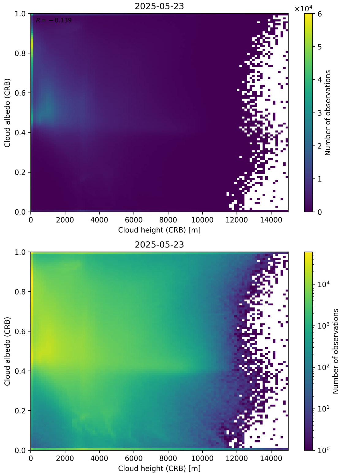
Figure 80: Scatter density plot of “Cloud height (CRB)” against “Cloud albedo (CRB)” for 2025-05-22 to 2025-05-24.
