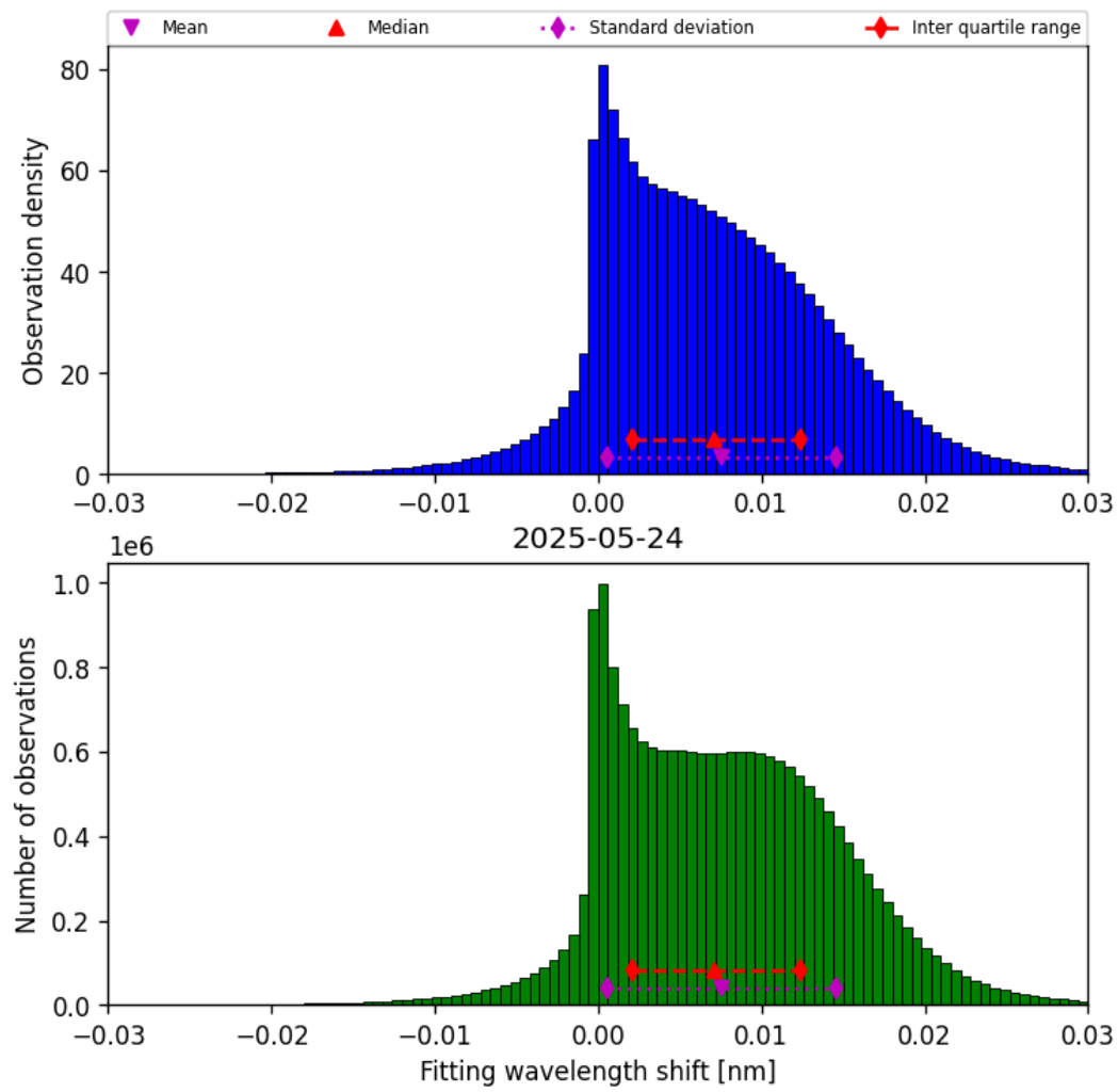
Figure 49: Histogram of “Fitting wavelength shift” for 2025-05-23 to 2025-05-25
