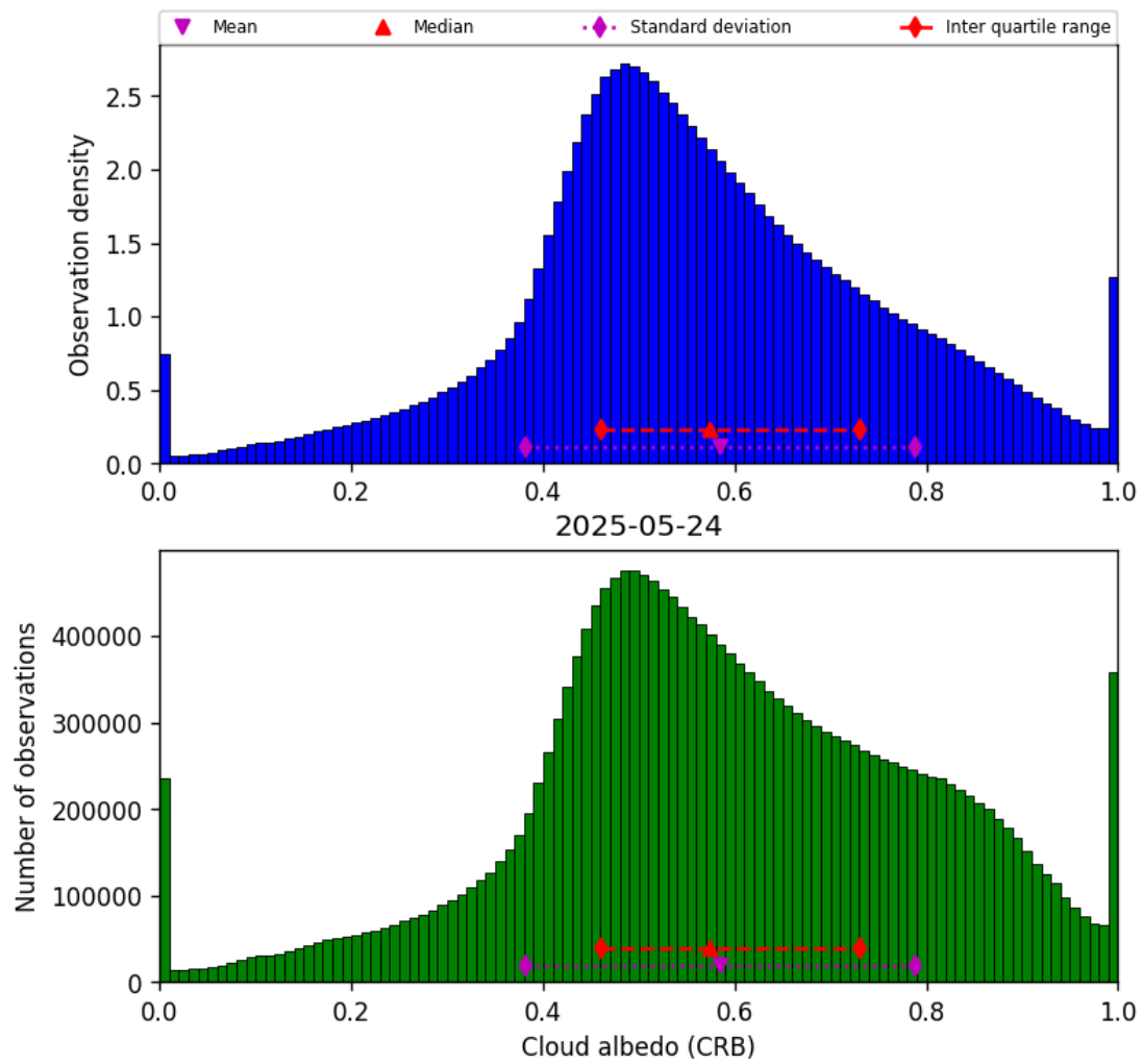
Figure 44: Histogram of “Cloud albedo (CRB)” for 2025-05-23 to 2025-05-25
