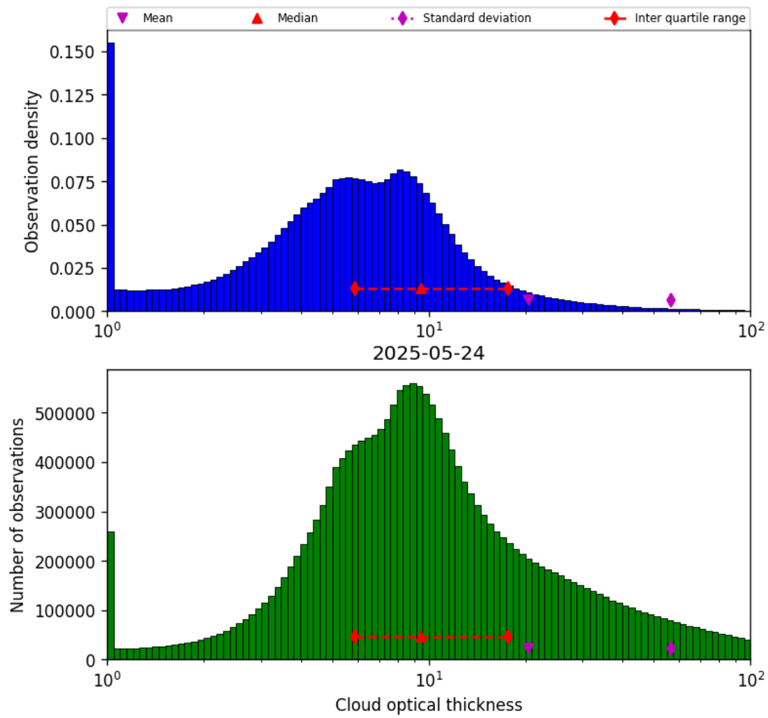
Figure 41: Histogram of “Cloud optical thickness” for 2025-05-23 to 2025-05-25
