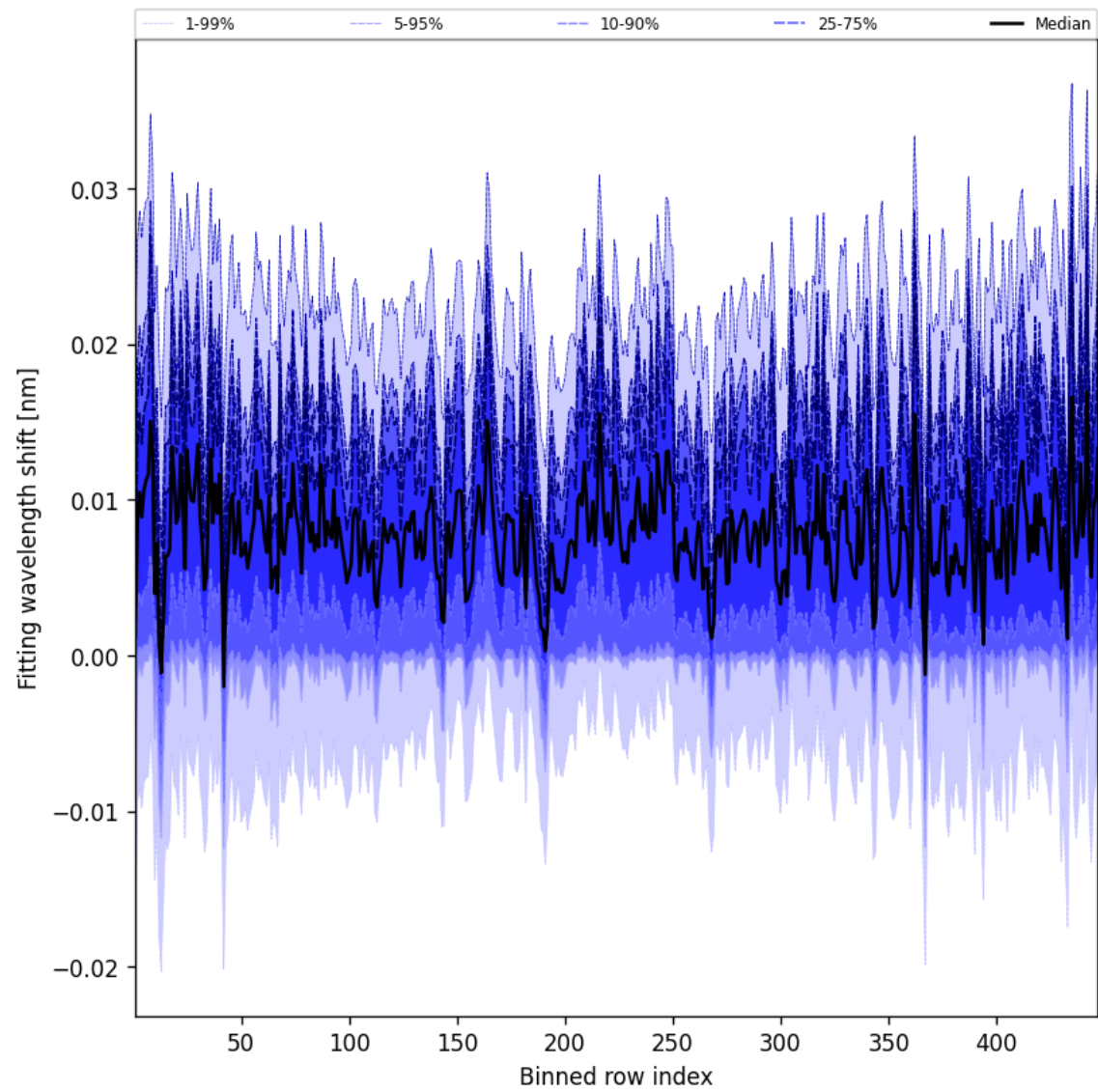
Figure 65: Along track statistics of “Fitting wavelength shift” for 2025-05-23 to 2025-05-25
