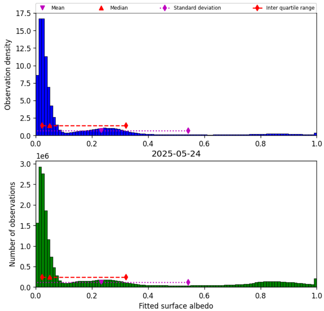
Figure 45: Histogram of “Fitted surface albedo” for 2025-05-23 to 2025-05-25
