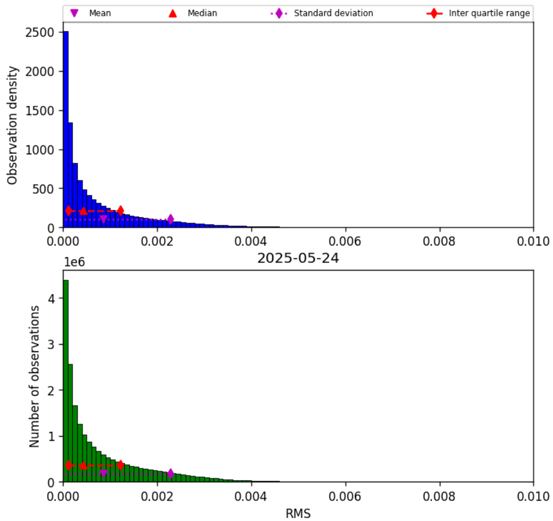
Figure 47: Histogram of “RMS” for 2025-05-23 to 2025-05-25
