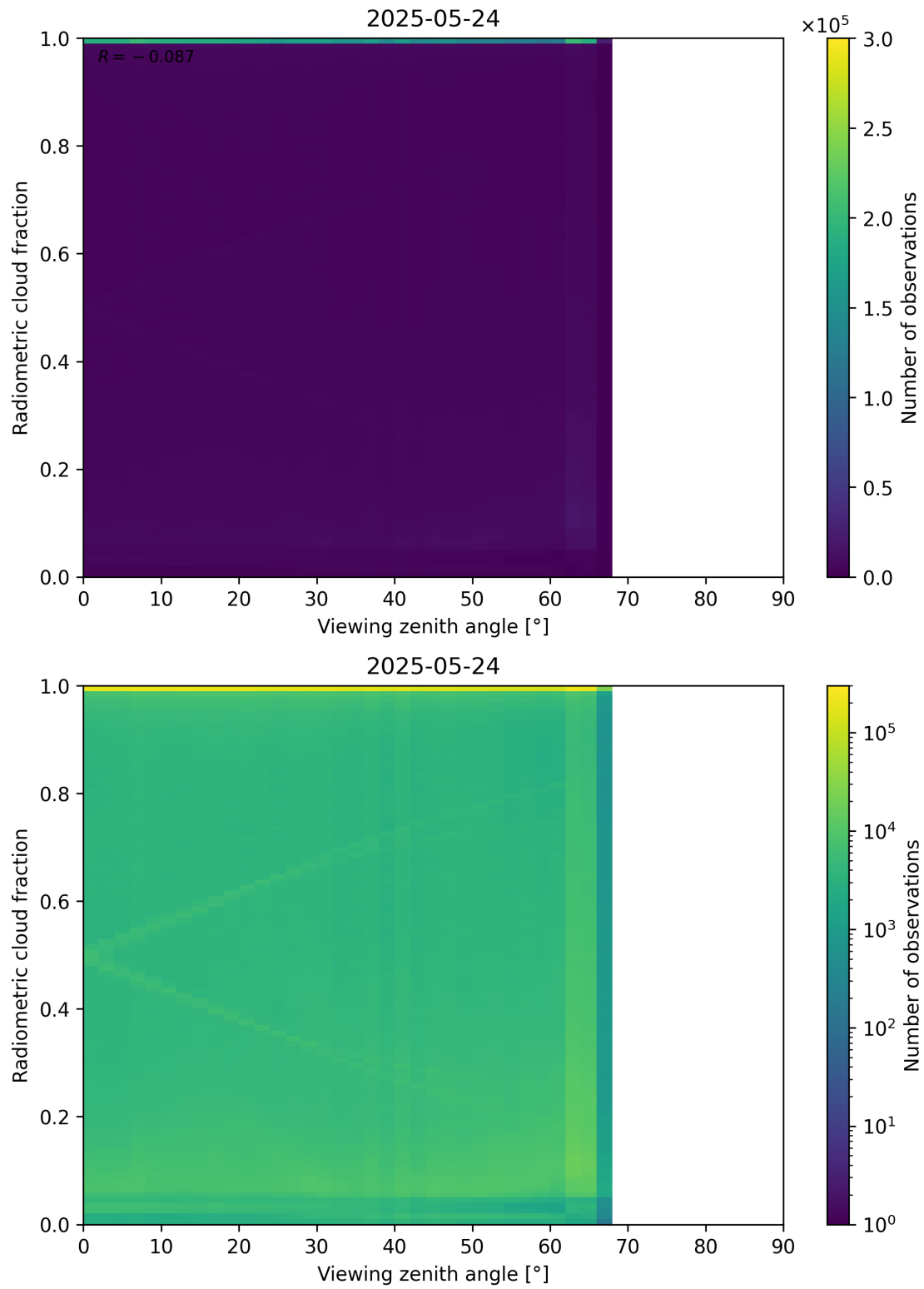
Figure 107: Scatter density plot of “Viewing zenith angle” against “Radiometric cloud fraction” for 2025-05-23 to 2025-05-25.
