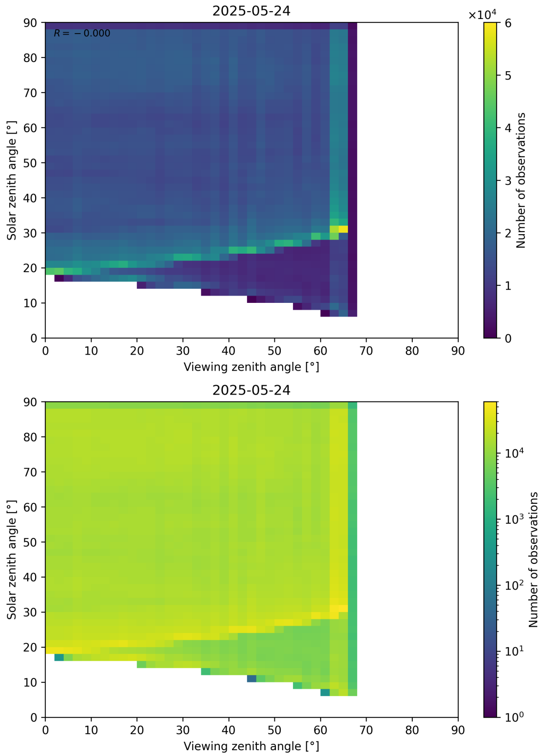
Figure 114: Scatter density plot of “Viewing zenith angle” against “Solar zenith angle” for 2025-05-23 to 2025-05-25.
