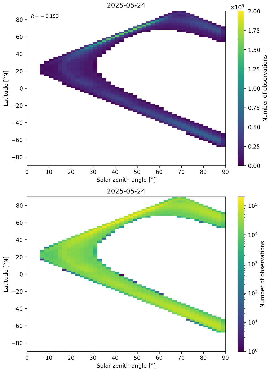
Figure 105: Scatter density plot of “Solar zenith angle” against “Latitude” for 2025-05-23 to 2025-05-25.
