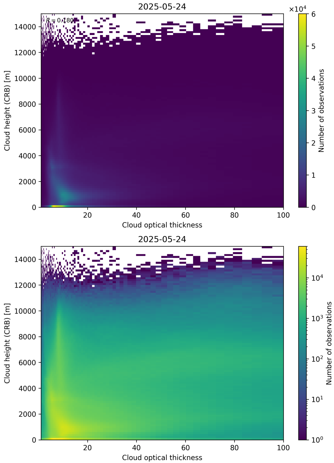
Figure 85: Scatter density plot of “Cloud optical thickness” against “Cloud height (CRB)” for 2025-05-23 to 2025-05-25.
