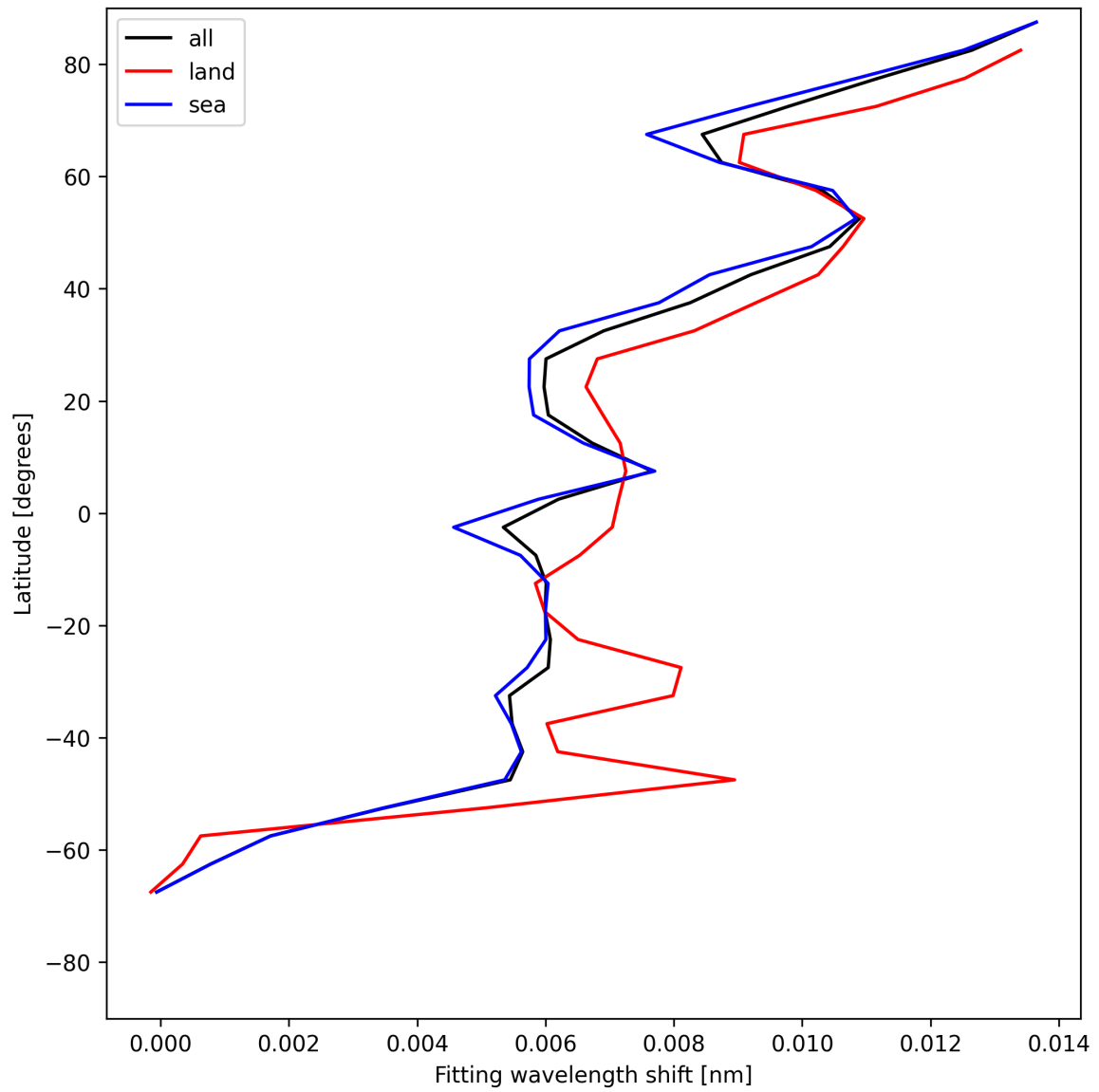
Figure 33: Zonal average of “Fitting wavelength shift” for 2025-05-23 to 2025-05-25.
