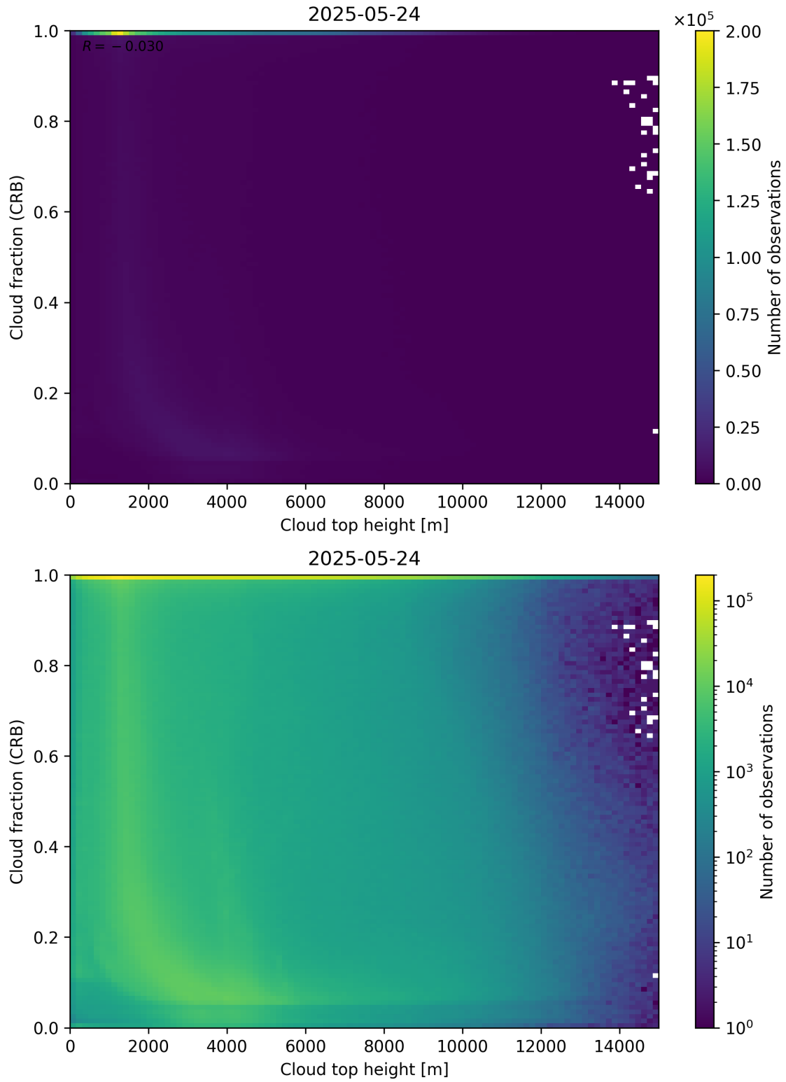
Figure 88: Scatter density plot of “Cloud top height” against “Cloud fraction (CRB)” for 2025-05-23 to 2025-05-25.
