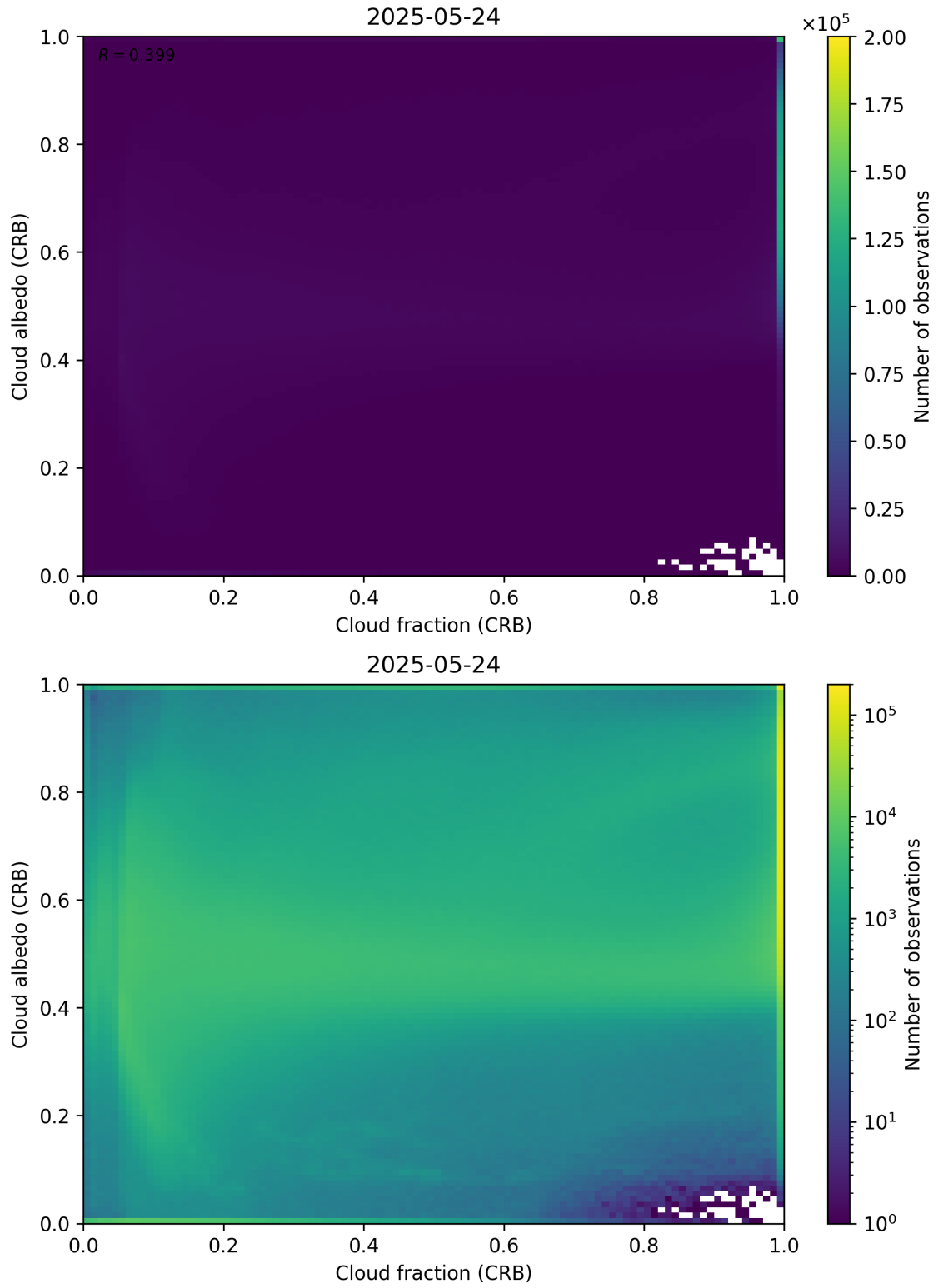
Figure 77: Scatter density plot of “Cloud fraction (CRB)” against “Cloud albedo (CRB)” for 2025-05-23 to 2025-05-25.
