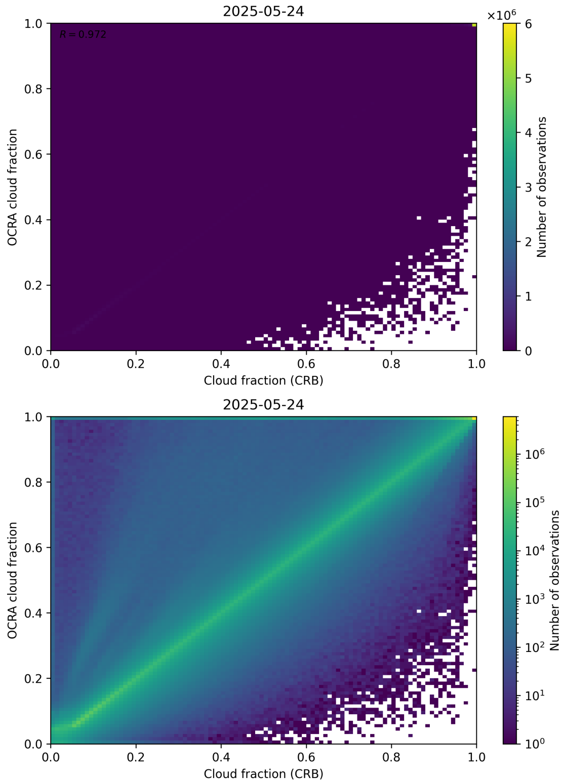
Figure 78: Scatter density plot of “Cloud fraction (CRB)” against “OCRA cloud fraction” for 2025-05-23 to 2025-05-25.
