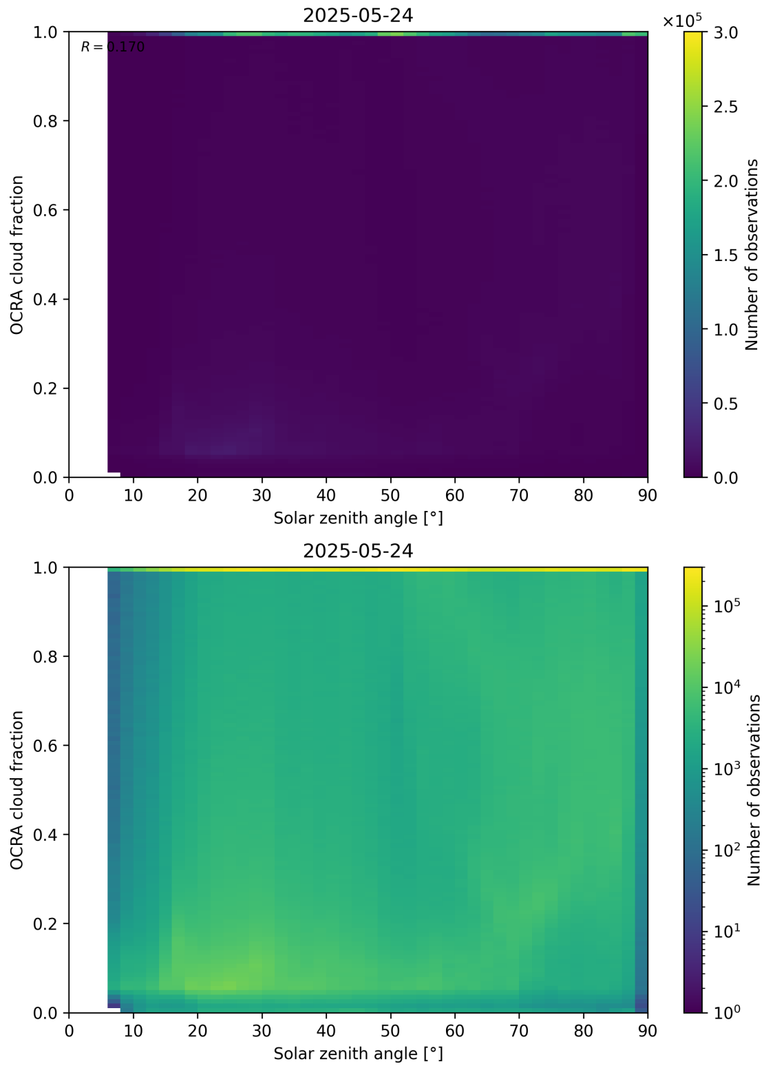
Figure 100: Scatter density plot of “Solar zenith angle” against “OCRA cloud fraction” for 2025-05-23 to 2025-05-25.
