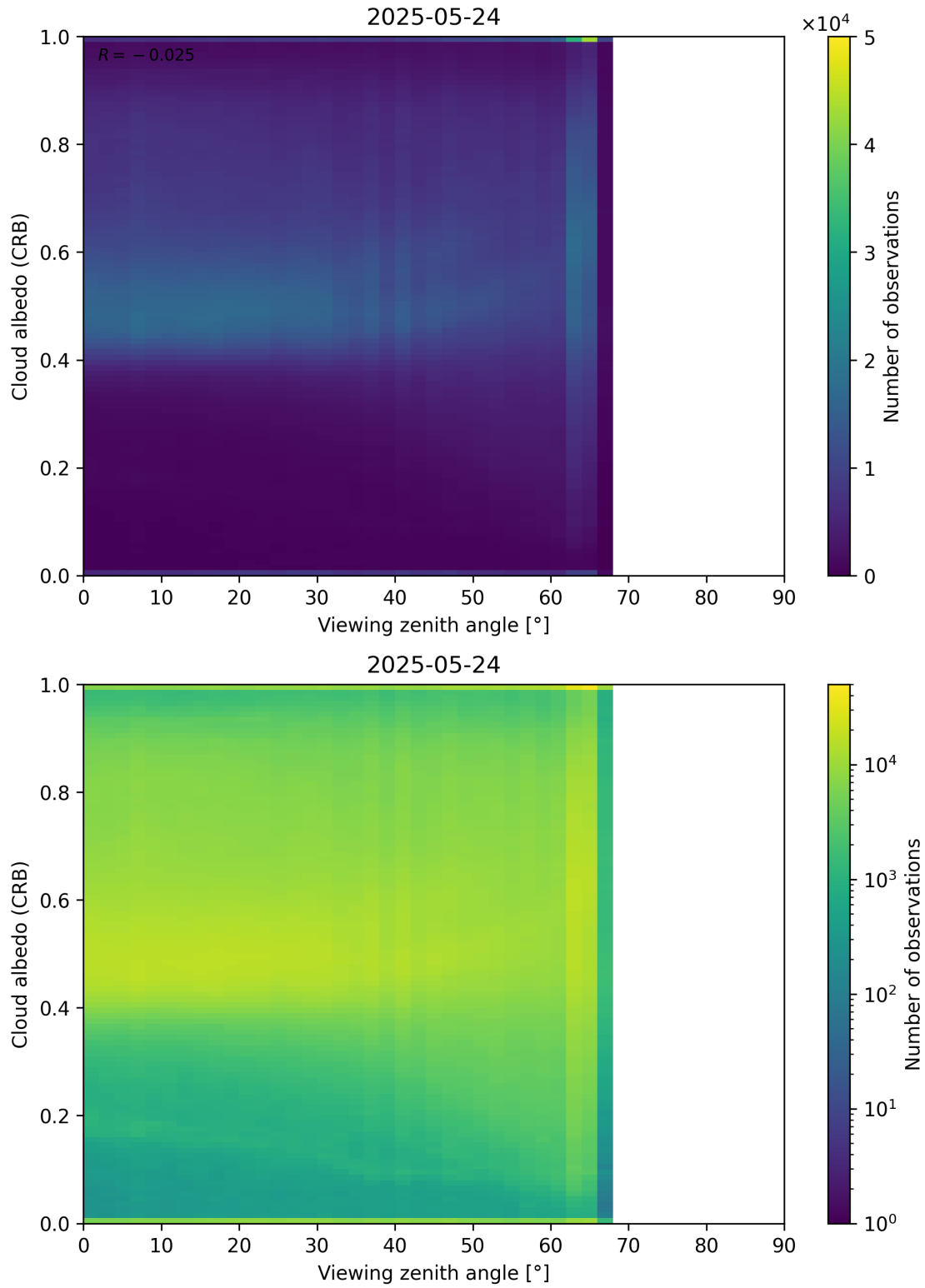
Figure 106: Scatter density plot of “Viewing zenith angle” against “Cloud albedo (CRB)” for 2025-05-23 to 2025-05-25.
