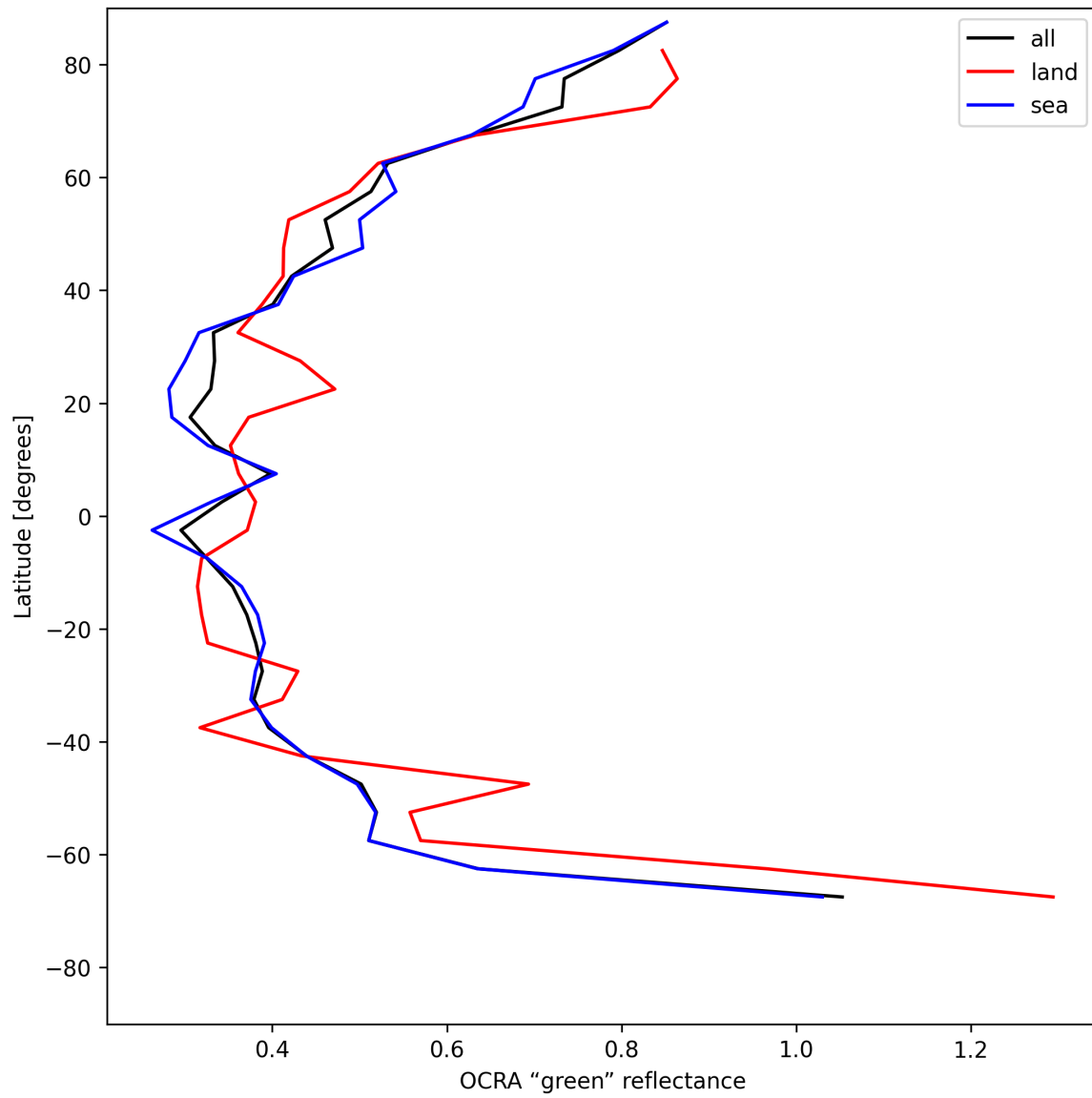
Figure 36: Zonal average of “OCRA “green” reflectance” for 2025-05-23 to 2025-05-25.
