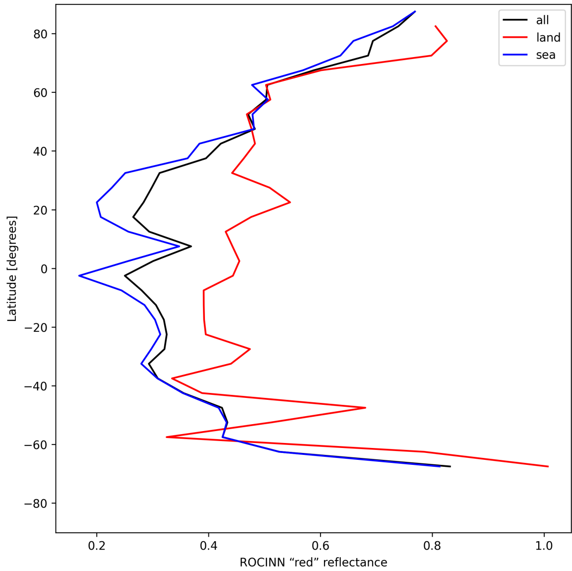
Figure 37: Zonal average of "ROCINN "red" reflectance" for 2025-05-23 to 2025-05-25.
