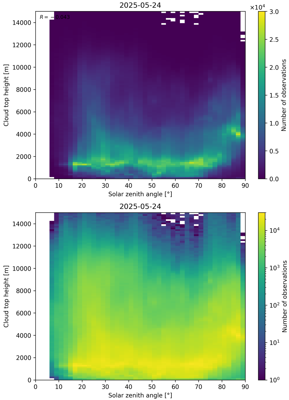
Figure 104: Scatter density plot of “Solar zenith angle” against “Cloud top height” for 2025-05-23 to 2025-05-25.
