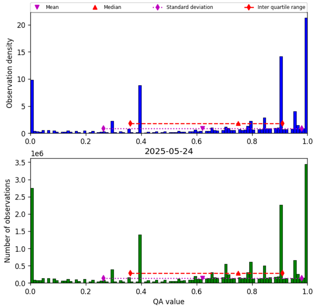
Figure 38: Histogram of “QA value” for 2025-05-23 to 2025-05-25
