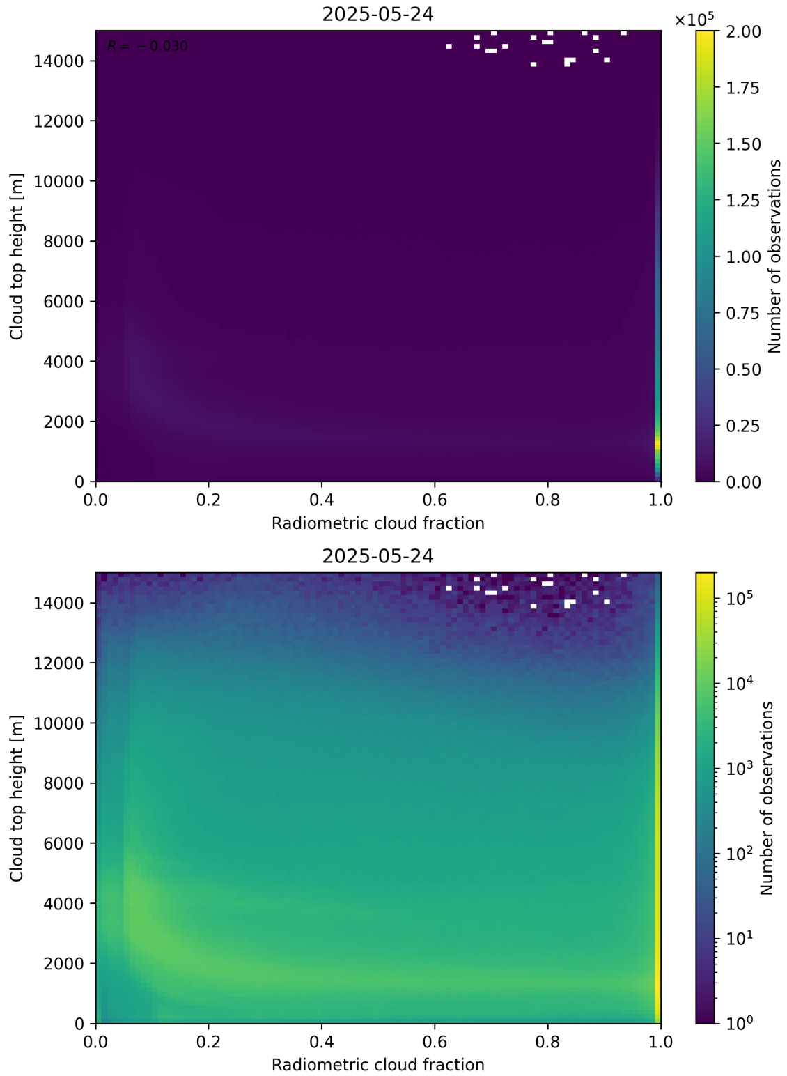
Figure 76: Scatter density plot of “Radiometric cloud fraction” against “Cloud top height” for 2025-05-23 to 2025-05-25.
