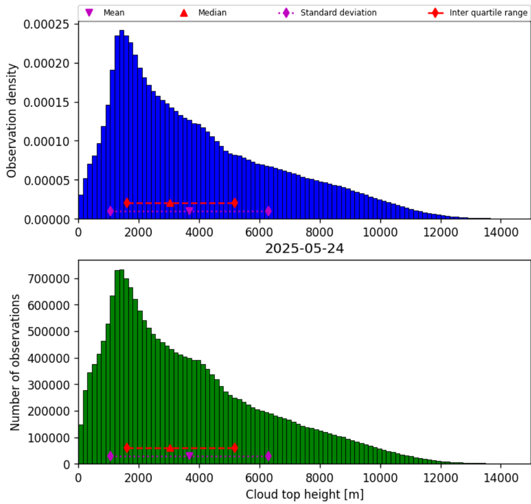
Figure 40: Histogram of “Cloud top height” for 2025-05-23 to 2025-05-25
