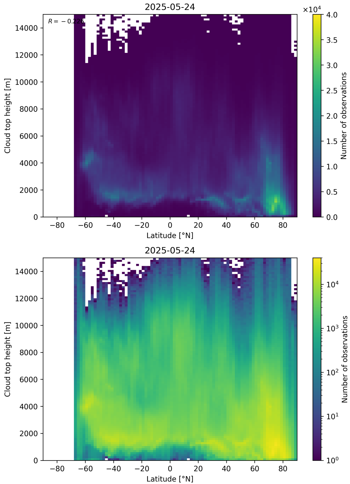
Figure 97: Scatter density plot of “Latitude” against “Cloud top height” for 2025-05-23 to 2025-05-25.
