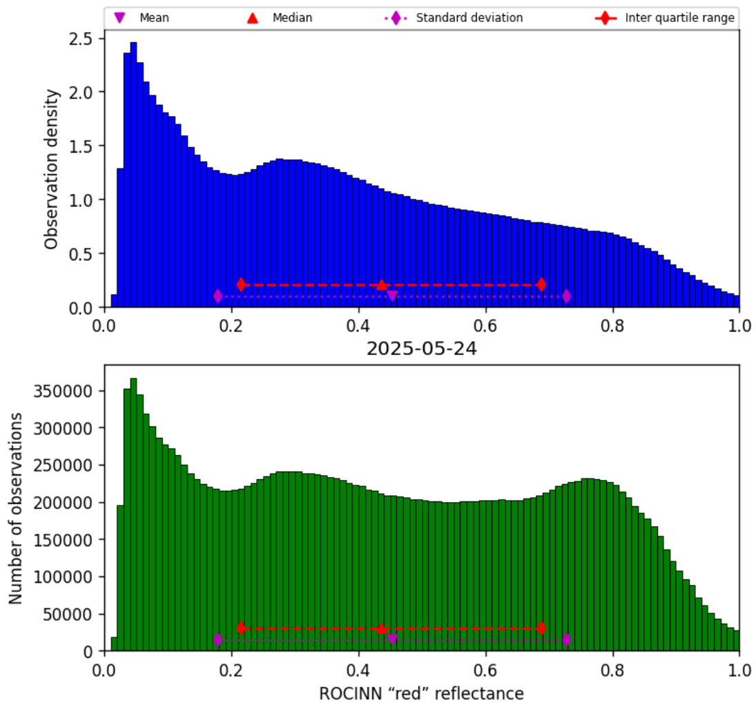
Figure 53: Histogram of “ROCINN “red” reflectance” for 2025-05-23 to 2025-05-25
