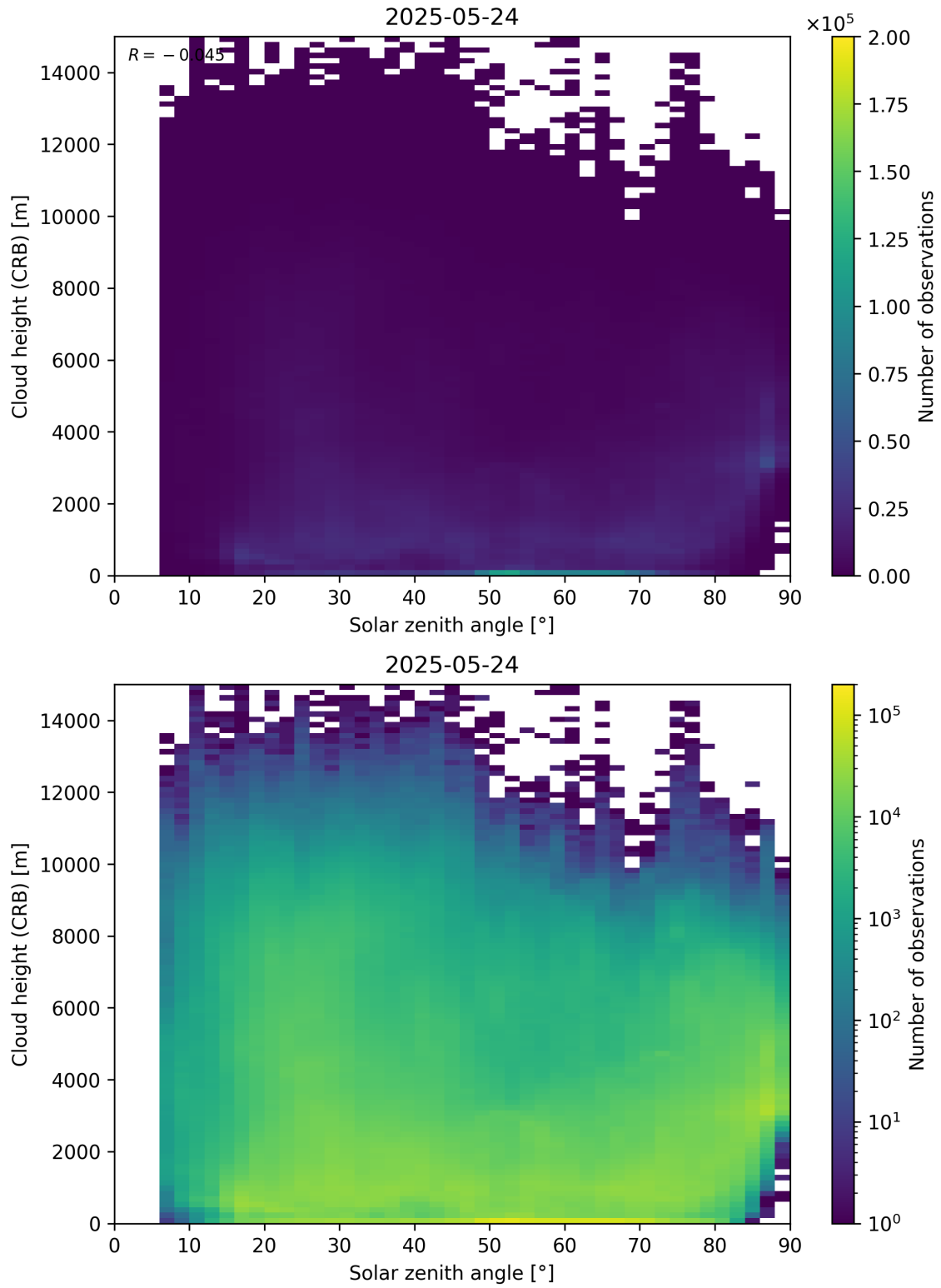
Figure 102: Scatter density plot of “Solar zenith angle” against “Cloud height (CRB)” for 2025-05-23 to 2025-05-25.
