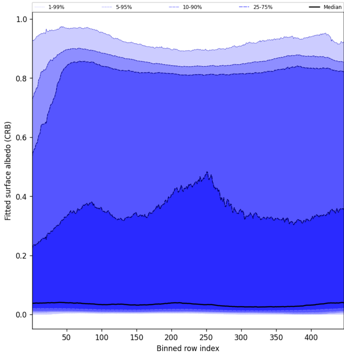
Figure 62: Along track statistics of “Fitted surface albedo (CRB)” for 2025-05-23 to 2025-05-25
