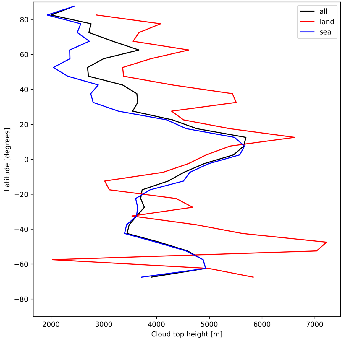
Figure 24: Zonal average of “Cloud top height” for 2025-05-23 to 2025-05-25.
