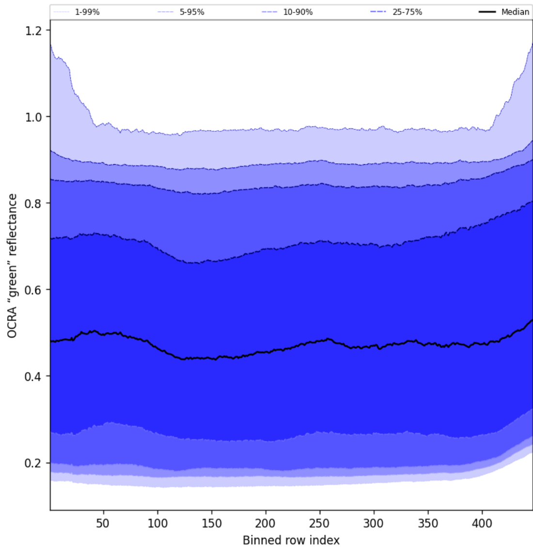
Figure 68: Along track statistics of “OCRA “green” reflectance” for 2025-05-23 to 2025-05-25
