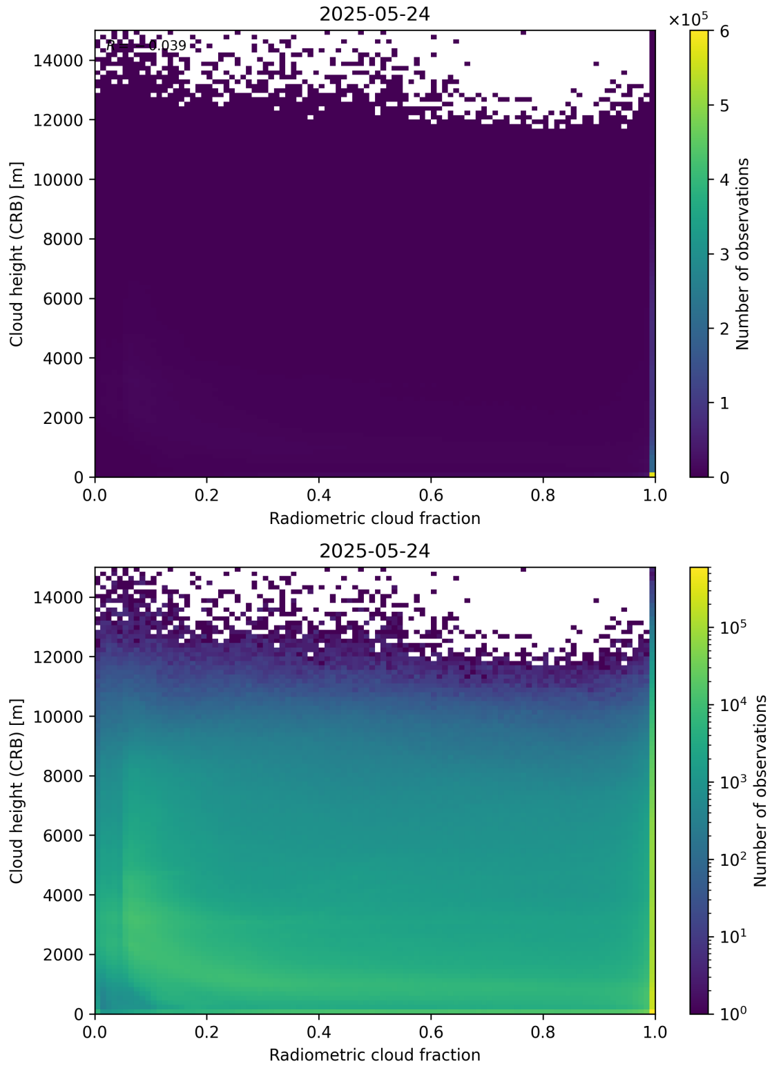
Figure 74: Scatter density plot of “Radiometric cloud fraction” against “Cloud height (CRB)” for 2025-05-23 to 2025-05-25.
