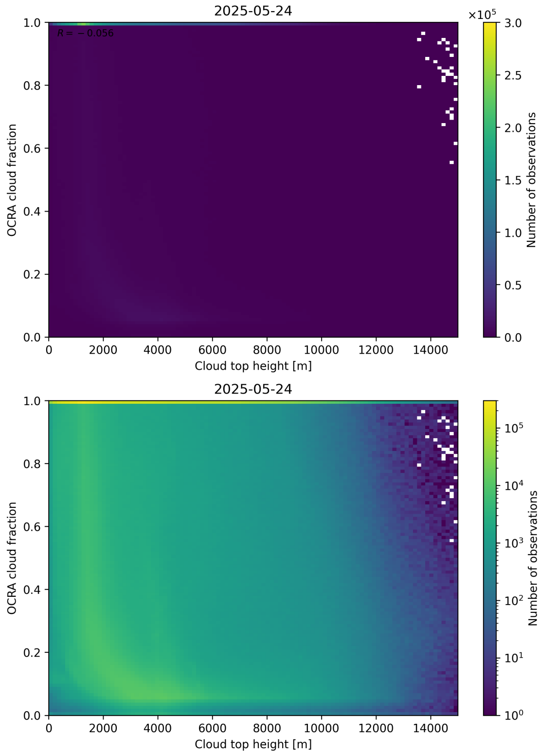
Figure 87: Scatter density plot of “Cloud top height” against “OCRA cloud fraction” for 2025-05-23 to 2025-05-25.
