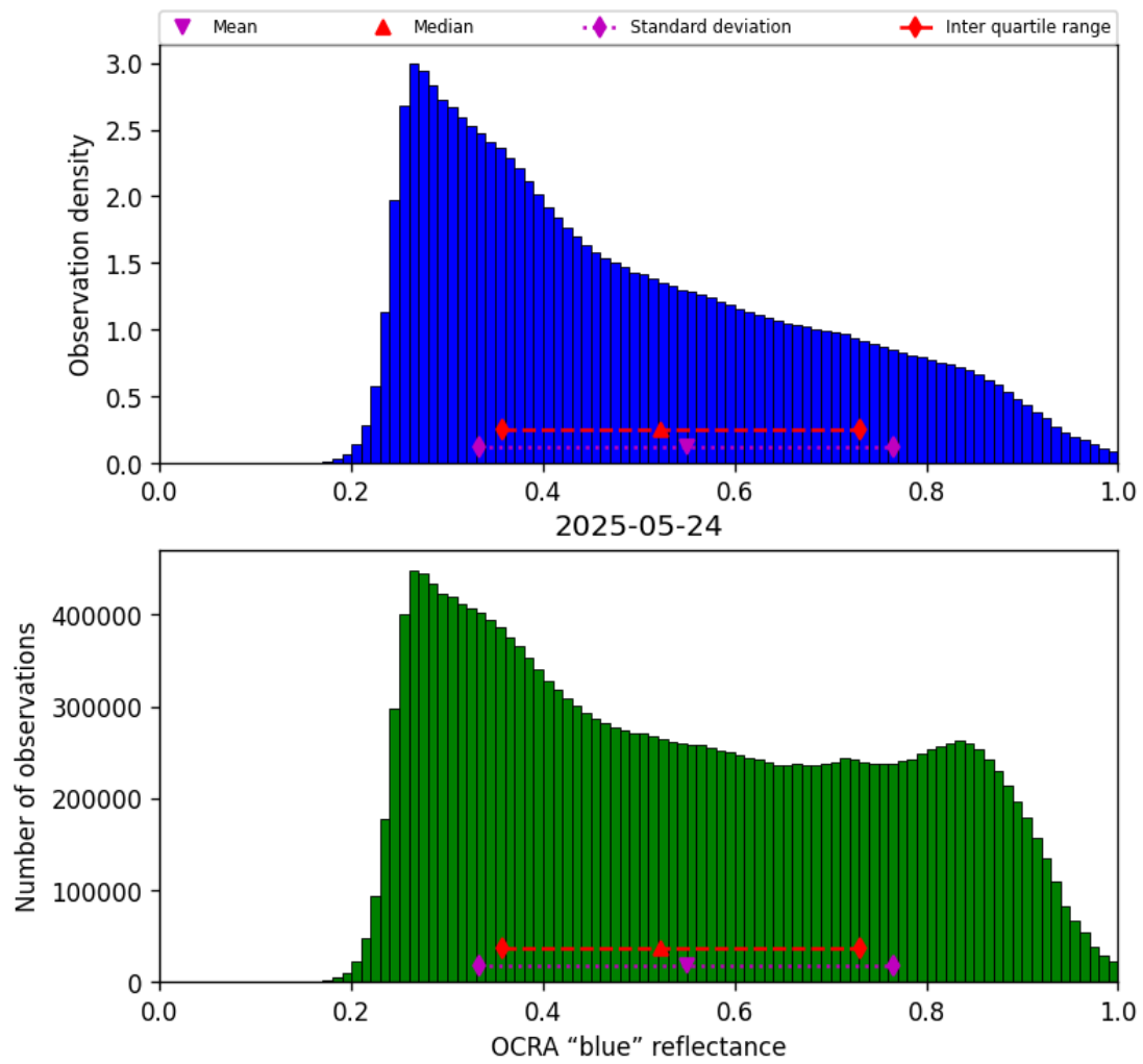
Figure 51: Histogram of “OCRA “blue” reflectance” for 2025-05-23 to 2025-05-25
