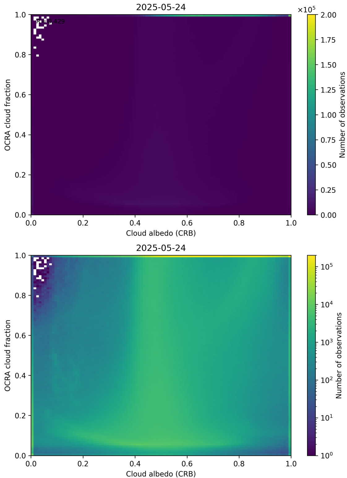
Figure 70: Scatter density plot of “Cloud albedo (CRB)” against “OCRA cloud fraction” for 2025-05-23 to 2025-05-25.
