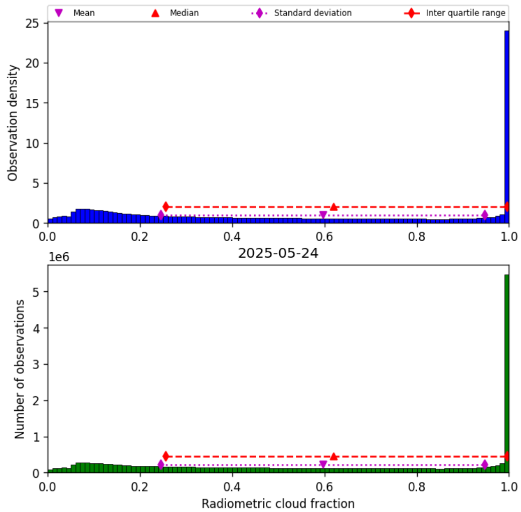
Figure 39: Histogram of “Radiometric cloud fraction” for 2025-05-23 to 2025-05-25
