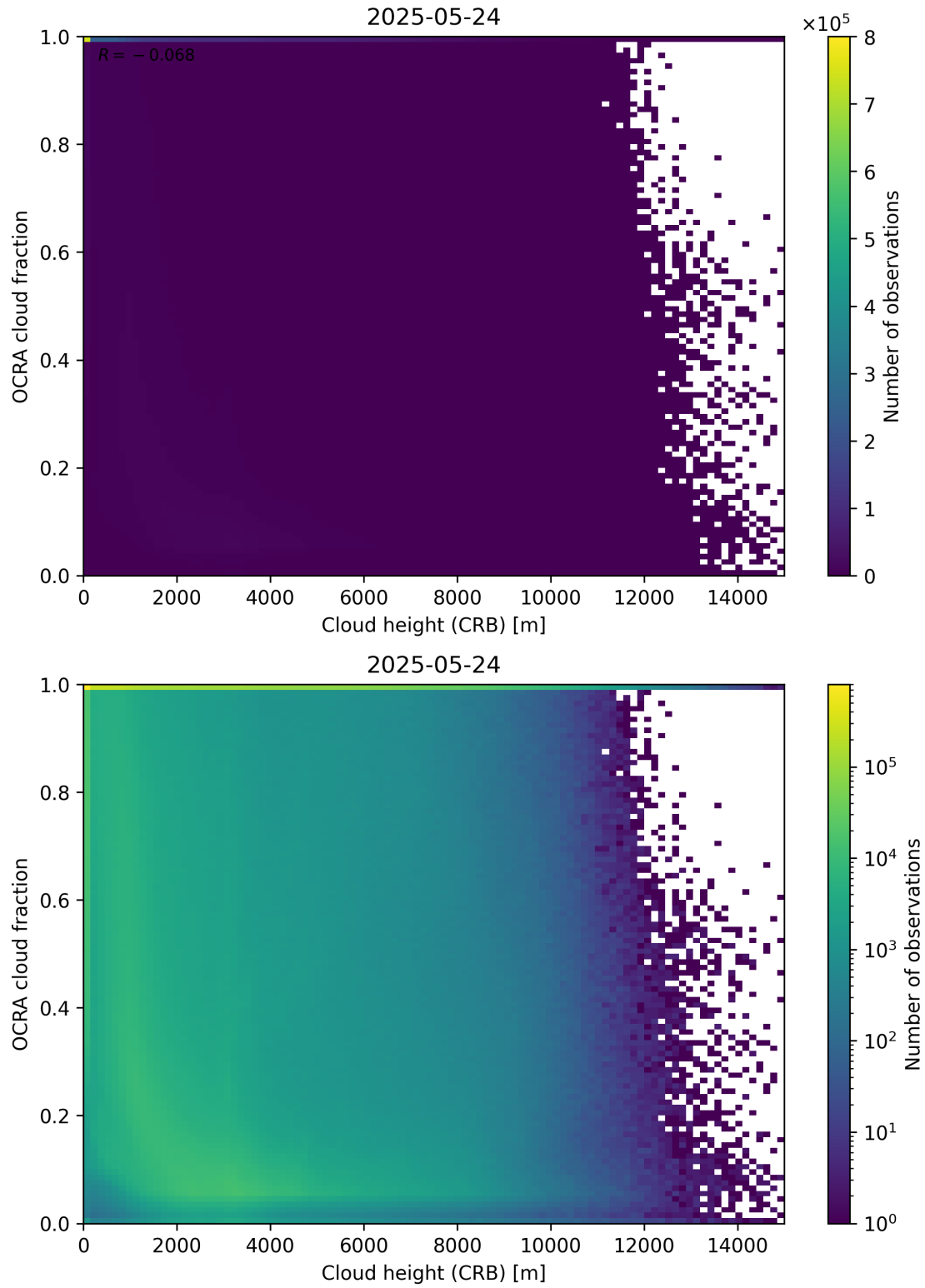
Figure 81: Scatter density plot of “Cloud height (CRB)” against “OCRA cloud fraction” for 2025-05-23 to 2025-05-25.
