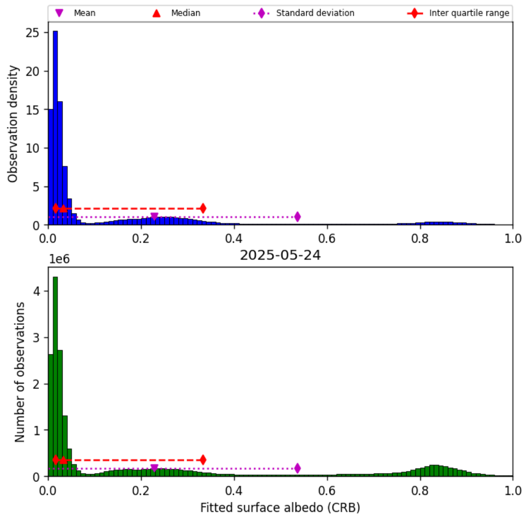
Figure 46: Histogram of “Fitted surface albedo (CRB)” for 2025-05-23 to 2025-05-25
