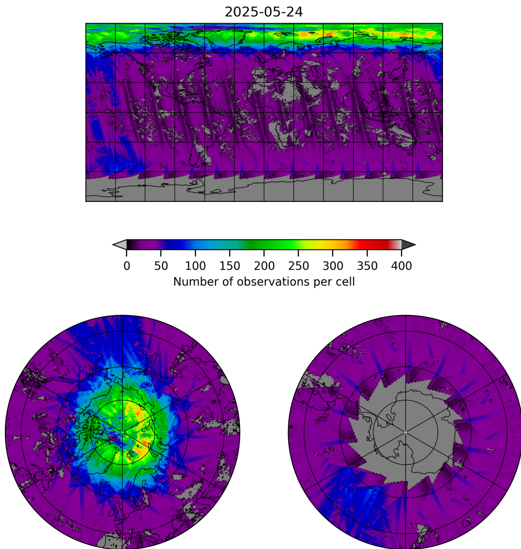
Figure 21: Map of the number of observations for 2025-05-23 to 2025-05-25
