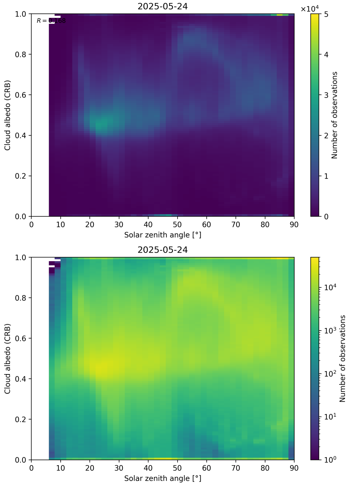
Figure 98: Scatter density plot of “Solar zenith angle” against “Cloud albedo (CRB)” for 2025-05-23 to 2025-05-25.
