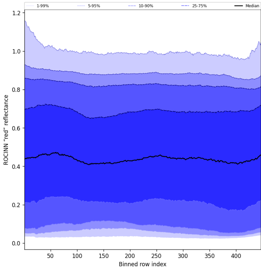
Figure 69: Along track statistics of “ROCINN “red” reflectance” for 2025-05-23 to 2025-05-25
