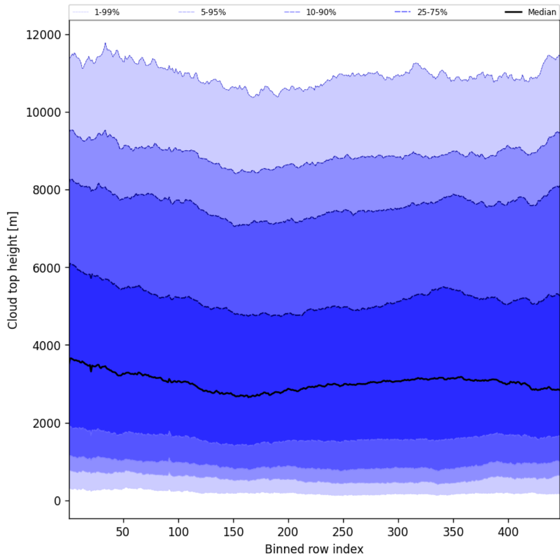
Figure 56: Along track statistics of “Cloud top height” for 2025-05-23 to 2025-05-25
