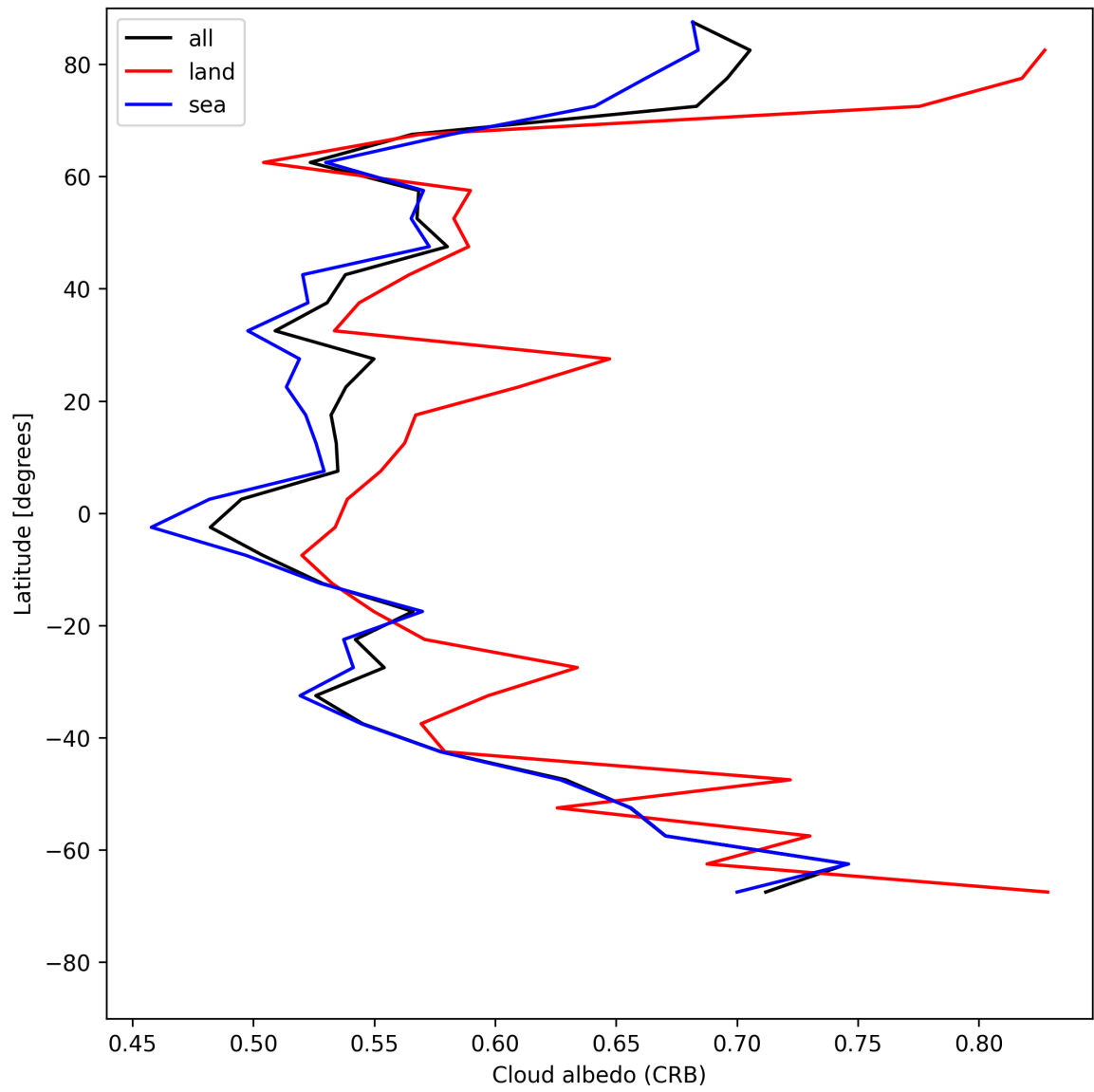
Figure 28: Zonal average of “Cloud albedo (CRB)” for 2025-05-23 to 2025-05-25.
