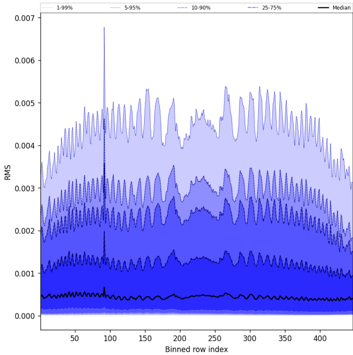
Figure 63: Along track statistics of “RMS” for 2025-05-23 to 2025-05-25
