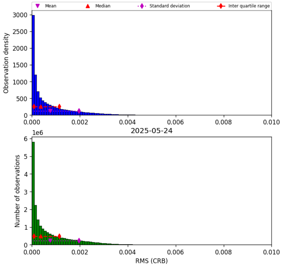
Figure 48: Histogram of “RMS (CRB)” for 2025-05-23 to 2025-05-25
