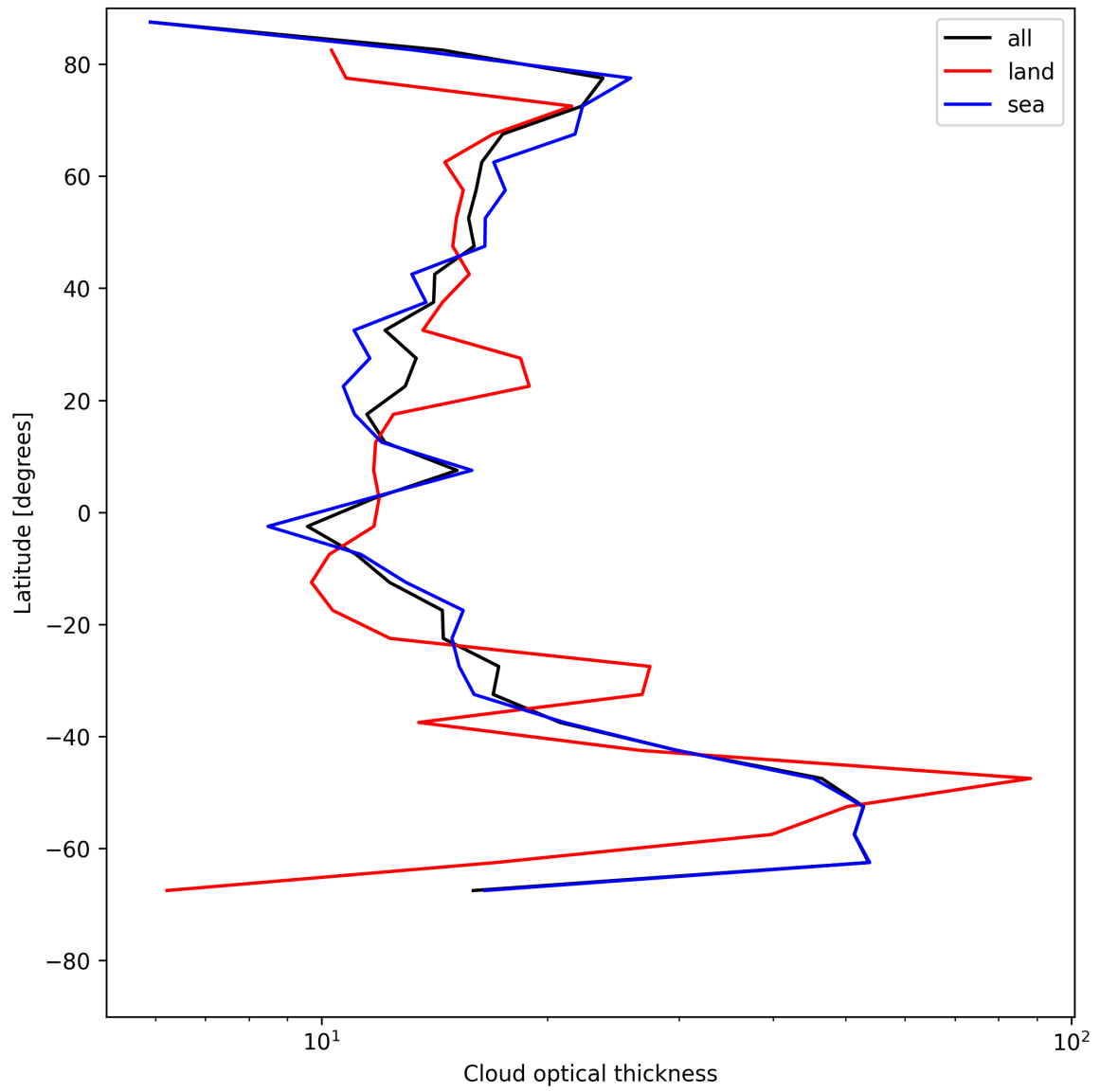
Figure 25: Zonal average of “Cloud optical thickness” for 2025-05-23 to 2025-05-25.
