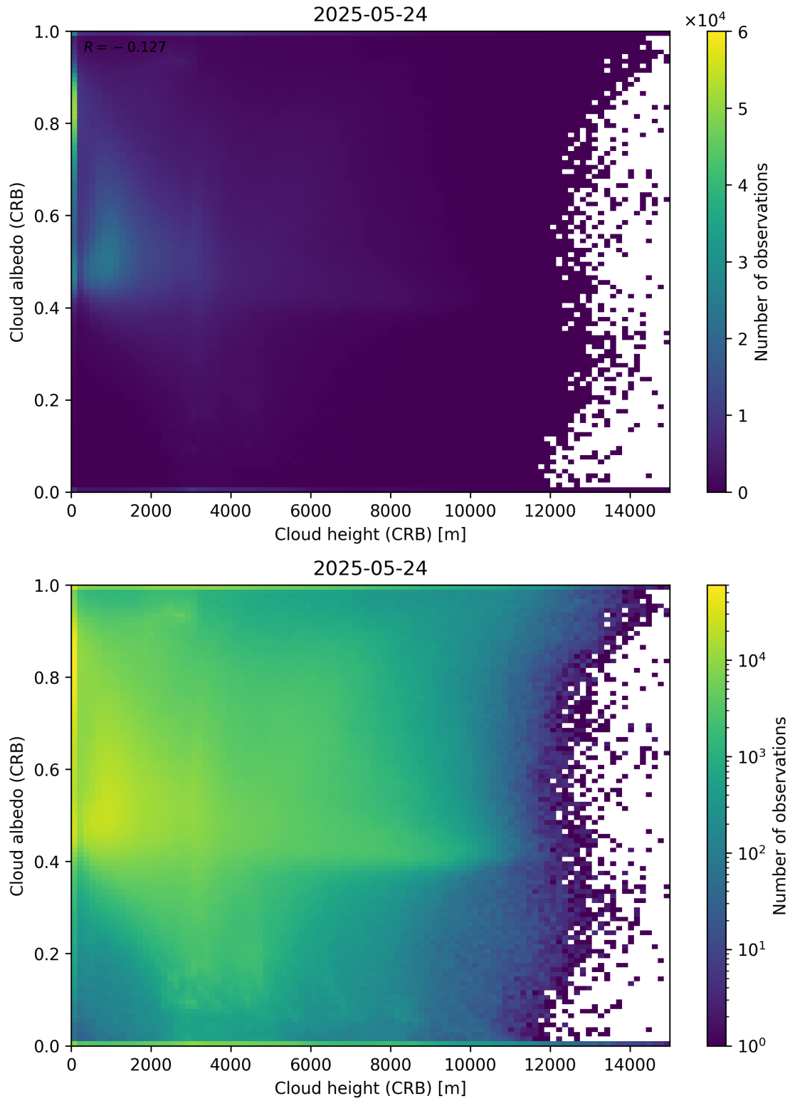
Figure 80: Scatter density plot of “Cloud height (CRB)” against “Cloud albedo (CRB)” for 2025-05-23 to 2025-05-25.
