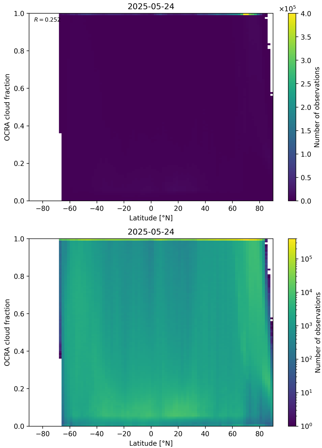
Figure 93: Scatter density plot of “Latitude” against “OCRA cloud fraction” for 2025-05-23 to 2025-05-25.
