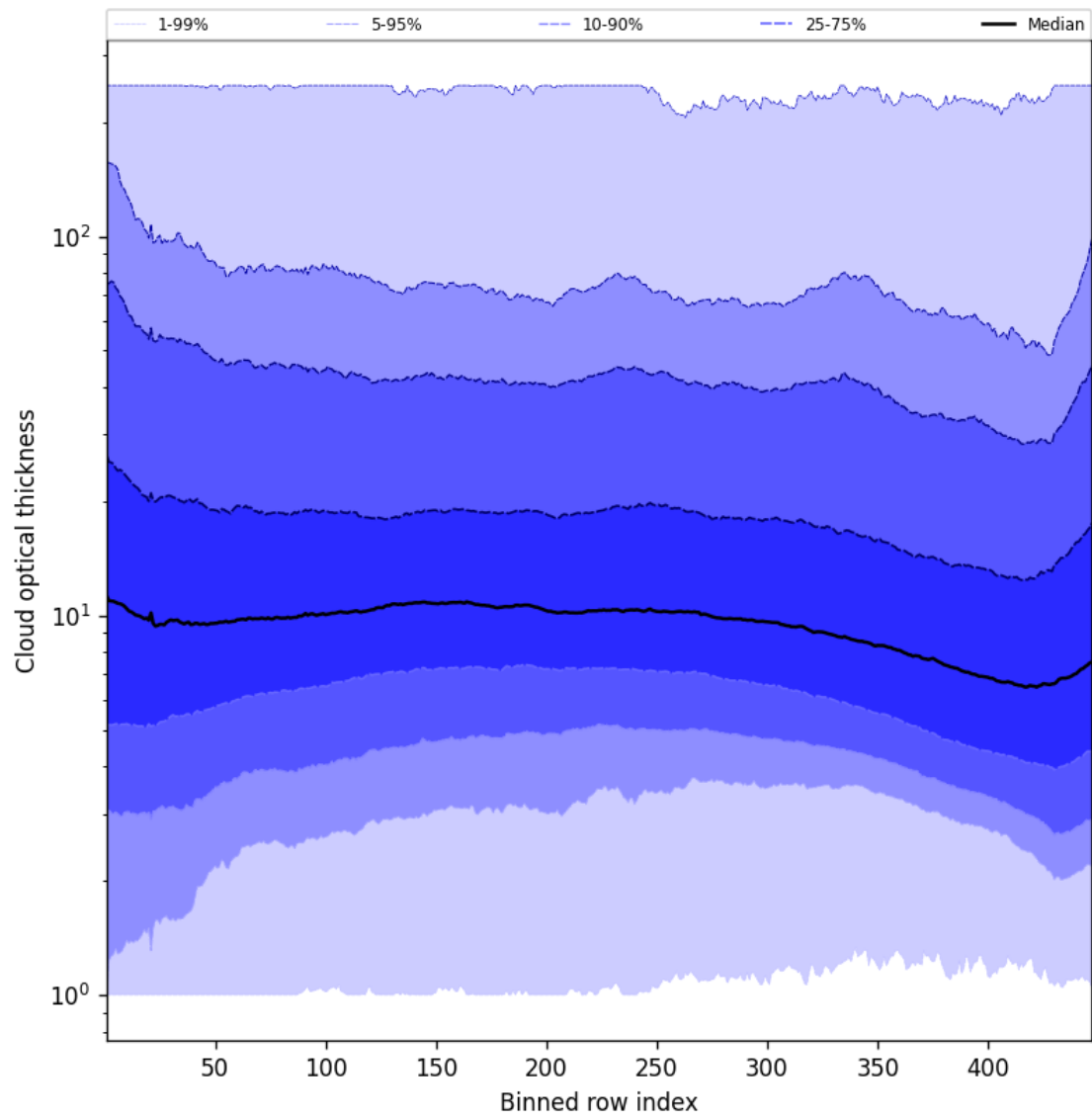
Figure 57: Along track statistics of “Cloud optical thickness” for 2025-05-23 to 2025-05-25
