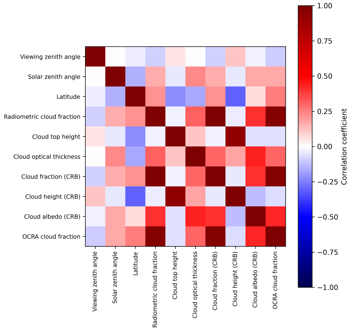
Figure 2: Map of correlation matrix for 2025-05-23 to 2025-05-25.
