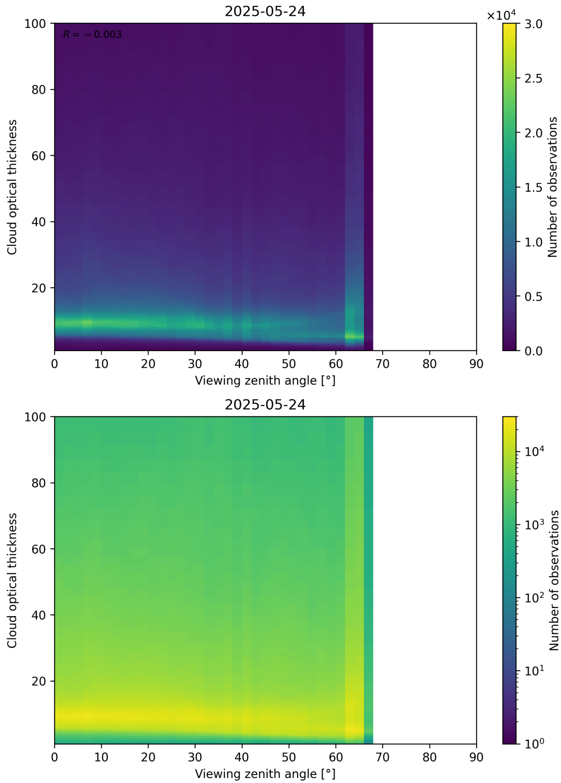
Figure 111: Scatter density plot of “Viewing zenith angle” against “Cloud optical thickness” for 2025-05-23 to 2025-05-25.
