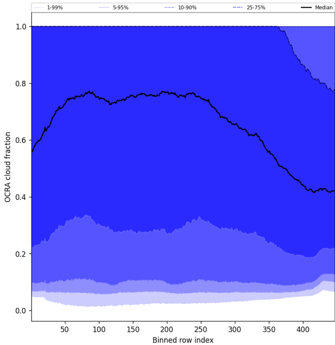
Figure 66: Along track statistics of “OCRA cloud fraction” for 2025-05-23 to 2025-05-25
