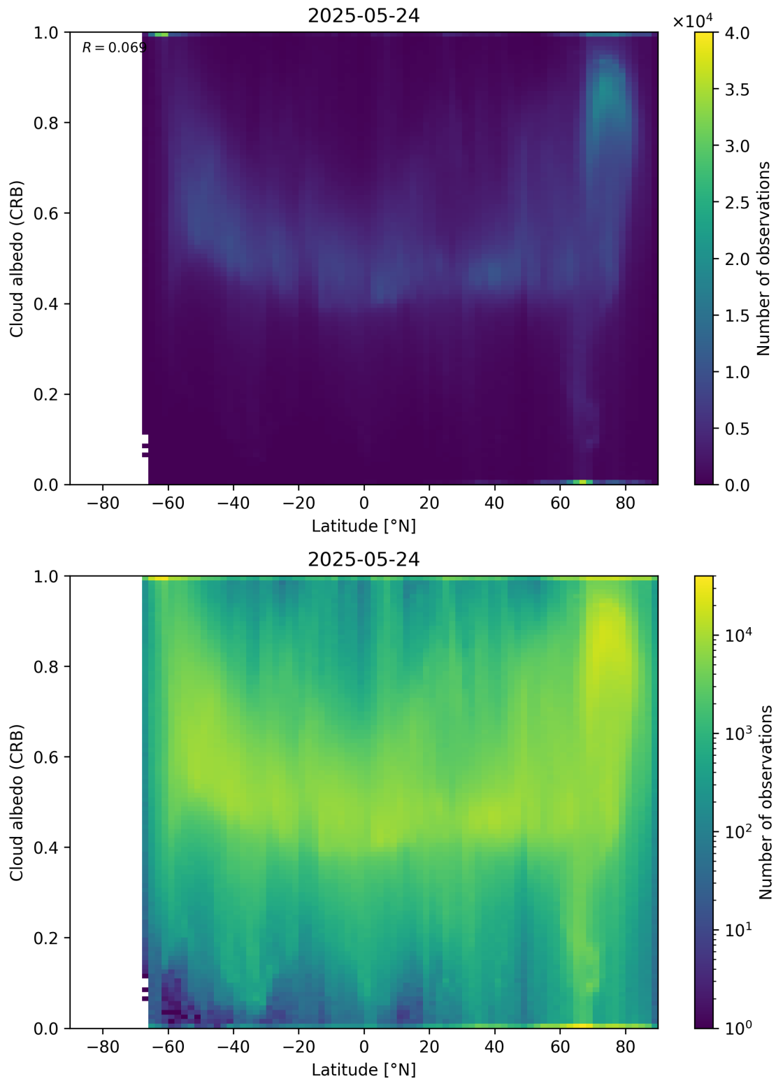
Figure 91: Scatter density plot of “Latitude” against “Cloud albedo (CRB)” for 2025-05-23 to 2025-05-25.
