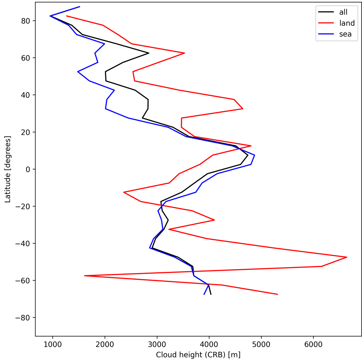
Figure 27: Zonal average of “Cloud height (CRB)” for 2025-05-23 to 2025-05-25.
