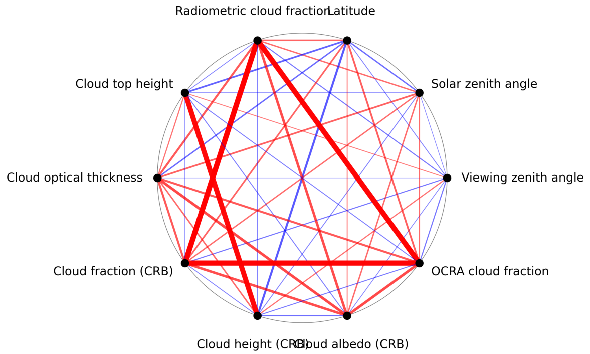
Figure 1: Map of correlation graph for 2025-05-23 to 2025-05-25.
