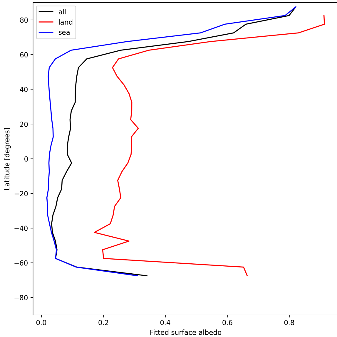
Figure 29: Zonal average of “Fitted surface albedo” for 2025-05-23 to 2025-05-25.
