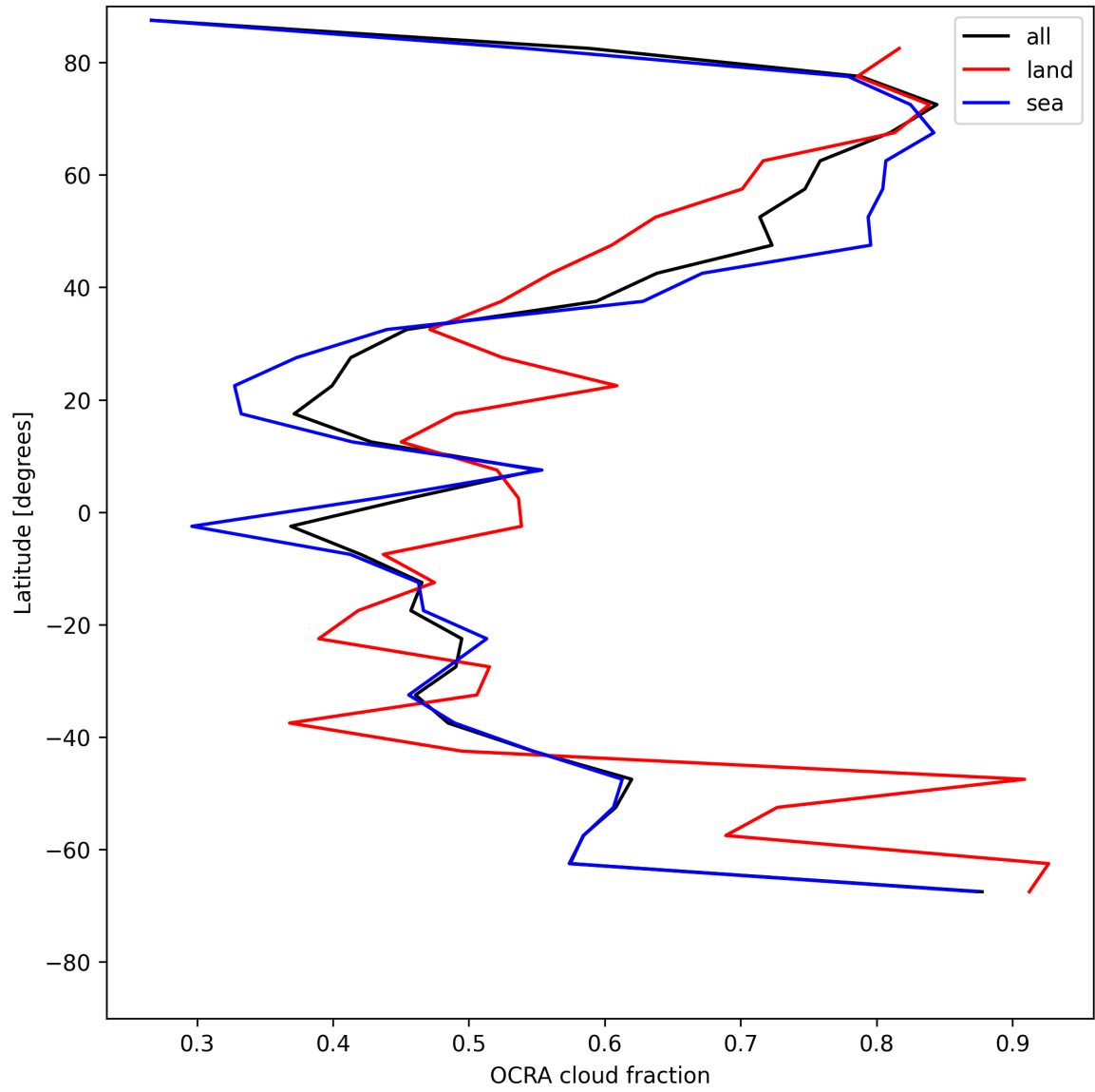
Figure 34: Zonal average of “OCRA cloud fraction” for 2025-05-23 to 2025-05-25.
