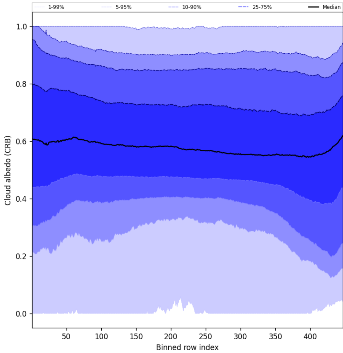
Figure 60: Along track statistics of “Cloud albedo (CRB)” for 2025-05-23 to 2025-05-25
