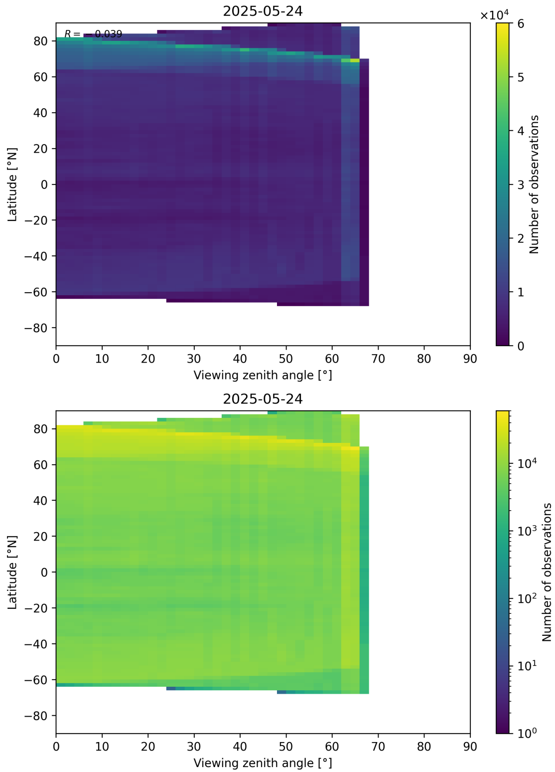
Figure 113: Scatter density plot of “Viewing zenith angle” against “Latitude” for 2025-05-23 to 2025-05-25.
