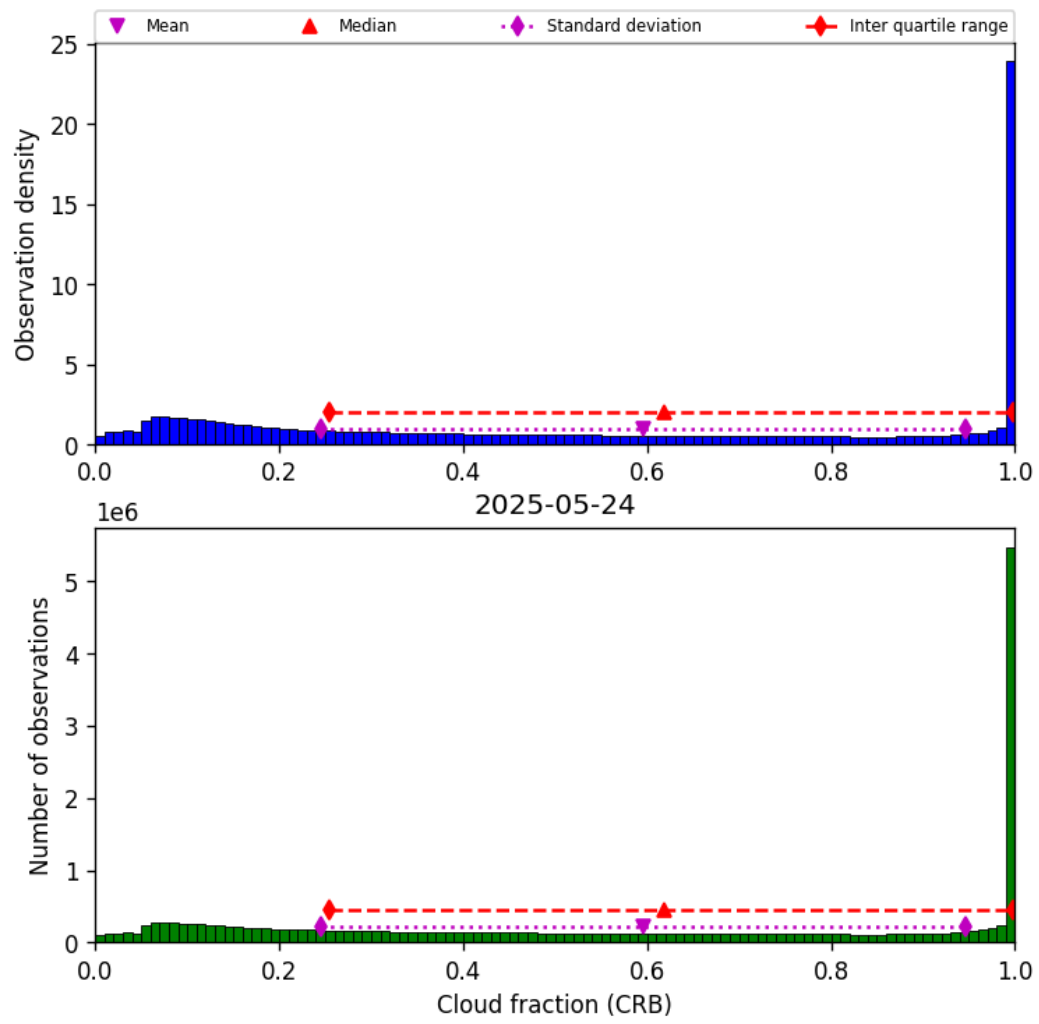
Figure 42: Histogram of “Cloud fraction (CRB)” for 2025-05-23 to 2025-05-25
