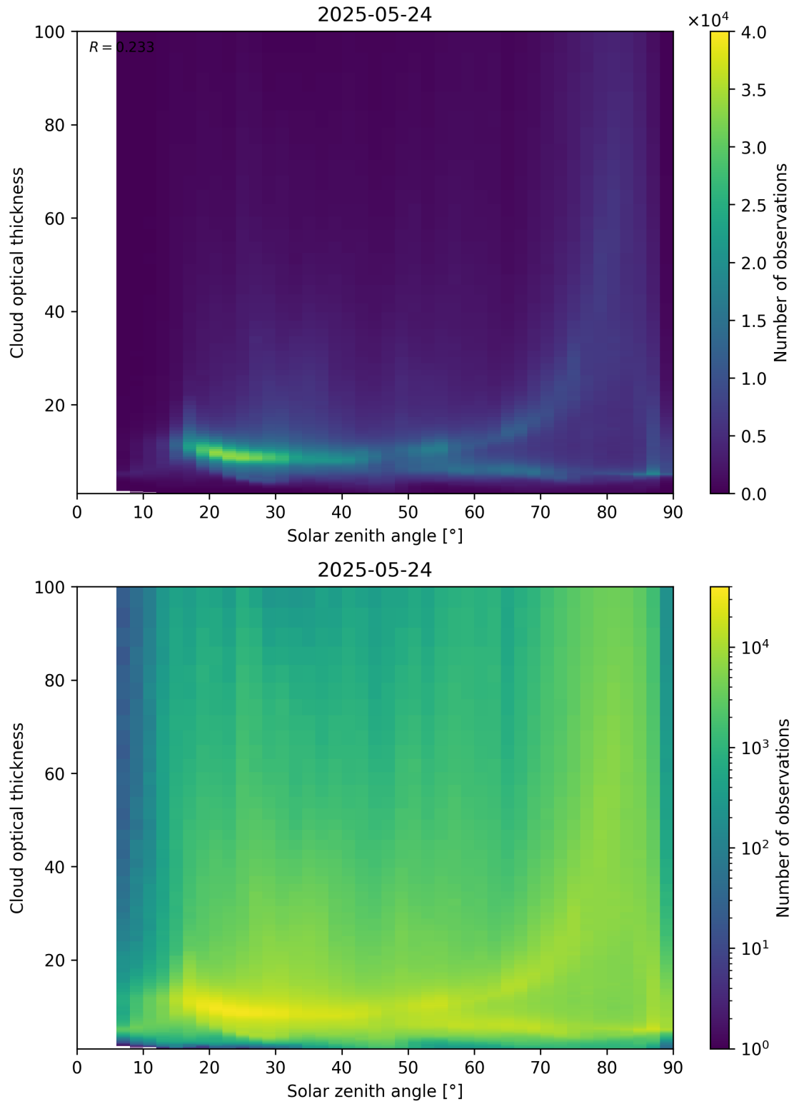
Figure 103: Scatter density plot of “Solar zenith angle” against “Cloud optical thickness” for 2025-05-23 to 2025-05-25.
