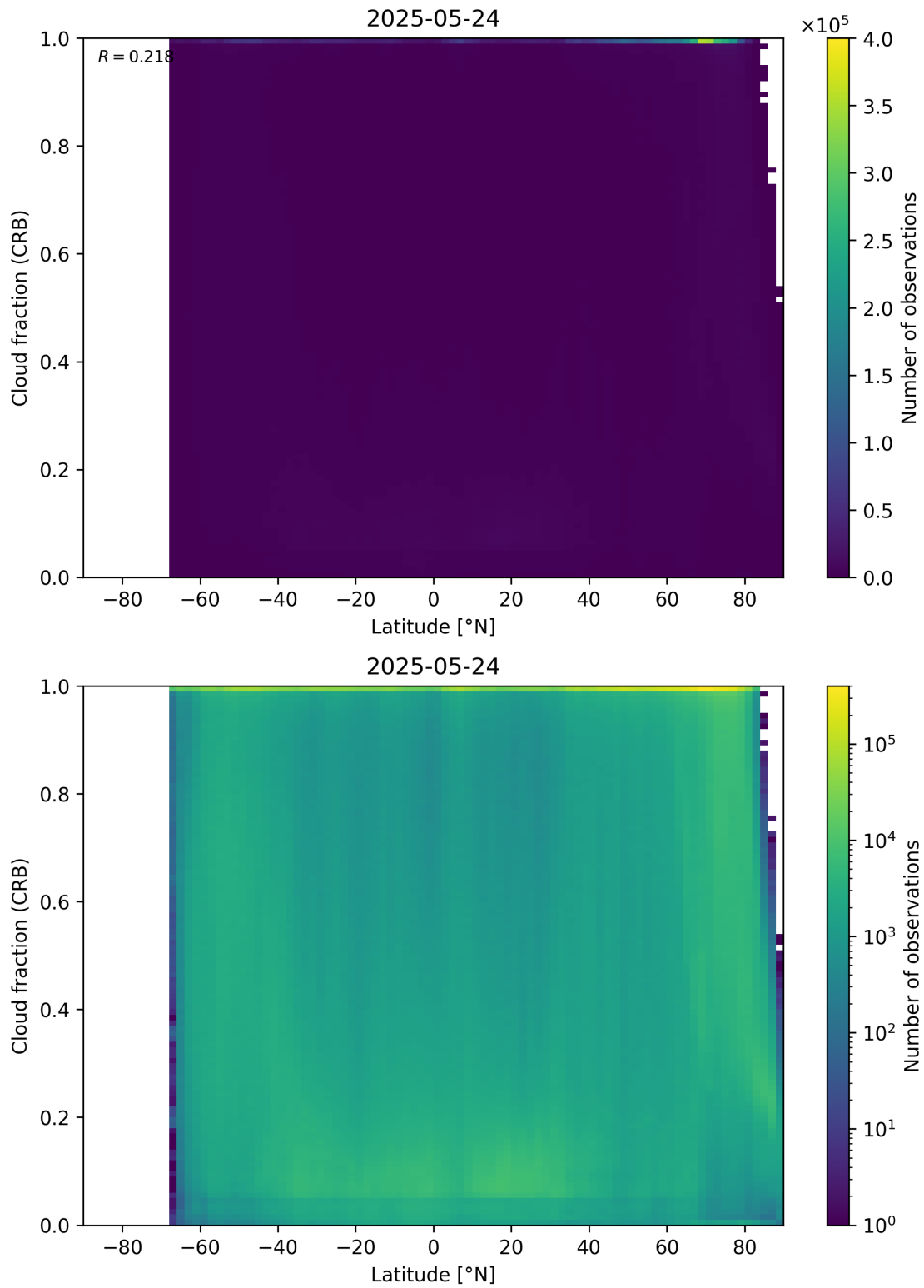
Figure 94: Scatter density plot of “Latitude” against “Cloud fraction (CRB)” for 2025-05-23 to 2025-05-25.
