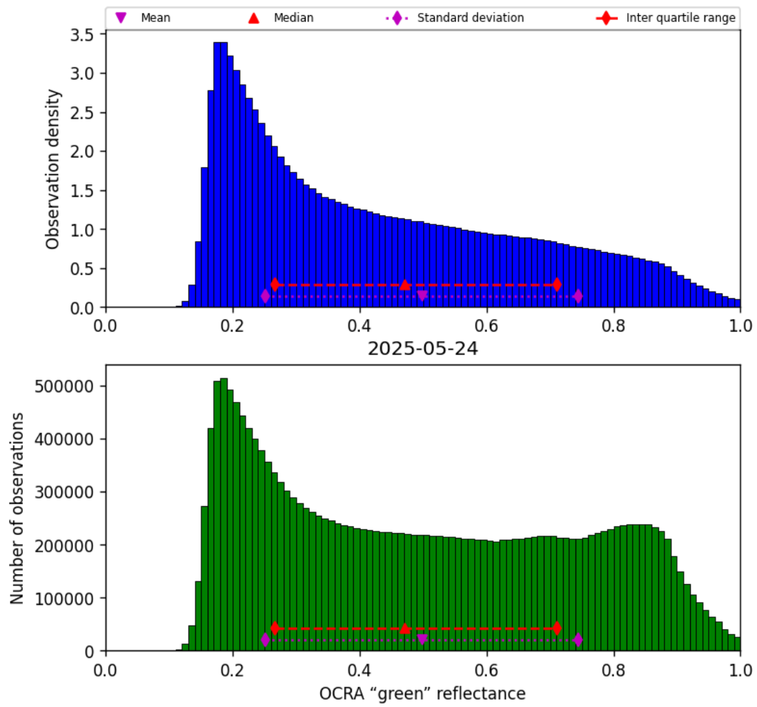
Figure 52: Histogram of “OCRA “green” reflectance” for 2025-05-23 to 2025-05-25
