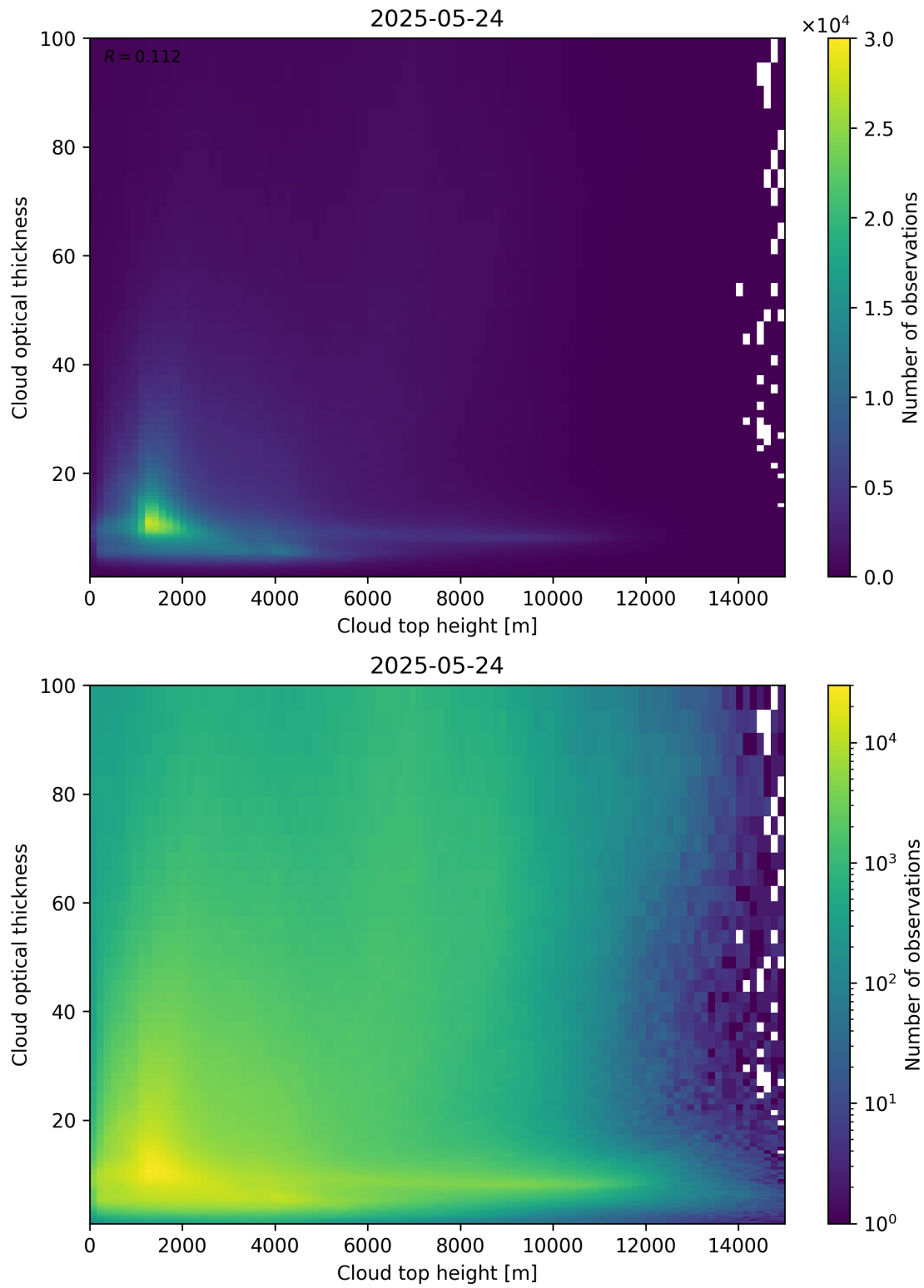
Figure 90: Scatter density plot of “Cloud top height” against “Cloud optical thickness” for 2025-05-23 to 2025-05-25.
