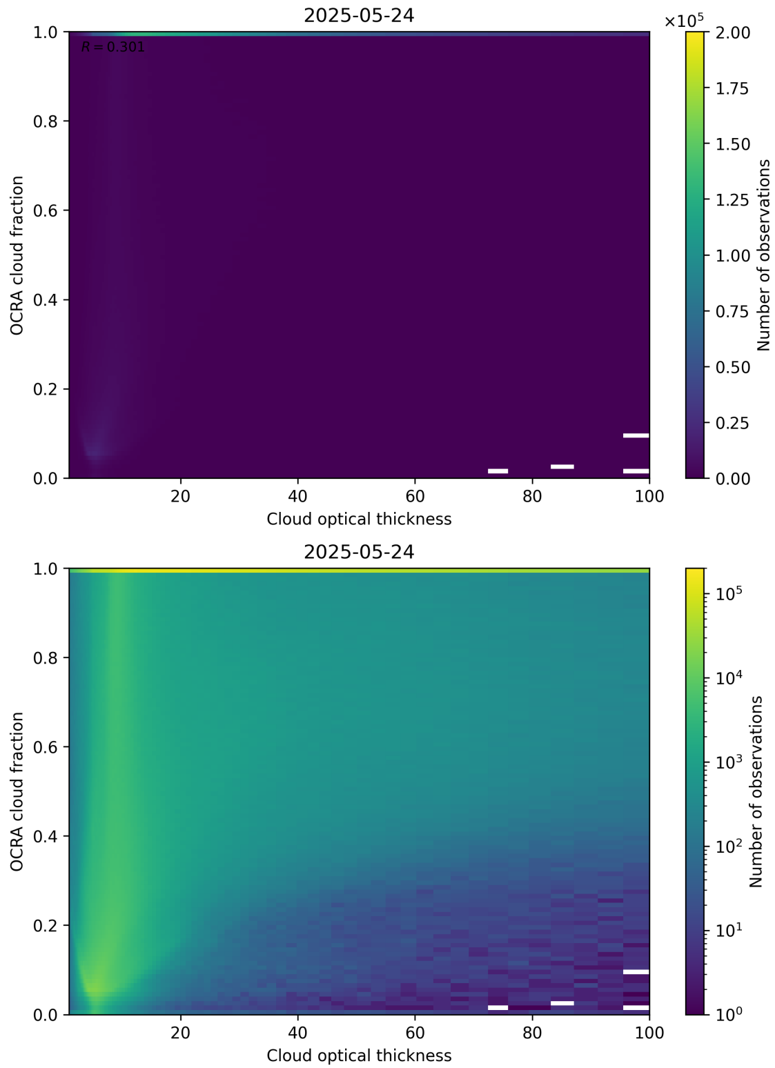
Figure 83: Scatter density plot of “Cloud optical thickness” against “OCRA cloud fraction” for 2025-05-23 to 2025-05-25.
