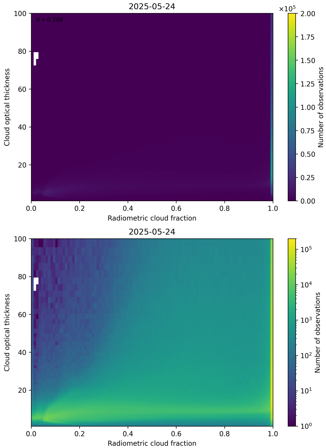
Figure 75: Scatter density plot of “Radiometric cloud fraction” against “Cloud optical thickness” for 2025-05-23 to 2025-05-25.
