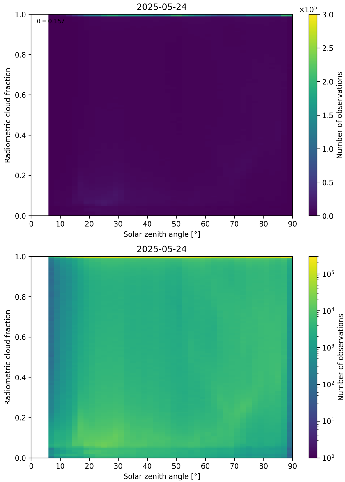
Figure 99: Scatter density plot of “Solar zenith angle” against “Radiometric cloud fraction” for 2025-05-23 to 2025-05-25.
