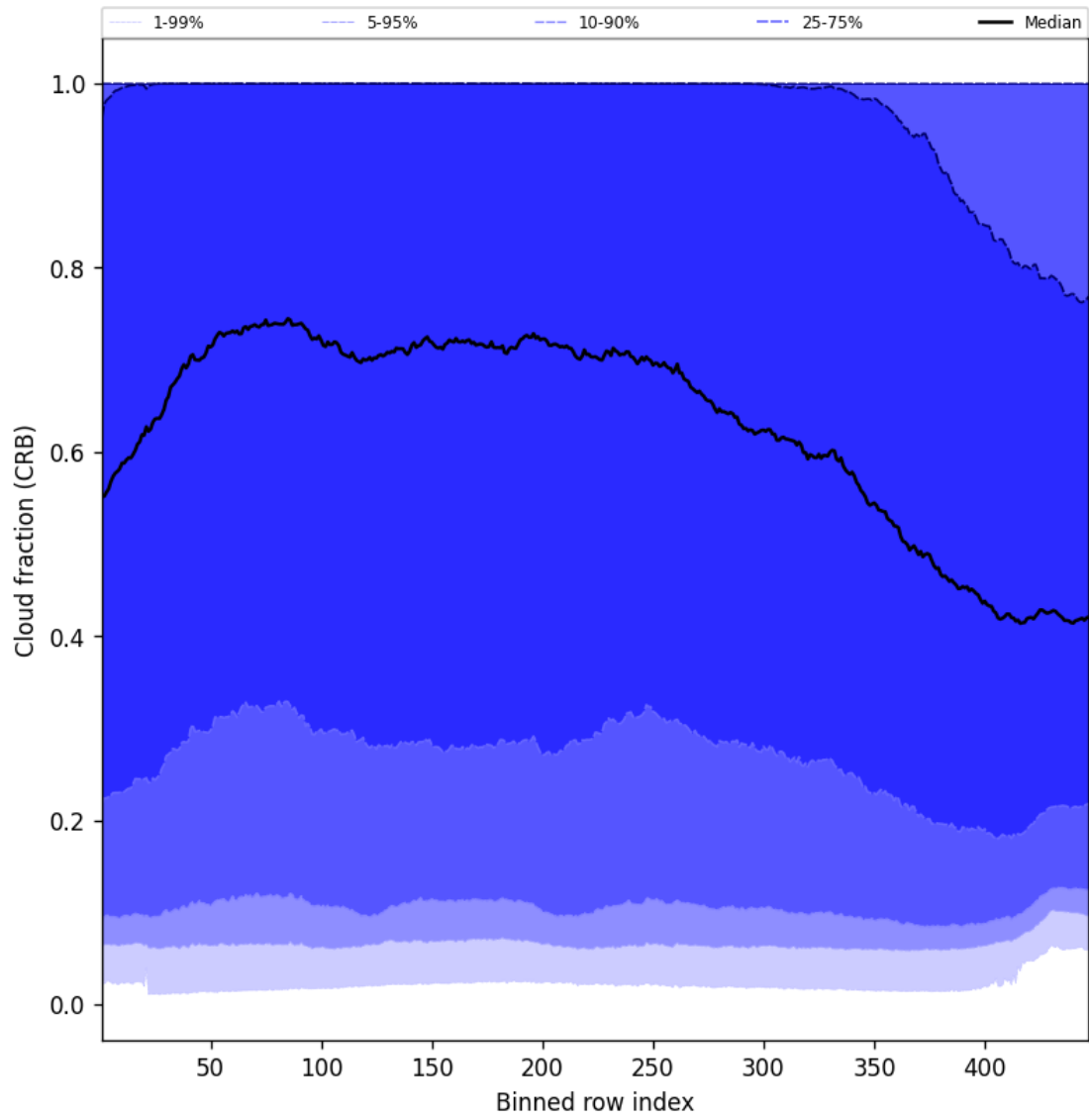
Figure 58: Along track statistics of “Cloud fraction (CRB)” for 2025-05-23 to 2025-05-25
