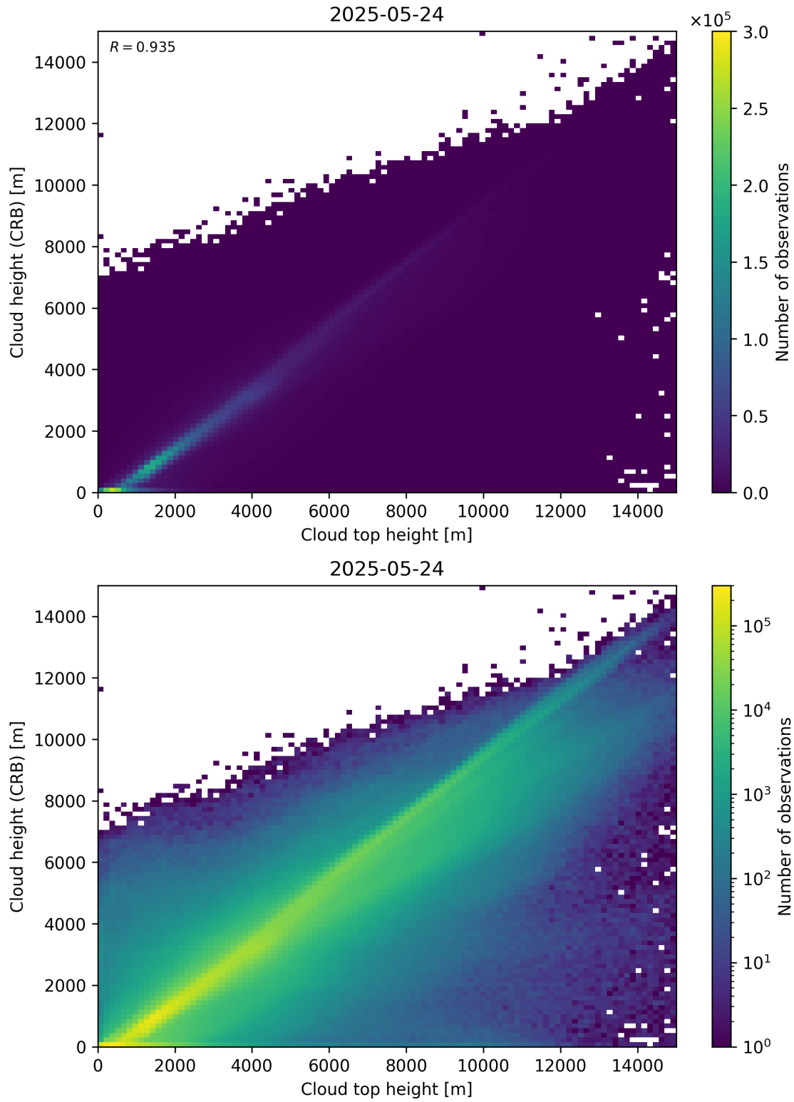
Figure 89: Scatter density plot of “Cloud top height” against “Cloud height (CRB)” for 2025-05-23 to 2025-05-25.
