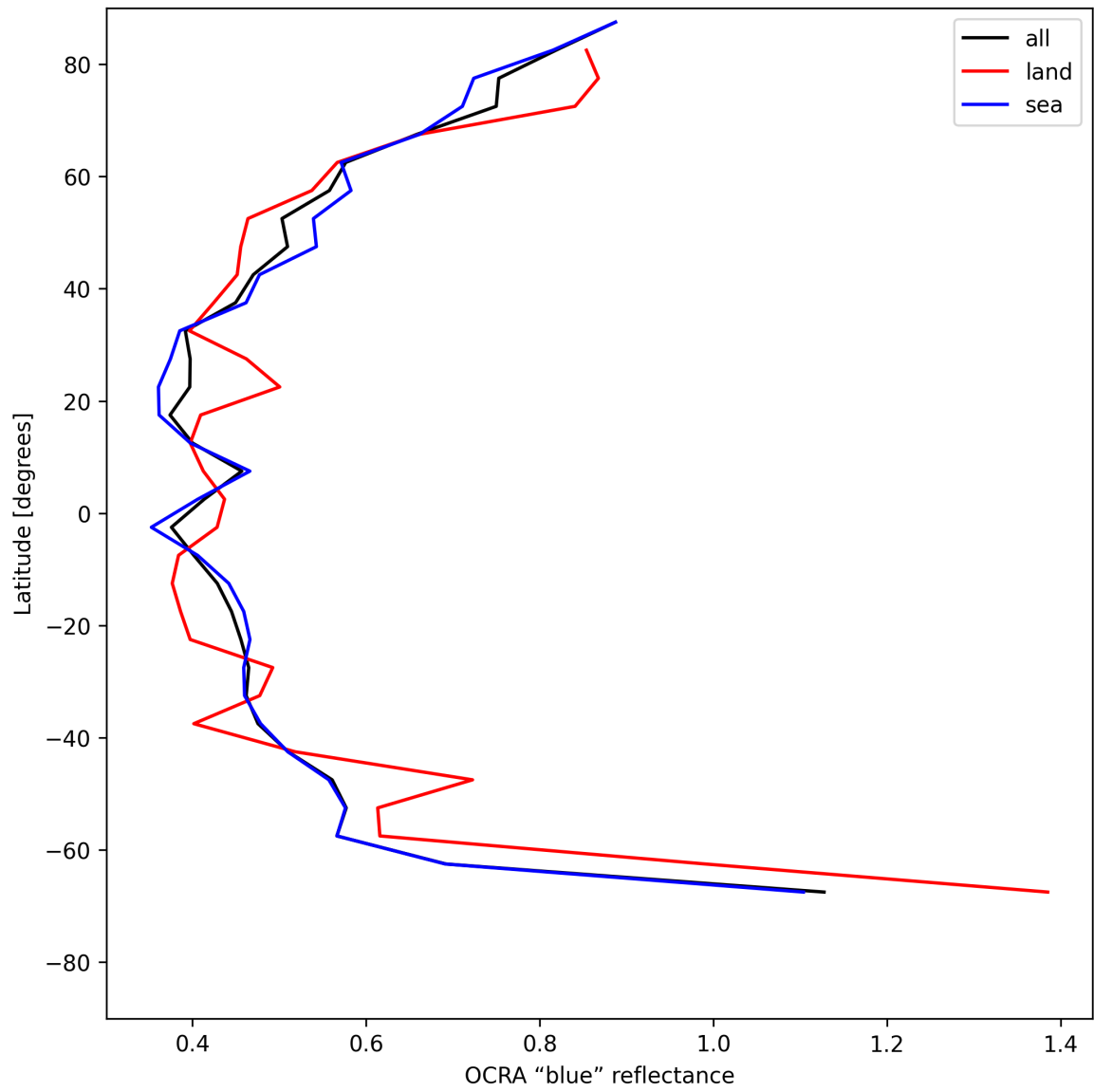
Figure 35: Zonal average of “OCRA “blue” reflectance” for 2025-05-23 to 2025-05-25.
