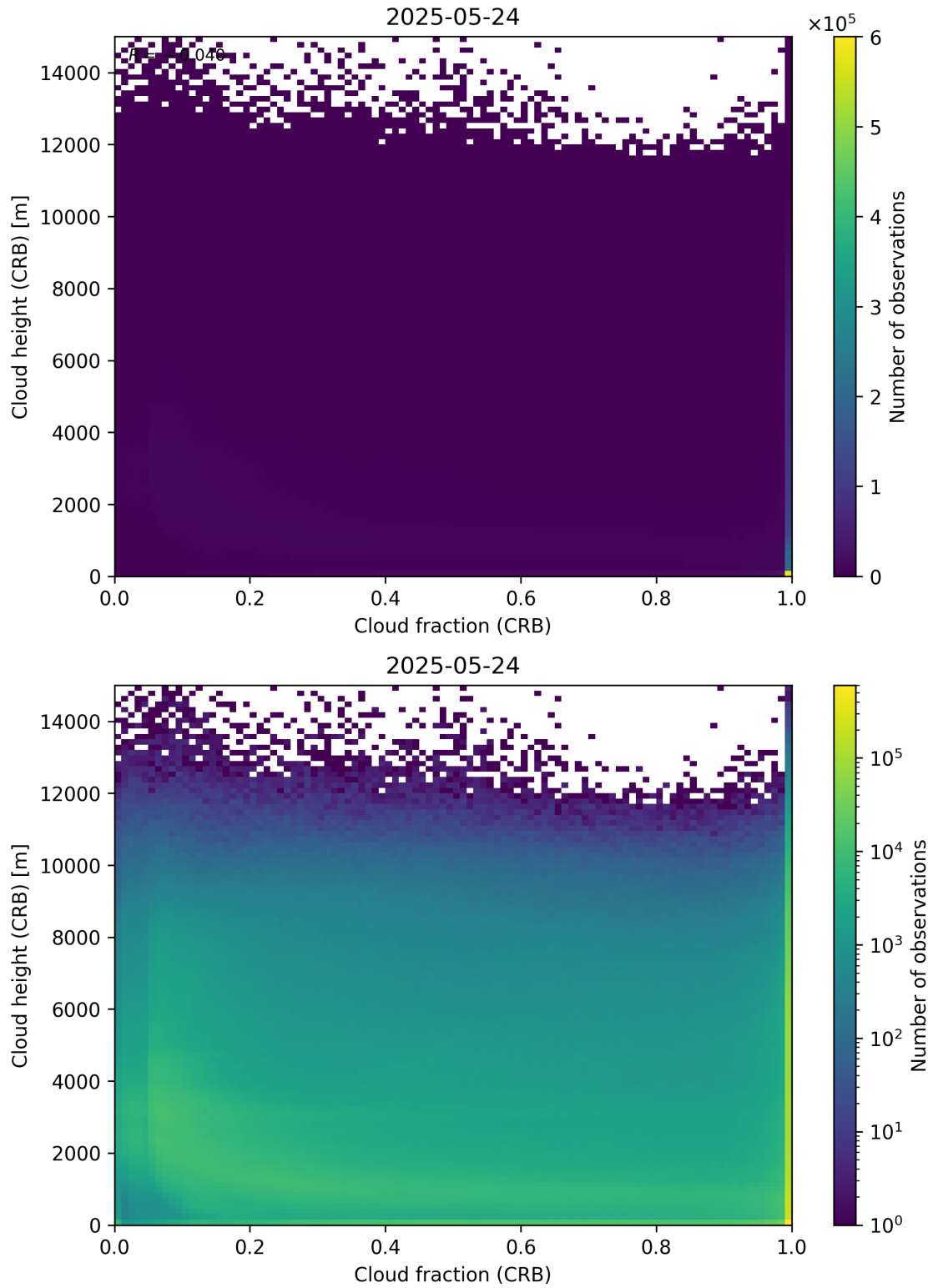
Figure 79: Scatter density plot of “Cloud fraction (CRB)” against “Cloud height (CRB)” for 2025-05-23 to 2025-05-25.
