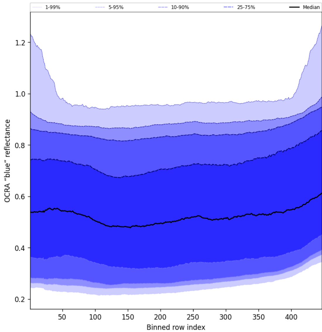
Figure 67: Along track statistics of "OCRA "blue" reflectance" for 2025-05-23 to 2025-05-25
