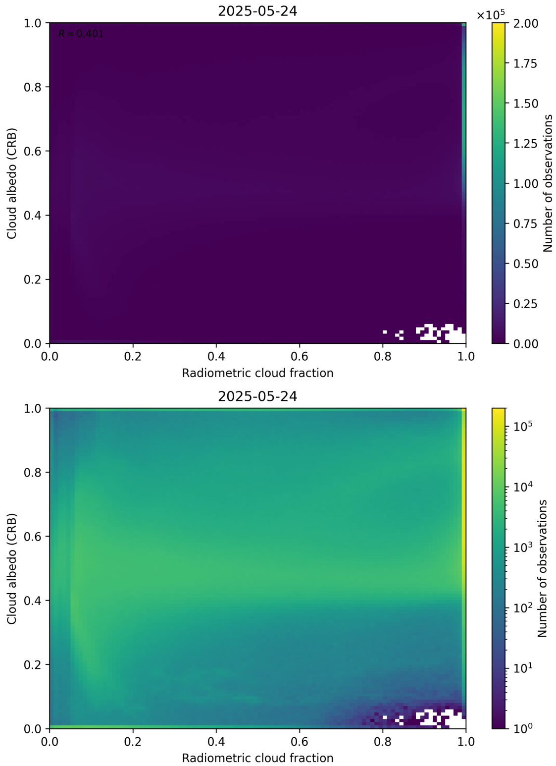
Figure 71: Scatter density plot of “Radiometric cloud fraction” against “Cloud albedo (CRB)” for 2025-05-23 to 2025-05-25.
