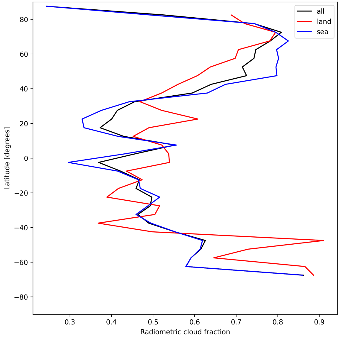
Figure 23: Zonal average of “Radiometric cloud fraction” for 2025-05-23 to 2025-05-25.
