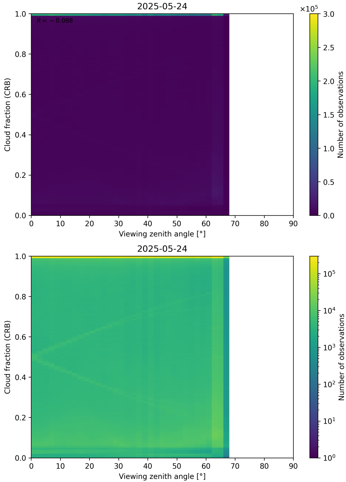
Figure 109: Scatter density plot of “Viewing zenith angle” against “Cloud fraction (CRB)” for 2025-05-23 to 2025-05-25.
