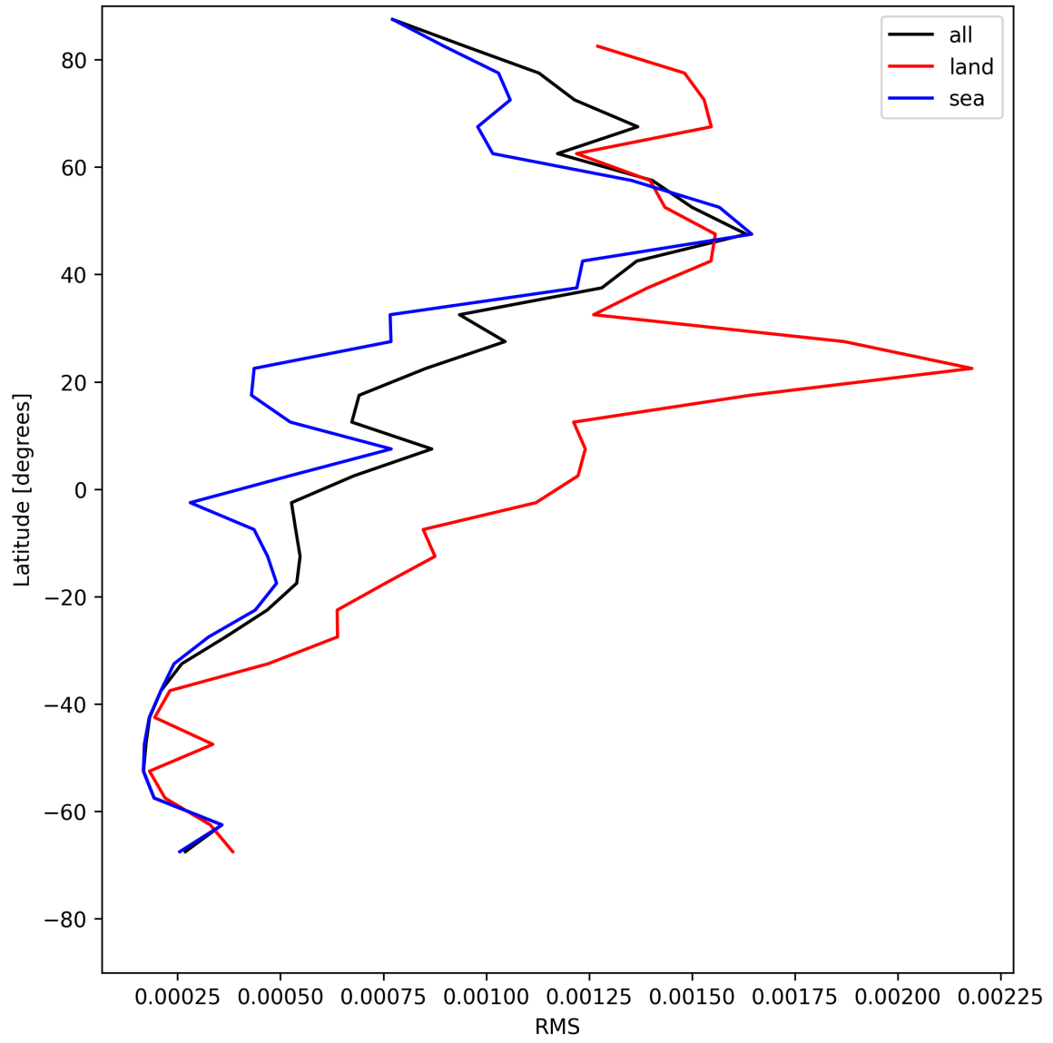
Figure 31: Zonal average of “RMS” for 2025-05-23 to 2025-05-25.
