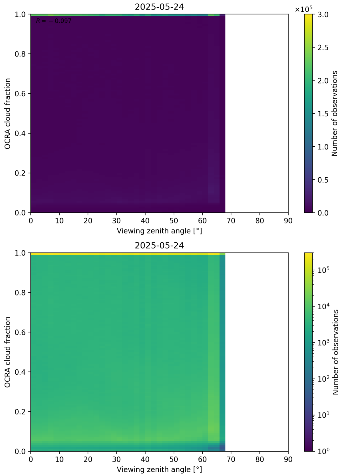
Figure 108: Scatter density plot of “Viewing zenith angle” against “OCRA cloud fraction” for 2025-05-23 to 2025-05-25.
