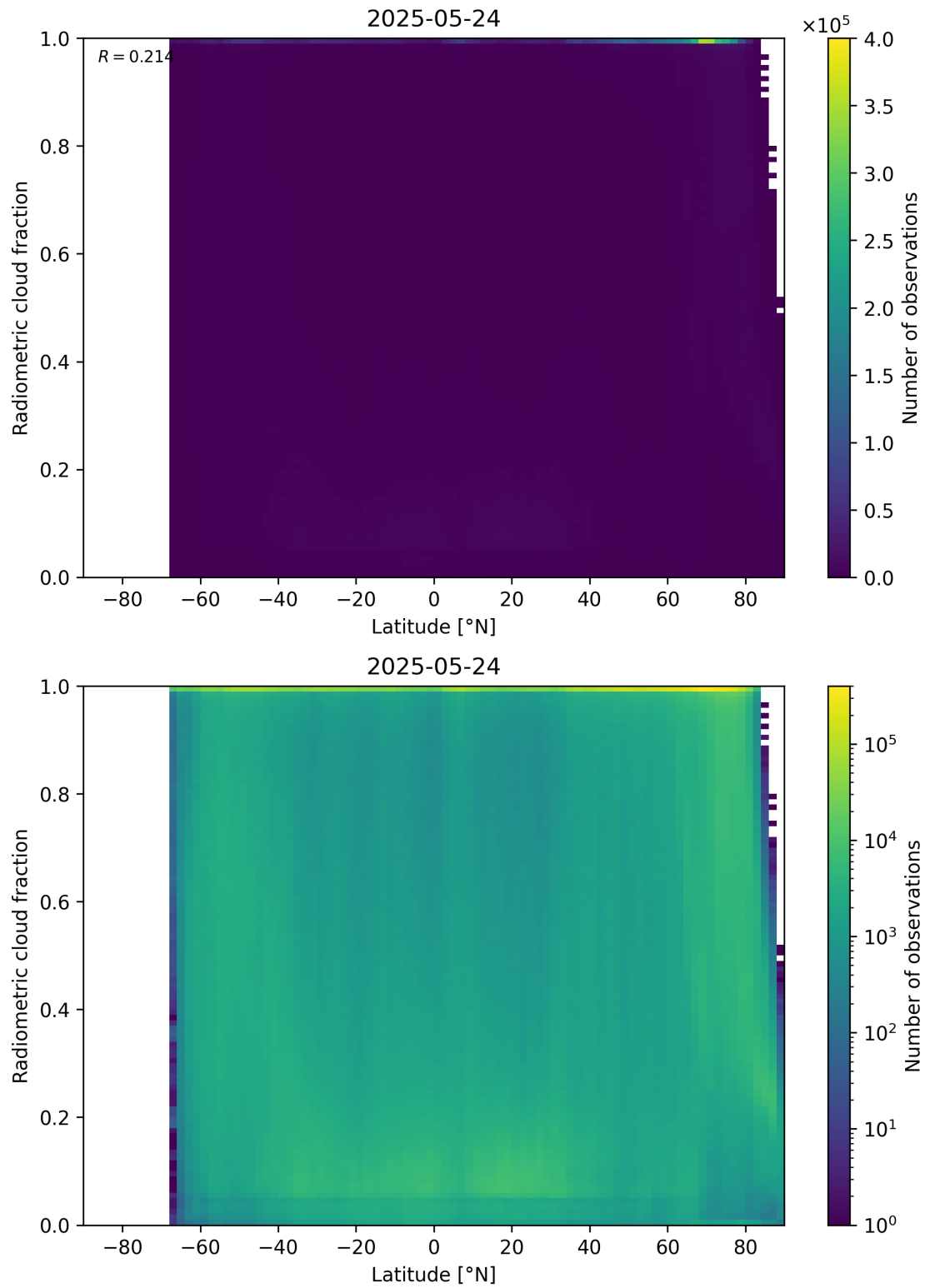
Figure 92: Scatter density plot of “Latitude” against “Radiometric cloud fraction” for 2025-05-23 to 2025-05-25.
