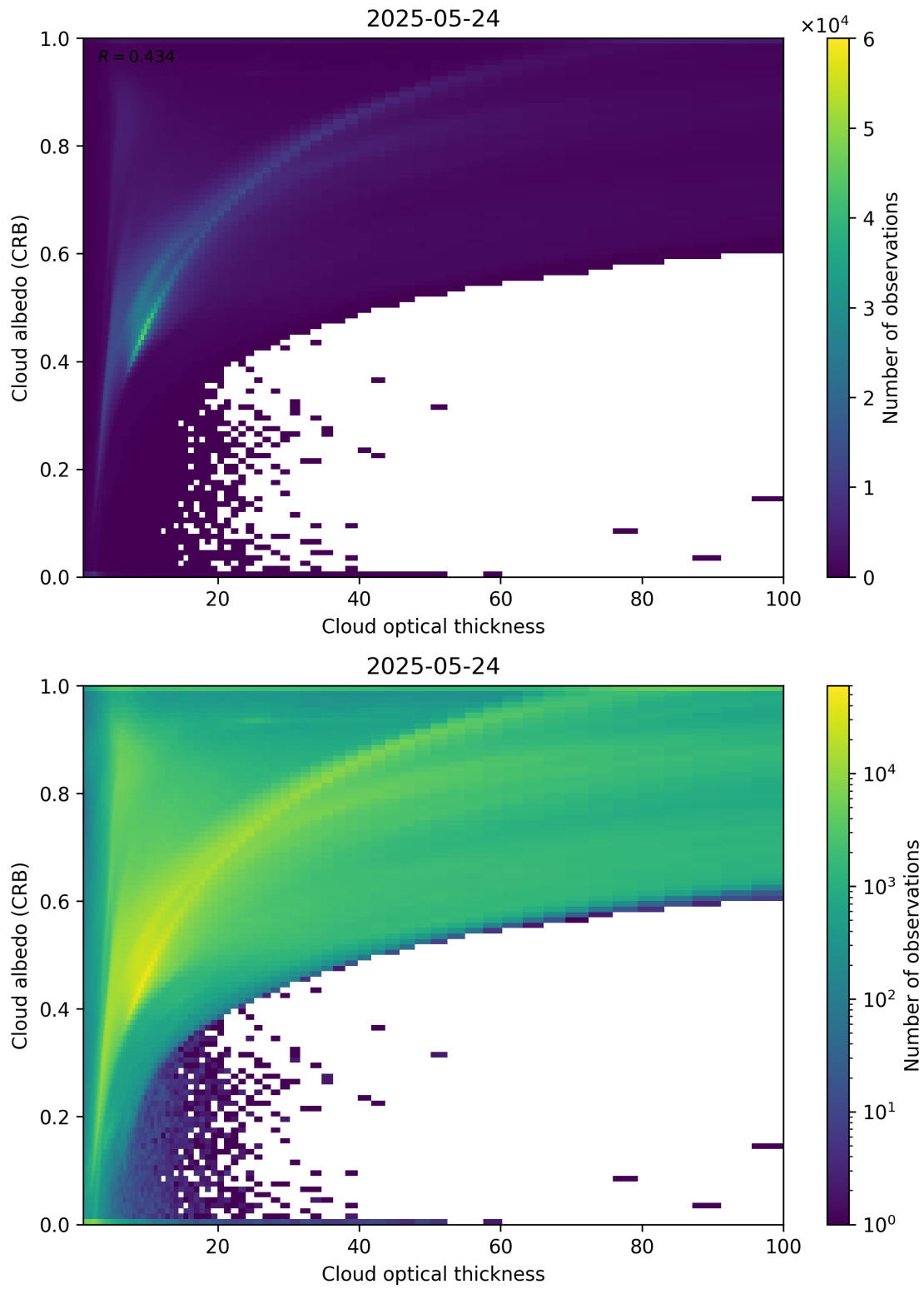
Figure 82: Scatter density plot of “Cloud optical thickness” against “Cloud albedo (CRB)” for 2025-05-23 to 2025-05-25.
