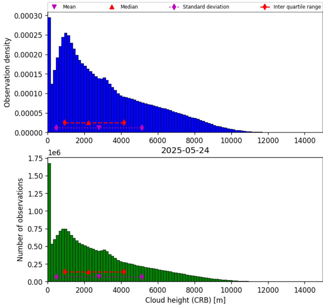
Figure 43: Histogram of “Cloud height (CRB)” for 2025-05-23 to 2025-05-25
