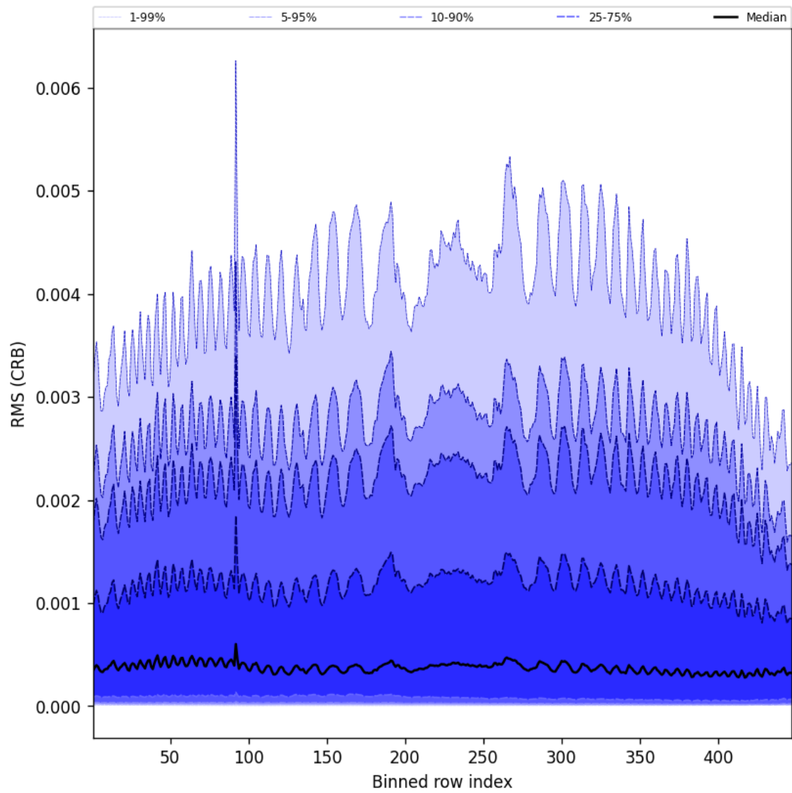
Figure 64: Along track statistics of “RMS (CRB)” for 2025-05-23 to 2025-05-25
