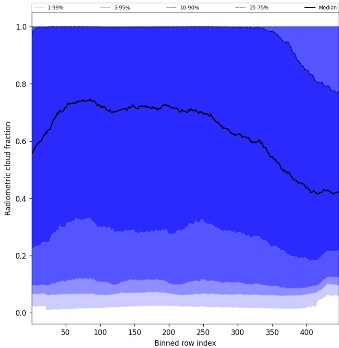
Figure 55: Along track statistics of “Radiometric cloud fraction” for 2025-05-23 to 2025-05-25
