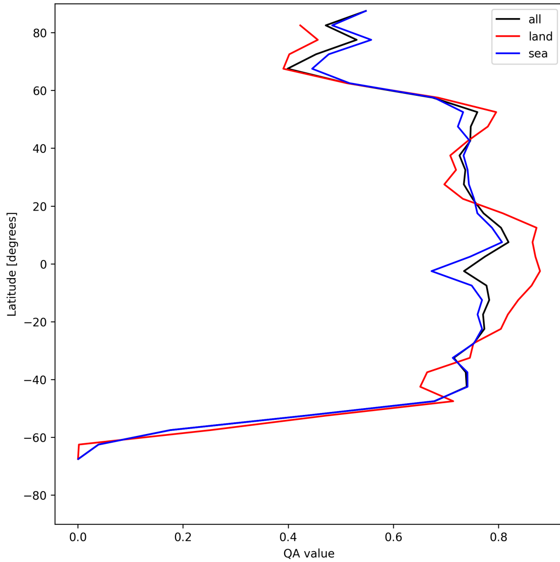
Figure 22: Zonal average of “QA value” for 2025-05-23 to 2025-05-25.
