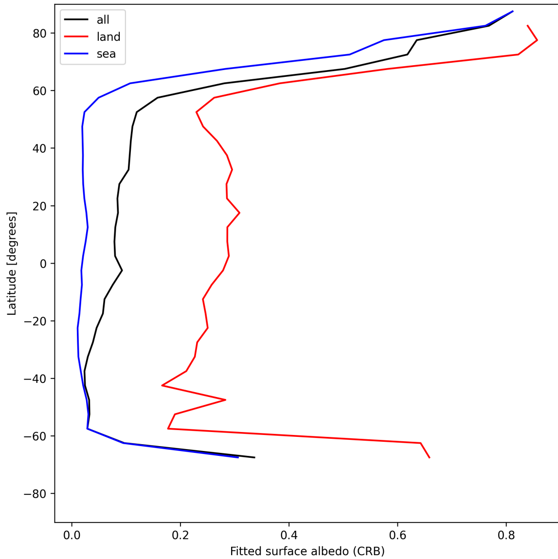
Figure 30: Zonal average of “Fitted surface albedo (CRB)” for 2025-05-23 to 2025-05-25.
