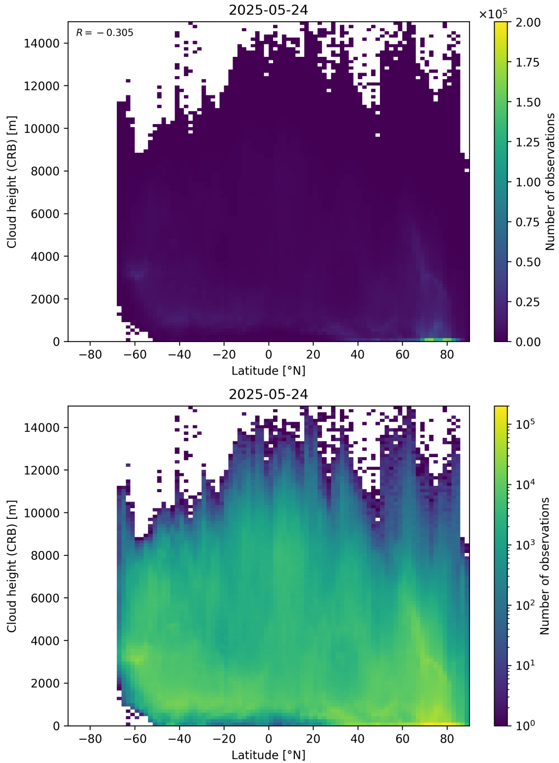
Figure 95: Scatter density plot of “Latitude” against “Cloud height (CRB)” for 2025-05-23 to 2025-05-25.
