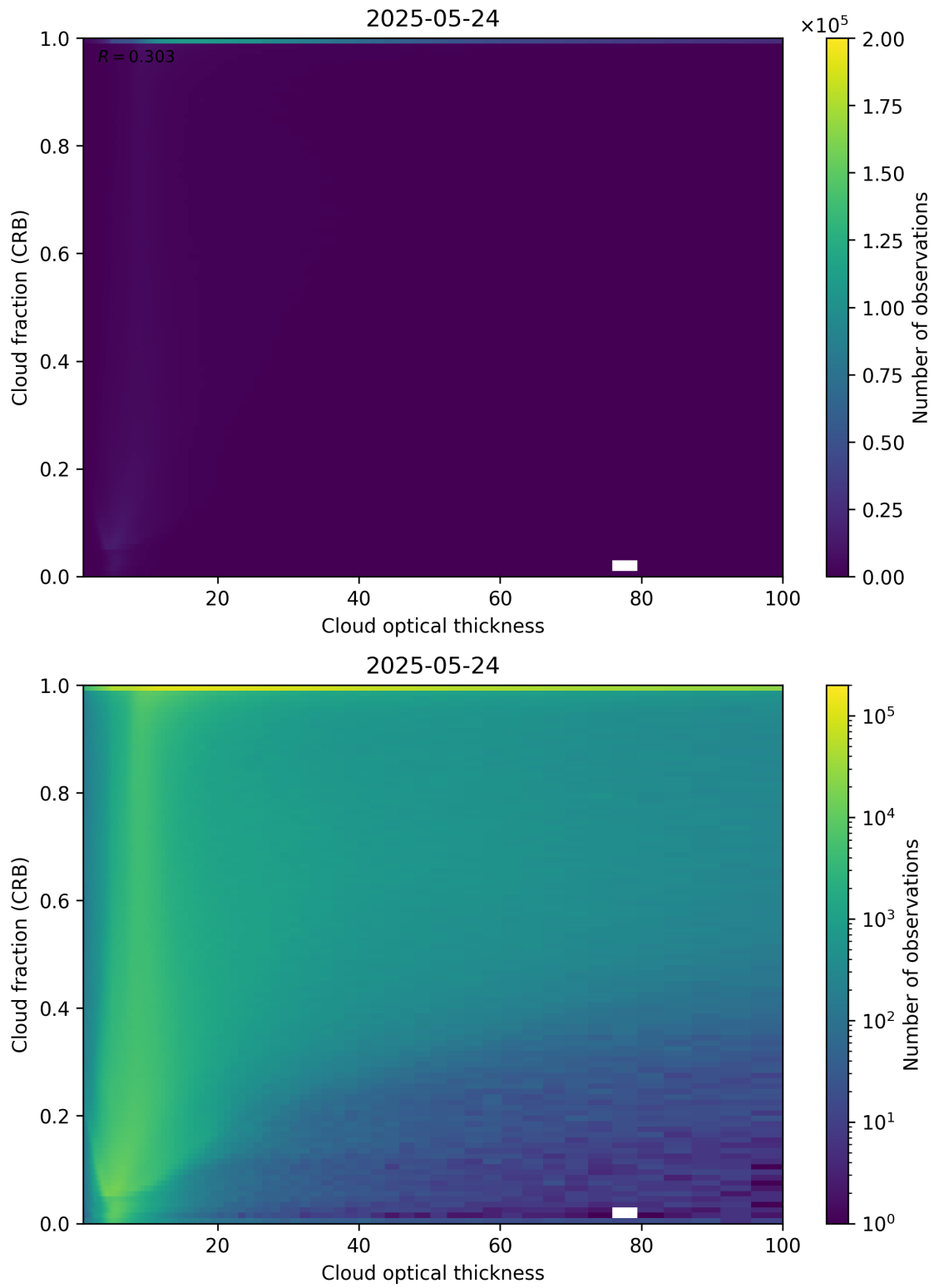
Figure 84: Scatter density plot of “Cloud optical thickness” against “Cloud fraction (CRB)” for 2025-05-23 to 2025-05-25.
