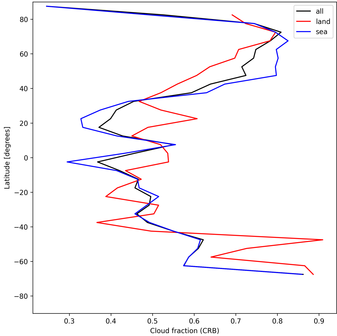
Figure 26: Zonal average of “Cloud fraction (CRB)” for 2025-05-23 to 2025-05-25.
