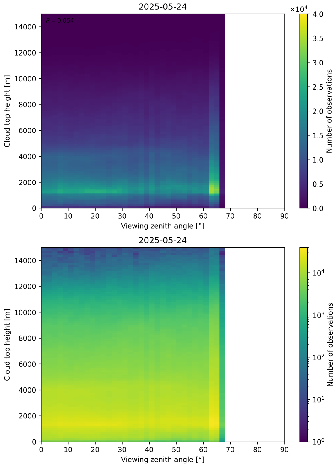
Figure 112: Scatter density plot of “Viewing zenith angle” against “Cloud top height” for 2025-05-23 to 2025-05-25.
