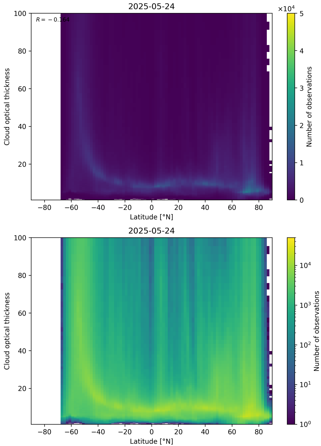
Figure 96: Scatter density plot of “Latitude” against “Cloud optical thickness” for 2025-05-23 to 2025-05-25.
