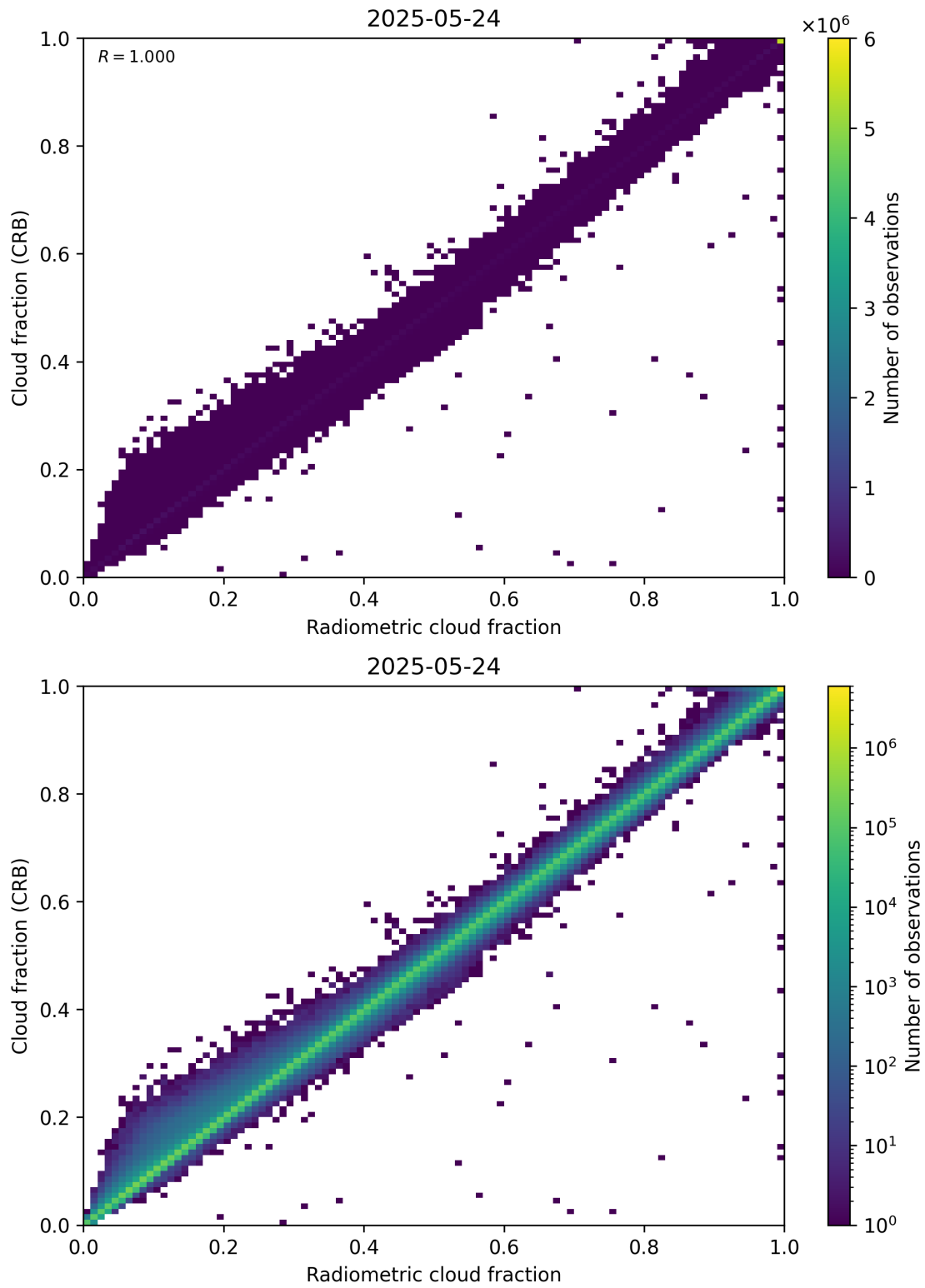
Figure 73: Scatter density plot of “Radiometric cloud fraction” against “Cloud fraction (CRB)” for 2025-05-23 to 2025-05-25.
