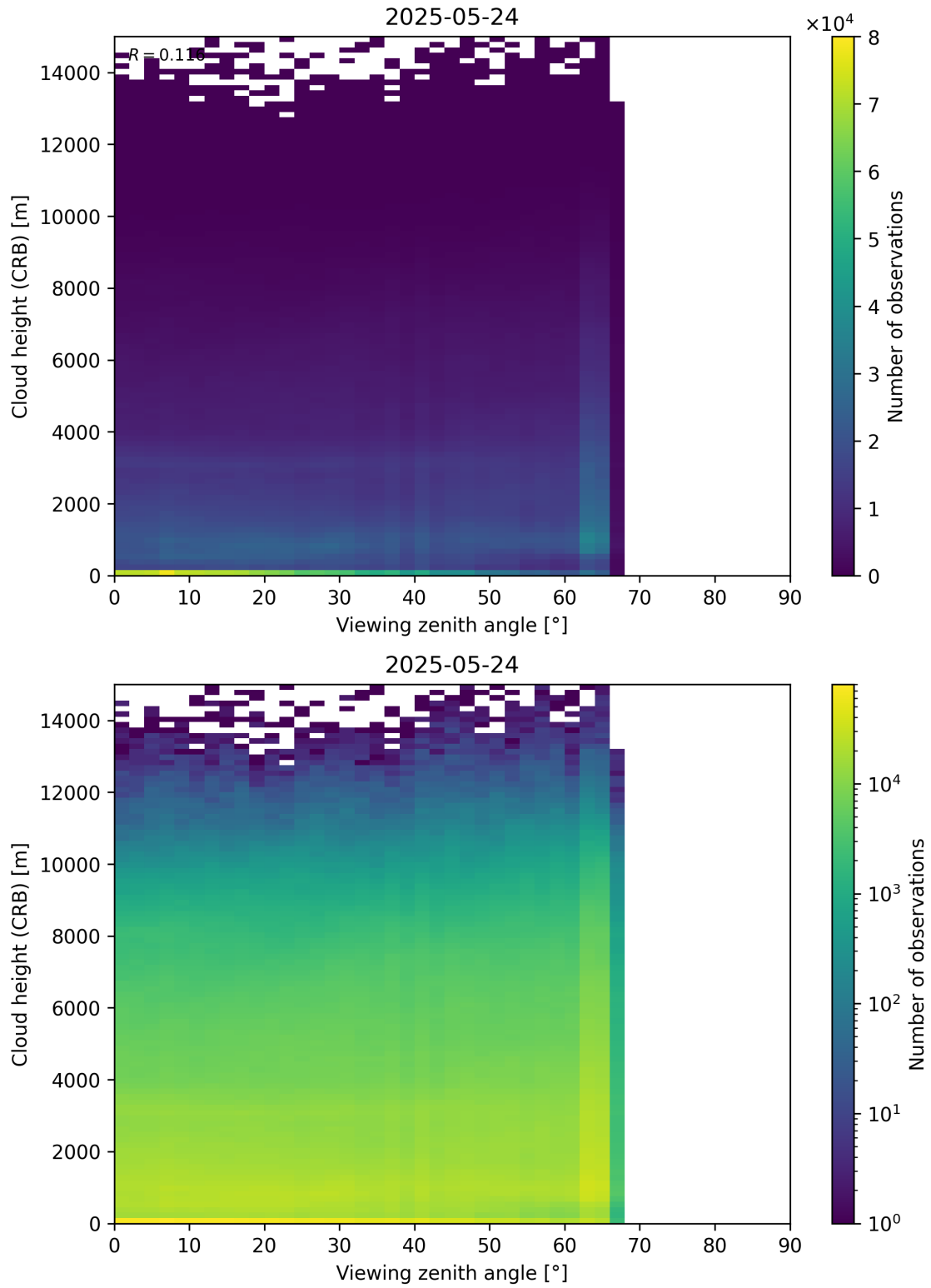
Figure 110: Scatter density plot of “Viewing zenith angle” against “Cloud height (CRB)” for 2025-05-23 to 2025-05-25.
