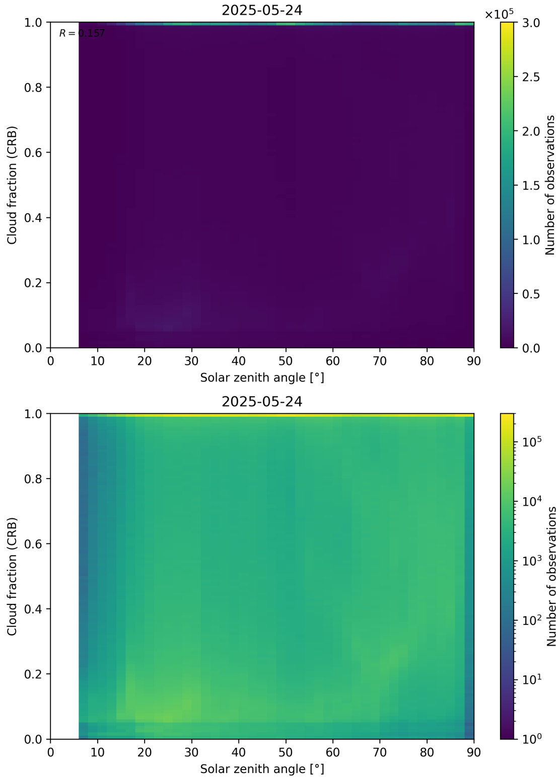
Figure 101: Scatter density plot of “Solar zenith angle” against “Cloud fraction (CRB)” for 2025-05-23 to 2025-05-25.
