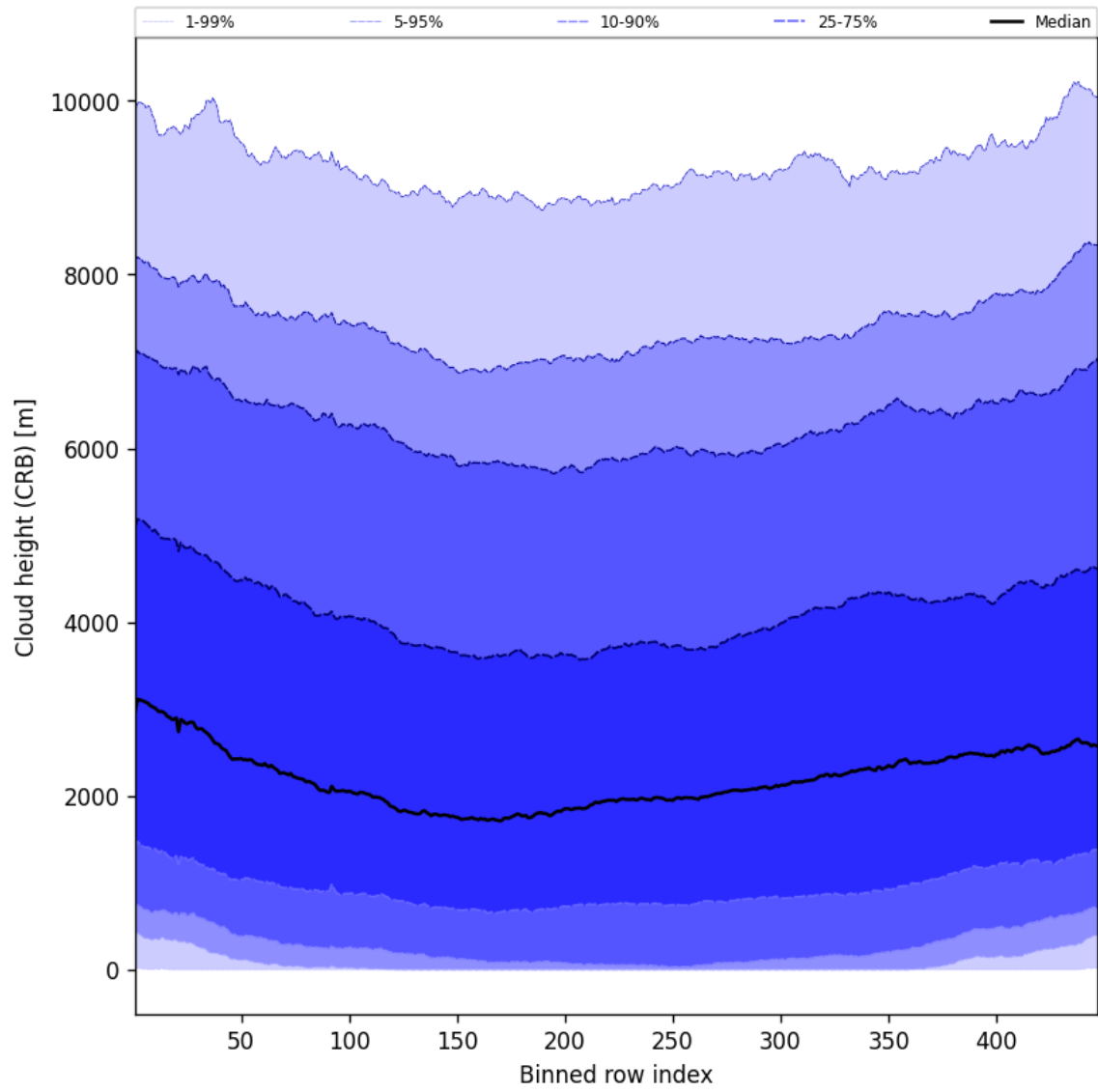
Figure 59: Along track statistics of “Cloud height (CRB)” for 2025-05-23 to 2025-05-25
