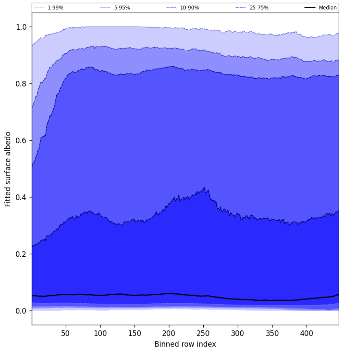
Figure 61: Along track statistics of “Fitted surface albedo” for 2025-05-23 to 2025-05-25
