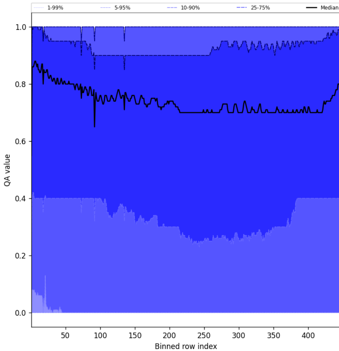
Figure 54: Along track statistics of “QA value” for 2025-05-23 to 2025-05-25
