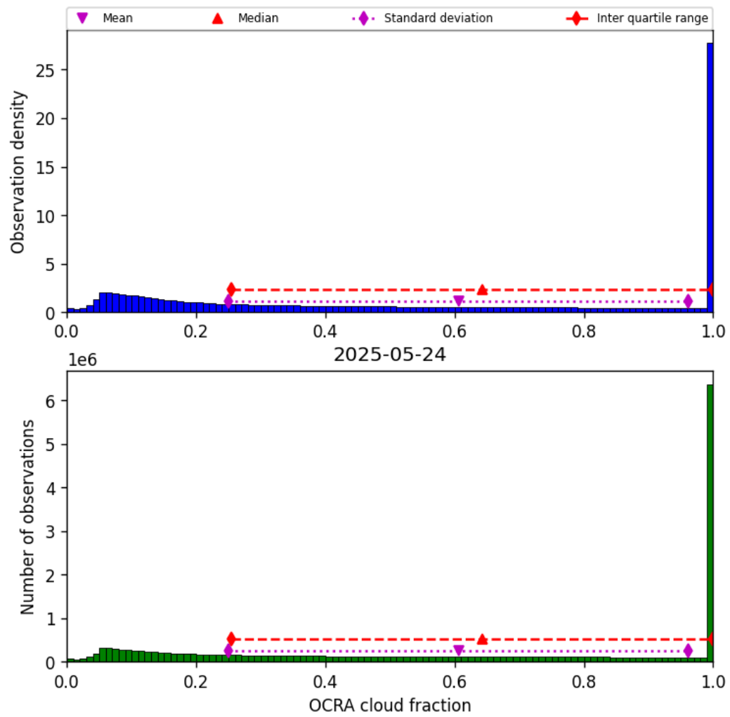
Figure 50: Histogram of “OCRA cloud fraction” for 2025-05-23 to 2025-05-25
