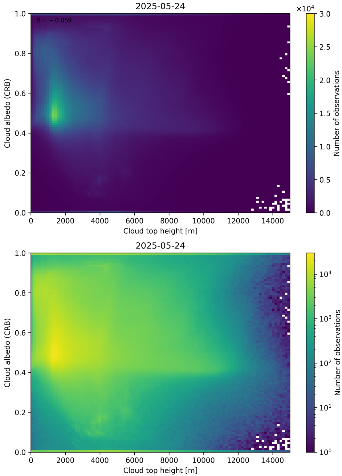
Figure 86: Scatter density plot of “Cloud top height” against “Cloud albedo (CRB)” for 2025-05-23 to 2025-05-25.
