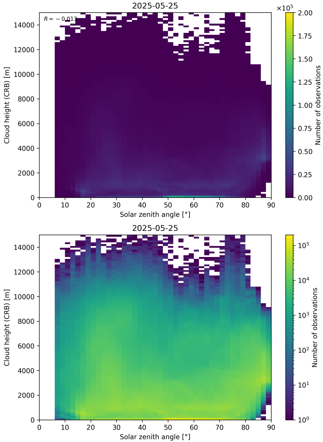
Figure 102: Scatter density plot of “Solar zenith angle” against “Cloud height (CRB)” for 2025-05-24 to 2025-05-26.
