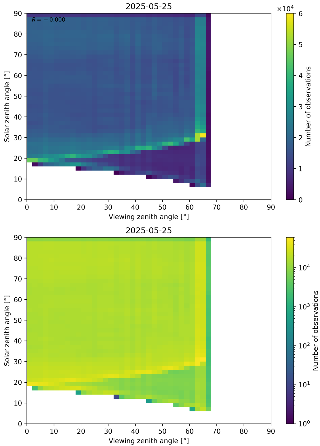
Figure 114: Scatter density plot of “Viewing zenith angle” against “Solar zenith angle” for 2025-05-24 to 2025-05-26.
