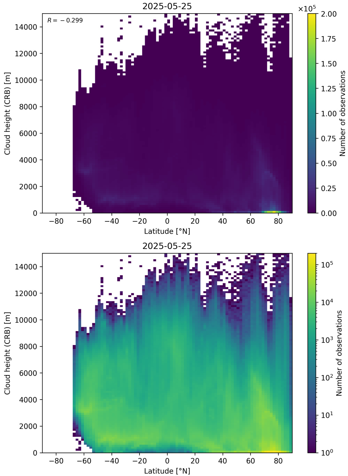
Figure 95: Scatter density plot of “Latitude” against “Cloud height (CRB)” for 2025-05-24 to 2025-05-26.
