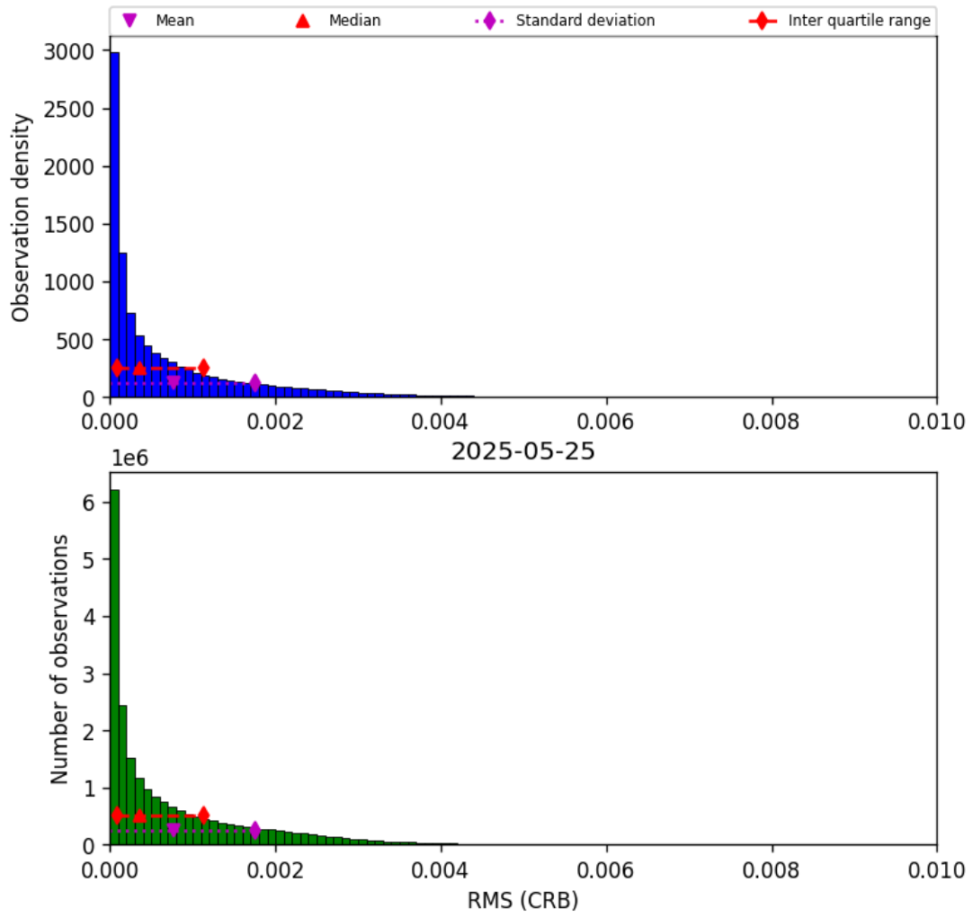
Figure 48: Histogram of “RMS (CRB)” for 2025-05-24 to 2025-05-26
