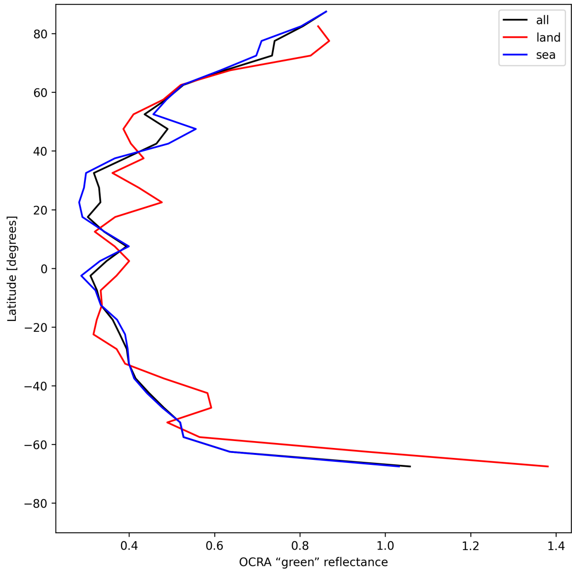
Figure 36: Zonal average of “OCRA “green” reflectance” for 2025-05-24 to 2025-05-26.
