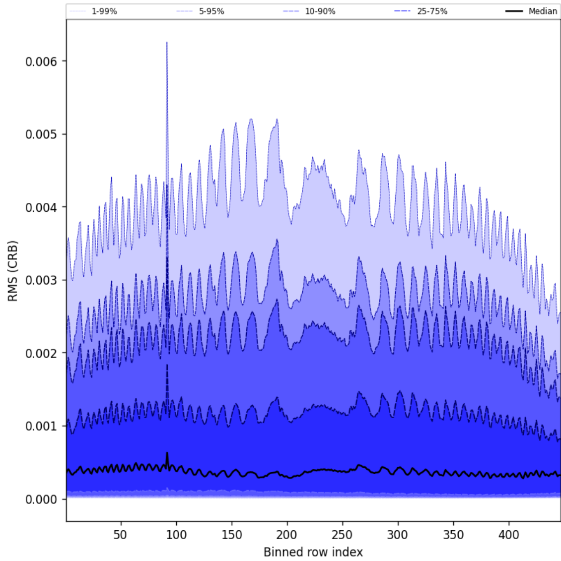
Figure 64: Along track statistics of “RMS (CRB)” for 2025-05-24 to 2025-05-26
