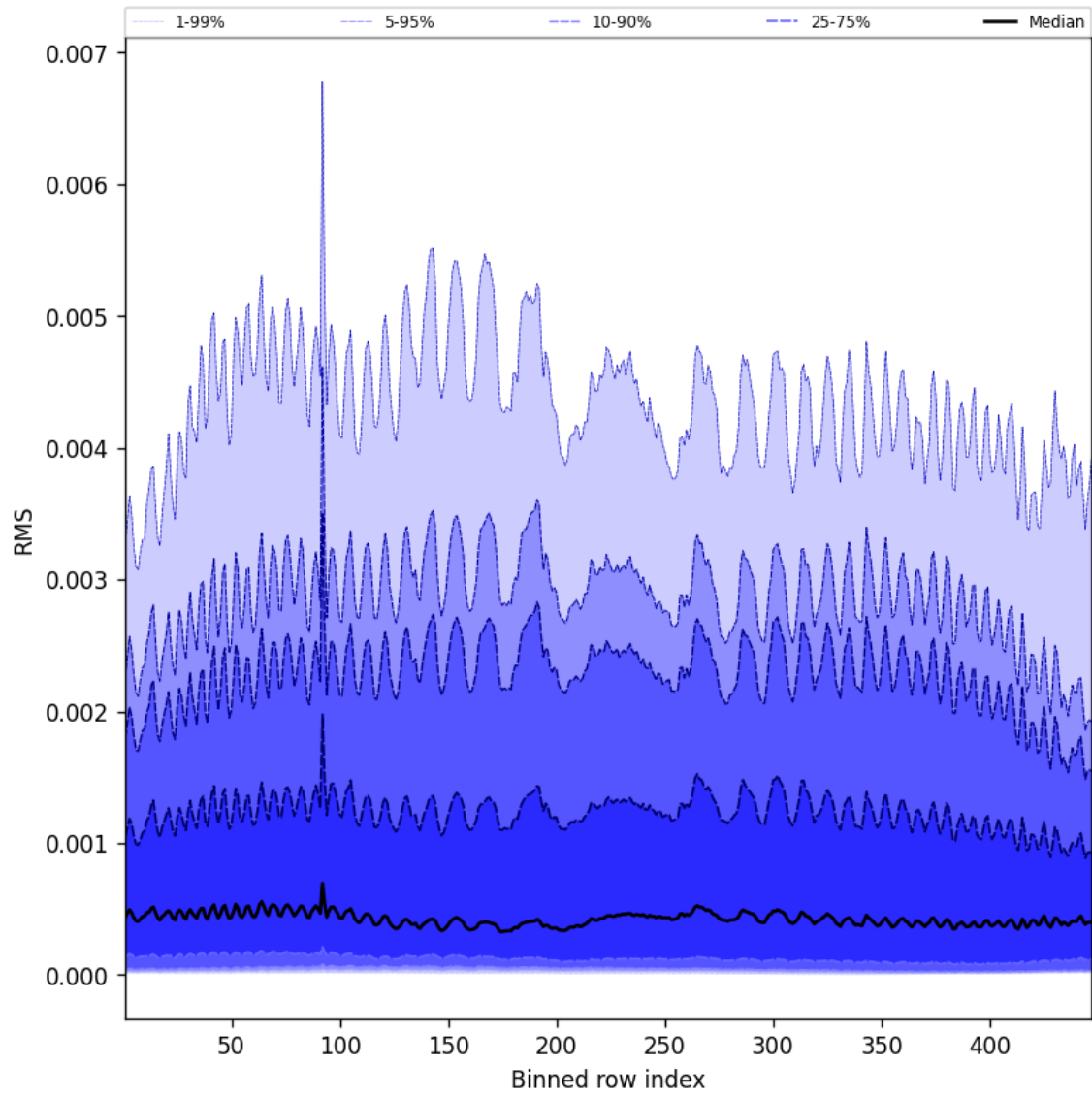
Figure 63: Along track statistics of “RMS” for 2025-05-24 to 2025-05-26
