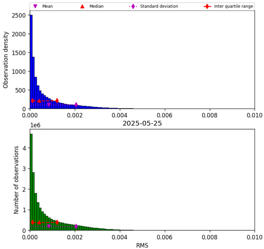
Figure 47: Histogram of “RMS” for 2025-05-24 to 2025-05-26
