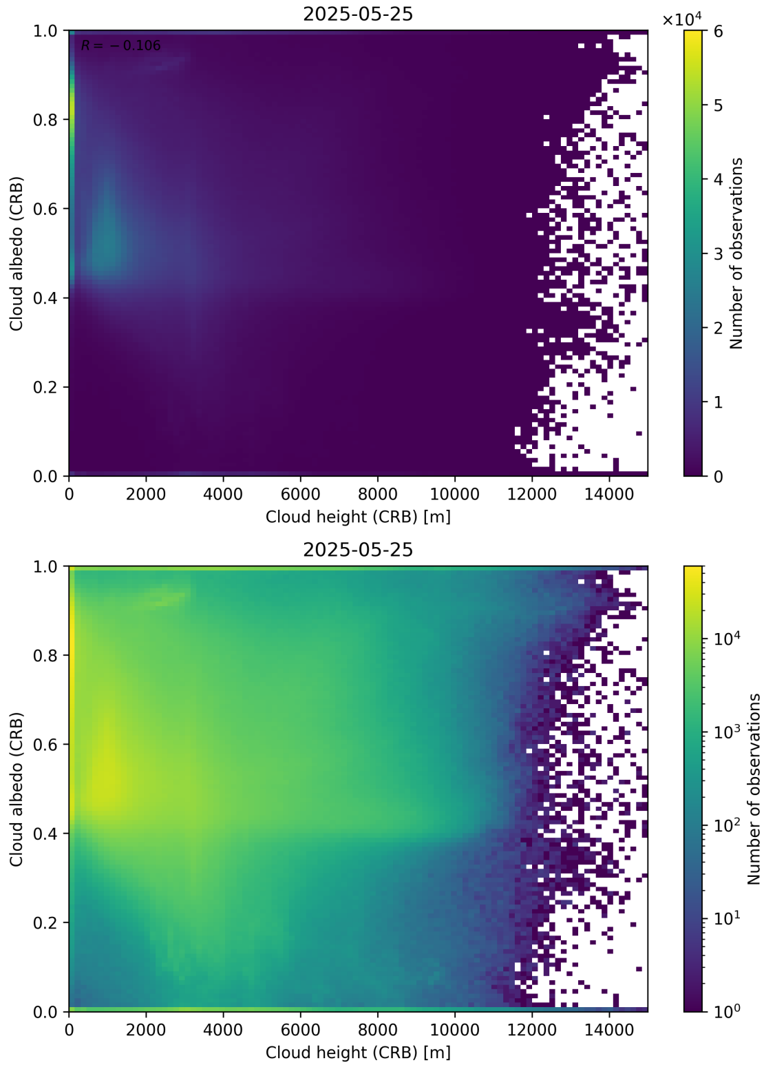
Figure 80: Scatter density plot of “Cloud height (CRB)” against “Cloud albedo (CRB)” for 2025-05-24 to 2025-05-26.
