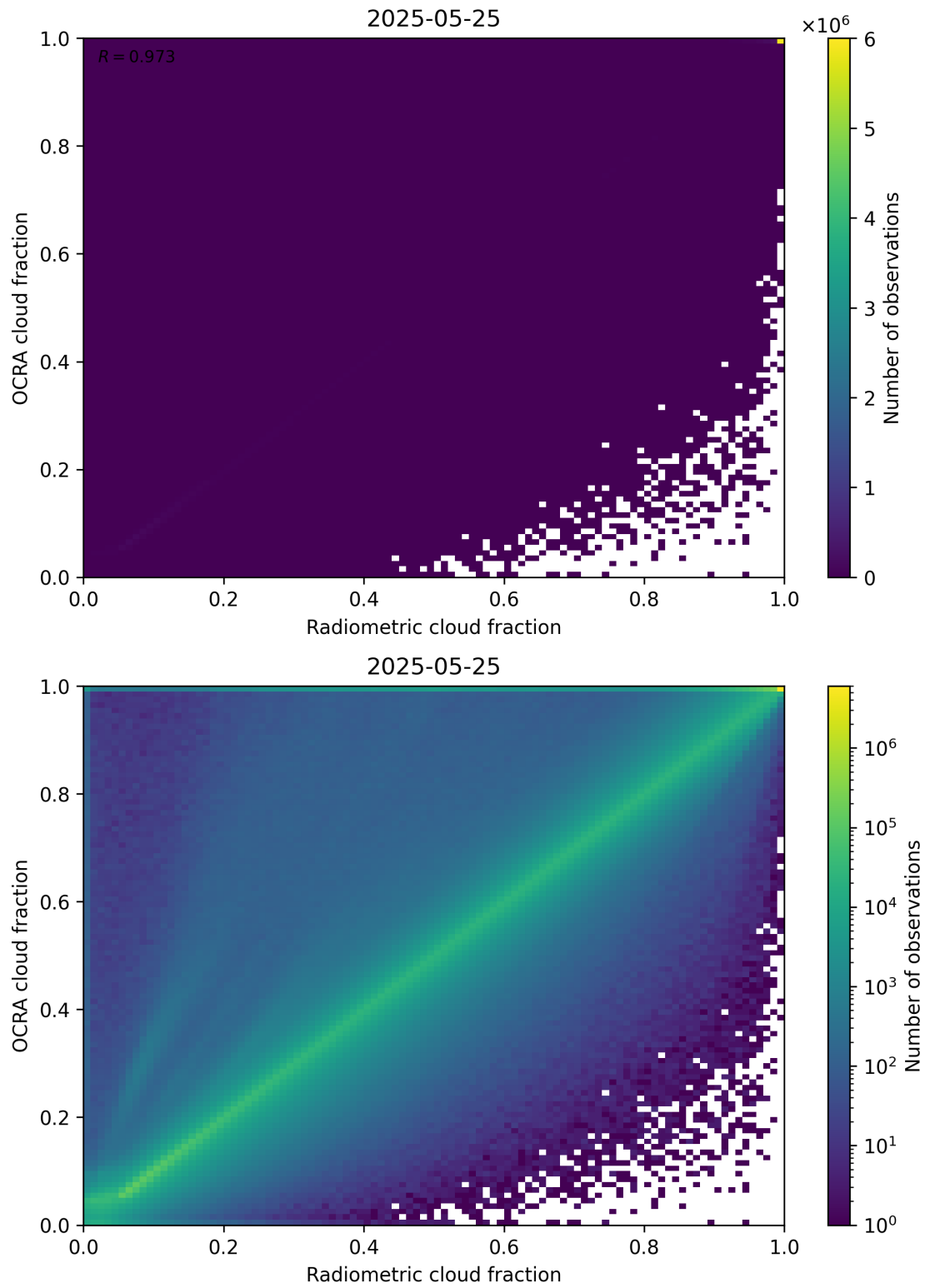
Figure 72: Scatter density plot of “Radiometric cloud fraction” against “OCRA cloud fraction” for 2025-05-24 to 2025-05-26.
