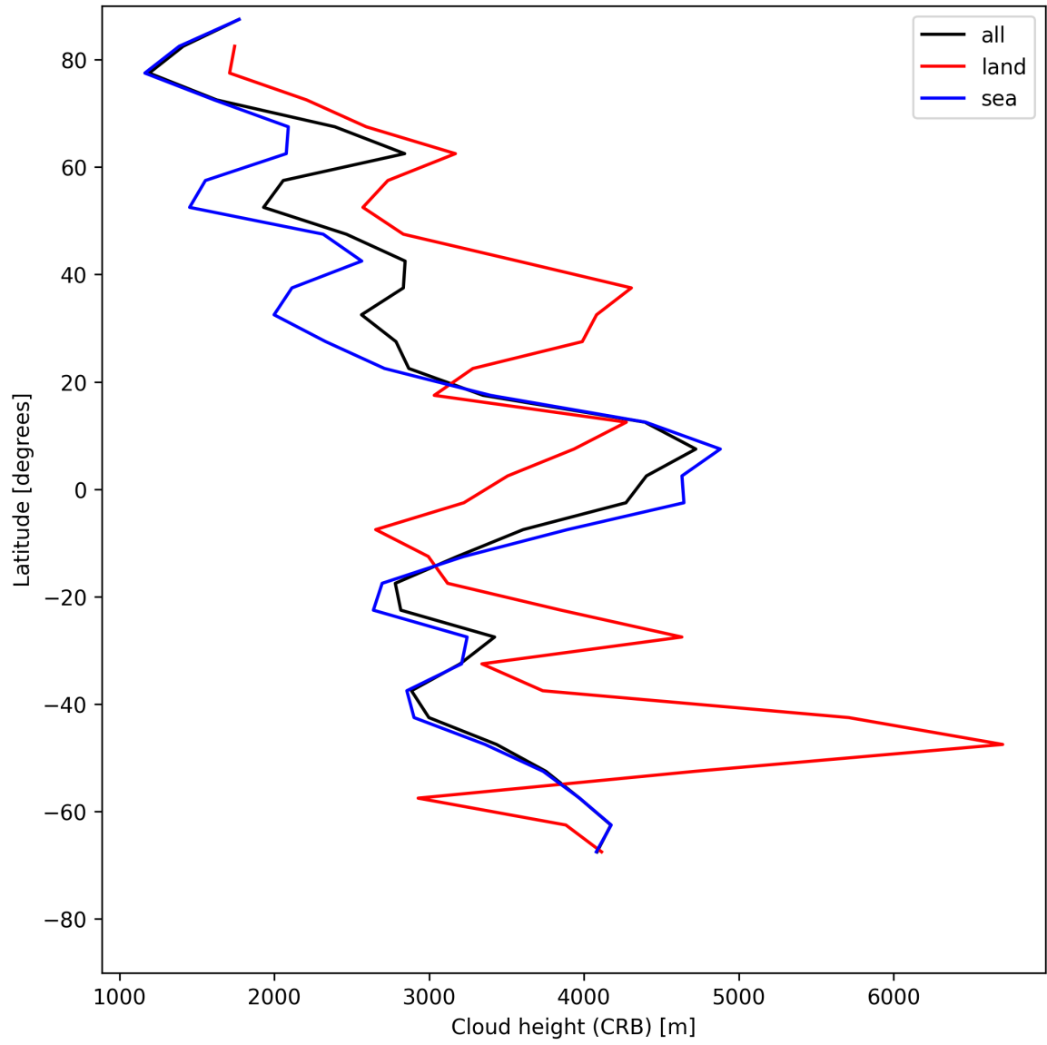
Figure 27: Zonal average of “Cloud height (CRB)” for 2025-05-24 to 2025-05-26.
