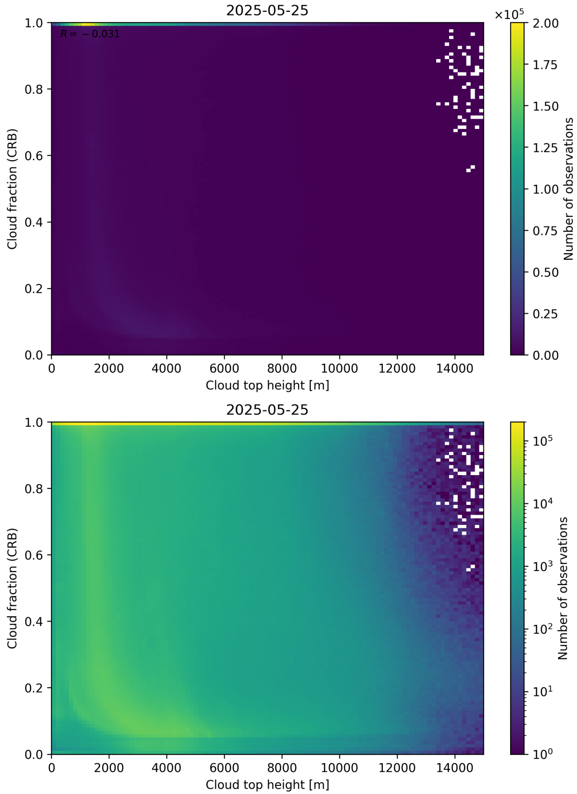
Figure 88: Scatter density plot of “Cloud top height” against “Cloud fraction (CRB)” for 2025-05-24 to 2025-05-26.
