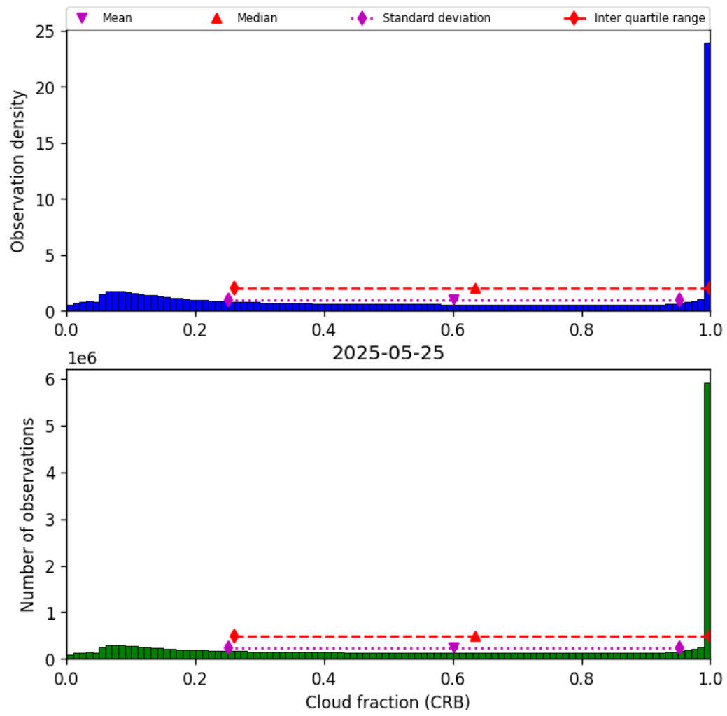
Figure 42: Histogram of “Cloud fraction (CRB)” for 2025-05-24 to 2025-05-26
