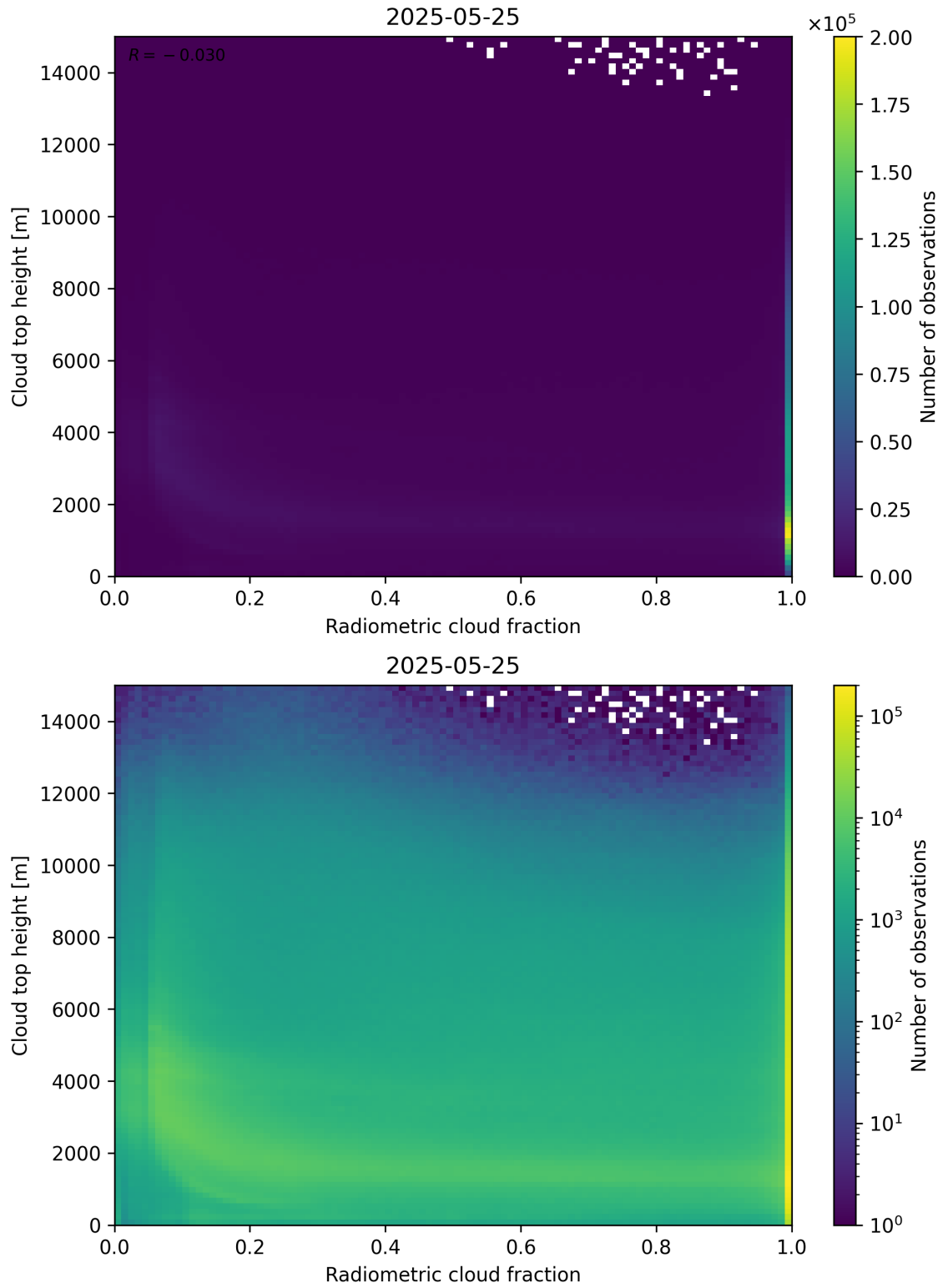
Figure 76: Scatter density plot of “Radiometric cloud fraction” against “Cloud top height” for 2025-05-24 to 2025-05-26.
