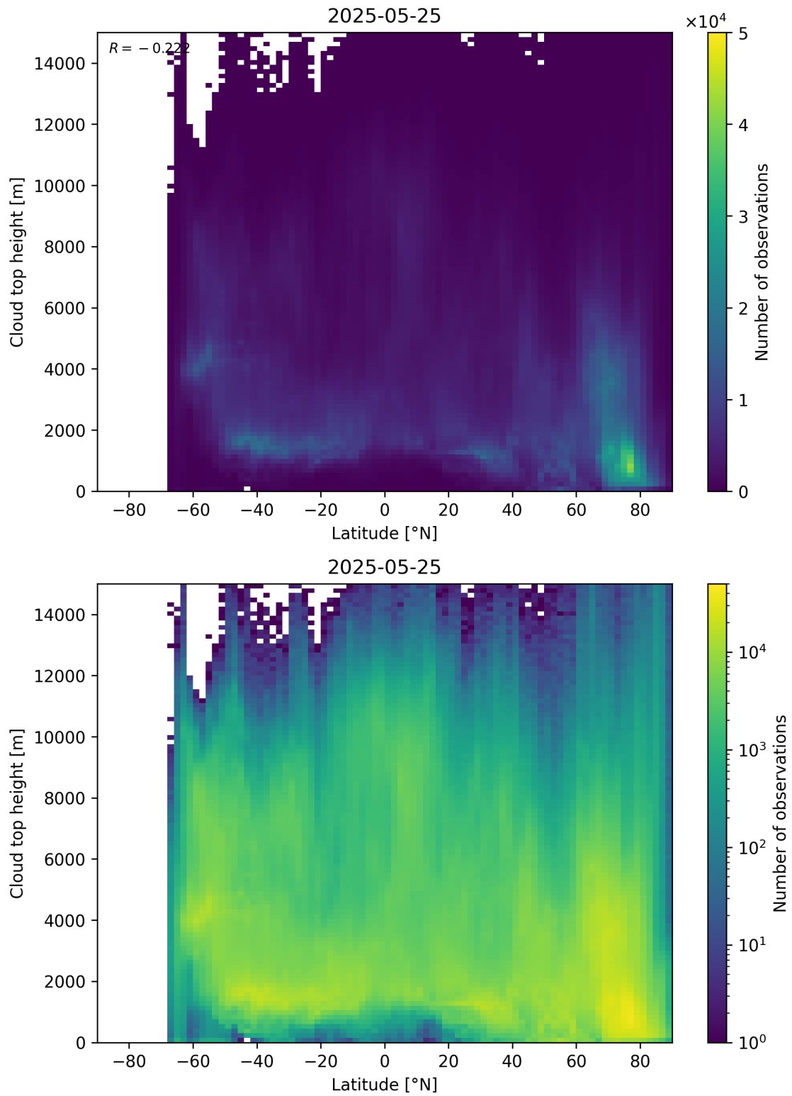
Figure 97: Scatter density plot of “Latitude” against “Cloud top height” for 2025-05-24 to 2025-05-26.
