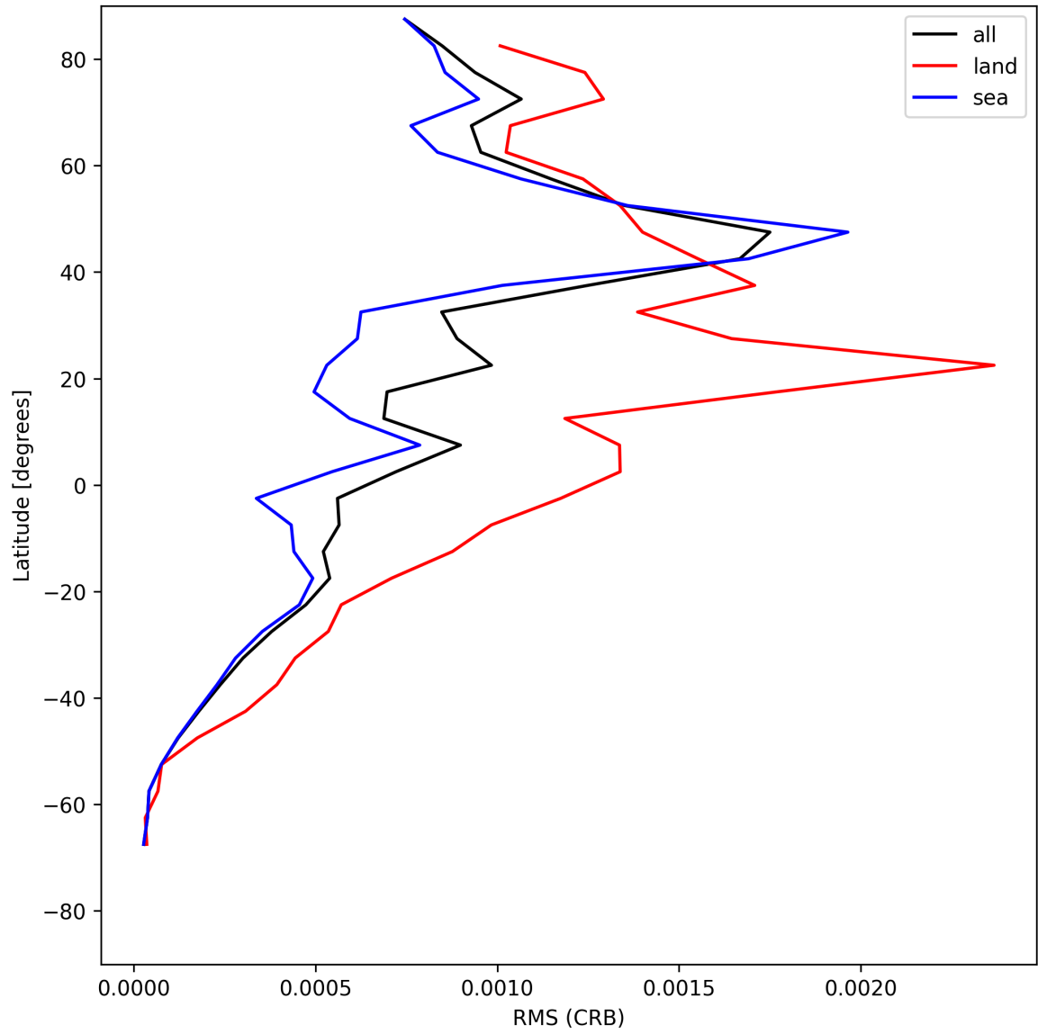
Figure 32: Zonal average of “RMS (CRB)” for 2025-05-24 to 2025-05-26.
