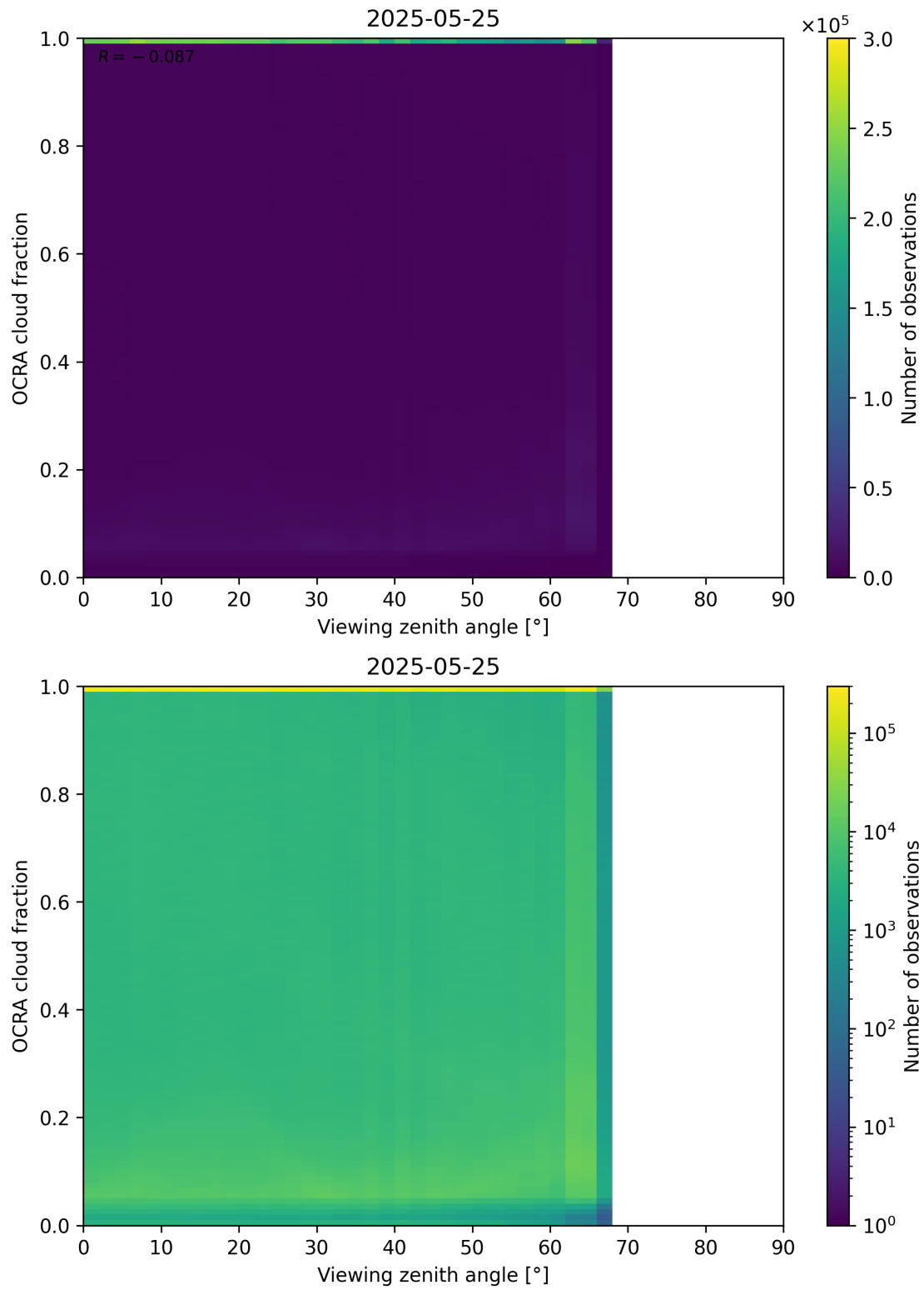
Figure 108: Scatter density plot of “Viewing zenith angle” against “OCRA cloud fraction” for 2025-05-24 to 2025-05-26.
