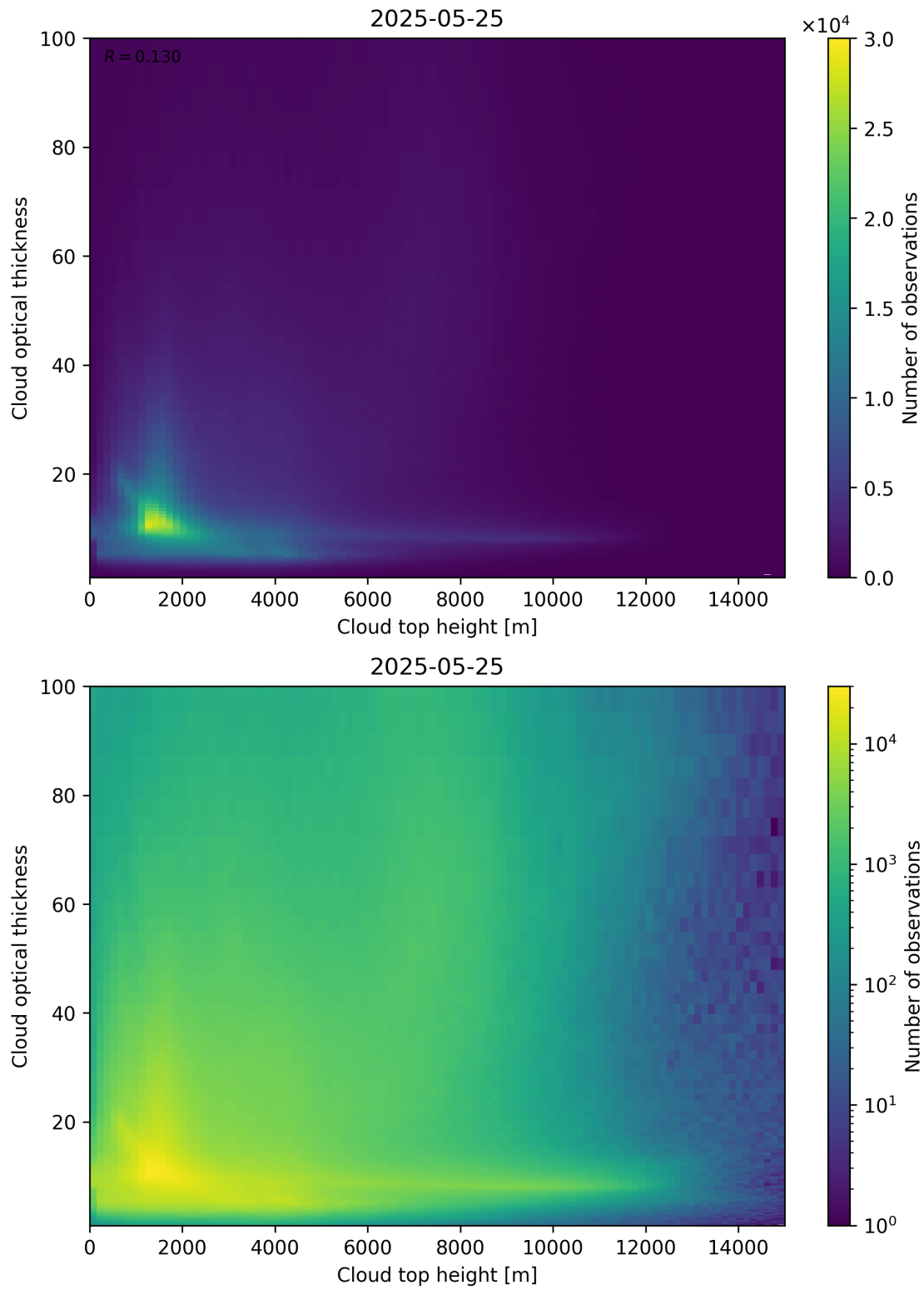
Figure 90: Scatter density plot of “Cloud top height” against “Cloud optical thickness” for 2025-05-24 to 2025-05-26.
