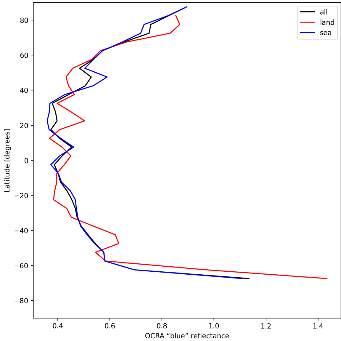
Figure 35: Zonal average of "OCRA "blue" reflectance" for 2025-05-24 to 2025-05-26.
