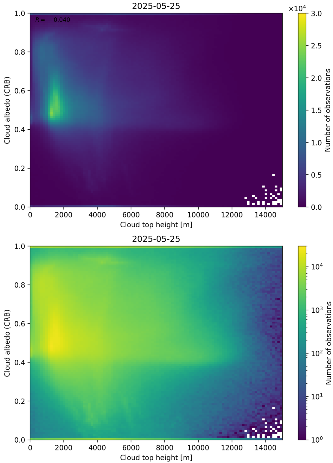
Figure 86: Scatter density plot of “Cloud top height” against “Cloud albedo (CRB)” for 2025-05-24 to 2025-05-26.
