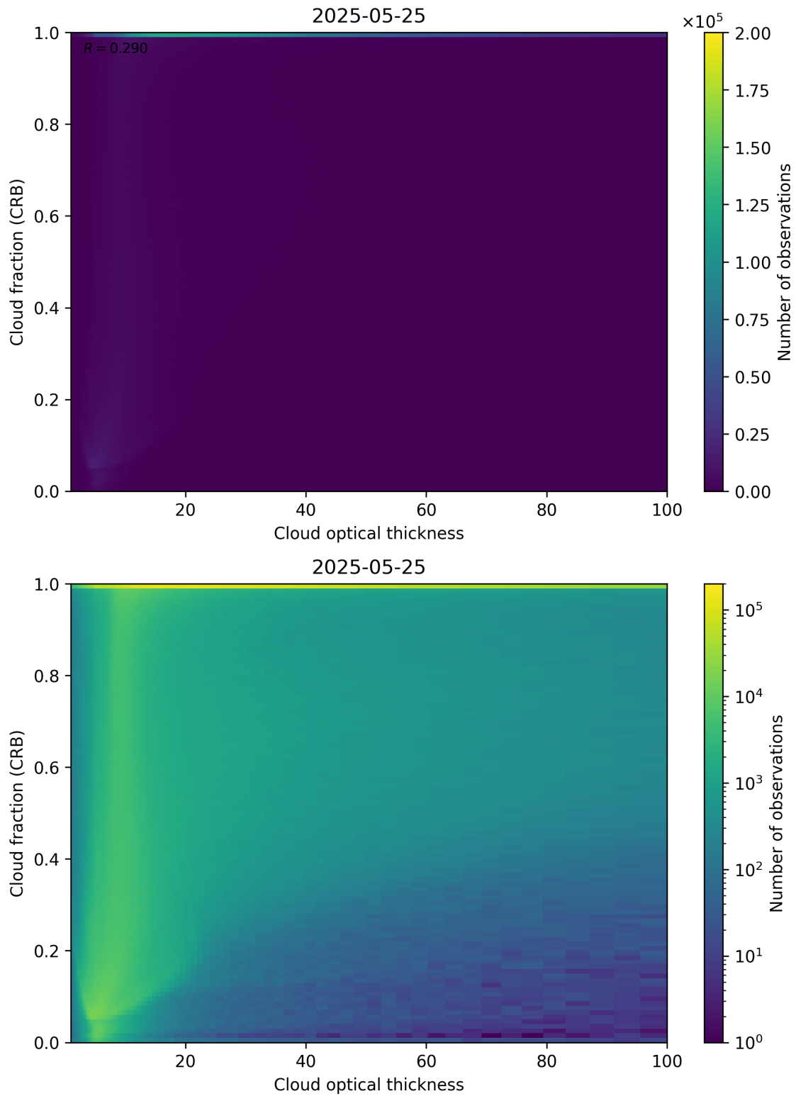
Figure 84: Scatter density plot of “Cloud optical thickness” against “Cloud fraction (CRB)” for 2025-05-24 to 2025-05-26.
