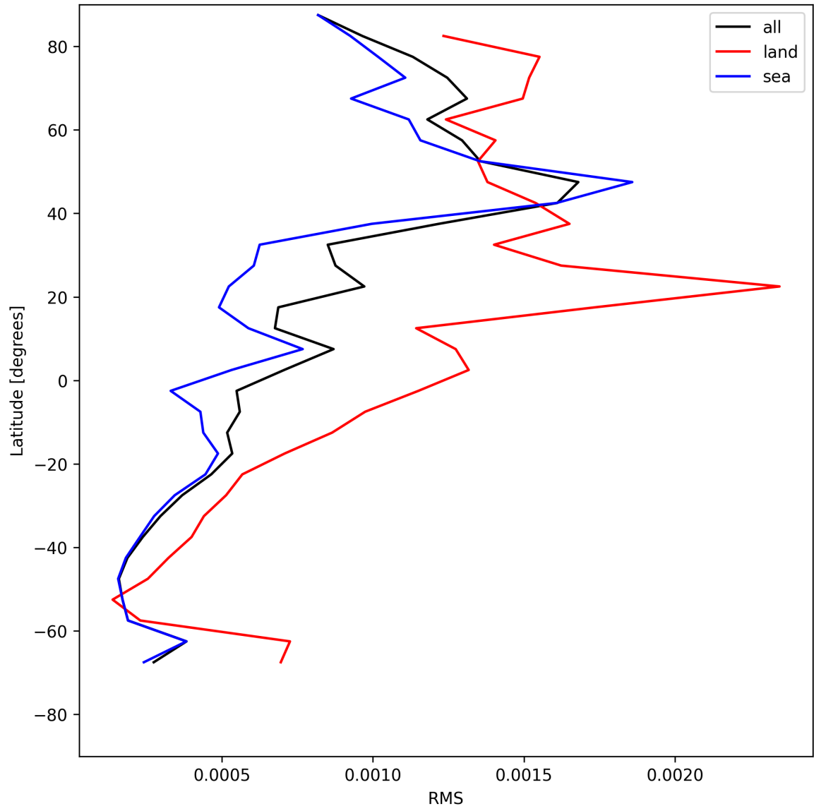
Figure 31: Zonal average of “RMS” for 2025-05-24 to 2025-05-26.
