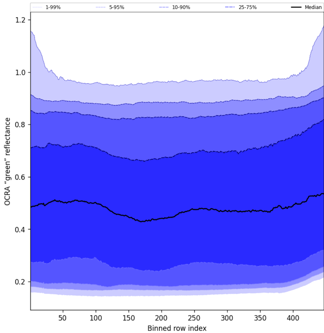
Figure 68: Along track statistics of “OCRA “green” reflectance” for 2025-05-24 to 2025-05-26
