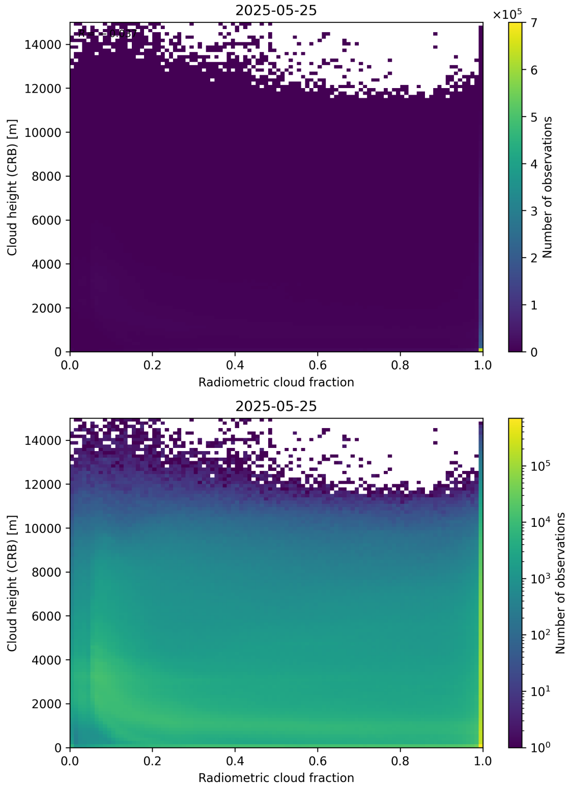
Figure 74: Scatter density plot of “Radiometric cloud fraction” against “Cloud height (CRB)” for 2025-05-24 to 2025-05-26.
