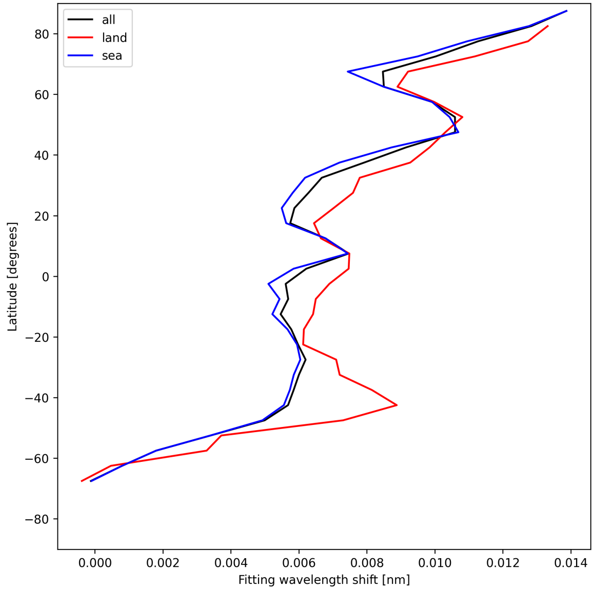
Figure 33: Zonal average of “Fitting wavelength shift” for 2025-05-24 to 2025-05-26.
