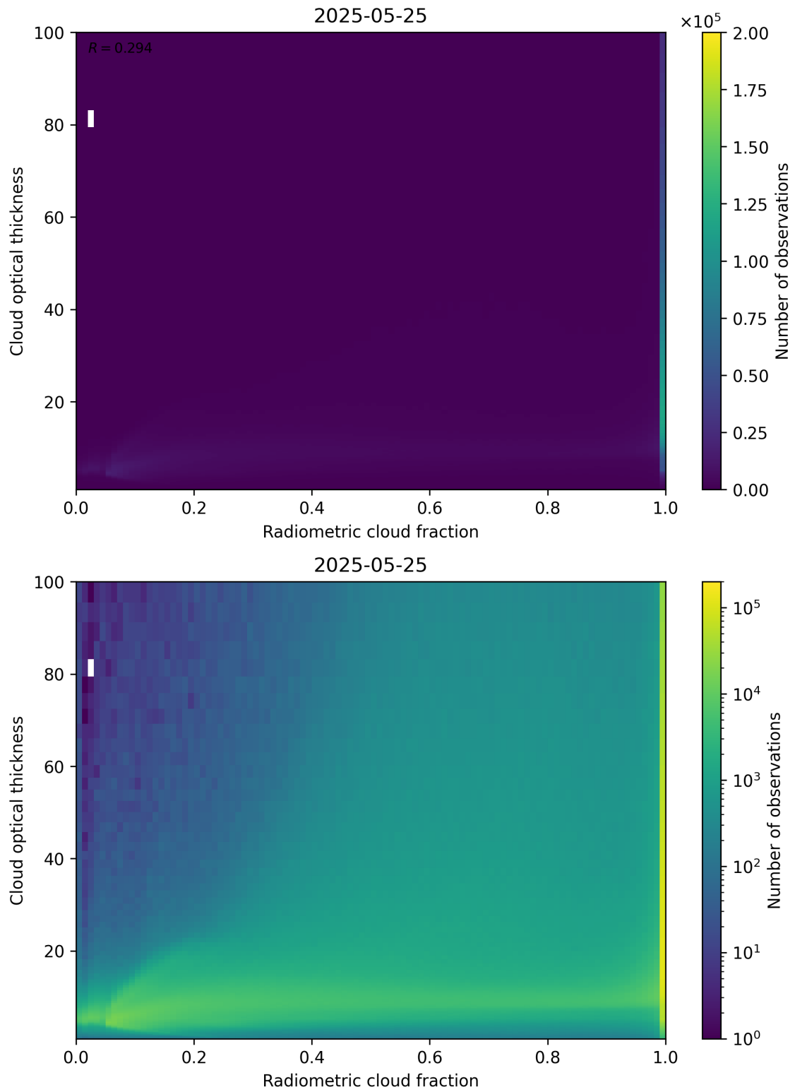
Figure 75: Scatter density plot of “Radiometric cloud fraction” against “Cloud optical thickness” for 2025-05-24 to 2025-05-26.
