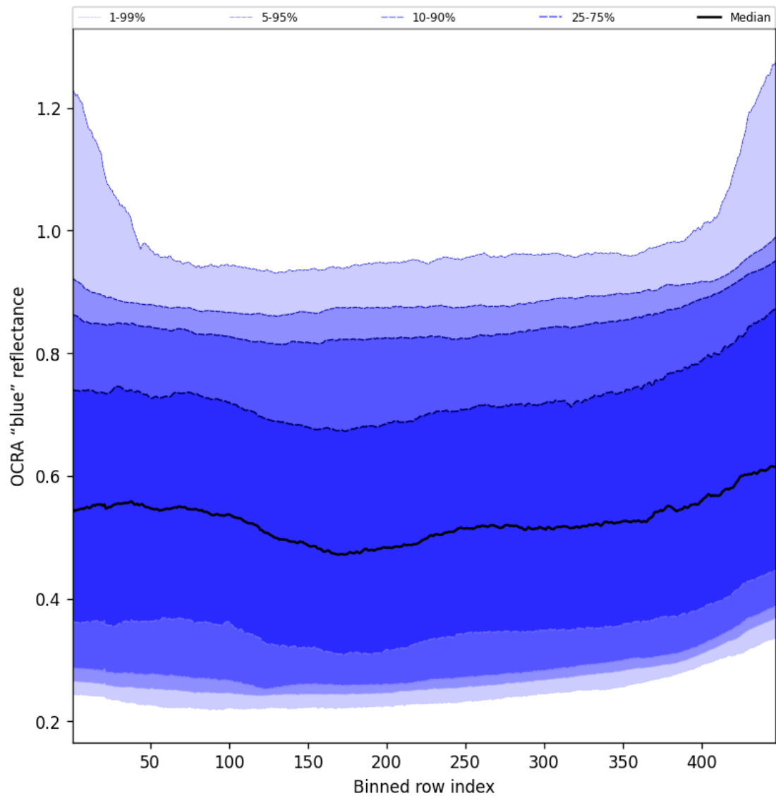
Figure 67: Along track statistics of “OCRA “blue” reflectance” for 2025-05-24 to 2025-05-26
