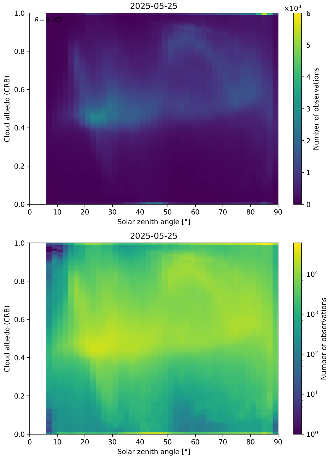
Figure 98: Scatter density plot of “Solar zenith angle” against “Cloud albedo (CRB)” for 2025-05-24 to 2025-05-26.
