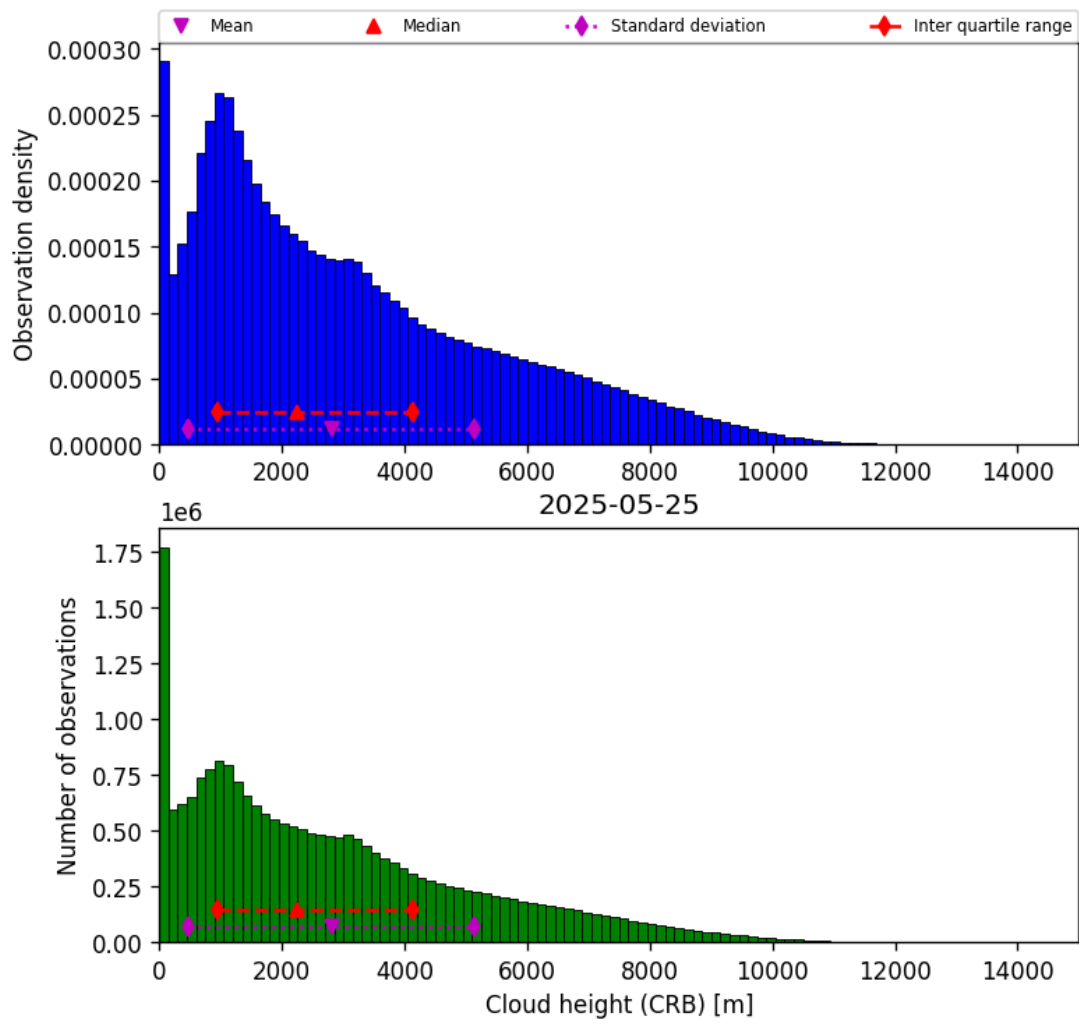
Figure 43: Histogram of “Cloud height (CRB)” for 2025-05-24 to 2025-05-26
