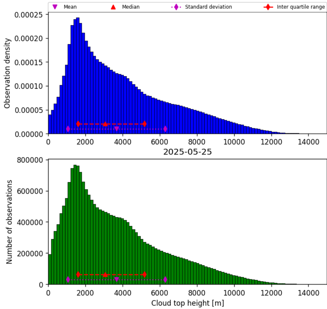
Figure 40: Histogram of “Cloud top height” for 2025-05-24 to 2025-05-26
