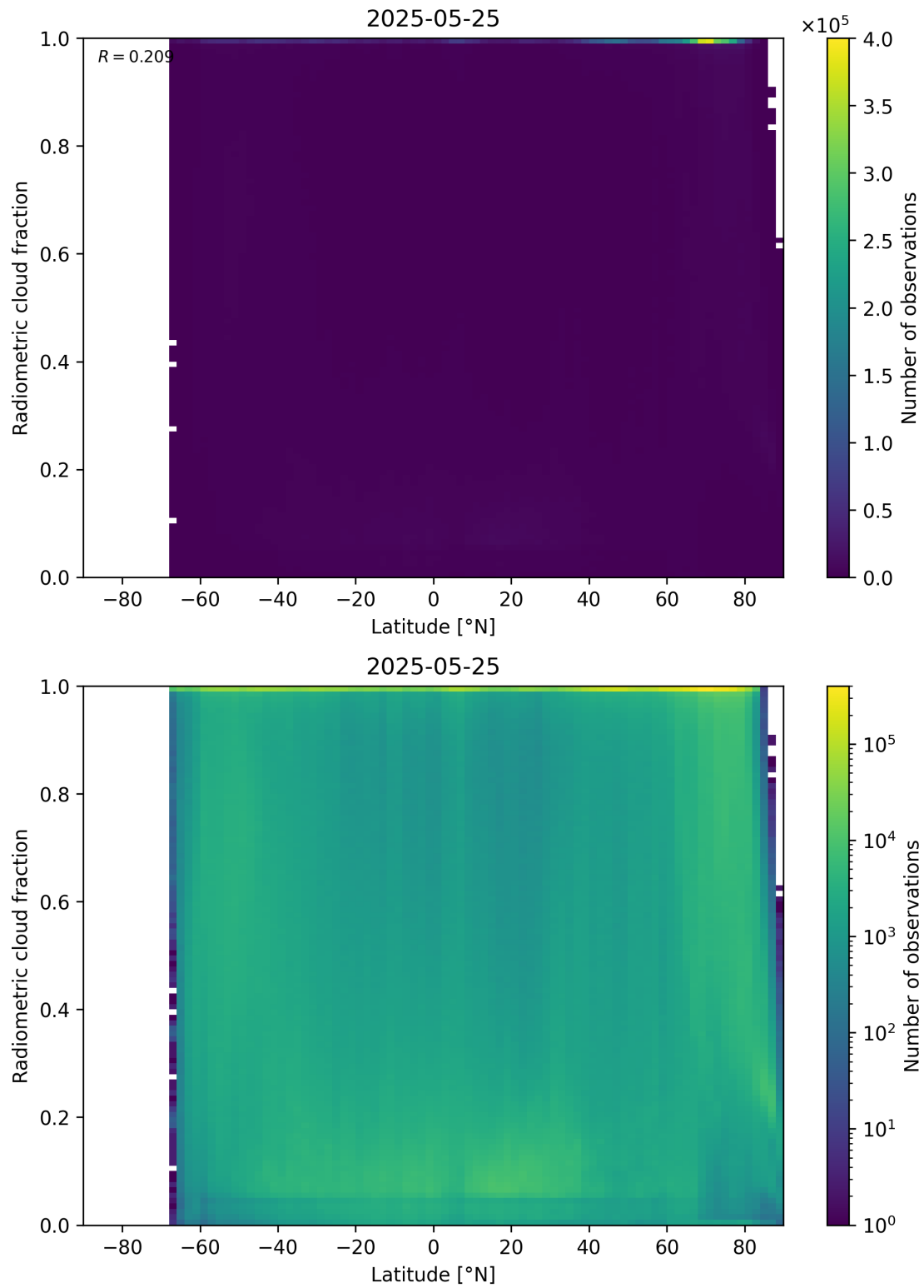
Figure 92: Scatter density plot of “Latitude” against “Radiometric cloud fraction” for 2025-05-24 to 2025-05-26.
