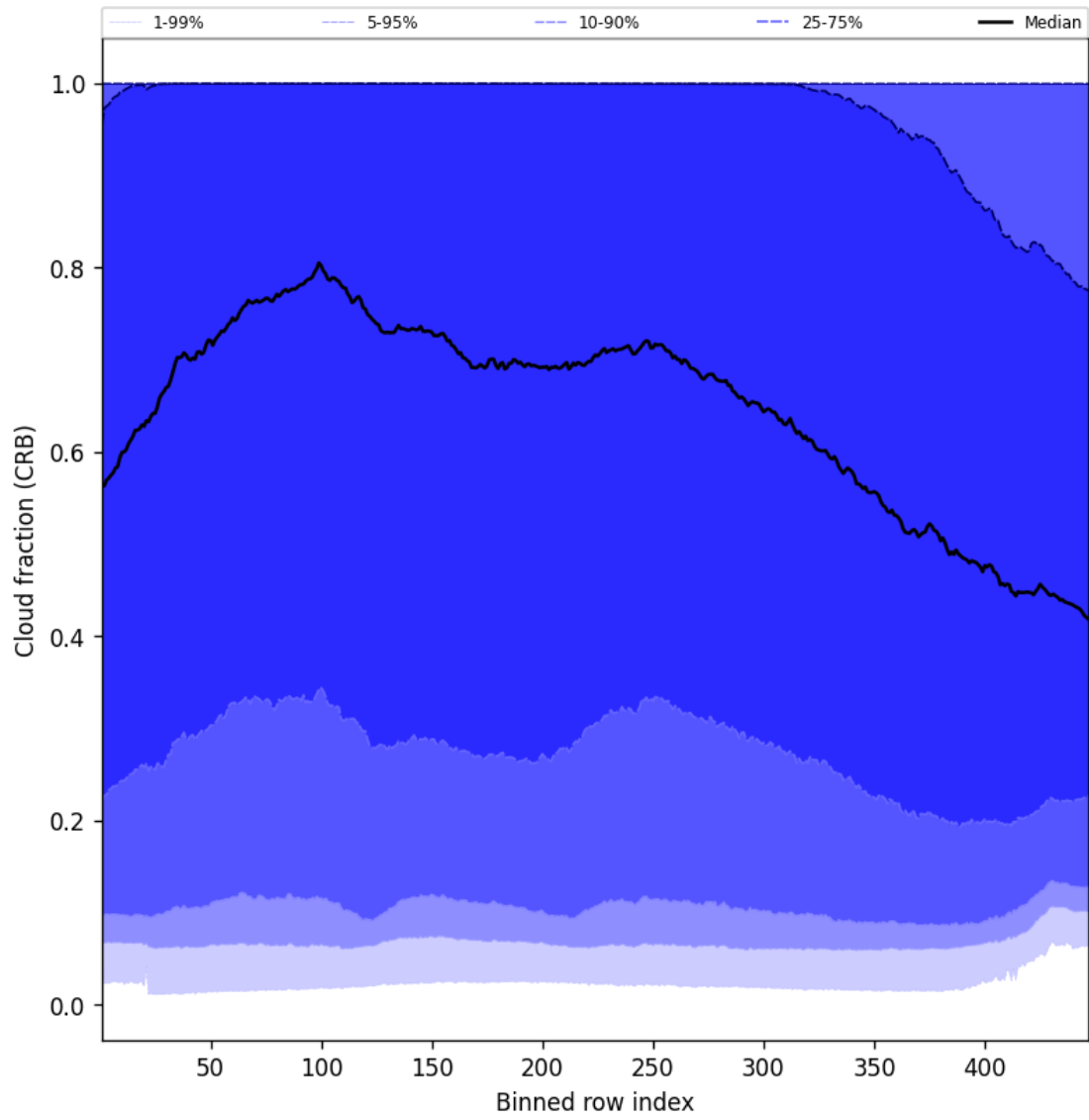
Figure 58: Along track statistics of “Cloud fraction (CRB)” for 2025-05-24 to 2025-05-26
