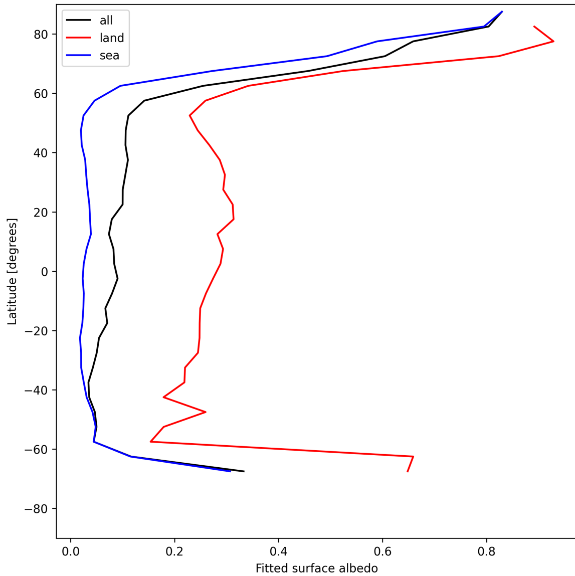
Figure 29: Zonal average of “Fitted surface albedo” for 2025-05-24 to 2025-05-26.
