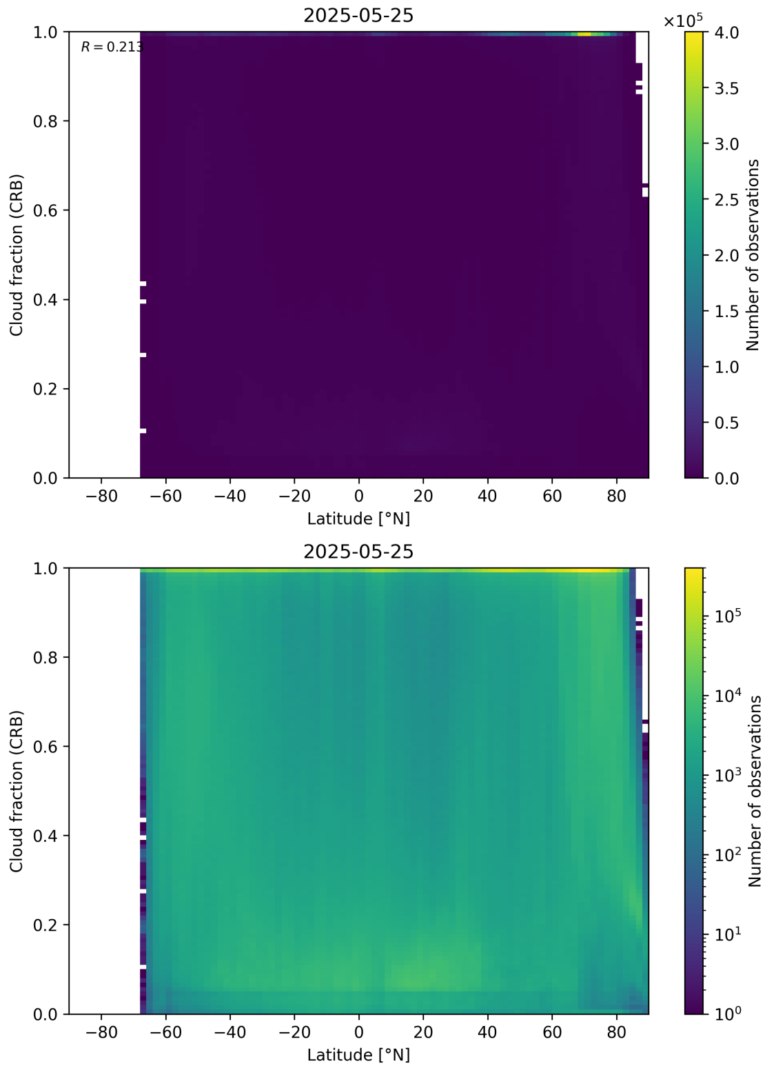
Figure 94: Scatter density plot of “Latitude” against “Cloud fraction (CRB)” for 2025-05-24 to 2025-05-26.
