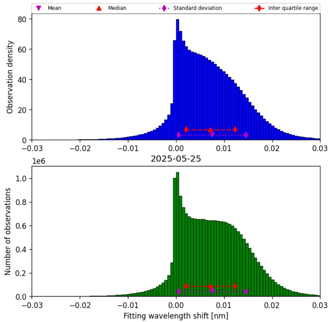
Figure 49: Histogram of “Fitting wavelength shift” for 2025-05-24 to 2025-05-26
