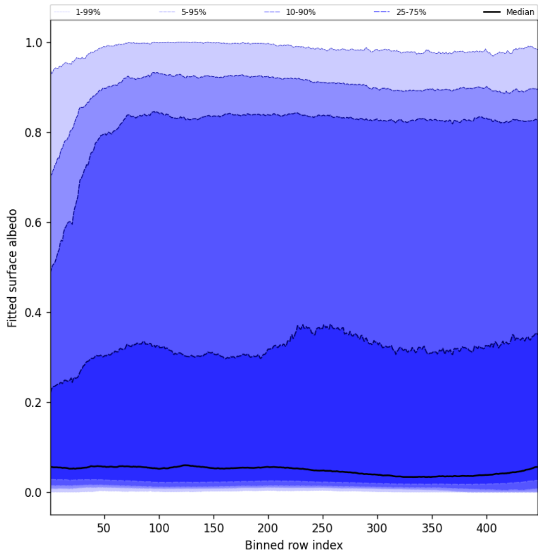
Figure 61: Along track statistics of “Fitted surface albedo” for 2025-05-24 to 2025-05-26
