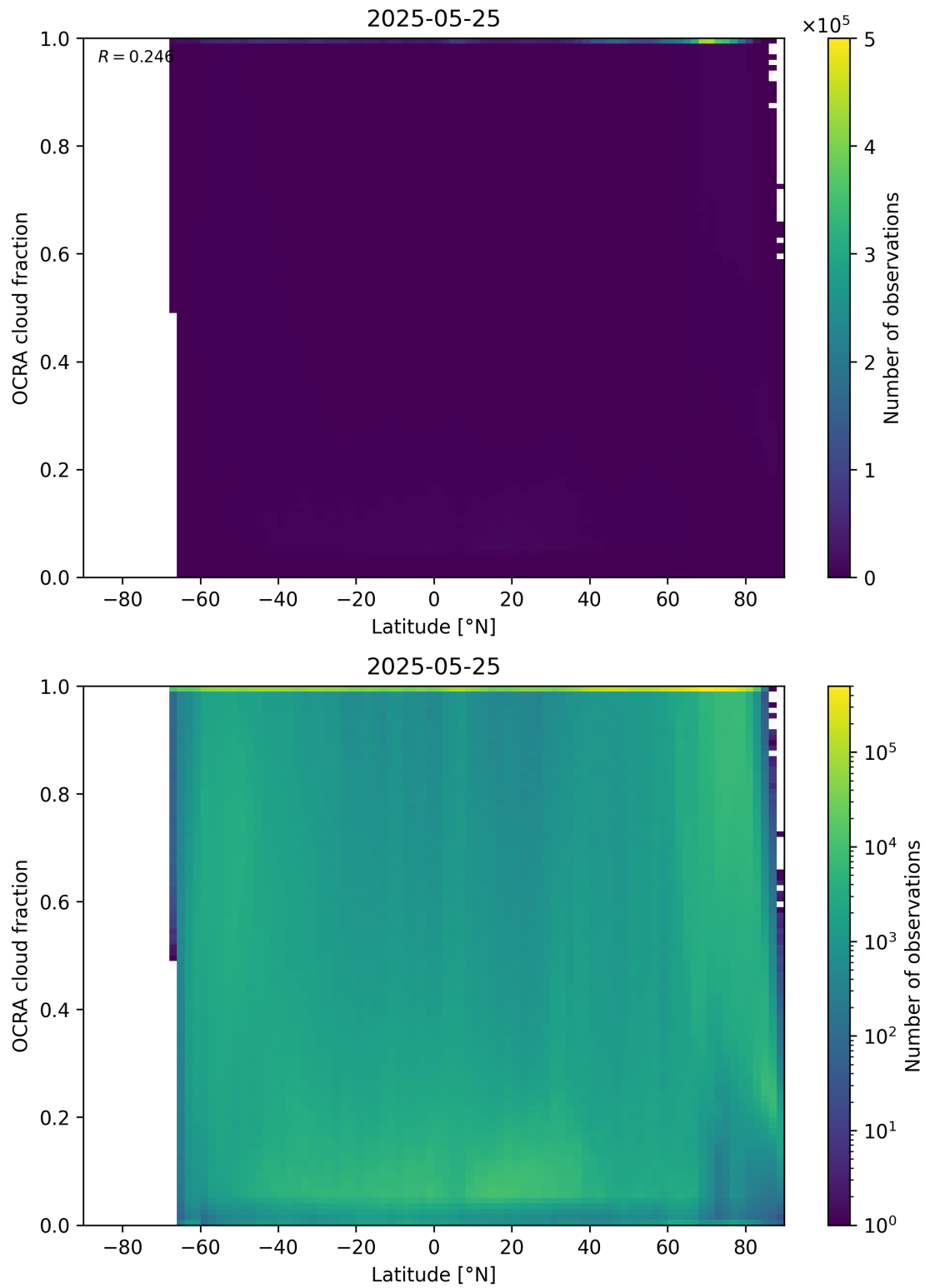
Figure 93: Scatter density plot of “Latitude” against “OCRA cloud fraction” for 2025-05-24 to 2025-05-26.
