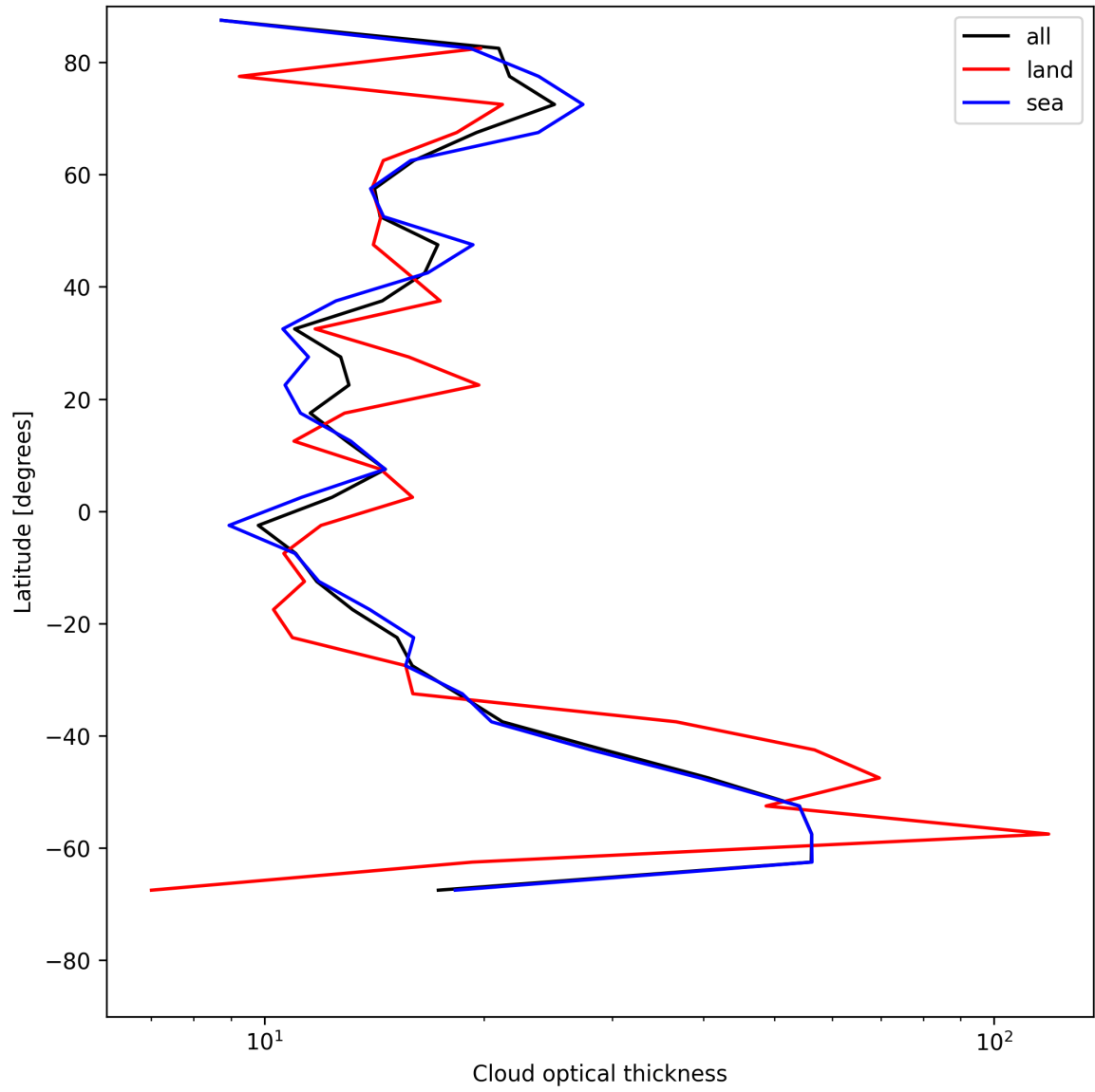
Figure 25: Zonal average of “Cloud optical thickness” for 2025-05-24 to 2025-05-26.
