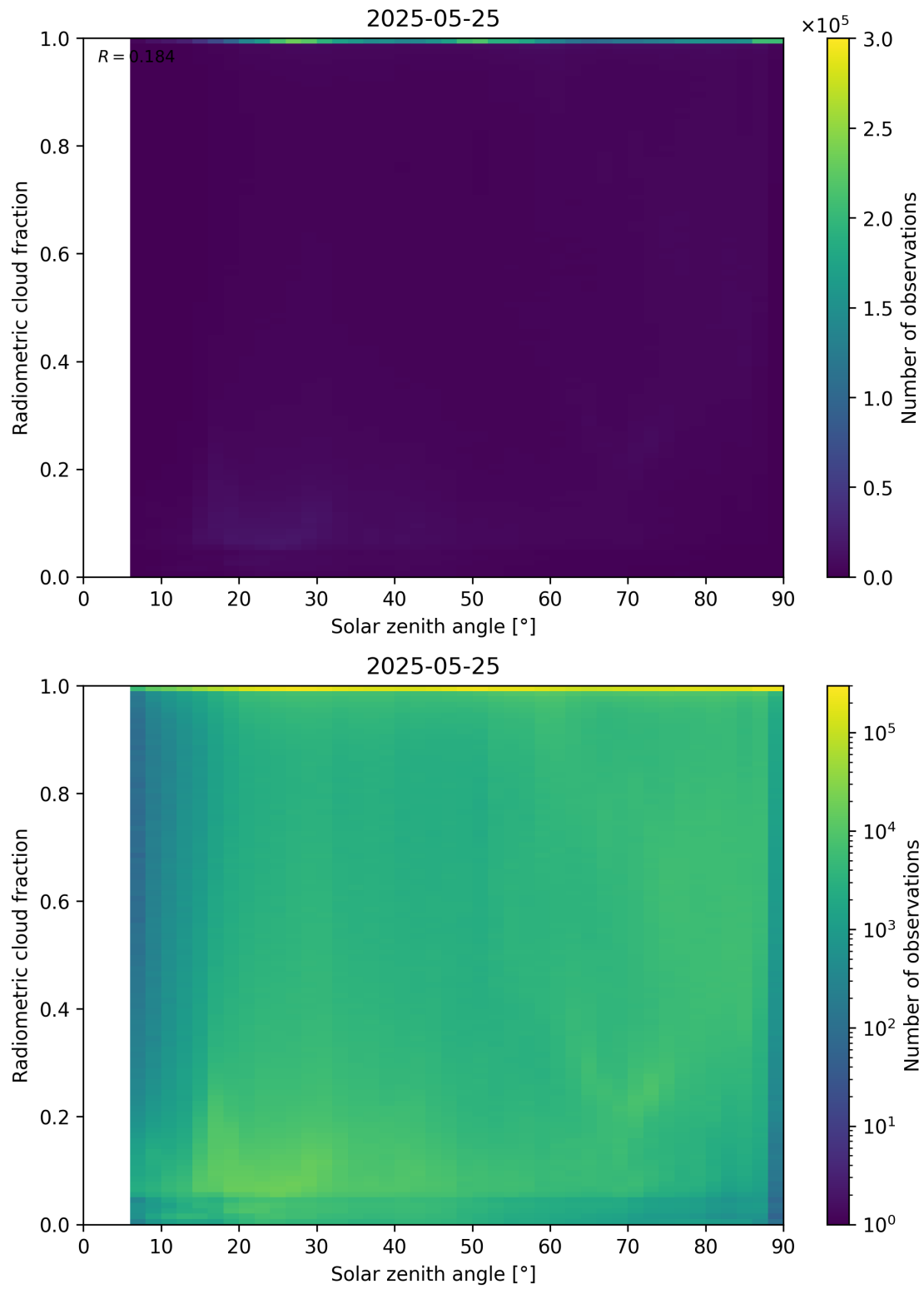
Figure 99: Scatter density plot of “Solar zenith angle” against “Radiometric cloud fraction” for 2025-05-24 to 2025-05-26.
