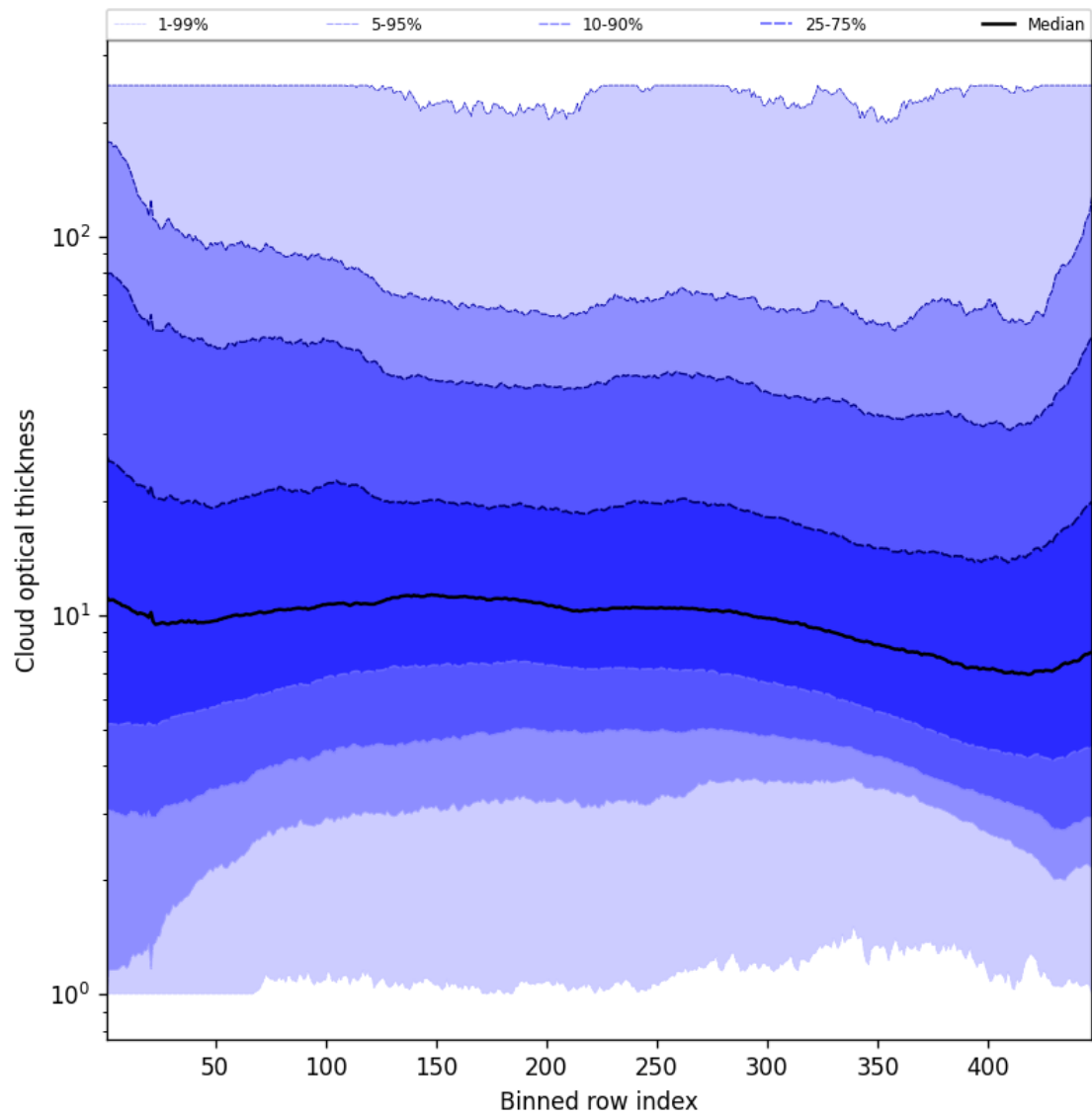
Figure 57: Along track statistics of “Cloud optical thickness” for 2025-05-24 to 2025-05-26
