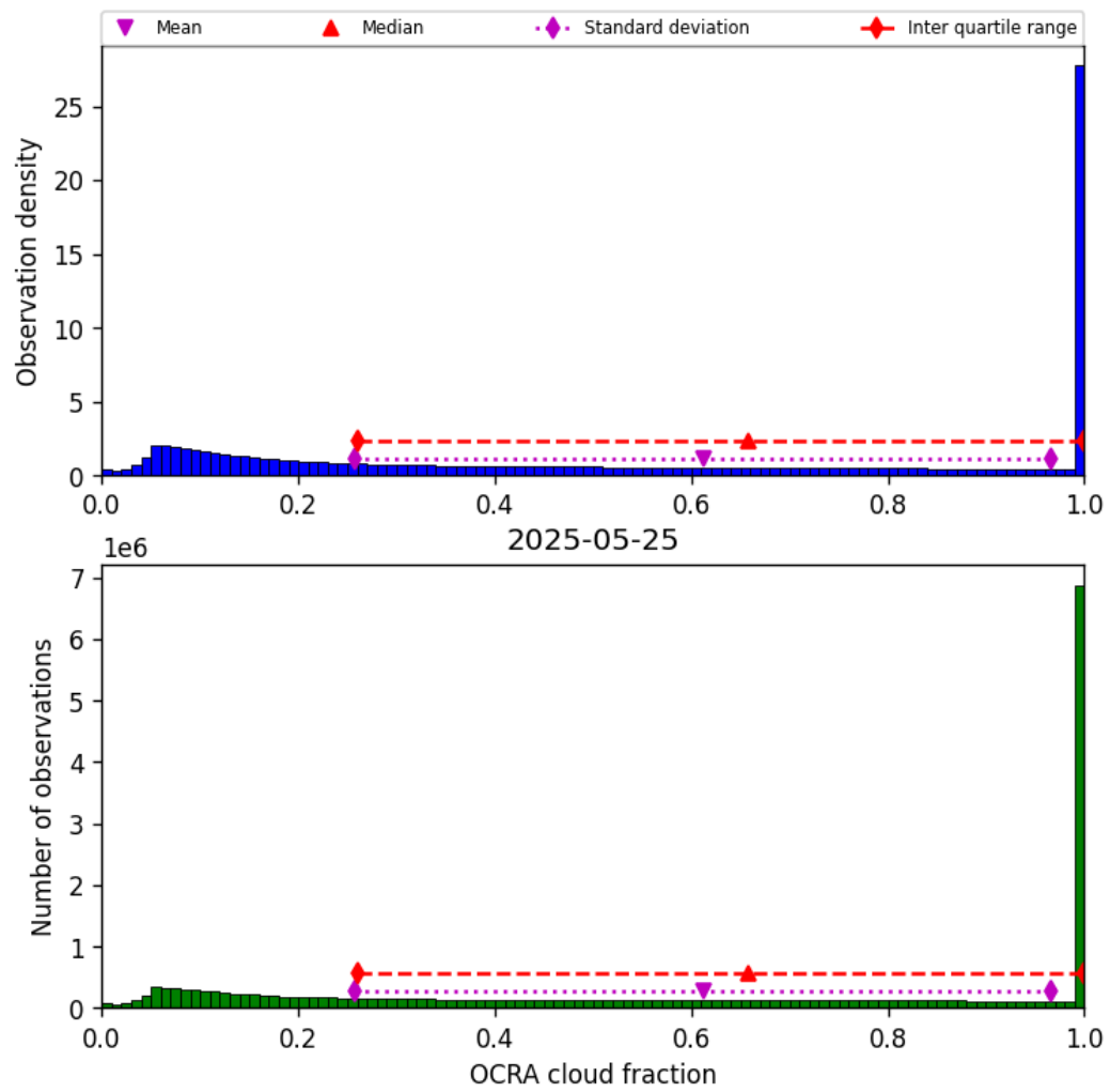
Figure 50: Histogram of “OCRA cloud fraction” for 2025-05-24 to 2025-05-26
