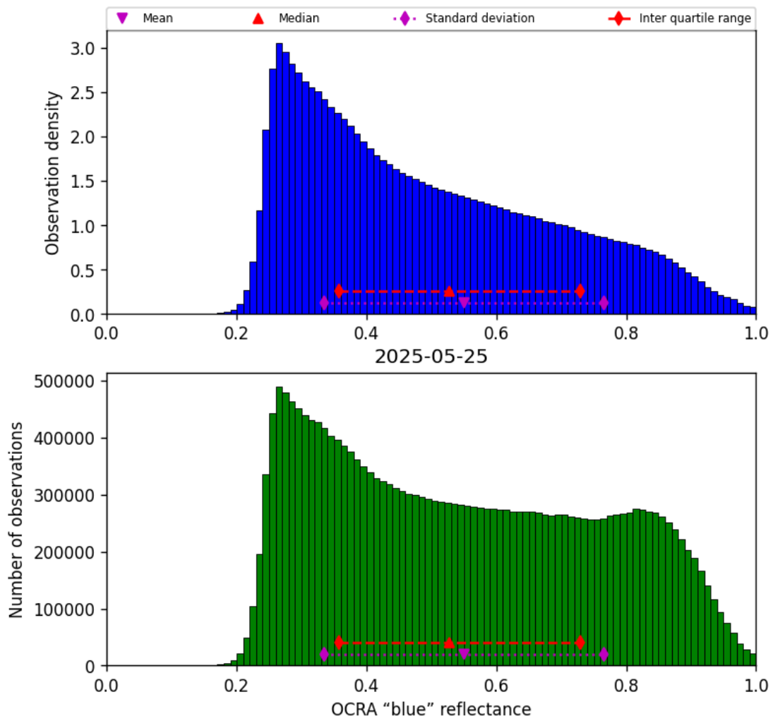
Figure 51: Histogram of “OCRA “blue” reflectance” for 2025-05-24 to 2025-05-26
