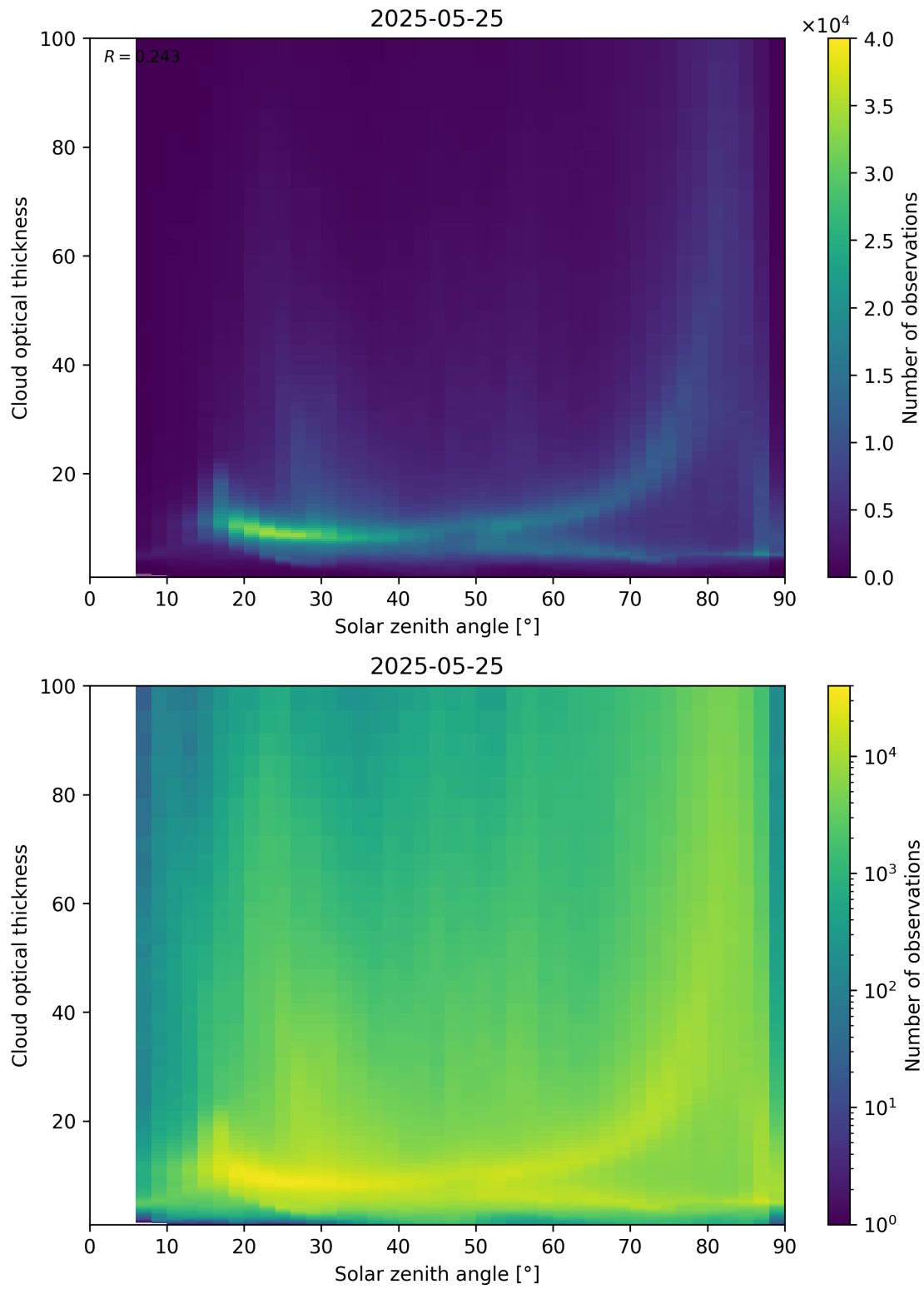
Figure 103: Scatter density plot of “Solar zenith angle” against “Cloud optical thickness” for 2025-05-24 to 2025-05-26.
