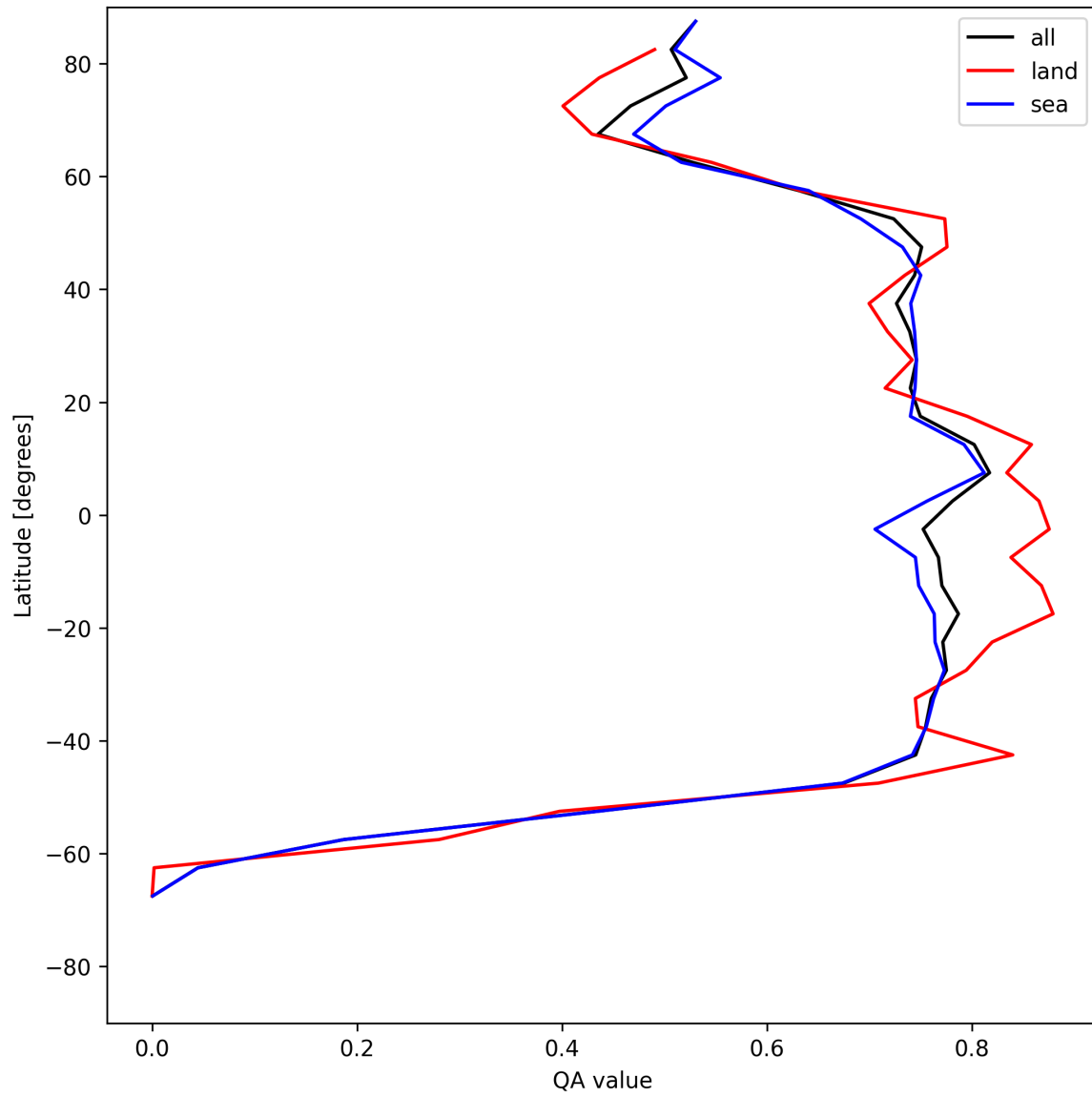
Figure 22: Zonal average of “QA value” for 2025-05-24 to 2025-05-26.
