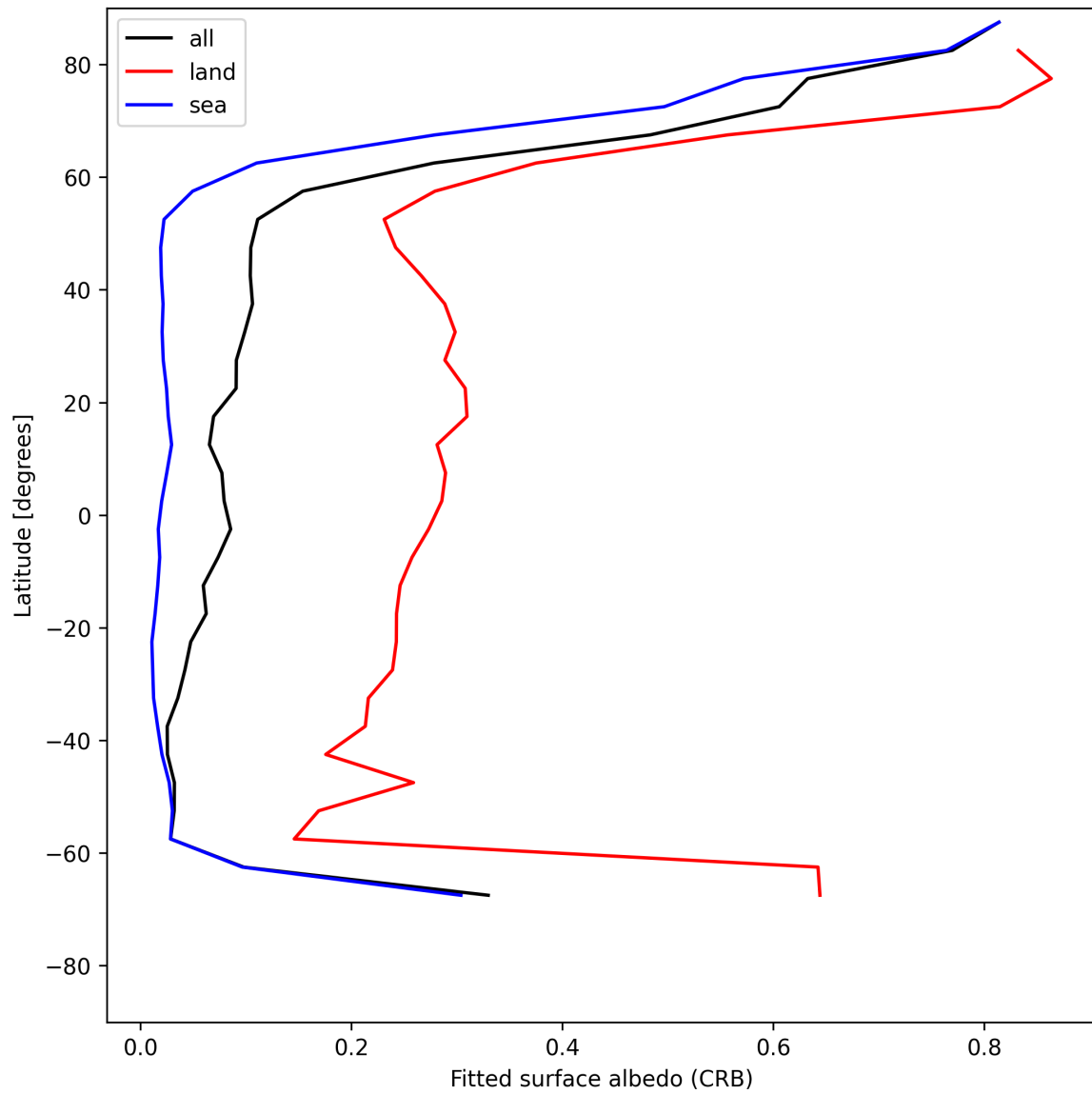
Figure 30: Zonal average of “Fitted surface albedo (CRB)” for 2025-05-24 to 2025-05-26.
