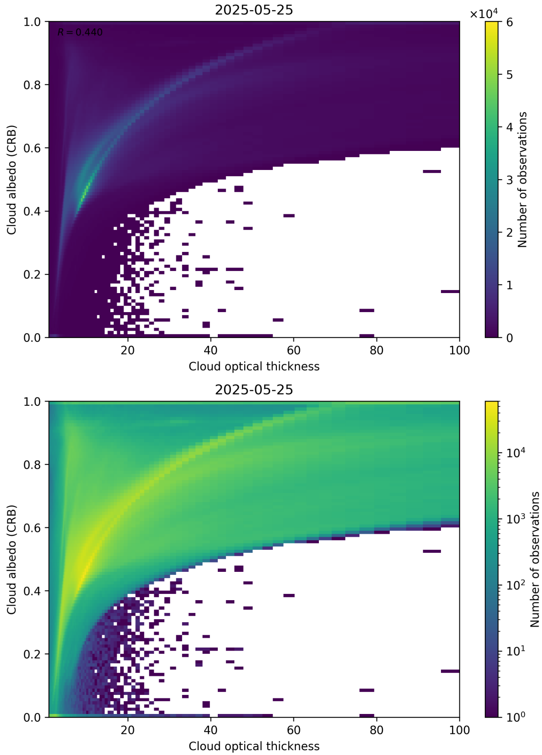
Figure 82: Scatter density plot of “Cloud optical thickness” against “Cloud albedo (CRB)” for 2025-05-24 to 2025-05-26.
