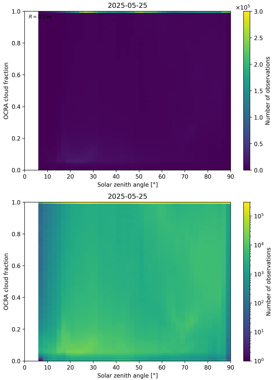
Figure 100: Scatter density plot of “Solar zenith angle” against “OCRA cloud fraction” for 2025-05-24 to 2025-05-26.
