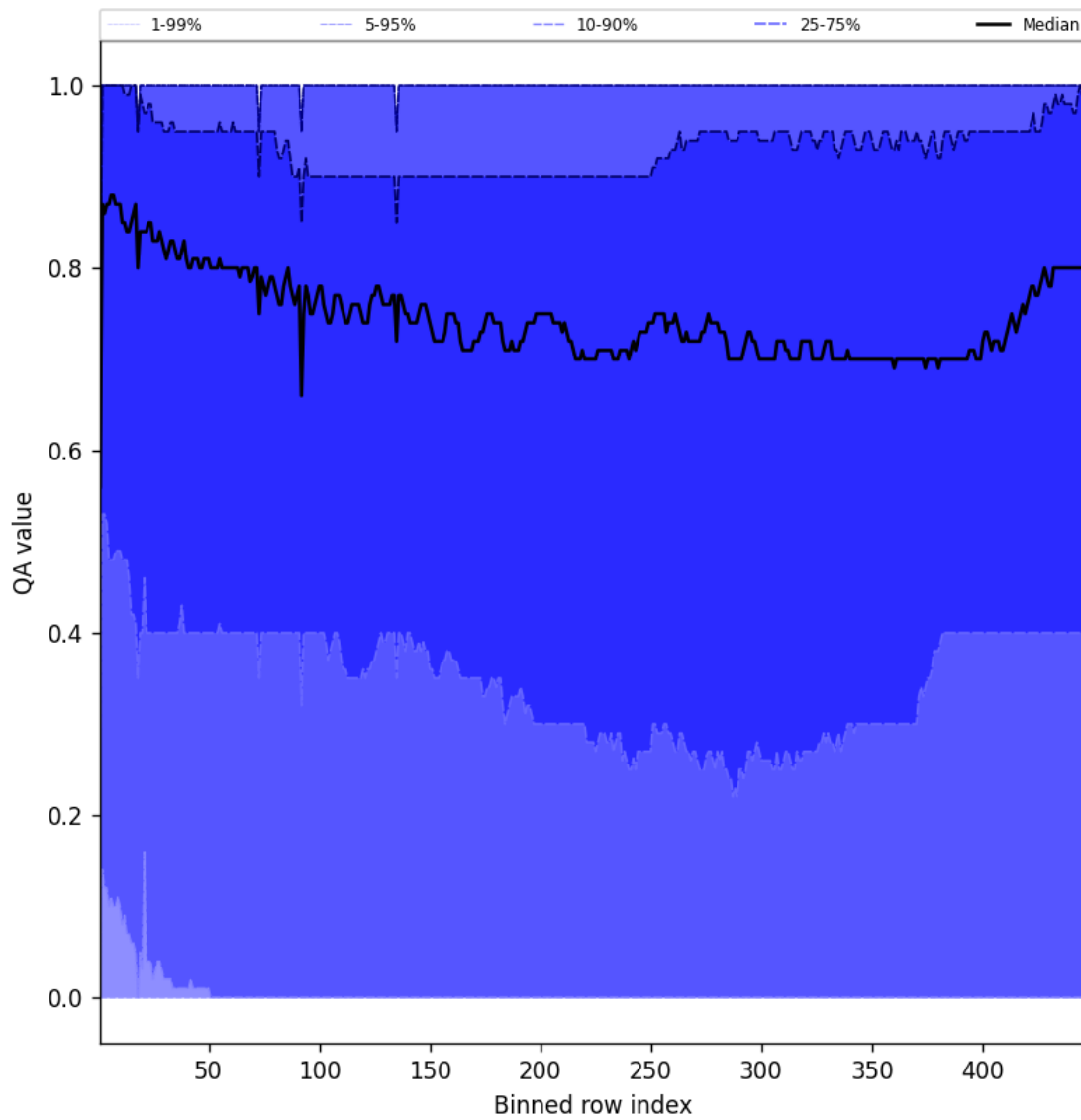
Figure 54: Along track statistics of “QA value” for 2025-05-24 to 2025-05-26
