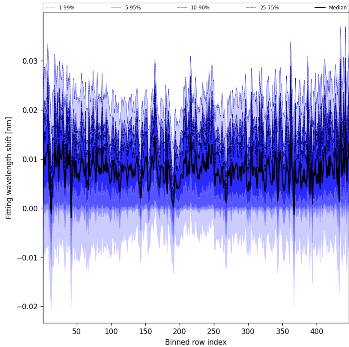
Figure 65: Along track statistics of “Fitting wavelength shift” for 2025-05-24 to 2025-05-26
