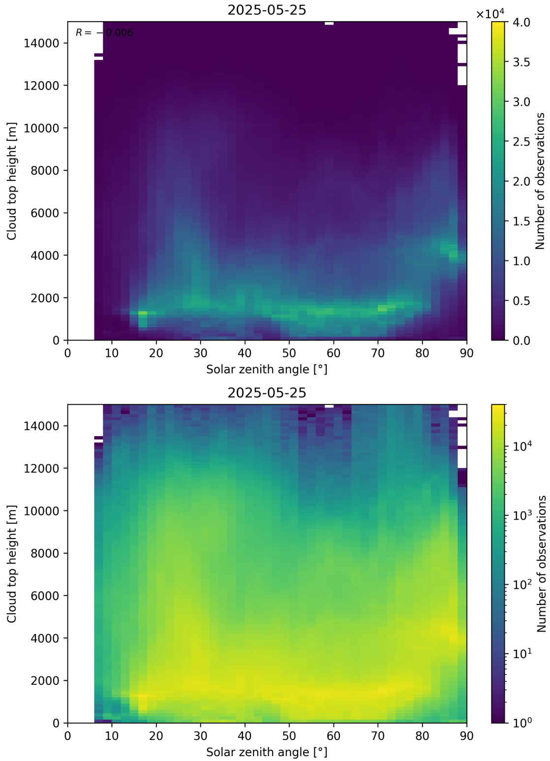
Figure 104: Scatter density plot of “Solar zenith angle” against “Cloud top height” for 2025-05-24 to 2025-05-26.
