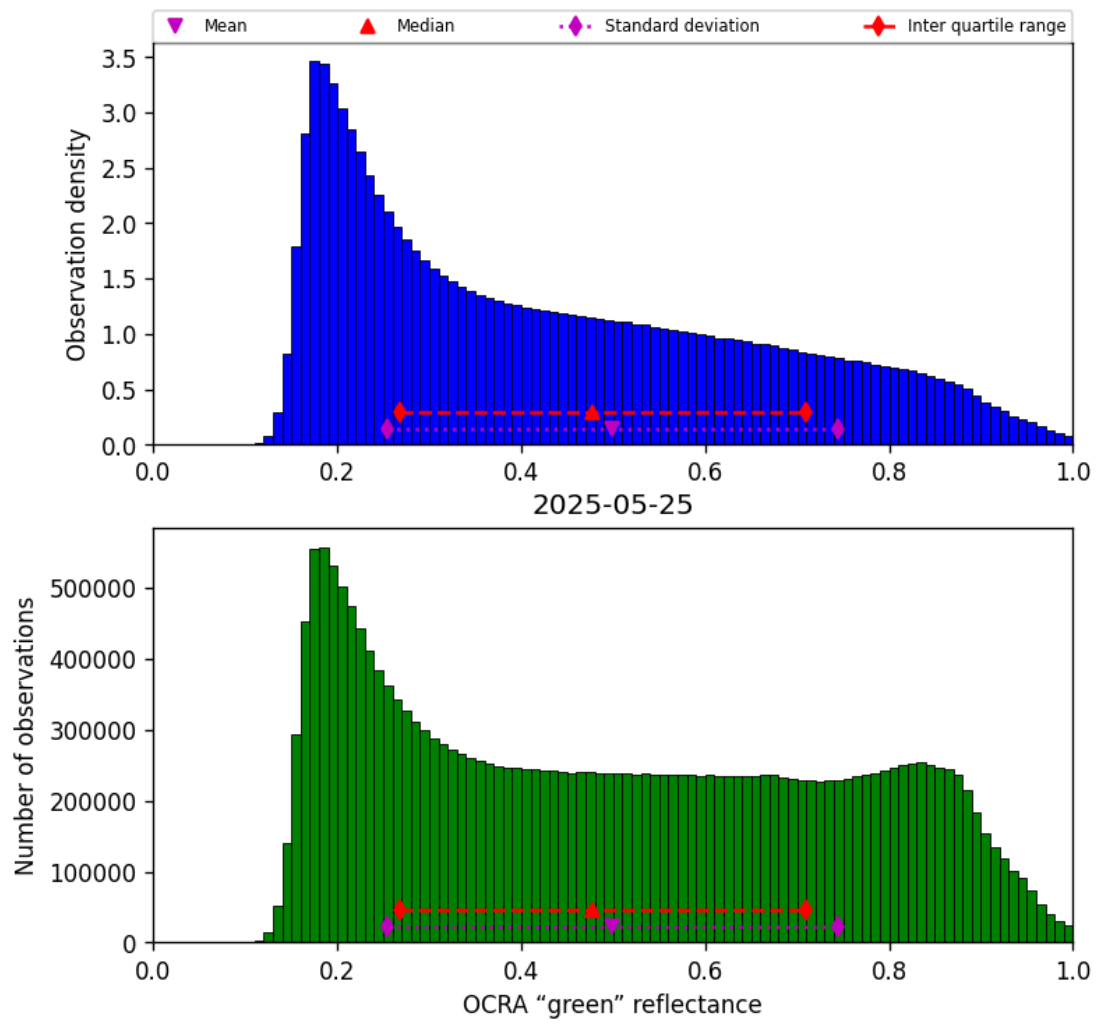
Figure 52: Histogram of “OCRA “green” reflectance” for 2025-05-24 to 2025-05-26
