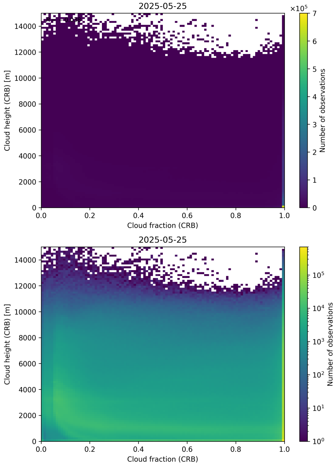
Figure 79: Scatter density plot of “Cloud fraction (CRB)” against “Cloud height (CRB)” for 2025-05-24 to 2025-05-26.
