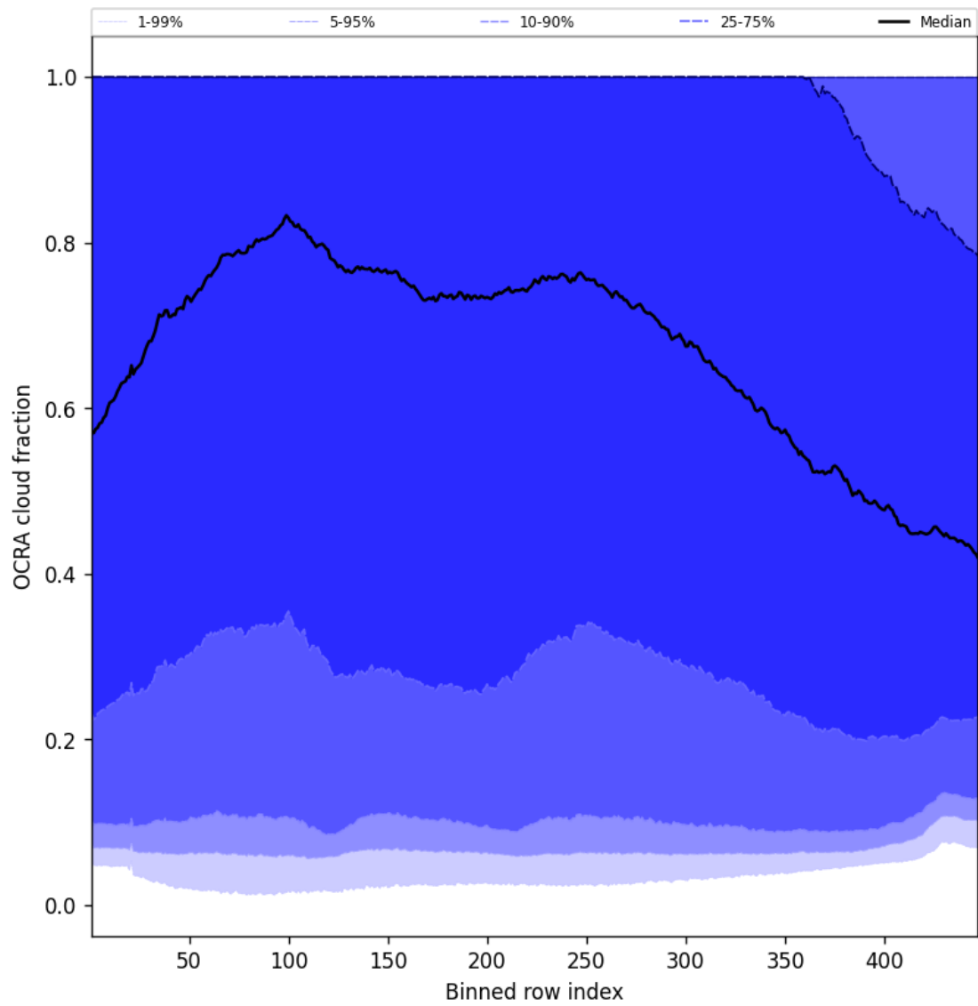
Figure 66: Along track statistics of “OCRA cloud fraction” for 2025-05-24 to 2025-05-26
