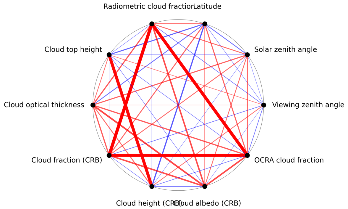
Figure 1: Map of correlation graph for 2025-05-24 to 2025-05-26.
