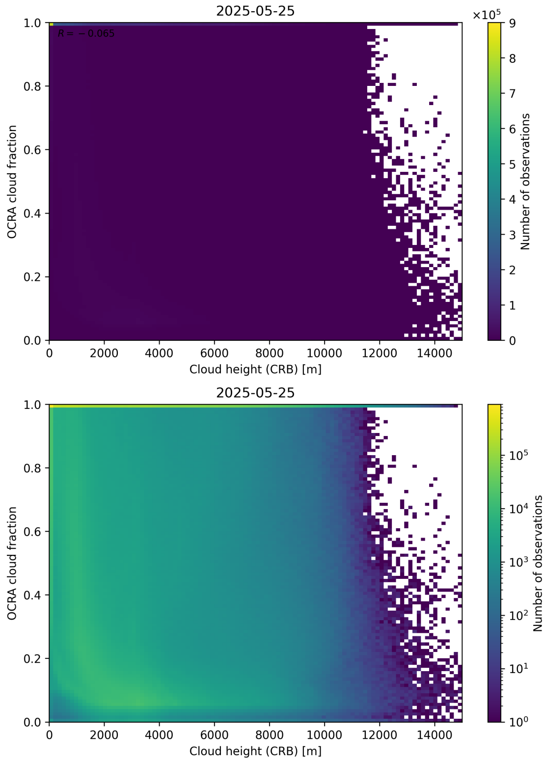
Figure 81: Scatter density plot of “Cloud height (CRB)” against “OCRA cloud fraction” for 2025-05-24 to 2025-05-26.
