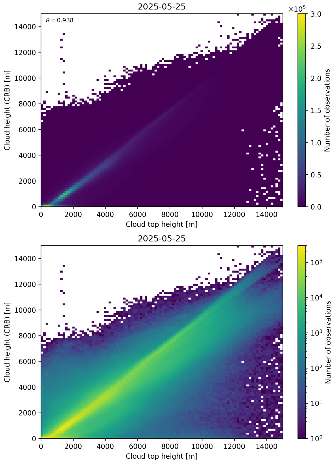
Figure 89: Scatter density plot of “Cloud top height” against “Cloud height (CRB)” for 2025-05-24 to 2025-05-26.
