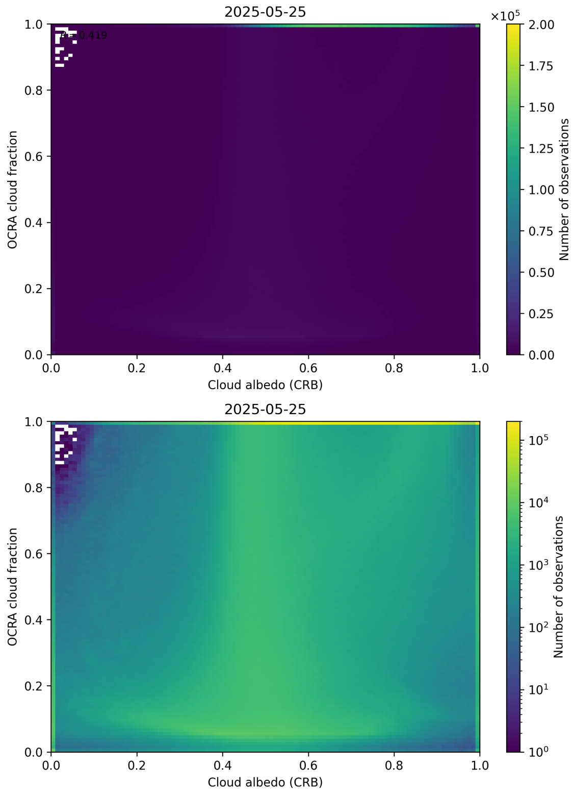
Figure 70: Scatter density plot of “Cloud albedo (CRB)” against “OCRA cloud fraction” for 2025-05-24 to 2025-05-26.
