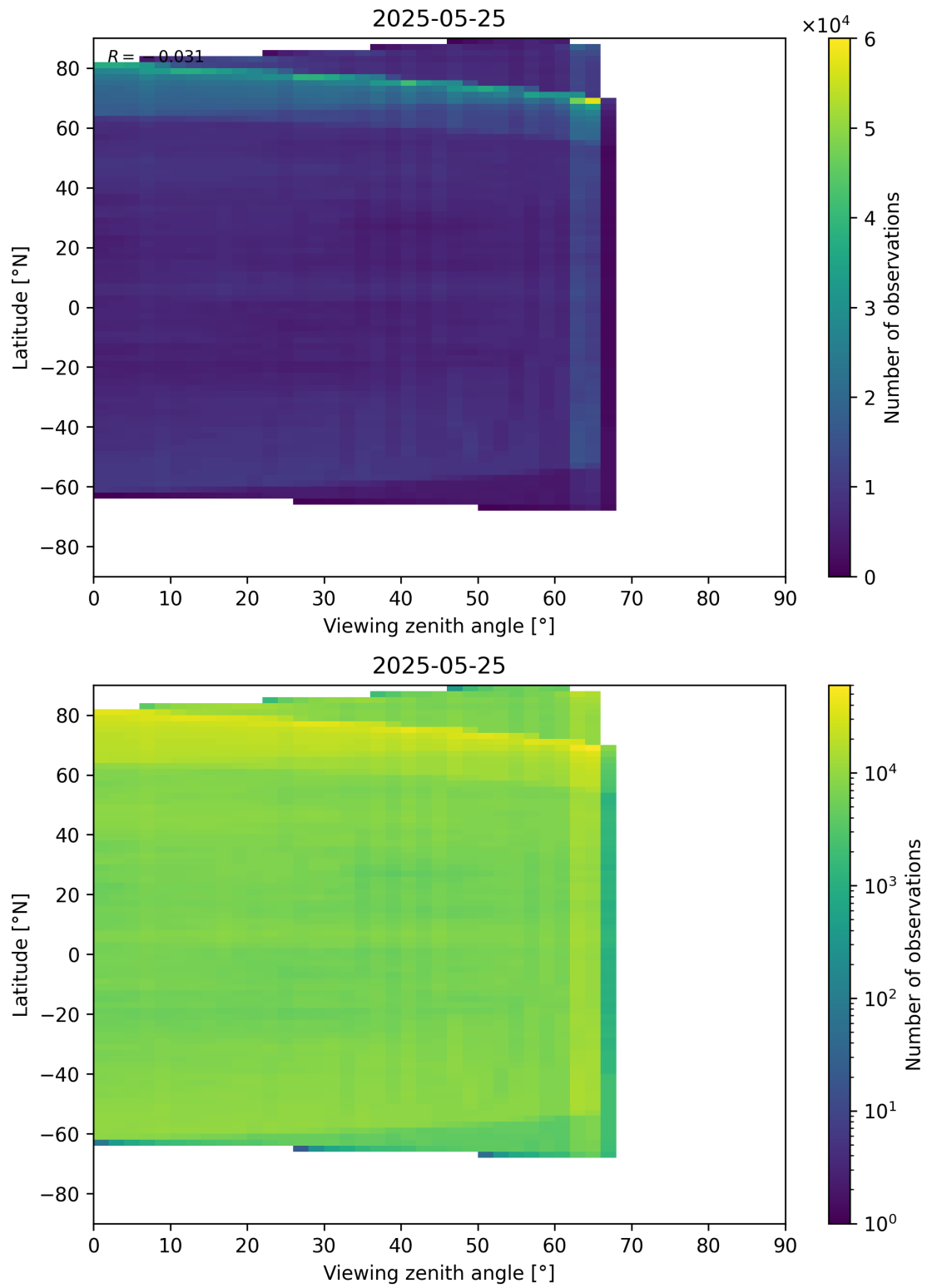
Figure 113: Scatter density plot of “Viewing zenith angle” against “Latitude” for 2025-05-24 to 2025-05-26.
