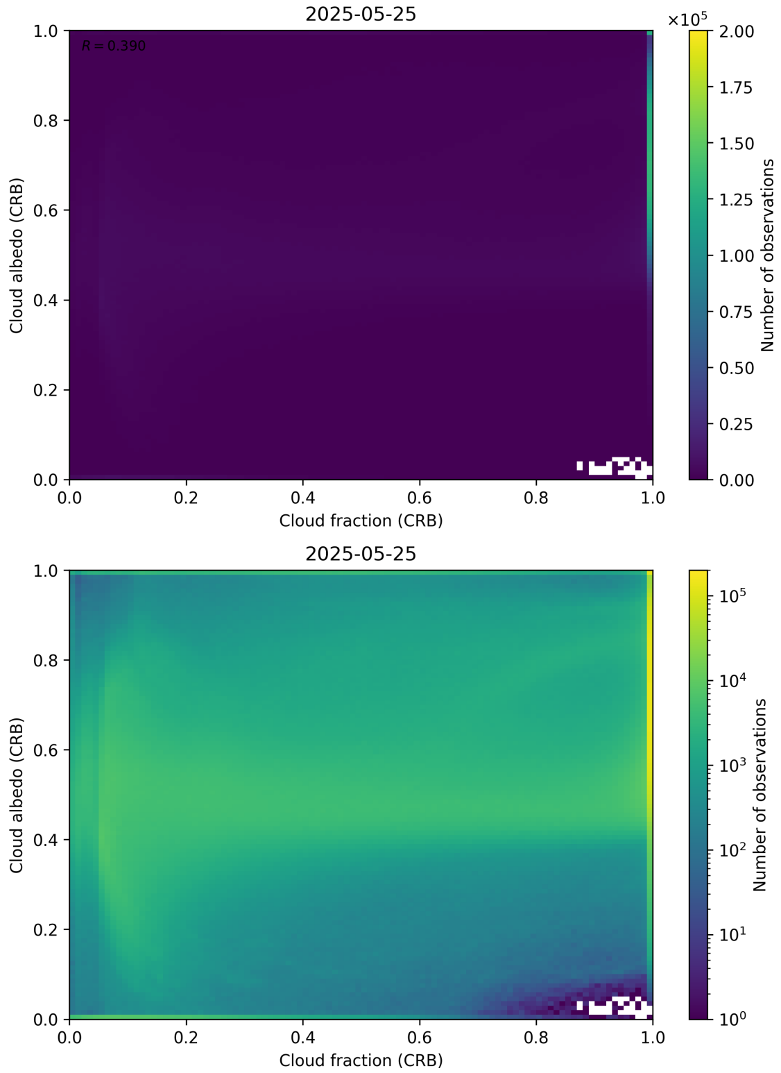
Figure 77: Scatter density plot of “Cloud fraction (CRB)” against “Cloud albedo (CRB)” for 2025-05-24 to 2025-05-26.
