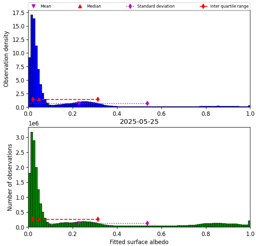
Figure 45: Histogram of “Fitted surface albedo” for 2025-05-24 to 2025-05-26
