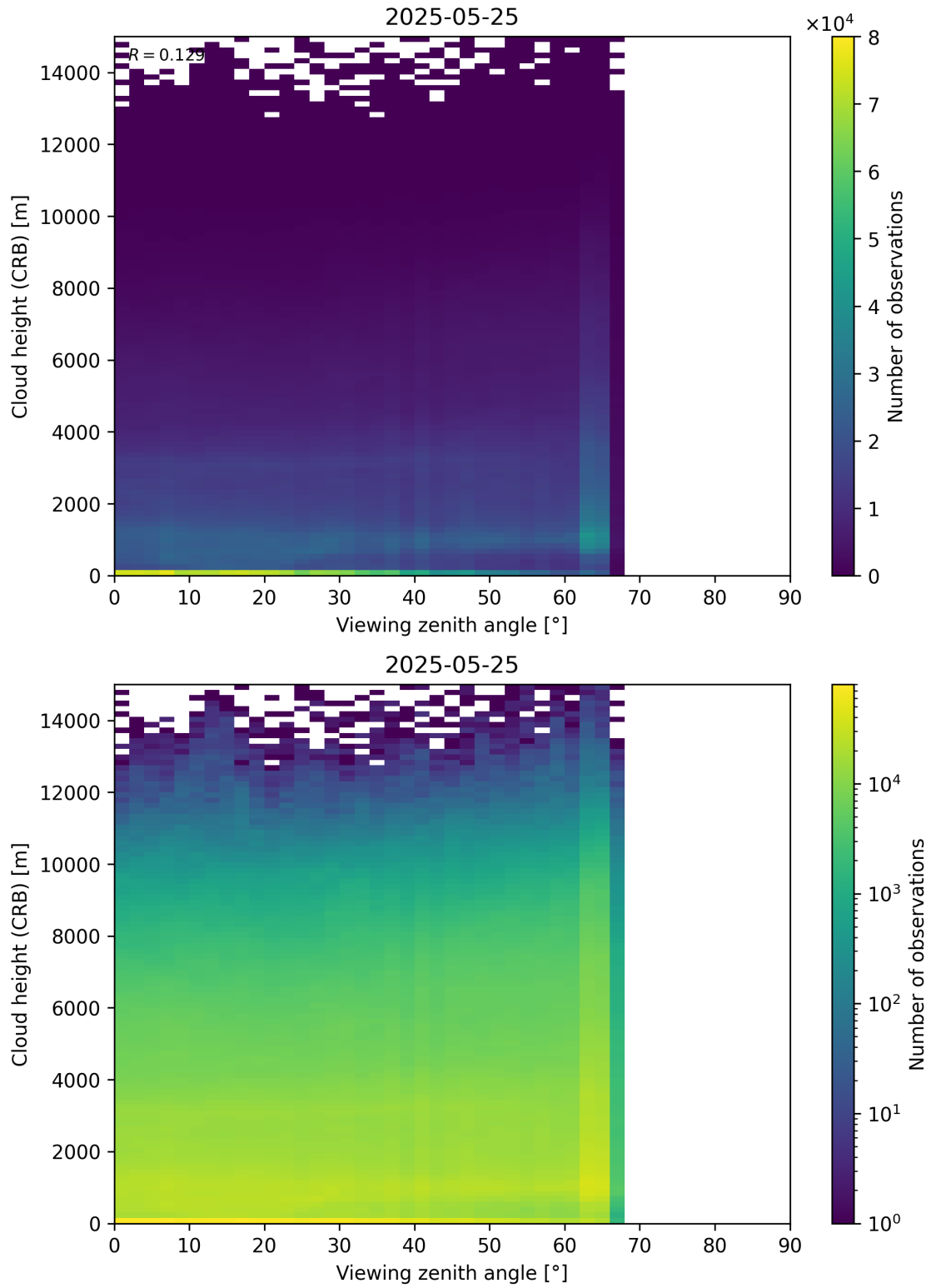
Figure 110: Scatter density plot of “Viewing zenith angle” against “Cloud height (CRB)” for 2025-05-24 to 2025-05-26.
