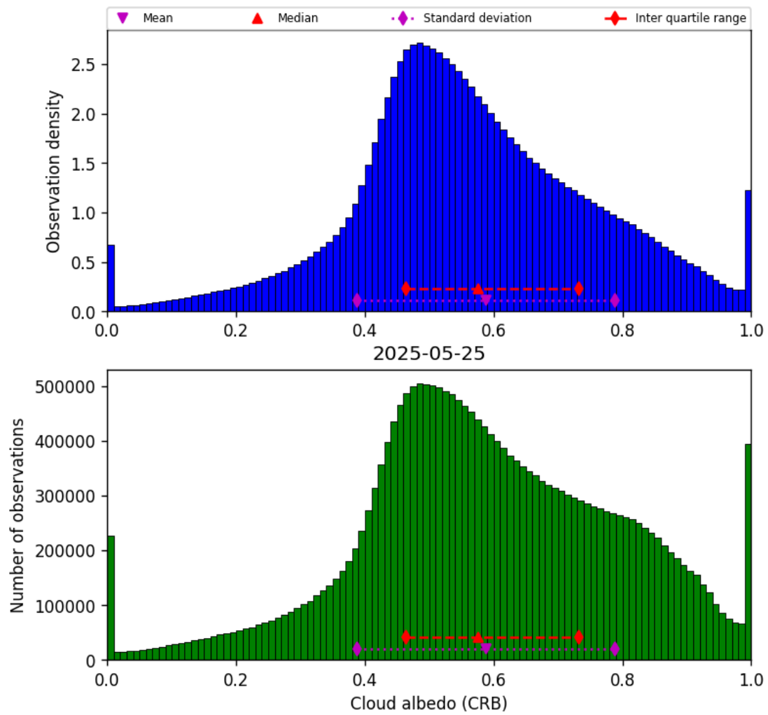
Figure 44: Histogram of “Cloud albedo (CRB)” for 2025-05-24 to 2025-05-26
