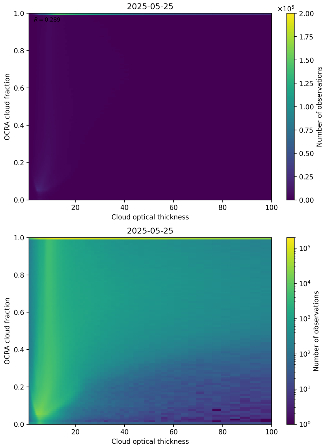
Figure 83: Scatter density plot of “Cloud optical thickness” against “OCRA cloud fraction” for 2025-05-24 to 2025-05-26.
