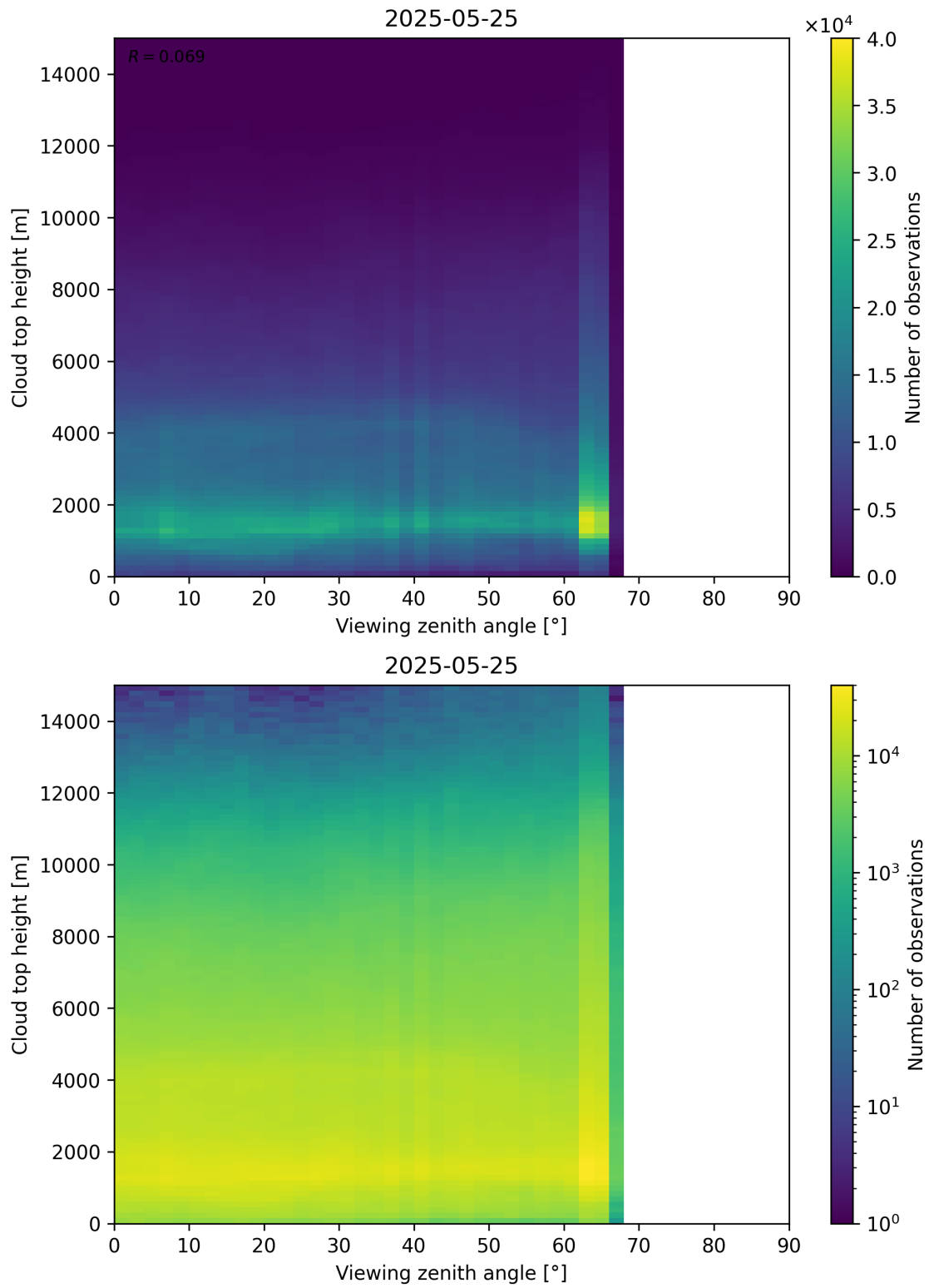
Figure 112: Scatter density plot of “Viewing zenith angle” against “Cloud top height” for 2025-05-24 to 2025-05-26.
