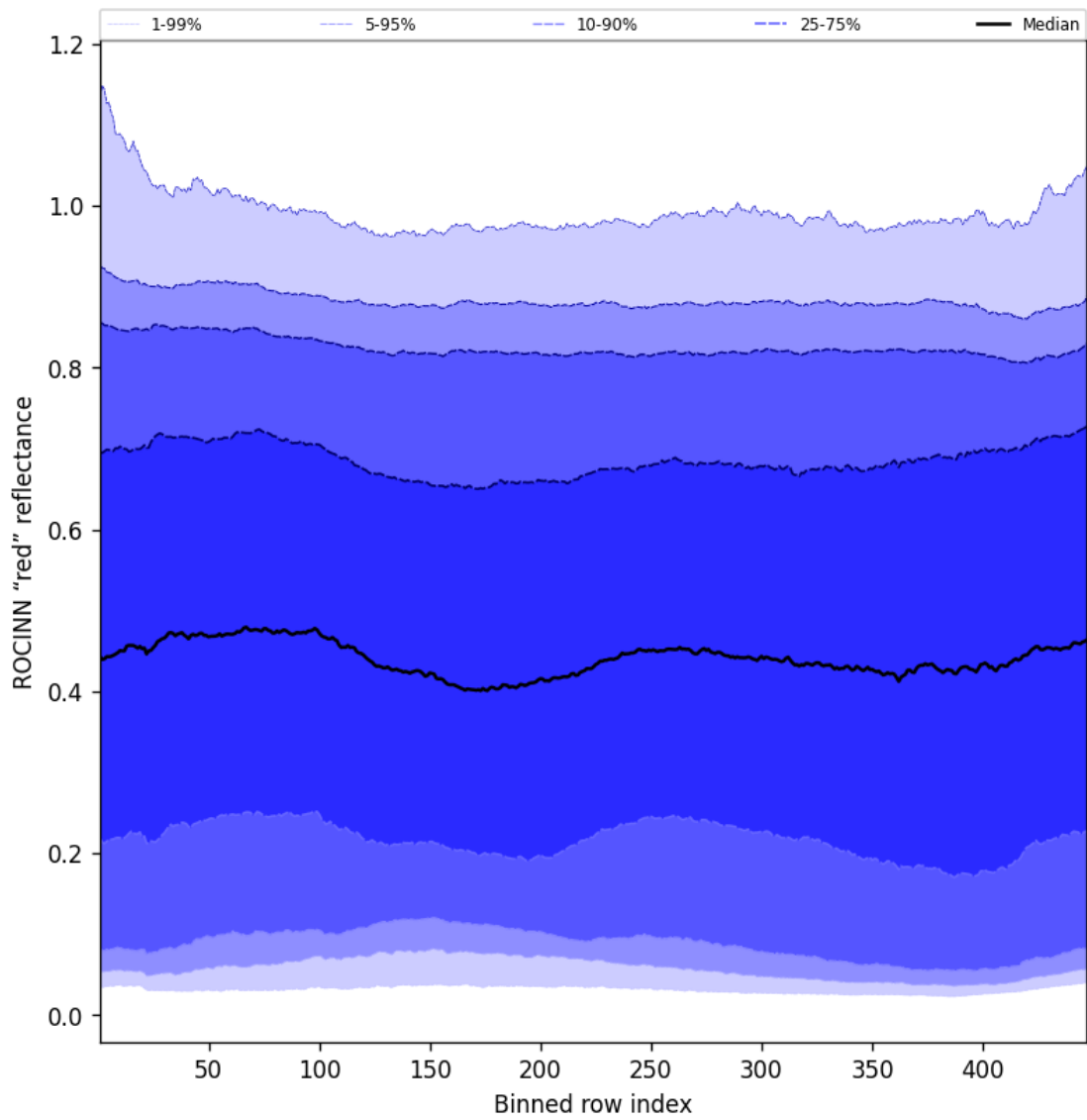
Figure 69: Along track statistics of “ROCINN “red” reflectance” for 2025-05-24 to 2025-05-26
