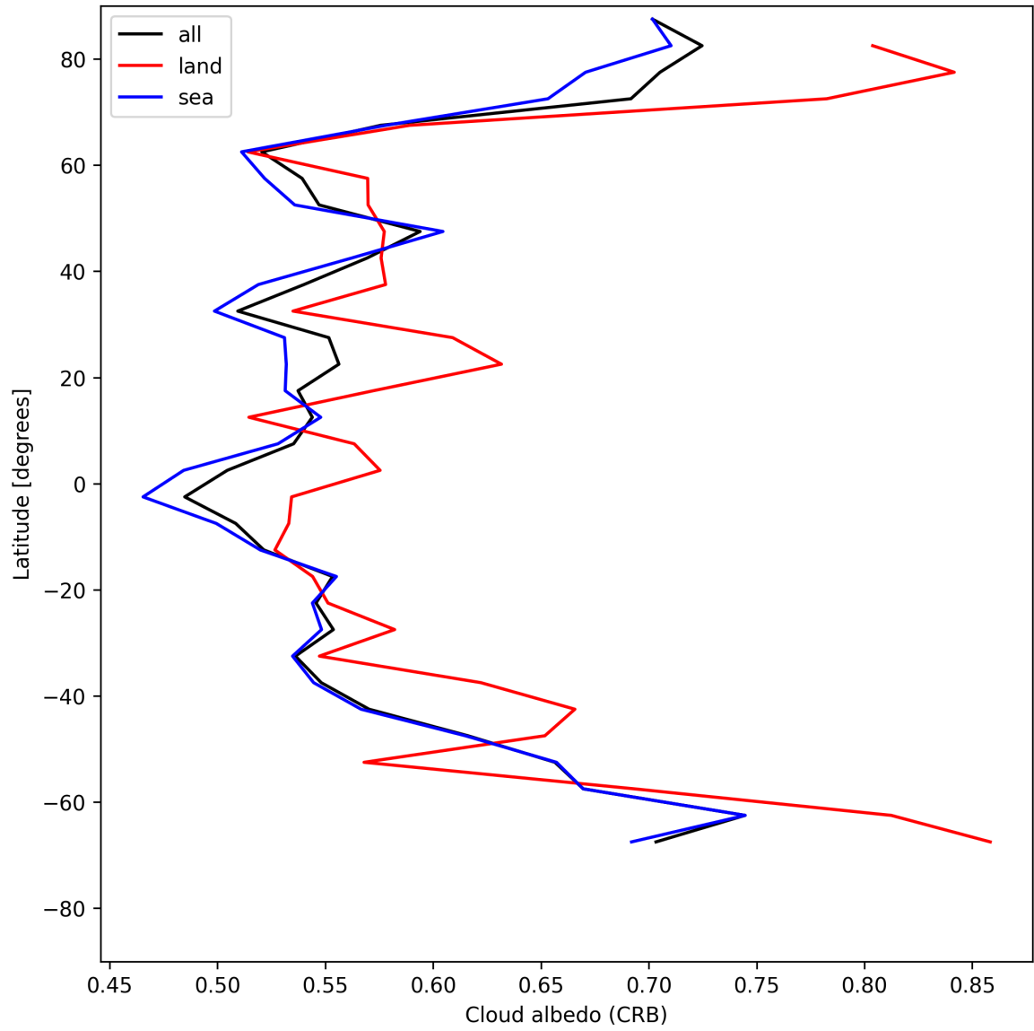
Figure 28: Zonal average of “Cloud albedo (CRB)” for 2025-05-24 to 2025-05-26.
