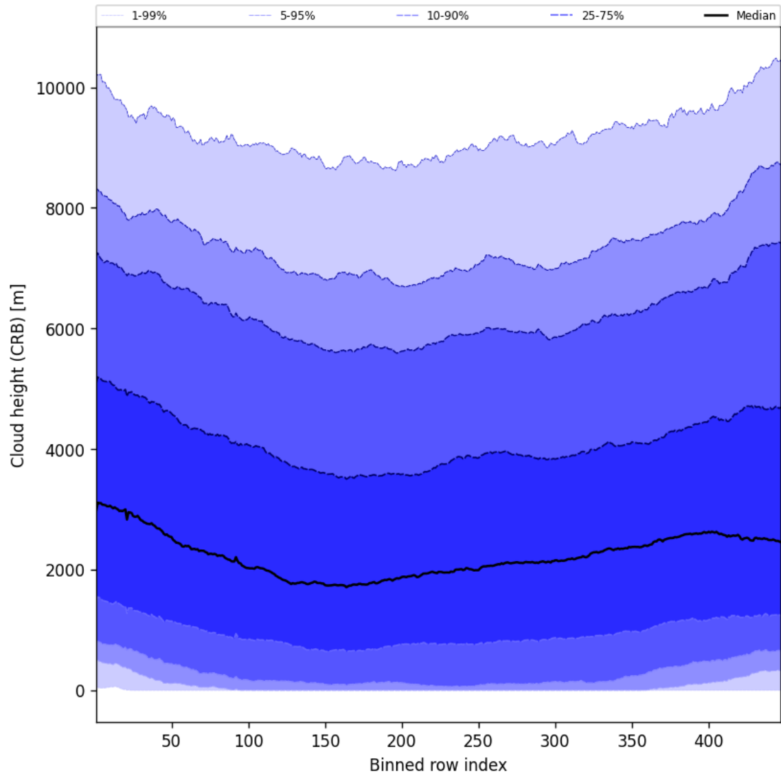
Figure 59: Along track statistics of “Cloud height (CRB)” for 2025-05-24 to 2025-05-26
