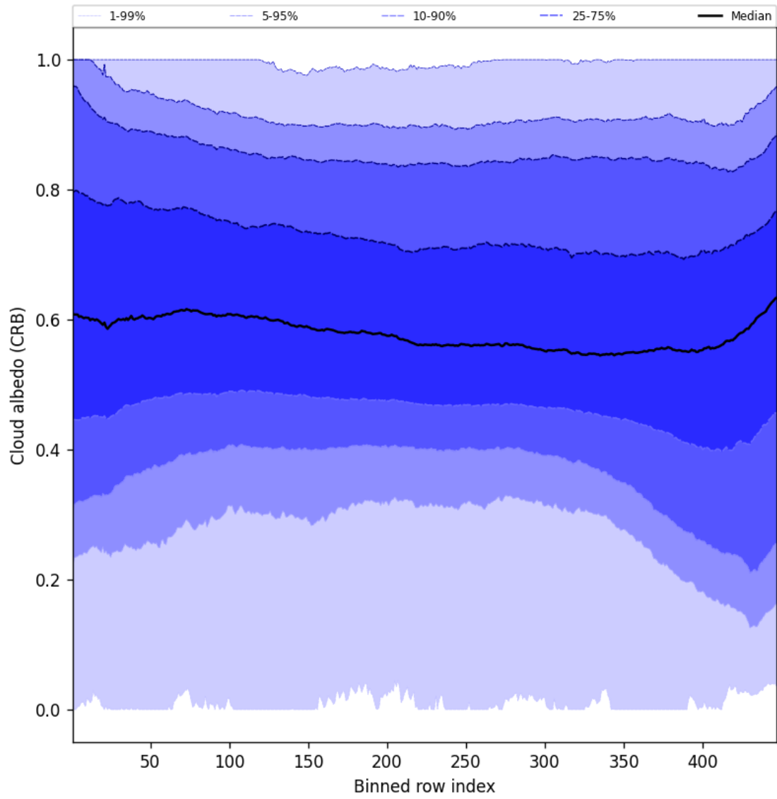
Figure 60: Along track statistics of “Cloud albedo (CRB)” for 2025-05-24 to 2025-05-26
