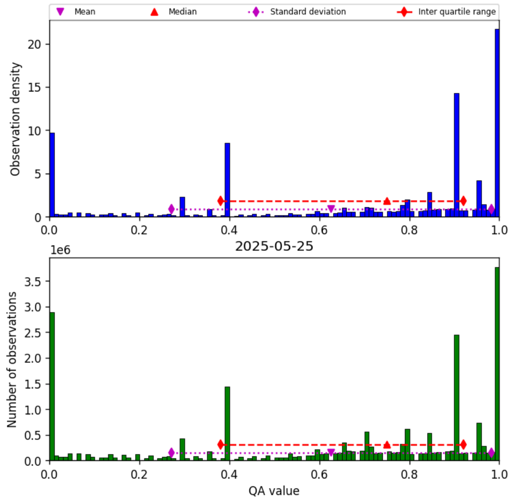
Figure 38: Histogram of “QA value” for 2025-05-24 to 2025-05-26
