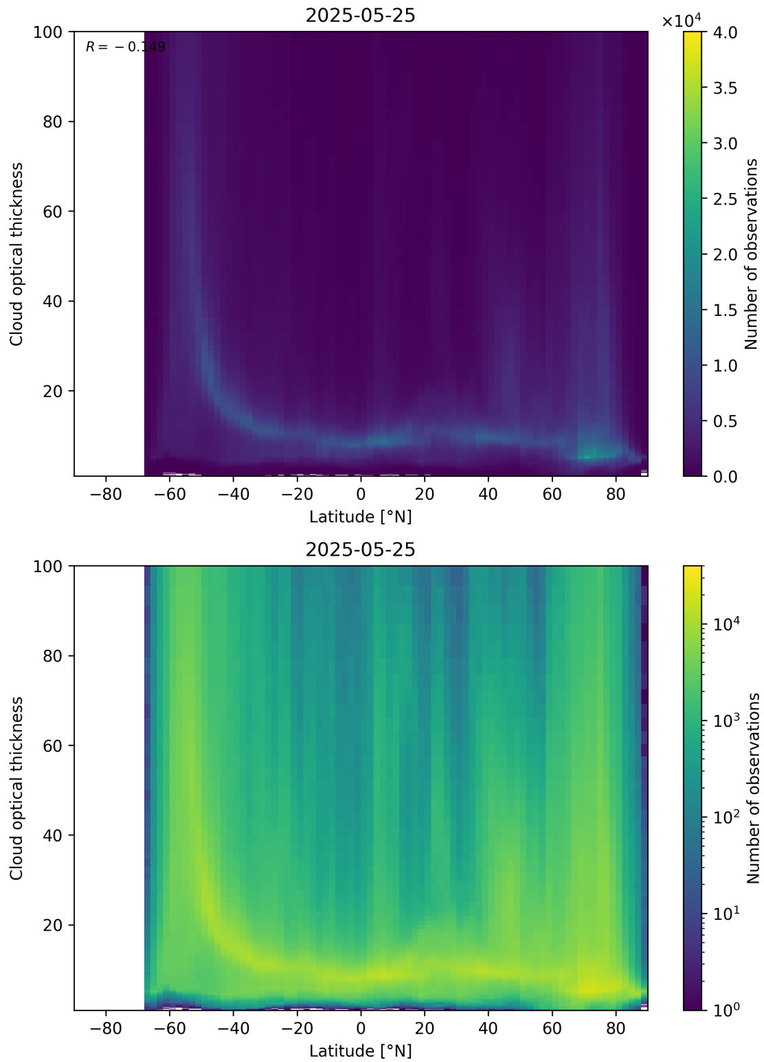
Figure 96: Scatter density plot of “Latitude” against “Cloud optical thickness” for 2025-05-24 to 2025-05-26.
