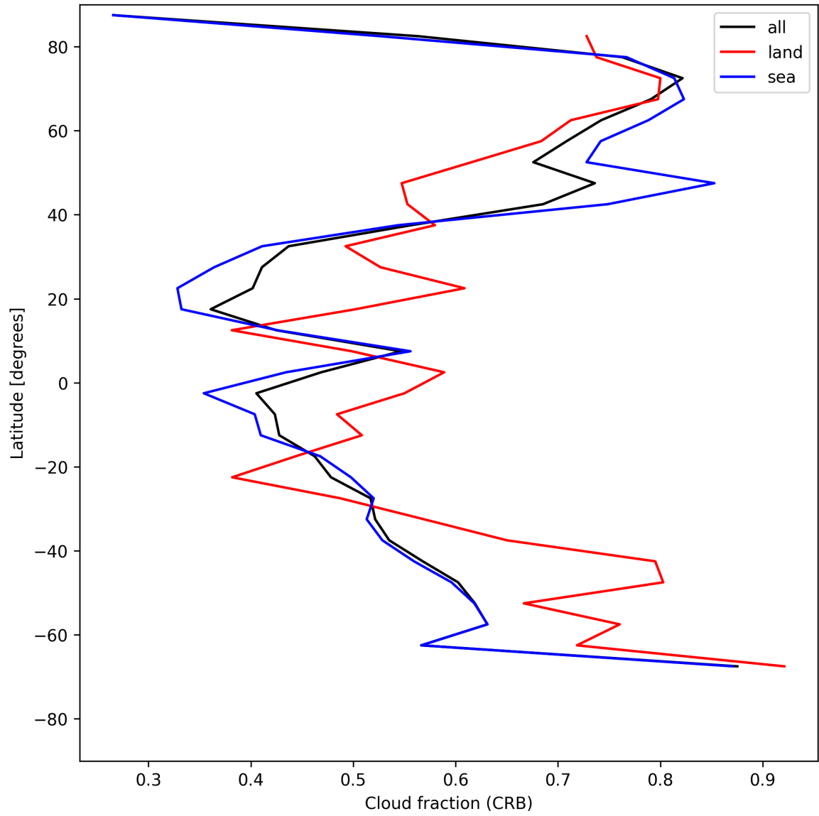
Figure 26: Zonal average of “Cloud fraction (CRB)” for 2025-05-24 to 2025-05-26.
