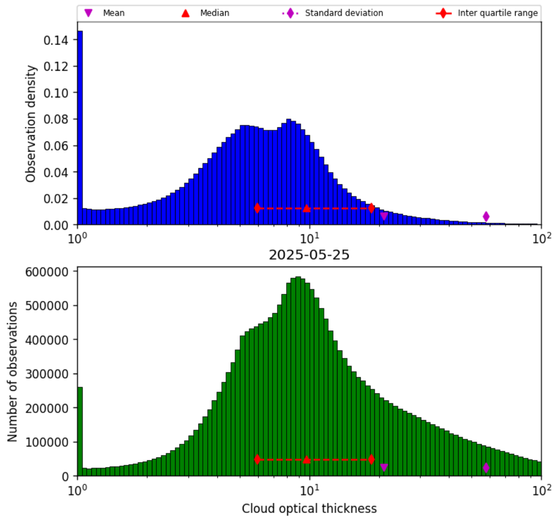
Figure 41: Histogram of “Cloud optical thickness” for 2025-05-24 to 2025-05-26
