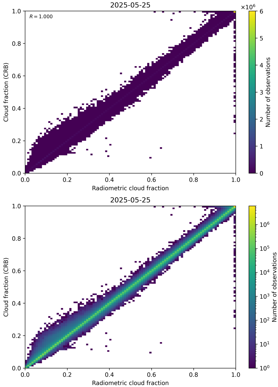
Figure 73: Scatter density plot of “Radiometric cloud fraction” against “Cloud fraction (CRB)” for 2025-05-24 to 2025-05-26.
