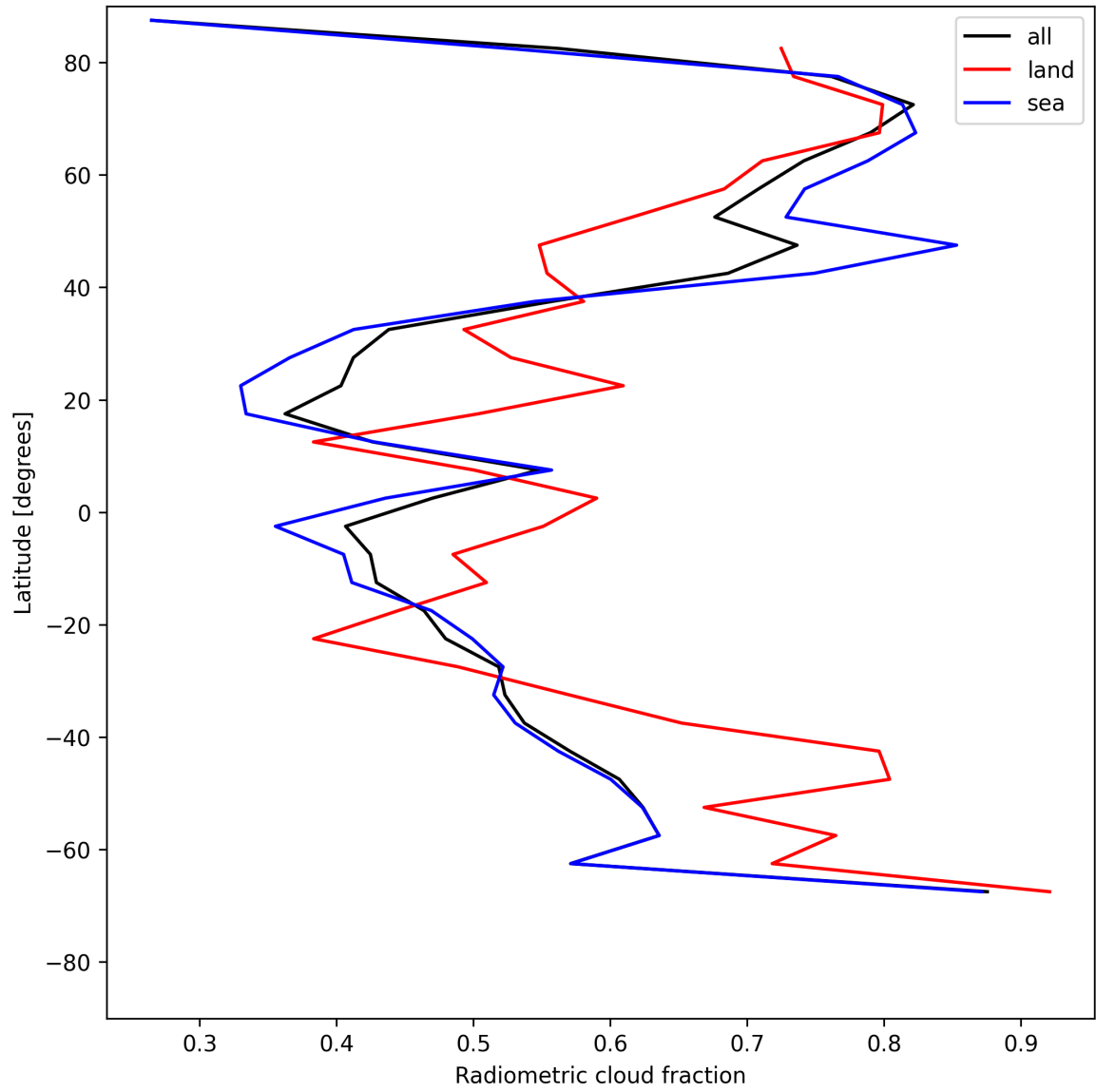
Figure 23: Zonal average of “Radiometric cloud fraction” for 2025-05-24 to 2025-05-26.
