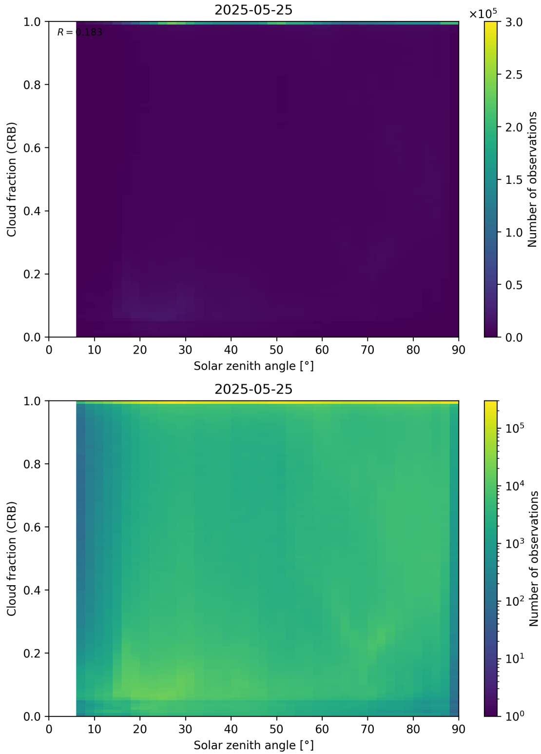
Figure 101: Scatter density plot of “Solar zenith angle” against “Cloud fraction (CRB)” for 2025-05-24 to 2025-05-26.
