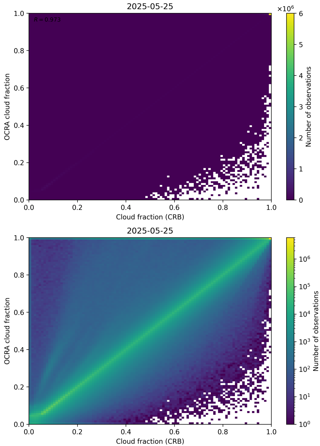
Figure 78: Scatter density plot of “Cloud fraction (CRB)” against “OCRA cloud fraction” for 2025-05-24 to 2025-05-26.
