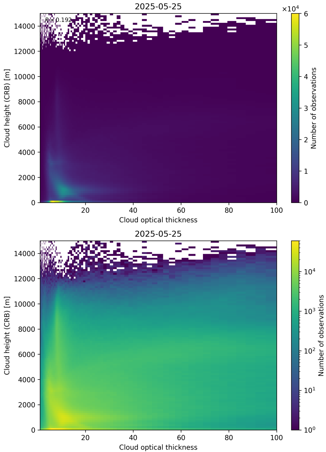
Figure 85: Scatter density plot of “Cloud optical thickness” against “Cloud height (CRB)” for 2025-05-24 to 2025-05-26.
