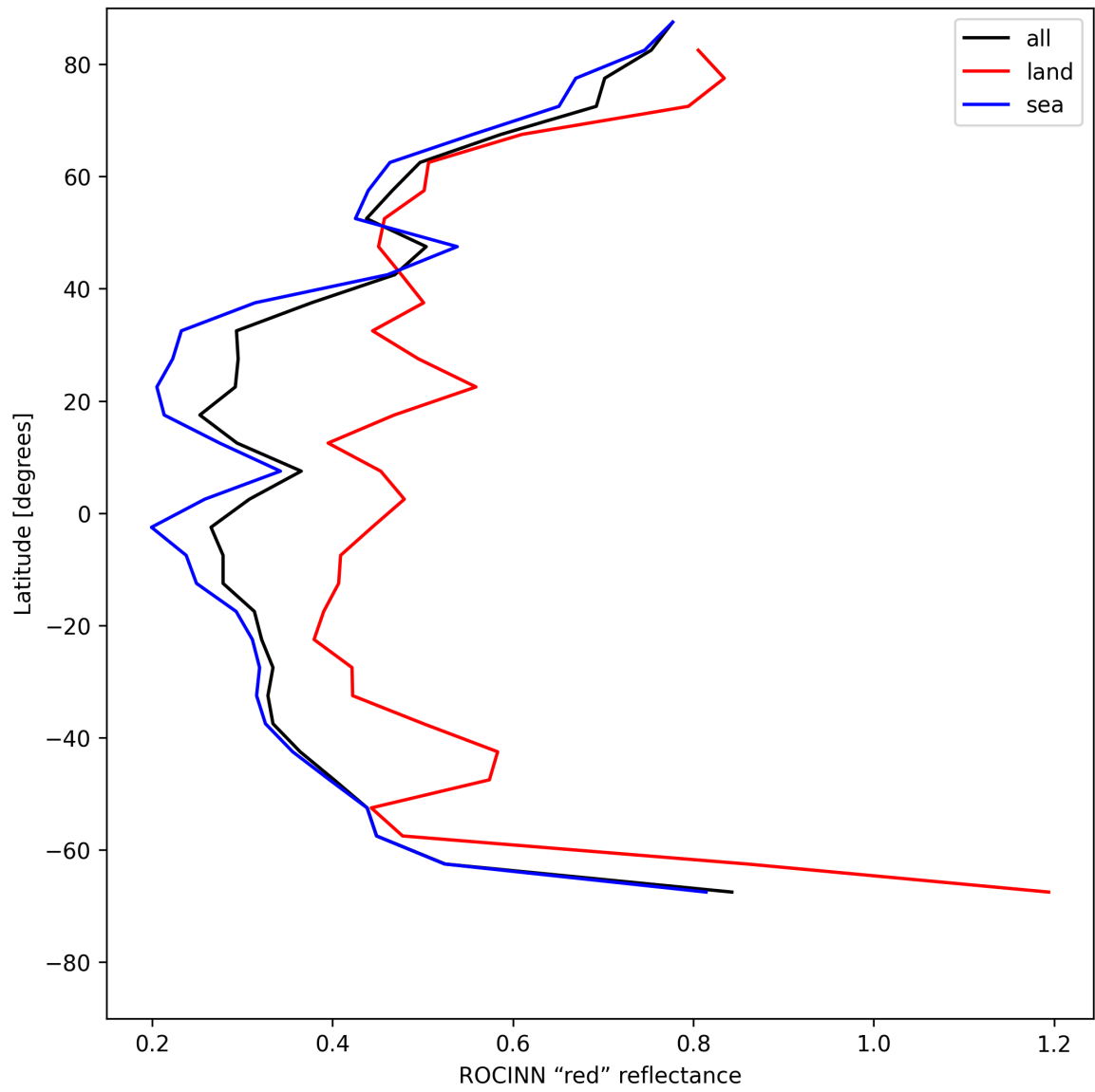
Figure 37: Zonal average of “ROCINN “red” reflectance” for 2025-05-24 to 2025-05-26.
