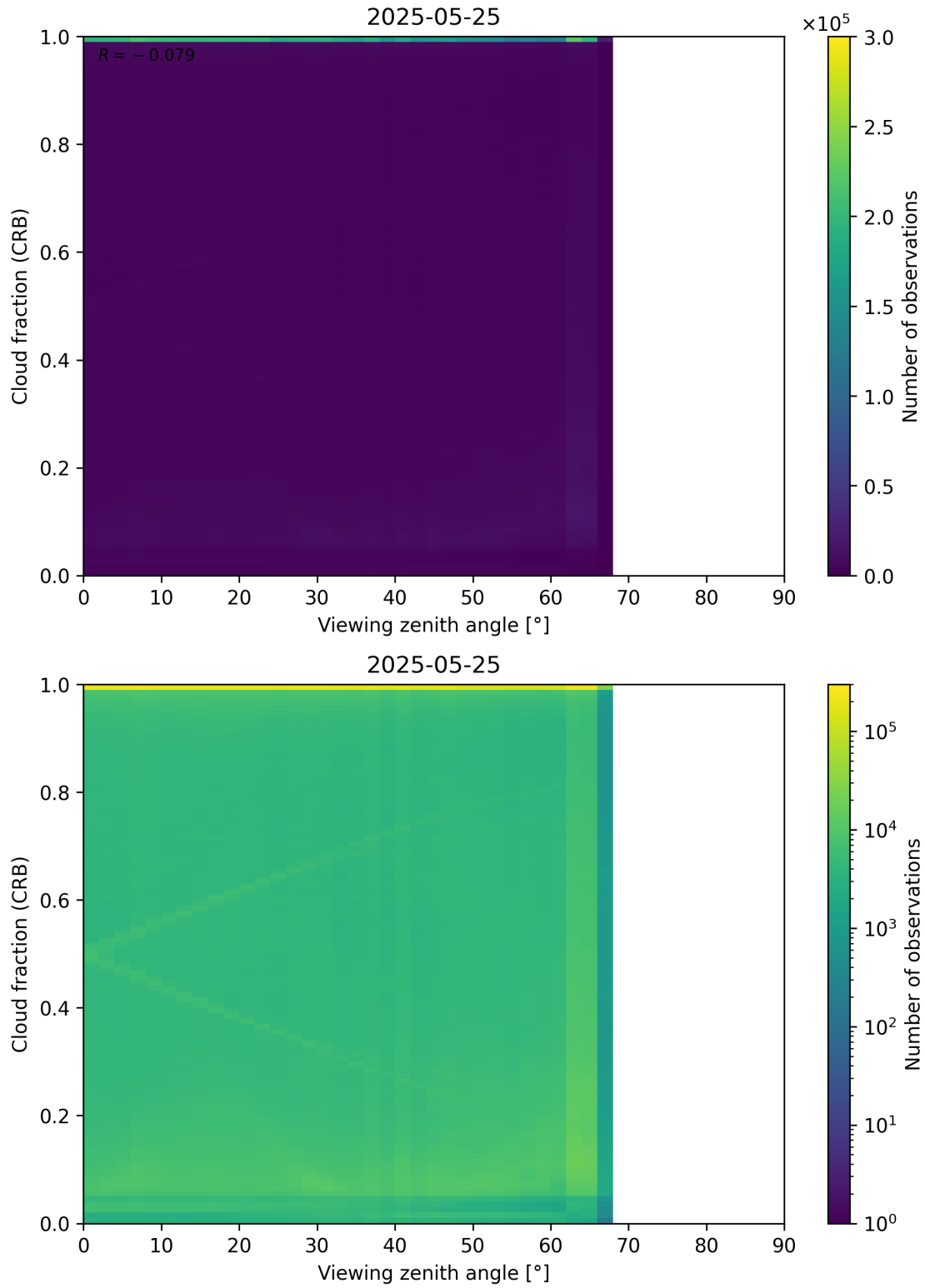
Figure 109: Scatter density plot of “Viewing zenith angle” against “Cloud fraction (CRB)” for 2025-05-24 to 2025-05-26.
