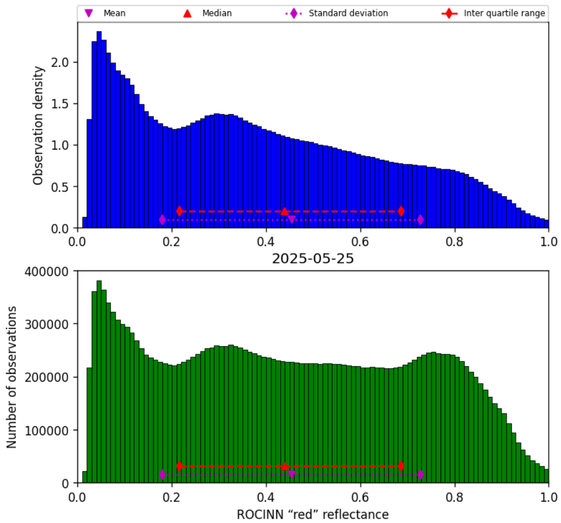
Figure 53: Histogram of “ROCINN “red” reflectance” for 2025-05-24 to 2025-05-26
