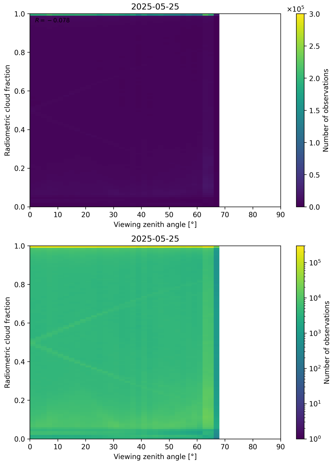
Figure 107: Scatter density plot of “Viewing zenith angle” against “Radiometric cloud fraction” for 2025-05-24 to 2025-05-26.
