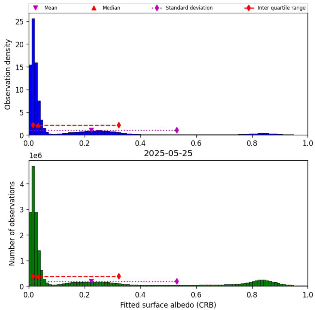
Figure 46: Histogram of “Fitted surface albedo (CRB)” for 2025-05-24 to 2025-05-26
