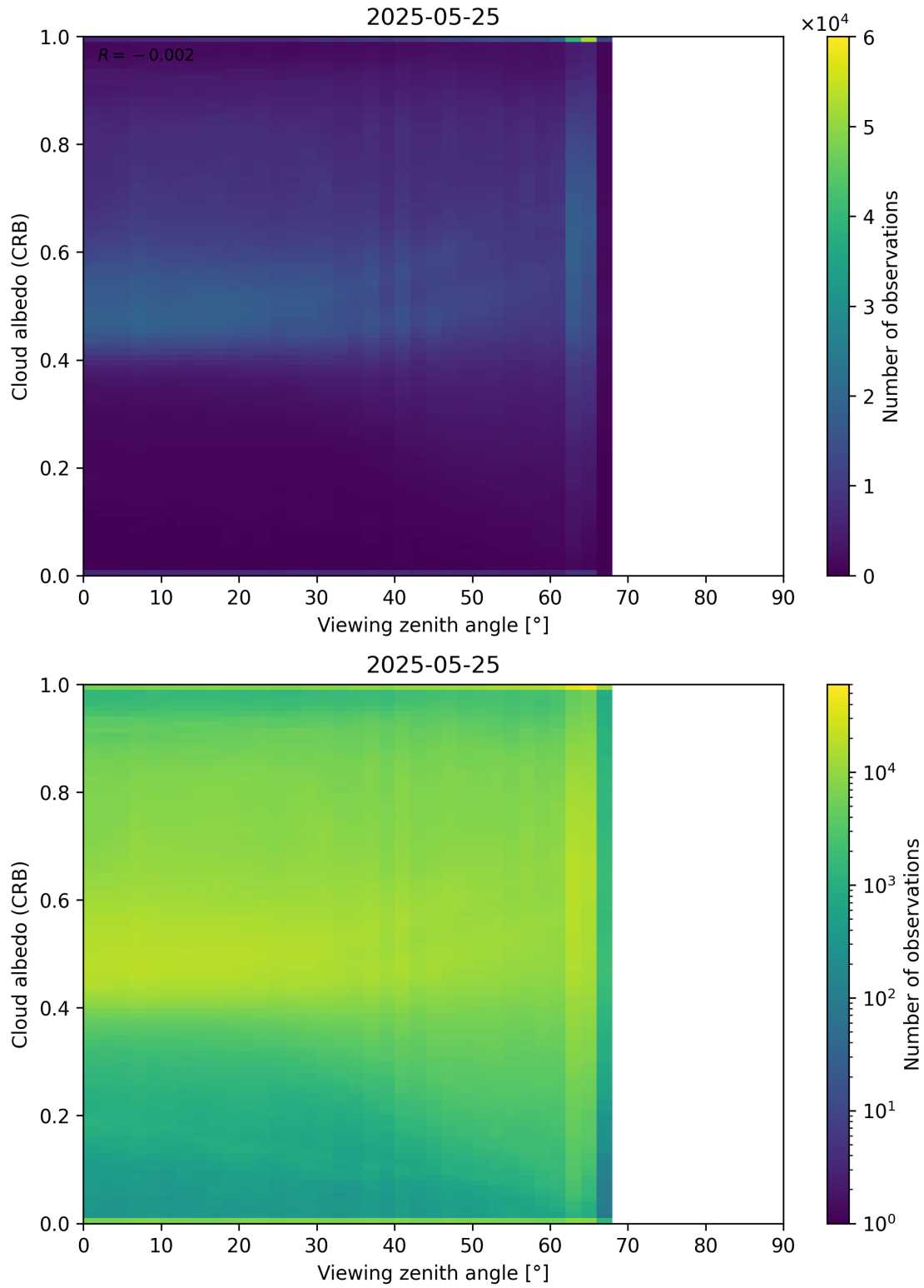
Figure 106: Scatter density plot of “Viewing zenith angle” against “Cloud albedo (CRB)” for 2025-05-24 to 2025-05-26.
