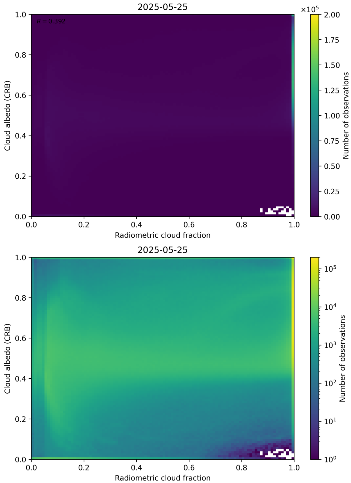
Figure 71: Scatter density plot of “Radiometric cloud fraction” against “Cloud albedo (CRB)” for 2025-05-24 to 2025-05-26.
