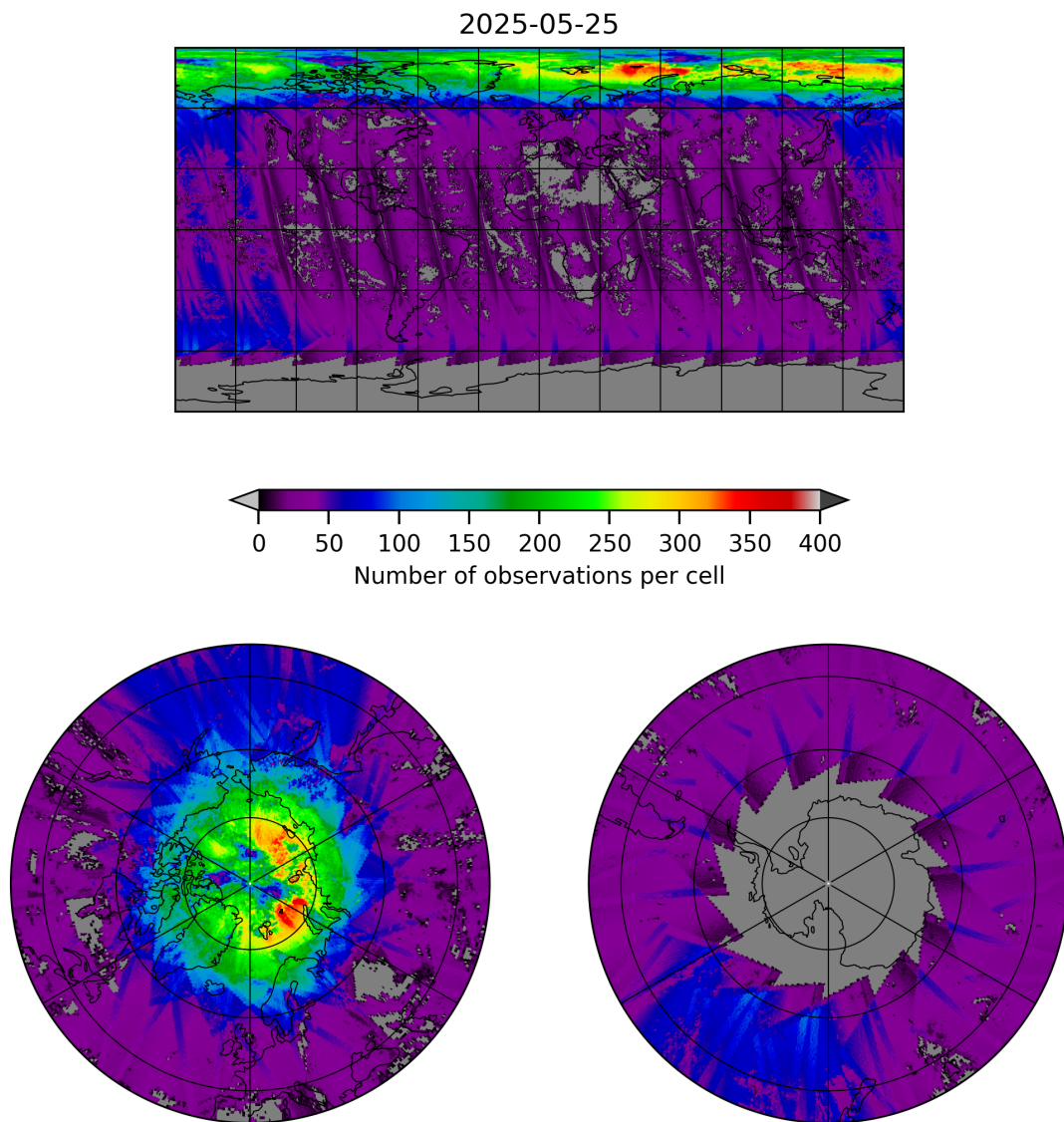
Figure 21: Map of the number of observations for 2025-05-24 to 2025-05-26
