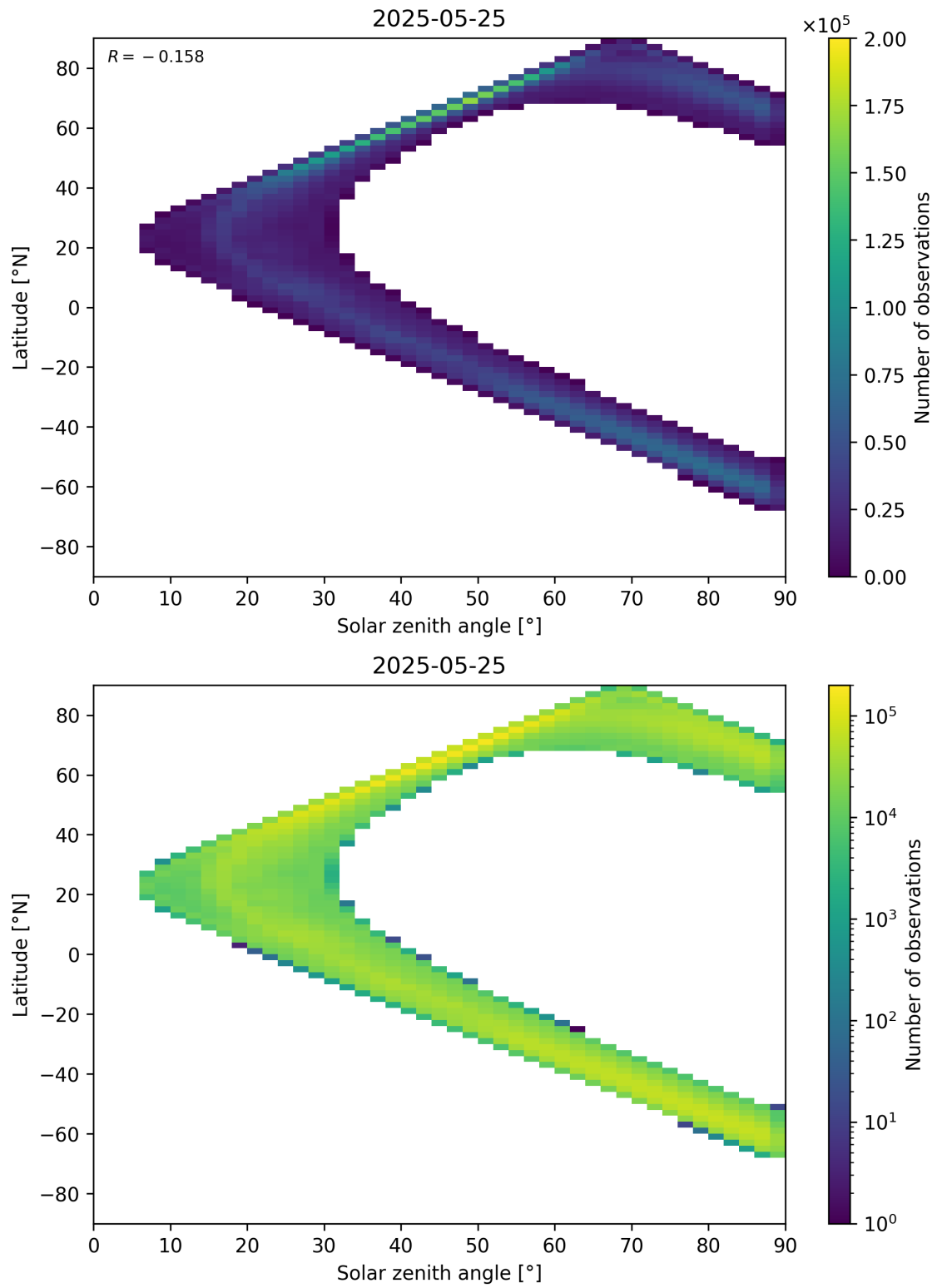
Figure 105: Scatter density plot of “Solar zenith angle” against “Latitude” for 2025-05-24 to 2025-05-26.
