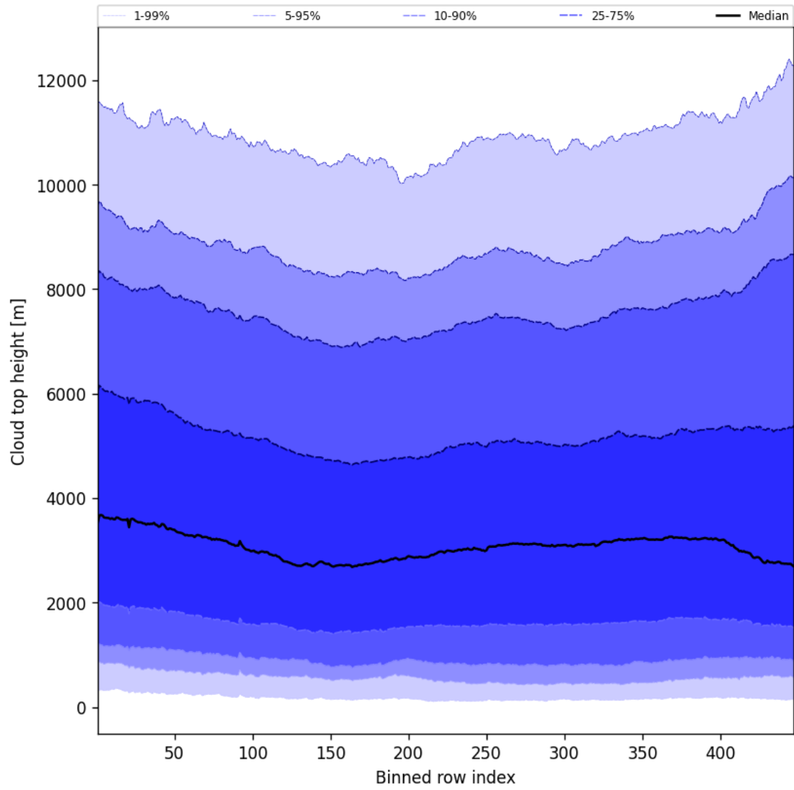
Figure 56: Along track statistics of “Cloud top height” for 2025-05-24 to 2025-05-26
