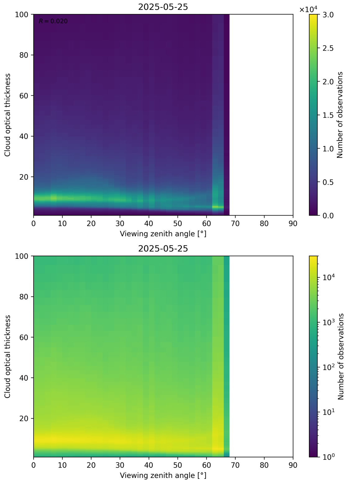
Figure 111: Scatter density plot of “Viewing zenith angle” against “Cloud optical thickness” for 2025-05-24 to 2025-05-26.
