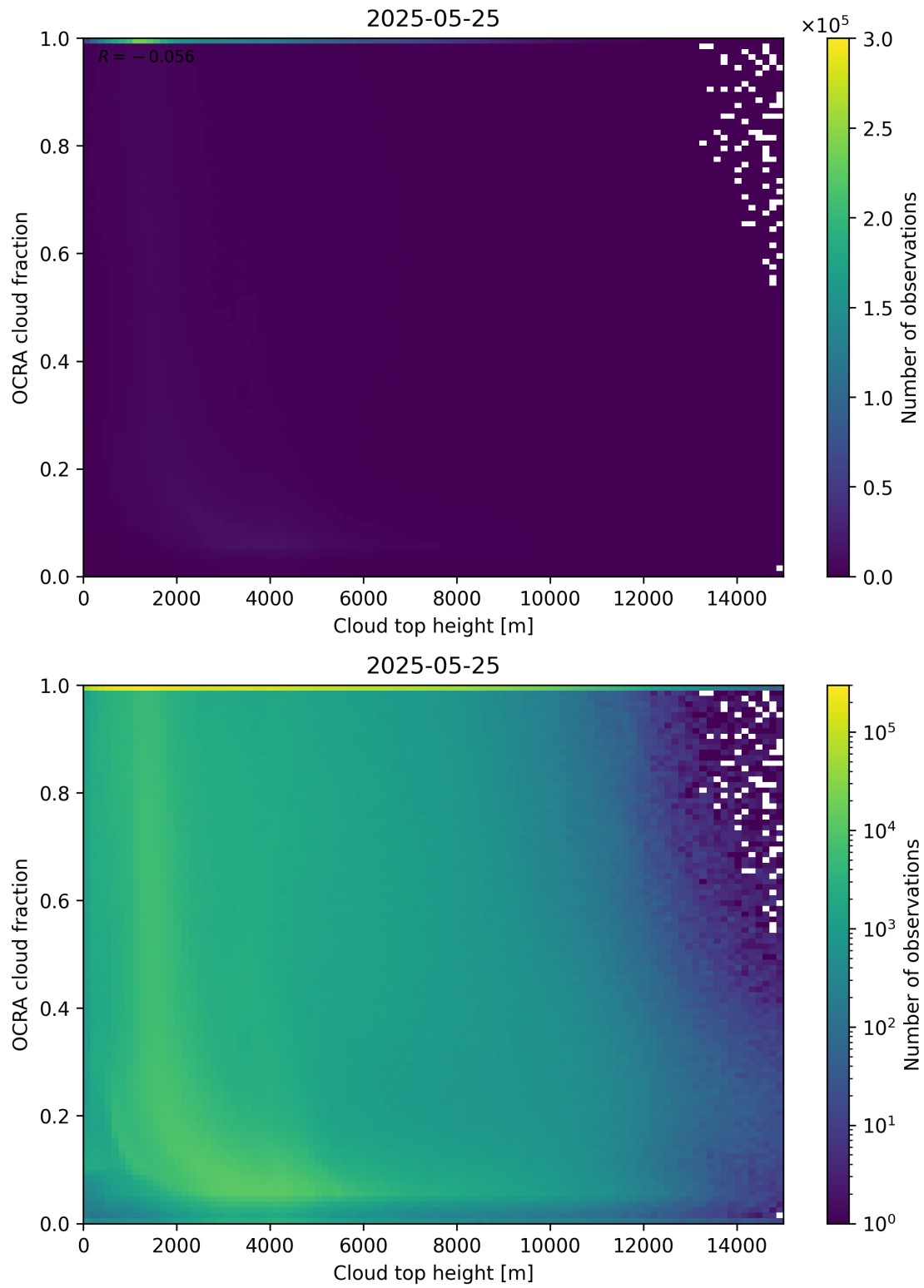
Figure 87: Scatter density plot of “Cloud top height” against “OCRA cloud fraction” for 2025-05-24 to 2025-05-26.
