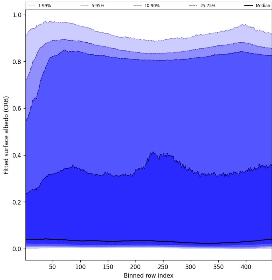
Figure 62: Along track statistics of “Fitted surface albedo (CRB)” for 2025-05-24 to 2025-05-26
