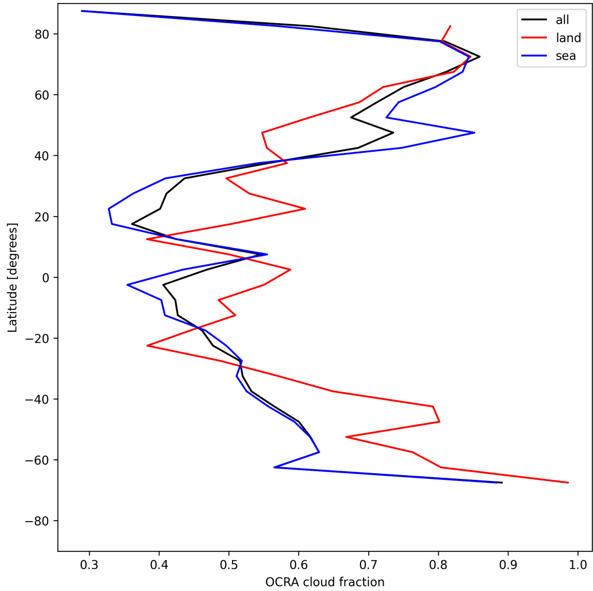
Figure 34: Zonal average of “OCRA cloud fraction” for 2025-05-24 to 2025-05-26.
