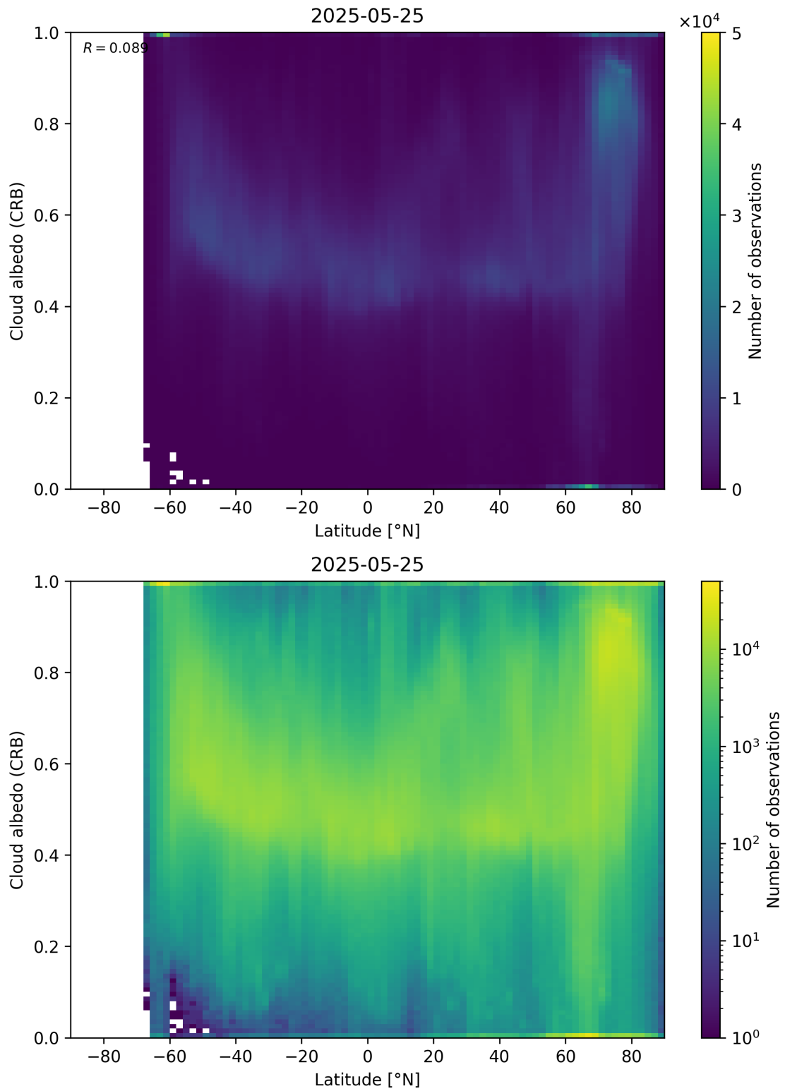
Figure 91: Scatter density plot of “Latitude” against “Cloud albedo (CRB)” for 2025-05-24 to 2025-05-26.
