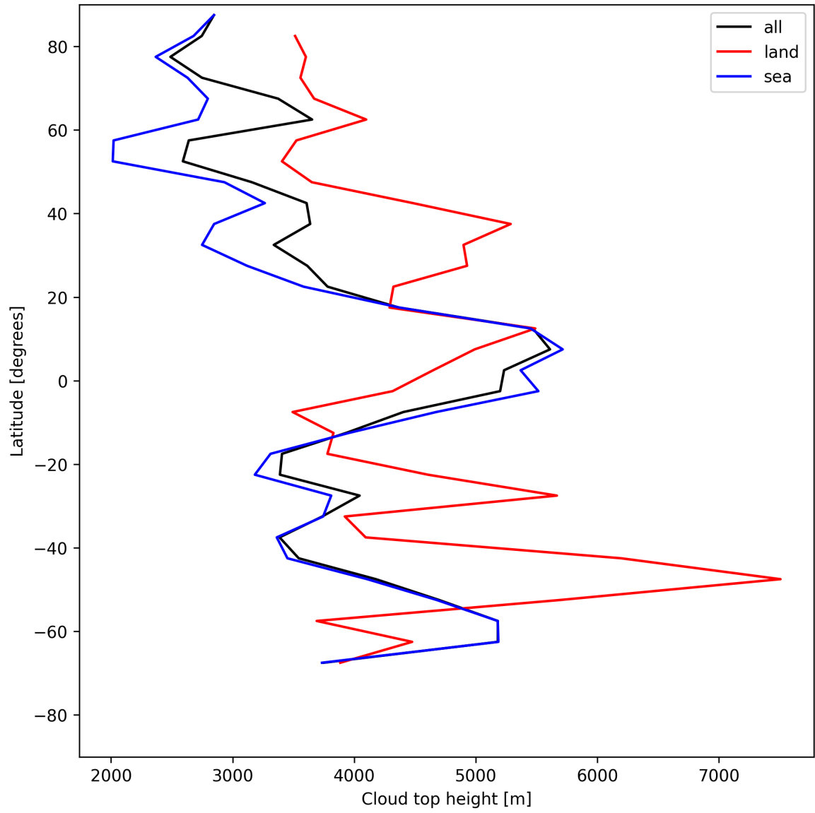
Figure 24: Zonal average of “Cloud top height” for 2025-05-24 to 2025-05-26.
