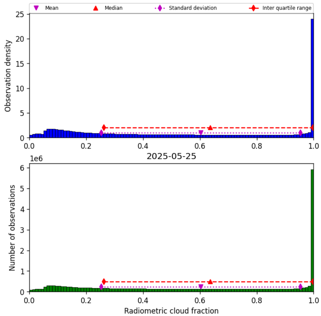
Figure 39: Histogram of “Radiometric cloud fraction” for 2025-05-24 to 2025-05-26
