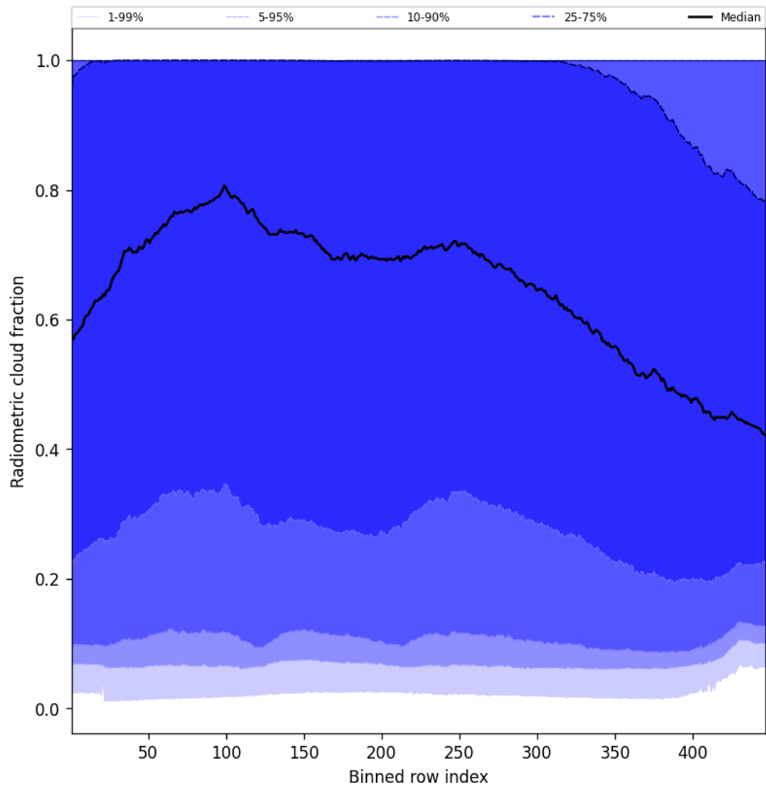
Figure 55: Along track statistics of “Radiometric cloud fraction” for 2025-05-24 to 2025-05-26
