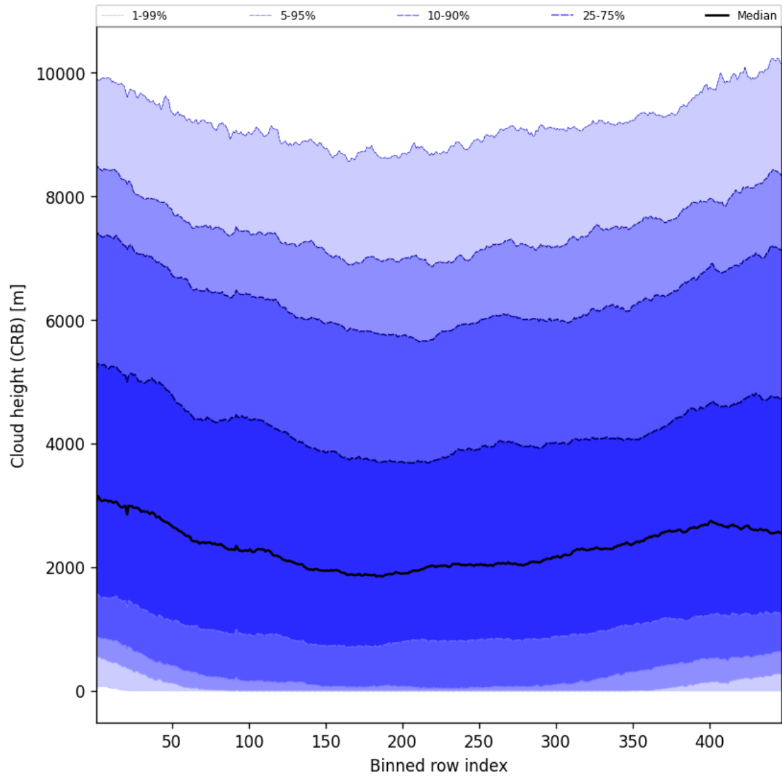
Figure 59: Along track statistics of “Cloud height (CRB)” for 2025-05-26 to 2025-05-27
