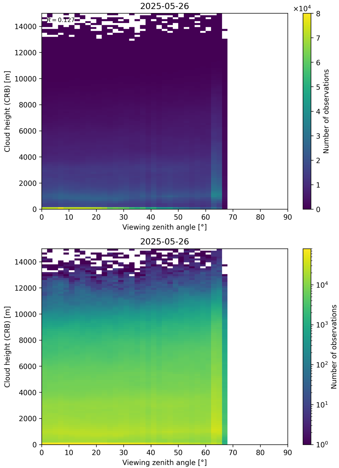
Figure 110: Scatter density plot of “Viewing zenith angle” against “Cloud height (CRB)” for 2025-05-26 to 2025-05-27.
