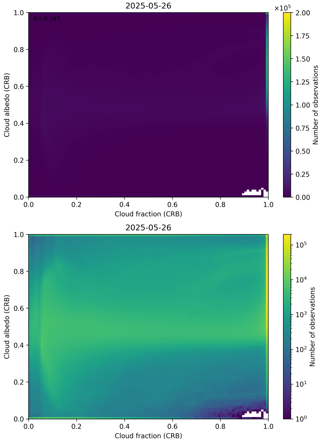
Figure 77: Scatter density plot of “Cloud fraction (CRB)” against “Cloud albedo (CRB)” for 2025-05-26 to 2025-05-27.
