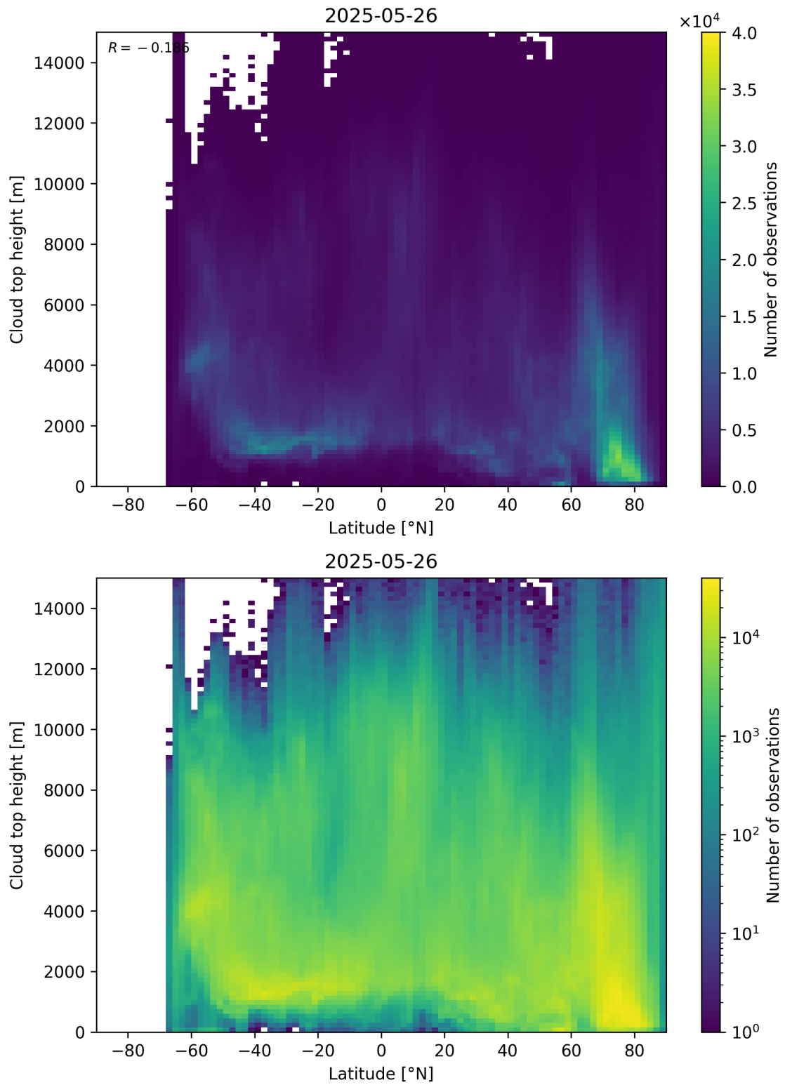
Figure 97: Scatter density plot of “Latitude” against “Cloud top height” for 2025-05-26 to 2025-05-27.
