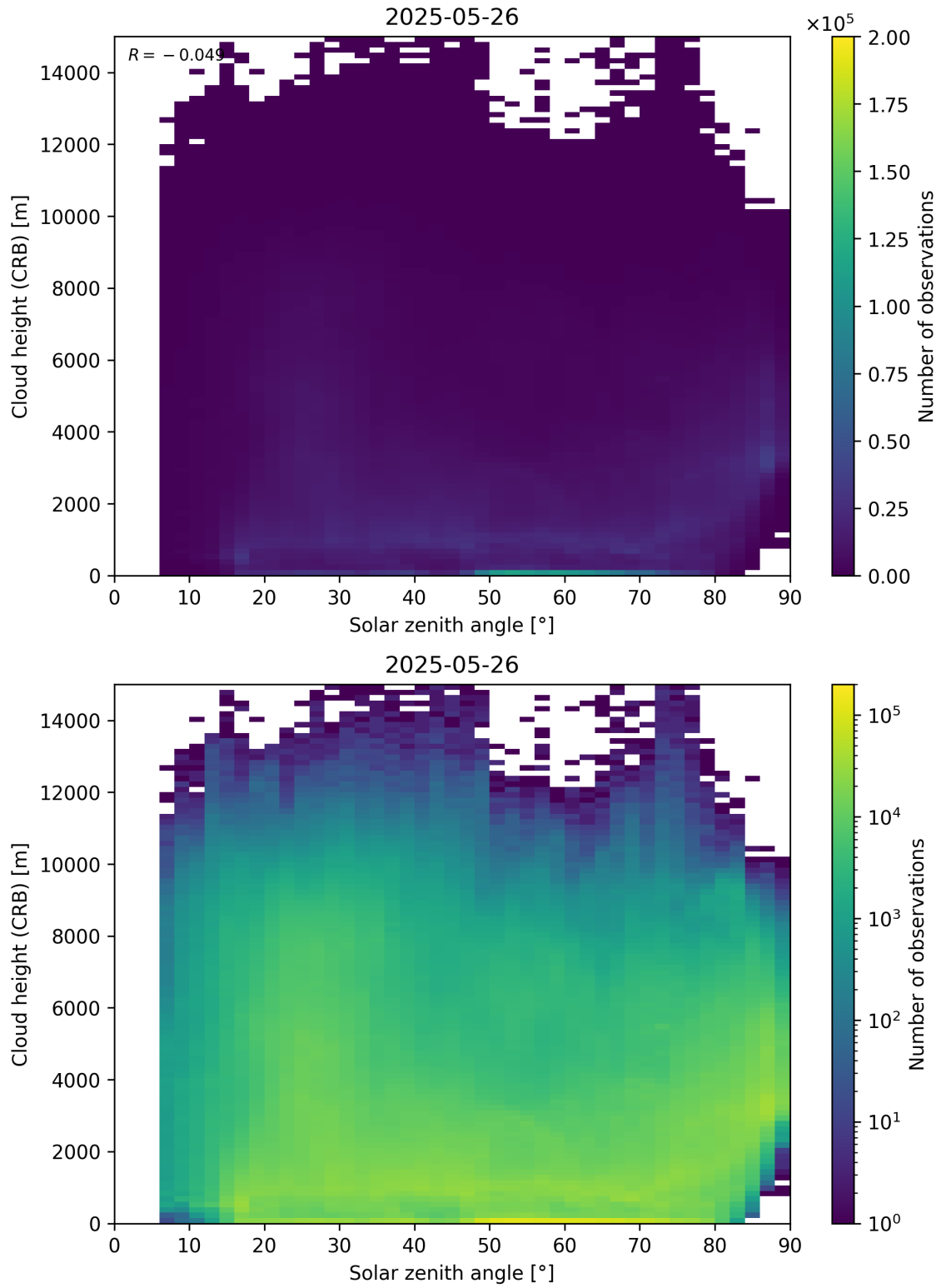
Figure 102: Scatter density plot of “Solar zenith angle” against “Cloud height (CRB)” for 2025-05-26 to 2025-05-27.
