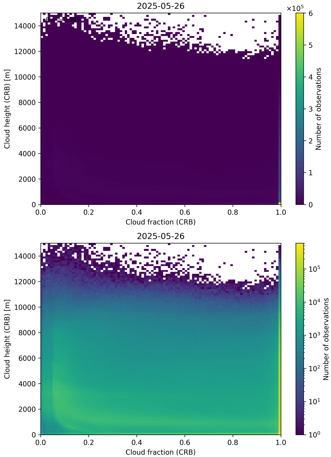
Figure 79: Scatter density plot of “Cloud fraction (CRB)” against “Cloud height (CRB)” for 2025-05-26 to 2025-05-27.
