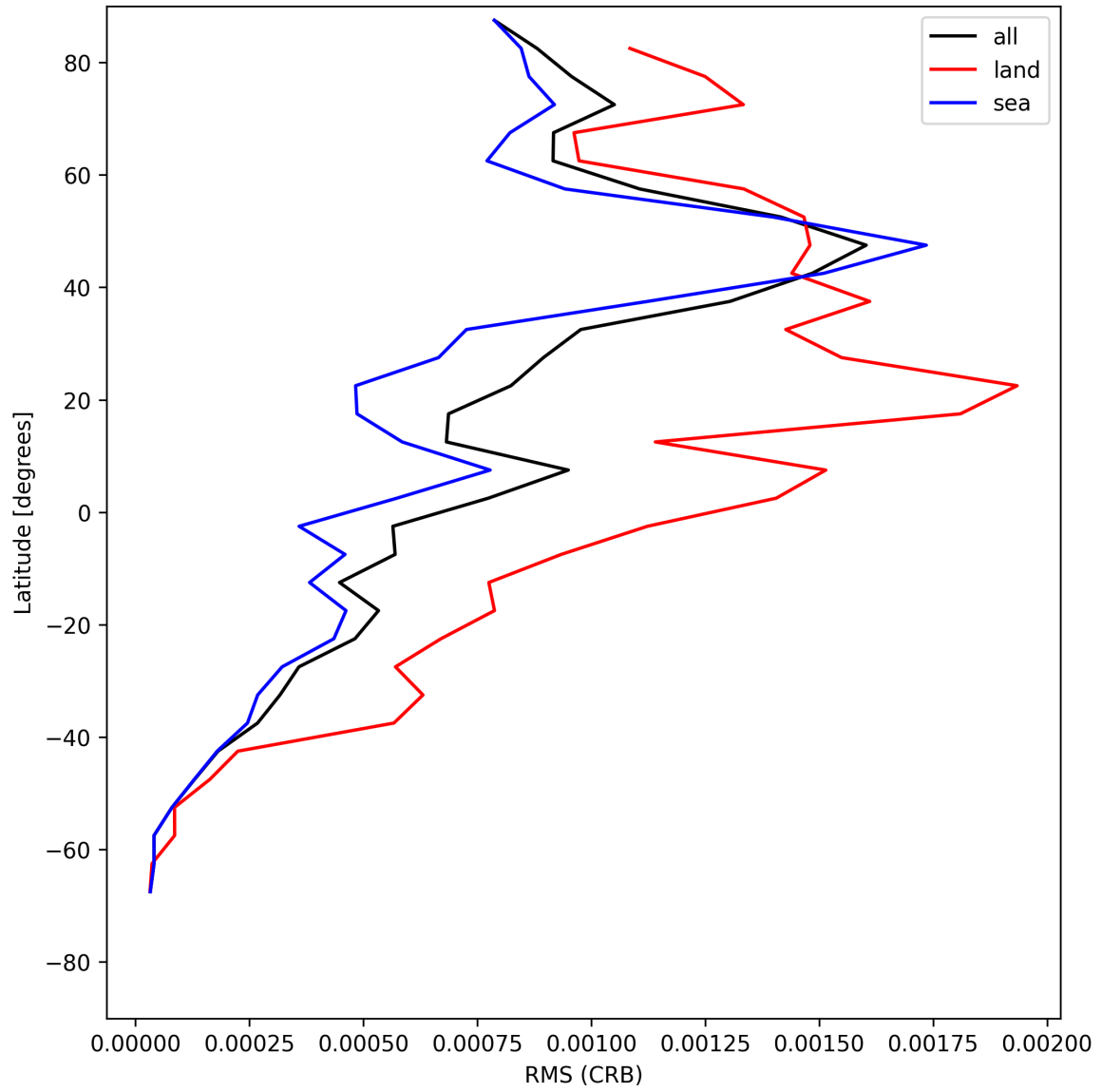
Figure 32: Zonal average of “RMS (CRB)” for 2025-05-26 to 2025-05-27.
