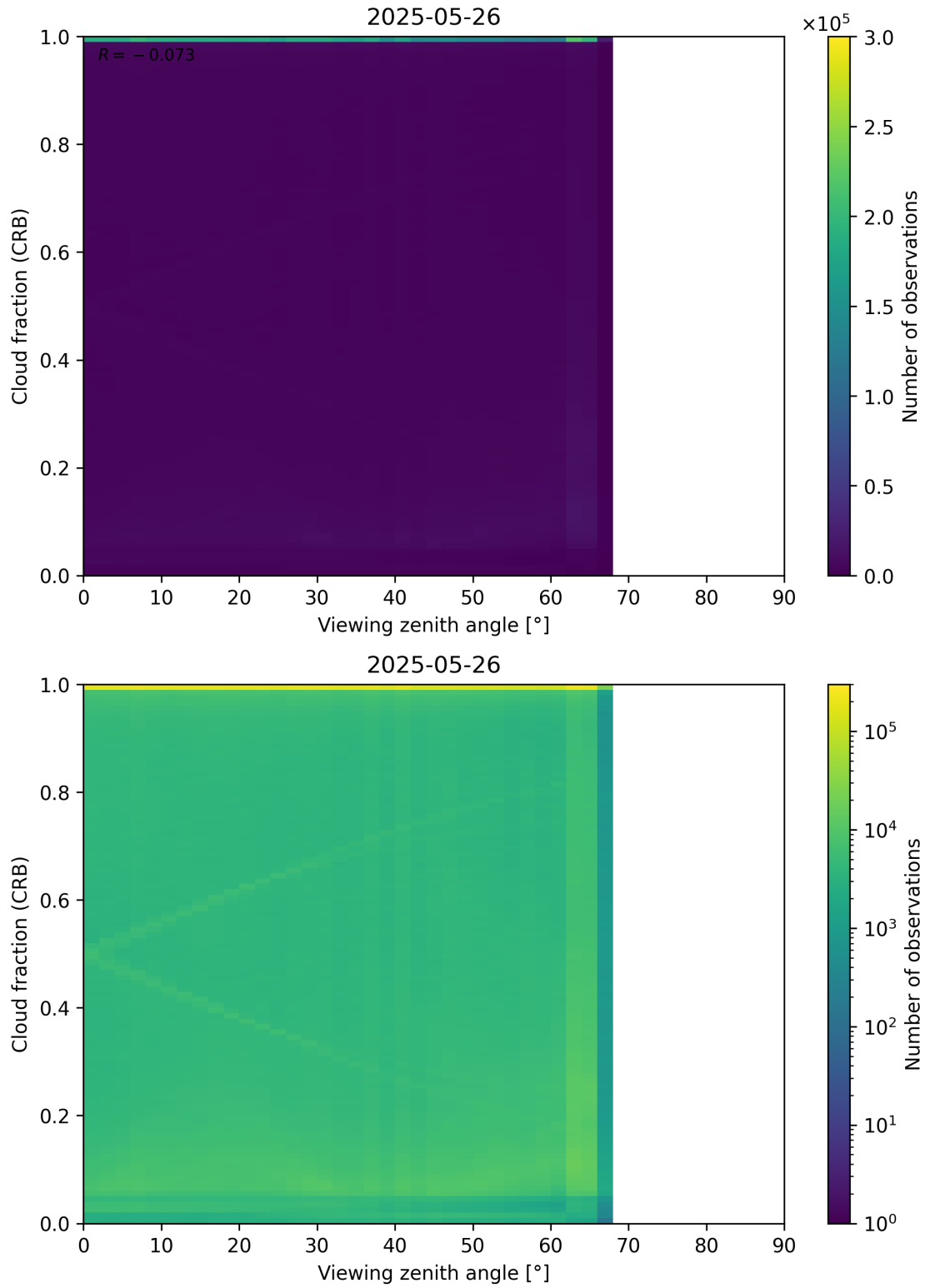
Figure 109: Scatter density plot of “Viewing zenith angle” against “Cloud fraction (CRB)” for 2025-05-26 to 2025-05-27.
