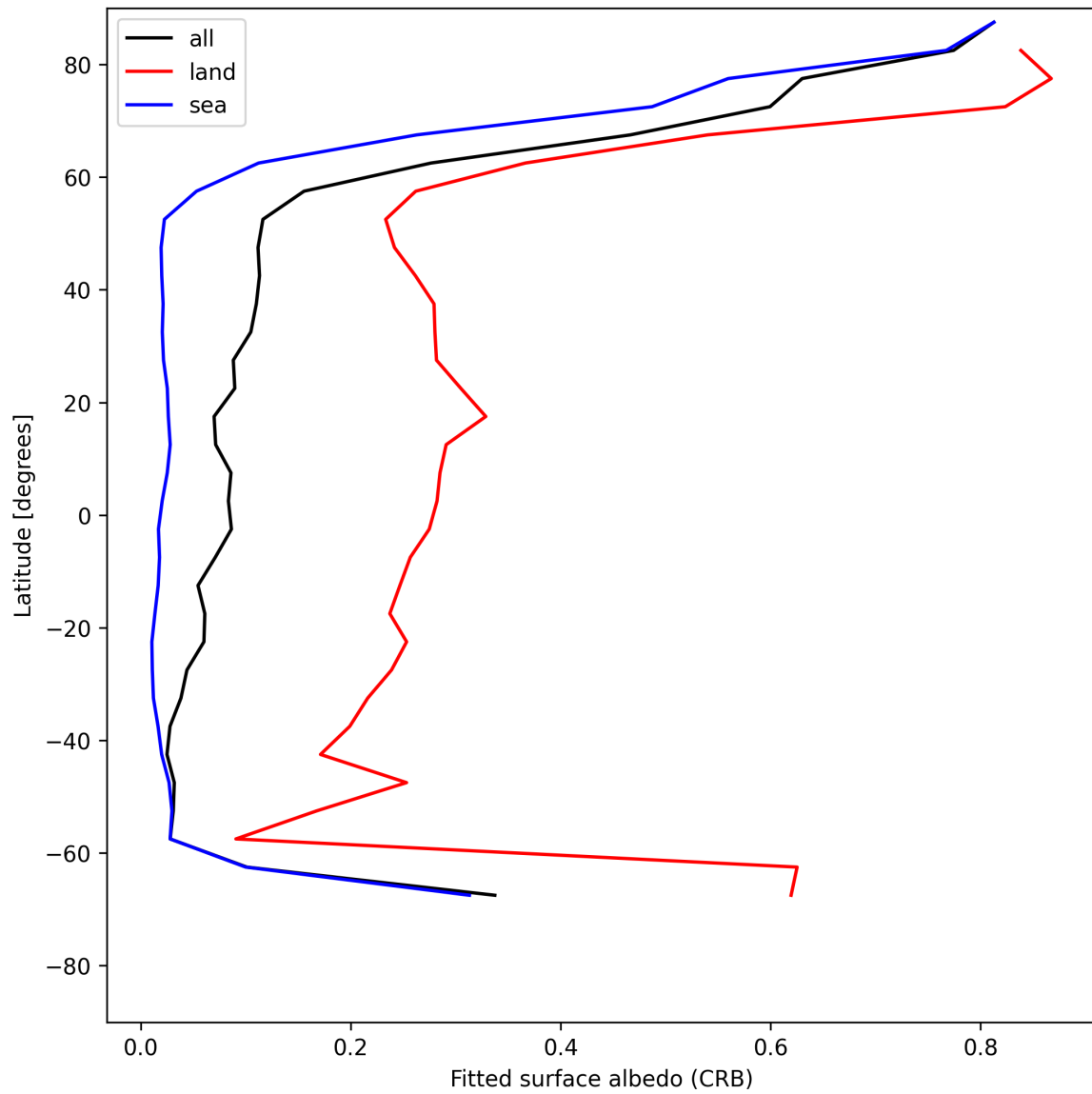
Figure 30: Zonal average of “Fitted surface albedo (CRB)” for 2025-05-26 to 2025-05-27.
