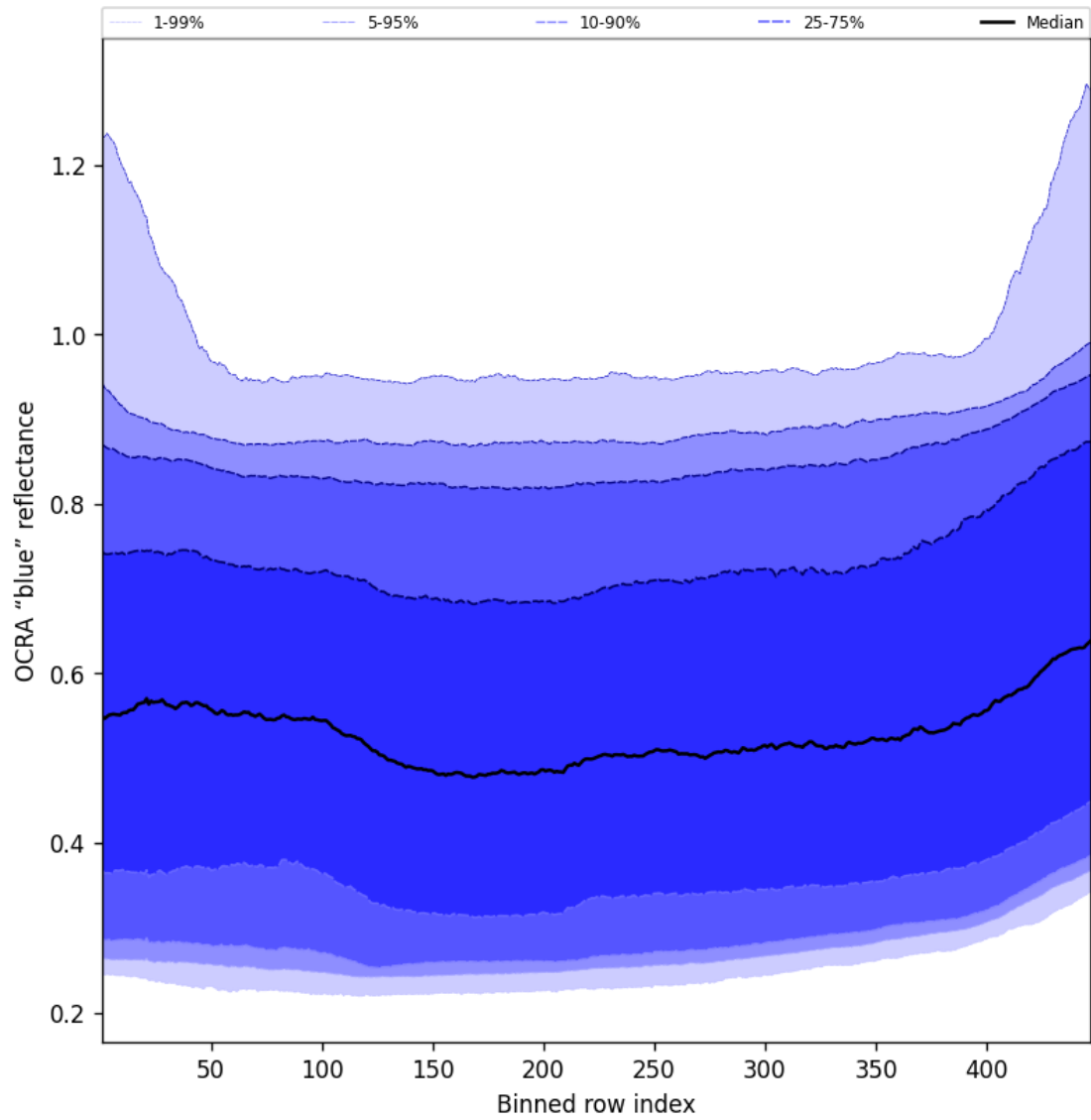
Figure 67: Along track statistics of "OCRA "blue" reflectance" for 2025-05-26 to 2025-05-27
