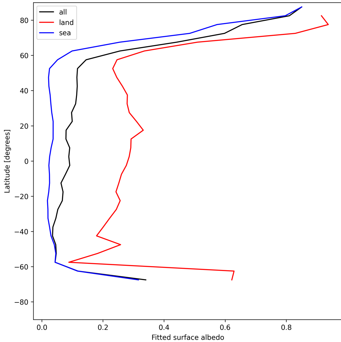
Figure 29: Zonal average of “Fitted surface albedo” for 2025-05-26 to 2025-05-27.
