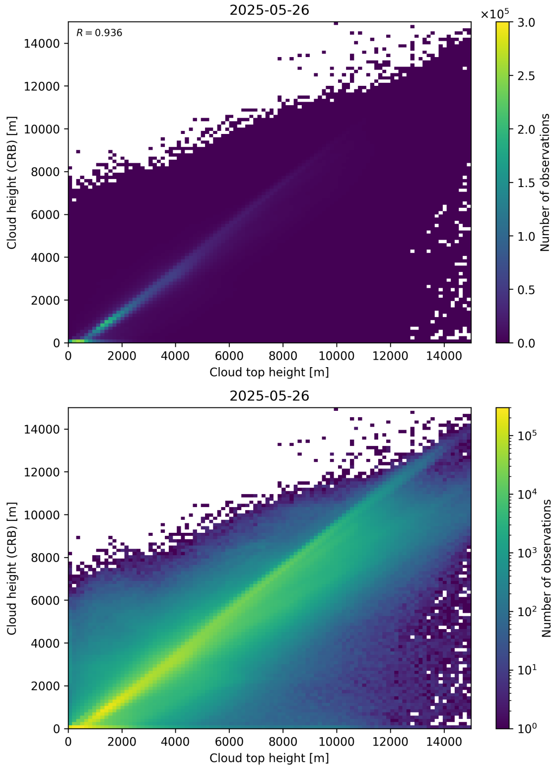
Figure 89: Scatter density plot of “Cloud top height” against “Cloud height (CRB)” for 2025-05-26 to 2025-05-27.
