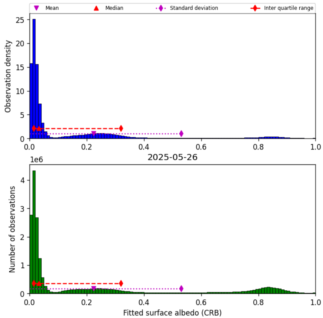
Figure 46: Histogram of “Fitted surface albedo (CRB)” for 2025-05-26 to 2025-05-27
