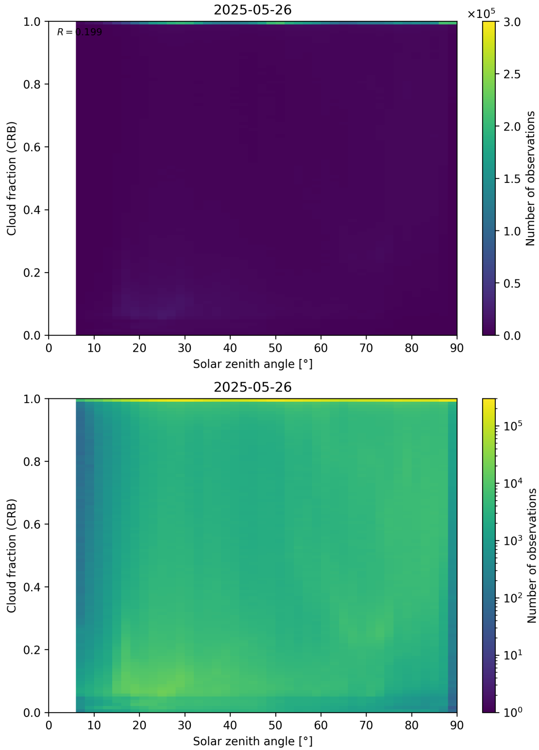
Figure 101: Scatter density plot of “Solar zenith angle” against “Cloud fraction (CRB)” for 2025-05-26 to 2025-05-27.
