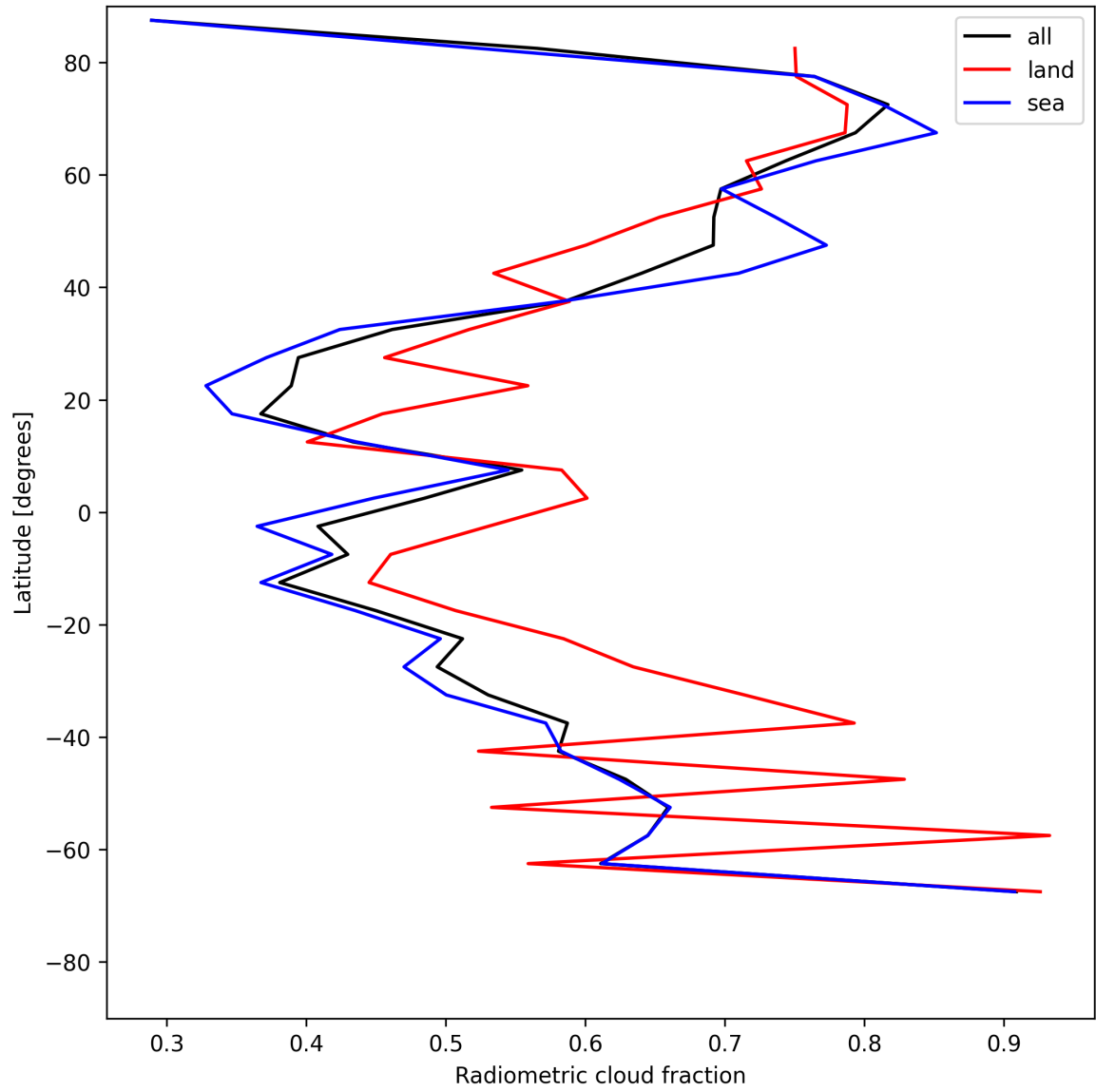
Figure 23: Zonal average of “Radiometric cloud fraction” for 2025-05-26 to 2025-05-27.
