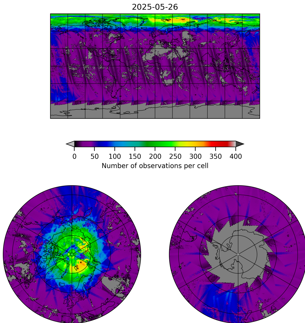
Figure 21: Map of the number of observations for 2025-05-26 to 2025-05-27
