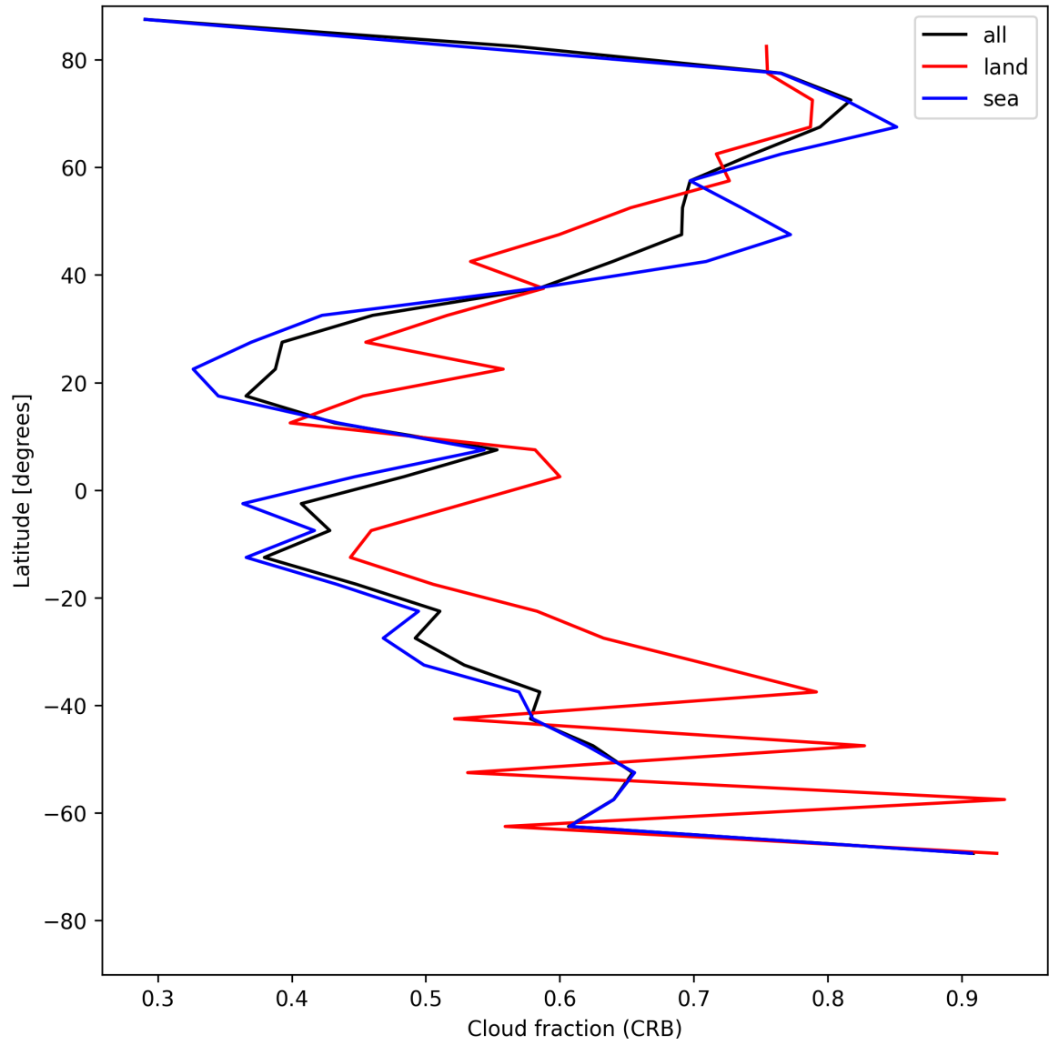
Figure 26: Zonal average of “Cloud fraction (CRB)” for 2025-05-26 to 2025-05-27.
