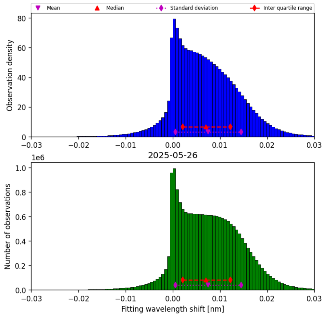
Figure 49: Histogram of “Fitting wavelength shift” for 2025-05-26 to 2025-05-27
