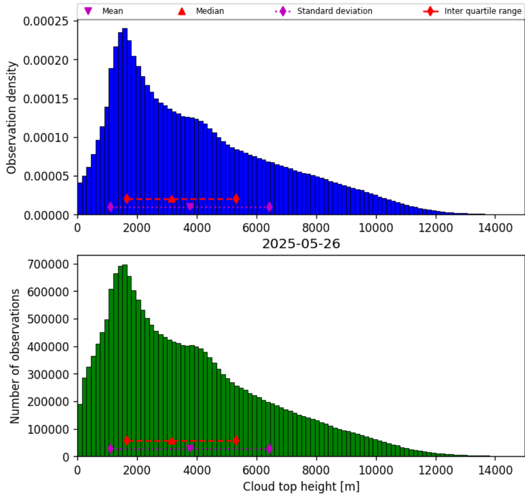
Figure 40: Histogram of “Cloud top height” for 2025-05-26 to 2025-05-27
