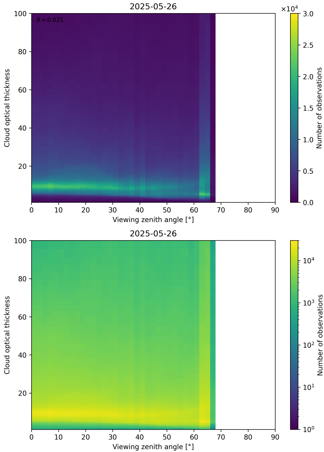
Figure 111: Scatter density plot of “Viewing zenith angle” against “Cloud optical thickness” for 2025-05-26 to 2025-05-27.
