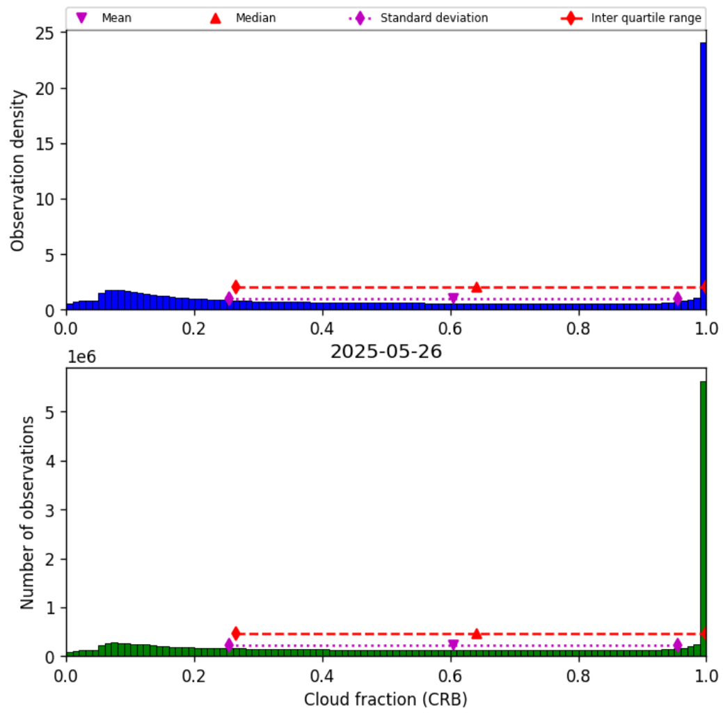
Figure 42: Histogram of “Cloud fraction (CRB)” for 2025-05-26 to 2025-05-27
