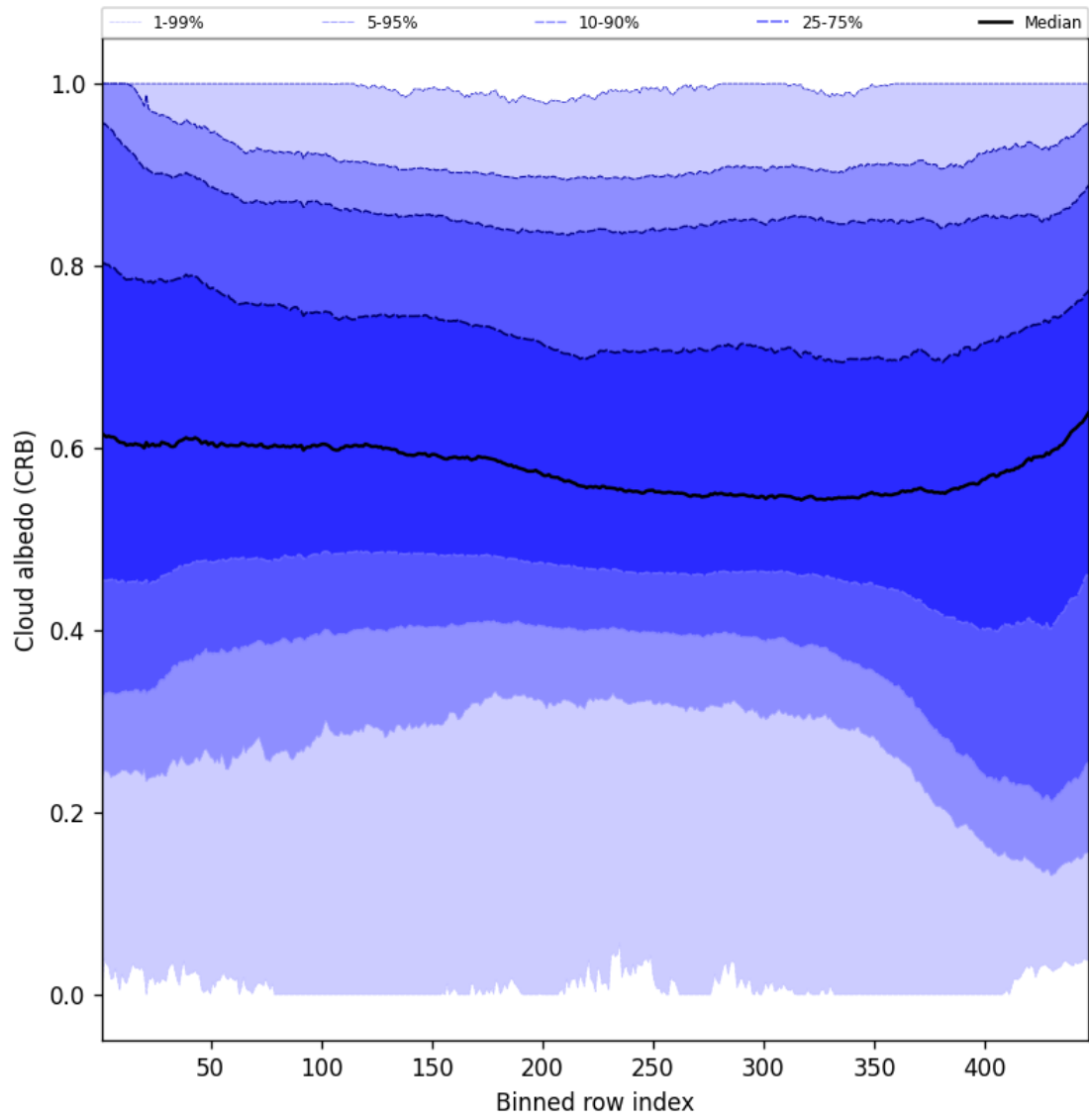
Figure 60: Along track statistics of “Cloud albedo (CRB)” for 2025-05-26 to 2025-05-27
