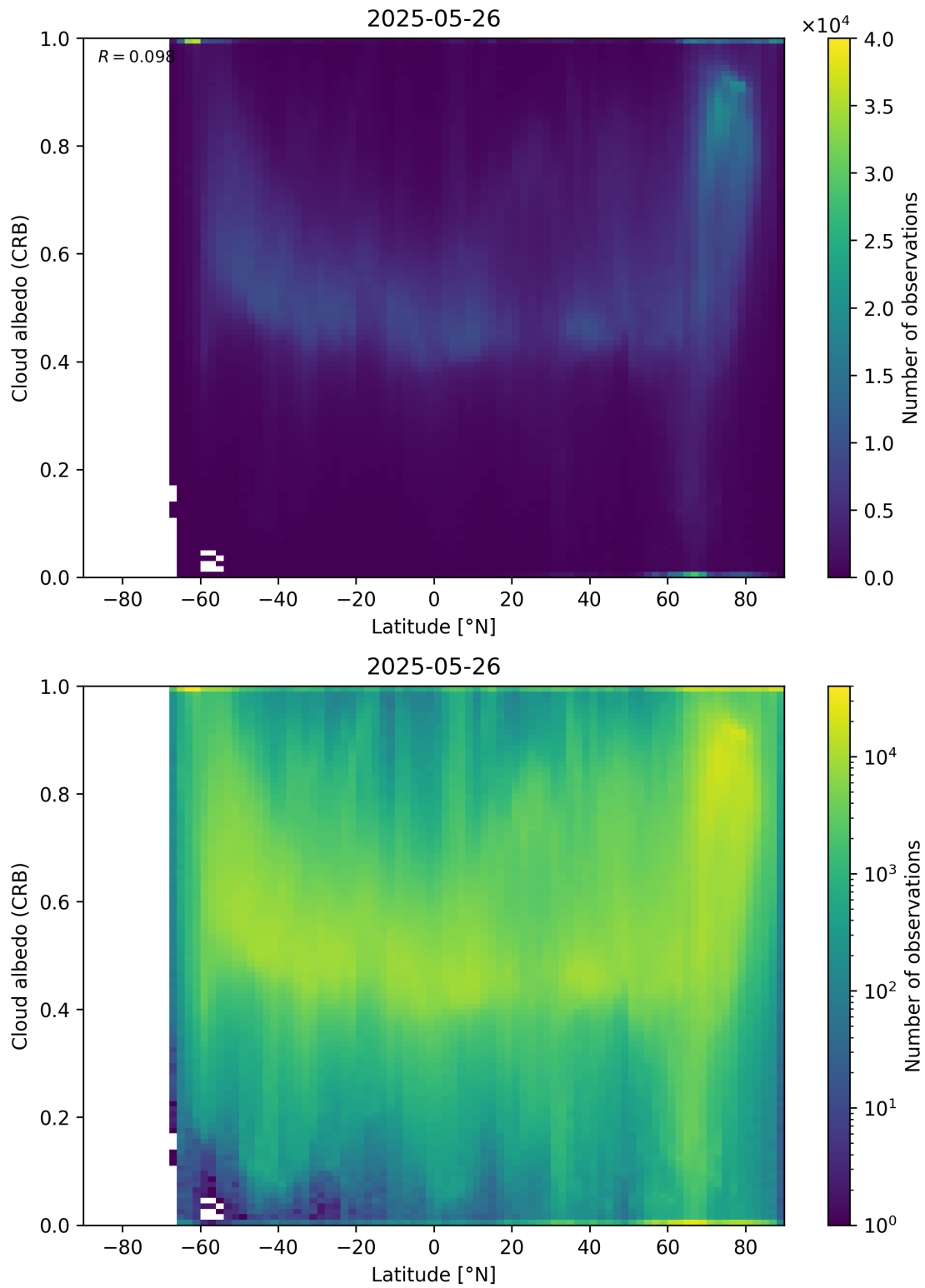
Figure 91: Scatter density plot of “Latitude” against “Cloud albedo (CRB)” for 2025-05-26 to 2025-05-27.
