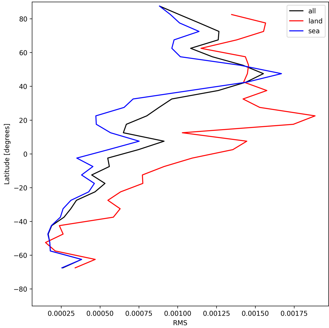
Figure 31: Zonal average of “RMS” for 2025-05-26 to 2025-05-27.
