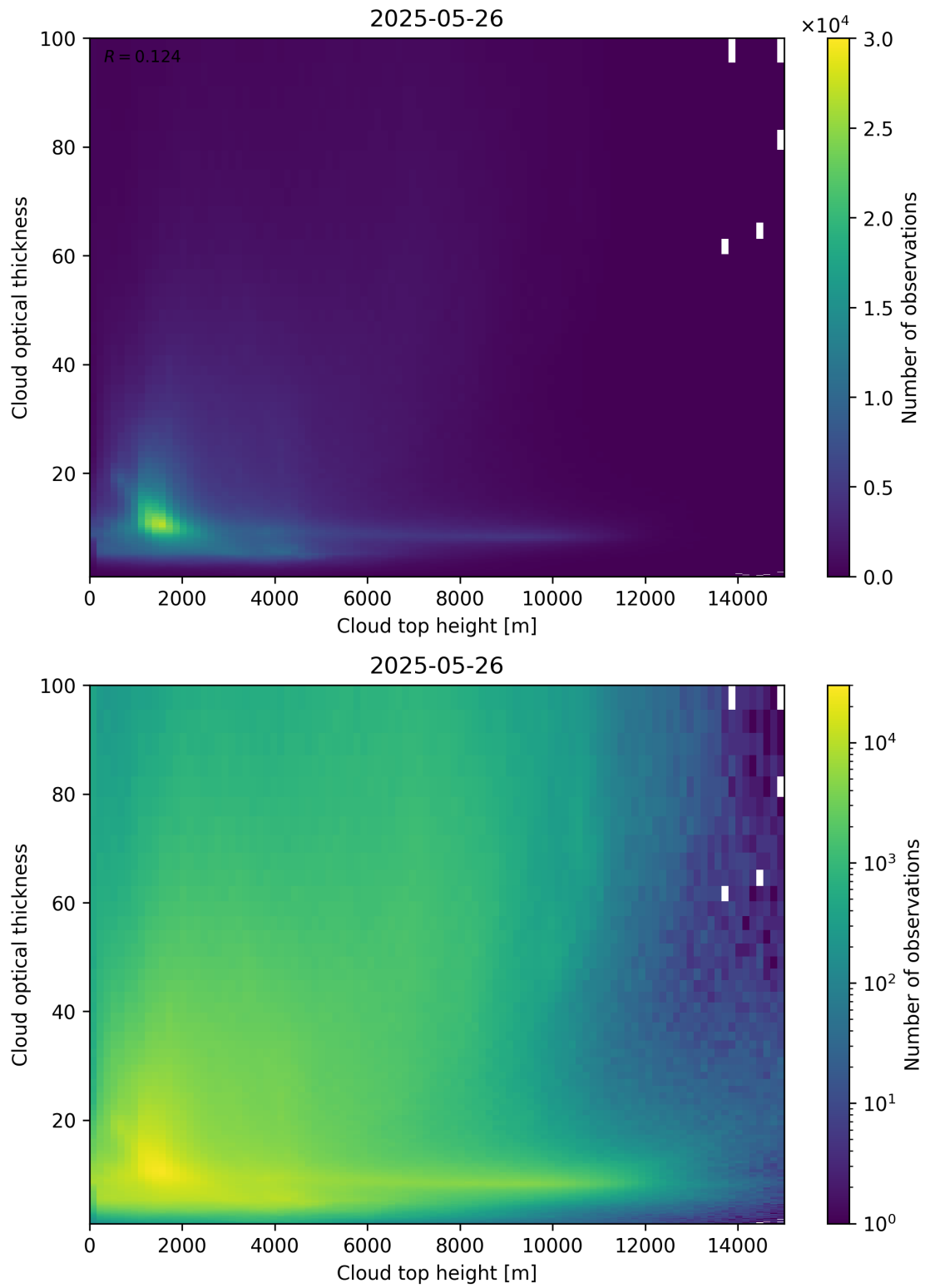
Figure 90: Scatter density plot of “Cloud top height” against “Cloud optical thickness” for 2025-05-26 to 2025-05-27.
