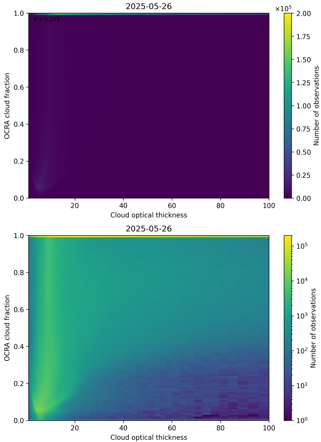
Figure 83: Scatter density plot of “Cloud optical thickness” against “OCRA cloud fraction” for 2025-05-26 to 2025-05-27.
