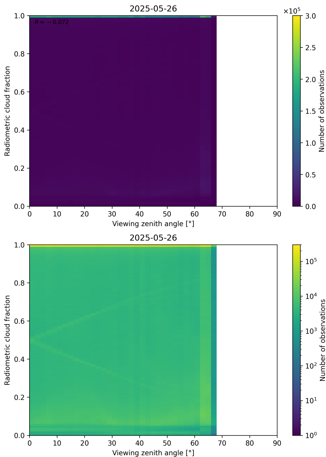
Figure 107: Scatter density plot of “Viewing zenith angle” against “Radiometric cloud fraction” for 2025-05-26 to 2025-05-27.
