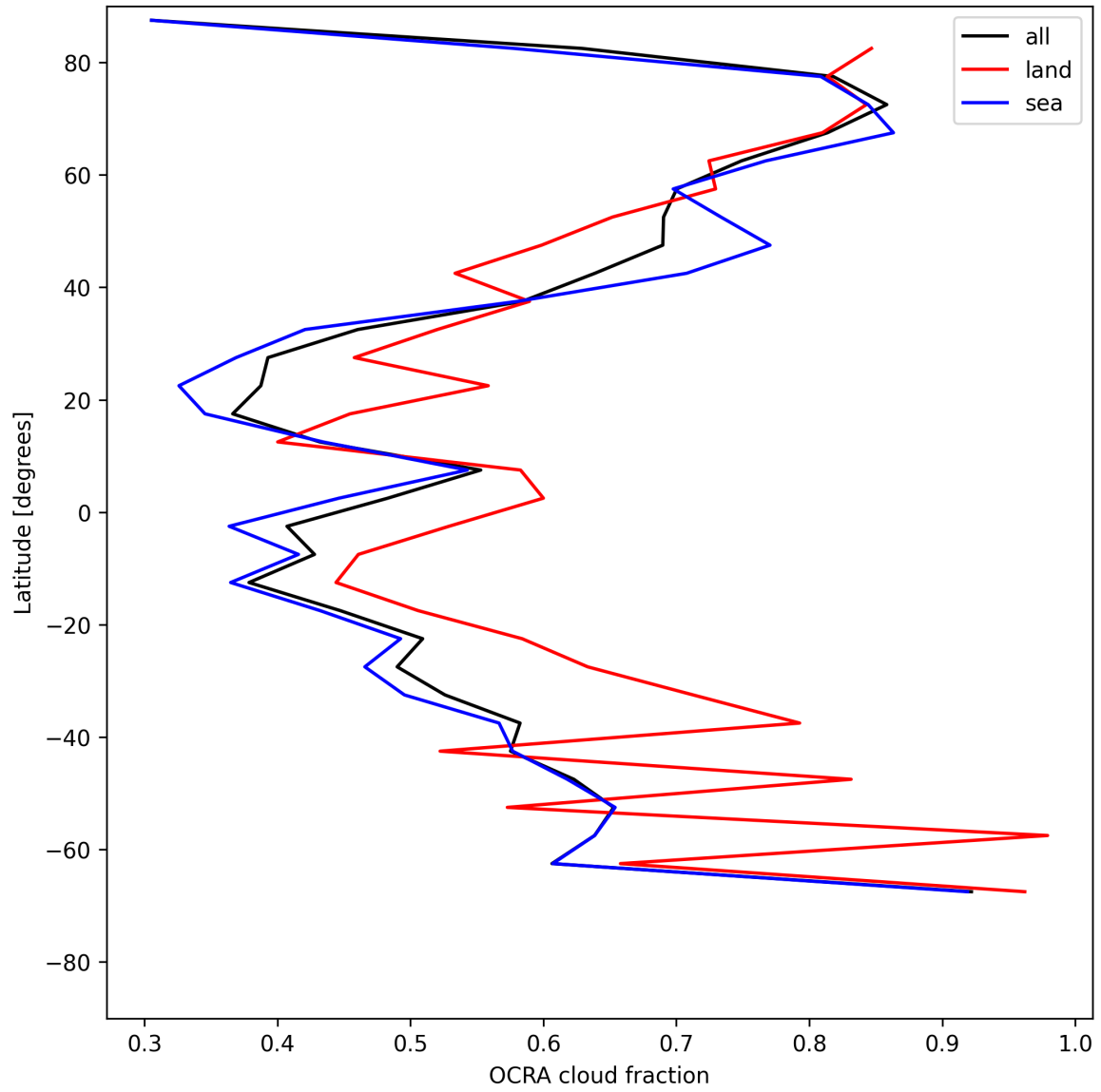
Figure 34: Zonal average of “OCRA cloud fraction” for 2025-05-26 to 2025-05-27.
