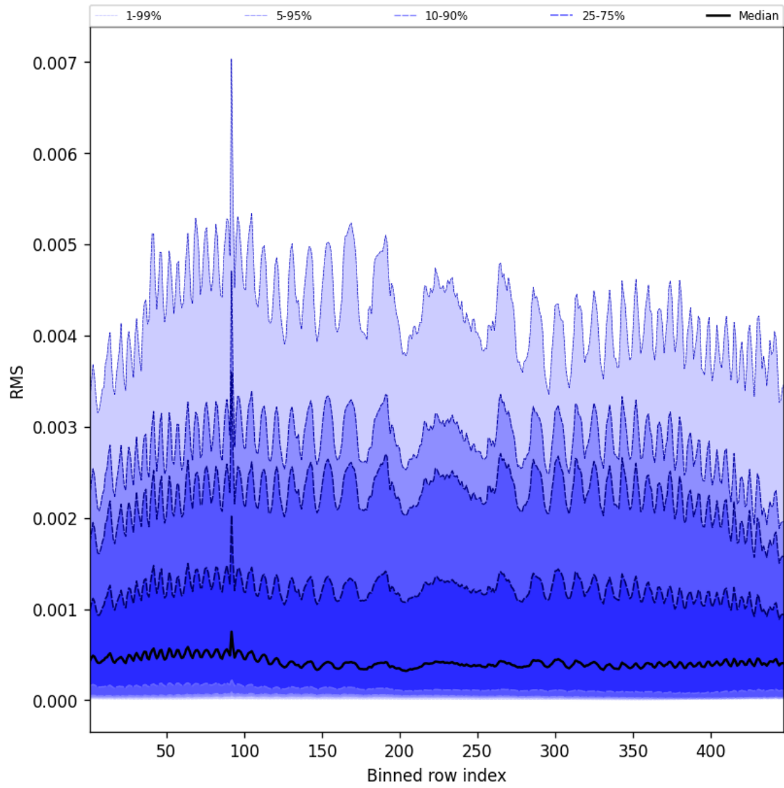
Figure 63: Along track statistics of “RMS” for 2025-05-26 to 2025-05-27
