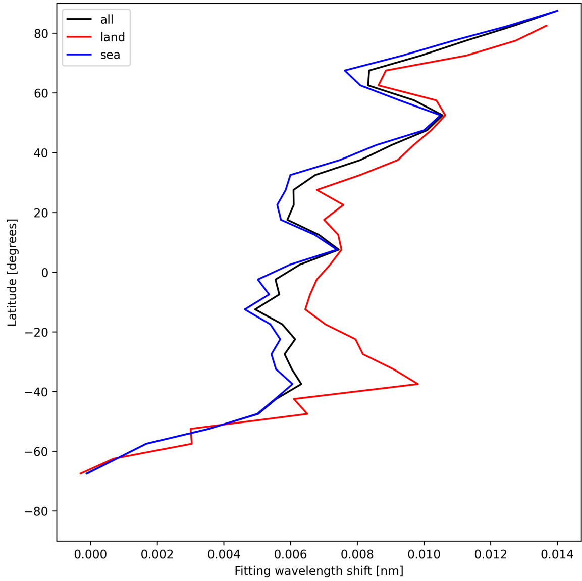
Figure 33: Zonal average of “Fitting wavelength shift” for 2025-05-26 to 2025-05-27.
