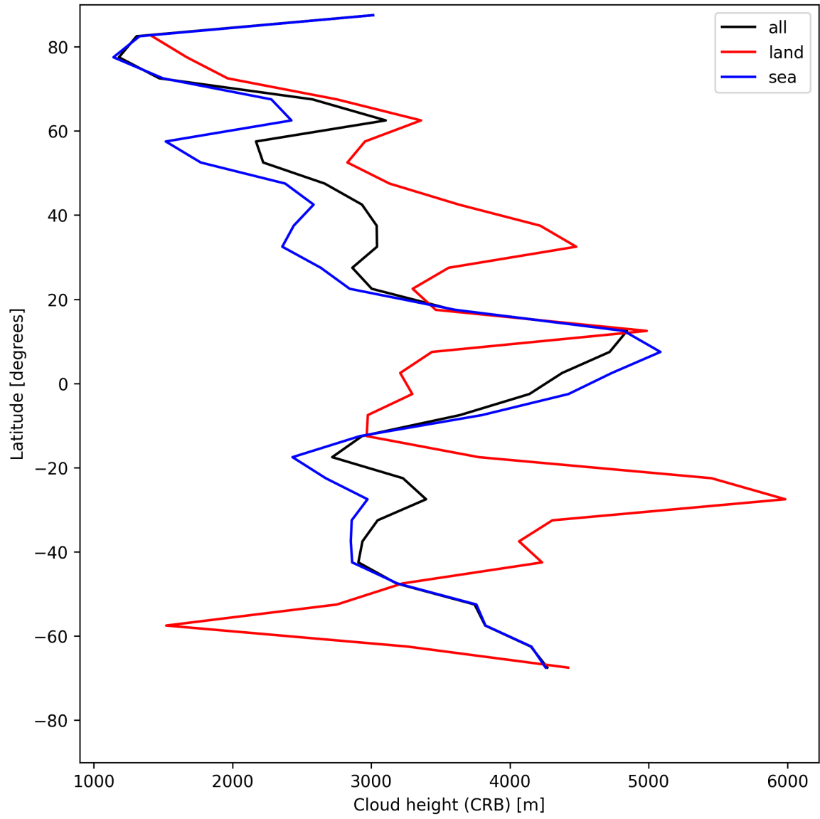
Figure 27: Zonal average of “Cloud height (CRB)” for 2025-05-26 to 2025-05-27.
