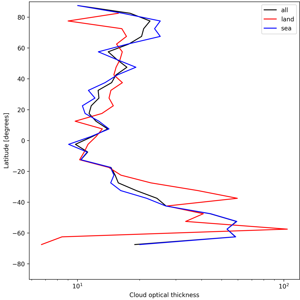
Figure 25: Zonal average of “Cloud optical thickness” for 2025-05-26 to 2025-05-27.
