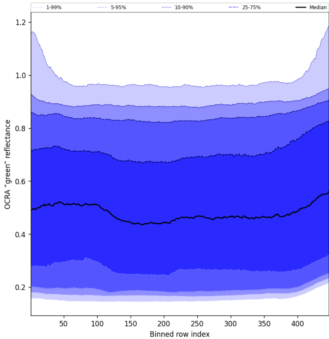
Figure 68: Along track statistics of "OCRA "green" reflectance" for 2025-05-26 to 2025-05-27
