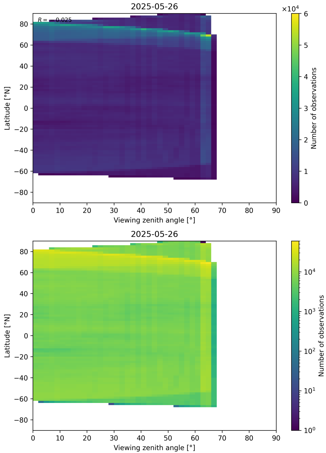
Figure 113: Scatter density plot of “Viewing zenith angle” against “Latitude” for 2025-05-26 to 2025-05-27.
