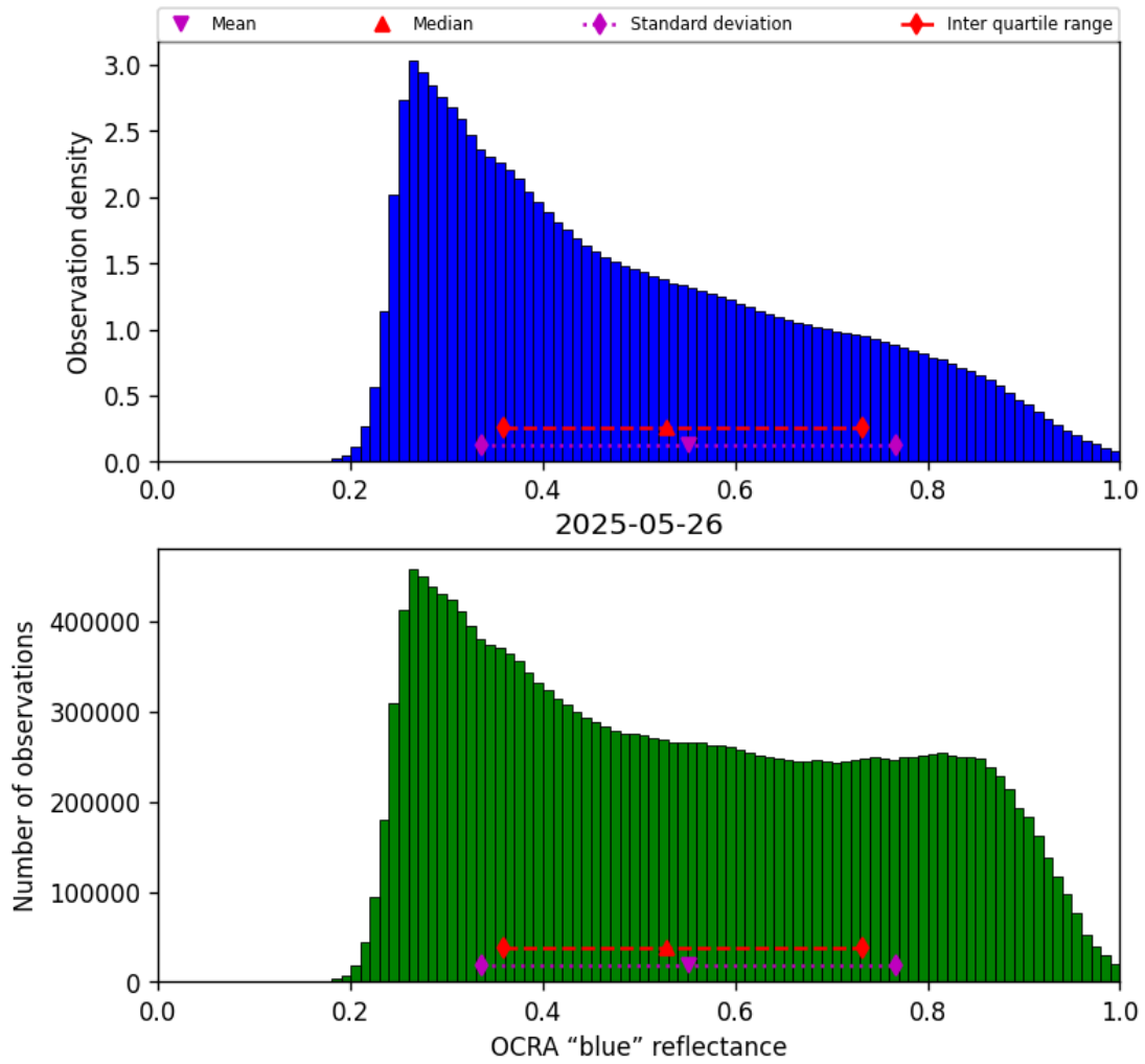
Figure 51: Histogram of “OCRA “blue” reflectance” for 2025-05-26 to 2025-05-27
