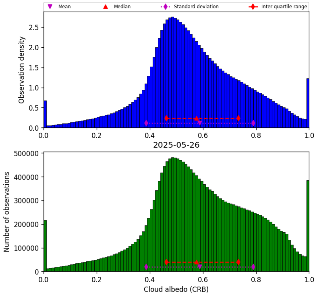
Figure 44: Histogram of “Cloud albedo (CRB)” for 2025-05-26 to 2025-05-27
