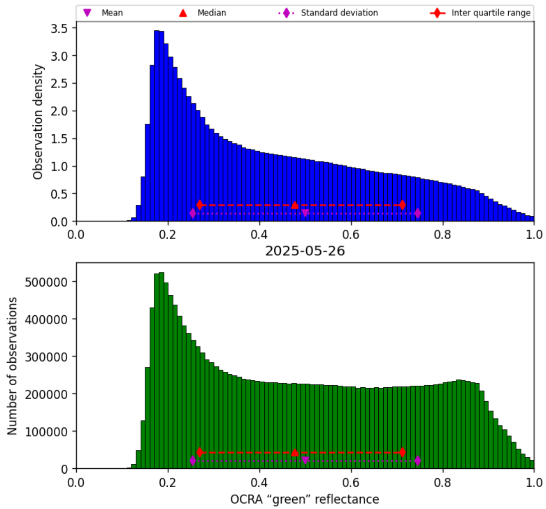
Figure 52: Histogram of “OCRA “green” reflectance” for 2025-05-26 to 2025-05-27
