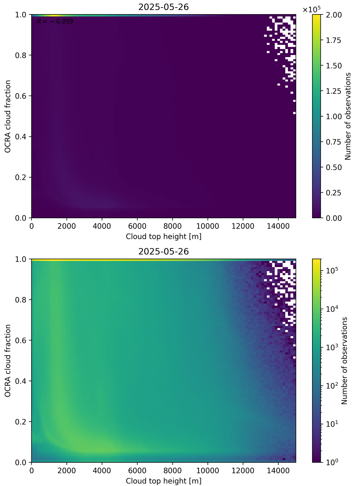
Figure 87: Scatter density plot of “Cloud top height” against “OCRA cloud fraction” for 2025-05-26 to 2025-05-27.
