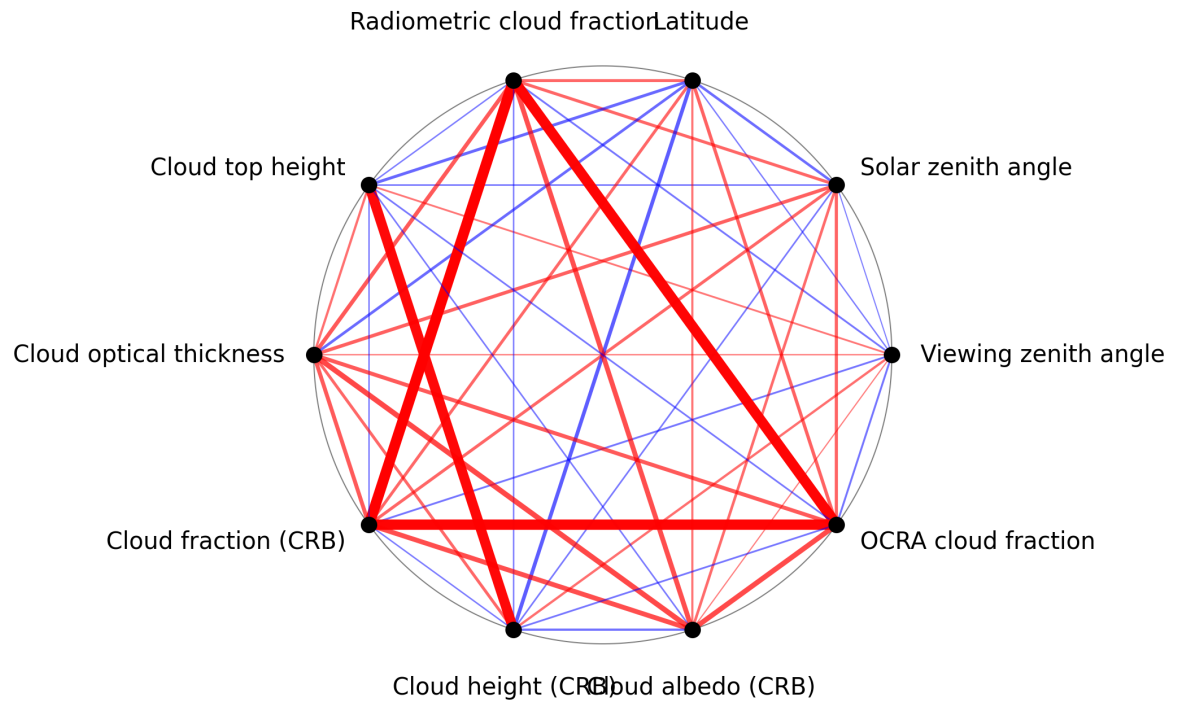
Figure 1: Map of correlation graph for 2025-05-26 to 2025-05-27.
