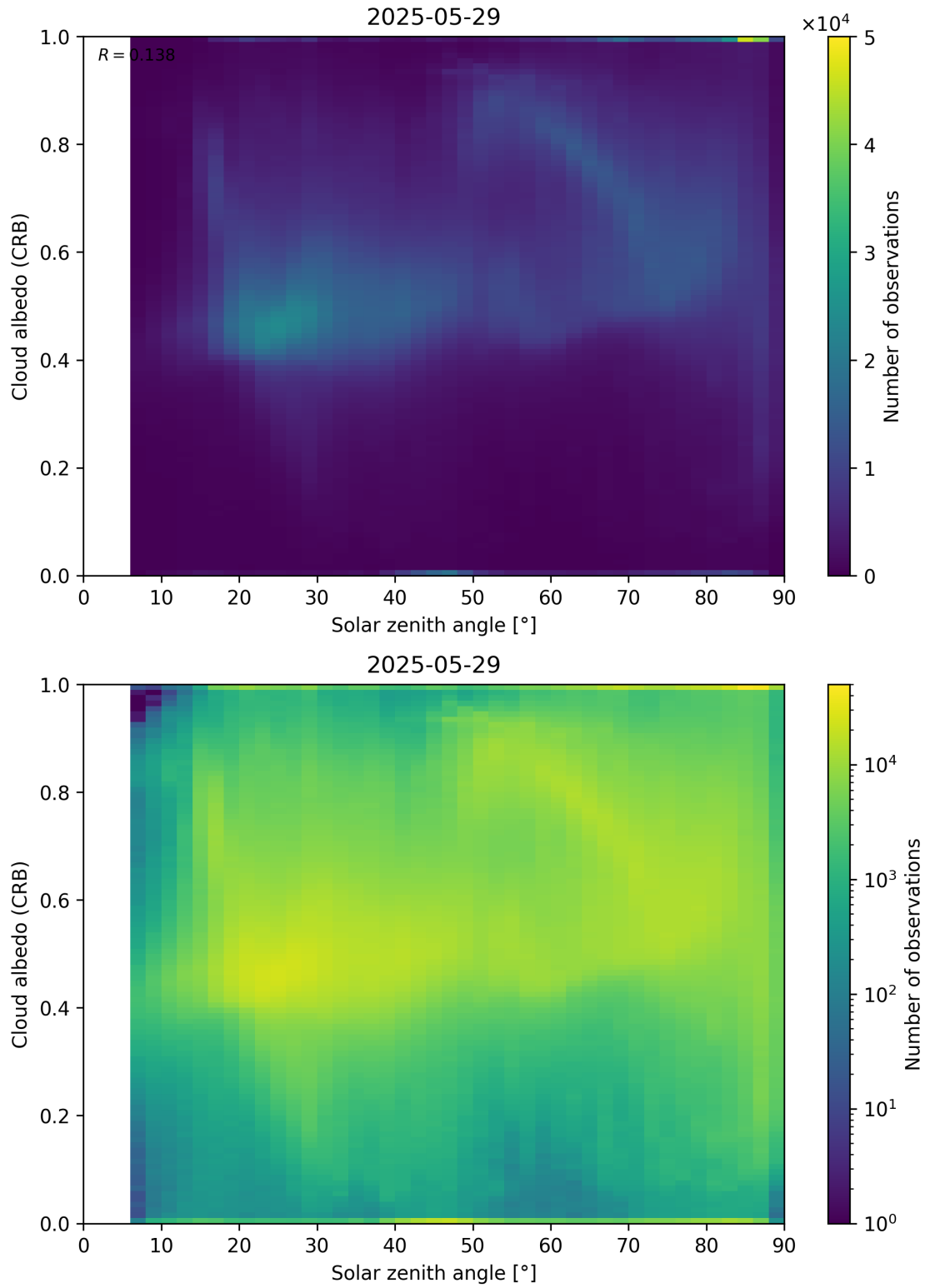
Figure 98: Scatter density plot of “Solar zenith angle” against “Cloud albedo (CRB)” for 2025-05-28 to 2025-05-30.
