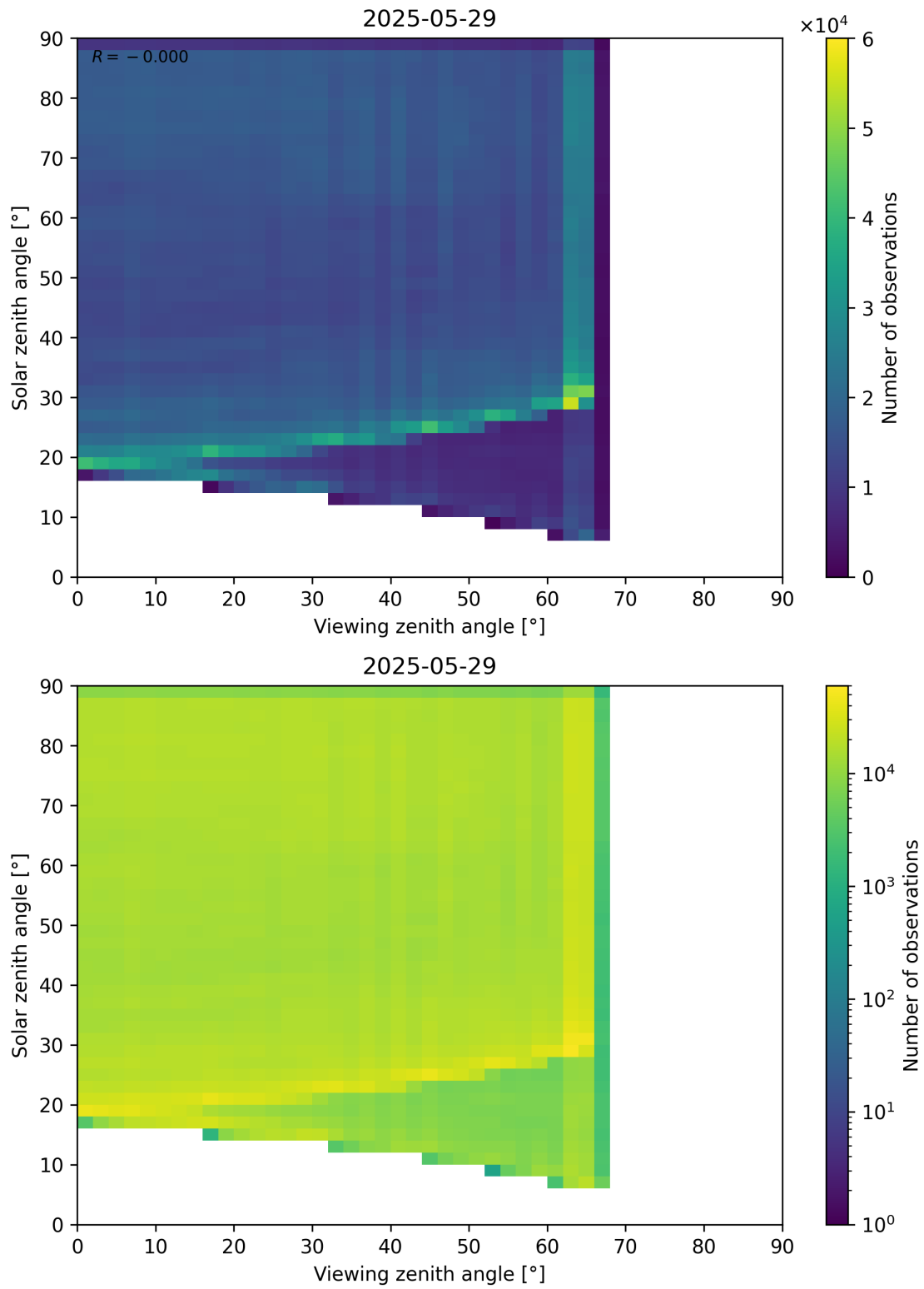
Figure 114: Scatter density plot of “Viewing zenith angle” against “Solar zenith angle” for 2025-05-28 to 2025-05-30.
