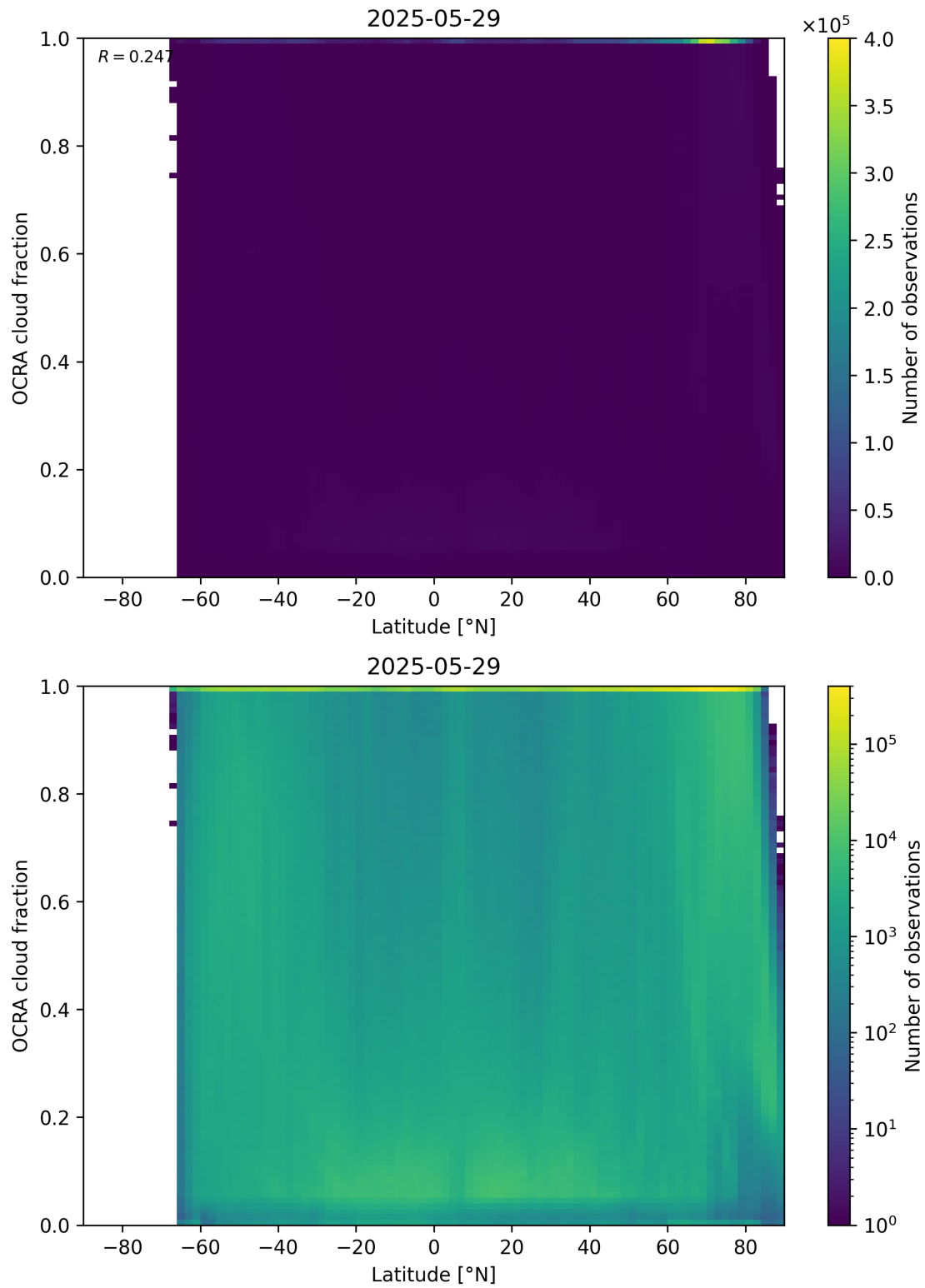
Figure 93: Scatter density plot of “Latitude” against “OCRA cloud fraction” for 2025-05-28 to 2025-05-30.
