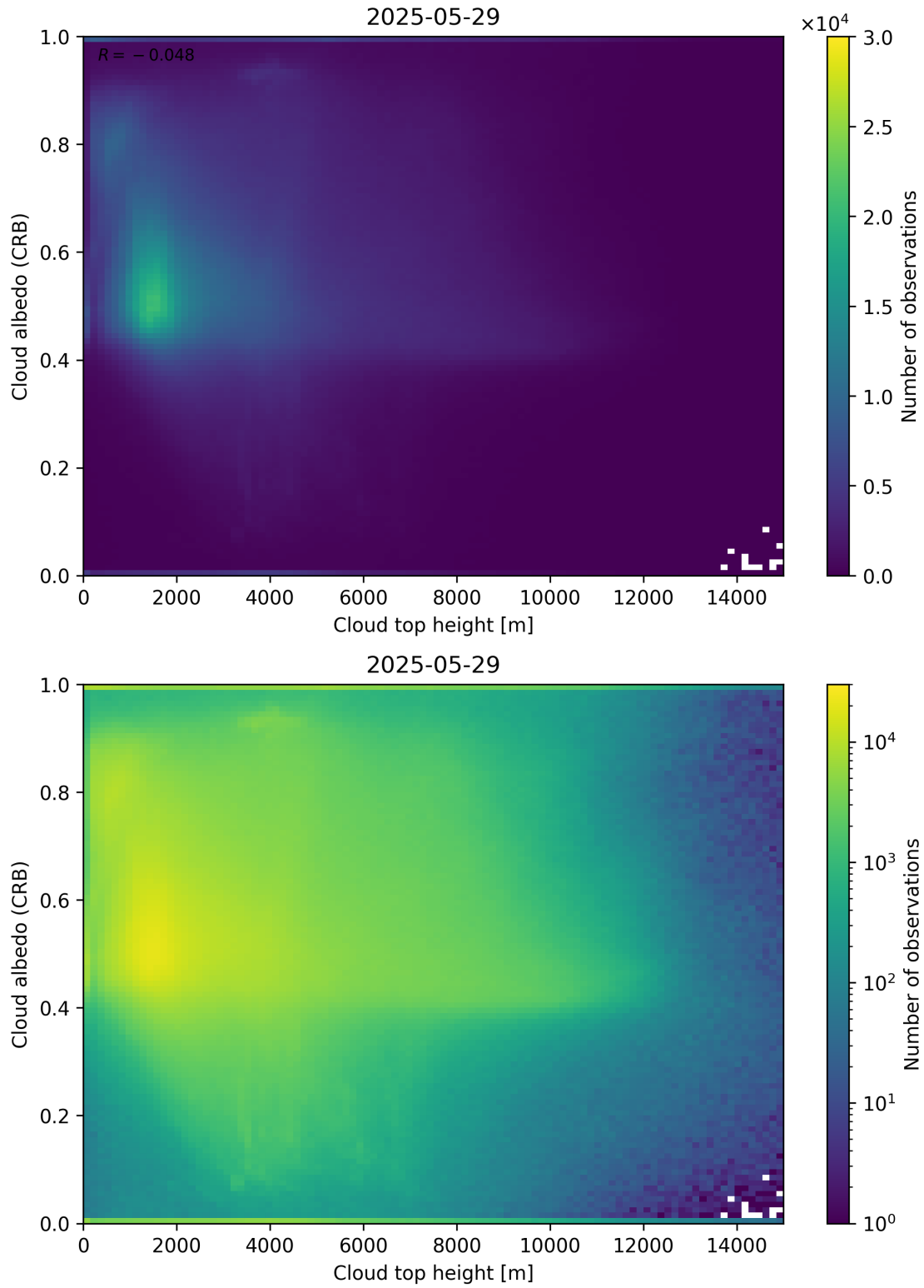
Figure 86: Scatter density plot of “Cloud top height” against “Cloud albedo (CRB)” for 2025-05-28 to 2025-05-30.
