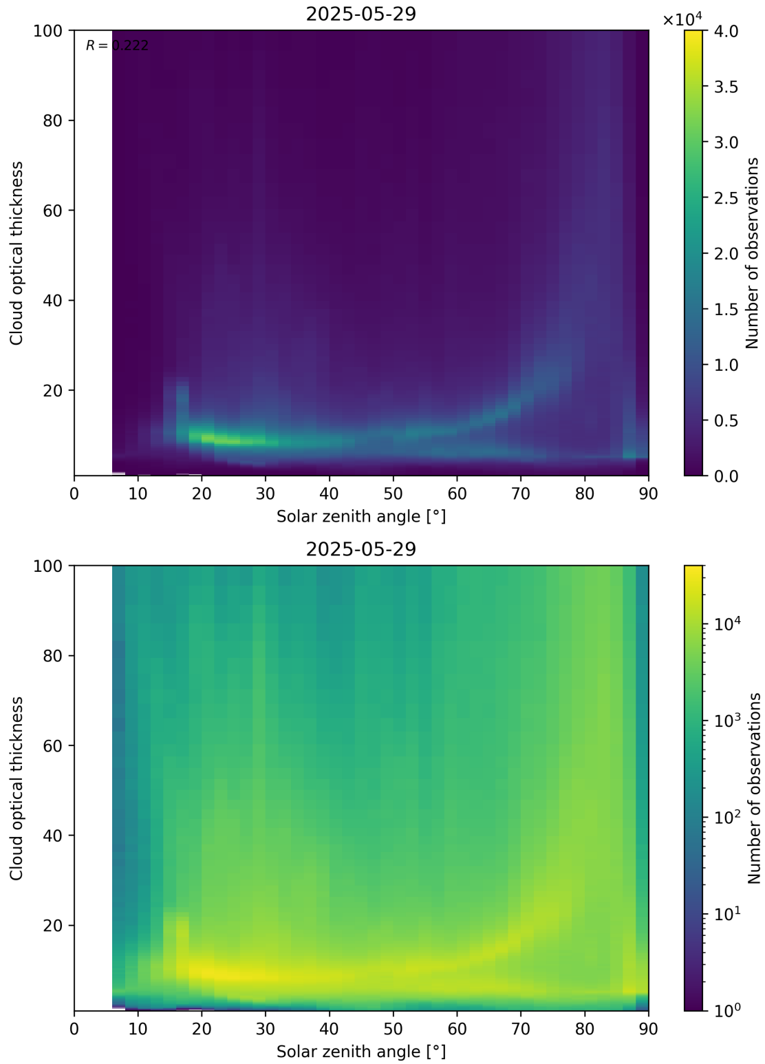
Figure 103: Scatter density plot of “Solar zenith angle” against “Cloud optical thickness” for 2025-05-28 to 2025-05-30.
