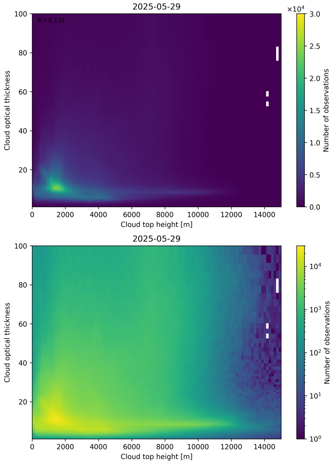
Figure 90: Scatter density plot of “Cloud top height” against “Cloud optical thickness” for 2025-05-28 to 2025-05-30.
