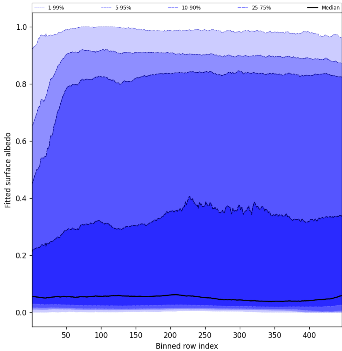
Figure 61: Along track statistics of “Fitted surface albedo” for 2025-05-28 to 2025-05-30
