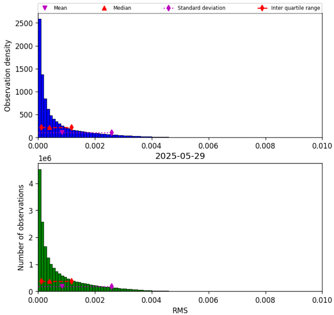
Figure 47: Histogram of “RMS” for 2025-05-28 to 2025-05-30
