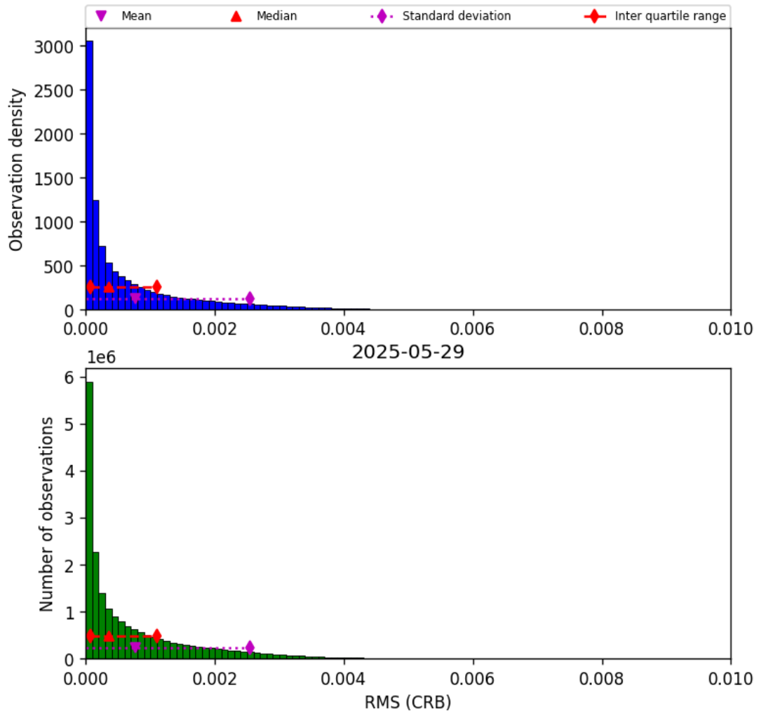
Figure 48: Histogram of “RMS (CRB)” for 2025-05-28 to 2025-05-30
