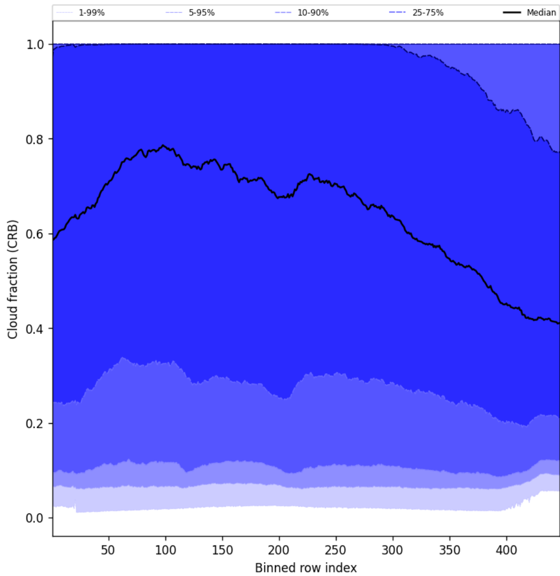
Figure 58: Along track statistics of “Cloud fraction (CRB)” for 2025-05-28 to 2025-05-30
