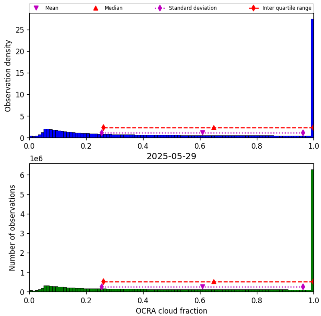
Figure 50: Histogram of “OCRA cloud fraction” for 2025-05-28 to 2025-05-30
