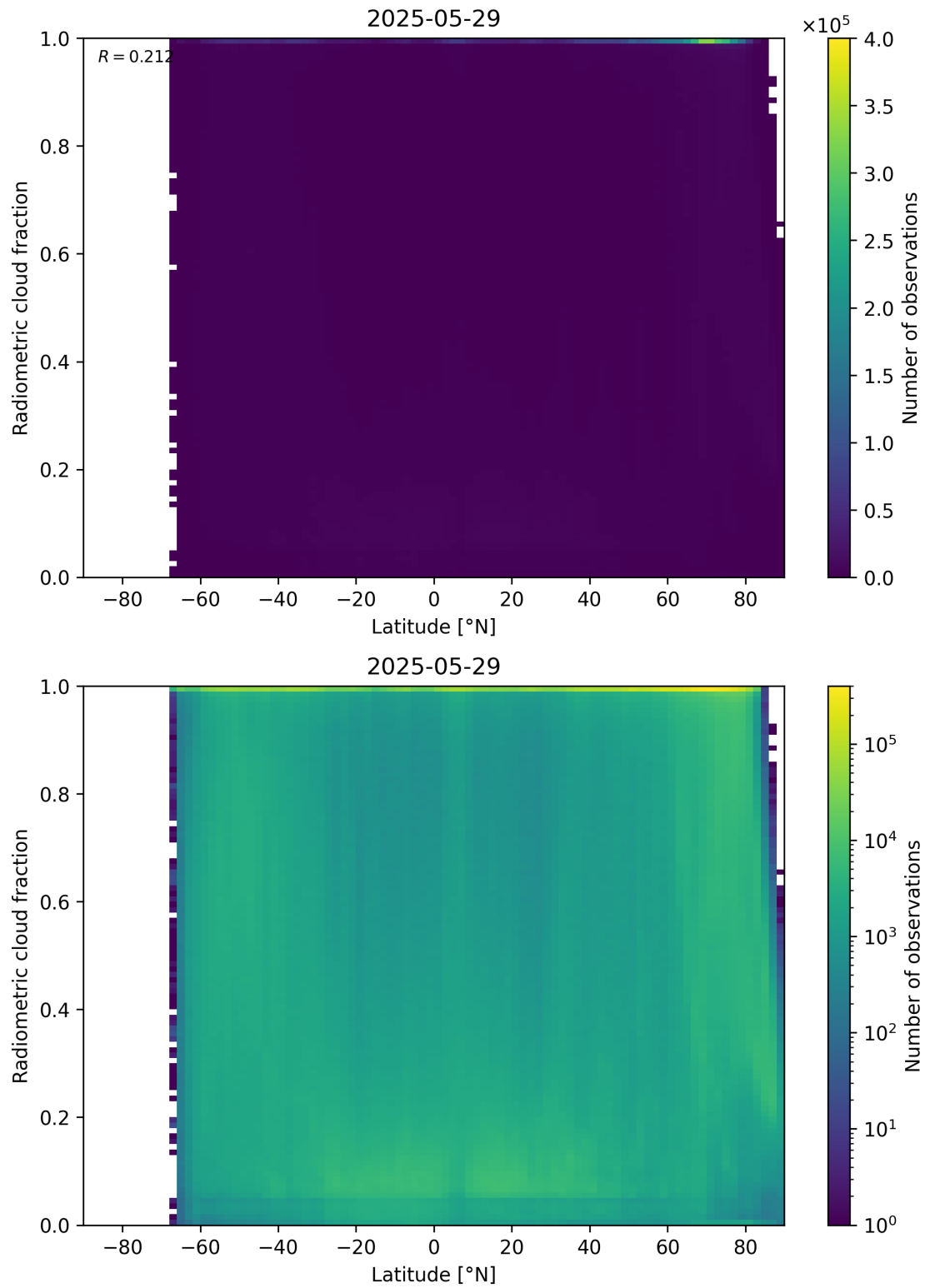
Figure 92: Scatter density plot of “Latitude” against “Radiometric cloud fraction” for 2025-05-28 to 2025-05-30.
