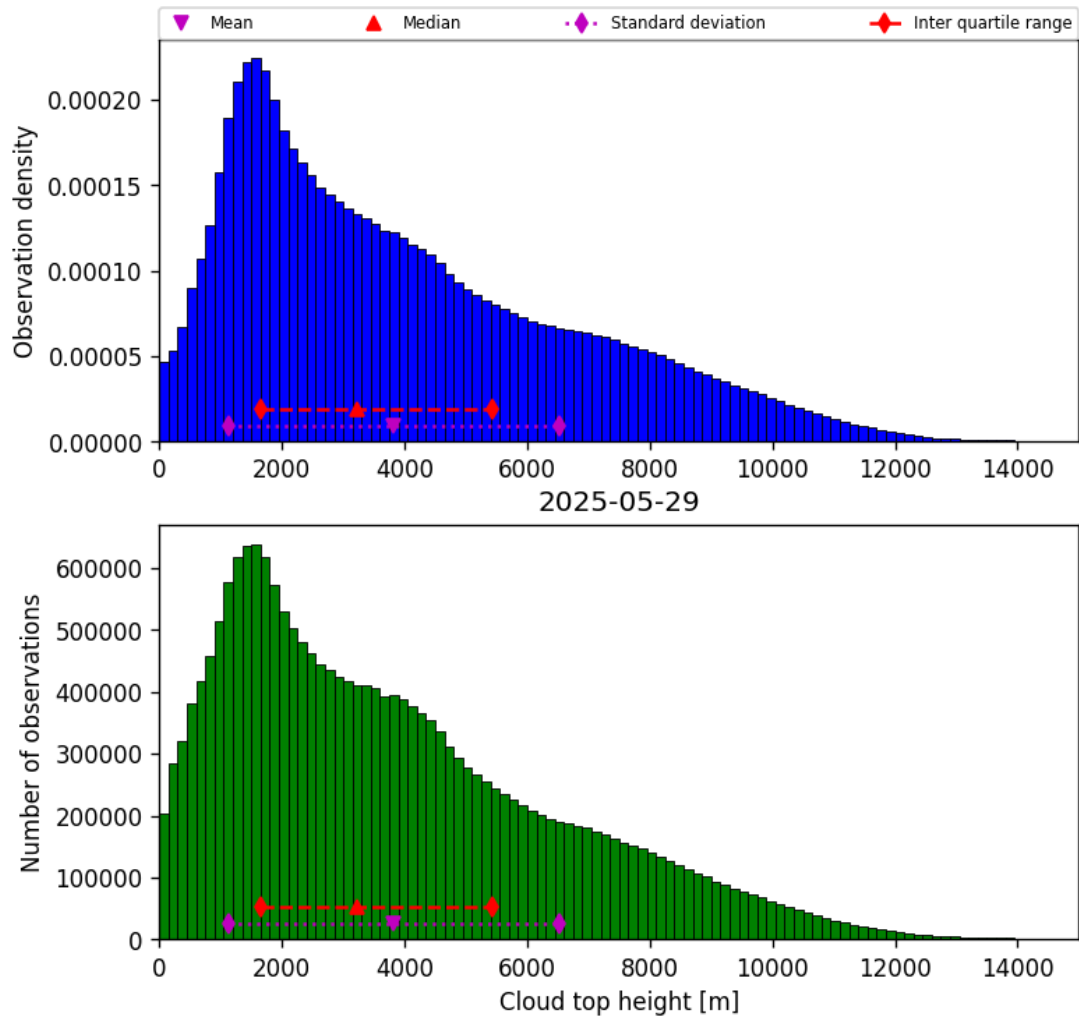
Figure 40: Histogram of “Cloud top height” for 2025-05-28 to 2025-05-30
