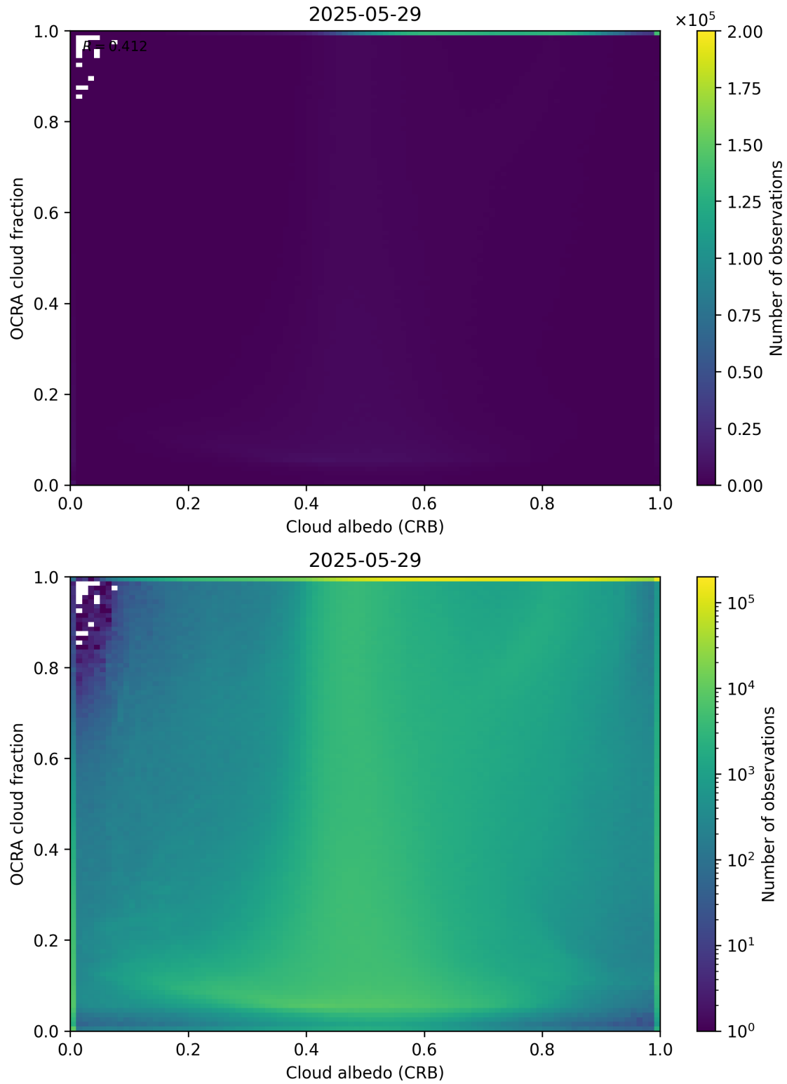
Figure 70: Scatter density plot of “Cloud albedo (CRB)” against “OCRA cloud fraction” for 2025-05-28 to 2025-05-30.
