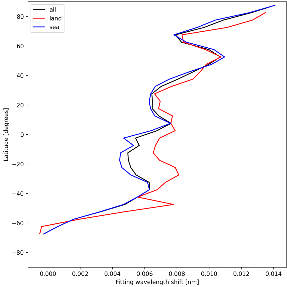
Figure 33: Zonal average of “Fitting wavelength shift” for 2025-05-28 to 2025-05-30.
