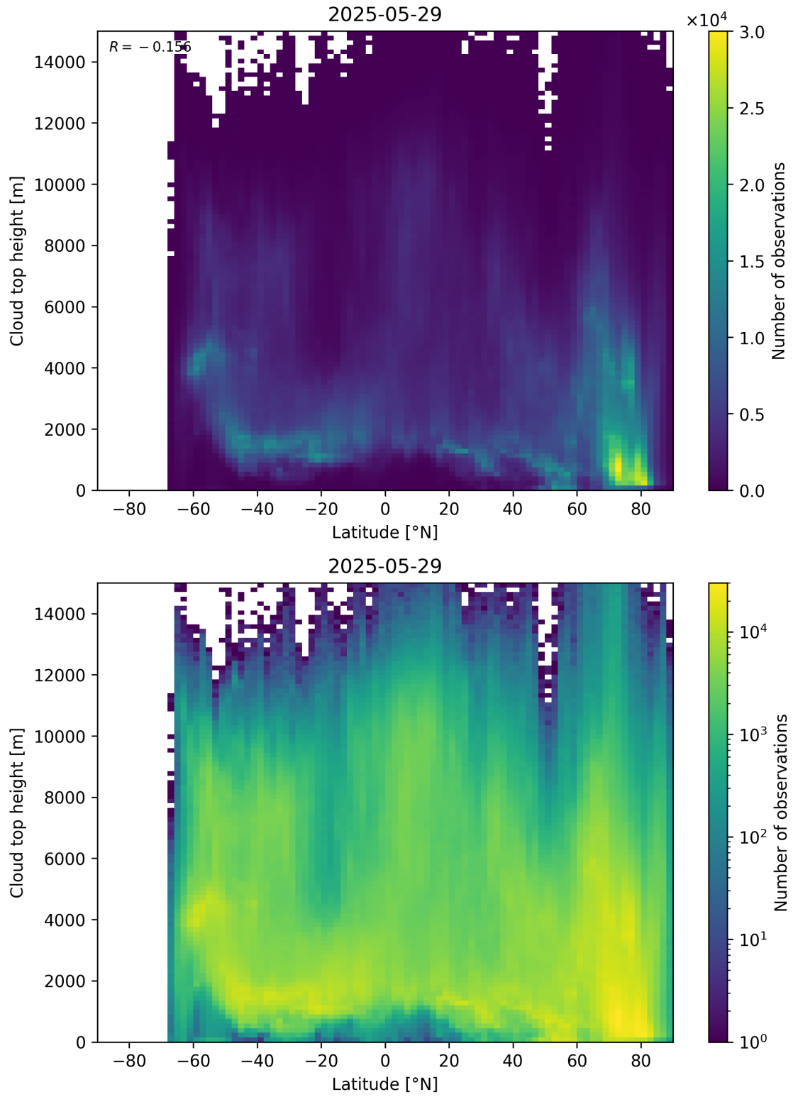
Figure 97: Scatter density plot of “Latitude” against “Cloud top height” for 2025-05-28 to 2025-05-30.
