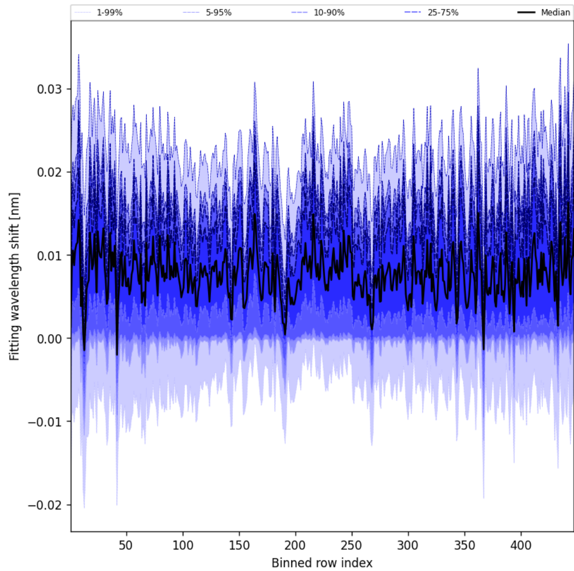
Figure 65: Along track statistics of “Fitting wavelength shift” for 2025-05-28 to 2025-05-30
