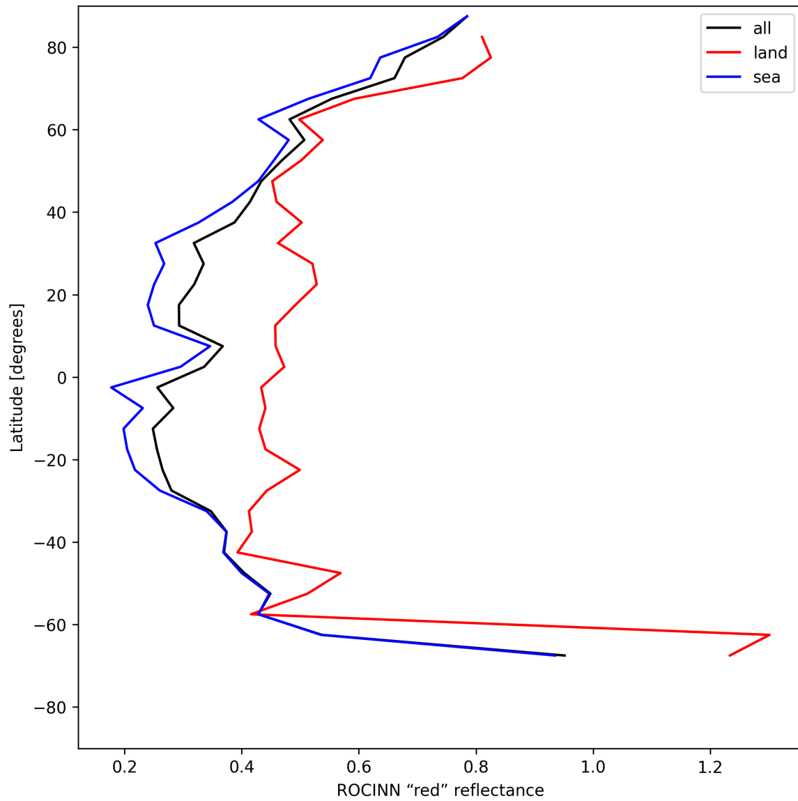
Figure 37: Zonal average of “ROCINN “red” reflectance” for 2025-05-28 to 2025-05-30.
