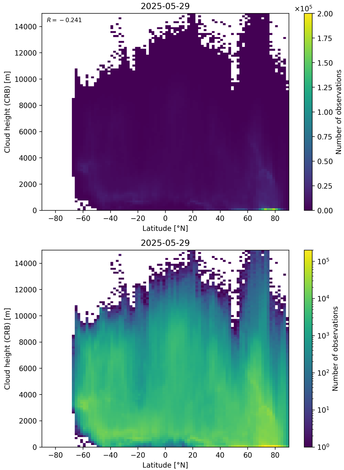
Figure 95: Scatter density plot of “Latitude” against “Cloud height (CRB)” for 2025-05-28 to 2025-05-30.
