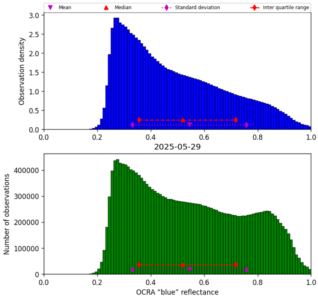
Figure 51: Histogram of “OCRA “blue” reflectance” for 2025-05-28 to 2025-05-30
