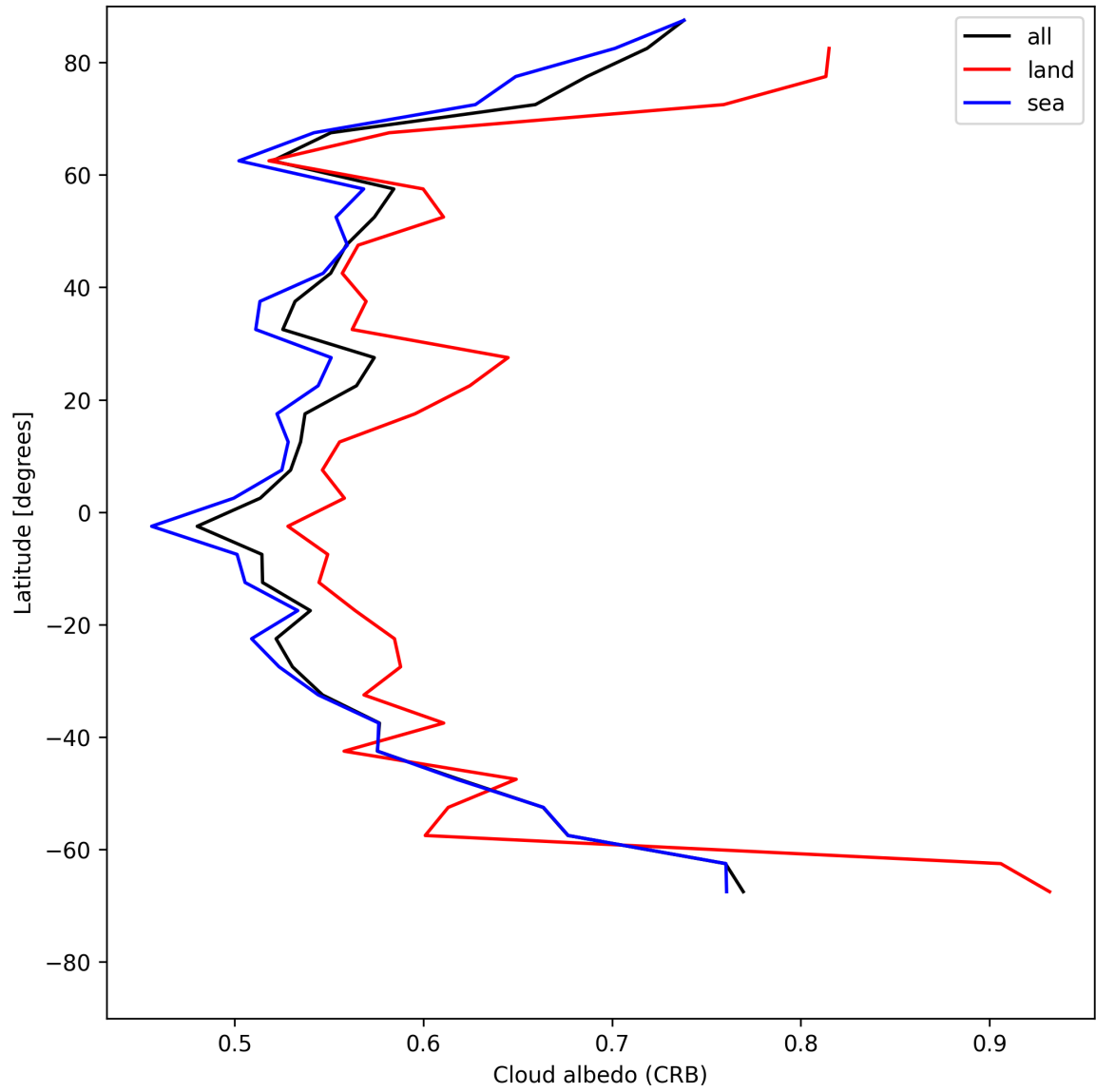
Figure 28: Zonal average of “Cloud albedo (CRB)” for 2025-05-28 to 2025-05-30.
