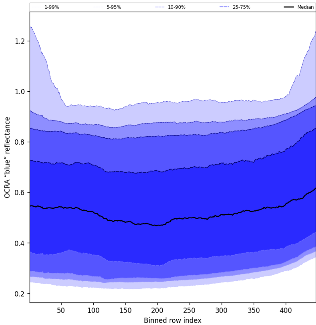
Figure 67: Along track statistics of "OCRA "blue" reflectance" for 2025-05-28 to 2025-05-30
