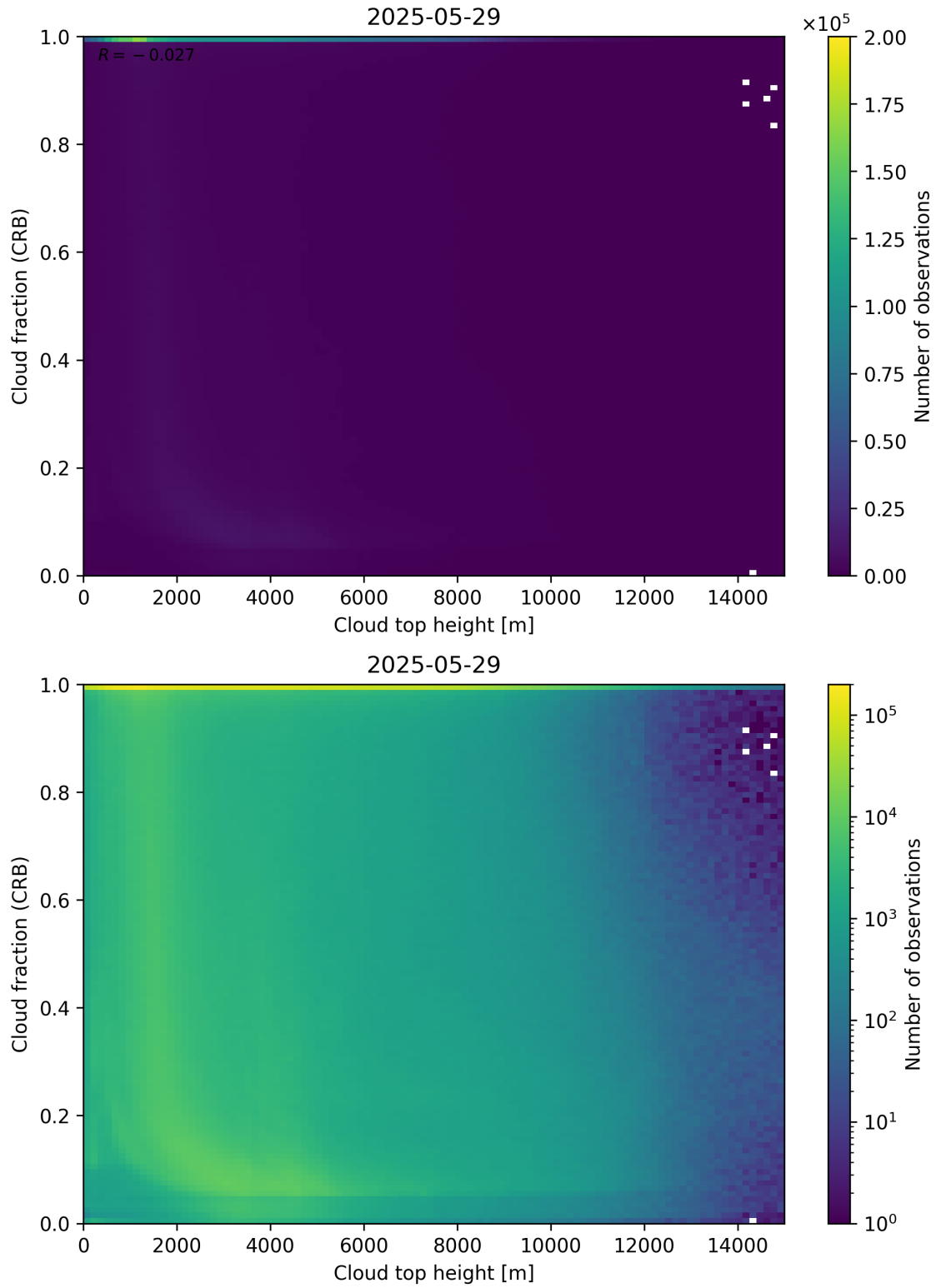
Figure 88: Scatter density plot of “Cloud top height” against “Cloud fraction (CRB)” for 2025-05-28 to 2025-05-30.
