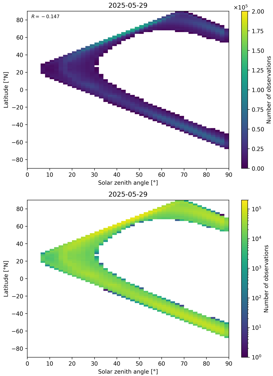
Figure 105: Scatter density plot of “Solar zenith angle” against “Latitude” for 2025-05-28 to 2025-05-30.
