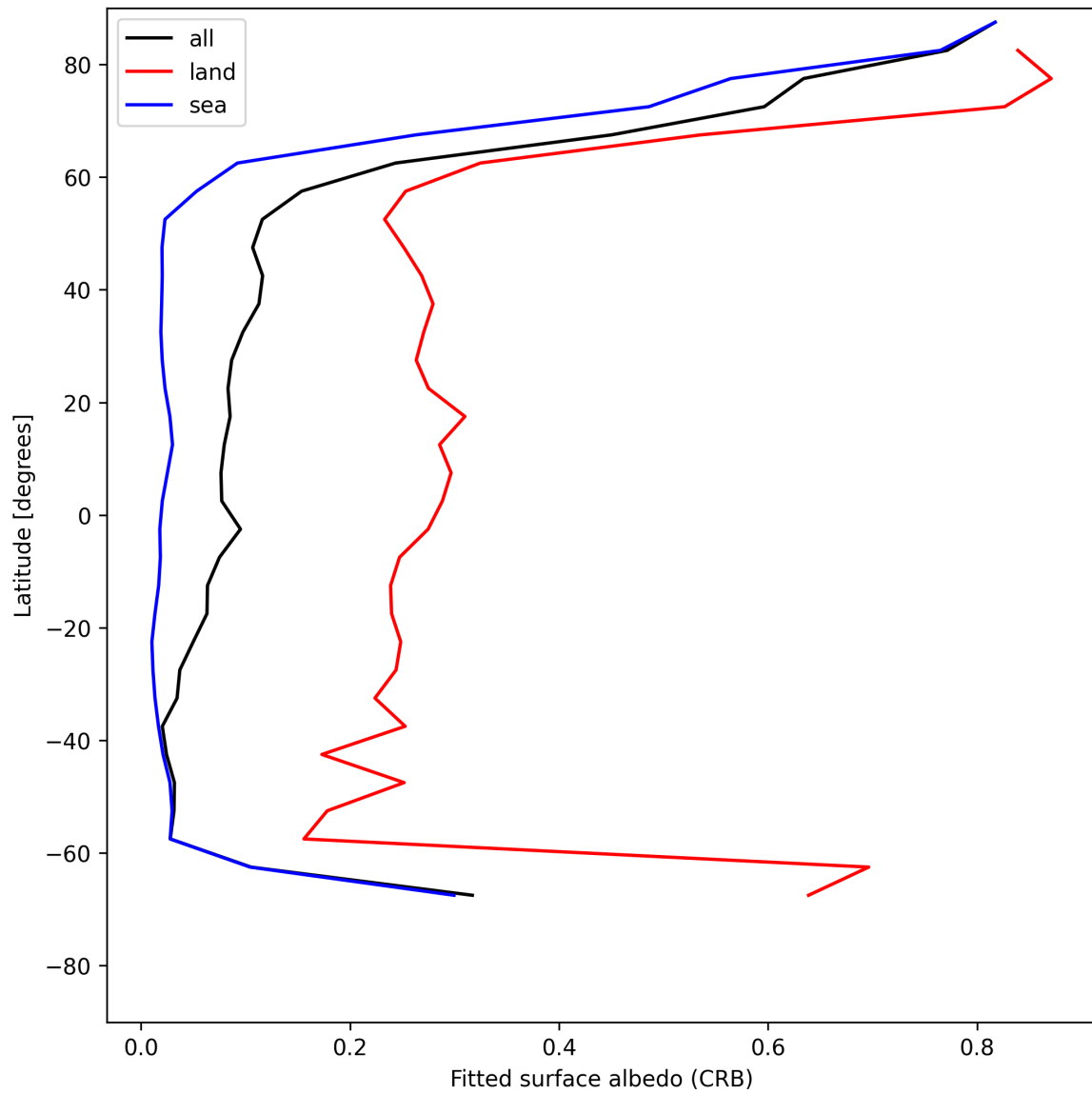
Figure 30: Zonal average of “Fitted surface albedo (CRB)” for 2025-05-28 to 2025-05-30.
