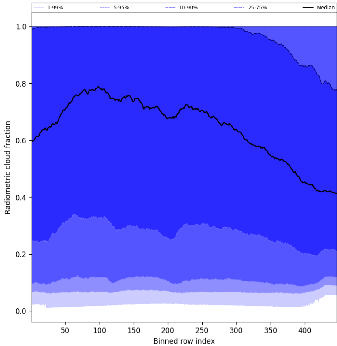
Figure 55: Along track statistics of “Radiometric cloud fraction” for 2025-05-28 to 2025-05-30
