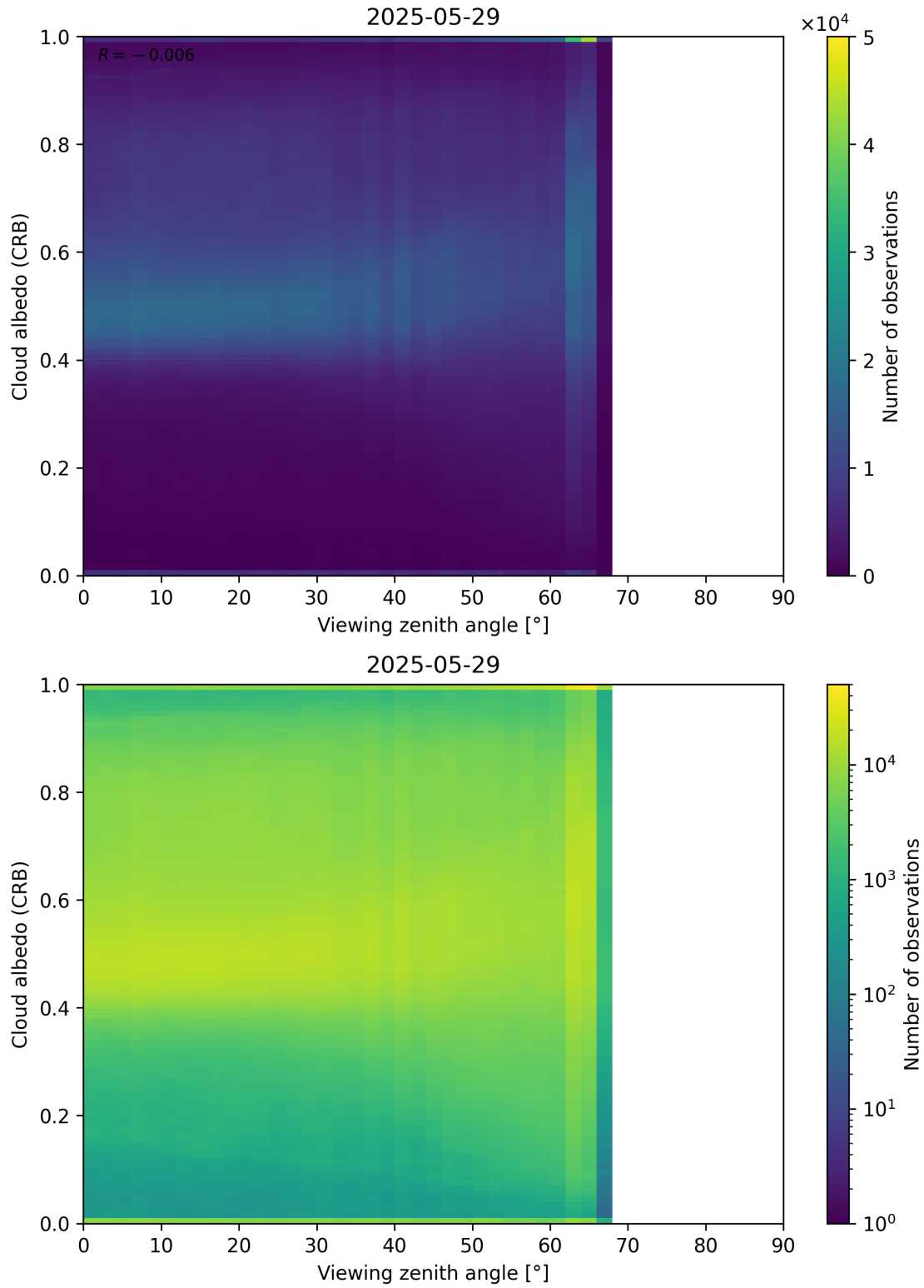
Figure 106: Scatter density plot of “Viewing zenith angle” against “Cloud albedo (CRB)” for 2025-05-28 to 2025-05-30.
