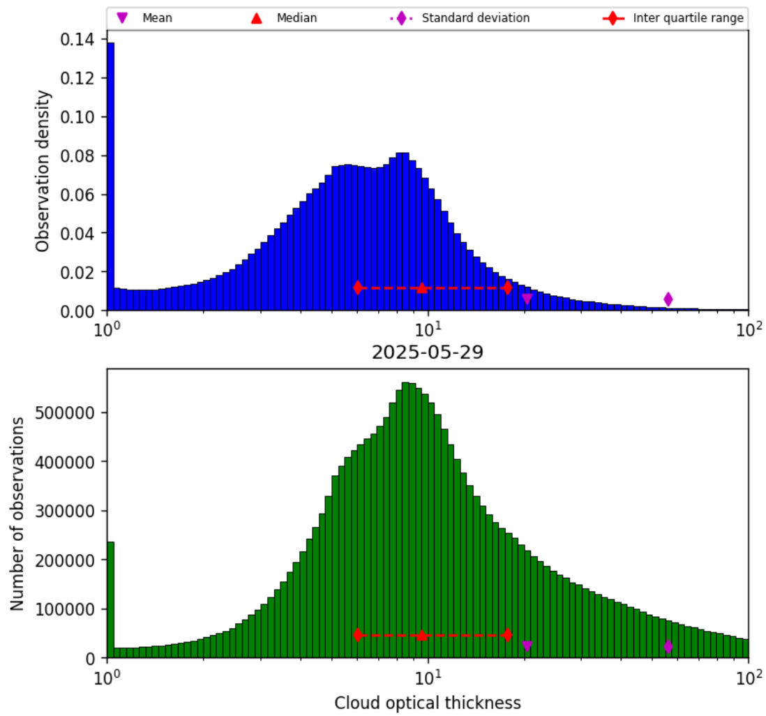
Figure 41: Histogram of “Cloud optical thickness” for 2025-05-28 to 2025-05-30
