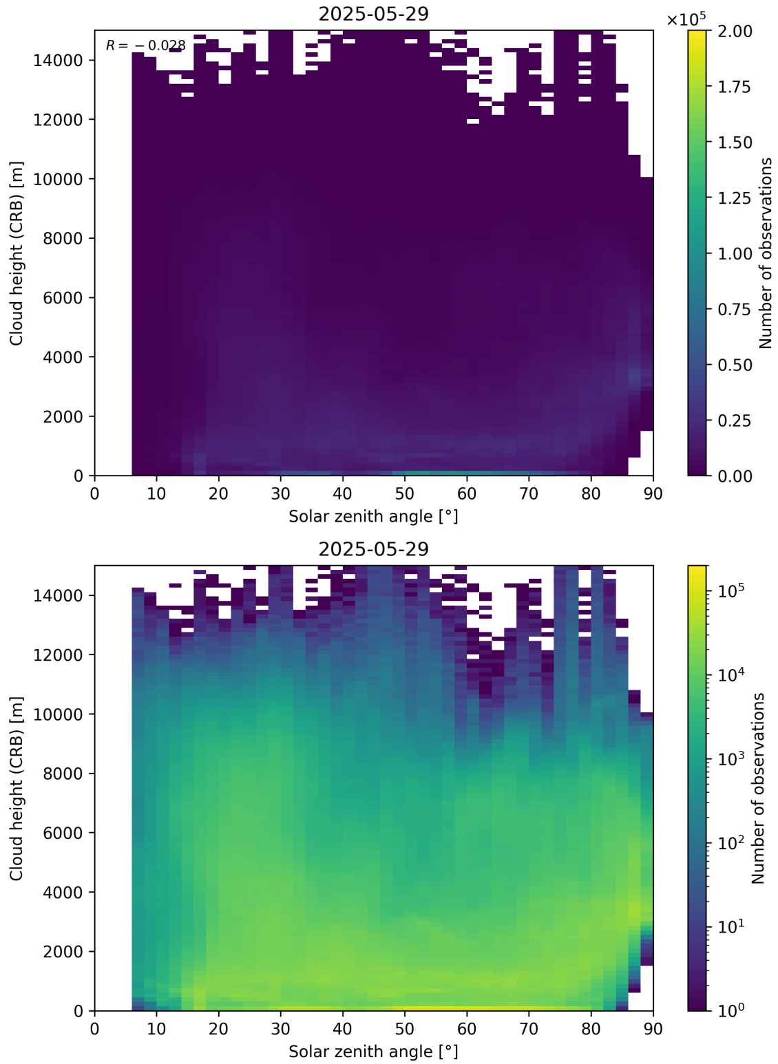
Figure 102: Scatter density plot of “Solar zenith angle” against “Cloud height (CRB)” for 2025-05-28 to 2025-05-30.
