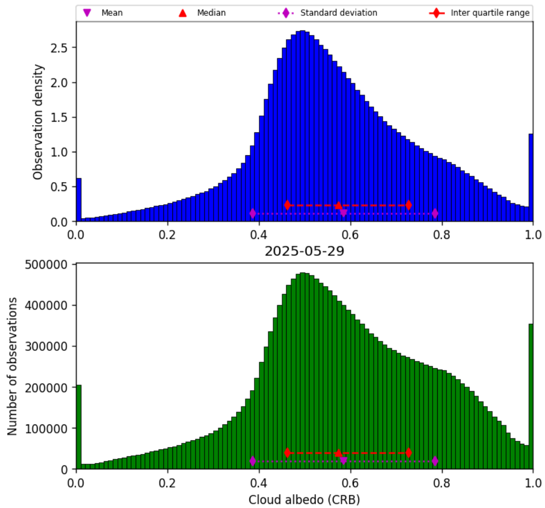
Figure 44: Histogram of “Cloud albedo (CRB)” for 2025-05-28 to 2025-05-30
