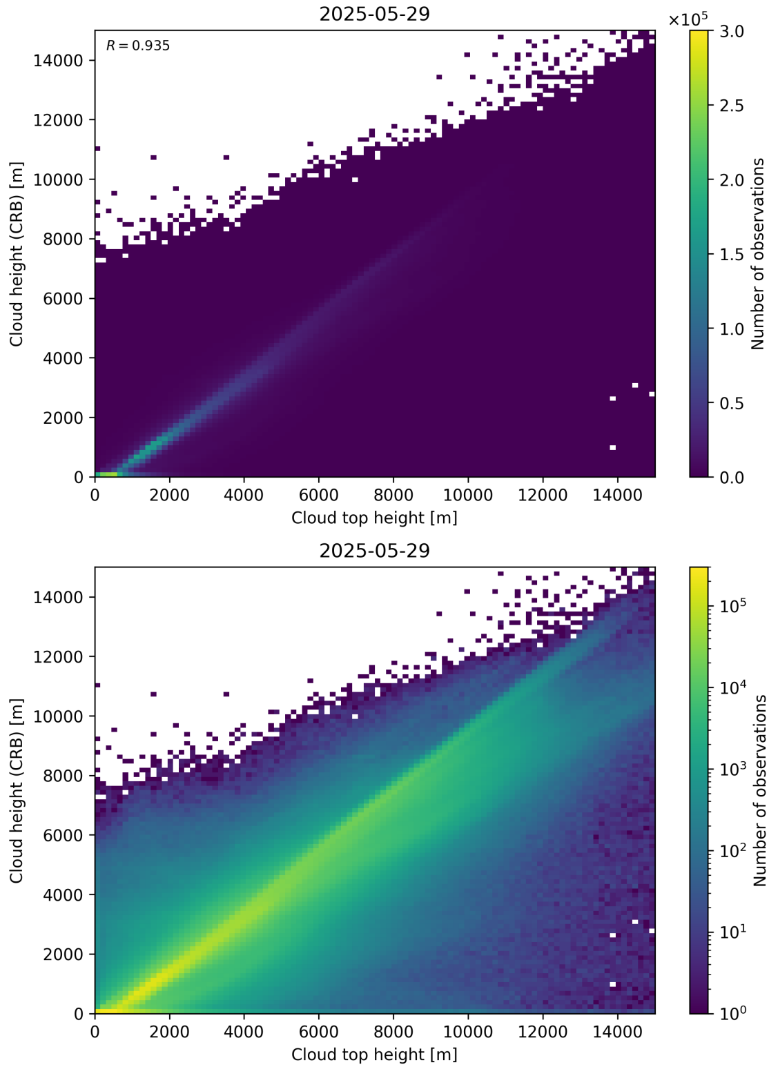
Figure 89: Scatter density plot of “Cloud top height” against “Cloud height (CRB)” for 2025-05-28 to 2025-05-30.
