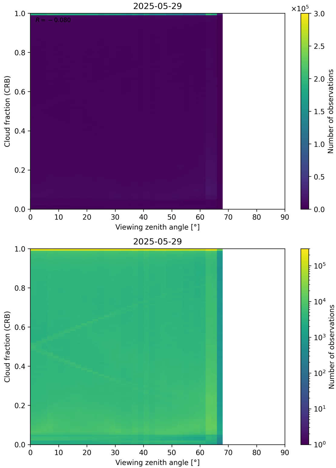
Figure 109: Scatter density plot of “Viewing zenith angle” against “Cloud fraction (CRB)” for 2025-05-28 to 2025-05-30.
