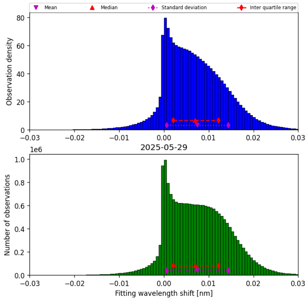
Figure 49: Histogram of “Fitting wavelength shift” for 2025-05-28 to 2025-05-30
