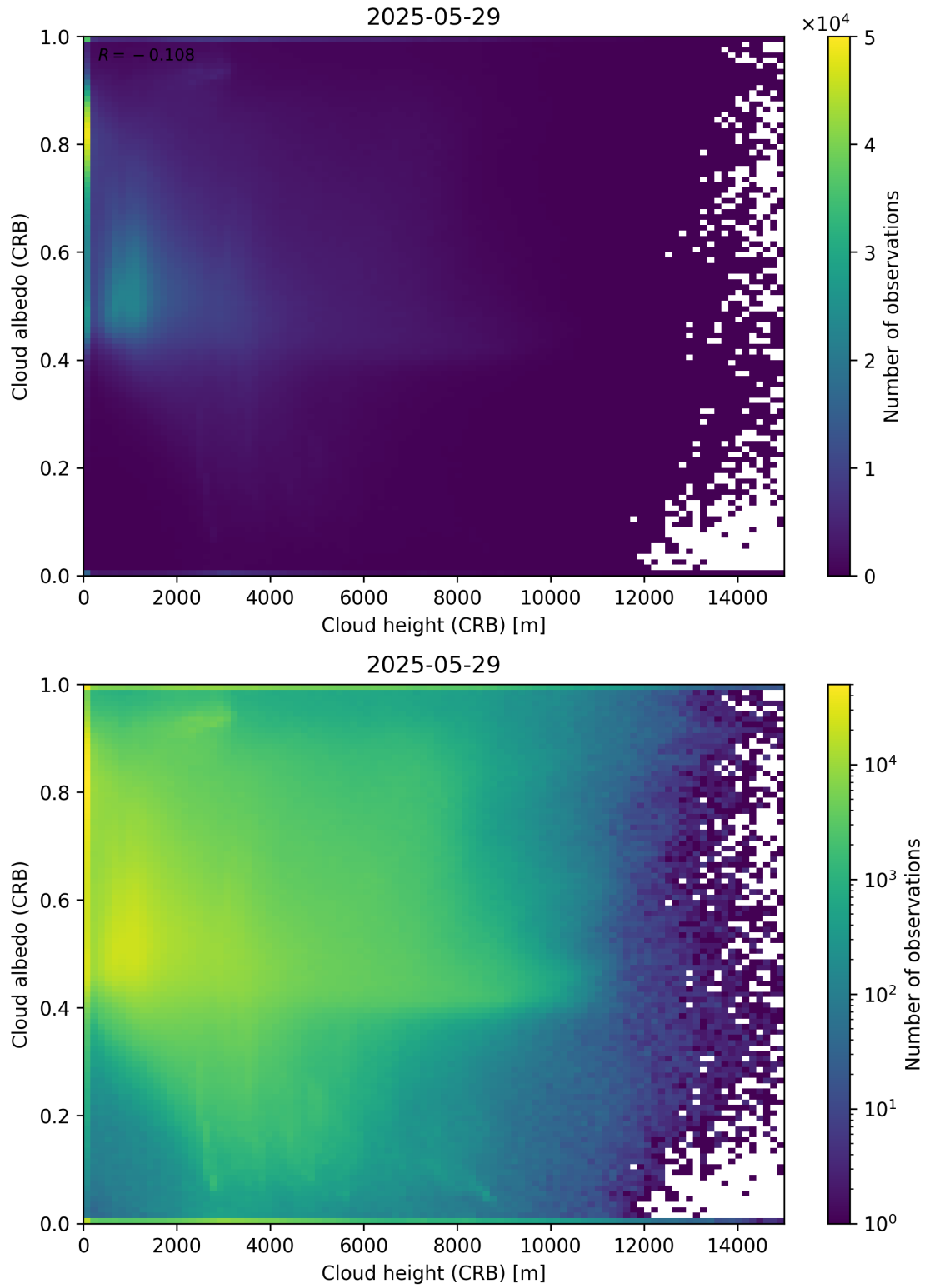
Figure 80: Scatter density plot of “Cloud height (CRB)” against “Cloud albedo (CRB)” for 2025-05-28 to 2025-05-30.
