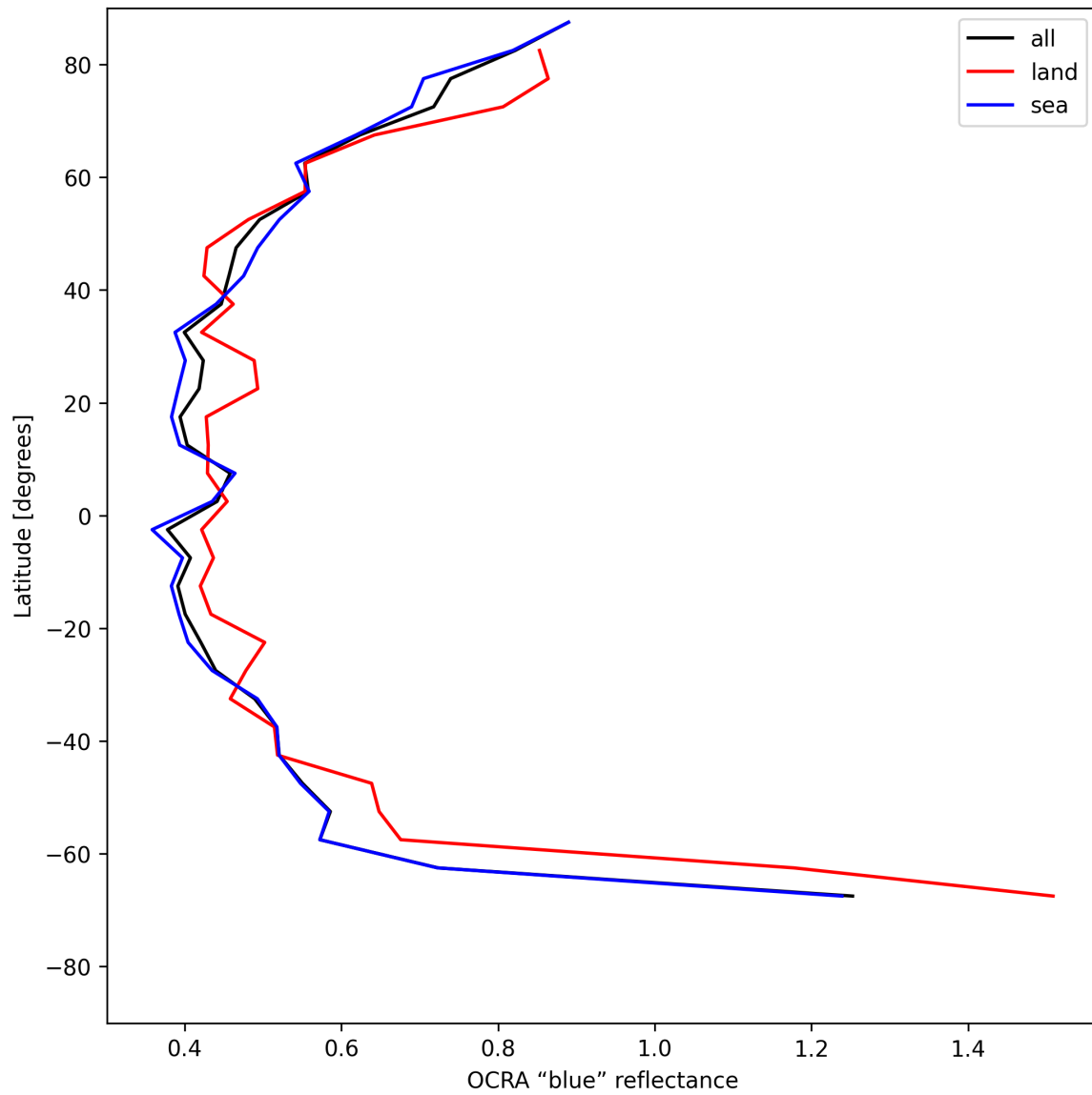
Figure 35: Zonal average of "OCRA "blue" reflectance" for 2025-05-28 to 2025-05-30.
