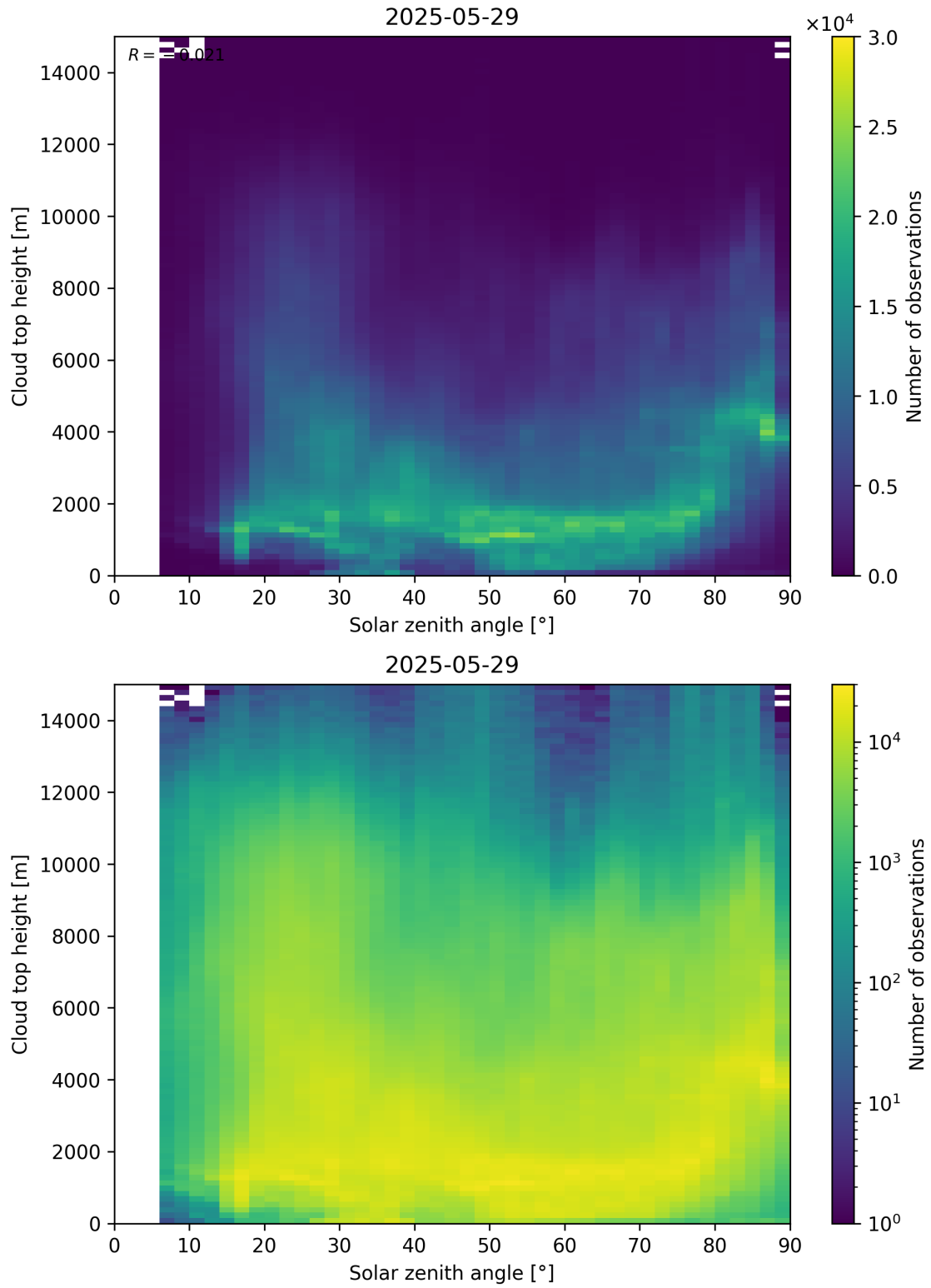
Figure 104: Scatter density plot of “Solar zenith angle” against “Cloud top height” for 2025-05-28 to 2025-05-30.
