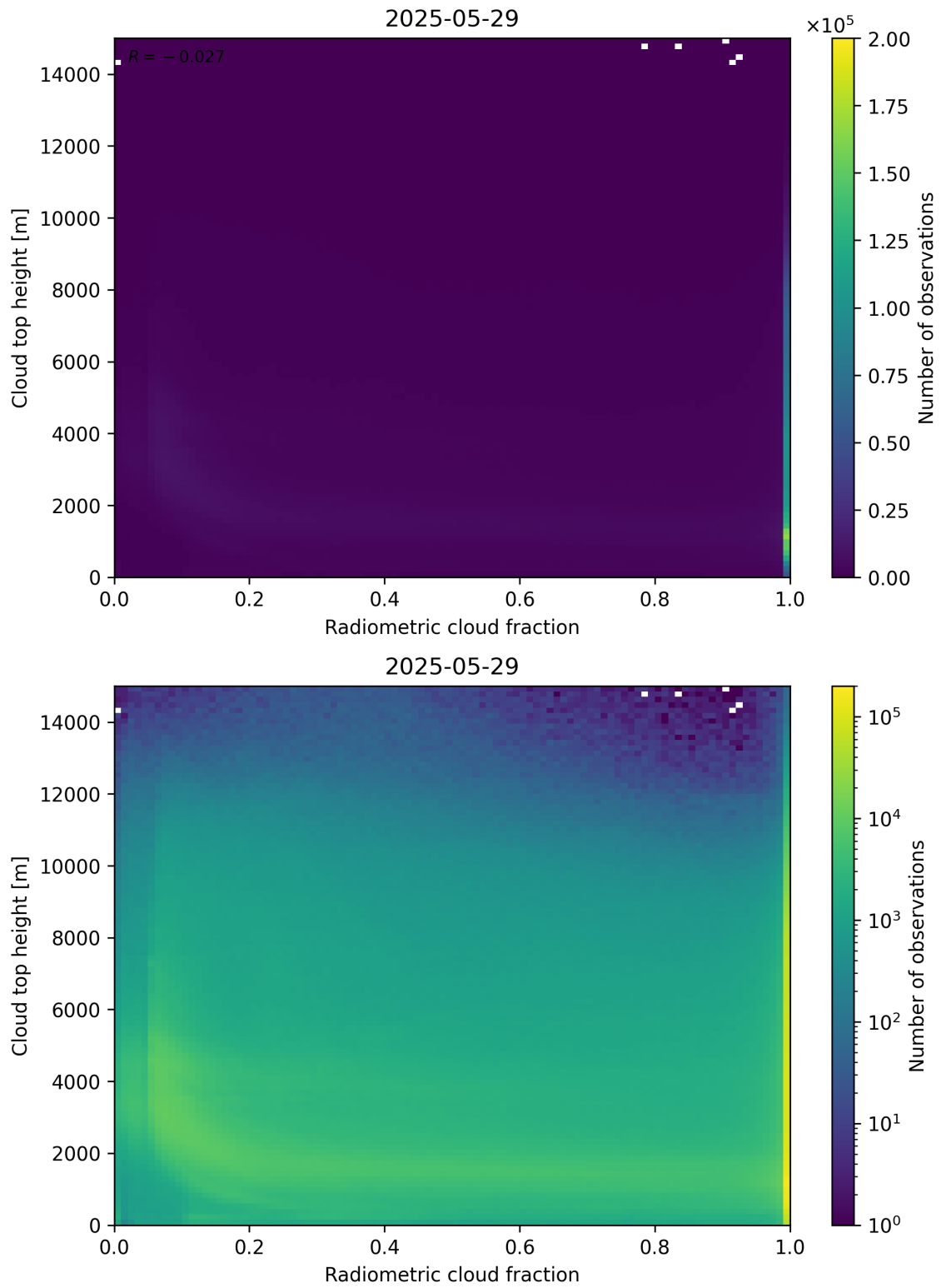
Figure 76: Scatter density plot of “Radiometric cloud fraction” against “Cloud top height” for 2025-05-28 to 2025-05-30.
