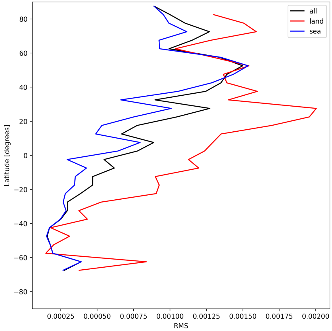
Figure 31: Zonal average of “RMS” for 2025-05-28 to 2025-05-30.
