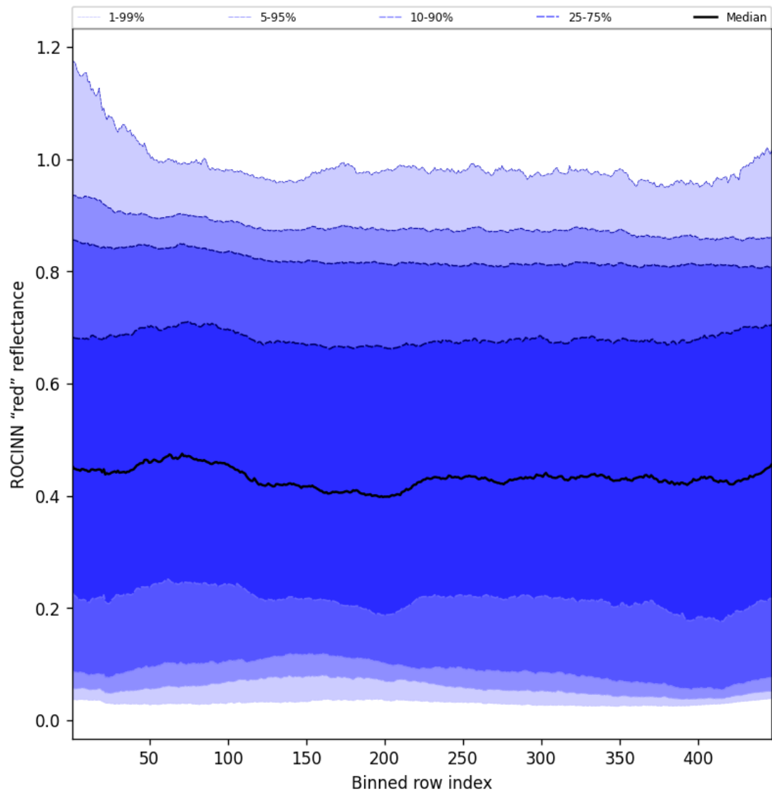
Figure 69: Along track statistics of "ROCINN "red" reflectance" for 2025-05-28 to 2025-05-30
