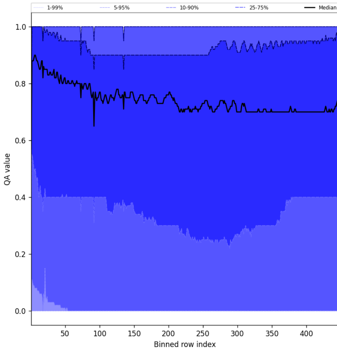
Figure 54: Along track statistics of “QA value” for 2025-05-28 to 2025-05-30
