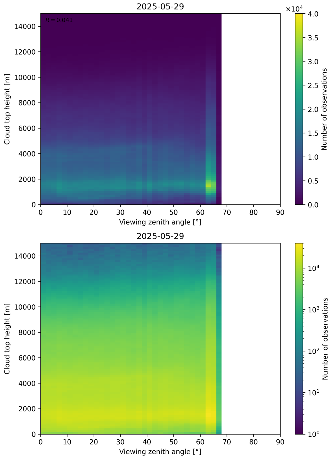
Figure 112: Scatter density plot of “Viewing zenith angle” against “Cloud top height” for 2025-05-28 to 2025-05-30.
