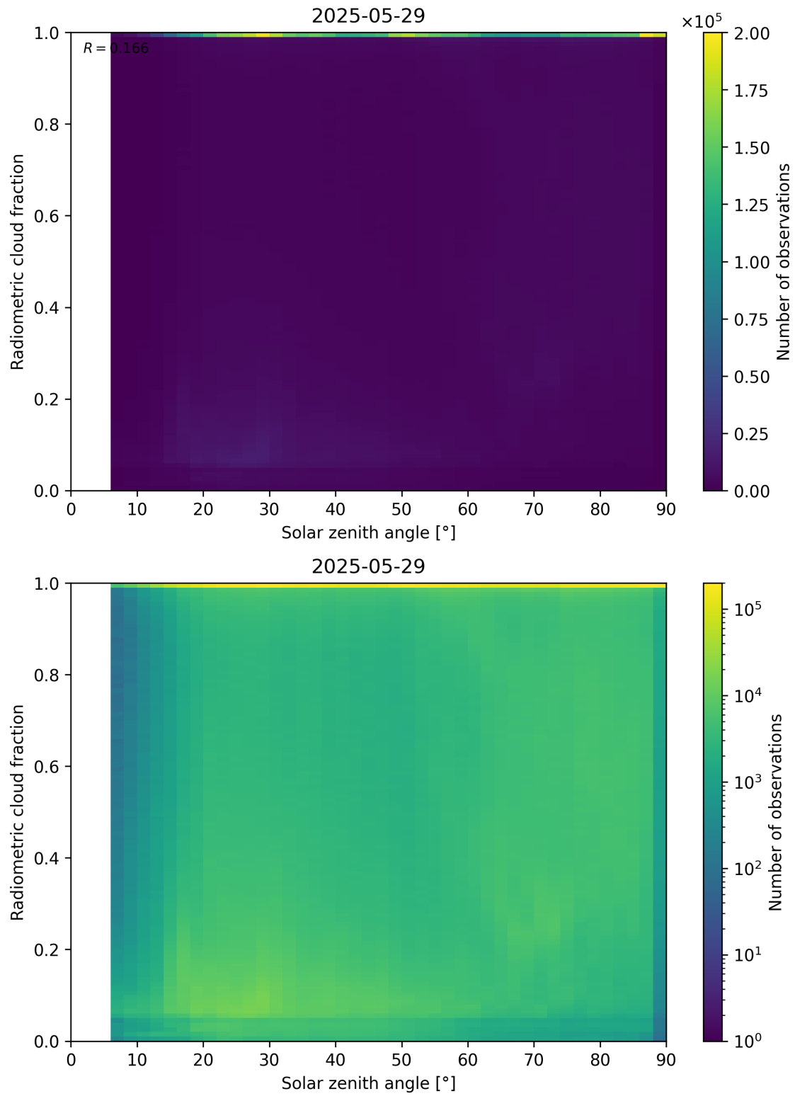
Figure 99: Scatter density plot of “Solar zenith angle” against “Radiometric cloud fraction” for 2025-05-28 to 2025-05-30.
