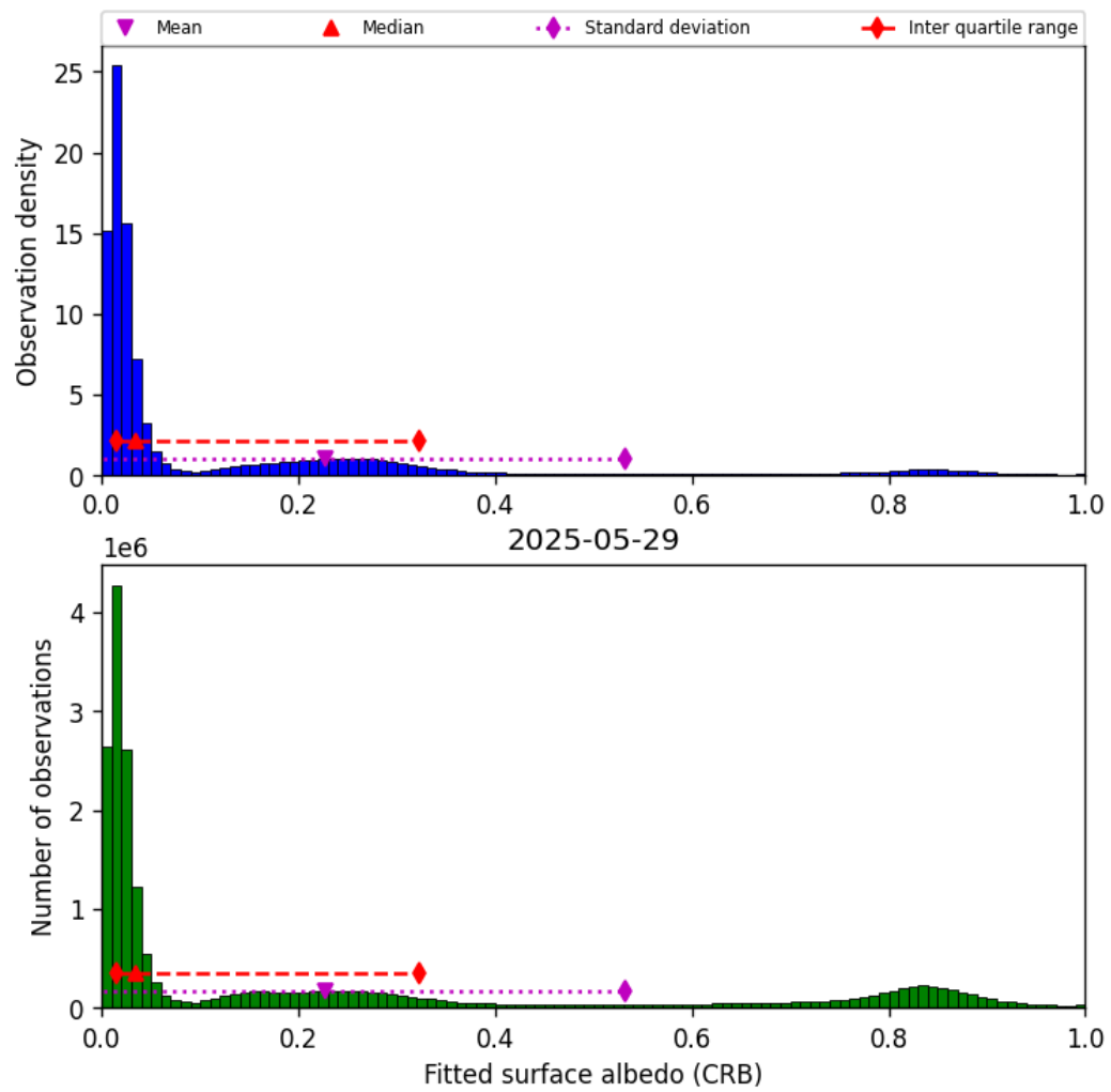
Figure 46: Histogram of “Fitted surface albedo (CRB)” for 2025-05-28 to 2025-05-30
