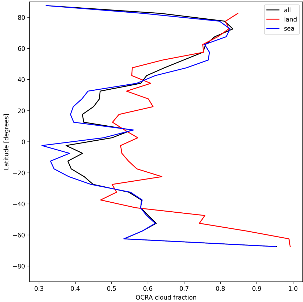
Figure 34: Zonal average of “OCRA cloud fraction” for 2025-05-28 to 2025-05-30.
