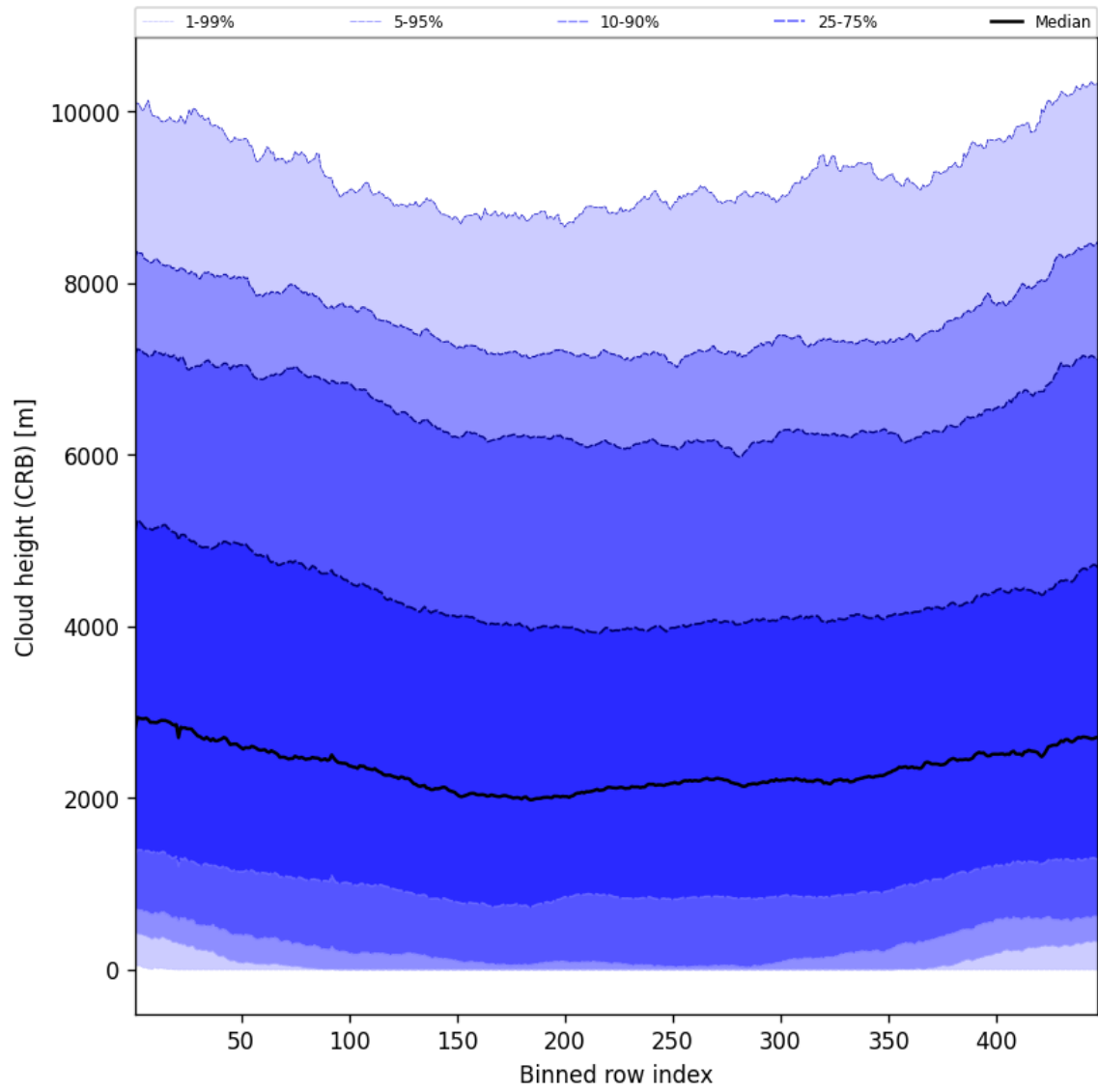
Figure 59: Along track statistics of “Cloud height (CRB)” for 2025-05-28 to 2025-05-30
