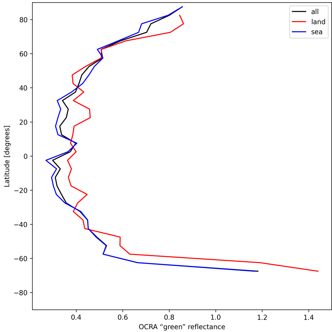
Figure 36: Zonal average of "OCRA "green" reflectance" for 2025-05-28 to 2025-05-30.
