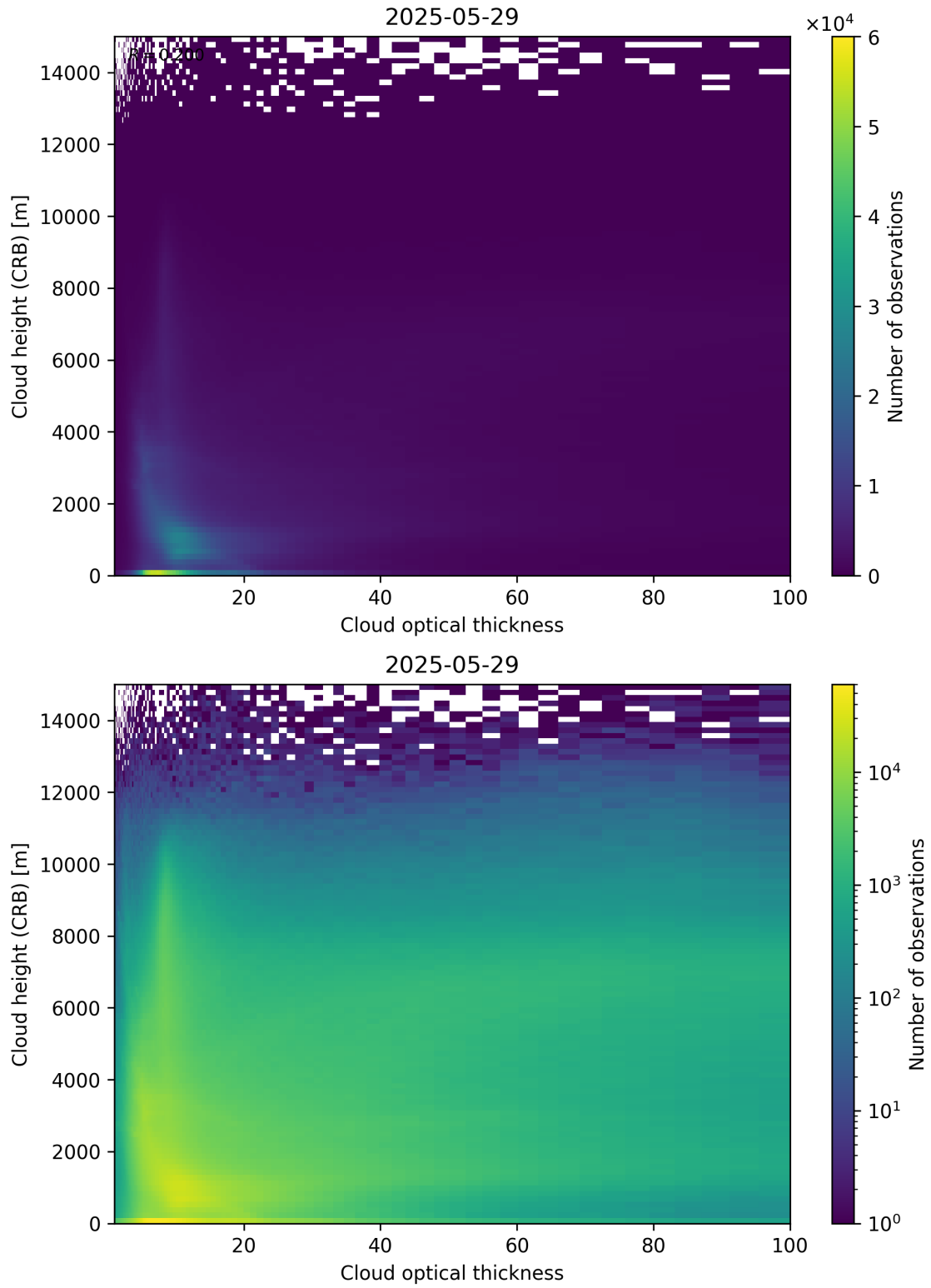
Figure 85: Scatter density plot of “Cloud optical thickness” against “Cloud height (CRB)” for 2025-05-28 to 2025-05-30.
