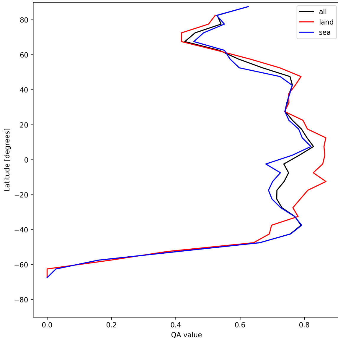
Figure 22: Zonal average of “QA value” for 2025-05-28 to 2025-05-30.
