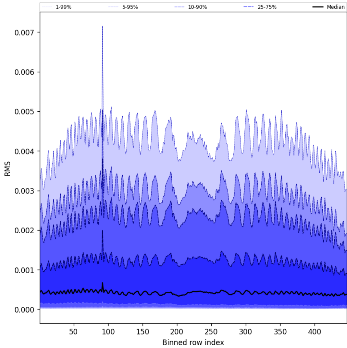
Figure 63: Along track statistics of “RMS” for 2025-05-28 to 2025-05-30
