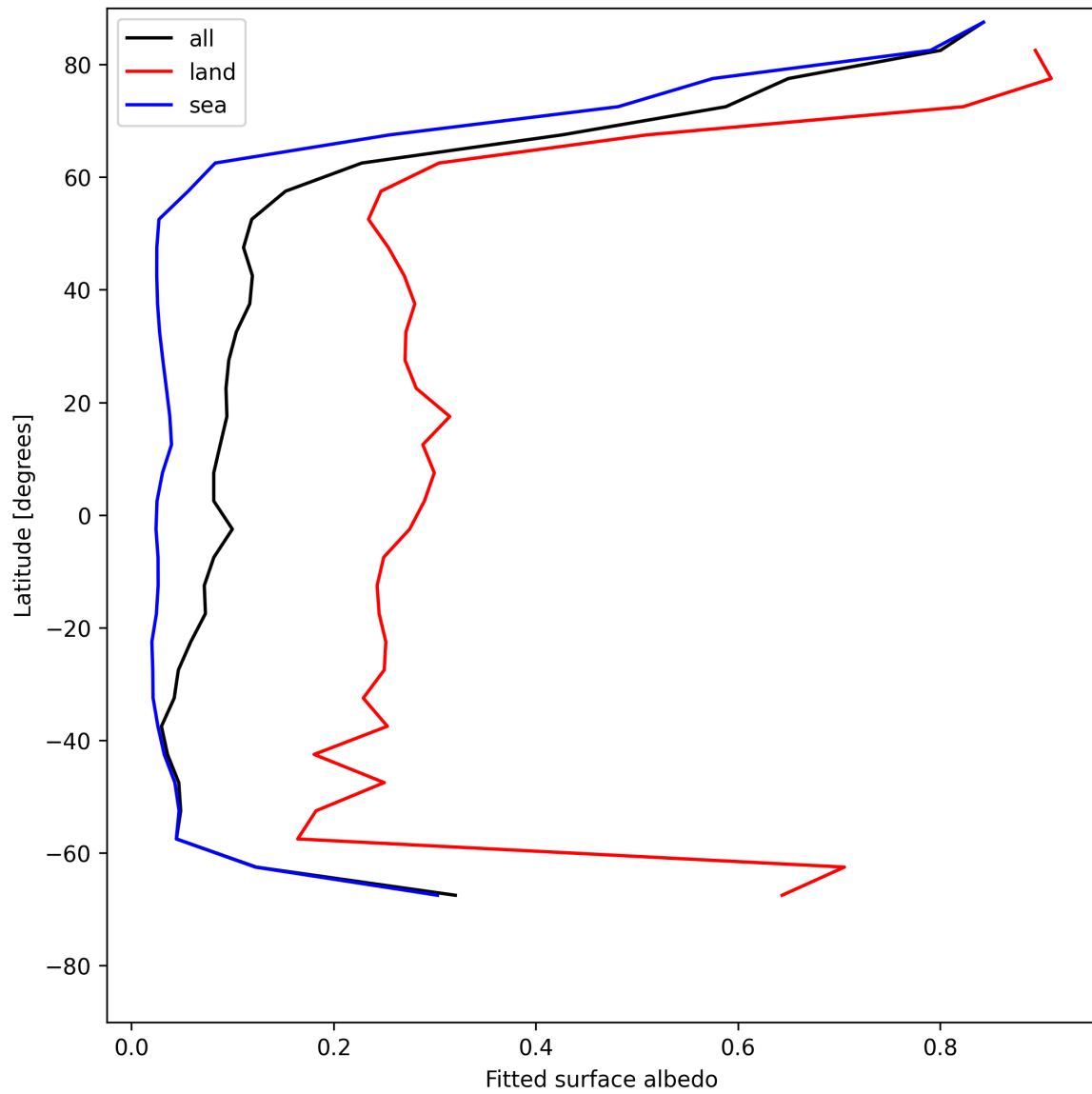
Figure 29: Zonal average of “Fitted surface albedo” for 2025-05-28 to 2025-05-30.
