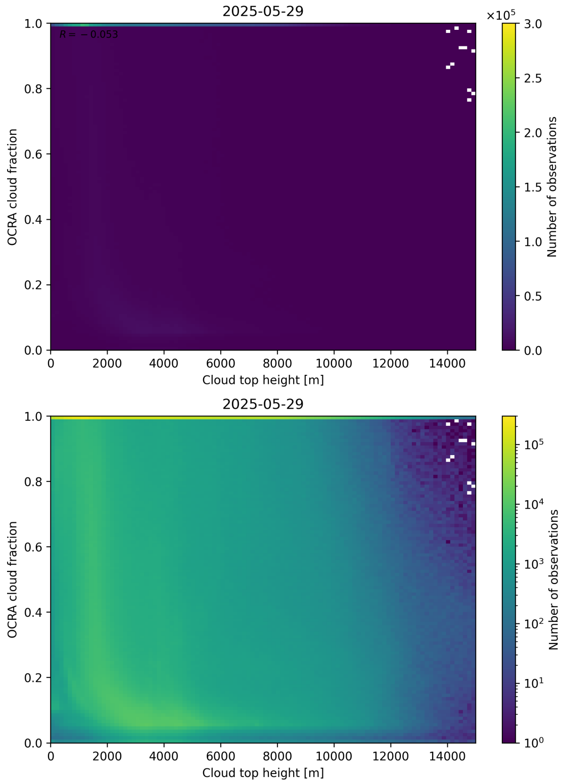
Figure 87: Scatter density plot of “Cloud top height” against “OCRA cloud fraction” for 2025-05-28 to 2025-05-30.
