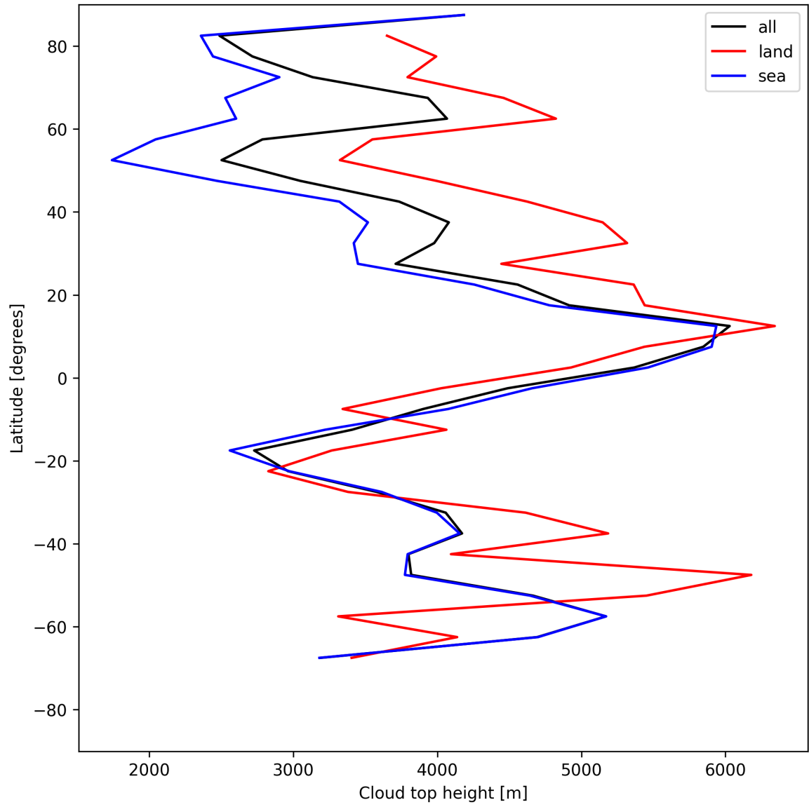
Figure 24: Zonal average of “Cloud top height” for 2025-05-28 to 2025-05-30.
