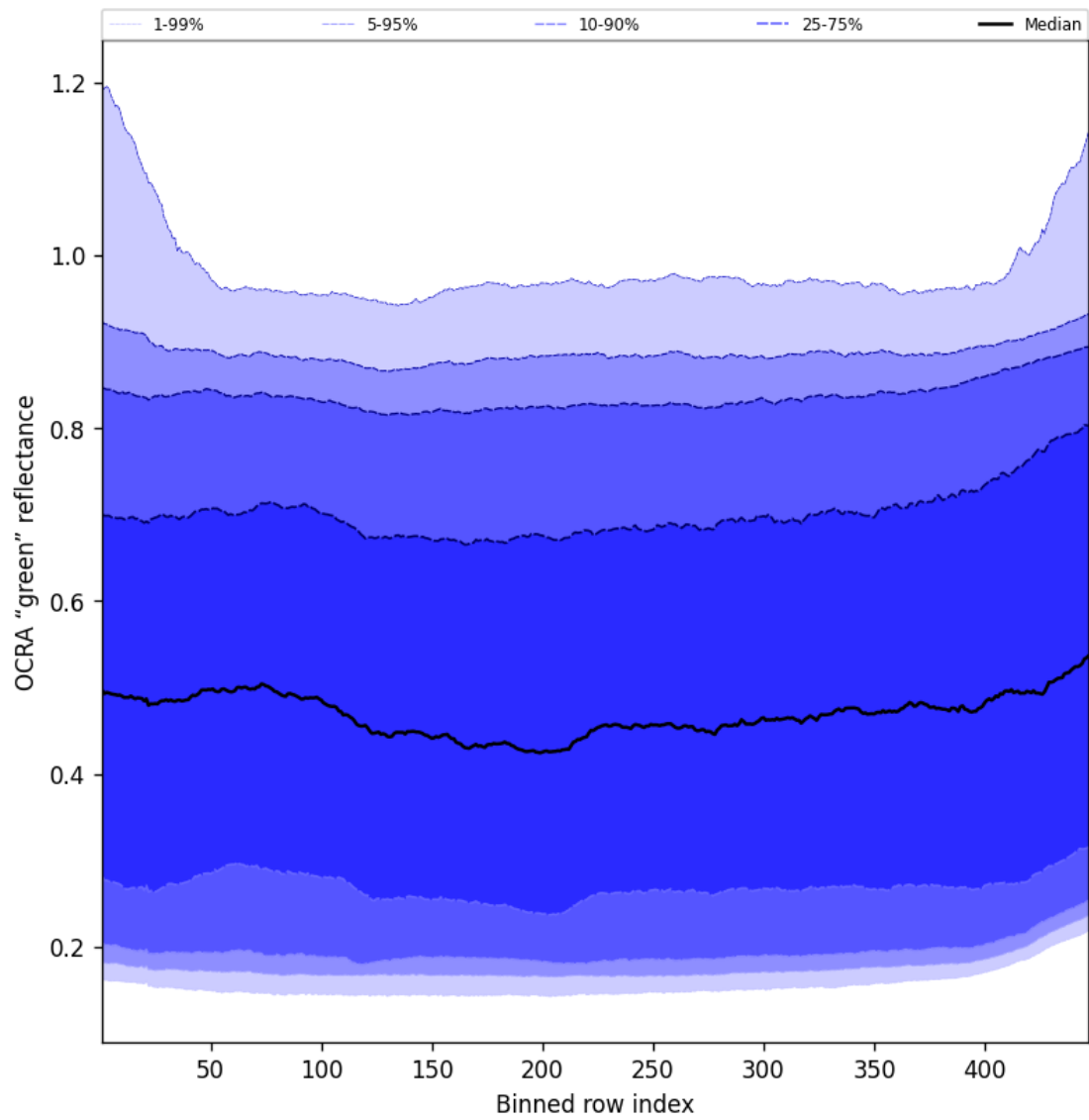
Figure 68: Along track statistics of "OCRA "green" reflectance" for 2025-05-28 to 2025-05-30
