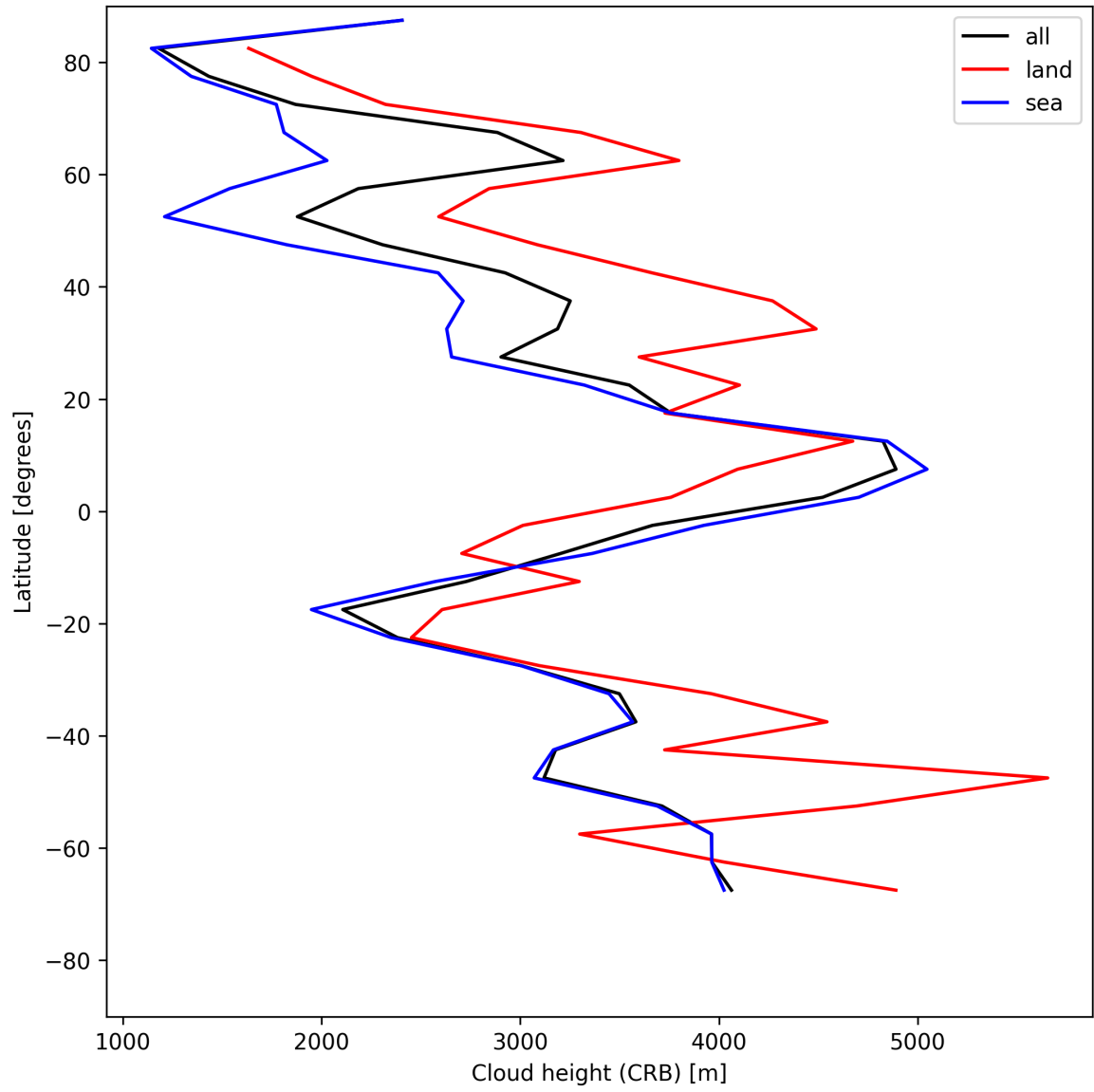
Figure 27: Zonal average of “Cloud height (CRB)” for 2025-05-28 to 2025-05-30.
