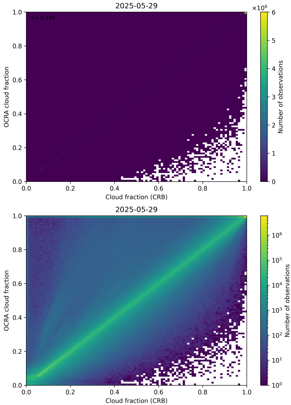
Figure 78: Scatter density plot of “Cloud fraction (CRB)” against “OCRA cloud fraction” for 2025-05-28 to 2025-05-30.
