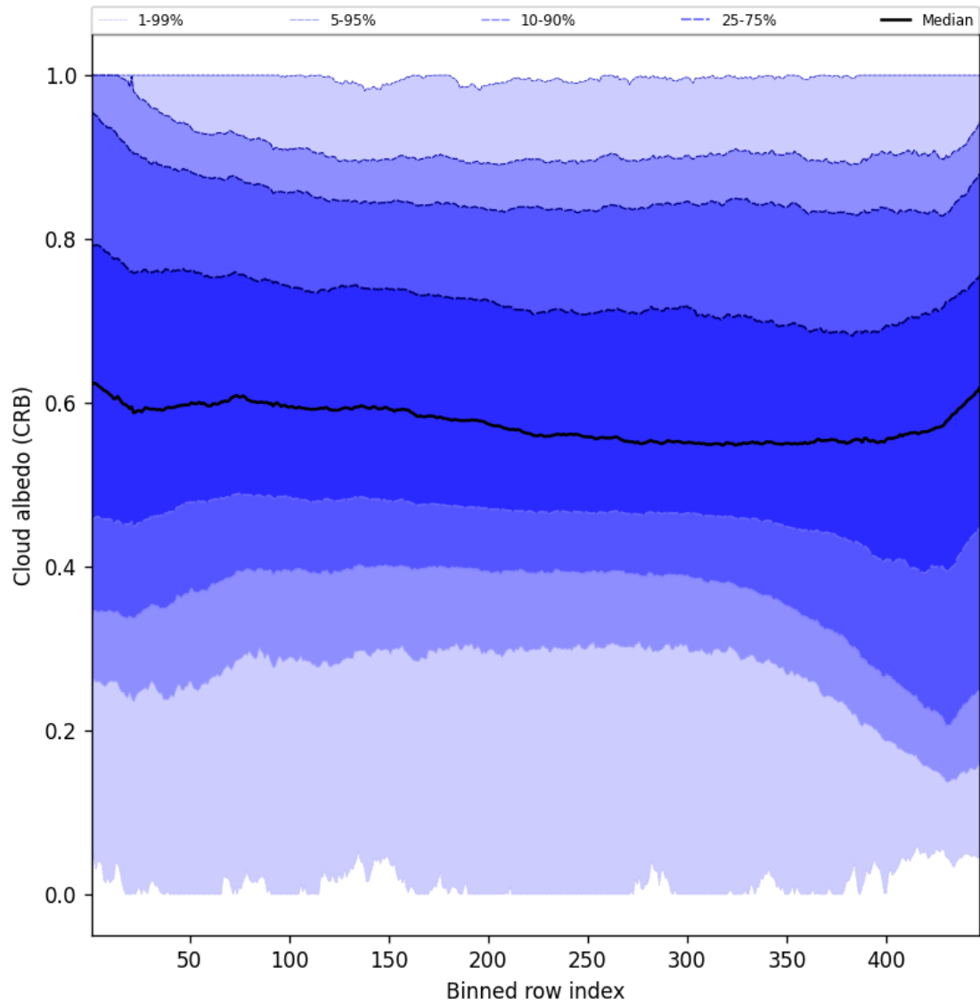
Figure 60: Along track statistics of “Cloud albedo (CRB)” for 2025-05-28 to 2025-05-30
