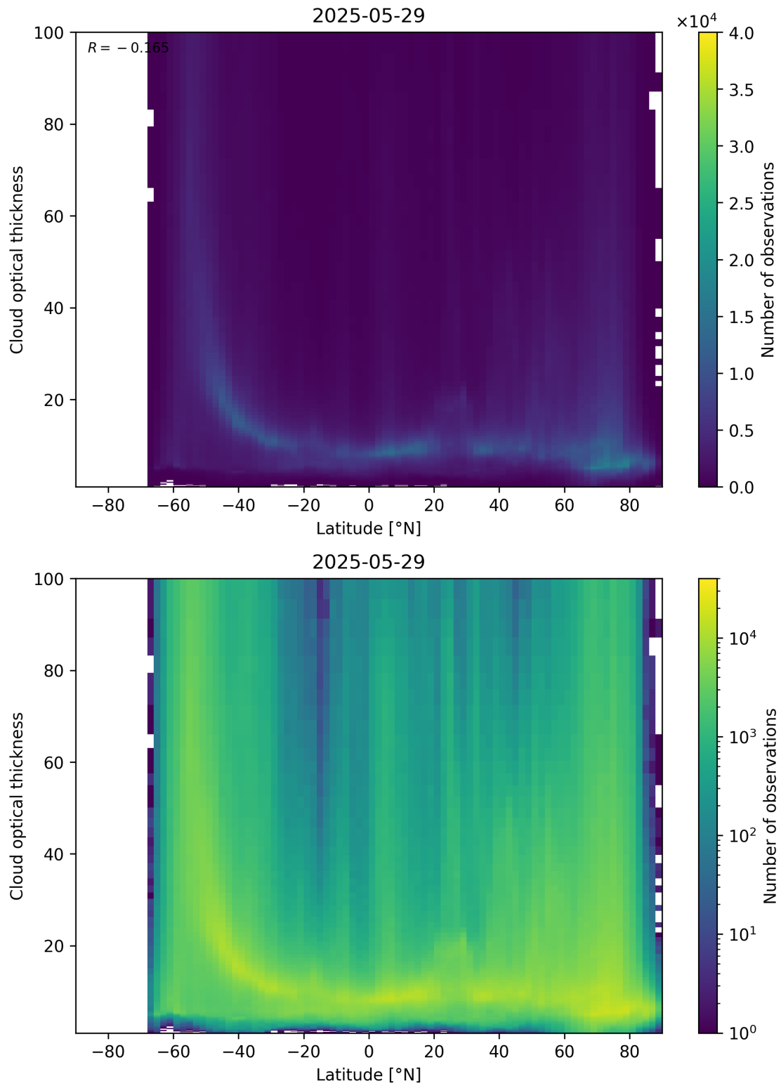
Figure 96: Scatter density plot of “Latitude” against “Cloud optical thickness” for 2025-05-28 to 2025-05-30.
