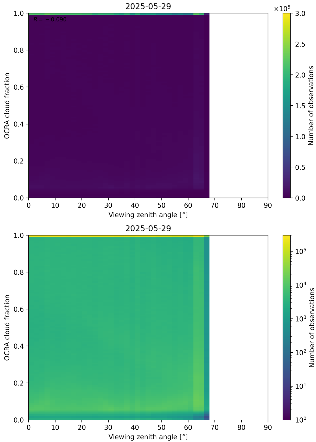
Figure 108: Scatter density plot of “Viewing zenith angle” against “OCRA cloud fraction” for 2025-05-28 to 2025-05-30.
