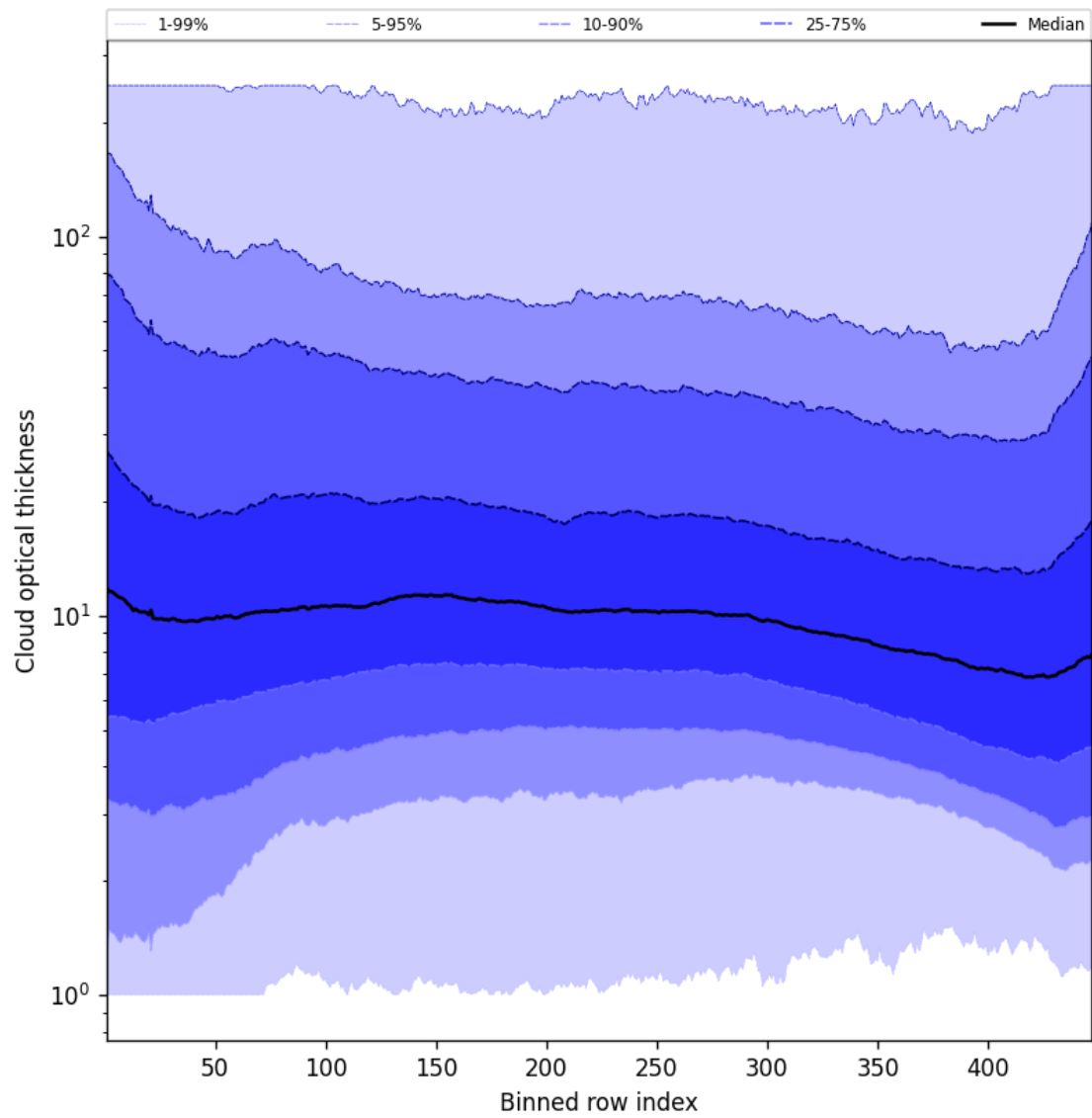
Figure 57: Along track statistics of “Cloud optical thickness” for 2025-05-28 to 2025-05-30
