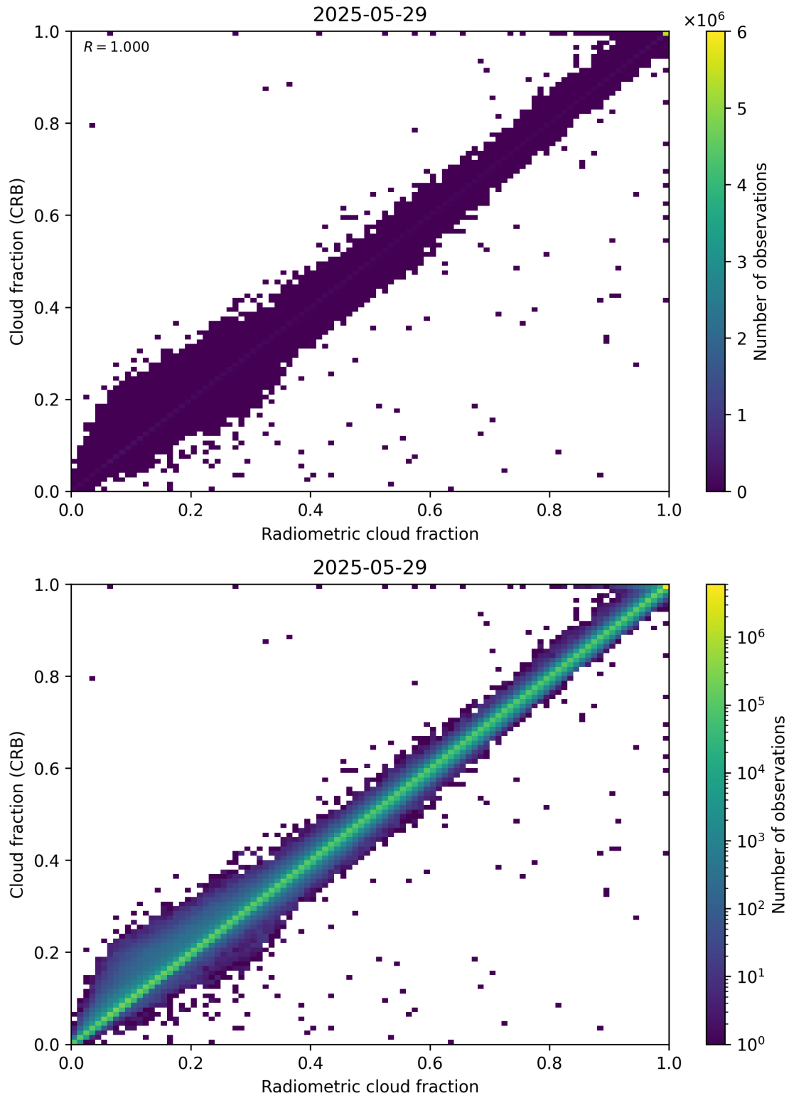
Figure 73: Scatter density plot of “Radiometric cloud fraction” against “Cloud fraction (CRB)” for 2025-05-28 to 2025-05-30.
