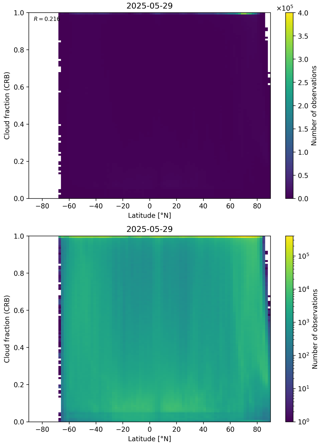
Figure 94: Scatter density plot of “Latitude” against “Cloud fraction (CRB)” for 2025-05-28 to 2025-05-30.
