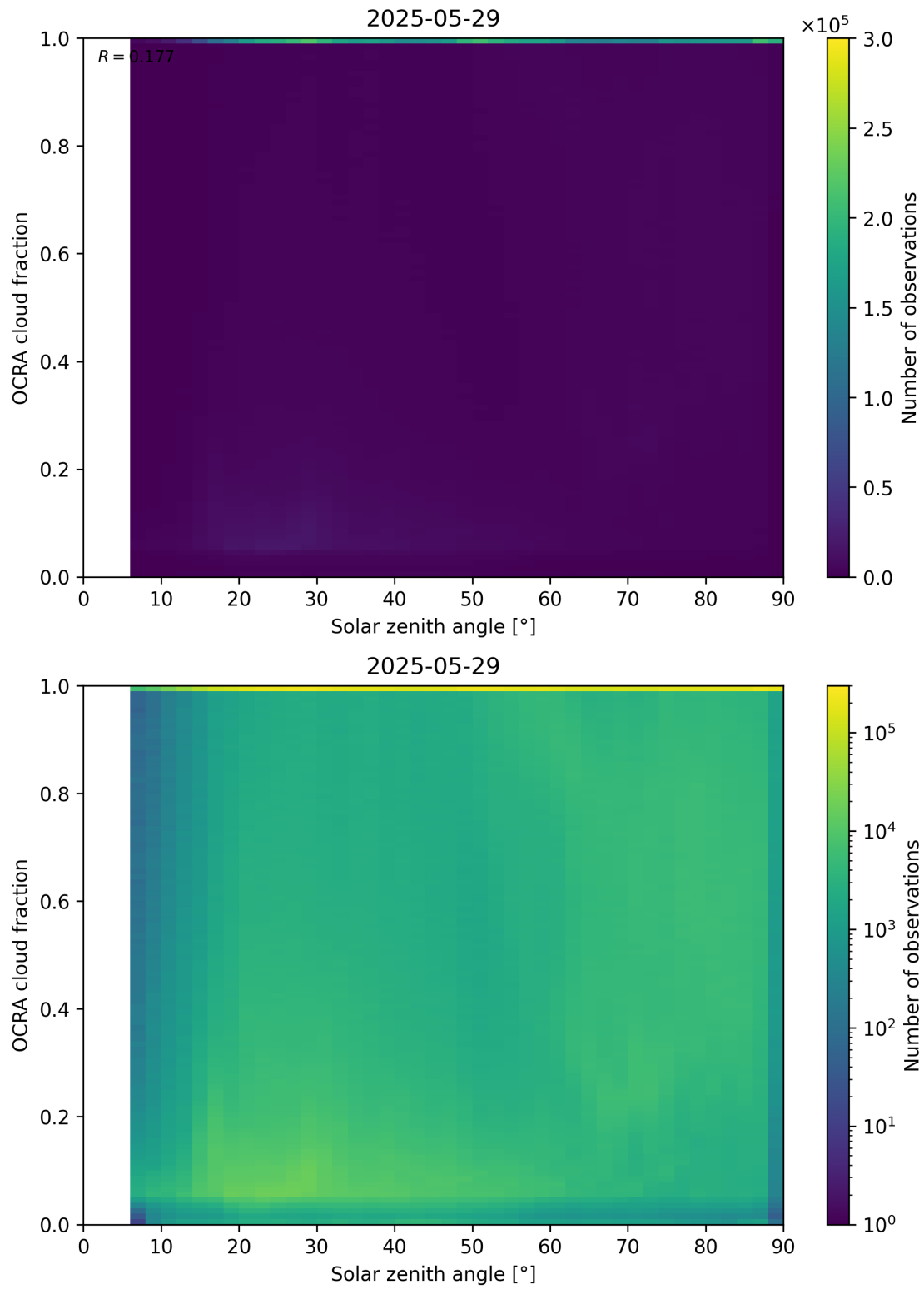
Figure 100: Scatter density plot of “Solar zenith angle” against “OCRA cloud fraction” for 2025-05-28 to 2025-05-30.
