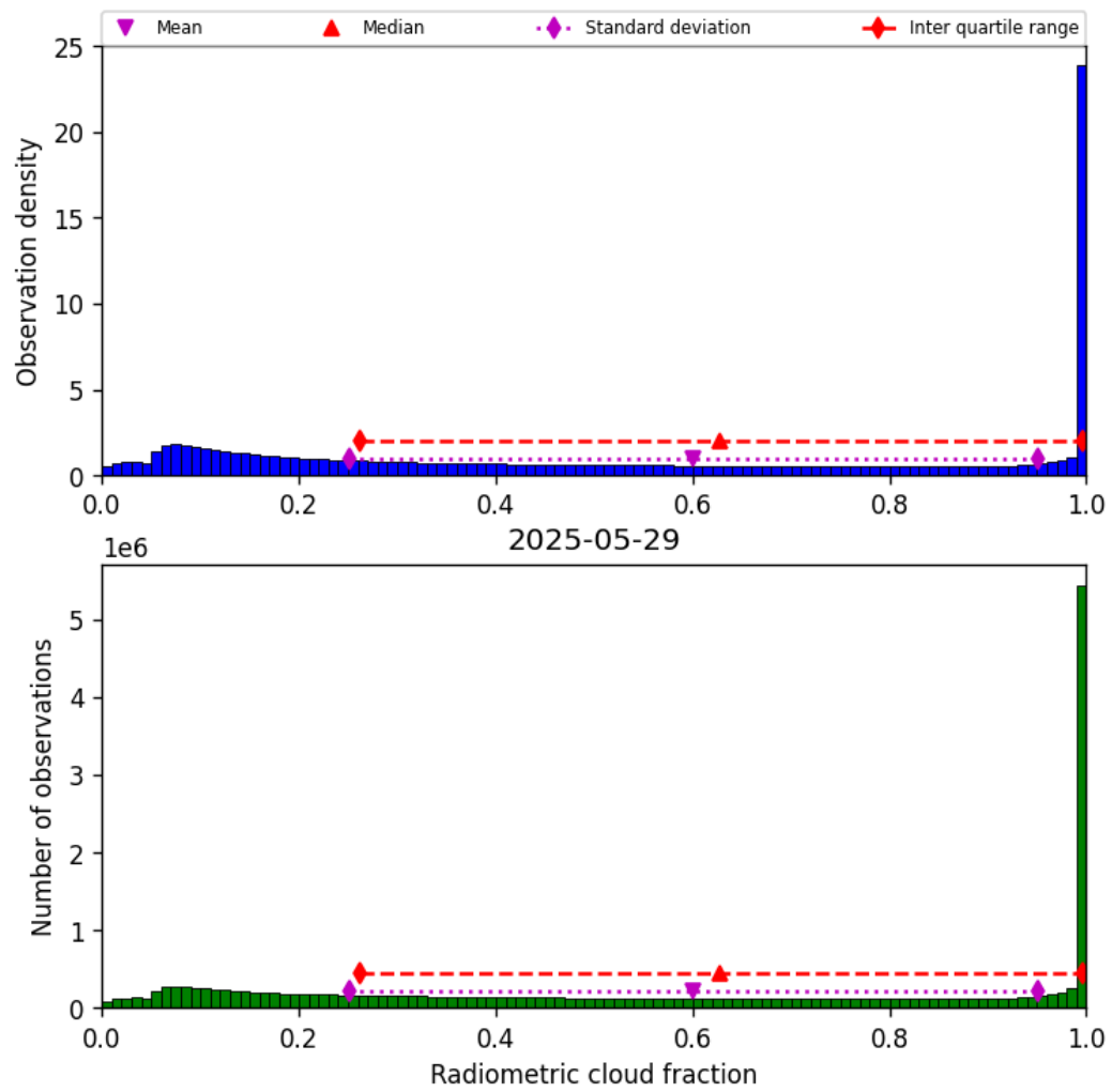
Figure 39: Histogram of “Radiometric cloud fraction” for 2025-05-28 to 2025-05-30
