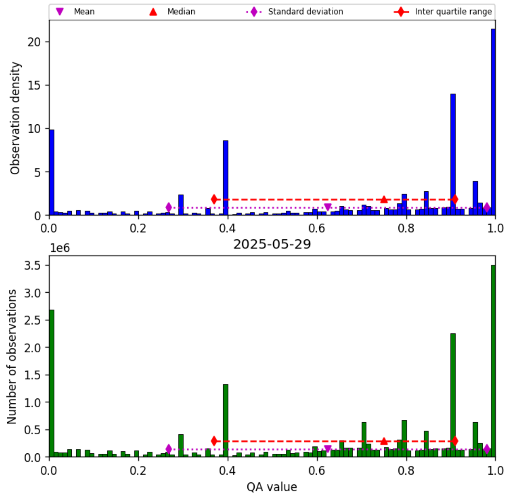
Figure 38: Histogram of “QA value” for 2025-05-28 to 2025-05-30
