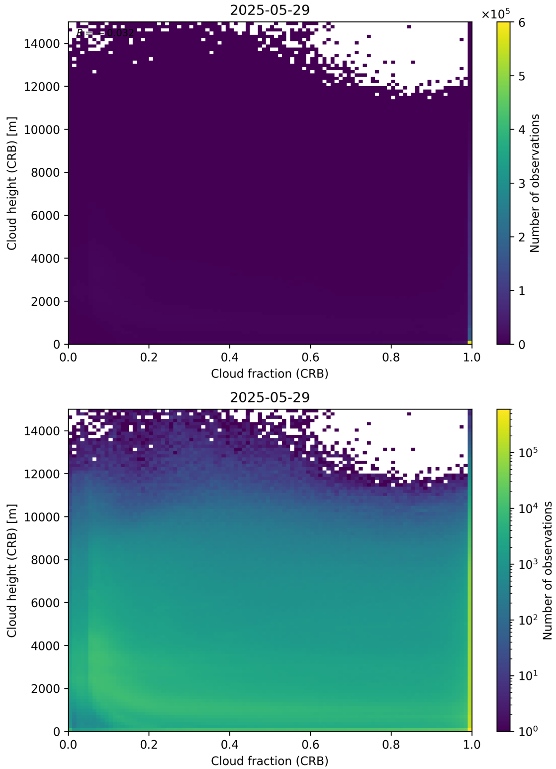
Figure 79: Scatter density plot of “Cloud fraction (CRB)” against “Cloud height (CRB)” for 2025-05-28 to 2025-05-30.
