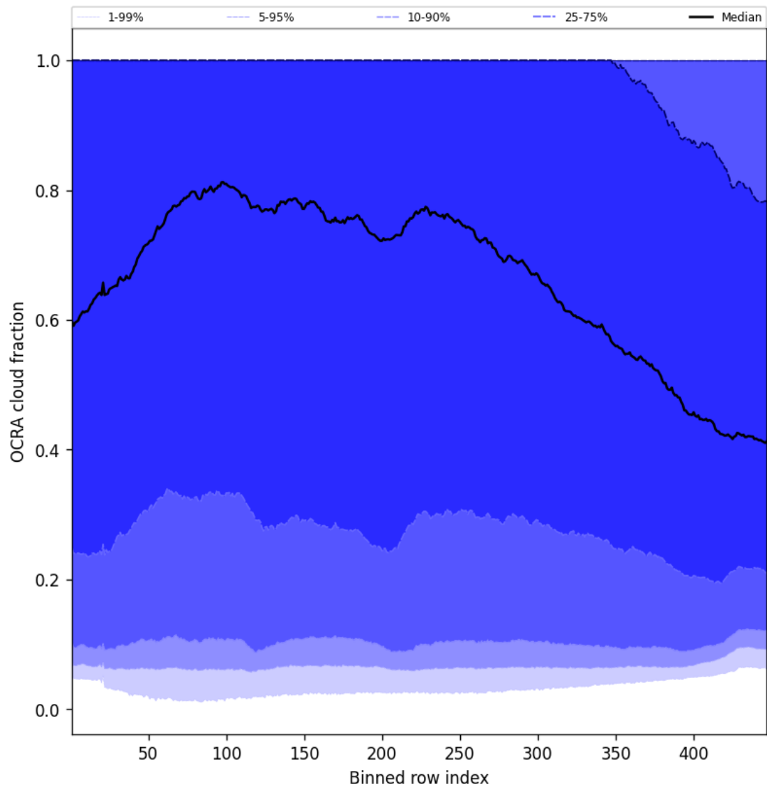
Figure 66: Along track statistics of “OCRA cloud fraction” for 2025-05-28 to 2025-05-30
