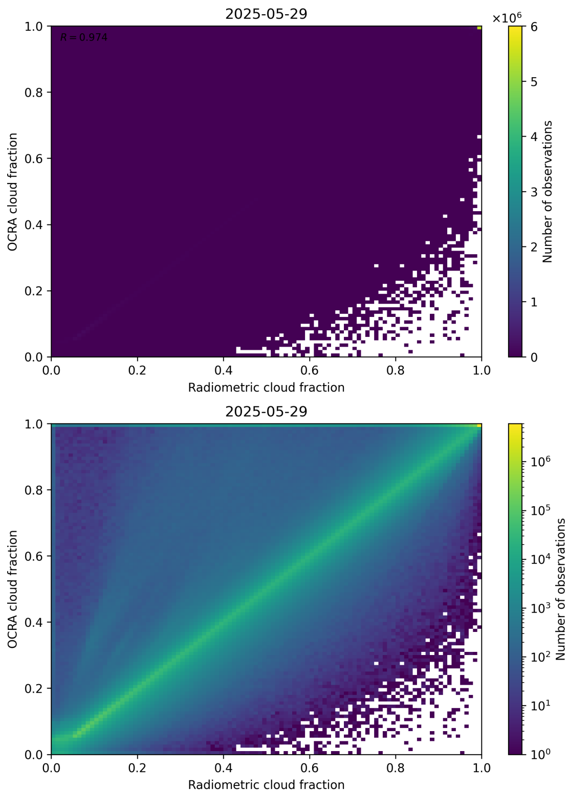
Figure 72: Scatter density plot of “Radiometric cloud fraction” against “OCRA cloud fraction” for 2025-05-28 to 2025-05-30.
