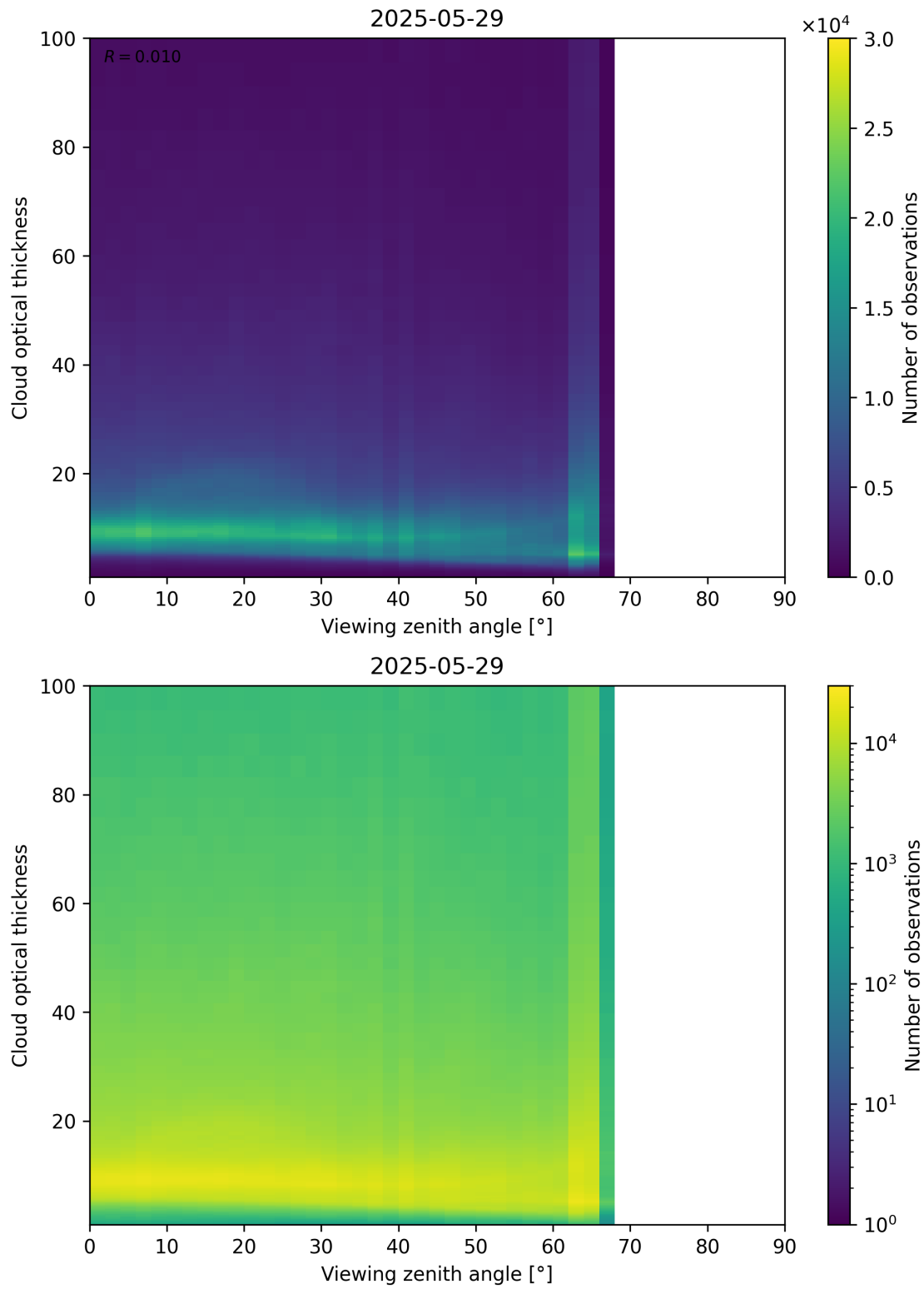
Figure 111: Scatter density plot of “Viewing zenith angle” against “Cloud optical thickness” for 2025-05-28 to 2025-05-30.
