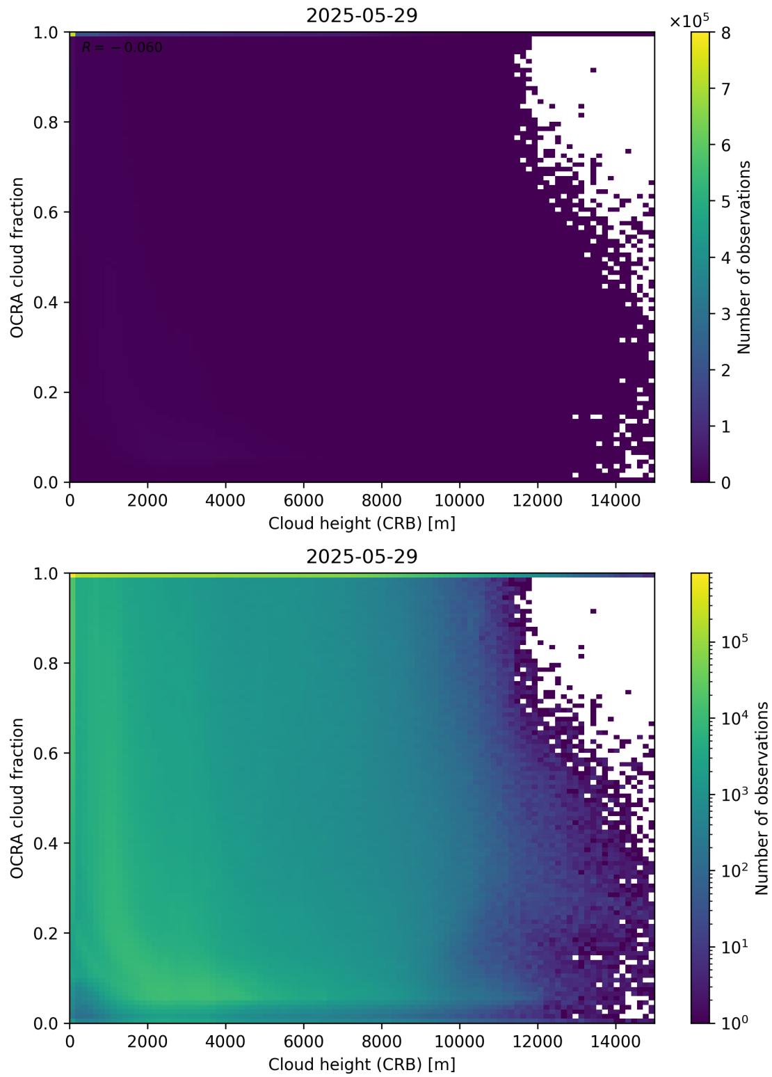
Figure 81: Scatter density plot of “Cloud height (CRB)” against “OCRA cloud fraction” for 2025-05-28 to 2025-05-30.
