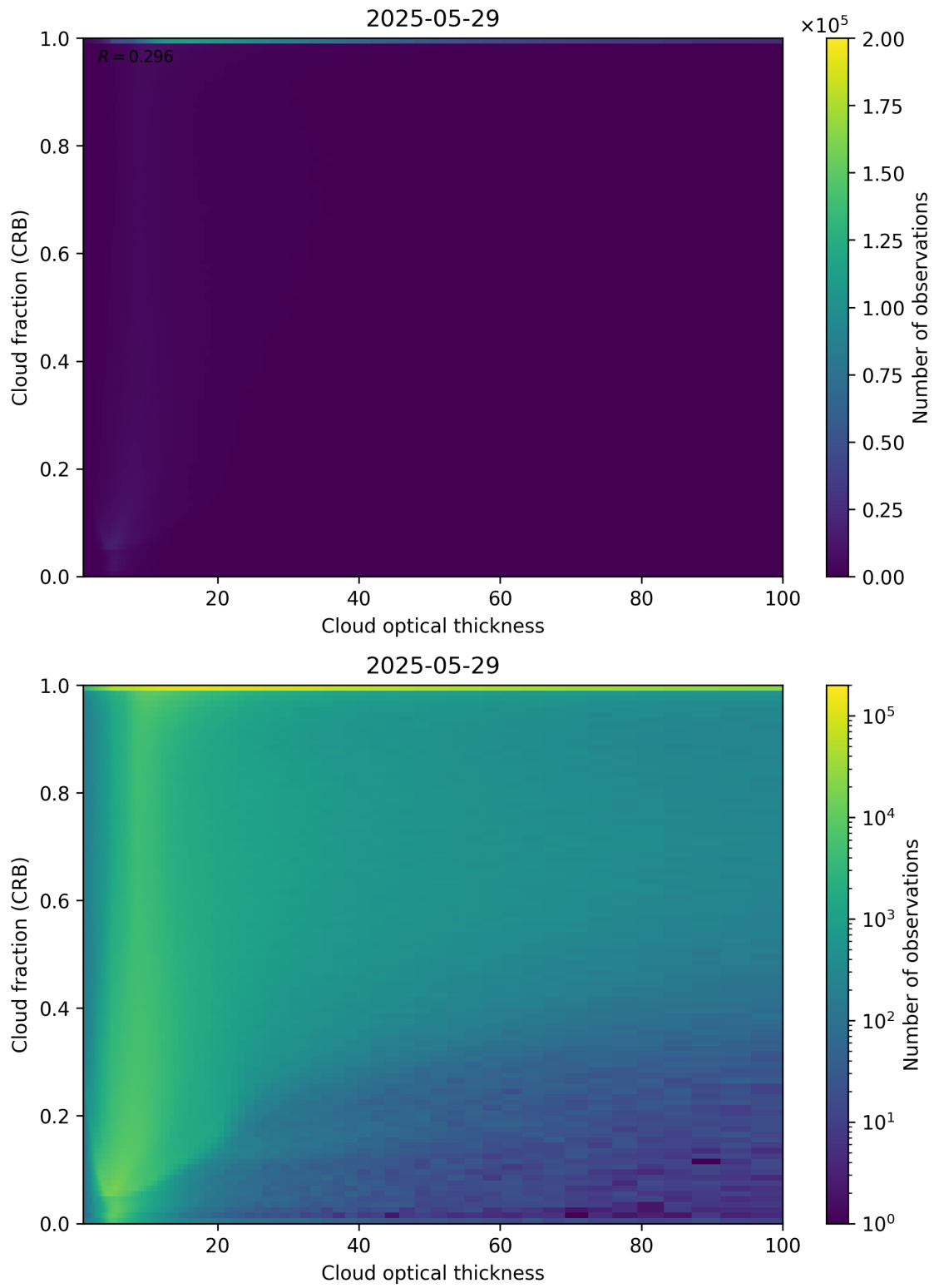
Figure 84: Scatter density plot of “Cloud optical thickness” against “Cloud fraction (CRB)” for 2025-05-28 to 2025-05-30.
