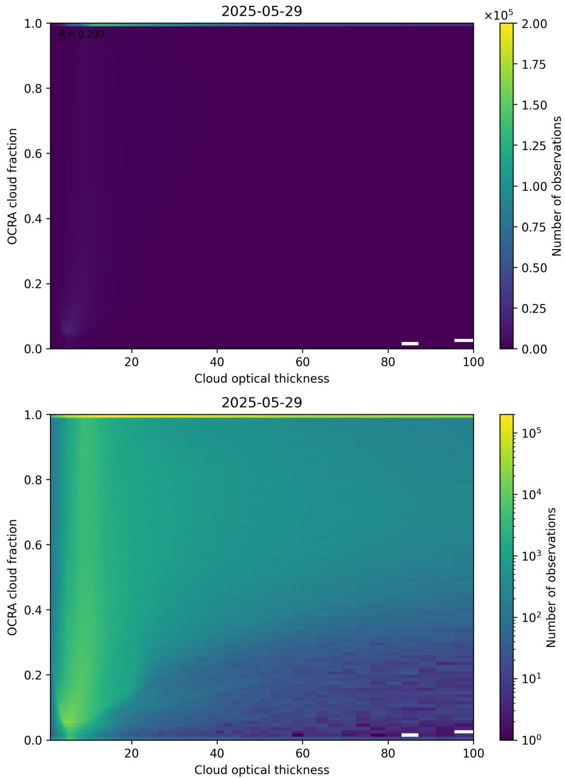
Figure 83: Scatter density plot of “Cloud optical thickness” against “OCRA cloud fraction” for 2025-05-28 to 2025-05-30.
