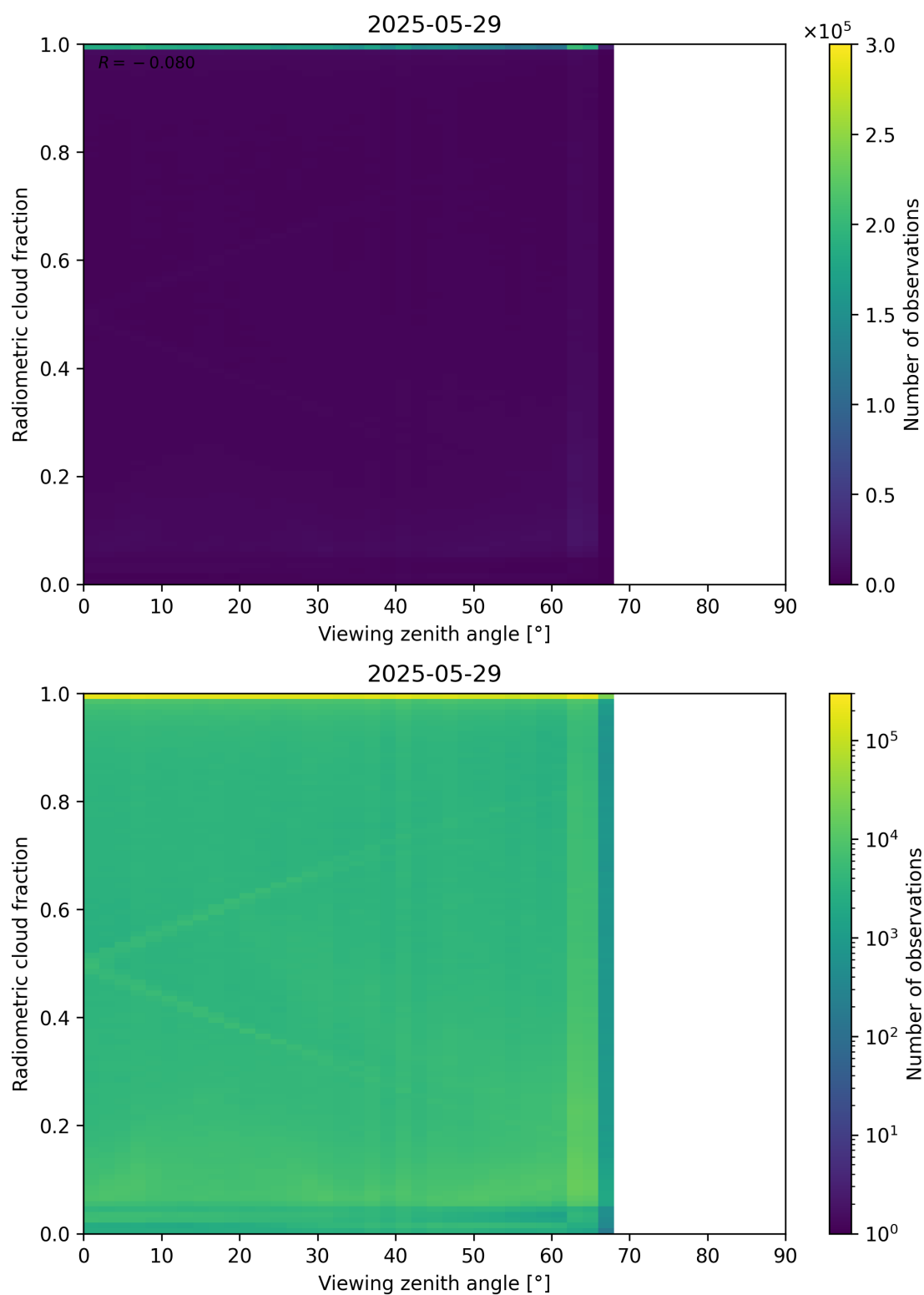
Figure 107: Scatter density plot of “Viewing zenith angle” against “Radiometric cloud fraction” for 2025-05-28 to 2025-05-30.
