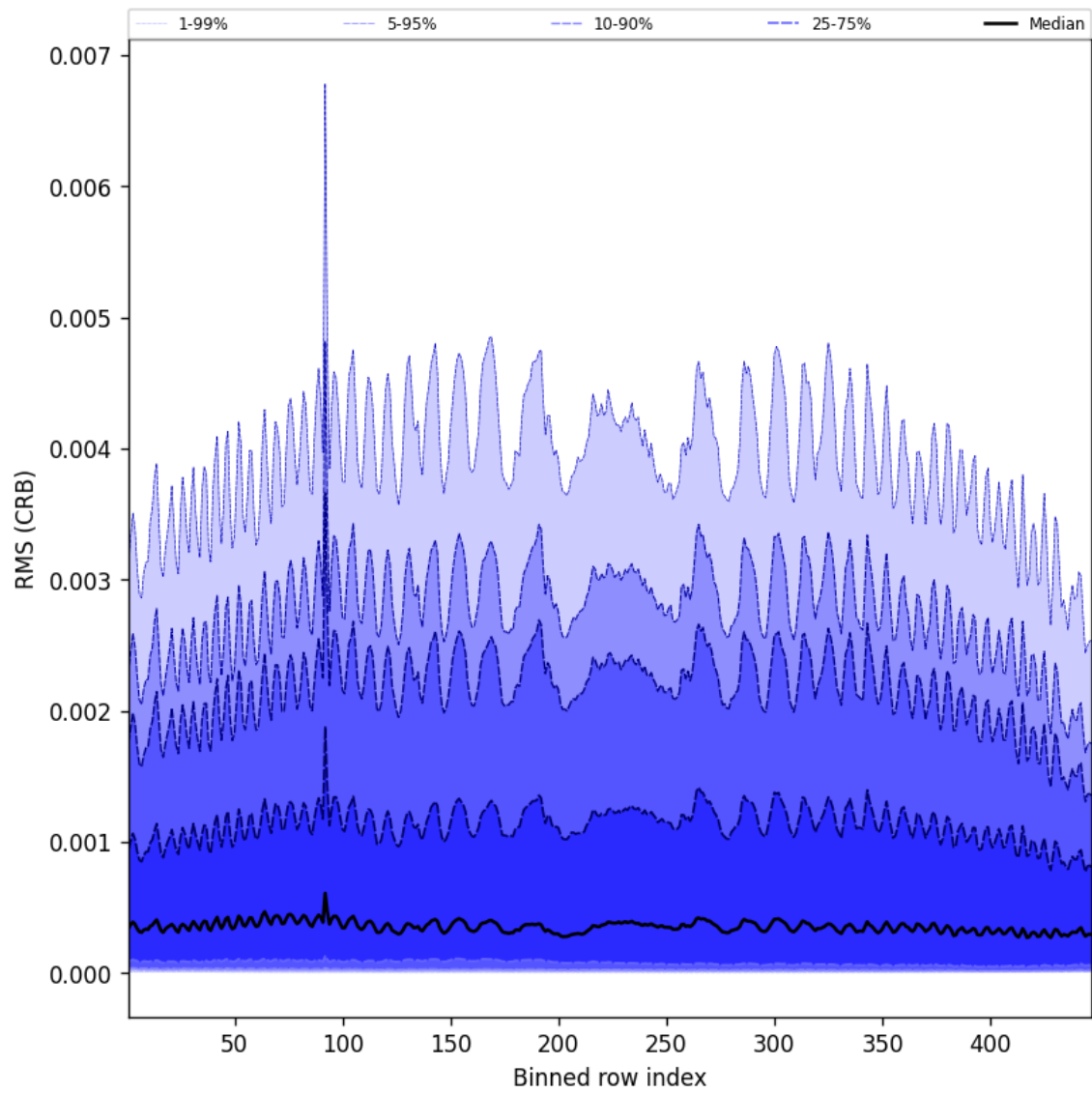
Figure 64: Along track statistics of “RMS (CRB)” for 2025-05-28 to 2025-05-30
