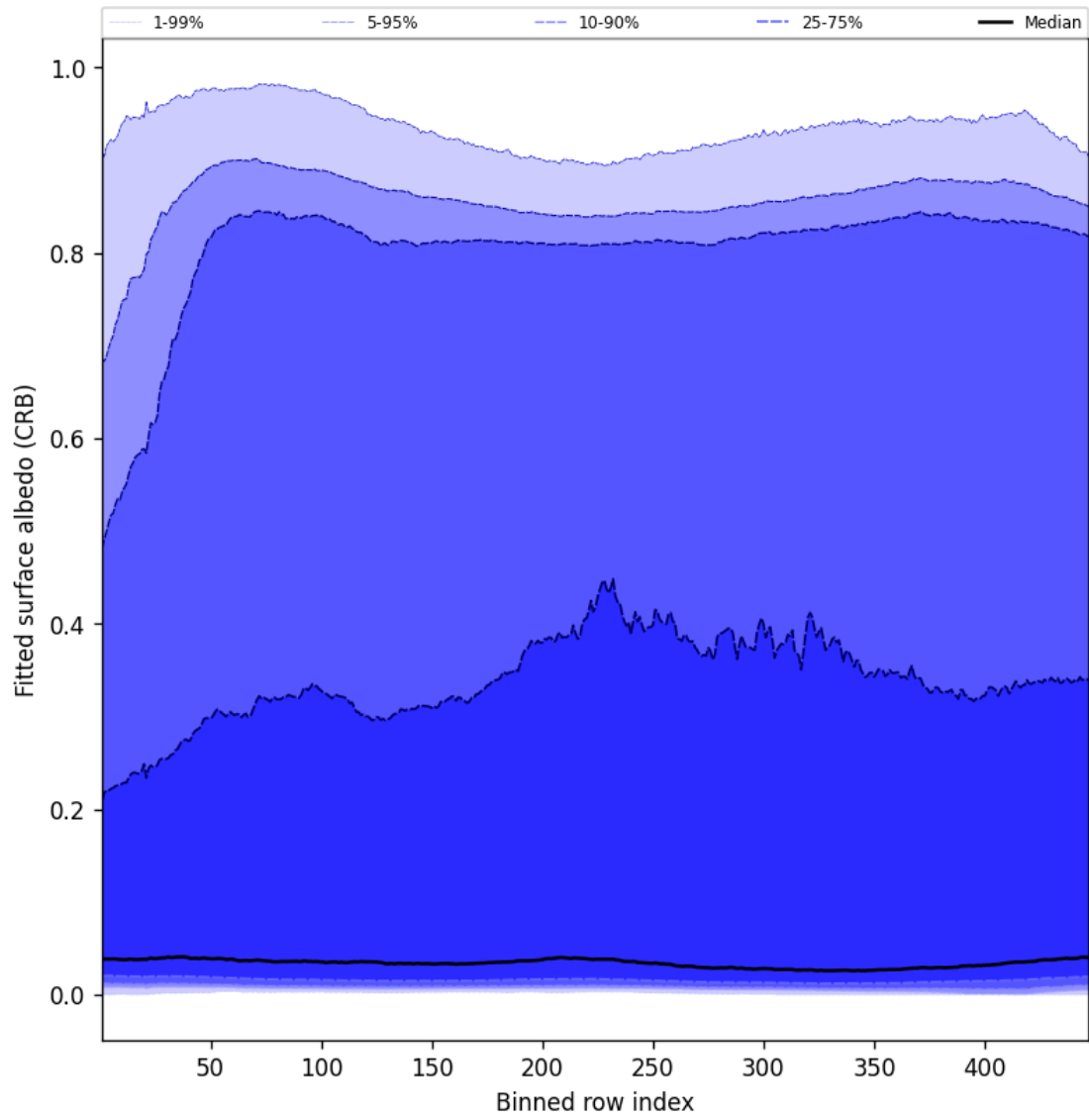
Figure 62: Along track statistics of “Fitted surface albedo (CRB)” for 2025-05-28 to 2025-05-30
