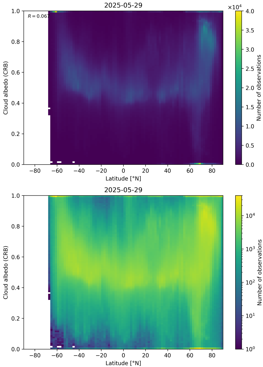
Figure 91: Scatter density plot of “Latitude” against “Cloud albedo (CRB)” for 2025-05-28 to 2025-05-30.
