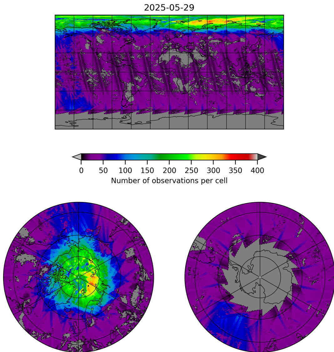
Figure 21: Map of the number of observations for 2025-05-28 to 2025-05-30
