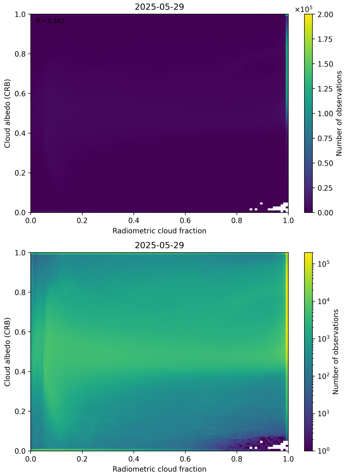
Figure 71: Scatter density plot of “Radiometric cloud fraction” against “Cloud albedo (CRB)” for 2025-05-28 to 2025-05-30.
