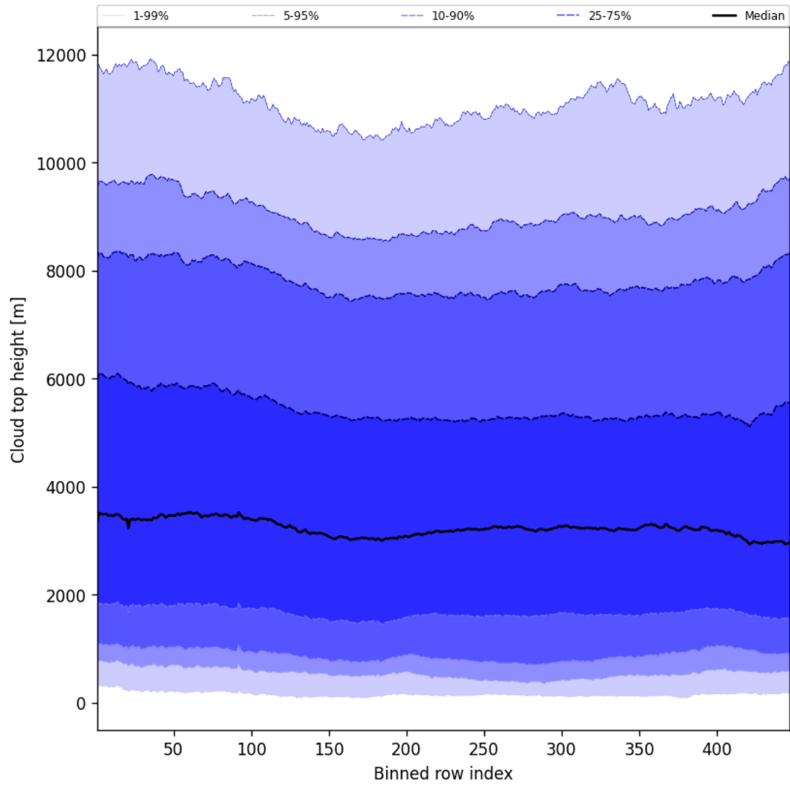
Figure 56: Along track statistics of “Cloud top height” for 2025-05-28 to 2025-05-30
