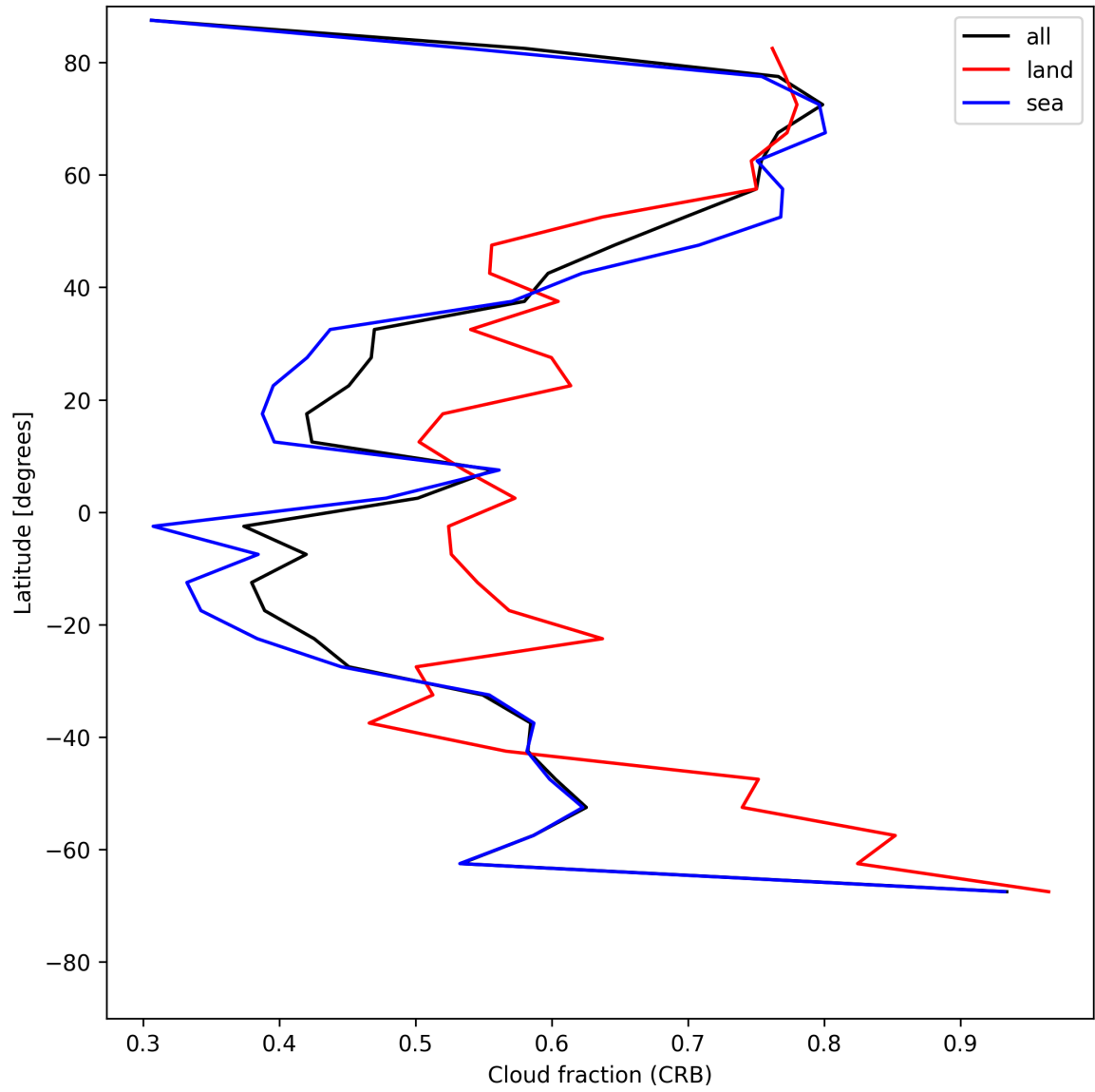
Figure 26: Zonal average of “Cloud fraction (CRB)” for 2025-05-28 to 2025-05-30.
