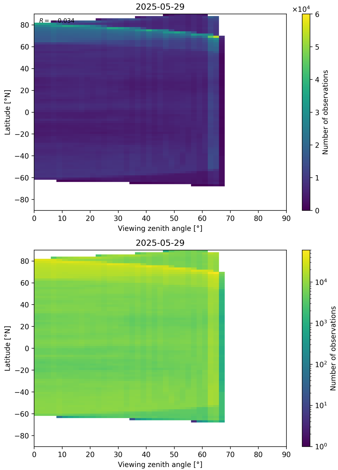
Figure 113: Scatter density plot of “Viewing zenith angle” against “Latitude” for 2025-05-28 to 2025-05-30.
