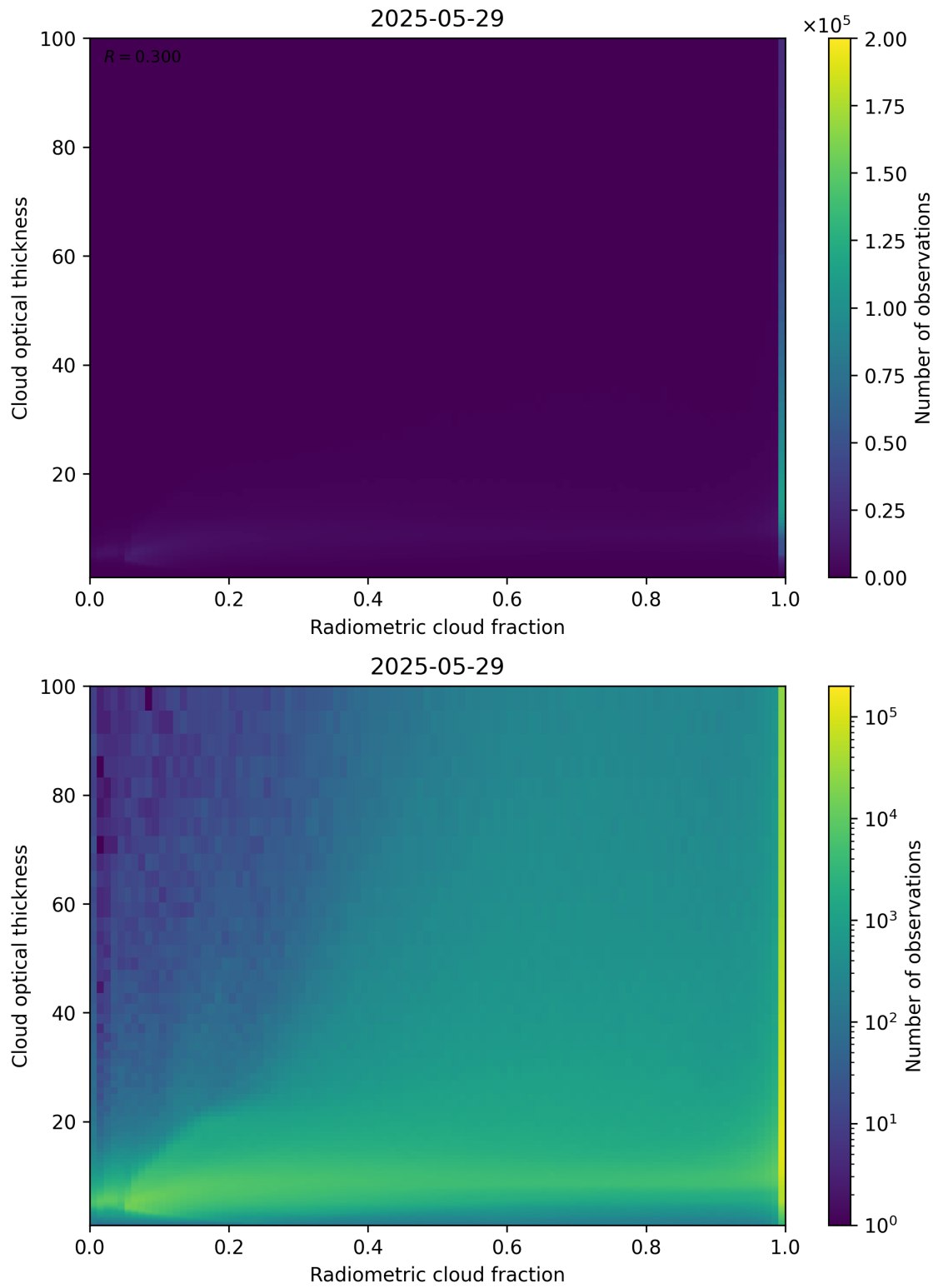
Figure 75: Scatter density plot of “Radiometric cloud fraction” against “Cloud optical thickness” for 2025-05-28 to 2025-05-30.
