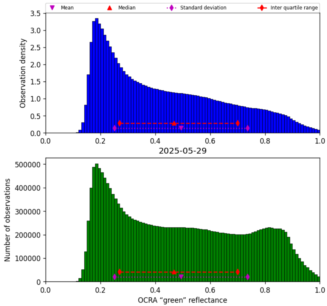
Figure 52: Histogram of “OCRA “green” reflectance” for 2025-05-28 to 2025-05-30
