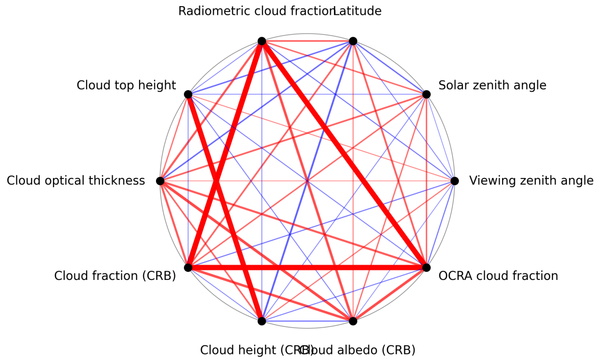
Figure 1: Map of correlation graph for 2025-05-28 to 2025-05-30.
