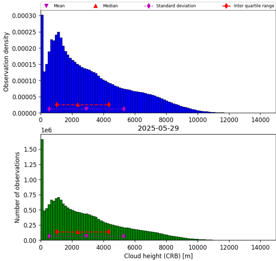
Figure 43: Histogram of “Cloud height (CRB)” for 2025-05-28 to 2025-05-30
