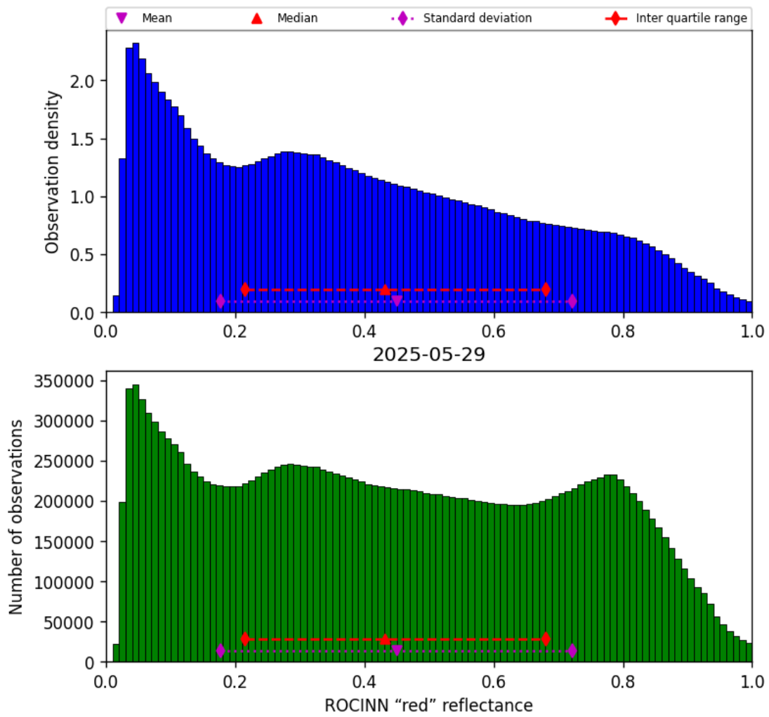
Figure 53: Histogram of “ROCINN “red” reflectance” for 2025-05-28 to 2025-05-30
