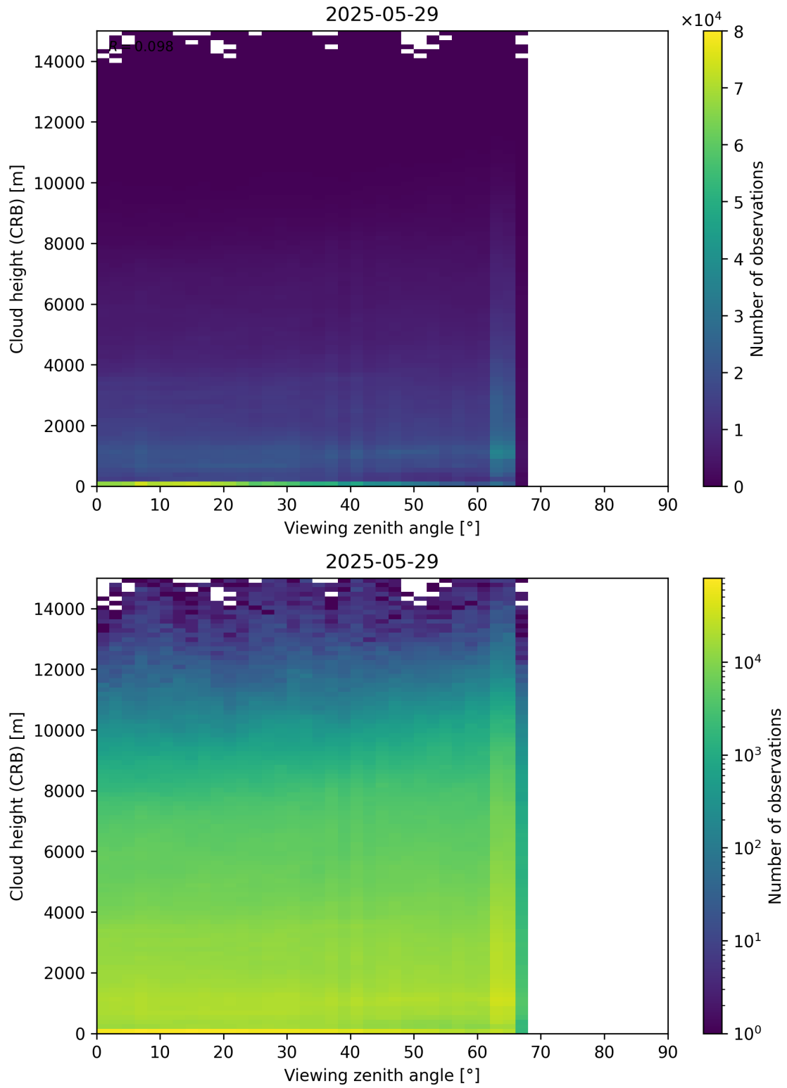
Figure 110: Scatter density plot of “Viewing zenith angle” against “Cloud height (CRB)” for 2025-05-28 to 2025-05-30.
