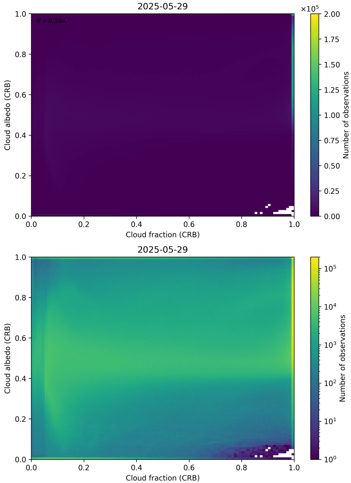
Figure 77: Scatter density plot of “Cloud fraction (CRB)” against “Cloud albedo (CRB)” for 2025-05-28 to 2025-05-30.
