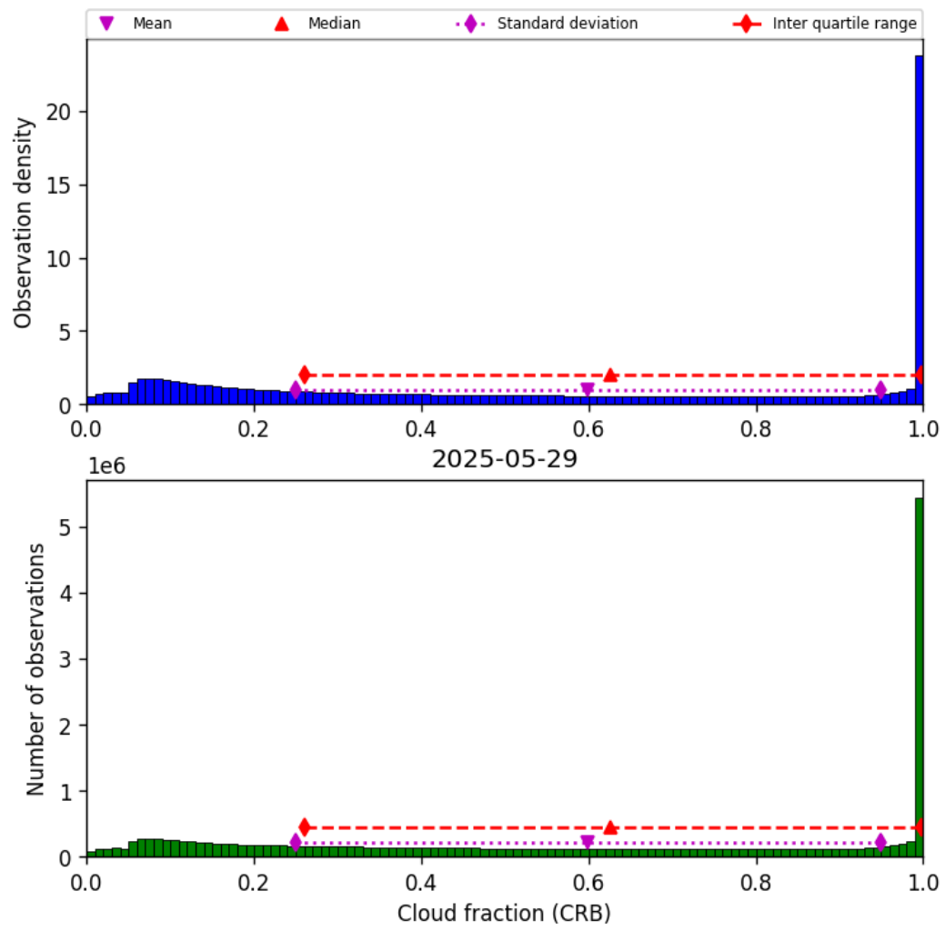
Figure 42: Histogram of “Cloud fraction (CRB)” for 2025-05-28 to 2025-05-30
