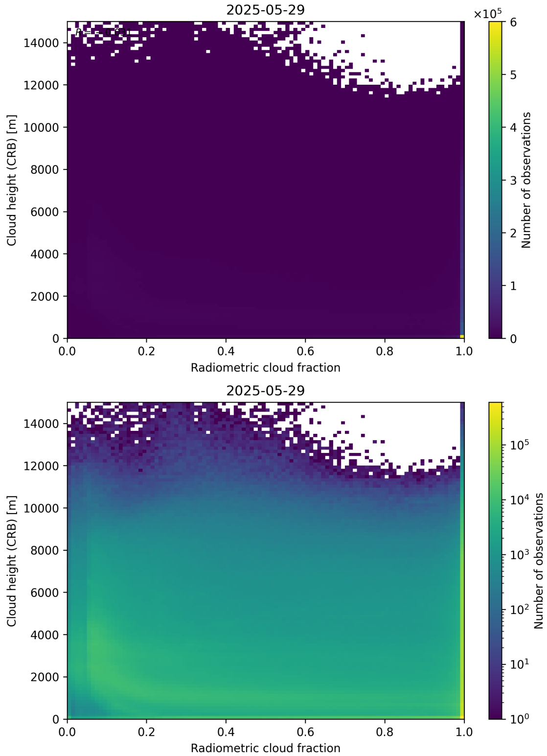
Figure 74: Scatter density plot of “Radiometric cloud fraction” against “Cloud height (CRB)” for 2025-05-28 to 2025-05-30.
