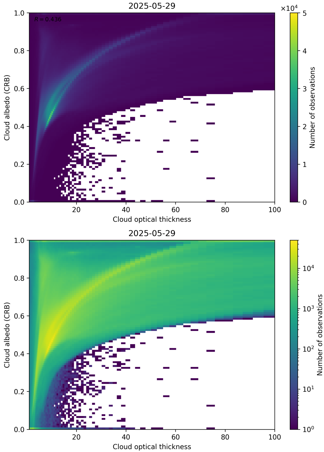
Figure 82: Scatter density plot of “Cloud optical thickness” against “Cloud albedo (CRB)” for 2025-05-28 to 2025-05-30.
