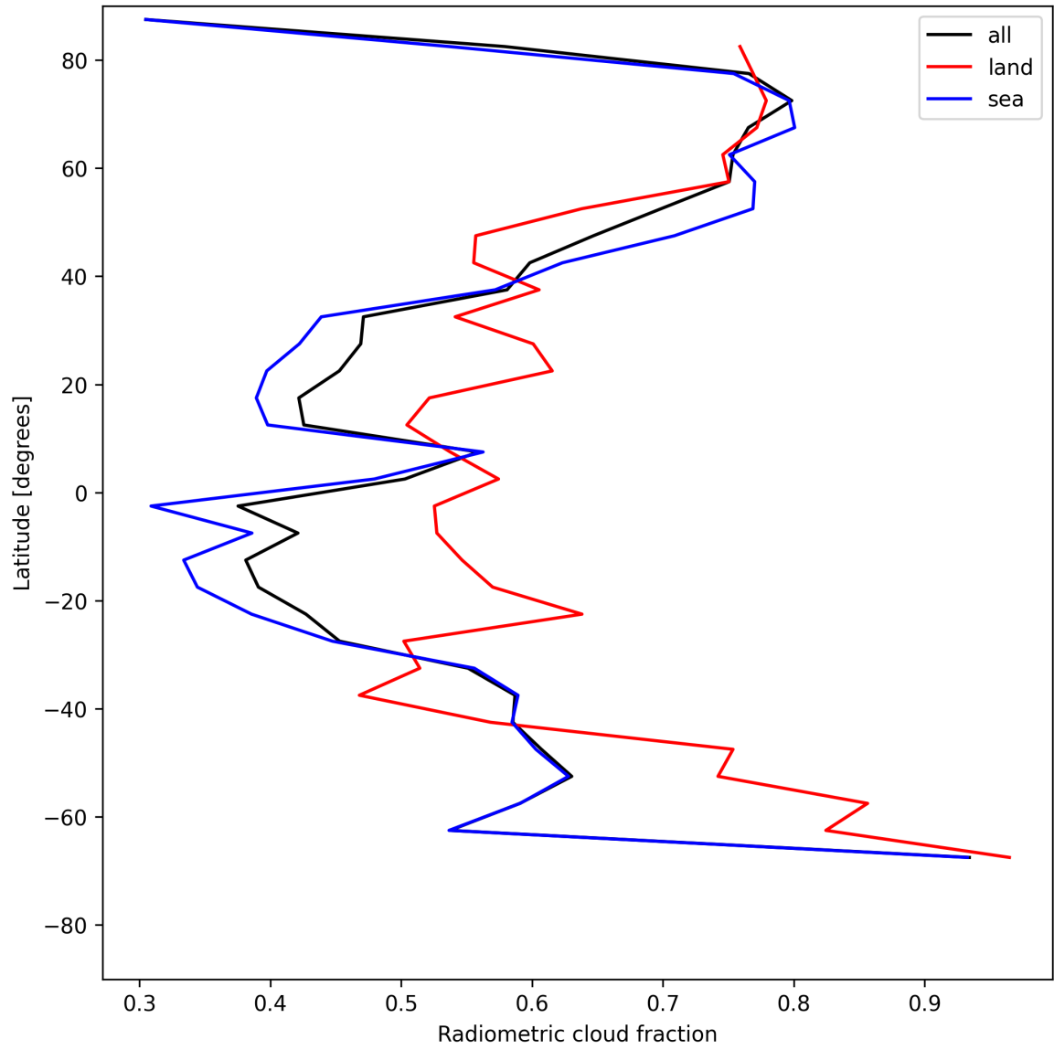
Figure 23: Zonal average of “Radiometric cloud fraction” for 2025-05-28 to 2025-05-30.
