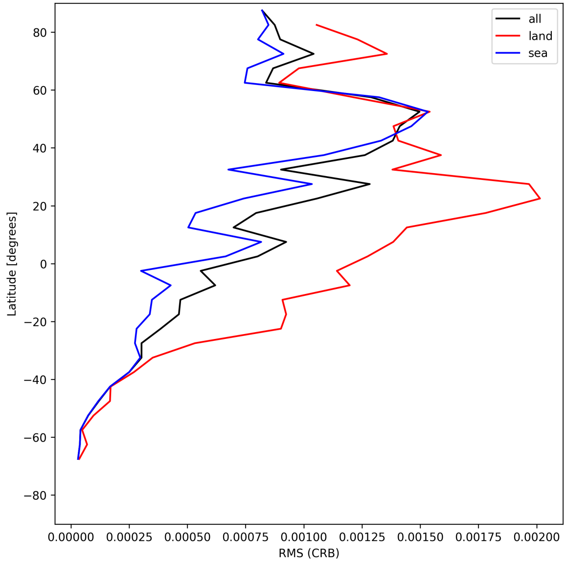
Figure 32: Zonal average of “RMS (CRB)” for 2025-05-28 to 2025-05-30.
