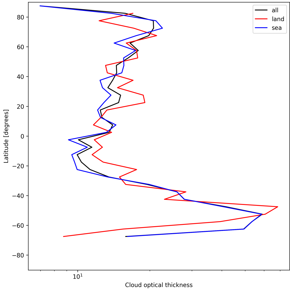
Figure 25: Zonal average of “Cloud optical thickness” for 2025-05-28 to 2025-05-30.
