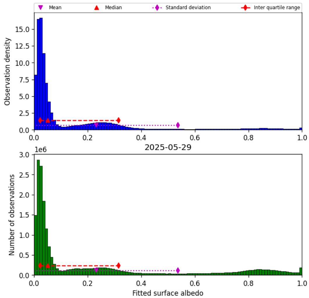
Figure 45: Histogram of “Fitted surface albedo” for 2025-05-28 to 2025-05-30
