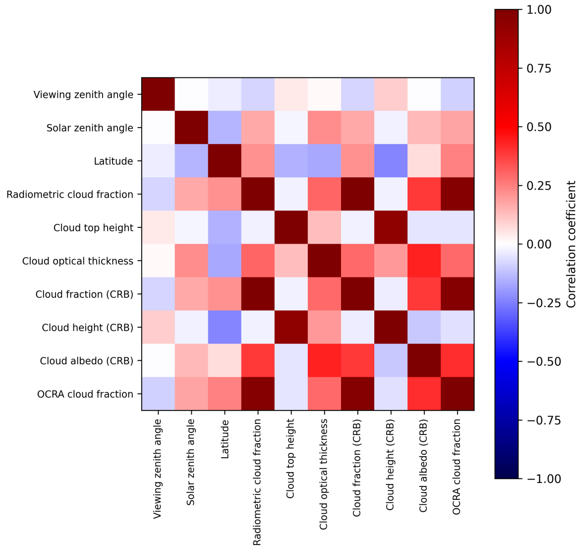
Figure 2: Map of correlation matrix for 2025-05-28 to 2025-05-30.
