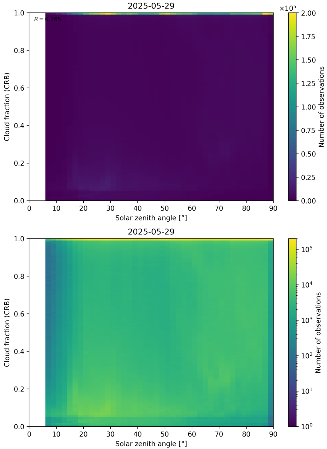
Figure 101: Scatter density plot of “Solar zenith angle” against “Cloud fraction (CRB)” for 2025-05-28 to 2025-05-30.
